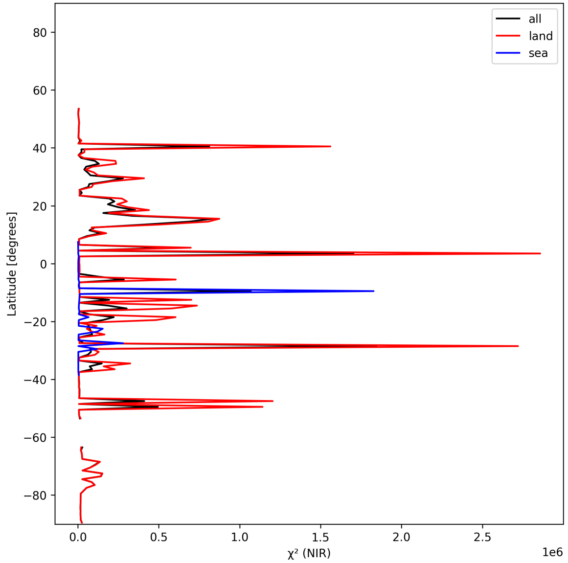
Figure 17: Zonal average of “ \chi^2 (NIR)” for 2025-11-27 to 2025-11-28.
