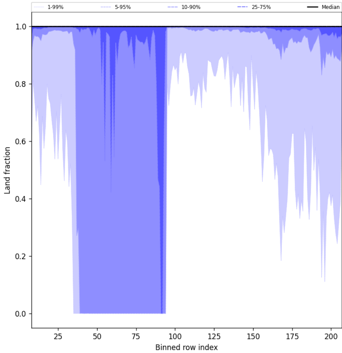
Figure 45: Along track statistics of "Land fraction" for 2025-11-27 to 2025-11-28
