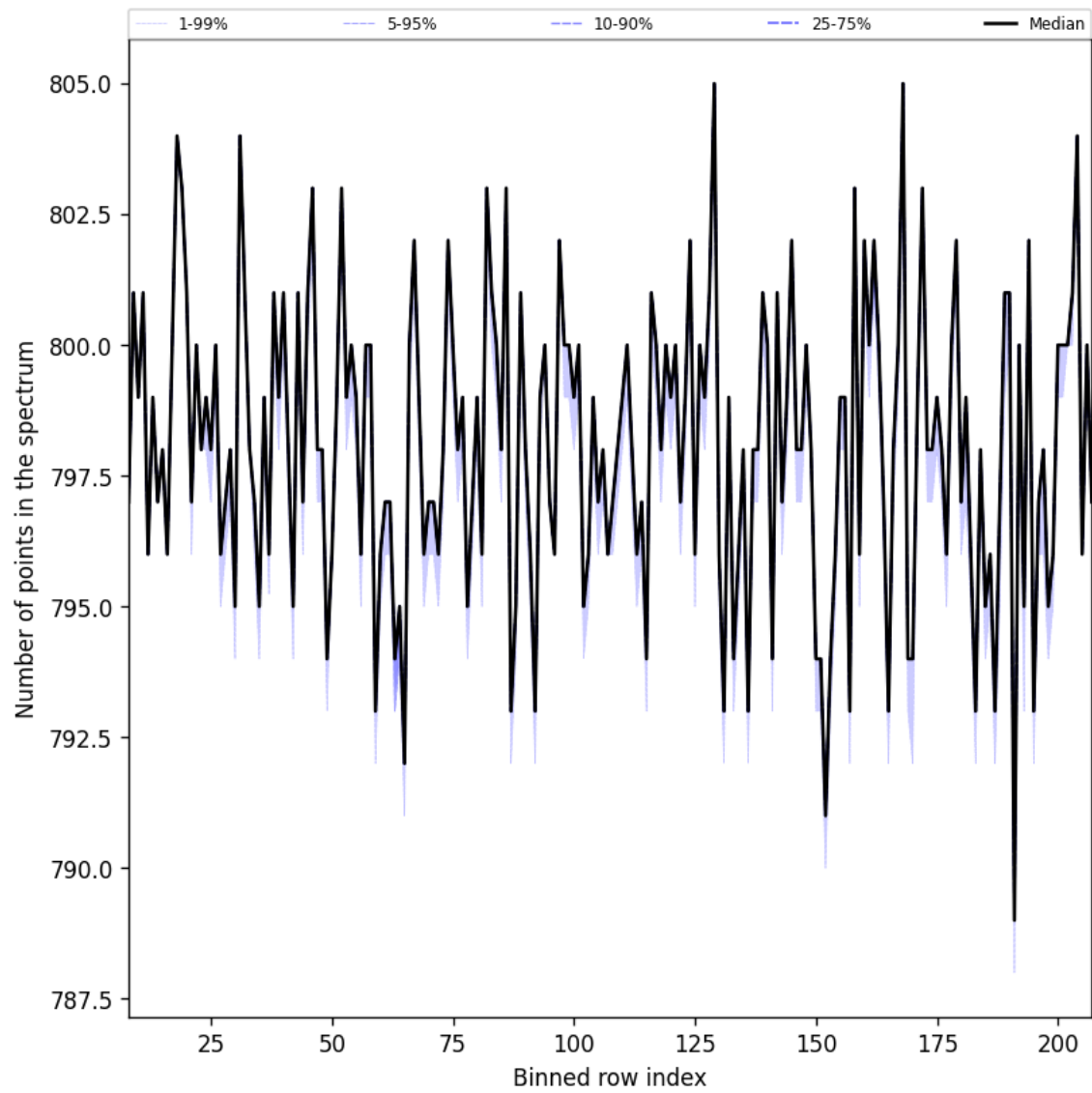
Figure 38: Along track statistics of “Number of points in the spectrum” for 2025-11-27 to 2025-11-28
