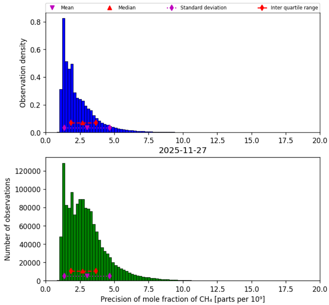
Figure 24: Histogram of “Precision of mole fraction of CH 4 ” for 2025-11-27 to 2025-11-28
