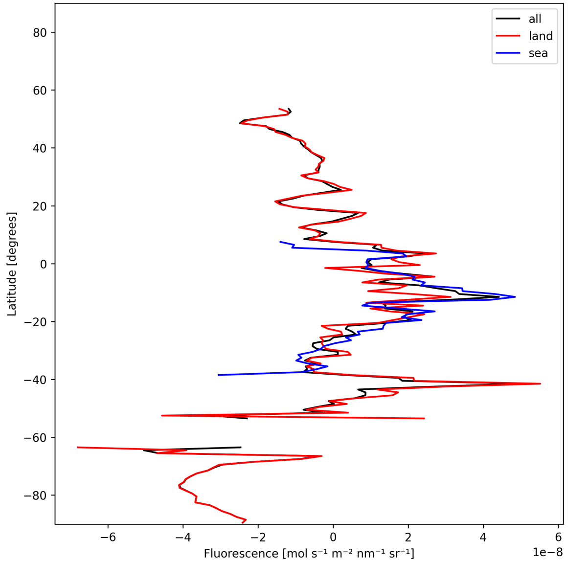
Figure 20: Zonal average of “Fluorescence” for 2025-11-27 to 2025-11-28.
