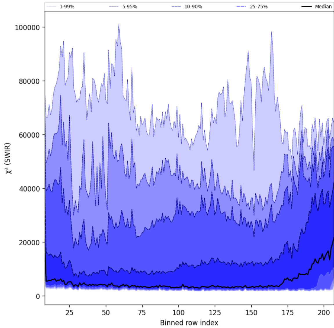
Figure 40: Along track statistics of “ \chi^2 (SWIR)” for 2025-11-27 to 2025-11-28
