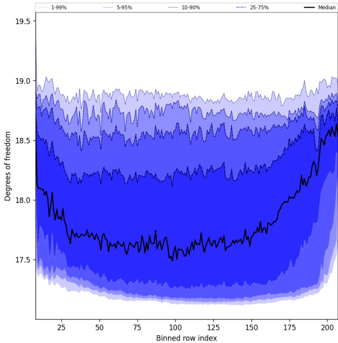
Figure 42: Along track statistics of “Degrees of freedom” for 2025-11-27 to 2025-11-28
