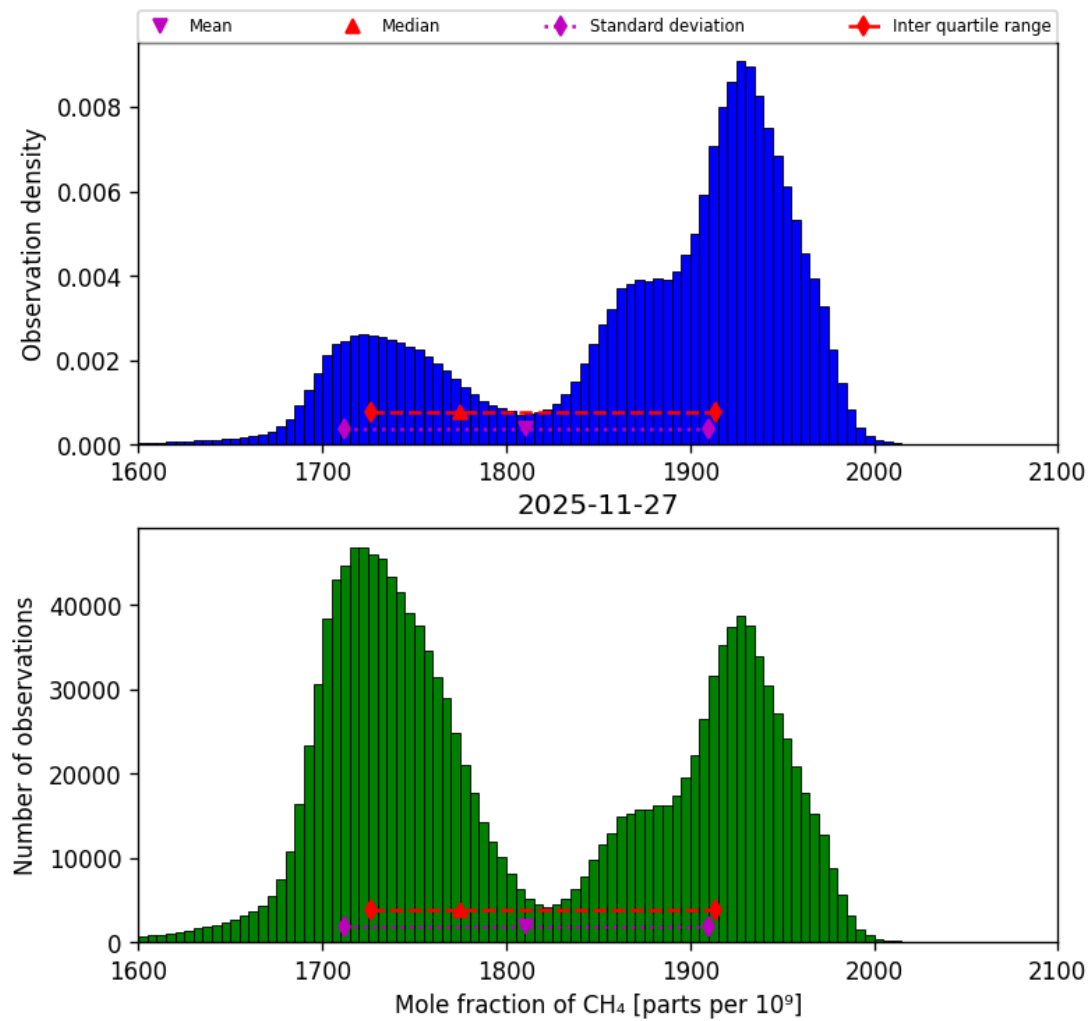
Figure 23: Histogram of “Mole fraction of CH 4 ” for 2025-11-27 to 2025-11-28
