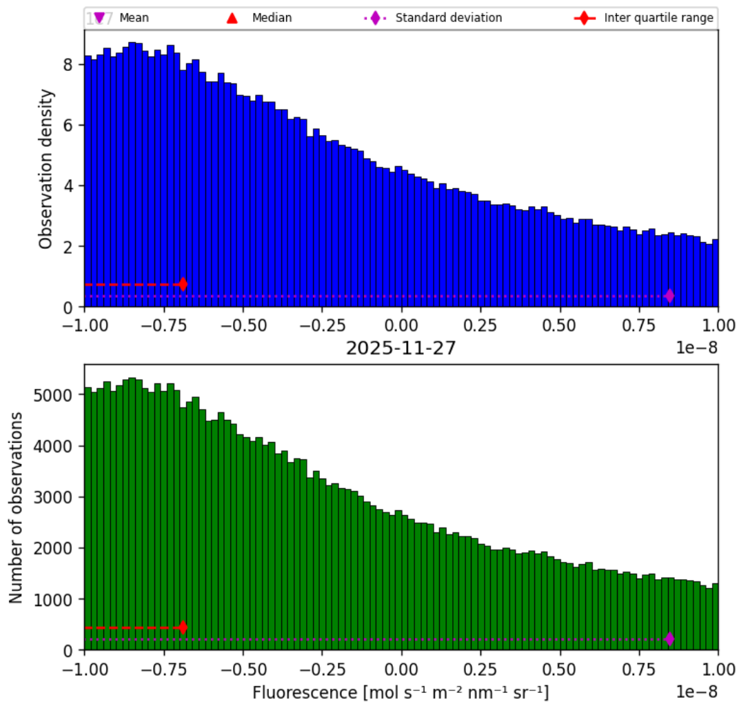
Figure 32: Histogram of “Fluorescence” for 2025-11-27 to 2025-11-28
