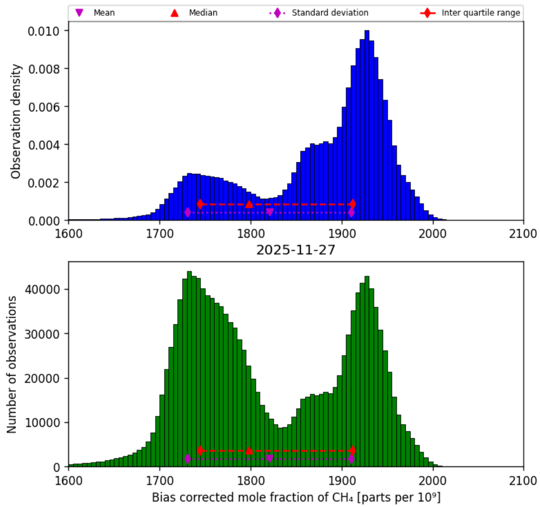
Figure 25: Histogram of “Bias corrected mole fraction of CH 4 ” for 2025-11-27 to 2025-11-28
