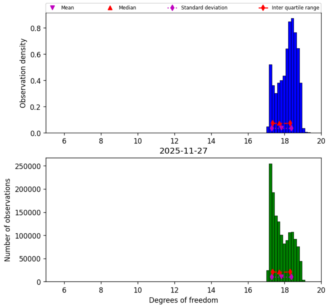
Figure 30: Histogram of “Degrees of freedom” for 2025-11-27 to 2025-11-28
