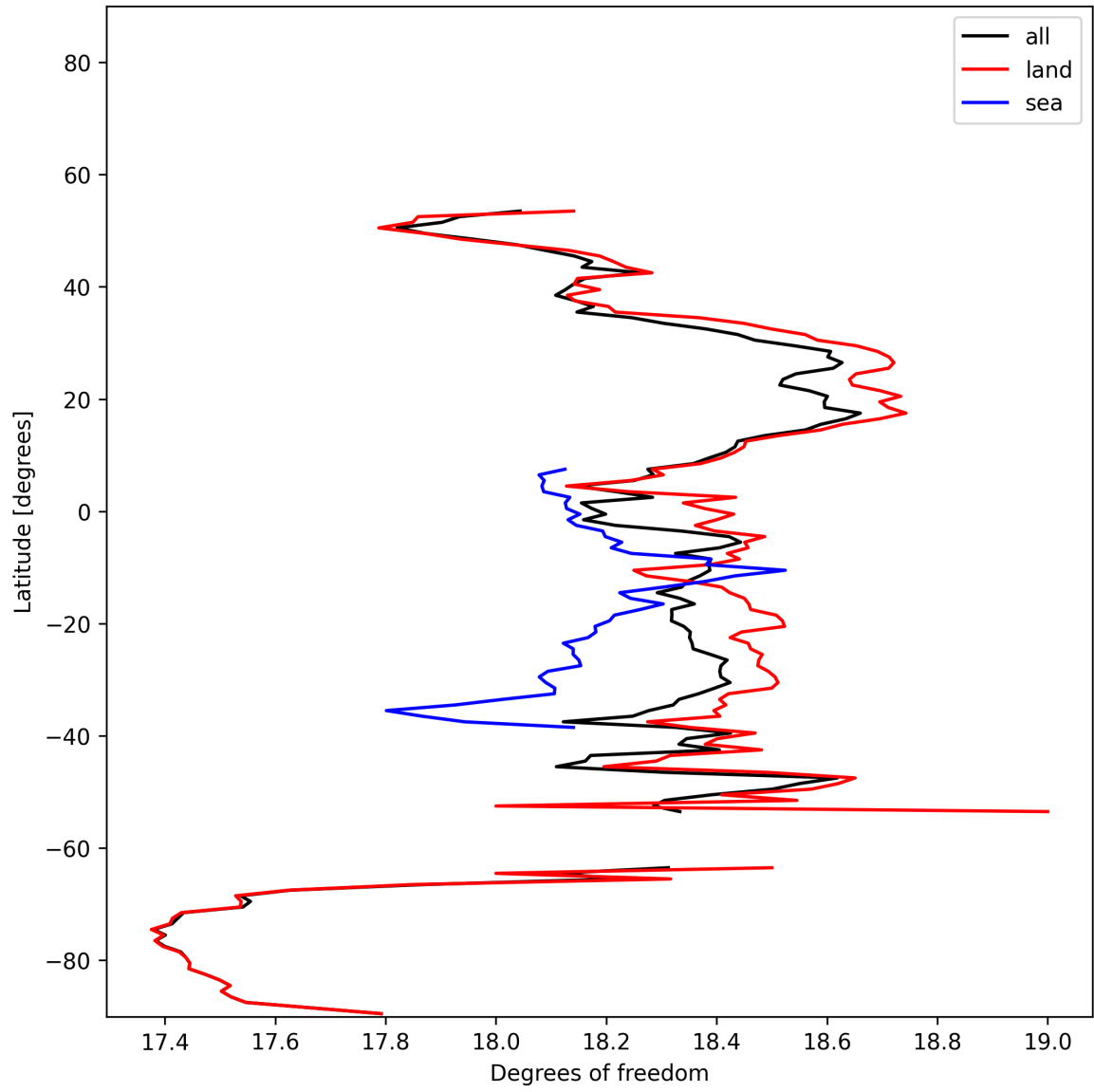
Figure 18: Zonal average of “Degrees of freedom” for 2025-11-27 to 2025-11-28.
