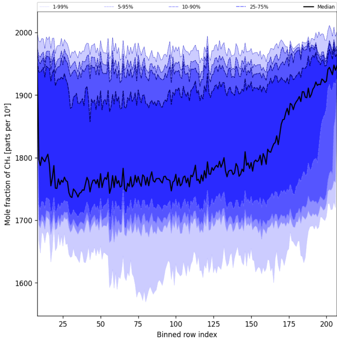
Figure 35: Along track statistics of “Mole fraction of CH 4 ” for 2025-11-27 to 2025-11-28
