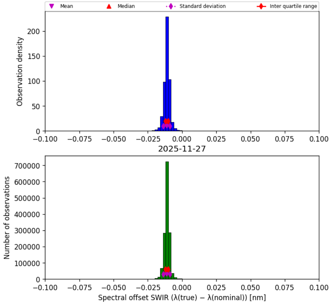
Figure 27: Histogram of “Spectral offset SWIR ( \lambda_{\text{true}} - \lambda_{\text{nominal}} )” for 2025-11-27 to 2025-11-28
