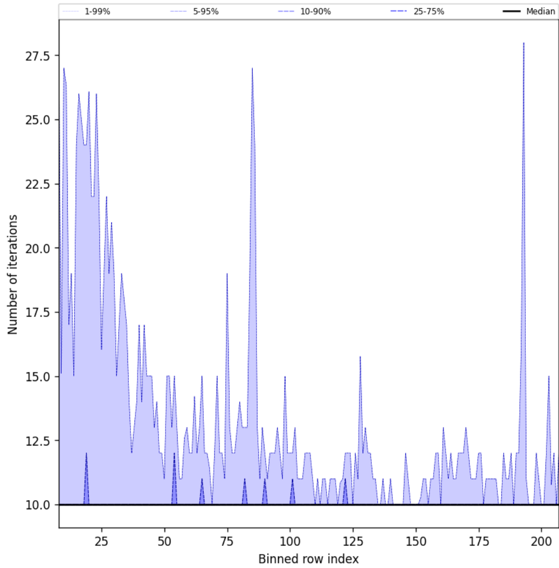
Figure 43: Along track statistics of “Number of iterations” for 2025-11-27 to 2025-11-28
