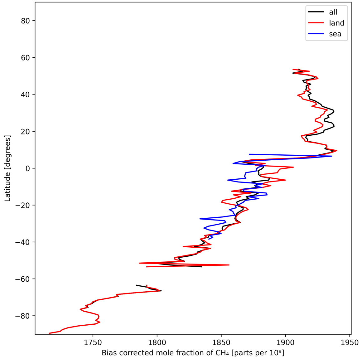
Figure 13: Zonal average of “Bias corrected mole fraction of CH 4 ” for 2025-11-27 to 2025-11-28.
