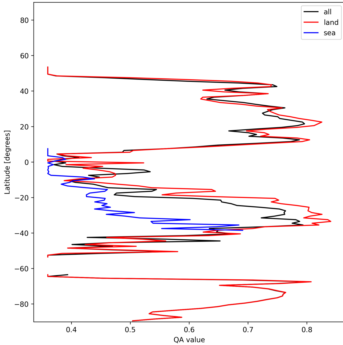
Figure 10: Zonal average of “QA value” for 2025-11-27 to 2025-11-28.
