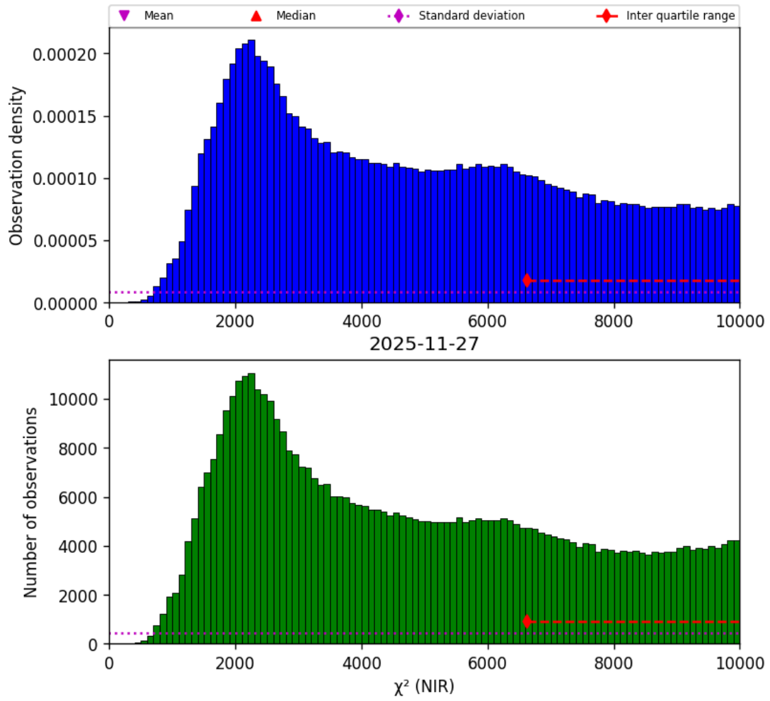
Figure 29: Histogram of “ \chi^2 (NIR)” for 2025-11-27 to 2025-11-28
