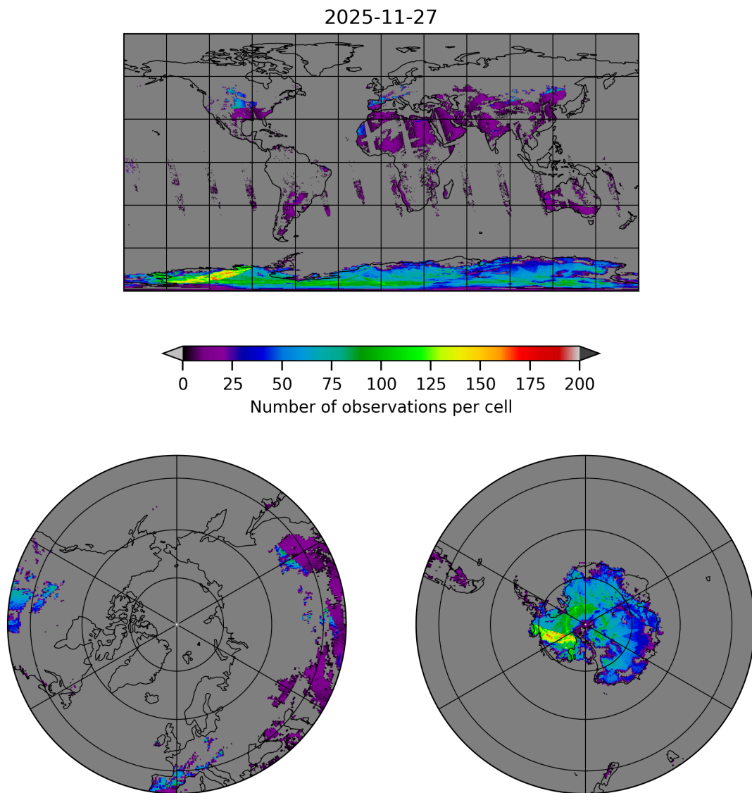
Figure 9: Map of the number of observations for 2025-11-27 to 2025-11-28
