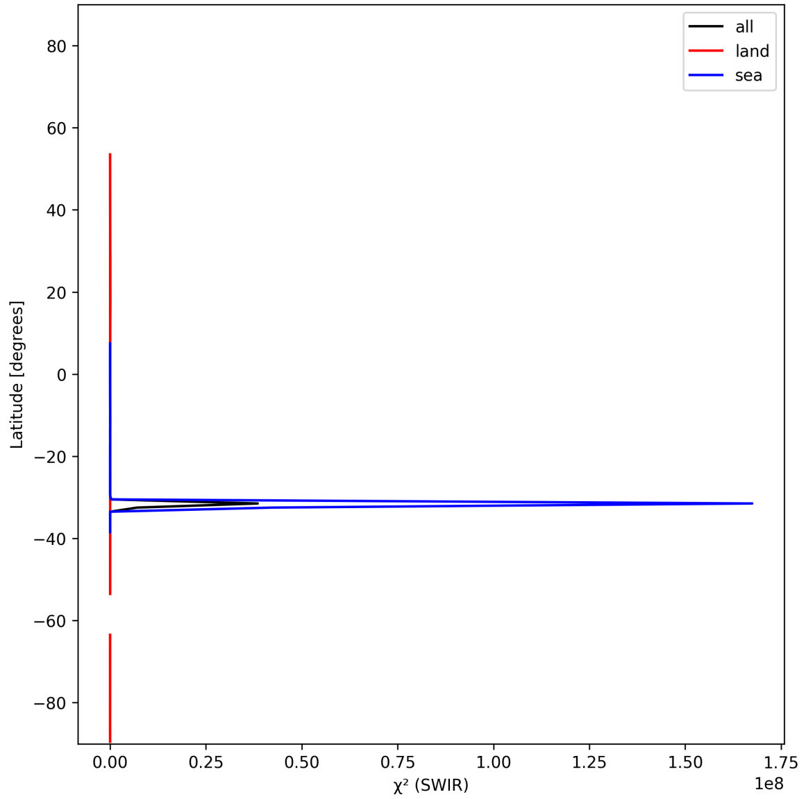
Figure 16: Zonal average of “ \chi^2 (SWIR)” for 2025-11-27 to 2025-11-28.
