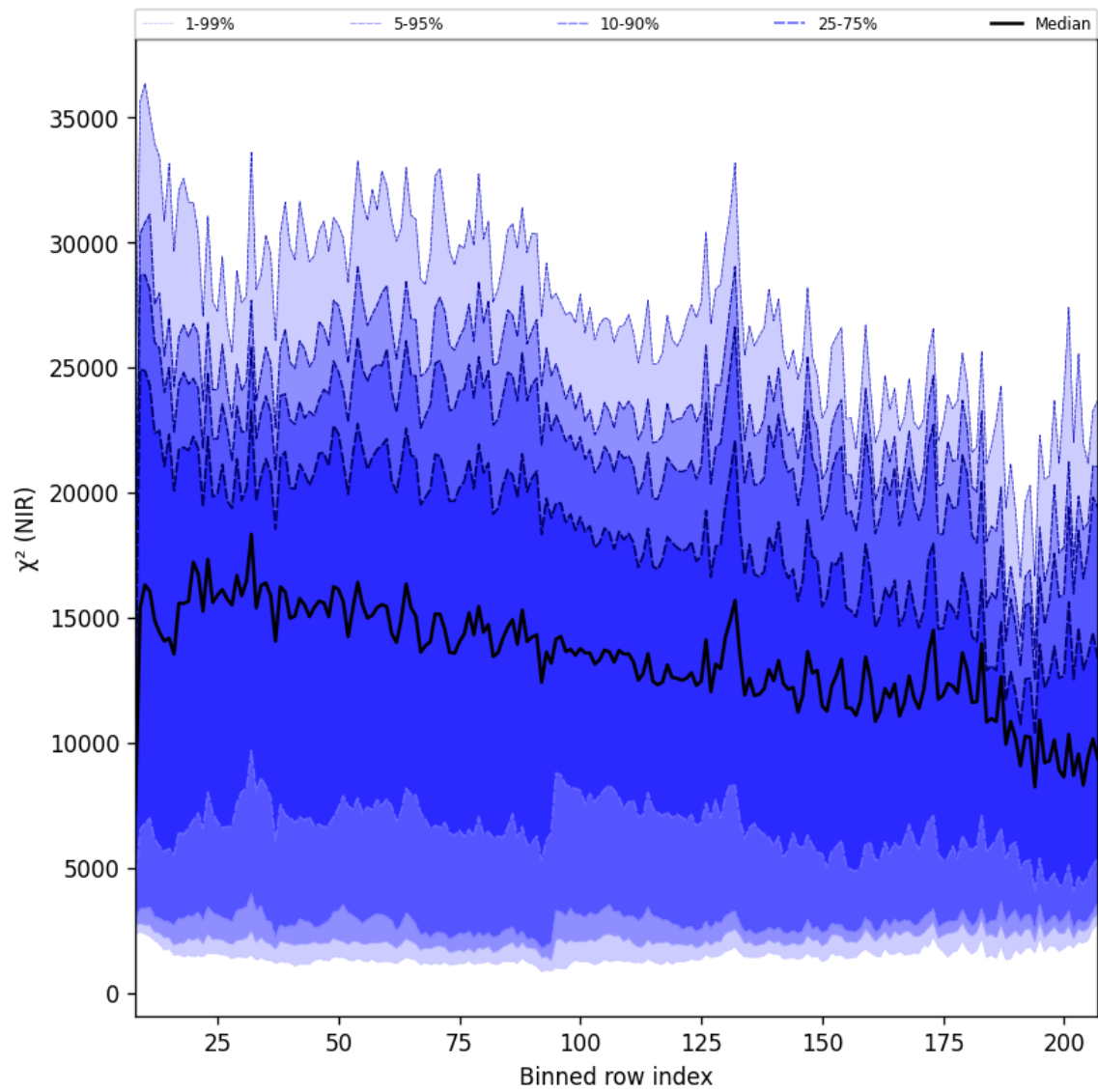
Figure 41: Along track statistics of “ \chi^2 (NIR)” for 2025-11-27 to 2025-11-28
