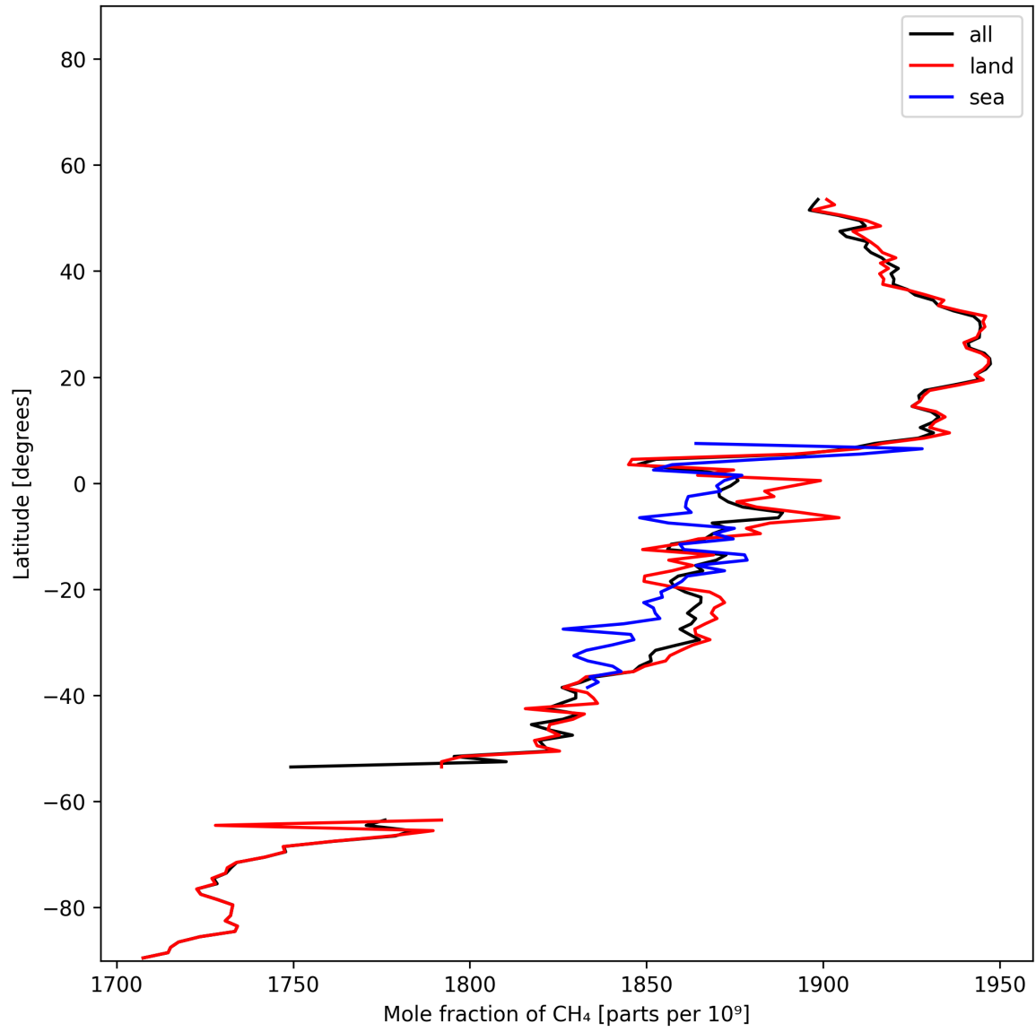
Figure 11: Zonal average of “Mole fraction of CH 4 ” for 2025-11-27 to 2025-11-28.
