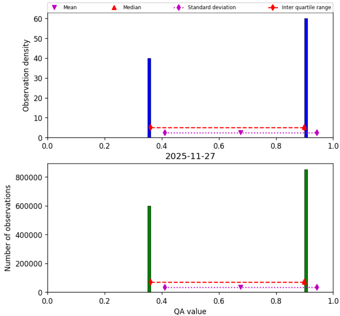
Figure 22: Histogram of “QA value” for 2025-11-27 to 2025-11-28
