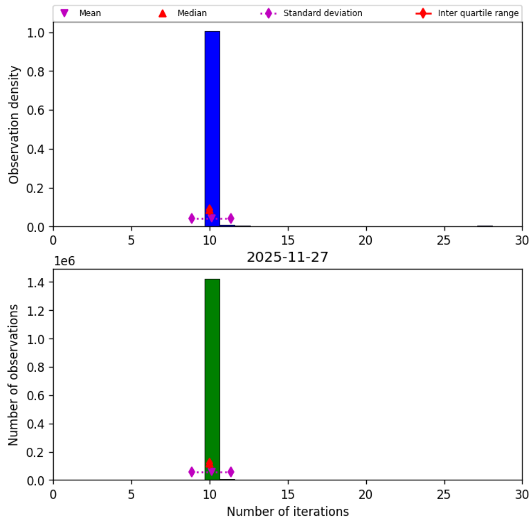
Figure 31: Histogram of “Number of iterations” for 2025-11-27 to 2025-11-28
