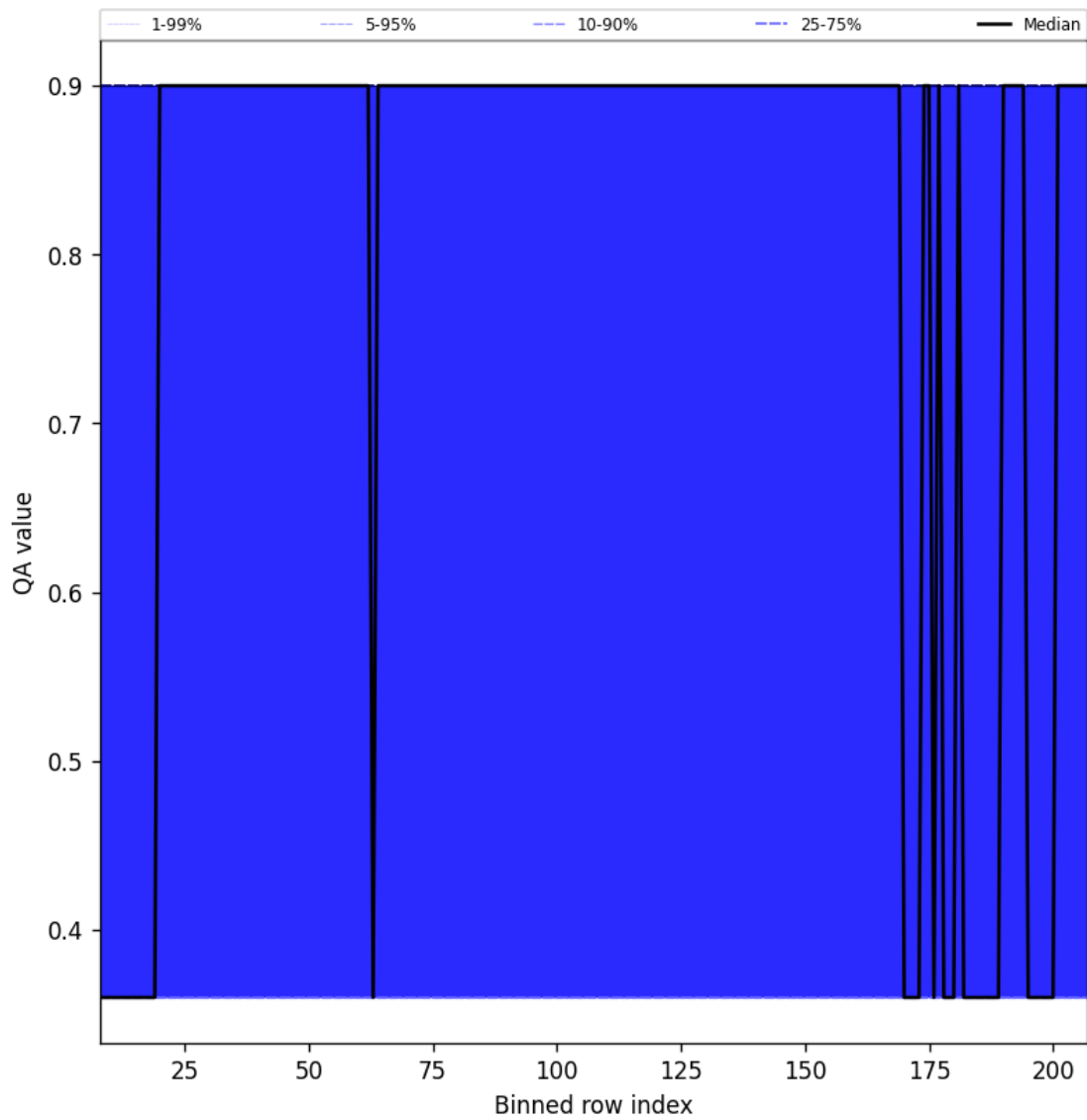
Figure 34: Along track statistics of “QA value” for 2025-11-27 to 2025-11-28
