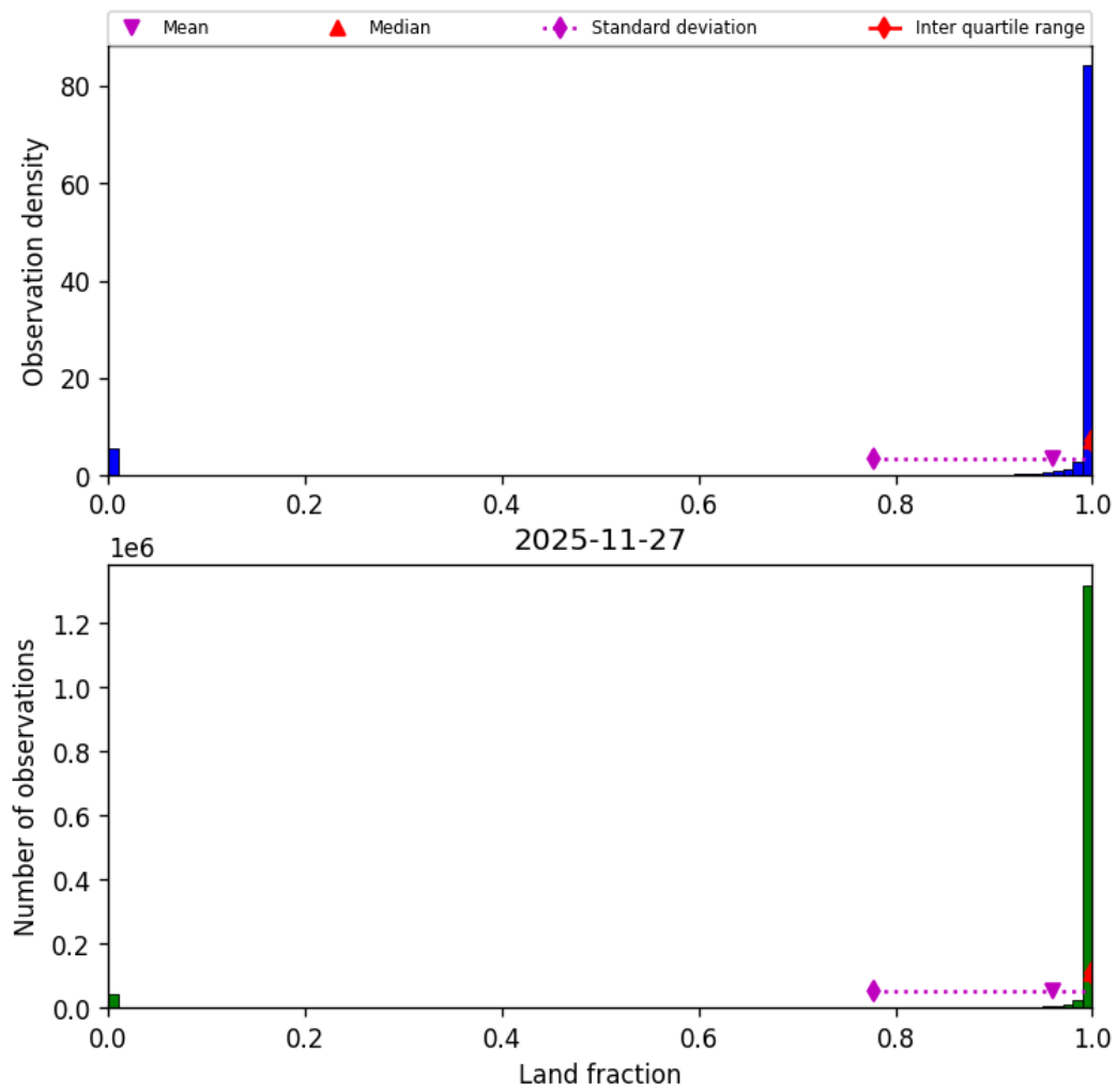
Figure 33: Histogram of “Land fraction” for 2025-11-27 to 2025-11-28
