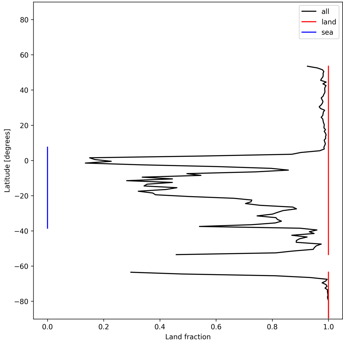
Figure 21: Zonal average of “Land fraction” for 2025-11-27 to 2025-11-28.
