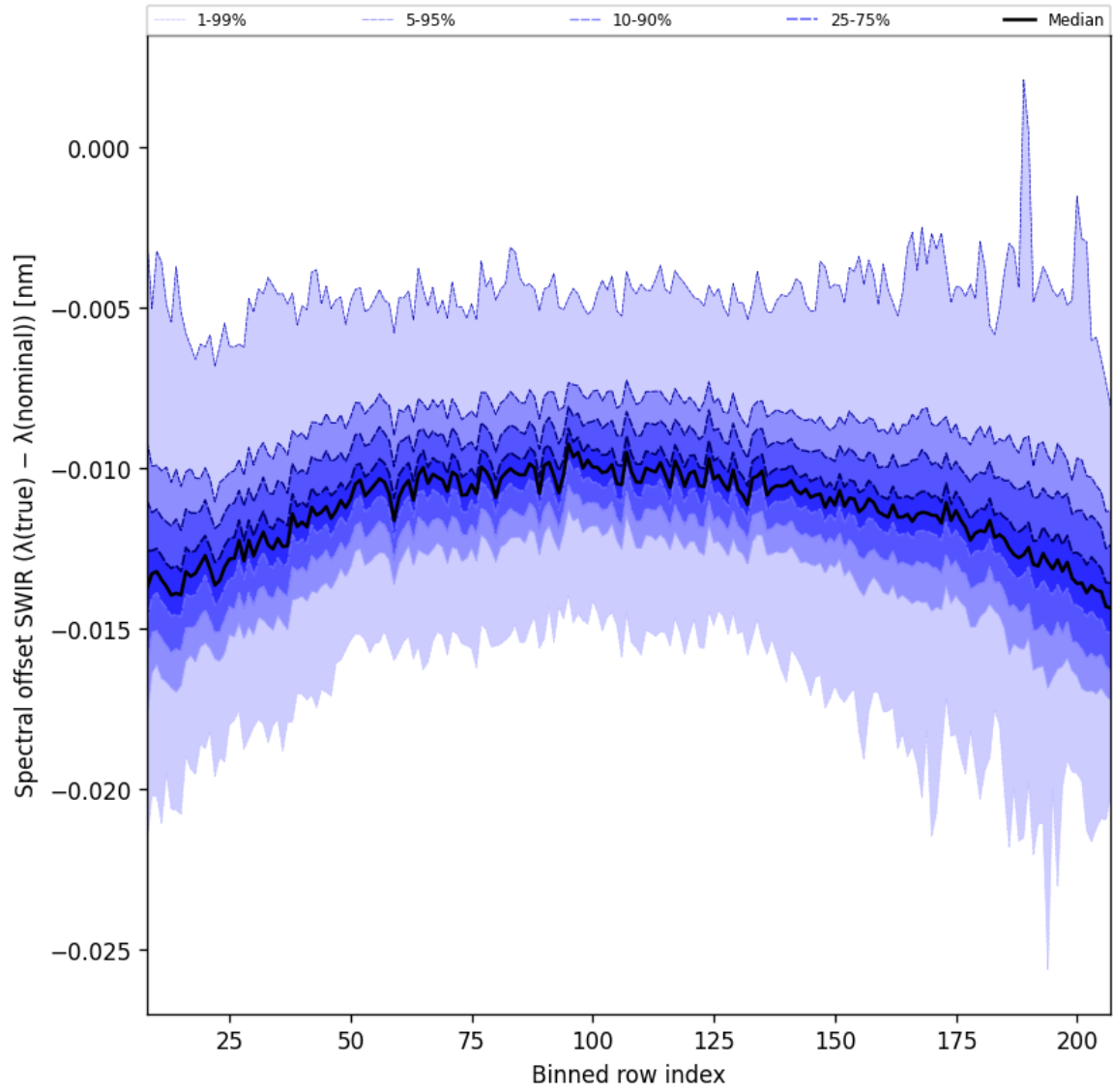
Figure 39: Along track statistics of “Spectral offset SWIR ( \lambda_{\text{true}} - \lambda_{\text{nominal}} )” for 2025-11-27 to 2025-11-28
