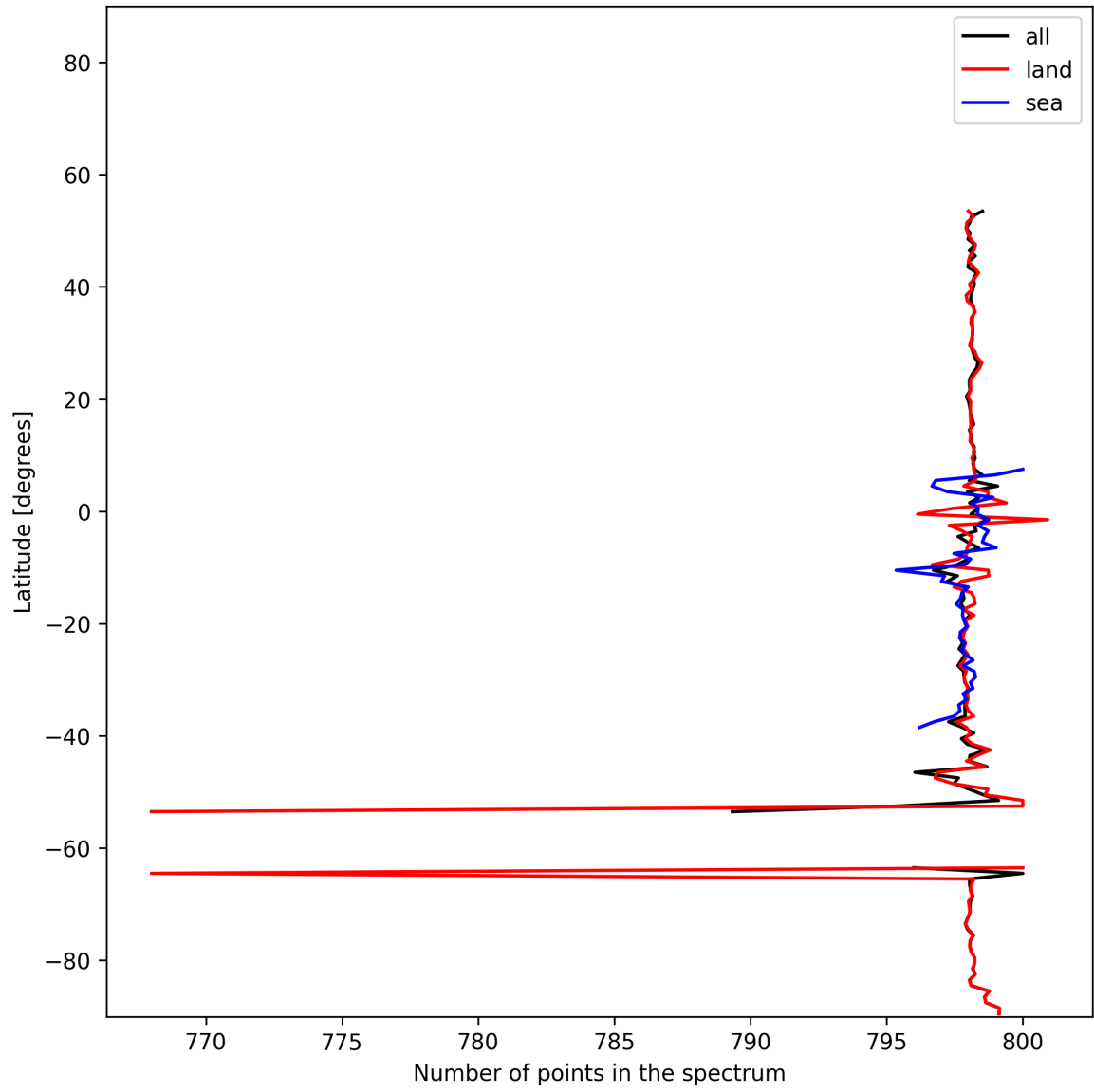
Figure 14: Zonal average of “Number of points in the spectrum” for 2025-11-27 to 2025-11-28.
