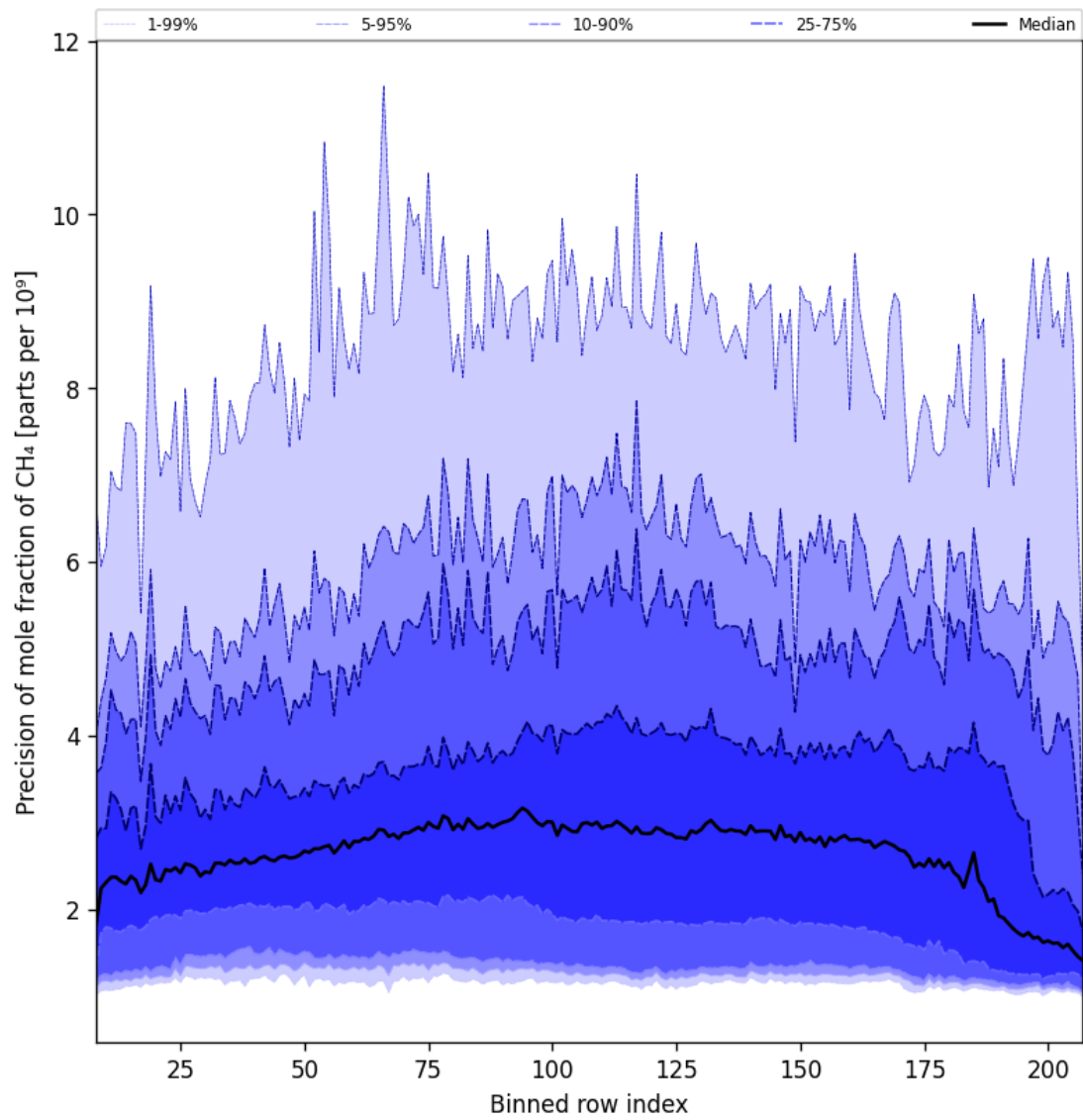
Figure 36: Along track statistics of “Precision of mole fraction of CH 4 ” for 2025-11-27 to 2025-11-28
