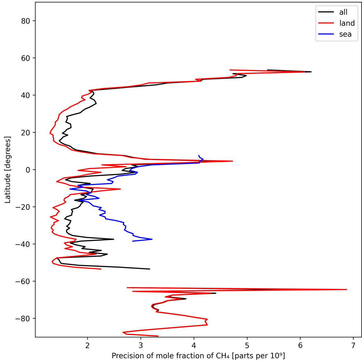
Figure 12: Zonal average of “Precision of mole fraction of CH 4 ” for 2025-11-27 to 2025-11-28.
