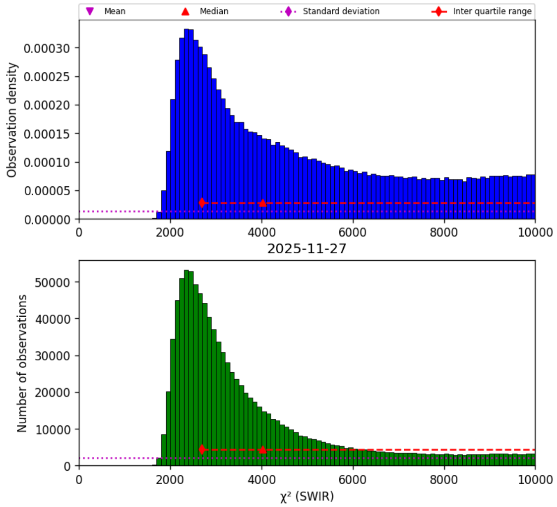
Figure 28: Histogram of “ \chi^2 (SWIR)” for 2025-11-27 to 2025-11-28
