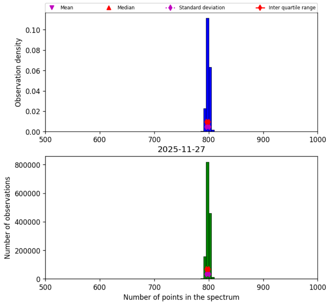
Figure 26: Histogram of “Number of points in the spectrum” for 2025-11-27 to 2025-11-28
