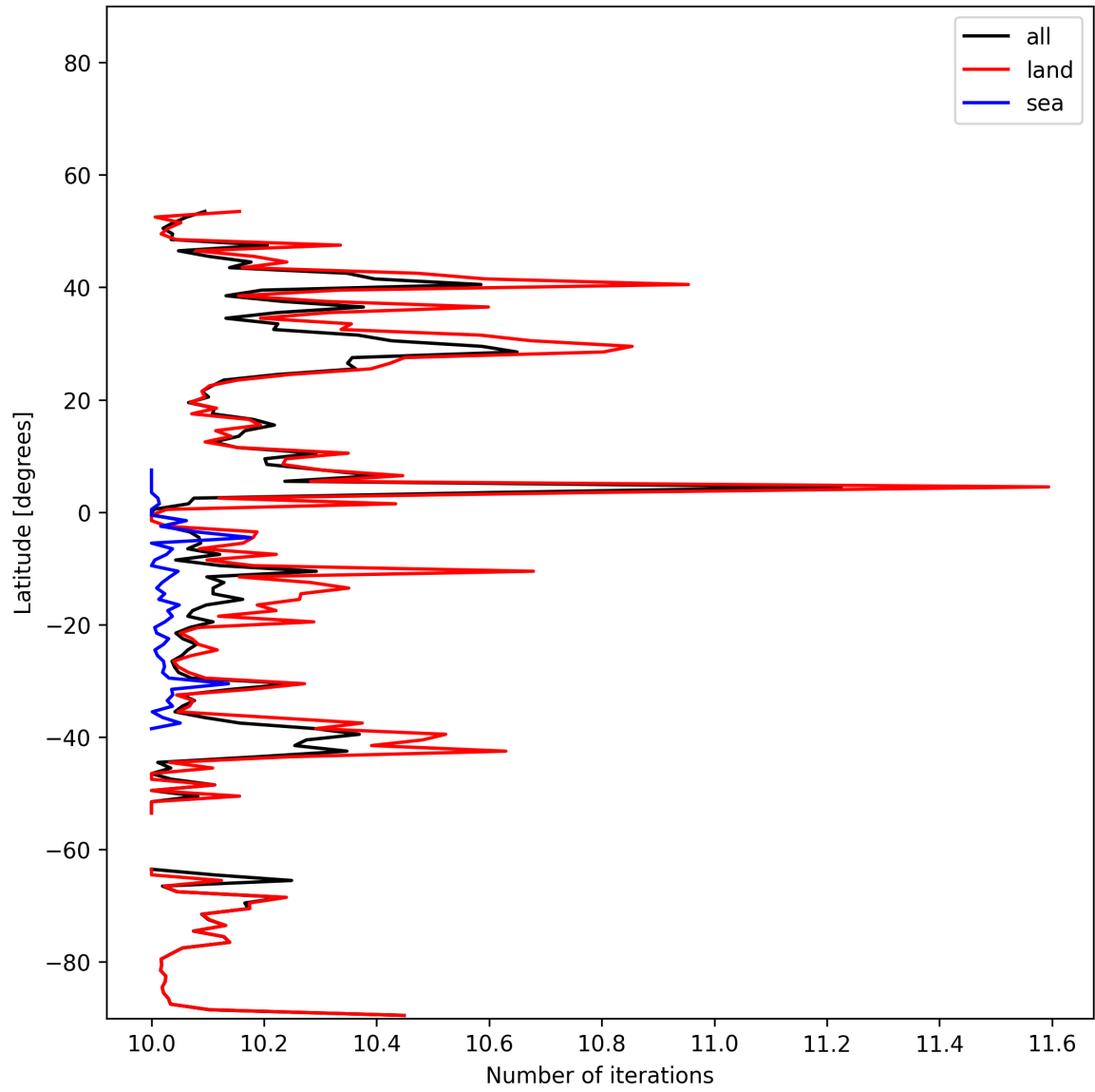
Figure 19: Zonal average of “Number of iterations” for 2025-11-27 to 2025-11-28.
