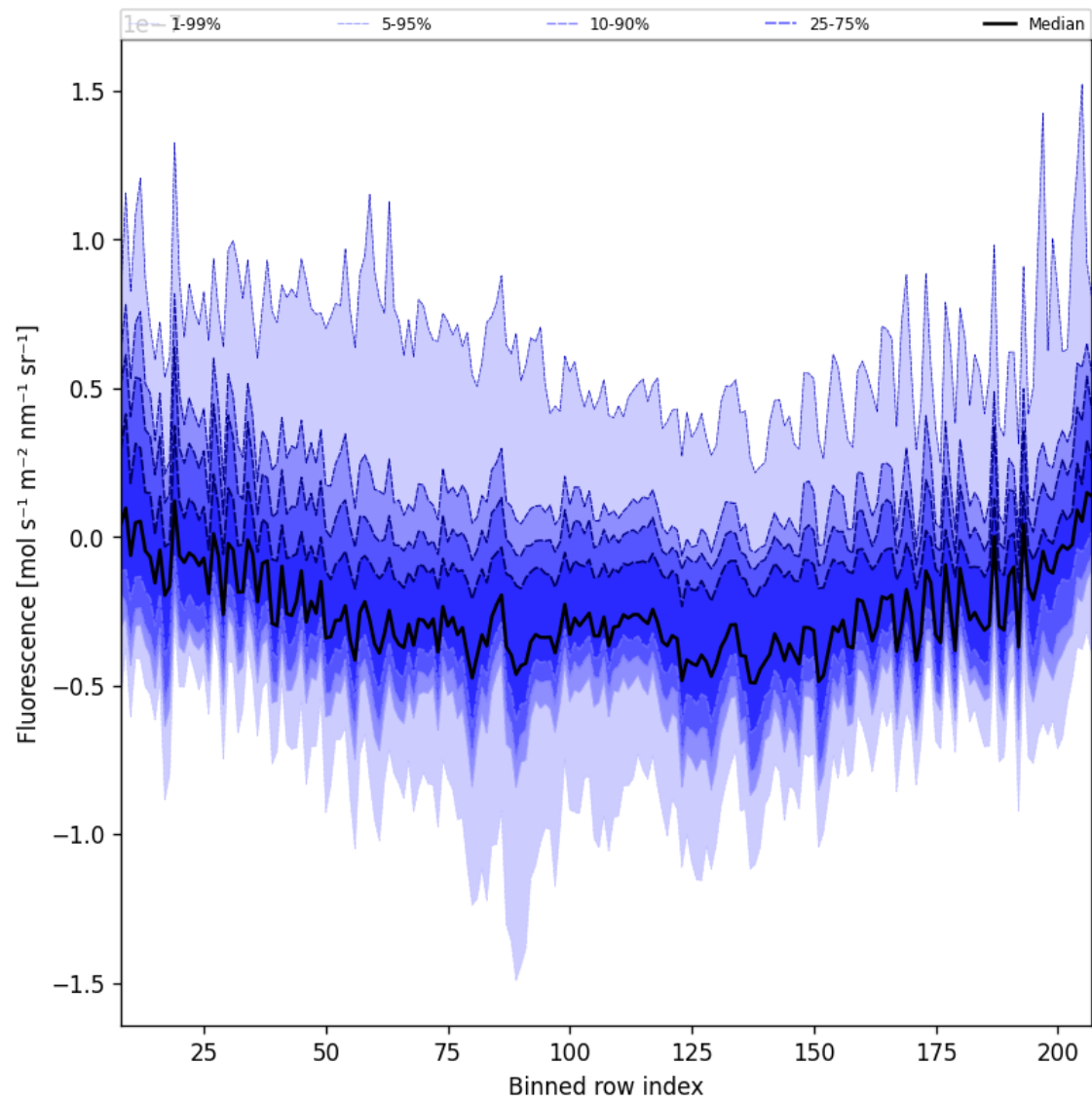
Figure 44: Along track statistics of “Fluorescence” for 2025-11-27 to 2025-11-28
