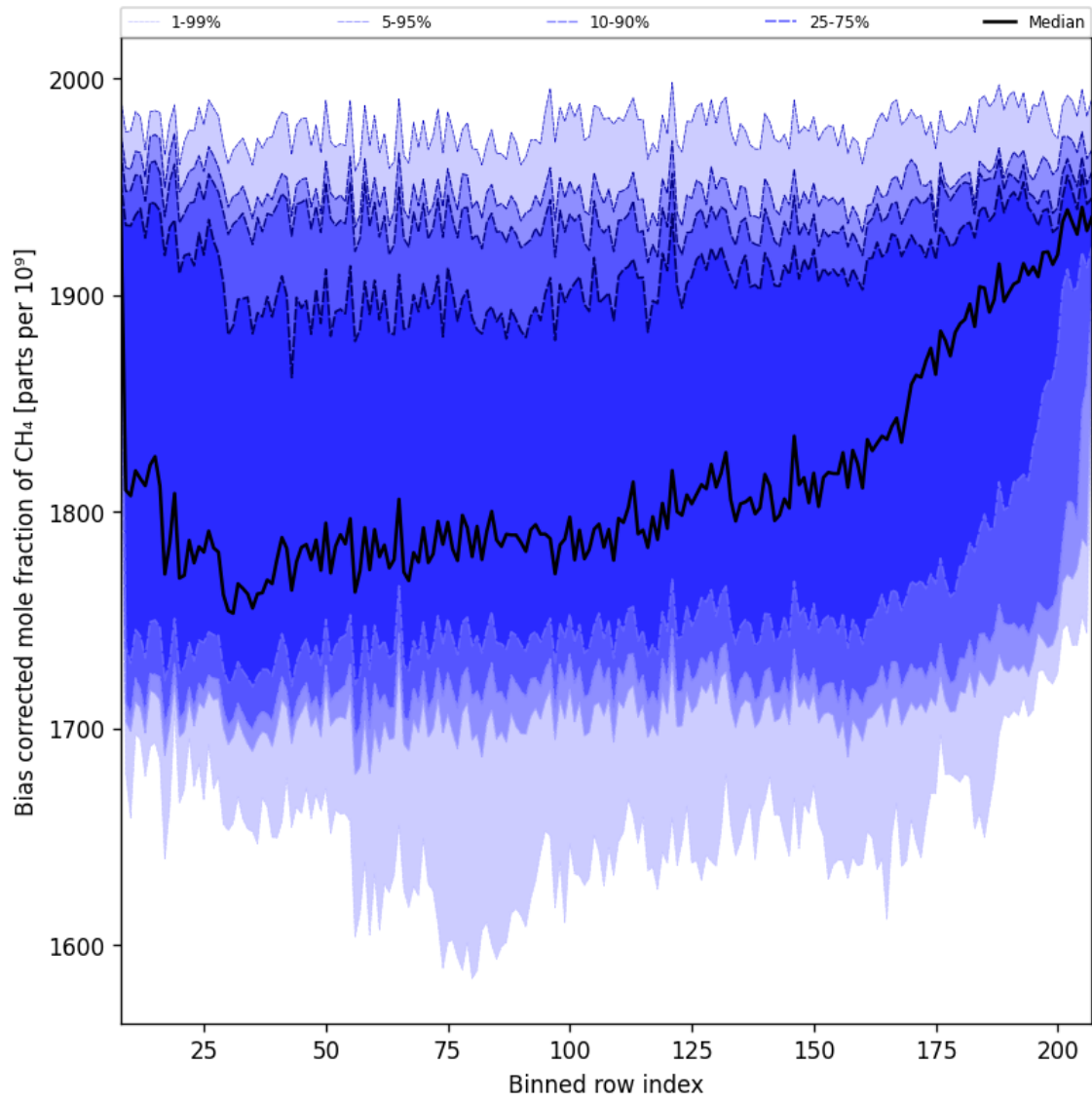
Figure 37: Along track statistics of “Bias corrected mole fraction of CH 4 ” for 2025-11-27 to 2025-11-28
