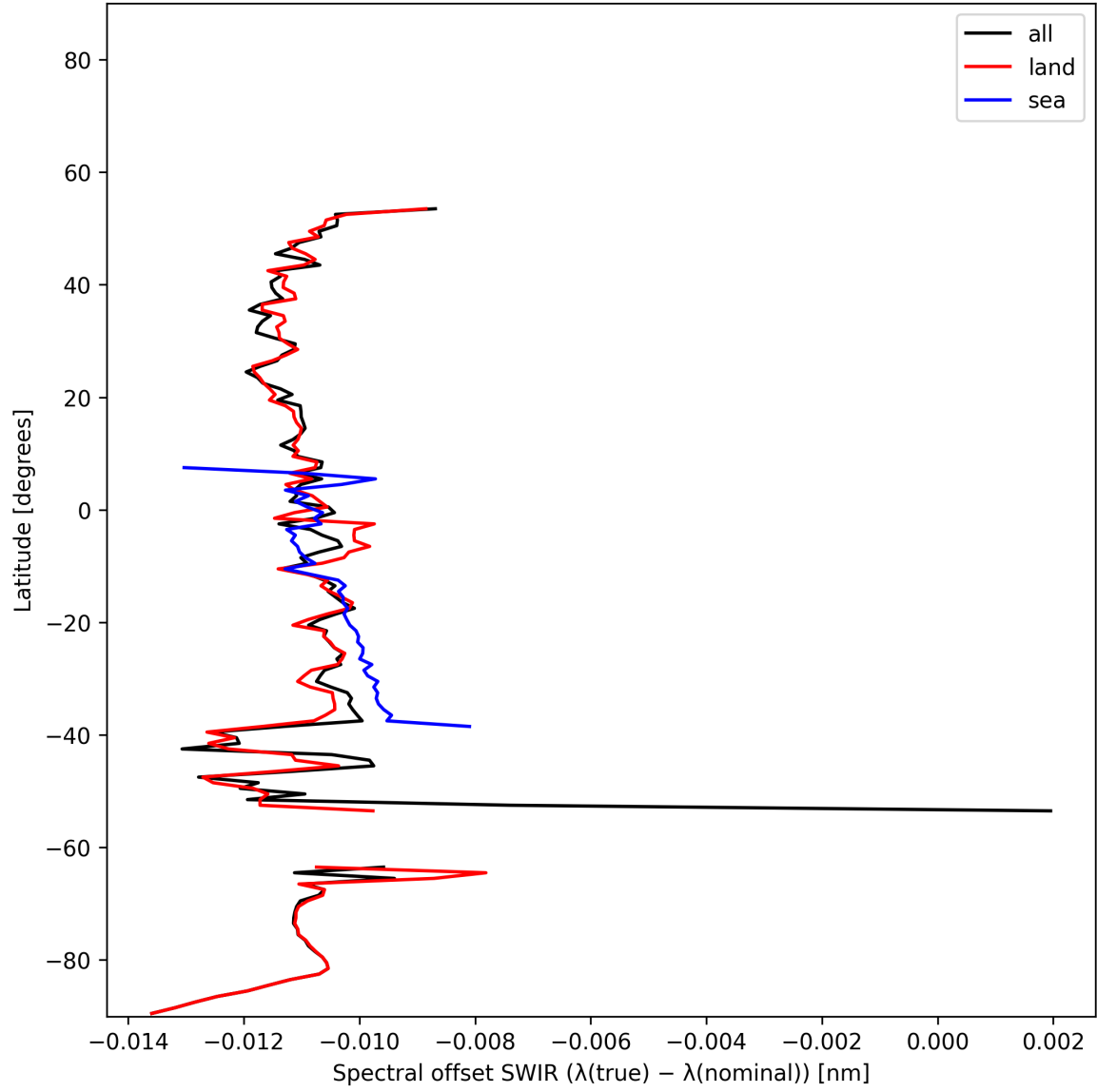
Figure 15: Zonal average of “Spectral offset SWIR ( \lambda_{\text{true}} - \lambda_{\text{nominal}} )” for 2025-11-27 to 2025-11-28.
