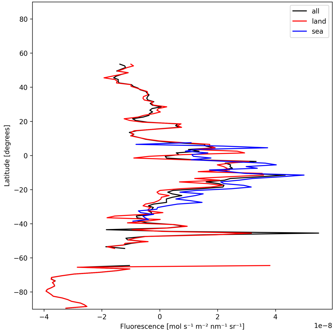
Figure 20: Zonal average of “Fluorescence” for 2025-11-28 to 2025-11-29.
