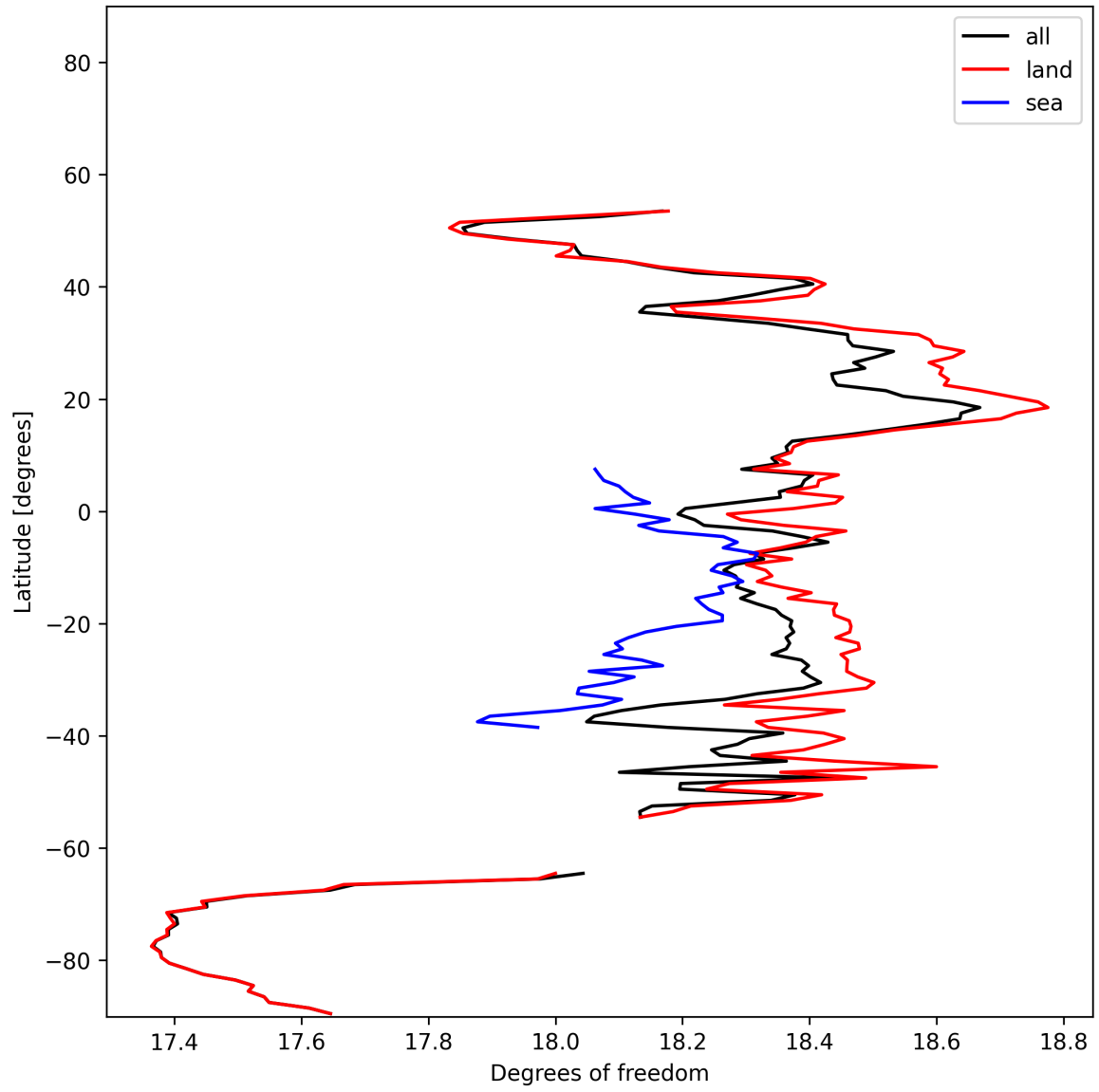
Figure 18: Zonal average of “Degrees of freedom” for 2025-11-28 to 2025-11-29.
