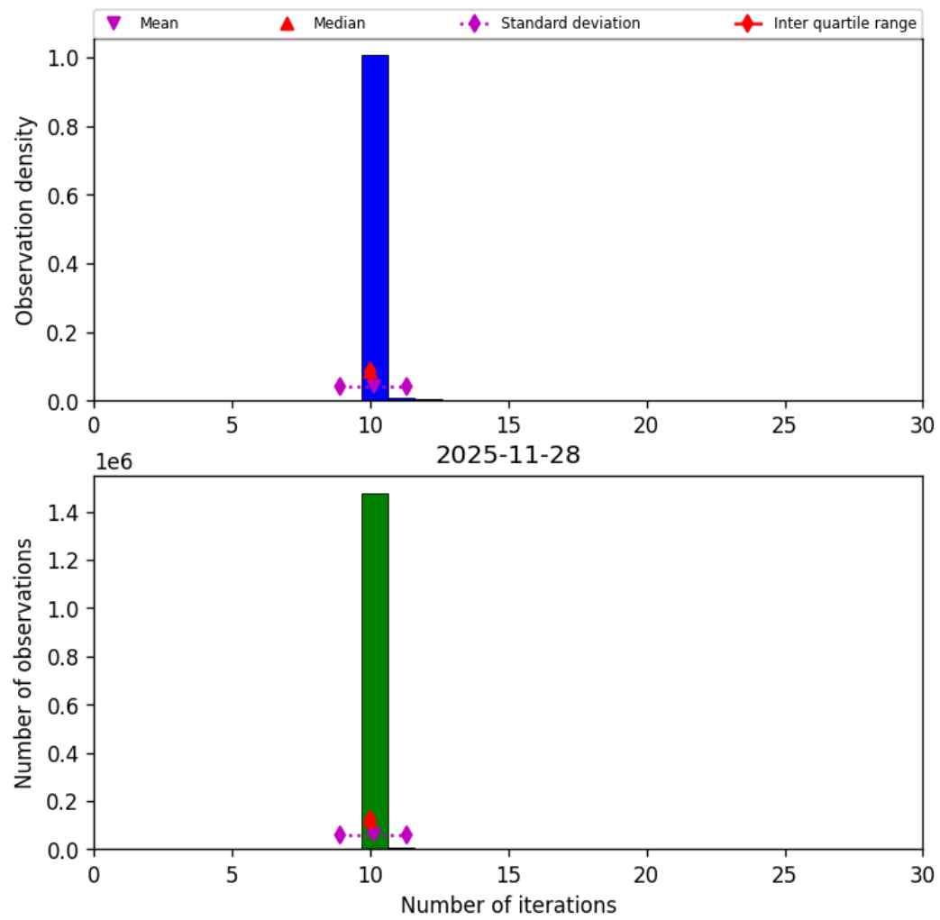
Figure 31: Histogram of “Number of iterations” for 2025-11-28 to 2025-11-29
