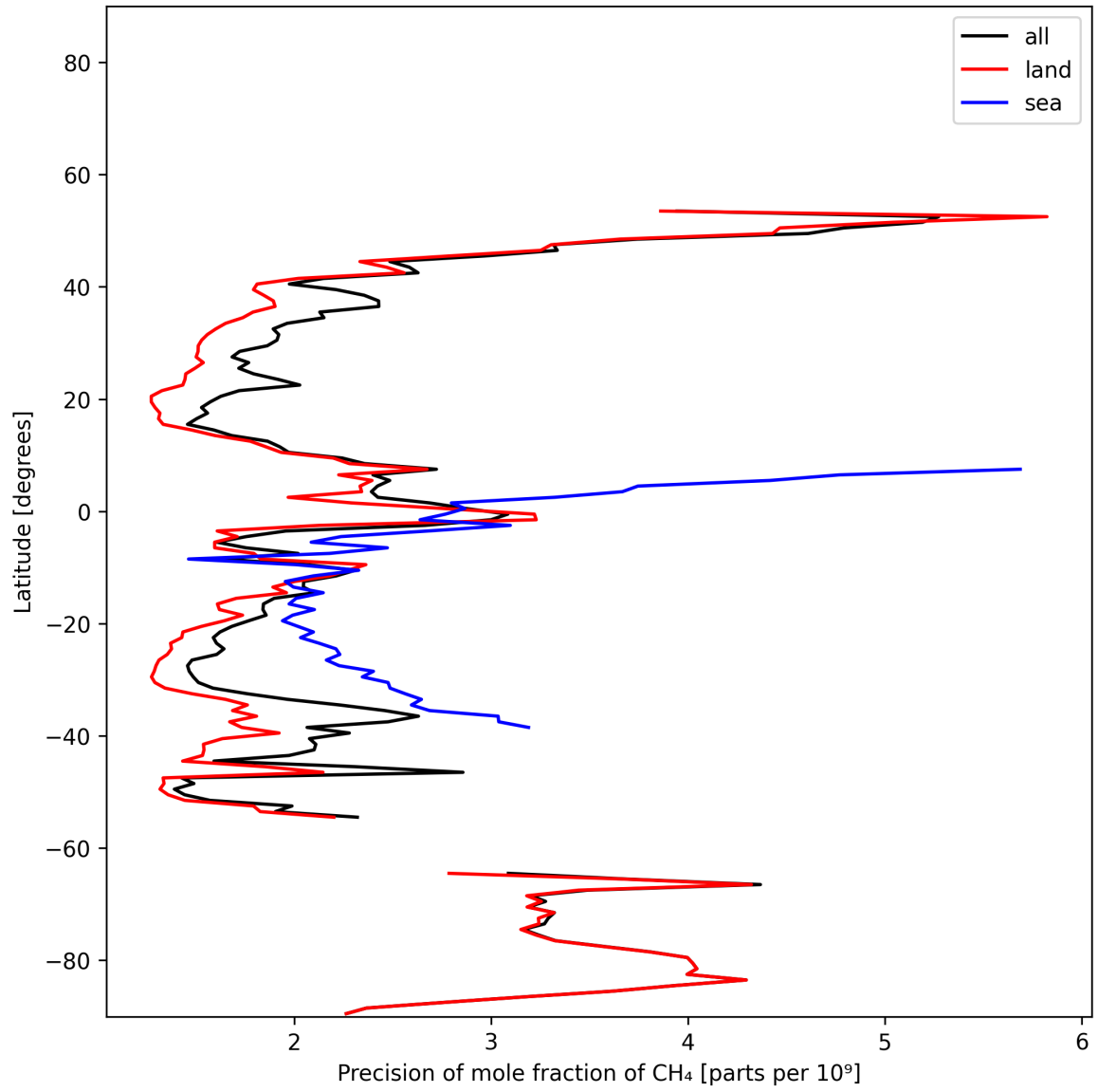
Figure 12: Zonal average of “Precision of mole fraction of CH 4 ” for 2025-11-28 to 2025-11-29.
