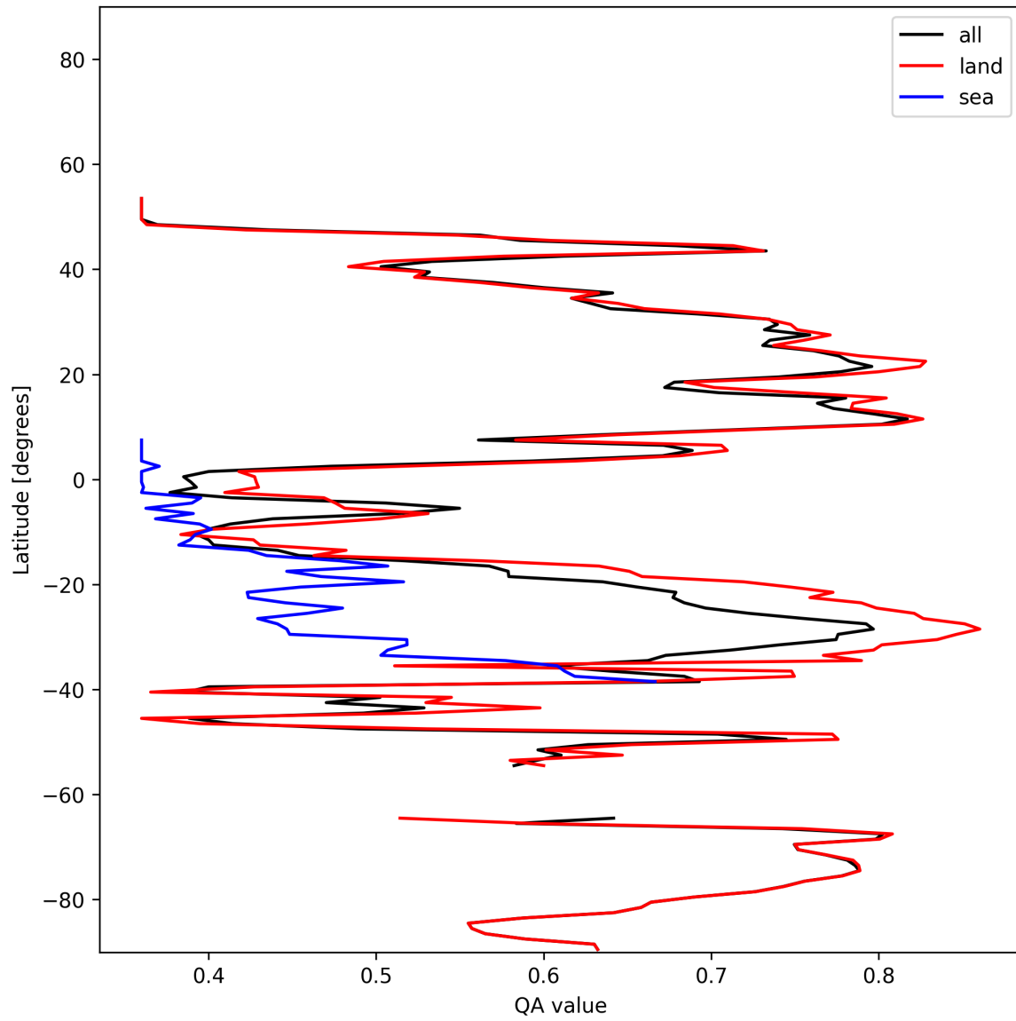
Figure 10: Zonal average of “QA value” for 2025-11-28 to 2025-11-29.
