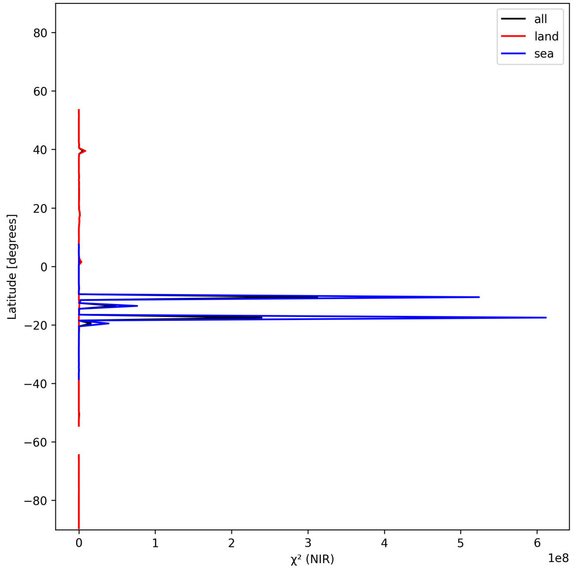
Figure 17: Zonal average of “ \chi^2 (NIR)” for 2025-11-28 to 2025-11-29.
