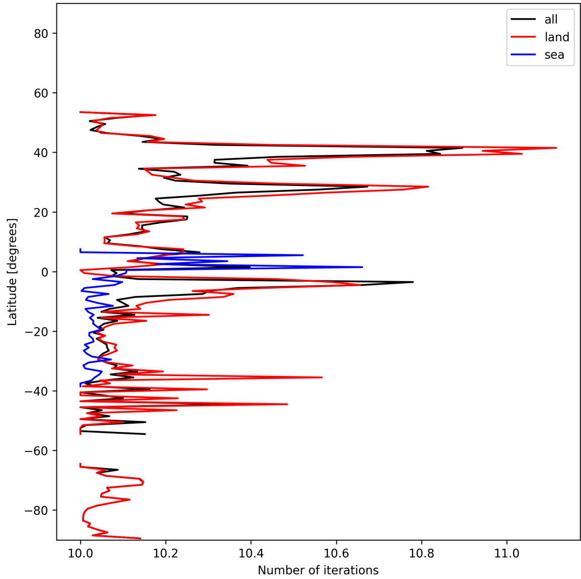
Figure 19: Zonal average of “Number of iterations” for 2025-11-28 to 2025-11-29.
