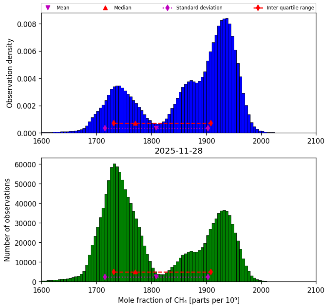
Figure 23: Histogram of “Mole fraction of CH 4 ” for 2025-11-28 to 2025-11-29
