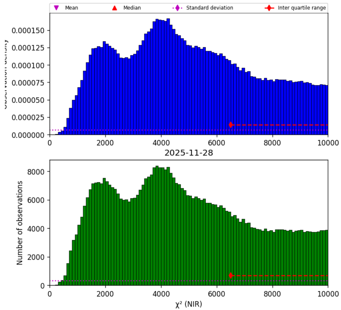
Figure 29: Histogram of “ \chi^2 (NIR)” for 2025-11-28 to 2025-11-29
