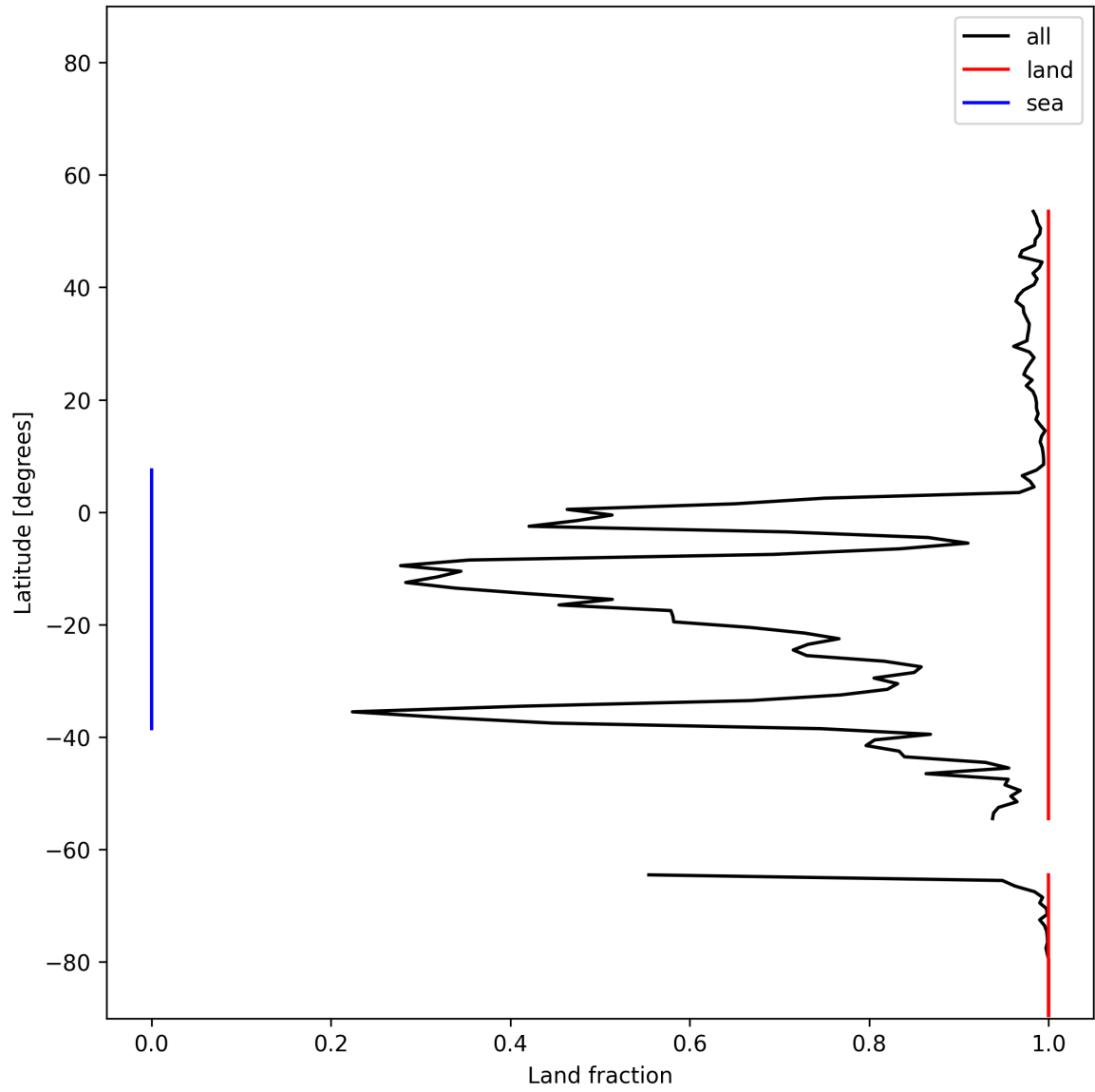
Figure 21: Zonal average of “Land fraction” for 2025-11-28 to 2025-11-29.
