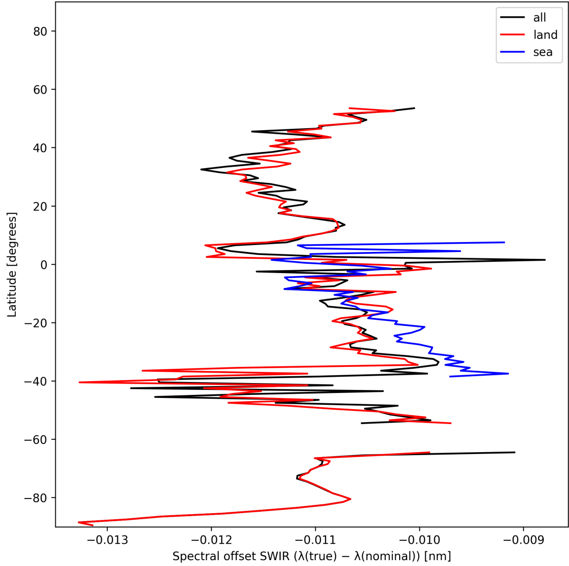
Figure 15: Zonal average of “Spectral offset SWIR ( \lambda_{\text{true}} - \lambda_{\text{nominal}} )” for 2025-11-28 to 2025-11-29.
