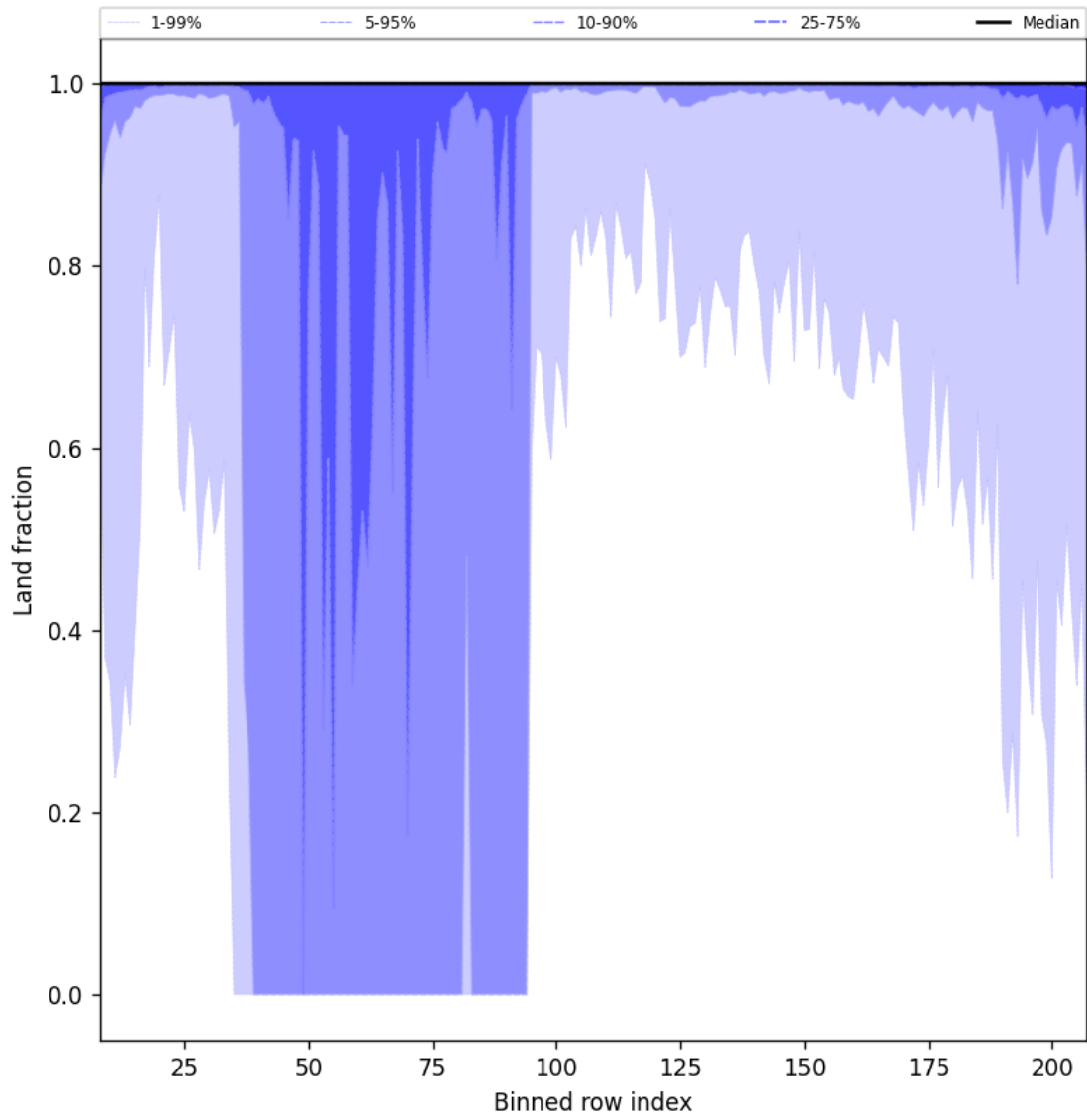
Figure 45: Along track statistics of “Land fraction” for 2025-11-28 to 2025-11-29
