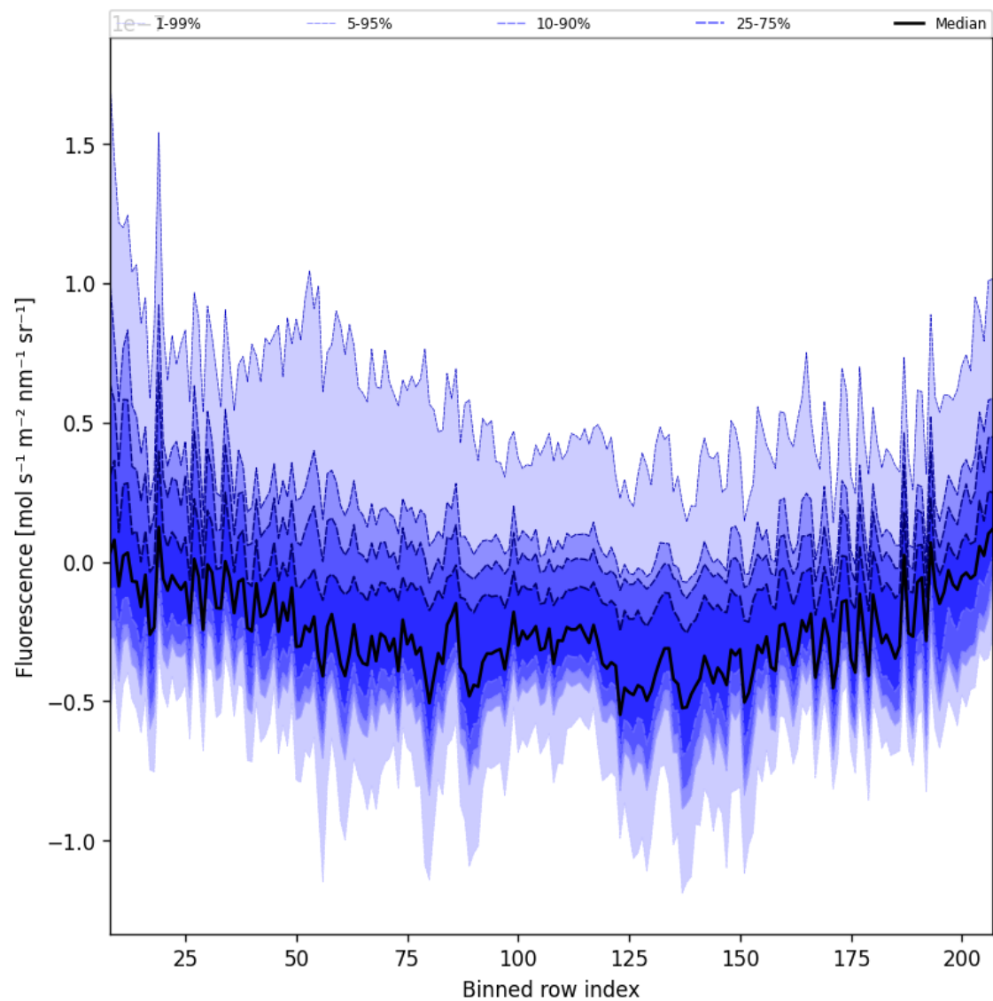
Figure 44: Along track statistics of “Fluorescence” for 2025-11-28 to 2025-11-29
