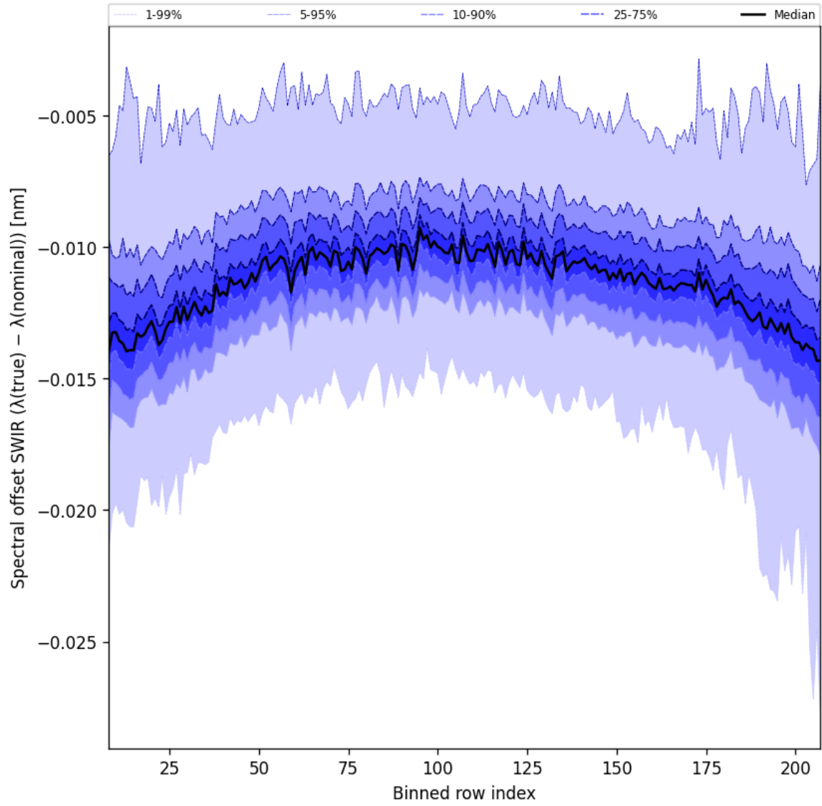
Figure 39: Along track statistics of “Spectral offset SWIR ( \lambda_{\text{true}} - \lambda_{\text{nominal}} )” for 2025-11-28 to 2025-11-29
