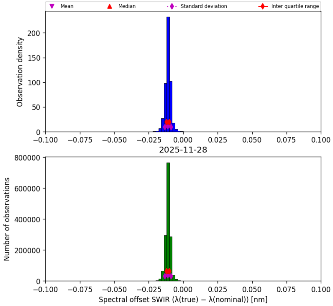
Figure 27: Histogram of “Spectral offset SWIR ( \lambda_{\text{true}} - \lambda_{\text{nominal}} )” for 2025-11-28 to 2025-11-29
