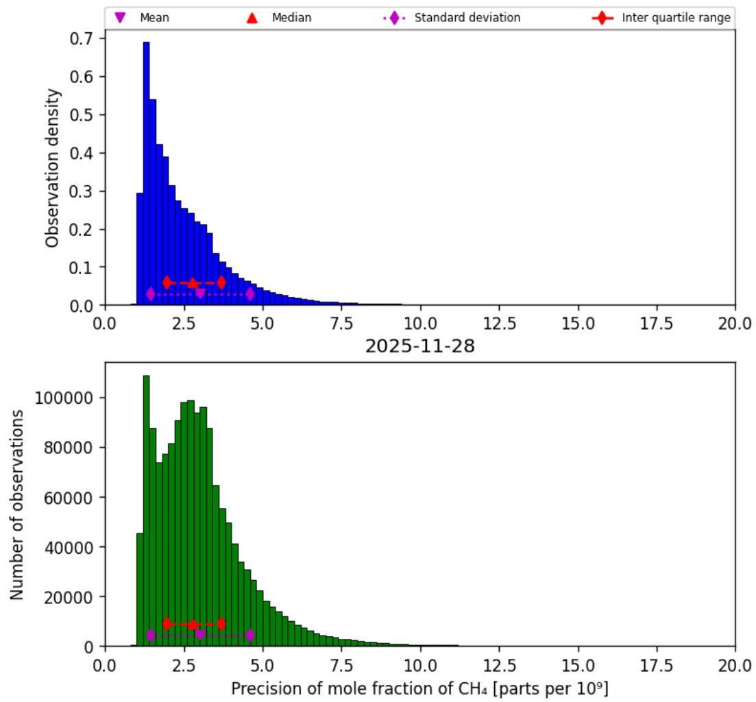
Figure 24: Histogram of “Precision of mole fraction of CH 4 ” for 2025-11-28 to 2025-11-29
