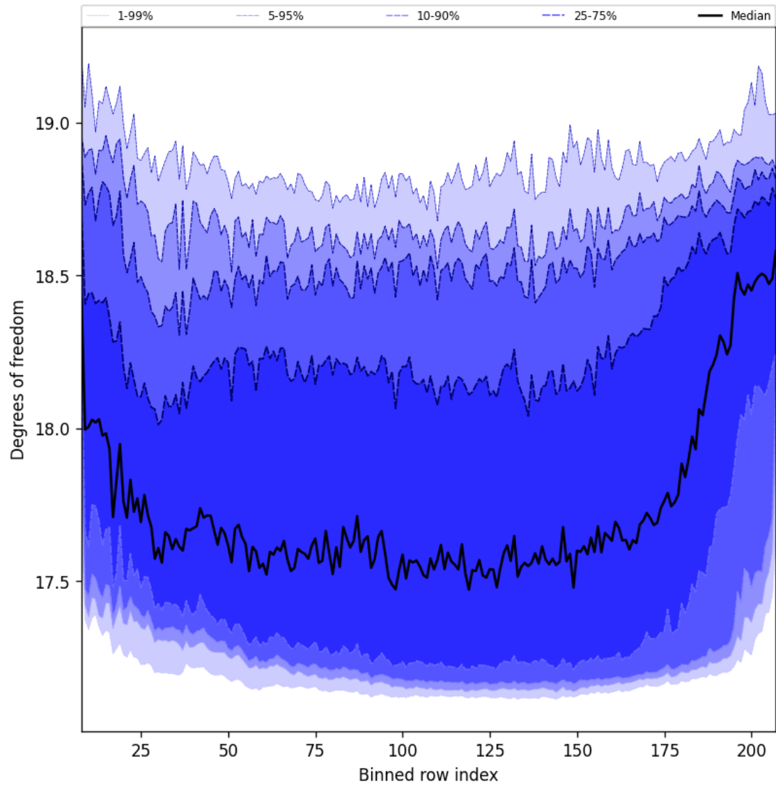
Figure 42: Along track statistics of “Degrees of freedom” for 2025-11-28 to 2025-11-29
