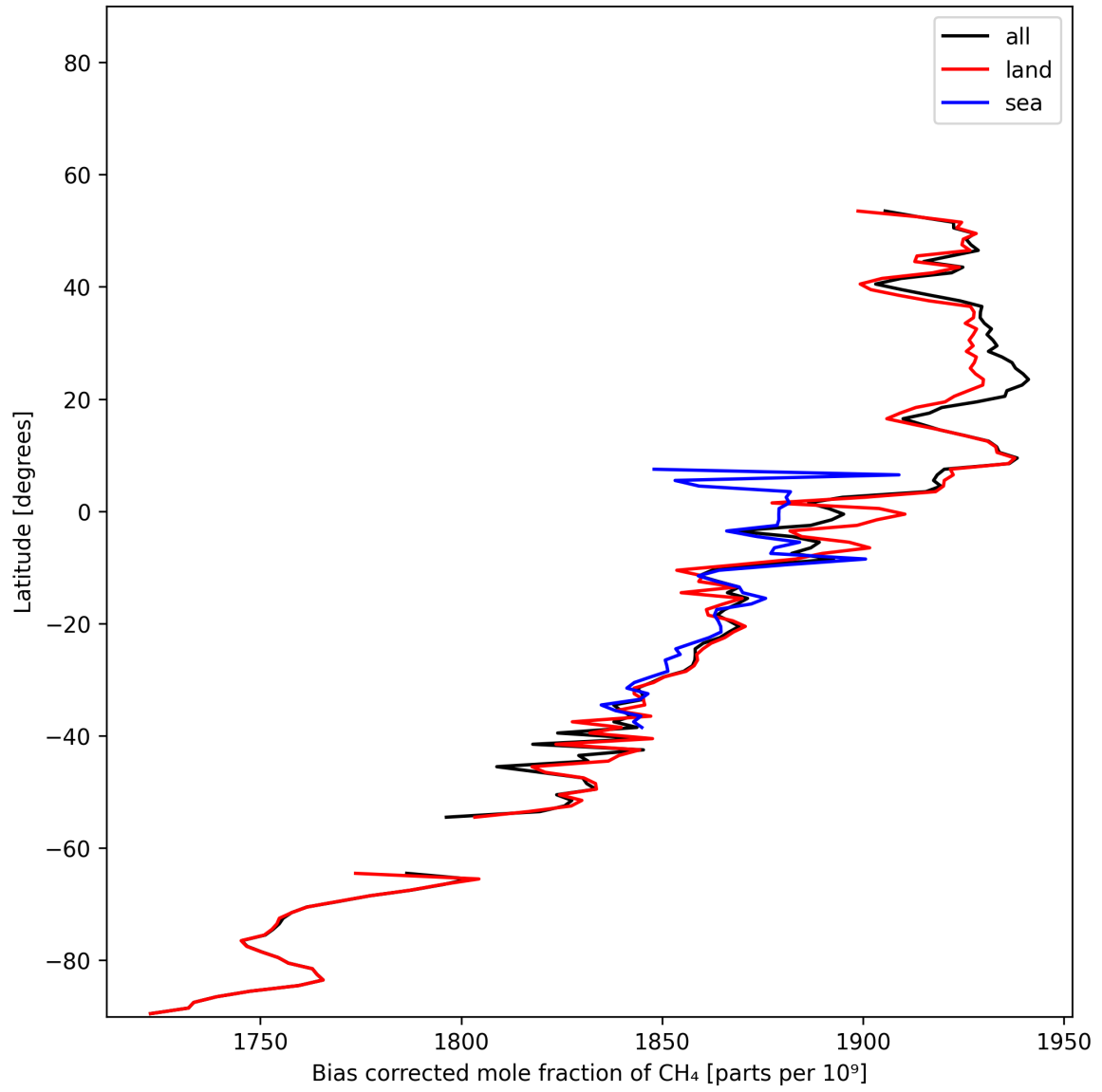
Figure 13: Zonal average of “Bias corrected mole fraction of CH 4 ” for 2025-11-28 to 2025-11-29.
