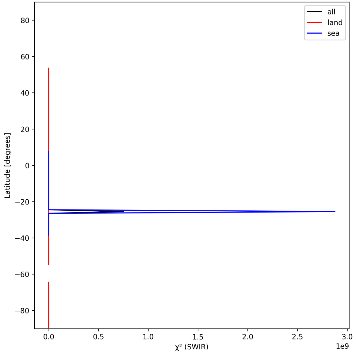
Figure 16: Zonal average of “ \chi^2 (SWIR)” for 2025-11-28 to 2025-11-29.
