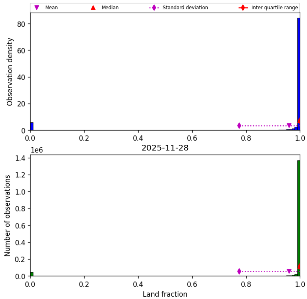
Figure 33: Histogram of "Land fraction" for 2025-11-28 to 2025-11-29
