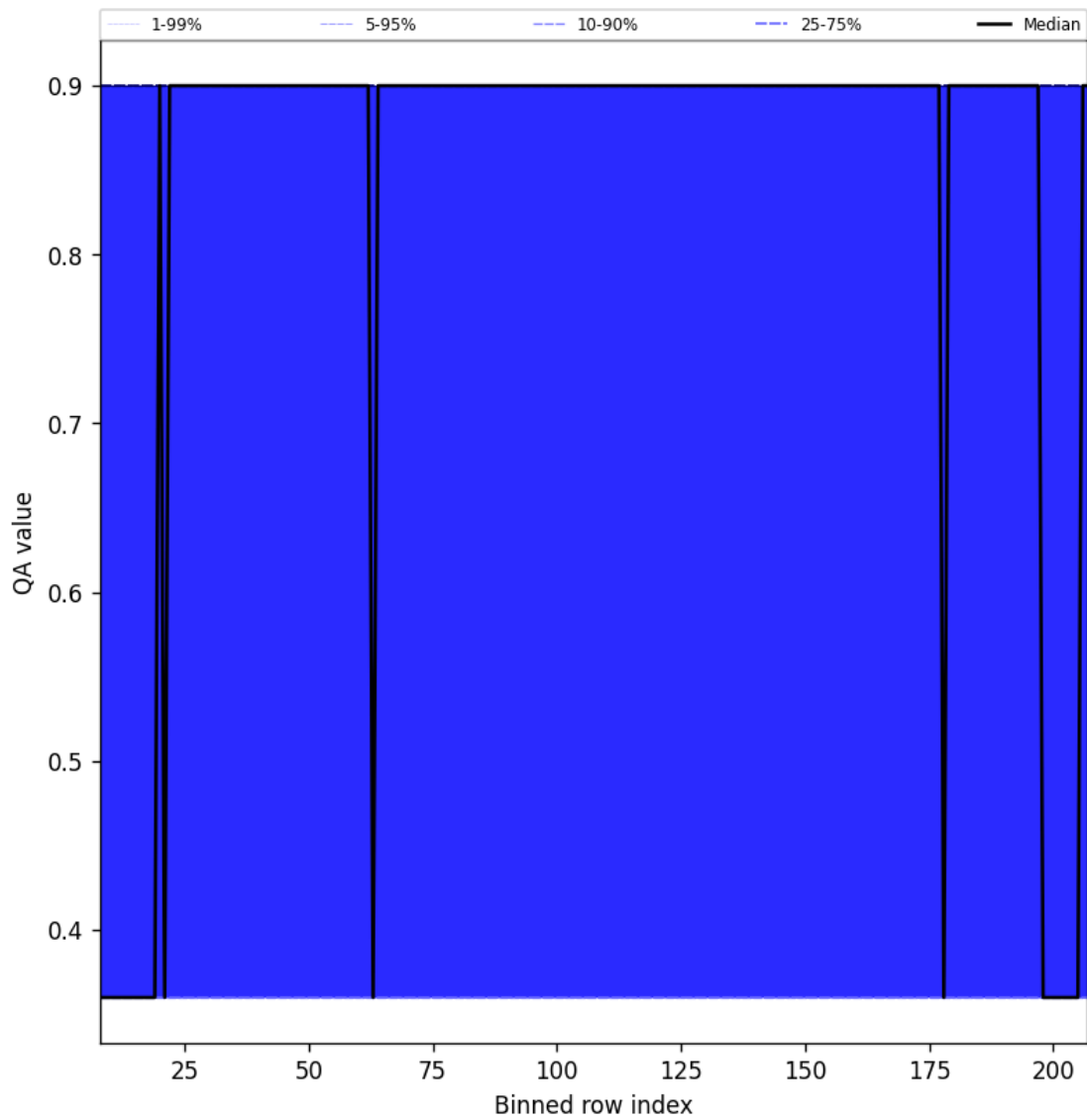
Figure 34: Along track statistics of “QA value” for 2025-11-28 to 2025-11-29
