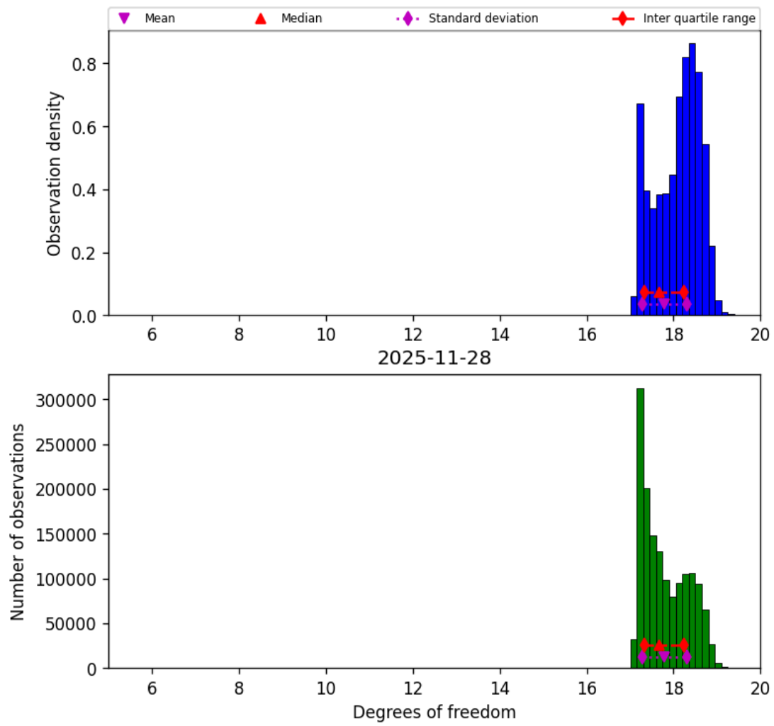
Figure 30: Histogram of “Degrees of freedom” for 2025-11-28 to 2025-11-29
