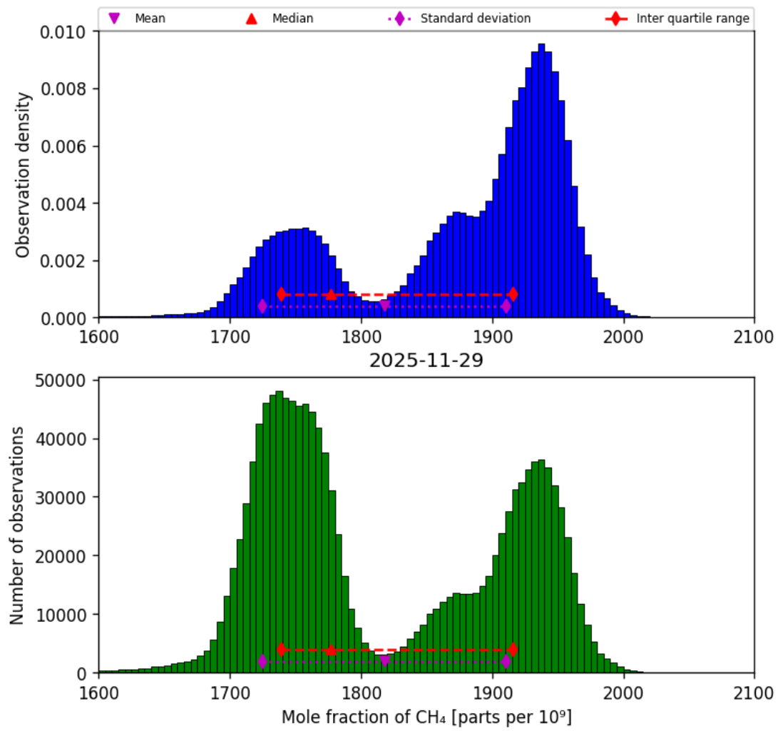
Figure 23: Histogram of “Mole fraction of CH 4 ” for 2025-11-29 to 2025-11-30
