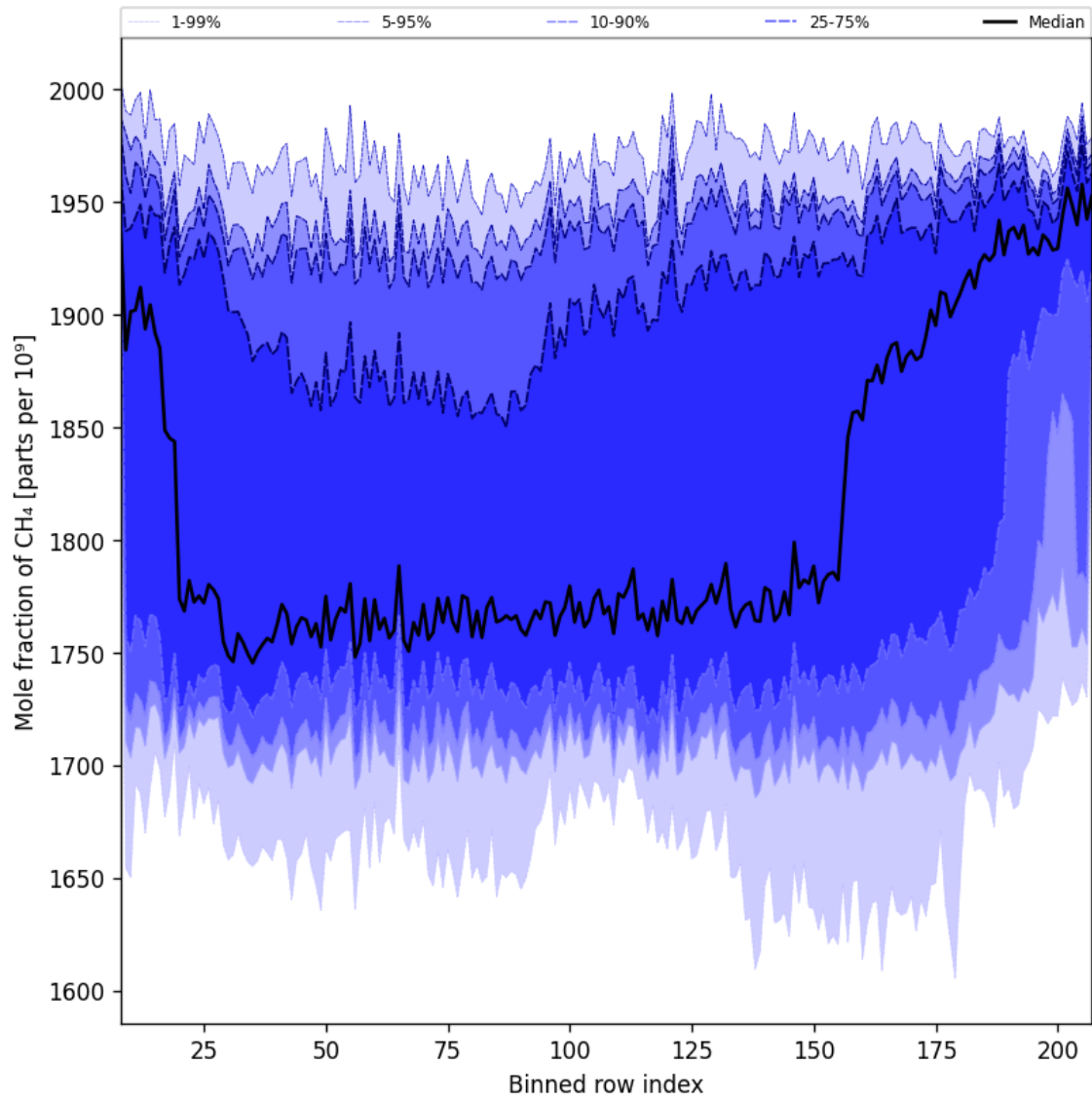
Figure 35: Along track statistics of “Mole fraction of CH 4 ” for 2025-11-29 to 2025-11-30
