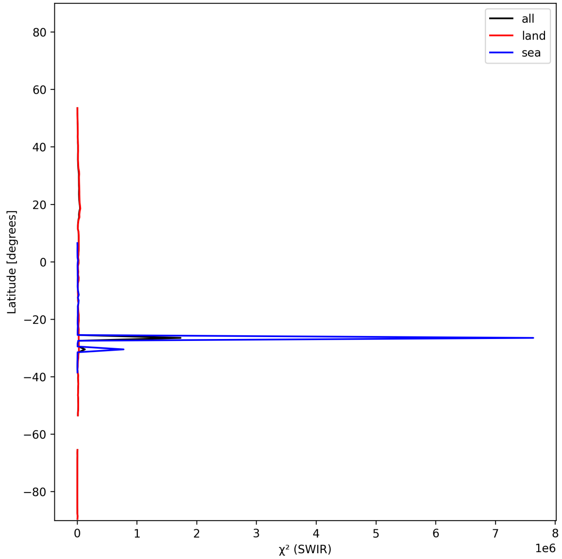
Figure 16: Zonal average of “ \chi^2 (SWIR)” for 2025-11-29 to 2025-11-30.
