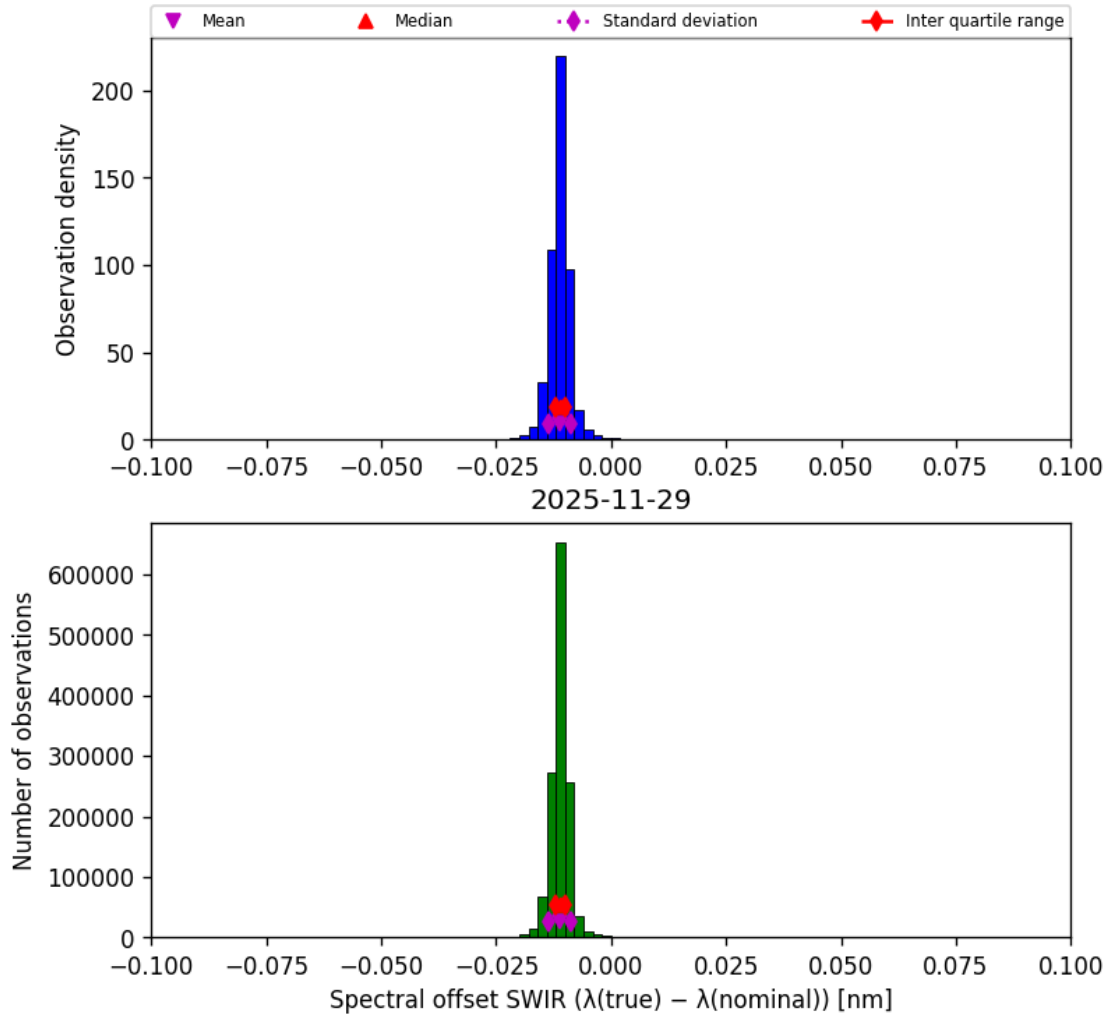
Figure 27: Histogram of “Spectral offset SWIR ( \lambda_{\text{true}} - \lambda_{\text{nominal}} )” for 2025-11-29 to 2025-11-30
