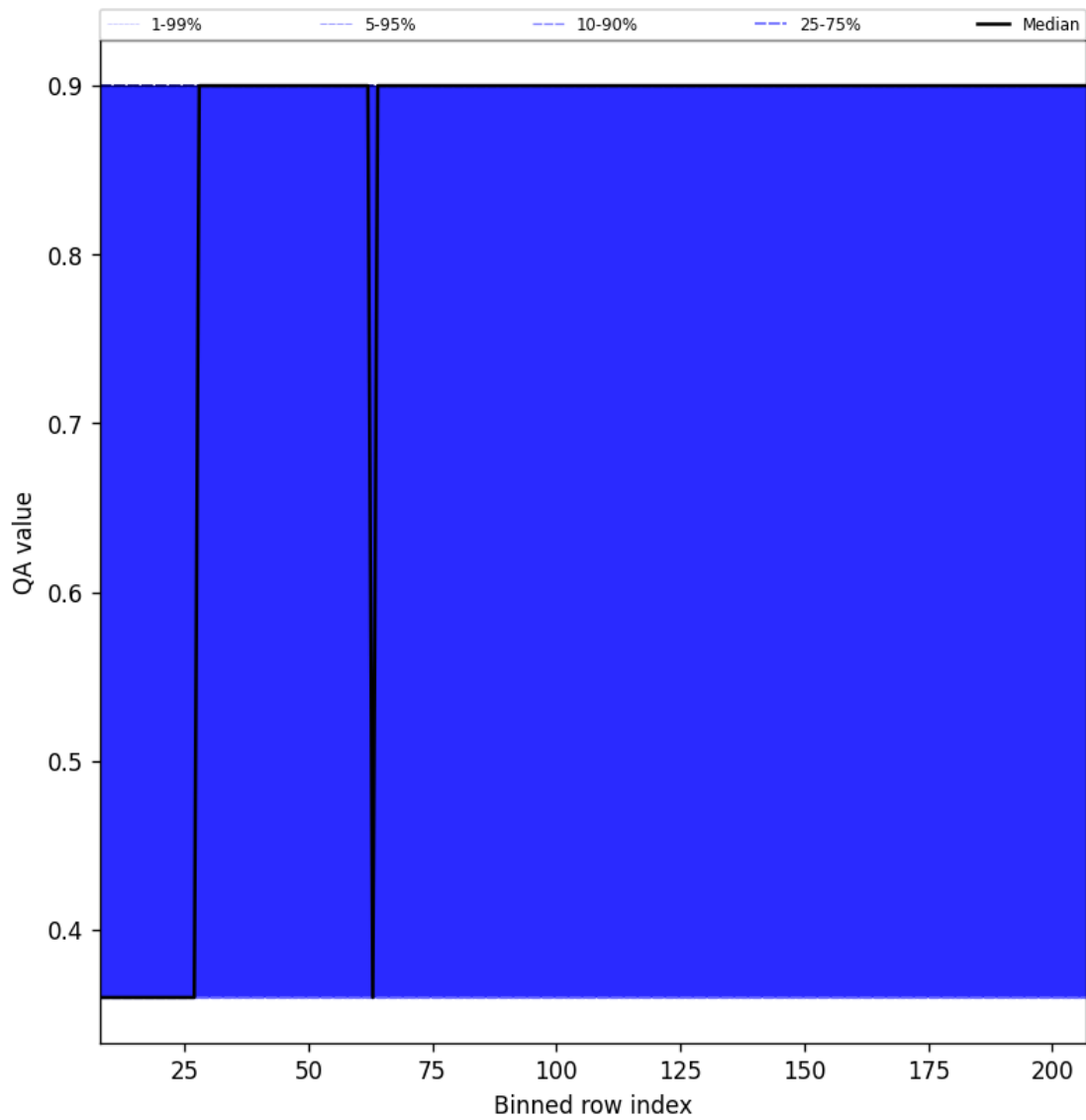
Figure 34: Along track statistics of “QA value” for 2025-11-29 to 2025-11-30
