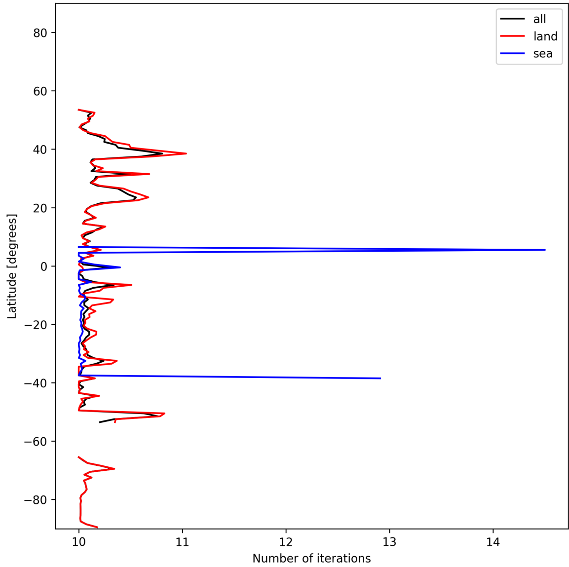
Figure 19: Zonal average of “Number of iterations” for 2025-11-29 to 2025-11-30.
