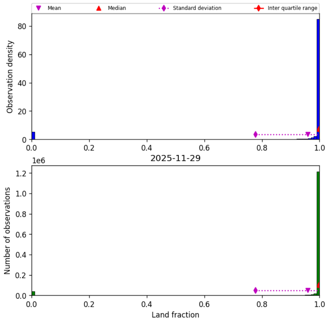
Figure 33: Histogram of “Land fraction” for 2025-11-29 to 2025-11-30
