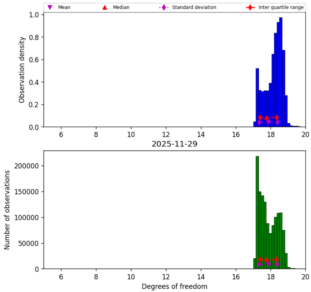
Figure 30: Histogram of “Degrees of freedom” for 2025-11-29 to 2025-11-30
