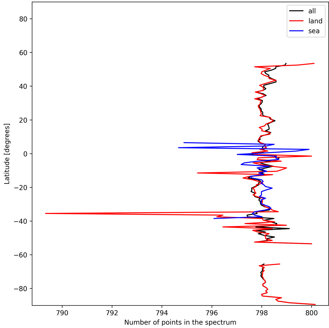
Figure 14: Zonal average of “Number of points in the spectrum” for 2025-11-29 to 2025-11-30.
