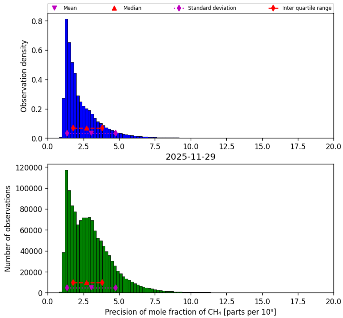
Figure 24: Histogram of “Precision of mole fraction of CH 4 ” for 2025-11-29 to 2025-11-30
