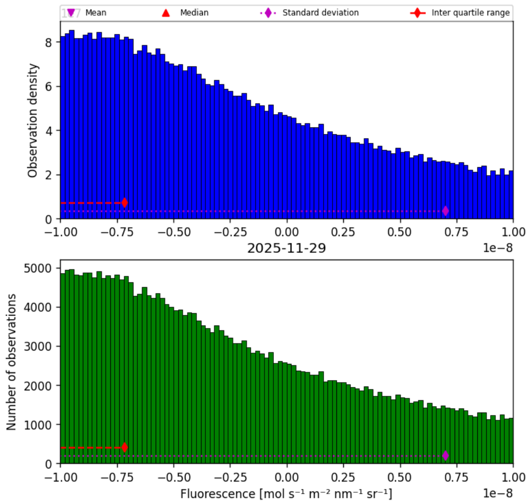
Figure 32: Histogram of “Fluorescence” for 2025-11-29 to 2025-11-30
