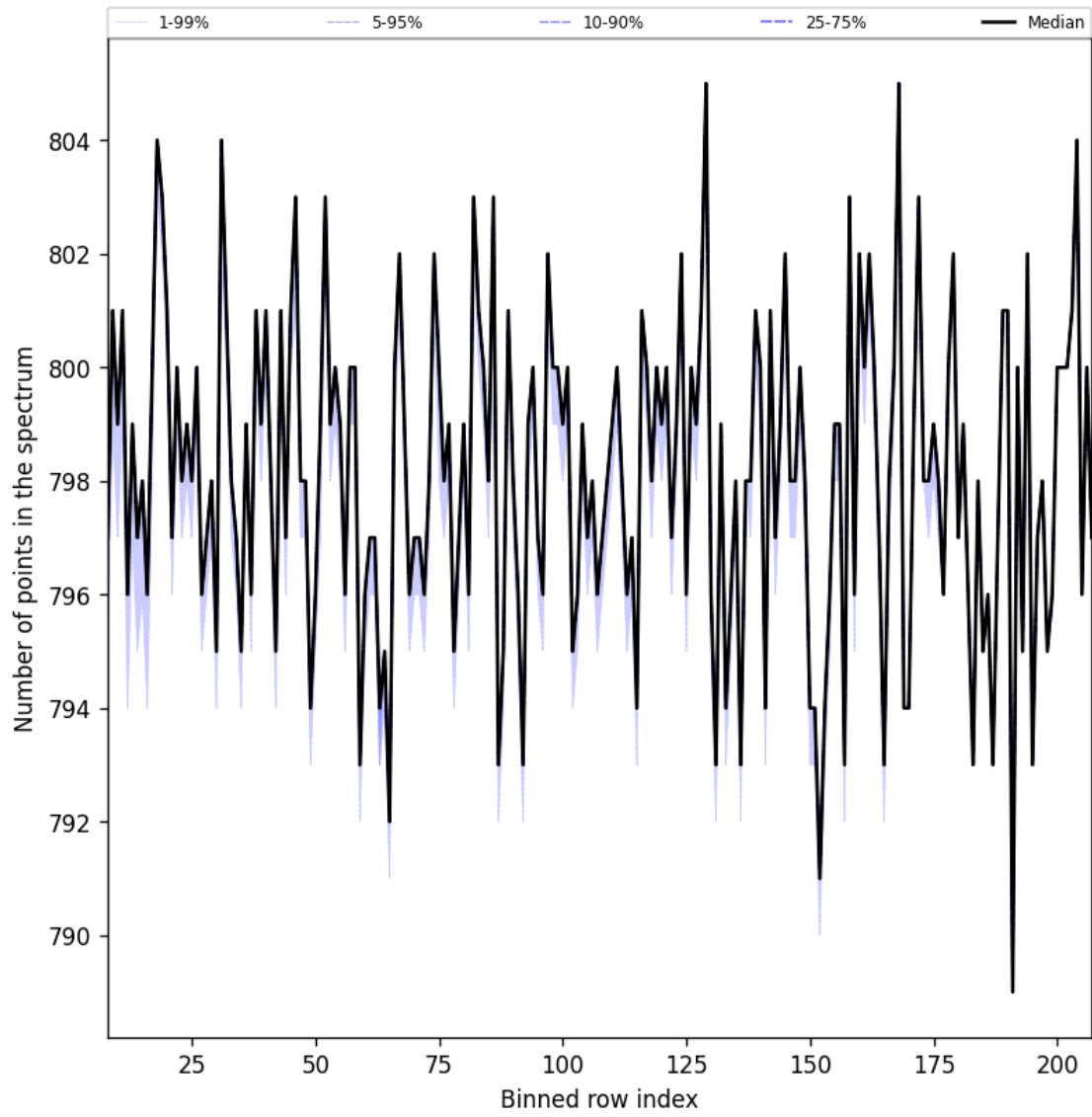
Figure 38: Along track statistics of “Number of points in the spectrum” for 2025-11-29 to 2025-11-30
