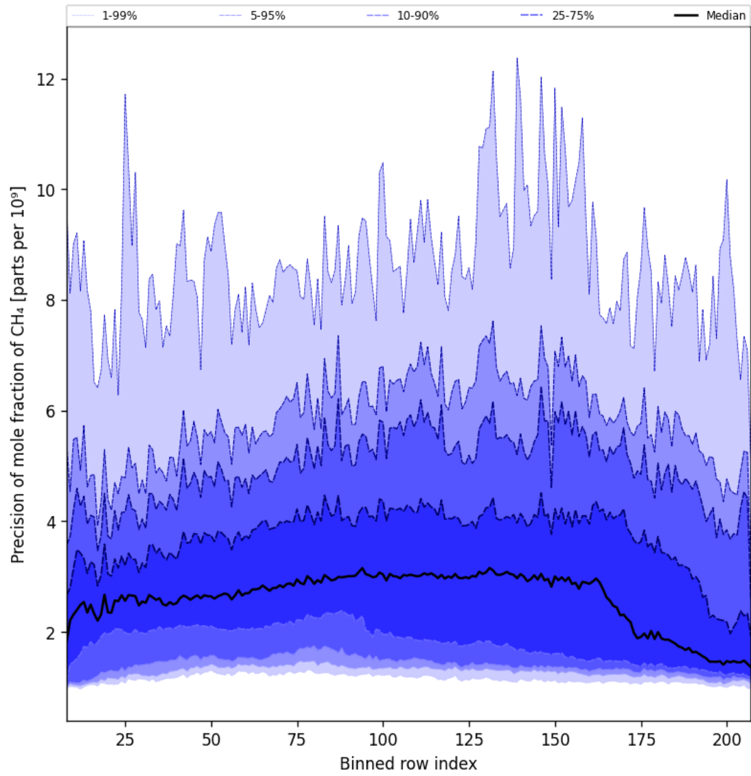
Figure 36: Along track statistics of “Precision of mole fraction of CH 4 ” for 2025-11-29 to 2025-11-30
