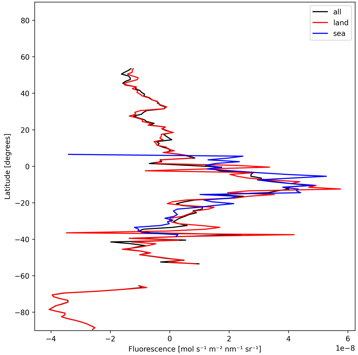
Figure 20: Zonal average of “Fluorescence” for 2025-11-29 to 2025-11-30.
