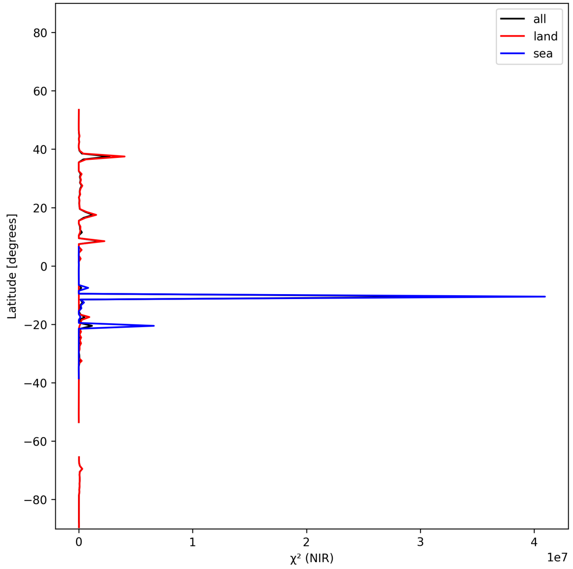
Figure 17: Zonal average of “ \chi^2 (NIR)” for 2025-11-29 to 2025-11-30.
