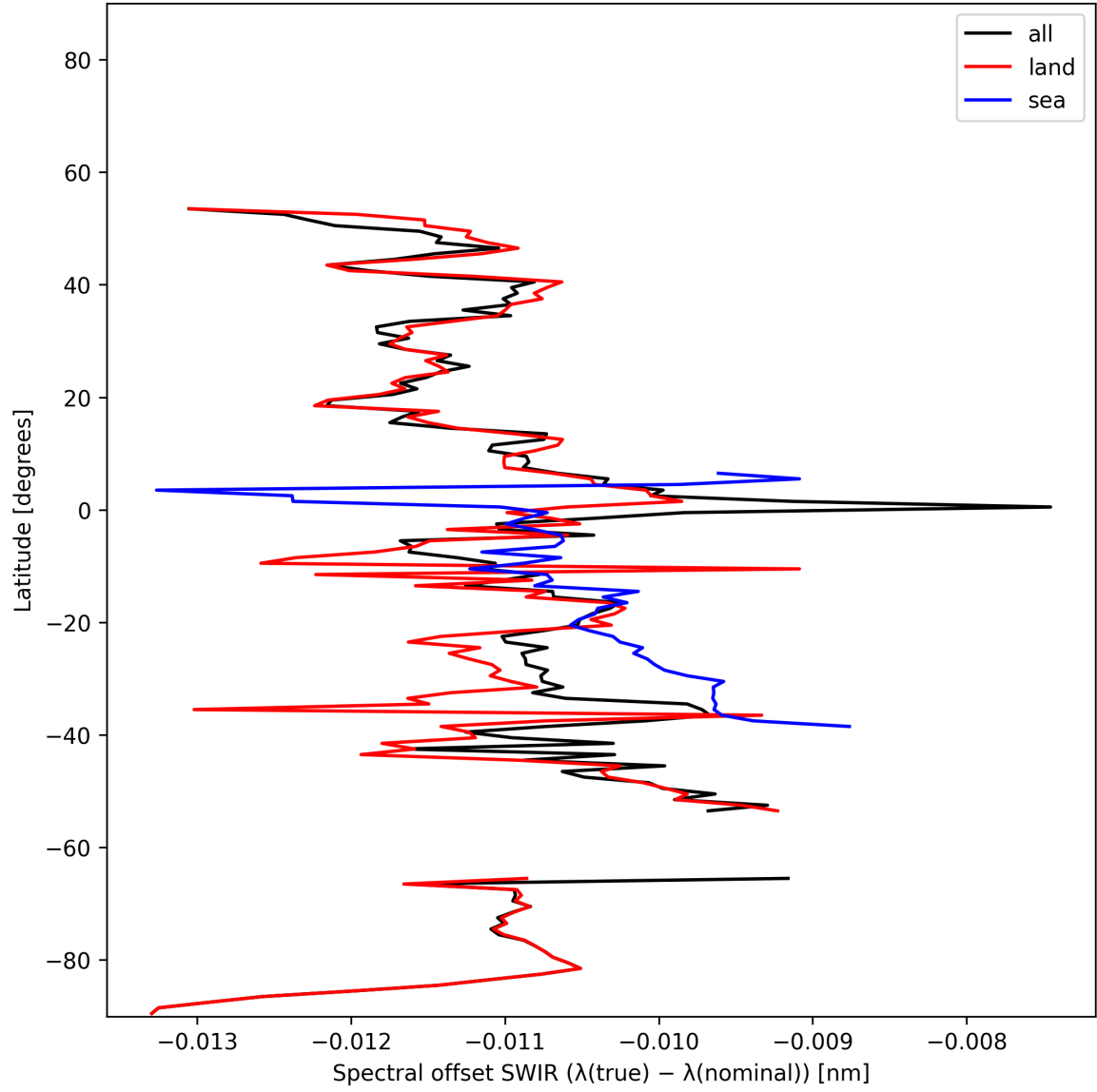
Figure 15: Zonal average of “Spectral offset SWIR ( \lambda_{\text{true}} - \lambda_{\text{nominal}} )” for 2025-11-29 to 2025-11-30.
