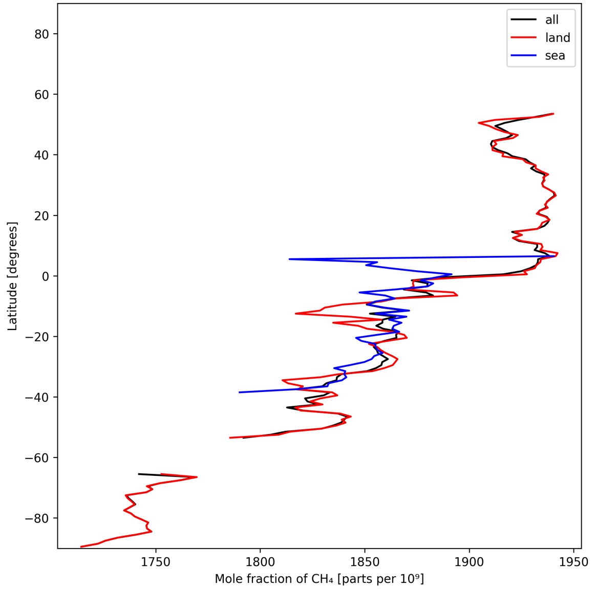
Figure 11: Zonal average of “Mole fraction of CH 4 ” for 2025-11-29 to 2025-11-30.
