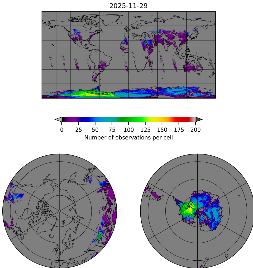
Figure 9: Map of the number of observations for 2025-11-29 to 2025-11-30
