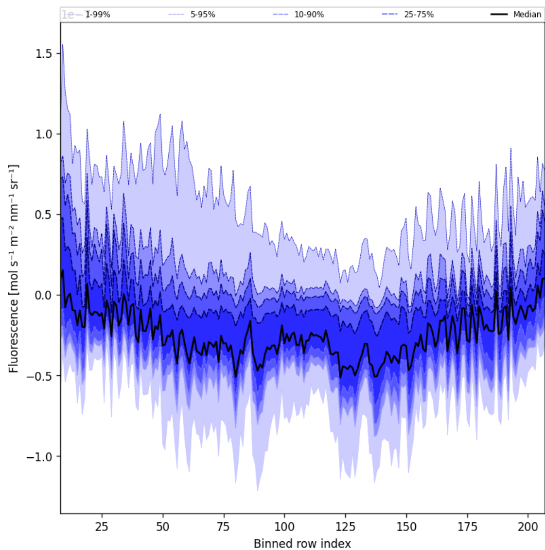
Figure 44: Along track statistics of “Fluorescence” for 2025-11-29 to 2025-11-30
