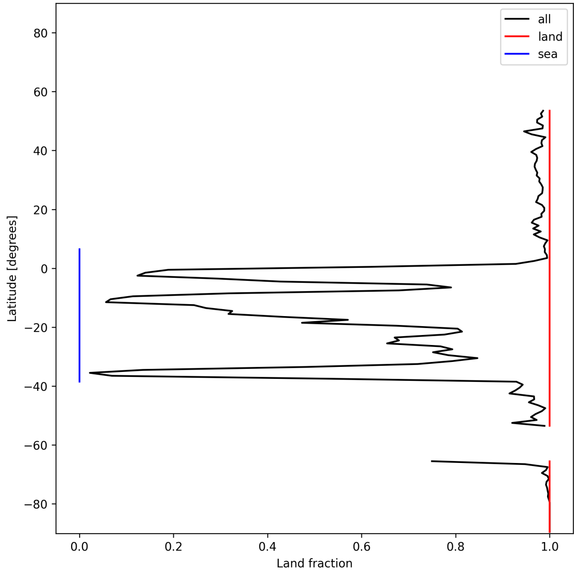
Figure 21: Zonal average of “Land fraction” for 2025-11-29 to 2025-11-30.
