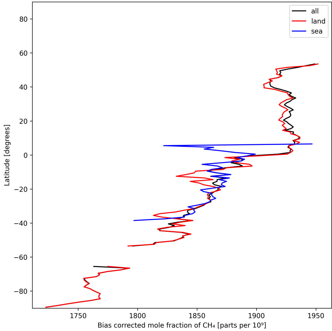
Figure 13: Zonal average of “Bias corrected mole fraction of CH 4 ” for 2025-11-29 to 2025-11-30.
