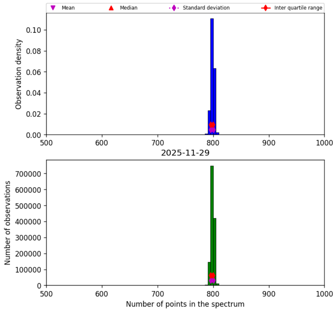
Figure 26: Histogram of “Number of points in the spectrum” for 2025-11-29 to 2025-11-30
