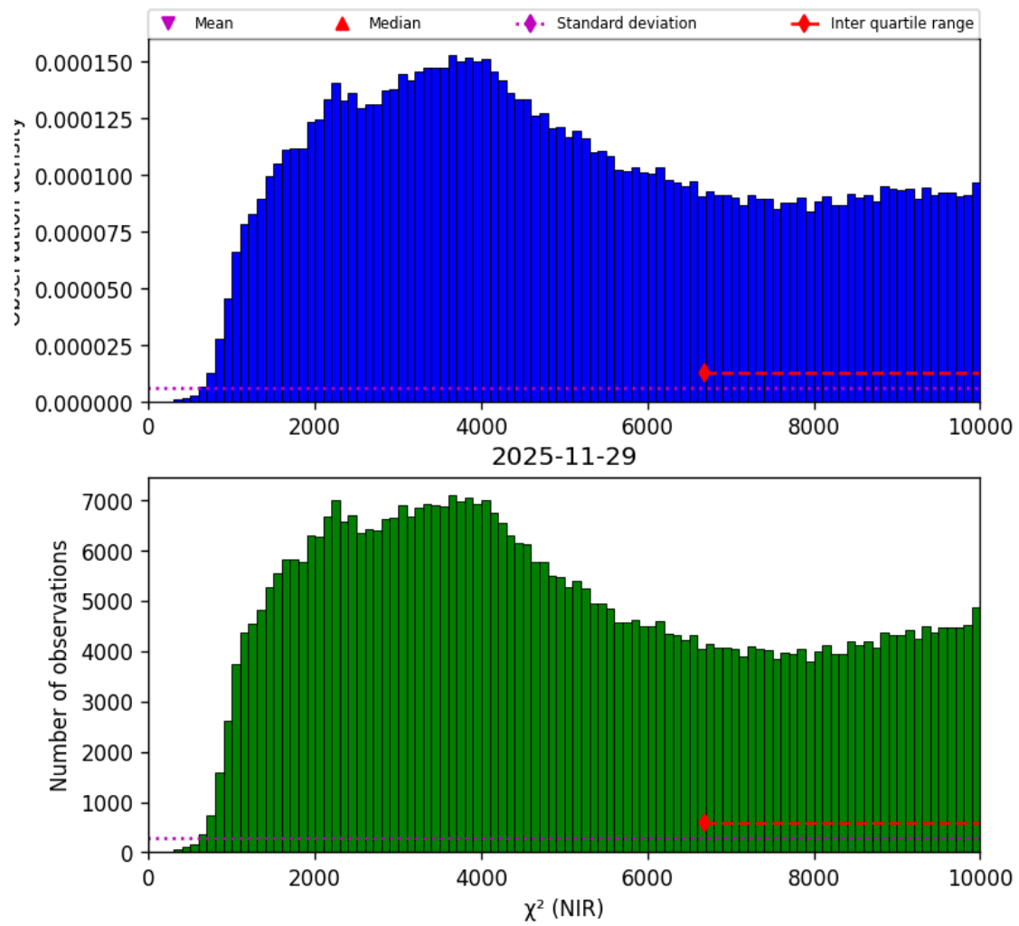
Figure 29: Histogram of “ \chi^2 (NIR)” for 2025-11-29 to 2025-11-30
