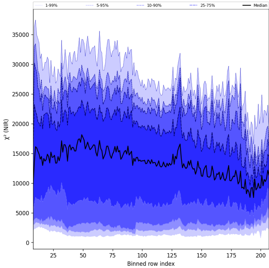
Figure 41: Along track statistics of “ \chi^2 (NIR)” for 2025-11-29 to 2025-11-30
