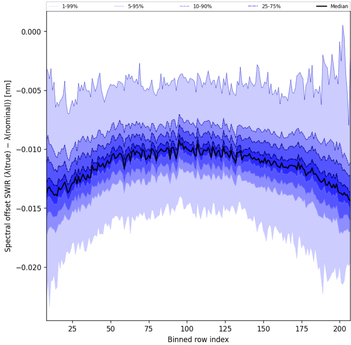
Figure 39: Along track statistics of “Spectral offset SWIR ( \lambda_{\text{true}} - \lambda_{\text{nominal}} )” for 2025-11-29 to 2025-11-30
