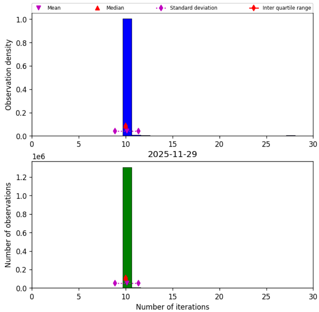
Figure 31: Histogram of "Number of iterations" for 2025-11-29 to 2025-11-30
