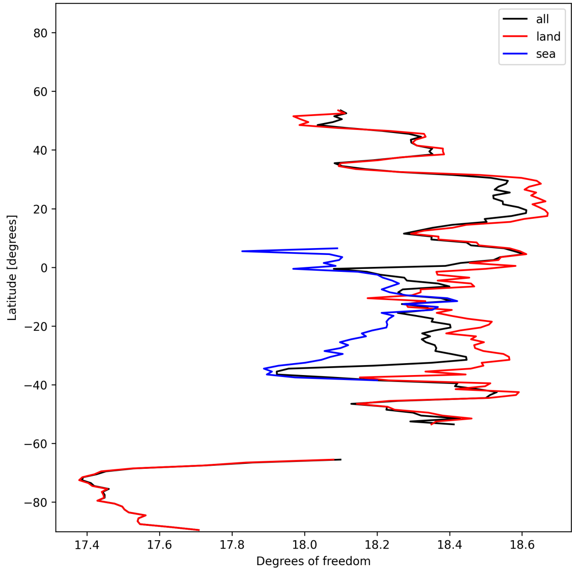
Figure 18: Zonal average of “Degrees of freedom” for 2025-11-29 to 2025-11-30.
