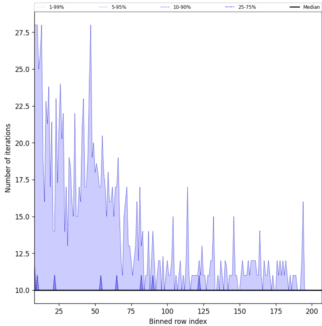
Figure 43: Along track statistics of “Number of iterations” for 2025-11-29 to 2025-11-30
