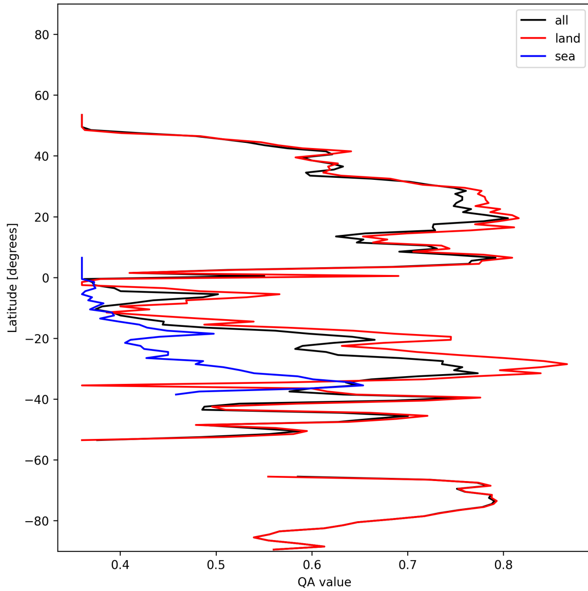
Figure 10: Zonal average of “QA value” for 2025-11-29 to 2025-11-30.
