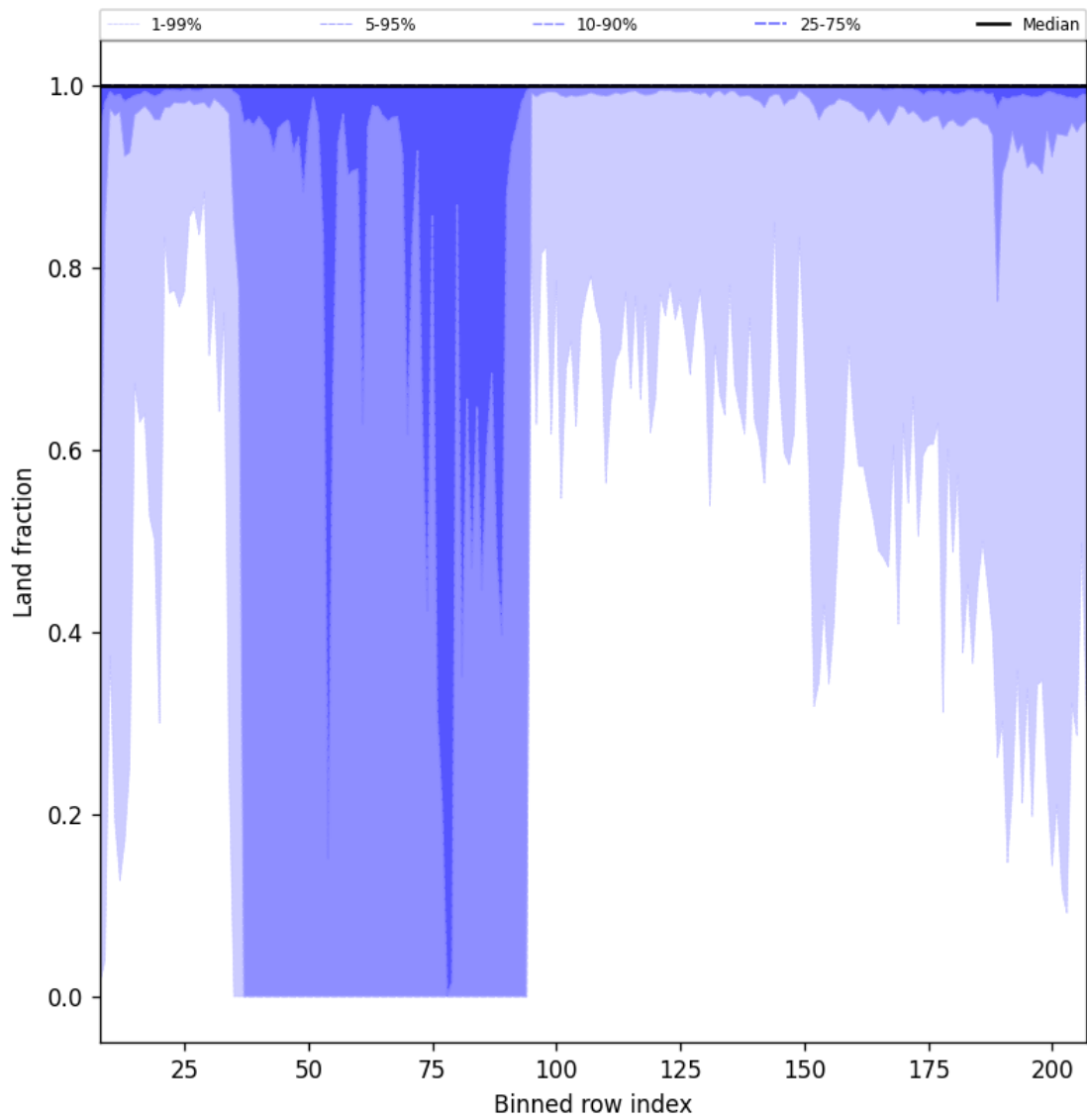
Figure 45: Along track statistics of "Land fraction" for 2025-11-29 to 2025-11-30
