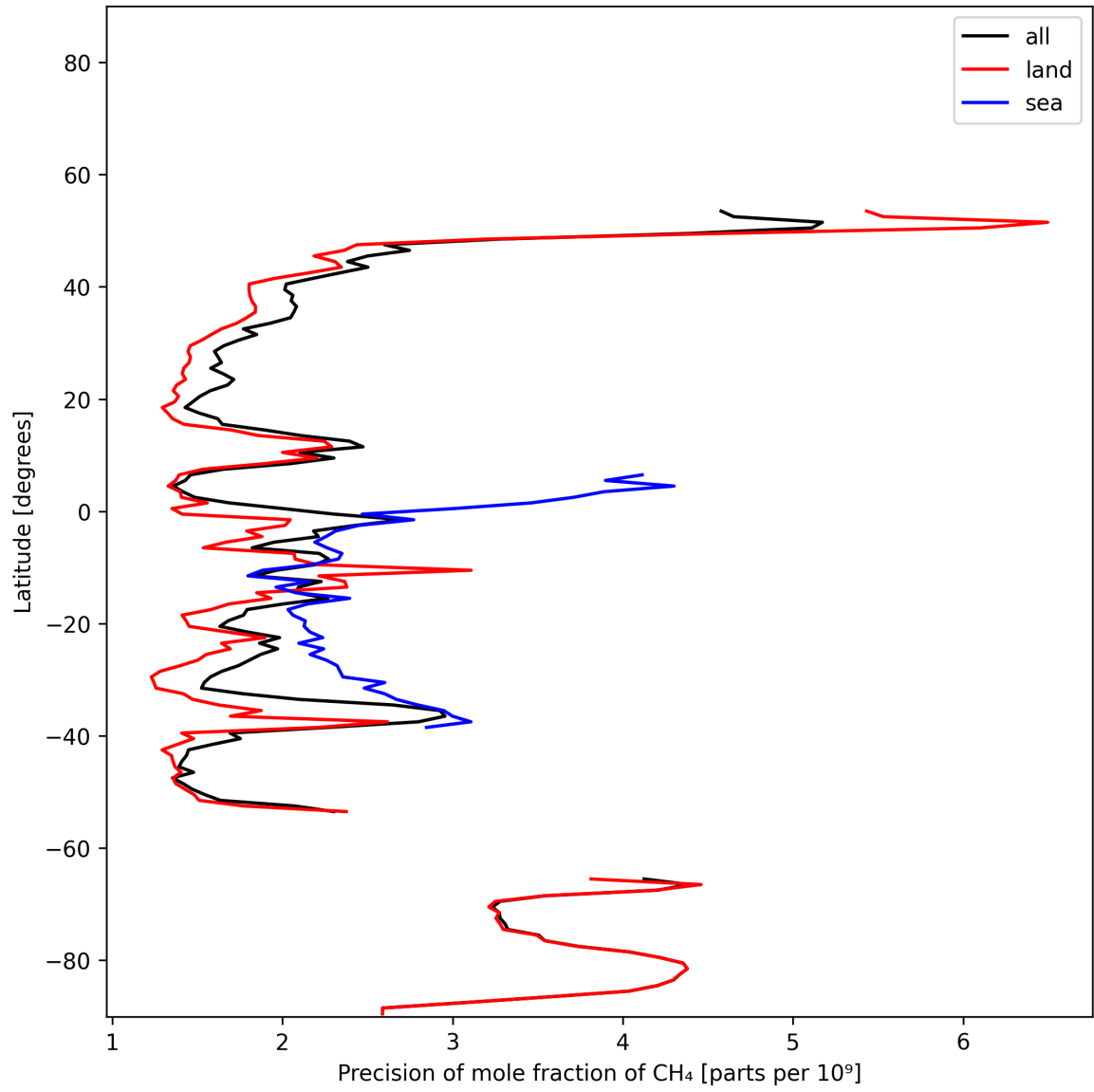
Figure 12: Zonal average of “Precision of mole fraction of CH 4 ” for 2025-11-29 to 2025-11-30.
