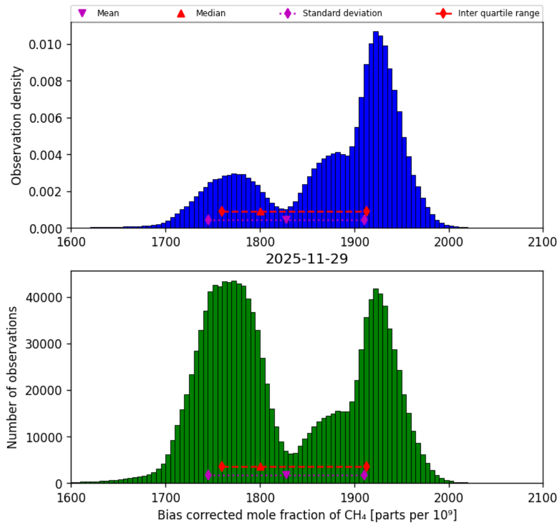
Figure 25: Histogram of “Bias corrected mole fraction of CH 4 ” for 2025-11-29 to 2025-11-30
