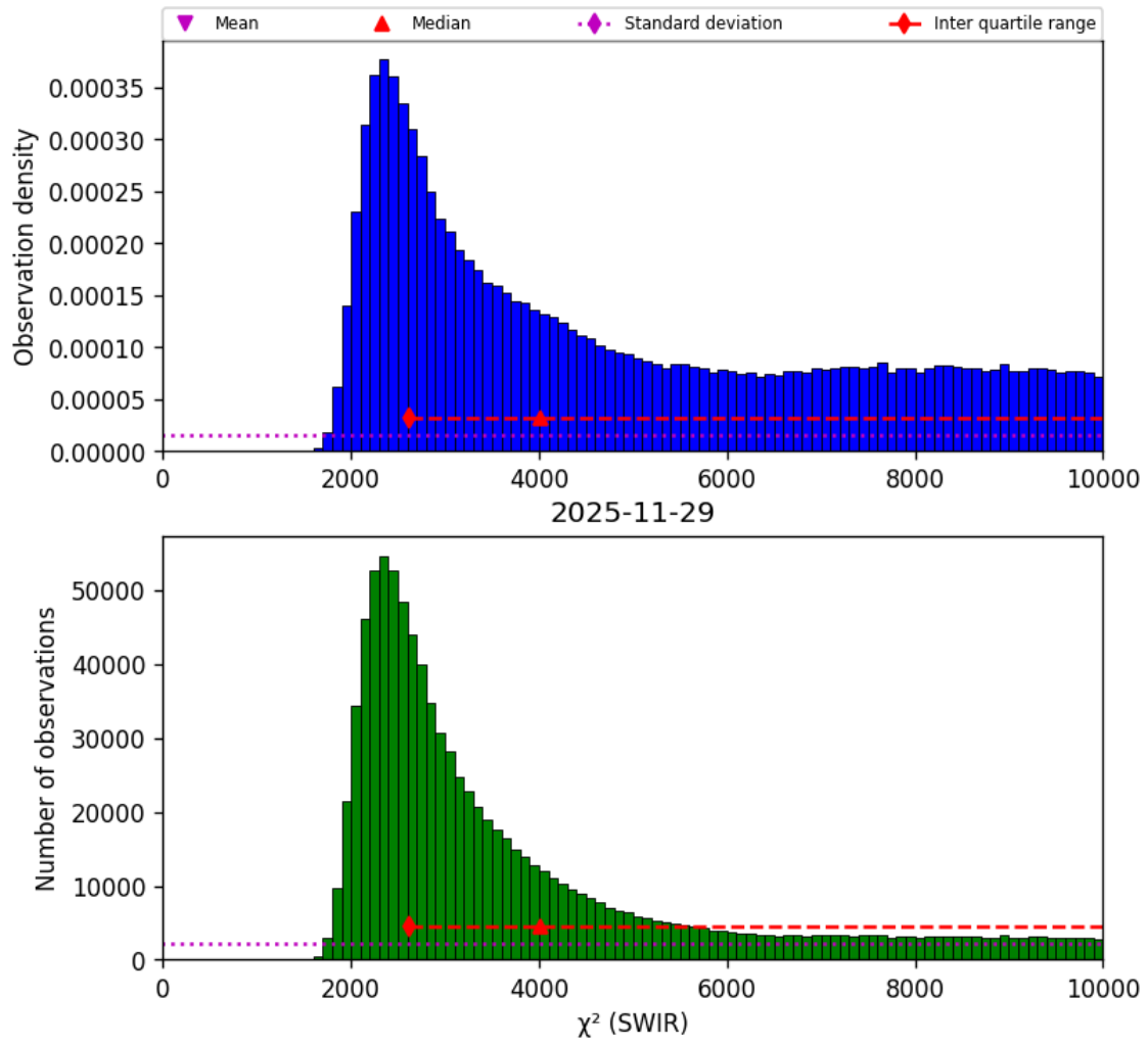
Figure 28: Histogram of “ \chi^2 (SWIR)” for 2025-11-29 to 2025-11-30
