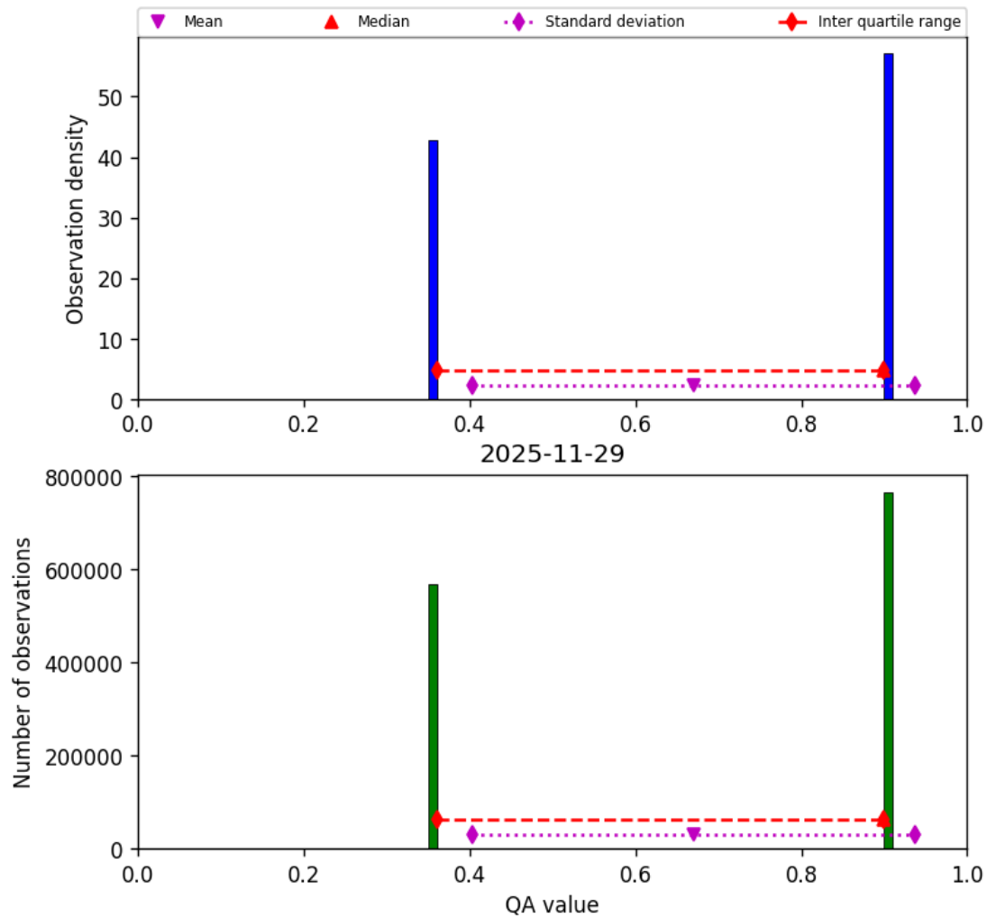
Figure 22: Histogram of “QA value” for 2025-11-29 to 2025-11-30
