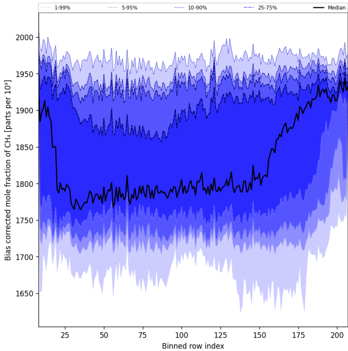
Figure 37: Along track statistics of “Bias corrected mole fraction of \text{CH}_4 ” for 2025-11-29 to 2025-11-30
