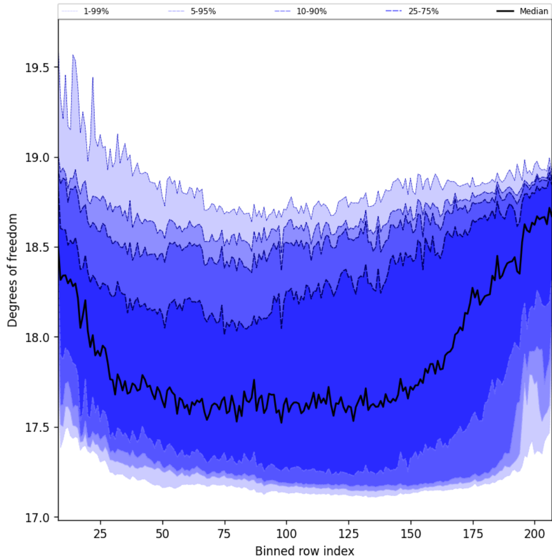
Figure 42: Along track statistics of “Degrees of freedom” for 2025-11-29 to 2025-11-30
