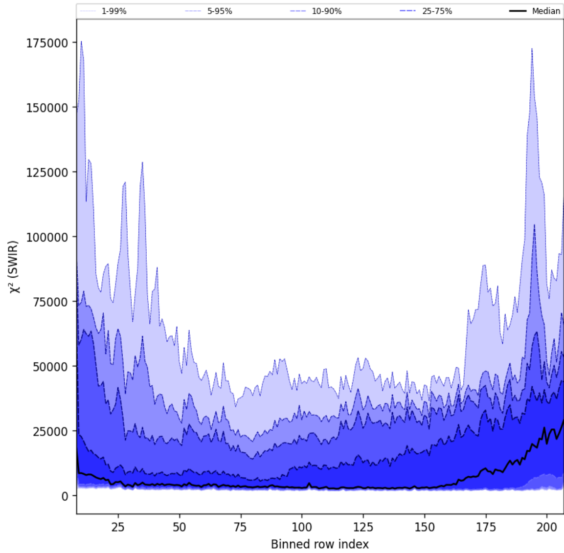
Figure 40: Along track statistics of “ \chi^2 (SWIR)” for 2025-11-29 to 2025-11-30
