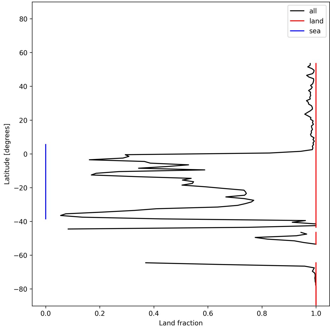
Figure 21: Zonal average of “Land fraction” for 2025-11-30 to 2025-12-01.
