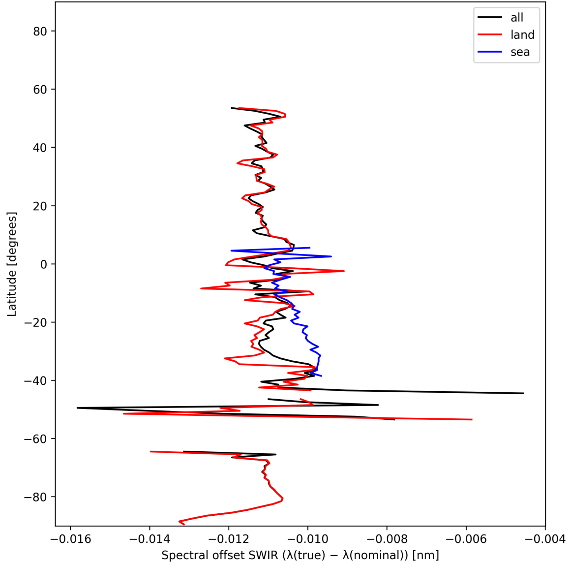
Figure 15: Zonal average of “Spectral offset SWIR ( \lambda_{\text{true}} - \lambda_{\text{nominal}} )” for 2025-11-30 to 2025-12-01.
