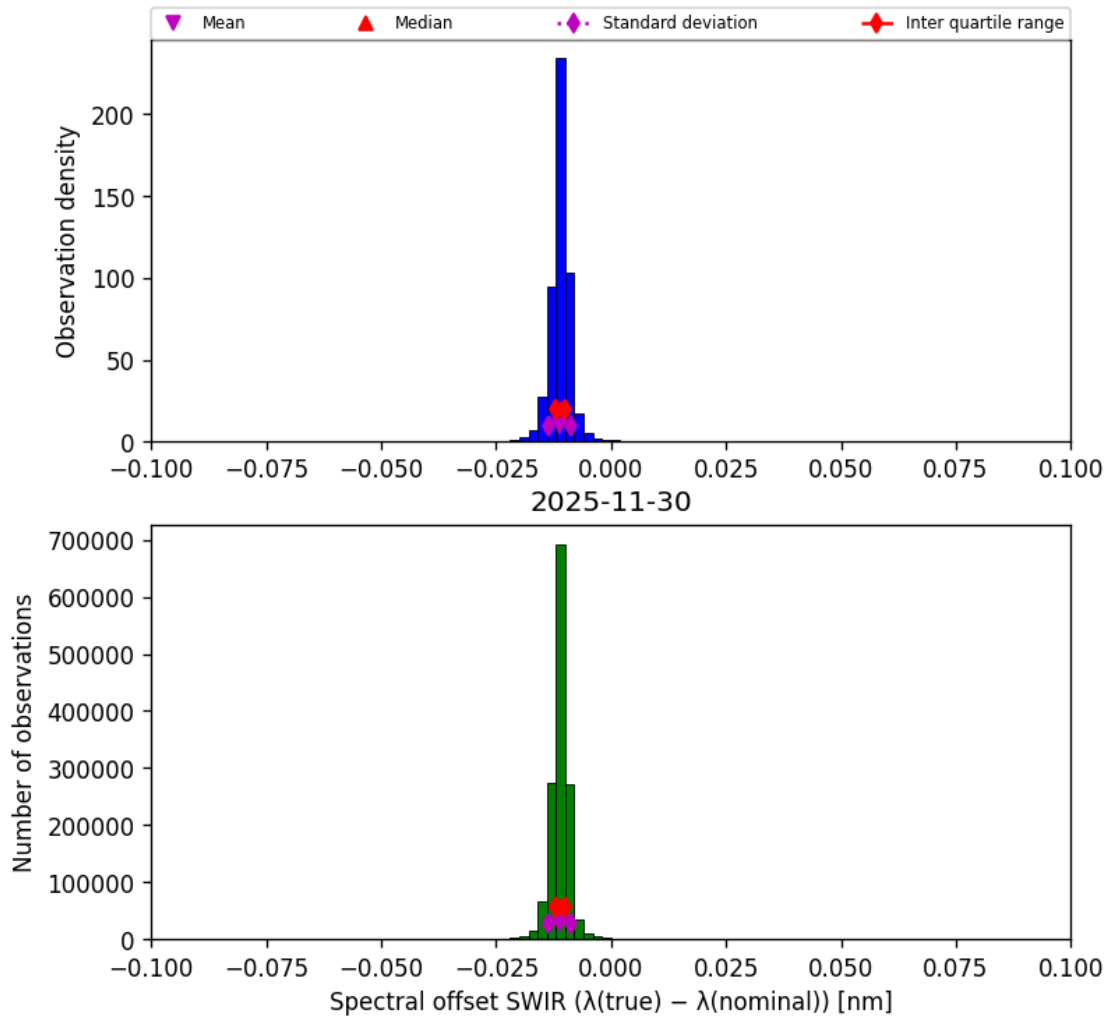
Figure 27: Histogram of “Spectral offset SWIR ( \lambda_{\text{true}} - \lambda_{\text{nominal}} )” for 2025-11-30 to 2025-12-01
