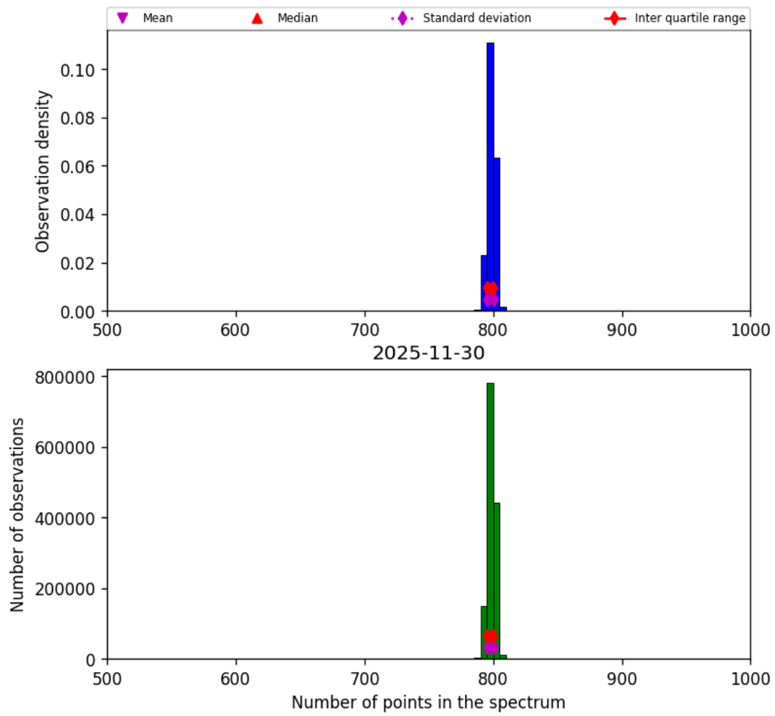
Figure 26: Histogram of “Number of points in the spectrum” for 2025-11-30 to 2025-12-01
