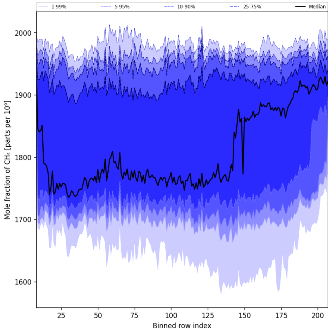
Figure 35: Along track statistics of “Mole fraction of CH 4 ” for 2025-11-30 to 2025-12-01
