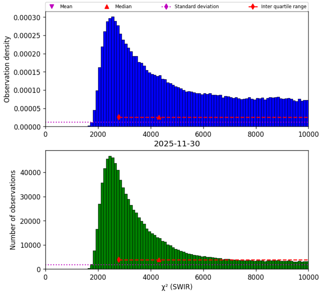
Figure 28: Histogram of " \chi^2 (SWIR)" for 2025-11-30 to 2025-12-01
