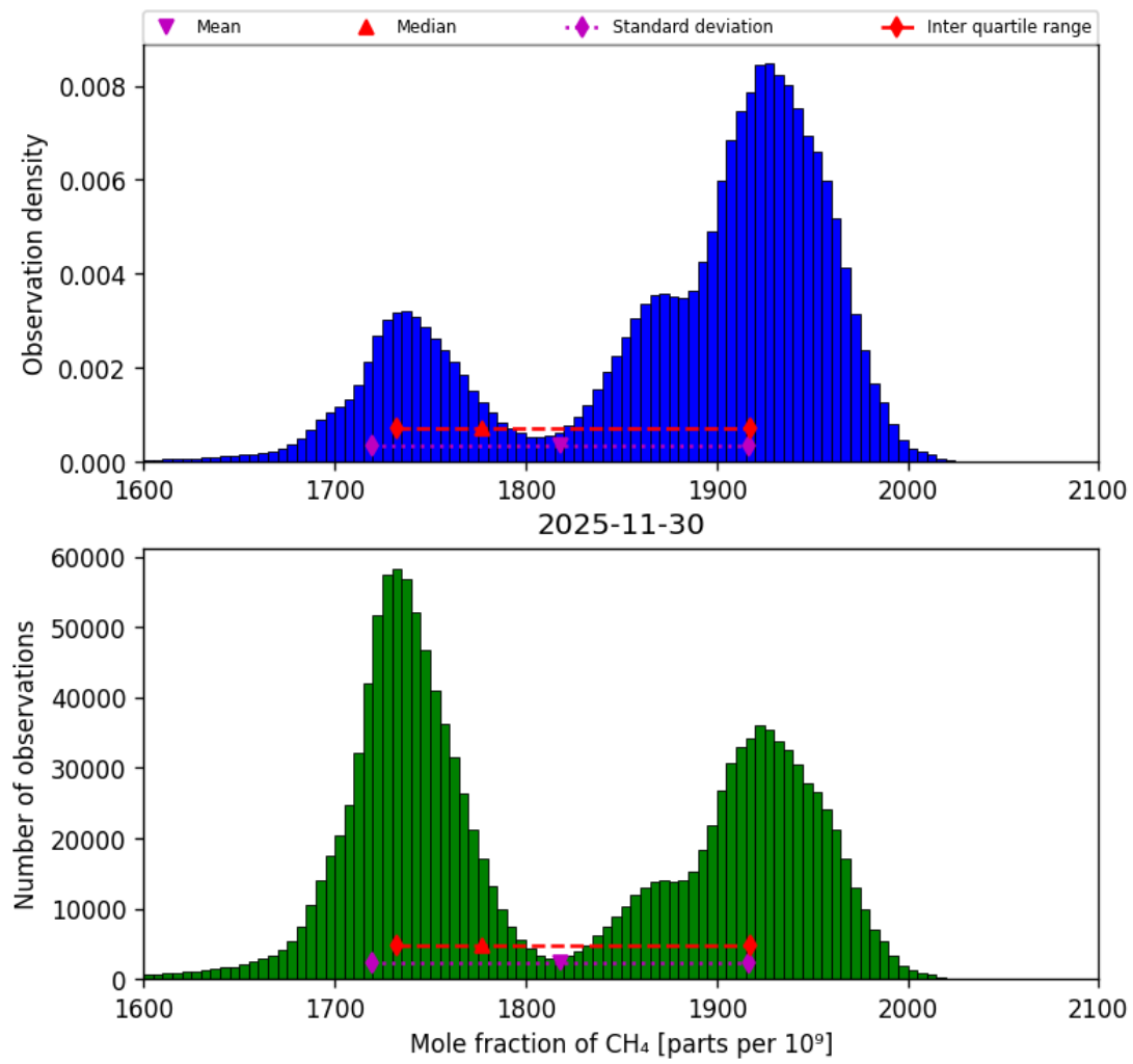
Figure 23: Histogram of “Mole fraction of CH 4 ” for 2025-11-30 to 2025-12-01
