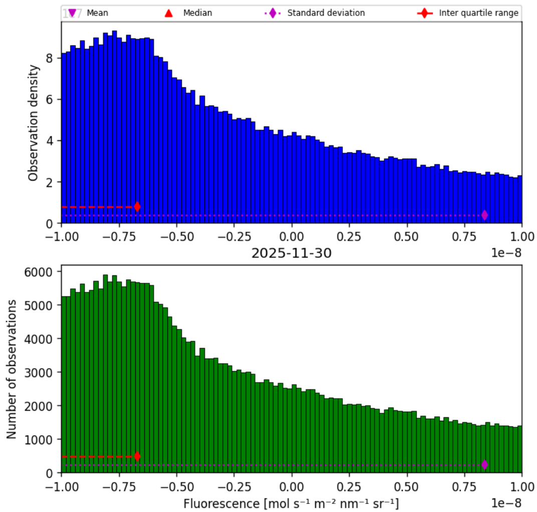
Figure 32: Histogram of “Fluorescence” for 2025-11-30 to 2025-12-01
