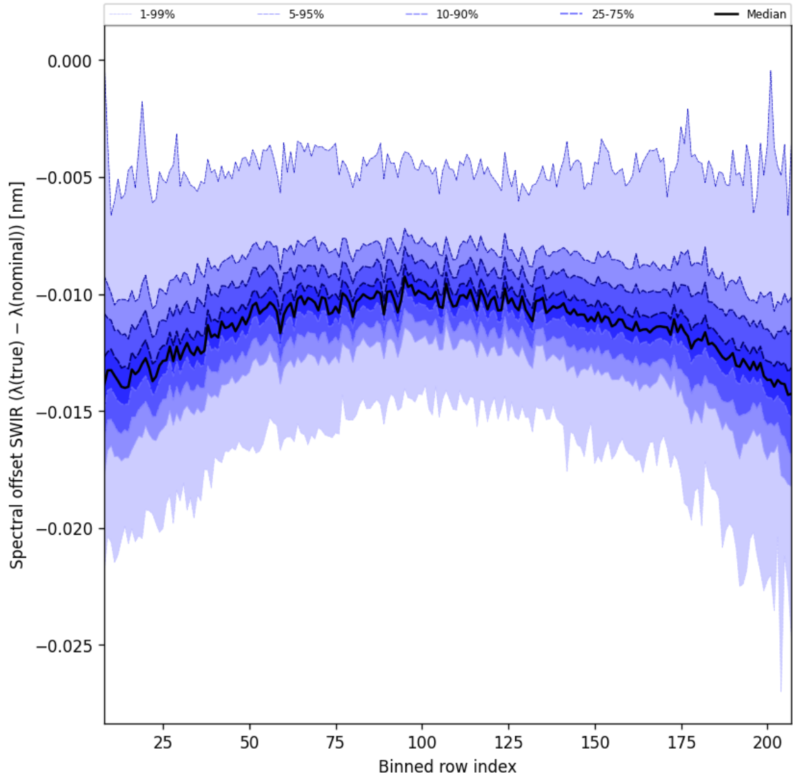
Figure 39: Along track statistics of “Spectral offset SWIR ( \lambda_{\text{true}} - \lambda_{\text{nominal}} )” for 2025-11-30 to 2025-12-01
