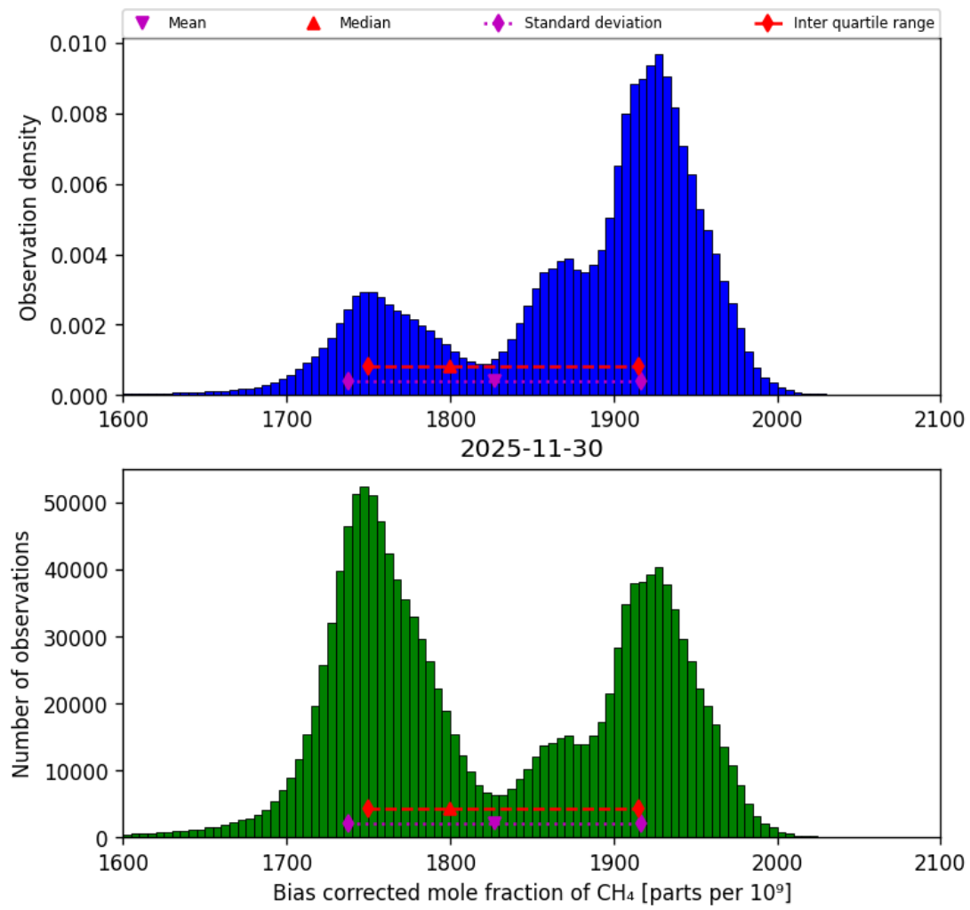
Figure 25: Histogram of “Bias corrected mole fraction of CH 4 ” for 2025-11-30 to 2025-12-01
