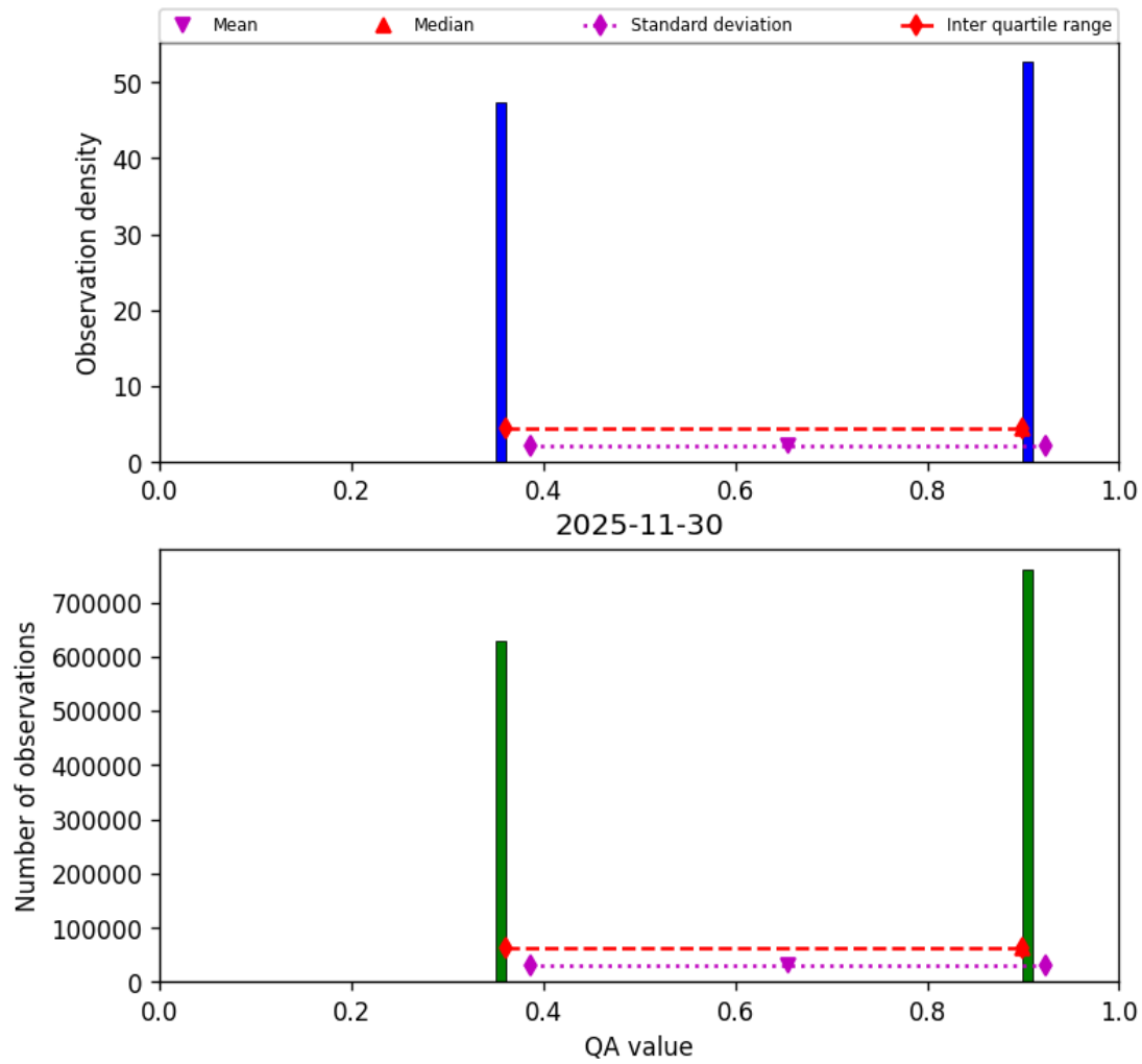
Figure 22: Histogram of “QA value” for 2025-11-30 to 2025-12-01
