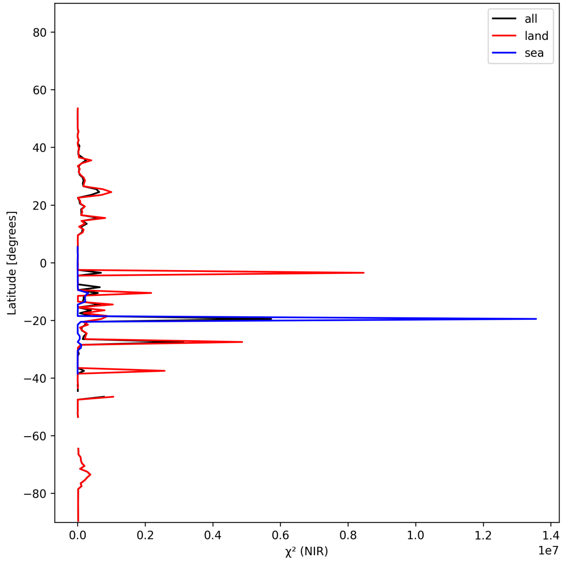
Figure 17: Zonal average of “ \chi^2 (NIR)” for 2025-11-30 to 2025-12-01.
