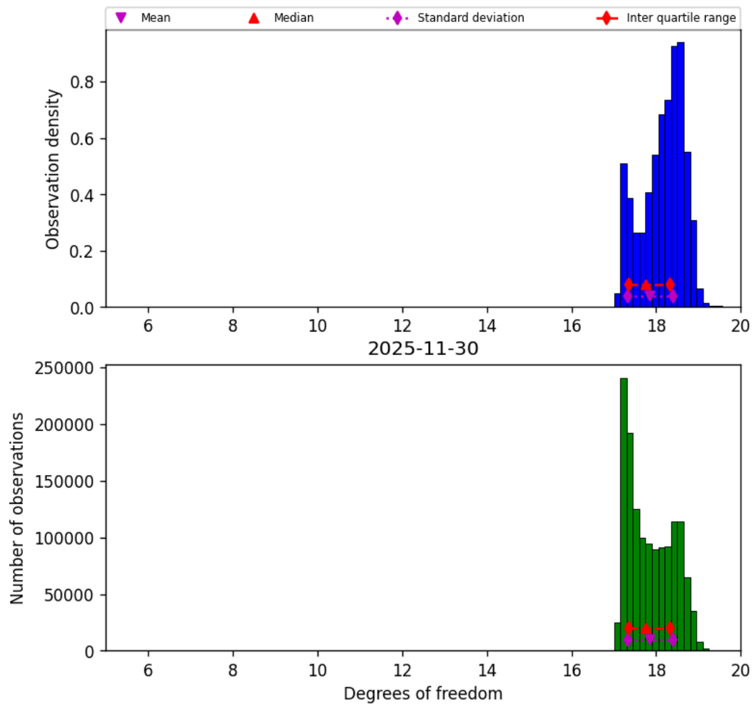
Figure 30: Histogram of “Degrees of freedom” for 2025-11-30 to 2025-12-01
