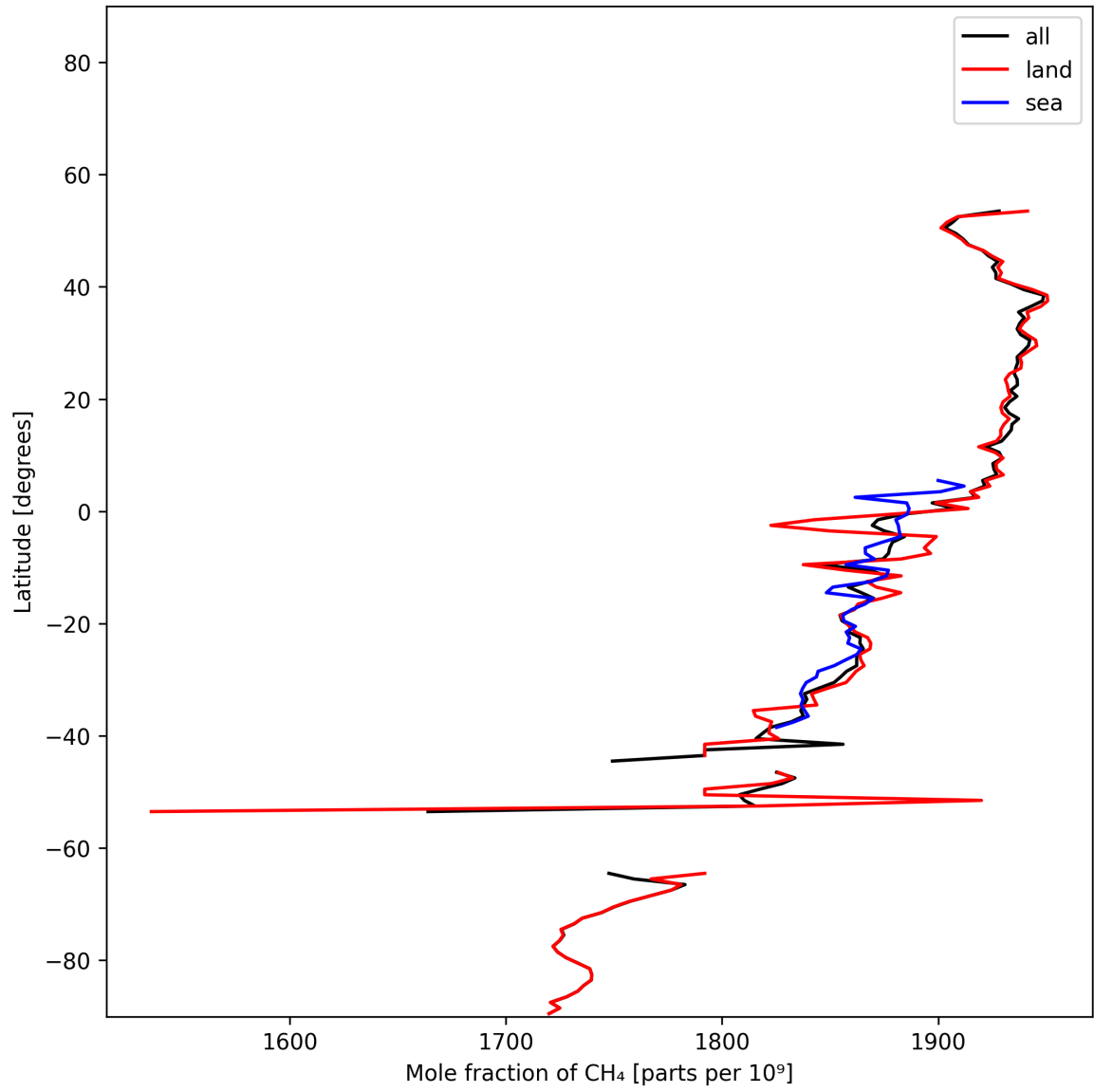
Figure 11: Zonal average of “Mole fraction of CH 4 ” for 2025-11-30 to 2025-12-01.
