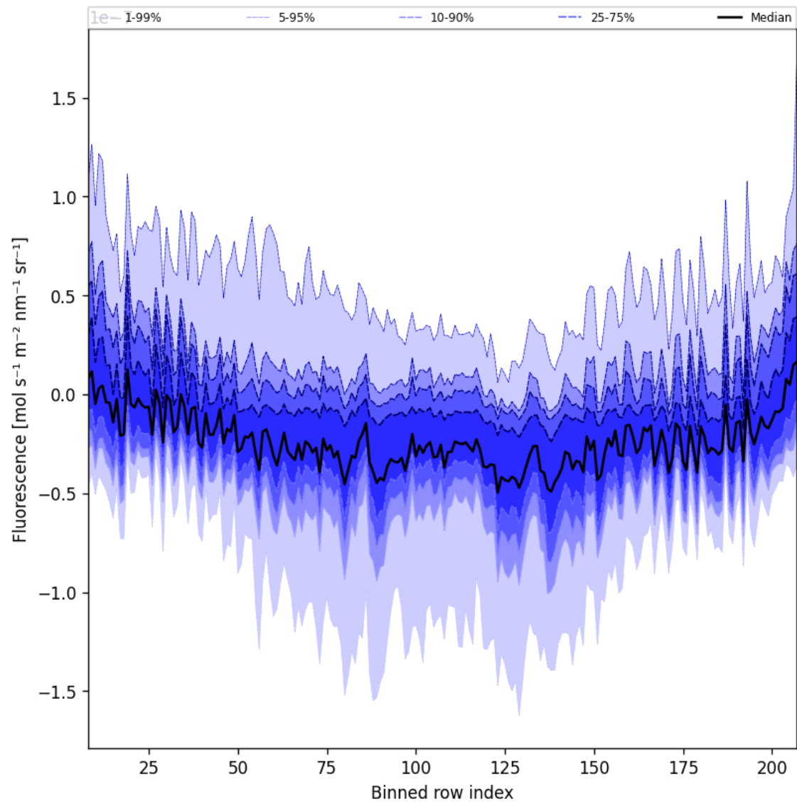
Figure 44: Along track statistics of “Fluorescence” for 2025-11-30 to 2025-12-01
