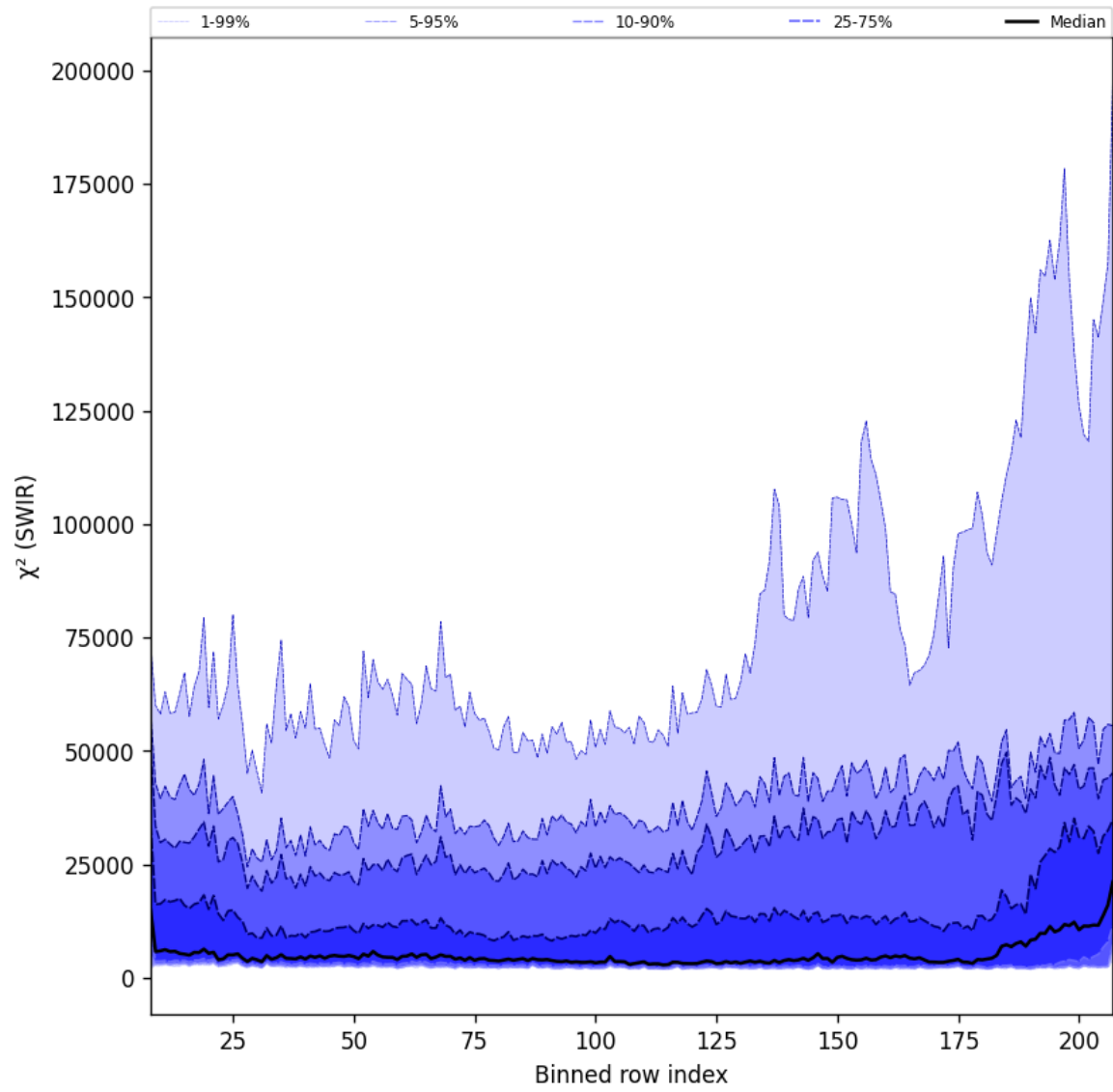
Figure 40: Along track statistics of “ \chi^2 (SWIR)” for 2025-11-30 to 2025-12-01
