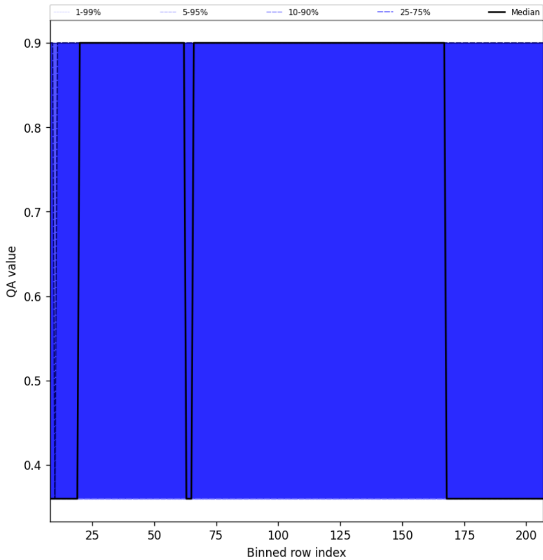
Figure 34: Along track statistics of “QA value” for 2025-11-30 to 2025-12-01
