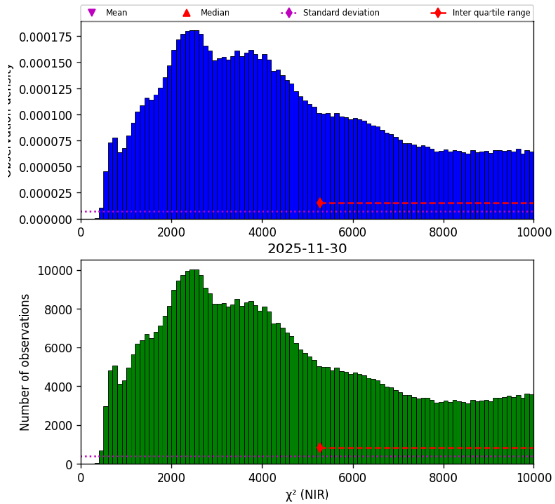
Figure 29: Histogram of “ \chi^2 (NIR)” for 2025-11-30 to 2025-12-01
