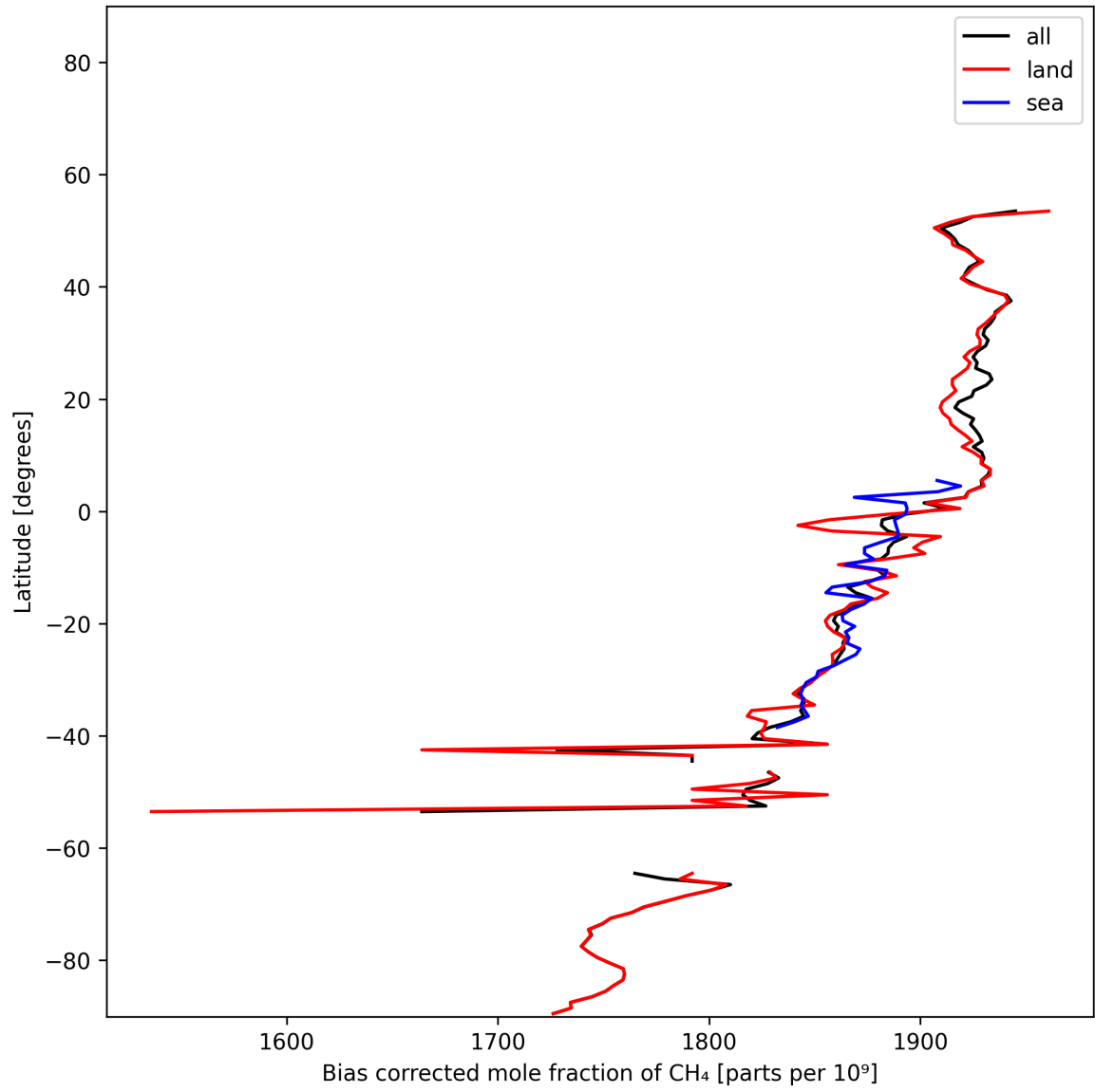
Figure 13: Zonal average of “Bias corrected mole fraction of CH 4 ” for 2025-11-30 to 2025-12-01.
