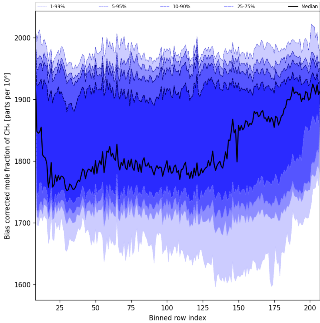
Figure 37: Along track statistics of “Bias corrected mole fraction of CH 4 ” for 2025-11-30 to 2025-12-01
