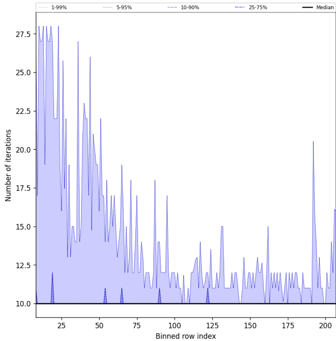
Figure 43: Along track statistics of “Number of iterations” for 2025-11-30 to 2025-12-01
