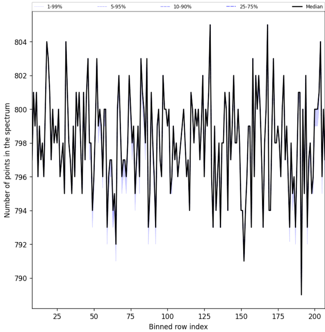
Figure 38: Along track statistics of “Number of points in the spectrum” for 2025-11-30 to 2025-12-01
