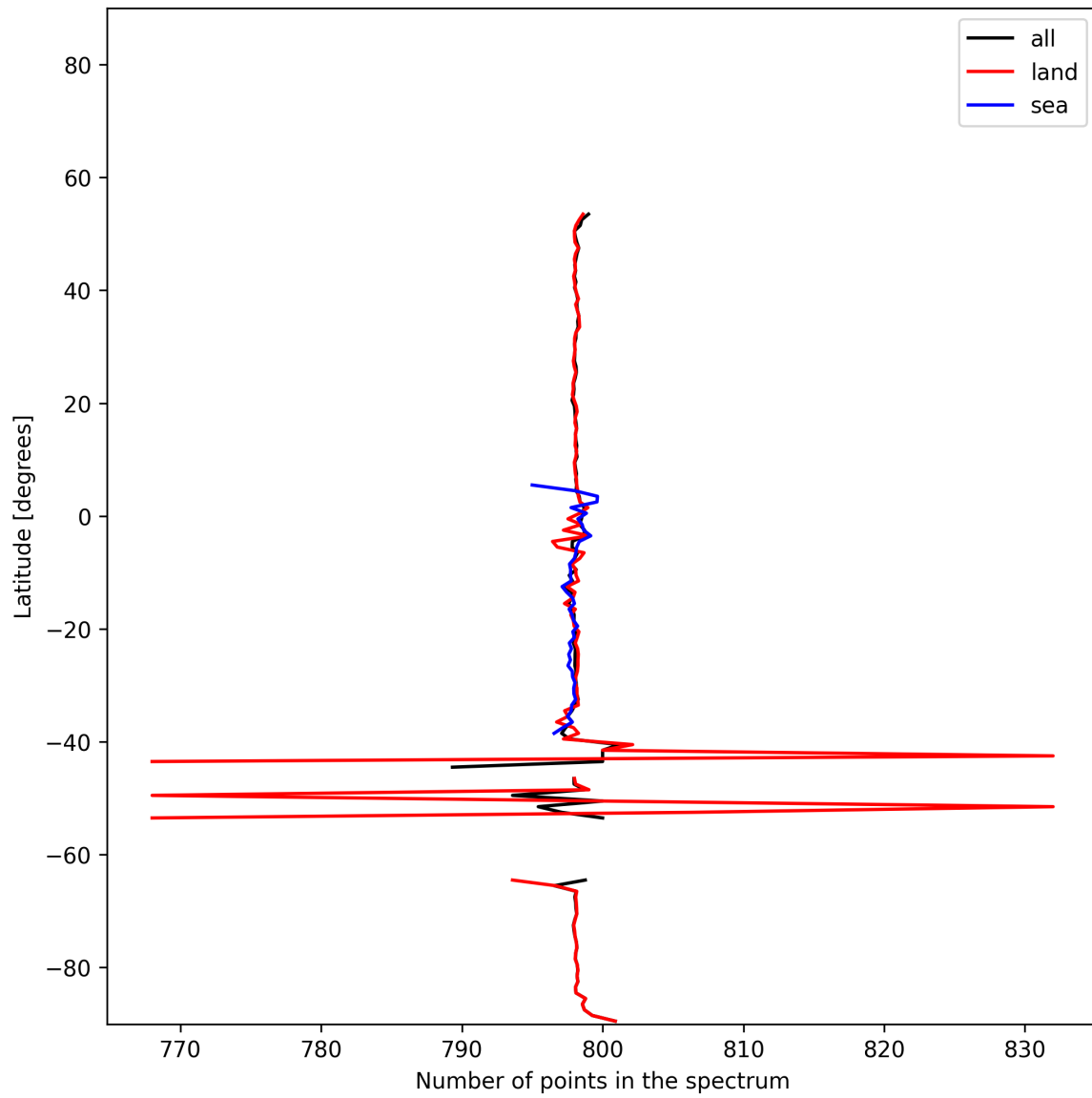
Figure 14: Zonal average of “Number of points in the spectrum” for 2025-11-30 to 2025-12-01.
