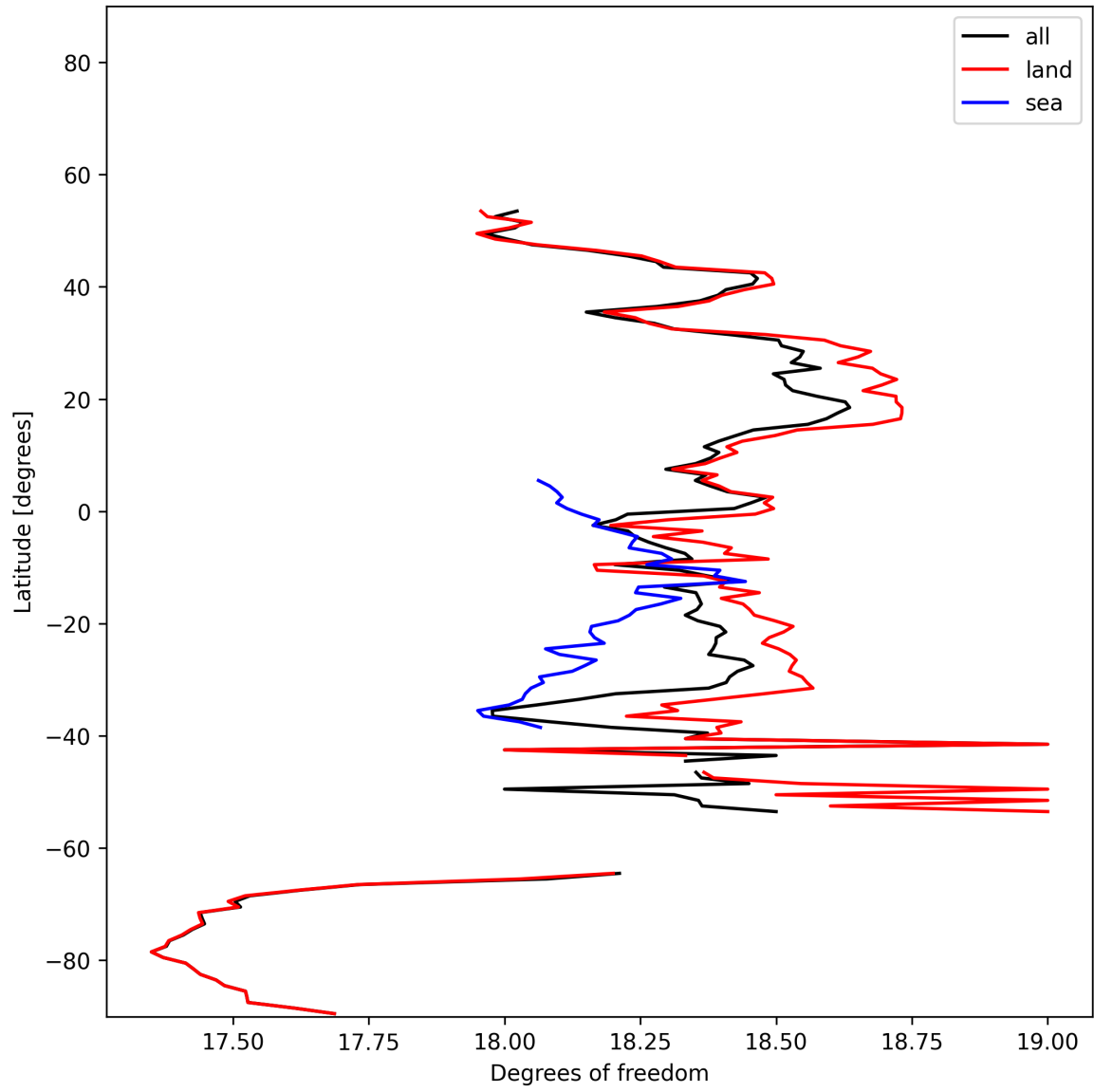
Figure 18: Zonal average of “Degrees of freedom” for 2025-11-30 to 2025-12-01.
