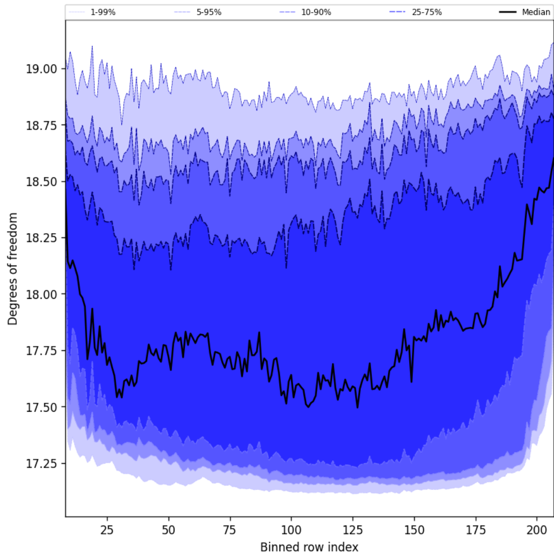
Figure 42: Along track statistics of “Degrees of freedom” for 2025-11-30 to 2025-12-01
