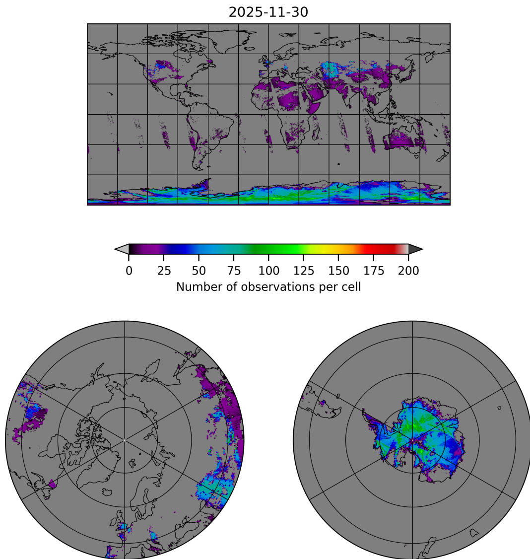
Figure 9: Map of the number of observations for 2025-11-30 to 2025-12-01
