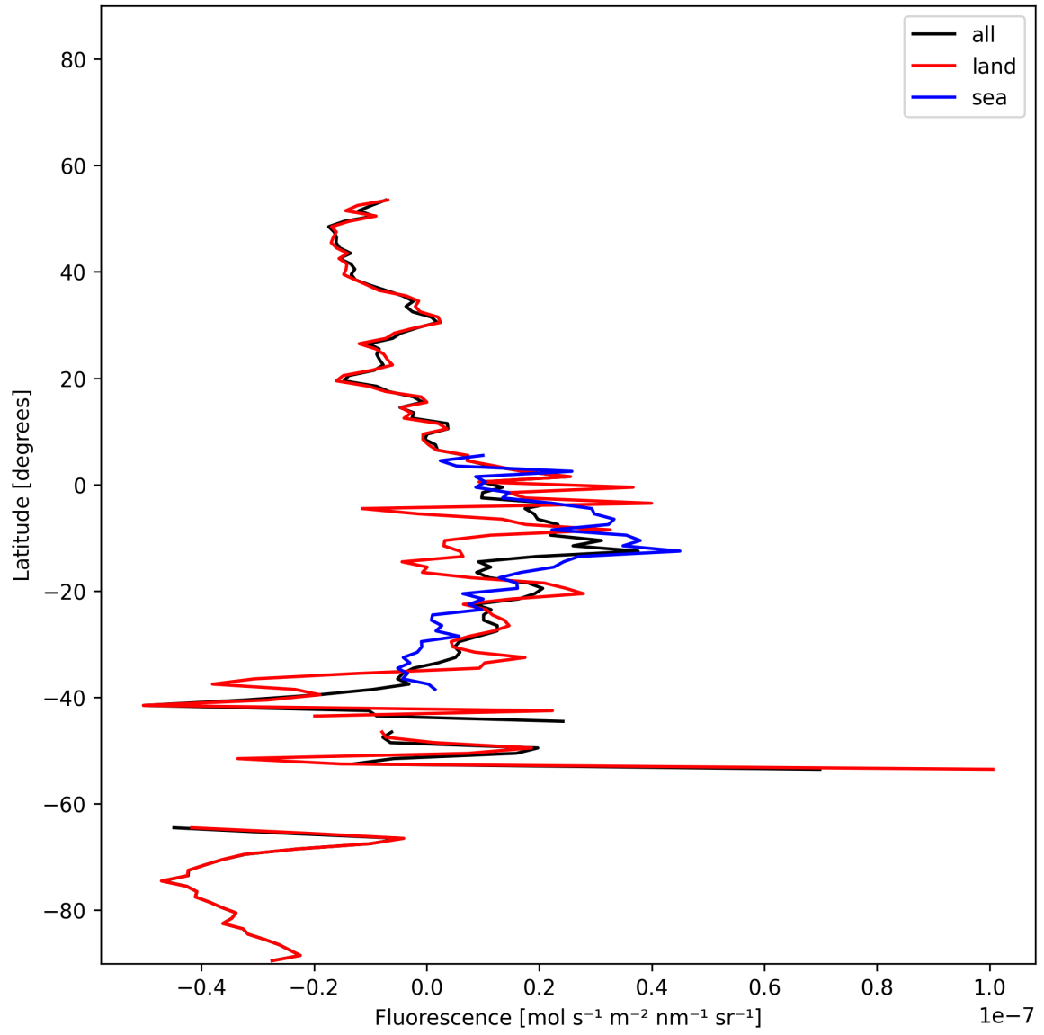
Figure 20: Zonal average of “Fluorescence” for 2025-11-30 to 2025-12-01.
