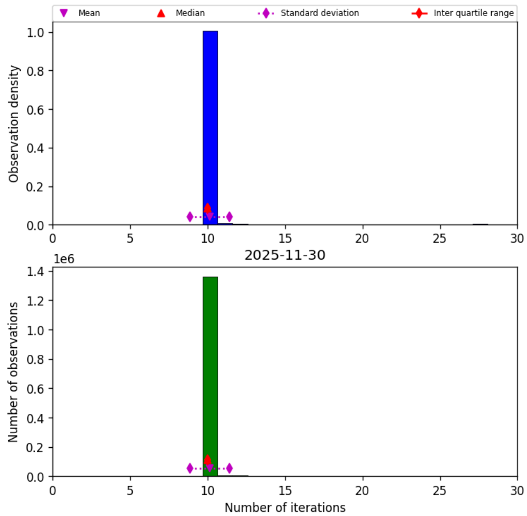
Figure 31: Histogram of “Number of iterations” for 2025-11-30 to 2025-12-01
