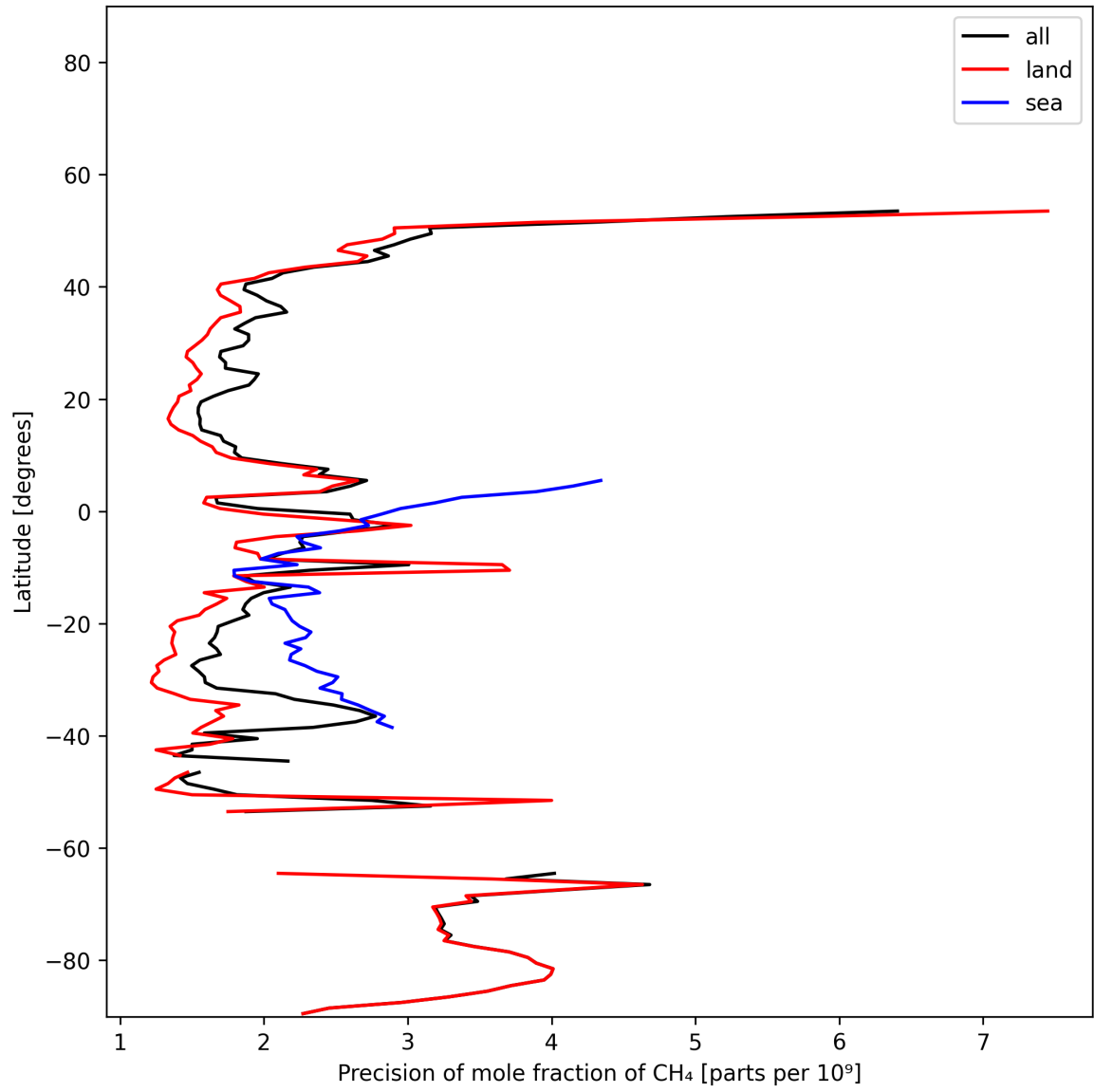
Figure 12: Zonal average of “Precision of mole fraction of CH 4 ” for 2025-11-30 to 2025-12-01.
