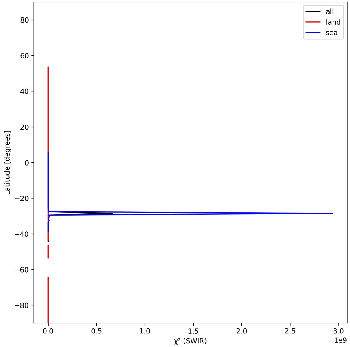
Figure 16: Zonal average of “ \chi^2 (SWIR)” for 2025-11-30 to 2025-12-01.
