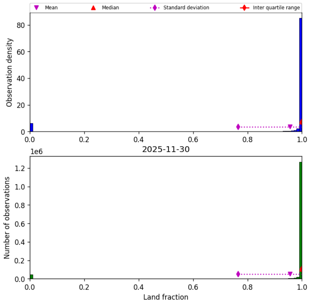
Figure 33: Histogram of “Land fraction” for 2025-11-30 to 2025-12-01
