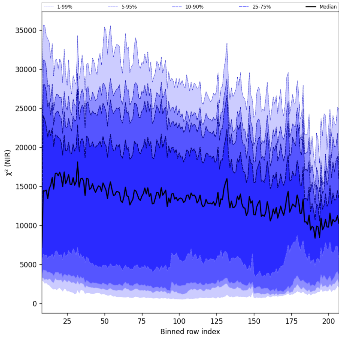
Figure 41: Along track statistics of “ \chi^2 (NIR)” for 2025-11-30 to 2025-12-01
