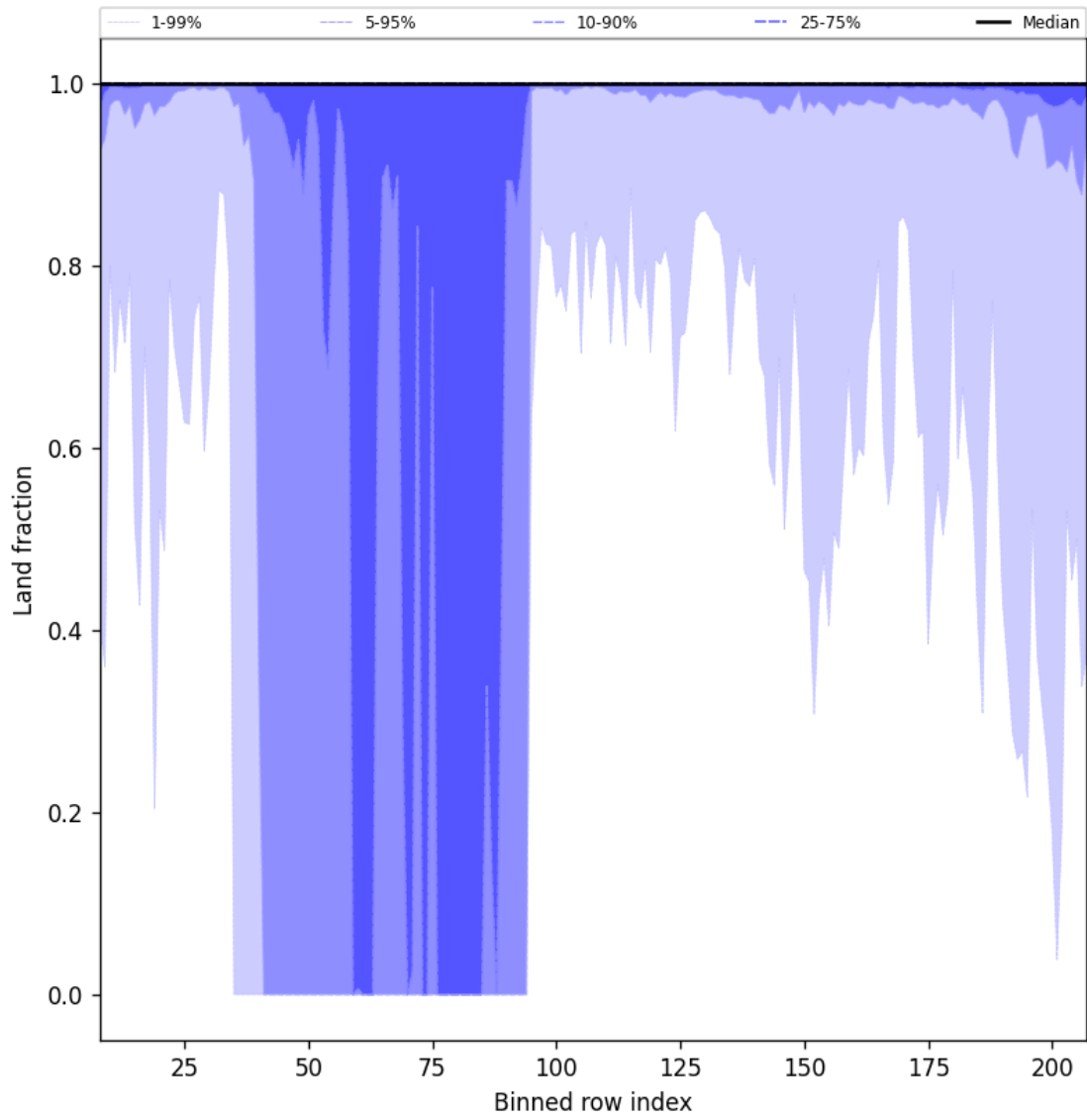
Figure 45: Along track statistics of "Land fraction" for 2025-11-30 to 2025-12-01
