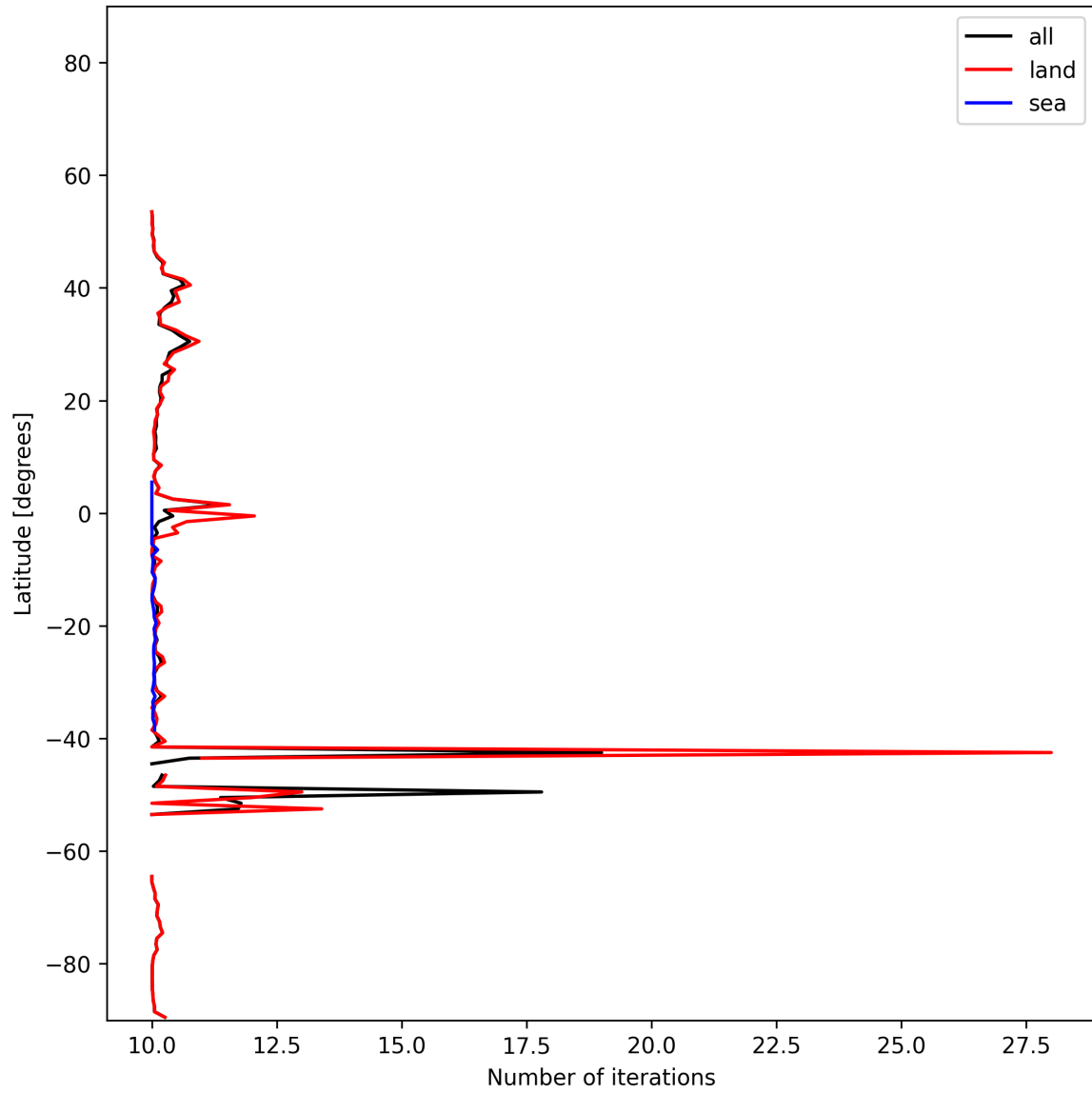
Figure 19: Zonal average of “Number of iterations” for 2025-11-30 to 2025-12-01.
