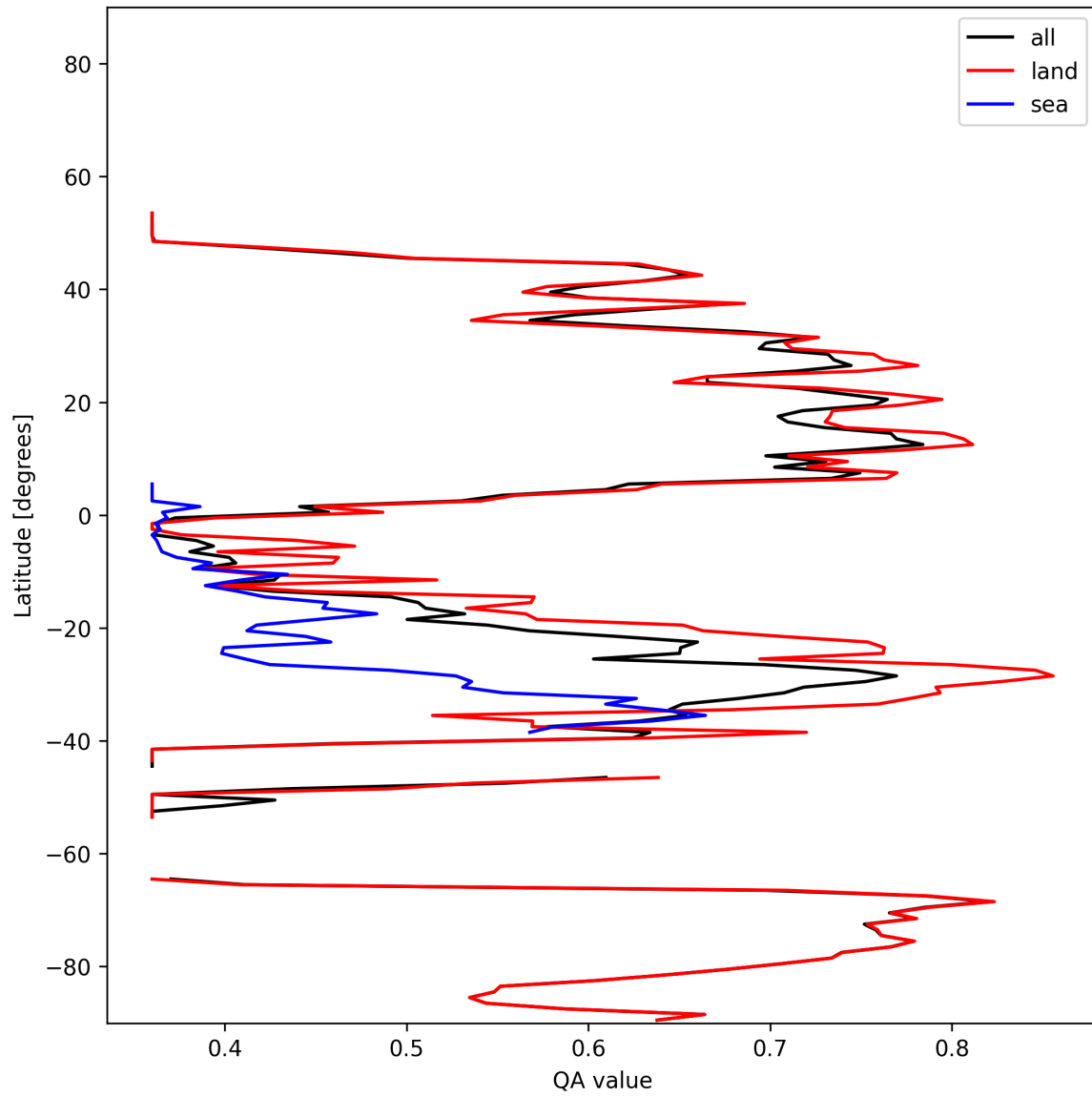
Figure 10: Zonal average of “QA value” for 2025-11-30 to 2025-12-01.
