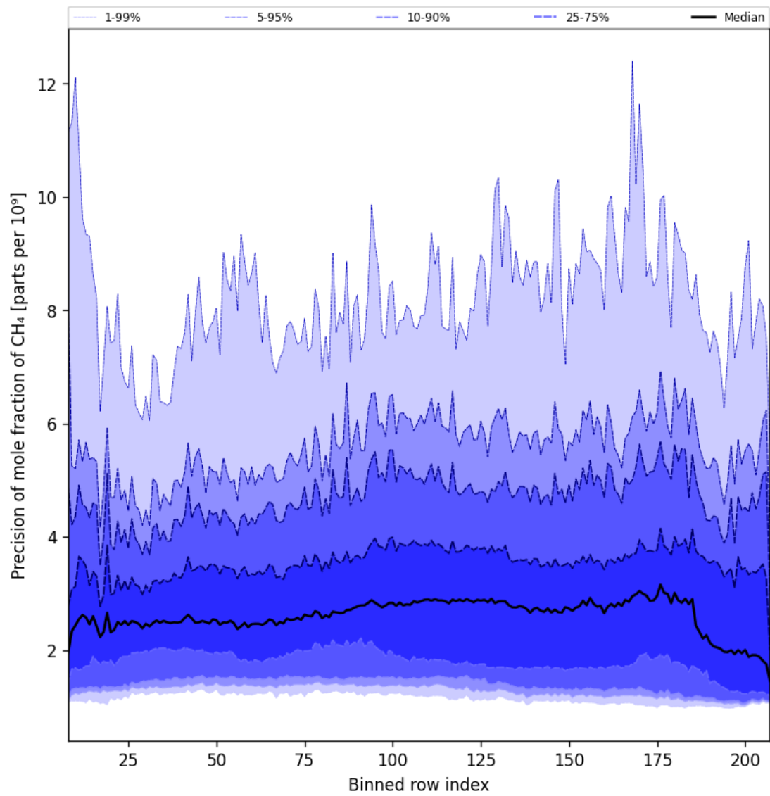
Figure 36: Along track statistics of “Precision of mole fraction of CH 4 ” for 2025-11-30 to 2025-12-01
