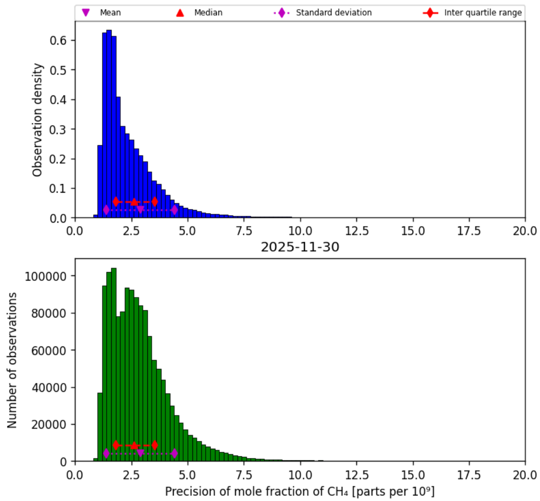
Figure 24: Histogram of “Precision of mole fraction of CH 4 ” for 2025-11-30 to 2025-12-01
