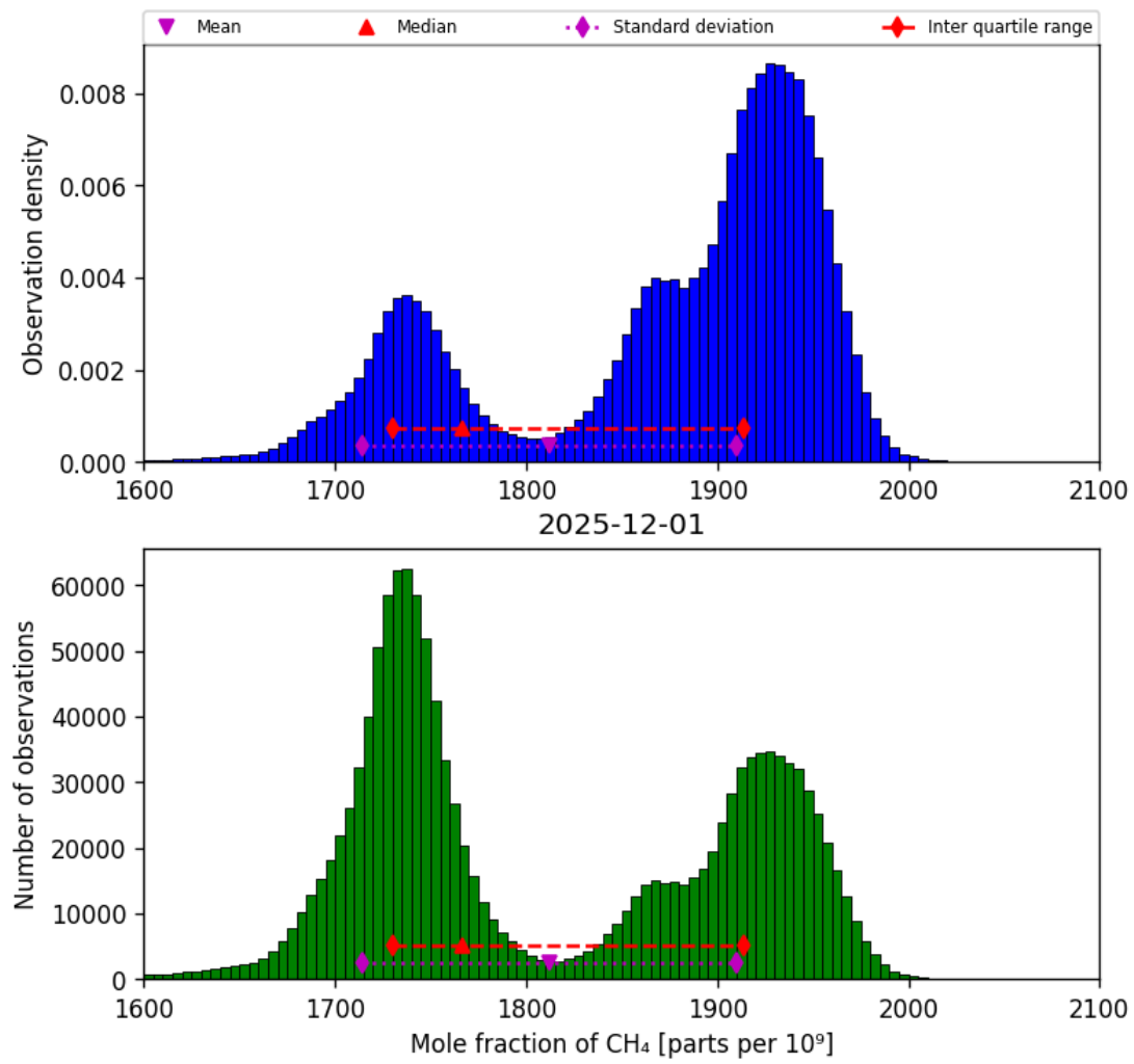
Figure 23: Histogram of “Mole fraction of CH 4 ” for 2025-12-01 to 2025-12-01
