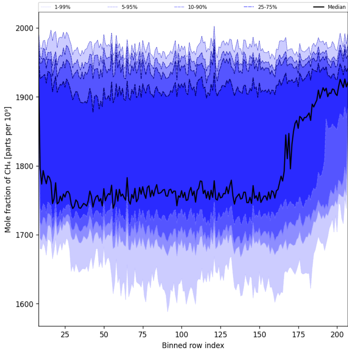
Figure 35: Along track statistics of “Mole fraction of CH 4 ” for 2025-12-01 to 2025-12-01
