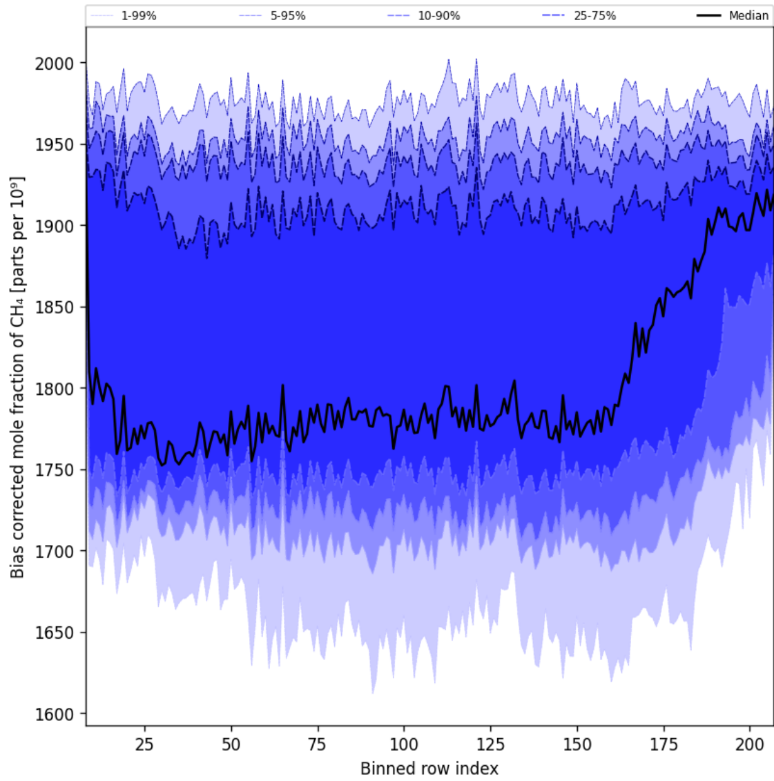
Figure 37: Along track statistics of “Bias corrected mole fraction of CH 4 ” for 2025-12-01 to 2025-12-01
