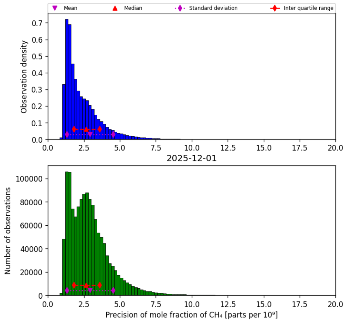
Figure 24: Histogram of “Precision of mole fraction of CH 4 ” for 2025-12-01 to 2025-12-01
