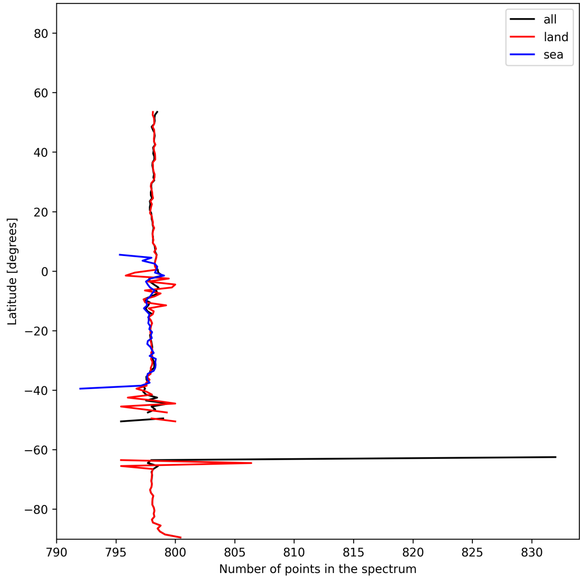
Figure 14: Zonal average of “Number of points in the spectrum” for 2025-12-01 to 2025-12-01.
