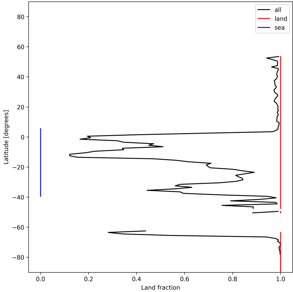
Figure 21: Zonal average of “Land fraction” for 2025-12-01 to 2025-12-01.
