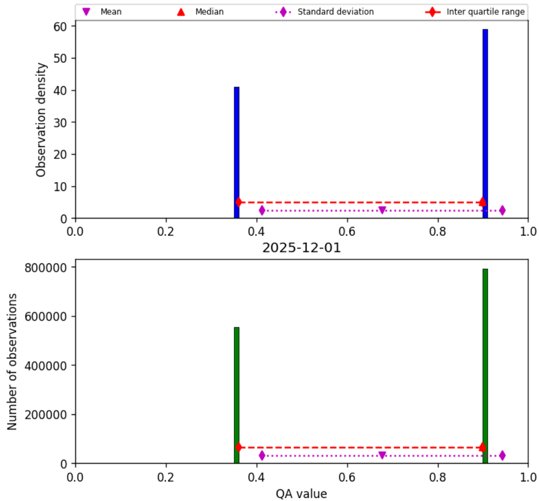
Figure 22: Histogram of “QA value” for 2025-12-01 to 2025-12-01
