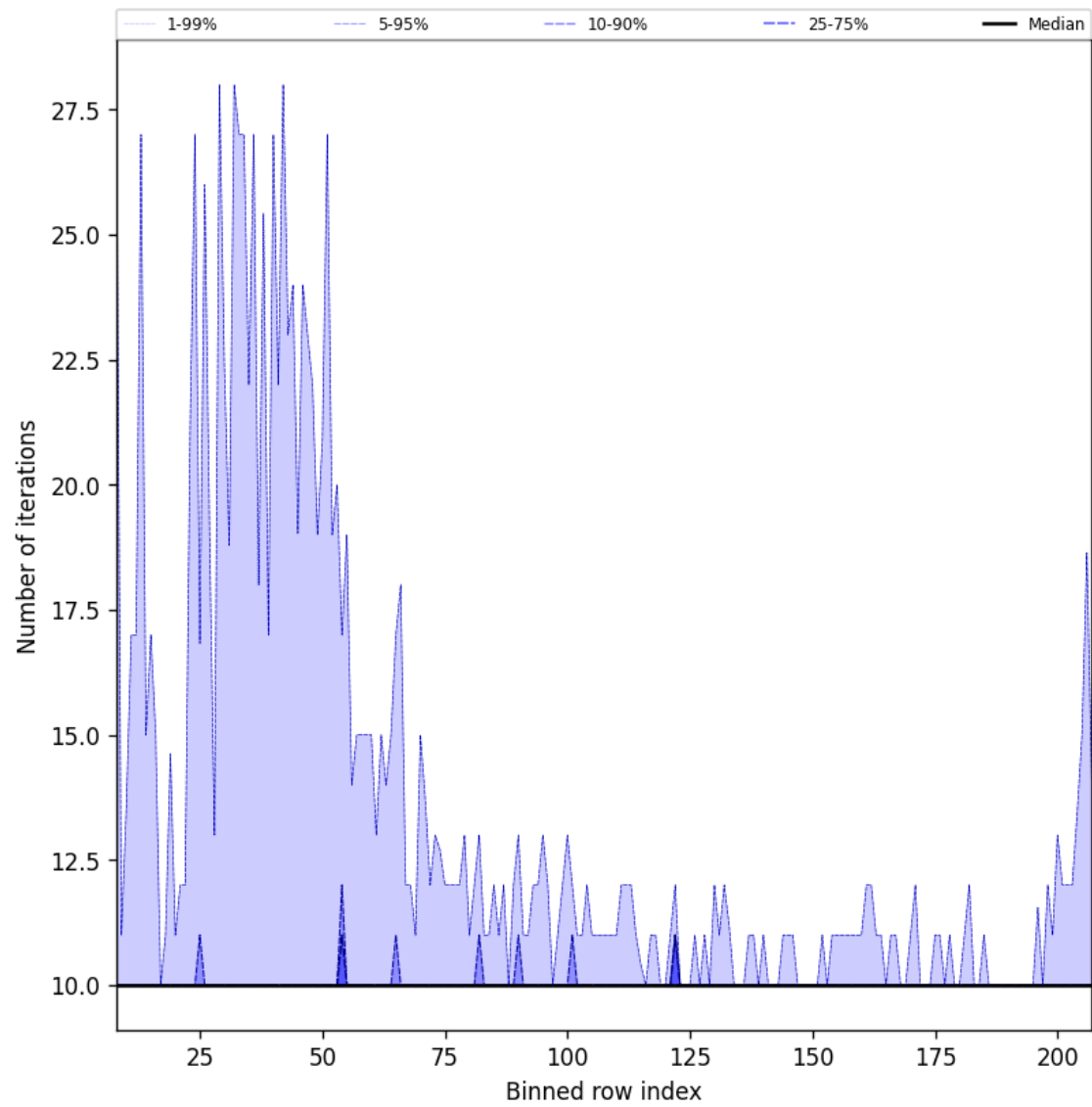
Figure 43: Along track statistics of “Number of iterations” for 2025-12-01 to 2025-12-01
