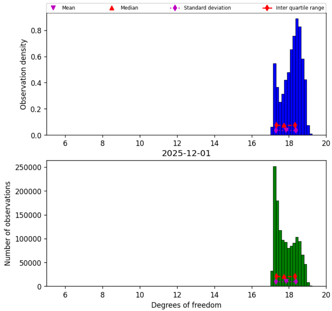
Figure 30: Histogram of “Degrees of freedom” for 2025-12-01 to 2025-12-01
