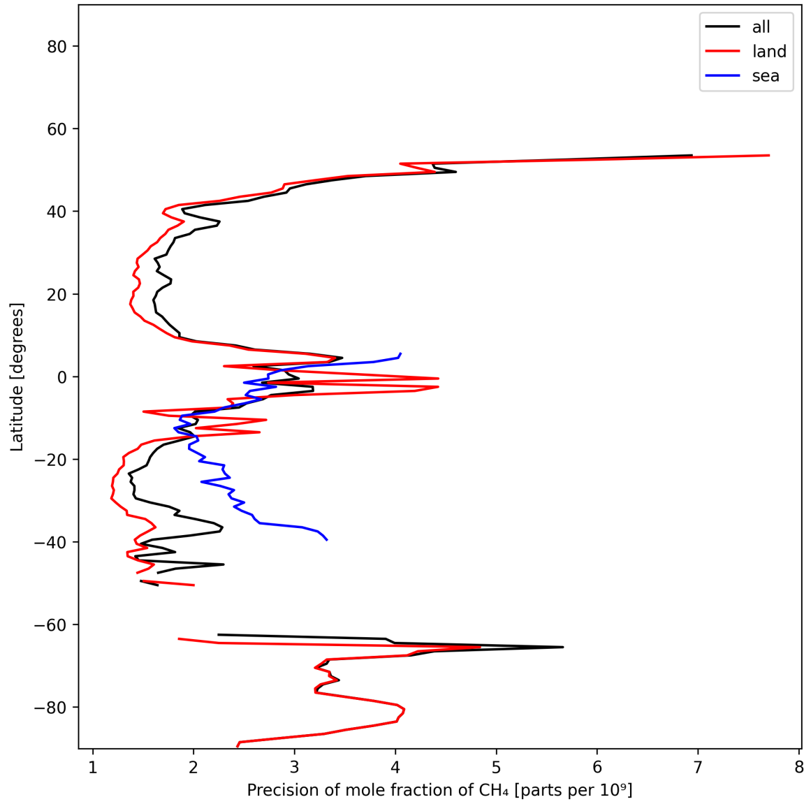
Figure 12: Zonal average of “Precision of mole fraction of CH 4 ” for 2025-12-01 to 2025-12-01.
