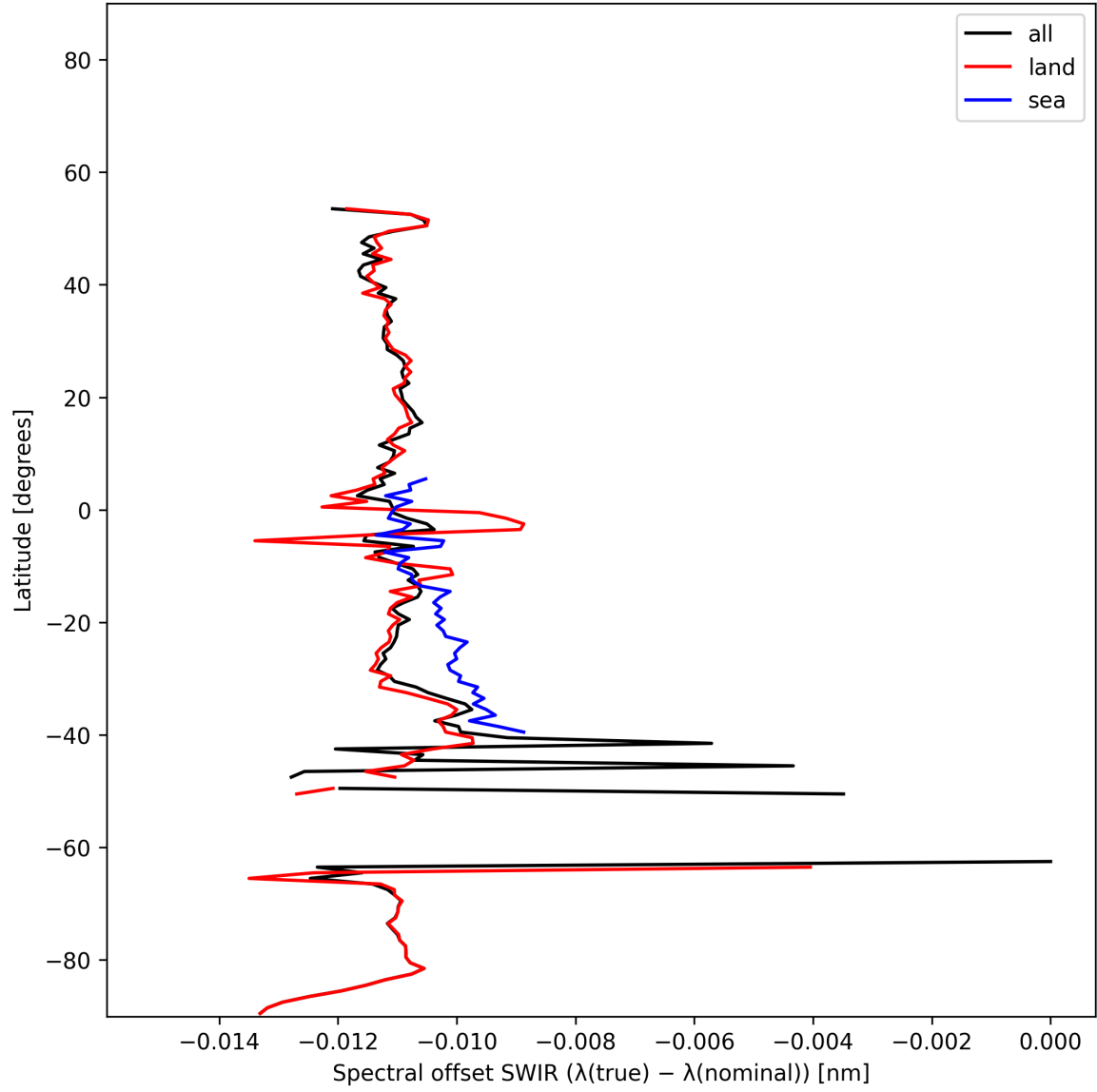
Figure 15: Zonal average of “Spectral offset SWIR ( \lambda_{\text{true}} - \lambda_{\text{nominal}} )” for 2025-12-01 to 2025-12-01.
