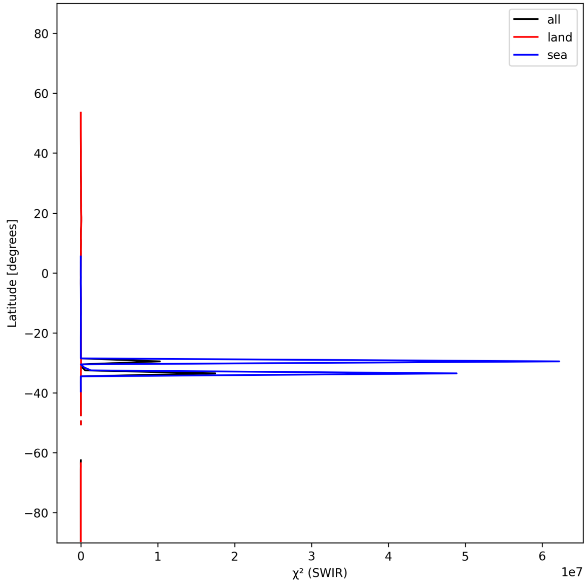
Figure 16: Zonal average of “ \chi^2 (SWIR)” for 2025-12-01 to 2025-12-01.
