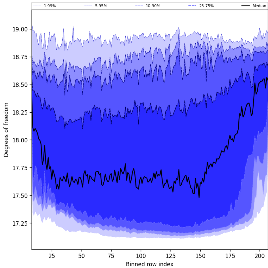
Figure 42: Along track statistics of “Degrees of freedom” for 2025-12-01 to 2025-12-01
