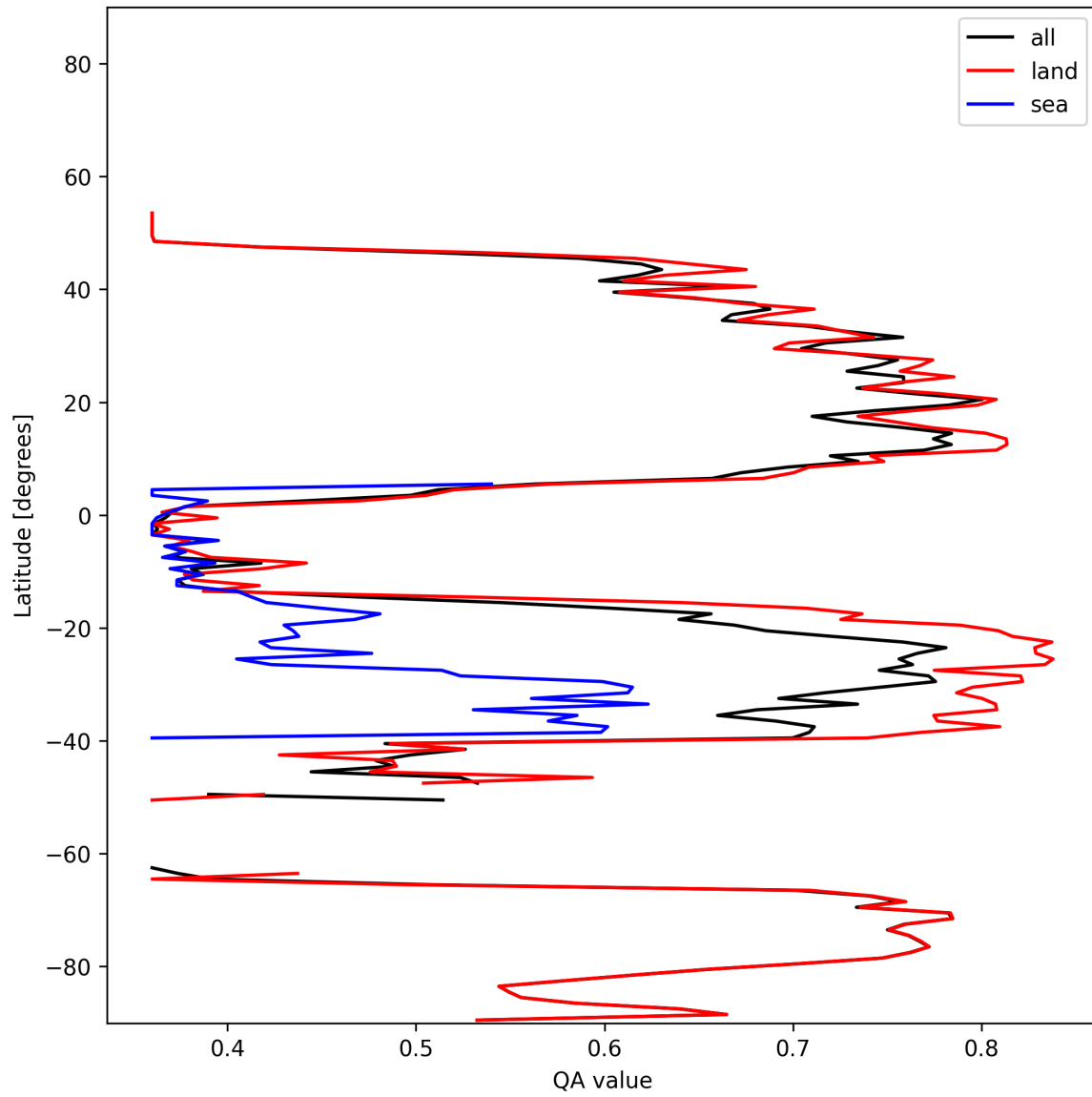
Figure 10: Zonal average of “QA value” for 2025-12-01 to 2025-12-01.
