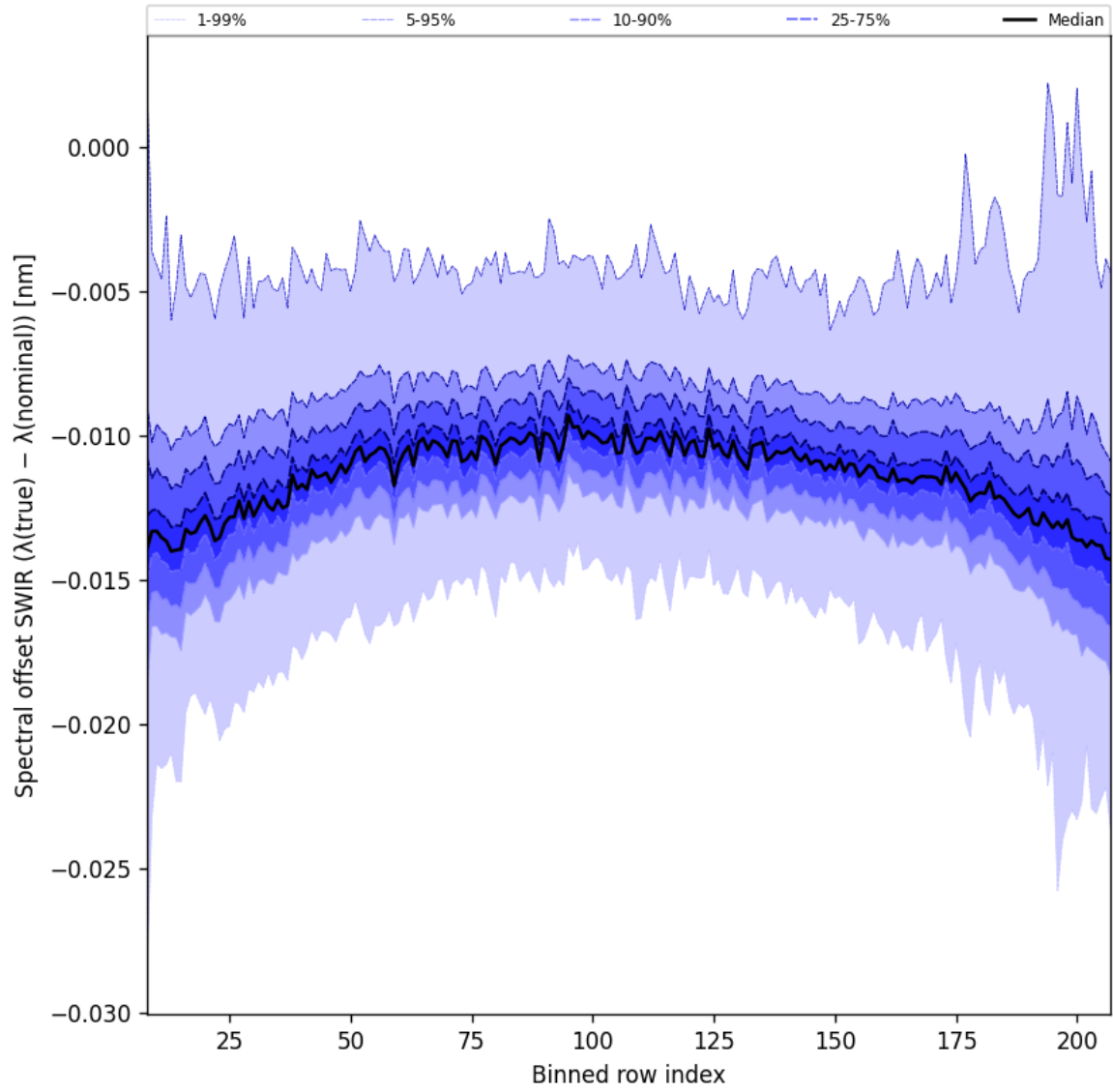
Figure 39: Along track statistics of “Spectral offset SWIR ( \lambda_{\text{true}} - \lambda_{\text{nominal}} )” for 2025-12-01 to 2025-12-01
