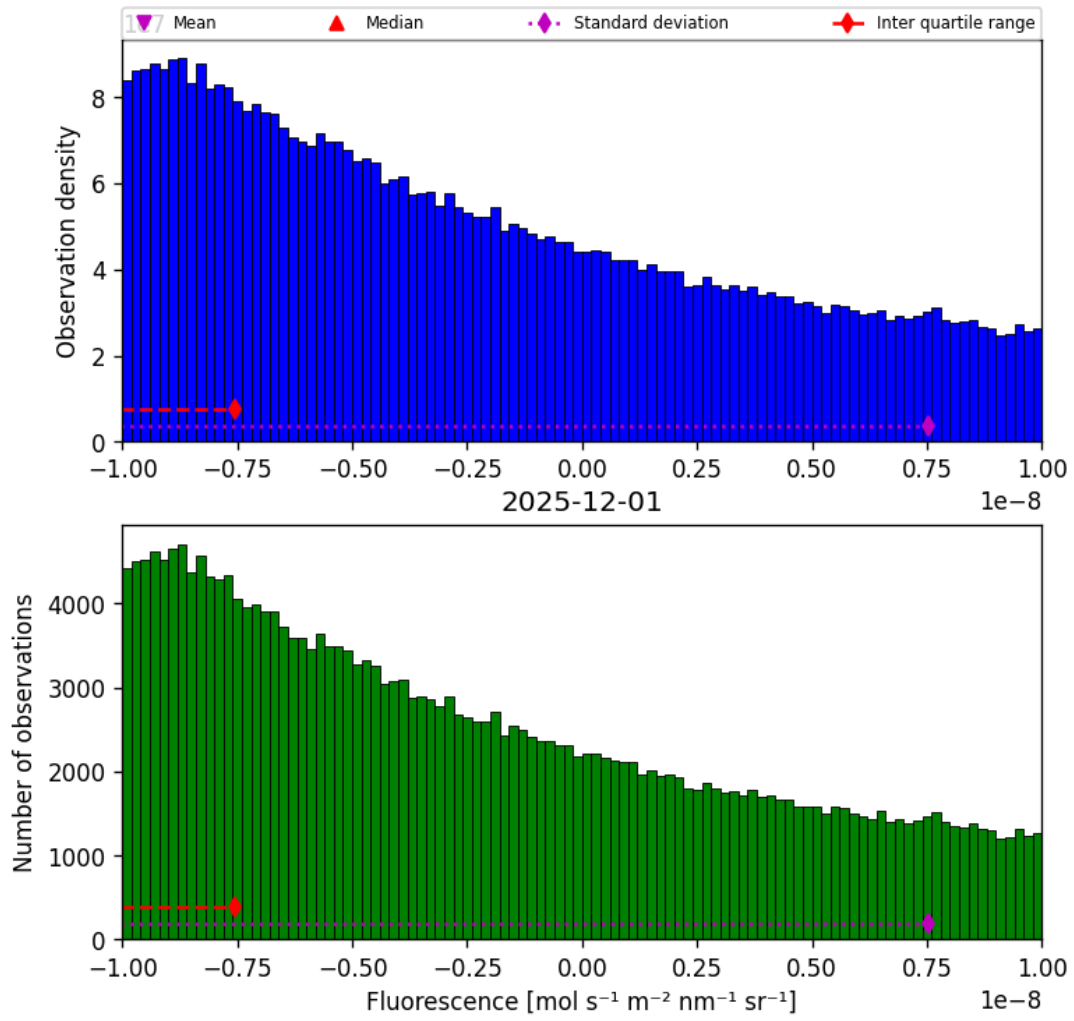
Figure 32: Histogram of “Fluorescence” for 2025-12-01 to 2025-12-01
