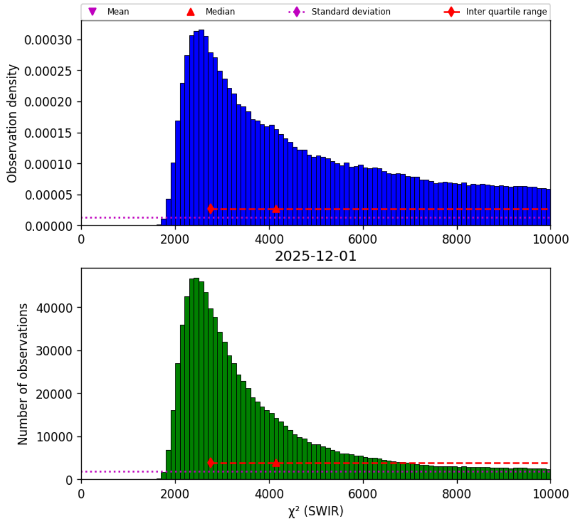
Figure 28: Histogram of " \chi^2 (SWIR)" for 2025-12-01 to 2025-12-01
