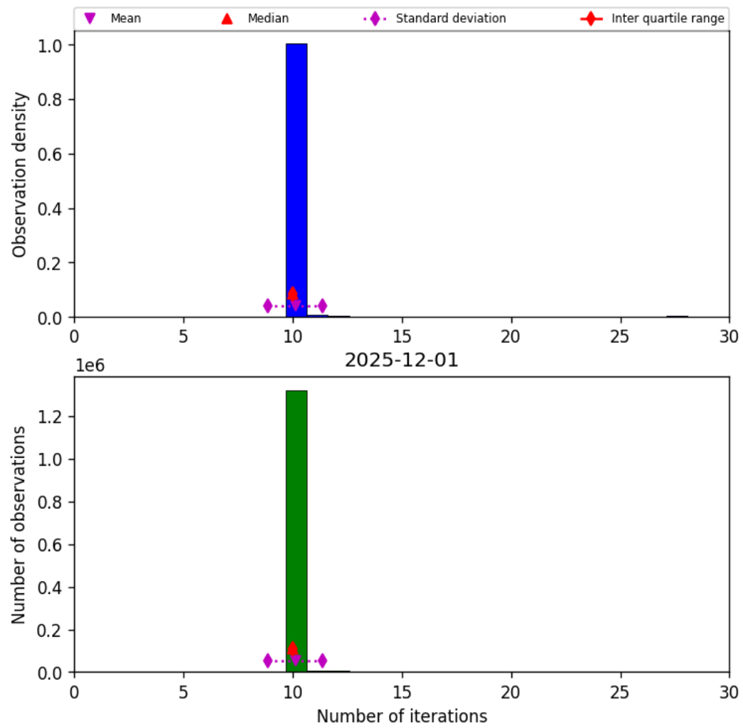
Figure 31: Histogram of “Number of iterations” for 2025-12-01 to 2025-12-01
