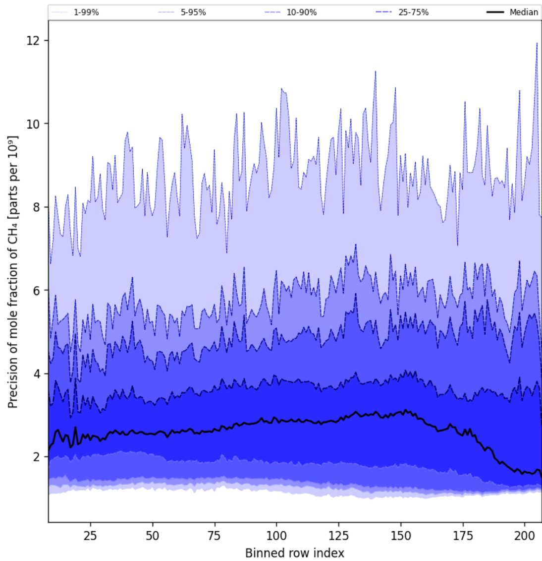
Figure 36: Along track statistics of “Precision of mole fraction of CH 4 ” for 2025-12-01 to 2025-12-01
