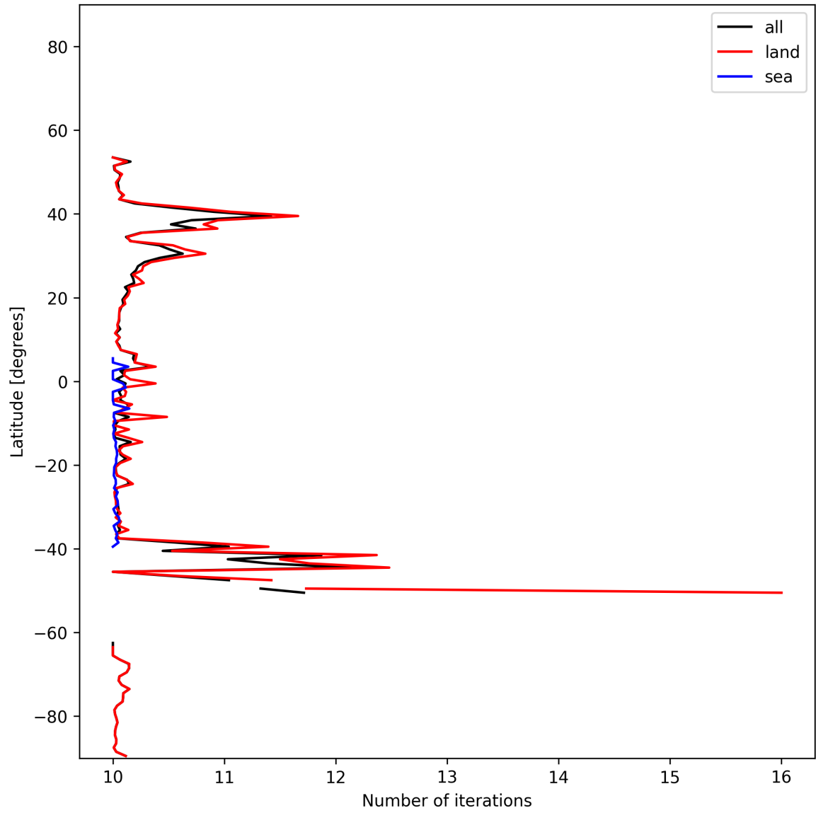
Figure 19: Zonal average of “Number of iterations” for 2025-12-01 to 2025-12-01.
