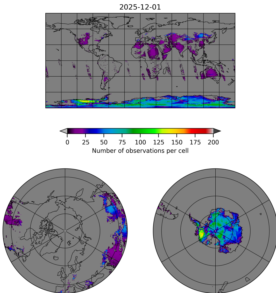
Figure 9: Map of the number of observations for 2025-12-01 to 2025-12-01
