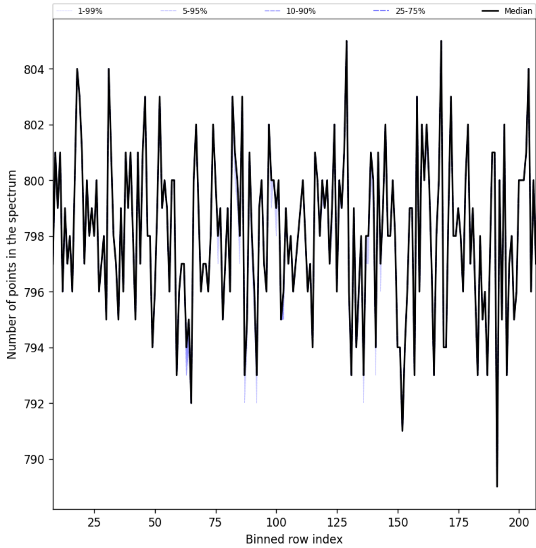
Figure 38: Along track statistics of “Number of points in the spectrum” for 2025-12-01 to 2025-12-01
