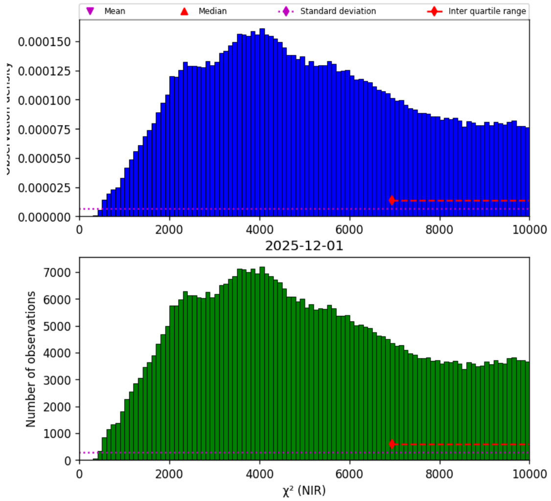
Figure 29: Histogram of “ \chi^2 (NIR)” for 2025-12-01 to 2025-12-01
