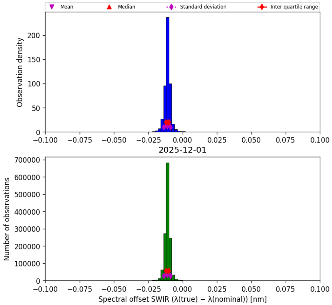
Figure 27: Histogram of “Spectral offset SWIR ( \lambda_{\text{true}} - \lambda_{\text{nominal}} )” for 2025-12-01 to 2025-12-01
