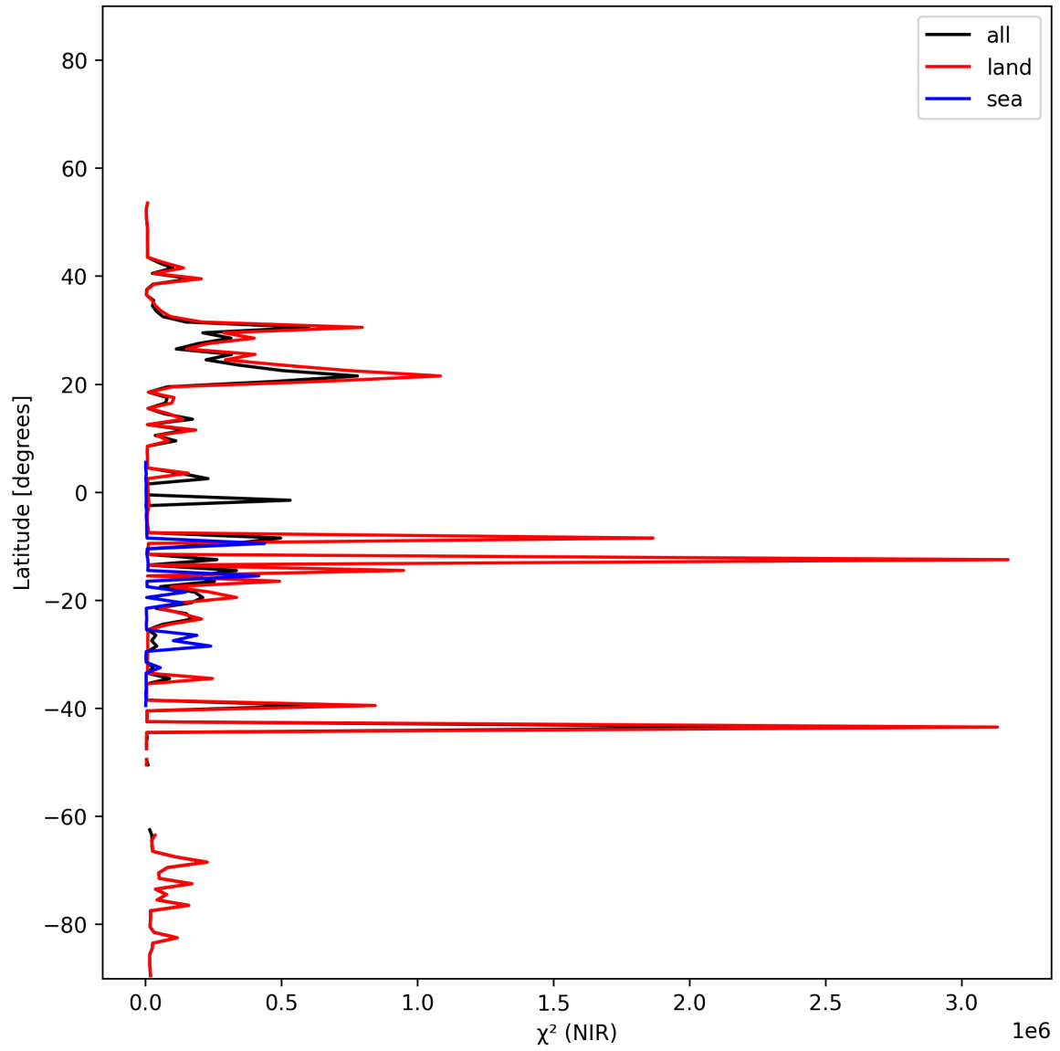
Figure 17: Zonal average of “ \chi^2 (NIR)” for 2025-12-01 to 2025-12-01.
