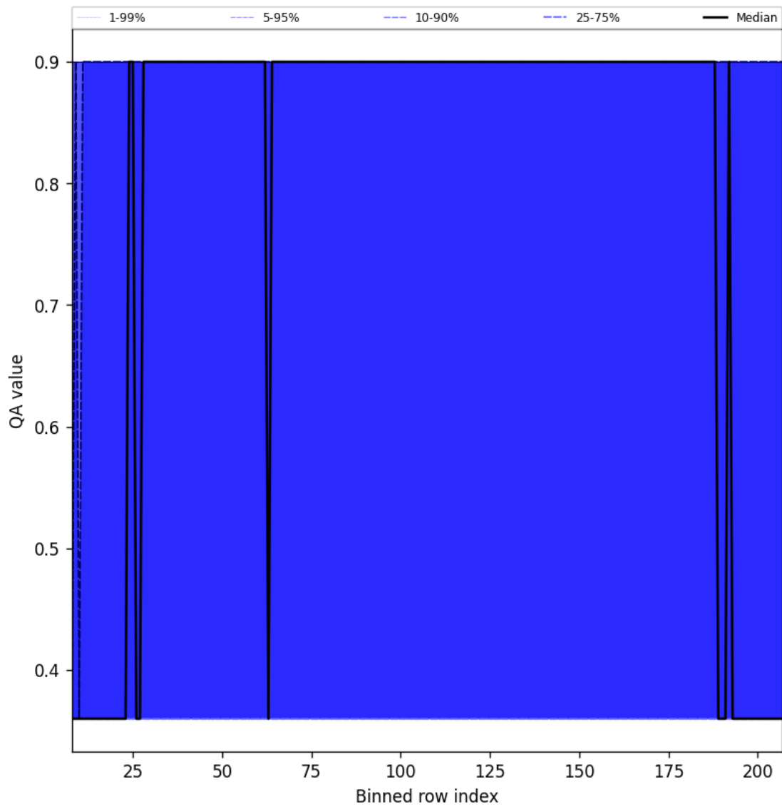
Figure 34: Along track statistics of “QA value” for 2025-12-01 to 2025-12-01
