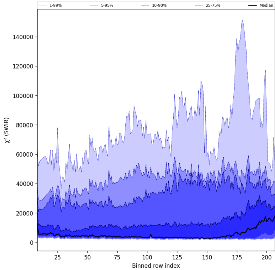
Figure 40: Along track statistics of “ \chi^2 (SWIR)” for 2025-12-01 to 2025-12-01
