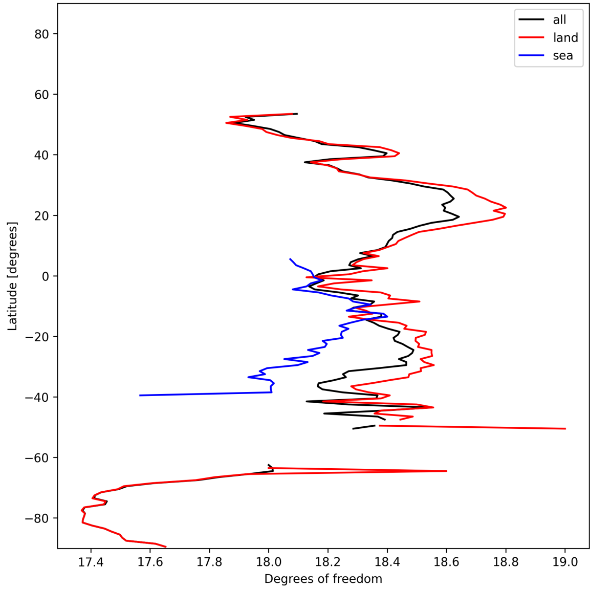
Figure 18: Zonal average of “Degrees of freedom” for 2025-12-01 to 2025-12-01.
