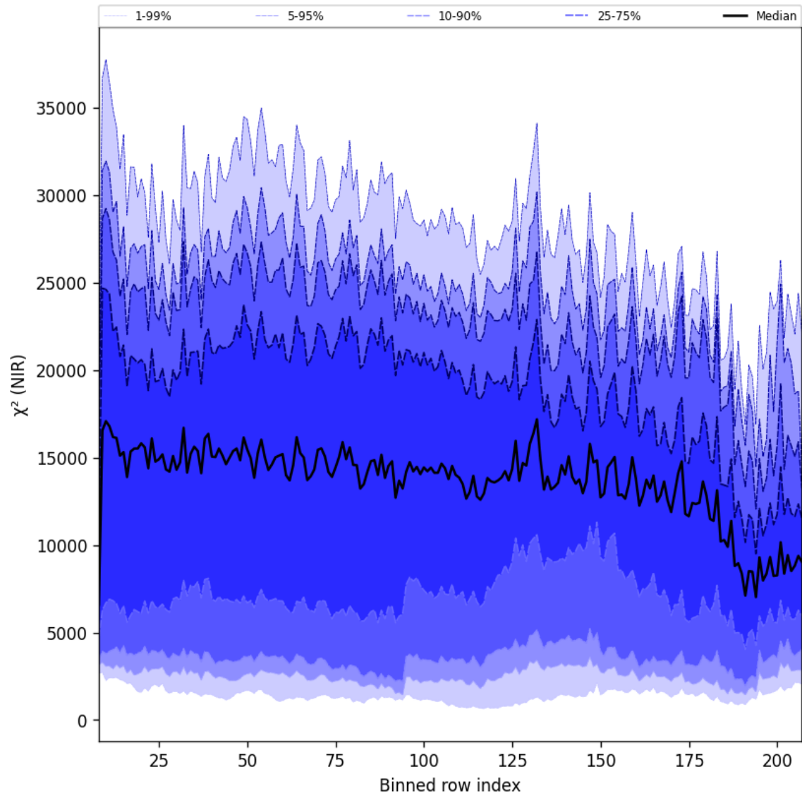
Figure 41: Along track statistics of " \chi^2 (NIR)" for 2025-12-01 to 2025-12-01
