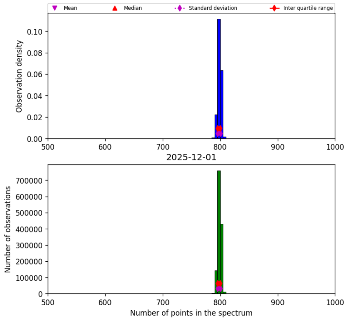
Figure 26: Histogram of “Number of points in the spectrum” for 2025-12-01 to 2025-12-01
