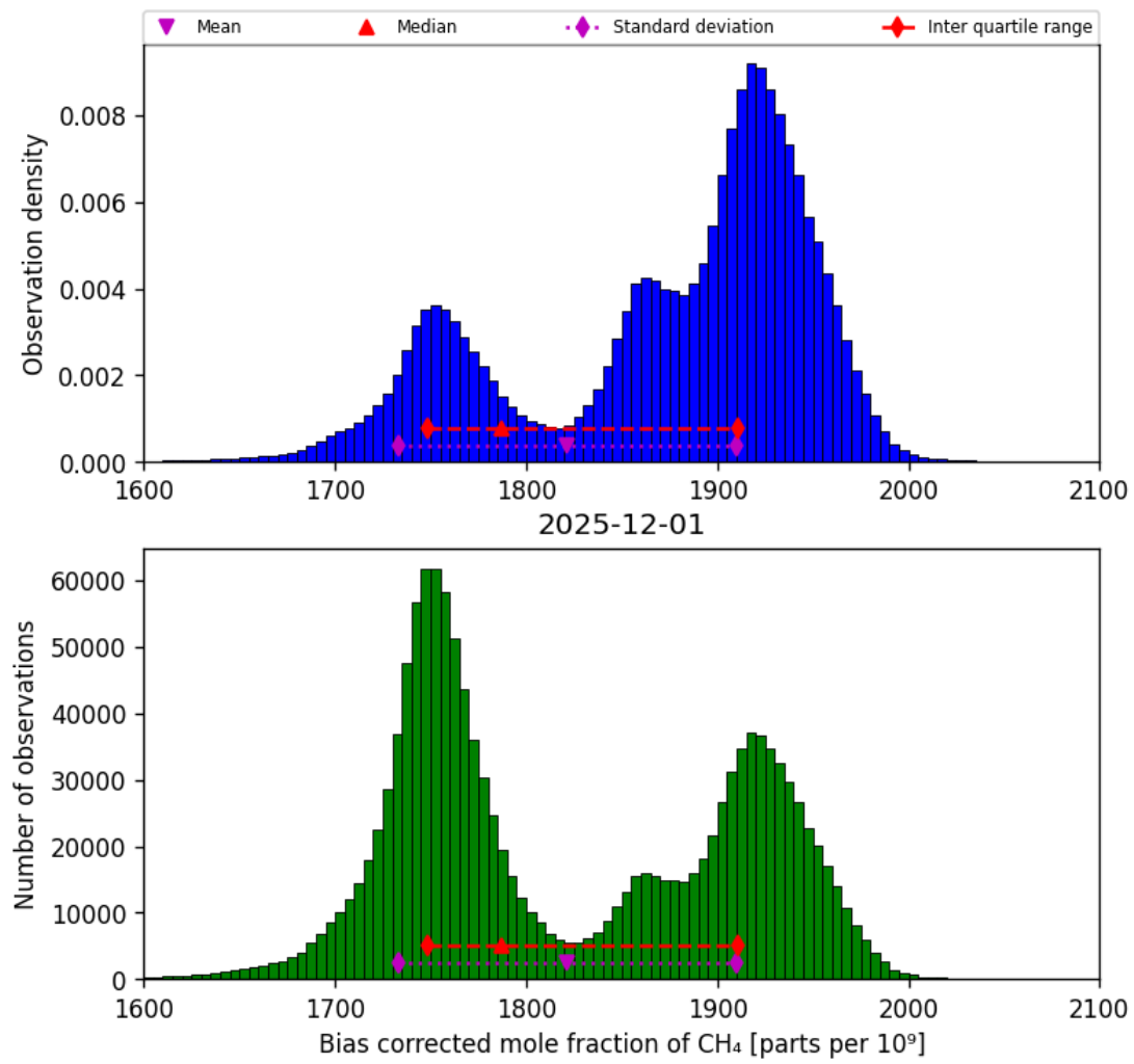
Figure 25: Histogram of “Bias corrected mole fraction of CH 4 ” for 2025-12-01 to 2025-12-01
