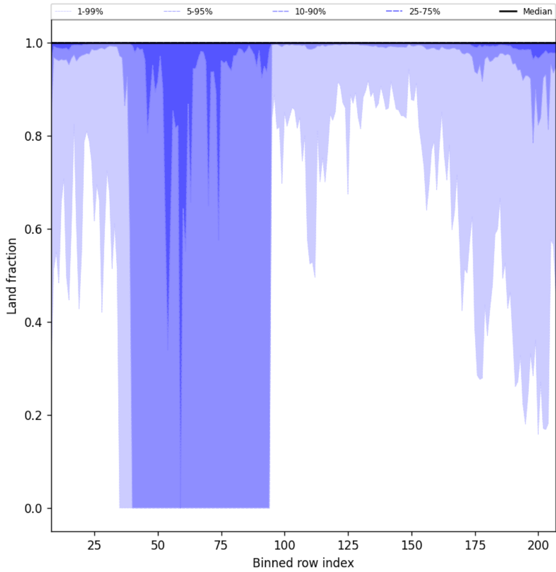
Figure 45: Along track statistics of "Land fraction" for 2025-12-01 to 2025-12-01
