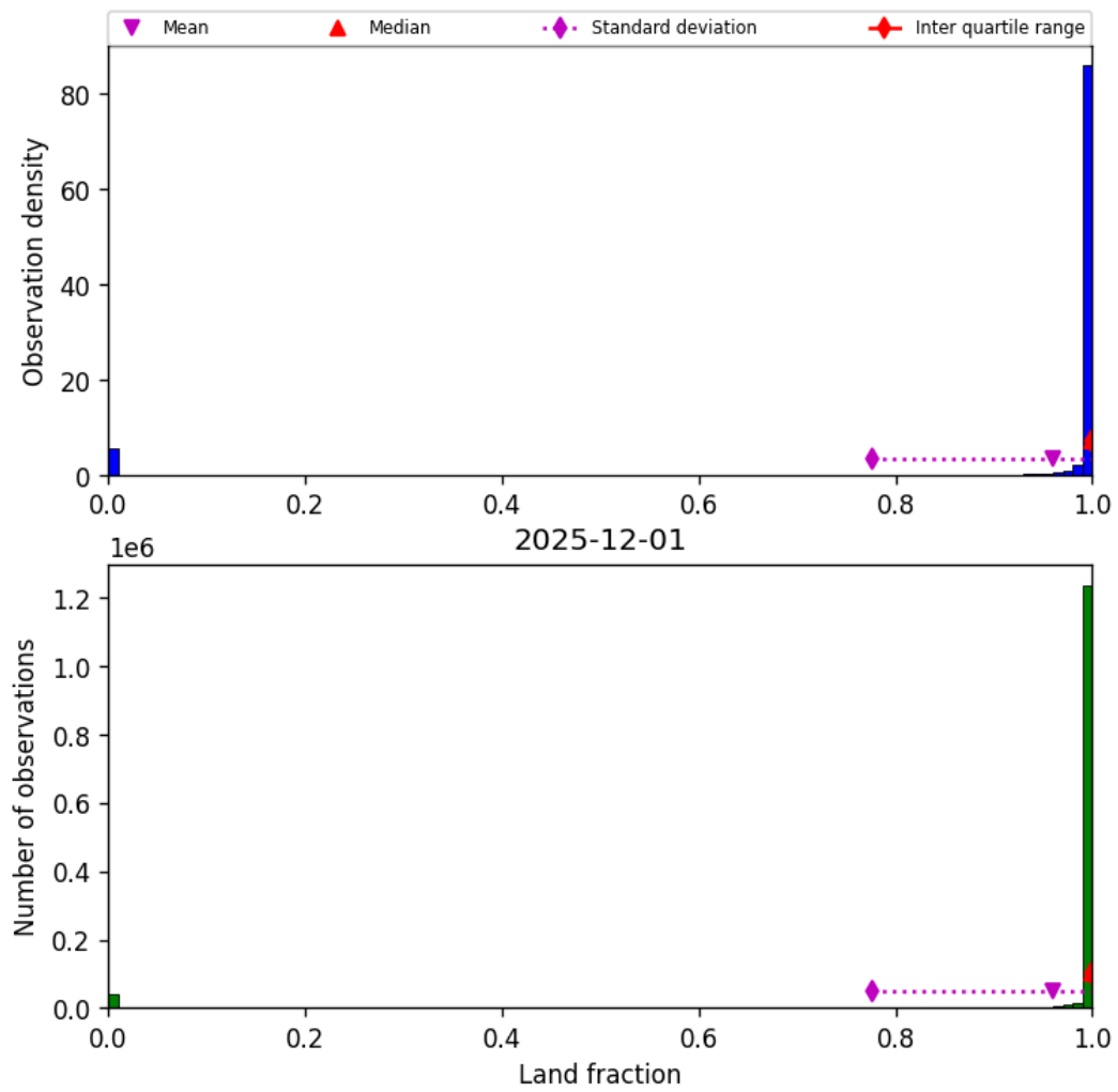
Figure 33: Histogram of “Land fraction” for 2025-12-01 to 2025-12-01
