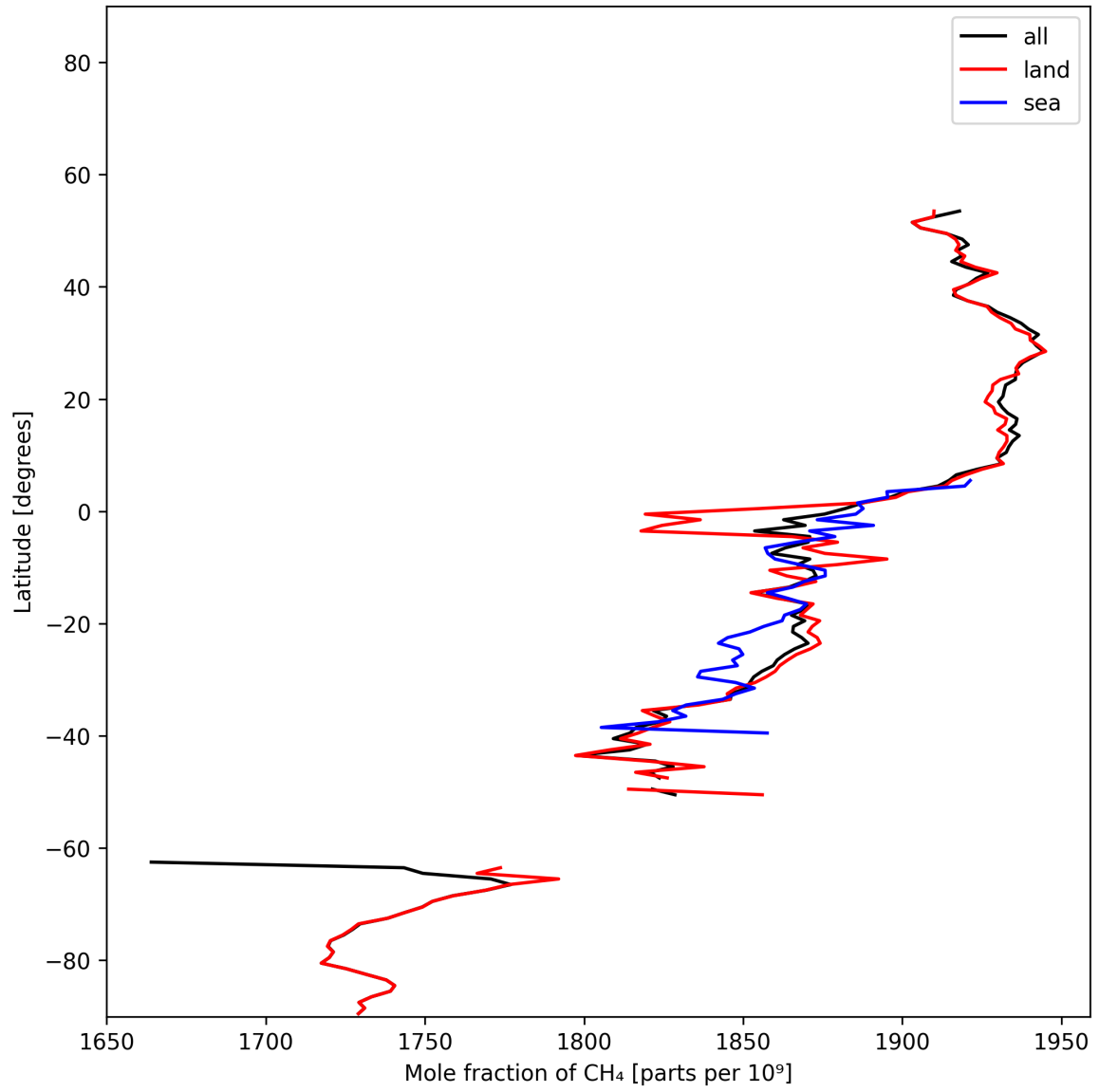
Figure 11: Zonal average of “Mole fraction of CH 4 ” for 2025-12-01 to 2025-12-01.
