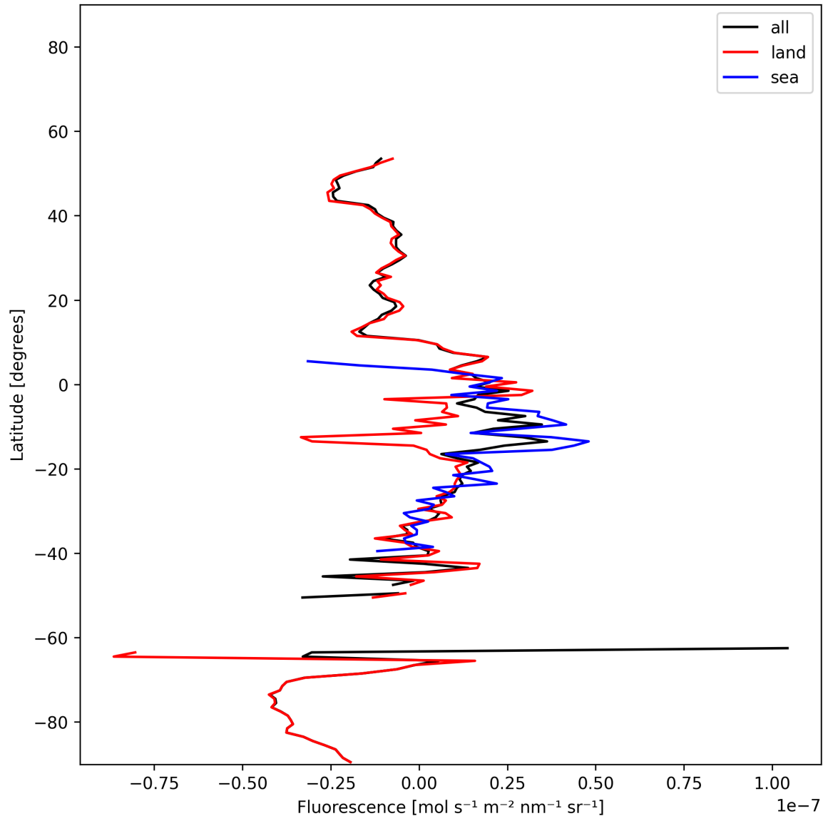
Figure 20: Zonal average of “Fluorescence” for 2025-12-01 to 2025-12-01.
