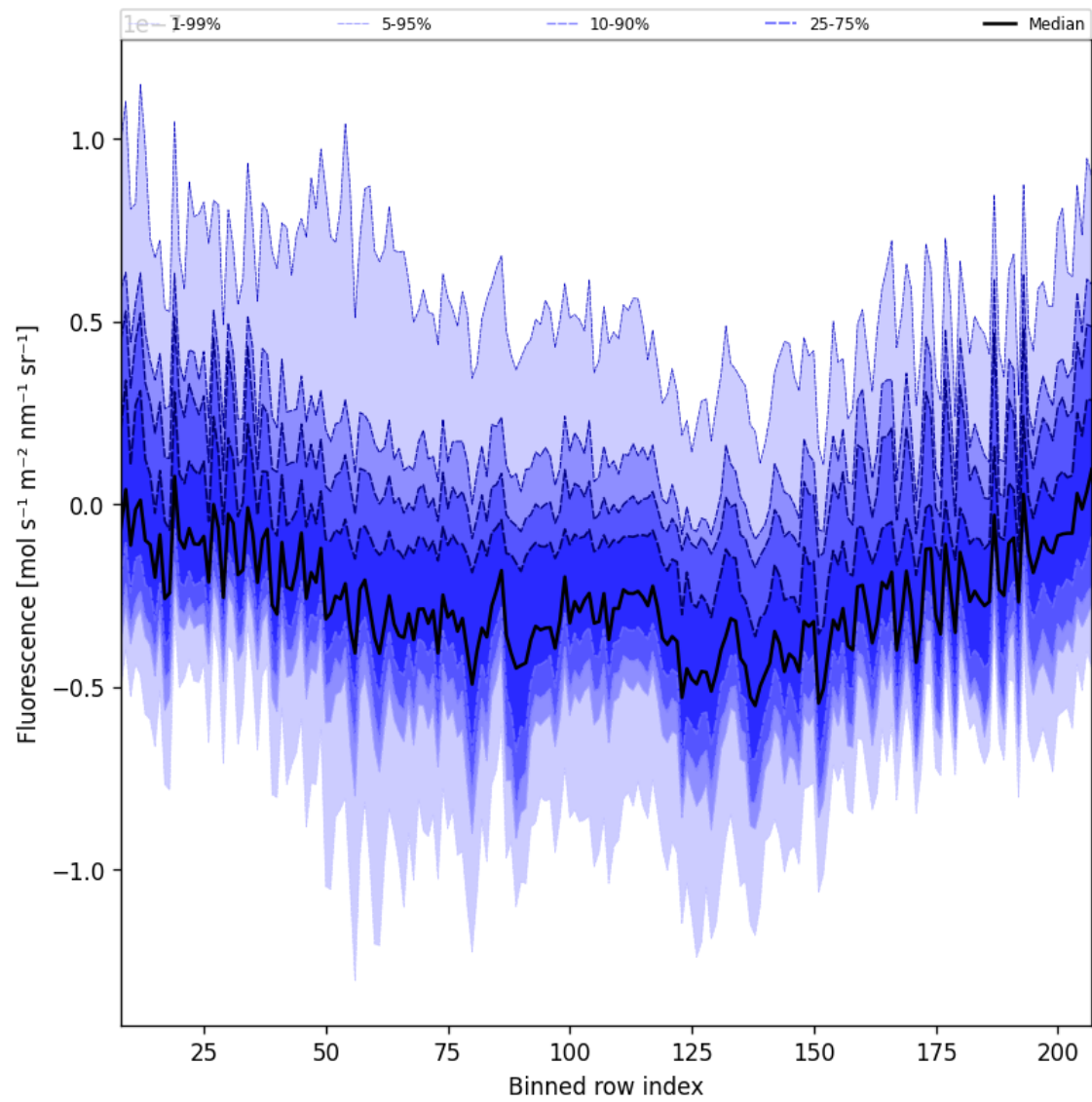
Figure 44: Along track statistics of “Fluorescence” for 2025-12-01 to 2025-12-01
