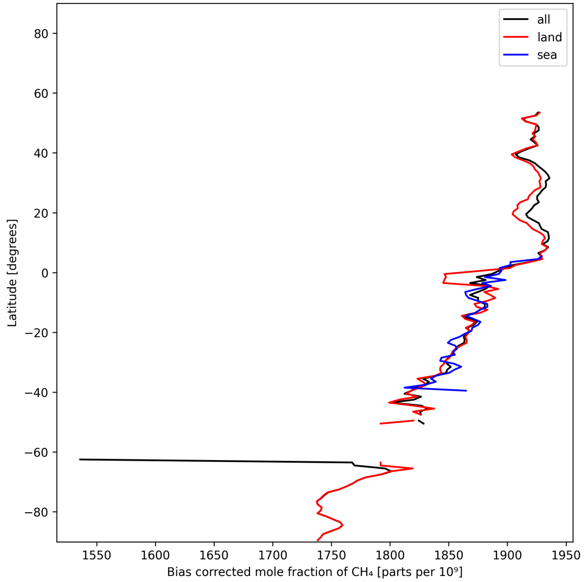
Figure 13: Zonal average of “Bias corrected mole fraction of CH 4 ” for 2025-12-01 to 2025-12-01.
