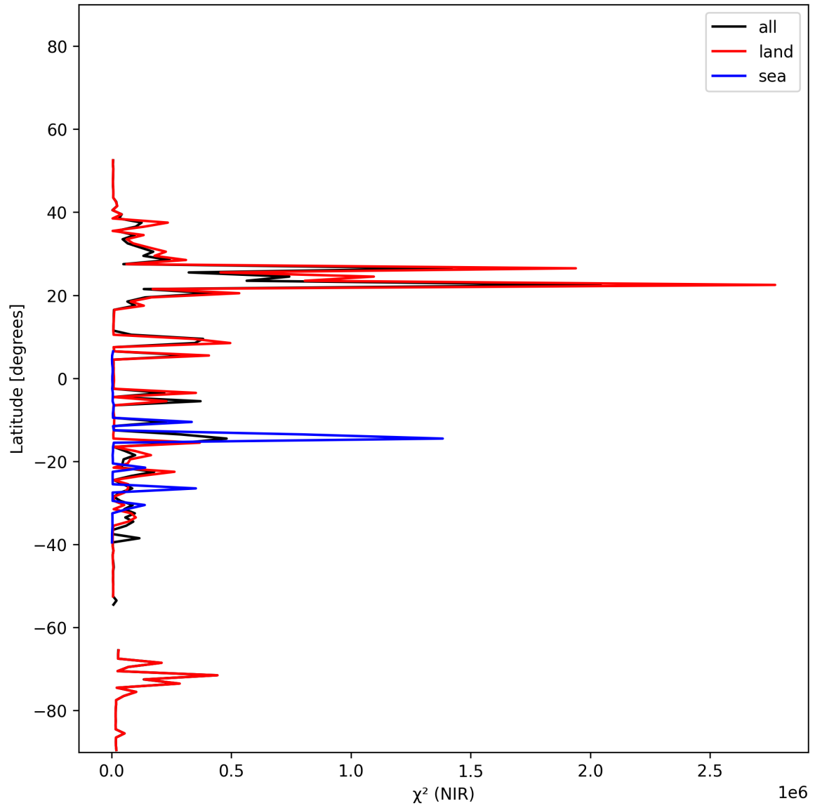
Figure 17: Zonal average of “ \chi^2 (NIR)” for 2025-12-02 to 2025-12-02.
