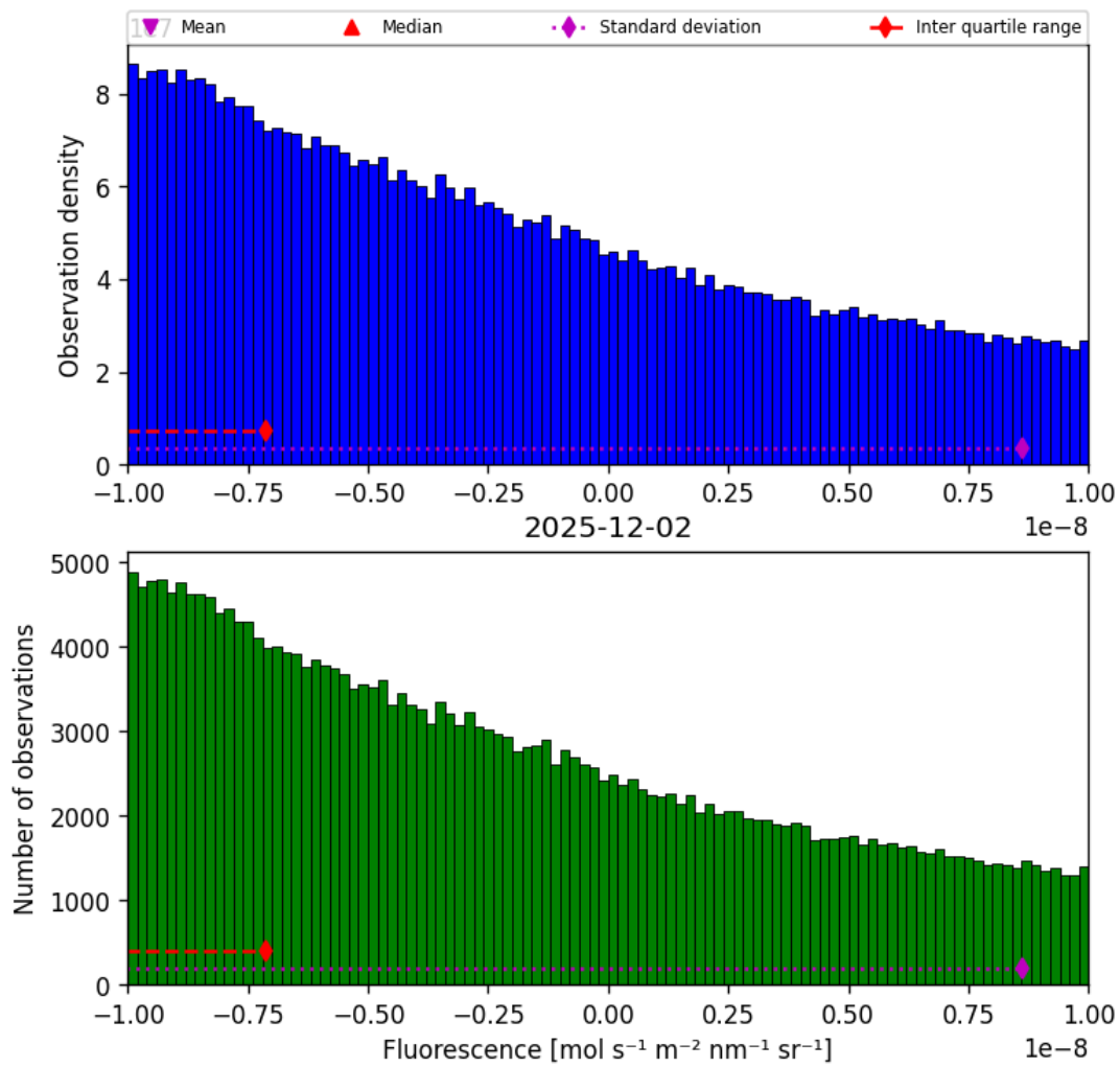
Figure 32: Histogram of “Fluorescence” for 2025-12-02 to 2025-12-02
