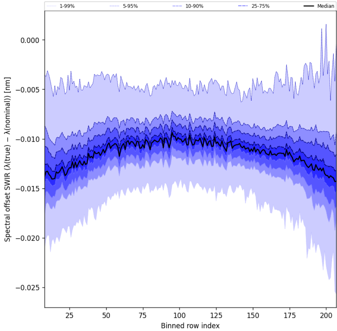
Figure 39: Along track statistics of “Spectral offset SWIR ( \lambda_{\text{true}} - \lambda_{\text{nominal}} )” for 2025-12-02 to 2025-12-02
