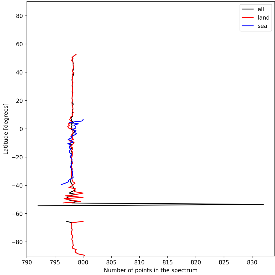
Figure 14: Zonal average of “Number of points in the spectrum” for 2025-12-02 to 2025-12-02.
