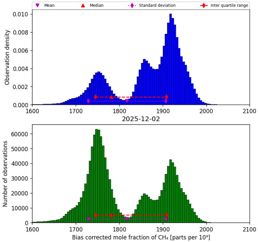
Figure 25: Histogram of “Bias corrected mole fraction of CH 4 ” for 2025-12-02 to 2025-12-02
