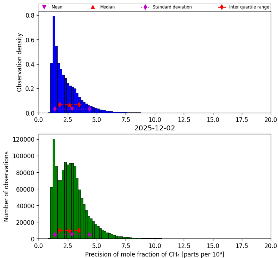
Figure 24: Histogram of “Precision of mole fraction of CH 4 ” for 2025-12-02 to 2025-12-02
