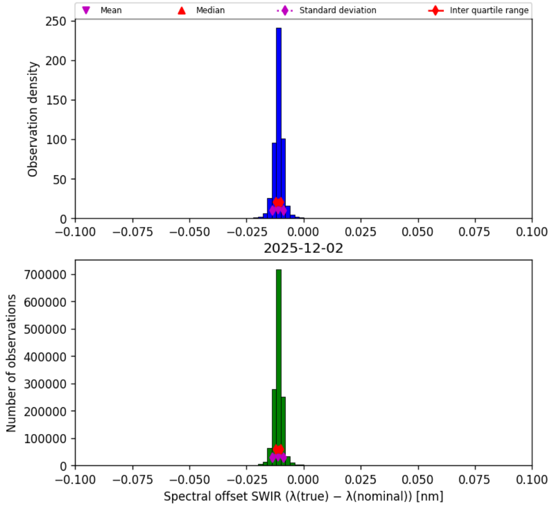
Figure 27: Histogram of “Spectral offset SWIR ( \lambda_{\text{true}} - \lambda_{\text{nominal}} )” for 2025-12-02 to 2025-12-02
