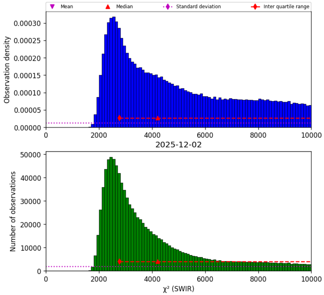
Figure 28: Histogram of “ \chi^2 (SWIR)” for 2025-12-02 to 2025-12-02
