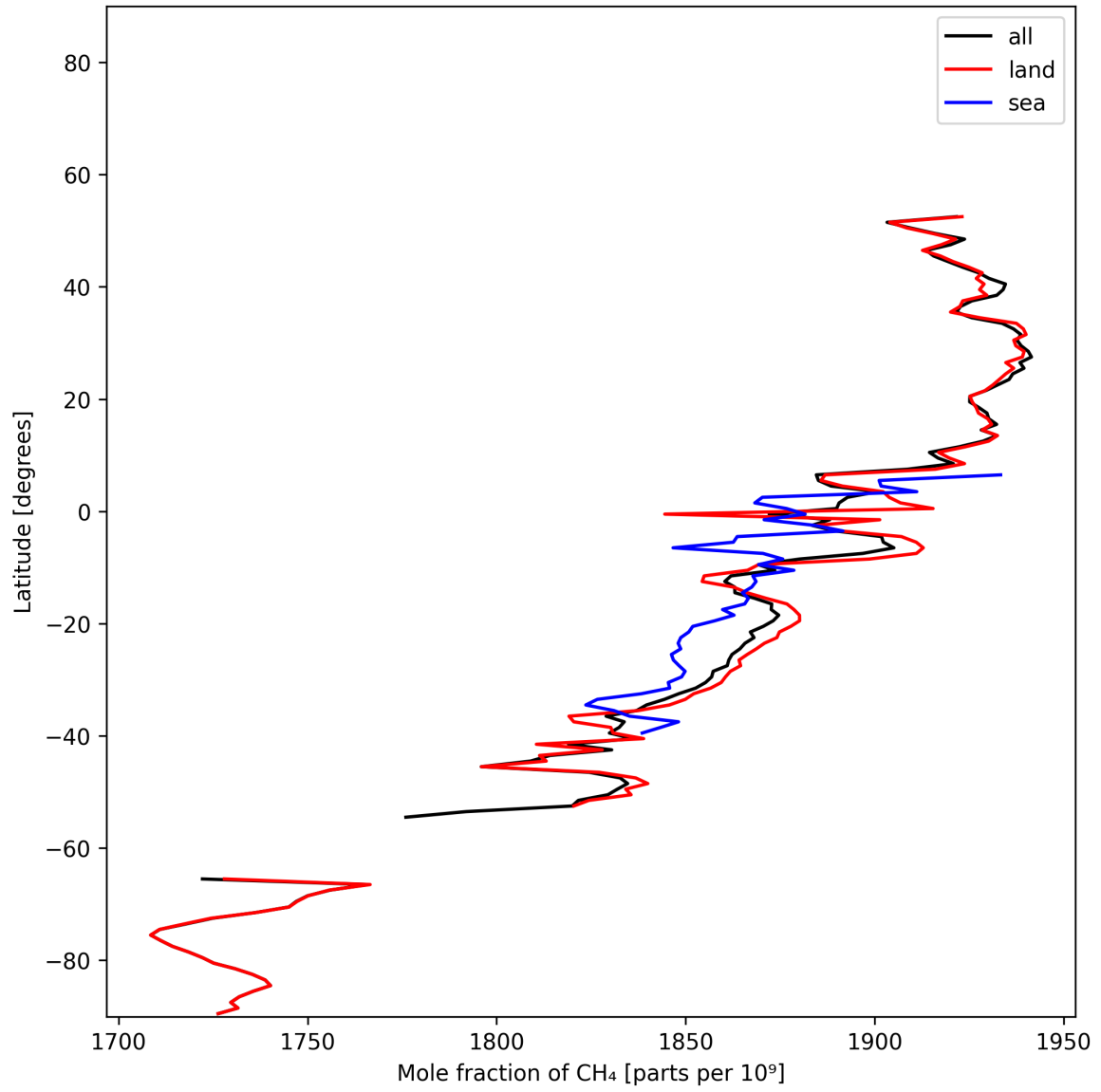
Figure 11: Zonal average of “Mole fraction of \text{CH}_4 ” for 2025-12-02 to 2025-12-02.
