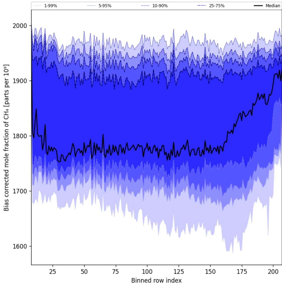
Figure 37: Along track statistics of “Bias corrected mole fraction of CH 4 ” for 2025-12-02 to 2025-12-02
