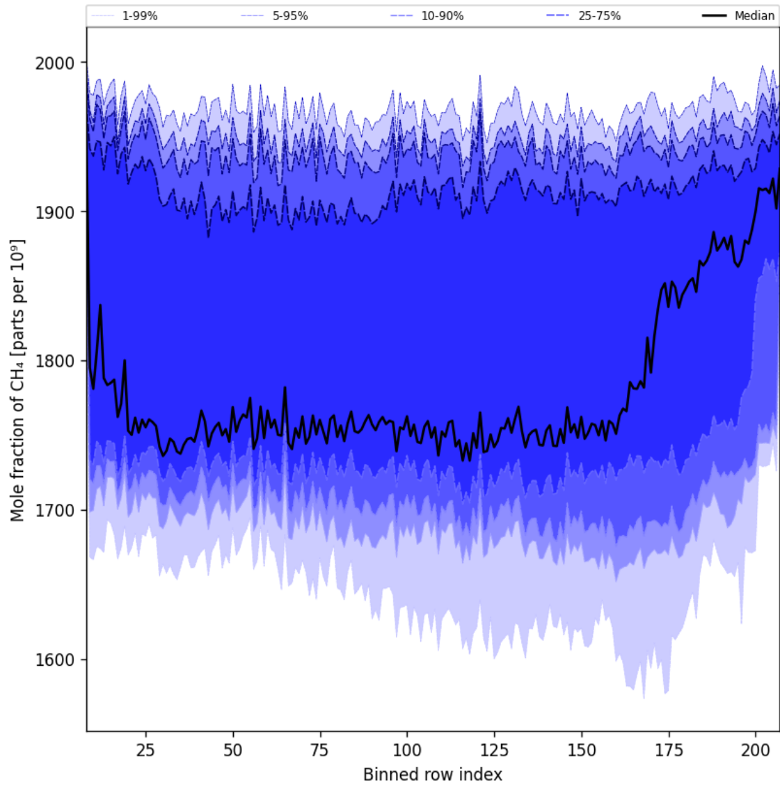
Figure 35: Along track statistics of “Mole fraction of CH 4 ” for 2025-12-02 to 2025-12-02
