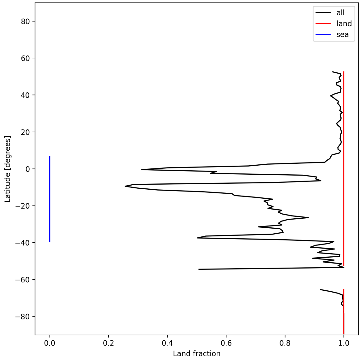
Figure 21: Zonal average of “Land fraction” for 2025-12-02 to 2025-12-02.
