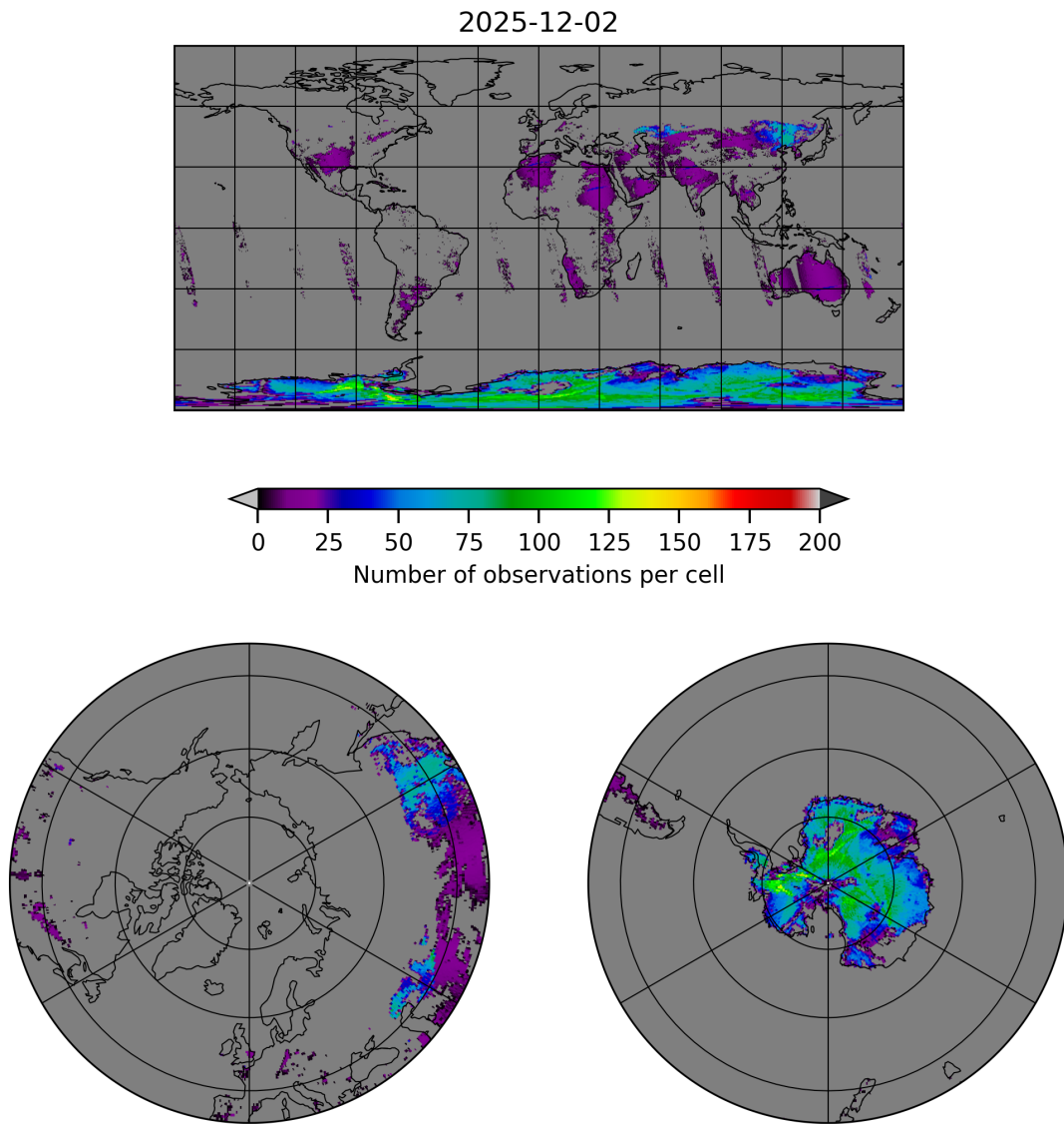
Figure 9: Map of the number of observations for 2025-12-02 to 2025-12-02
