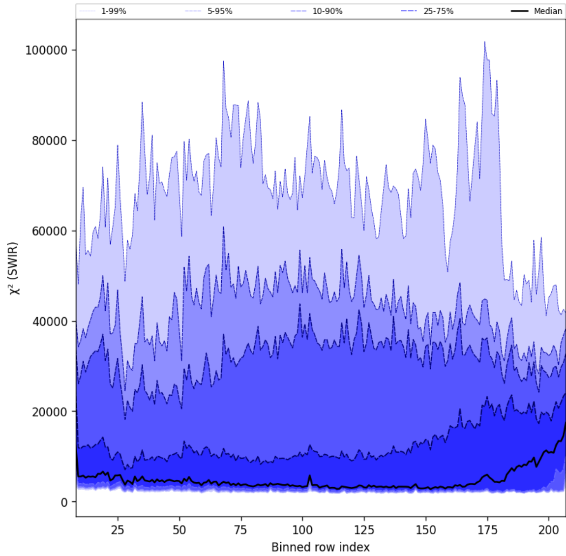
Figure 40: Along track statistics of “ \chi^2 (SWIR)” for 2025-12-02 to 2025-12-02
