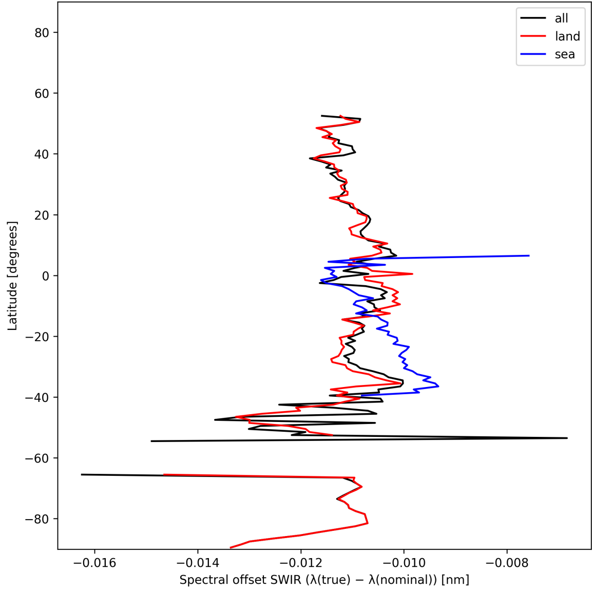
Figure 15: Zonal average of “Spectral offset SWIR ( \lambda_{\text{true}} - \lambda_{\text{nominal}} )” for 2025-12-02 to 2025-12-02.
