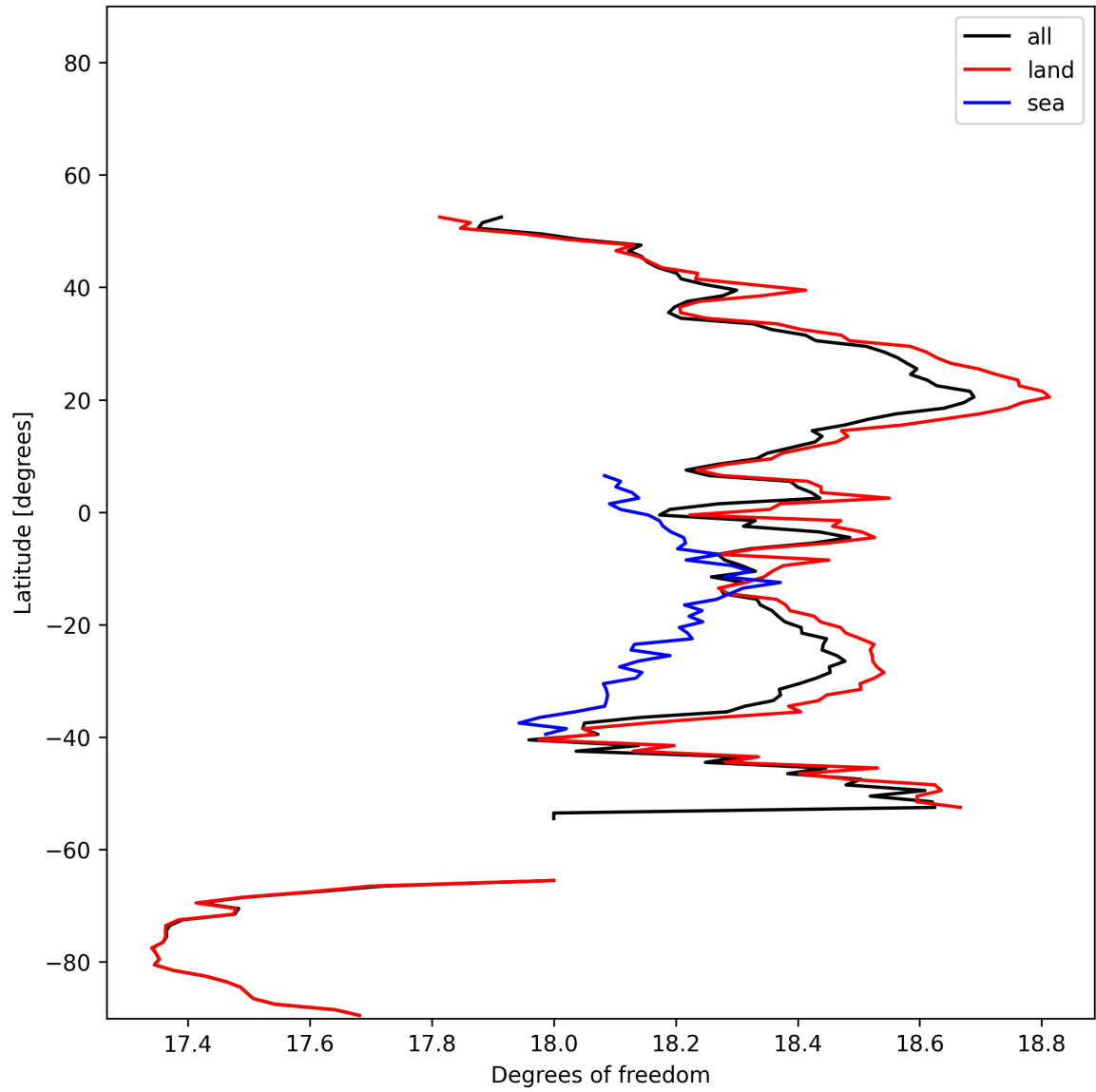
Figure 18: Zonal average of “Degrees of freedom” for 2025-12-02 to 2025-12-02.
