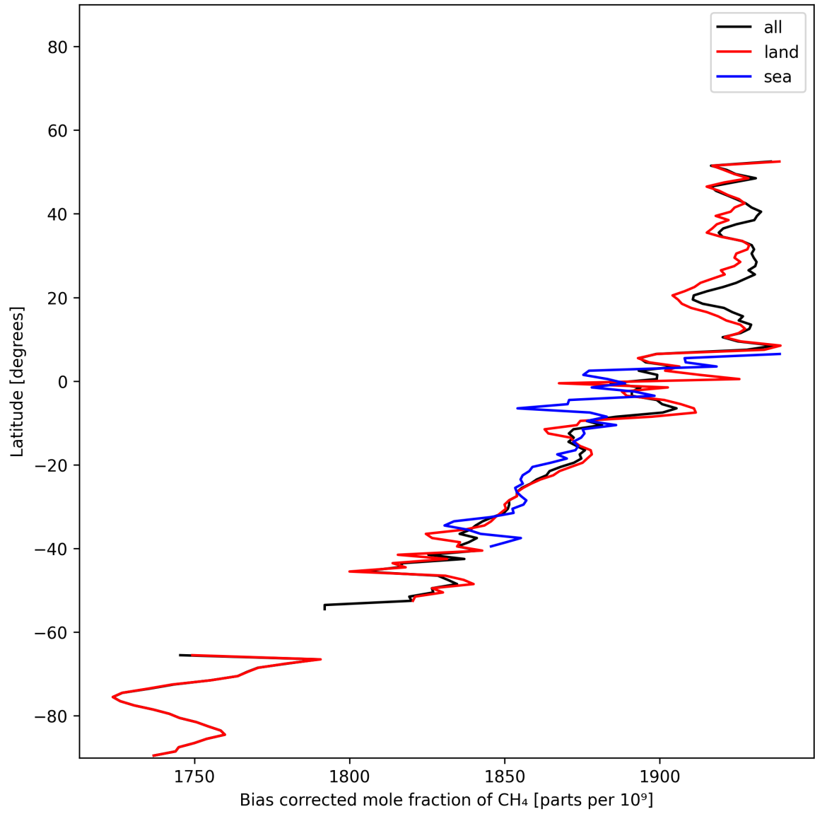
Figure 13: Zonal average of “Bias corrected mole fraction of CH 4 ” for 2025-12-02 to 2025-12-02.
