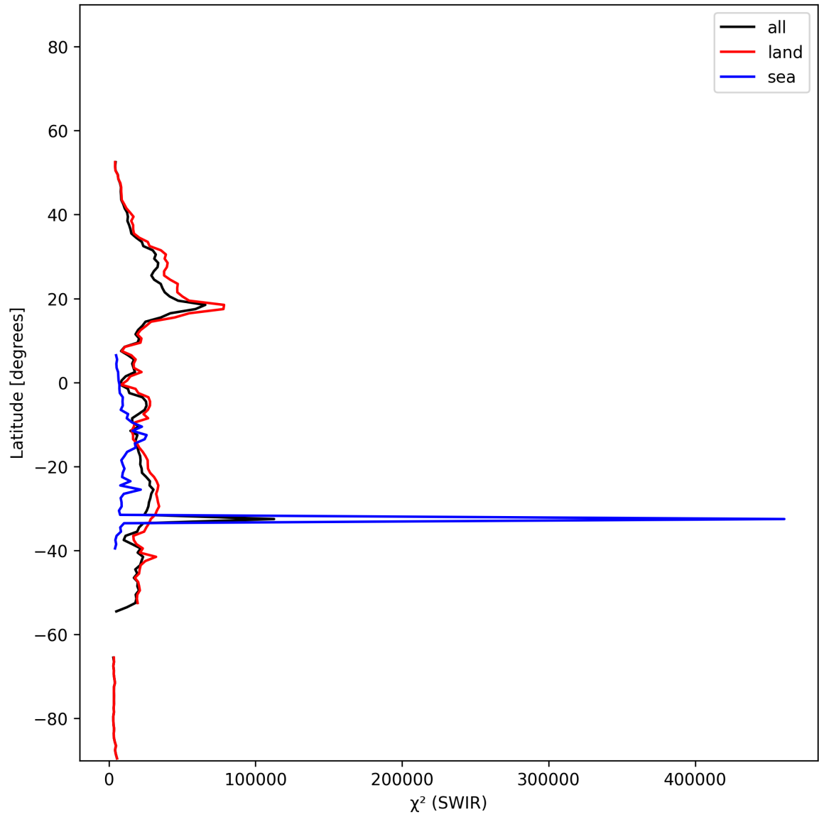
Figure 16: Zonal average of “ \chi^2 (SWIR)” for 2025-12-02 to 2025-12-02.
