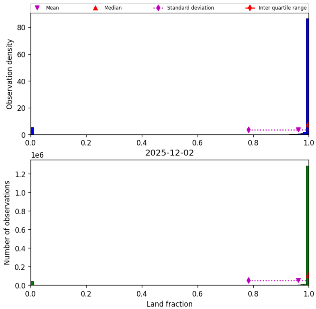
Figure 33: Histogram of “Land fraction” for 2025-12-02 to 2025-12-02
