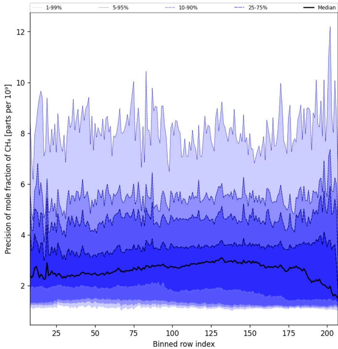
Figure 36: Along track statistics of “Precision of mole fraction of CH 4 ” for 2025-12-02 to 2025-12-02
