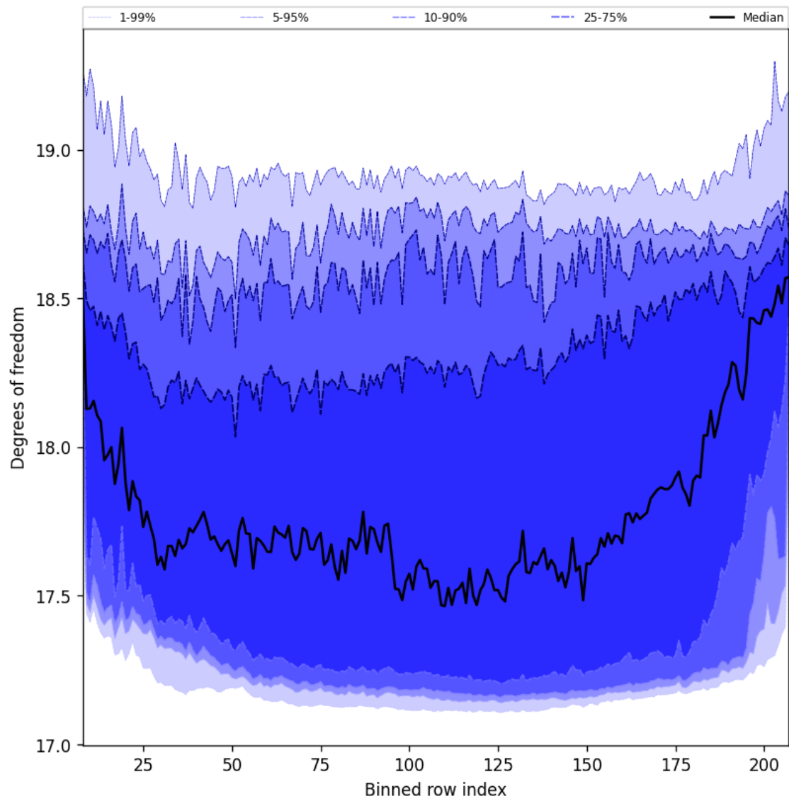
Figure 42: Along track statistics of “Degrees of freedom” for 2025-12-02 to 2025-12-02
