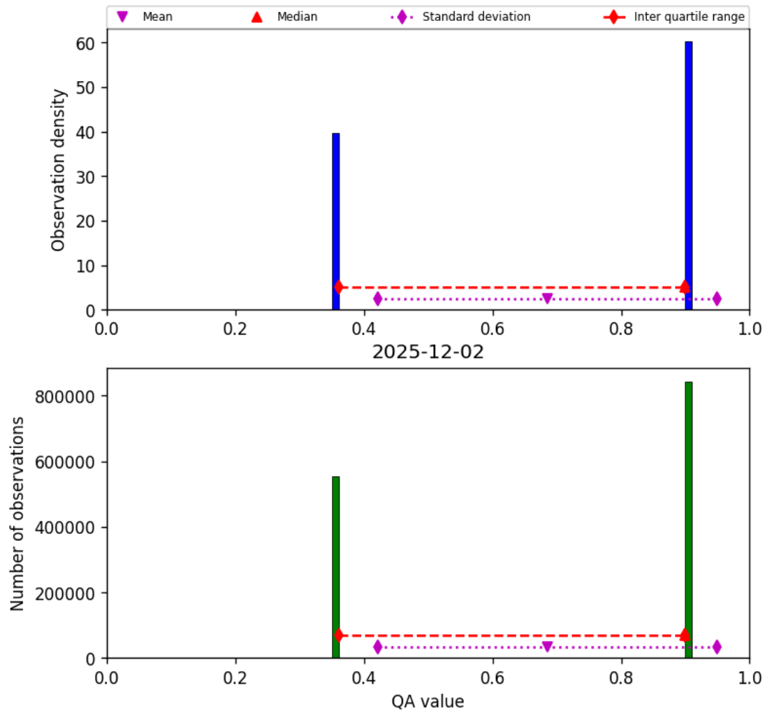
Figure 22: Histogram of “QA value” for 2025-12-02 to 2025-12-02
