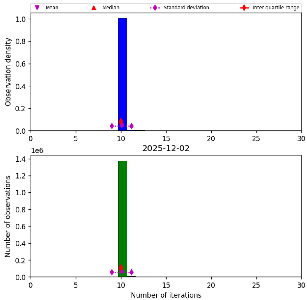
Figure 31: Histogram of “Number of iterations” for 2025-12-02 to 2025-12-02
