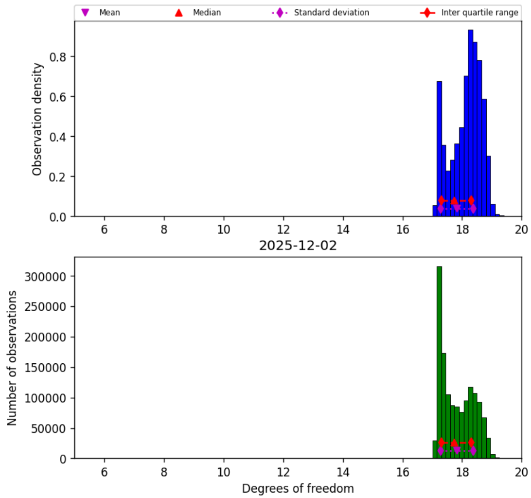
Figure 30: Histogram of “Degrees of freedom” for 2025-12-02 to 2025-12-02
