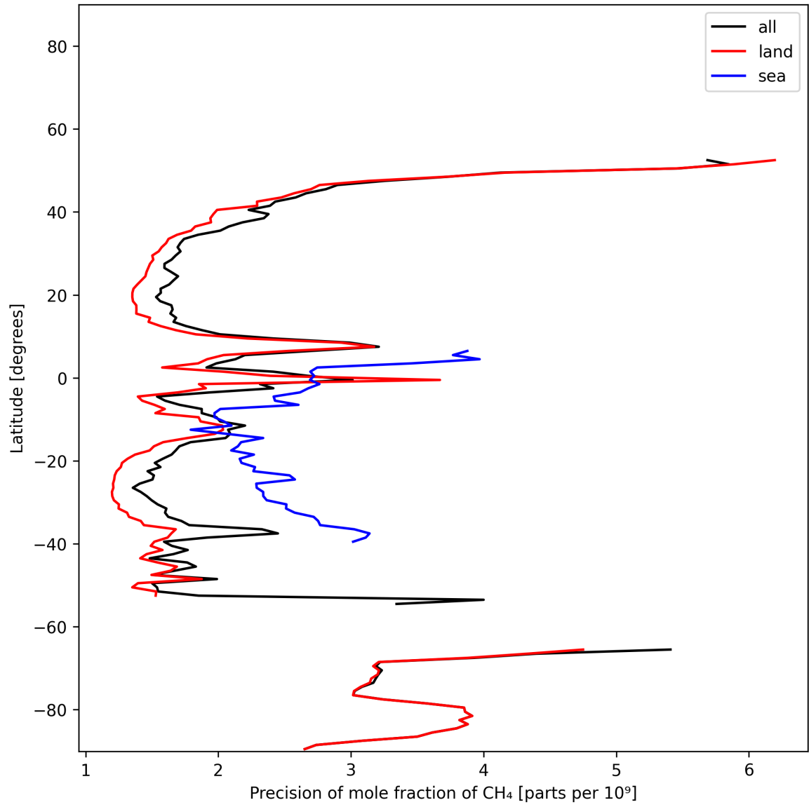
Figure 12: Zonal average of “Precision of mole fraction of CH 4 ” for 2025-12-02 to 2025-12-02.
