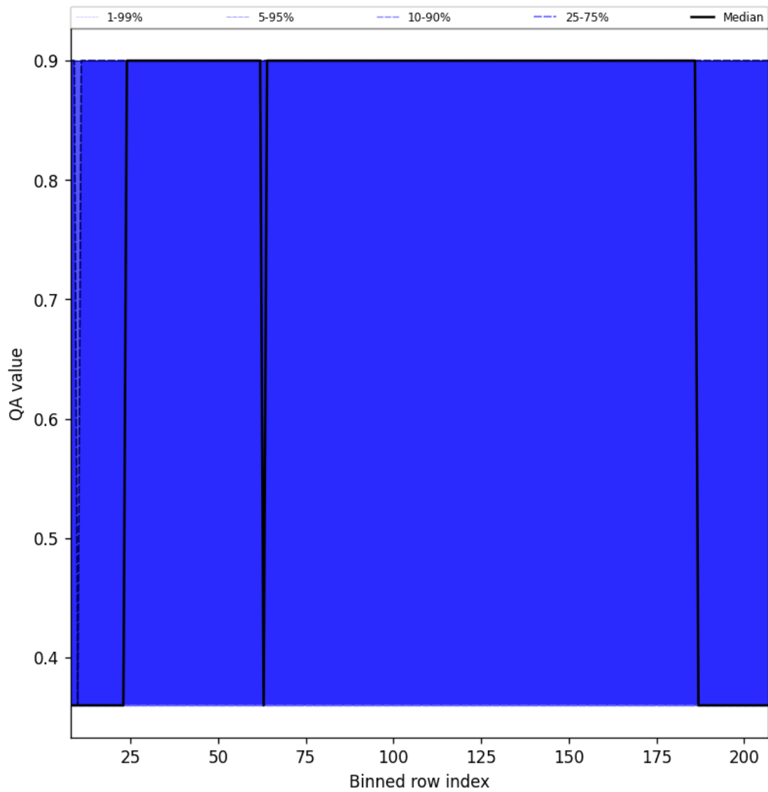
Figure 34: Along track statistics of “QA value” for 2025-12-02 to 2025-12-02
