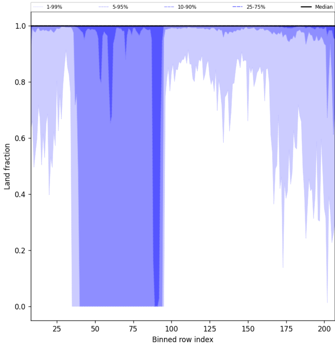
Figure 45: Along track statistics of "Land fraction" for 2025-12-02 to 2025-12-02
