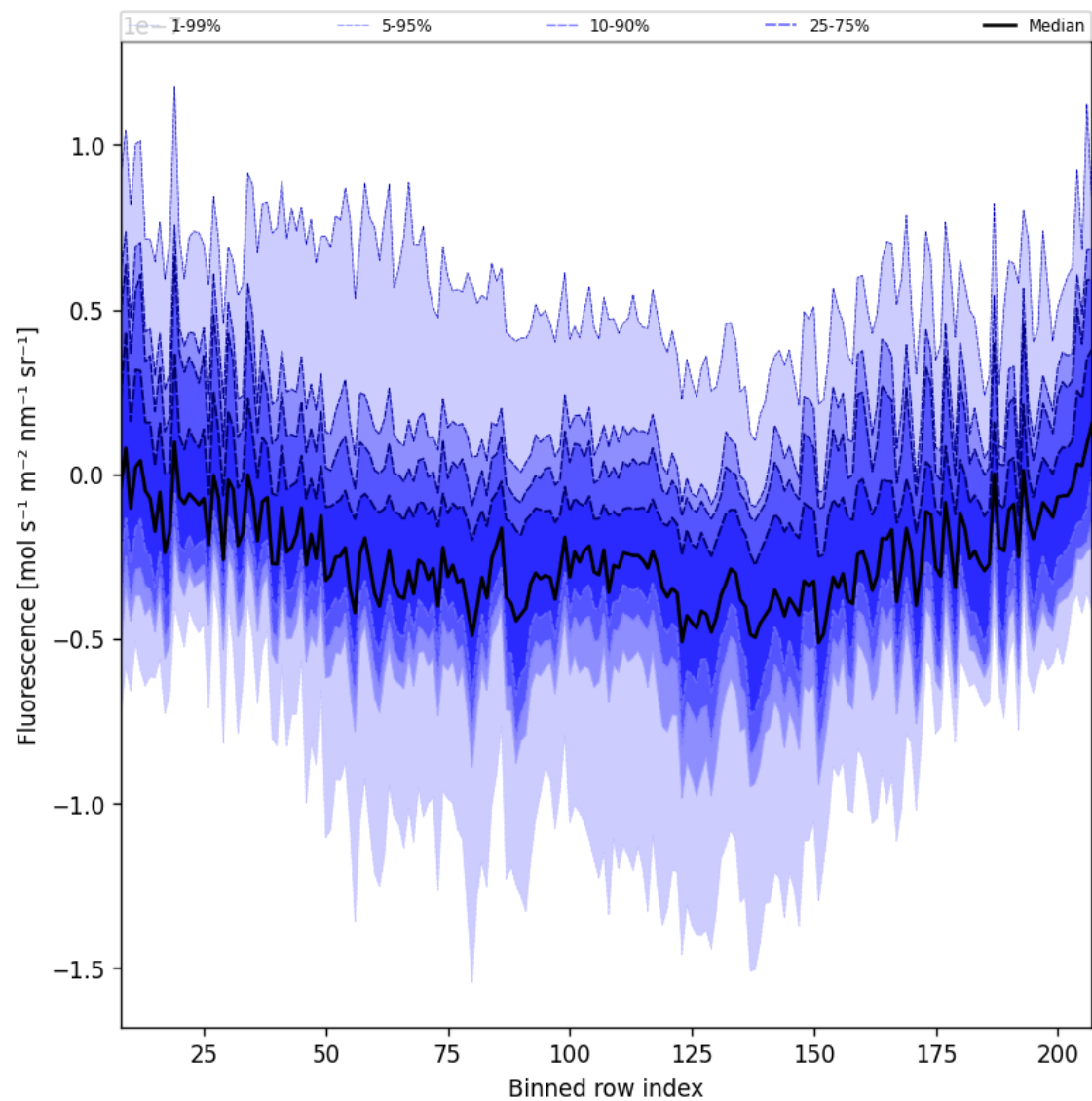
Figure 44: Along track statistics of “Fluorescence” for 2025-12-02 to 2025-12-02
