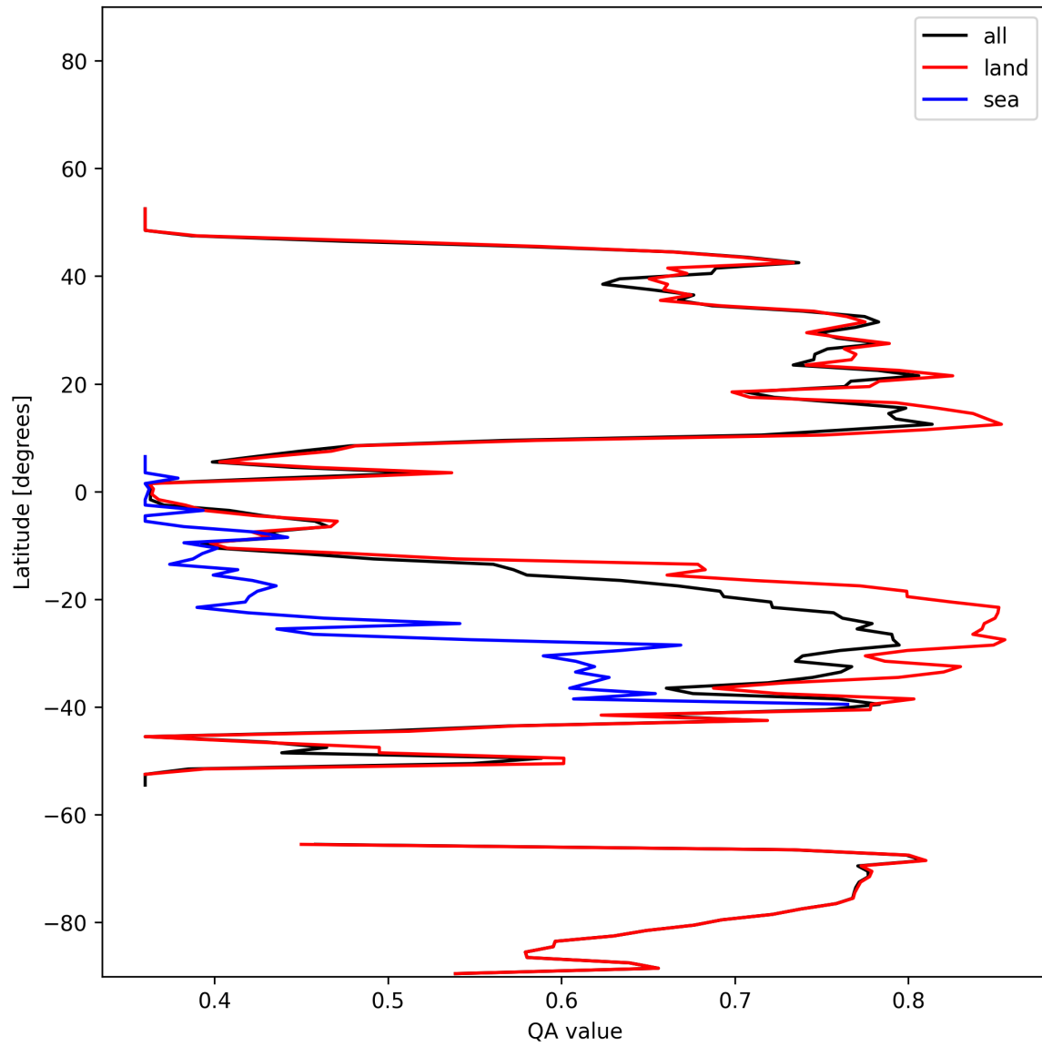
Figure 10: Zonal average of “QA value” for 2025-12-02 to 2025-12-02.
