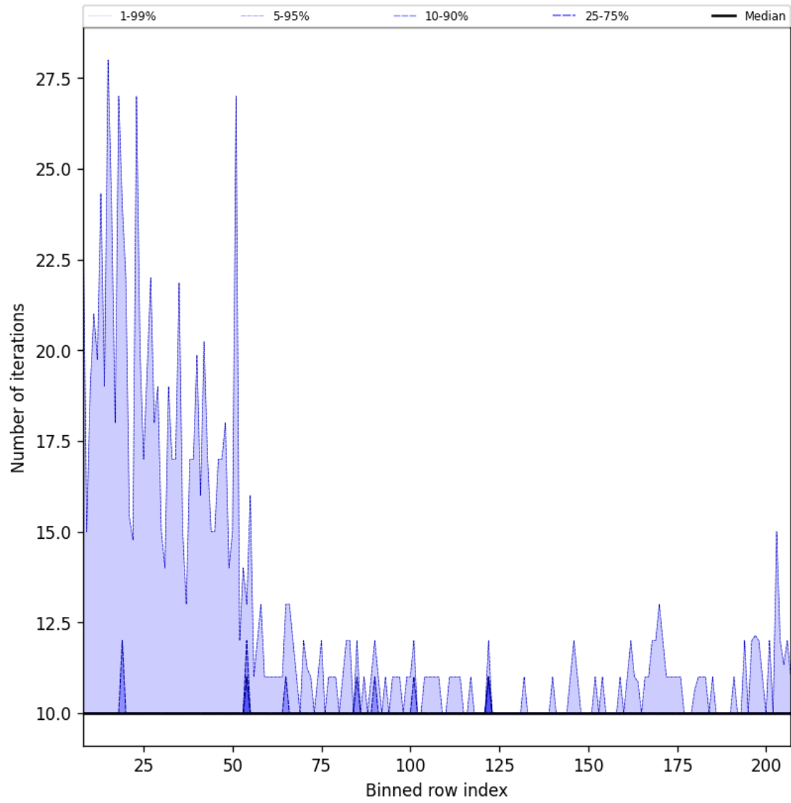
Figure 43: Along track statistics of “Number of iterations” for 2025-12-02 to 2025-12-02
