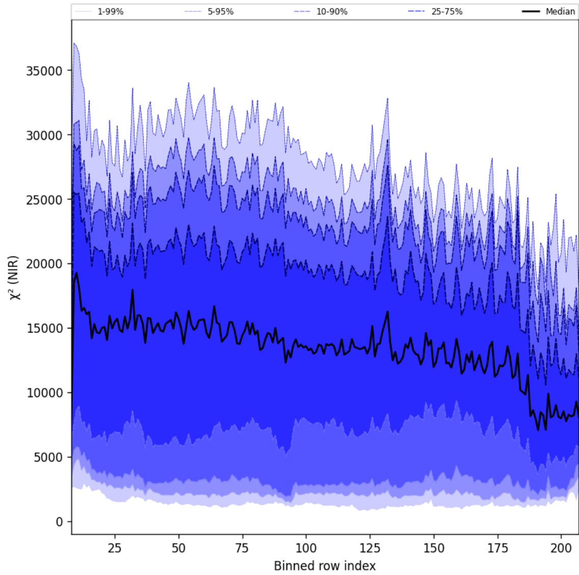
Figure 41: Along track statistics of “ \chi^2 (NIR)” for 2025-12-02 to 2025-12-02
