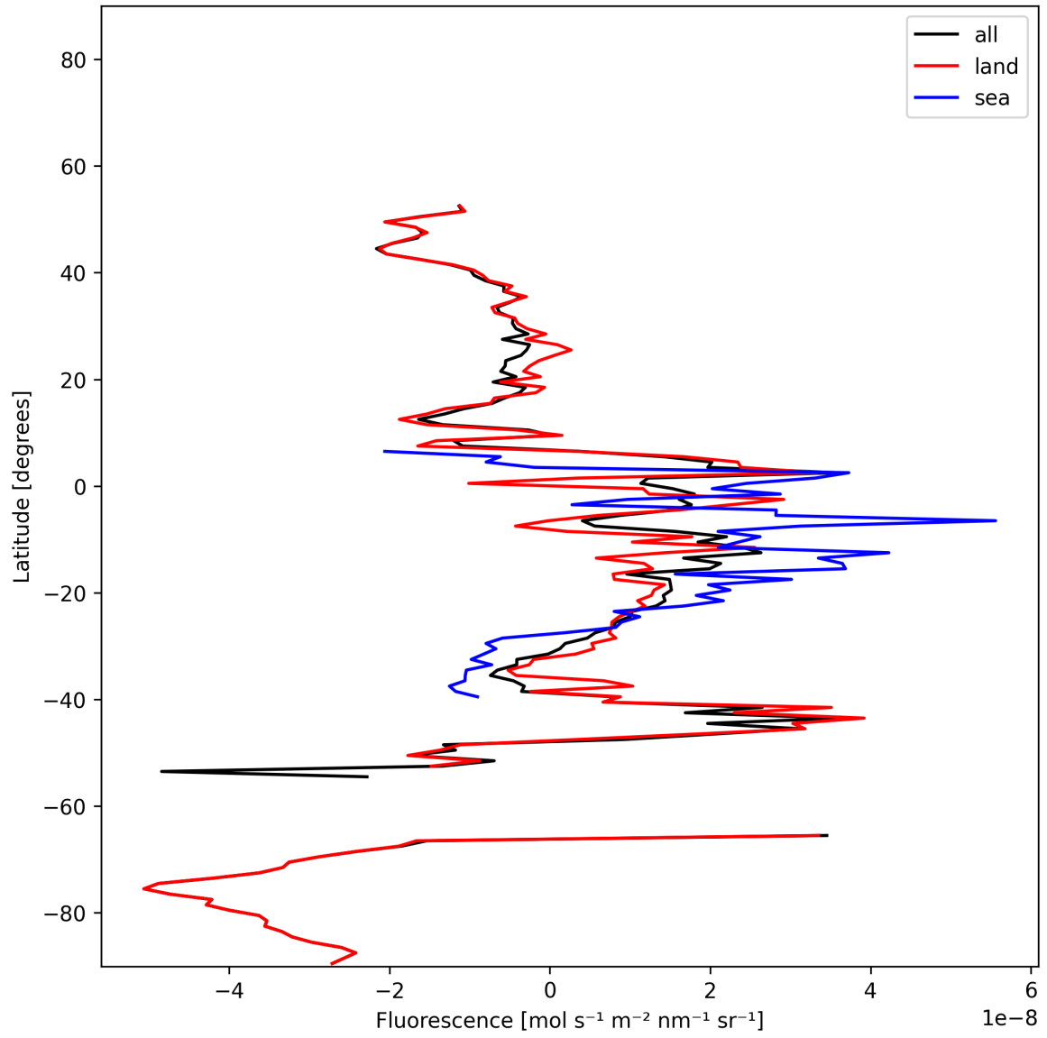
Figure 20: Zonal average of “Fluorescence” for 2025-12-02 to 2025-12-02.
