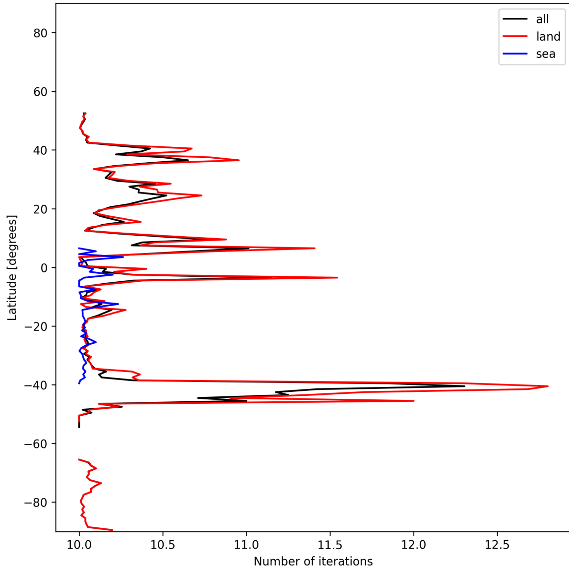
Figure 19: Zonal average of “Number of iterations” for 2025-12-02 to 2025-12-02.
