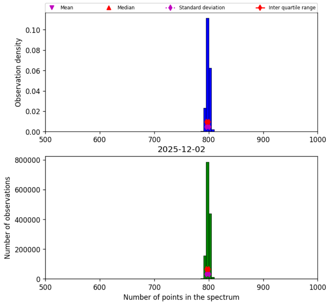
Figure 26: Histogram of “Number of points in the spectrum” for 2025-12-02 to 2025-12-02
