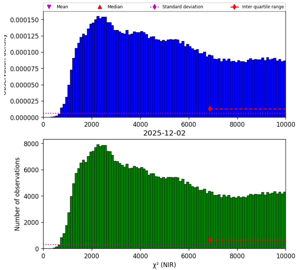
Figure 29: Histogram of “ \chi^2 (NIR)” for 2025-12-02 to 2025-12-02
