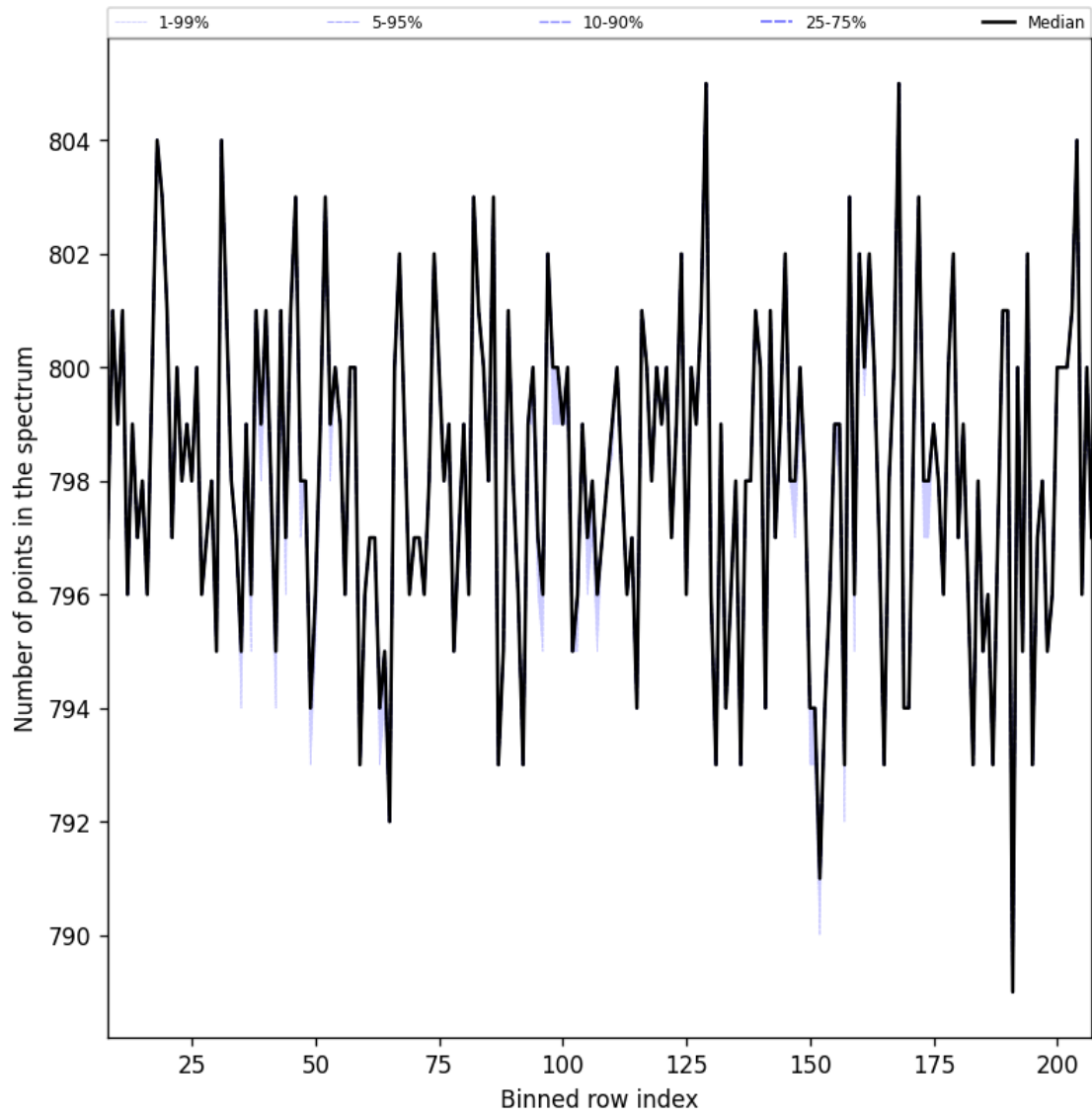
Figure 38: Along track statistics of “Number of points in the spectrum” for 2025-12-02 to 2025-12-02
