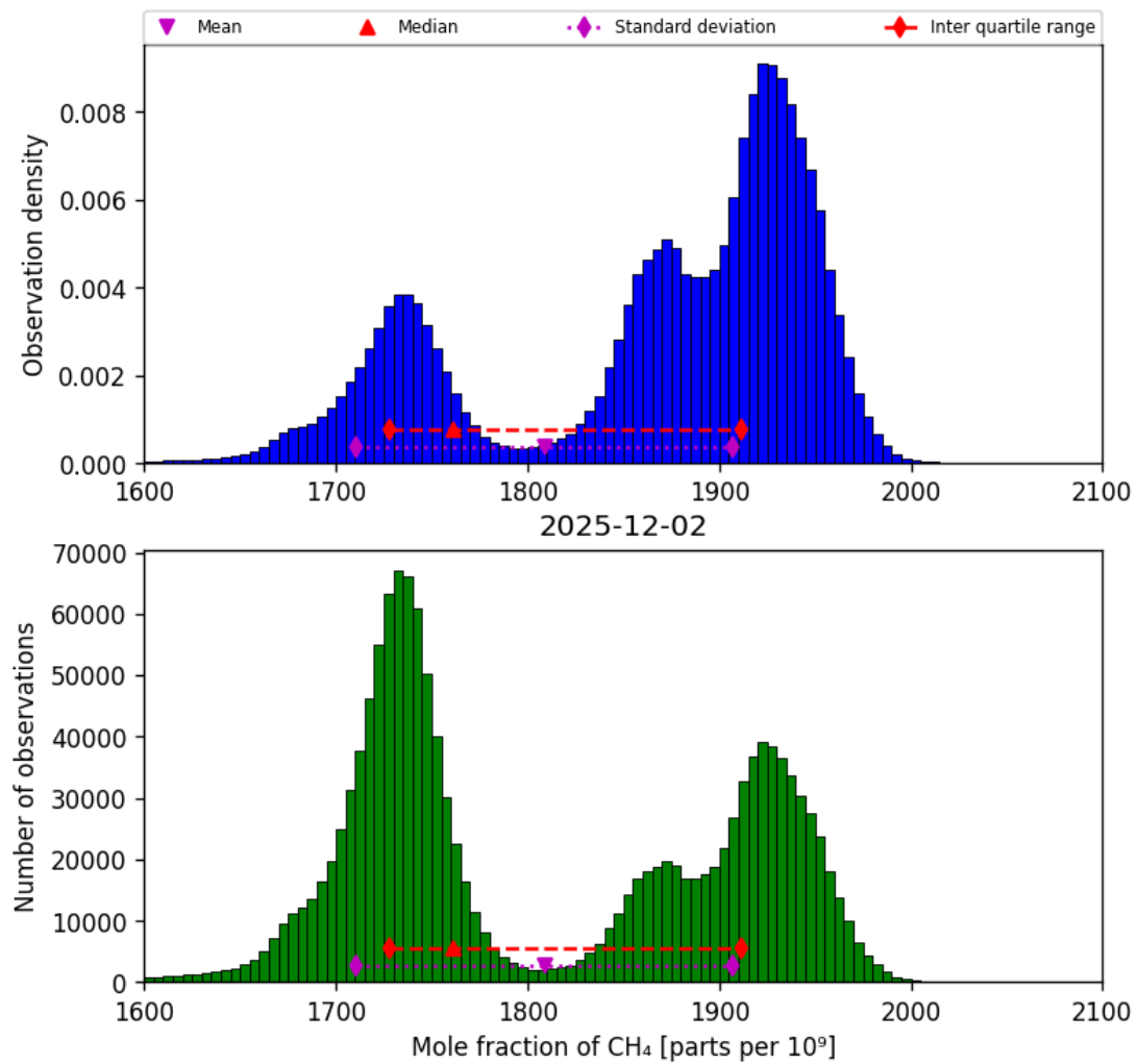
Figure 23: Histogram of “Mole fraction of CH 4 ” for 2025-12-02 to 2025-12-02
