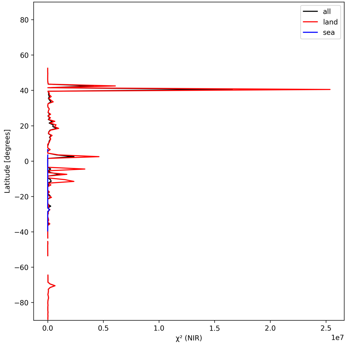
Figure 17: Zonal average of “ \chi^2 (NIR)” for 2025-12-03 to 2025-12-04.
