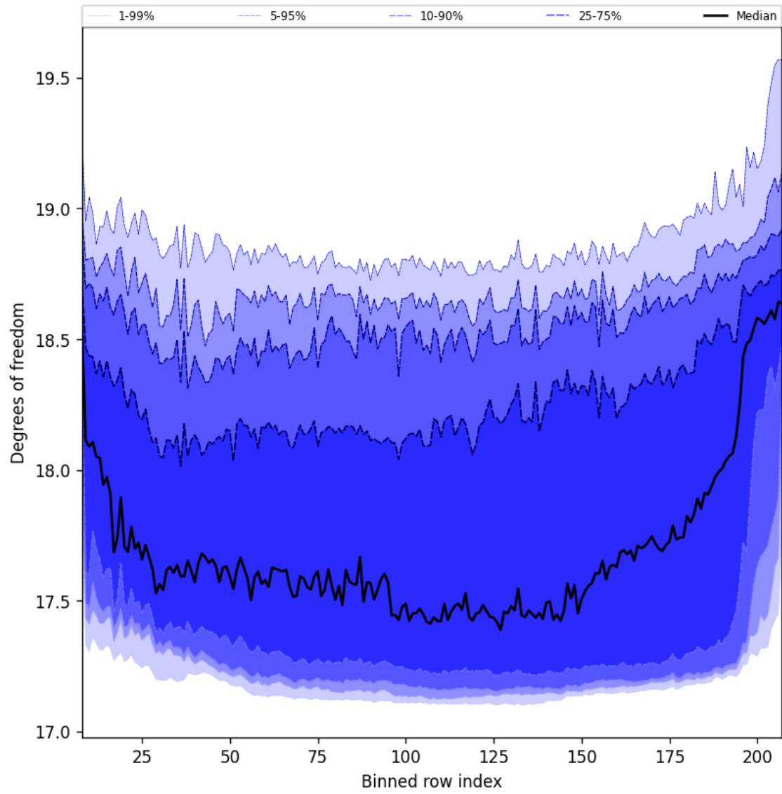
Figure 42: Along track statistics of “Degrees of freedom” for 2025-12-03 to 2025-12-04
