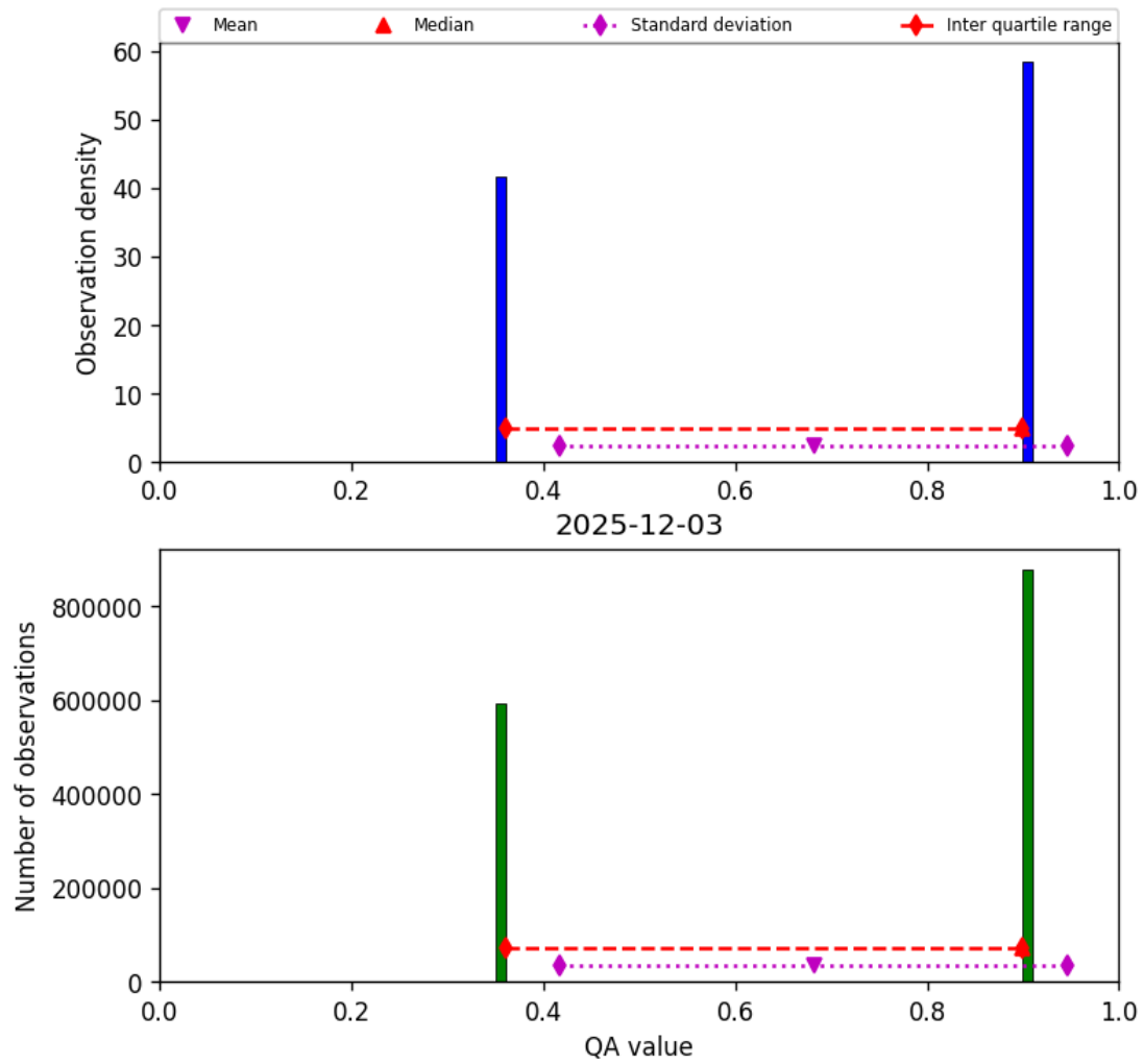
Figure 22: Histogram of “QA value” for 2025-12-03 to 2025-12-04
