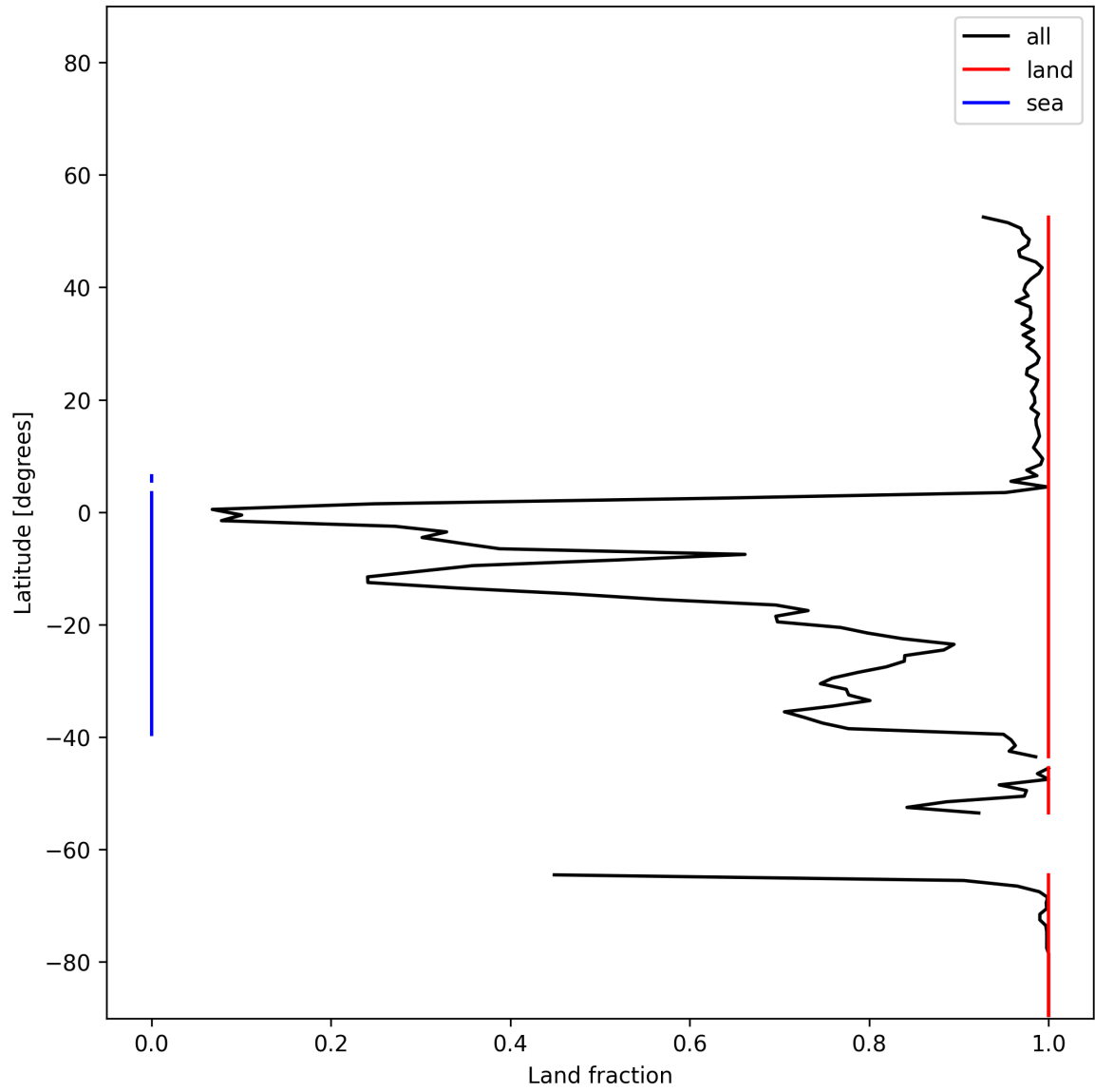
Figure 21: Zonal average of “Land fraction” for 2025-12-03 to 2025-12-04.
