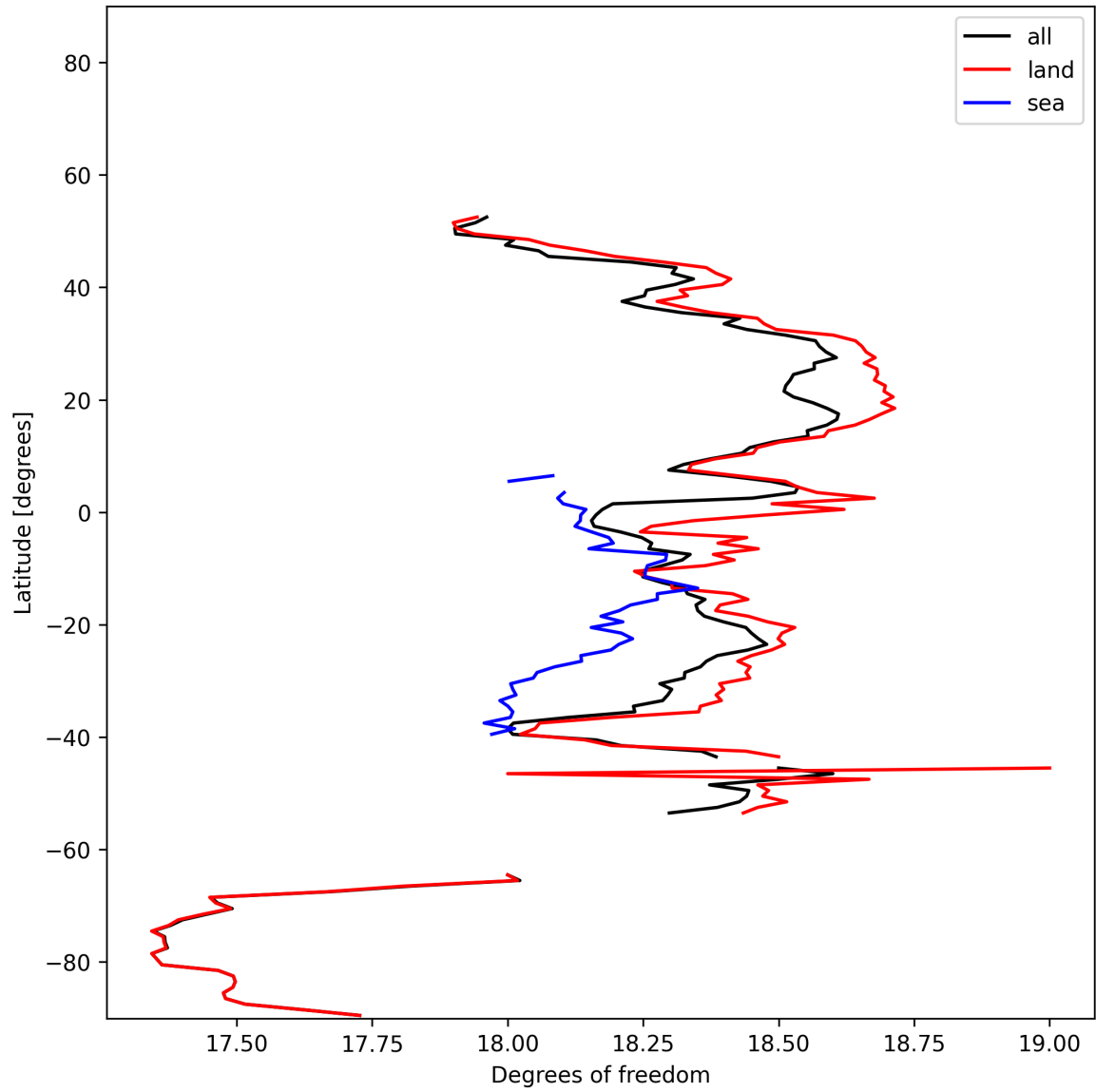
Figure 18: Zonal average of “Degrees of freedom” for 2025-12-03 to 2025-12-04.
