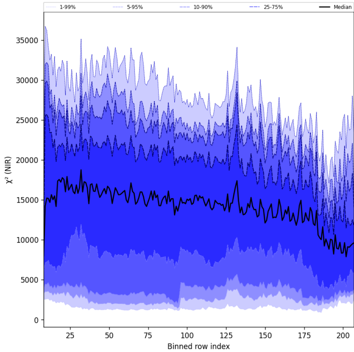
Figure 41: Along track statistics of “ \chi^2 (NIR)” for 2025-12-03 to 2025-12-04
