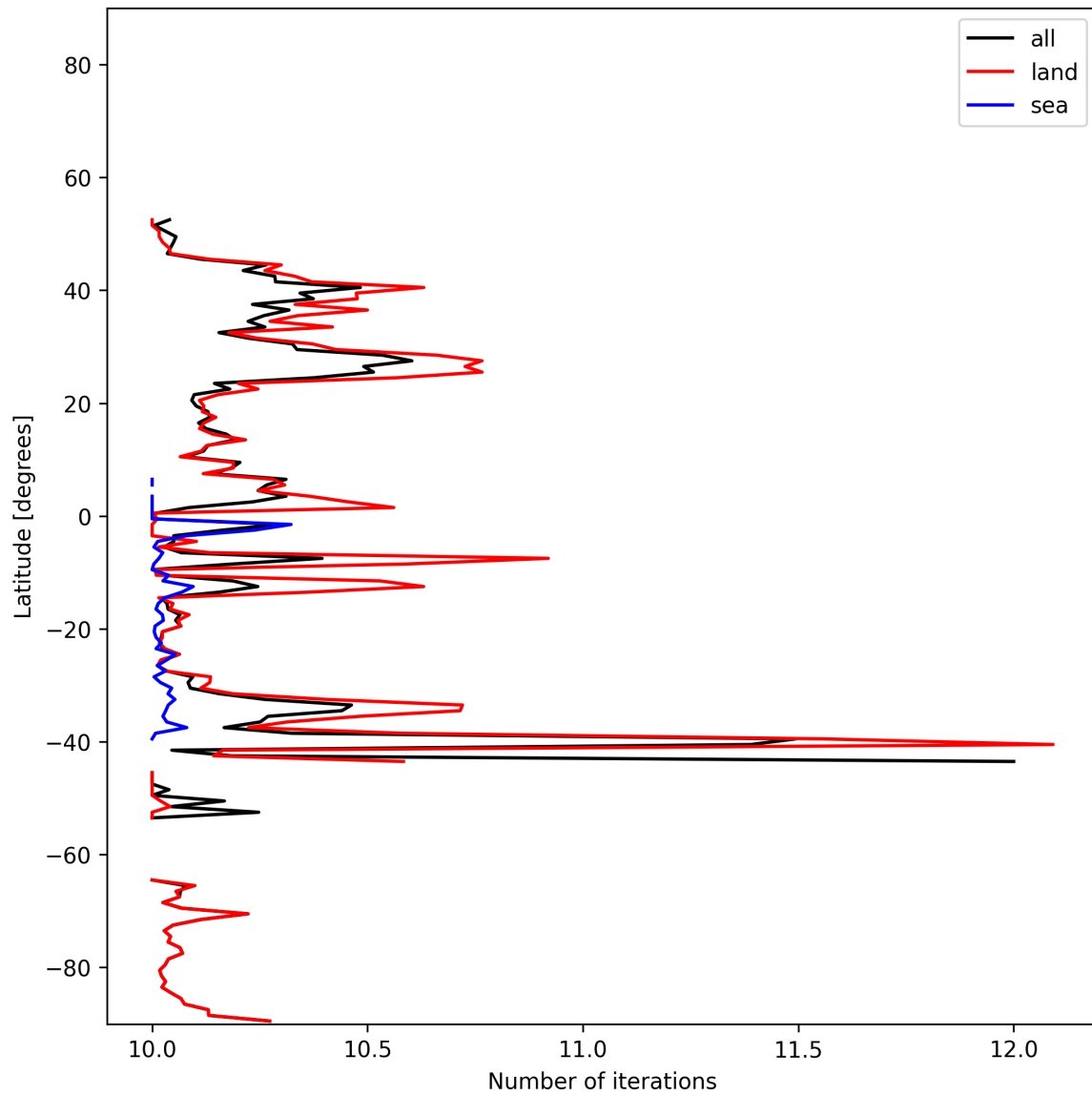
Figure 19: Zonal average of “Number of iterations” for 2025-12-03 to 2025-12-04.
