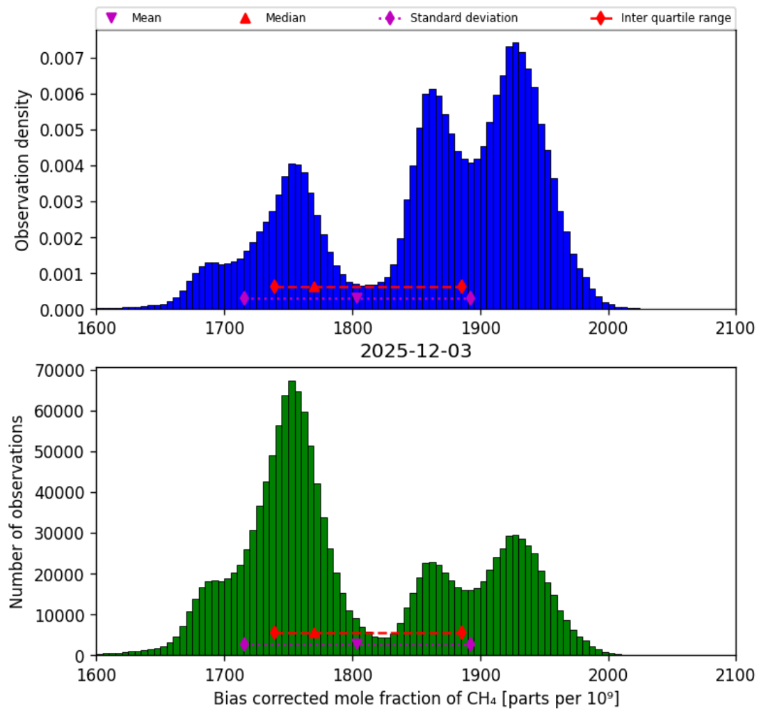
Figure 25: Histogram of “Bias corrected mole fraction of CH 4 ” for 2025-12-03 to 2025-12-04
