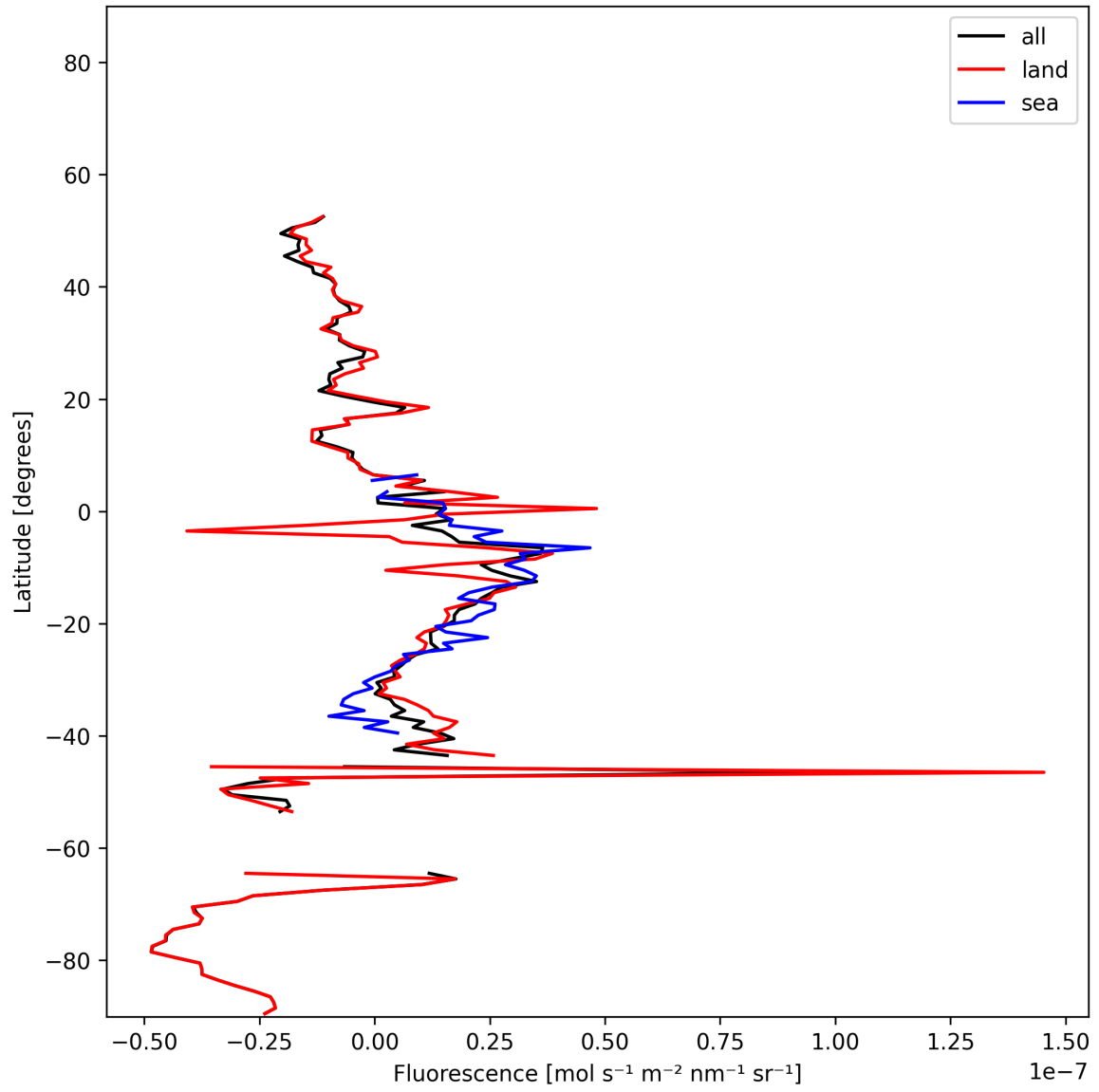
Figure 20: Zonal average of “Fluorescence” for 2025-12-03 to 2025-12-04.
