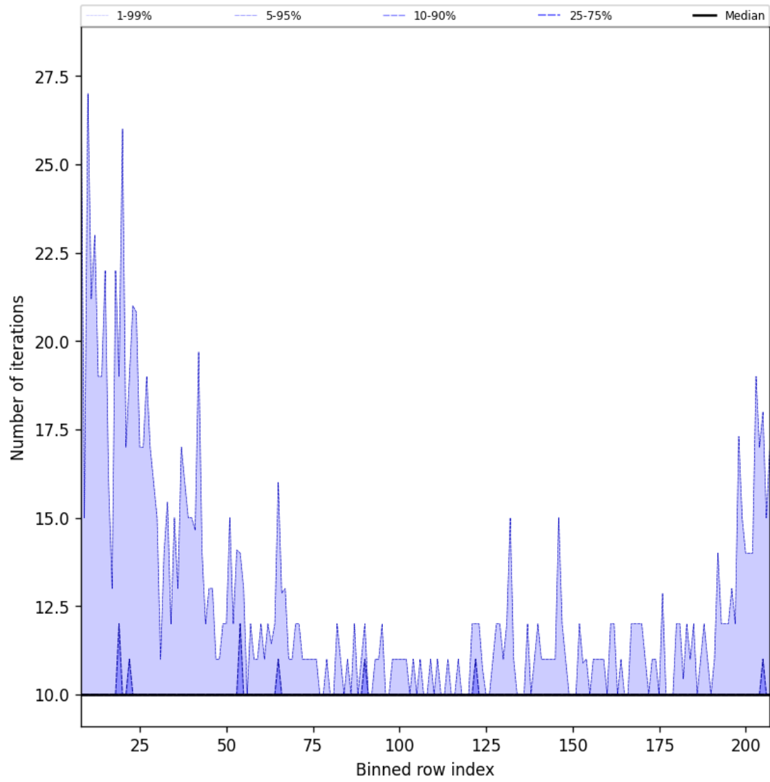
Figure 43: Along track statistics of “Number of iterations” for 2025-12-03 to 2025-12-04
