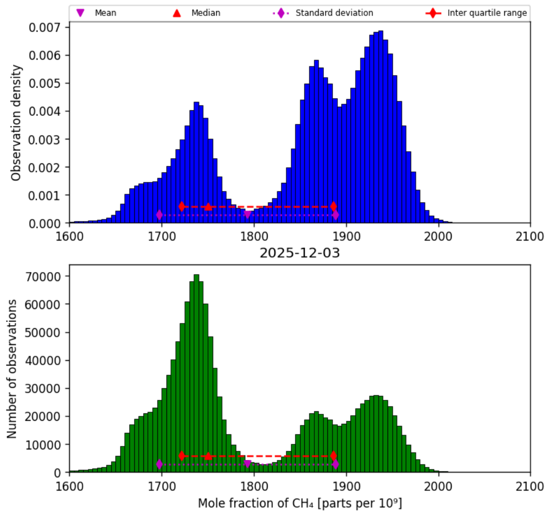
Figure 23: Histogram of “Mole fraction of CH 4 ” for 2025-12-03 to 2025-12-04
