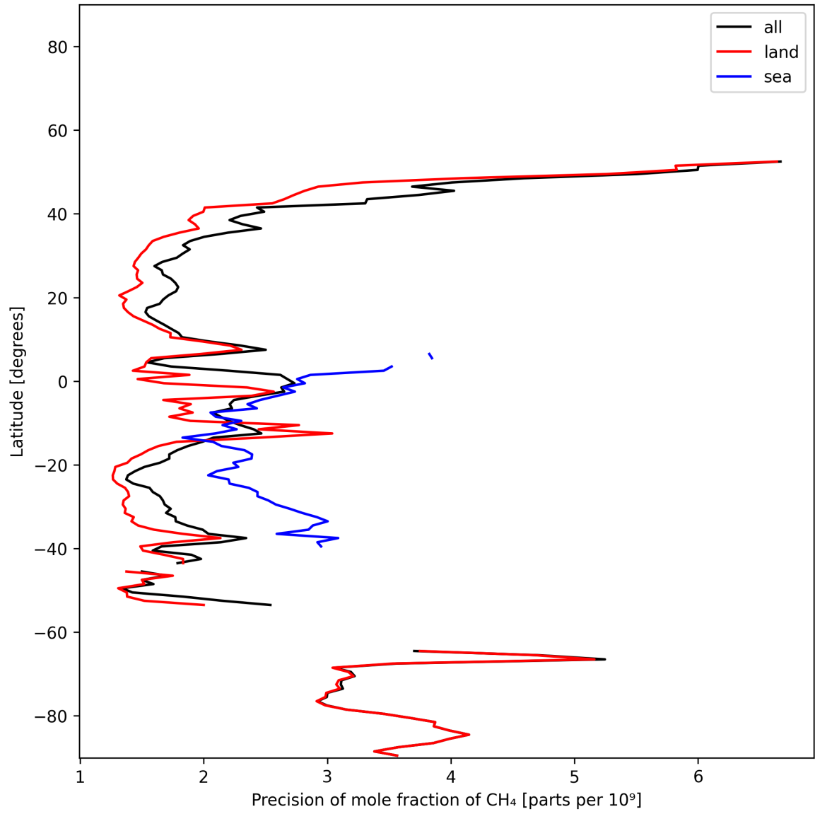
Figure 12: Zonal average of “Precision of mole fraction of CH 4 ” for 2025-12-03 to 2025-12-04.
