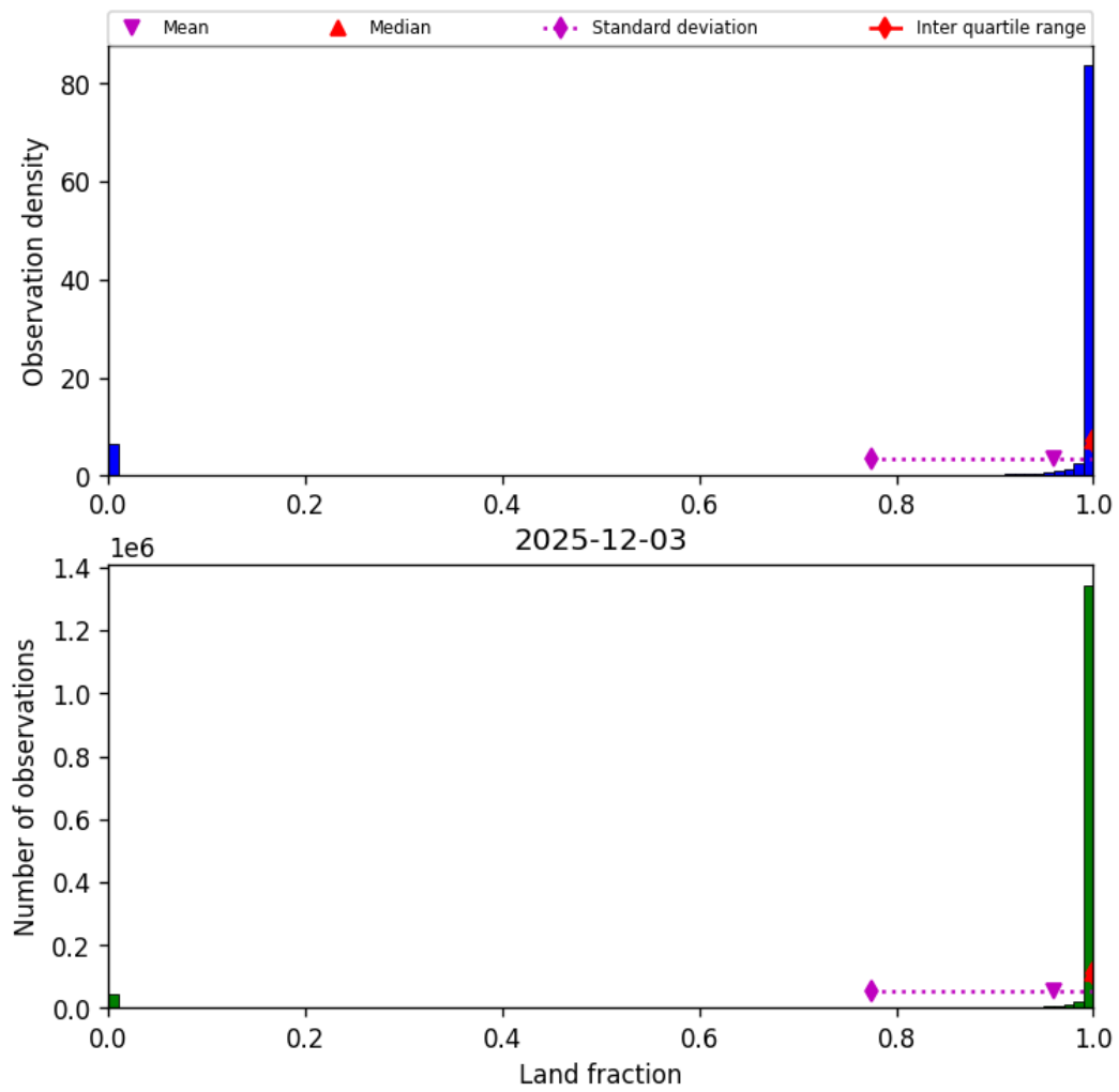
Figure 33: Histogram of “Land fraction” for 2025-12-03 to 2025-12-04
