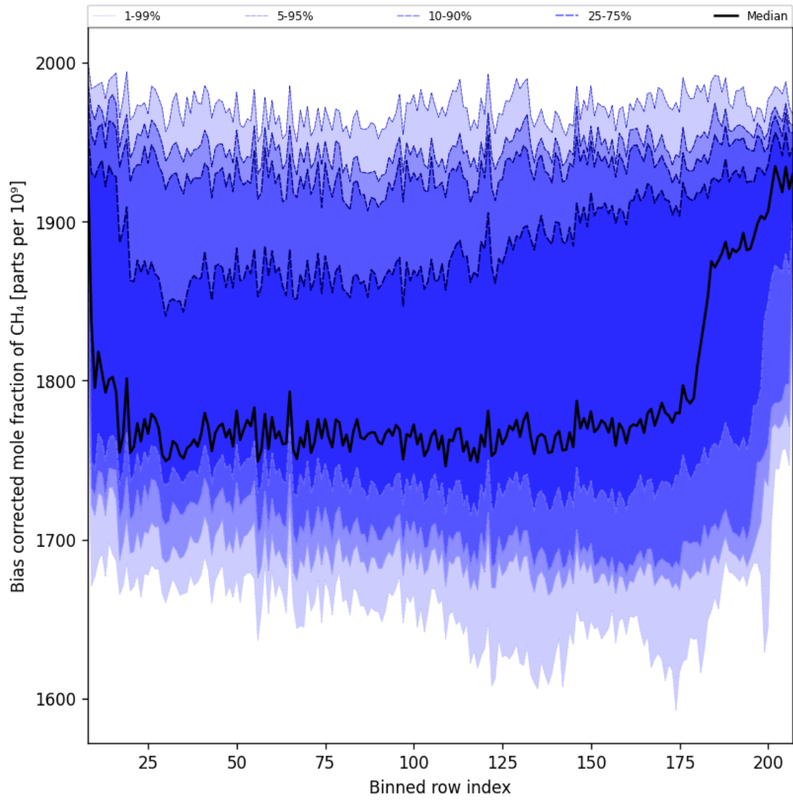
Figure 37: Along track statistics of “Bias corrected mole fraction of CH 4 ” for 2025-12-03 to 2025-12-04
