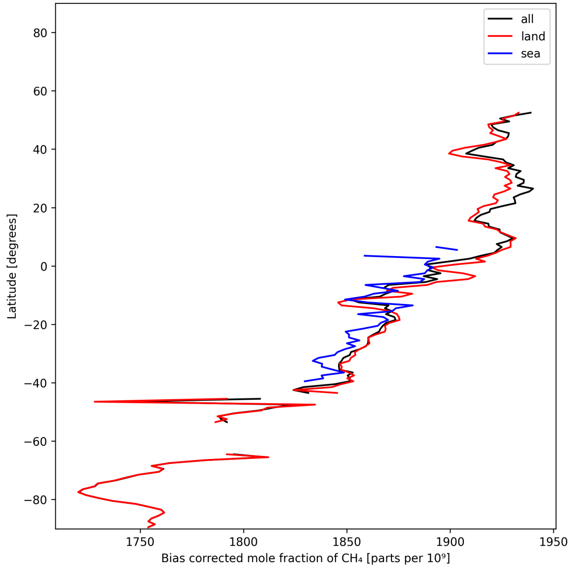
Figure 13: Zonal average of “Bias corrected mole fraction of CH 4 ” for 2025-12-03 to 2025-12-04.
