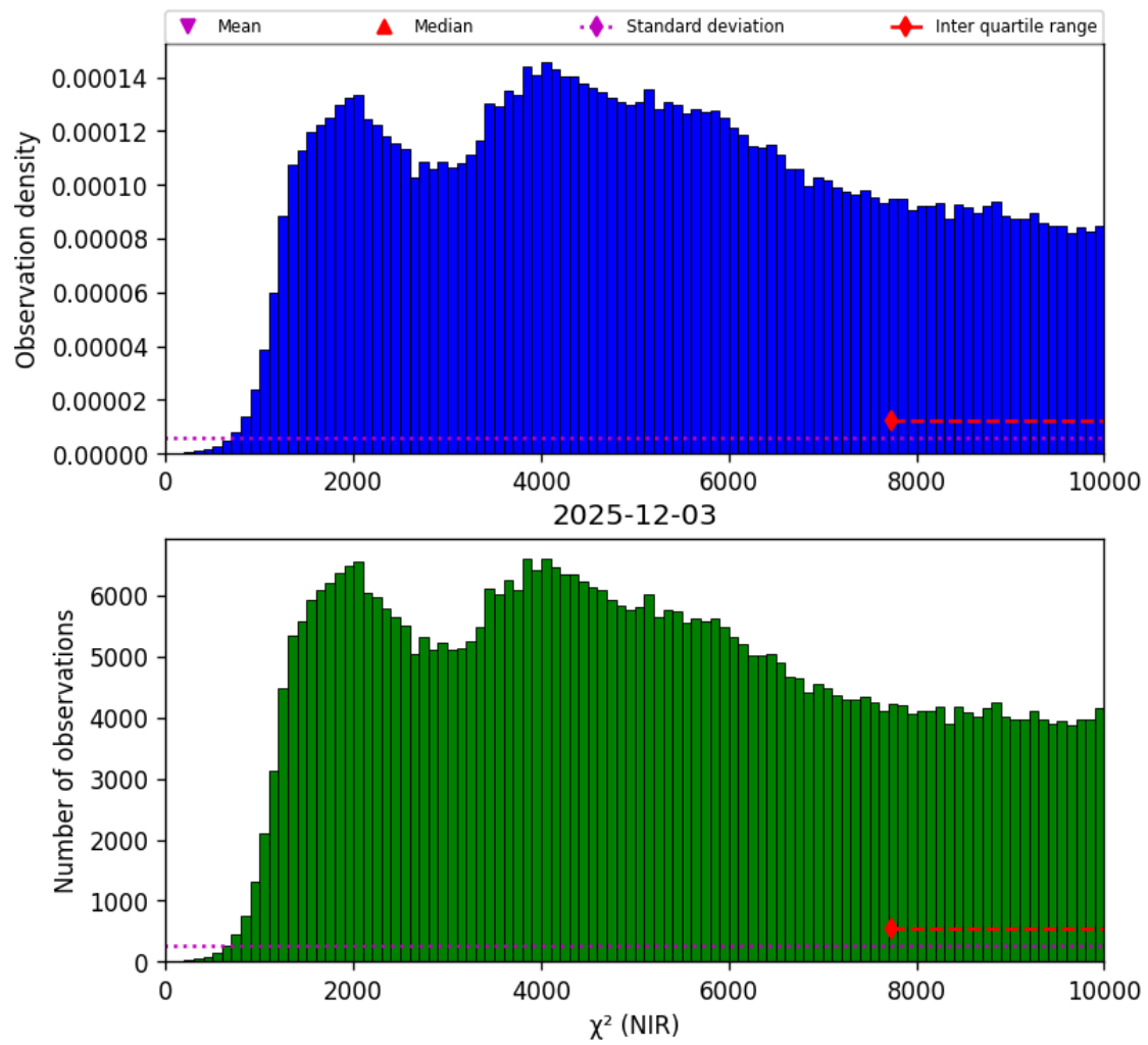
Figure 29: Histogram of " \chi^2 (NIR)" for 2025-12-03 to 2025-12-04
