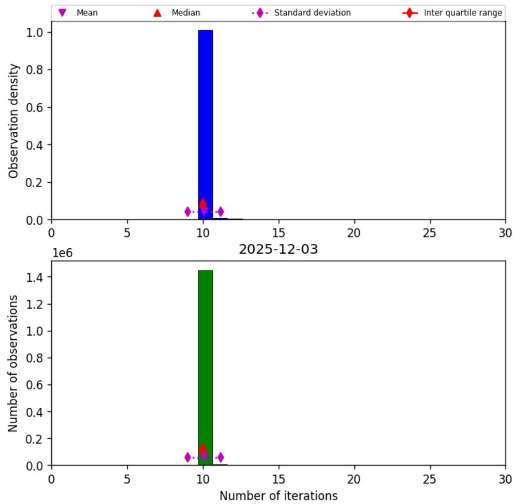
Figure 31: Histogram of “Number of iterations” for 2025-12-03 to 2025-12-04
