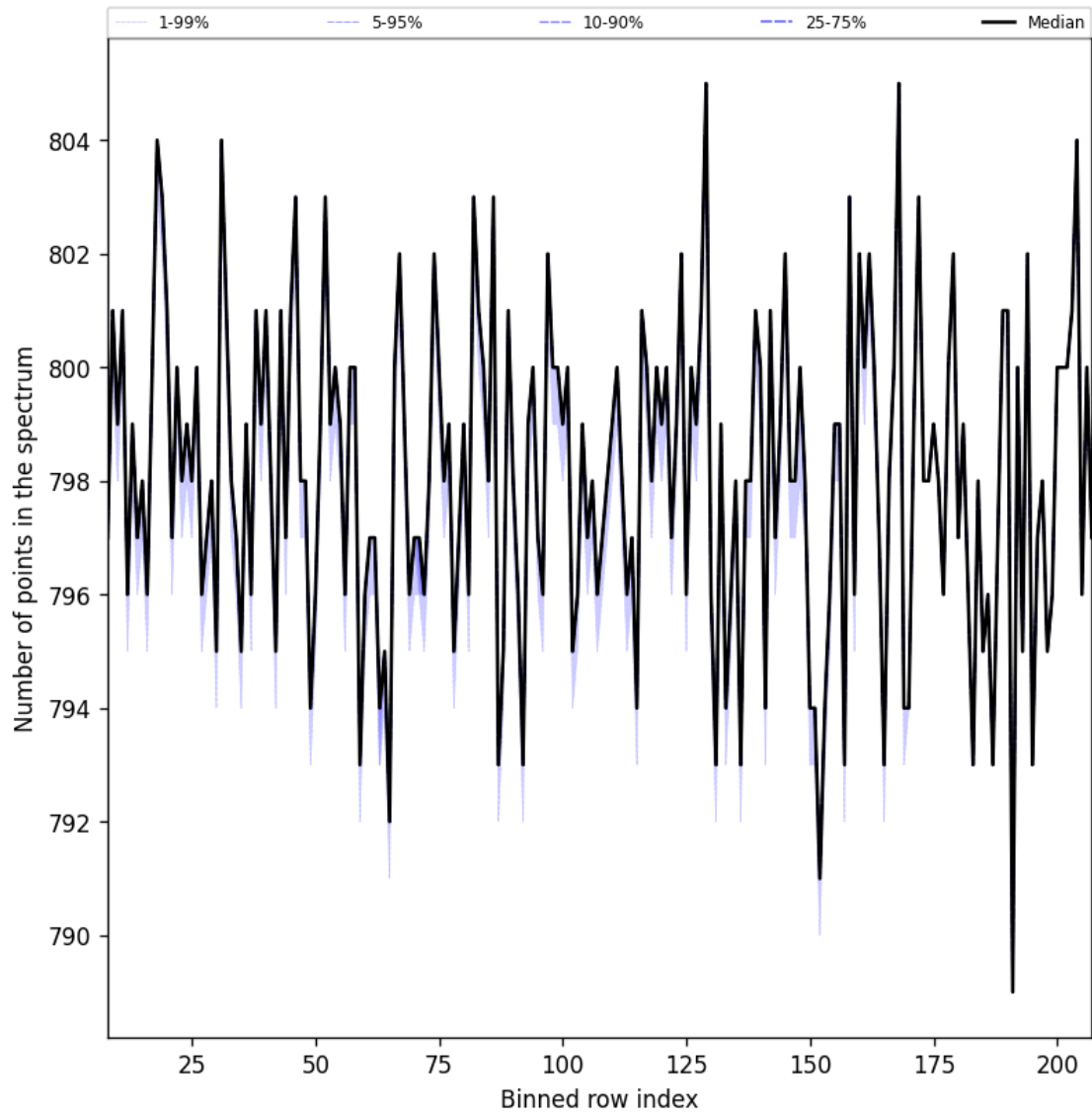
Figure 38: Along track statistics of “Number of points in the spectrum” for 2025-12-03 to 2025-12-04
