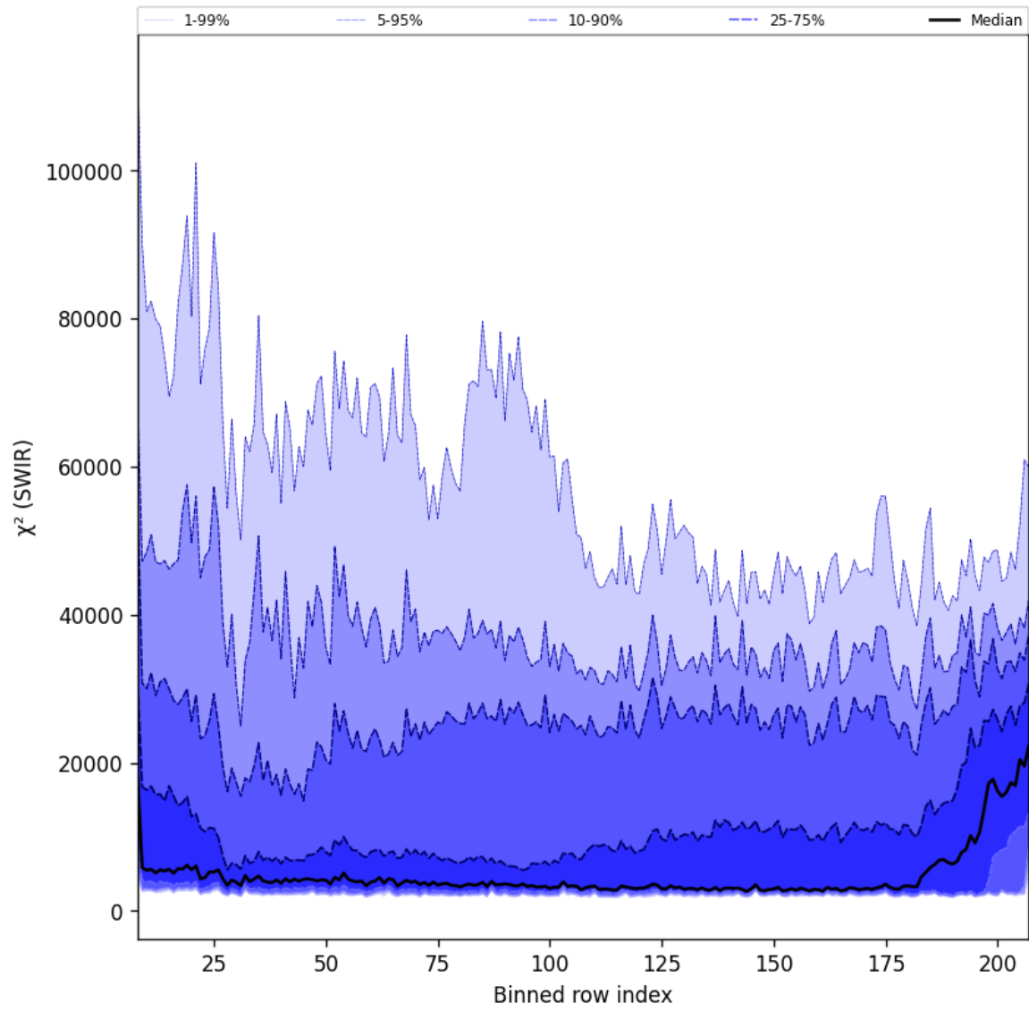
Figure 40: Along track statistics of “ \chi^2 (SWIR)” for 2025-12-03 to 2025-12-04
