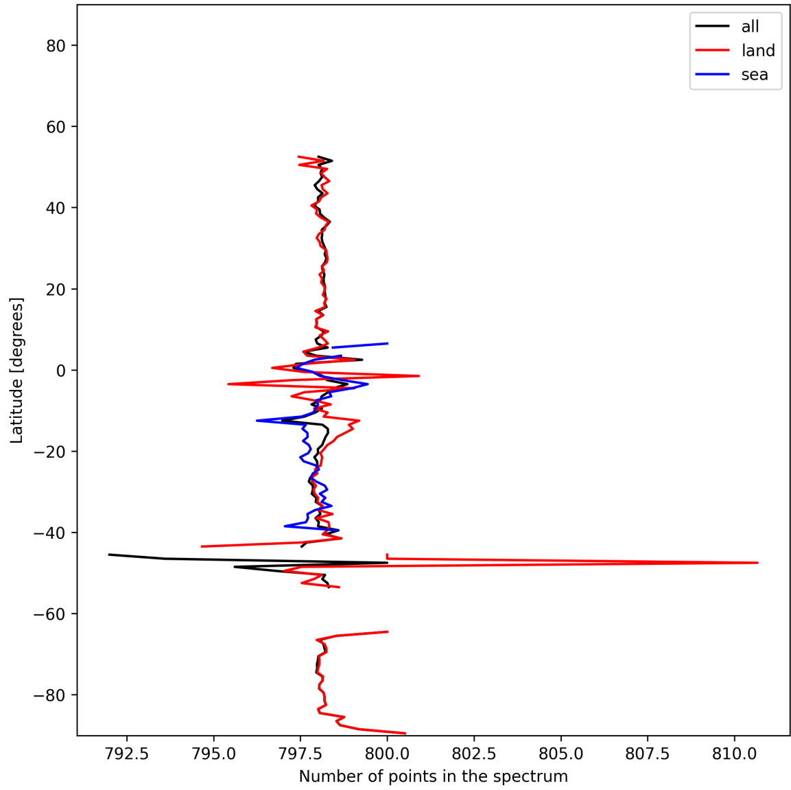
Figure 14: Zonal average of “Number of points in the spectrum” for 2025-12-03 to 2025-12-04.
