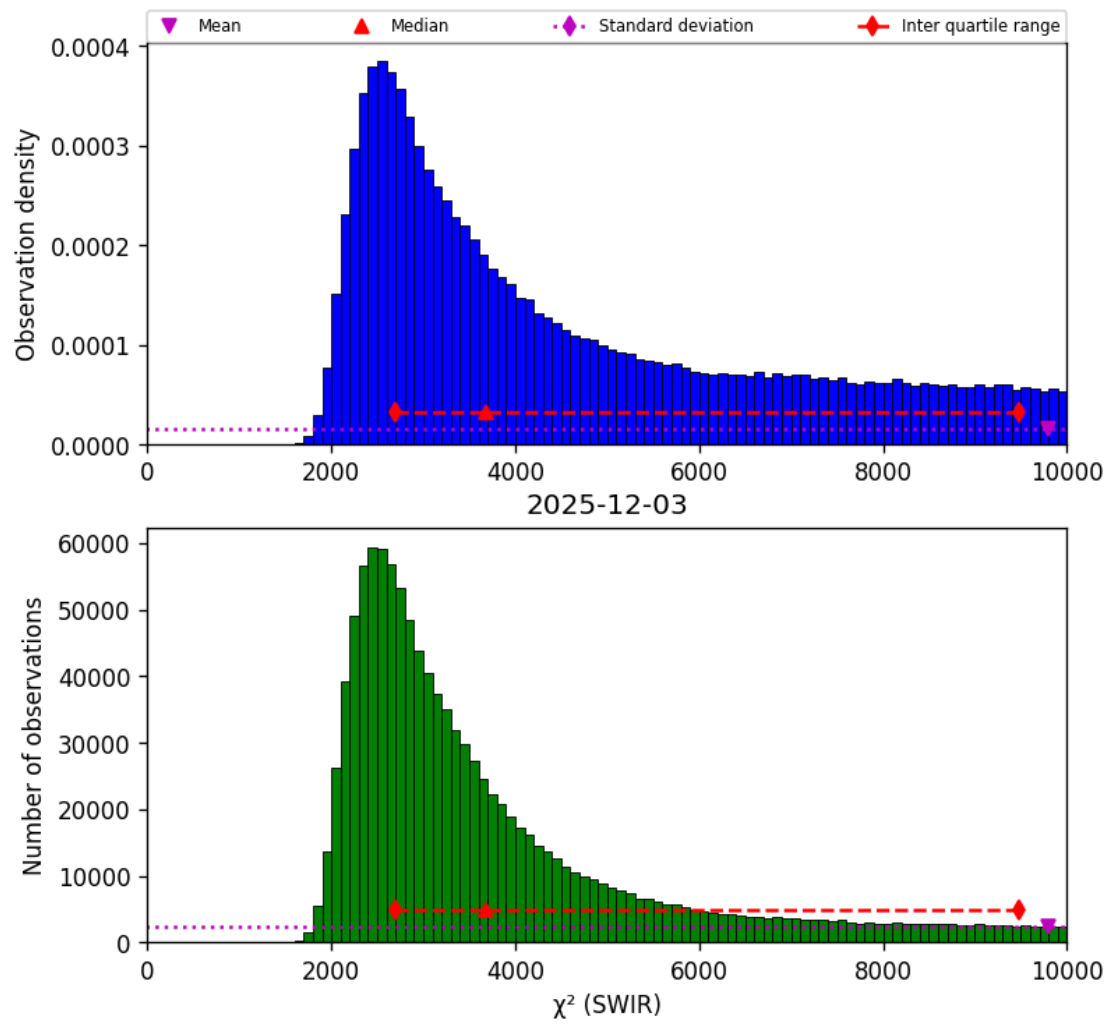
Figure 28: Histogram of " \chi^2 (SWIR)" for 2025-12-03 to 2025-12-04
