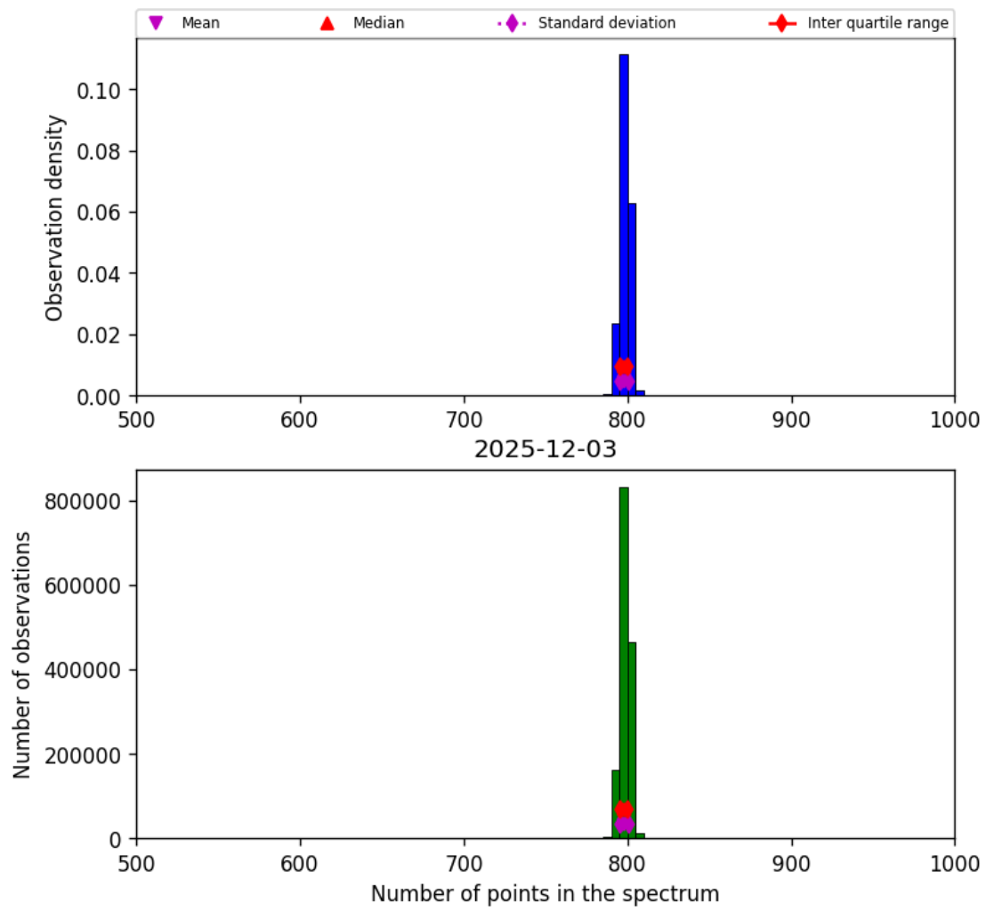
Figure 26: Histogram of “Number of points in the spectrum” for 2025-12-03 to 2025-12-04
