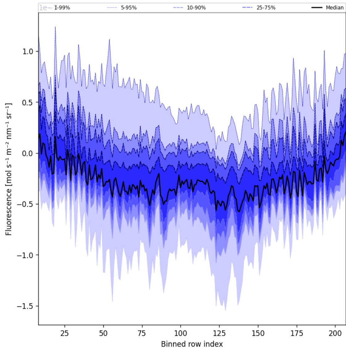
Figure 44: Along track statistics of “Fluorescence” for 2025-12-03 to 2025-12-04
