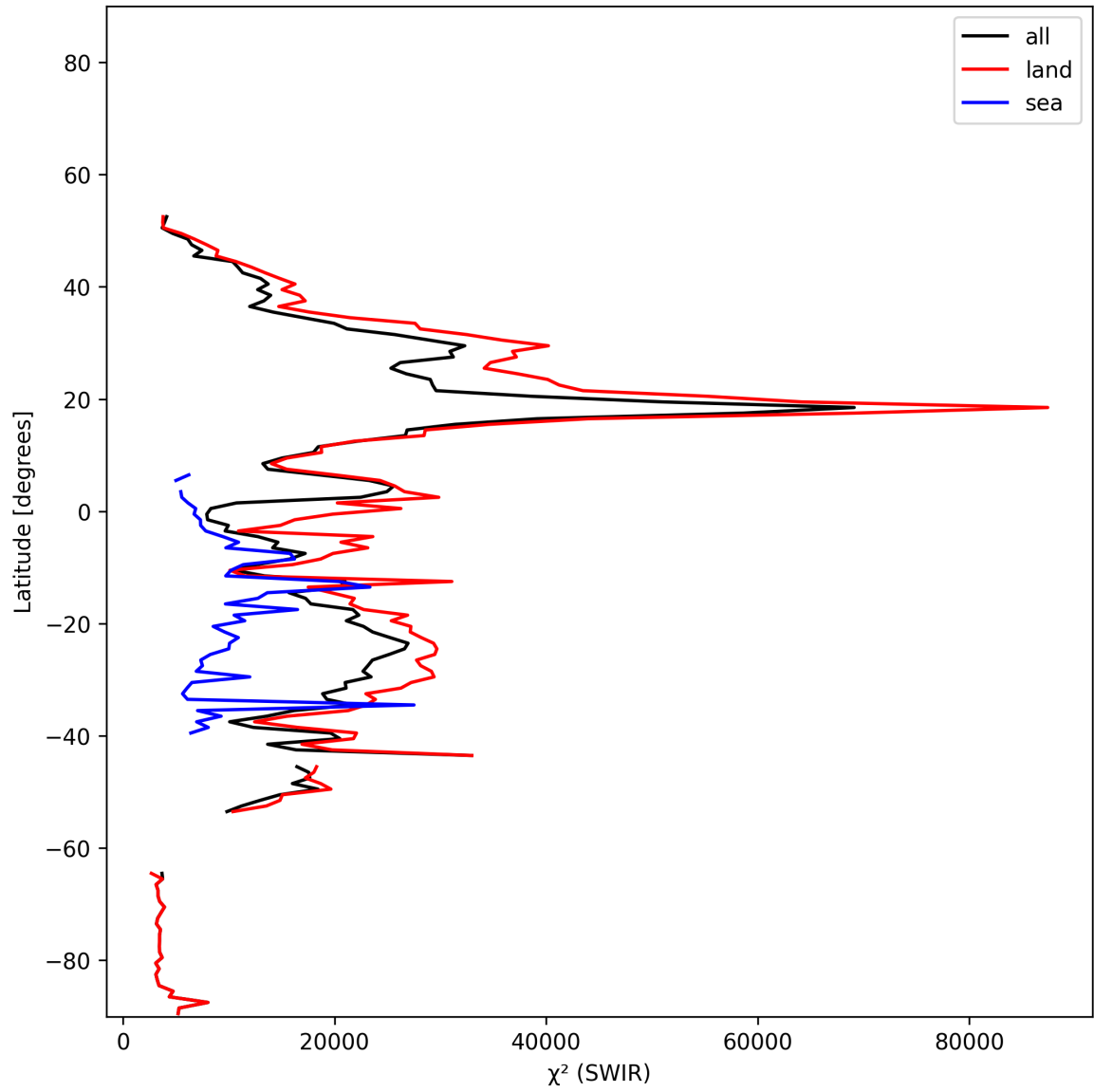
Figure 16: Zonal average of “ \chi^2 (SWIR)” for 2025-12-03 to 2025-12-04.
