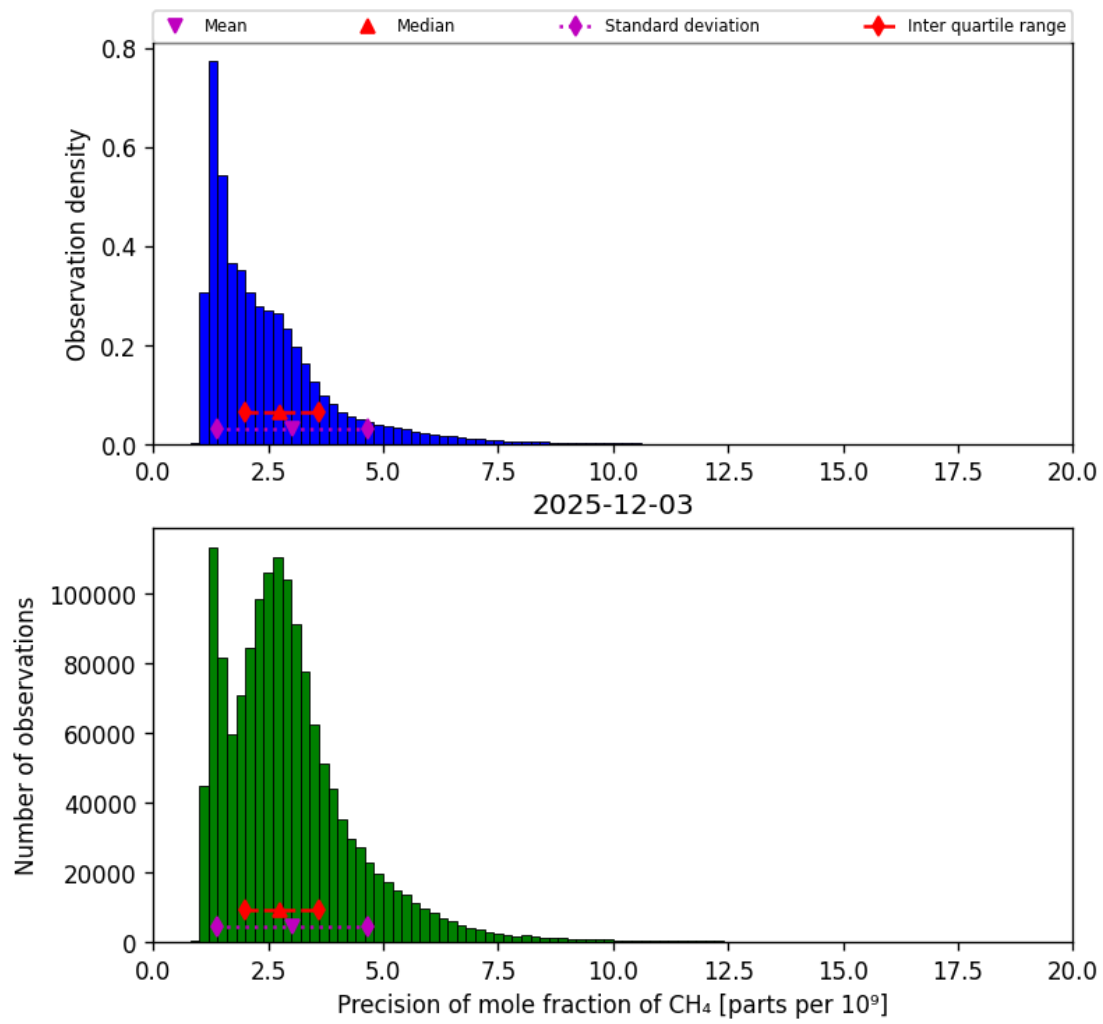
Figure 24: Histogram of “Precision of mole fraction of CH 4 ” for 2025-12-03 to 2025-12-04
