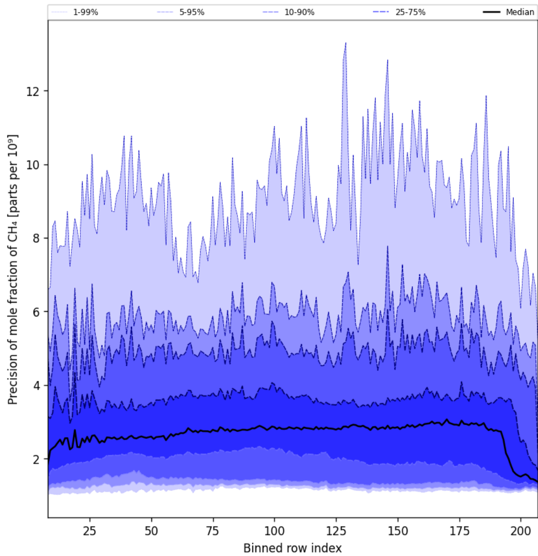
Figure 36: Along track statistics of “Precision of mole fraction of CH 4 ” for 2025-12-03 to 2025-12-04
