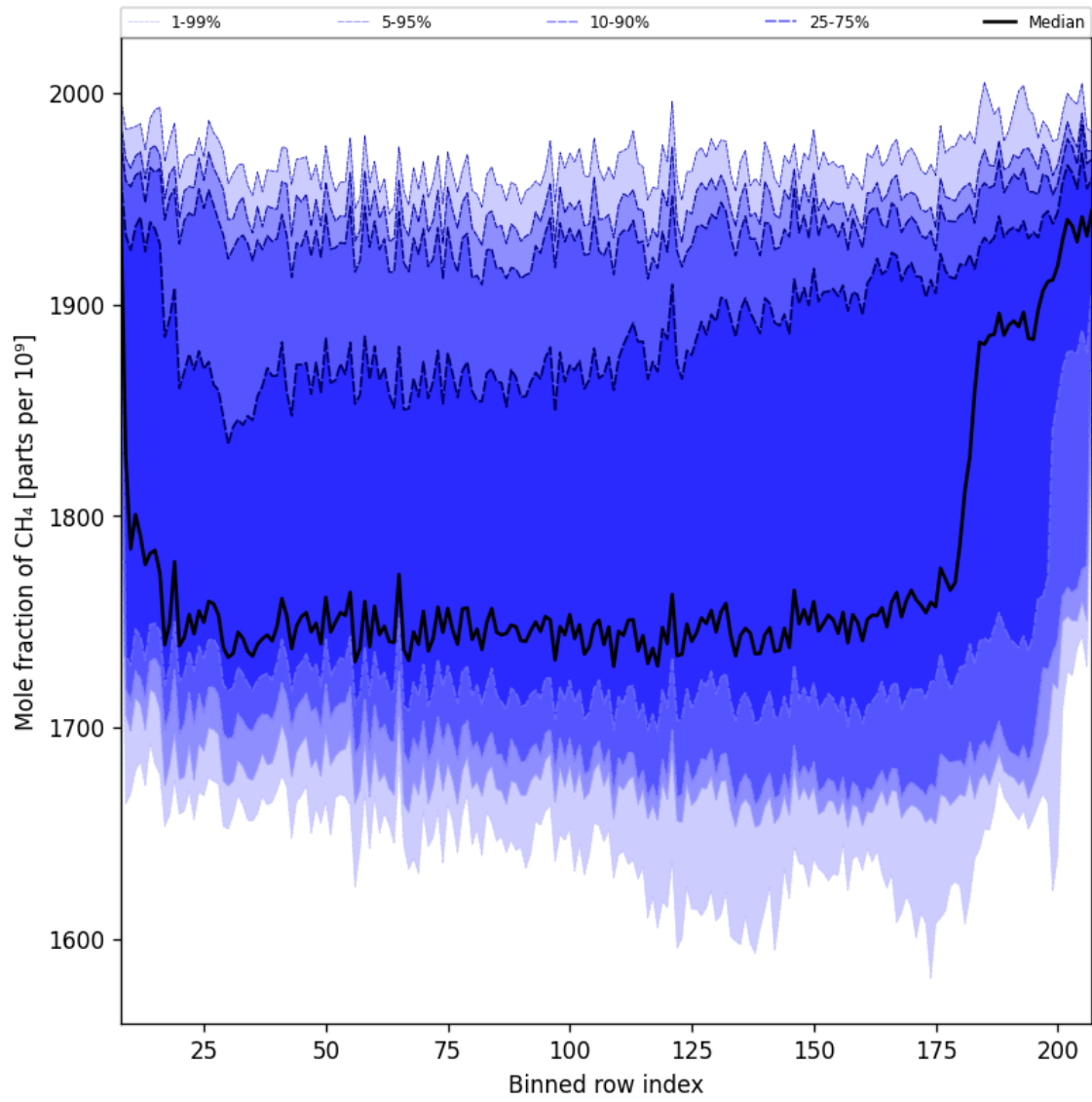
Figure 35: Along track statistics of “Mole fraction of CH 4 ” for 2025-12-03 to 2025-12-04
