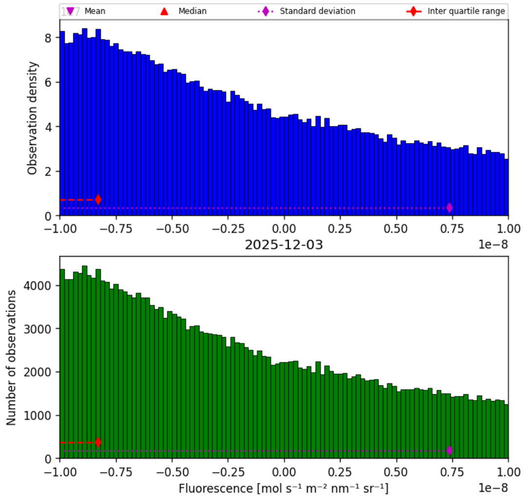
Figure 32: Histogram of “Fluorescence” for 2025-12-03 to 2025-12-04
