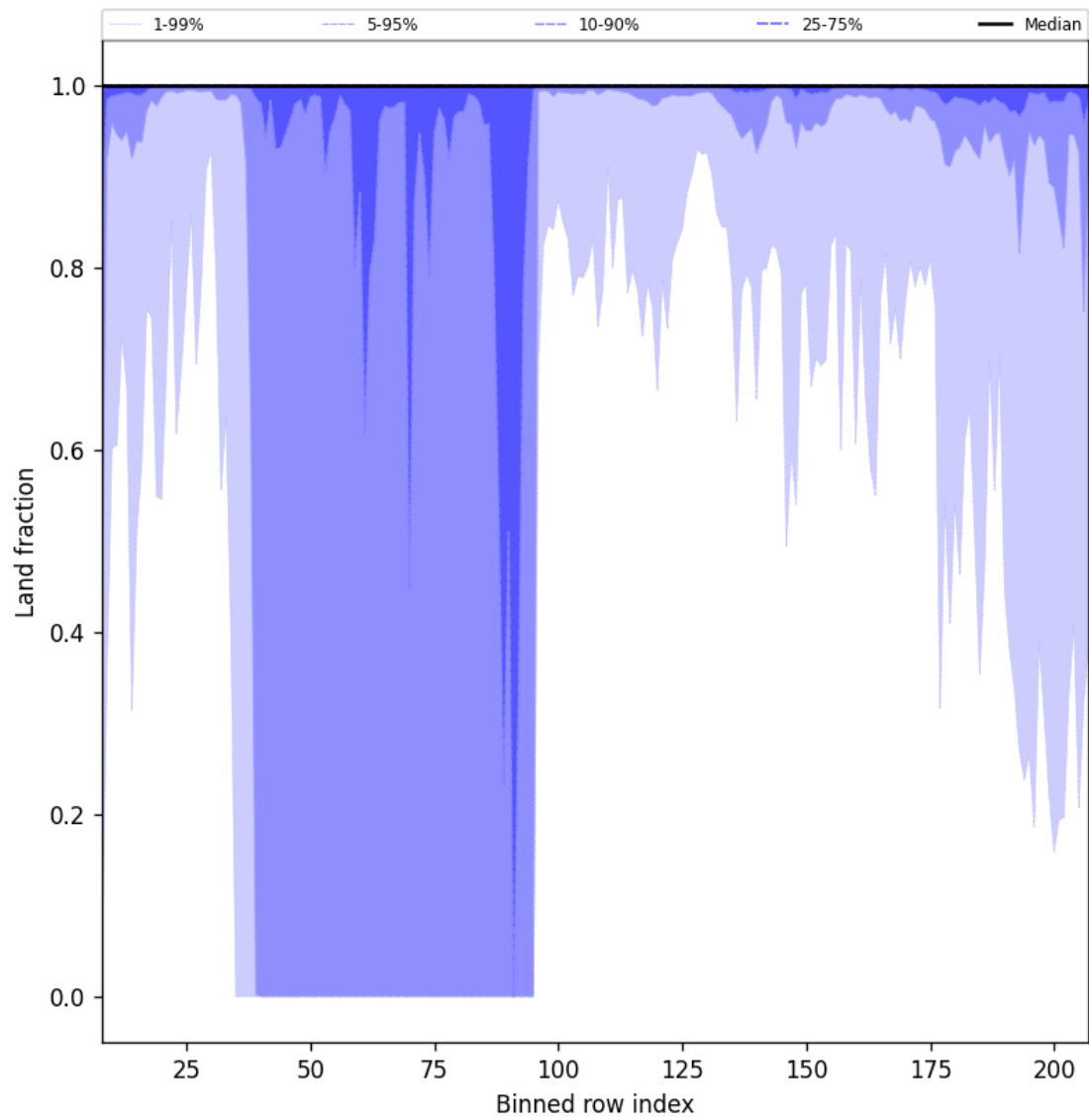
Figure 45: Along track statistics of "Land fraction" for 2025-12-03 to 2025-12-04
