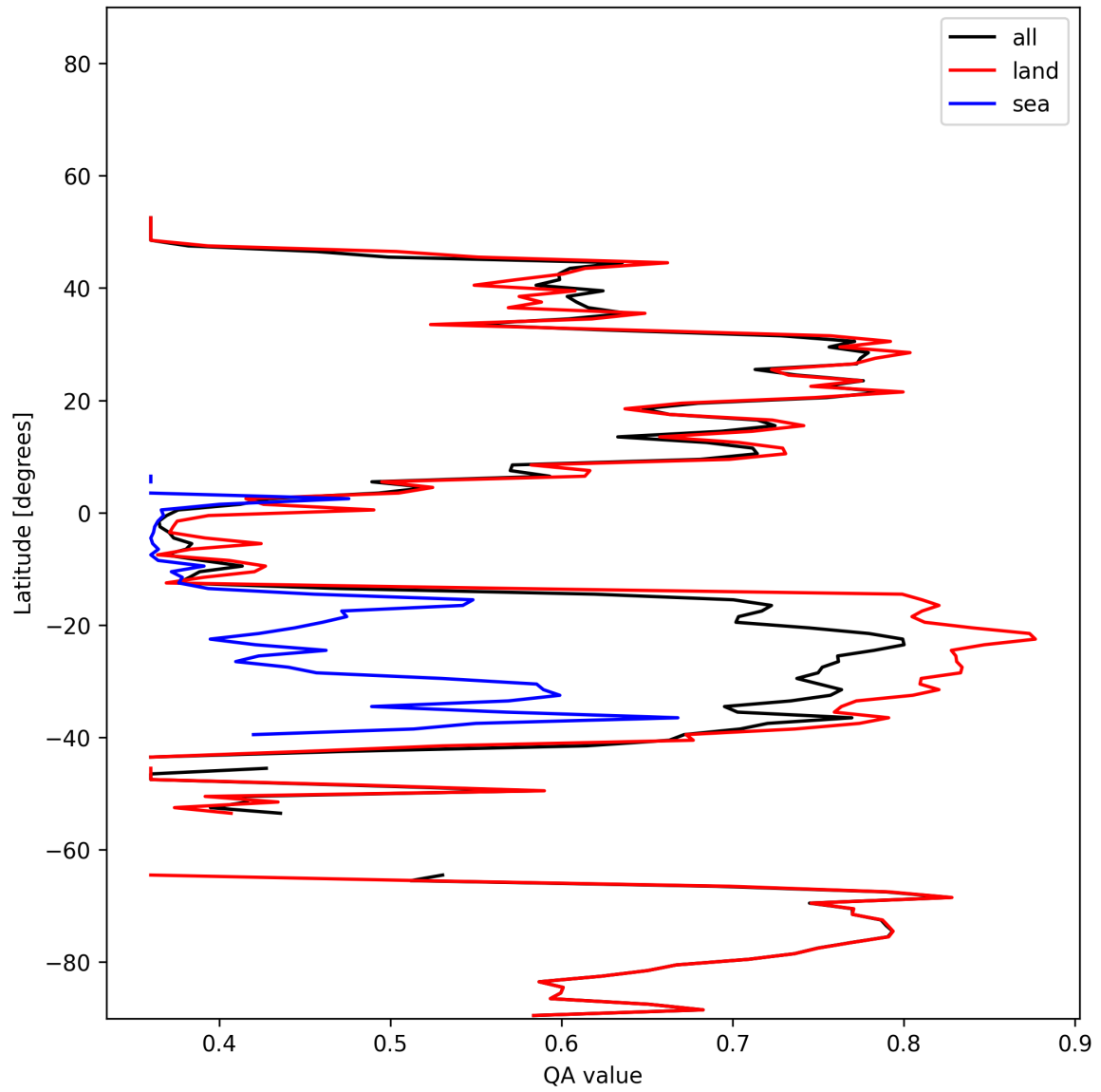
Figure 10: Zonal average of “QA value” for 2025-12-03 to 2025-12-04.
