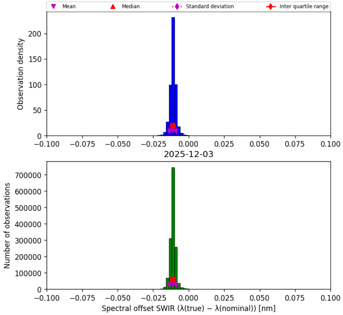
Figure 27: Histogram of “Spectral offset SWIR ( \lambda_{\text{true}} - \lambda_{\text{nominal}} )” for 2025-12-03 to 2025-12-04
