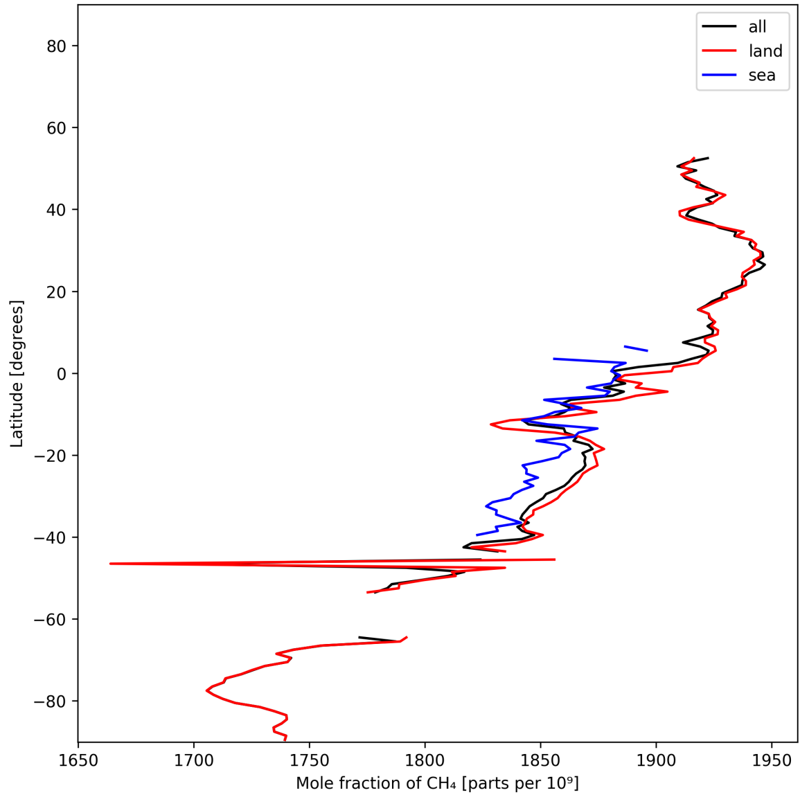
Figure 11: Zonal average of “Mole fraction of CH 4 ” for 2025-12-03 to 2025-12-04.
