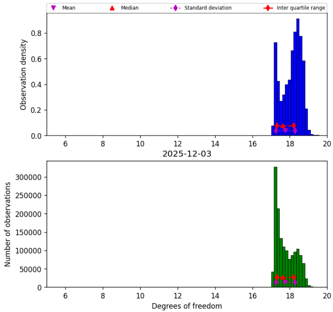
Figure 30: Histogram of “Degrees of freedom” for 2025-12-03 to 2025-12-04
