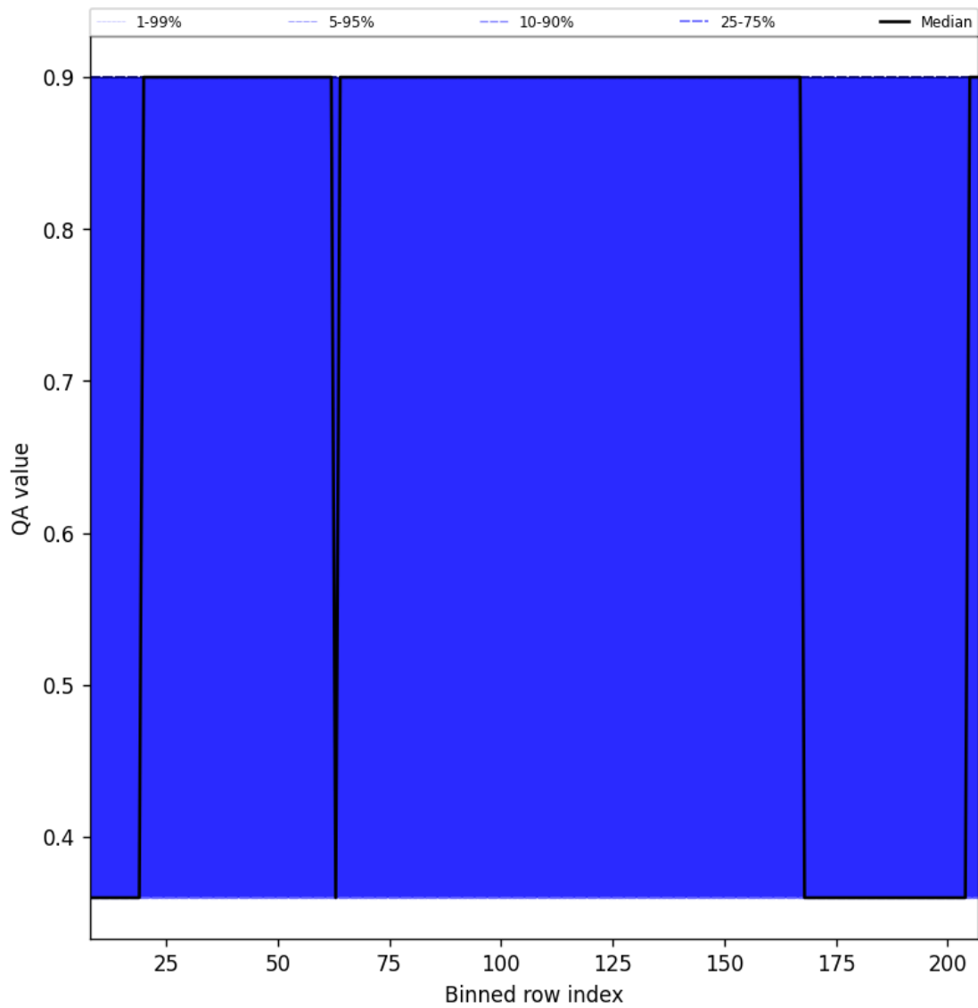
Figure 34: Along track statistics of “QA value” for 2025-12-03 to 2025-12-04
