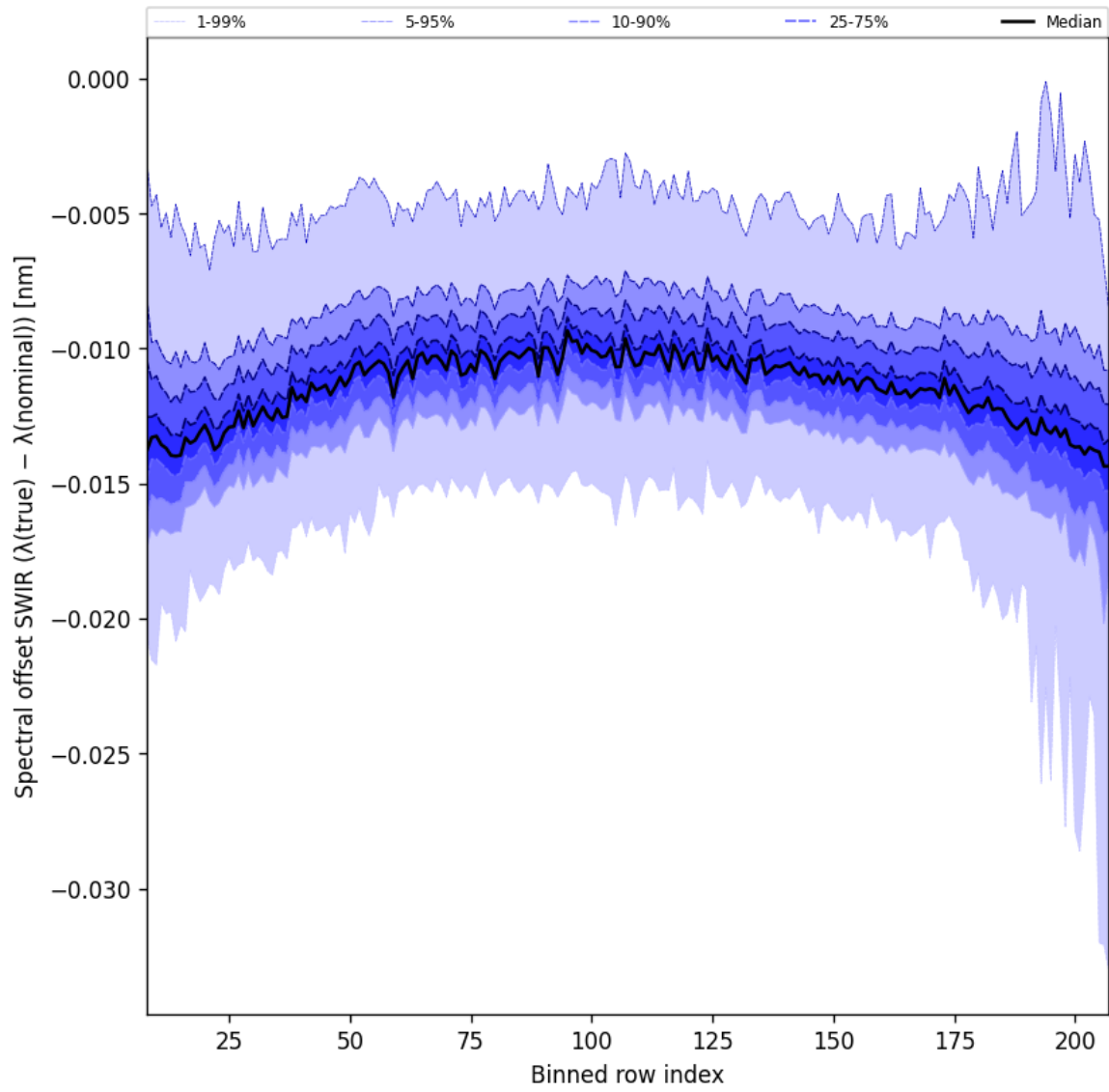
Figure 39: Along track statistics of “Spectral offset SWIR ( \lambda_{\text{true}} - \lambda_{\text{nominal}} )” for 2025-12-03 to 2025-12-04
