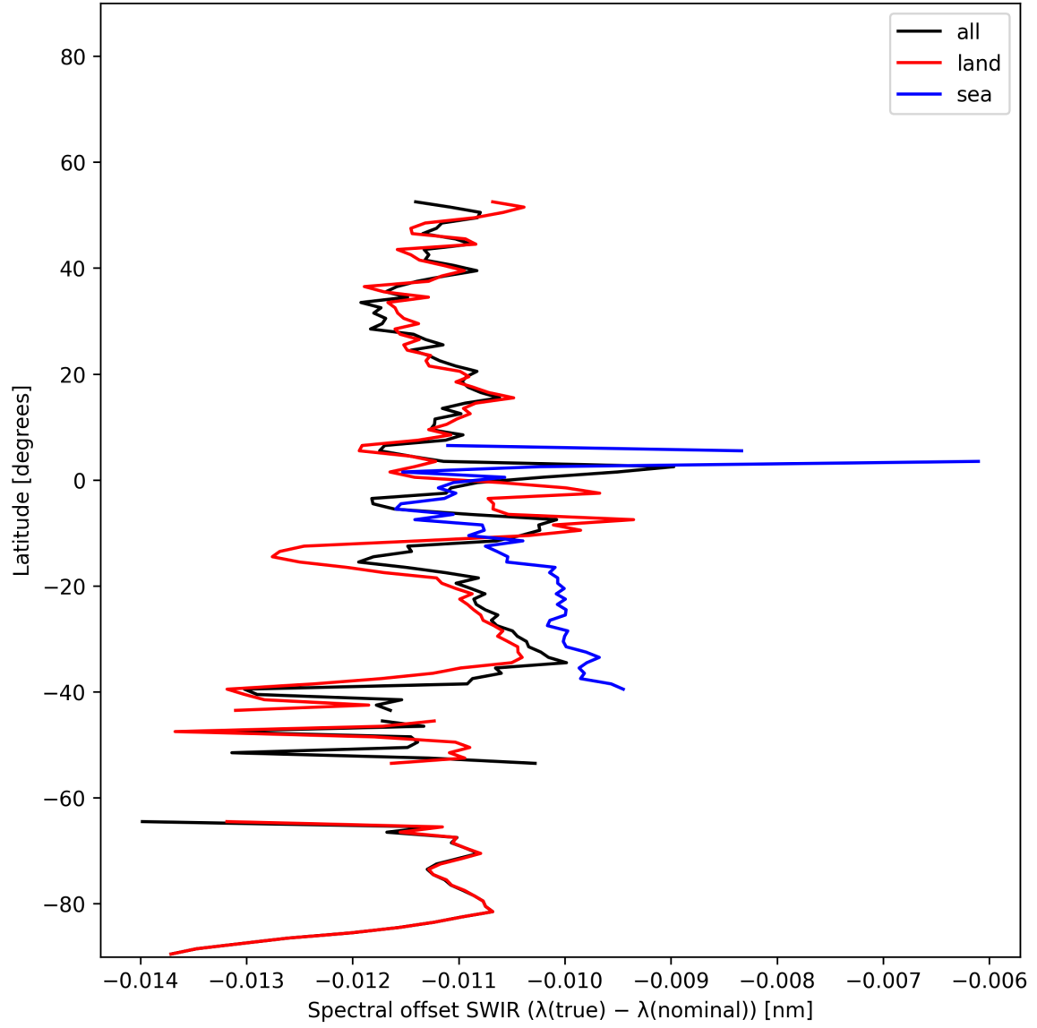
Figure 15: Zonal average of “Spectral offset SWIR ( \lambda_{\text{true}} - \lambda_{\text{nominal}} )” for 2025-12-03 to 2025-12-04.
