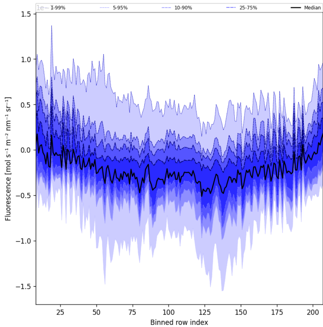
Figure 44: Along track statistics of “Fluorescence” for 2025-12-04 to 2025-12-05
