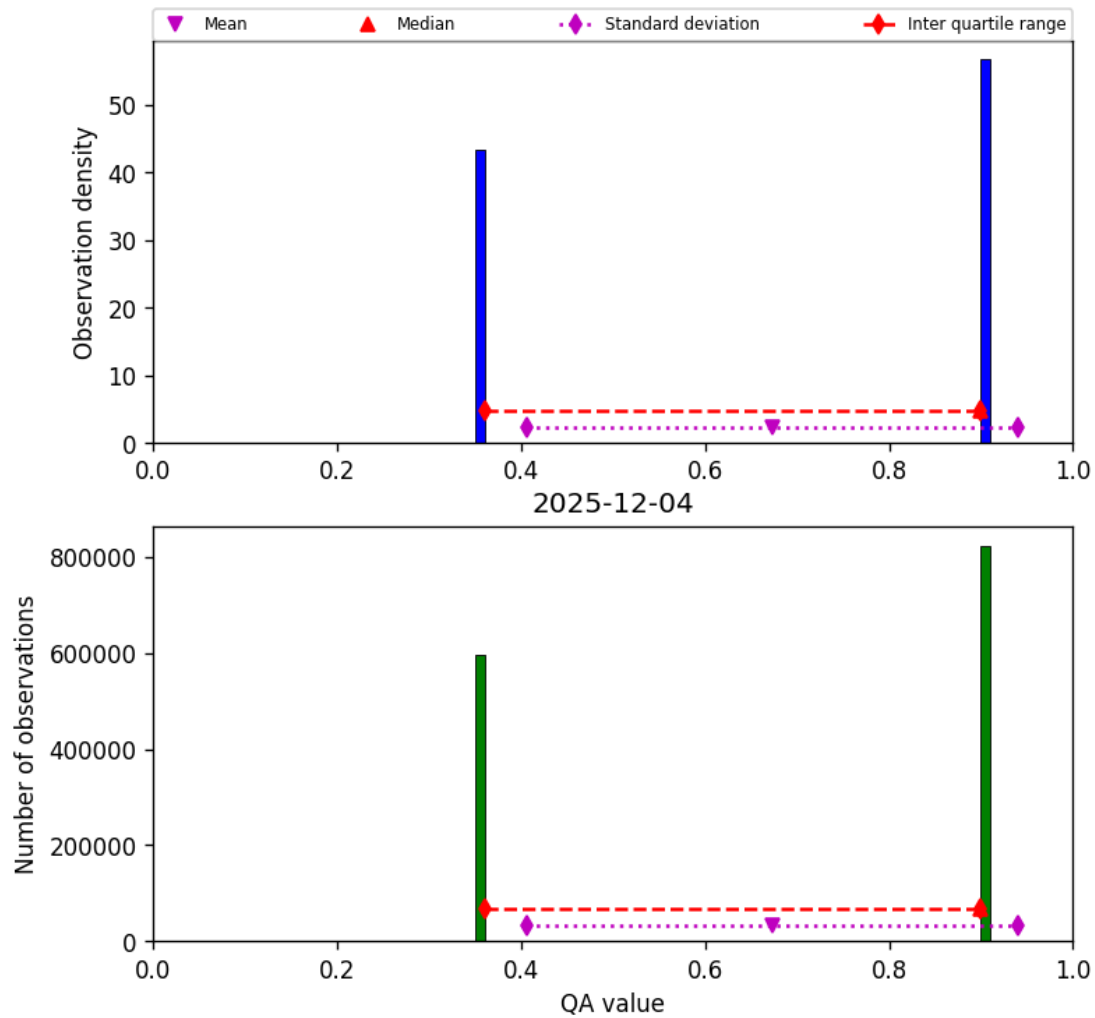
Figure 22: Histogram of “QA value” for 2025-12-04 to 2025-12-05
