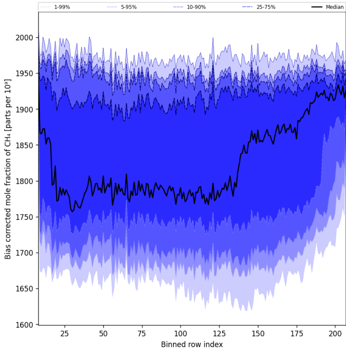
Figure 37: Along track statistics of “Bias corrected mole fraction of CH 4 ” for 2025-12-04 to 2025-12-05
