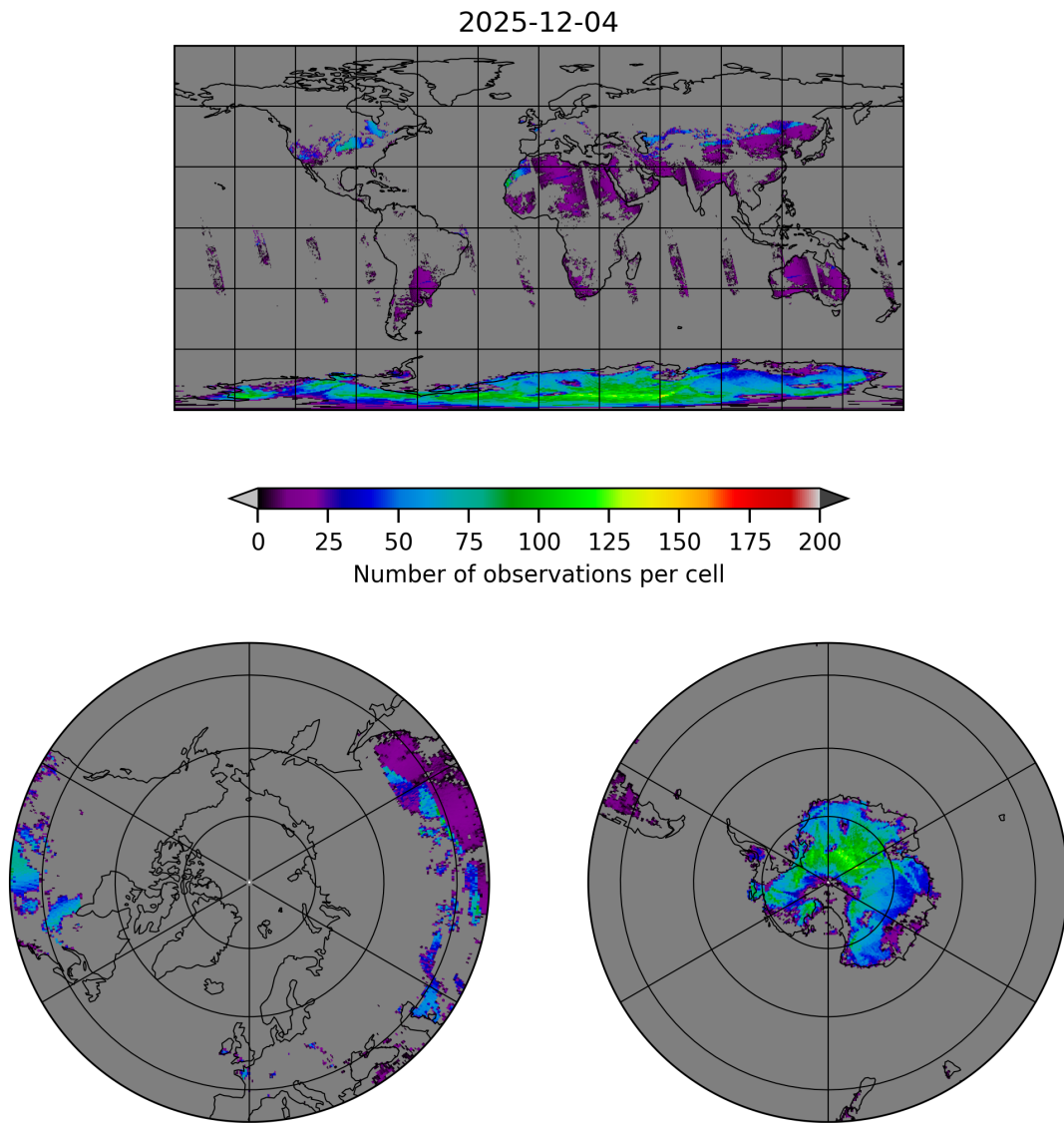
Figure 9: Map of the number of observations for 2025-12-04 to 2025-12-05
