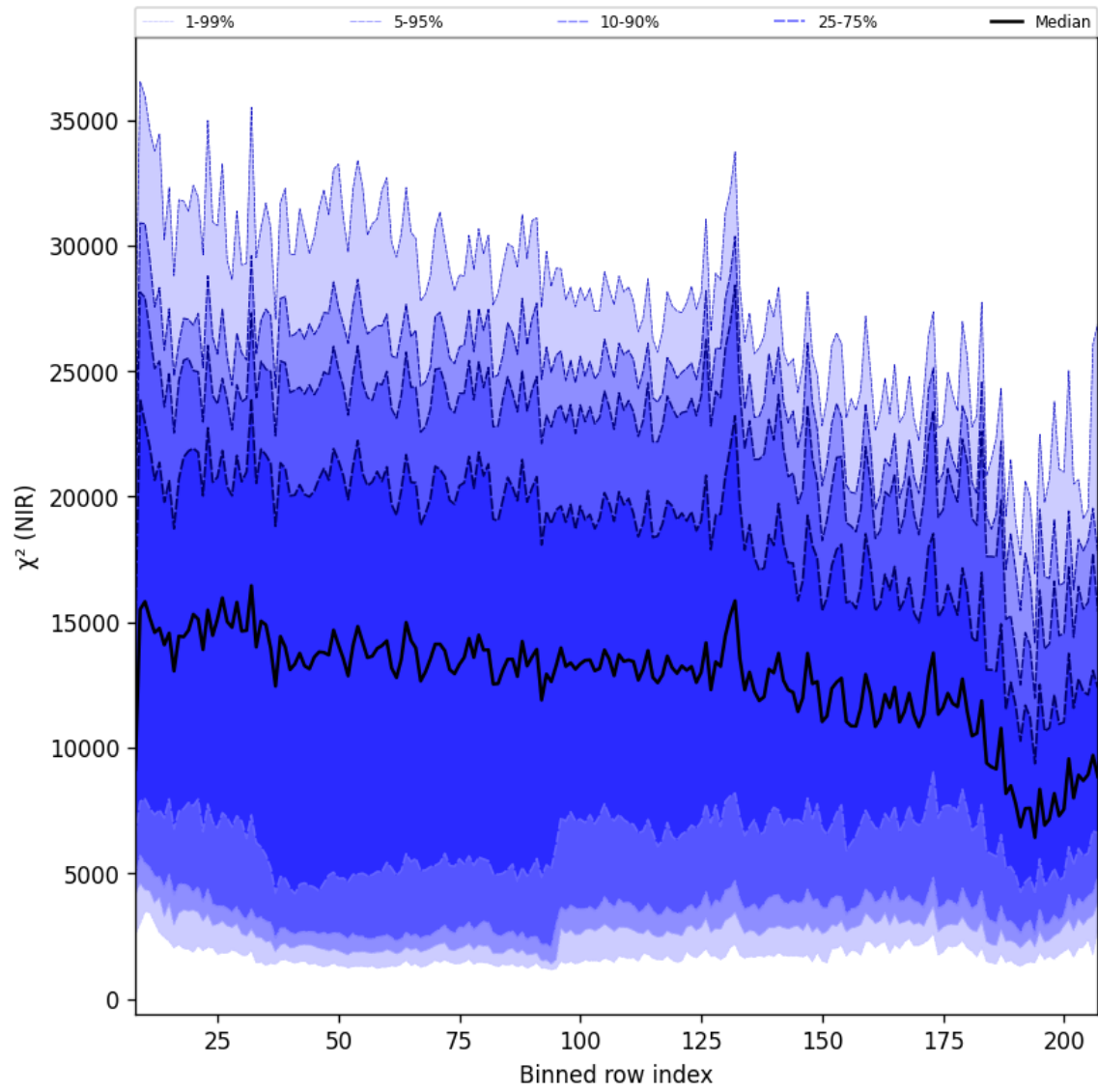
Figure 41: Along track statistics of “ \chi^2 (NIR)” for 2025-12-04 to 2025-12-05
