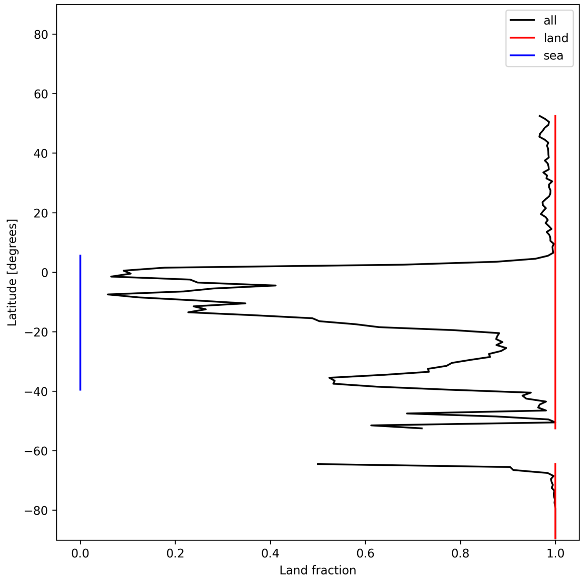
Figure 21: Zonal average of “Land fraction” for 2025-12-04 to 2025-12-05.
