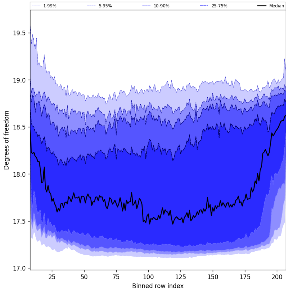
Figure 42: Along track statistics of “Degrees of freedom” for 2025-12-04 to 2025-12-05
