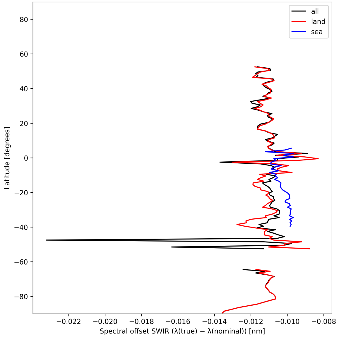
Figure 15: Zonal average of “Spectral offset SWIR ( \lambda_{\text{true}} - \lambda_{\text{nominal}} )” for 2025-12-04 to 2025-12-05.
