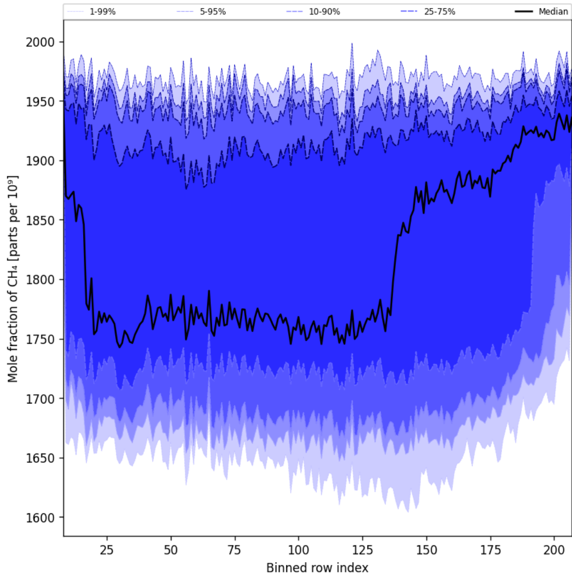
Figure 35: Along track statistics of “Mole fraction of CH 4 ” for 2025-12-04 to 2025-12-05
