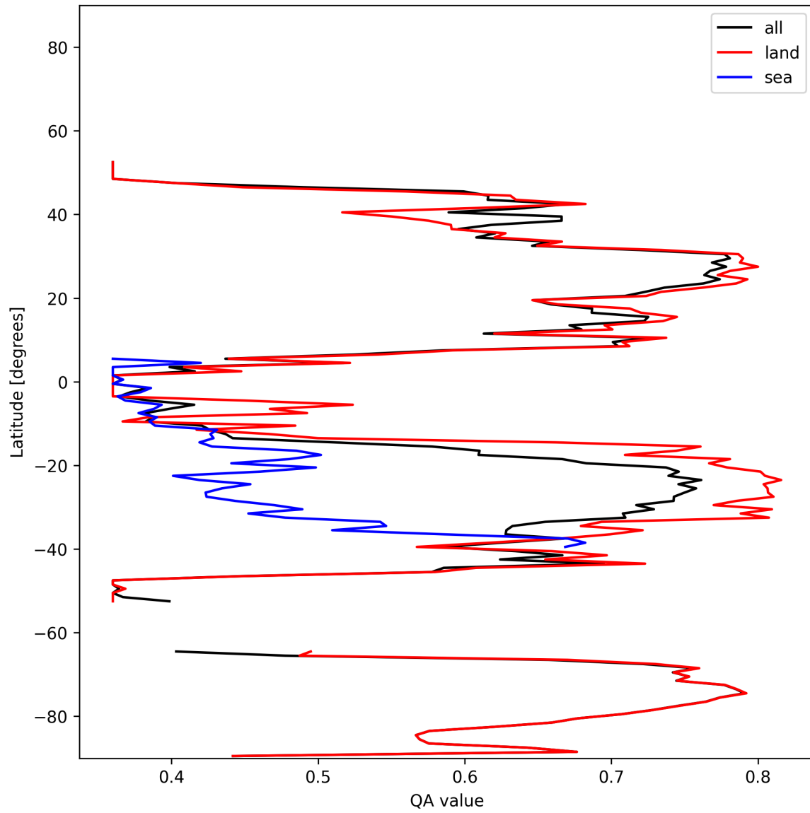
Figure 10: Zonal average of "QA value" for 2025-12-04 to 2025-12-05.
