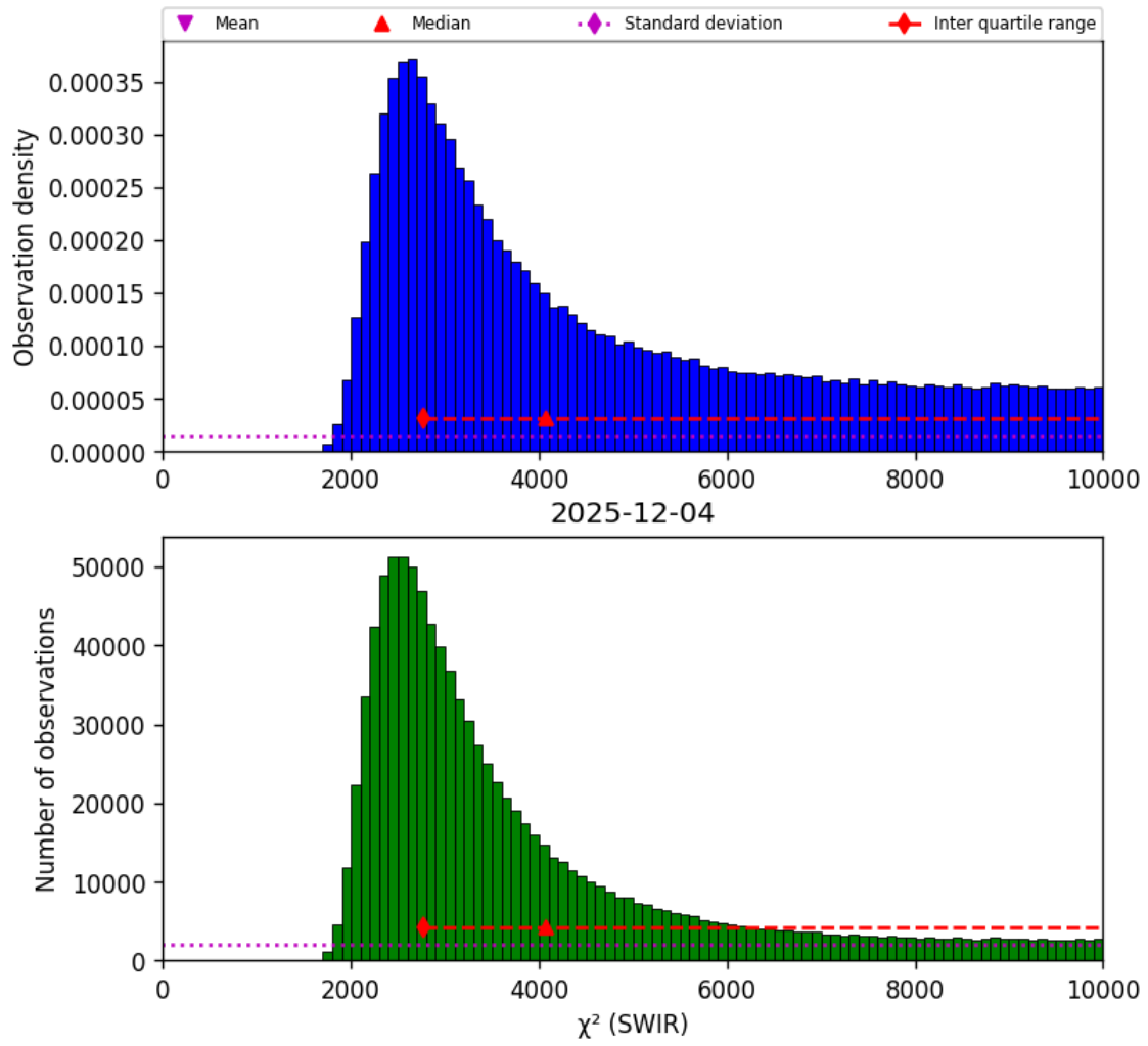
Figure 28: Histogram of “ \chi^2 (SWIR)” for 2025-12-04 to 2025-12-05
