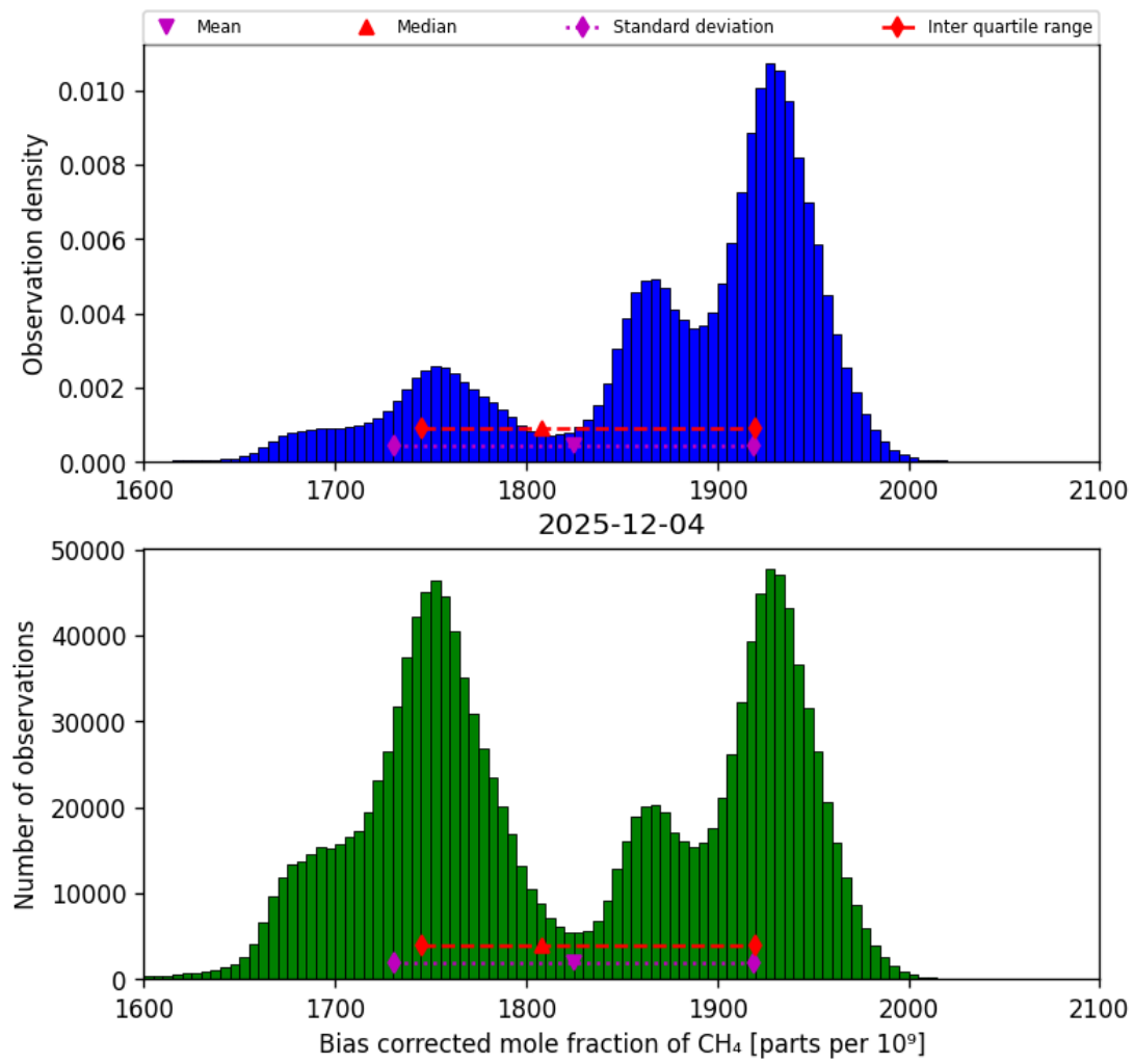
Figure 25: Histogram of “Bias corrected mole fraction of CH 4 ” for 2025-12-04 to 2025-12-05
