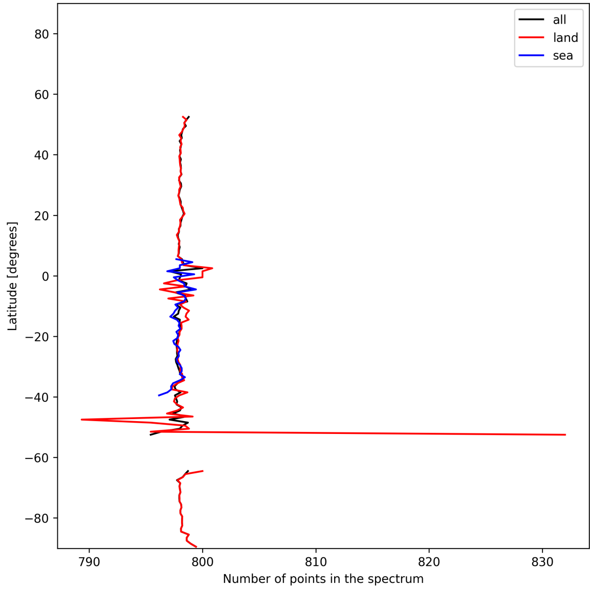
Figure 14: Zonal average of “Number of points in the spectrum” for 2025-12-04 to 2025-12-05.
