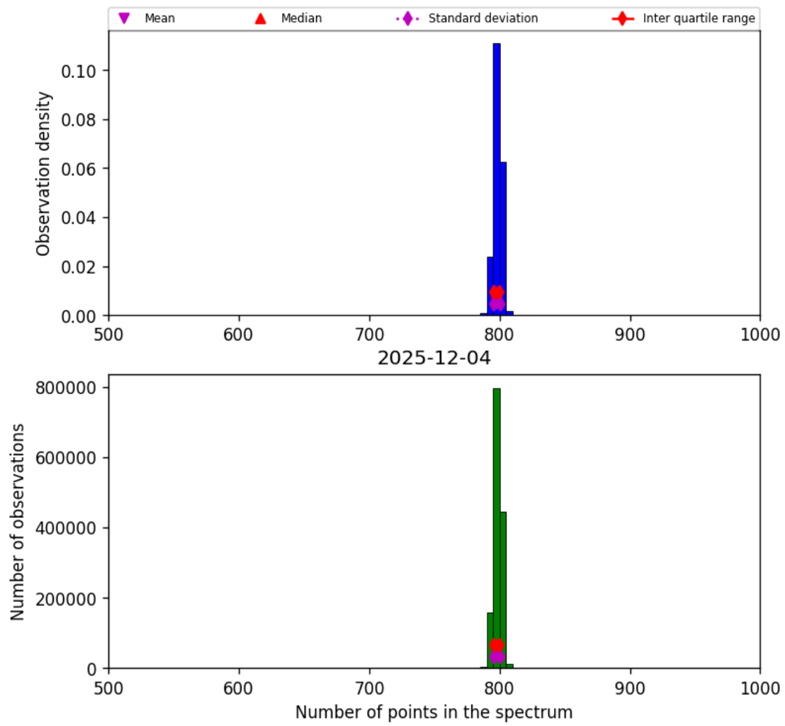
Figure 26: Histogram of “Number of points in the spectrum” for 2025-12-04 to 2025-12-05
