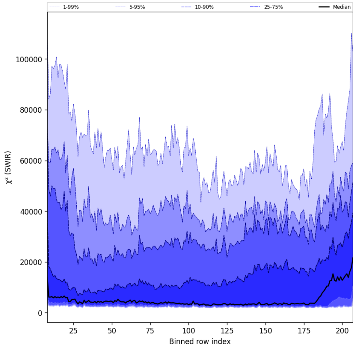
Figure 40: Along track statistics of “ \chi^2 (SWIR)” for 2025-12-04 to 2025-12-05
