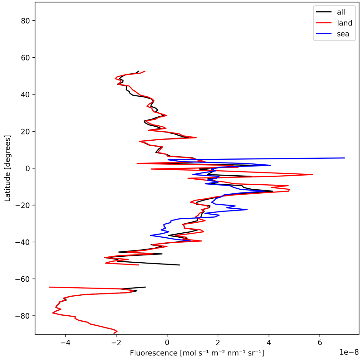
Figure 20: Zonal average of “Fluorescence” for 2025-12-04 to 2025-12-05.
