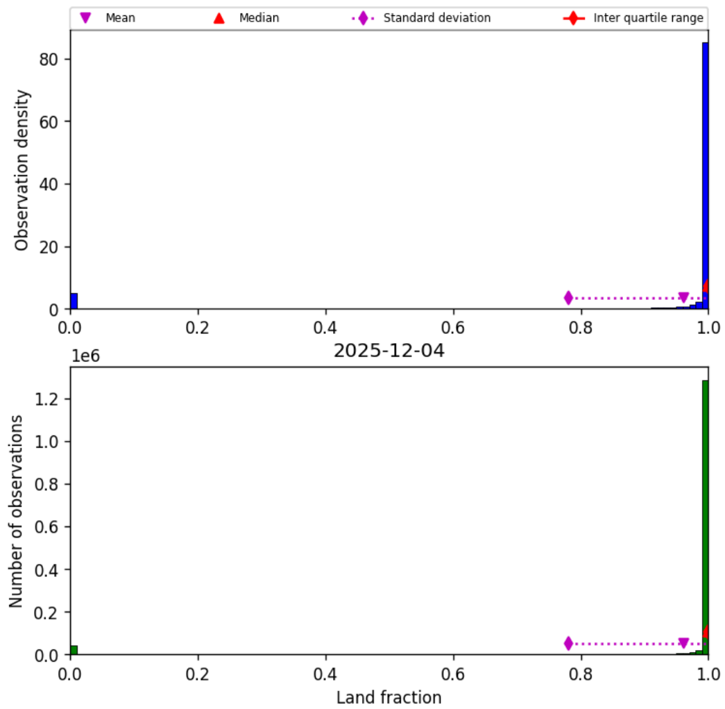
Figure 33: Histogram of “Land fraction” for 2025-12-04 to 2025-12-05
