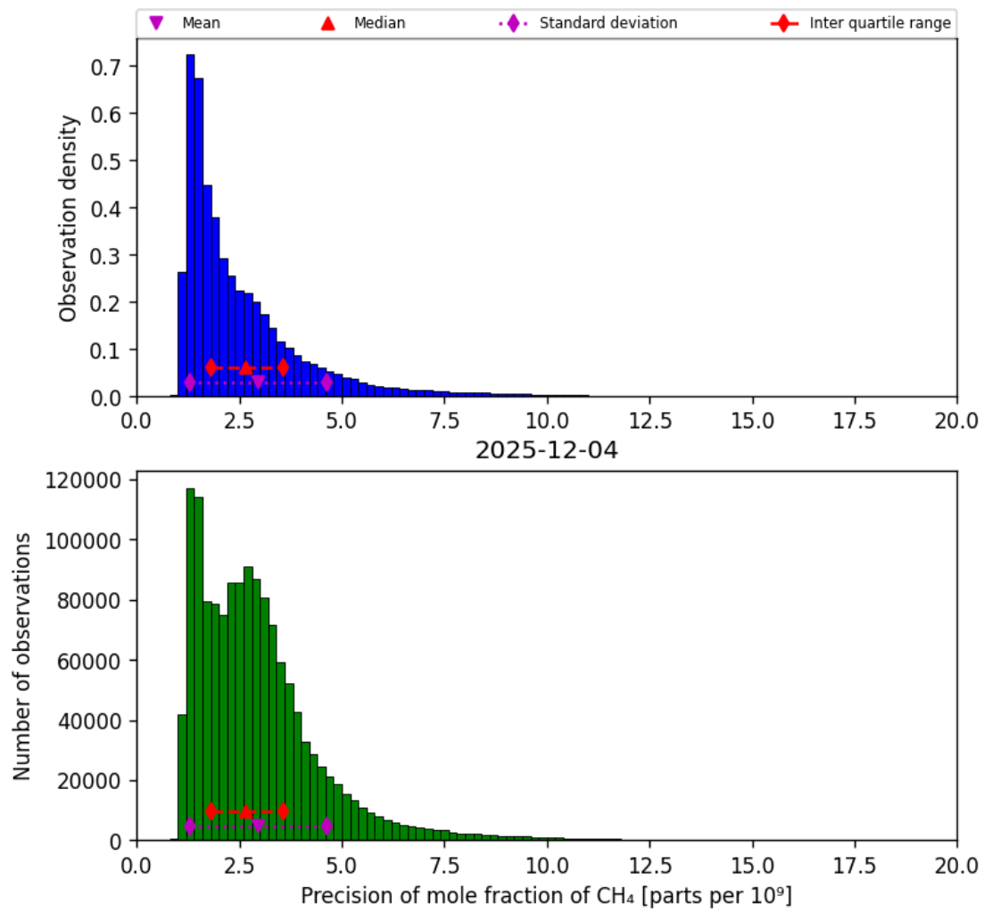
Figure 24: Histogram of “Precision of mole fraction of CH 4 ” for 2025-12-04 to 2025-12-05
