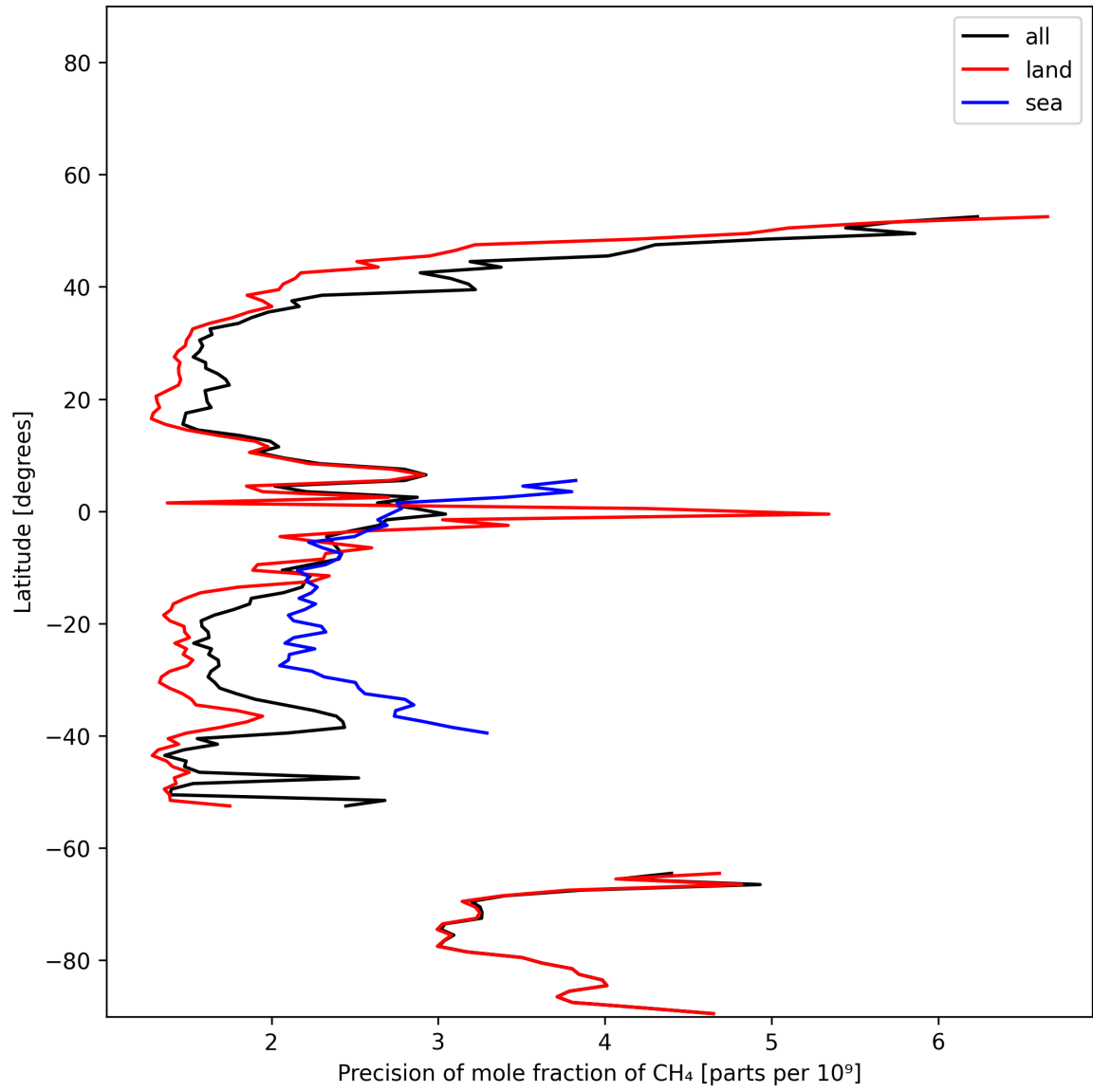
Figure 12: Zonal average of “Precision of mole fraction of CH 4 ” for 2025-12-04 to 2025-12-05.
