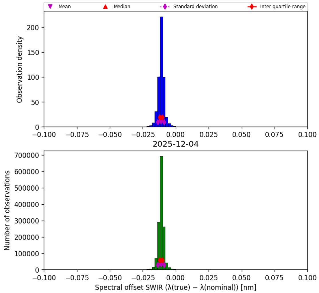
Figure 27: Histogram of “Spectral offset SWIR ( \lambda_{\text{true}} - \lambda_{\text{nominal}} )” for 2025-12-04 to 2025-12-05
