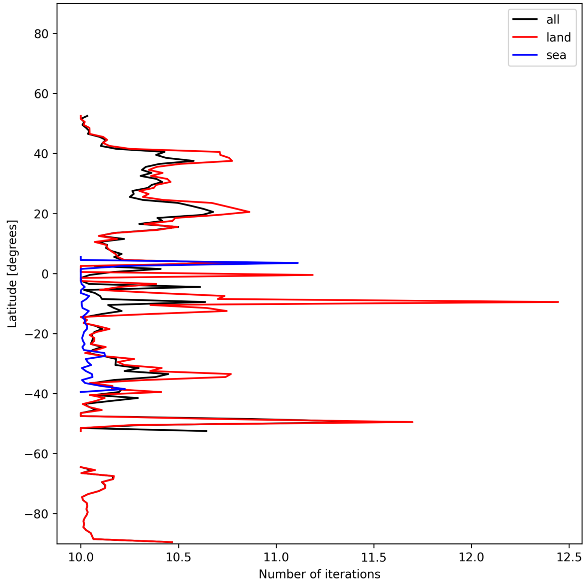
Figure 19: Zonal average of “Number of iterations” for 2025-12-04 to 2025-12-05.
