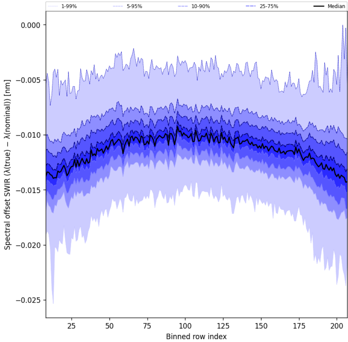
Figure 39: Along track statistics of “Spectral offset SWIR ( \lambda_{\text{true}} - \lambda_{\text{nominal}} )” for 2025-12-04 to 2025-12-05
