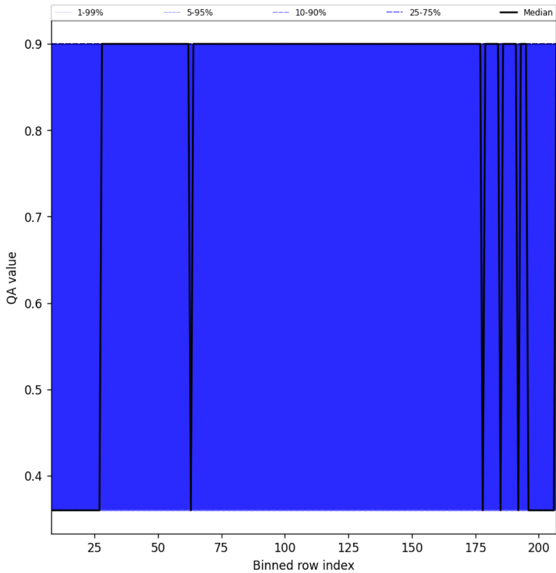
Figure 34: Along track statistics of “QA value” for 2025-12-04 to 2025-12-05
