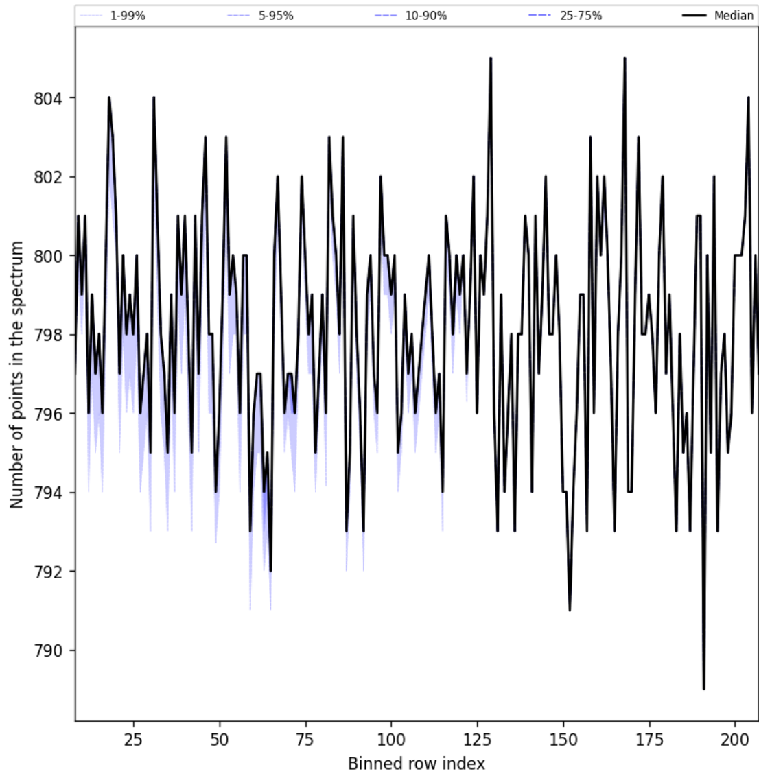
Figure 38: Along track statistics of “Number of points in the spectrum” for 2025-12-04 to 2025-12-05
