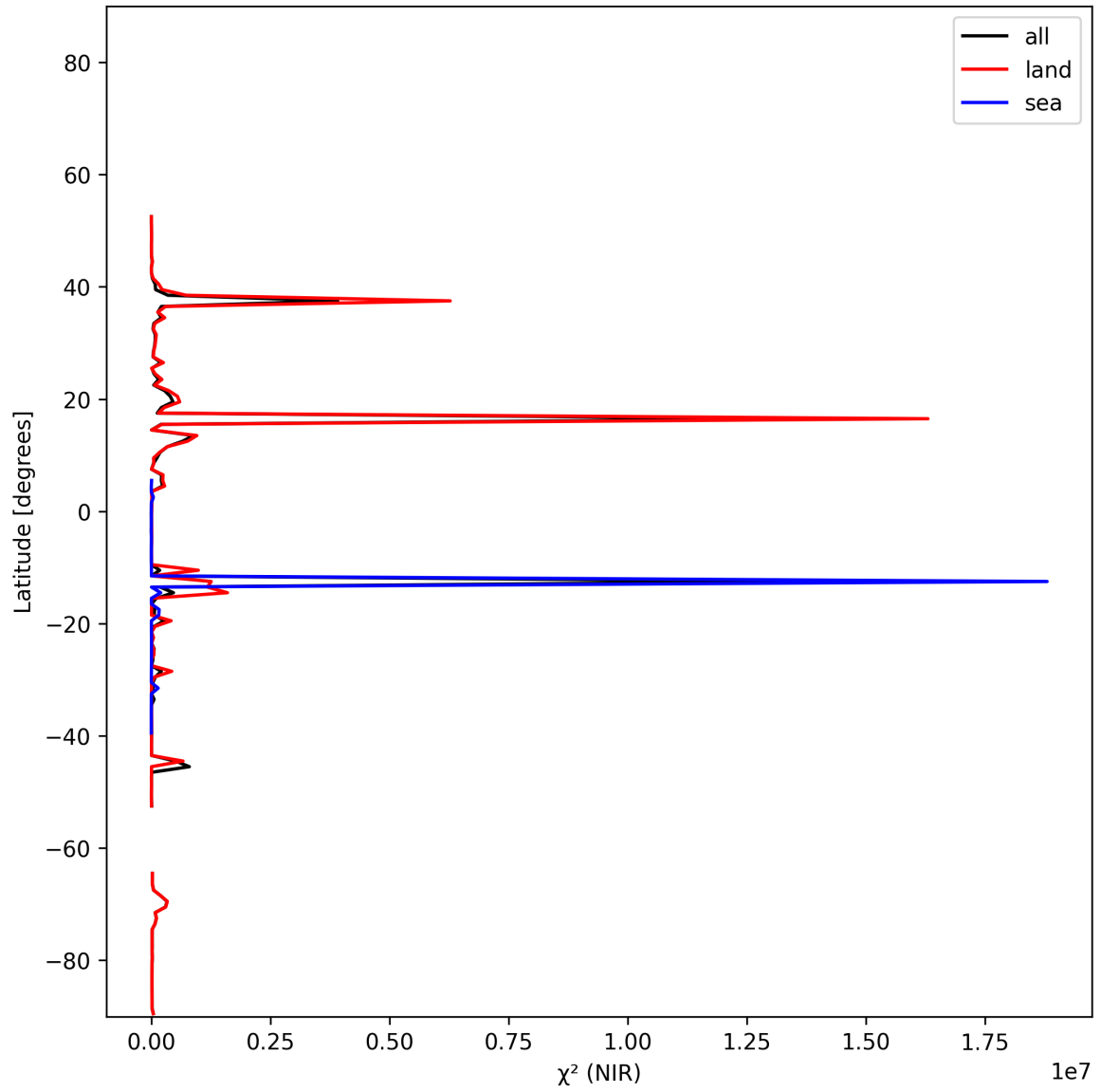
Figure 17: Zonal average of “ \chi^2 (NIR)” for 2025-12-04 to 2025-12-05.
