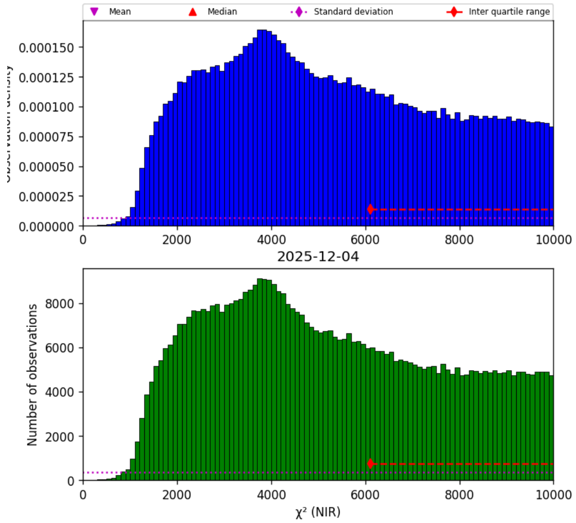
Figure 29: Histogram of “ \chi^2 (NIR)” for 2025-12-04 to 2025-12-05
