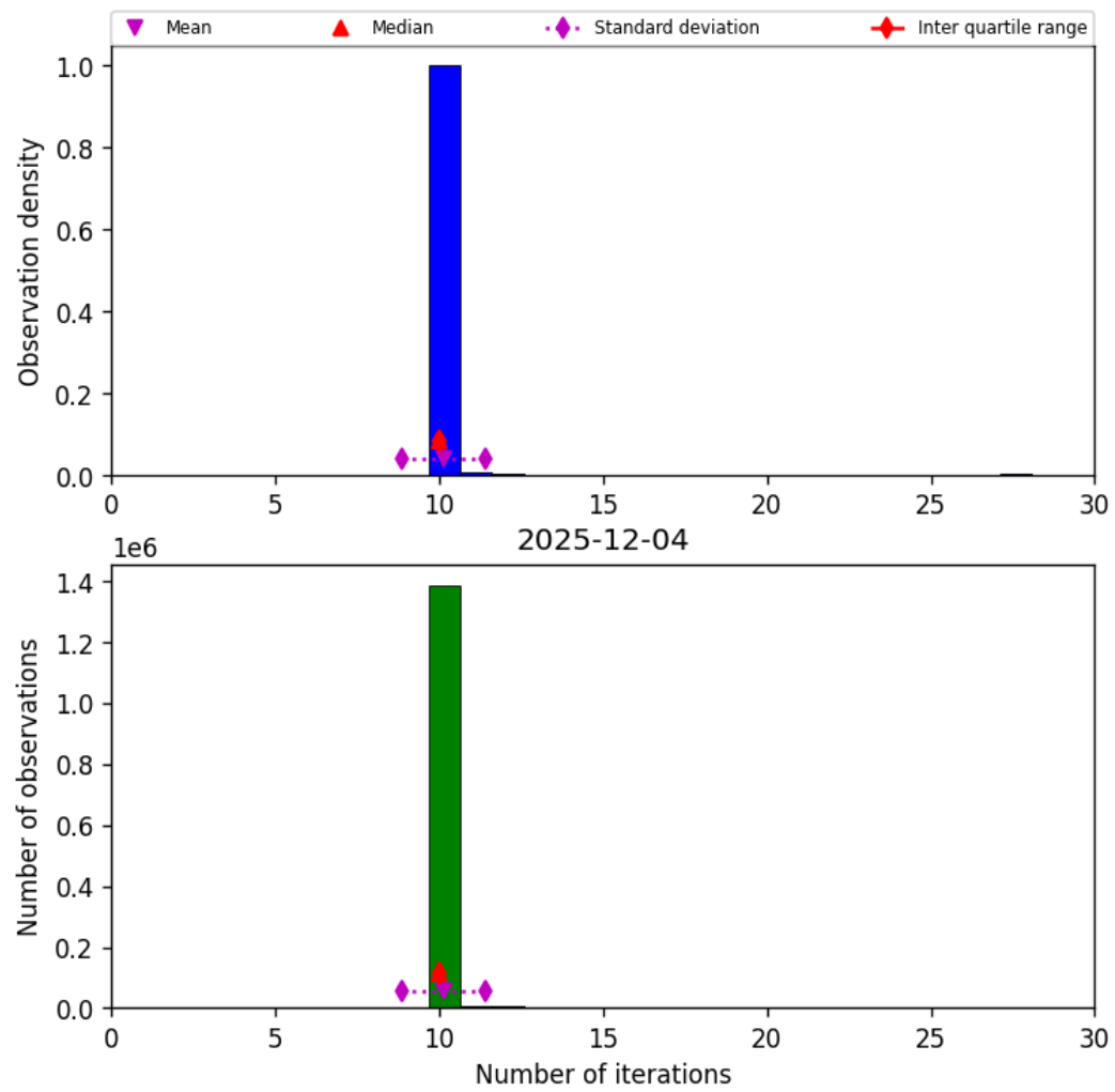
Figure 31: Histogram of "Number of iterations" for 2025-12-04 to 2025-12-05
