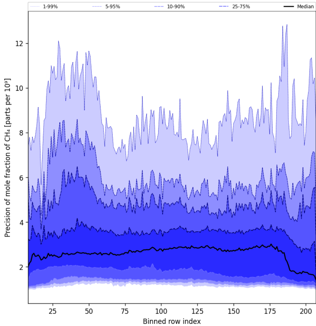
Figure 36: Along track statistics of “Precision of mole fraction of CH 4 ” for 2025-12-04 to 2025-12-05
