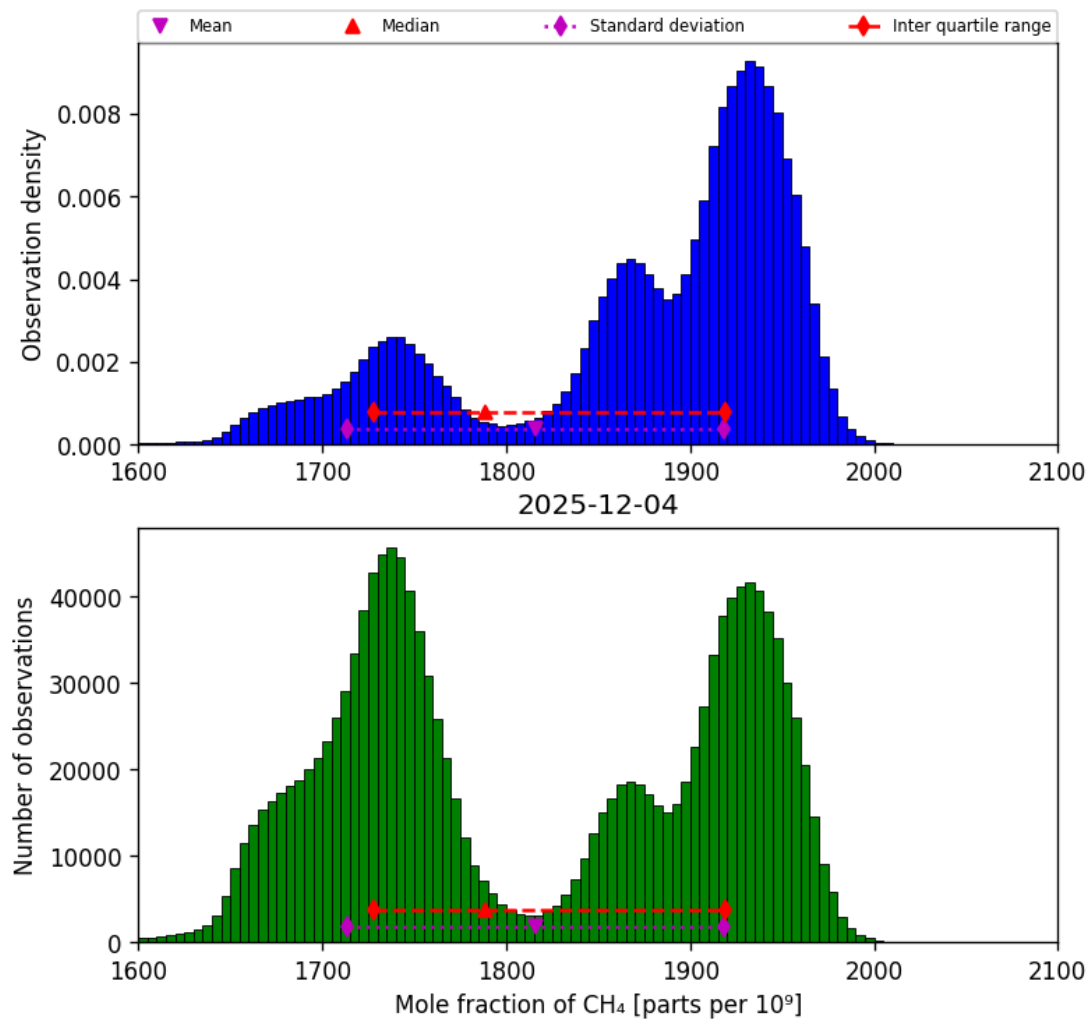
Figure 23: Histogram of “Mole fraction of CH 4 ” for 2025-12-04 to 2025-12-05
