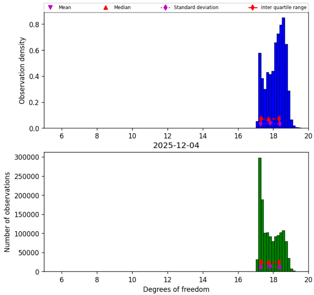
Figure 30: Histogram of “Degrees of freedom” for 2025-12-04 to 2025-12-05
