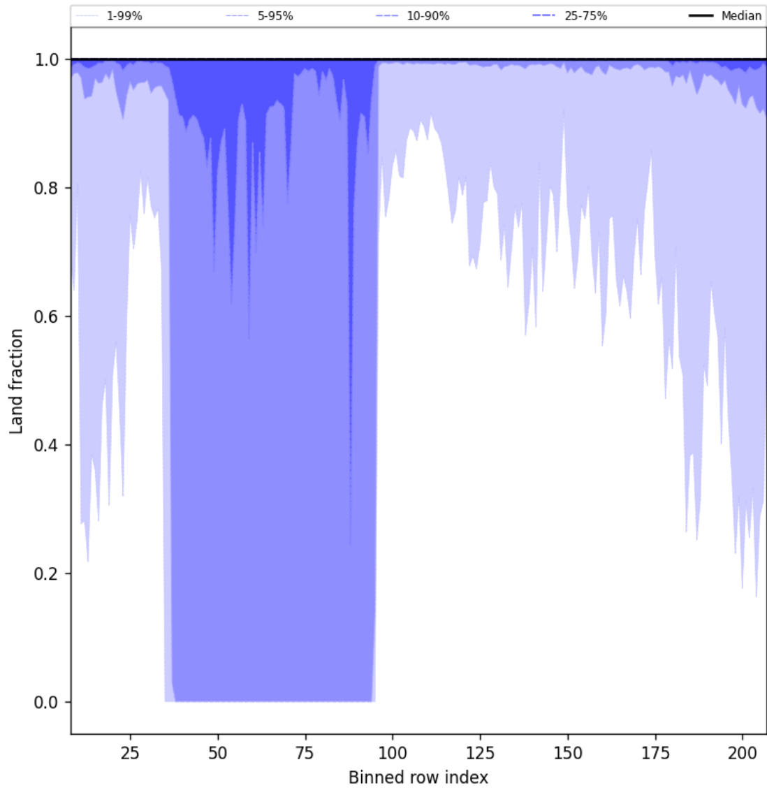
Figure 45: Along track statistics of “Land fraction” for 2025-12-04 to 2025-12-05
