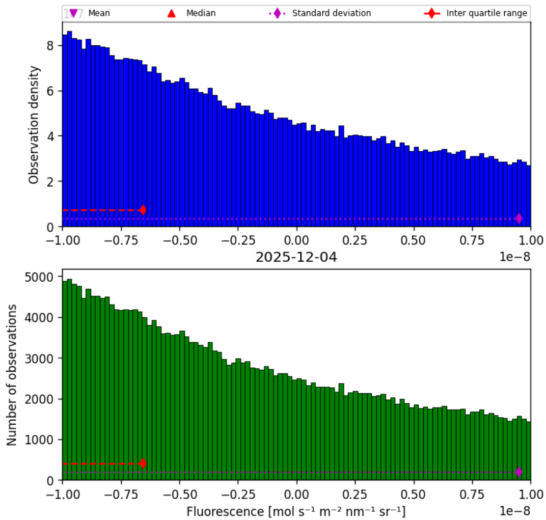
Figure 32: Histogram of “Fluorescence” for 2025-12-04 to 2025-12-05
