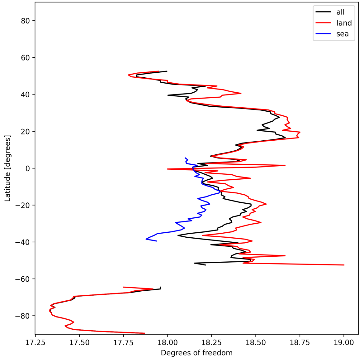
Figure 18: Zonal average of “Degrees of freedom” for 2025-12-04 to 2025-12-05.
