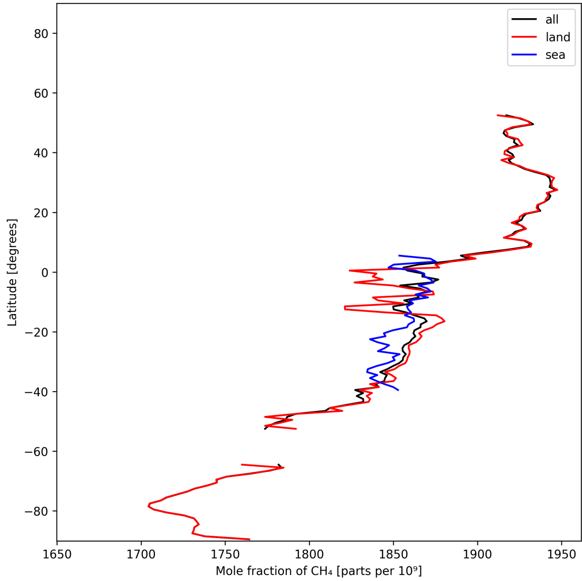
Figure 11: Zonal average of “Mole fraction of \text{CH}_4 ” for 2025-12-04 to 2025-12-05.
