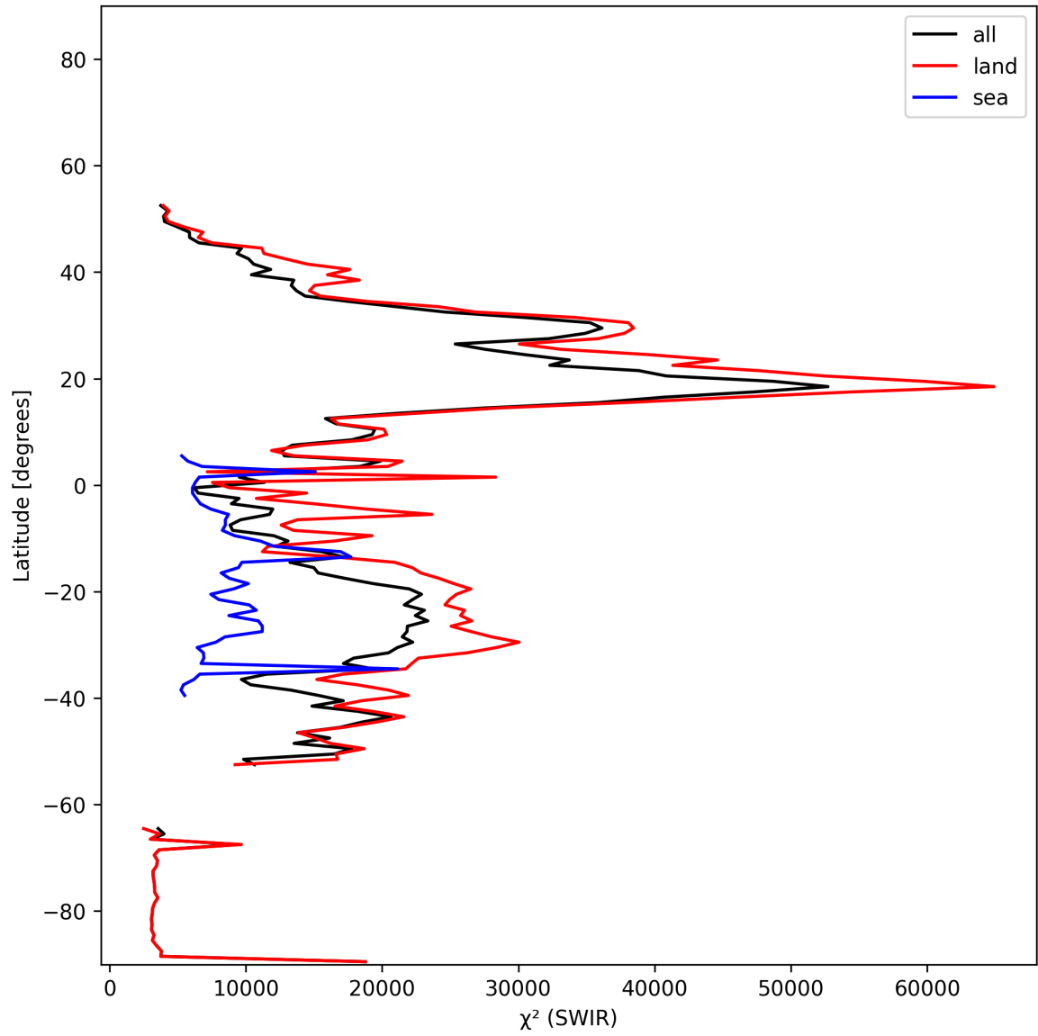
Figure 16: Zonal average of “ \chi^2 (SWIR)” for 2025-12-04 to 2025-12-05.
