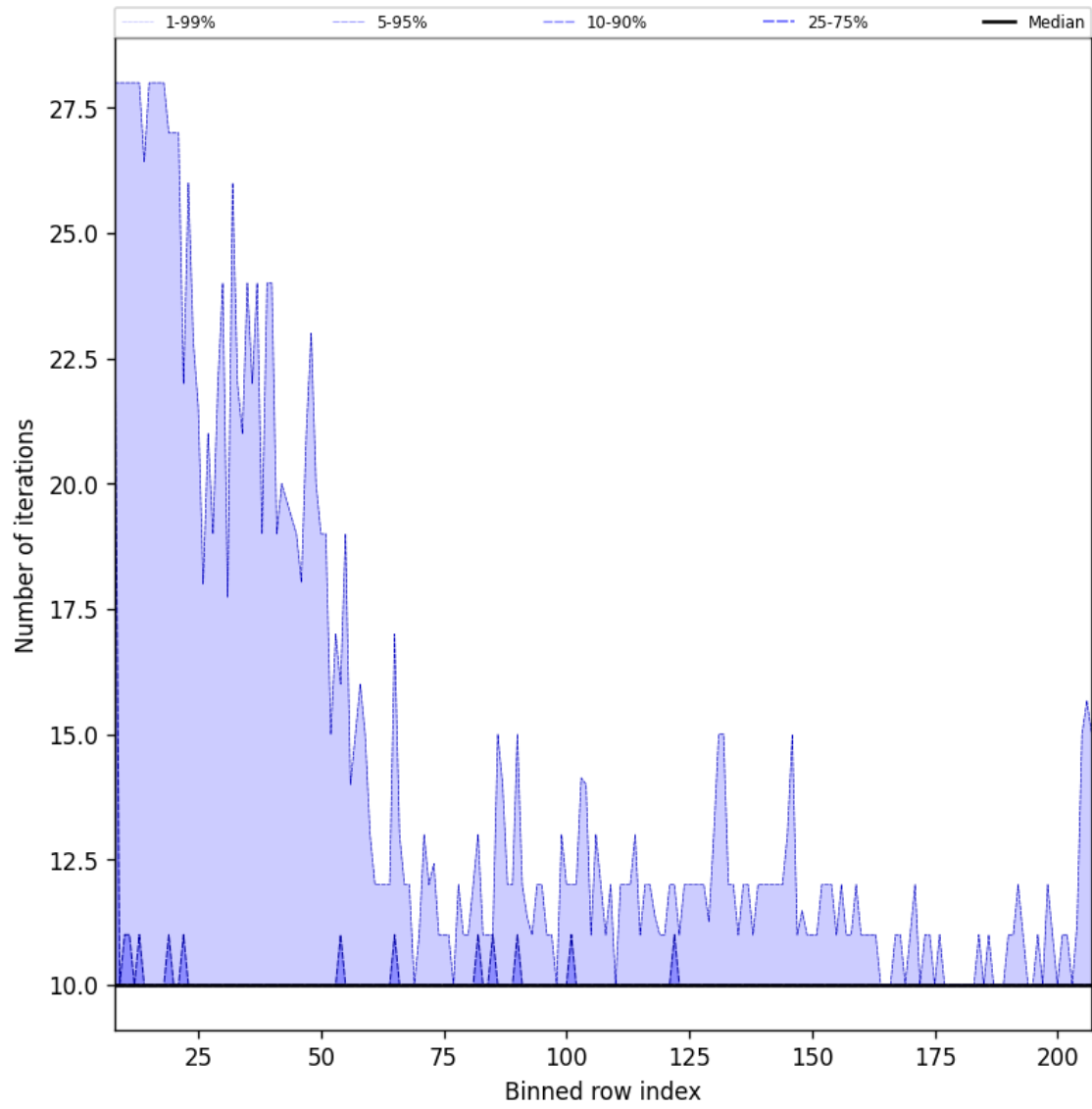
Figure 43: Along track statistics of “Number of iterations” for 2025-12-04 to 2025-12-05
