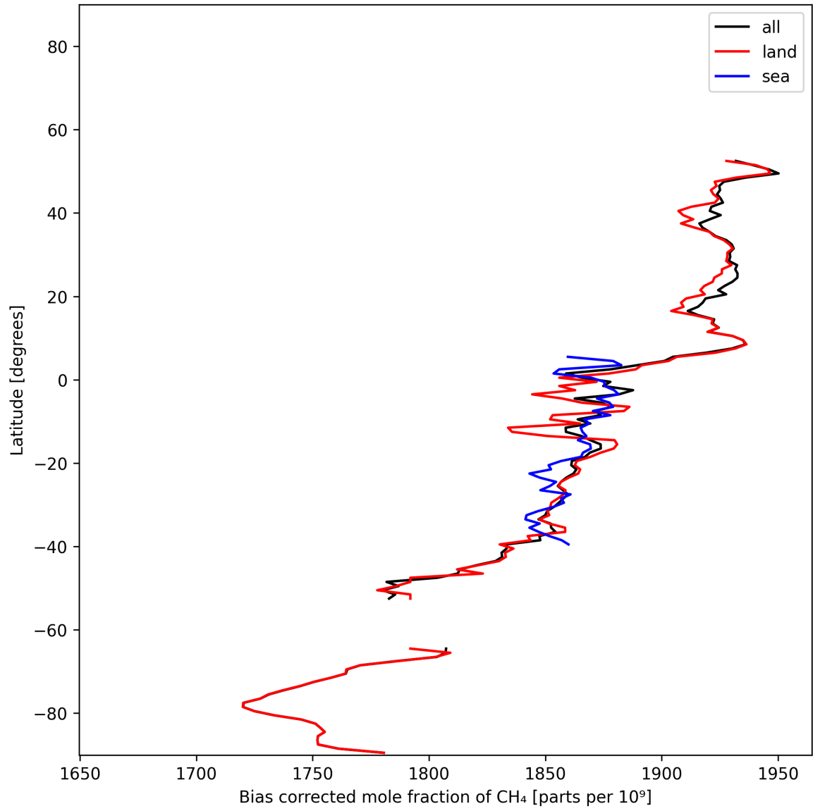
Figure 13: Zonal average of “Bias corrected mole fraction of CH 4 ” for 2025-12-04 to 2025-12-05.
