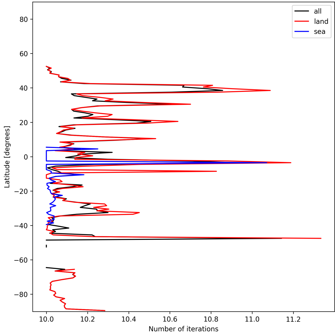
Figure 19: Zonal average of “Number of iterations” for 2025-12-05 to 2025-12-06.
