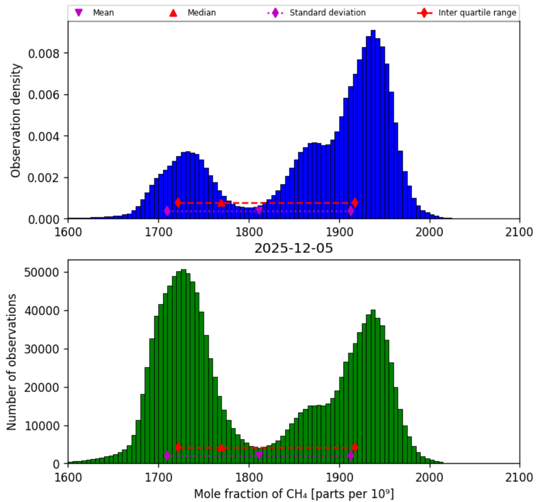
Figure 23: Histogram of “Mole fraction of CH 4 ” for 2025-12-05 to 2025-12-06
