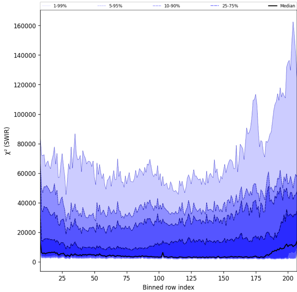
Figure 40: Along track statistics of “ \chi^2 (SWIR)” for 2025-12-05 to 2025-12-06
