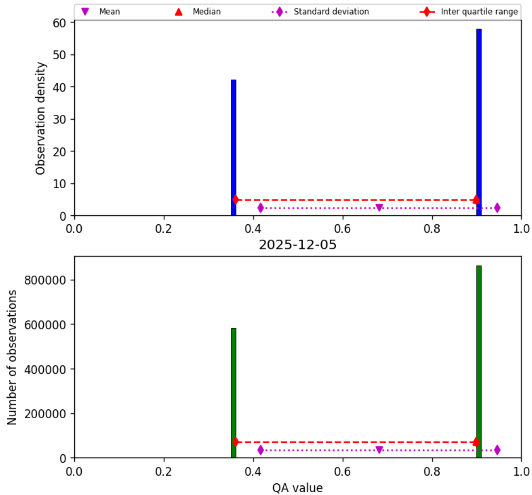
Figure 22: Histogram of “QA value” for 2025-12-05 to 2025-12-06
