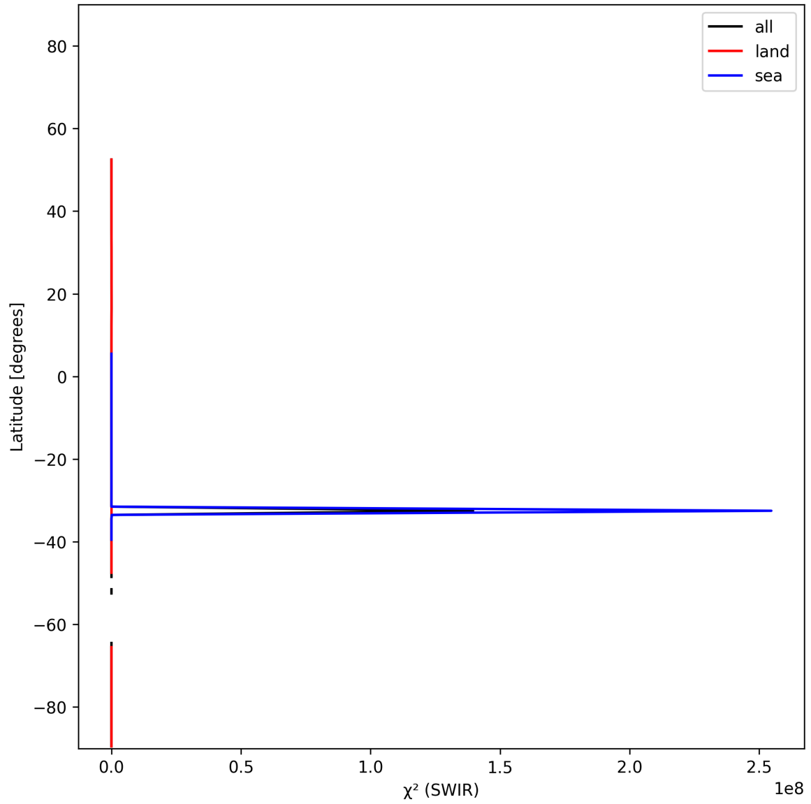
Figure 16: Zonal average of “ \chi^2 (SWIR)” for 2025-12-05 to 2025-12-06.
