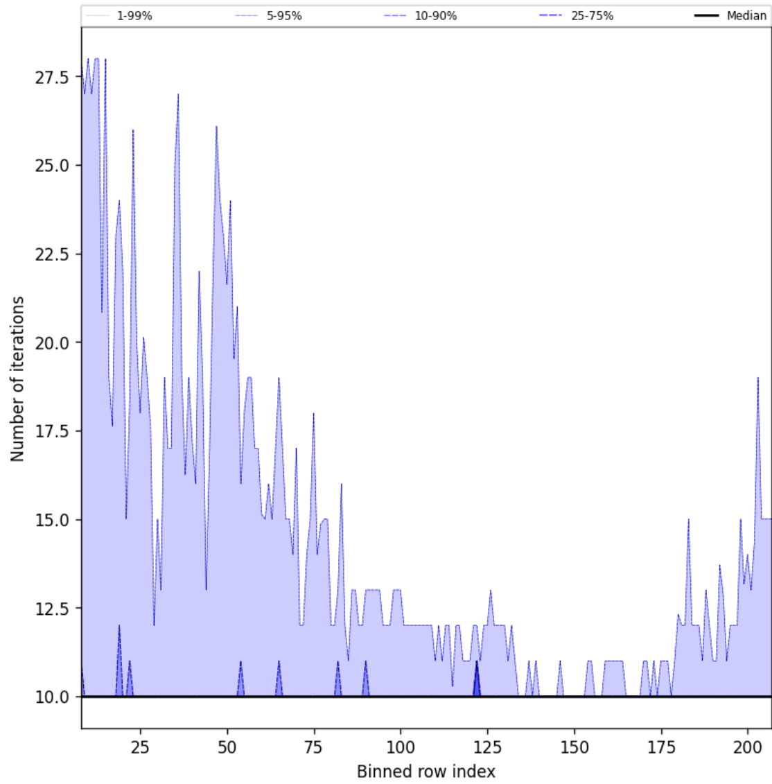
Figure 43: Along track statistics of “Number of iterations” for 2025-12-05 to 2025-12-06
