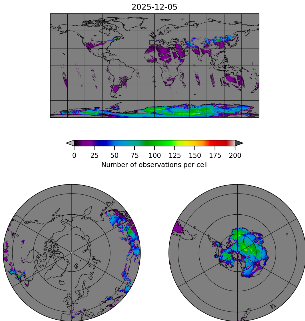
Figure 9: Map of the number of observations for 2025-12-05 to 2025-12-06
