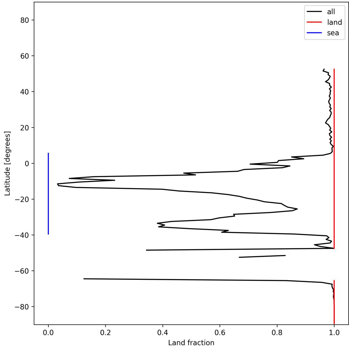
Figure 21: Zonal average of “Land fraction” for 2025-12-05 to 2025-12-06.
