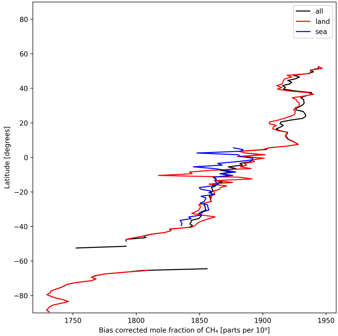
Figure 13: Zonal average of “Bias corrected mole fraction of CH 4 ” for 2025-12-05 to 2025-12-06.
