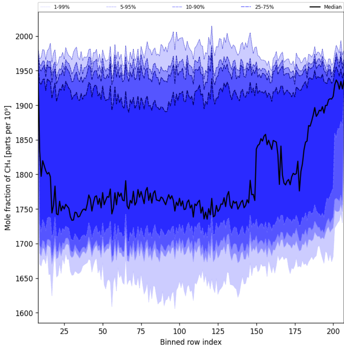
Figure 35: Along track statistics of “Mole fraction of CH 4 ” for 2025-12-05 to 2025-12-06
