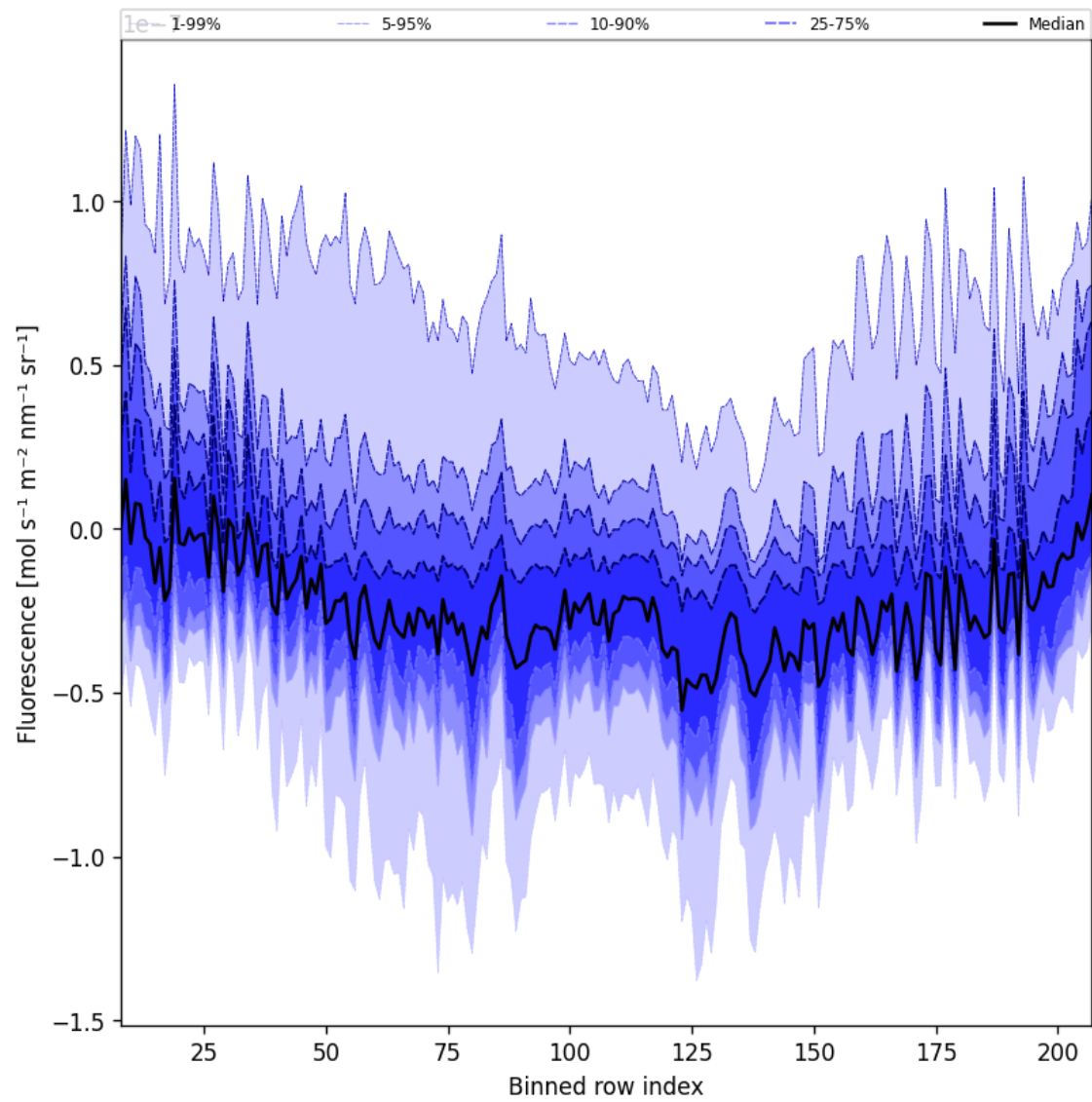
Figure 44: Along track statistics of “Fluorescence” for 2025-12-05 to 2025-12-06
