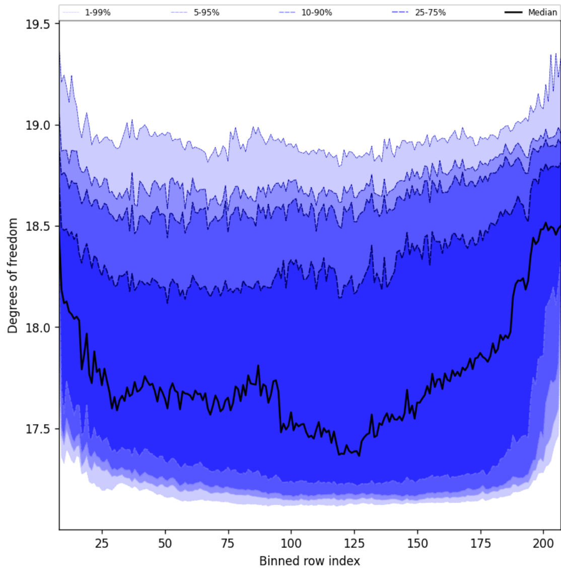
Figure 42: Along track statistics of “Degrees of freedom” for 2025-12-05 to 2025-12-06
