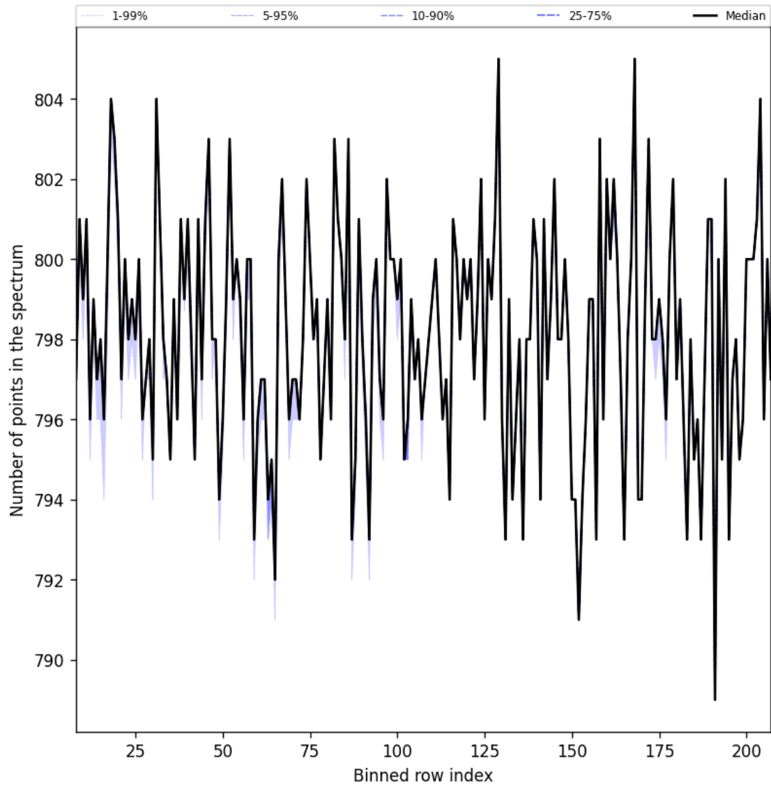
Figure 38: Along track statistics of “Number of points in the spectrum” for 2025-12-05 to 2025-12-06
