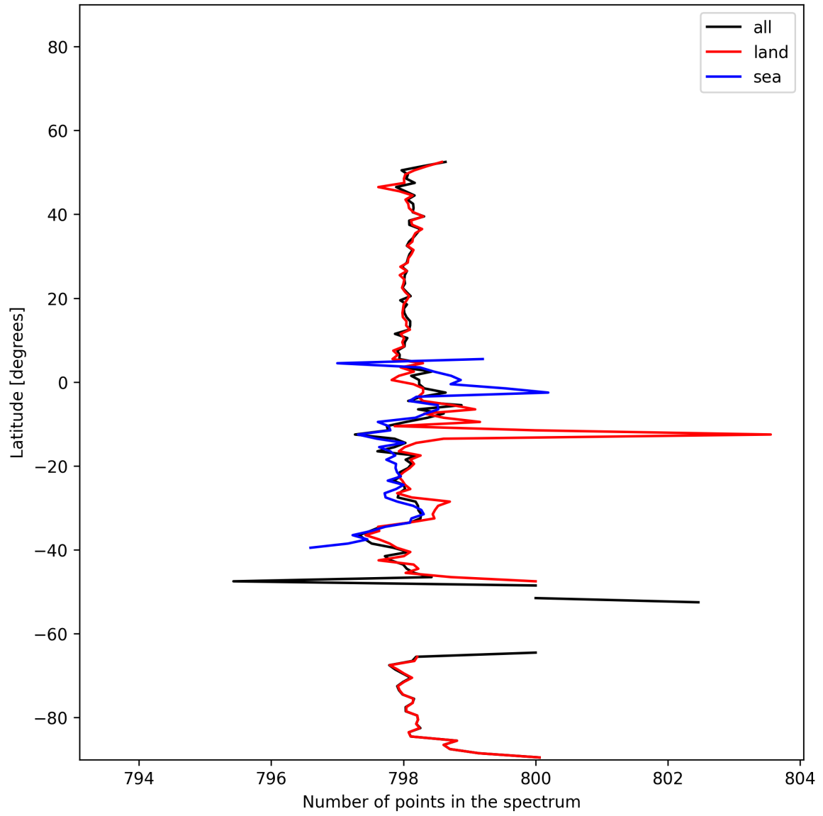
Figure 14: Zonal average of “Number of points in the spectrum” for 2025-12-05 to 2025-12-06.
