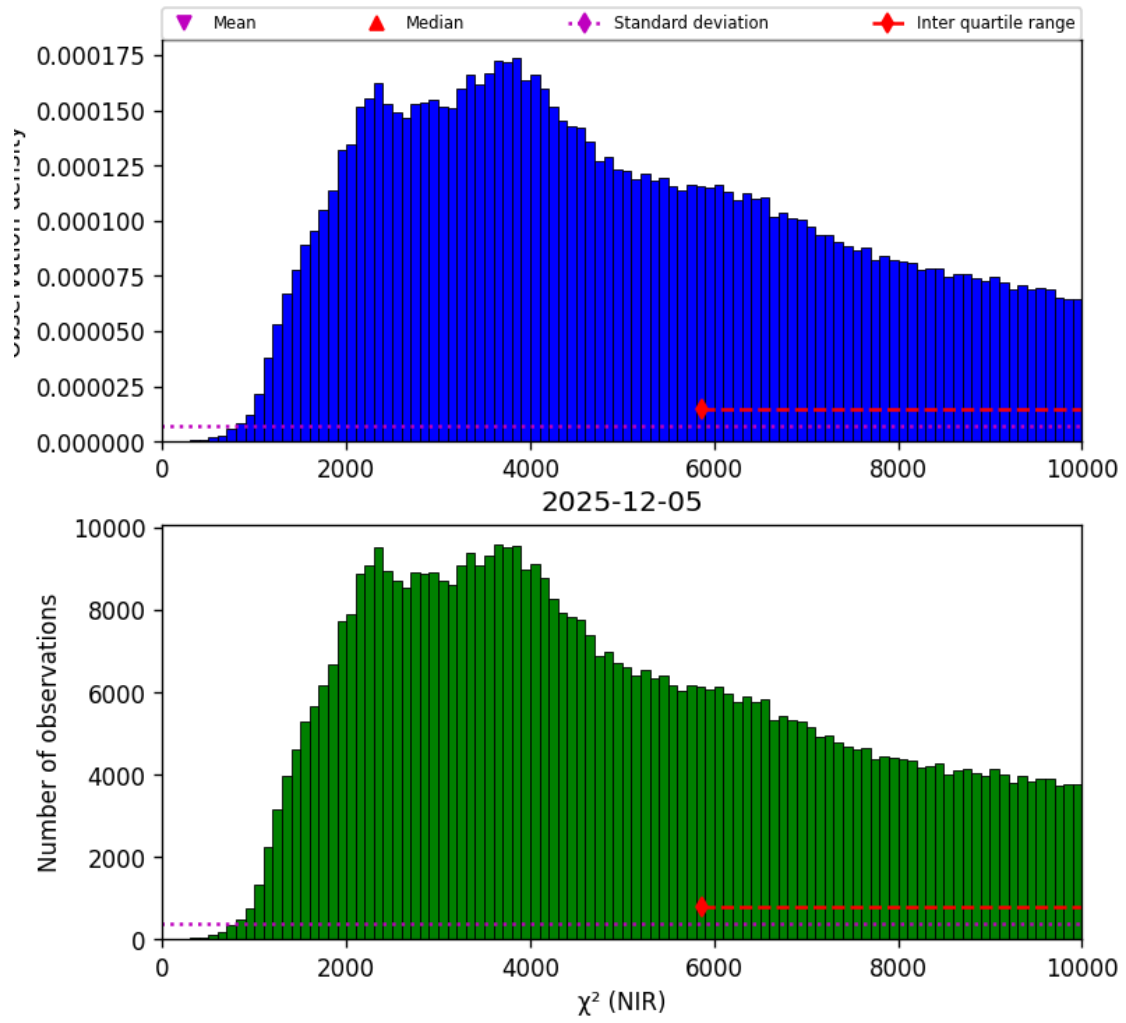
Figure 29: Histogram of “ \chi^2 (NIR)” for 2025-12-05 to 2025-12-06
