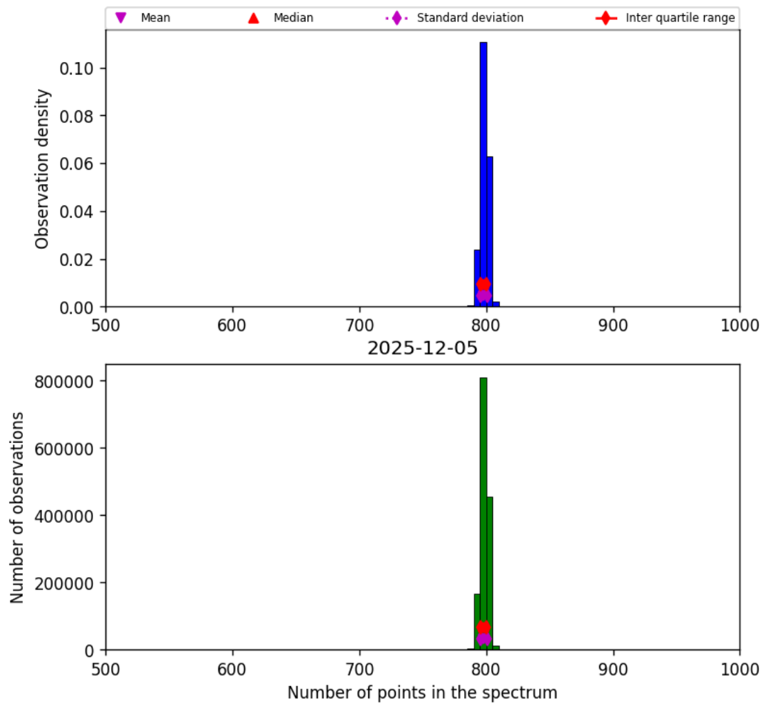
Figure 26: Histogram of “Number of points in the spectrum” for 2025-12-05 to 2025-12-06
