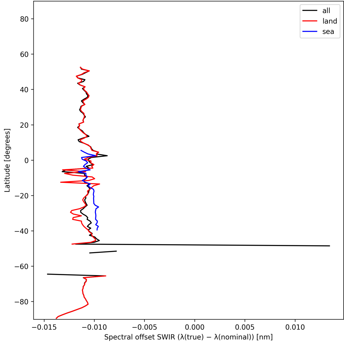
Figure 15: Zonal average of “Spectral offset SWIR ( \lambda_{\text{true}} - \lambda_{\text{nominal}} )” for 2025-12-05 to 2025-12-06.
