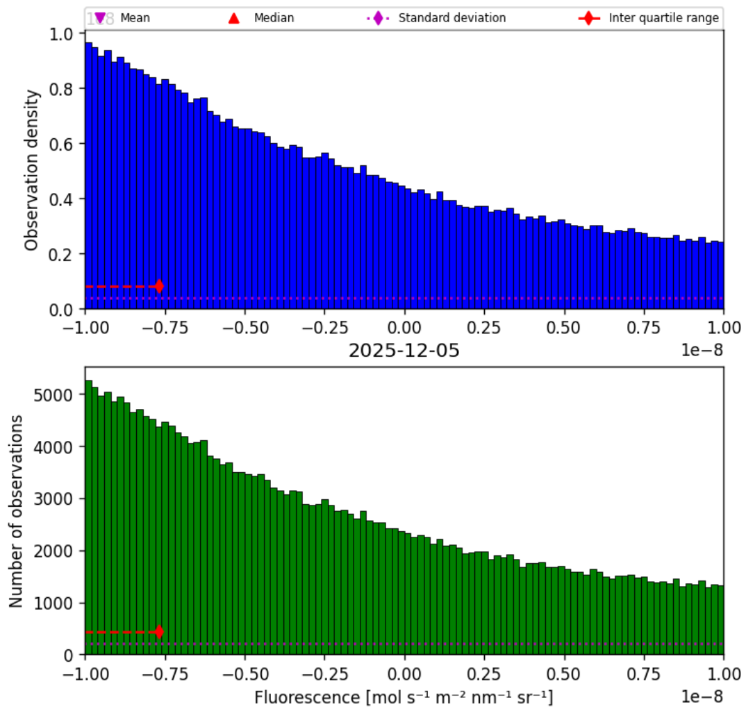
Figure 32: Histogram of “Fluorescence” for 2025-12-05 to 2025-12-06
