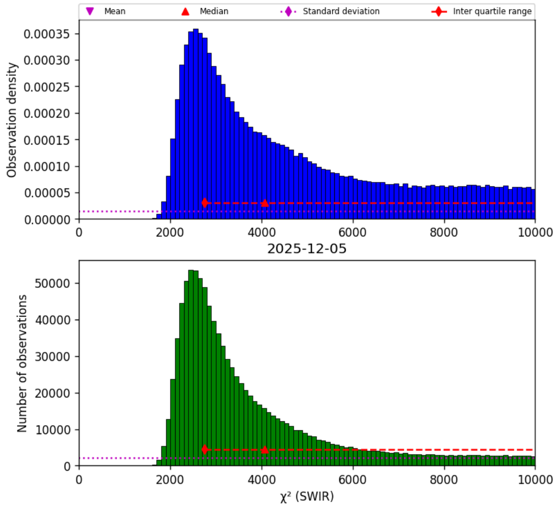
Figure 28: Histogram of " \chi^2 (SWIR)" for 2025-12-05 to 2025-12-06
