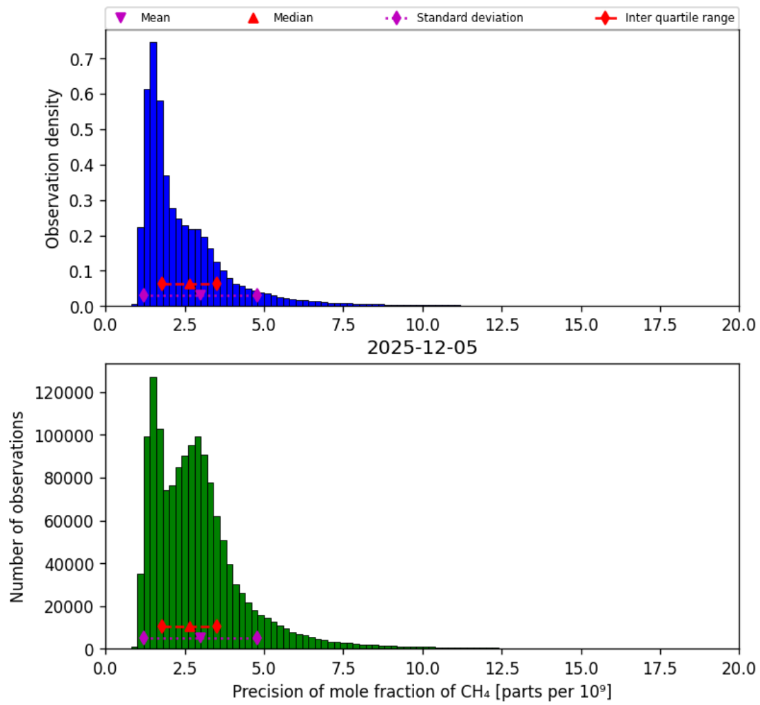
Figure 24: Histogram of “Precision of mole fraction of CH 4 ” for 2025-12-05 to 2025-12-06
