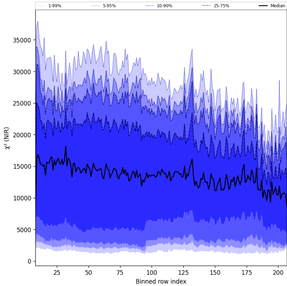
Figure 41: Along track statistics of “ \chi^2 (NIR)” for 2025-12-05 to 2025-12-06
