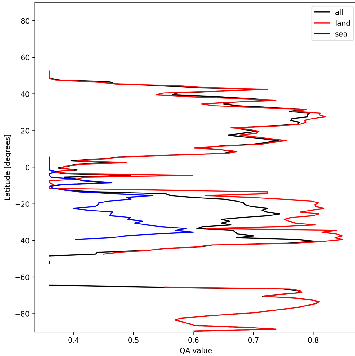
Figure 10: Zonal average of “QA value” for 2025-12-05 to 2025-12-06.
