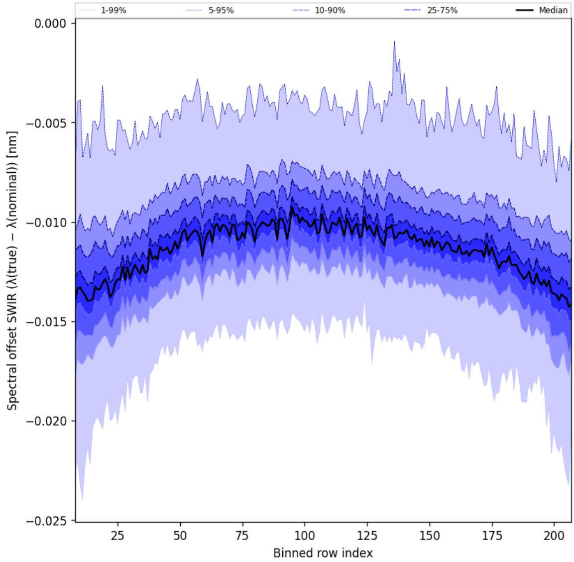
Figure 39: Along track statistics of “Spectral offset SWIR ( \lambda_{\text{true}} - \lambda_{\text{nominal}} )” for 2025-12-05 to 2025-12-06
