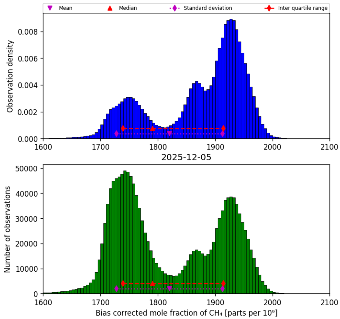
Figure 25: Histogram of “Bias corrected mole fraction of CH 4 ” for 2025-12-05 to 2025-12-06
