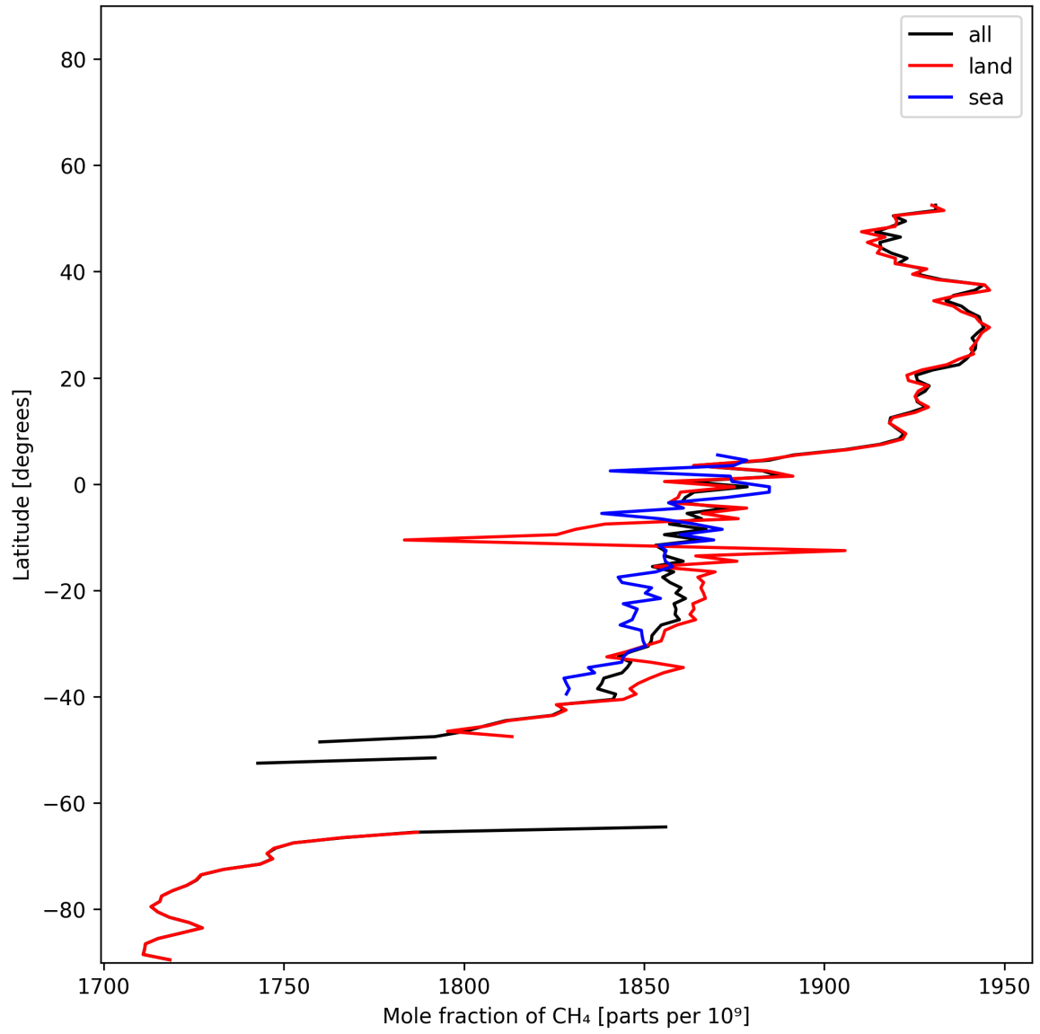
Figure 11: Zonal average of “Mole fraction of \text{CH}_4 ” for 2025-12-05 to 2025-12-06.
