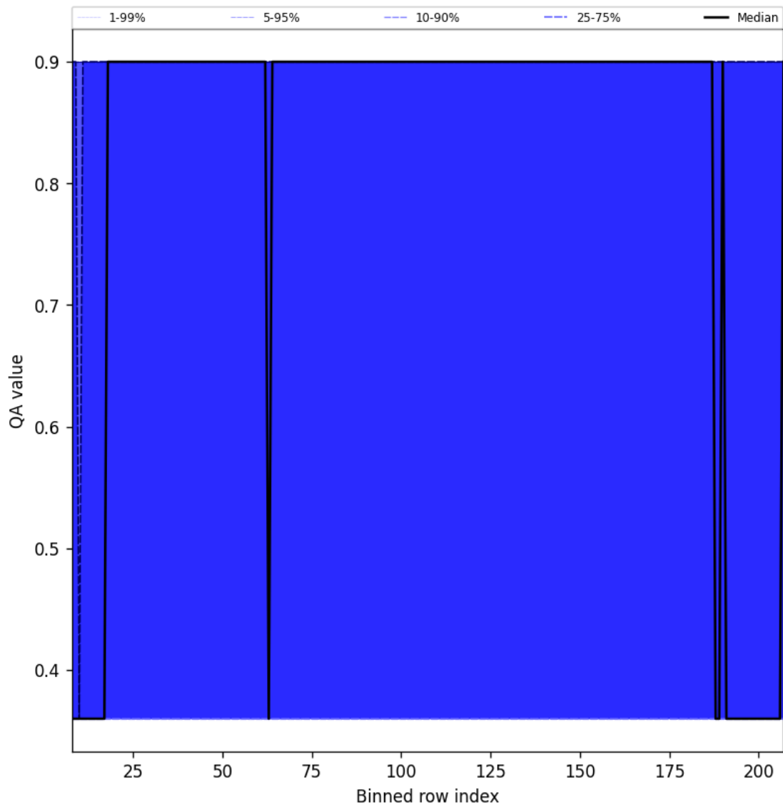
Figure 34: Along track statistics of “QA value” for 2025-12-05 to 2025-12-06
