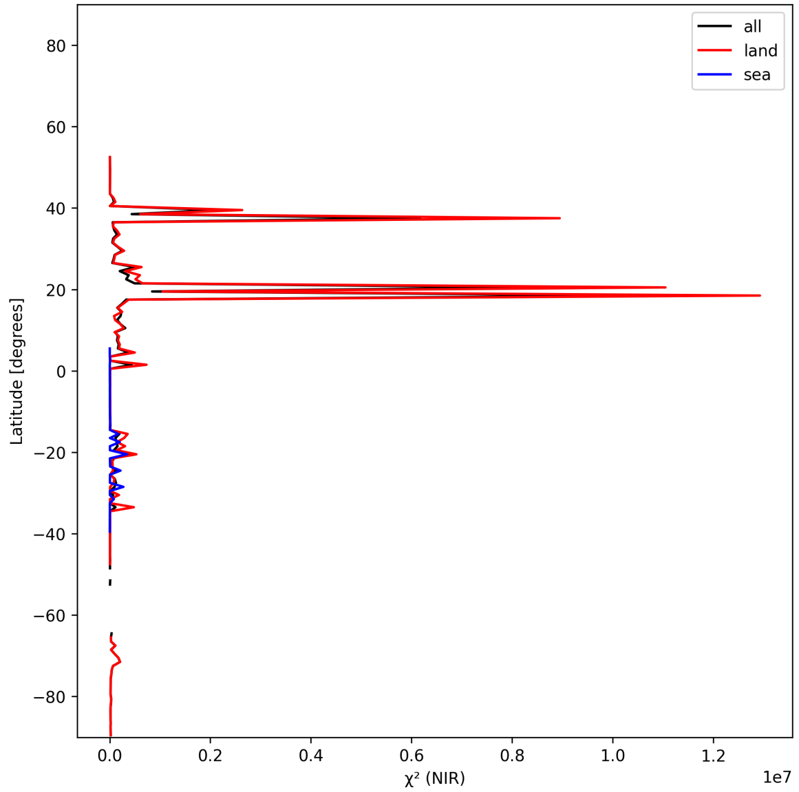
Figure 17: Zonal average of “ \chi^2 (NIR)” for 2025-12-05 to 2025-12-06.
