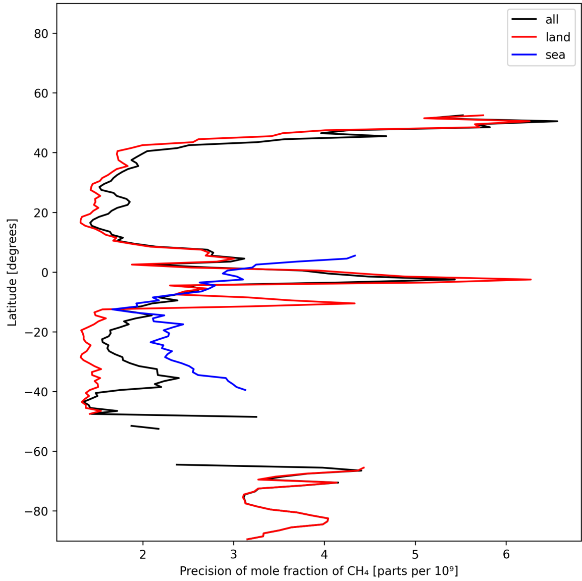
Figure 12: Zonal average of “Precision of mole fraction of CH 4 ” for 2025-12-05 to 2025-12-06.
