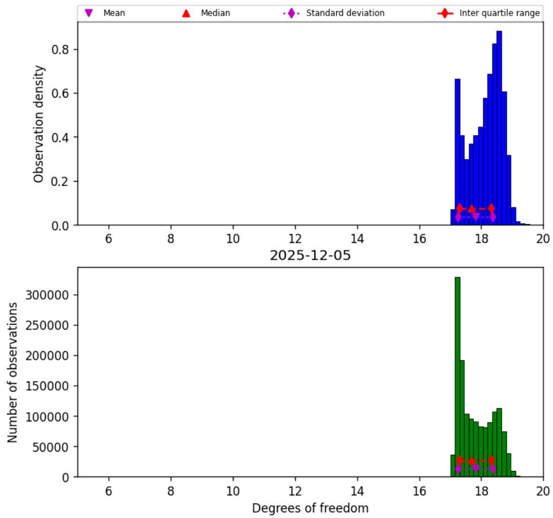
Figure 30: Histogram of “Degrees of freedom” for 2025-12-05 to 2025-12-06
