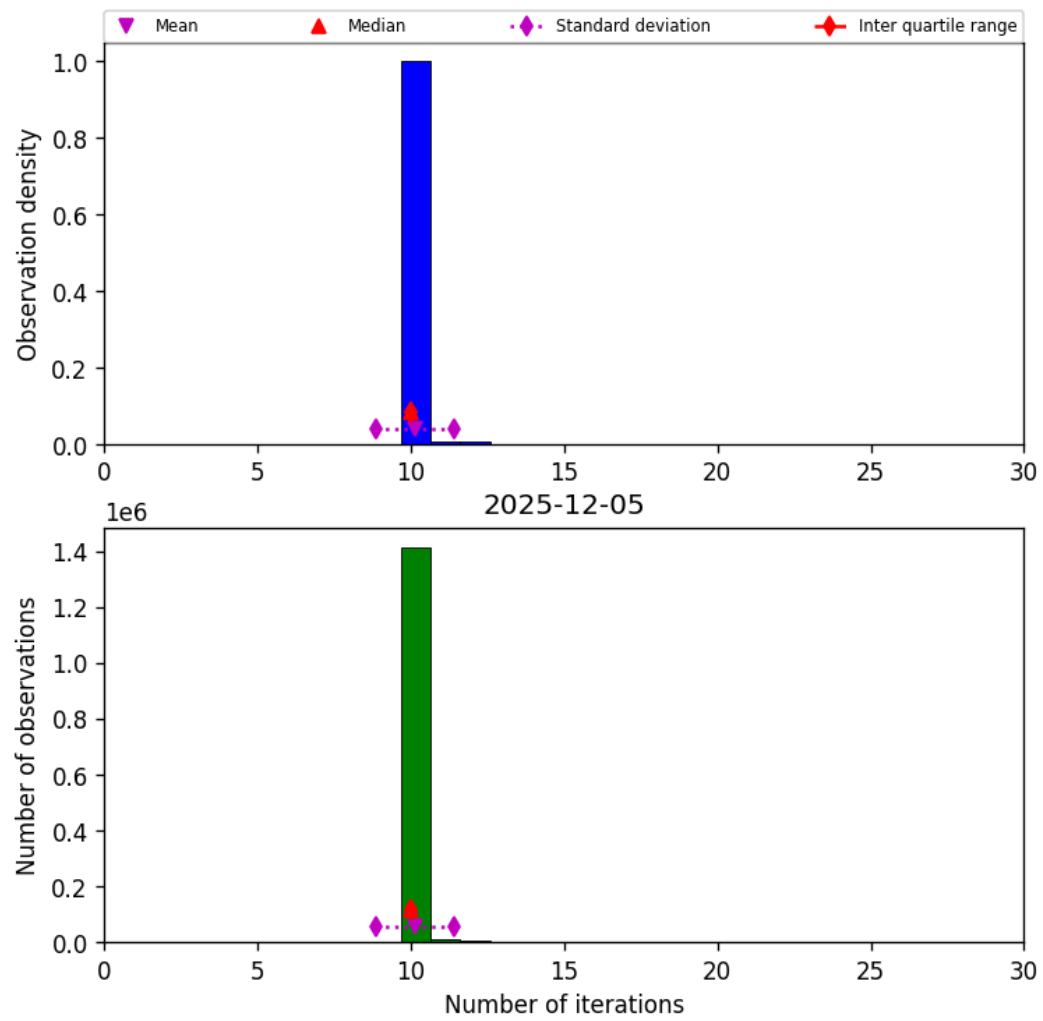
Figure 31: Histogram of “Number of iterations” for 2025-12-05 to 2025-12-06
