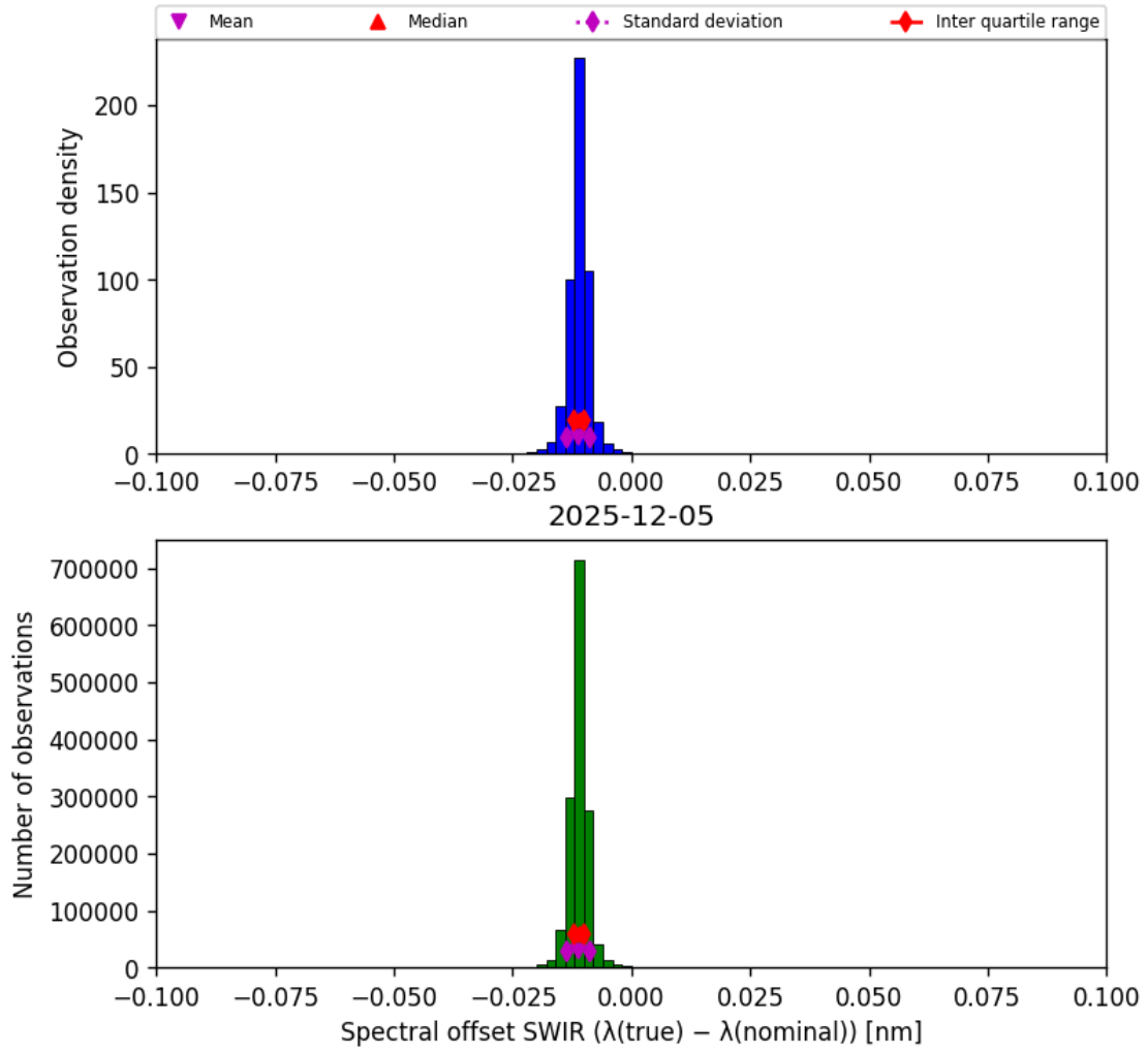
Figure 27: Histogram of “Spectral offset SWIR ( \lambda_{\text{true}} - \lambda_{\text{nominal}} )” for 2025-12-05 to 2025-12-06
