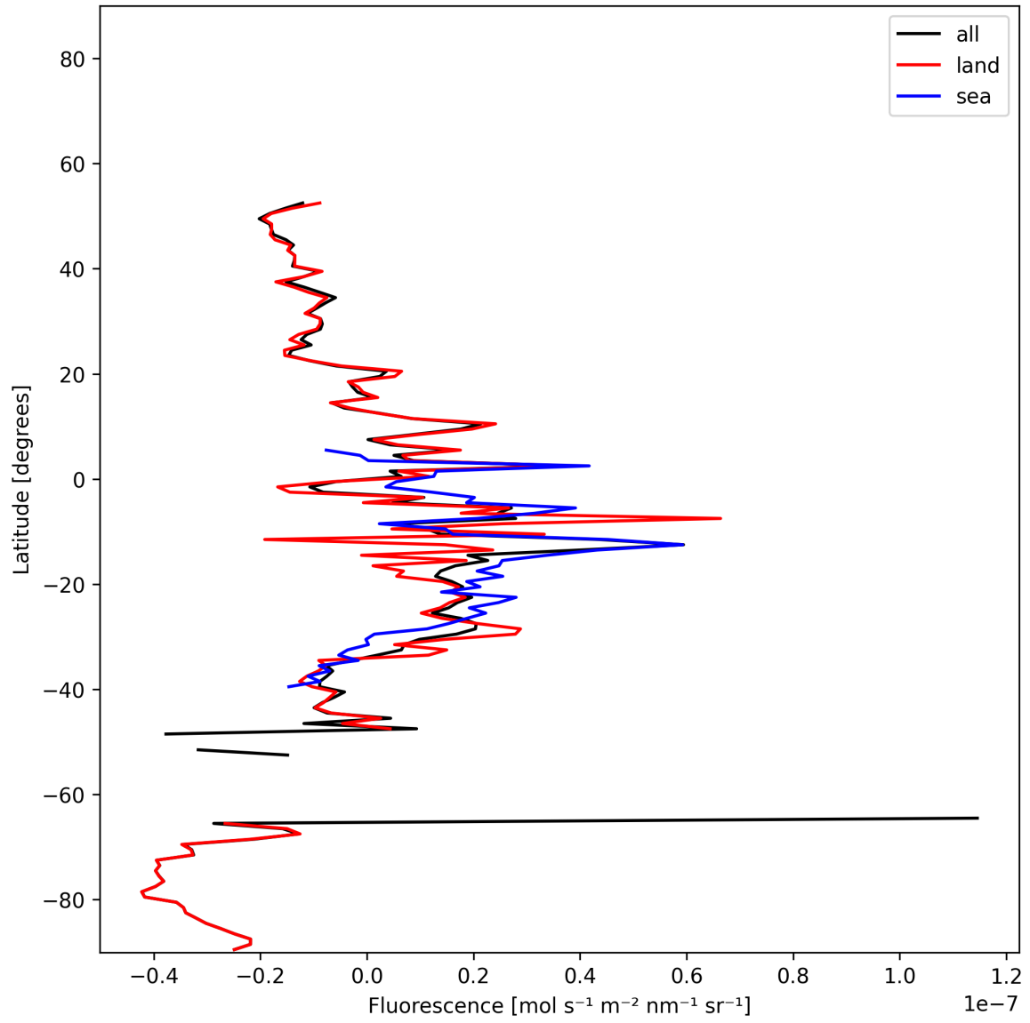
Figure 20: Zonal average of “Fluorescence” for 2025-12-05 to 2025-12-06.
