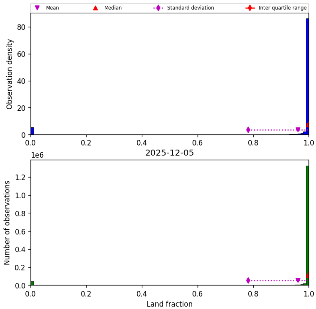
Figure 33: Histogram of “Land fraction” for 2025-12-05 to 2025-12-06
