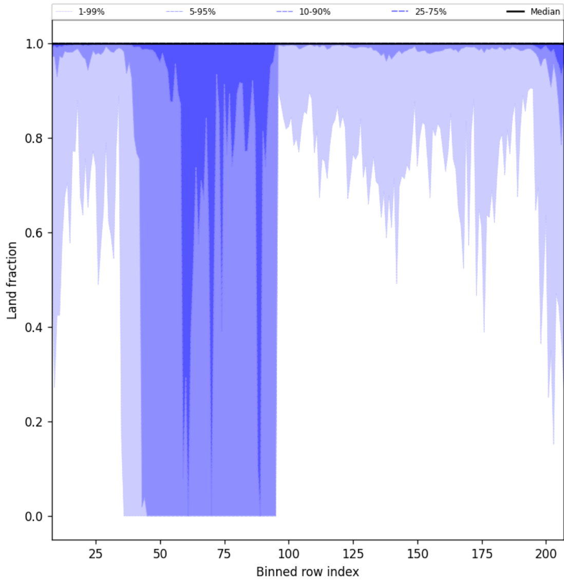
Figure 45: Along track statistics of "Land fraction" for 2025-12-05 to 2025-12-06
