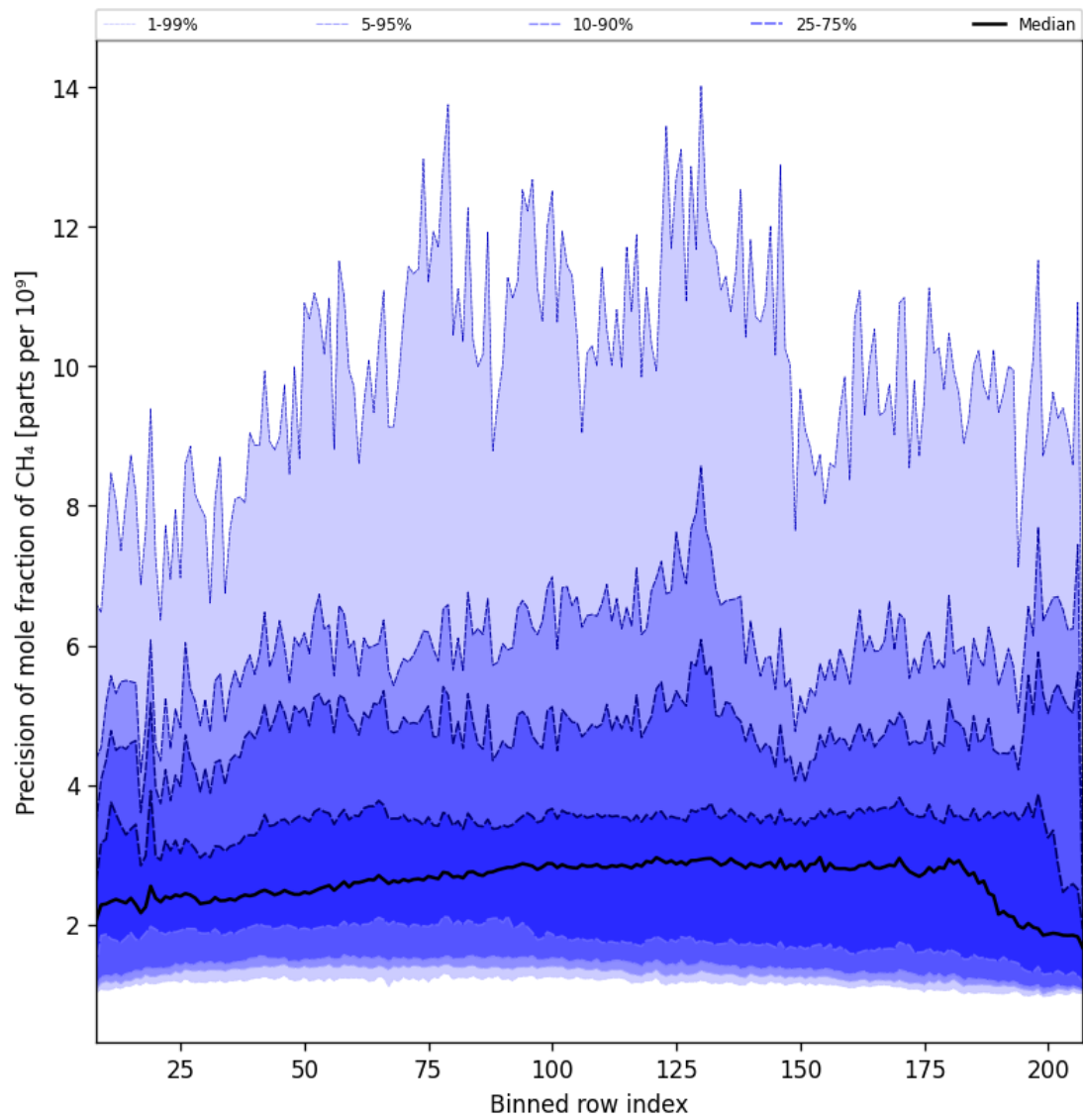
Figure 36: Along track statistics of “Precision of mole fraction of CH 4 ” for 2025-12-05 to 2025-12-06
