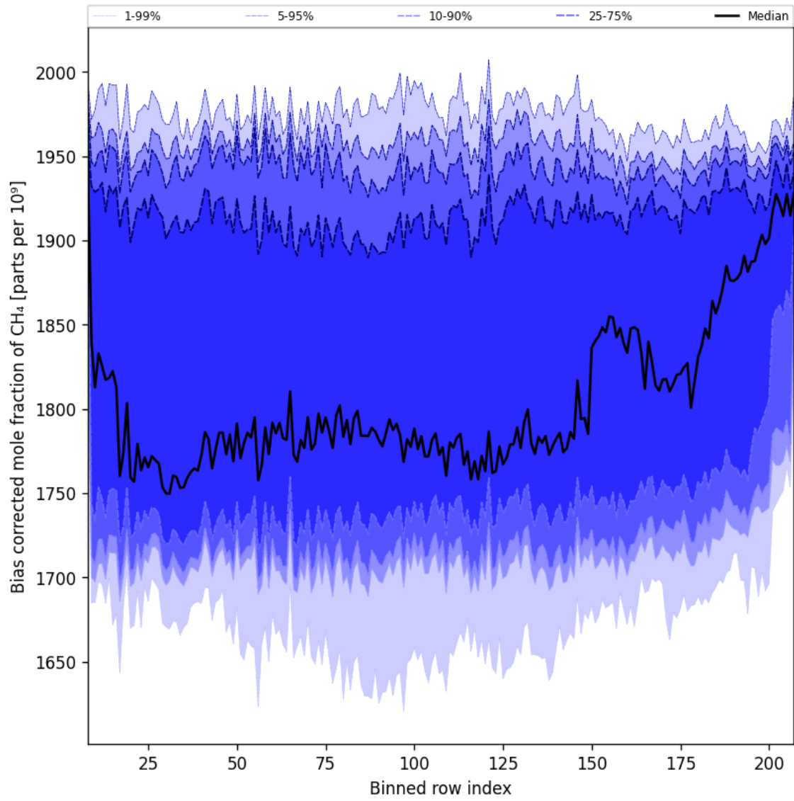
Figure 37: Along track statistics of “Bias corrected mole fraction of CH 4 ” for 2025-12-05 to 2025-12-06
