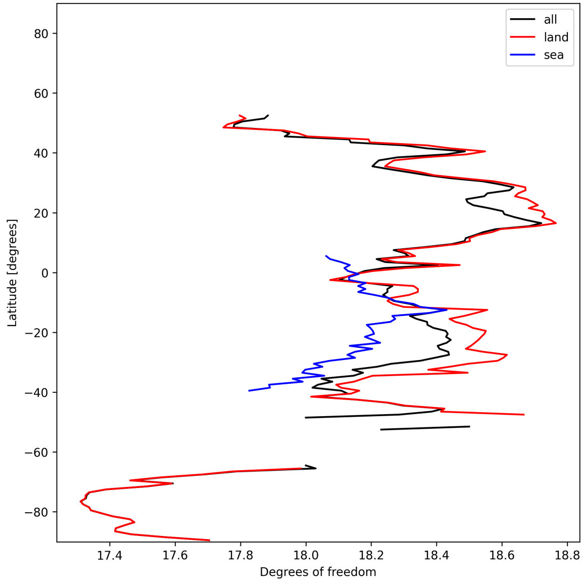
Figure 18: Zonal average of “Degrees of freedom” for 2025-12-05 to 2025-12-06.
