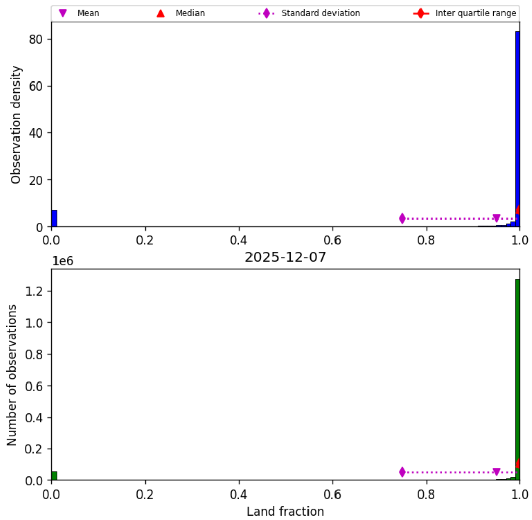
Figure 33: Histogram of “Land fraction” for 2025-12-07 to 2025-12-07
