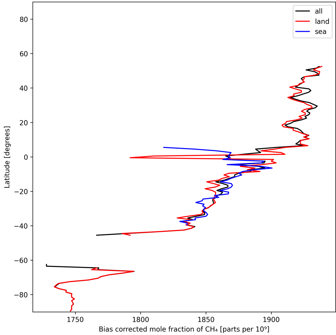
Figure 13: Zonal average of “Bias corrected mole fraction of \text{CH}_4 ” for 2025-12-07 to 2025-12-07.
