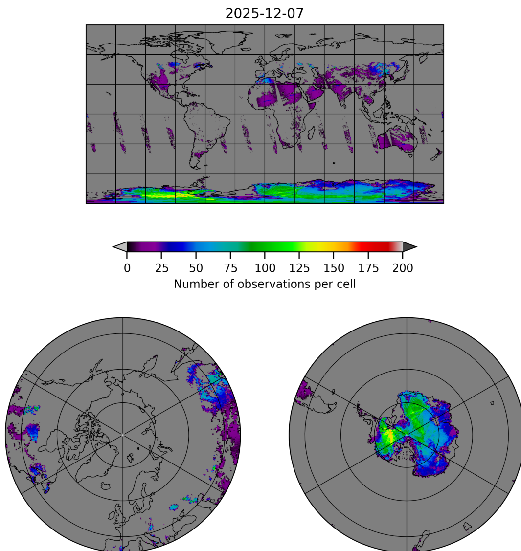
Figure 9: Map of the number of observations for 2025-12-07 to 2025-12-07
