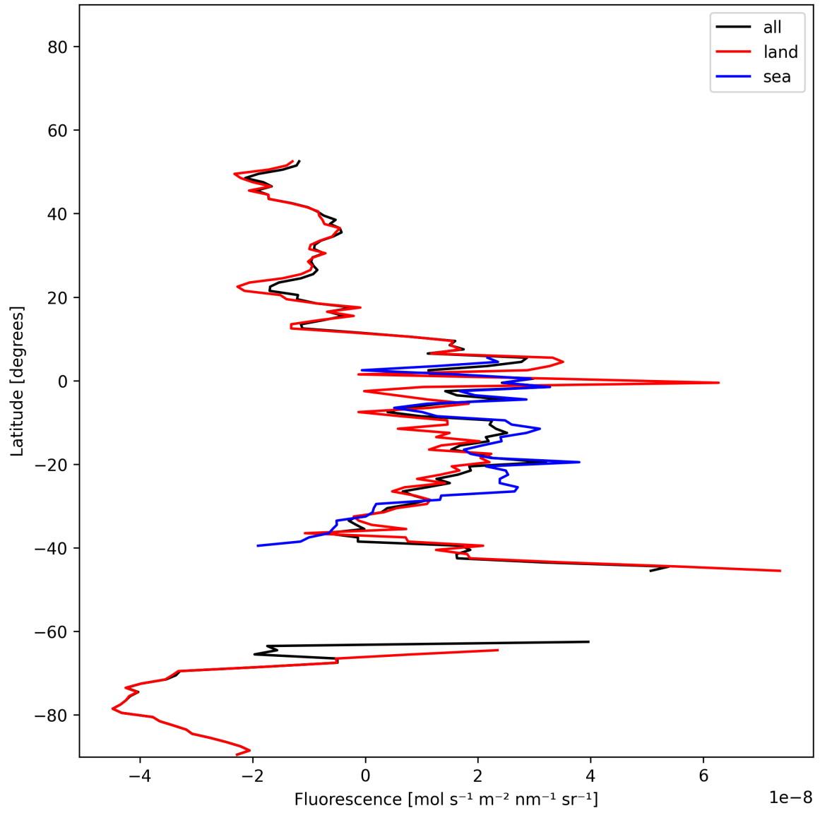
Figure 20: Zonal average of “Fluorescence” for 2025-12-07 to 2025-12-07.
