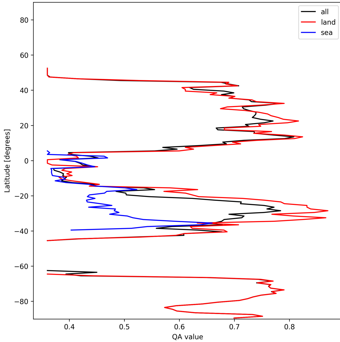
Figure 10: Zonal average of “QA value” for 2025-12-07 to 2025-12-07.
