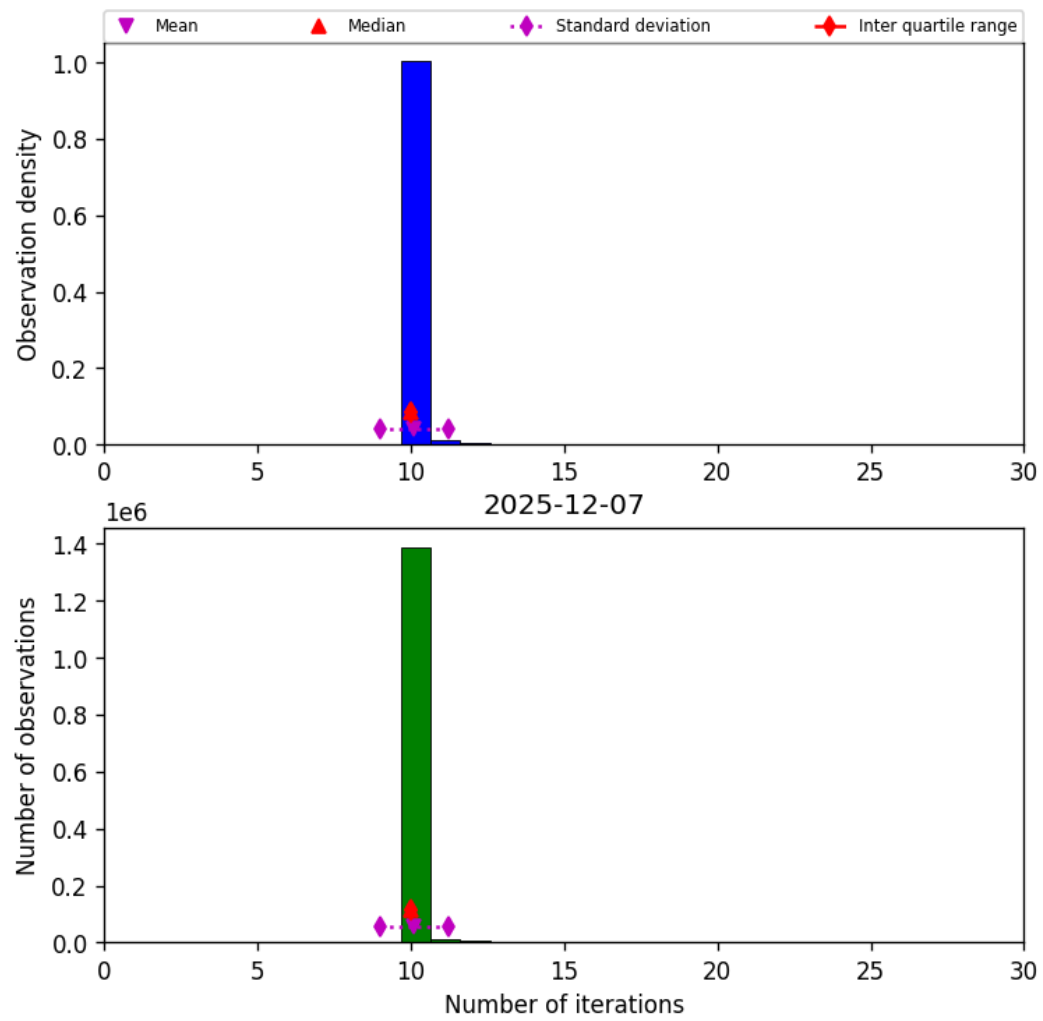
Figure 31: Histogram of “Number of iterations” for 2025-12-07 to 2025-12-07
