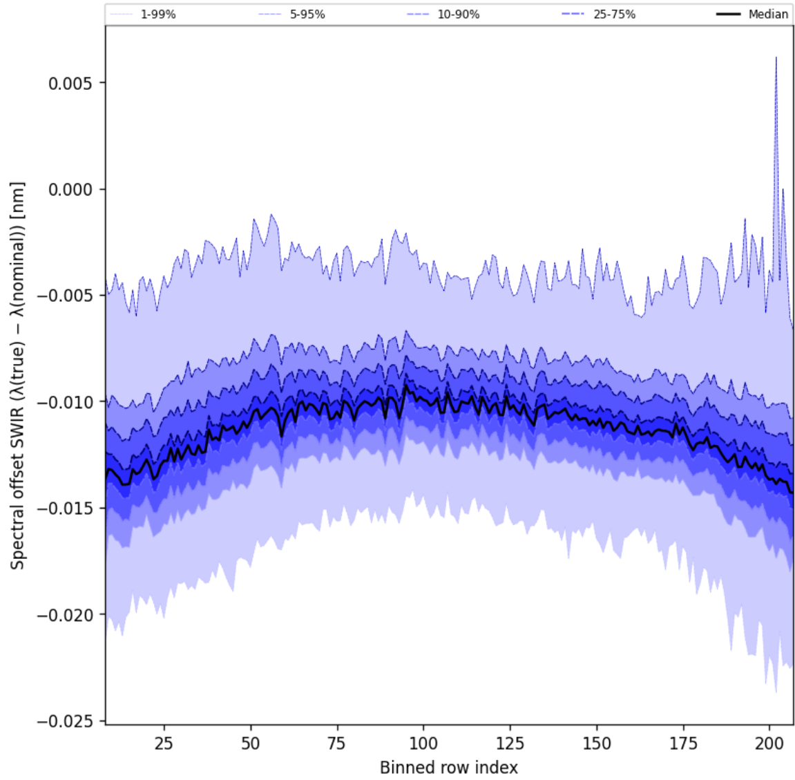
Figure 39: Along track statistics of “Spectral offset SWIR ( \lambda_{\text{true}} - \lambda_{\text{nominal}} )” for 2025-12-07 to 2025-12-07
