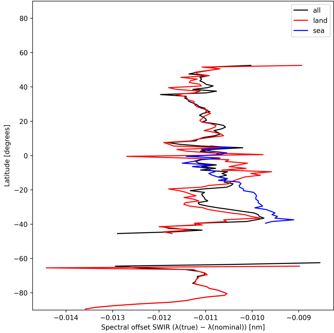
Figure 15: Zonal average of “Spectral offset SWIR ( \lambda_{\text{true}} - \lambda_{\text{nominal}} )” for 2025-12-07 to 2025-12-07.
