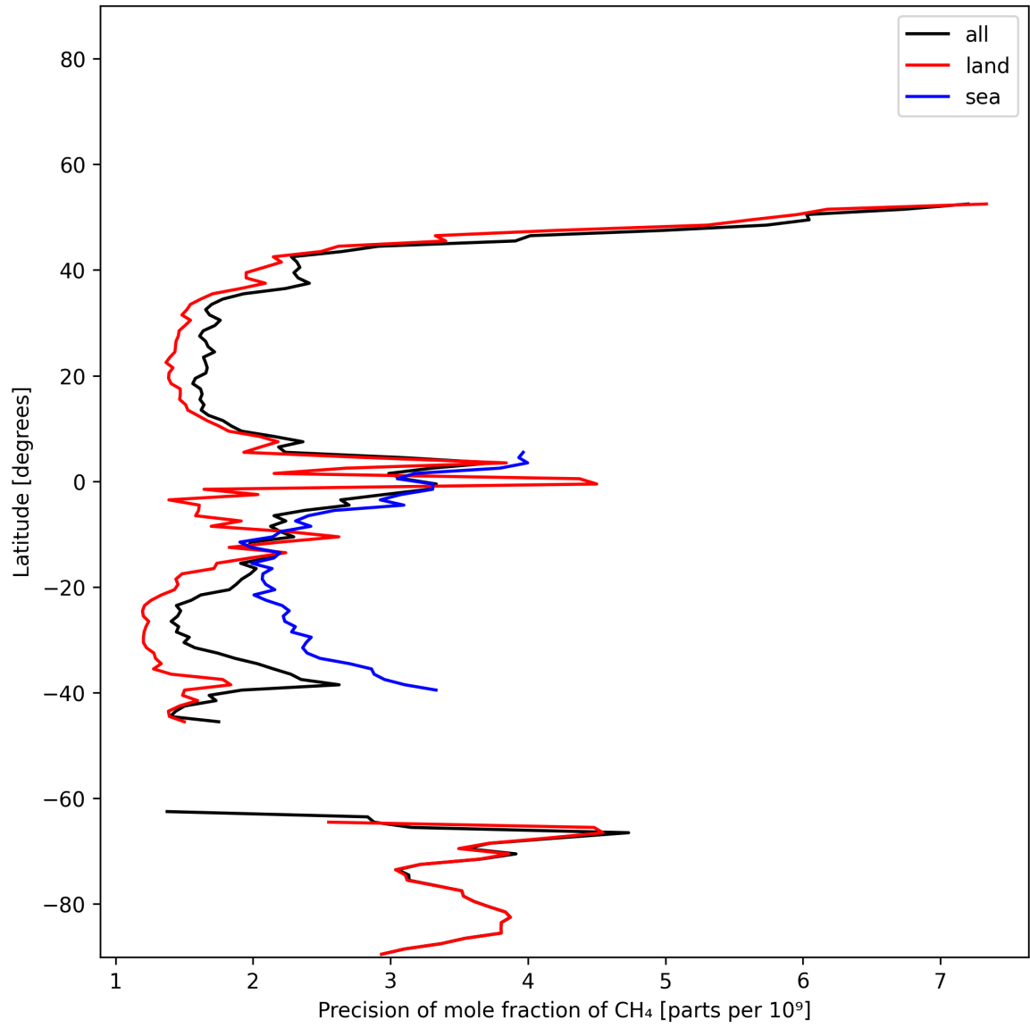
Figure 12: Zonal average of “Precision of mole fraction of CH 4 ” for 2025-12-07 to 2025-12-07.
