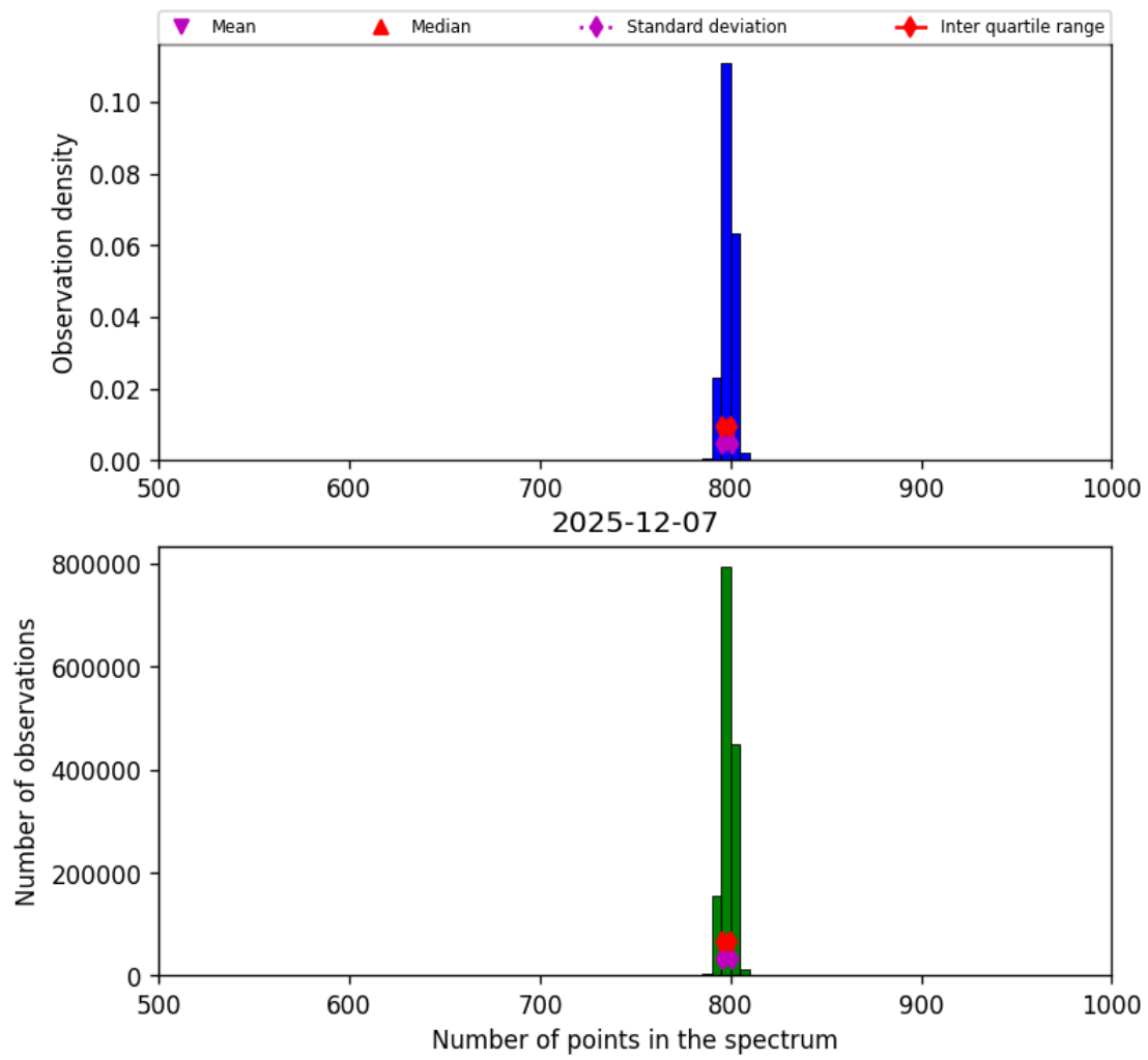
Figure 26: Histogram of “Number of points in the spectrum” for 2025-12-07 to 2025-12-07
