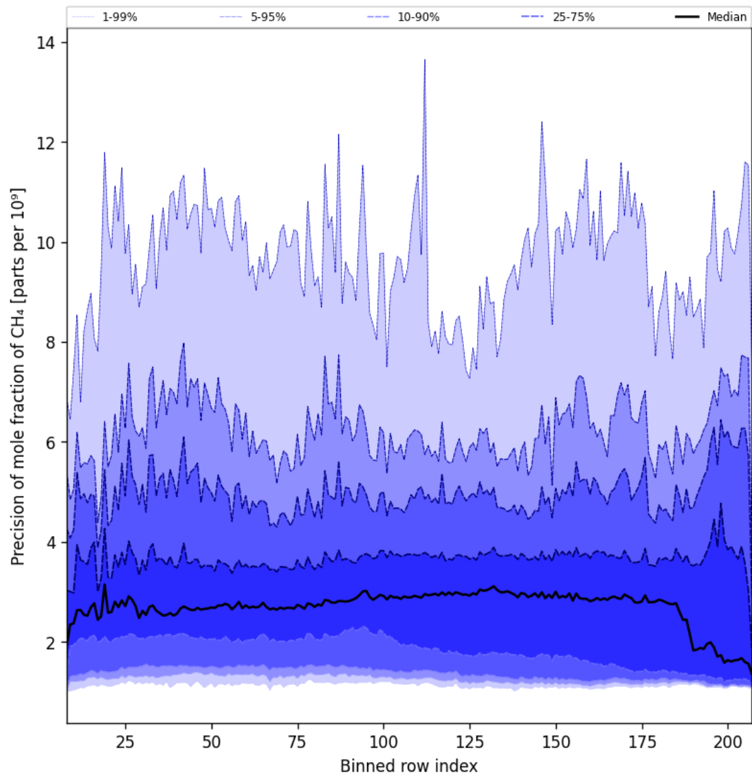
Figure 36: Along track statistics of "Precision of mole fraction of CH 4 " for 2025-12-07 to 2025-12-07
