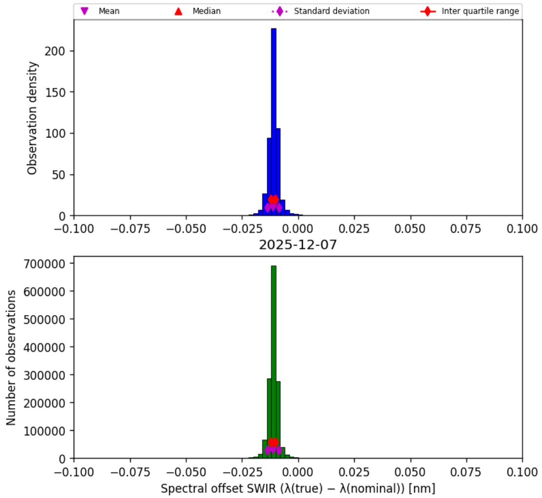
Figure 27: Histogram of “Spectral offset SWIR ( \lambda_{\text{true}} - \lambda_{\text{nominal}} )” for 2025-12-07 to 2025-12-07
