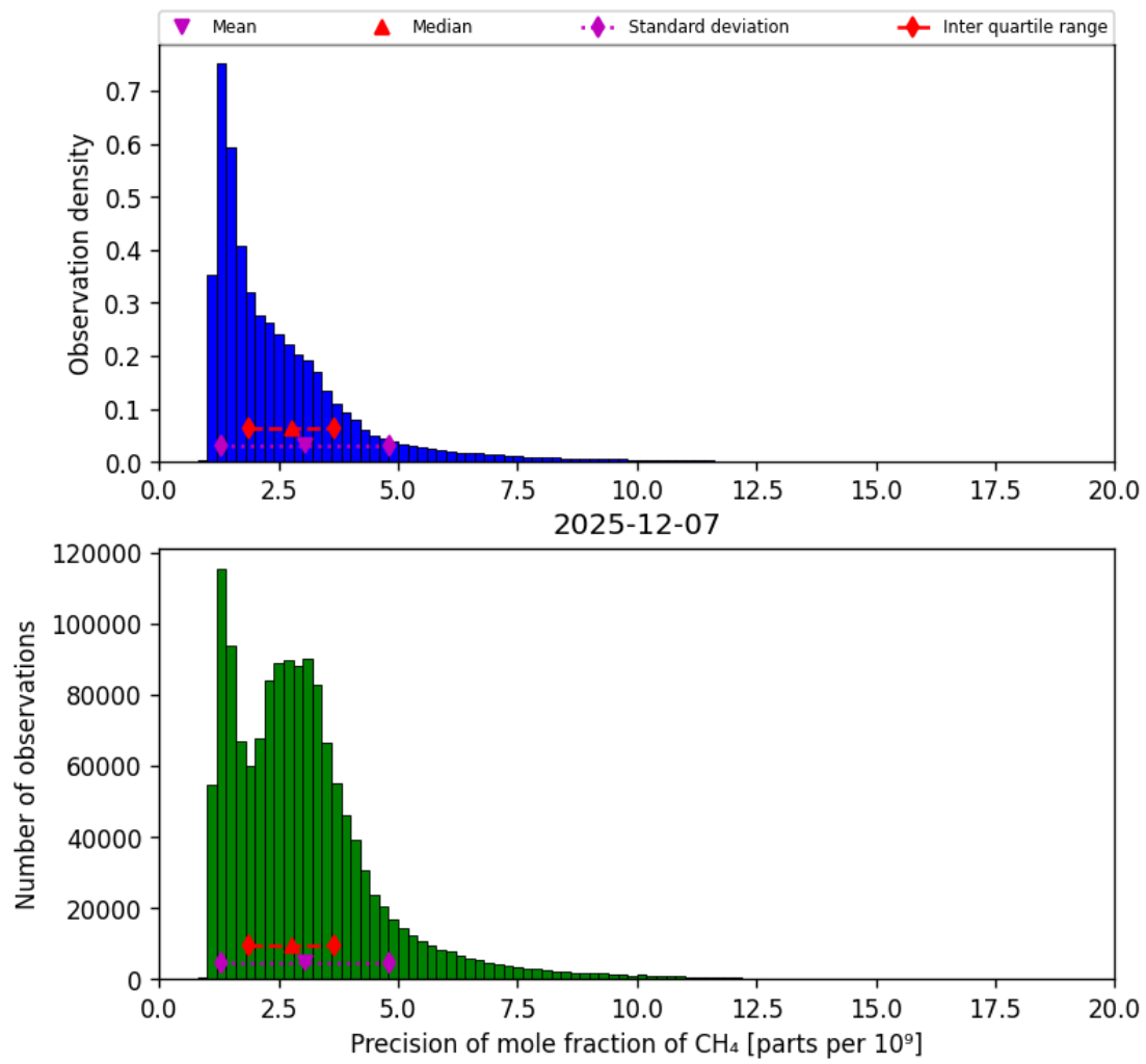
Figure 24: Histogram of “Precision of mole fraction of CH 4 ” for 2025-12-07 to 2025-12-07
