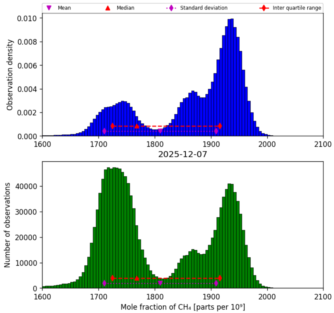
Figure 23: Histogram of “Mole fraction of CH 4 ” for 2025-12-07 to 2025-12-07
