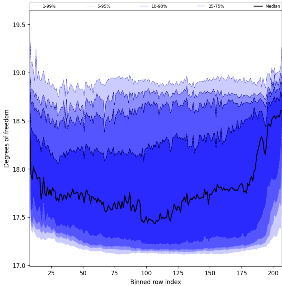
Figure 42: Along track statistics of “Degrees of freedom” for 2025-12-07 to 2025-12-07
