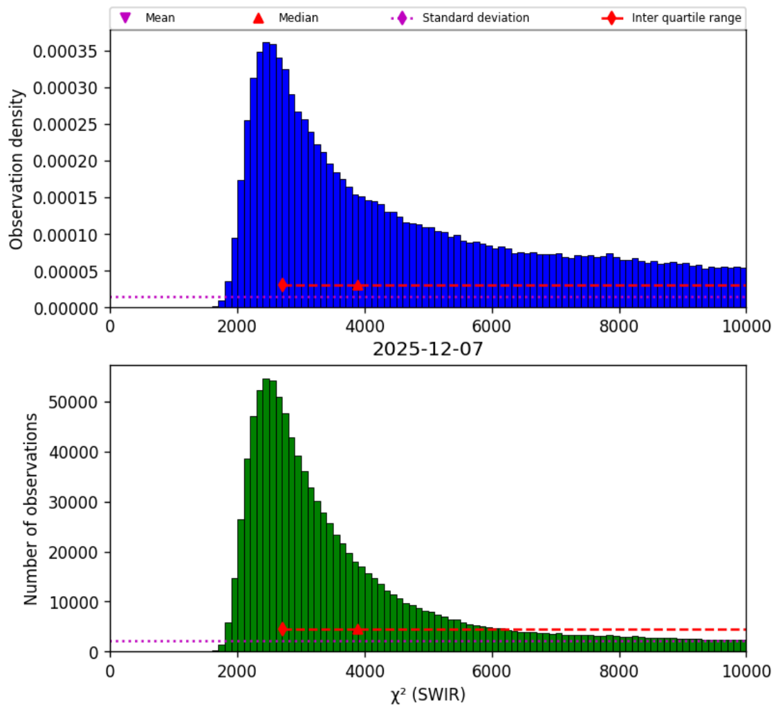
Figure 28: Histogram of “ \chi^2 (SWIR)” for 2025-12-07 to 2025-12-07
