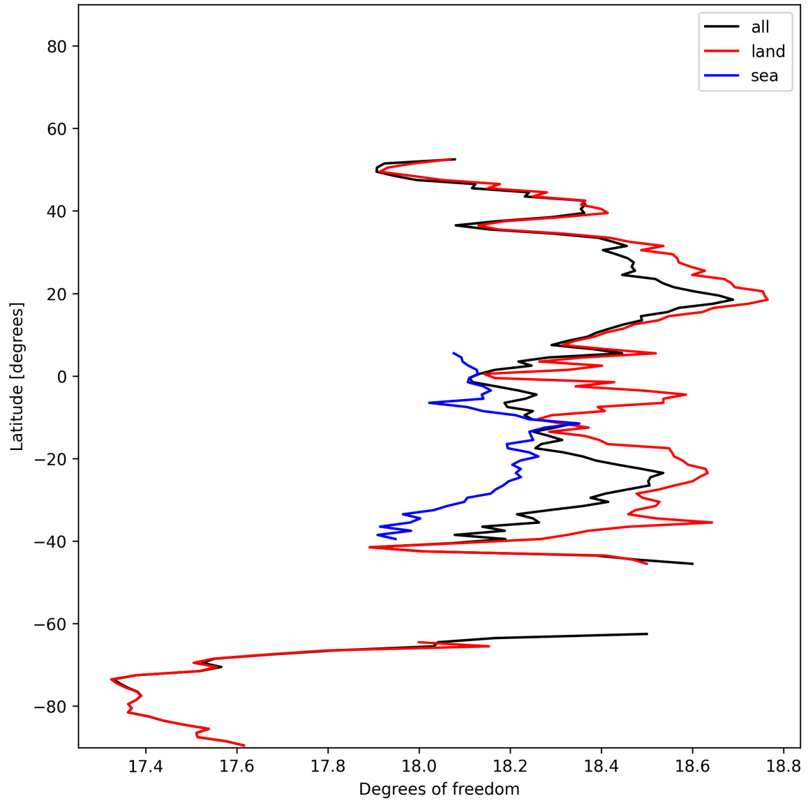
Figure 18: Zonal average of “Degrees of freedom” for 2025-12-07 to 2025-12-07.
