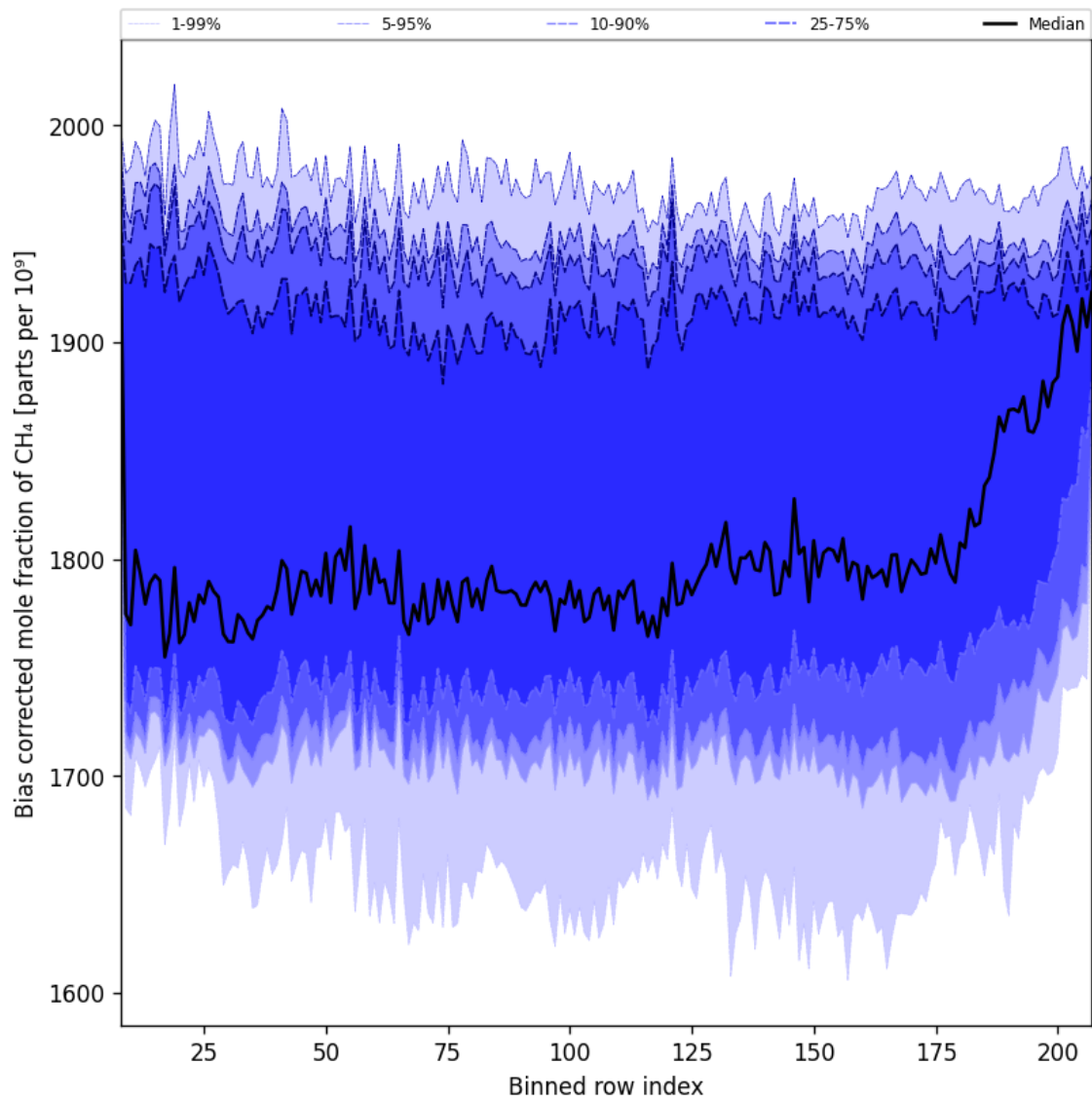
Figure 37: Along track statistics of “Bias corrected mole fraction of CH 4 ” for 2025-12-07 to 2025-12-07
