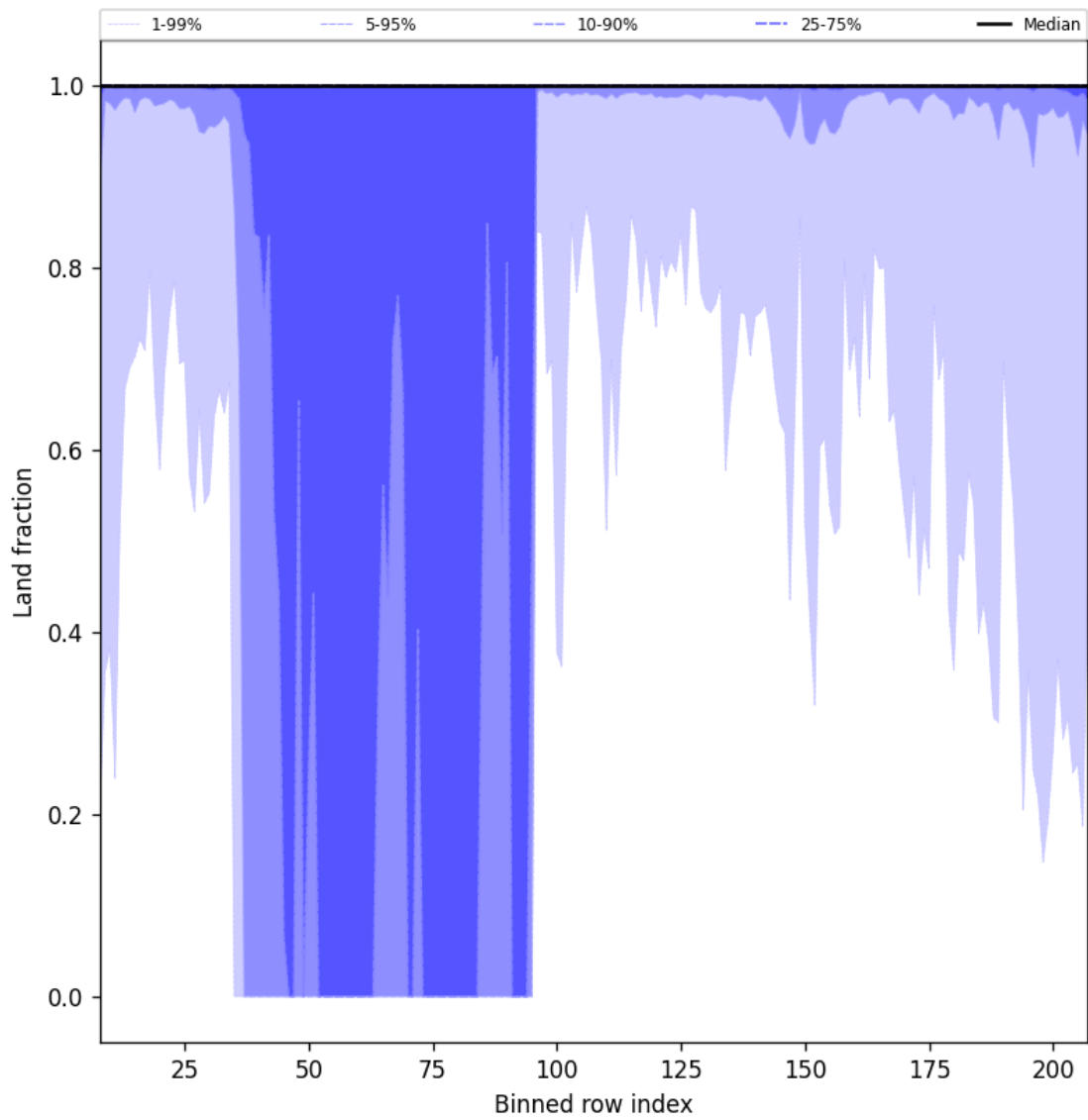
Figure 45: Along track statistics of “Land fraction” for 2025-12-07 to 2025-12-07
