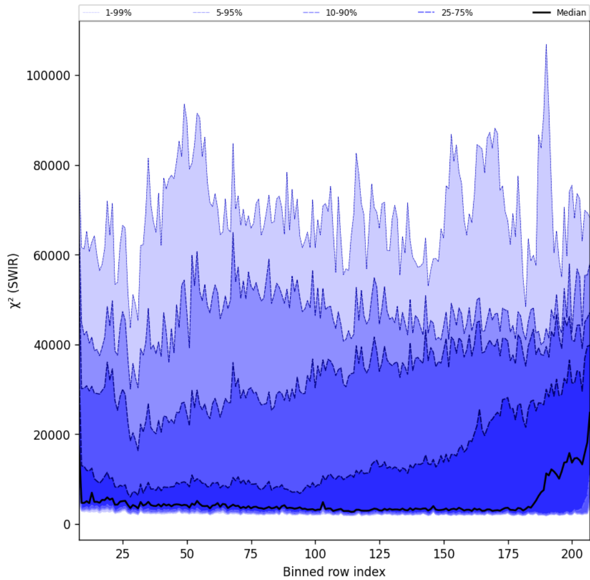
Figure 40: Along track statistics of “ \chi^2 (SWIR)” for 2025-12-07 to 2025-12-07
