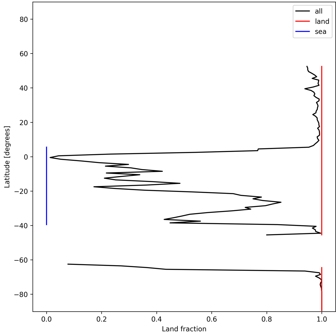
Figure 21: Zonal average of “Land fraction” for 2025-12-07 to 2025-12-07.
