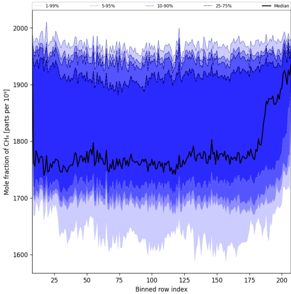
Figure 35: Along track statistics of “Mole fraction of CH 4 ” for 2025-12-07 to 2025-12-07
