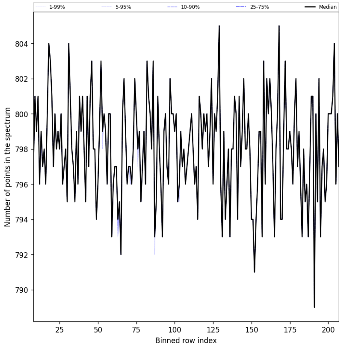
Figure 38: Along track statistics of “Number of points in the spectrum” for 2025-12-07 to 2025-12-07
