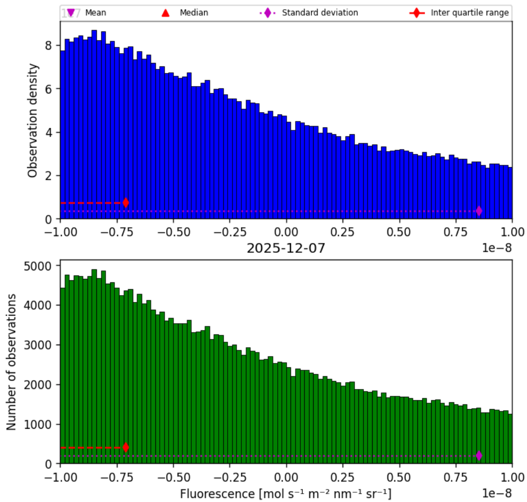
Figure 32: Histogram of “Fluorescence” for 2025-12-07 to 2025-12-07
