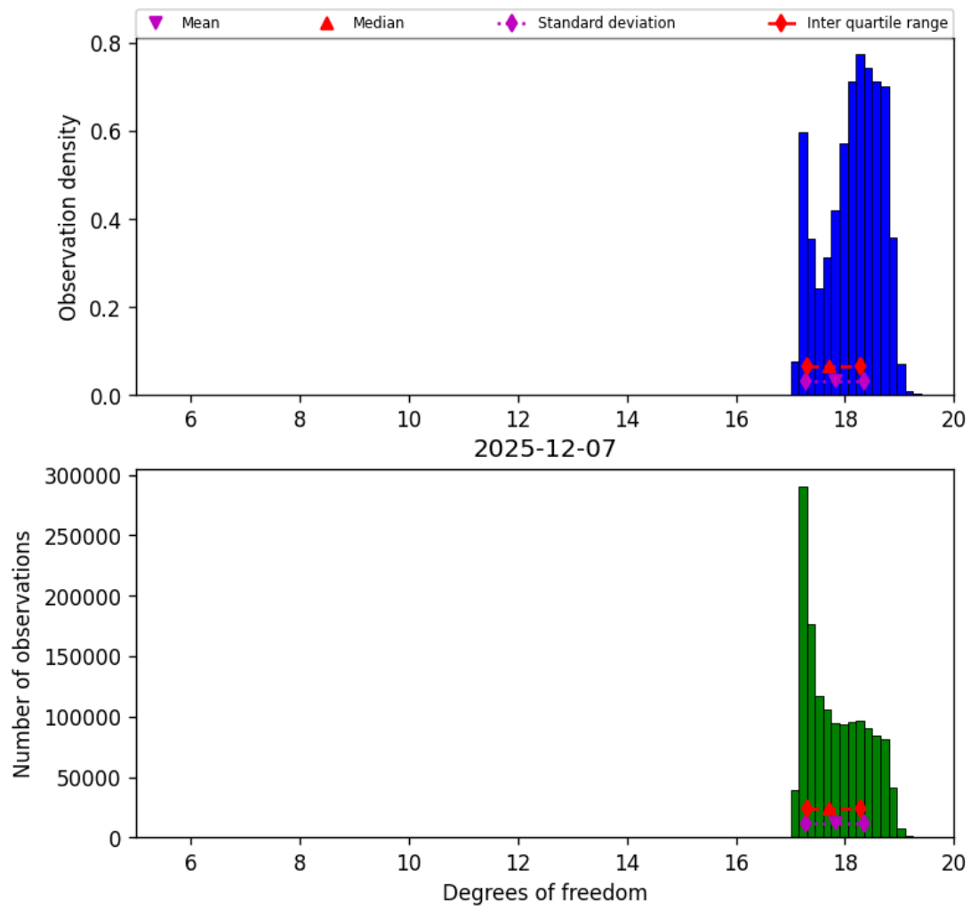
Figure 30: Histogram of “Degrees of freedom” for 2025-12-07 to 2025-12-07
