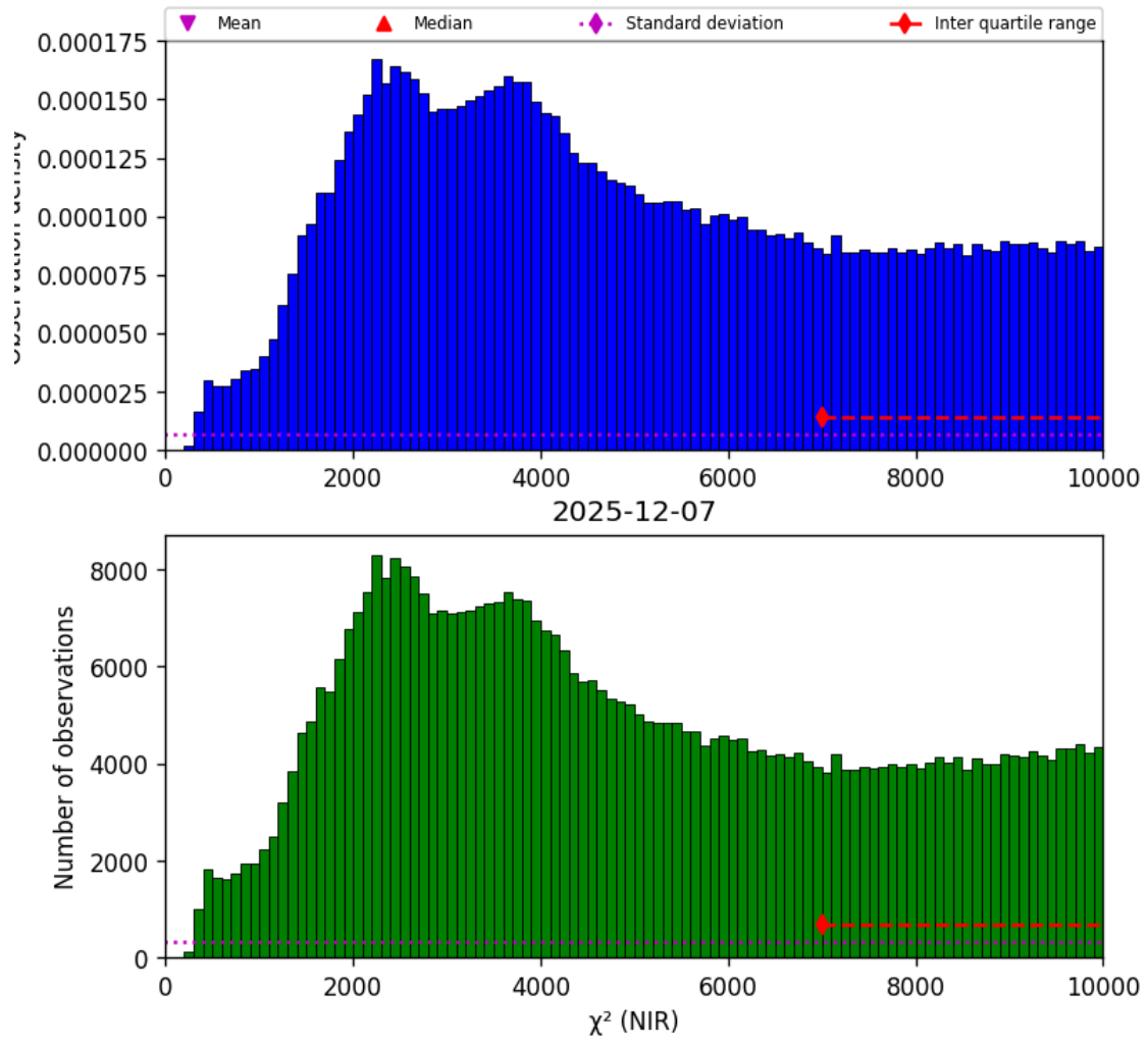
Figure 29: Histogram of “ \chi^2 (NIR)” for 2025-12-07 to 2025-12-07
