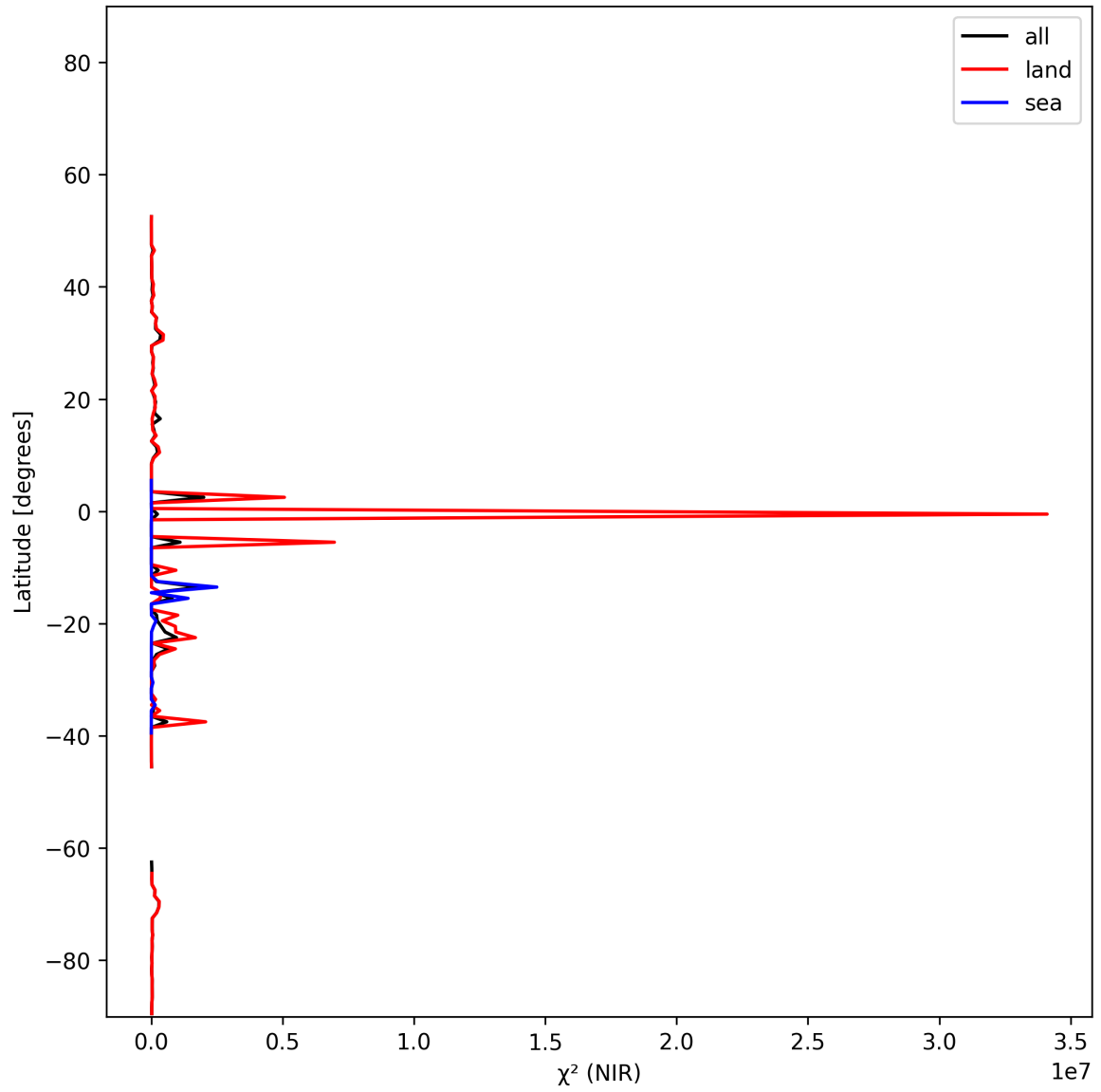
Figure 17: Zonal average of “ \chi^2 (NIR)” for 2025-12-07 to 2025-12-07.
