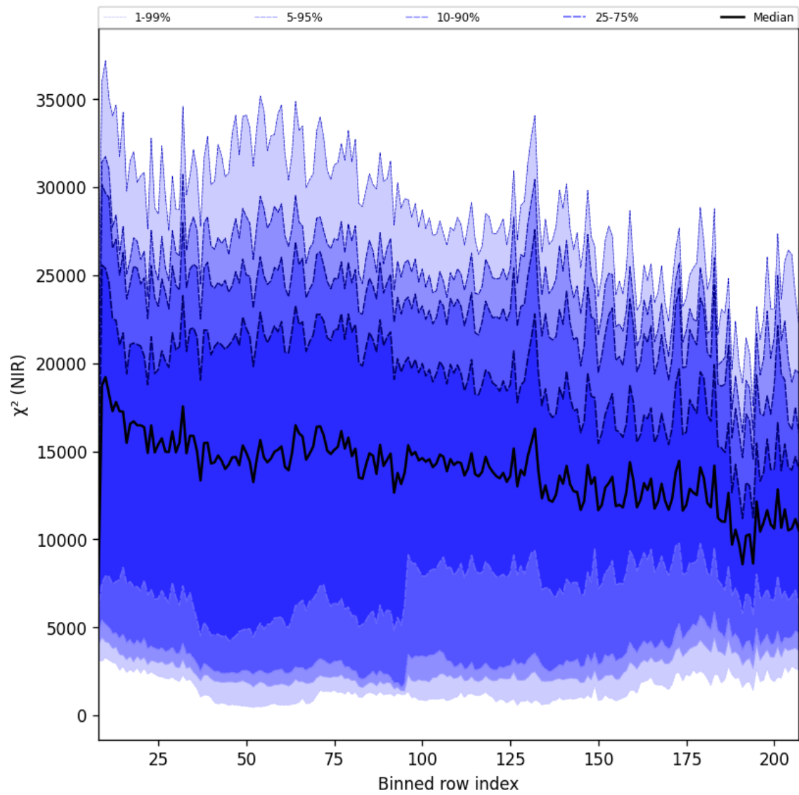
Figure 41: Along track statistics of “ \chi^2 (NIR)” for 2025-12-07 to 2025-12-07
