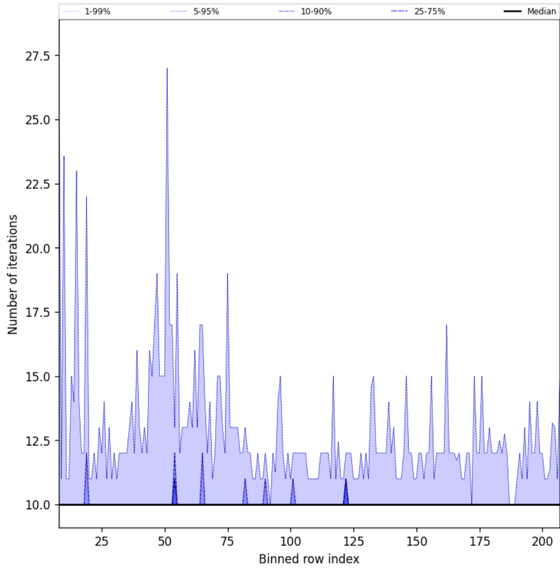
Figure 43: Along track statistics of “Number of iterations” for 2025-12-07 to 2025-12-07
