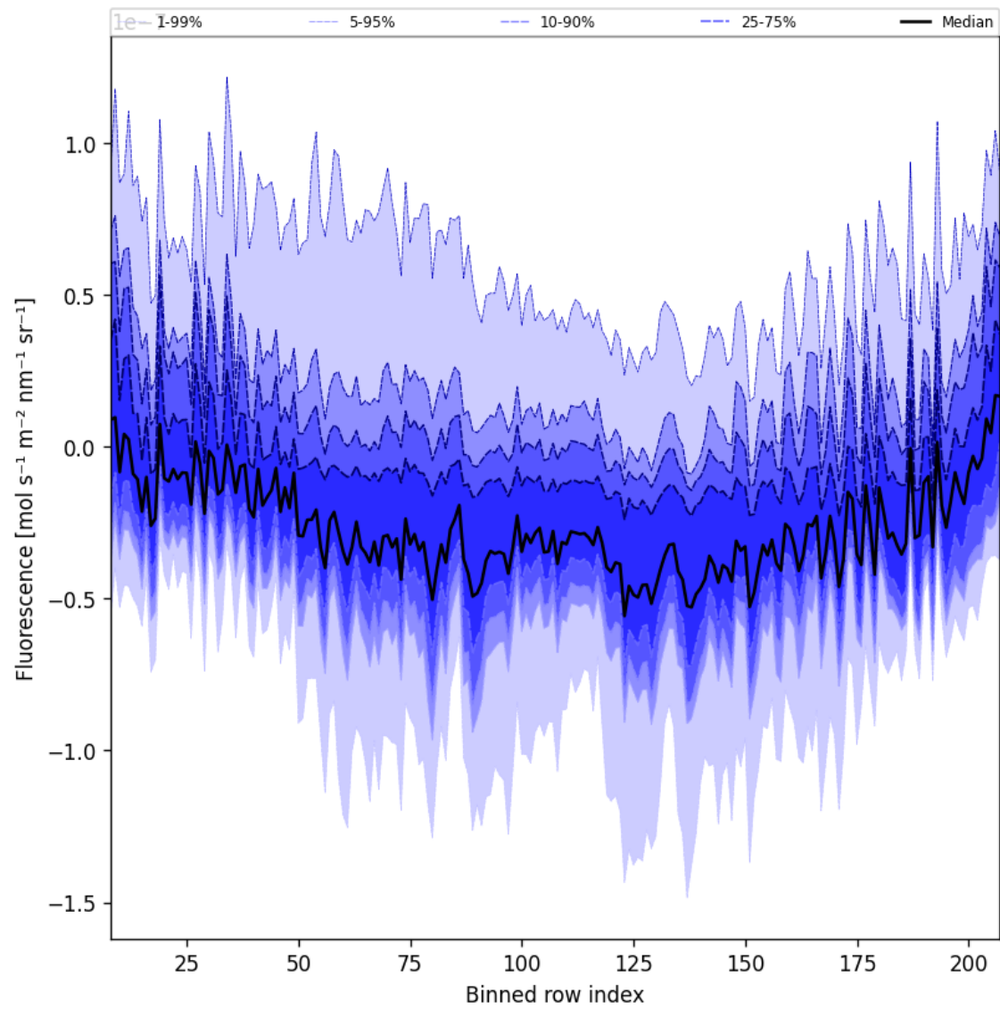
Figure 44: Along track statistics of “Fluorescence” for 2025-12-07 to 2025-12-07
