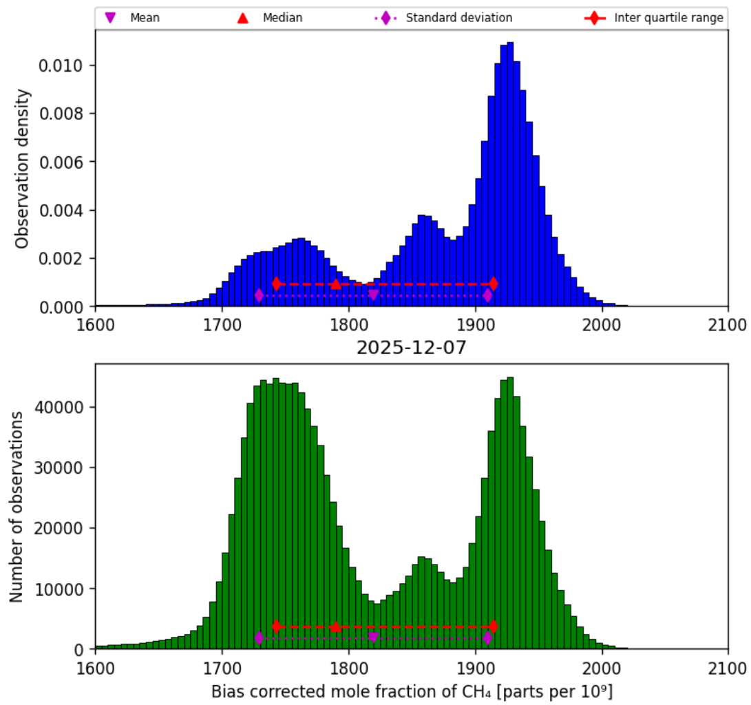
Figure 25: Histogram of “Bias corrected mole fraction of CH 4 ” for 2025-12-07 to 2025-12-07
