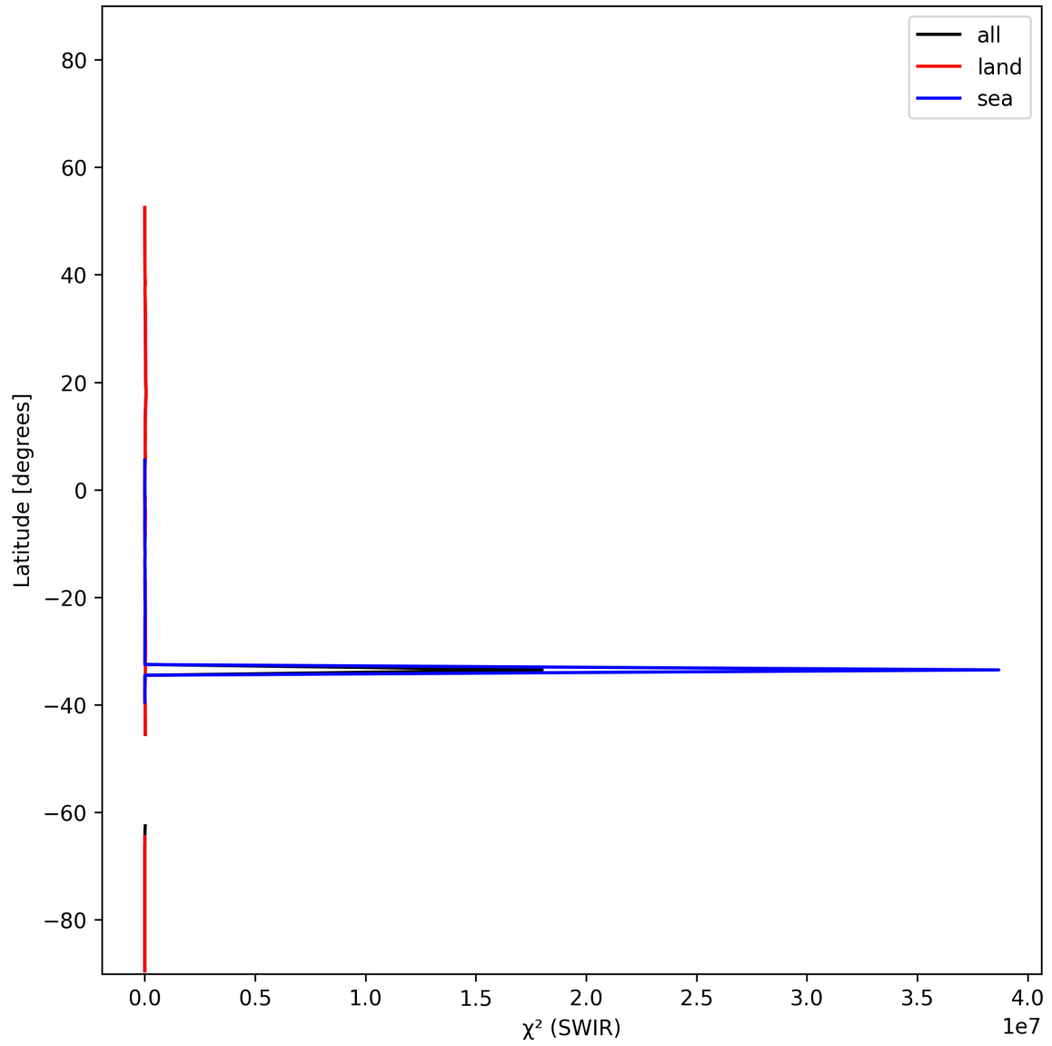
Figure 16: Zonal average of “ \chi^2 (SWIR)” for 2025-12-07 to 2025-12-07.
