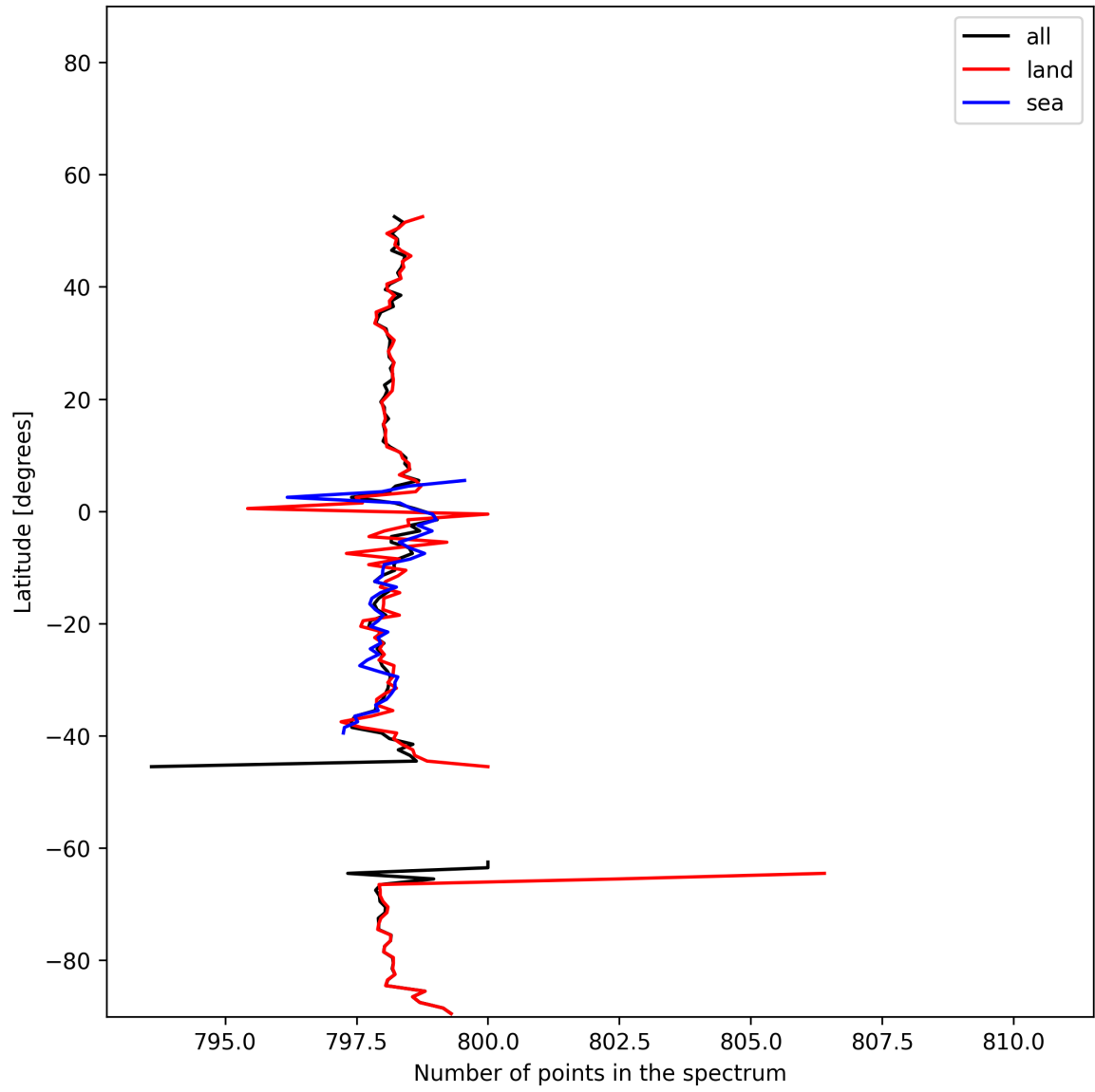
Figure 14: Zonal average of “Number of points in the spectrum” for 2025-12-07 to 2025-12-07.
