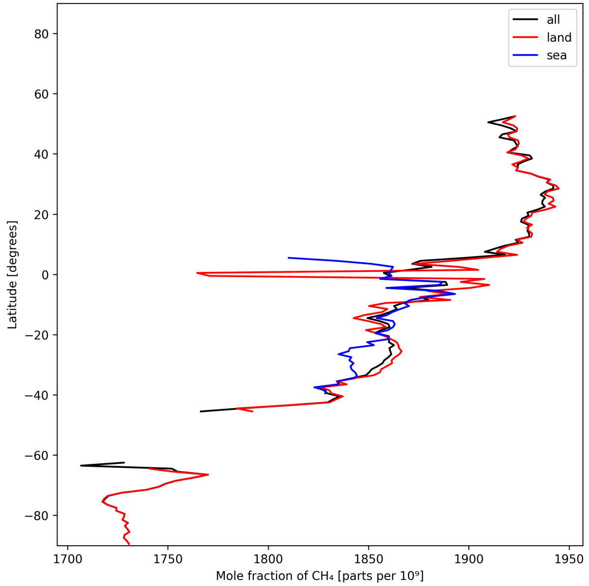
Figure 11: Zonal average of “Mole fraction of CH 4 ” for 2025-12-07 to 2025-12-07.
