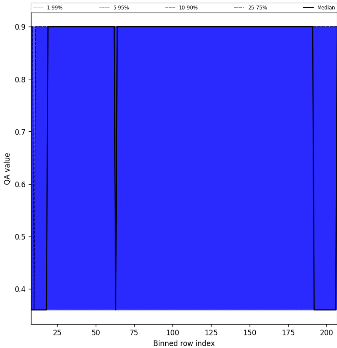
Figure 34: Along track statistics of “QA value” for 2025-12-07 to 2025-12-07
