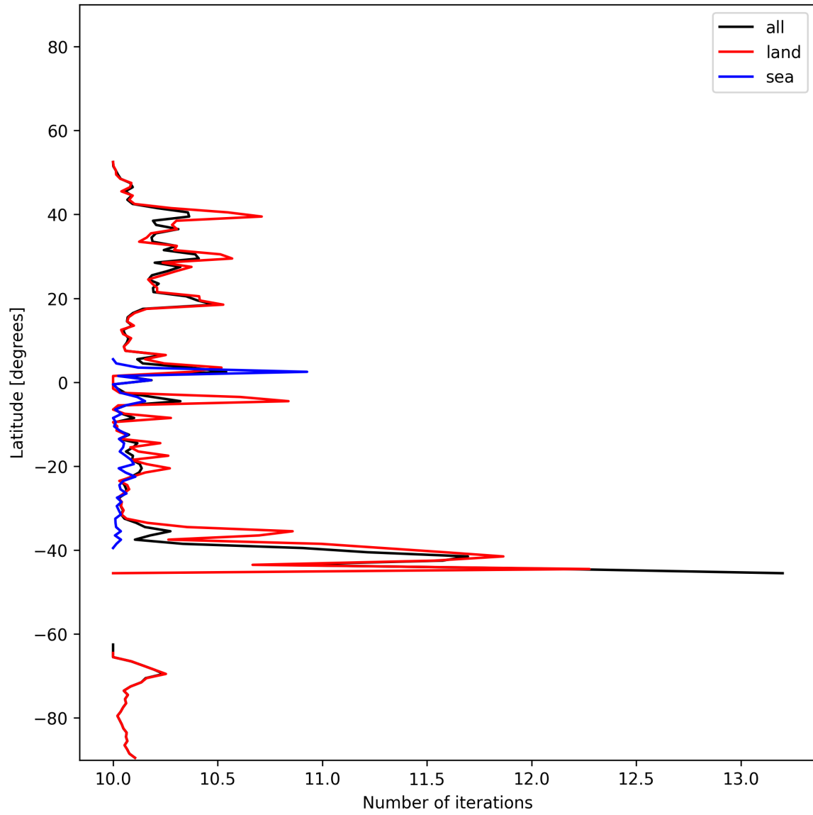
Figure 19: Zonal average of “Number of iterations” for 2025-12-07 to 2025-12-07.
