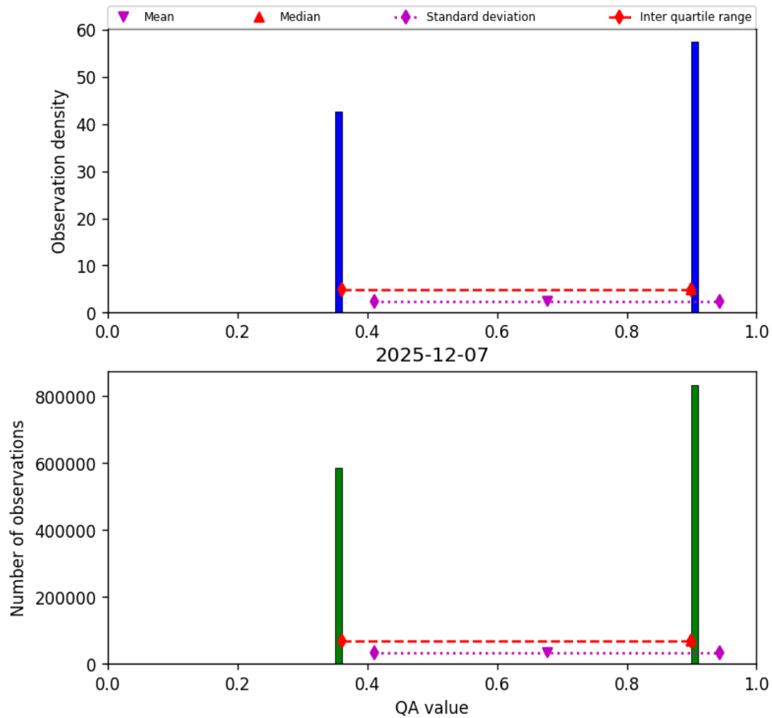
Figure 22: Histogram of “QA value” for 2025-12-07 to 2025-12-07
