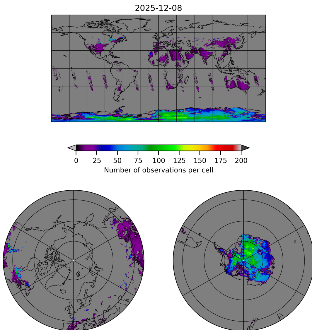
Figure 9: Map of the number of observations for 2025-12-08 to 2025-12-09
