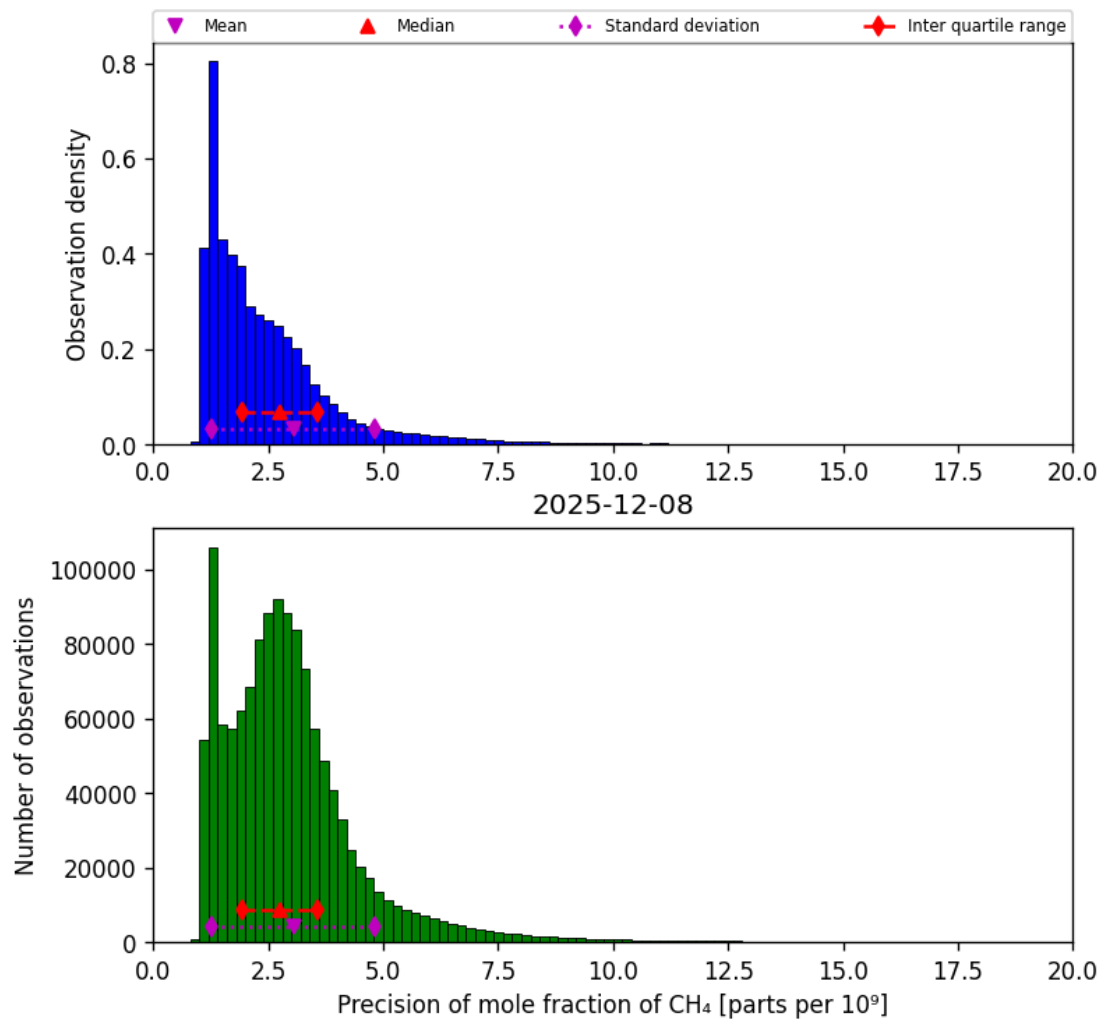
Figure 24: Histogram of “Precision of mole fraction of CH 4 ” for 2025-12-08 to 2025-12-09
