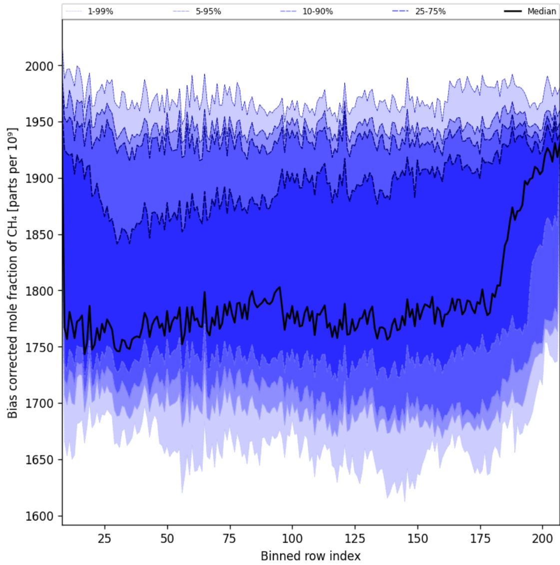
Figure 37: Along track statistics of “Bias corrected mole fraction of CH 4 ” for 2025-12-08 to 2025-12-09
