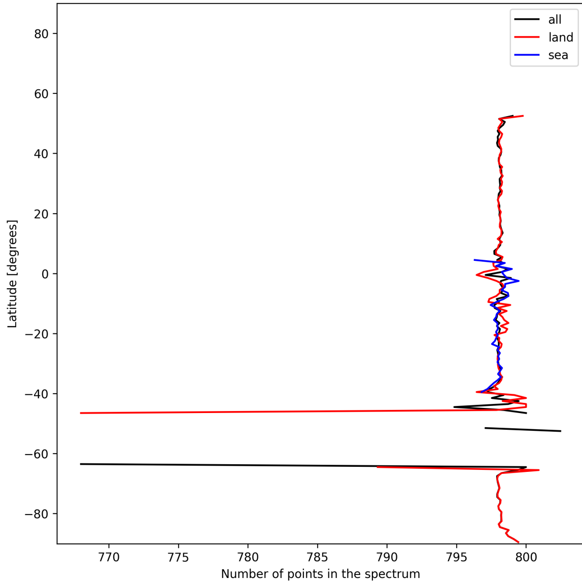
Figure 14: Zonal average of “Number of points in the spectrum” for 2025-12-08 to 2025-12-09.
