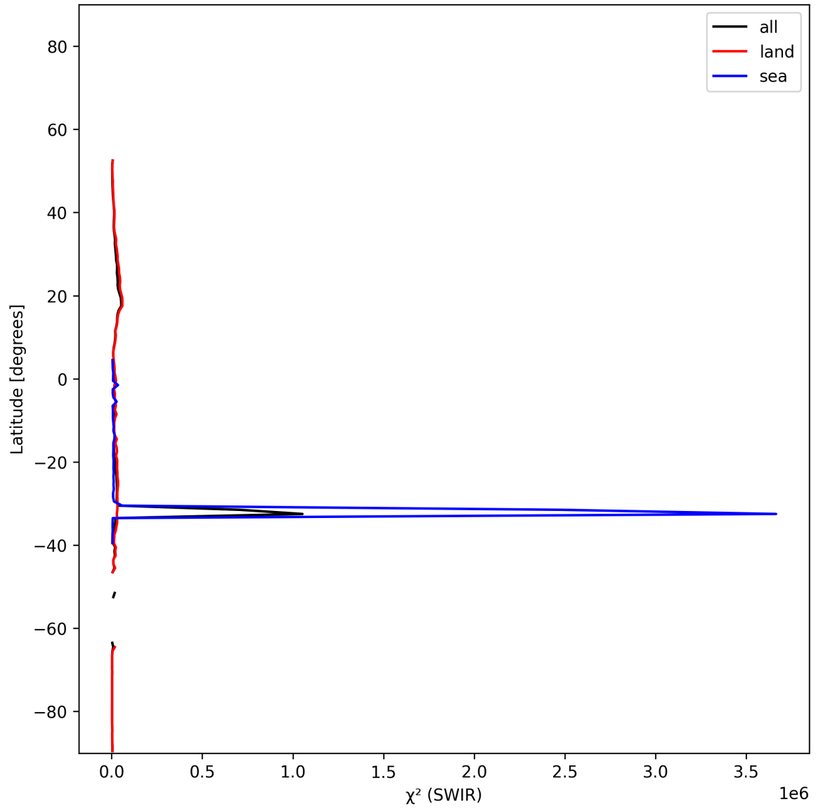
Figure 16: Zonal average of “ \chi^2 (SWIR)” for 2025-12-08 to 2025-12-09.
