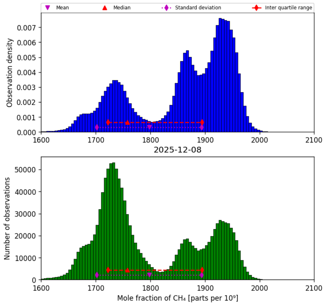
Figure 23: Histogram of “Mole fraction of CH 4 ” for 2025-12-08 to 2025-12-09
