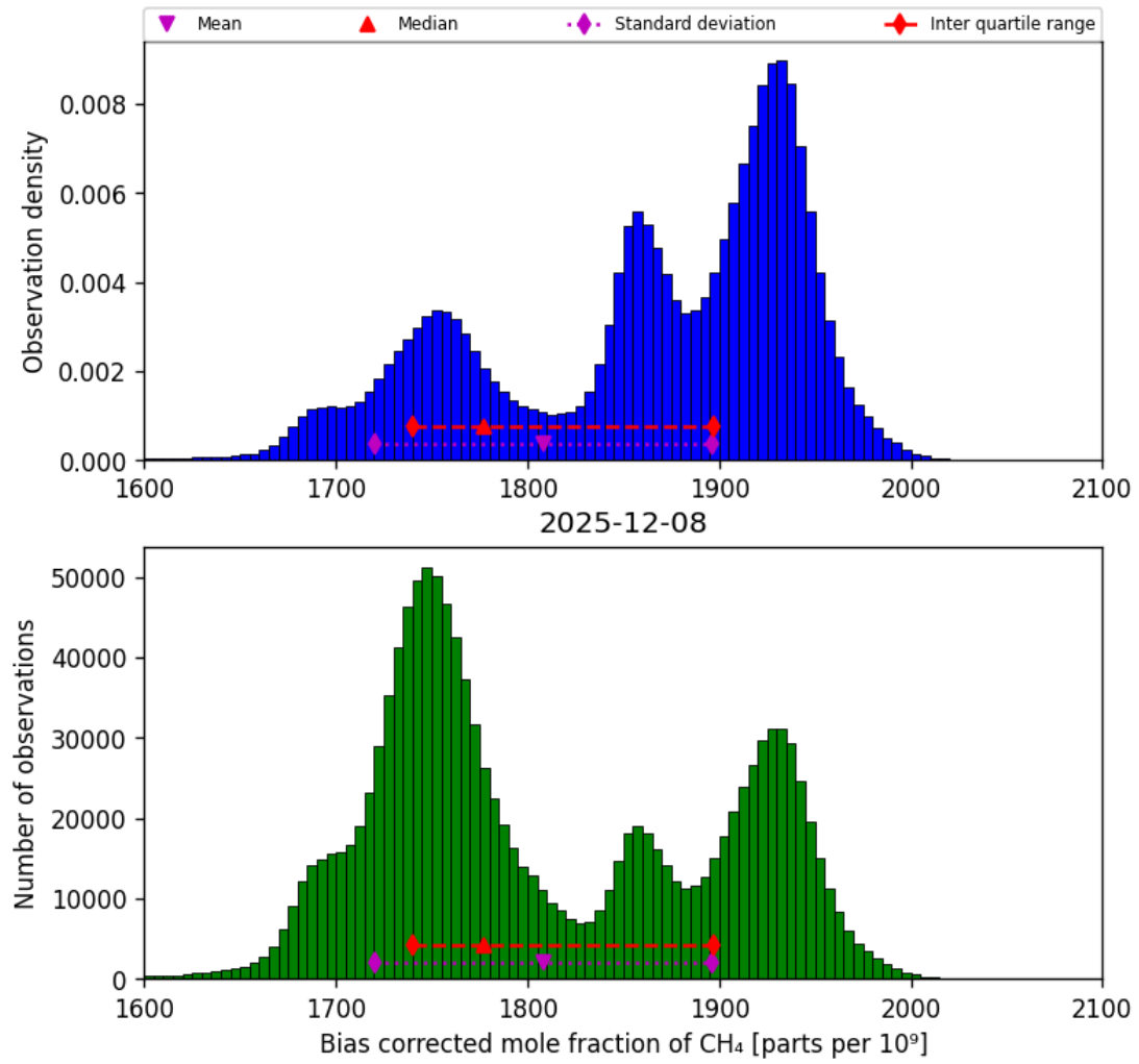
Figure 25: Histogram of “Bias corrected mole fraction of CH 4 ” for 2025-12-08 to 2025-12-09
