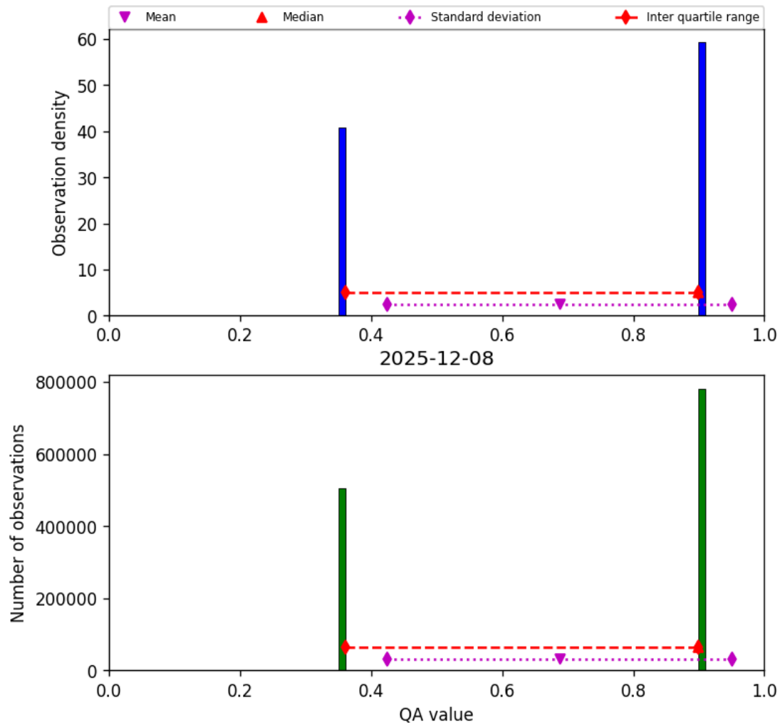
Figure 22: Histogram of “QA value” for 2025-12-08 to 2025-12-09
