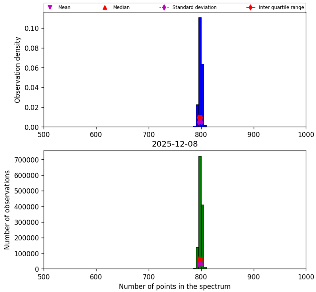
Figure 26: Histogram of “Number of points in the spectrum” for 2025-12-08 to 2025-12-09
