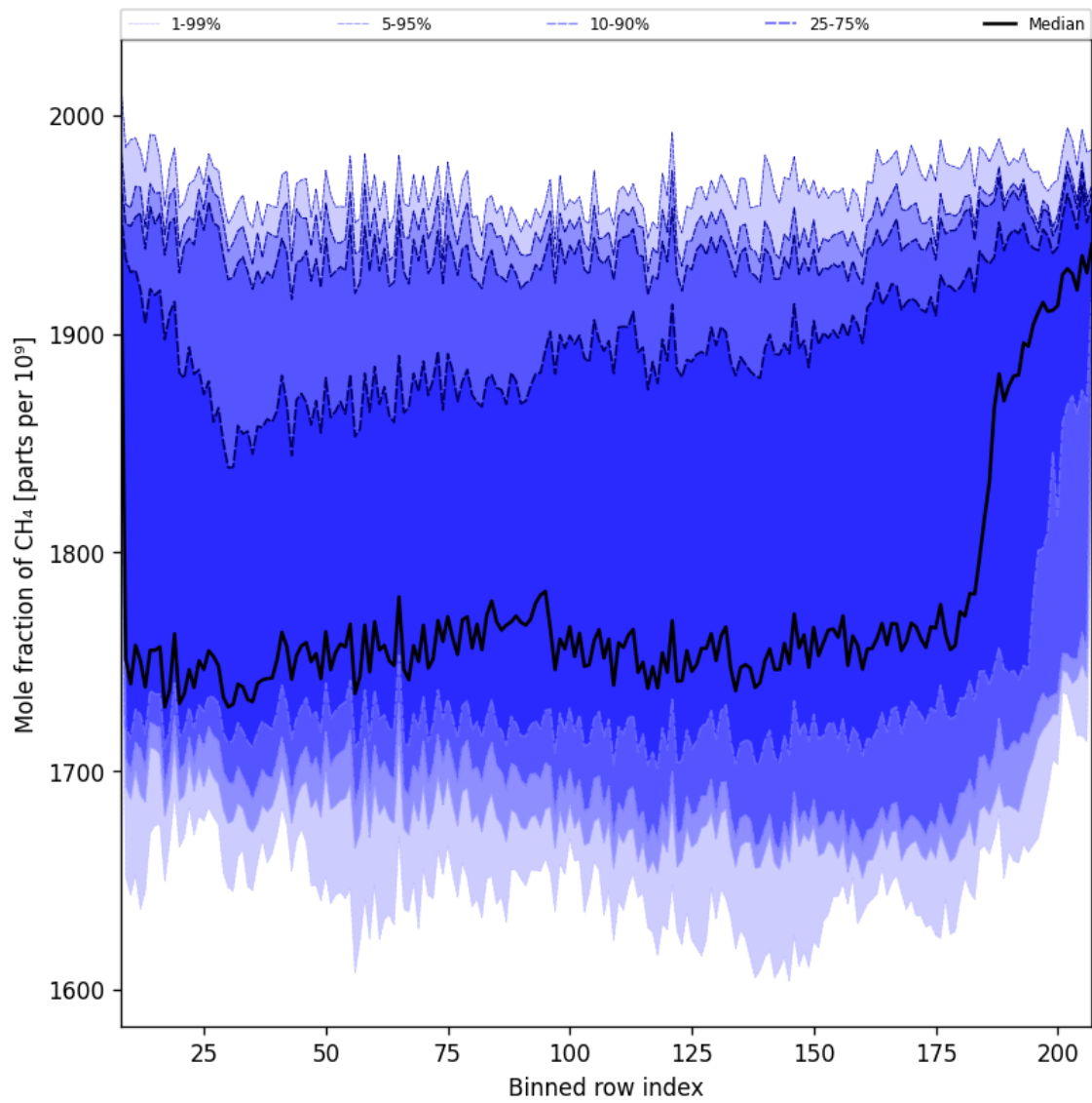
Figure 35: Along track statistics of “Mole fraction of CH 4 ” for 2025-12-08 to 2025-12-09
