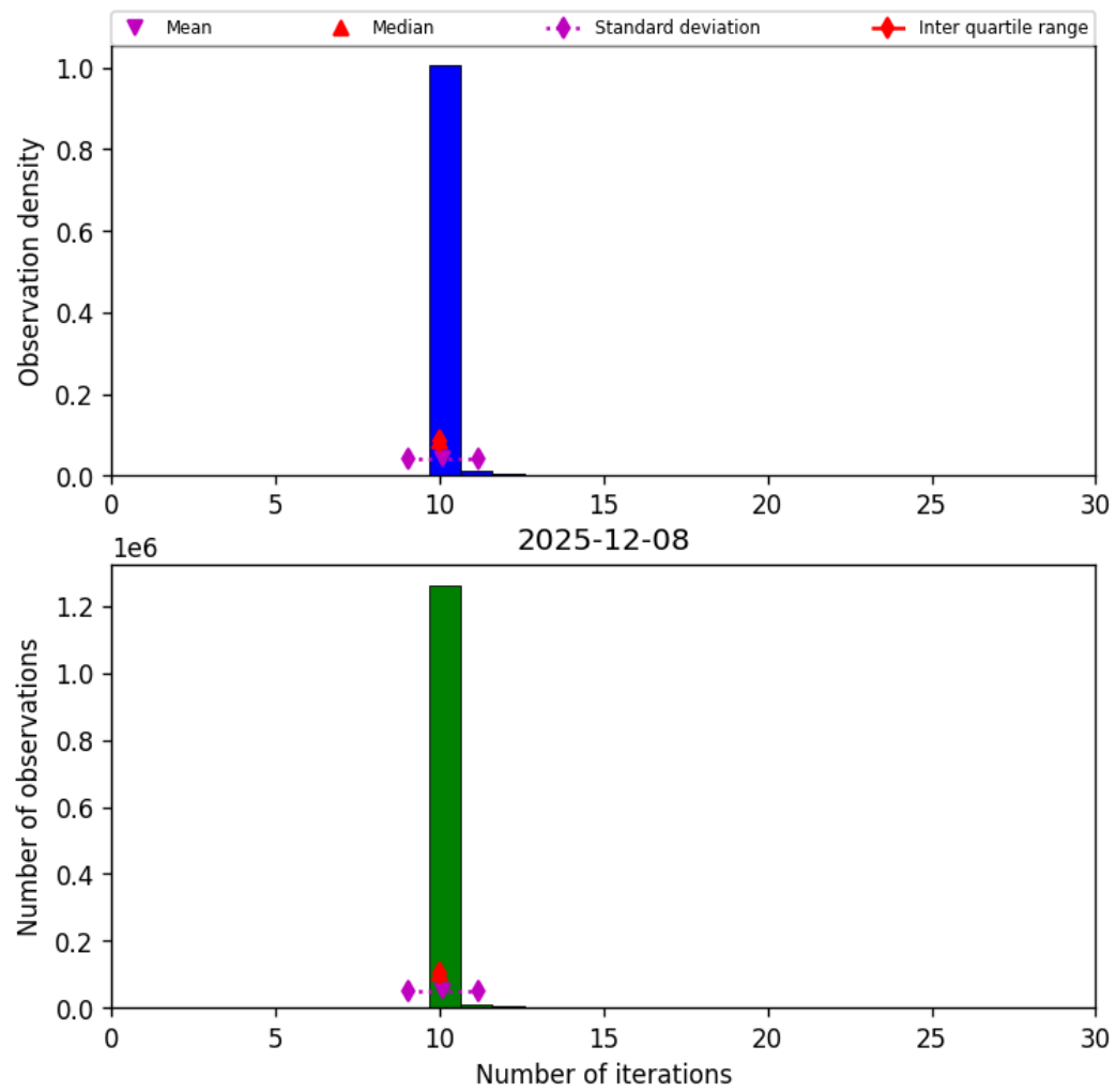
Figure 31: Histogram of “Number of iterations” for 2025-12-08 to 2025-12-09
