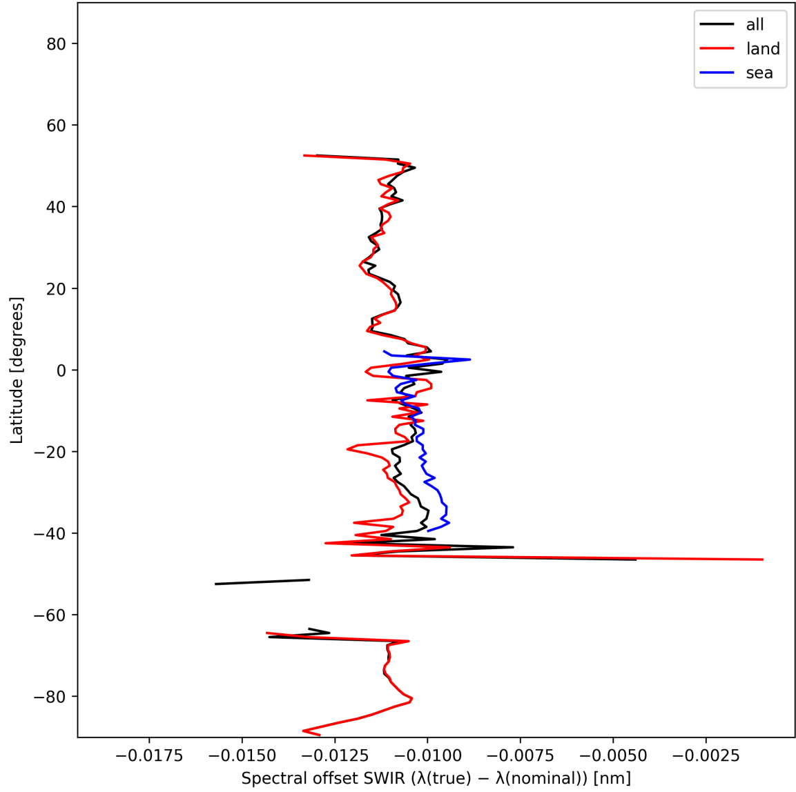
Figure 15: Zonal average of “Spectral offset SWIR ( \lambda_{\text{true}} - \lambda_{\text{nominal}} )” for 2025-12-08 to 2025-12-09.
