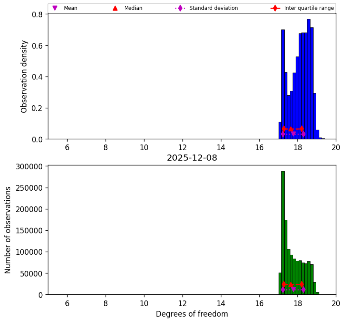
Figure 30: Histogram of “Degrees of freedom” for 2025-12-08 to 2025-12-09
