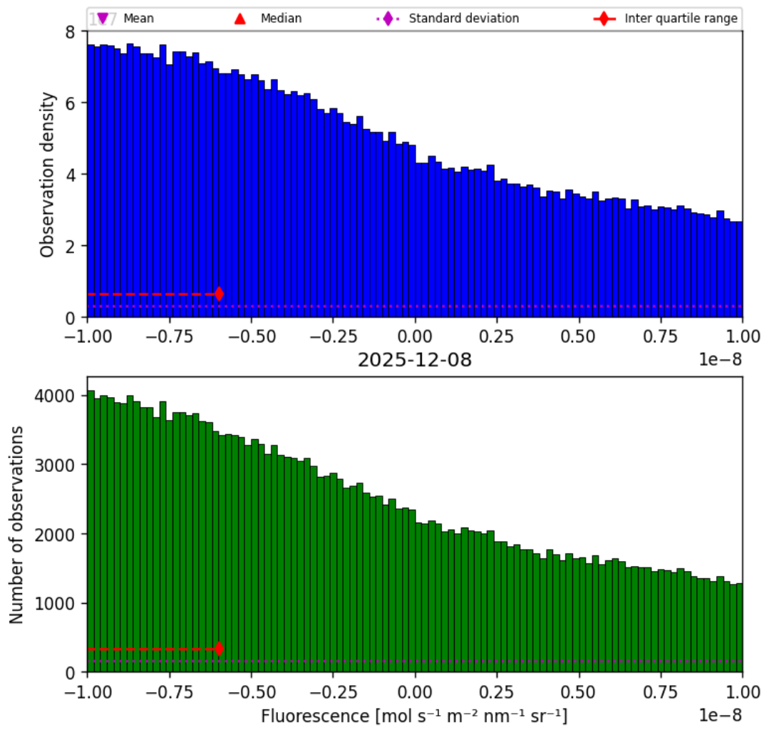
Figure 32: Histogram of “Fluorescence” for 2025-12-08 to 2025-12-09
