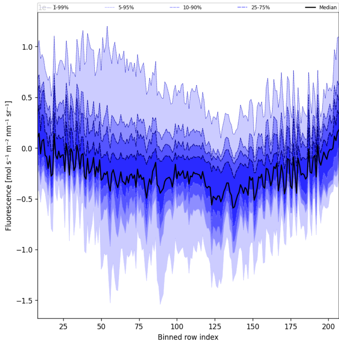
Figure 44: Along track statistics of “Fluorescence” for 2025-12-08 to 2025-12-09
