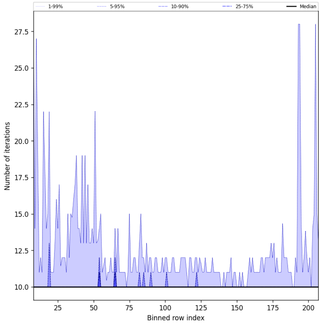
Figure 43: Along track statistics of “Number of iterations” for 2025-12-08 to 2025-12-09
