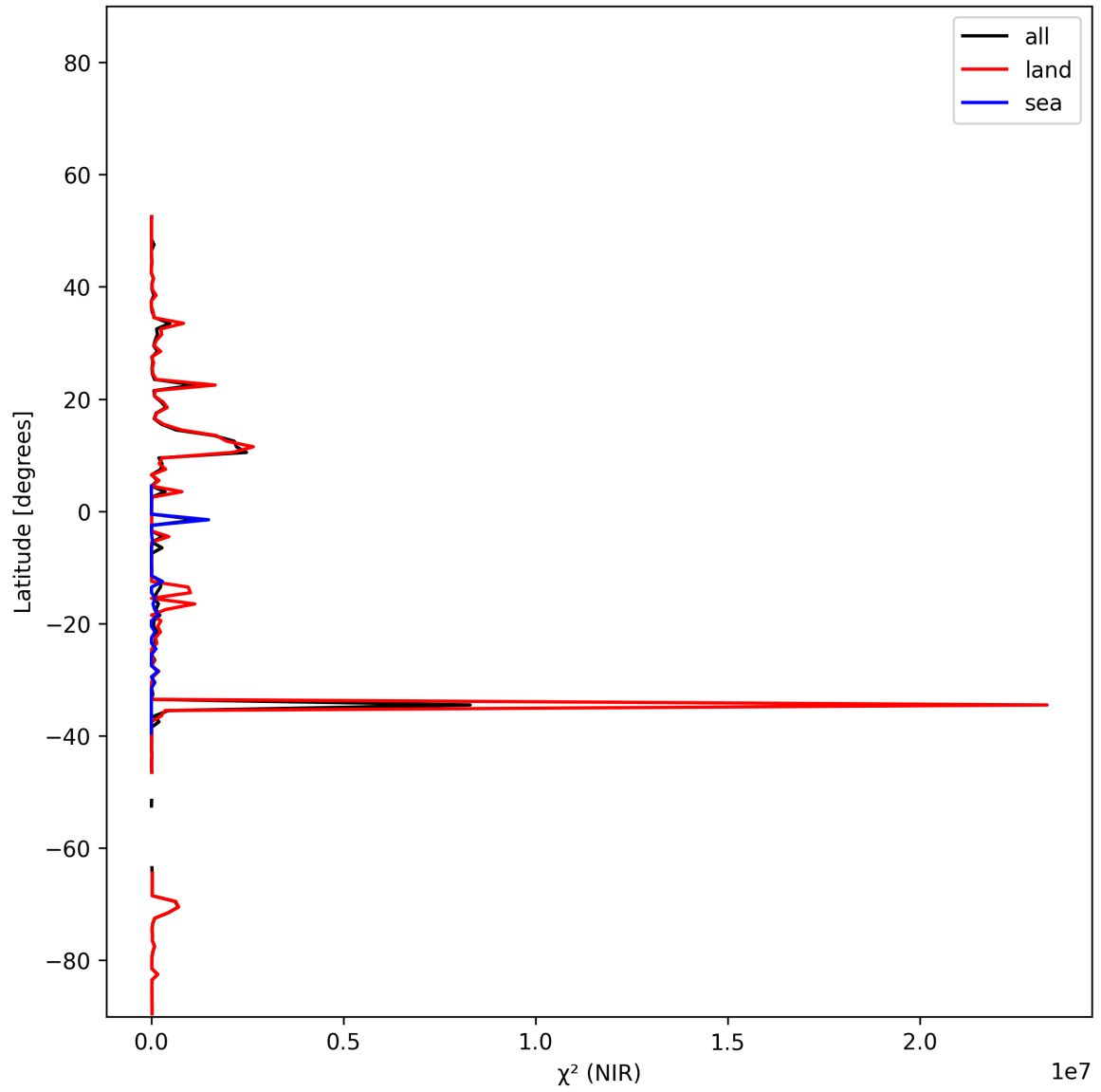
Figure 17: Zonal average of “ \chi^2 (NIR)” for 2025-12-08 to 2025-12-09.
