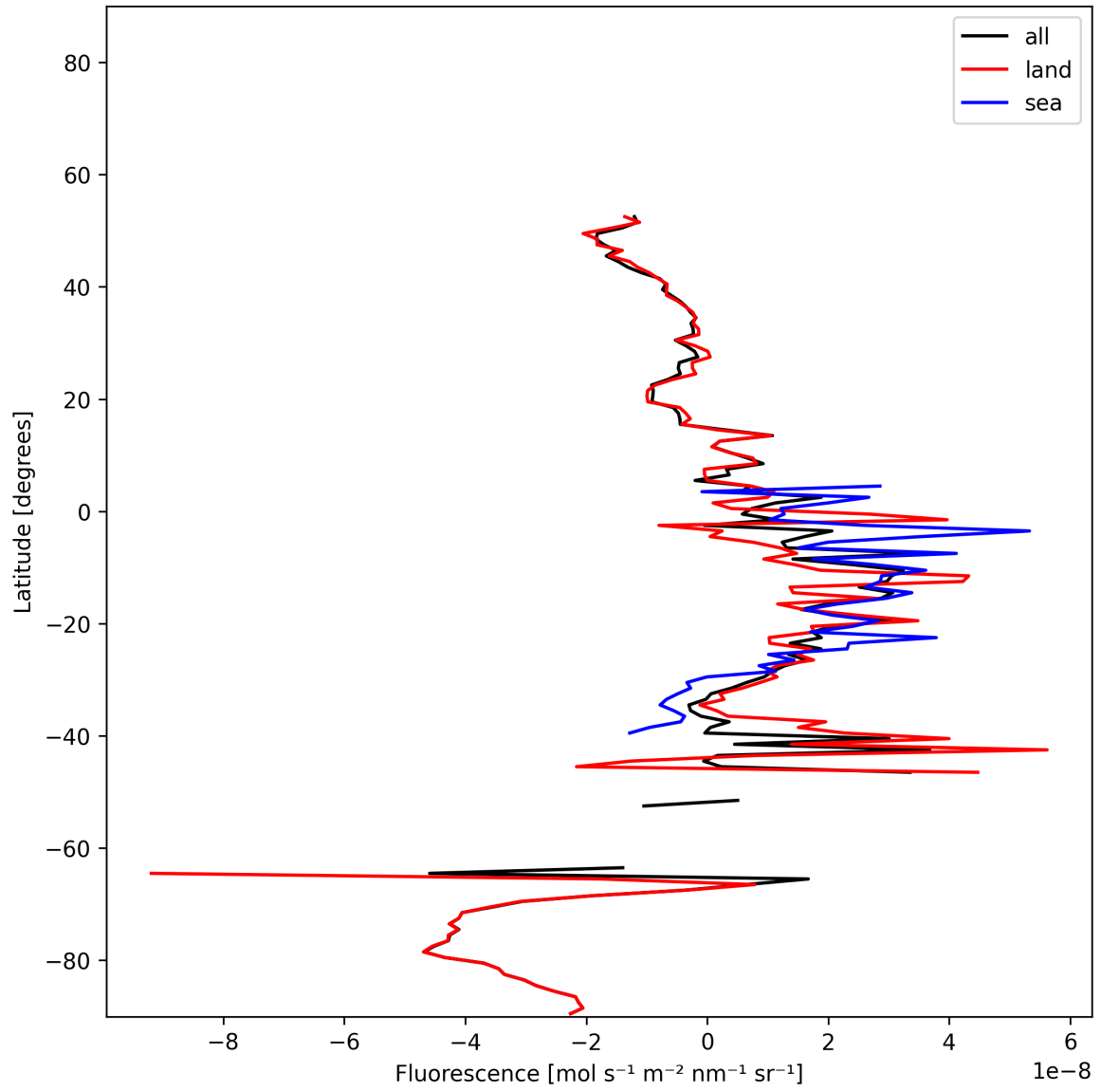
Figure 20: Zonal average of “Fluorescence” for 2025-12-08 to 2025-12-09.
