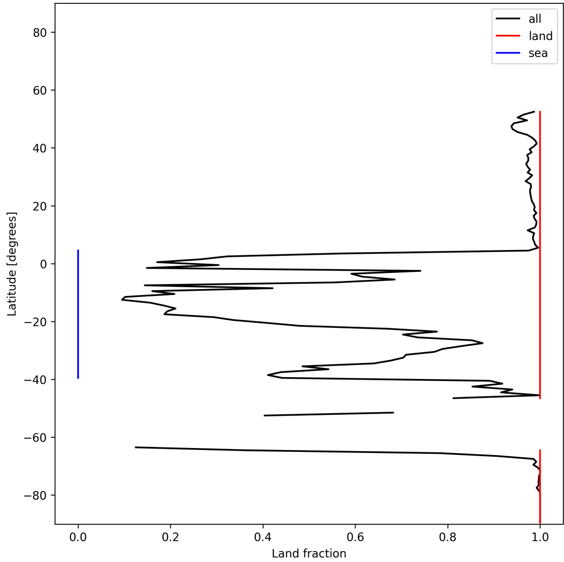
Figure 21: Zonal average of “Land fraction” for 2025-12-08 to 2025-12-09.
