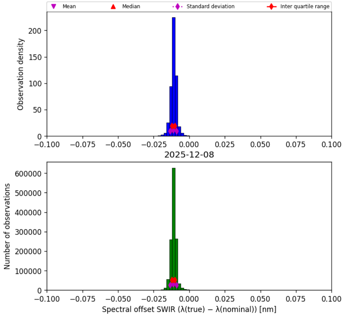
Figure 27: Histogram of “Spectral offset SWIR ( \lambda_{\text{true}} - \lambda_{\text{nominal}} )” for 2025-12-08 to 2025-12-09
