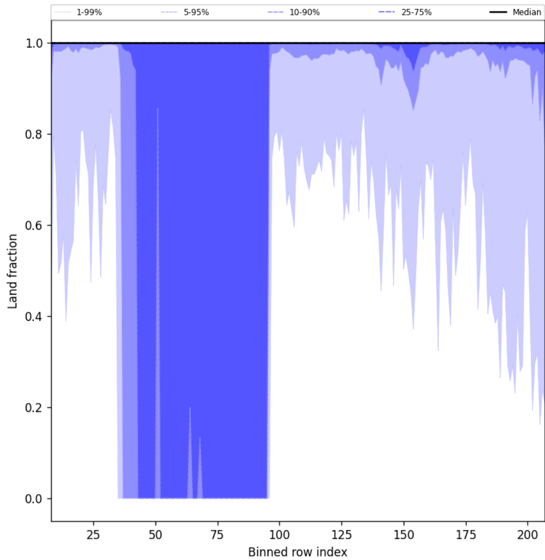
Figure 45: Along track statistics of “Land fraction” for 2025-12-08 to 2025-12-09
