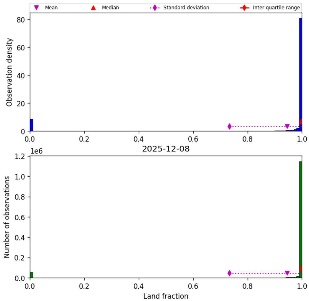
Figure 33: Histogram of “Land fraction” for 2025-12-08 to 2025-12-09
