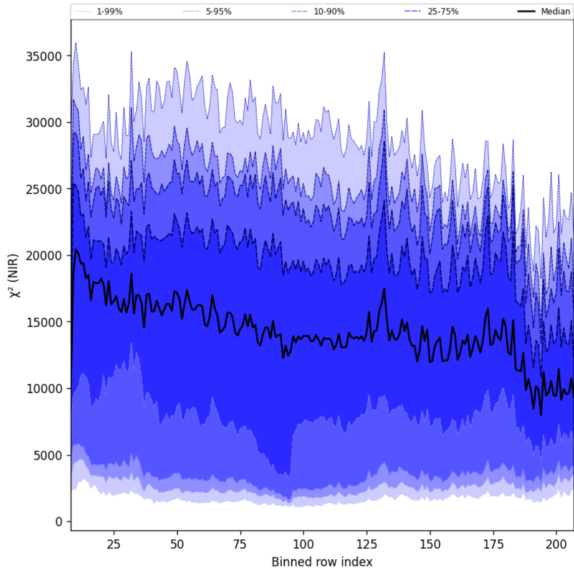
Figure 41: Along track statistics of “ \chi^2 (NIR)” for 2025-12-08 to 2025-12-09
