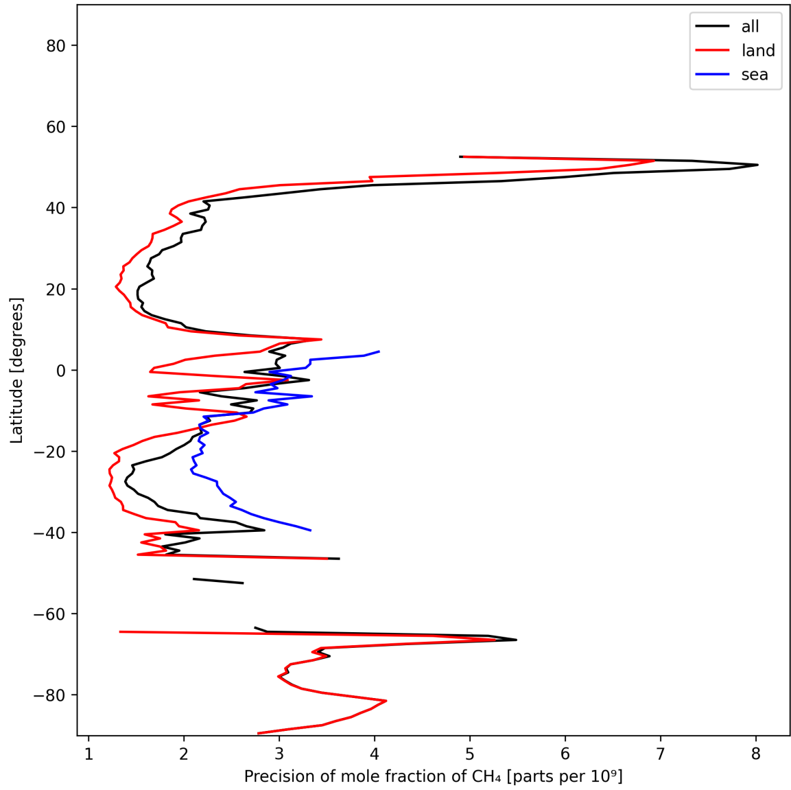
Figure 12: Zonal average of “Precision of mole fraction of CH 4 ” for 2025-12-08 to 2025-12-09.
