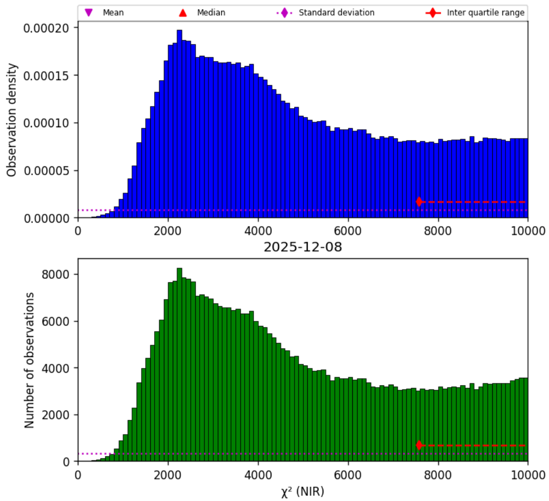
Figure 29: Histogram of " \chi^2 (NIR)" for 2025-12-08 to 2025-12-09
