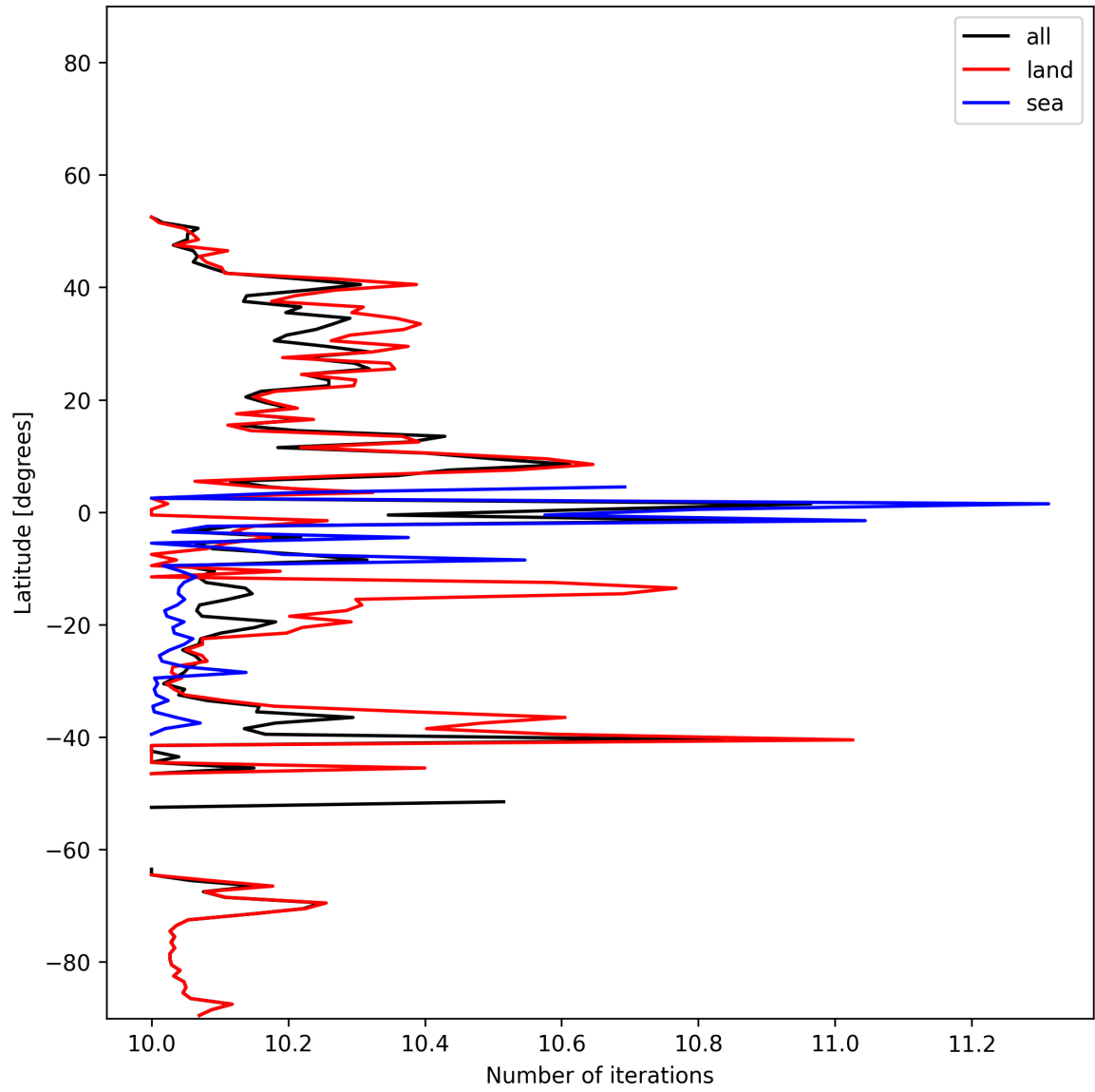
Figure 19: Zonal average of “Number of iterations” for 2025-12-08 to 2025-12-09.
