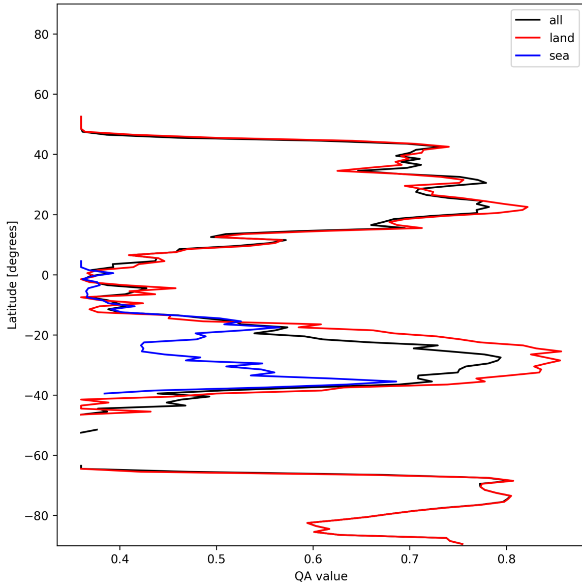
Figure 10: Zonal average of “QA value” for 2025-12-08 to 2025-12-09.
