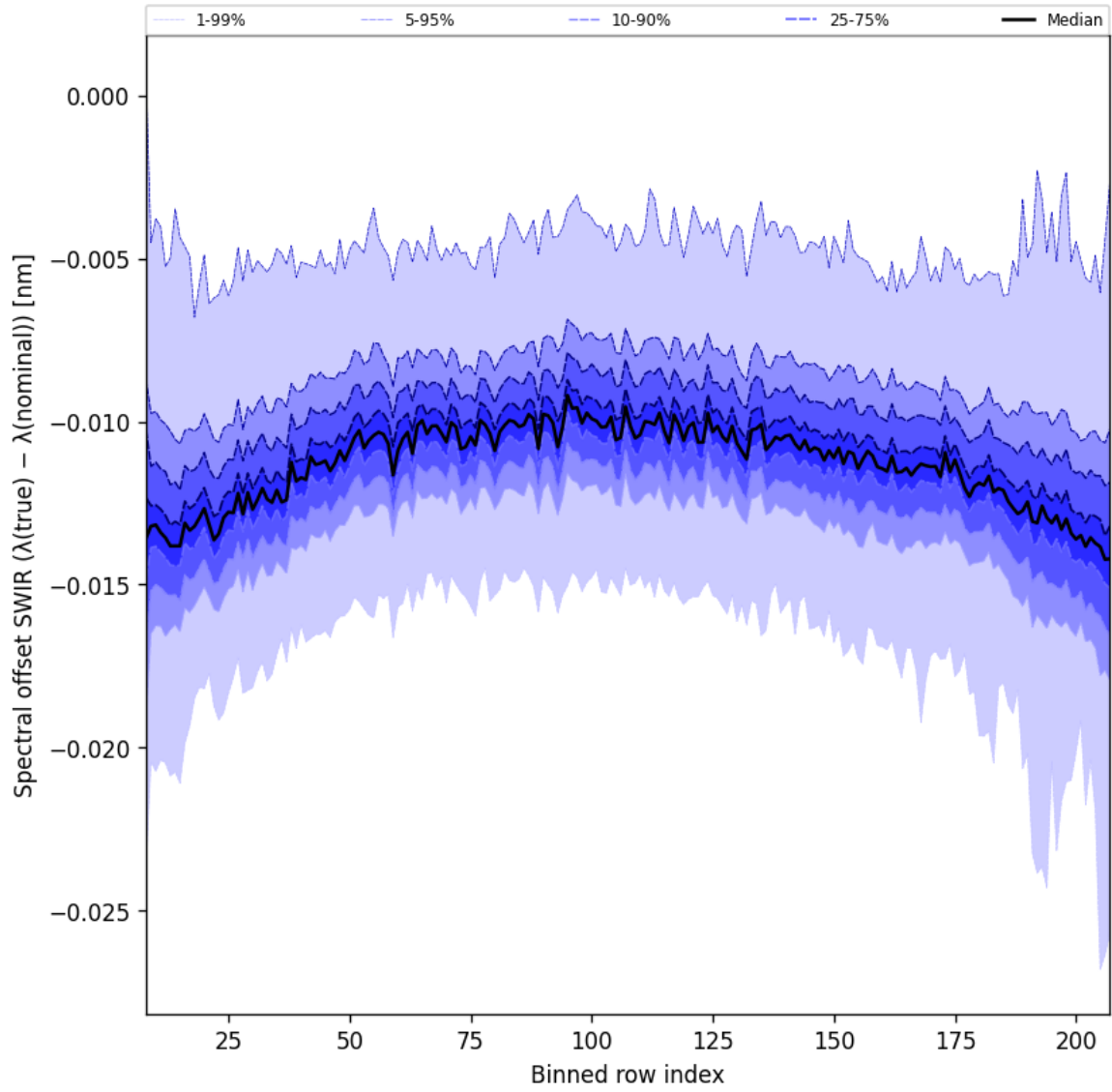
Figure 39: Along track statistics of “Spectral offset SWIR ( \lambda_{\text{true}} - \lambda_{\text{nominal}} )” for 2025-12-08 to 2025-12-09
