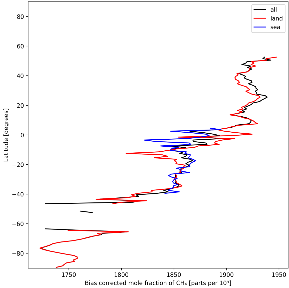
Figure 13: Zonal average of “Bias corrected mole fraction of CH 4 ” for 2025-12-08 to 2025-12-09.
