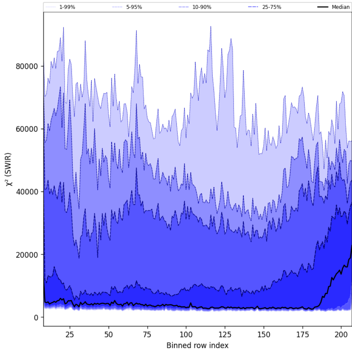
Figure 40: Along track statistics of “ \chi^2 (SWIR)” for 2025-12-08 to 2025-12-09
