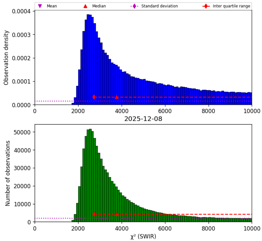
Figure 28: Histogram of “ \chi^2 (SWIR)” for 2025-12-08 to 2025-12-09
