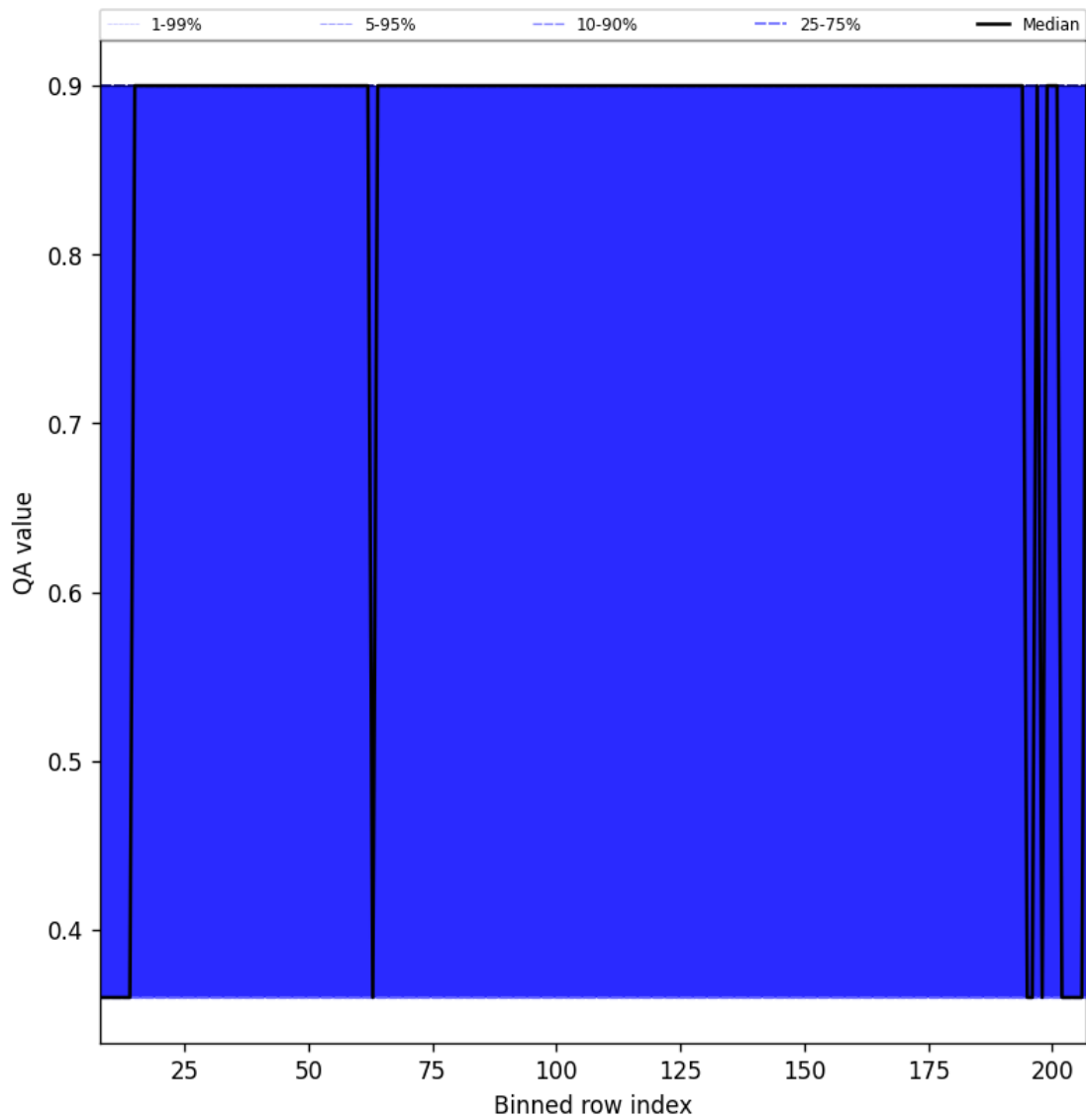
Figure 34: Along track statistics of “QA value” for 2025-12-08 to 2025-12-09
