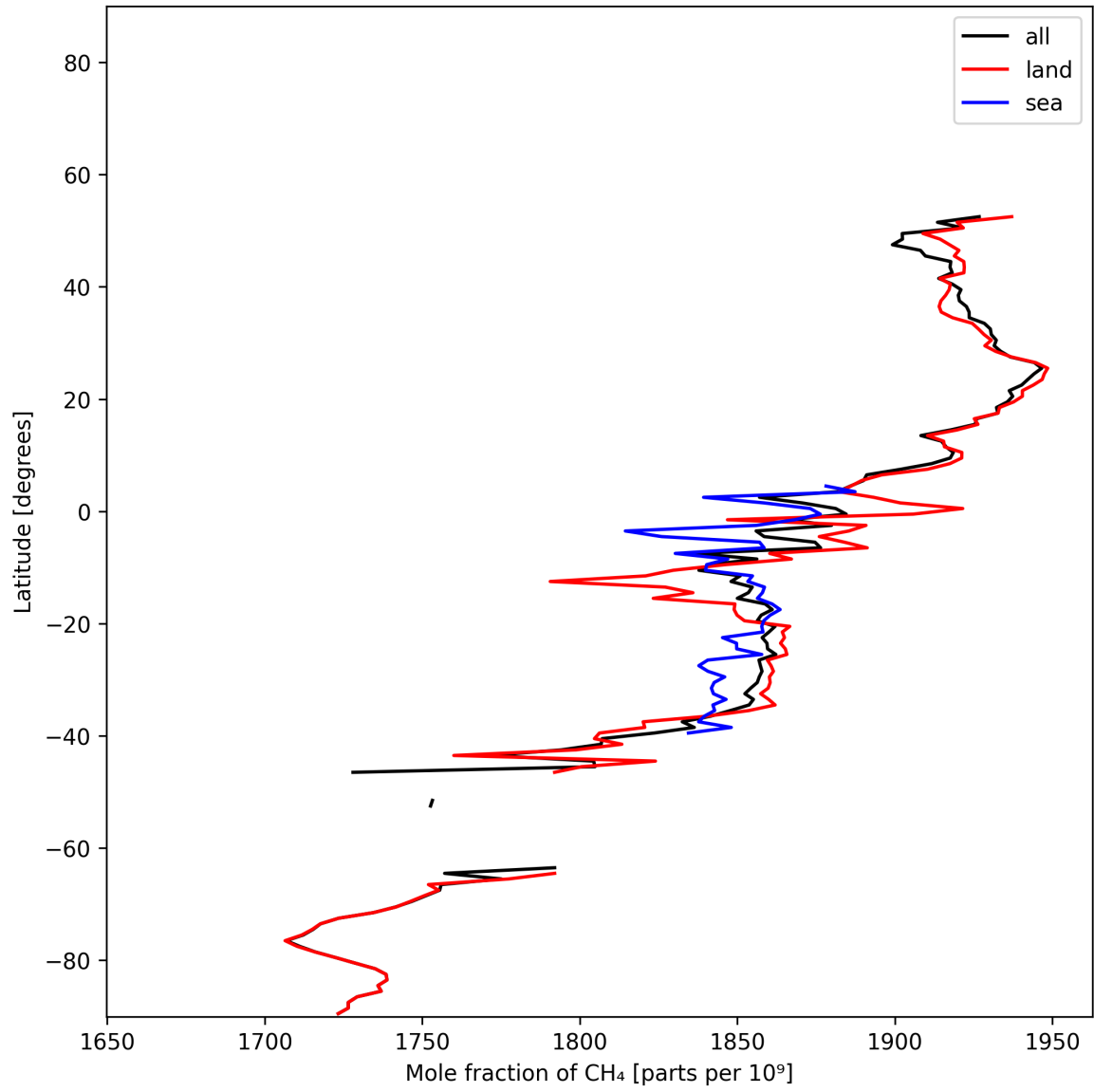
Figure 11: Zonal average of “Mole fraction of \text{CH}_4 ” for 2025-12-08 to 2025-12-09.
