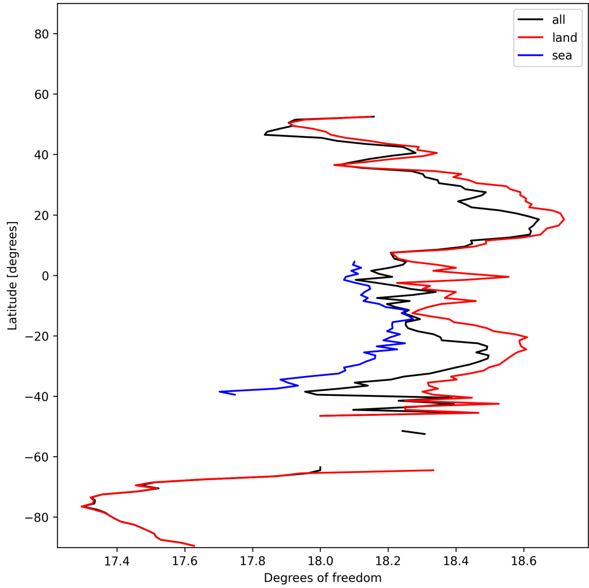
Figure 18: Zonal average of “Degrees of freedom” for 2025-12-08 to 2025-12-09.
