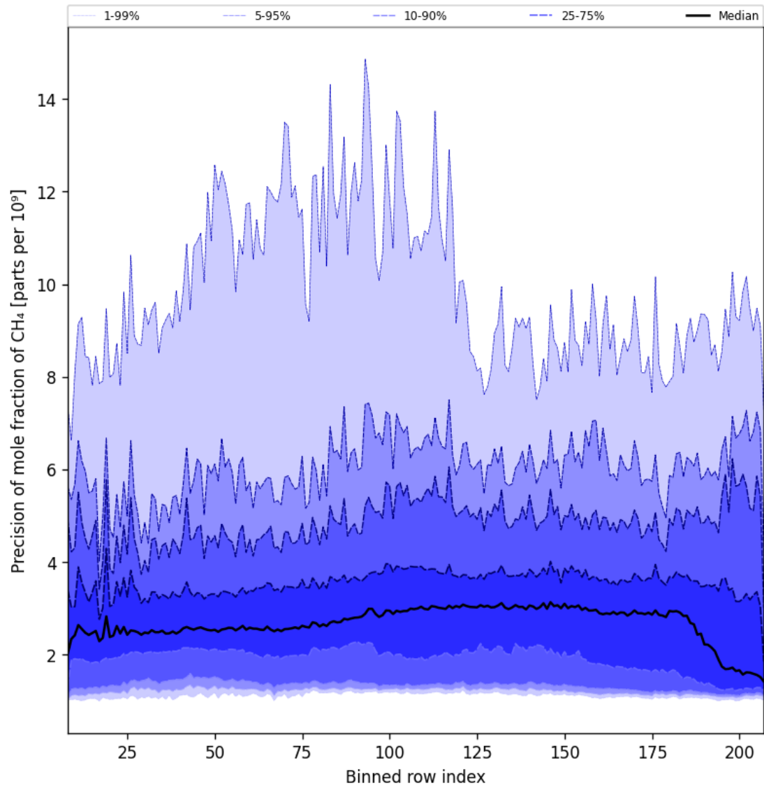
Figure 36: Along track statistics of “Precision of mole fraction of CH 4 ” for 2025-12-08 to 2025-12-09
