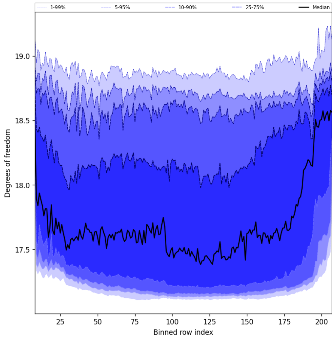
Figure 42: Along track statistics of “Degrees of freedom” for 2025-12-08 to 2025-12-09
