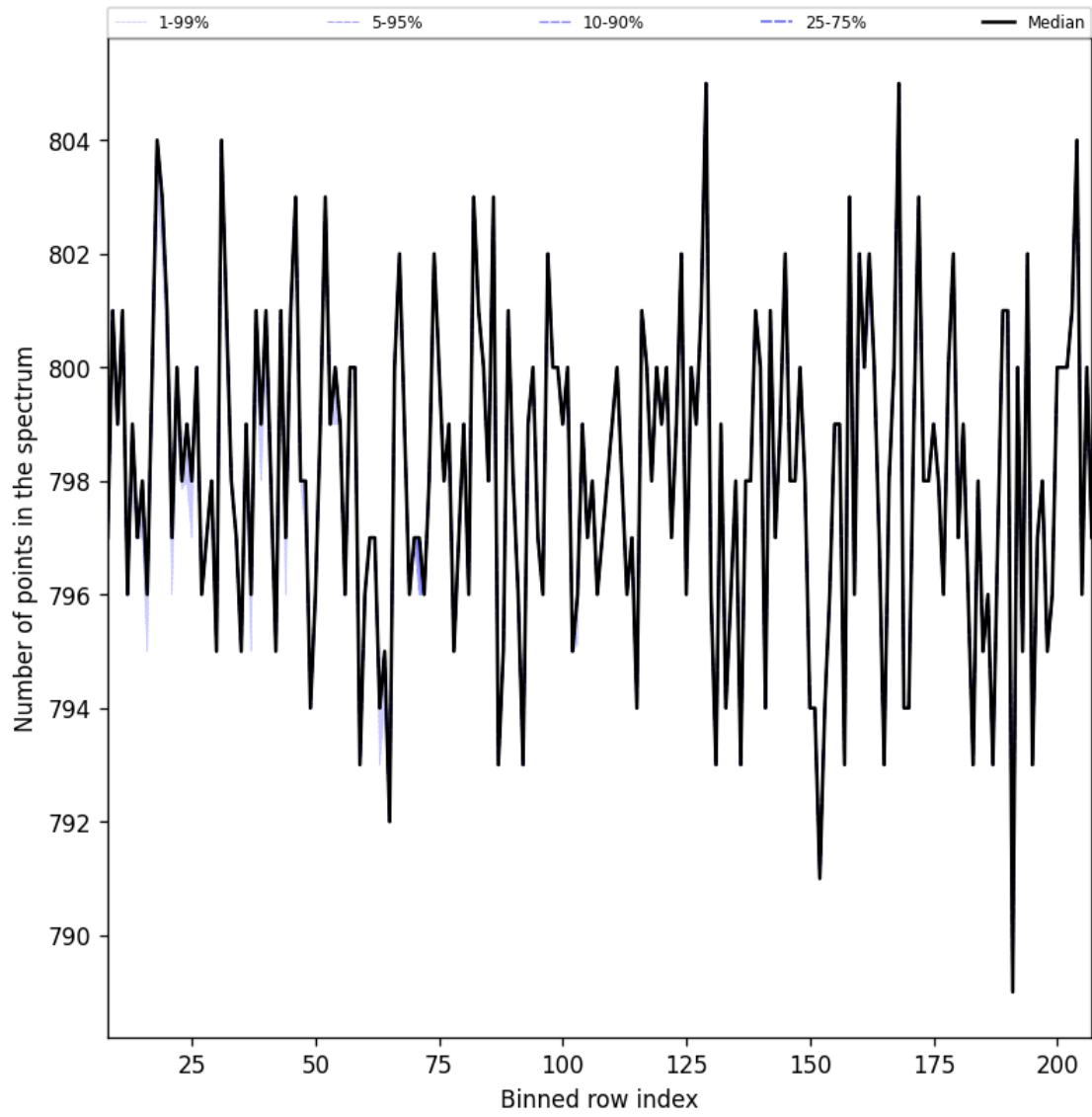
Figure 38: Along track statistics of “Number of points in the spectrum” for 2025-12-08 to 2025-12-09
