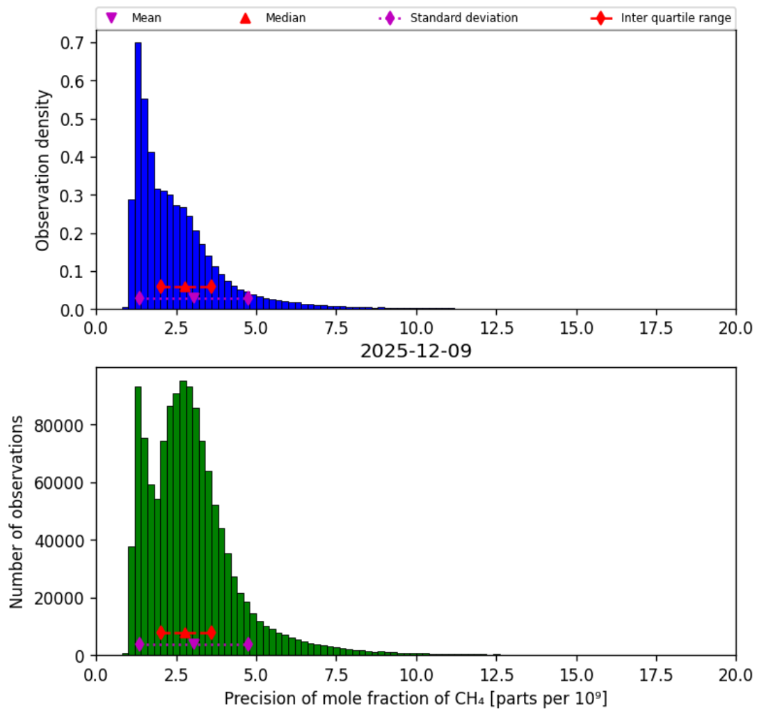
Figure 24: Histogram of “Precision of mole fraction of CH 4 ” for 2025-12-09 to 2025-12-10
