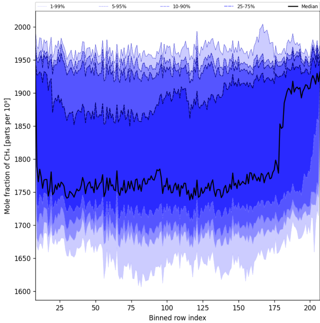
Figure 35: Along track statistics of “Mole fraction of CH 4 ” for 2025-12-09 to 2025-12-10
