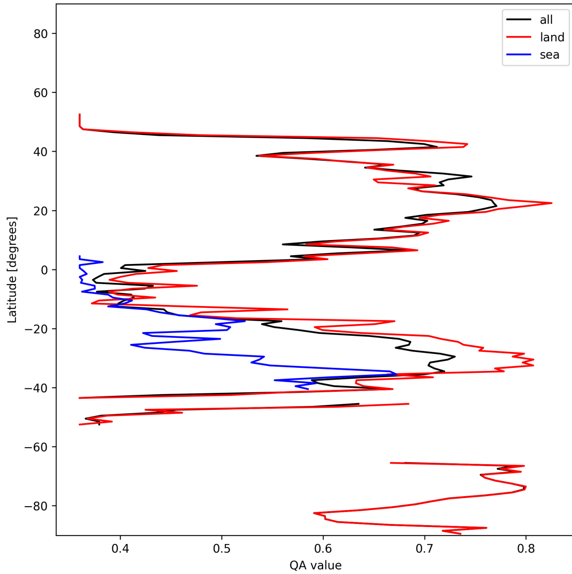
Figure 10: Zonal average of “QA value” for 2025-12-09 to 2025-12-10.
