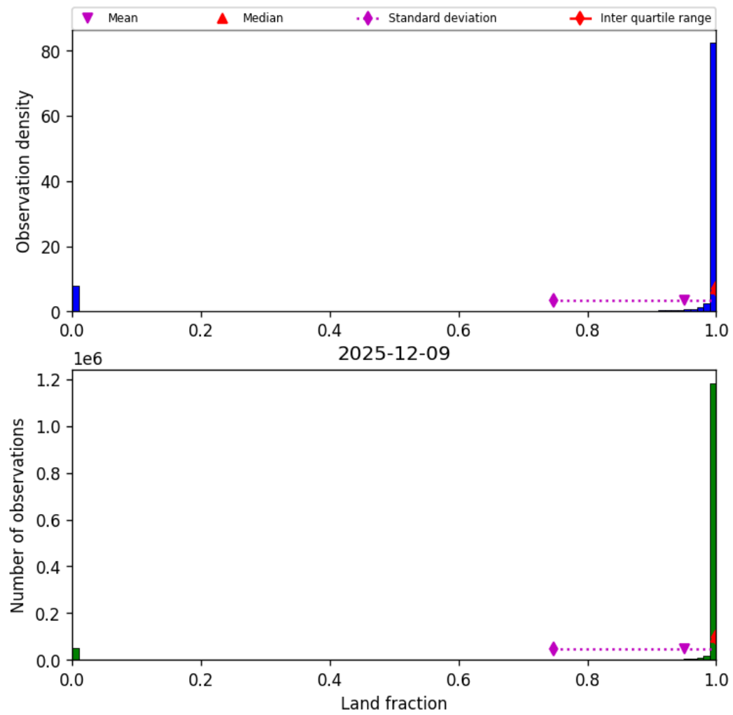
Figure 33: Histogram of “Land fraction” for 2025-12-09 to 2025-12-10
