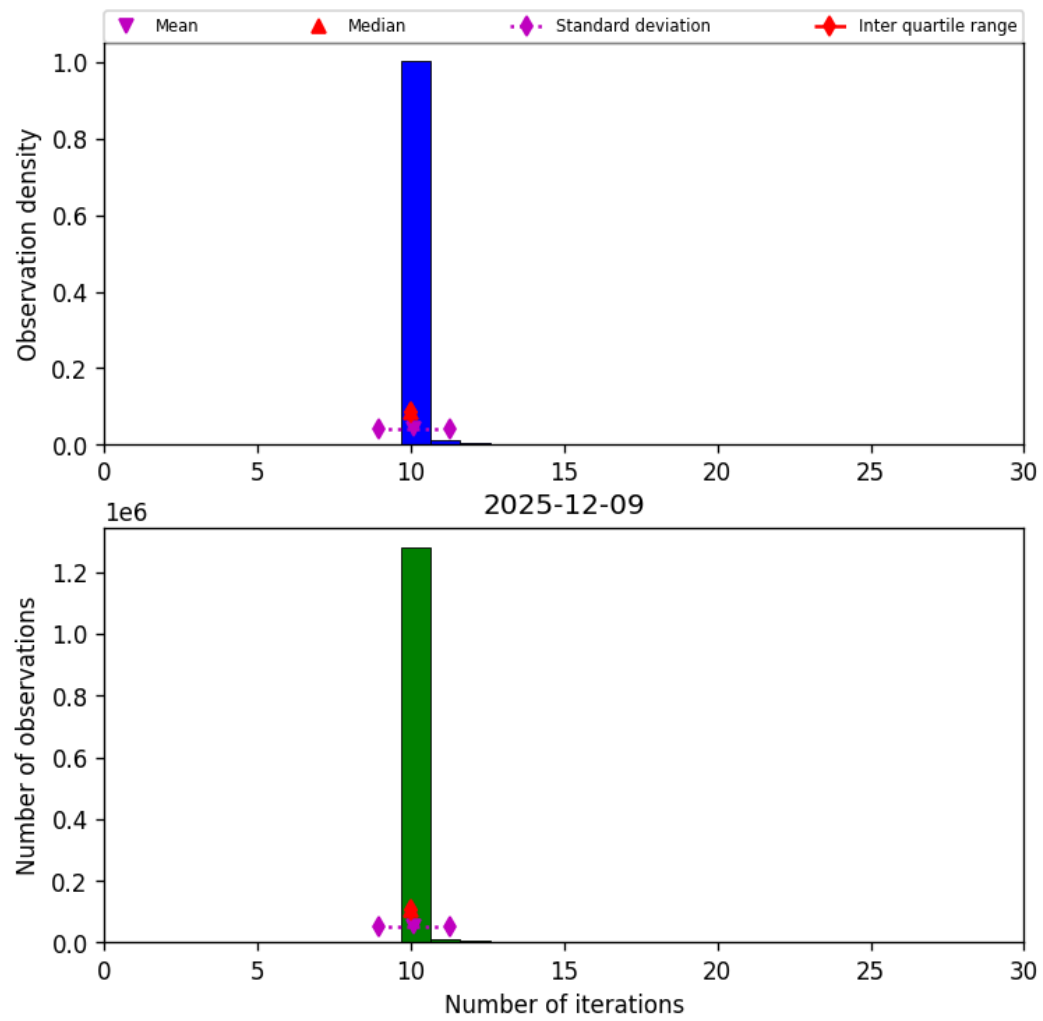
Figure 31: Histogram of “Number of iterations” for 2025-12-09 to 2025-12-10
