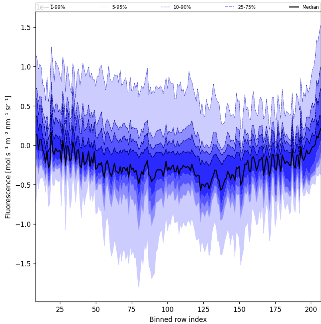
Figure 44: Along track statistics of “Fluorescence” for 2025-12-09 to 2025-12-10
