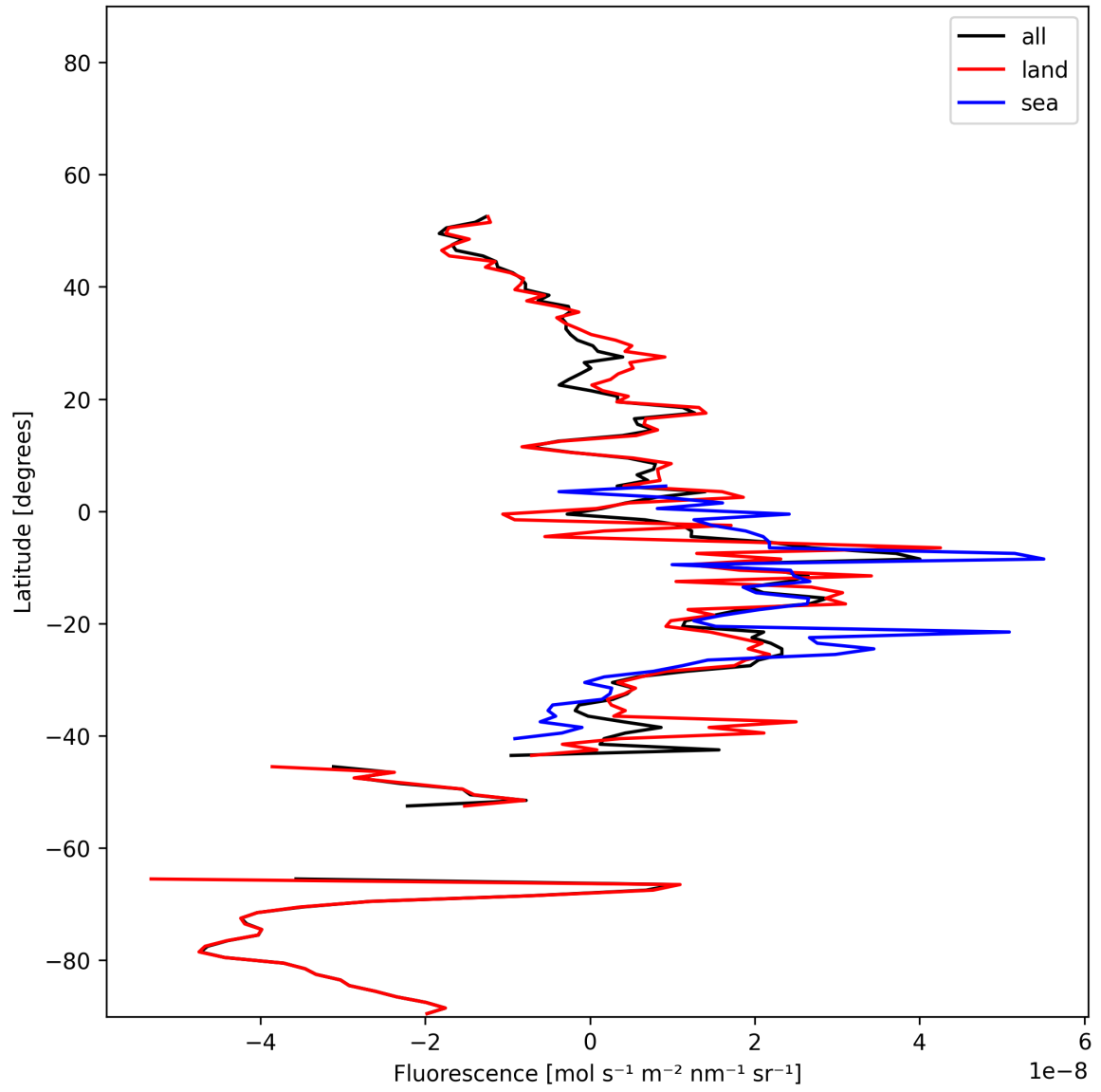
Figure 20: Zonal average of “Fluorescence” for 2025-12-09 to 2025-12-10.
