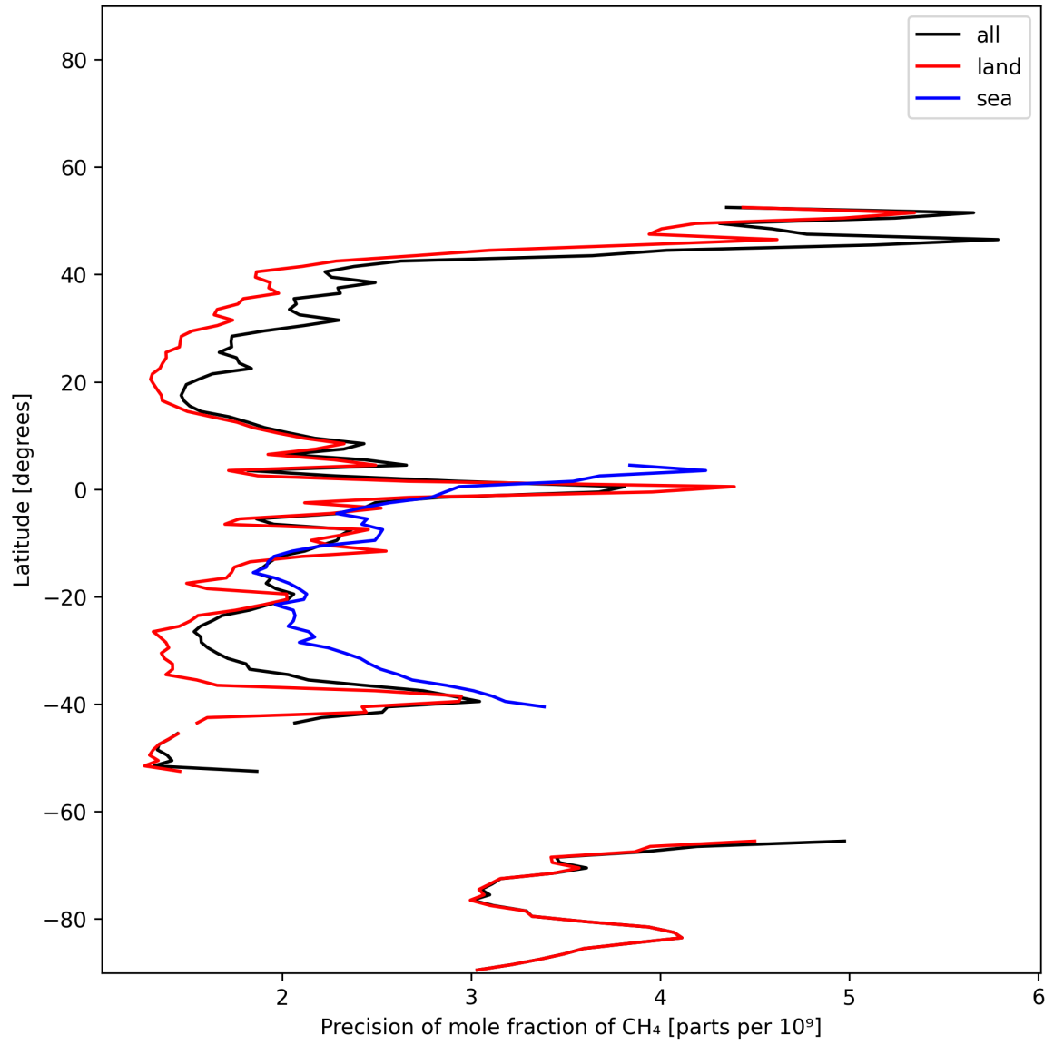
Figure 12: Zonal average of “Precision of mole fraction of CH 4 ” for 2025-12-09 to 2025-12-10.
