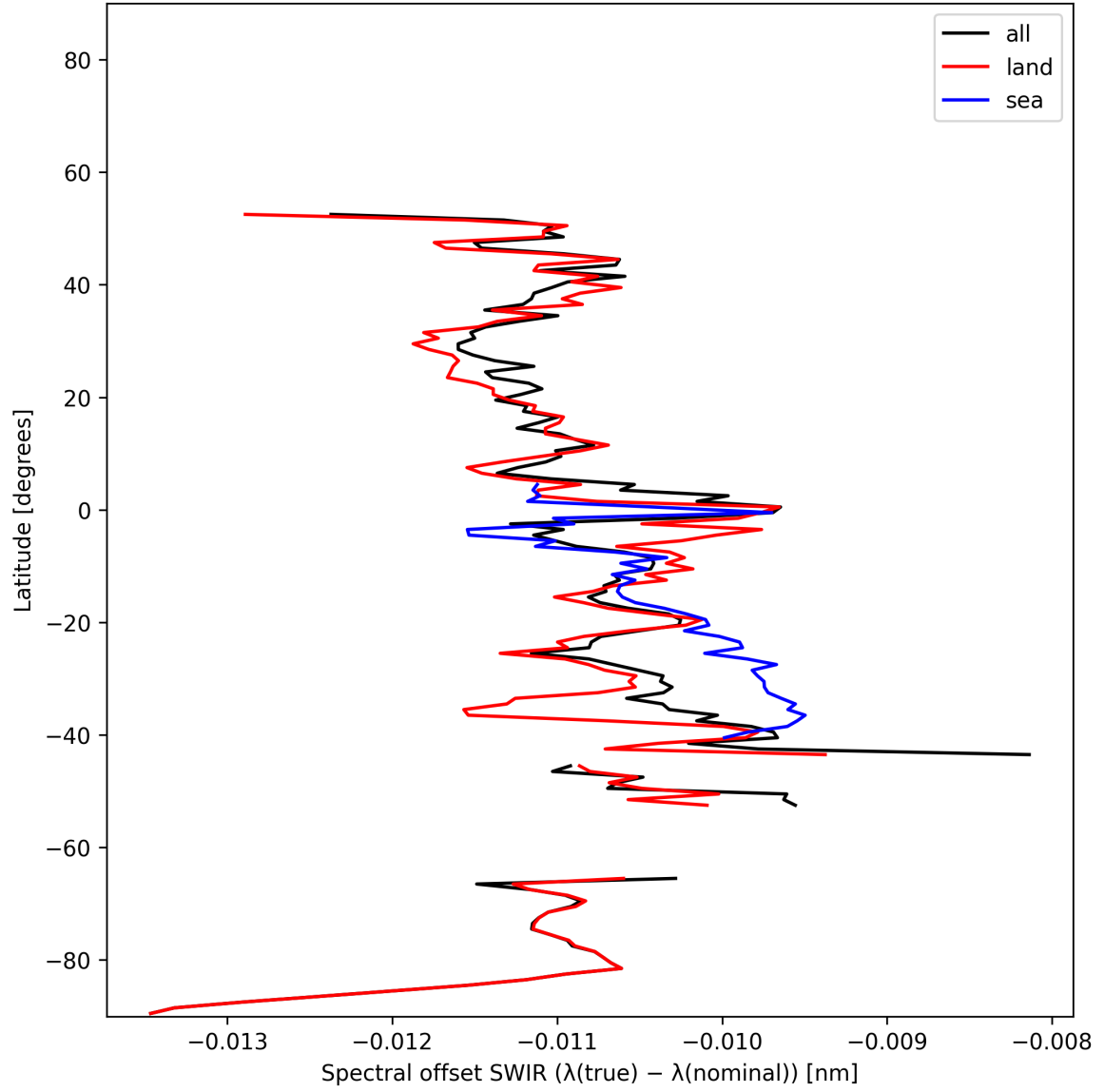
Figure 15: Zonal average of “Spectral offset SWIR ( \lambda_{\text{true}} - \lambda_{\text{nominal}} )” for 2025-12-09 to 2025-12-10.
