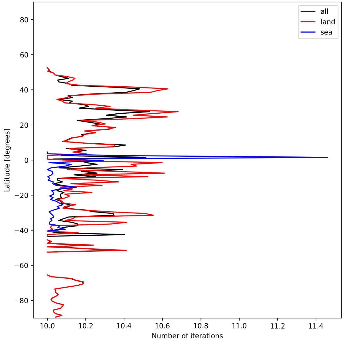
Figure 19: Zonal average of “Number of iterations” for 2025-12-09 to 2025-12-10.
