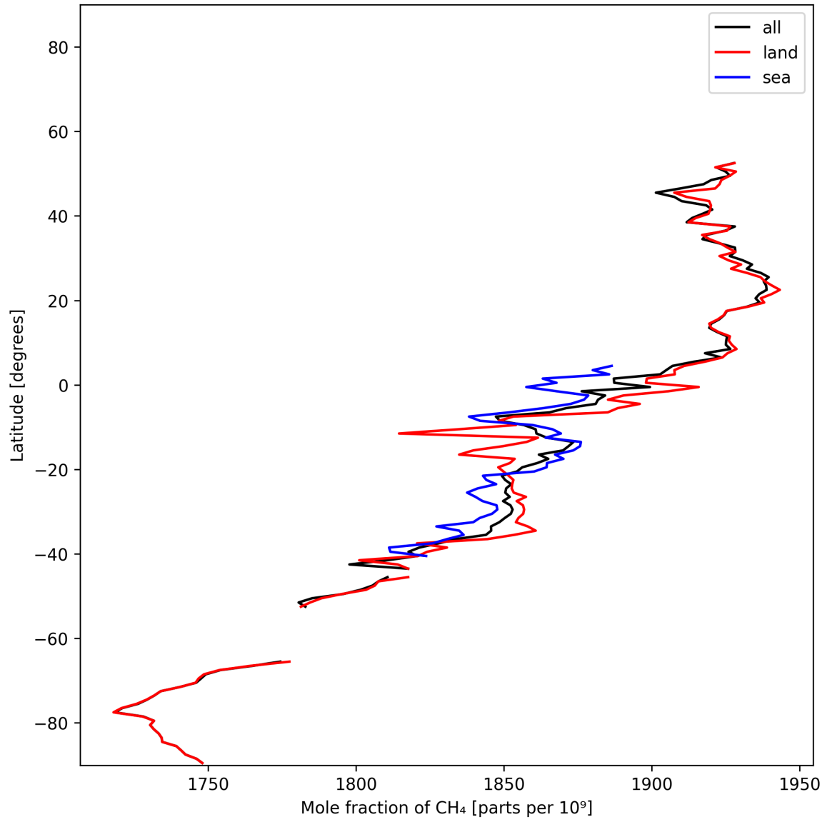
Figure 11: Zonal average of “Mole fraction of CH 4 ” for 2025-12-09 to 2025-12-10.
