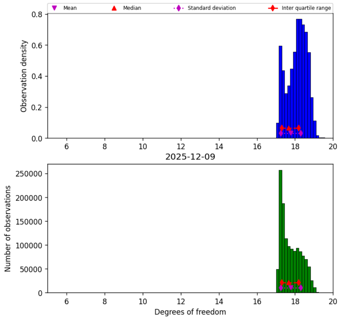
Figure 30: Histogram of “Degrees of freedom” for 2025-12-09 to 2025-12-10
