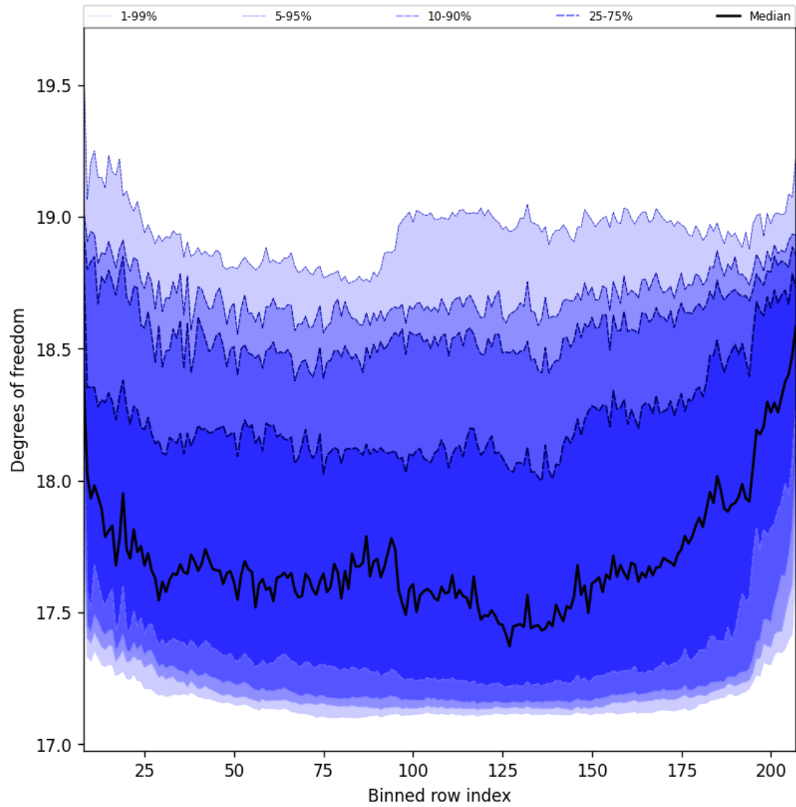
Figure 42: Along track statistics of “Degrees of freedom” for 2025-12-09 to 2025-12-10
