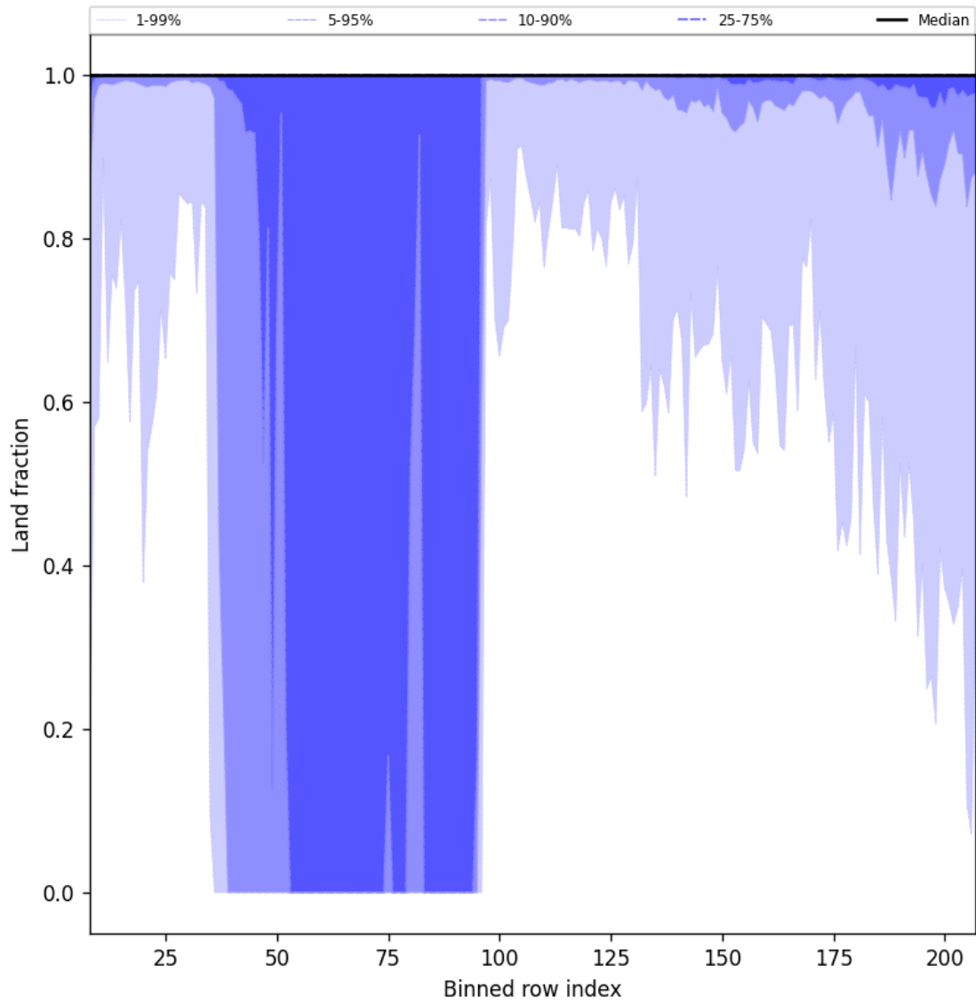
Figure 45: Along track statistics of "Land fraction" for 2025-12-09 to 2025-12-10
