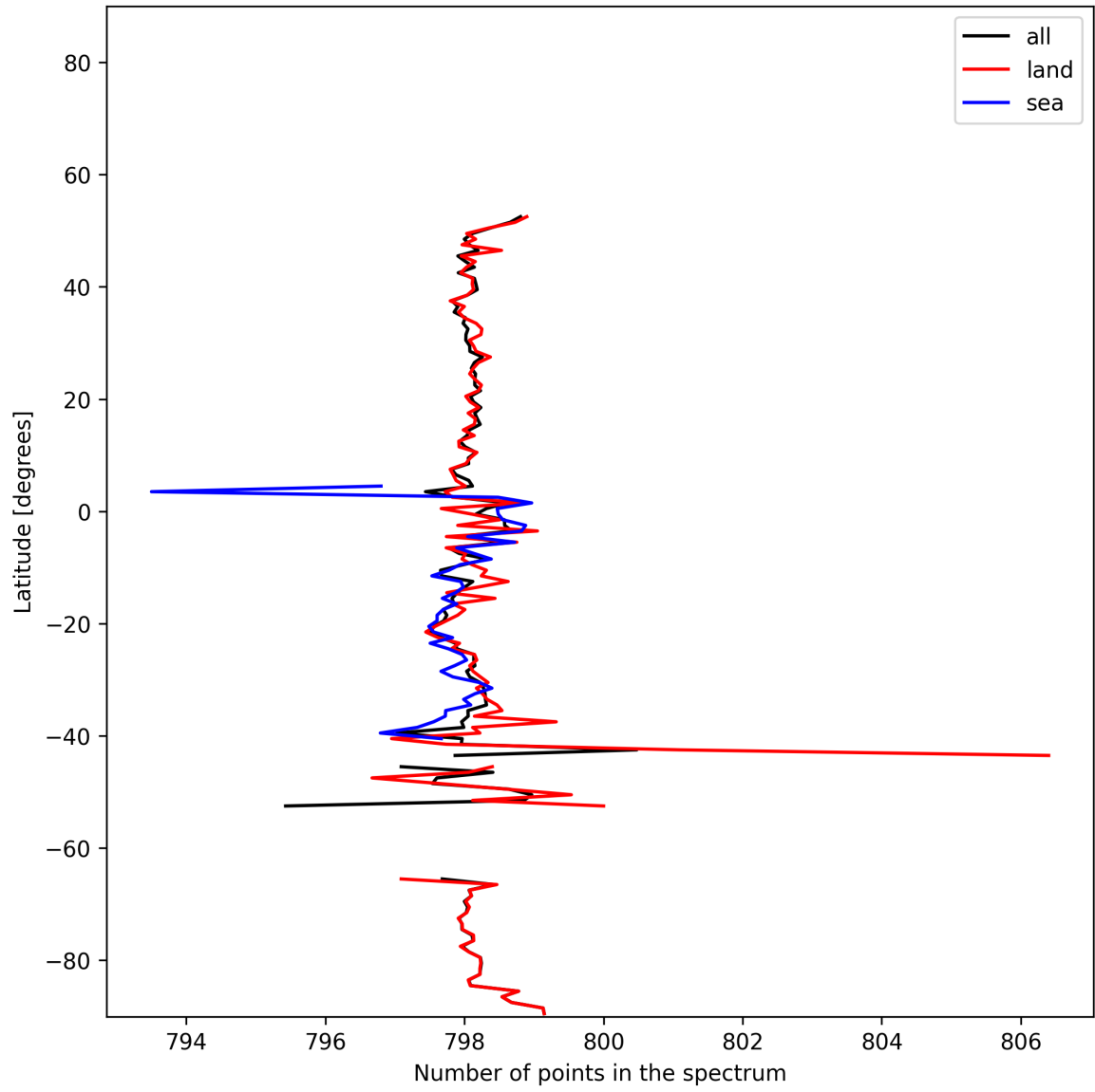
Figure 14: Zonal average of “Number of points in the spectrum” for 2025-12-09 to 2025-12-10.
