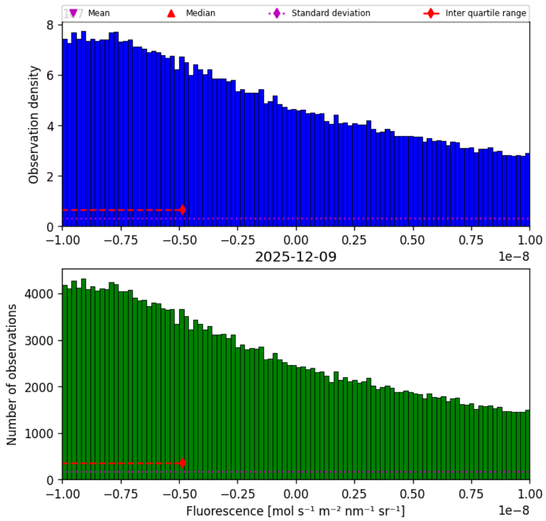
Figure 32: Histogram of “Fluorescence” for 2025-12-09 to 2025-12-10
