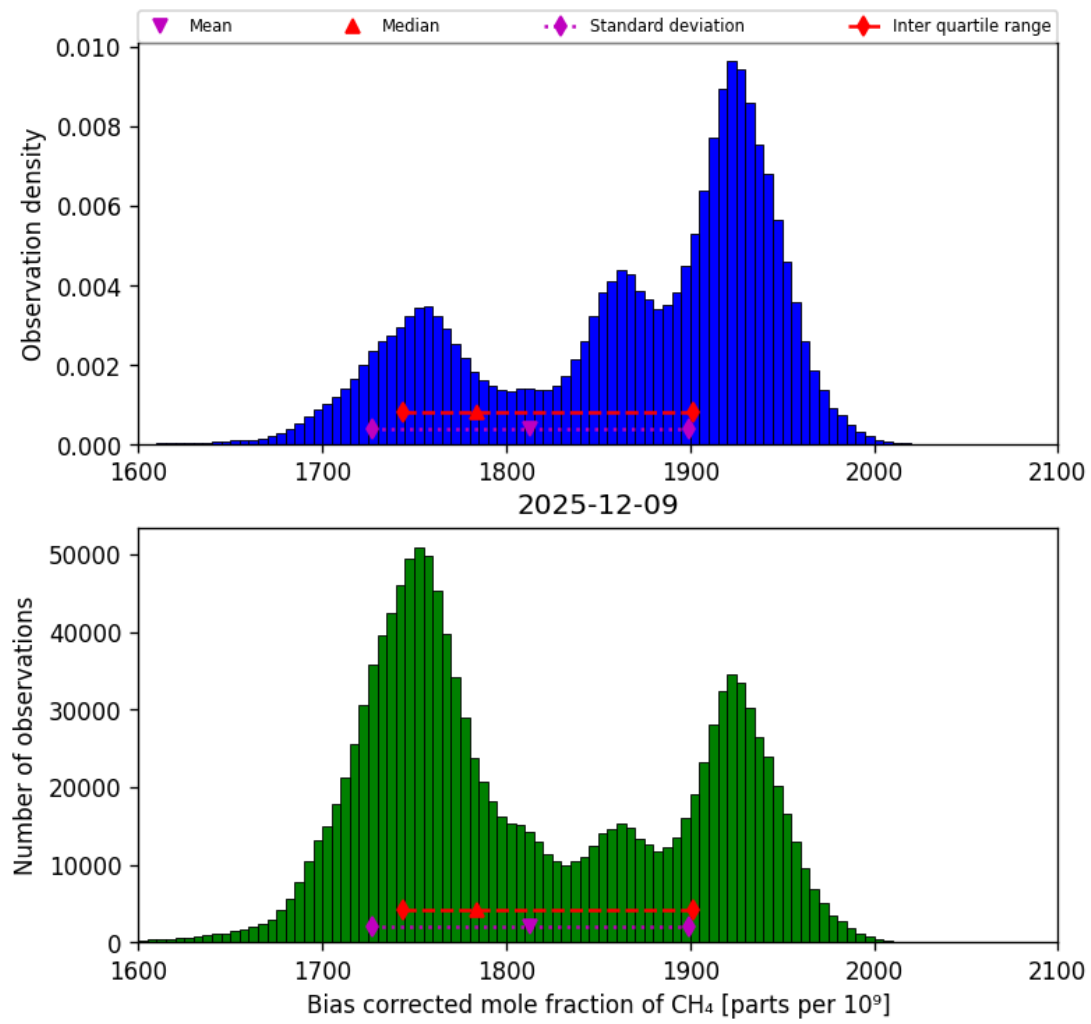
Figure 25: Histogram of “Bias corrected mole fraction of CH 4 ” for 2025-12-09 to 2025-12-10
