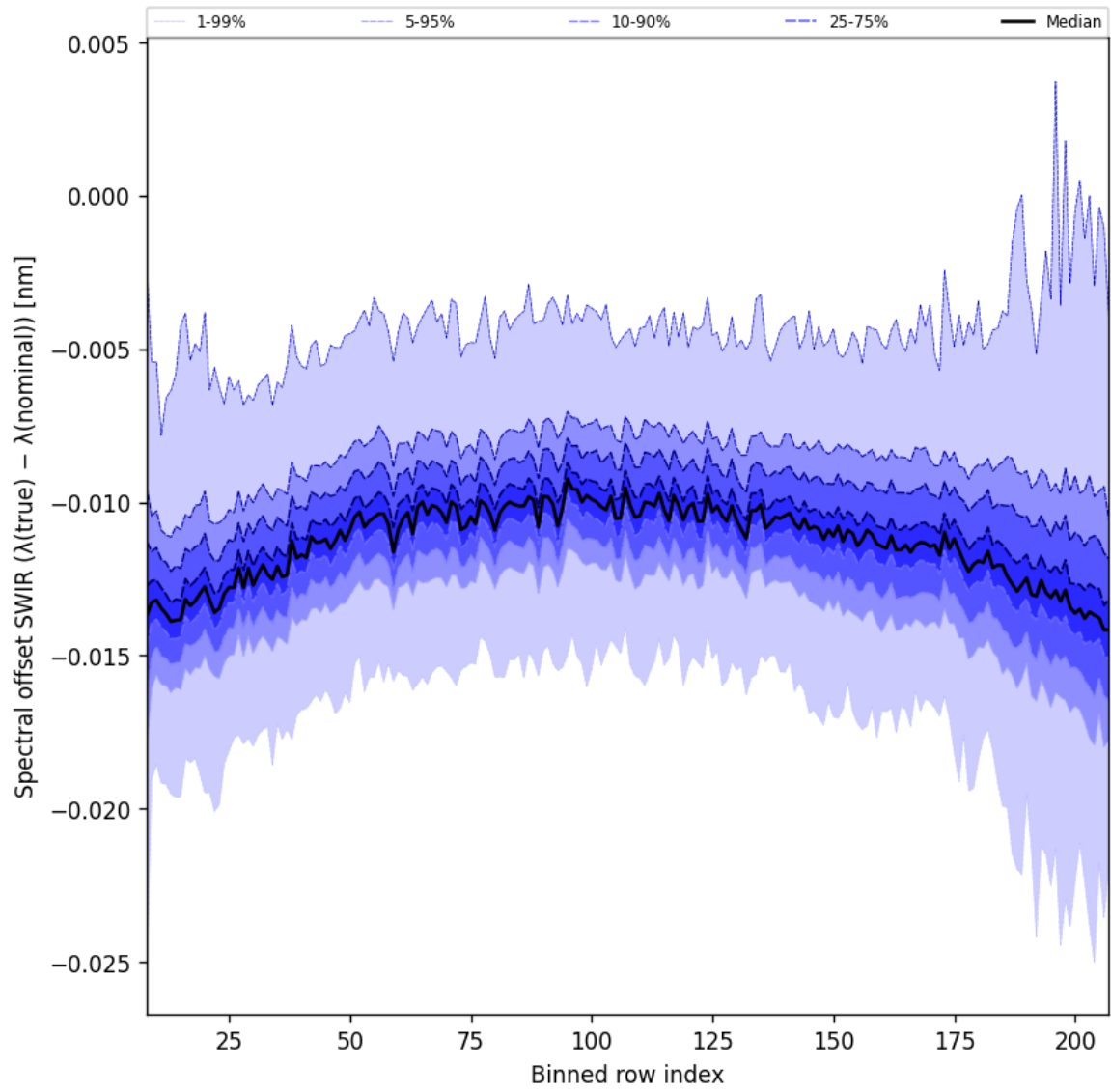
Figure 39: Along track statistics of “Spectral offset SWIR ( \lambda_{\text{true}} - \lambda_{\text{nominal}} )” for 2025-12-09 to 2025-12-10
