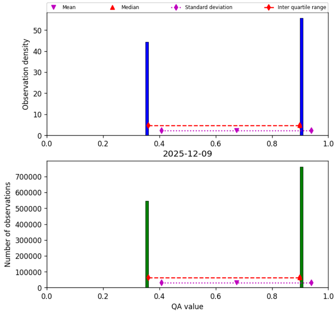
Figure 22: Histogram of “QA value” for 2025-12-09 to 2025-12-10
