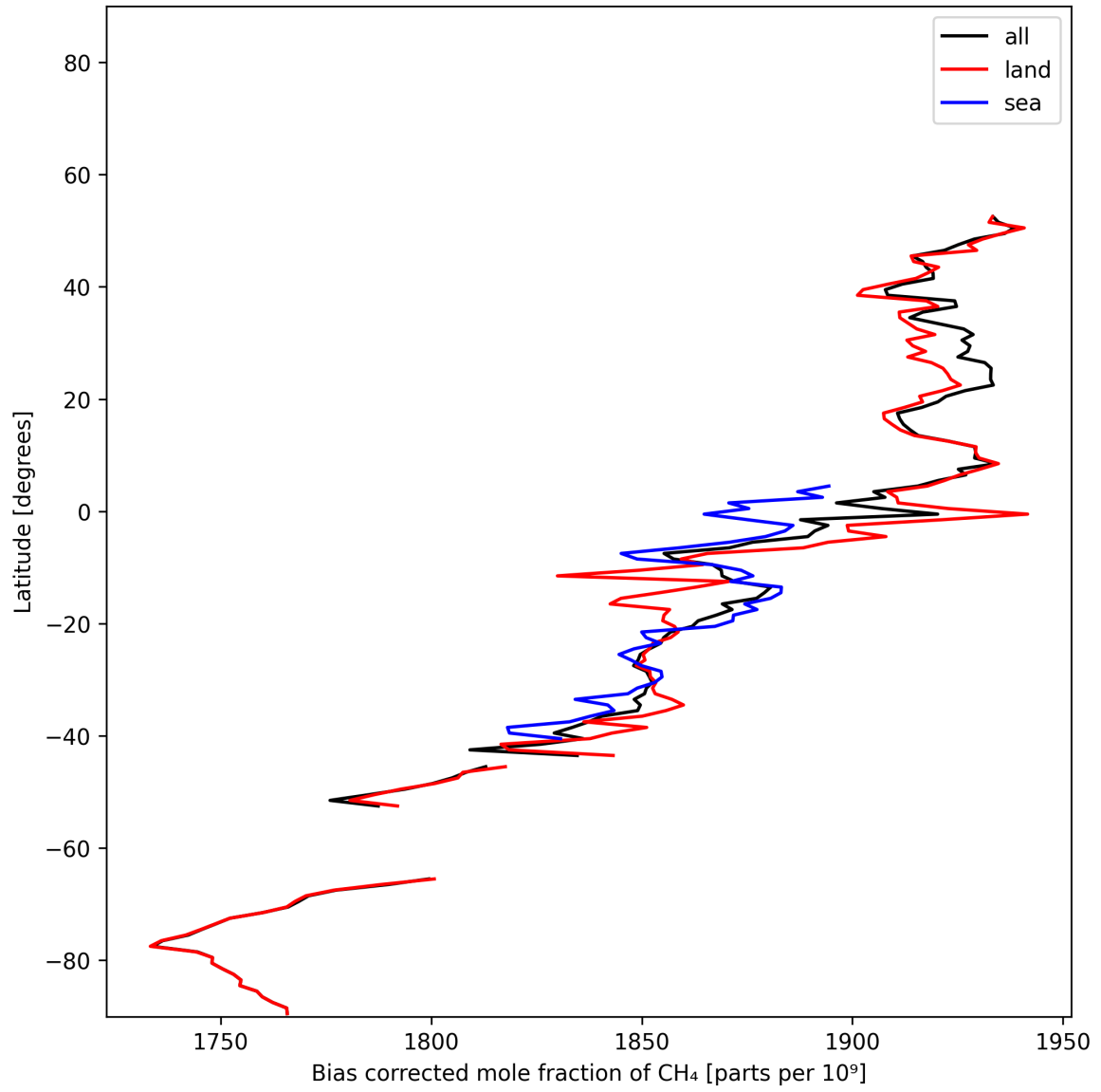
Figure 13: Zonal average of “Bias corrected mole fraction of CH 4 ” for 2025-12-09 to 2025-12-10.
