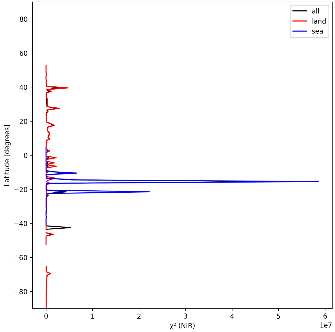
Figure 17: Zonal average of “ \chi^2 (NIR)” for 2025-12-09 to 2025-12-10.
