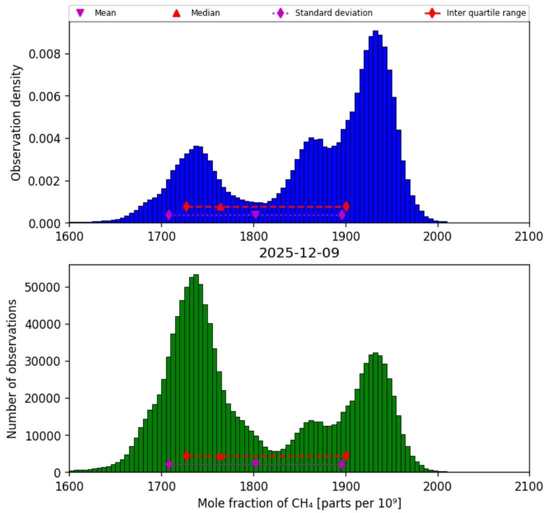
Figure 23: Histogram of “Mole fraction of CH 4 ” for 2025-12-09 to 2025-12-10
