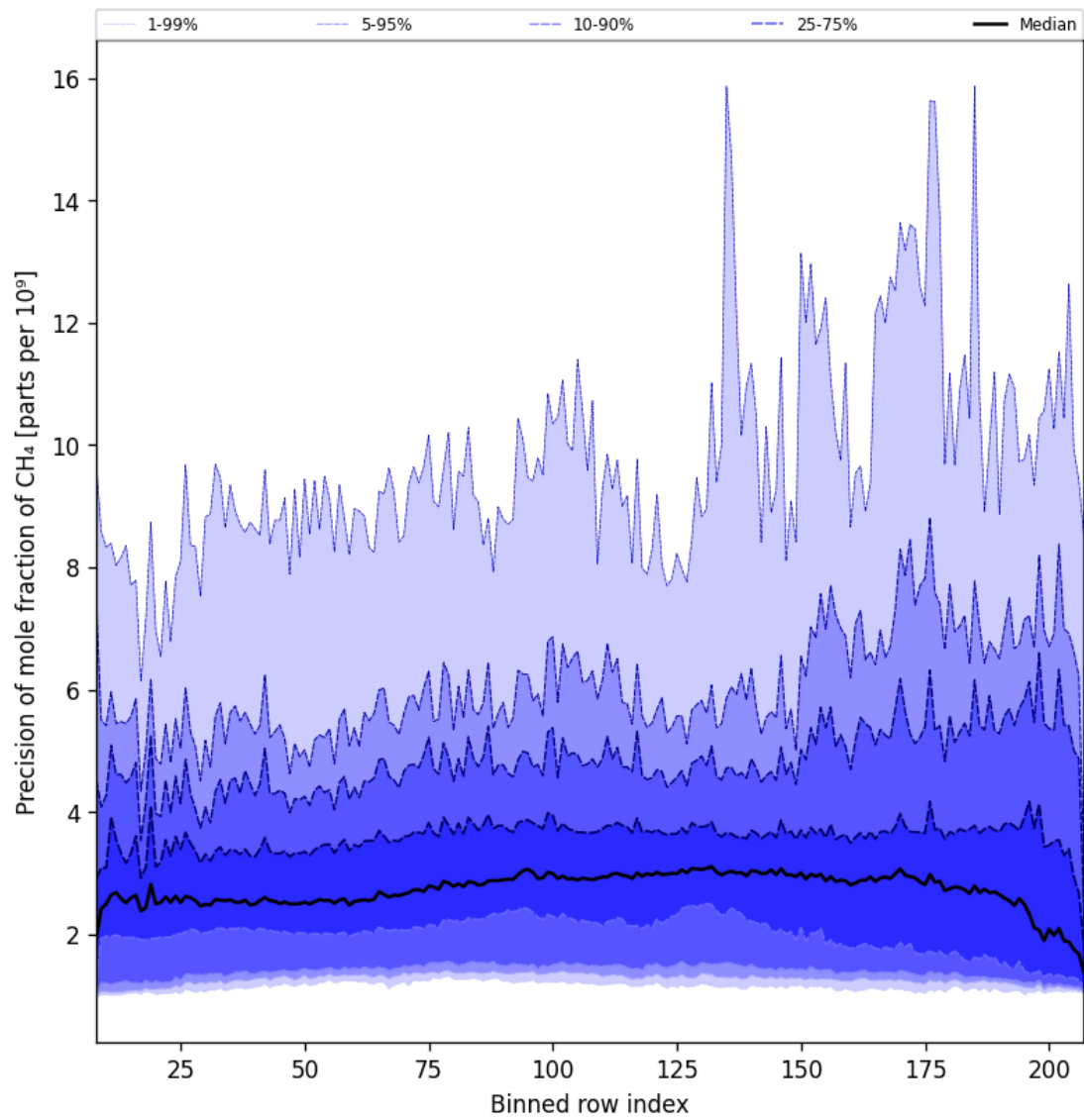
Figure 36: Along track statistics of “Precision of mole fraction of CH 4 ” for 2025-12-09 to 2025-12-10
