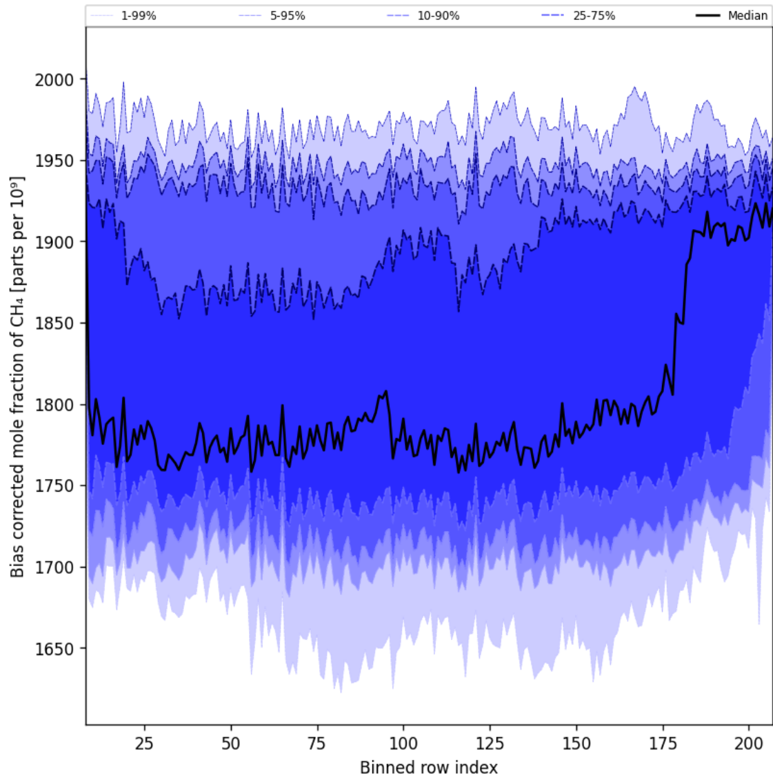
Figure 37: Along track statistics of “Bias corrected mole fraction of CH 4 ” for 2025-12-09 to 2025-12-10
