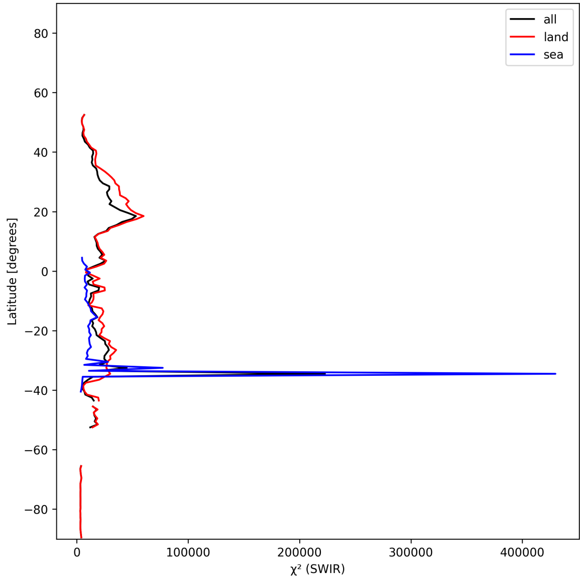
Figure 16: Zonal average of “ \chi^2 (SWIR)” for 2025-12-09 to 2025-12-10.
