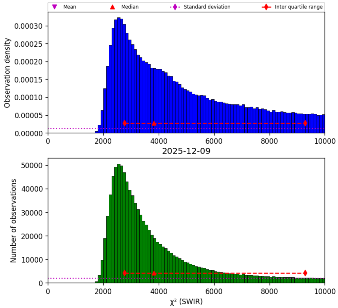
Figure 28: Histogram of “ \chi^2 (SWIR)” for 2025-12-09 to 2025-12-10
