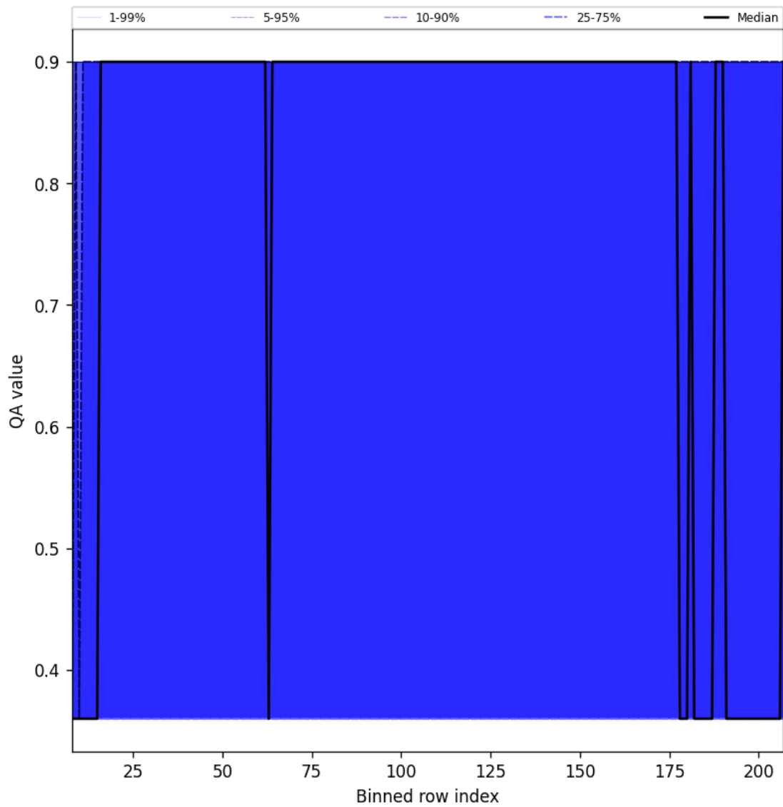
Figure 34: Along track statistics of “QA value” for 2025-12-09 to 2025-12-10
