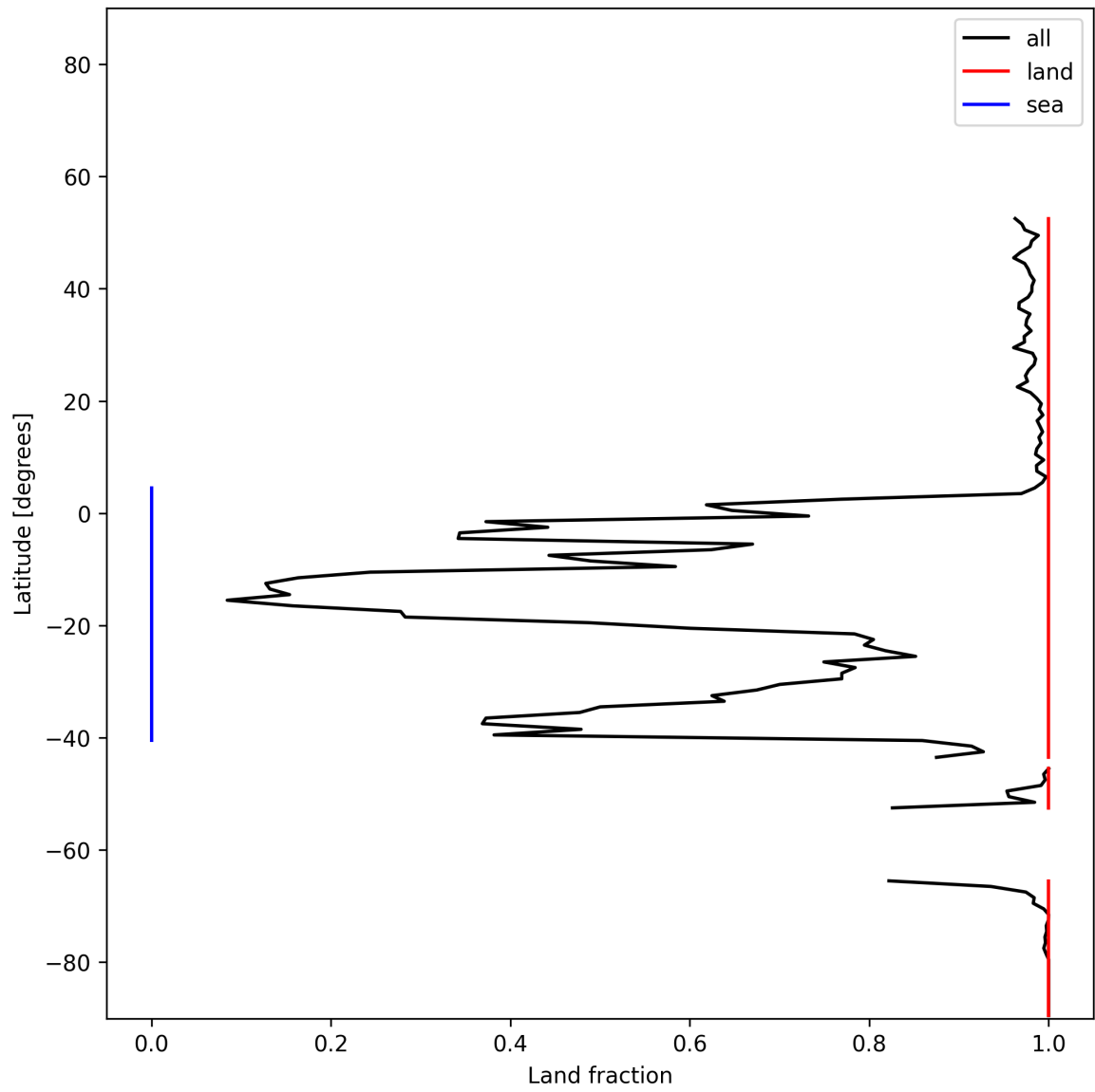
Figure 21: Zonal average of “Land fraction” for 2025-12-09 to 2025-12-10.
