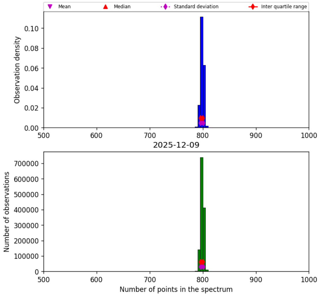
Figure 26: Histogram of “Number of points in the spectrum” for 2025-12-09 to 2025-12-10
