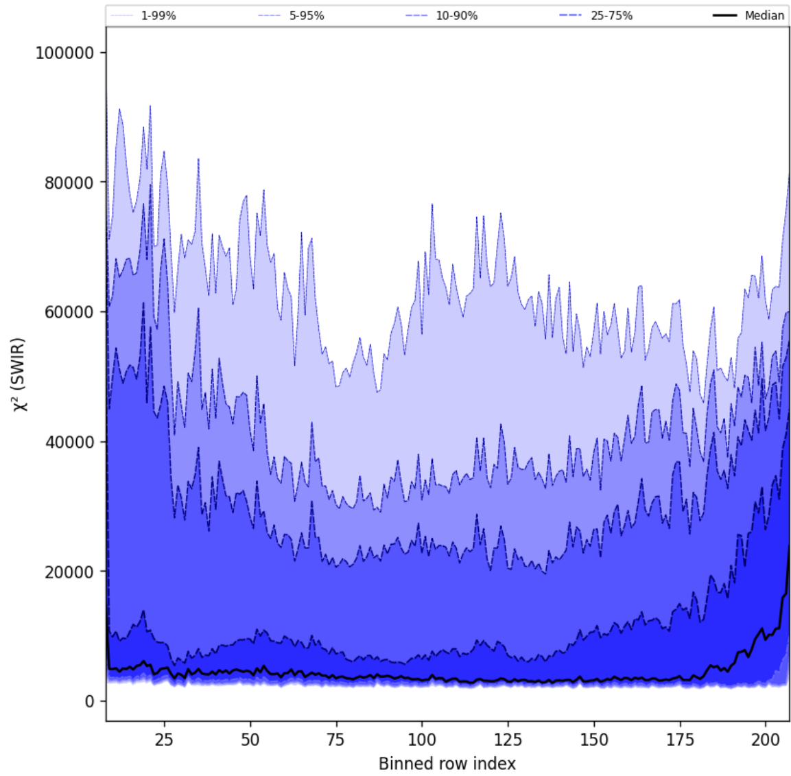
Figure 40: Along track statistics of “ \chi^2 (SWIR)” for 2025-12-09 to 2025-12-10
