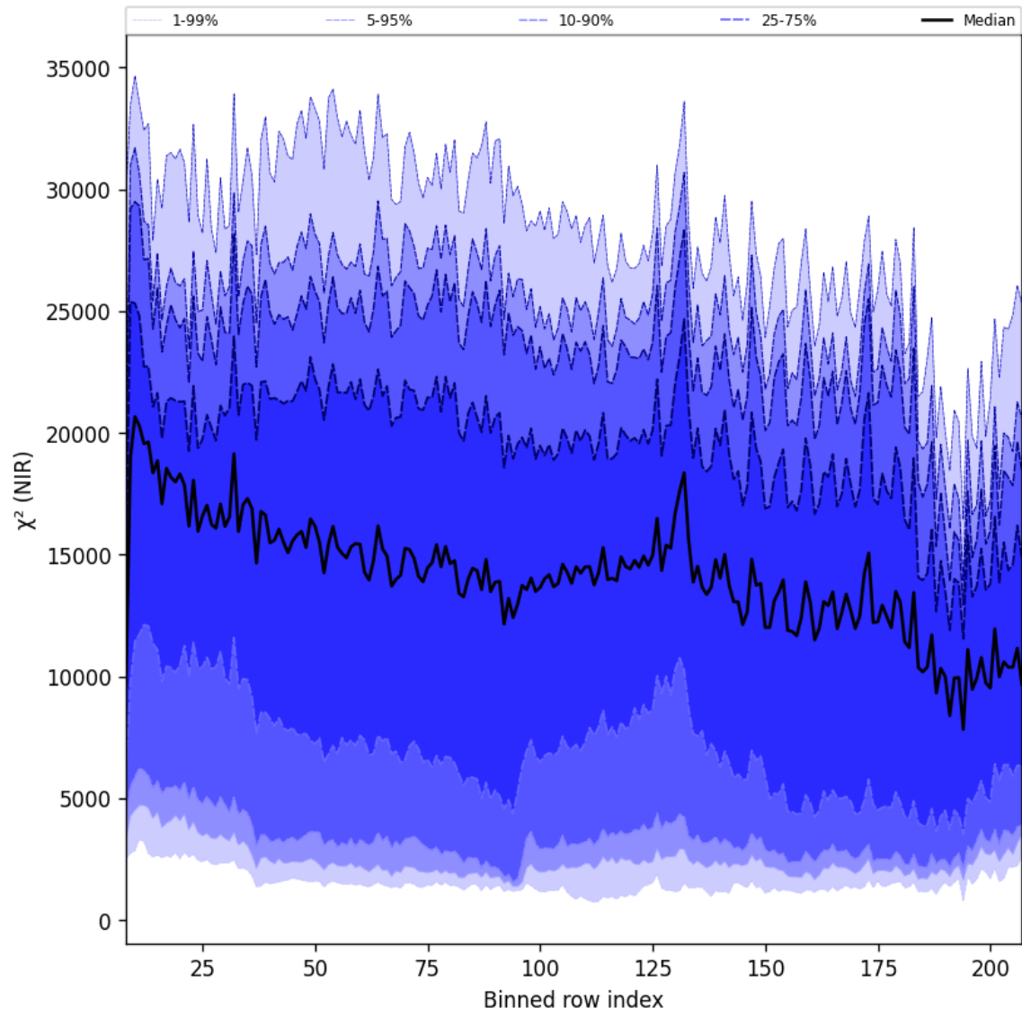
Figure 41: Along track statistics of “ \chi^2 (NIR)” for 2025-12-09 to 2025-12-10
