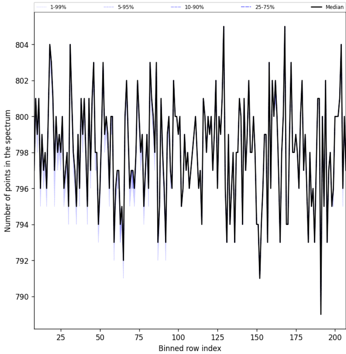
Figure 38: Along track statistics of “Number of points in the spectrum” for 2025-12-09 to 2025-12-10
