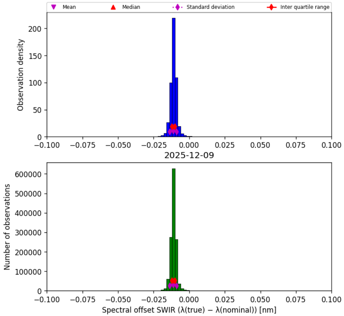
Figure 27: Histogram of “Spectral offset SWIR ( \lambda_{\text{true}} - \lambda_{\text{nominal}} )” for 2025-12-09 to 2025-12-10
