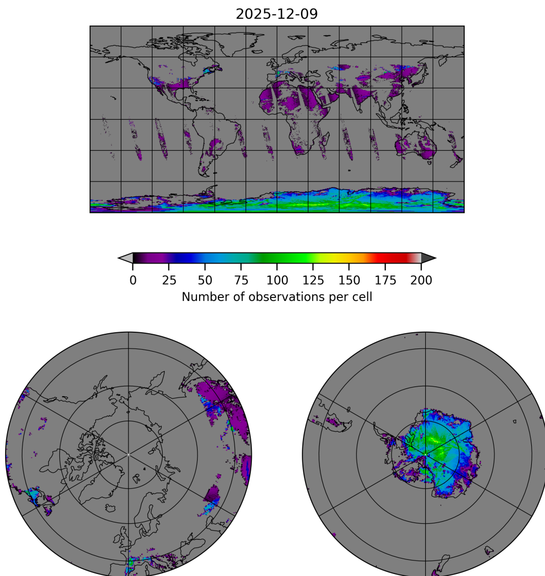
Figure 9: Map of the number of observations for 2025-12-09 to 2025-12-10
