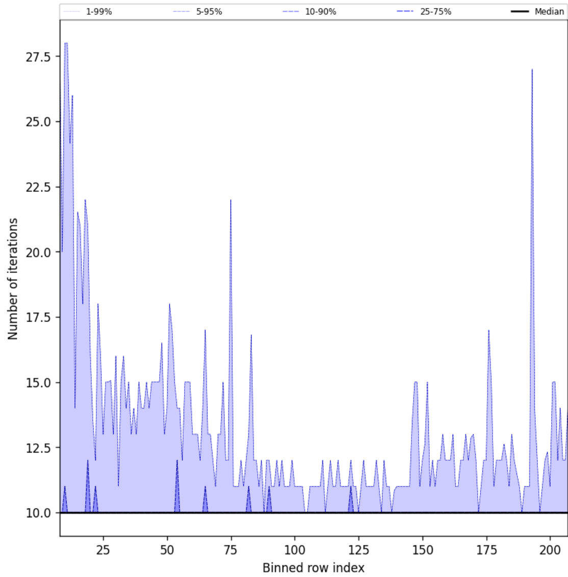
Figure 43: Along track statistics of “Number of iterations” for 2025-12-09 to 2025-12-10
