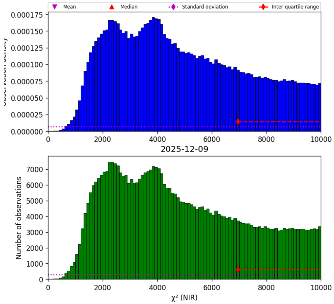
Figure 29: Histogram of “ \chi^2 (NIR)” for 2025-12-09 to 2025-12-10
