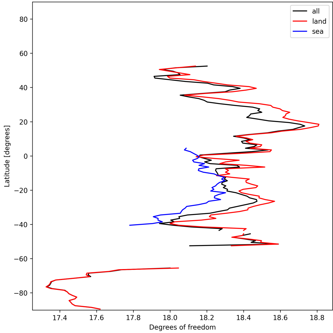
Figure 18: Zonal average of “Degrees of freedom” for 2025-12-09 to 2025-12-10.
