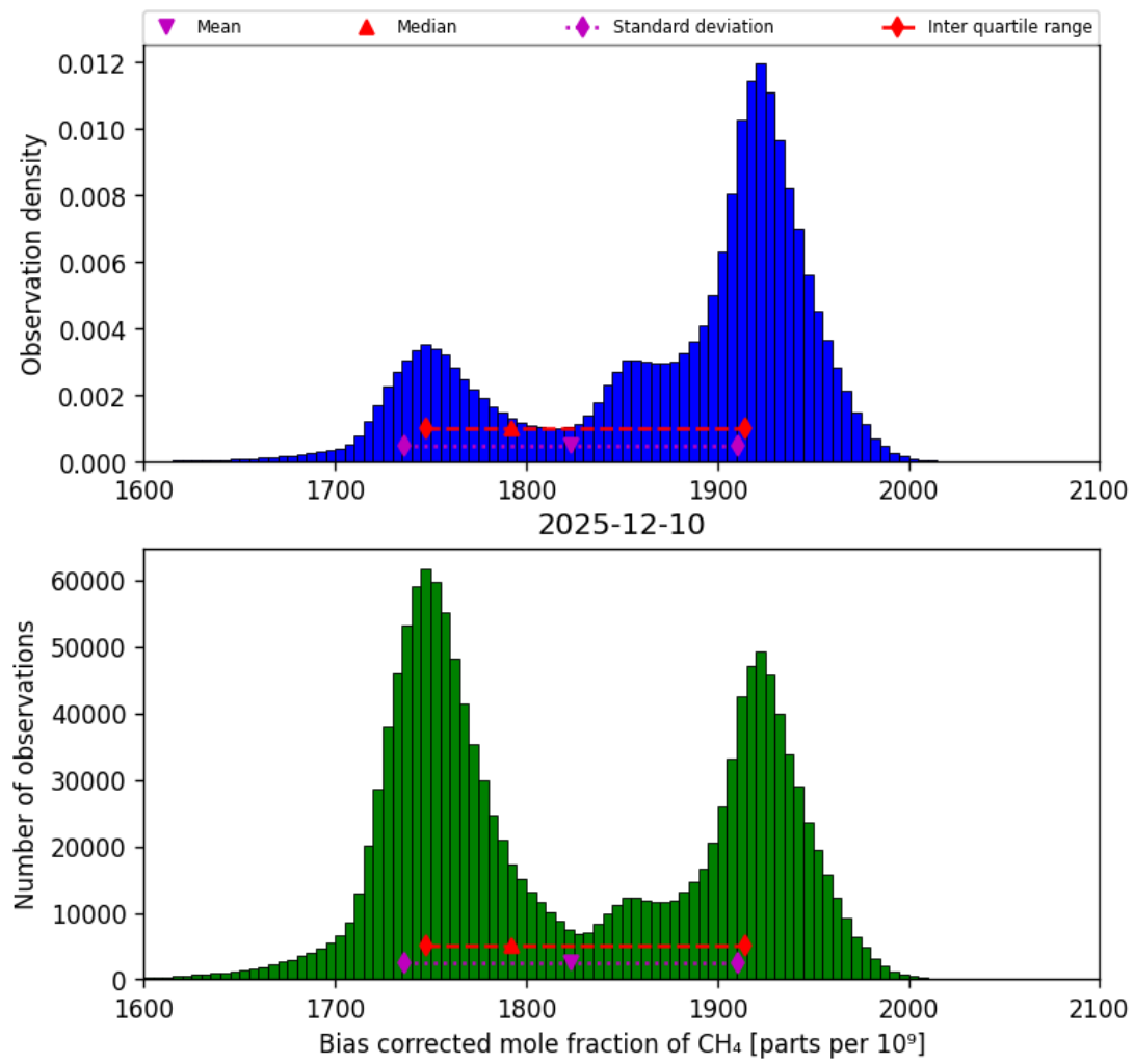
Figure 25: Histogram of “Bias corrected mole fraction of CH 4 ” for 2025-12-10 to 2025-12-11
