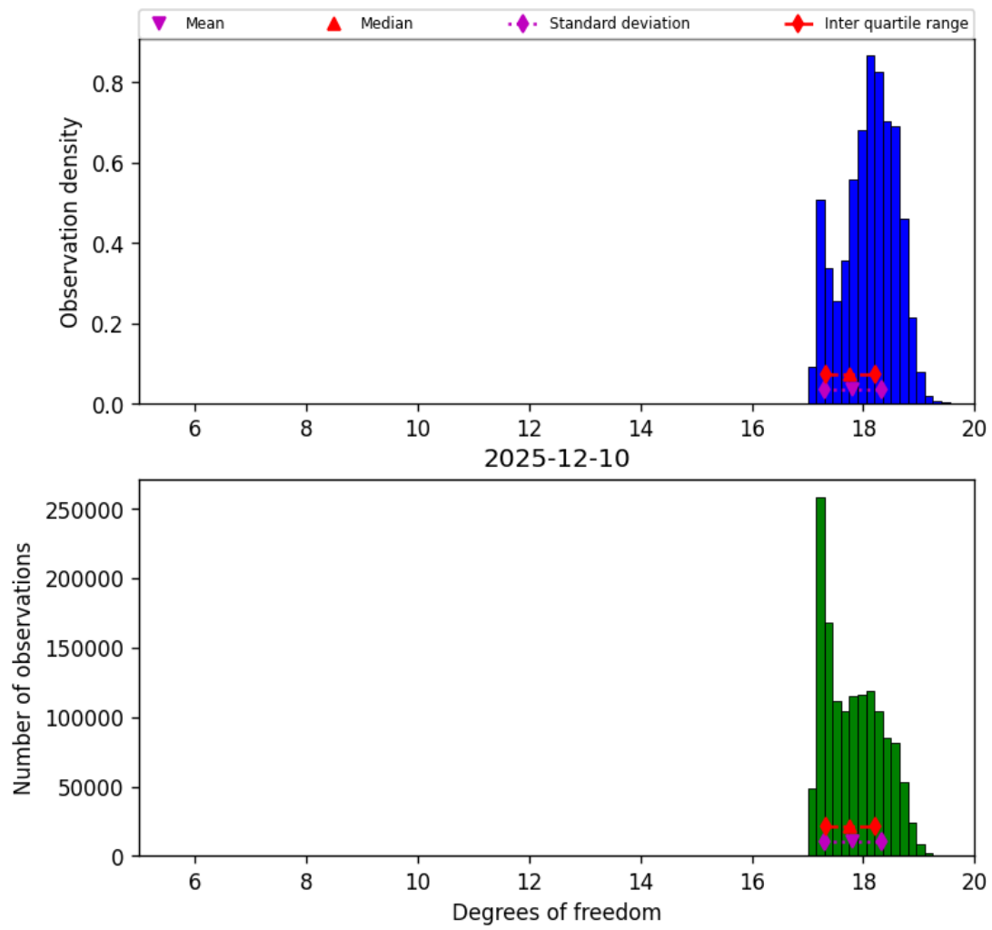
Figure 30: Histogram of “Degrees of freedom” for 2025-12-10 to 2025-12-11
