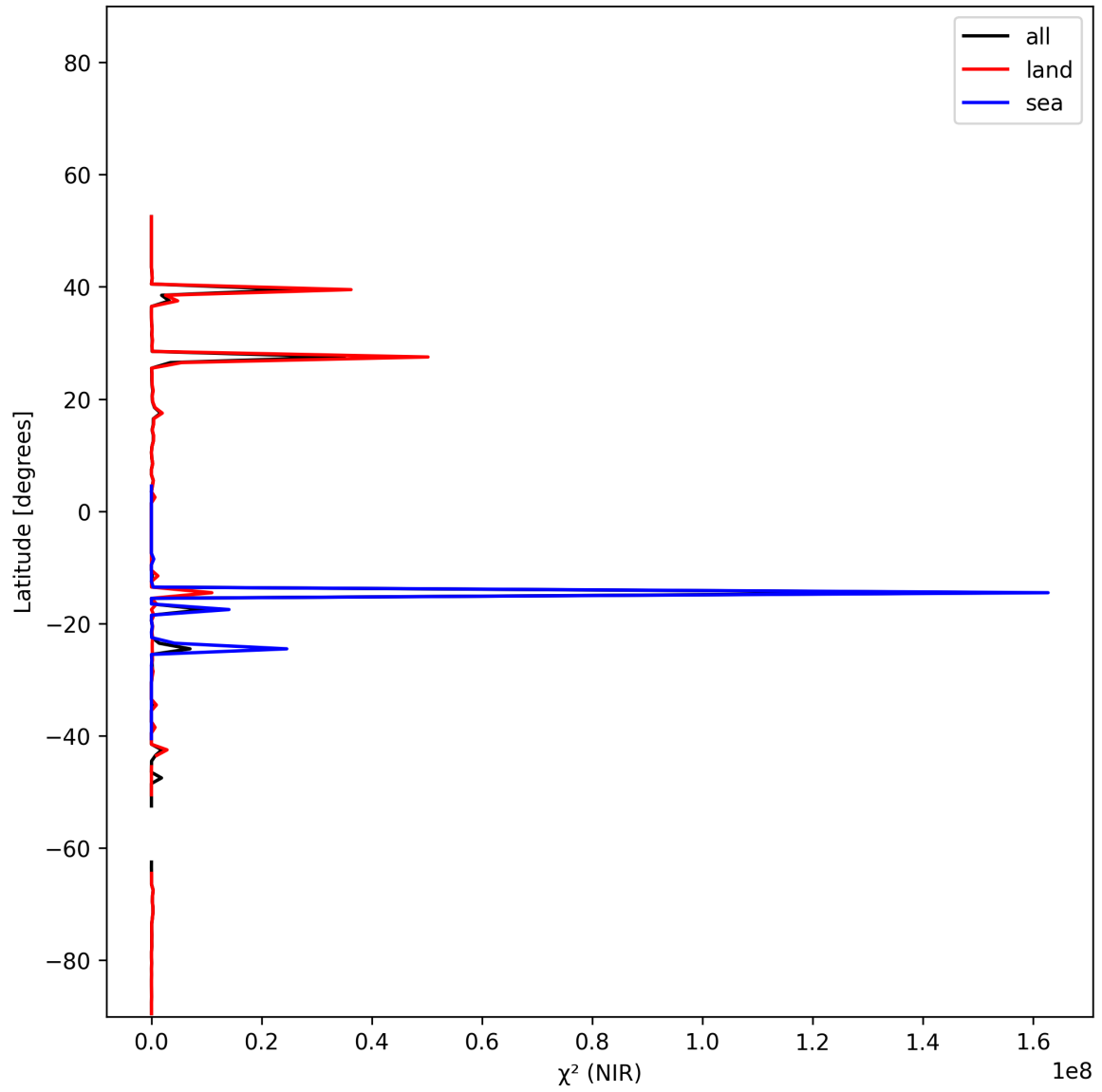
Figure 17: Zonal average of “ \chi^2 (NIR)” for 2025-12-10 to 2025-12-11.
