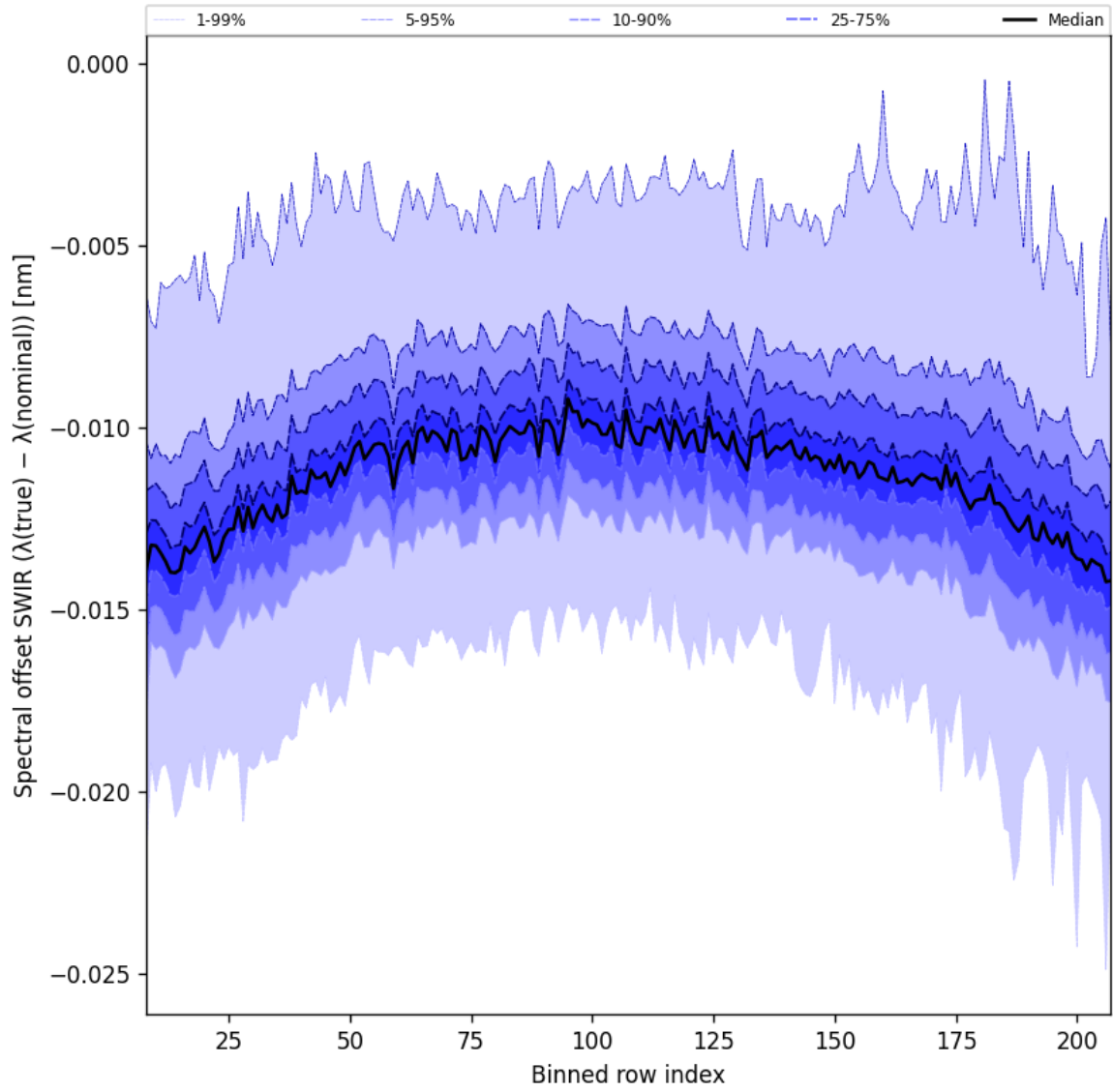
Figure 39: Along track statistics of “Spectral offset SWIR ( \lambda_{\text{true}} - \lambda_{\text{nominal}} )” for 2025-12-10 to 2025-12-11
