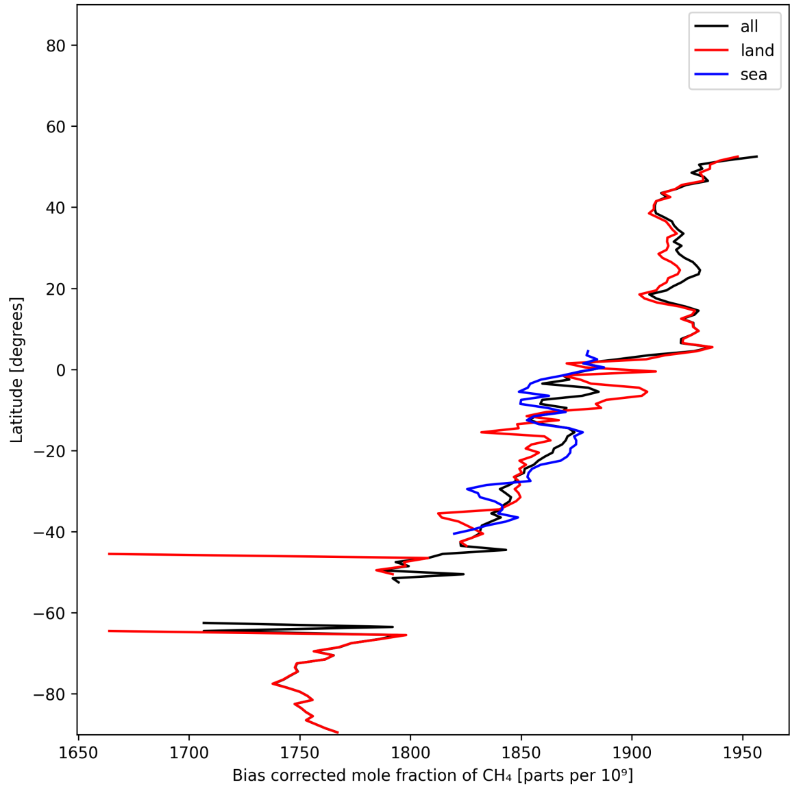
Figure 13: Zonal average of “Bias corrected mole fraction of \text{CH}_4 ” for 2025-12-10 to 2025-12-11.
