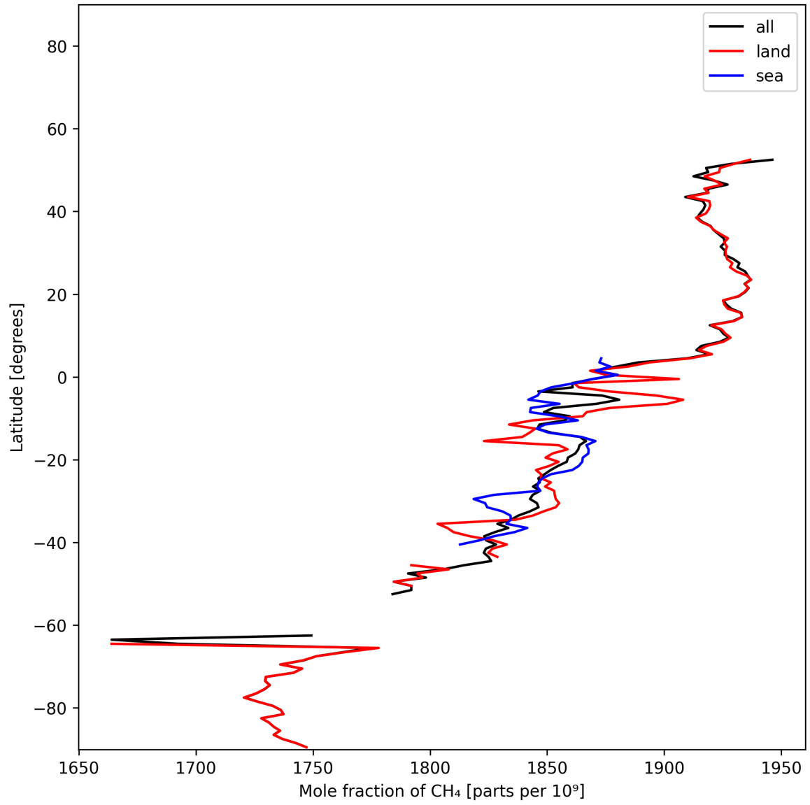
Figure 11: Zonal average of “Mole fraction of CH 4 ” for 2025-12-10 to 2025-12-11.
