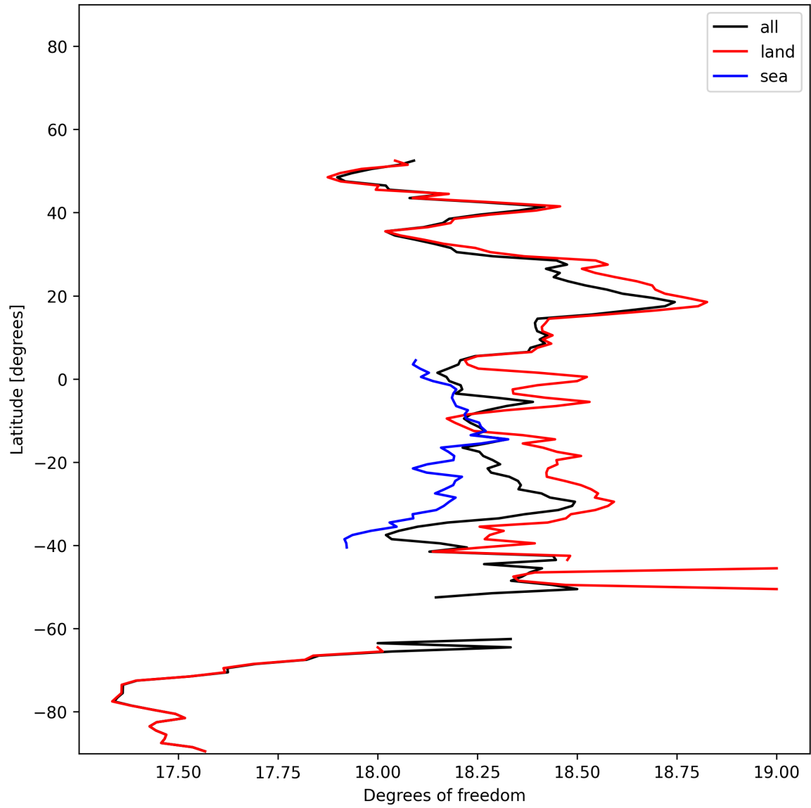
Figure 18: Zonal average of “Degrees of freedom” for 2025-12-10 to 2025-12-11.
