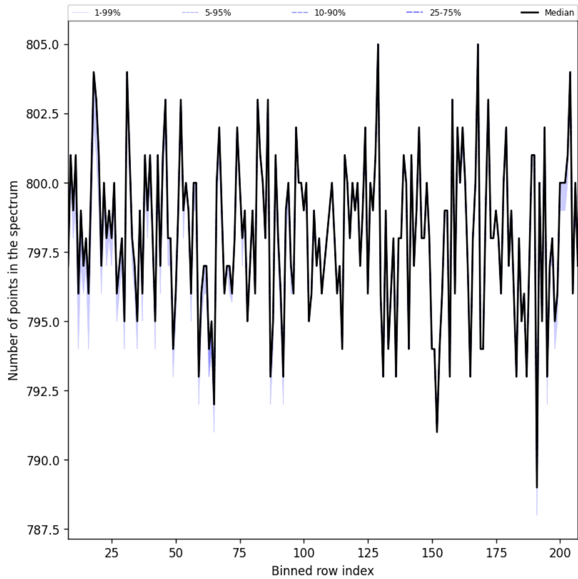
Figure 38: Along track statistics of “Number of points in the spectrum” for 2025-12-10 to 2025-12-11
