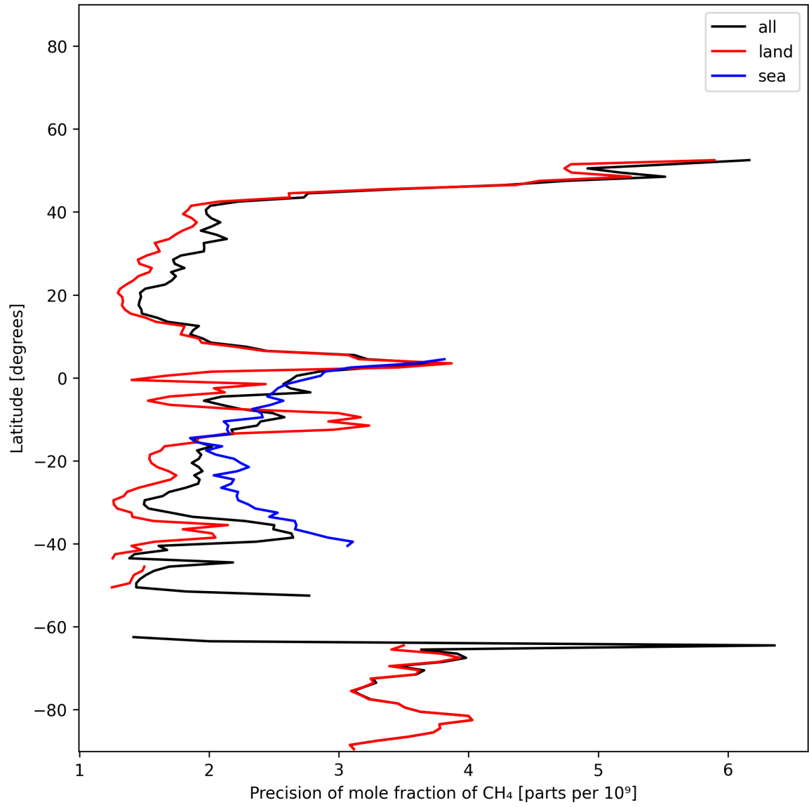
Figure 12: Zonal average of “Precision of mole fraction of CH 4 ” for 2025-12-10 to 2025-12-11.
