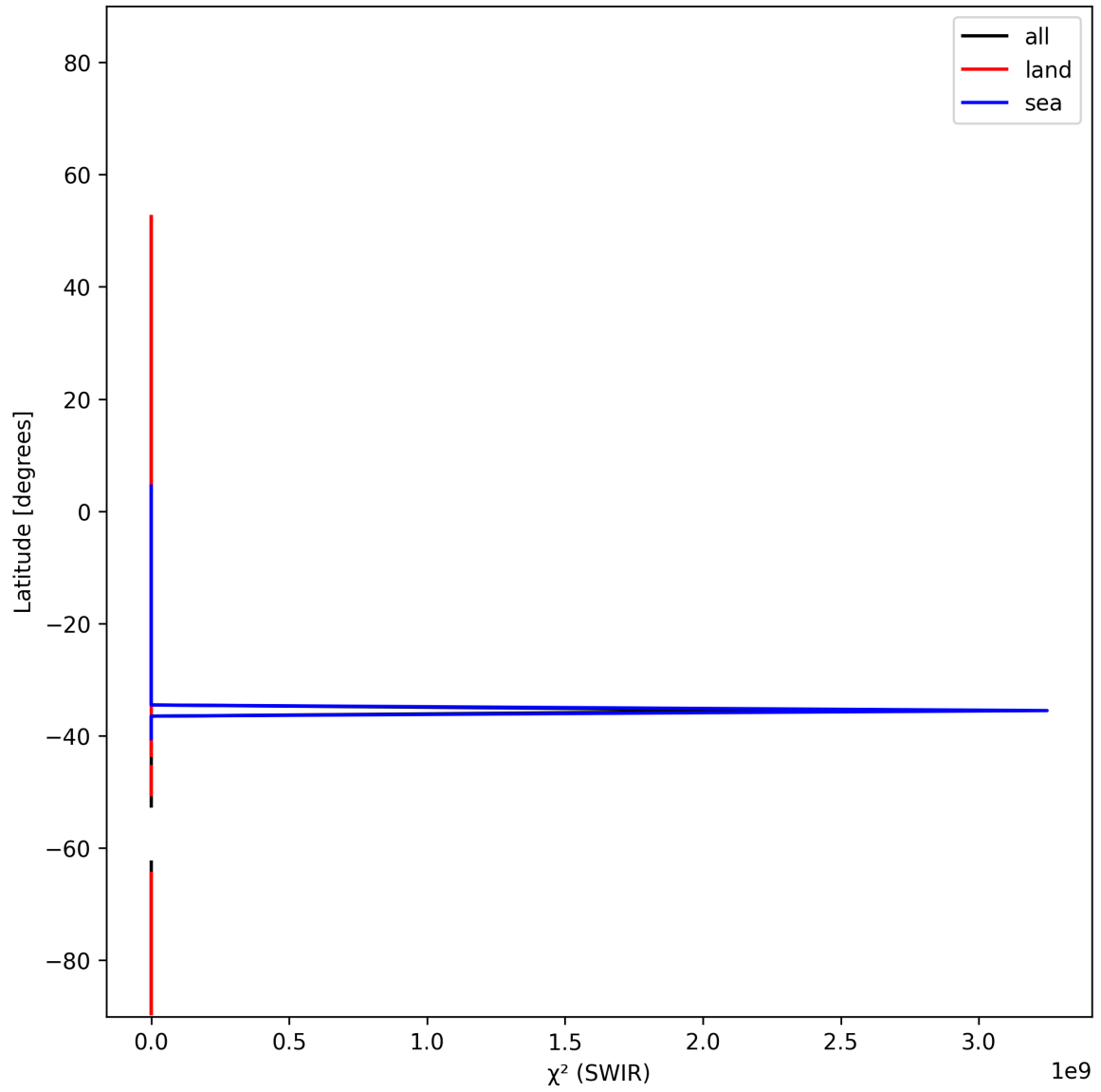
Figure 16: Zonal average of “ \chi^2 (SWIR)” for 2025-12-10 to 2025-12-11.
