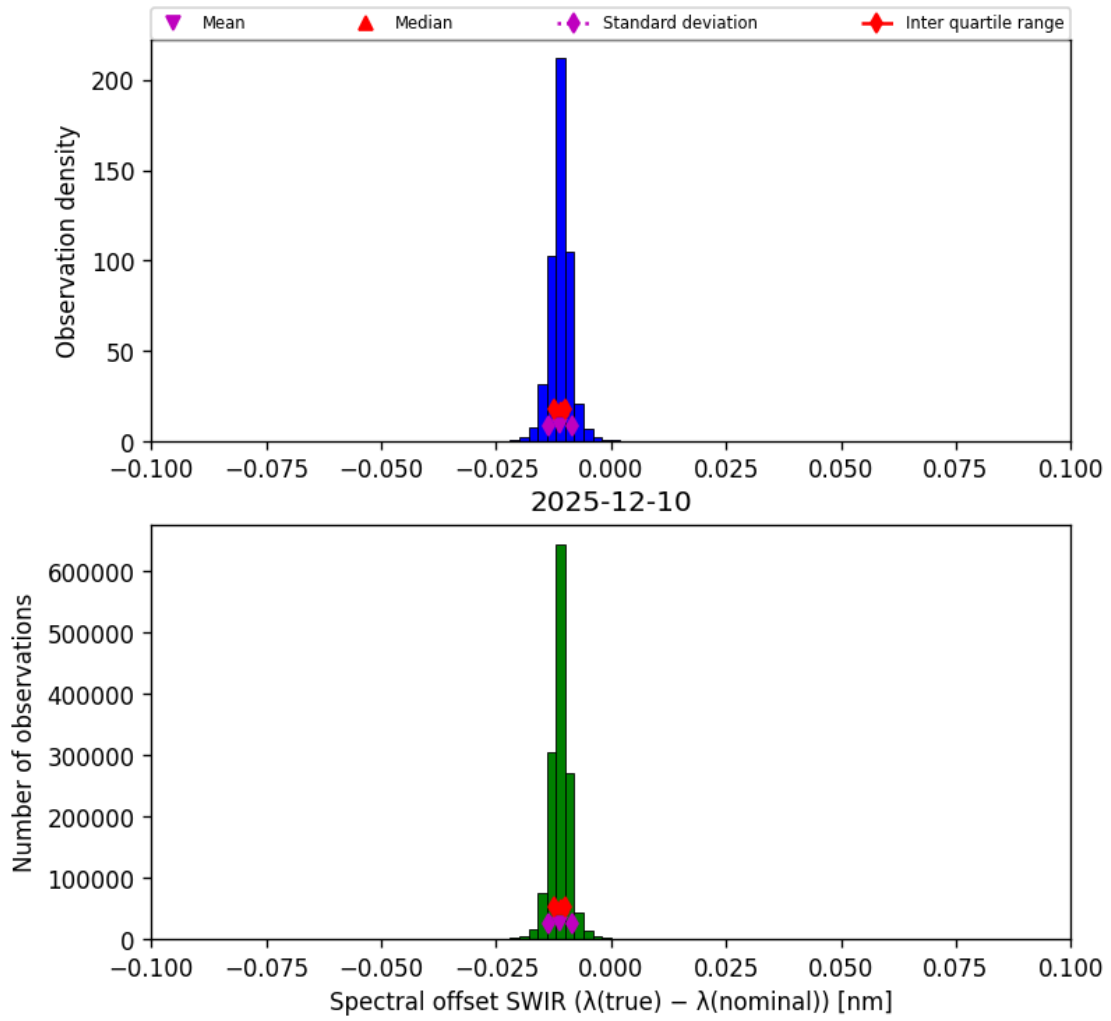
Figure 27: Histogram of “Spectral offset SWIR ( \lambda_{\text{true}} - \lambda_{\text{nominal}} )” for 2025-12-10 to 2025-12-11
