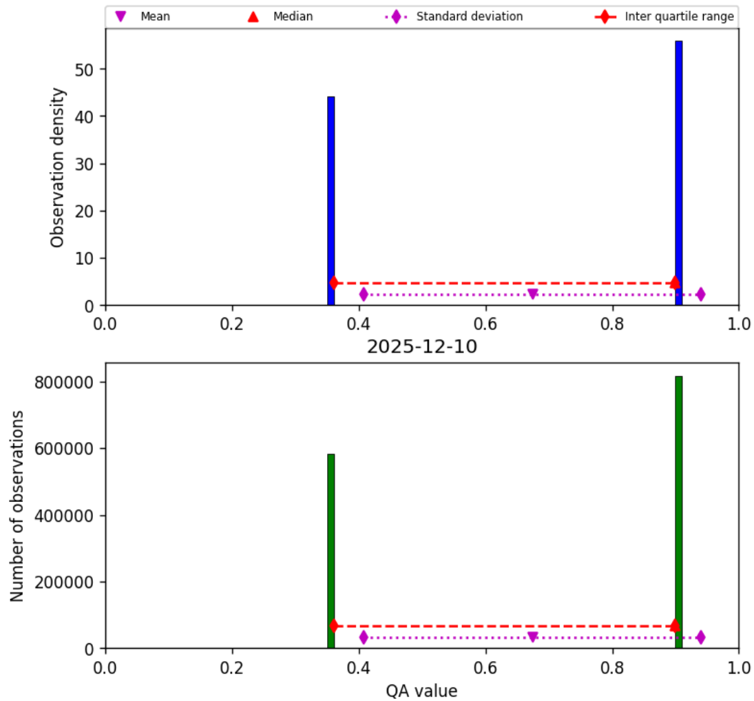
Figure 22: Histogram of “QA value” for 2025-12-10 to 2025-12-11
