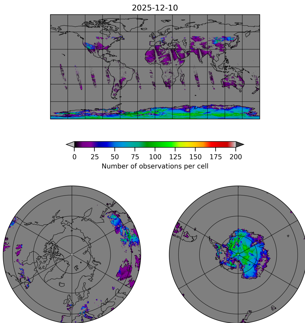
Figure 9: Map of the number of observations for 2025-12-10 to 2025-12-11
