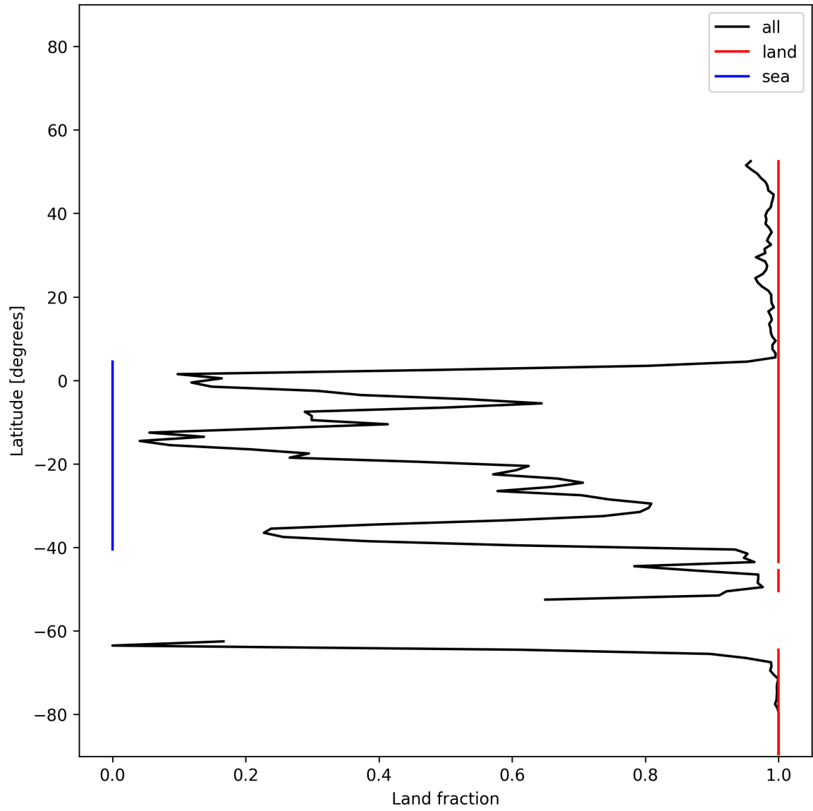
Figure 21: Zonal average of “Land fraction” for 2025-12-10 to 2025-12-11.
