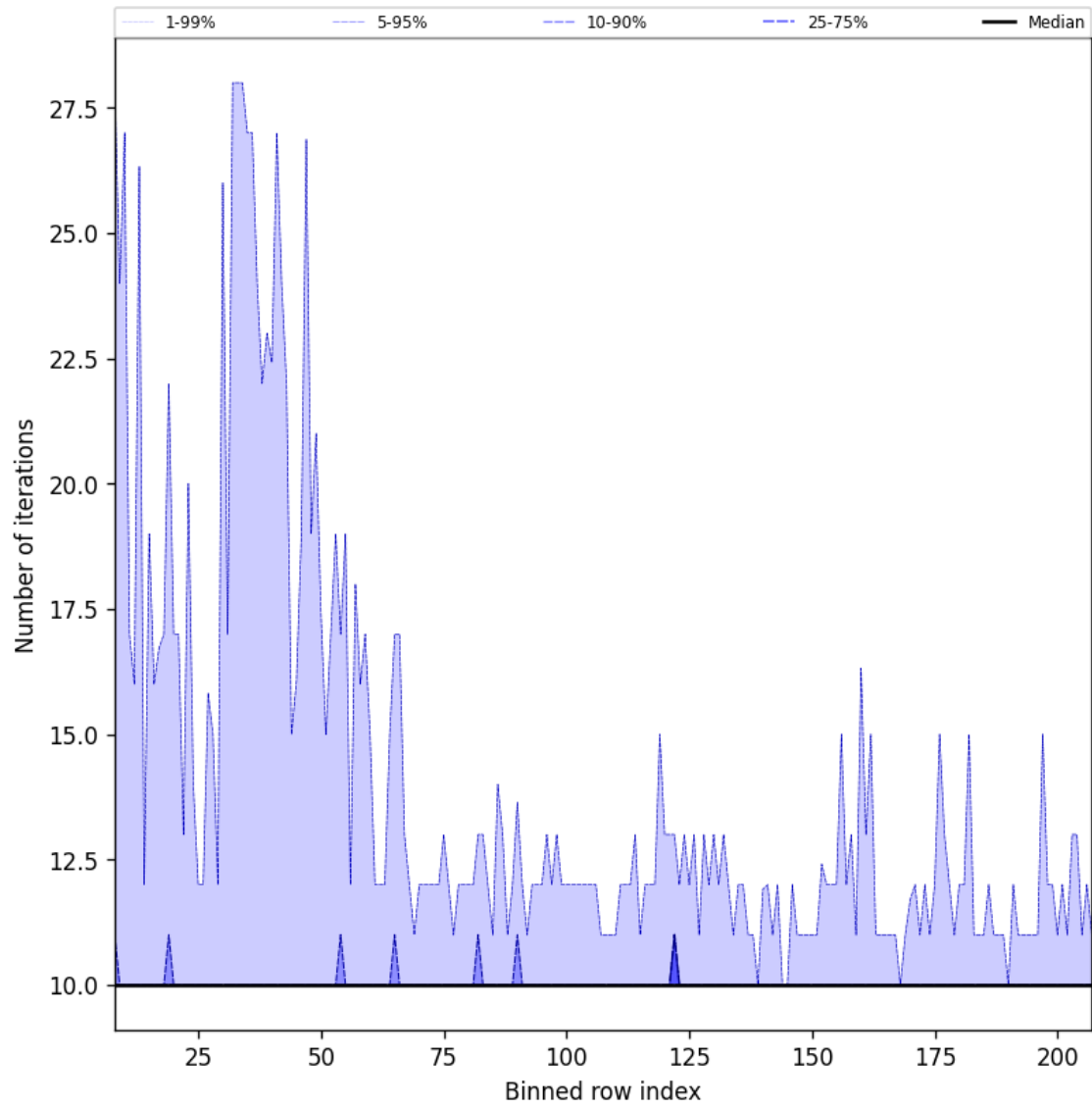
Figure 43: Along track statistics of “Number of iterations” for 2025-12-10 to 2025-12-11
