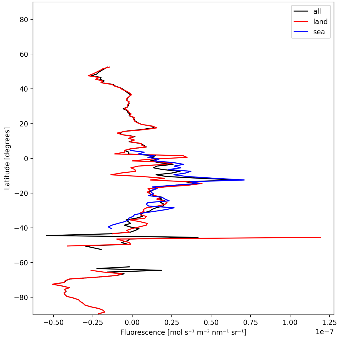
Figure 20: Zonal average of “Fluorescence” for 2025-12-10 to 2025-12-11.
