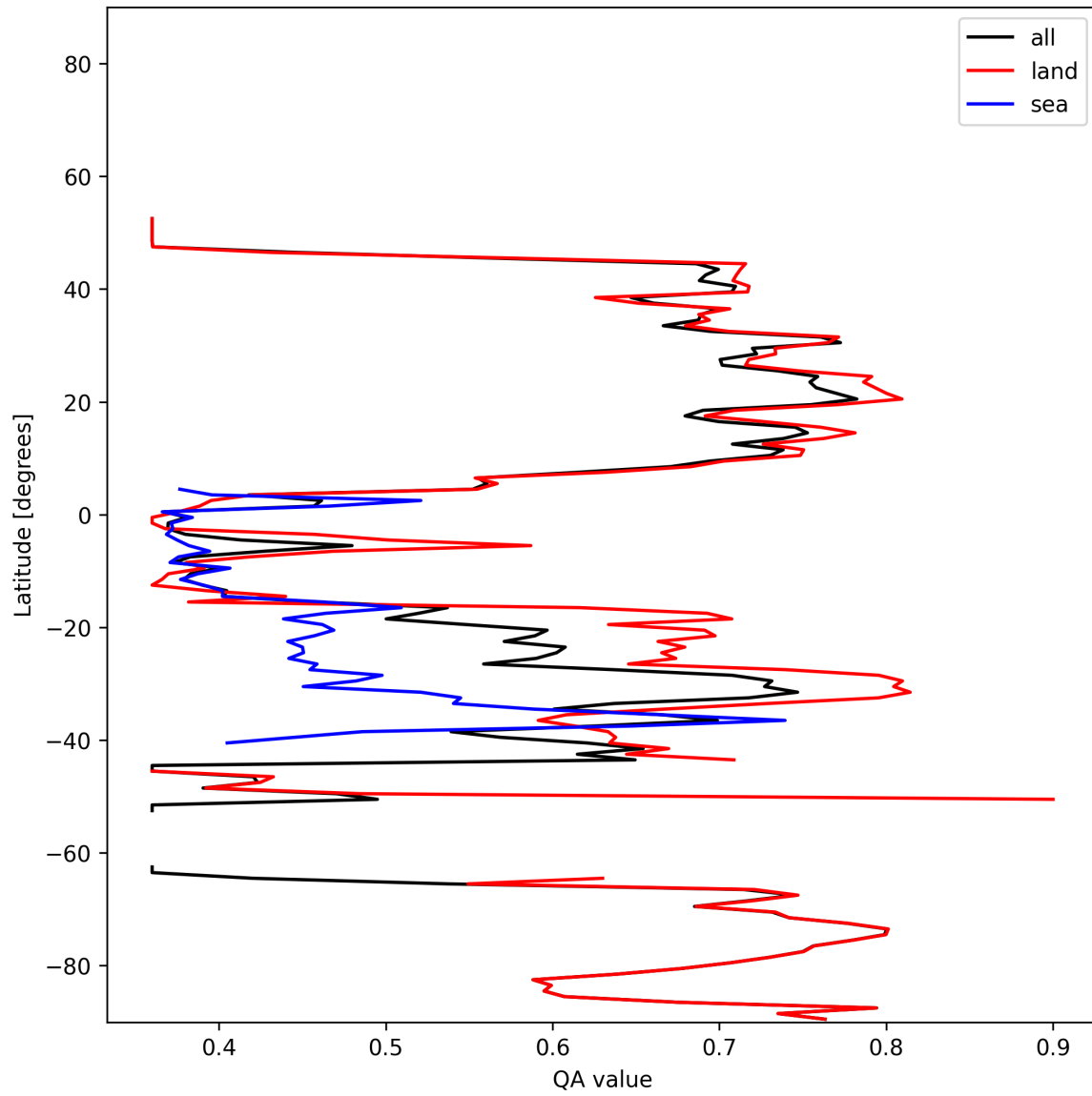
Figure 10: Zonal average of “QA value” for 2025-12-10 to 2025-12-11.
