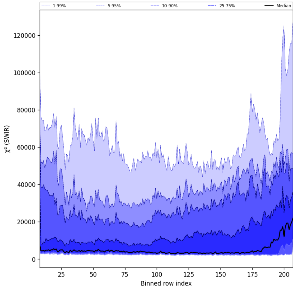
Figure 40: Along track statistics of “ \chi^2 (SWIR)” for 2025-12-10 to 2025-12-11
