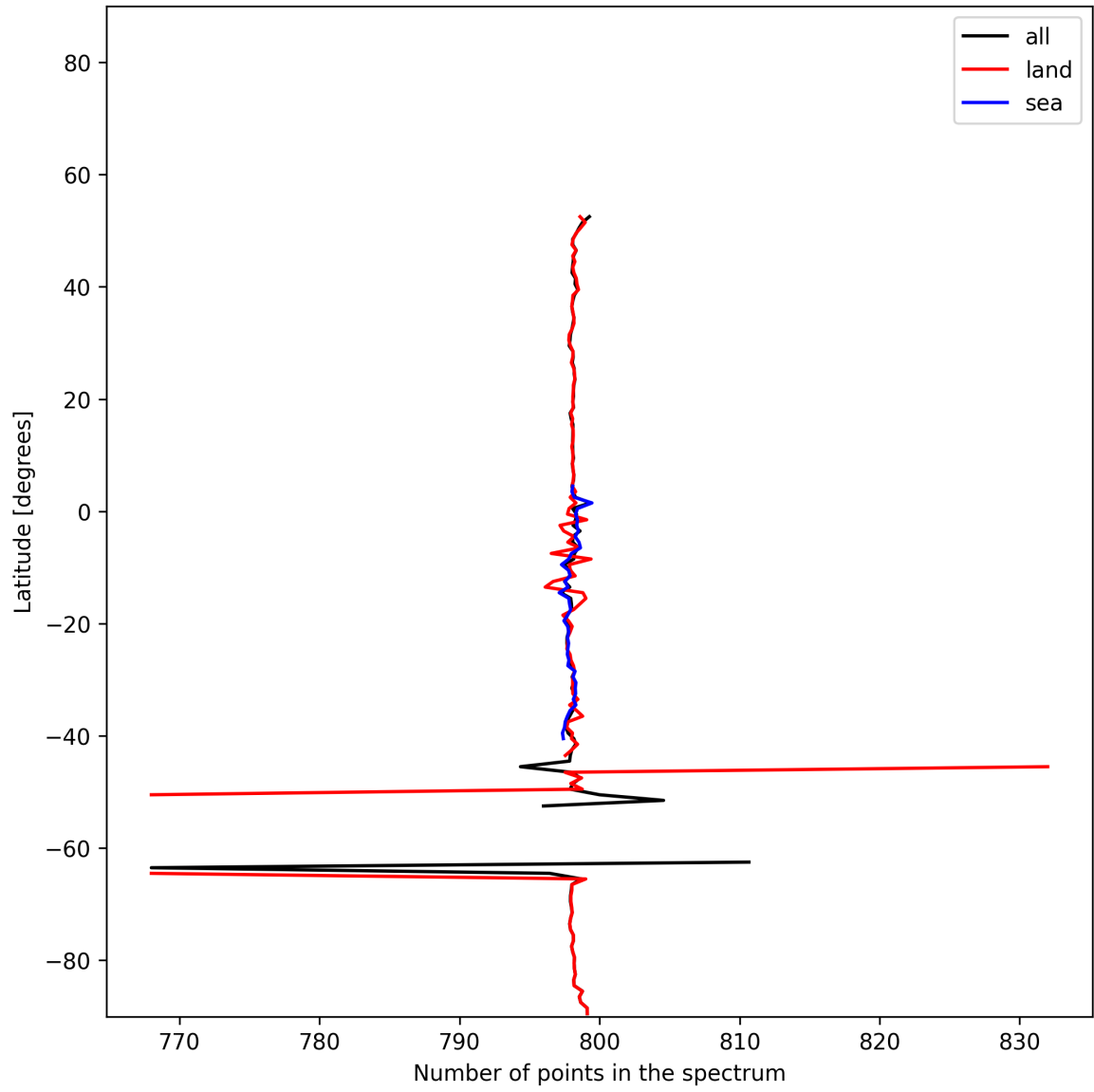
Figure 14: Zonal average of “Number of points in the spectrum” for 2025-12-10 to 2025-12-11.
