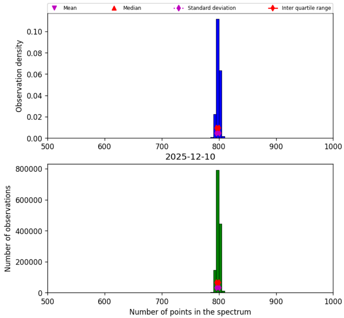
Figure 26: Histogram of “Number of points in the spectrum” for 2025-12-10 to 2025-12-11
