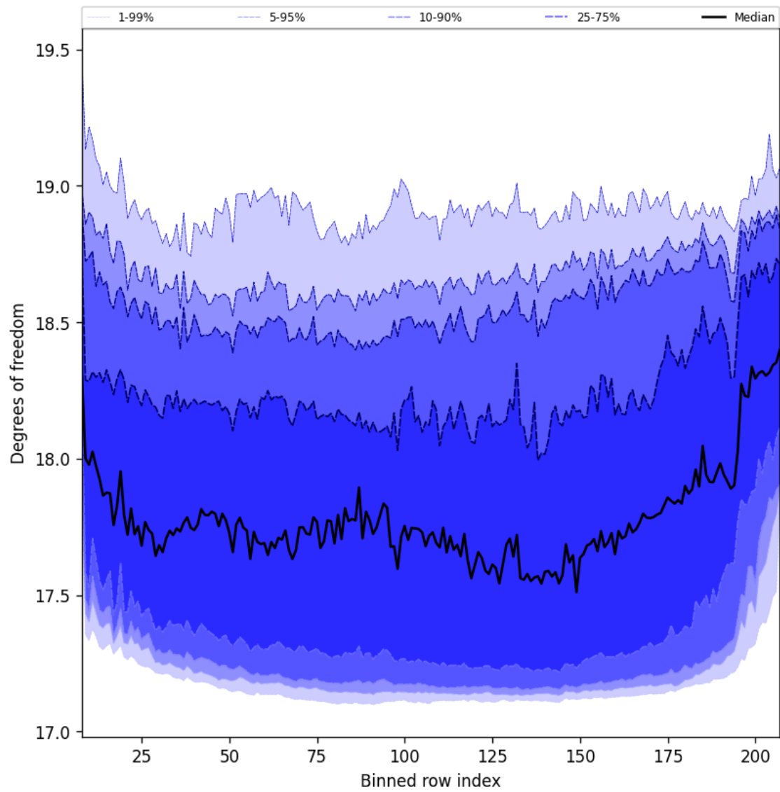
Figure 42: Along track statistics of “Degrees of freedom” for 2025-12-10 to 2025-12-11
