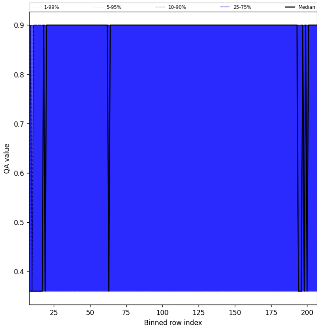
Figure 34: Along track statistics of “QA value” for 2025-12-10 to 2025-12-11
