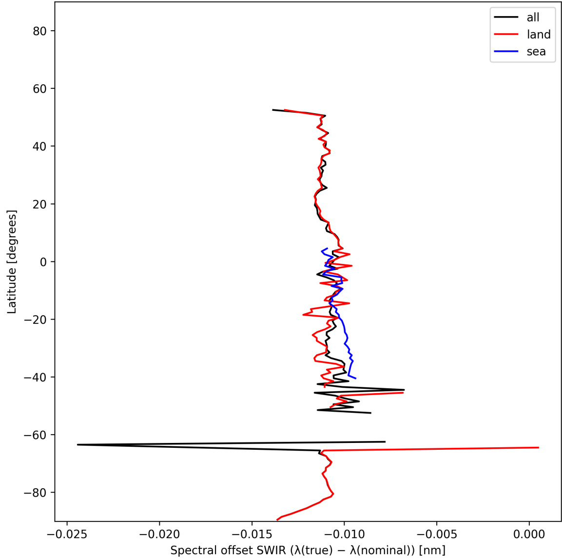
Figure 15: Zonal average of “Spectral offset SWIR ( \lambda_{\text{true}} - \lambda_{\text{nominal}} )” for 2025-12-10 to 2025-12-11.
