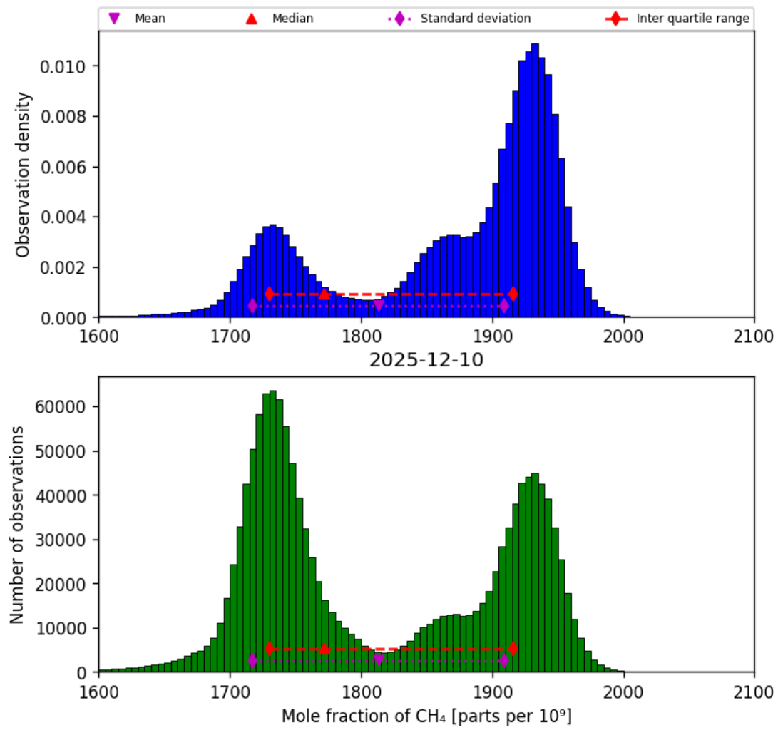
Figure 23: Histogram of “Mole fraction of CH 4 ” for 2025-12-10 to 2025-12-11
