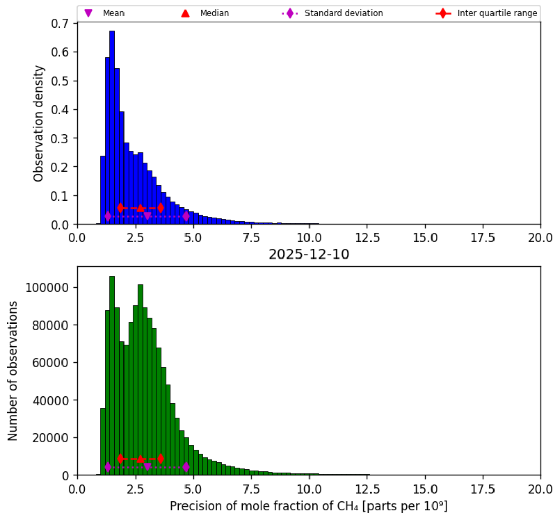
Figure 24: Histogram of “Precision of mole fraction of CH 4 ” for 2025-12-10 to 2025-12-11
