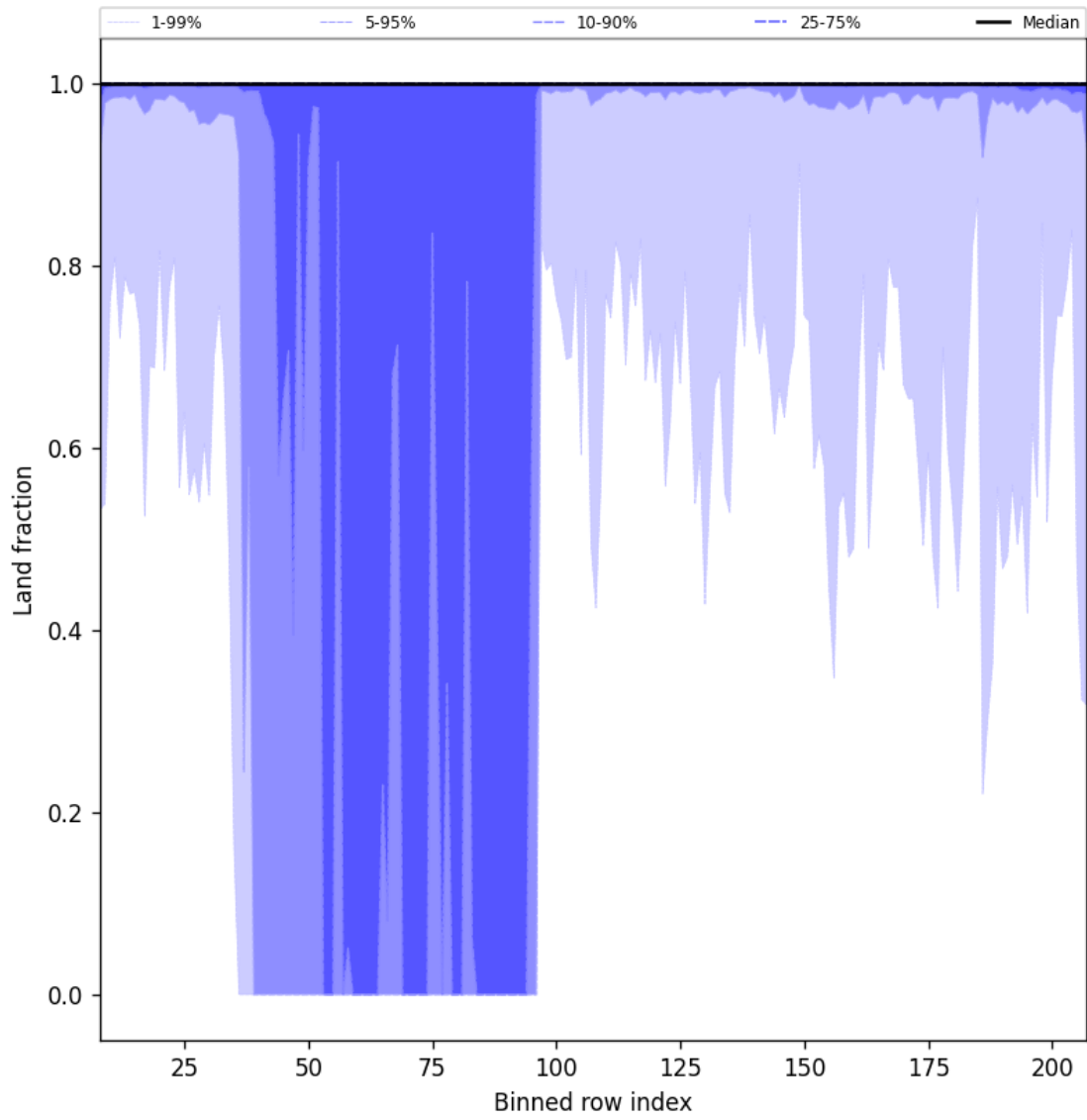
Figure 45: Along track statistics of “Land fraction” for 2025-12-10 to 2025-12-11
