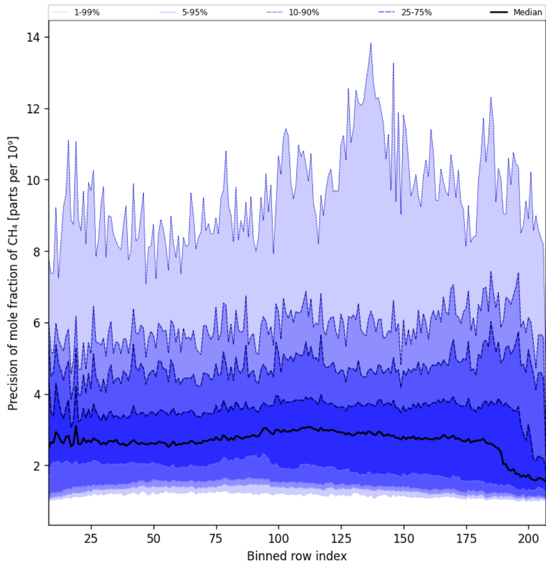
Figure 36: Along track statistics of “Precision of mole fraction of CH 4 ” for 2025-12-10 to 2025-12-11
