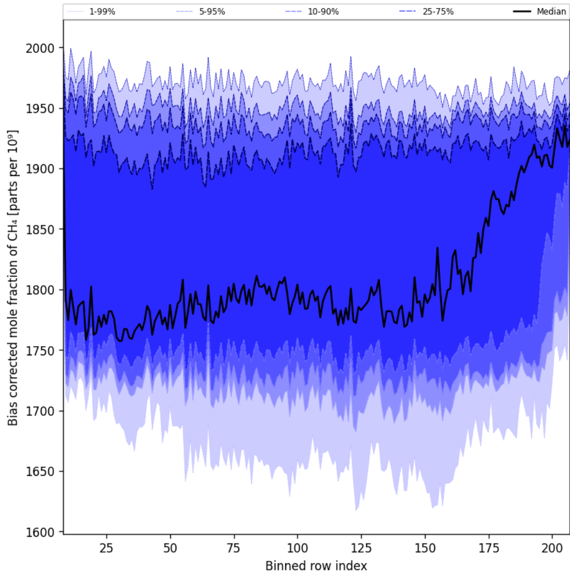
Figure 37: Along track statistics of “Bias corrected mole fraction of CH 4 ” for 2025-12-10 to 2025-12-11
