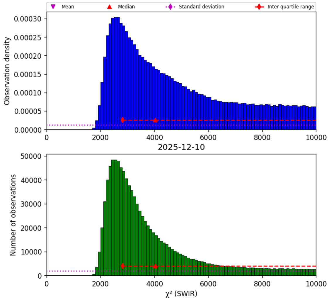
Figure 28: Histogram of “ \chi^2 (SWIR)” for 2025-12-10 to 2025-12-11
