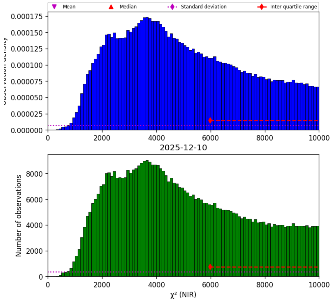
Figure 29: Histogram of “ \chi^2 (NIR)” for 2025-12-10 to 2025-12-11
