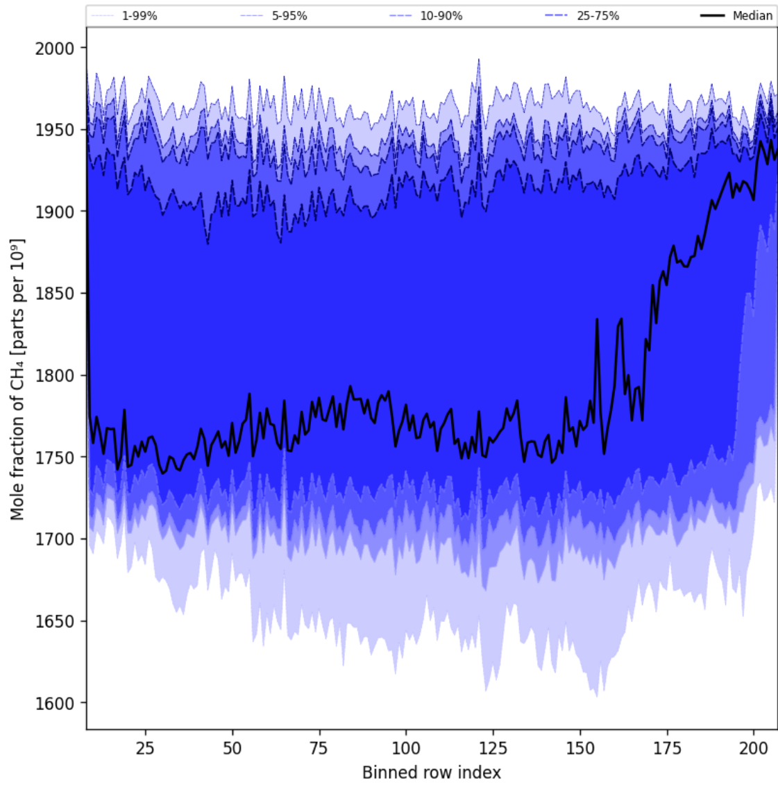
Figure 35: Along track statistics of “Mole fraction of CH 4 ” for 2025-12-10 to 2025-12-11
