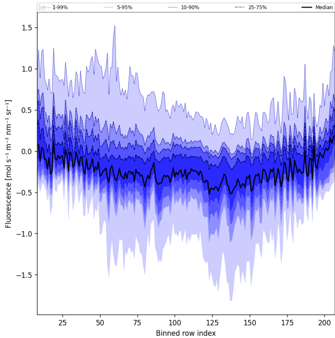
Figure 44: Along track statistics of “Fluorescence” for 2025-12-10 to 2025-12-11
