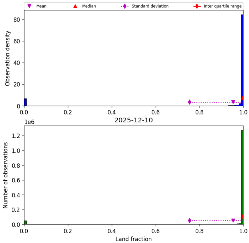
Figure 33: Histogram of “Land fraction” for 2025-12-10 to 2025-12-11
