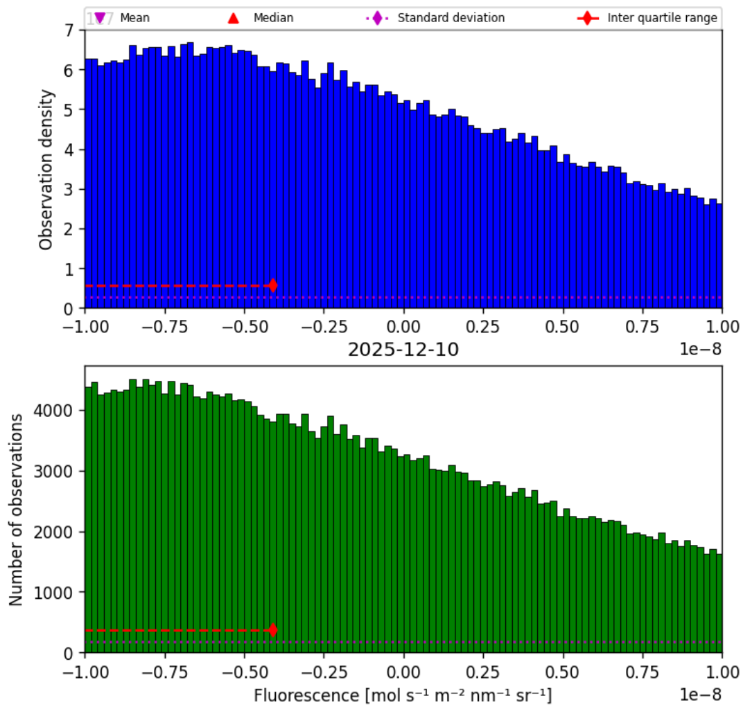
Figure 32: Histogram of “Fluorescence” for 2025-12-10 to 2025-12-11
