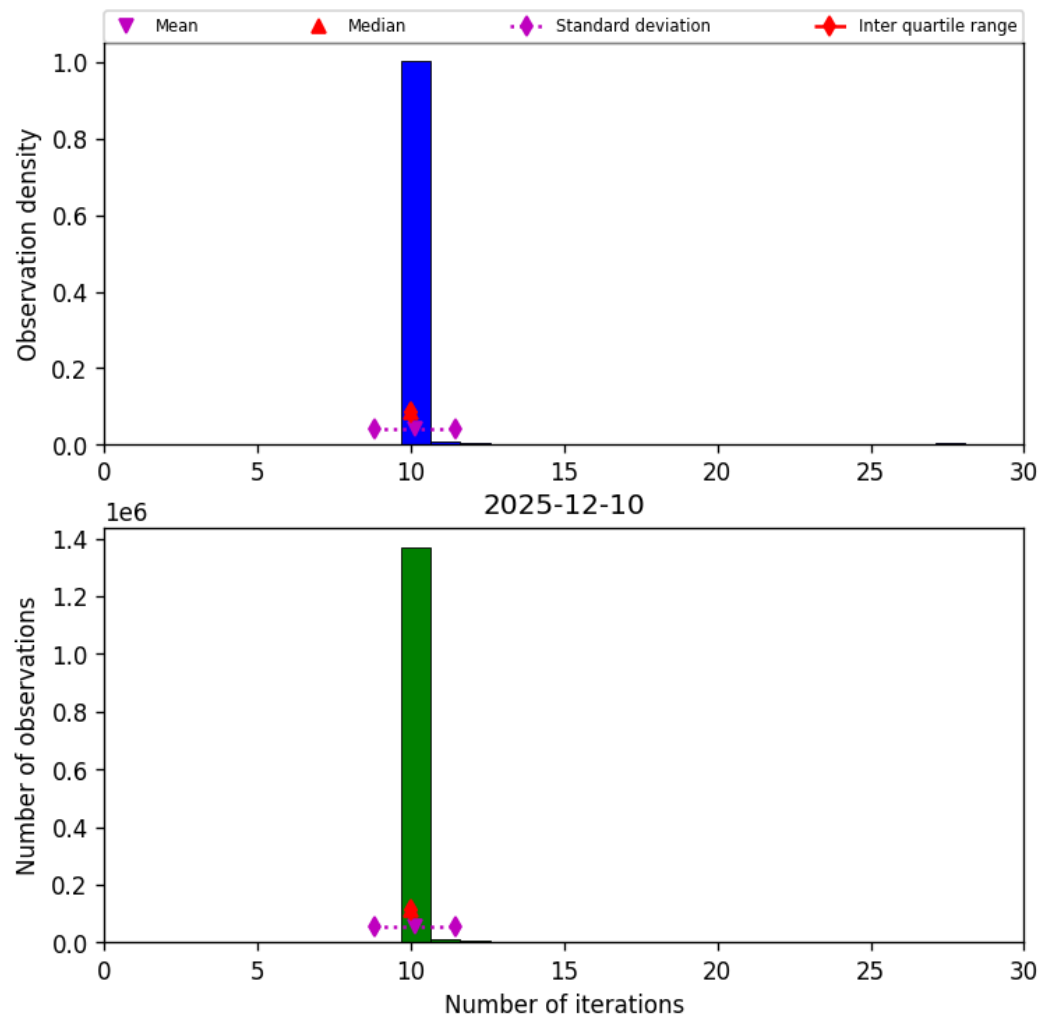
Figure 31: Histogram of “Number of iterations” for 2025-12-10 to 2025-12-11
