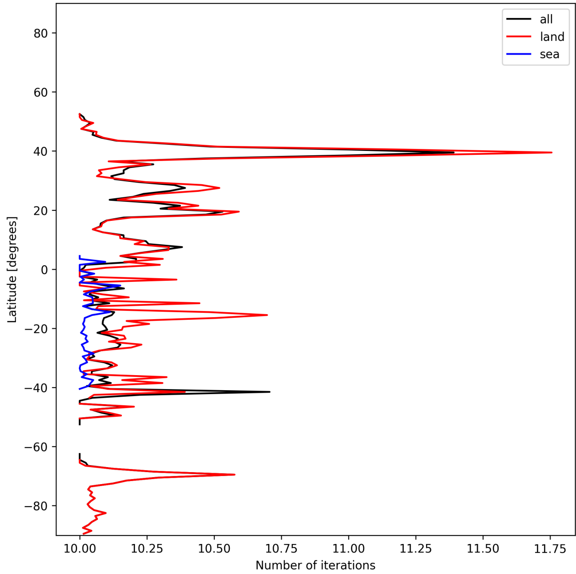
Figure 19: Zonal average of “Number of iterations” for 2025-12-10 to 2025-12-11.
