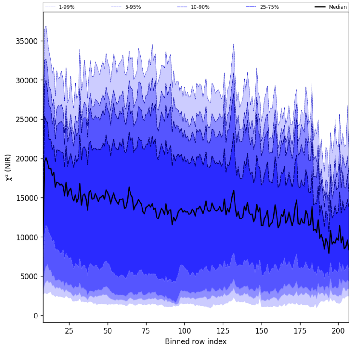
Figure 41: Along track statistics of “ \chi^2 (NIR)” for 2025-12-10 to 2025-12-11
