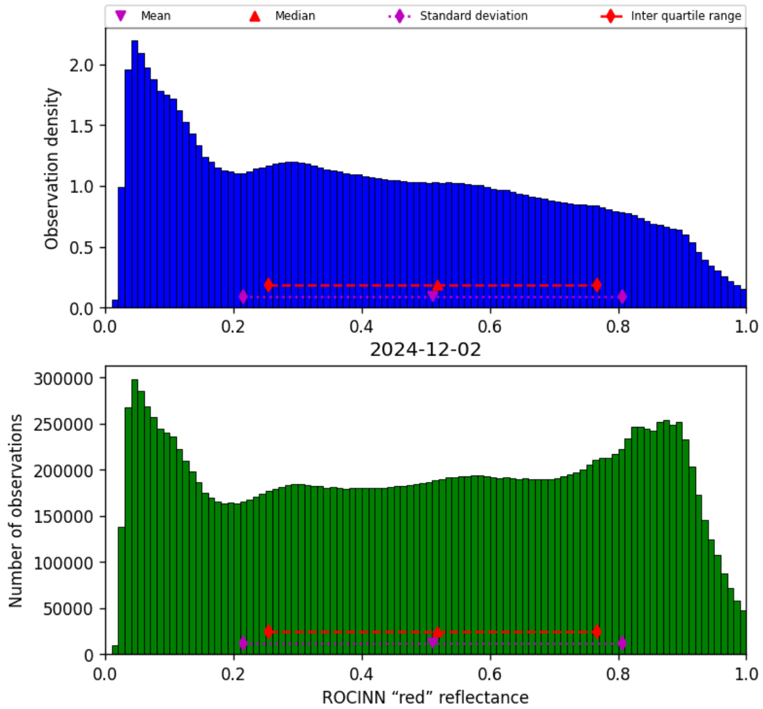
Figure 51: Histogram of “ROCINN “red” reflectance” for 2024-12-02 to 2024-12-03
