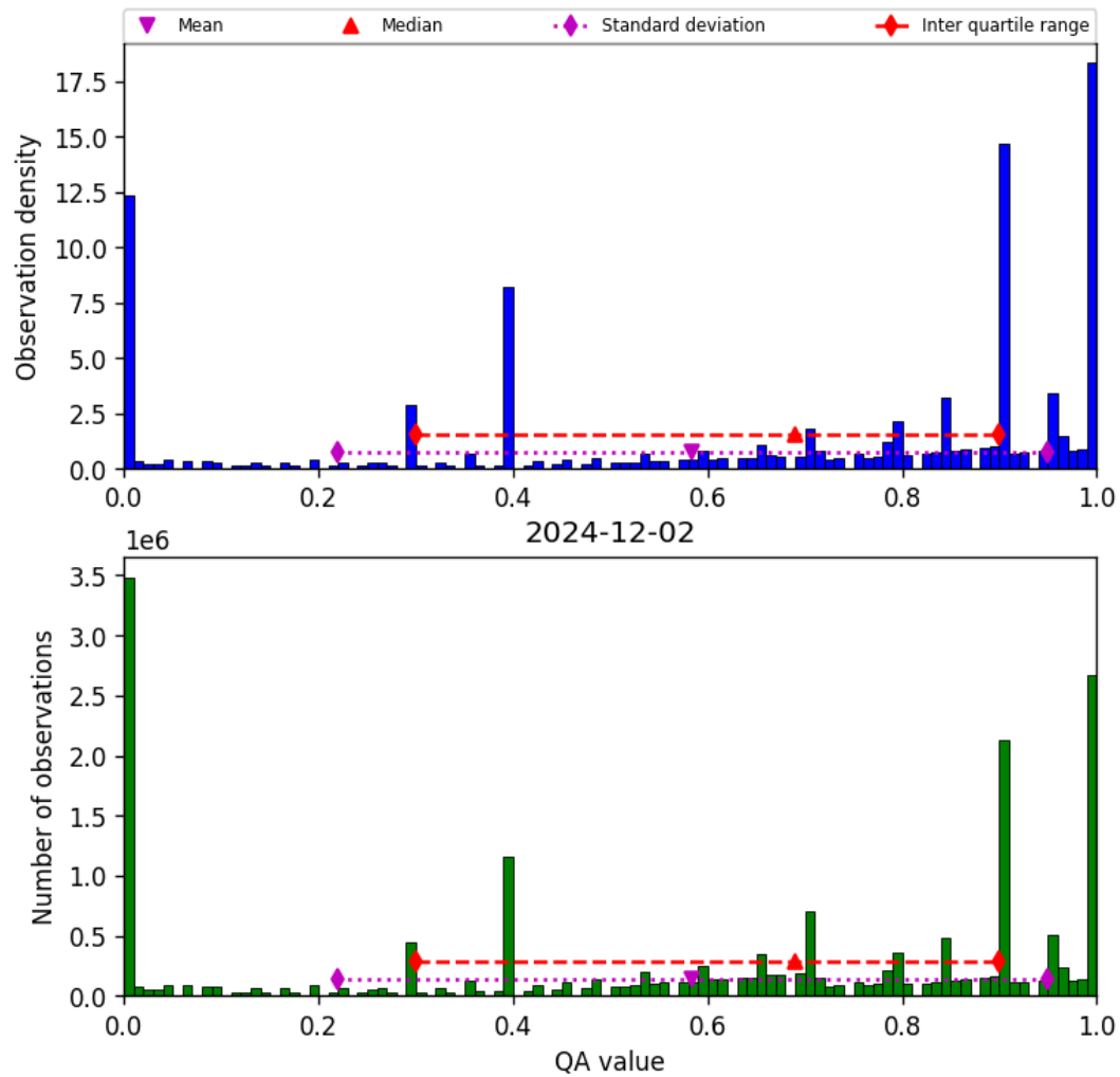
Figure 36: Histogram of “QA value” for 2024-12-02 to 2024-12-03
