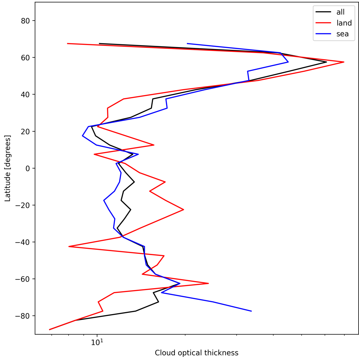
Figure 23: Zonal average of “Cloud optical thickness” for 2024-12-02 to 2024-12-03.
