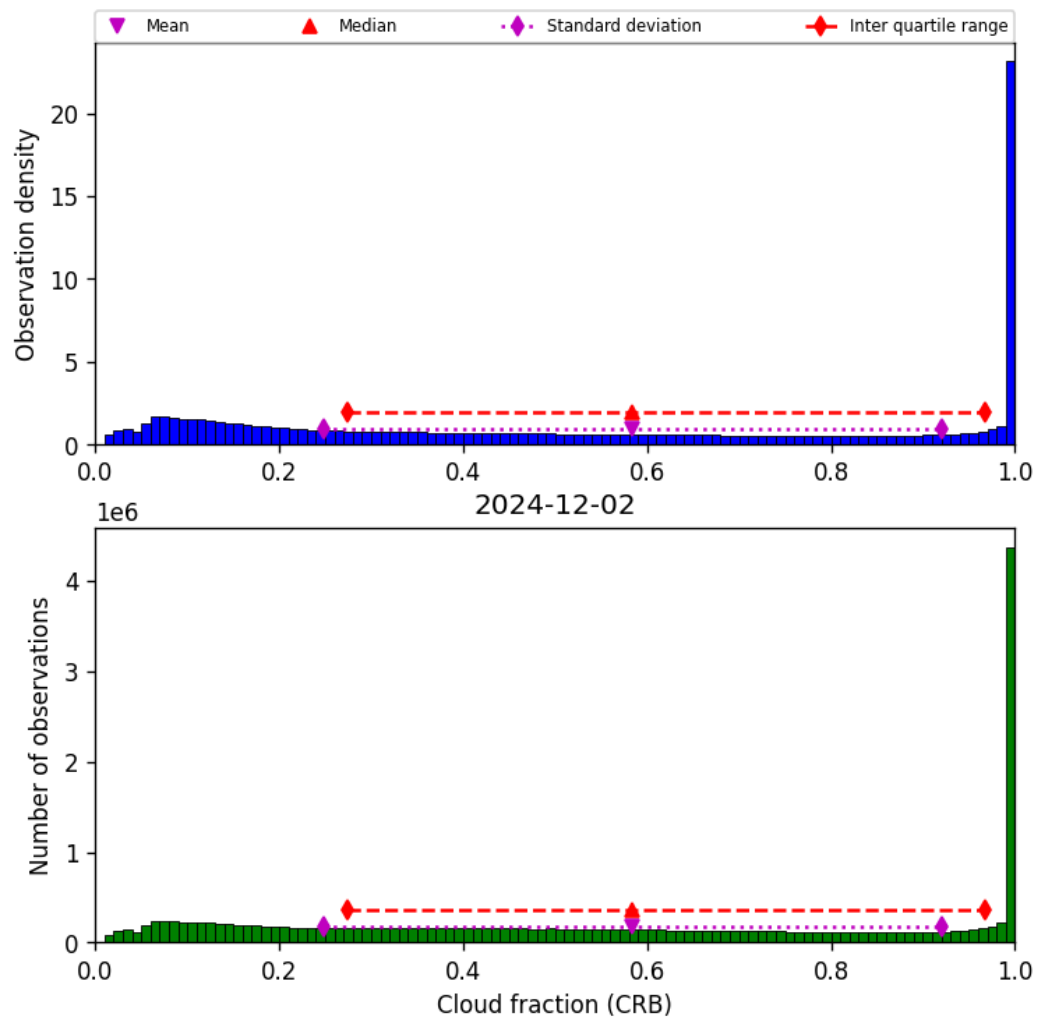
Figure 40: Histogram of “Cloud fraction (CRB)” for 2024-12-02 to 2024-12-03
