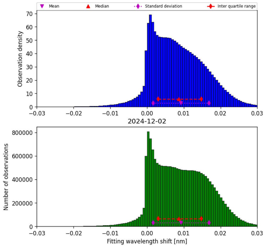
Figure 47: Histogram of “Fitting wavelength shift” for 2024-12-02 to 2024-12-03
