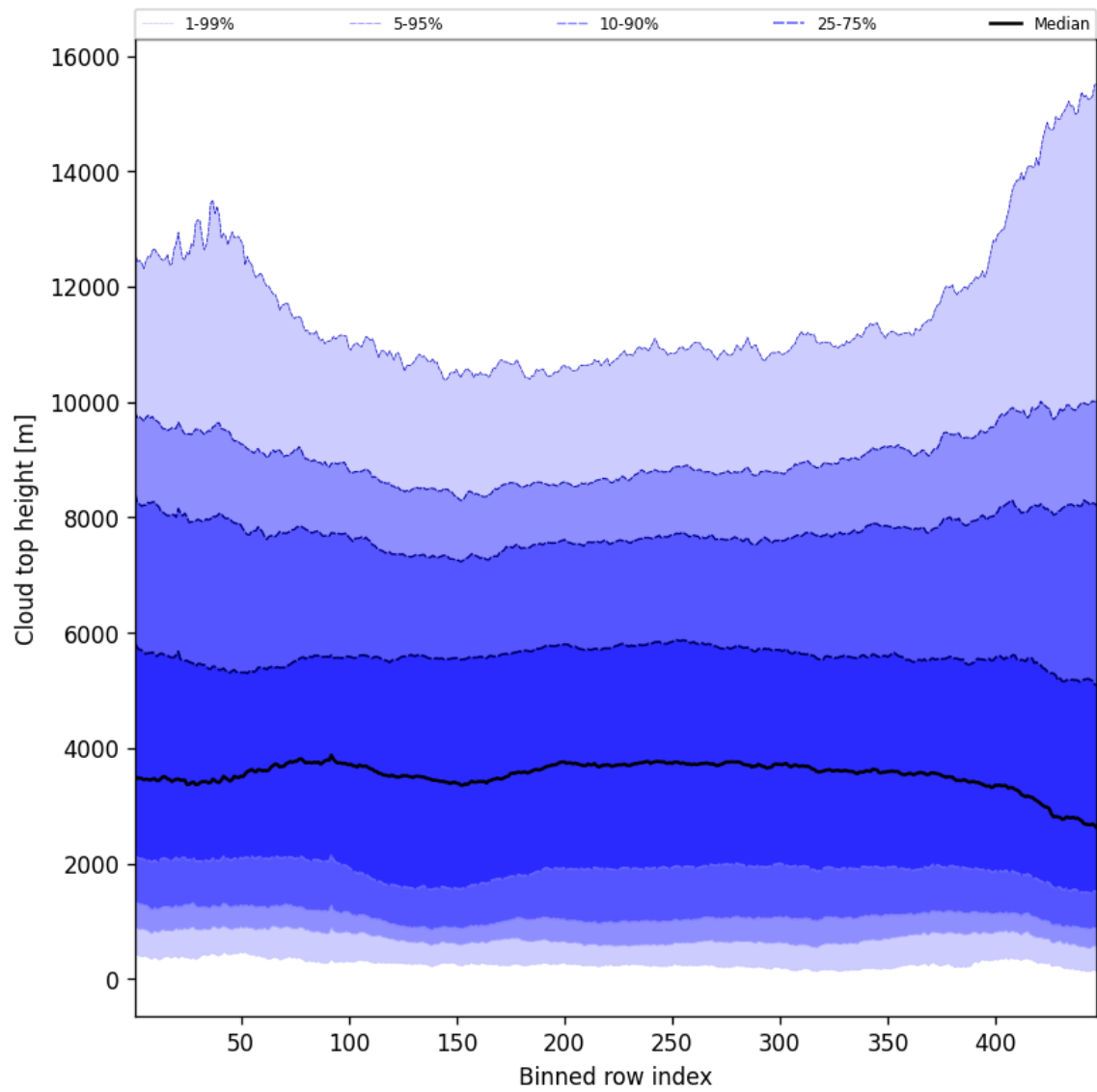
Figure 54: Along track statistics of “Cloud top height” for 2024-12-02 to 2024-12-03
