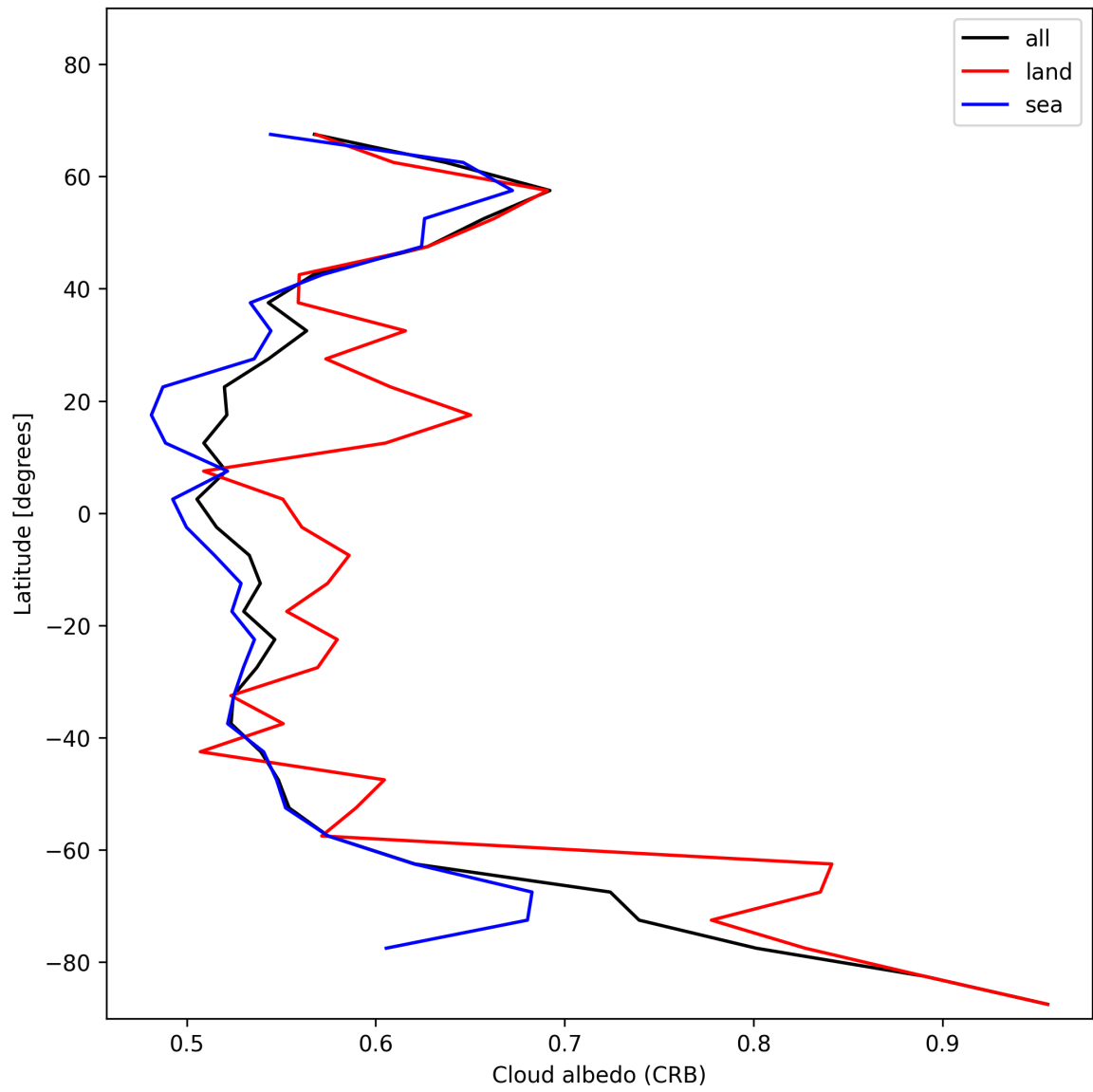
Figure 26: Zonal average of “Cloud albedo (CRB)” for 2024-12-02 to 2024-12-03.
