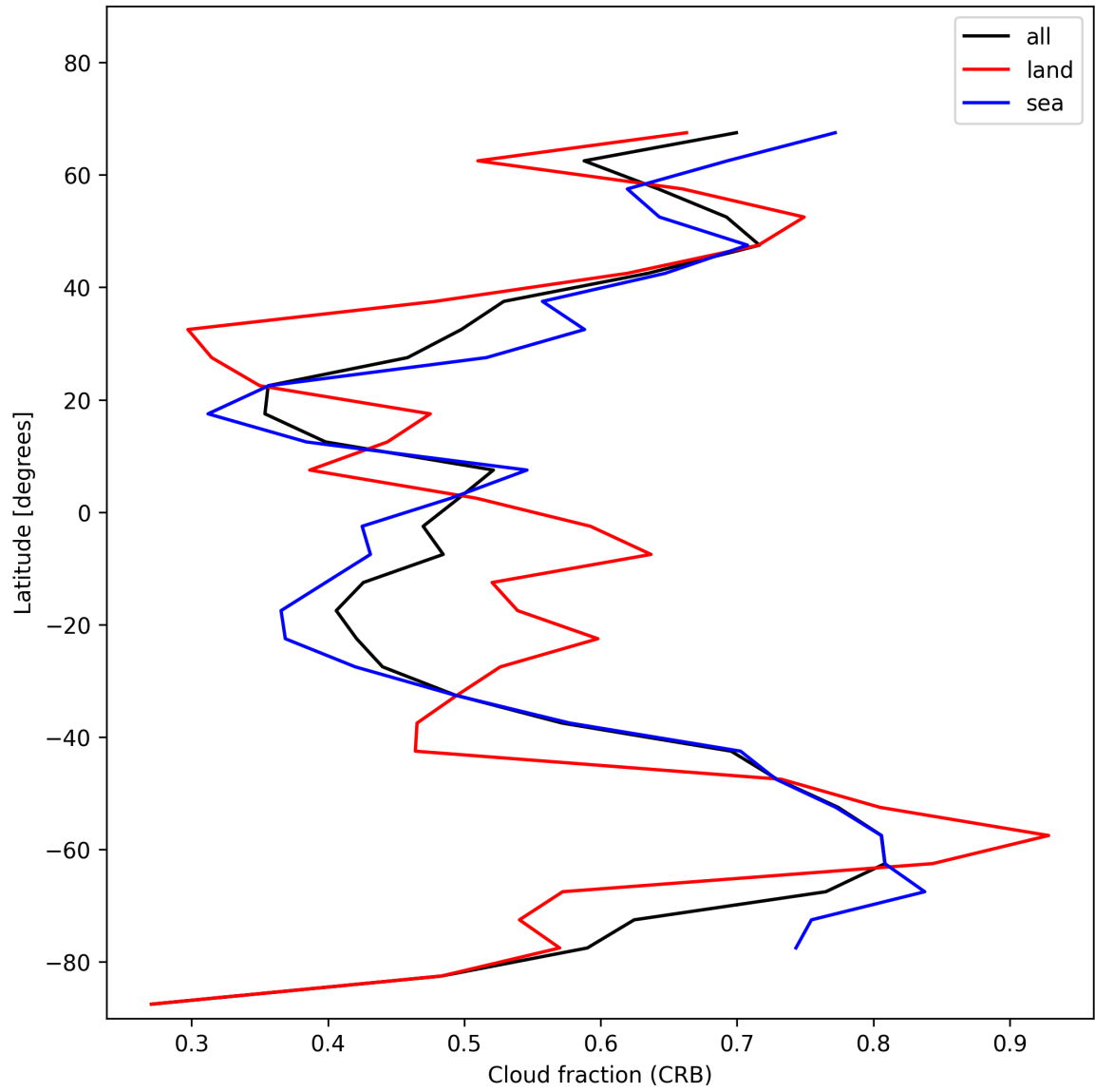
Figure 24: Zonal average of “Cloud fraction (CRB)” for 2024-12-02 to 2024-12-03.
