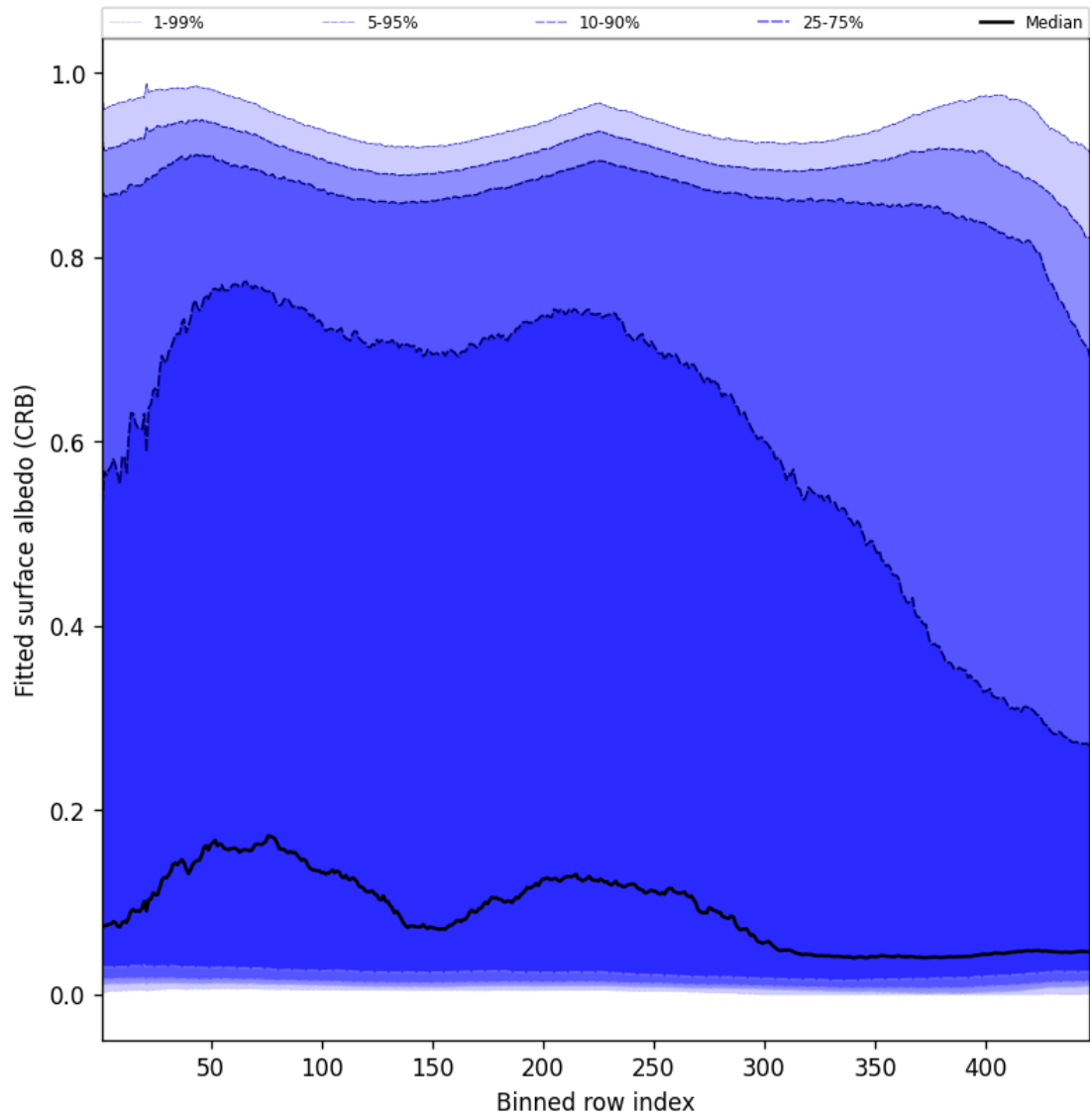
Figure 60: Along track statistics of “Fitted surface albedo (CRB)” for 2024-12-02 to 2024-12-03
