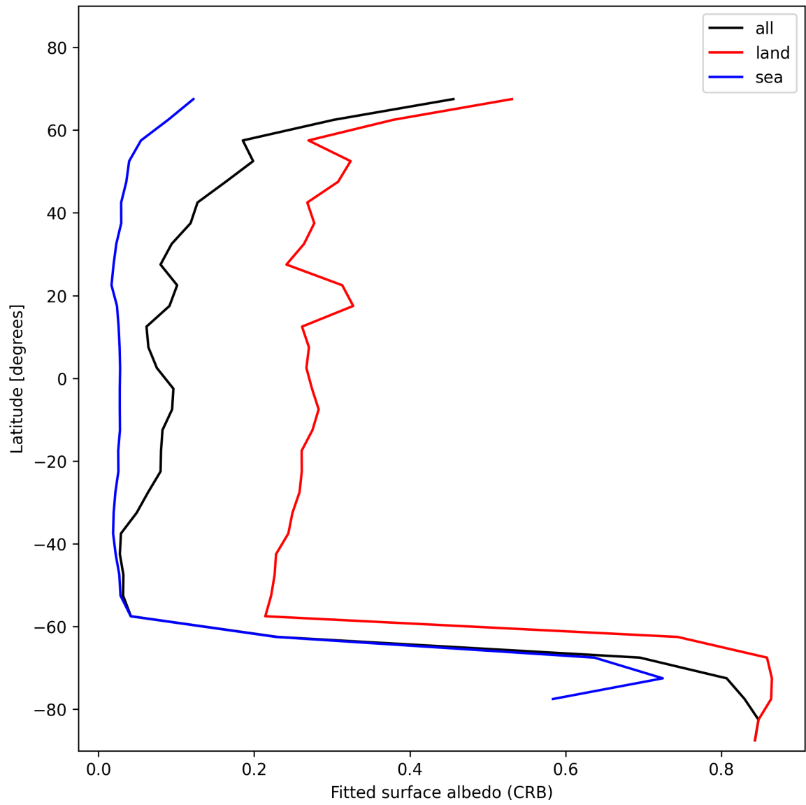
Figure 28: Zonal average of “Fitted surface albedo (CRB)” for 2024-12-02 to 2024-12-03.
