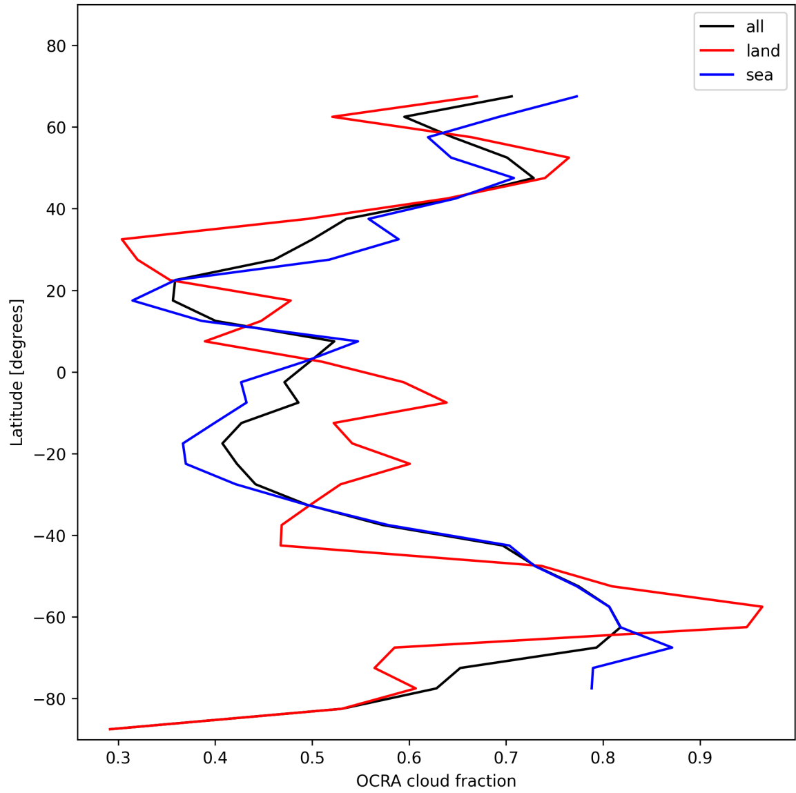
Figure 32: Zonal average of “OCRA cloud fraction” for 2024-12-02 to 2024-12-03.
