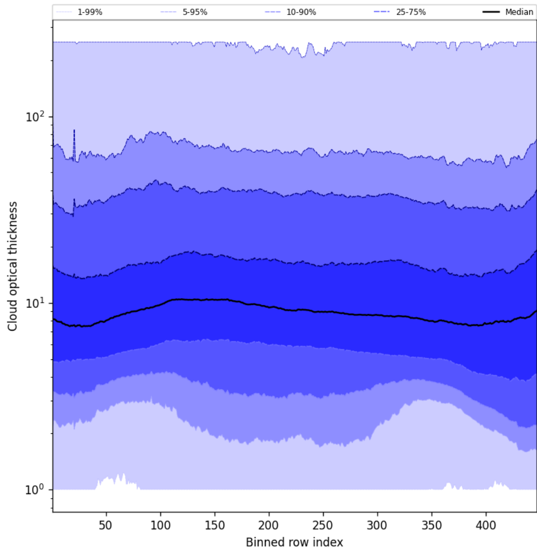
Figure 55: Along track statistics of “Cloud optical thickness” for 2024-12-02 to 2024-12-03
