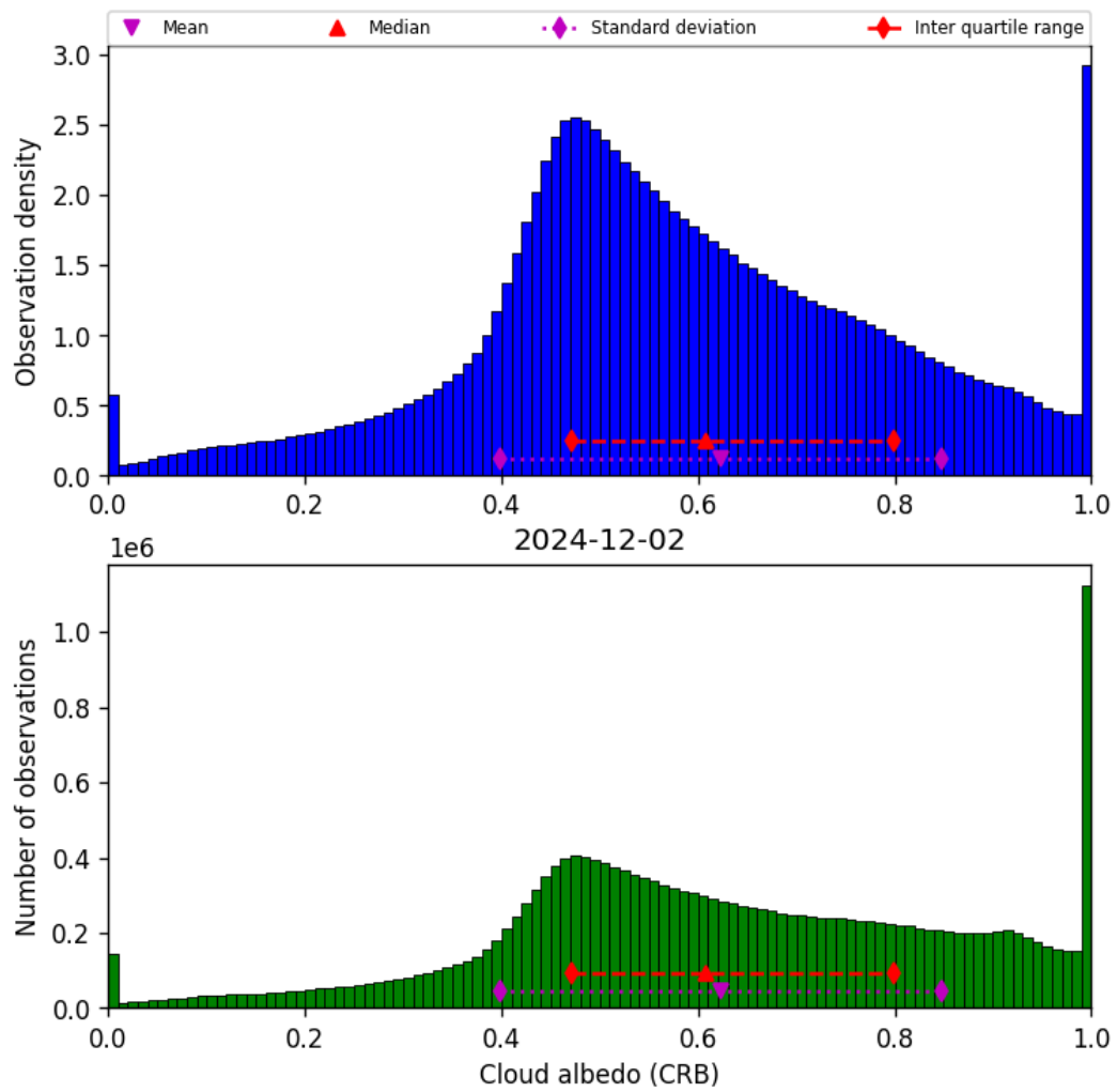
Figure 42: Histogram of “Cloud albedo (CRB)” for 2024-12-02 to 2024-12-03
