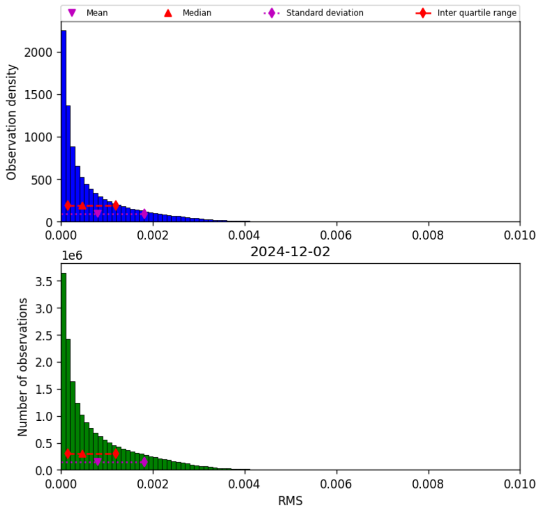
Figure 45: Histogram of “RMS” for 2024-12-02 to 2024-12-03
