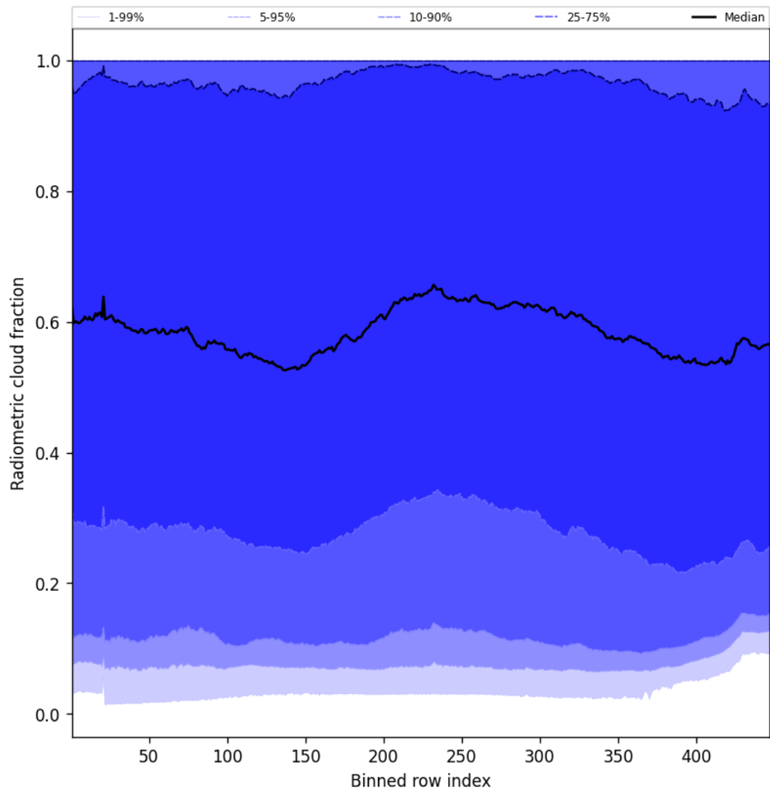
Figure 53: Along track statistics of “Radiometric cloud fraction” for 2024-12-02 to 2024-12-03
