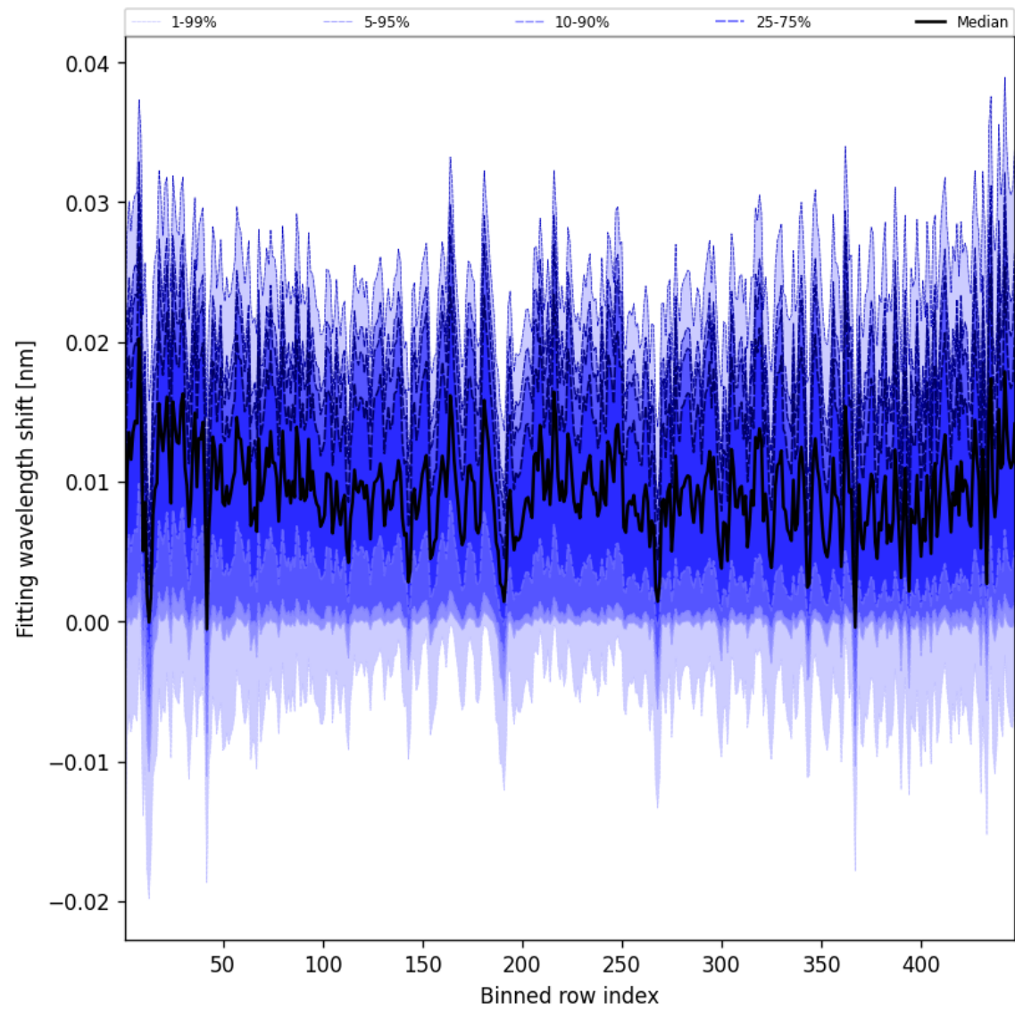
Figure 63: Along track statistics of “Fitting wavelength shift” for 2024-12-02 to 2024-12-03
