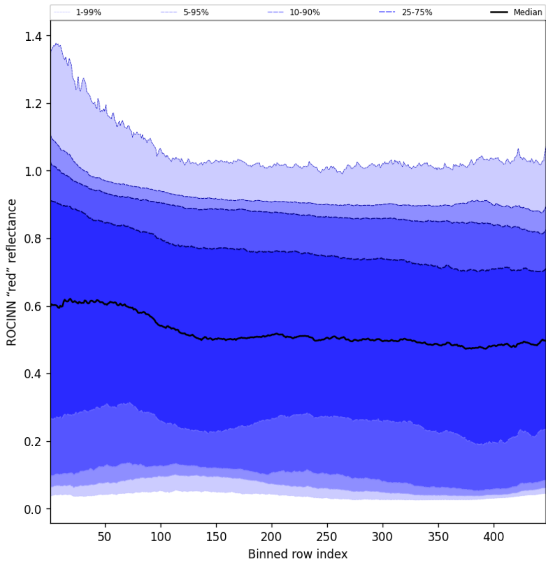
Figure 67: Along track statistics of "ROCINN "red" reflectance" for 2024-12-02 to 2024-12-03
