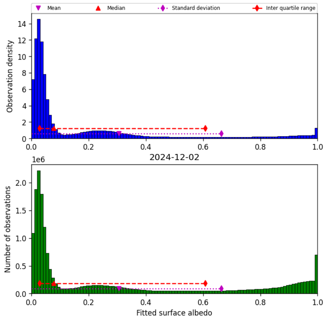
Figure 43: Histogram of “Fitted surface albedo” for 2024-12-02 to 2024-12-03
