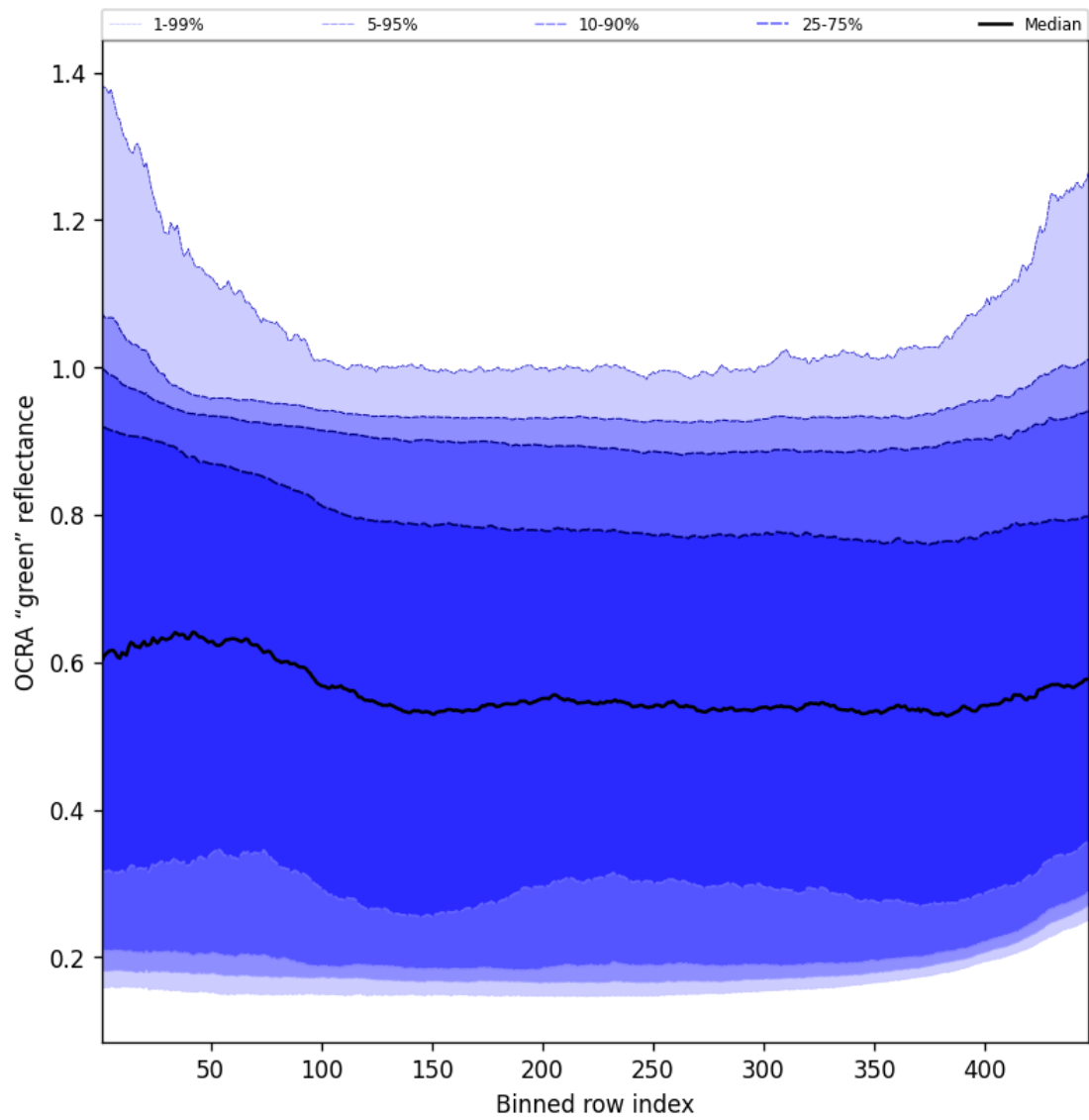
Figure 66: Along track statistics of “OCRA “green” reflectance” for 2024-12-02 to 2024-12-03
