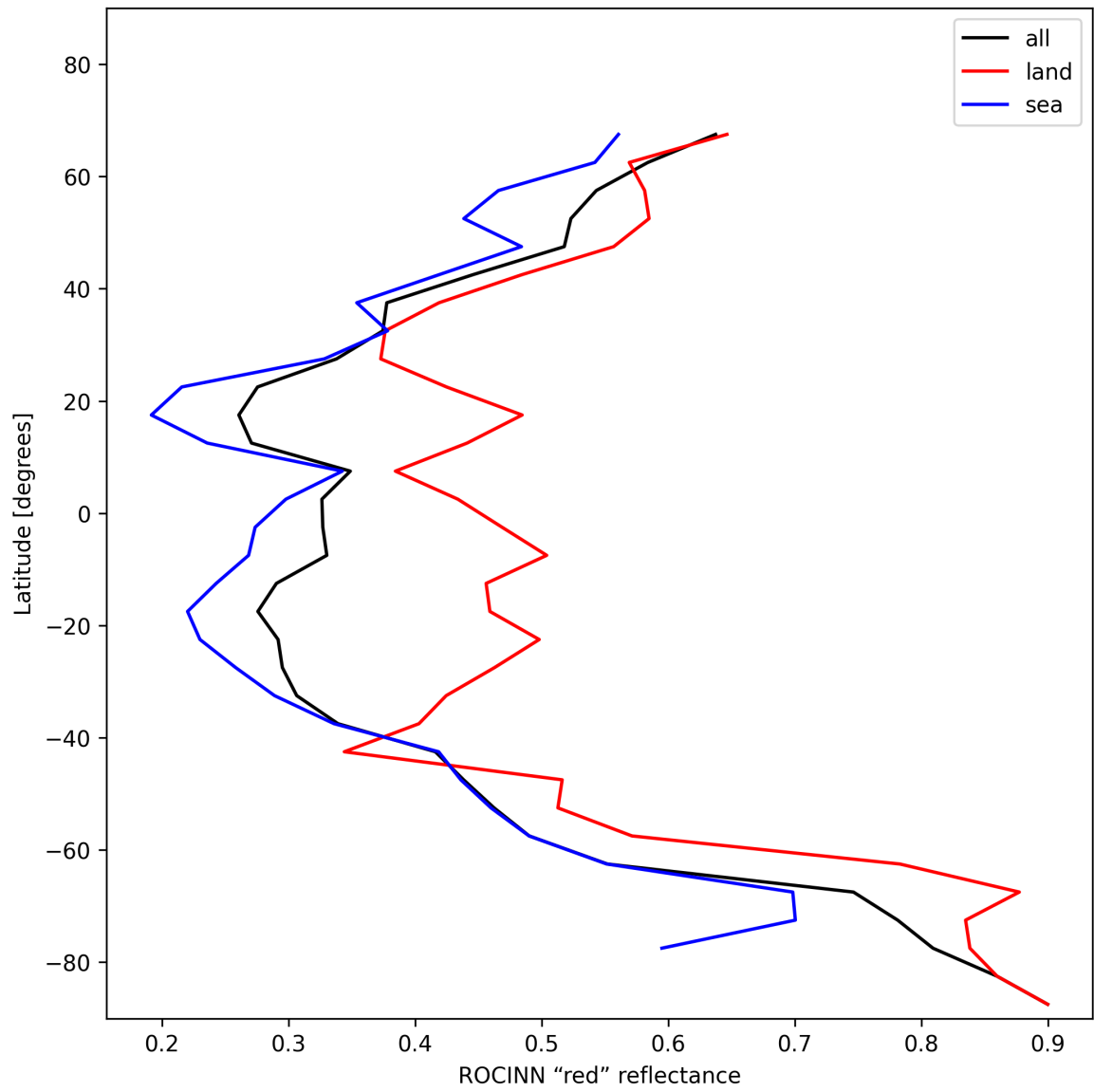
Figure 35: Zonal average of “ROCINN “red” reflectance” for 2024-12-02 to 2024-12-03.
