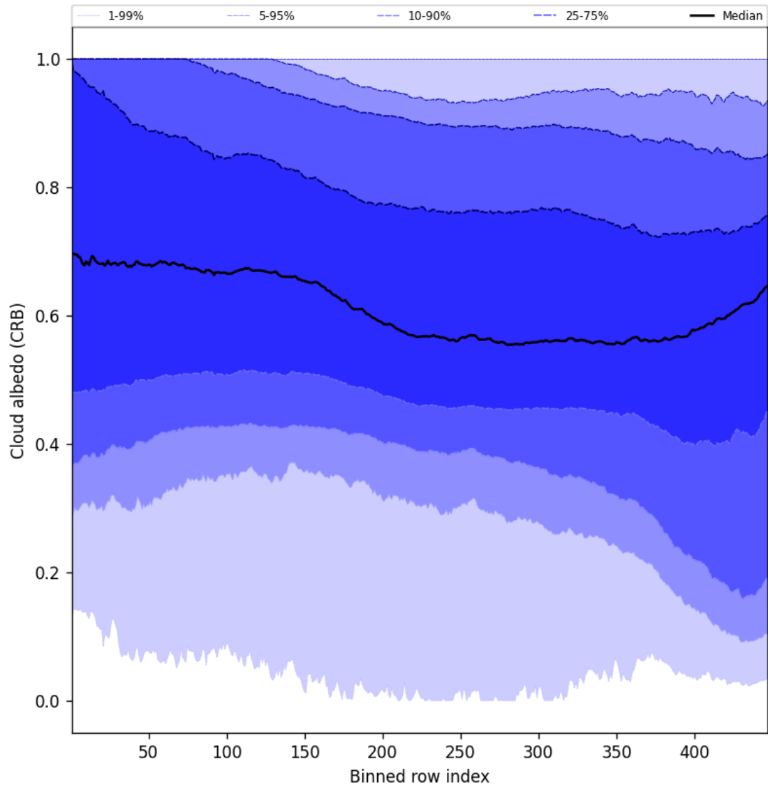
Figure 58: Along track statistics of “Cloud albedo (CRB)” for 2024-12-02 to 2024-12-03
