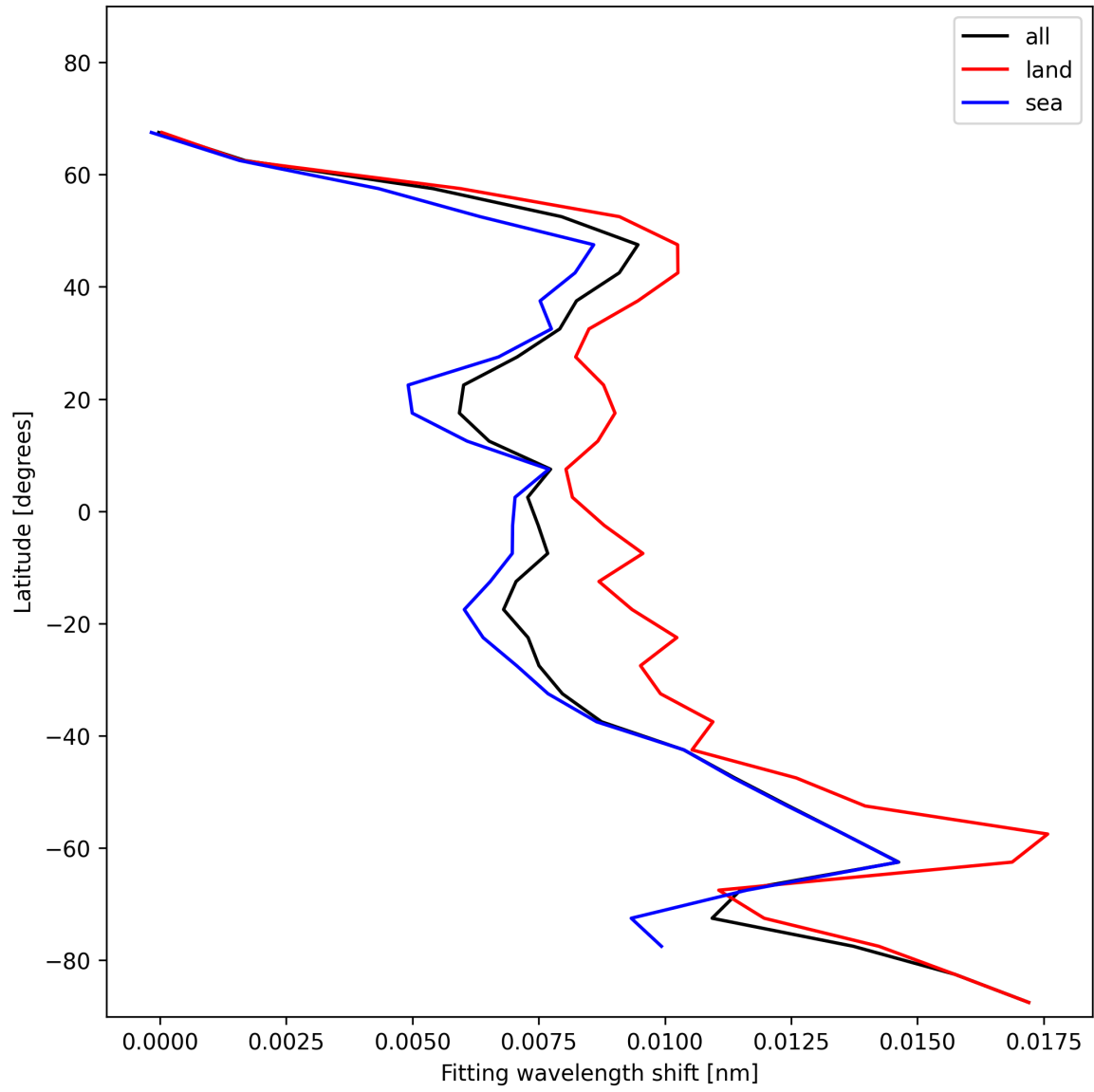
Figure 31: Zonal average of “Fitting wavelength shift” for 2024-12-02 to 2024-12-03.
