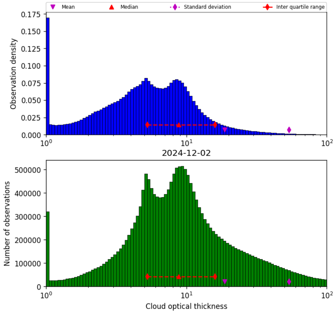
Figure 39: Histogram of “Cloud optical thickness” for 2024-12-02 to 2024-12-03
