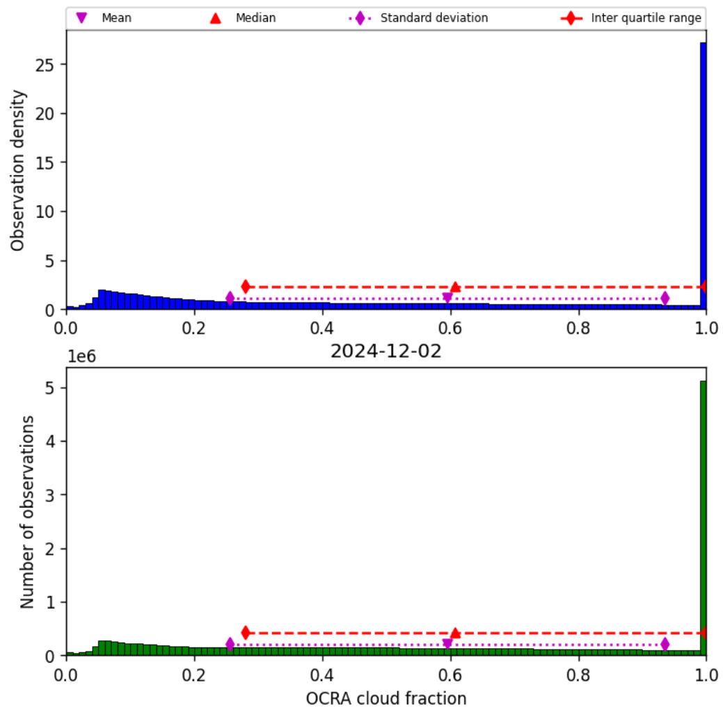
Figure 48: Histogram of “OCRA cloud fraction” for 2024-12-02 to 2024-12-03
