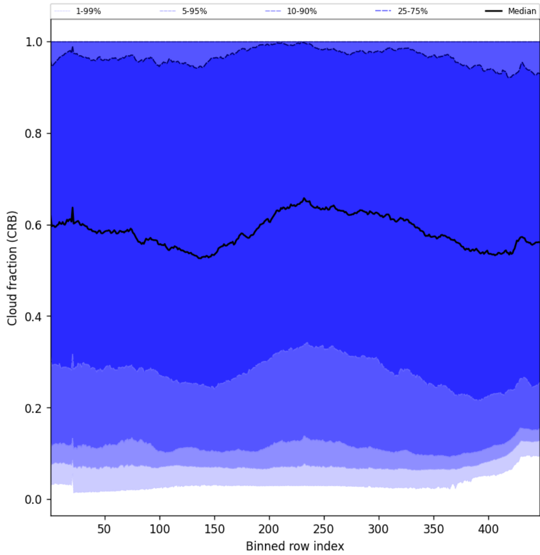
Figure 56: Along track statistics of “Cloud fraction (CRB)” for 2024-12-02 to 2024-12-03
