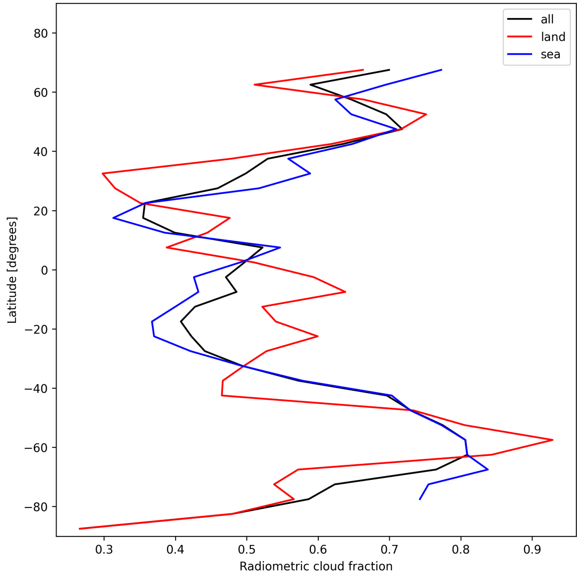
Figure 21: Zonal average of “Radiometric cloud fraction” for 2024-12-02 to 2024-12-03.
