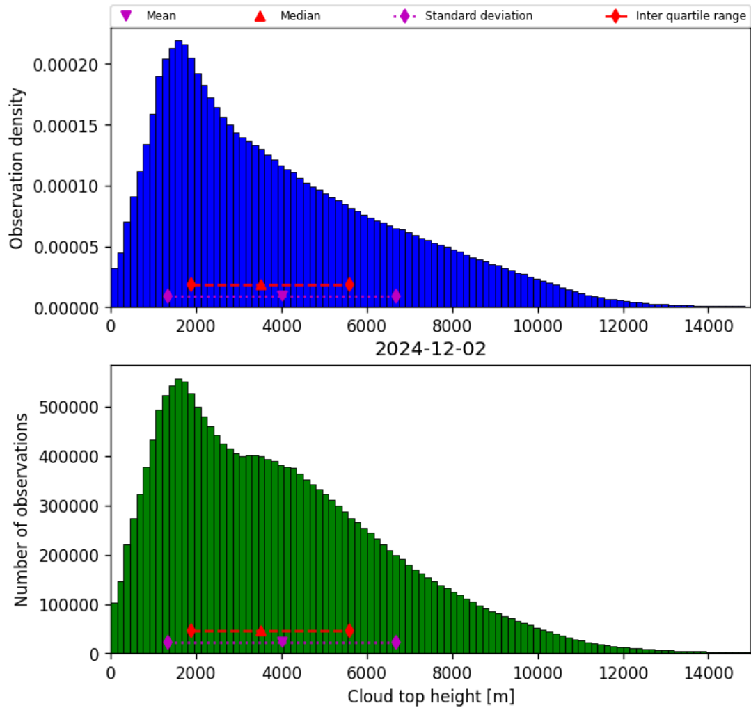
Figure 38: Histogram of “Cloud top height” for 2024-12-02 to 2024-12-03
