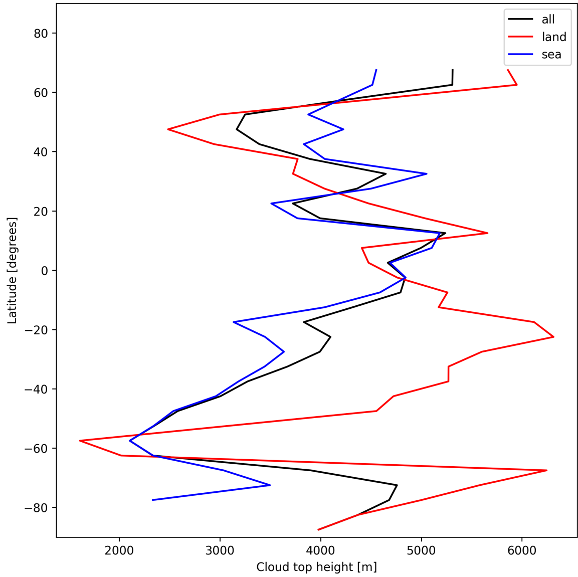
Figure 22: Zonal average of “Cloud top height” for 2024-12-02 to 2024-12-03.
