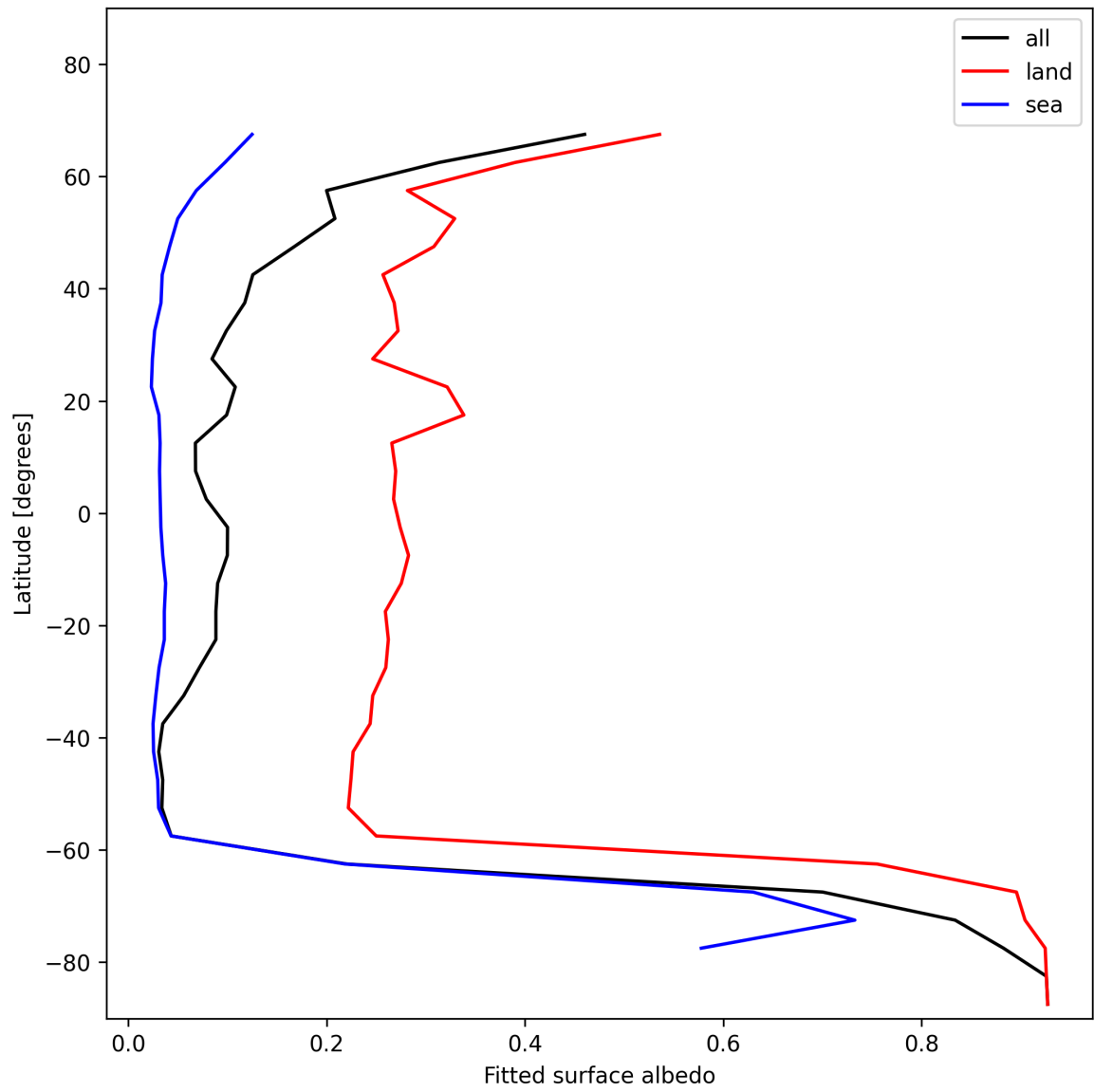
Figure 27: Zonal average of “Fitted surface albedo” for 2024-12-02 to 2024-12-03.
