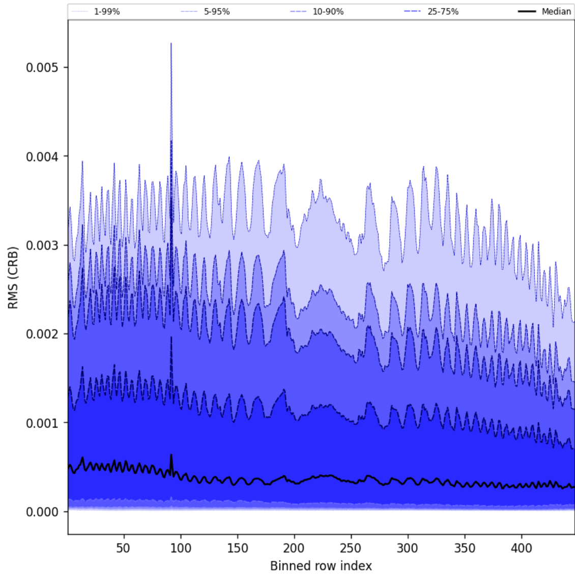
Figure 62: Along track statistics of “RMS (CRB)” for 2024-12-02 to 2024-12-03
