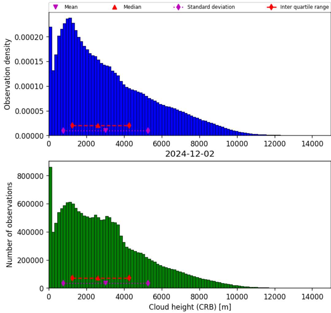
Figure 41: Histogram of “Cloud height (CRB)” for 2024-12-02 to 2024-12-03
