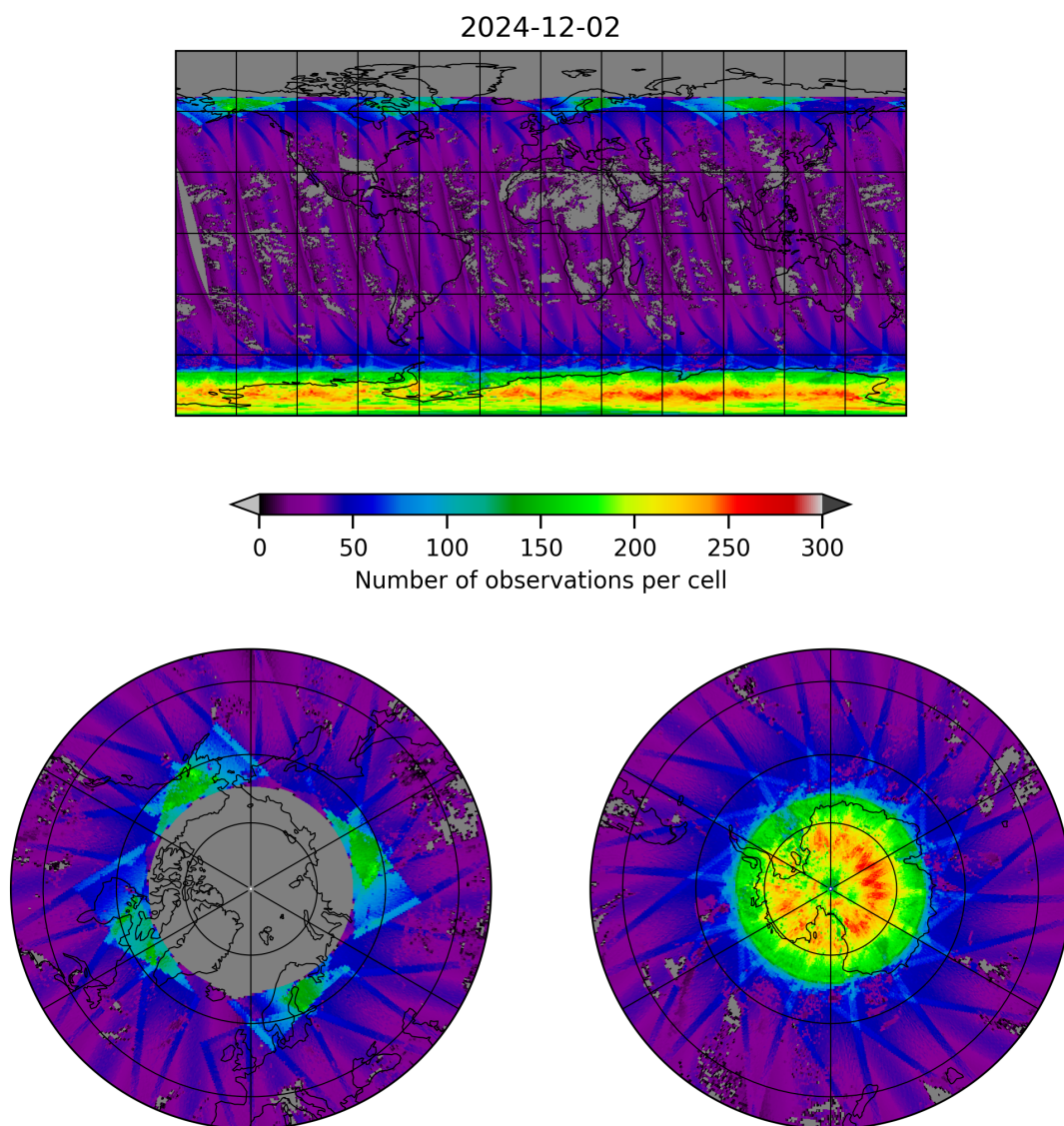
Figure 19: Map of the number of observations for 2024-12-02 to 2024-12-03
