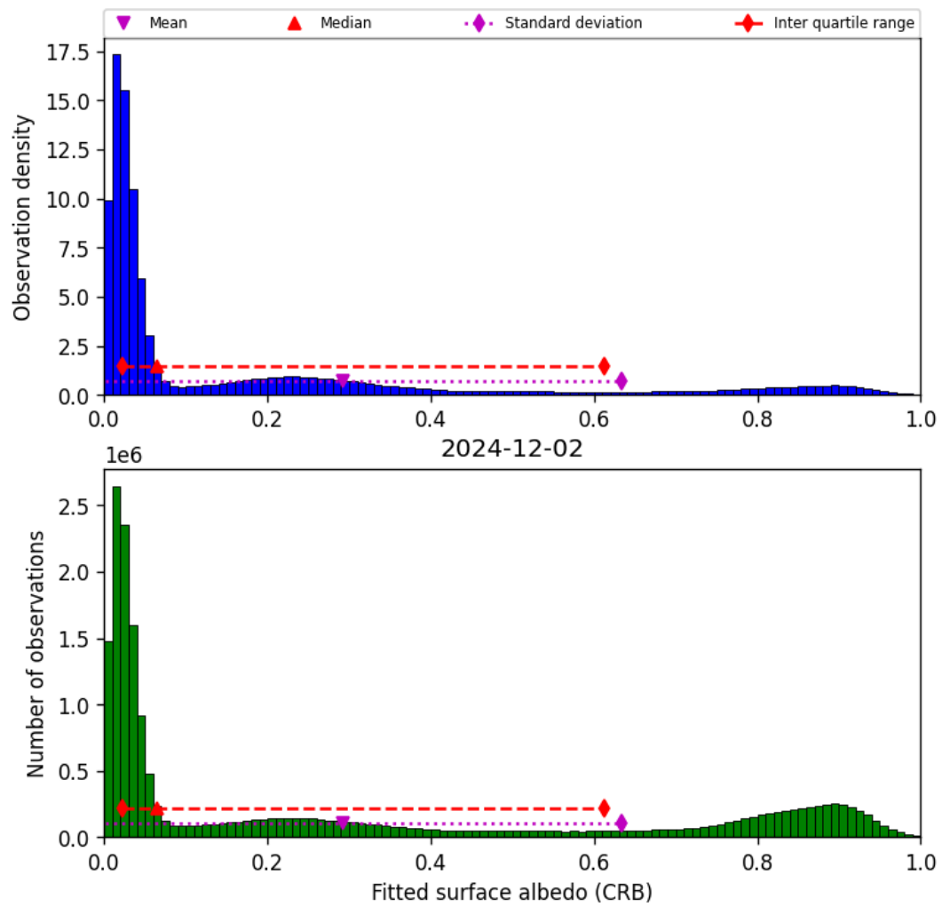
Figure 44: Histogram of “Fitted surface albedo (CRB)” for 2024-12-02 to 2024-12-03
