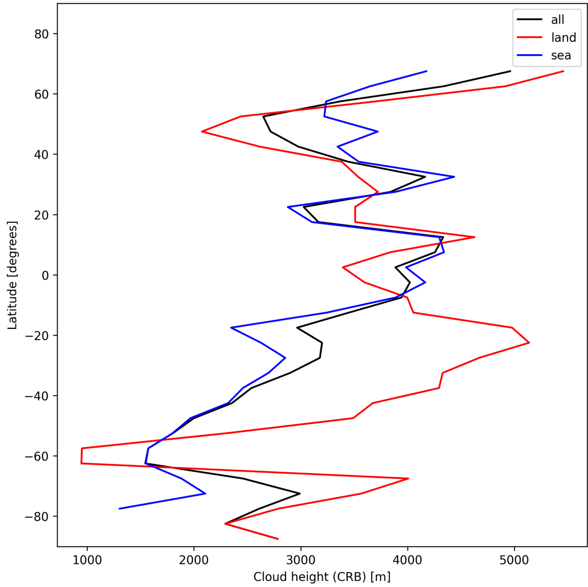
Figure 25: Zonal average of “Cloud height (CRB)” for 2024-12-02 to 2024-12-03.
