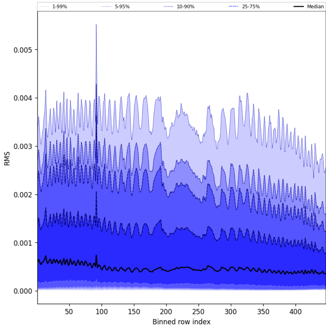
Figure 61: Along track statistics of “RMS” for 2024-12-02 to 2024-12-03
