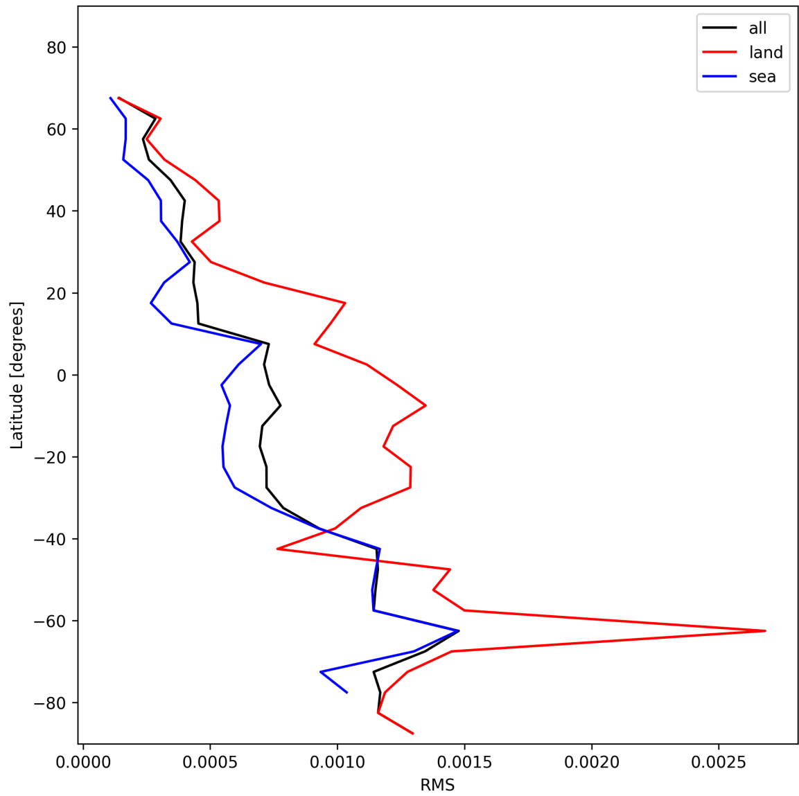
Figure 29: Zonal average of “RMS” for 2024-12-02 to 2024-12-03.
