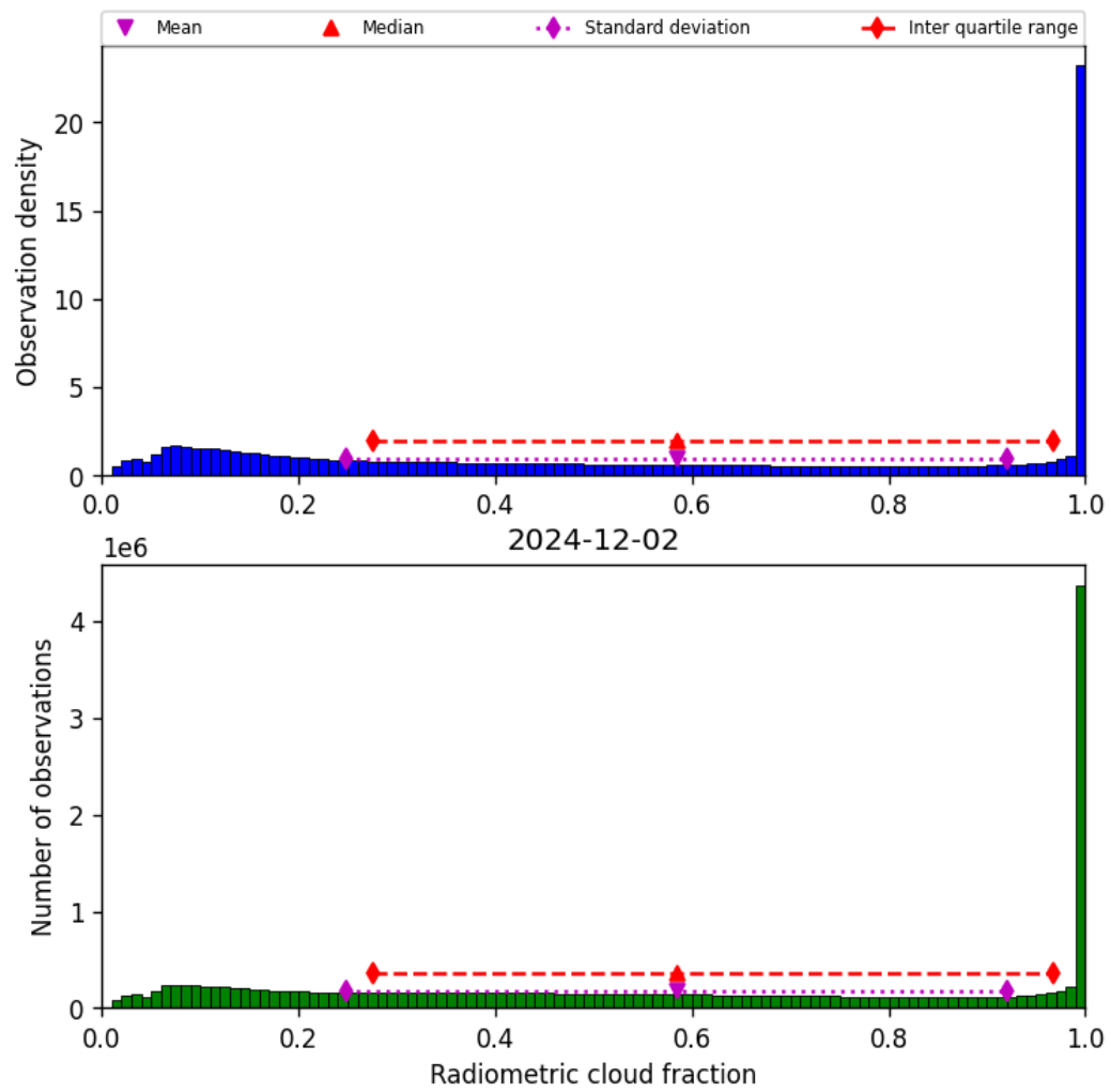
Figure 37: Histogram of “Radiometric cloud fraction” for 2024-12-02 to 2024-12-03
