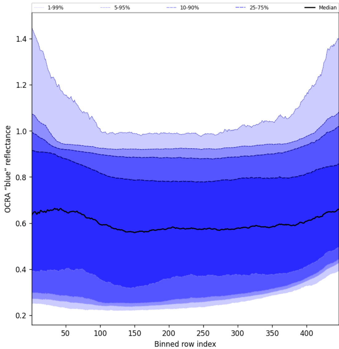
Figure 65: Along track statistics of “OCRA “blue” reflectance” for 2024-12-02 to 2024-12-03
