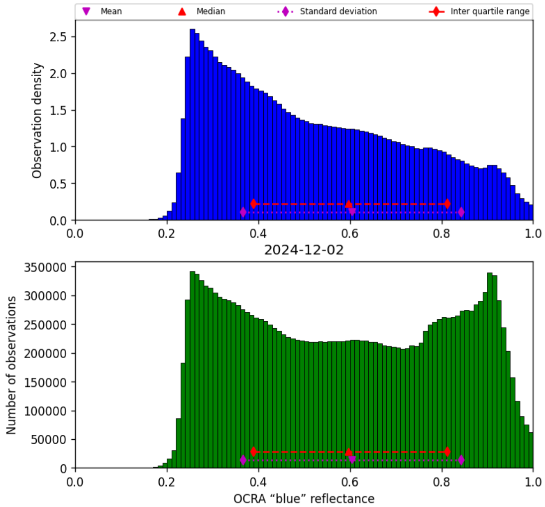
Figure 49: Histogram of “OCRA “blue” reflectance” for 2024-12-02 to 2024-12-03
