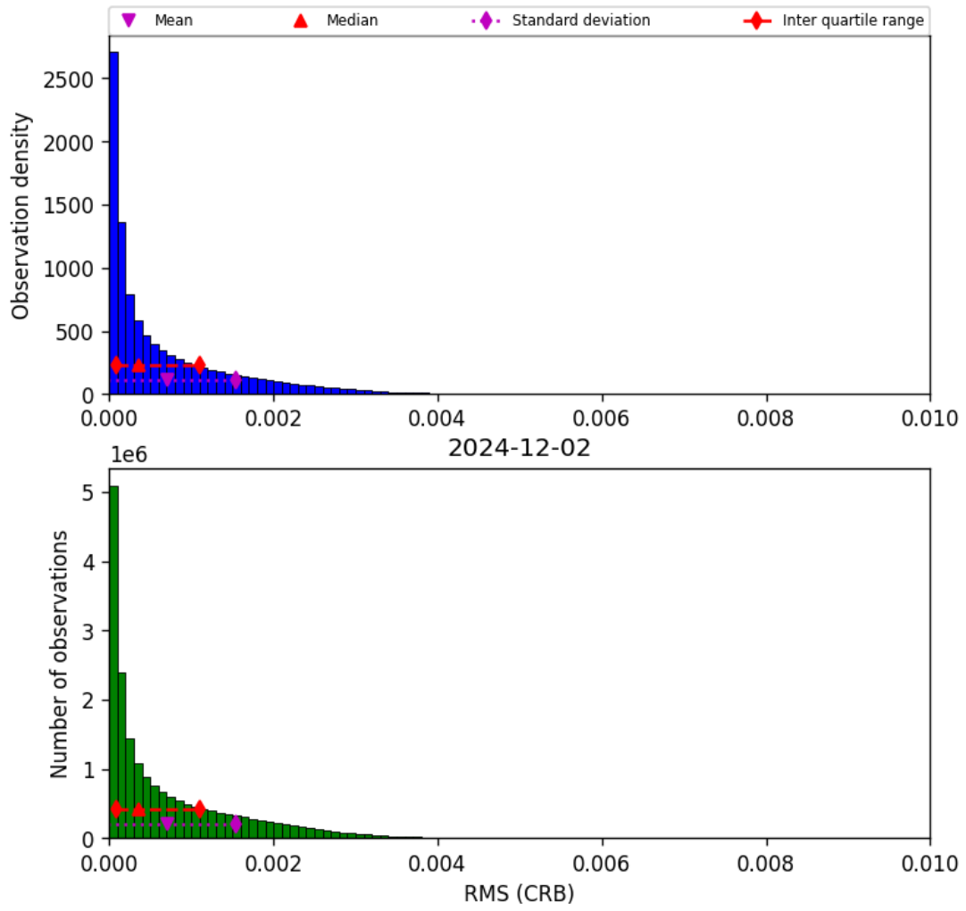
Figure 46: Histogram of “RMS (CRB)” for 2024-12-02 to 2024-12-03
