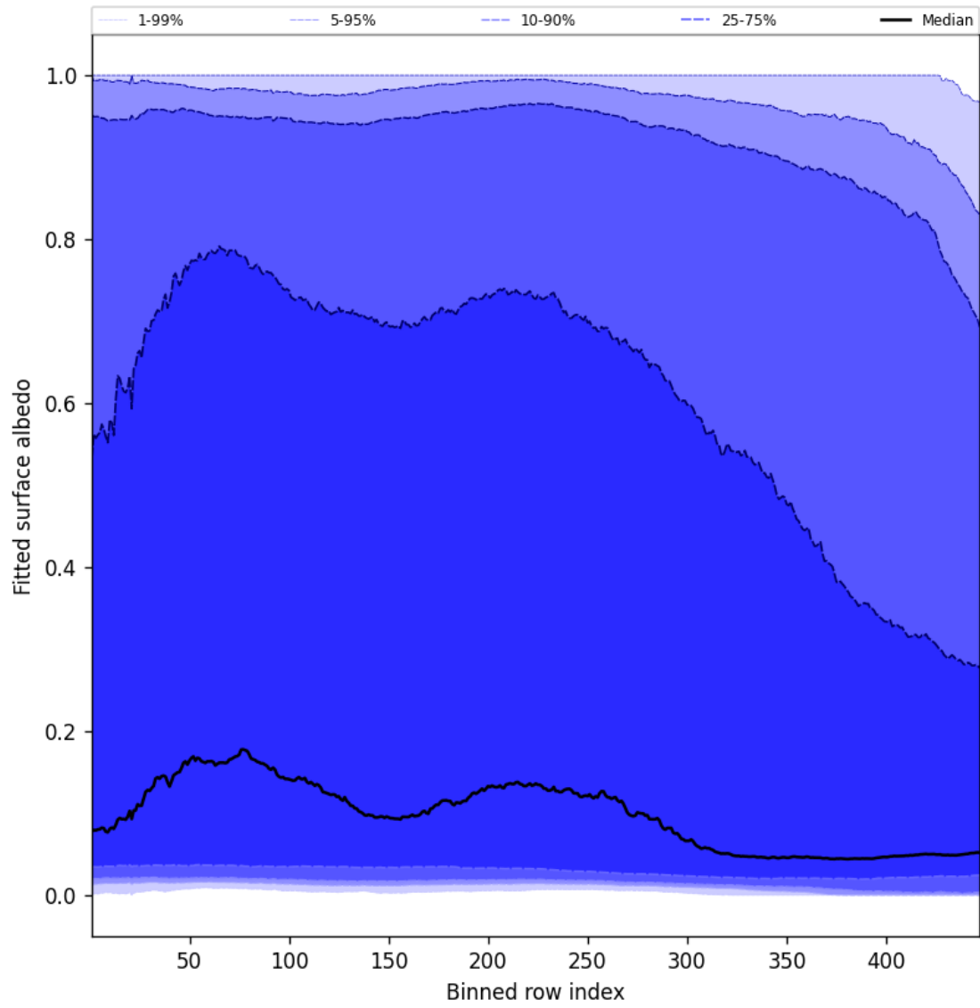
Figure 59: Along track statistics of “Fitted surface albedo” for 2024-12-02 to 2024-12-03
