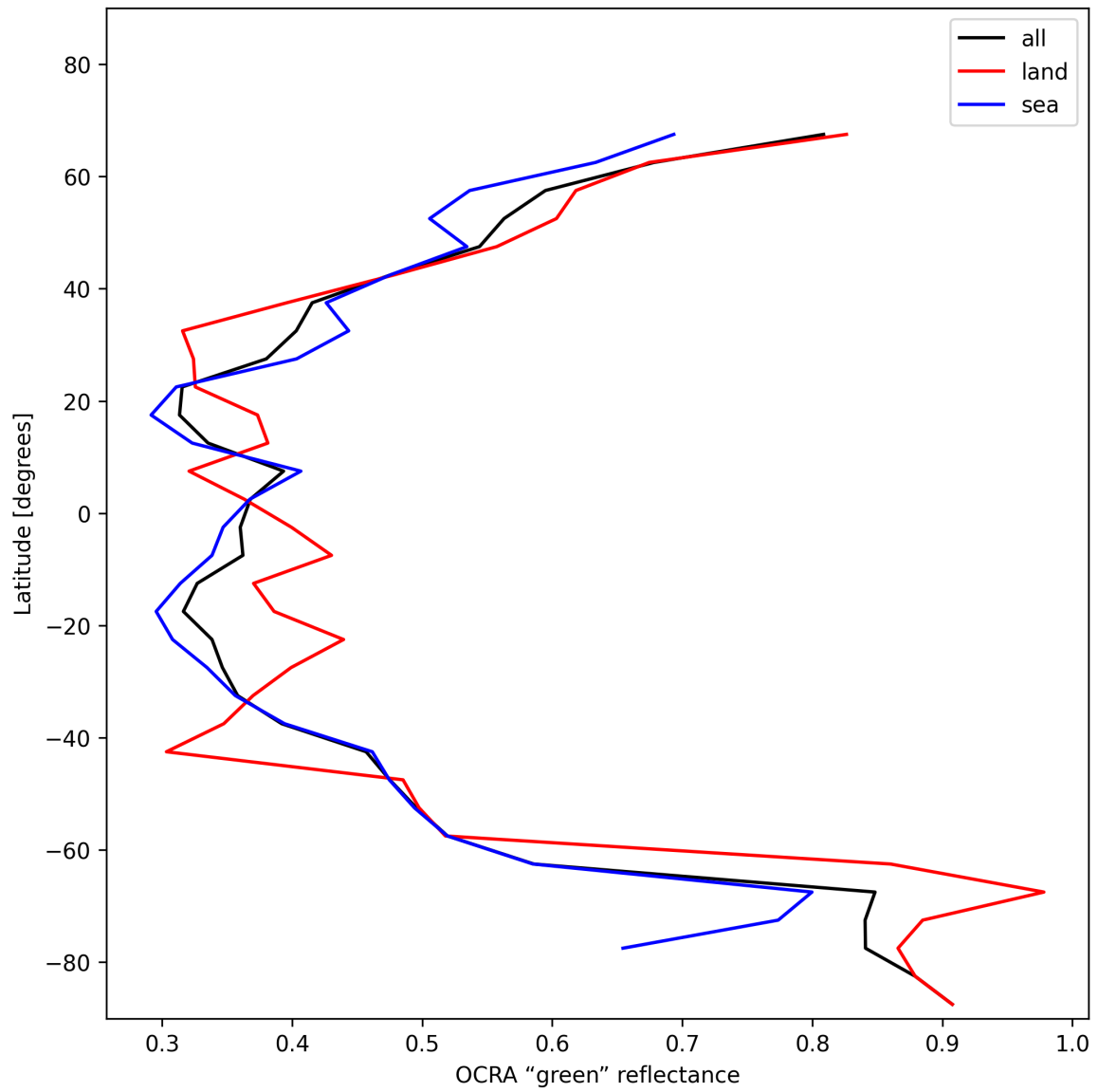
Figure 34: Zonal average of “OCRA “green” reflectance” for 2024-12-02 to 2024-12-03.
