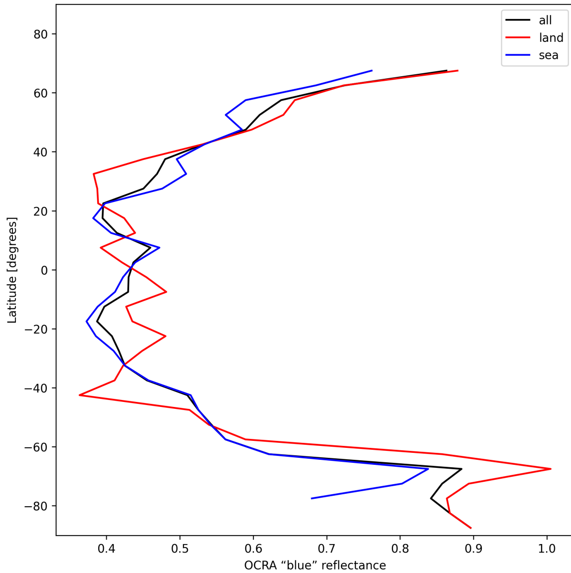
Figure 33: Zonal average of “OCRA “blue” reflectance” for 2024-12-02 to 2024-12-03.
