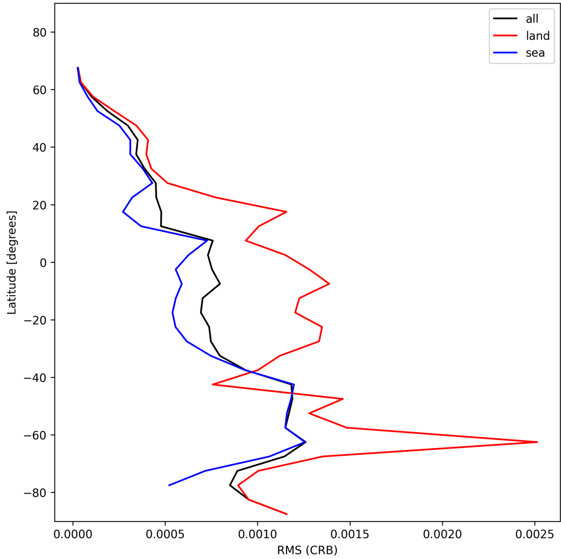
Figure 30: Zonal average of “RMS (CRB)” for 2024-12-02 to 2024-12-03.
