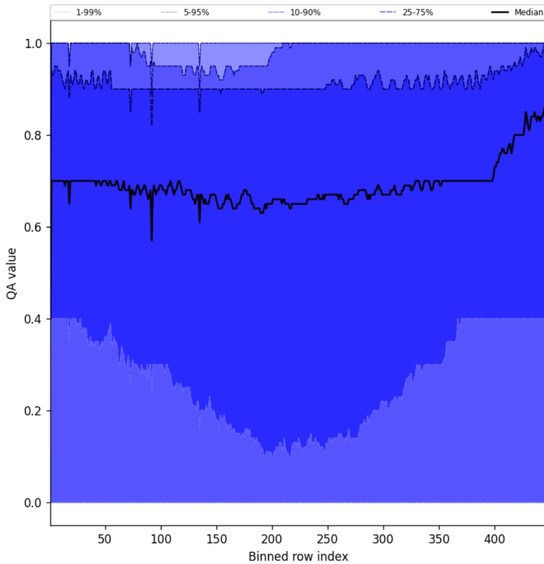
Figure 52: Along track statistics of “QA value” for 2024-12-02 to 2024-12-03
