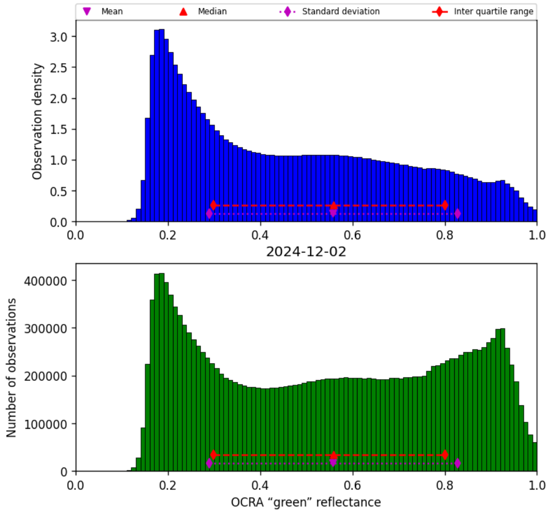
Figure 50: Histogram of “OCRA “green” reflectance” for 2024-12-02 to 2024-12-03
