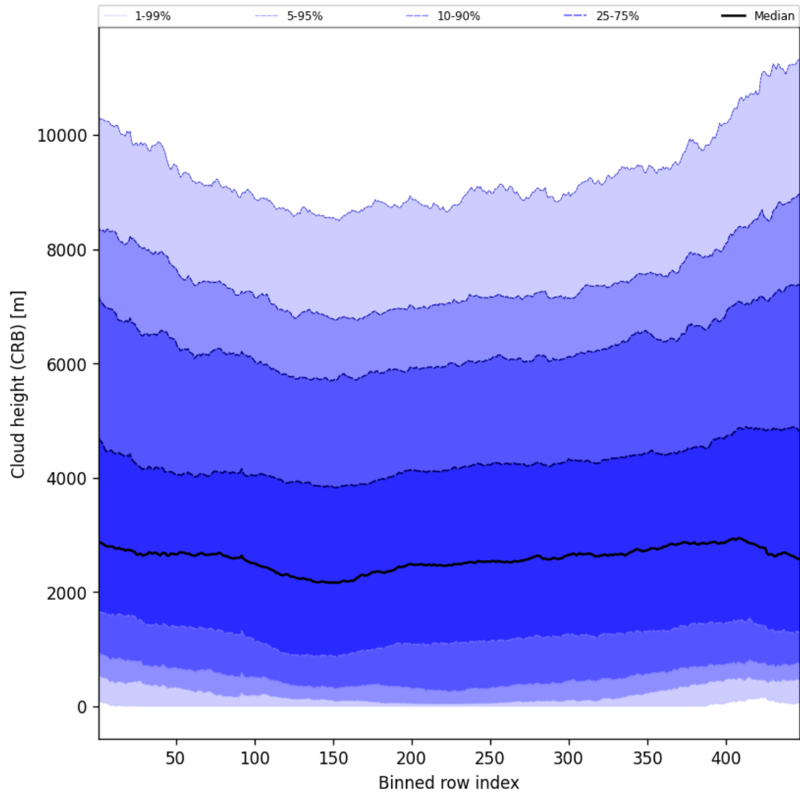
Figure 57: Along track statistics of “Cloud height (CRB)” for 2024-12-02 to 2024-12-03
