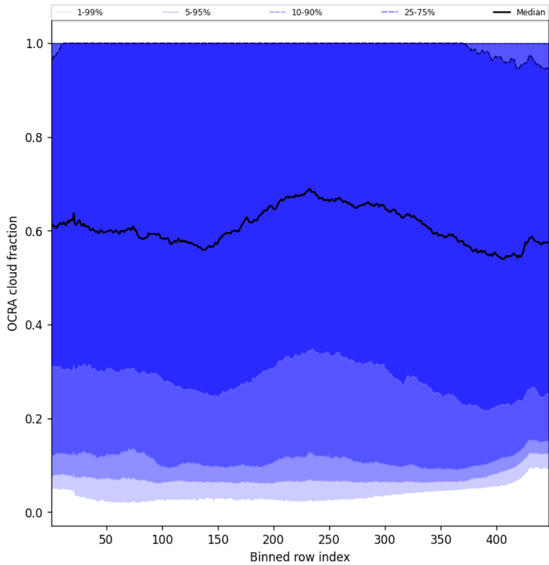
Figure 64: Along track statistics of “OCRA cloud fraction” for 2024-12-02 to 2024-12-03
