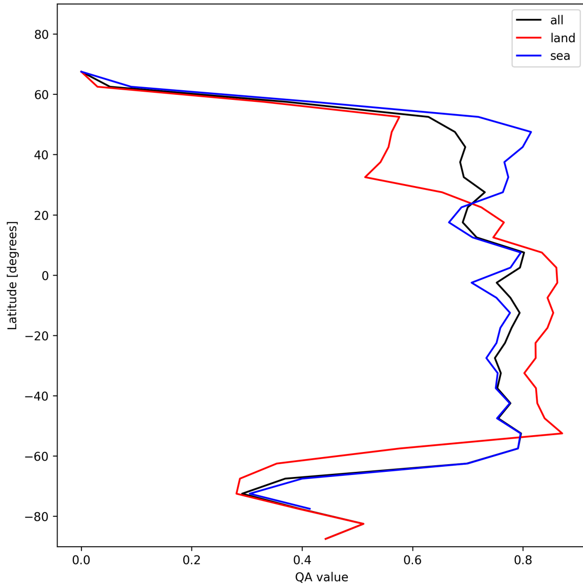
Figure 20: Zonal average of “QA value” for 2024-12-02 to 2024-12-03.
