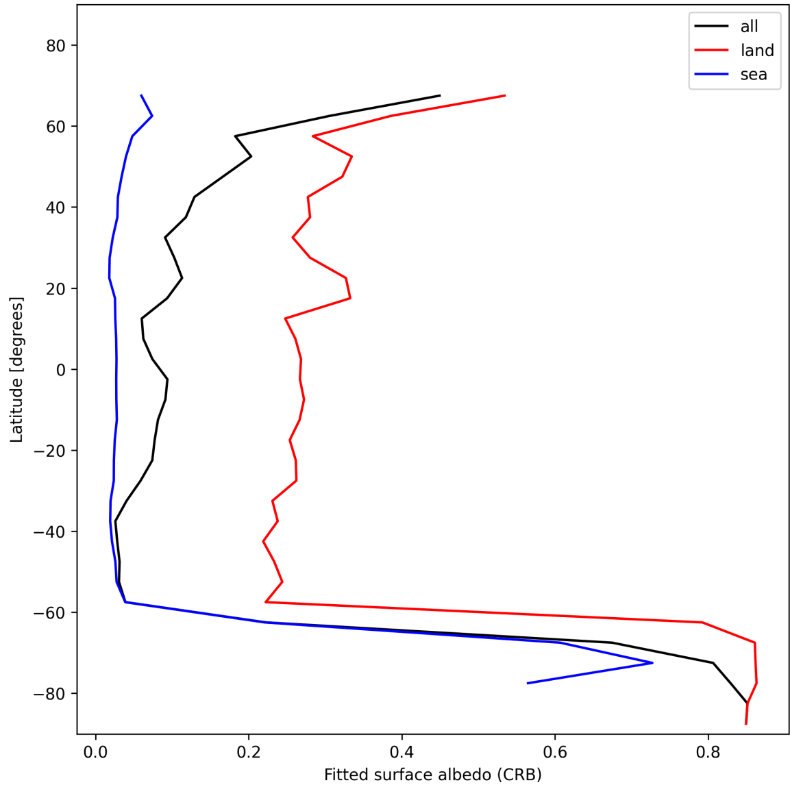
Figure 28: Zonal average of “Fitted surface albedo (CRB)” for 2024-12-04 to 2024-12-04.
