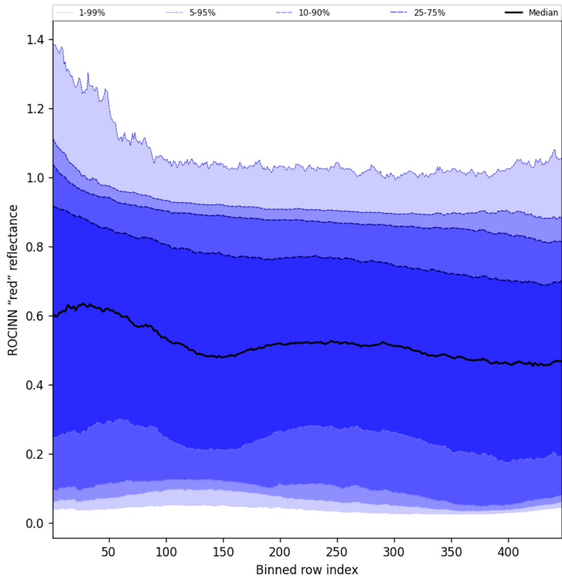
Figure 67: Along track statistics of "ROCINN "red" reflectance" for 2024-12-04 to 2024-12-04
