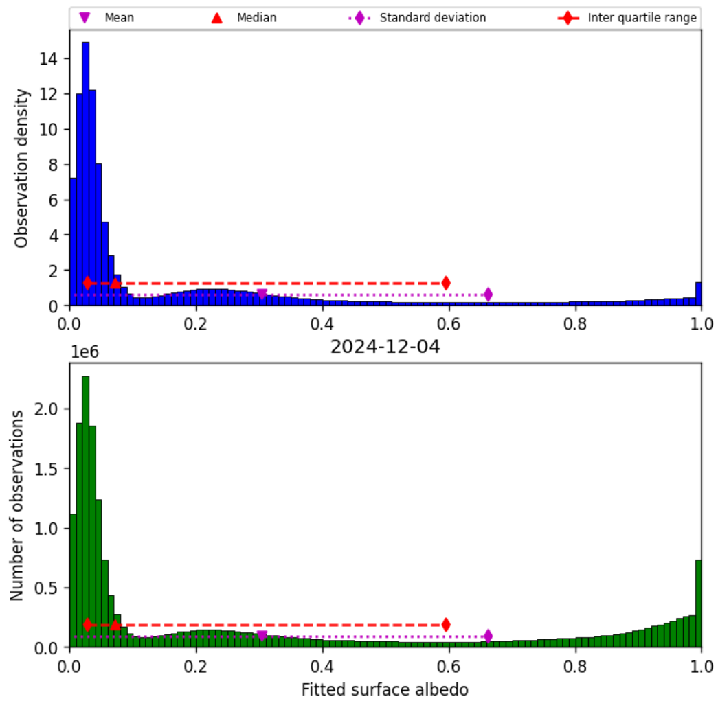
Figure 43: Histogram of “Fitted surface albedo” for 2024-12-04 to 2024-12-04
