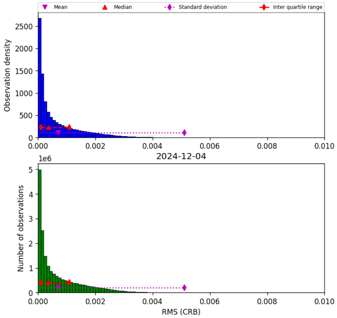
Figure 46: Histogram of “RMS (CRB)” for 2024-12-04 to 2024-12-04
