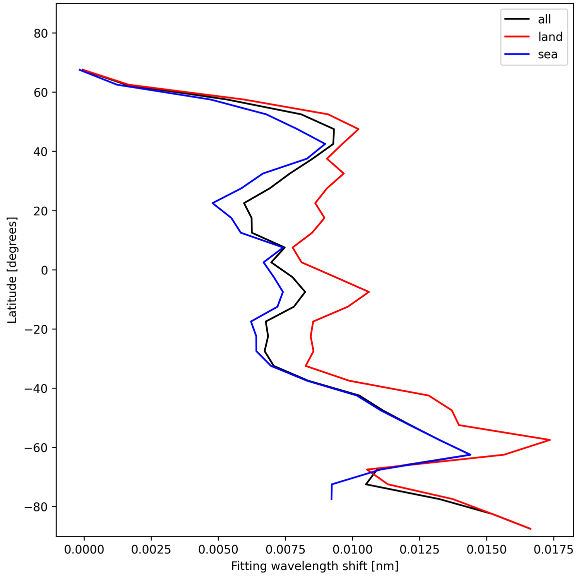
Figure 31: Zonal average of “Fitting wavelength shift” for 2024-12-04 to 2024-12-04.
