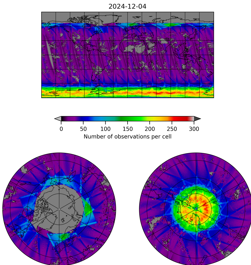
Figure 19: Map of the number of observations for 2024-12-04 to 2024-12-04
