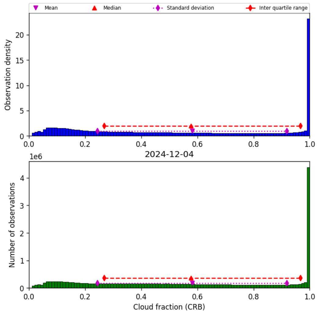
Figure 40: Histogram of “Cloud fraction (CRB)” for 2024-12-04 to 2024-12-04
