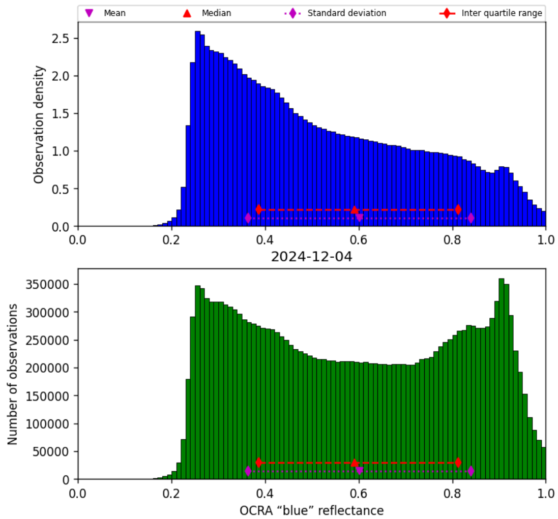
Figure 49: Histogram of “OCRA “blue” reflectance” for 2024-12-04 to 2024-12-04
