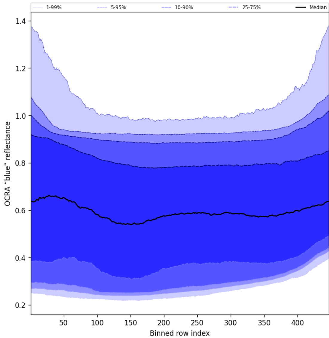
Figure 65: Along track statistics of “OCRA “blue” reflectance” for 2024-12-04 to 2024-12-04
