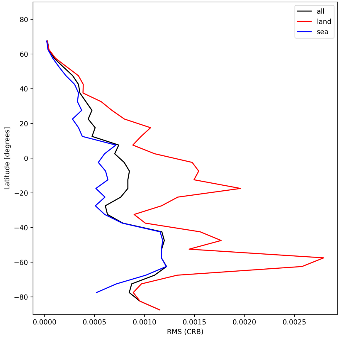
Figure 30: Zonal average of “RMS (CRB)” for 2024-12-04 to 2024-12-04.
