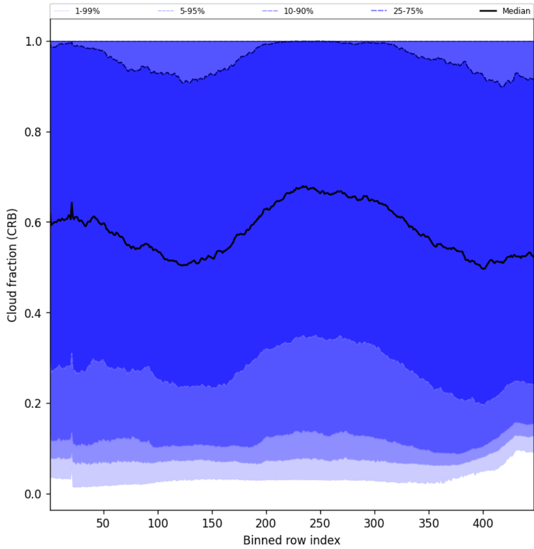
Figure 56: Along track statistics of “Cloud fraction (CRB)” for 2024-12-04 to 2024-12-04
