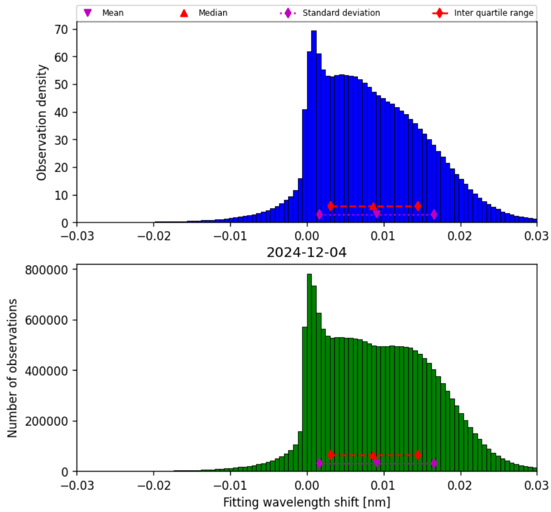
Figure 47: Histogram of “Fitting wavelength shift” for 2024-12-04 to 2024-12-04
