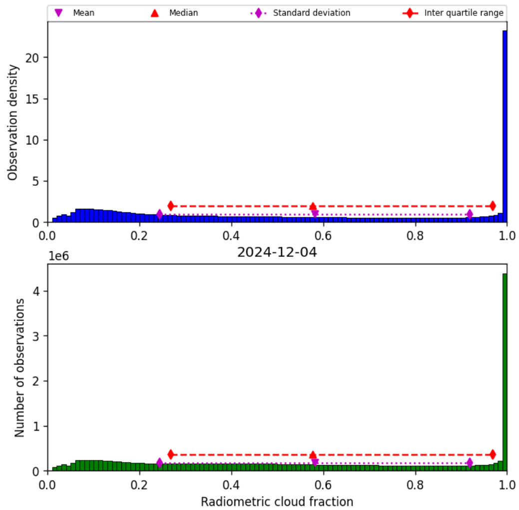
Figure 37: Histogram of “Radiometric cloud fraction” for 2024-12-04 to 2024-12-04
