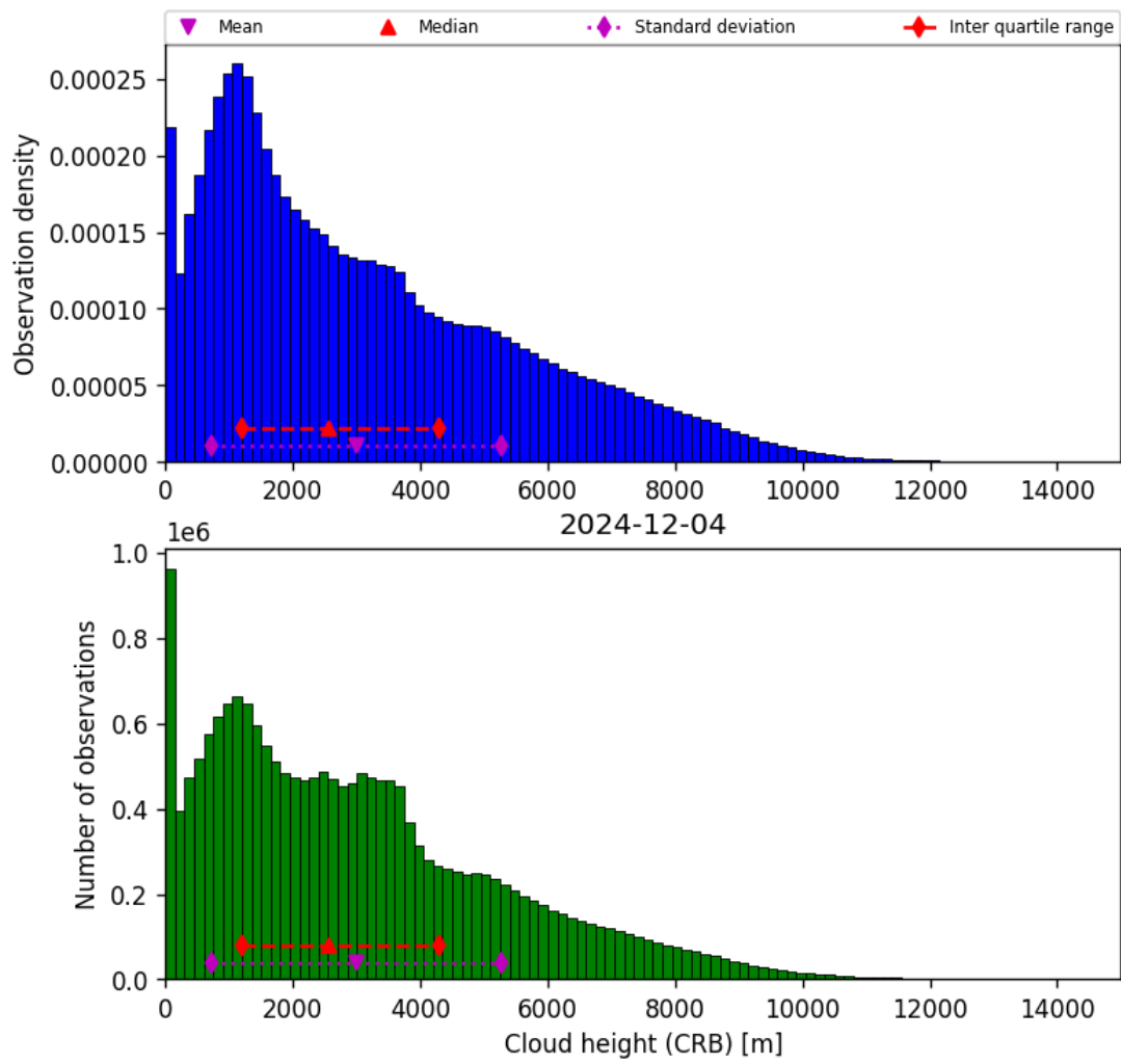
Figure 41: Histogram of “Cloud height (CRB)” for 2024-12-04 to 2024-12-04
