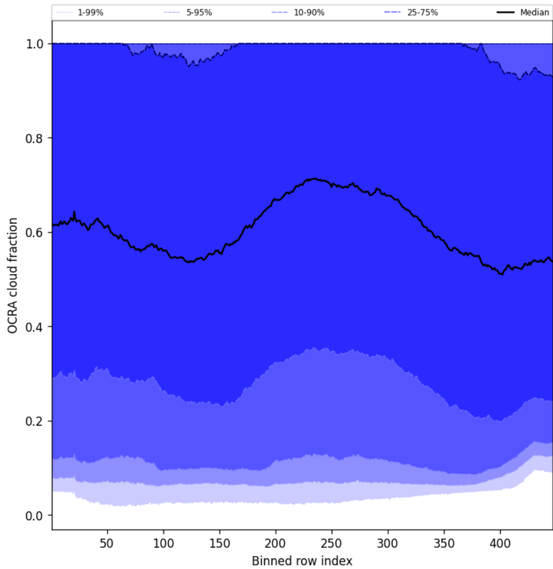
Figure 64: Along track statistics of “OCRA cloud fraction” for 2024-12-04 to 2024-12-04
