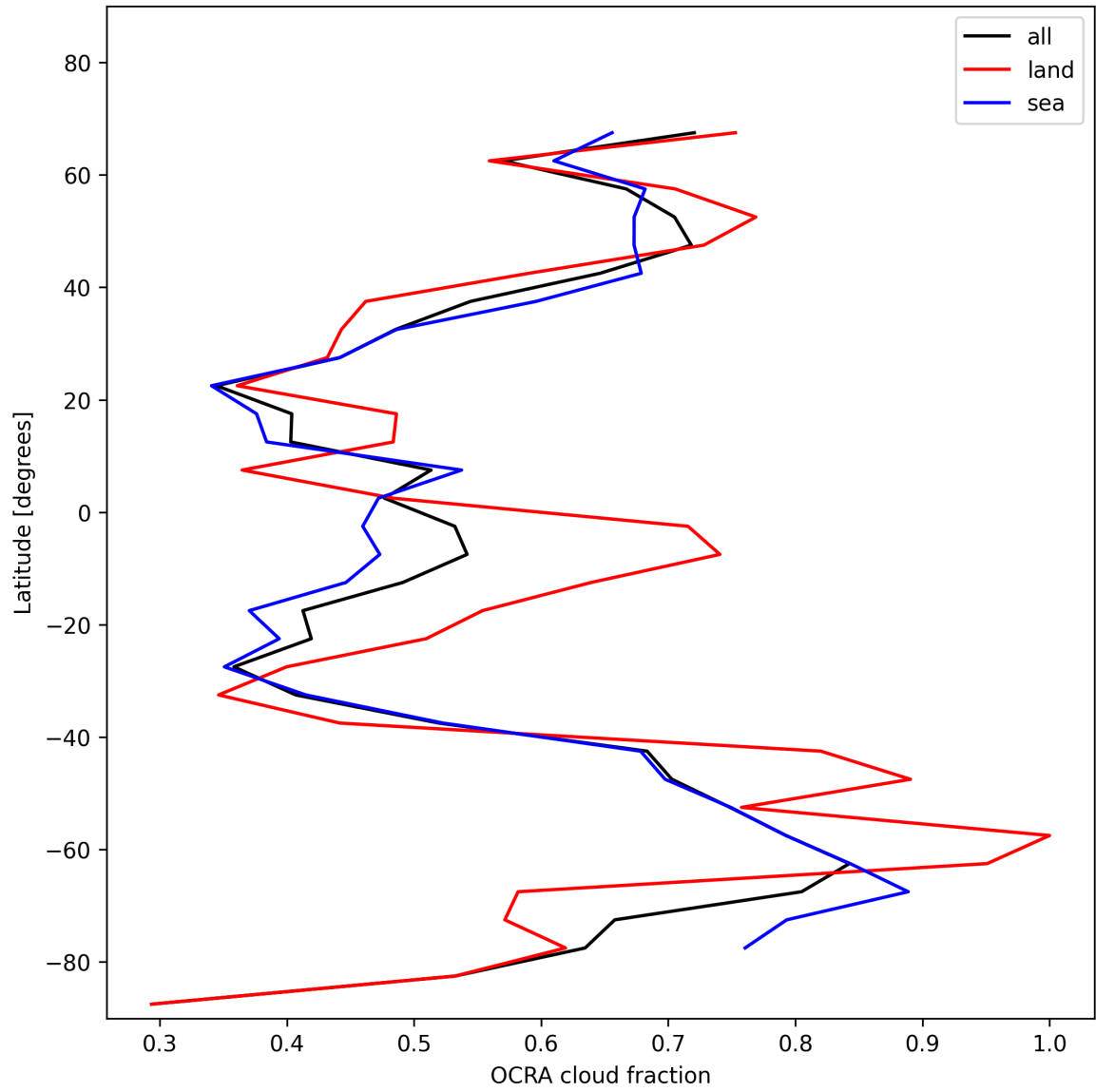
Figure 32: Zonal average of “OCRA cloud fraction” for 2024-12-04 to 2024-12-04.
