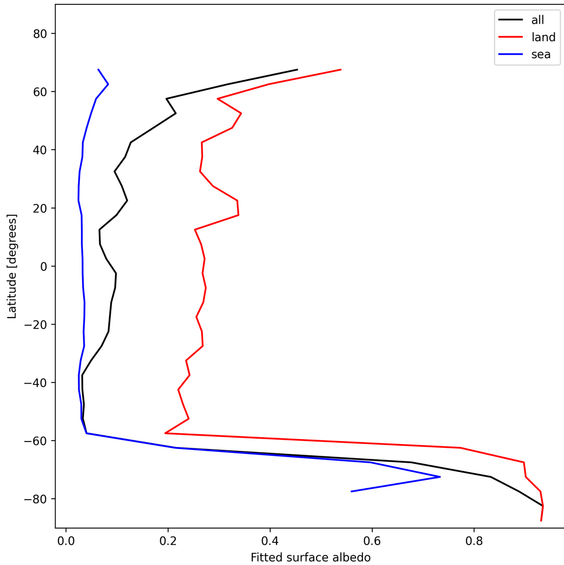
Figure 27: Zonal average of “Fitted surface albedo” for 2024-12-04 to 2024-12-04.
