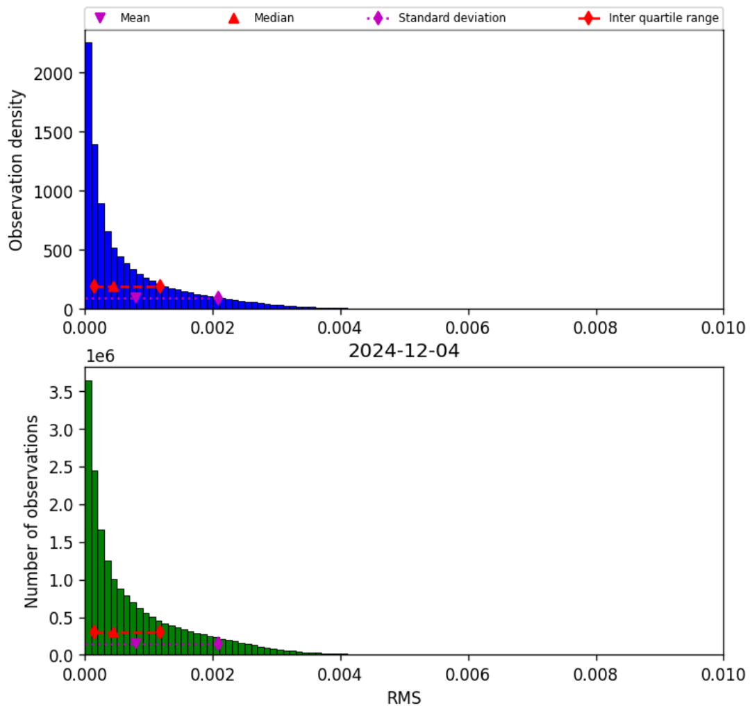
Figure 45: Histogram of “RMS” for 2024-12-04 to 2024-12-04
