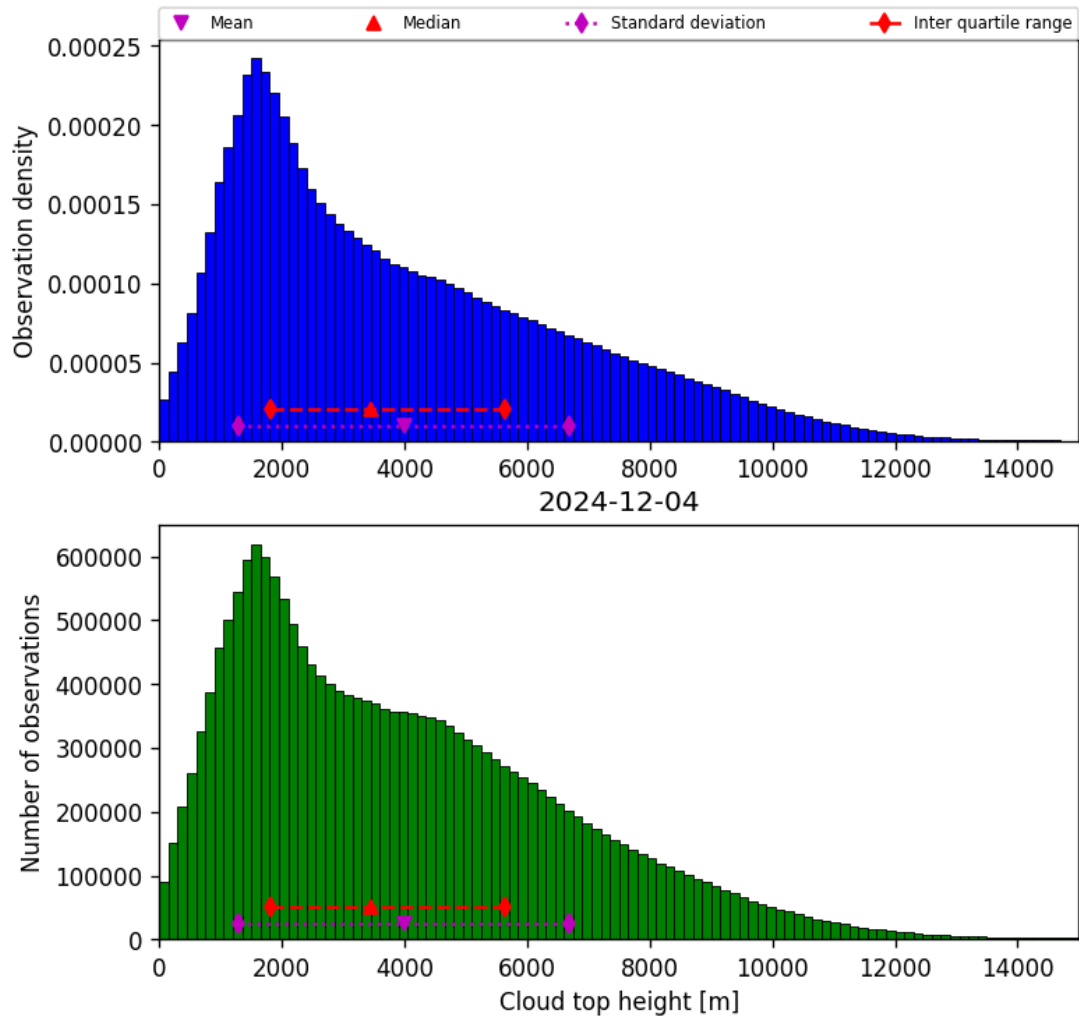
Figure 38: Histogram of “Cloud top height” for 2024-12-04 to 2024-12-04
