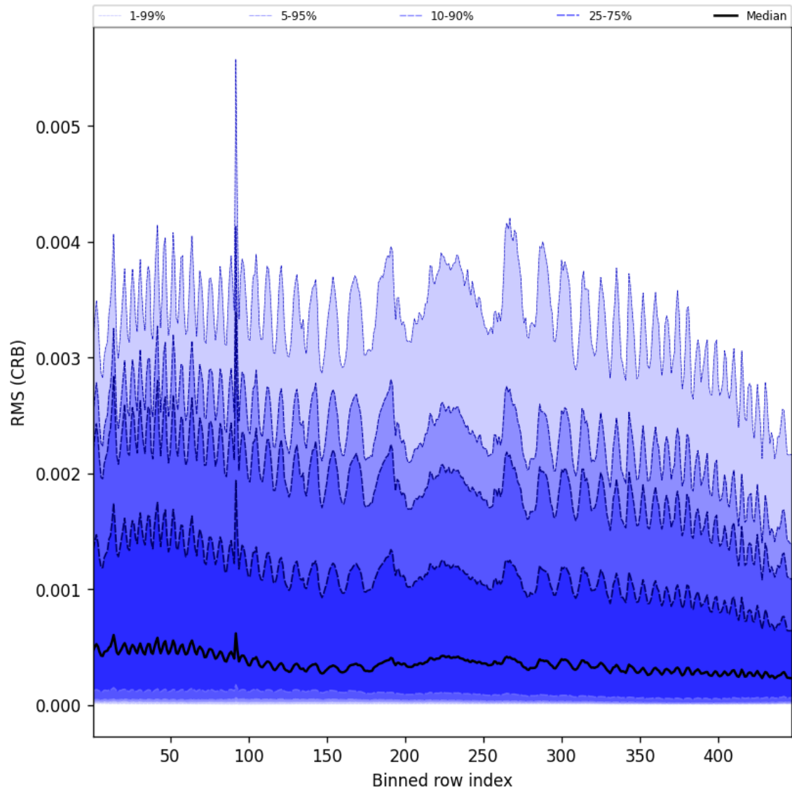
Figure 62: Along track statistics of “RMS (CRB)” for 2024-12-04 to 2024-12-04
