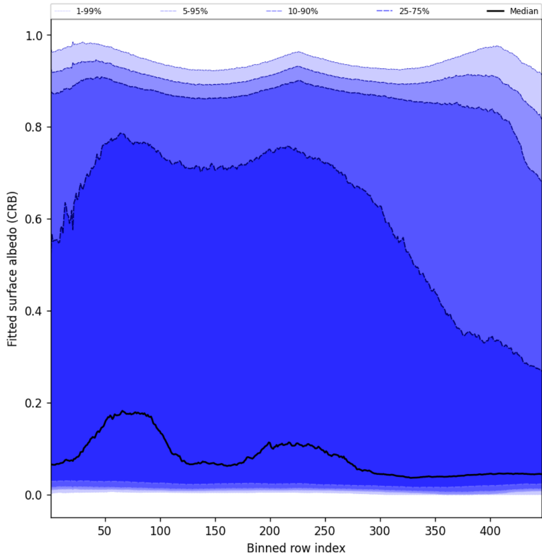
Figure 60: Along track statistics of “Fitted surface albedo (CRB)” for 2024-12-04 to 2024-12-04
