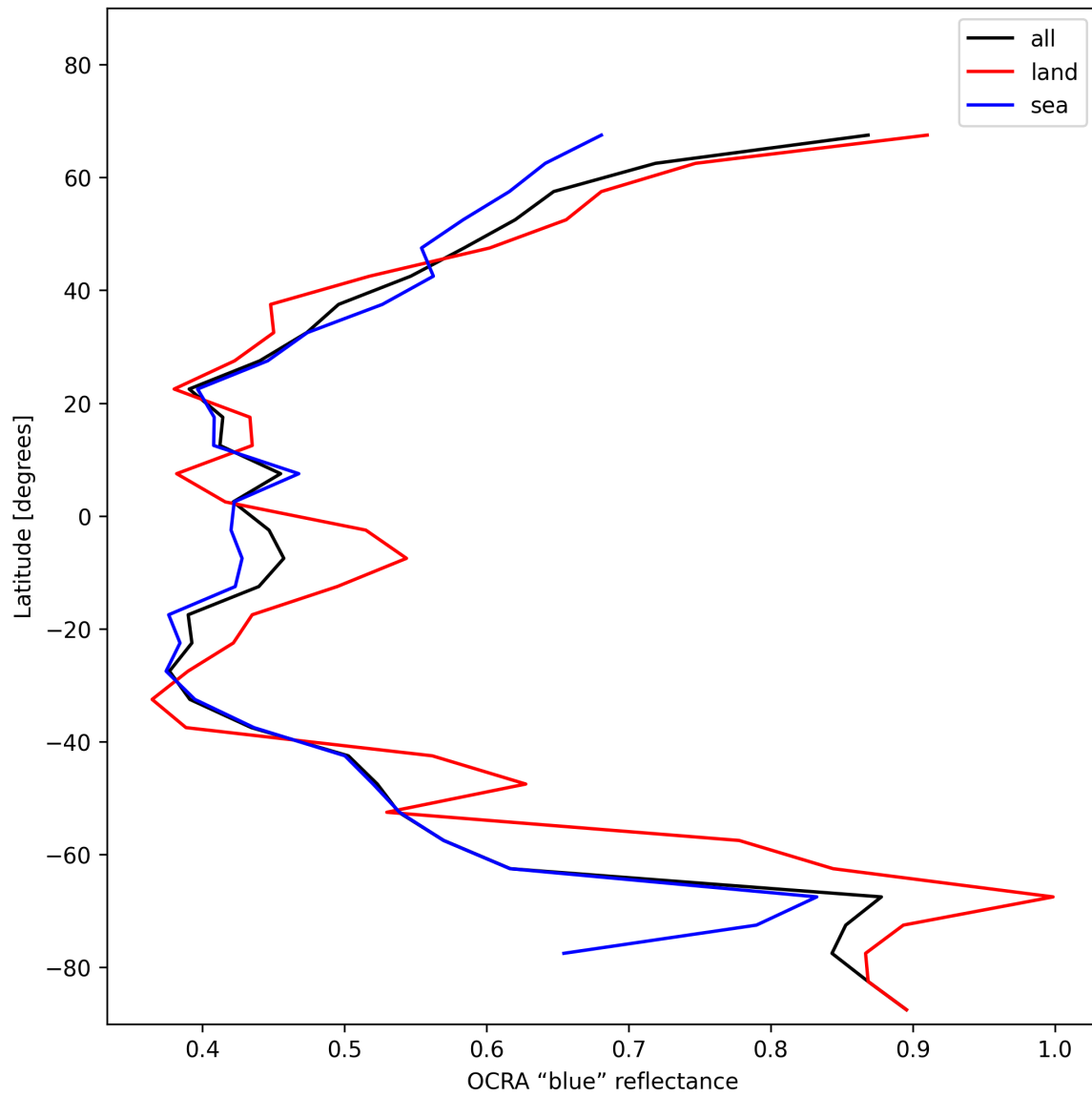
Figure 33: Zonal average of “OCRA “blue” reflectance” for 2024-12-04 to 2024-12-04.
