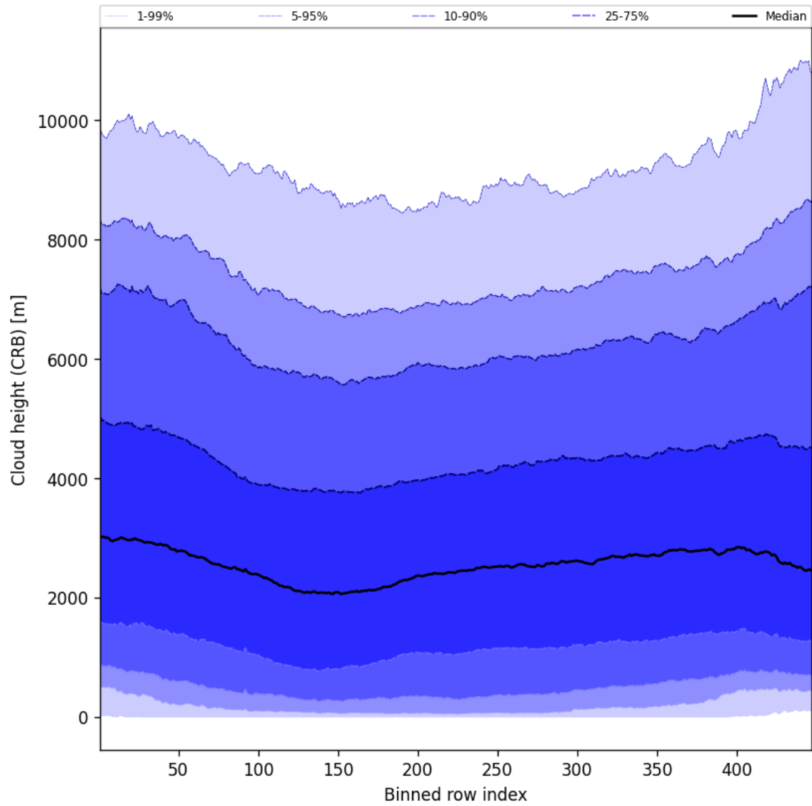
Figure 57: Along track statistics of “Cloud height (CRB)” for 2024-12-04 to 2024-12-04
