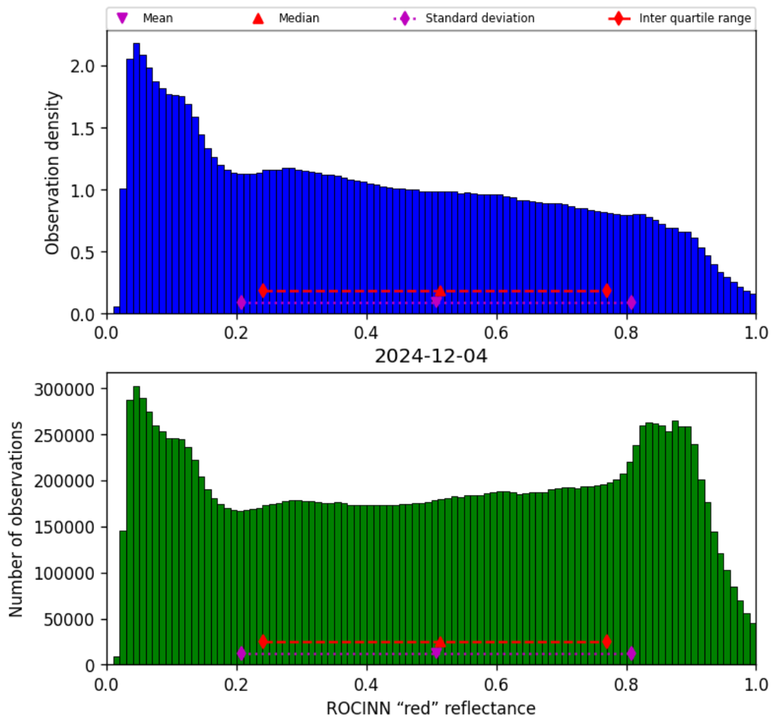
Figure 51: Histogram of “ROCINN “red” reflectance” for 2024-12-04 to 2024-12-04
