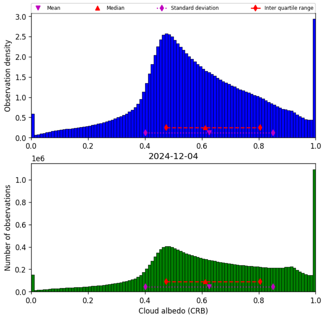
Figure 42: Histogram of “Cloud albedo (CRB)” for 2024-12-04 to 2024-12-04
