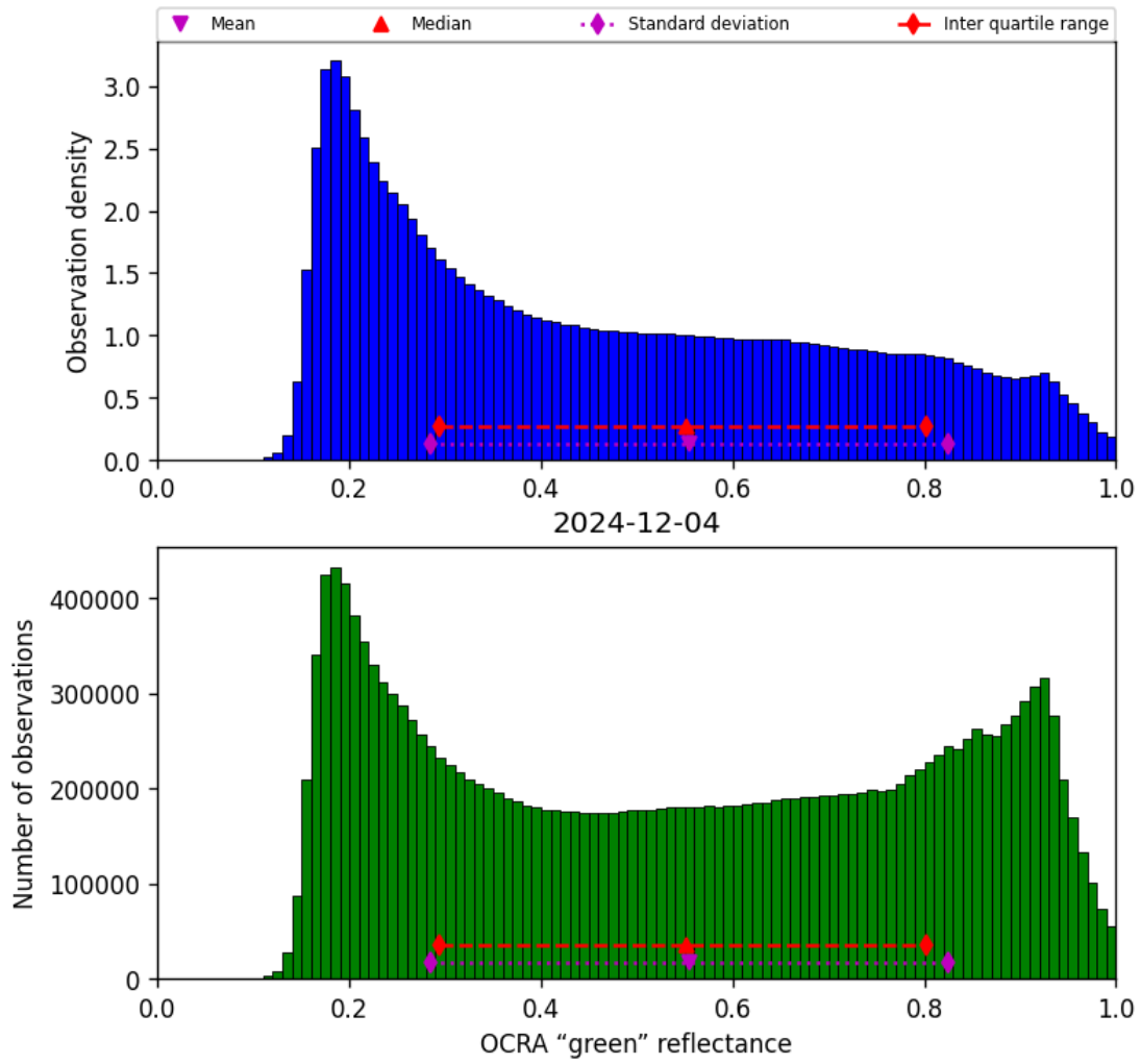
Figure 50: Histogram of “OCRA “green” reflectance” for 2024-12-04 to 2024-12-04
