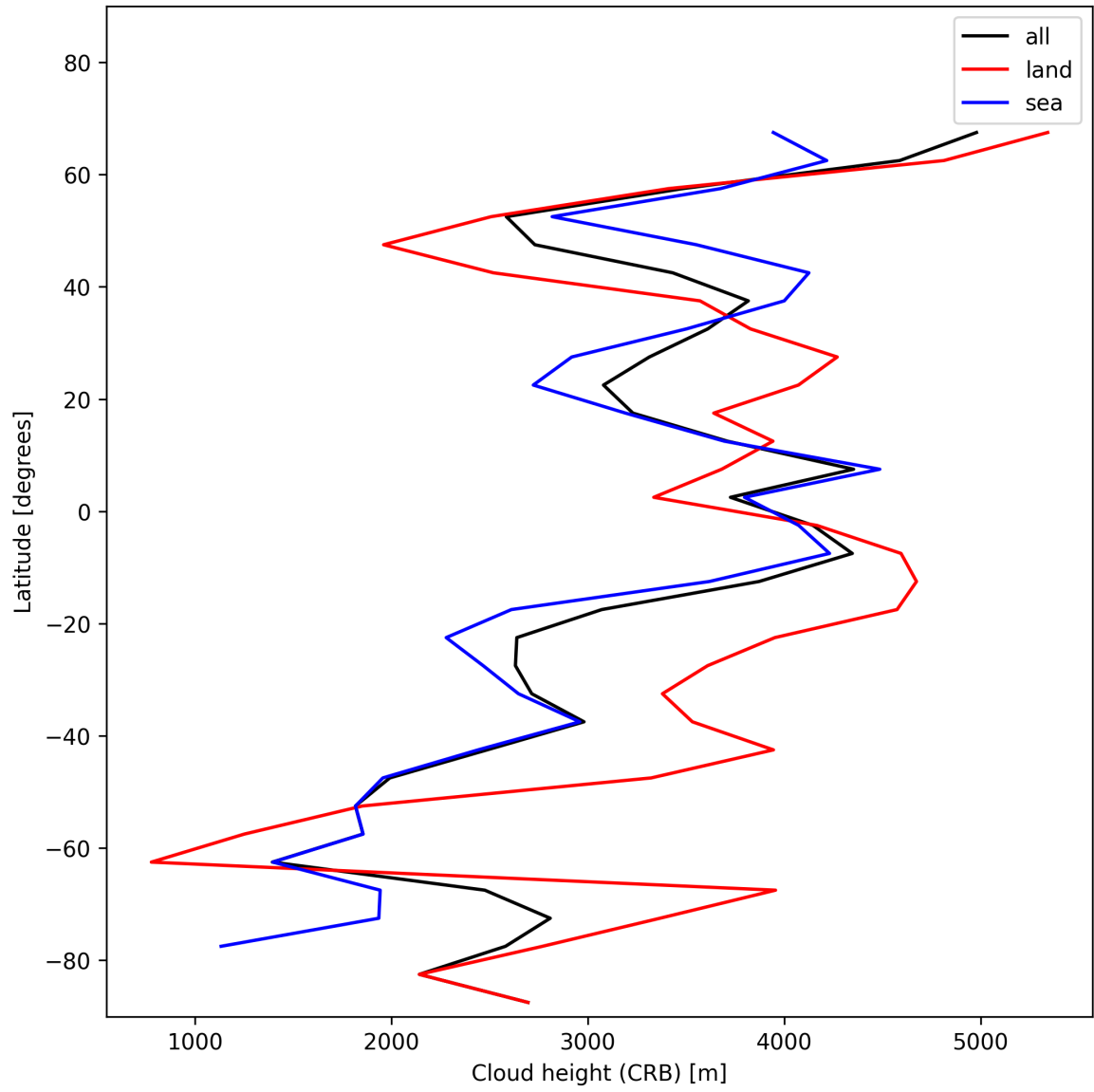
Figure 25: Zonal average of “Cloud height (CRB)” for 2024-12-04 to 2024-12-04.
