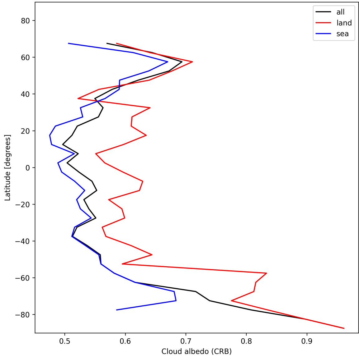
Figure 26: Zonal average of “Cloud albedo (CRB)” for 2024-12-04 to 2024-12-04.
