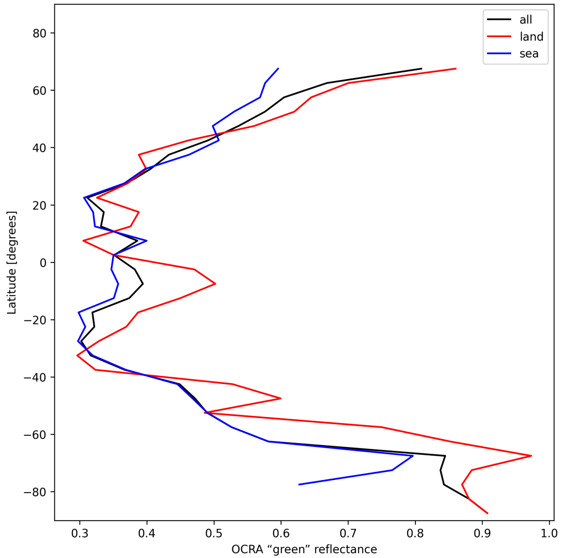
Figure 34: Zonal average of “OCRA “green” reflectance” for 2024-12-04 to 2024-12-04.
