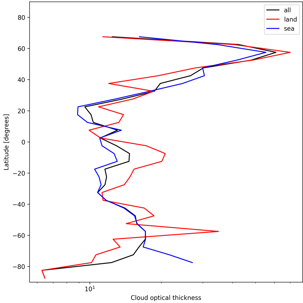
Figure 23: Zonal average of “Cloud optical thickness” for 2024-12-04 to 2024-12-04.
