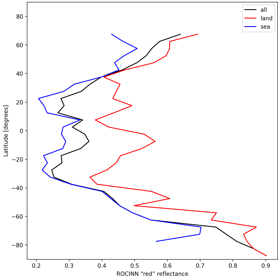
Figure 35: Zonal average of “ROCINN “red” reflectance” for 2024-12-04 to 2024-12-04.
