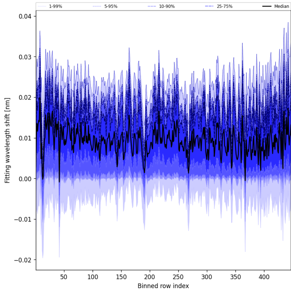
Figure 63: Along track statistics of “Fitting wavelength shift” for 2024-12-04 to 2024-12-04
