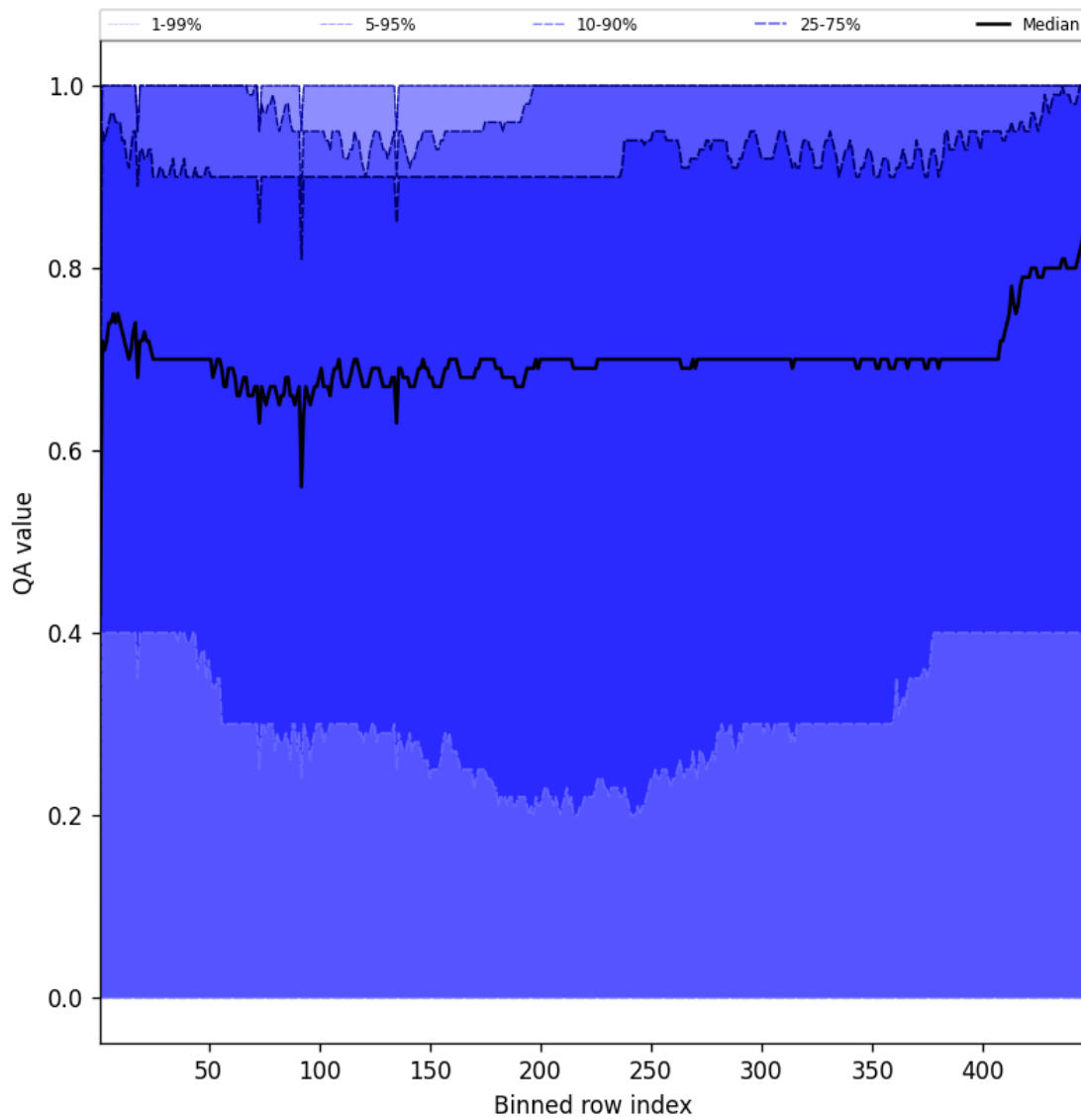
Figure 52: Along track statistics of “QA value” for 2024-12-04 to 2024-12-04
