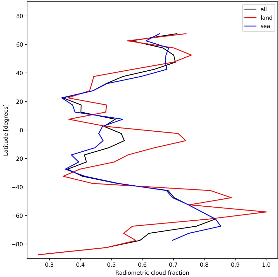
Figure 21: Zonal average of “Radiometric cloud fraction” for 2024-12-04 to 2024-12-04.
