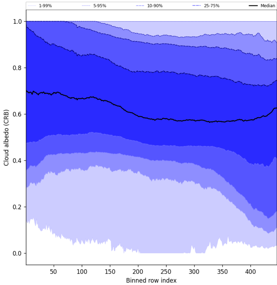
Figure 58: Along track statistics of “Cloud albedo (CRB)” for 2024-12-04 to 2024-12-04
