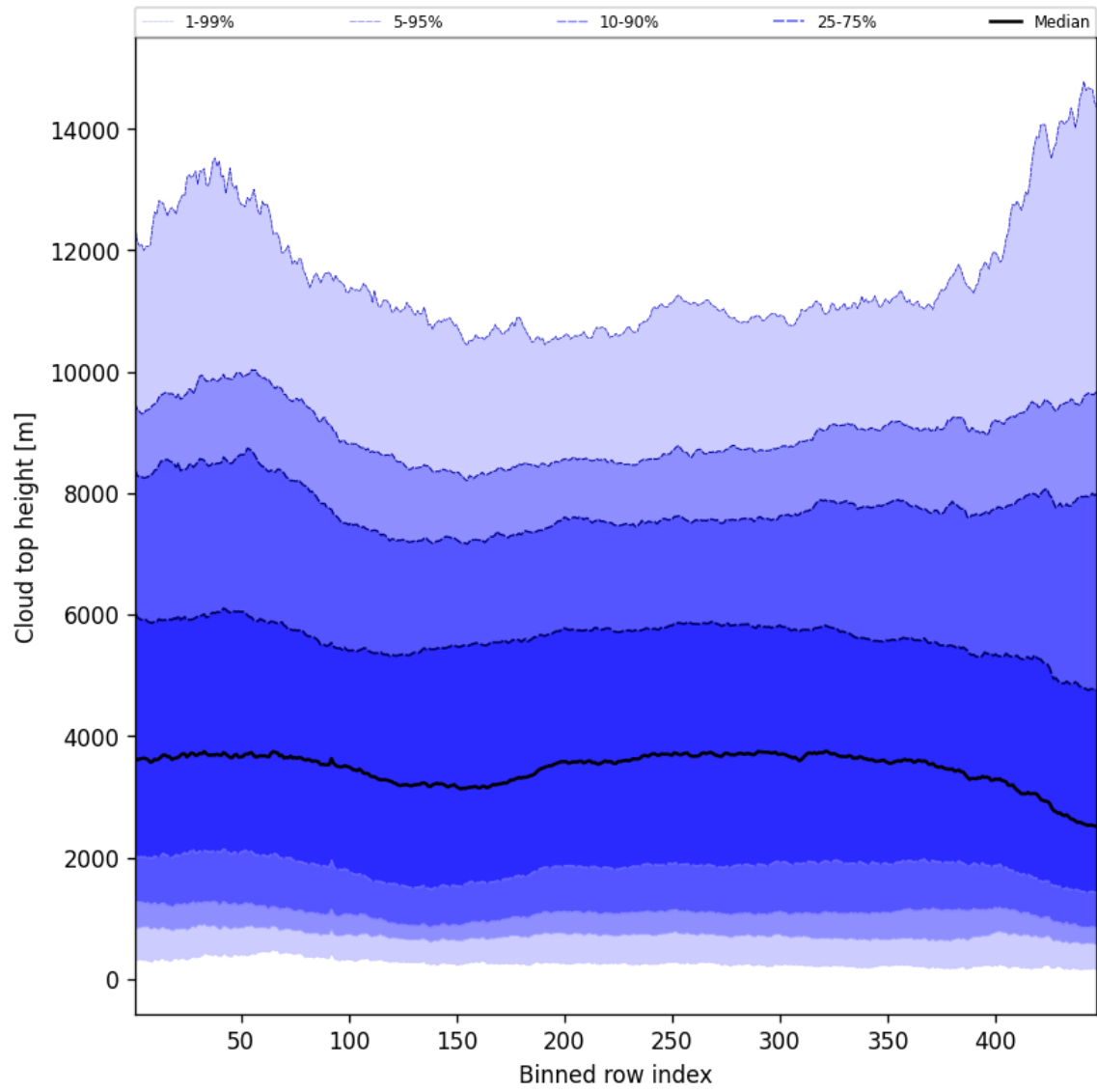
Figure 54: Along track statistics of “Cloud top height” for 2024-12-04 to 2024-12-04
