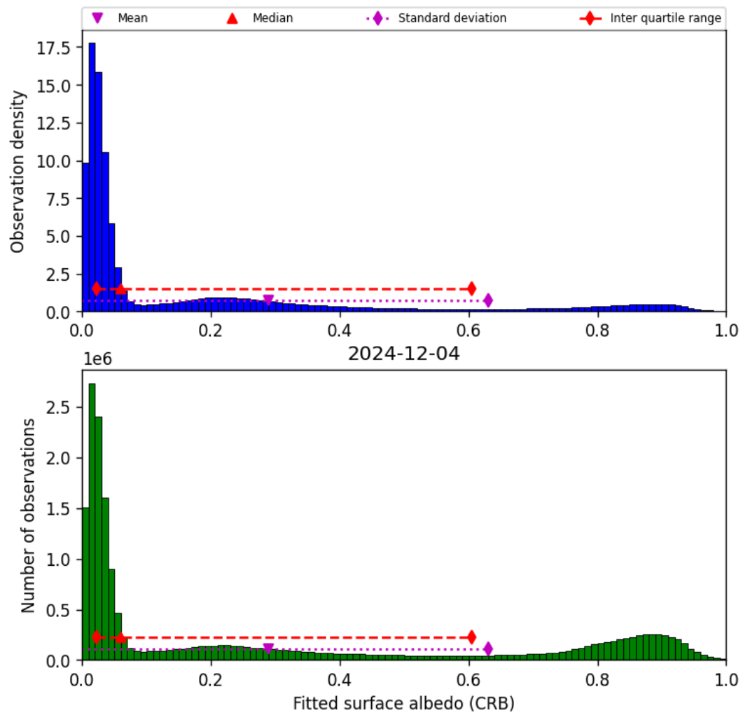
Figure 44: Histogram of “Fitted surface albedo (CRB)” for 2024-12-04 to 2024-12-04
