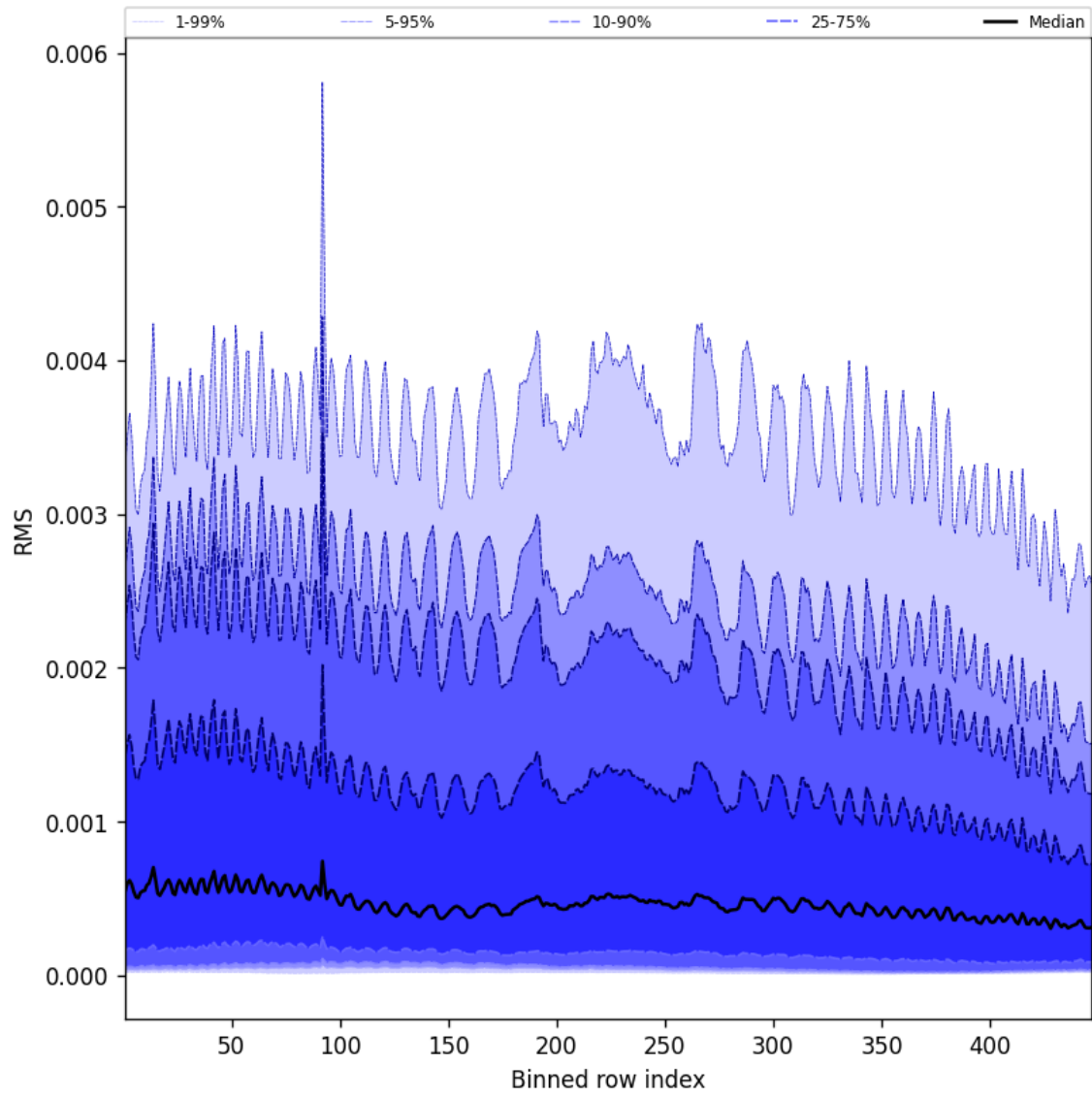
Figure 61: Along track statistics of “RMS” for 2024-12-04 to 2024-12-04
