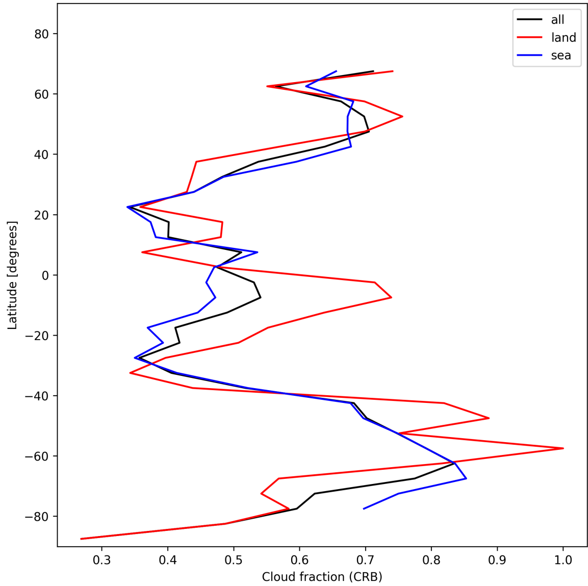
Figure 24: Zonal average of “Cloud fraction (CRB)” for 2024-12-04 to 2024-12-04.
