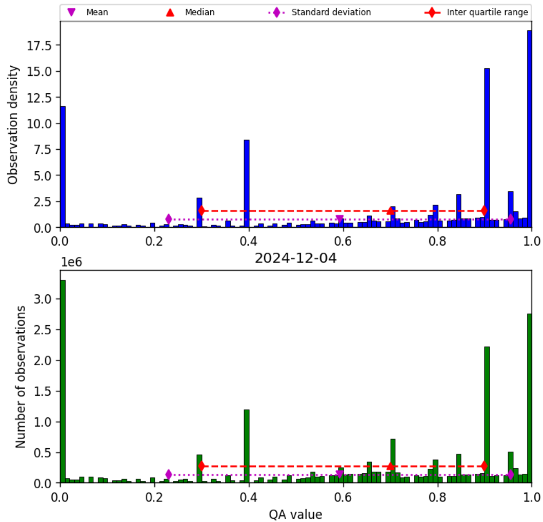
Figure 36: Histogram of “QA value” for 2024-12-04 to 2024-12-04
