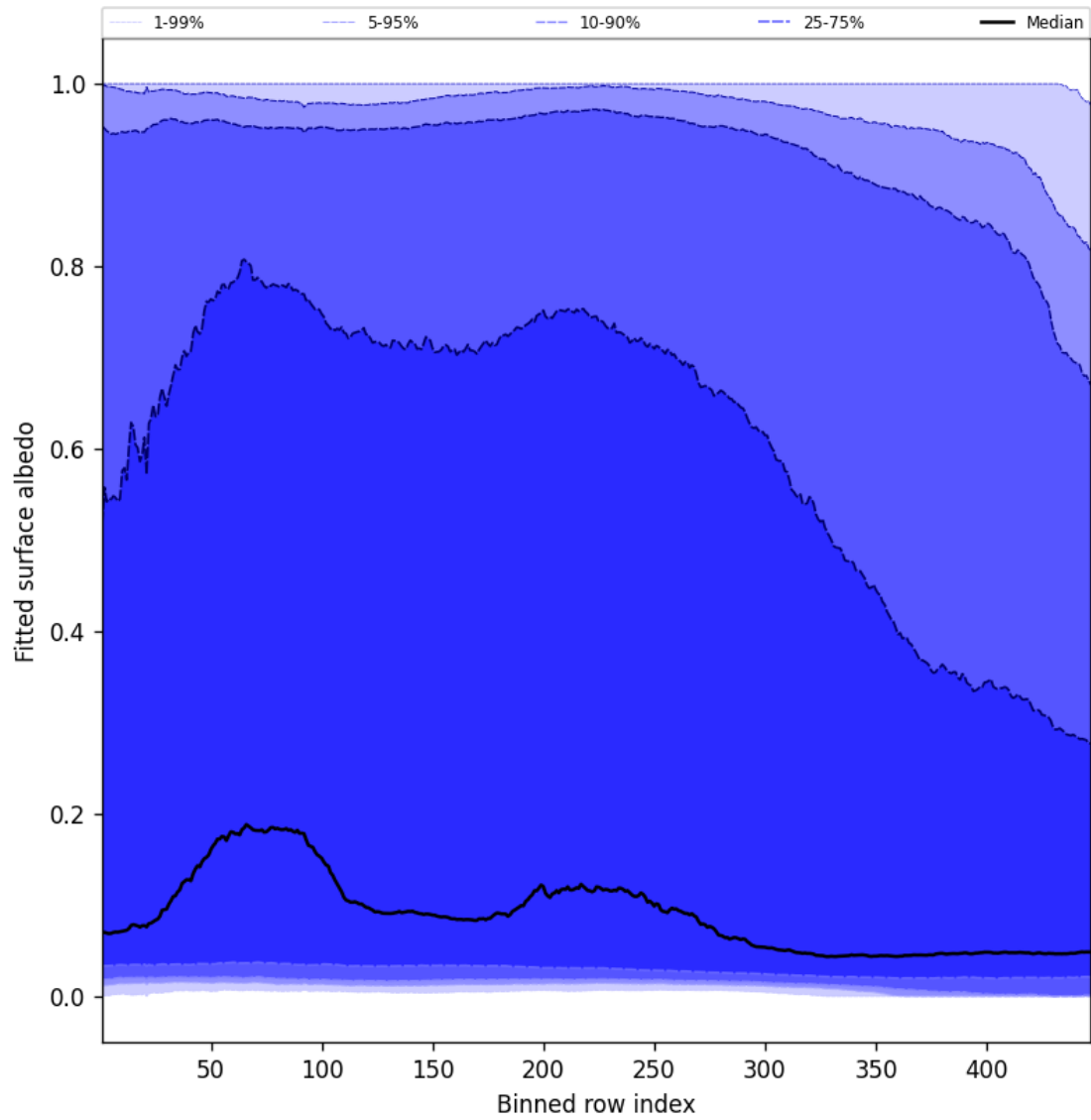
Figure 59: Along track statistics of “Fitted surface albedo” for 2024-12-04 to 2024-12-04
