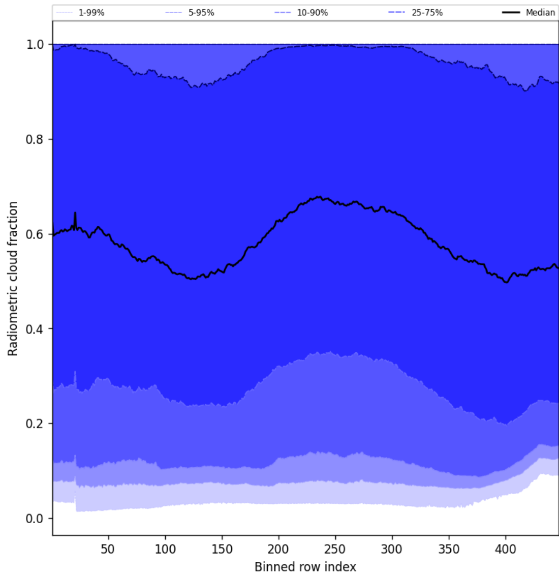
Figure 53: Along track statistics of “Radiometric cloud fraction” for 2024-12-04 to 2024-12-04
