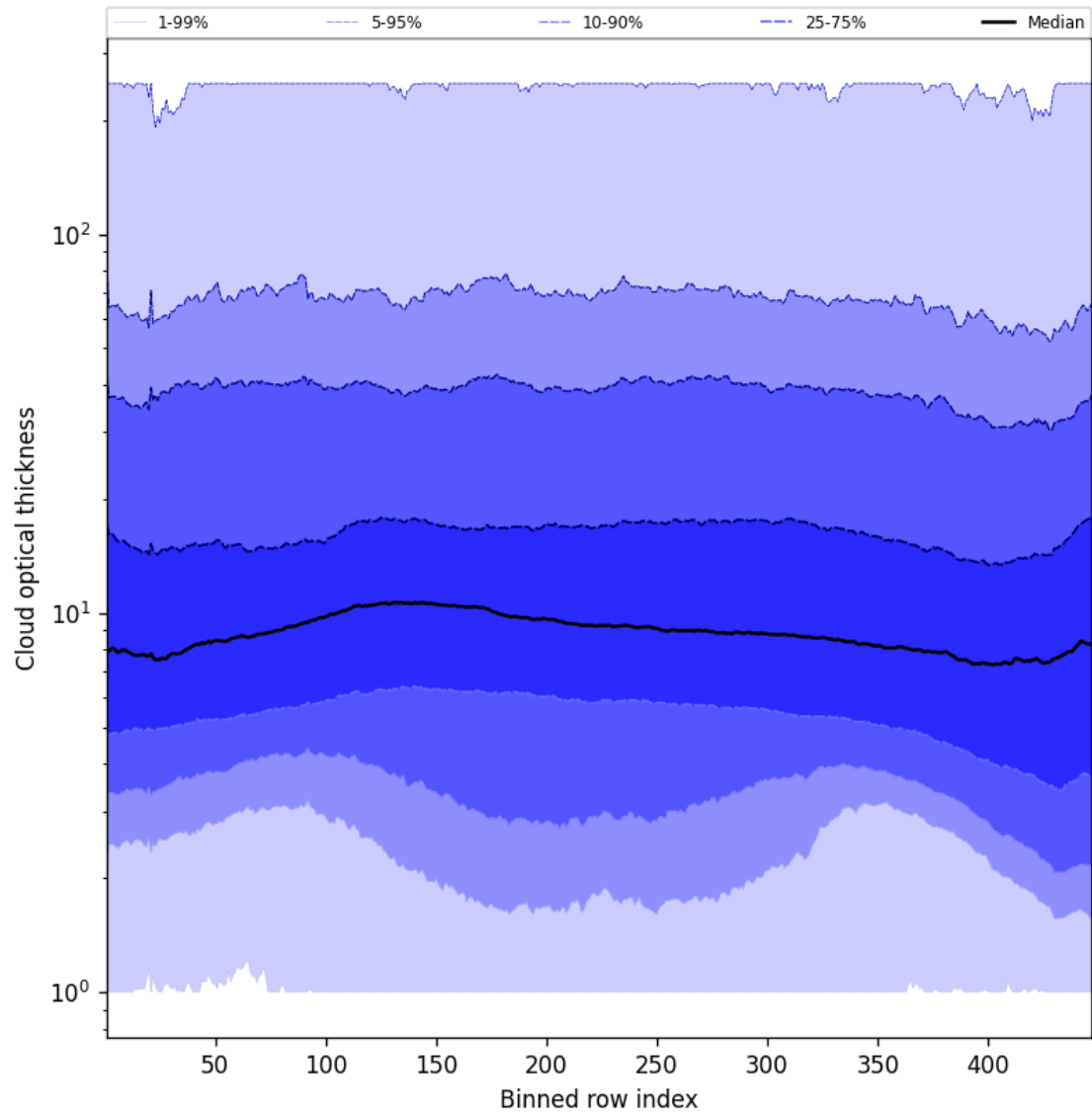
Figure 55: Along track statistics of “Cloud optical thickness” for 2024-12-04 to 2024-12-04
