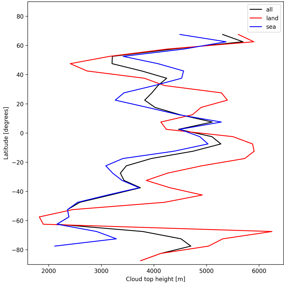
Figure 22: Zonal average of “Cloud top height” for 2024-12-04 to 2024-12-04.
