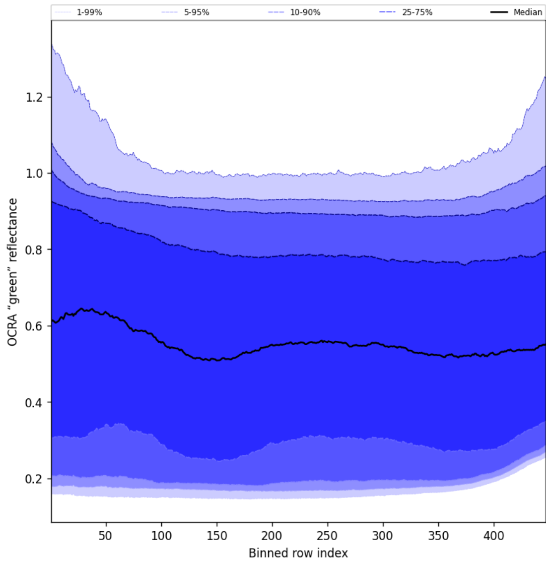
Figure 66: Along track statistics of “OCRA “green” reflectance” for 2024-12-04 to 2024-12-04
