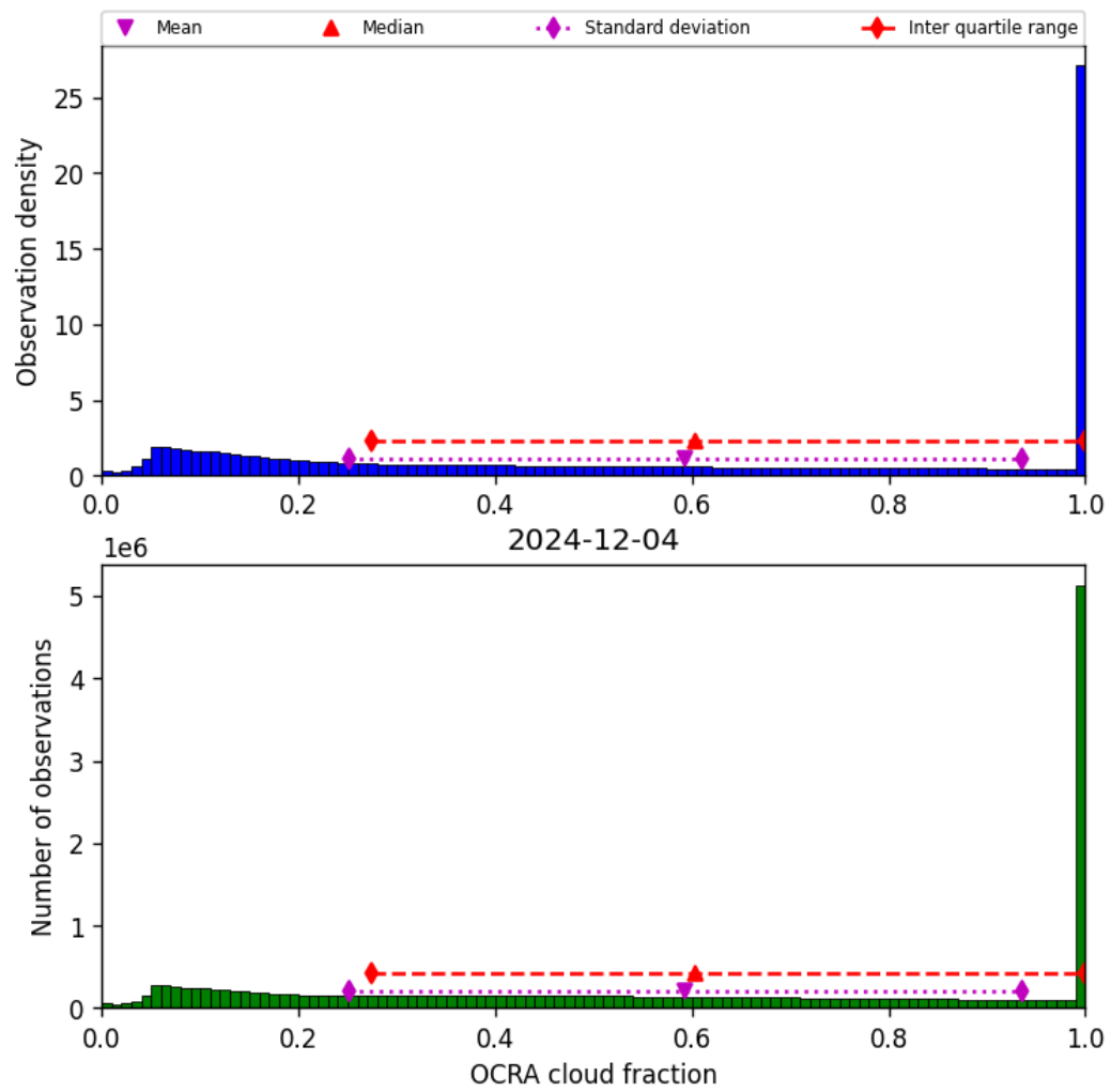
Figure 48: Histogram of “OCRA cloud fraction” for 2024-12-04 to 2024-12-04
