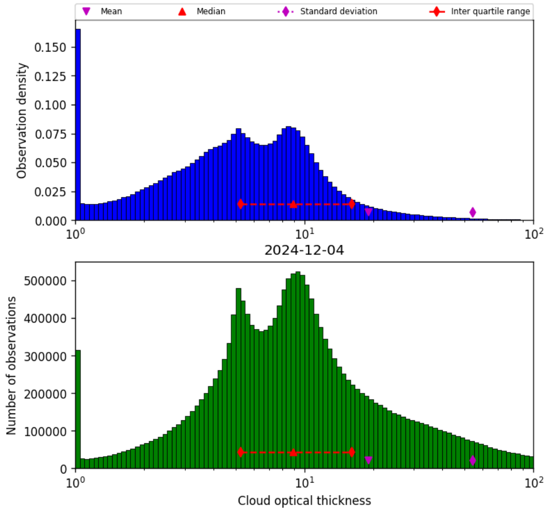
Figure 39: Histogram of “Cloud optical thickness” for 2024-12-04 to 2024-12-04
