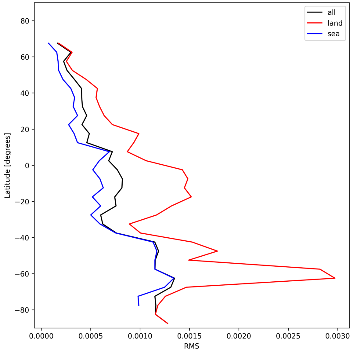
Figure 29: Zonal average of “RMS” for 2024-12-04 to 2024-12-04.
