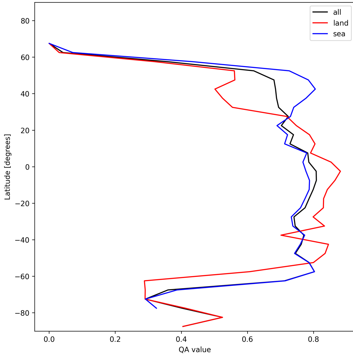
Figure 20: Zonal average of “QA value” for 2024-12-04 to 2024-12-04.
