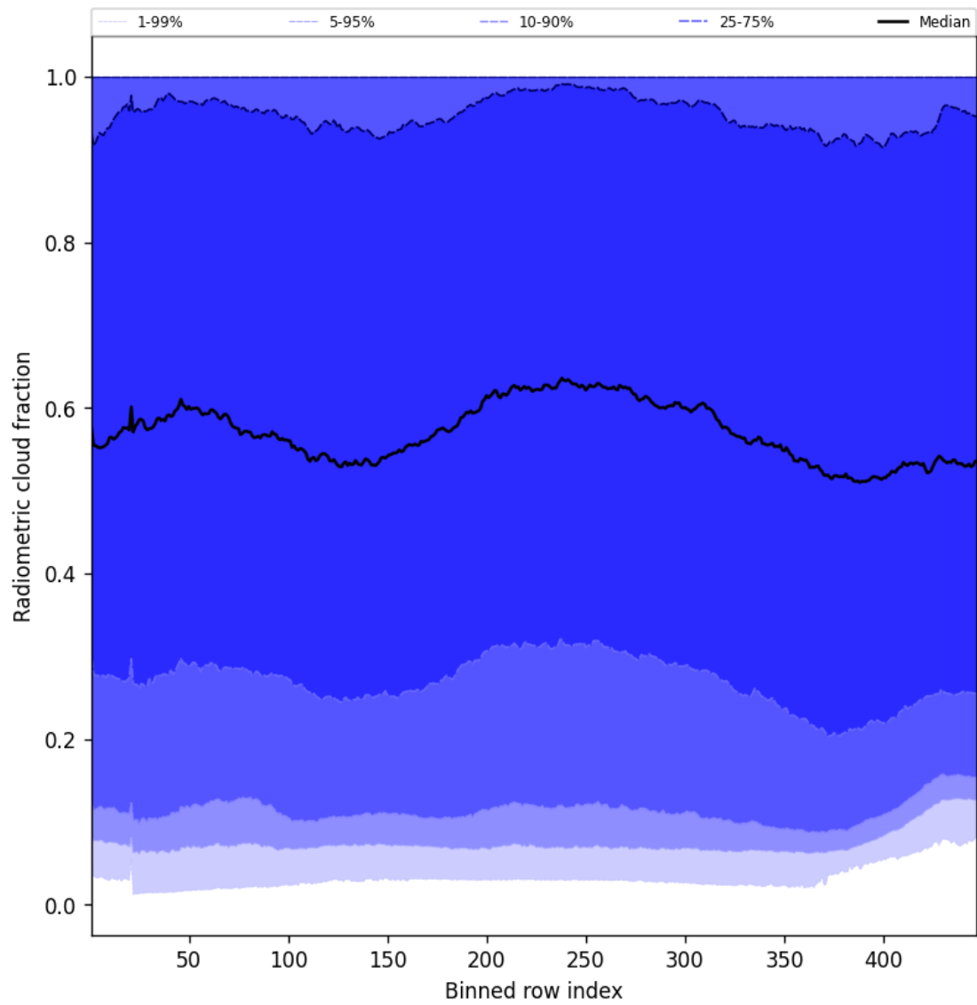
Figure 53: Along track statistics of “Radiometric cloud fraction” for 2024-12-06 to 2024-12-07
