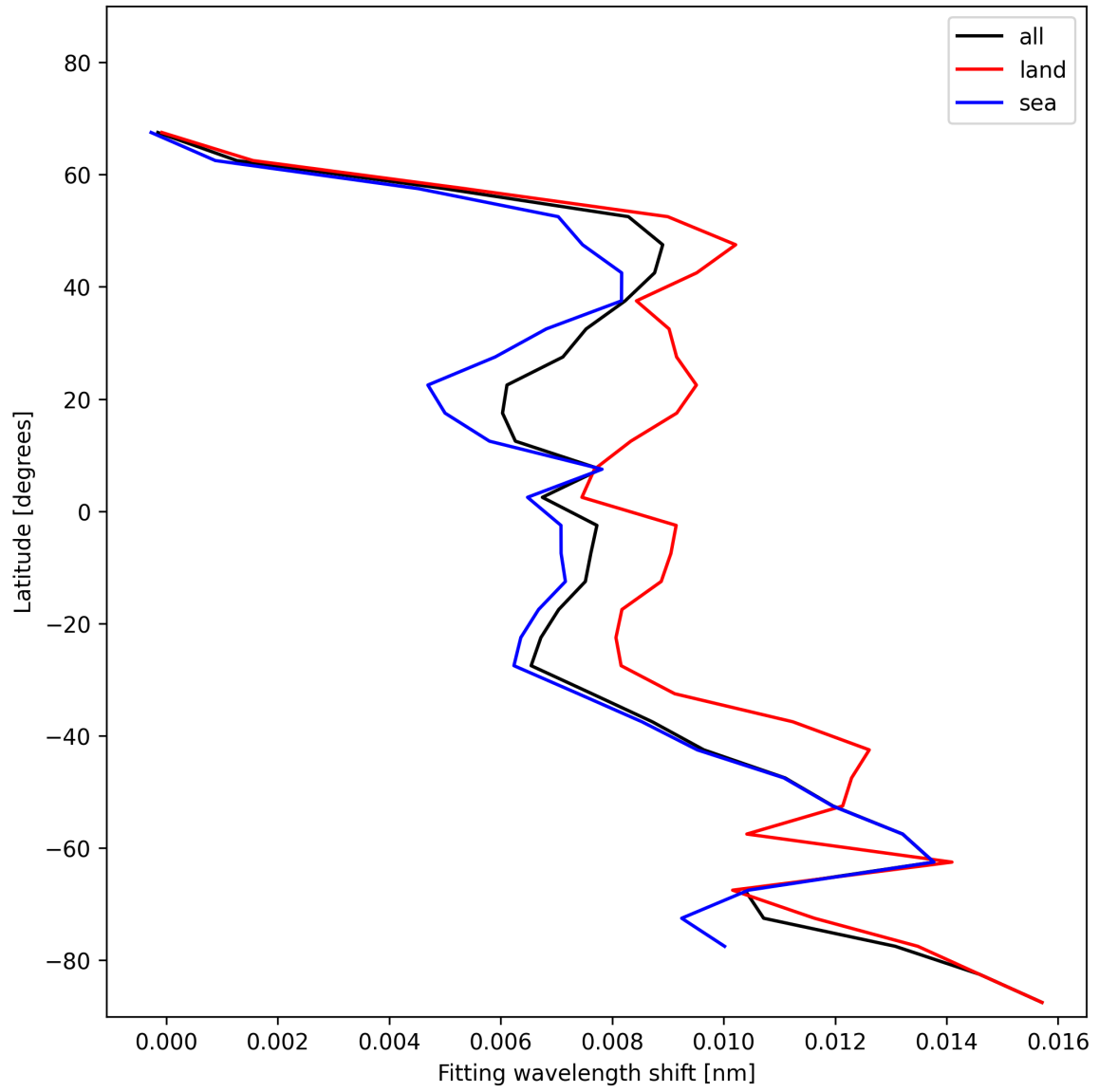
Figure 31: Zonal average of “Fitting wavelength shift” for 2024-12-06 to 2024-12-07.
