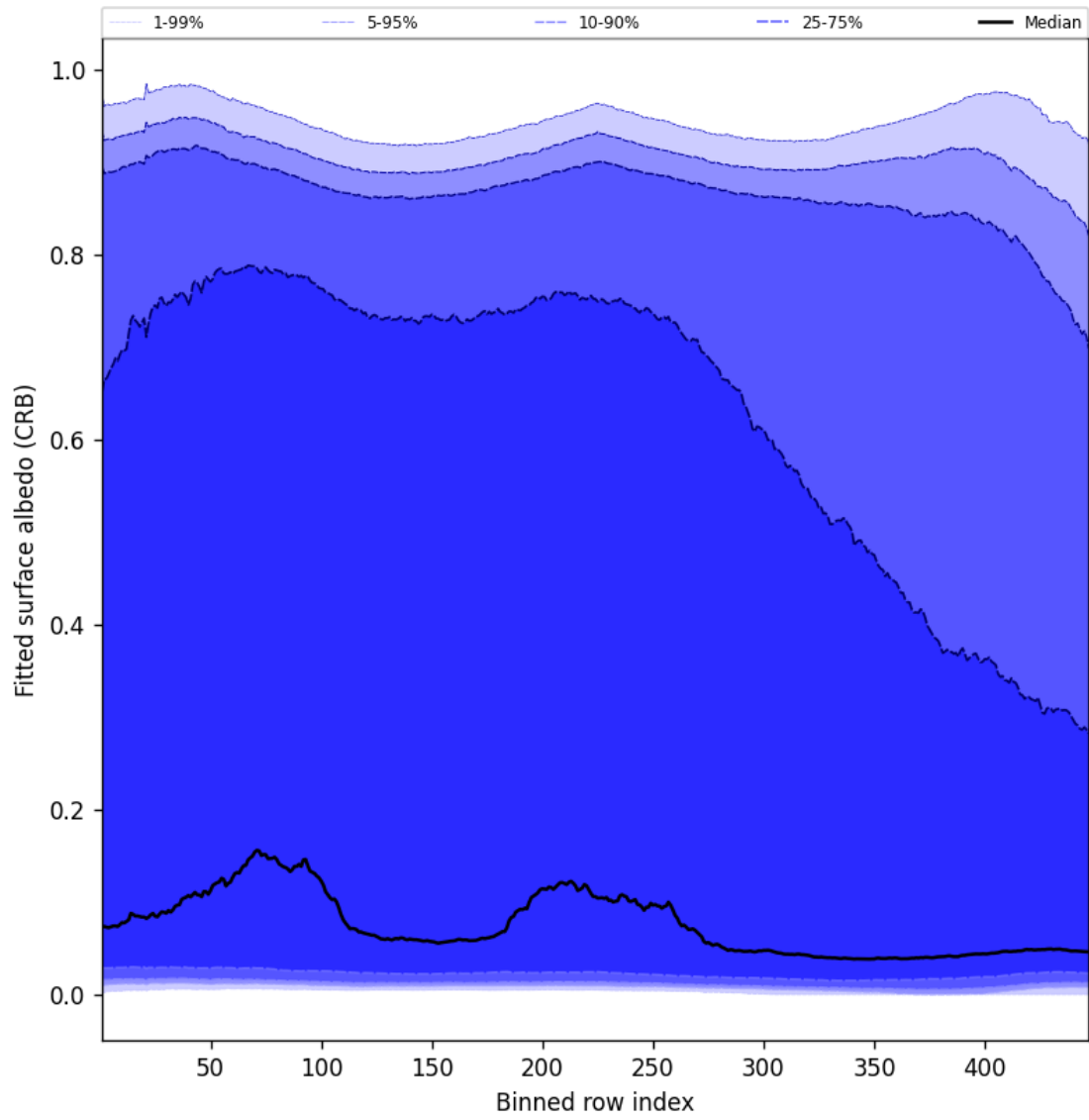
Figure 60: Along track statistics of “Fitted surface albedo (CRB)” for 2024-12-06 to 2024-12-07
