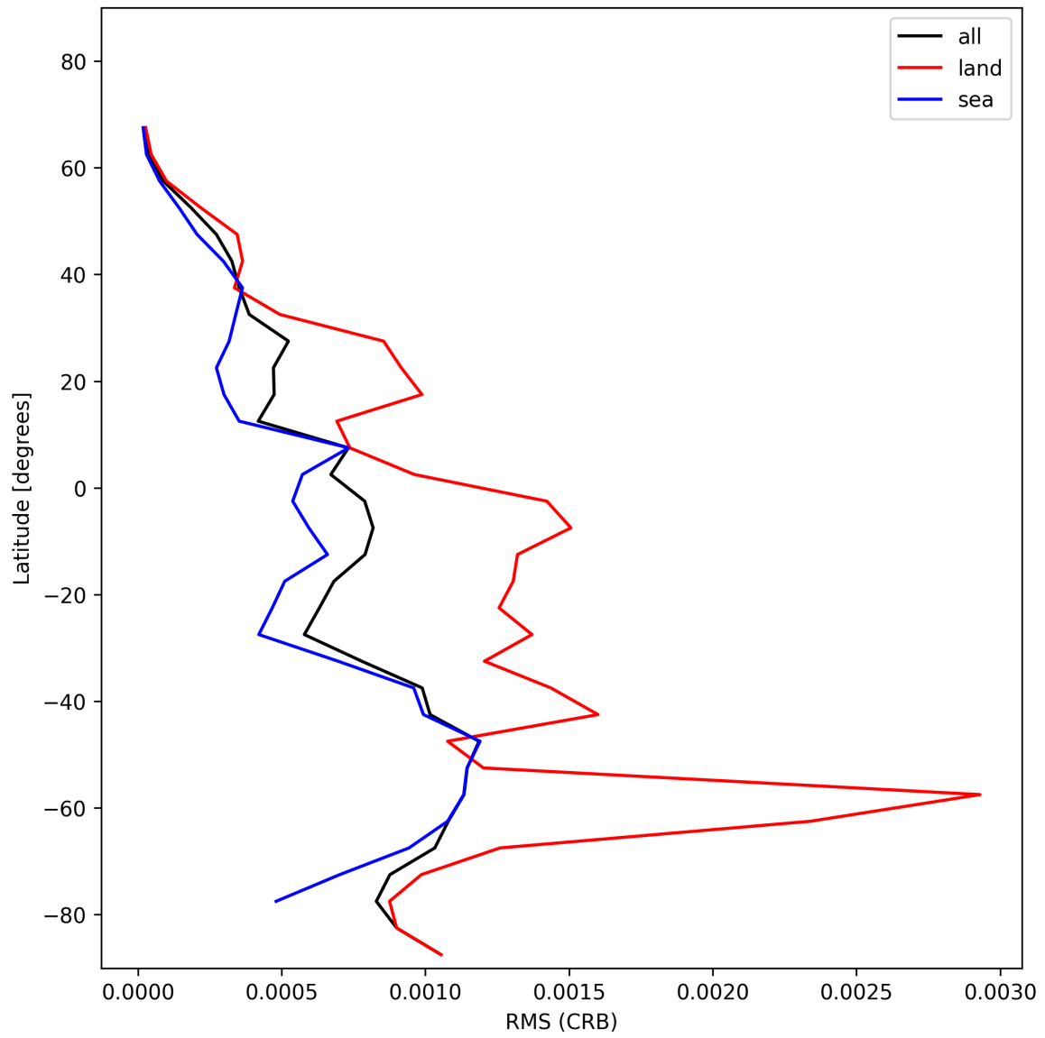
Figure 30: Zonal average of “RMS (CRB)” for 2024-12-06 to 2024-12-07.
