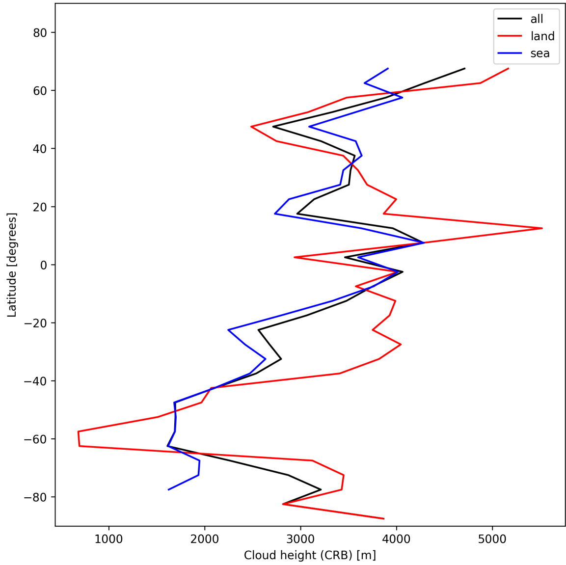
Figure 25: Zonal average of “Cloud height (CRB)” for 2024-12-06 to 2024-12-07.
