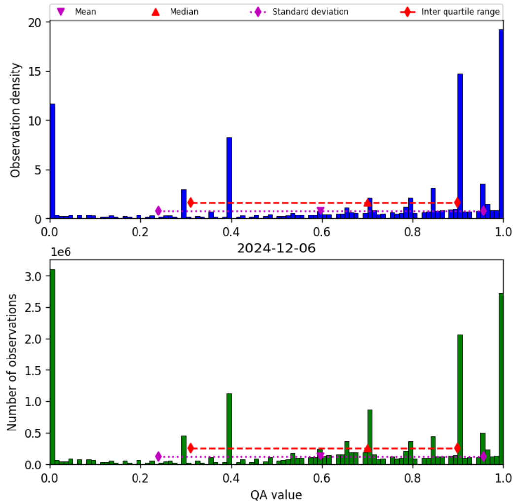
Figure 36: Histogram of “QA value” for 2024-12-06 to 2024-12-07
