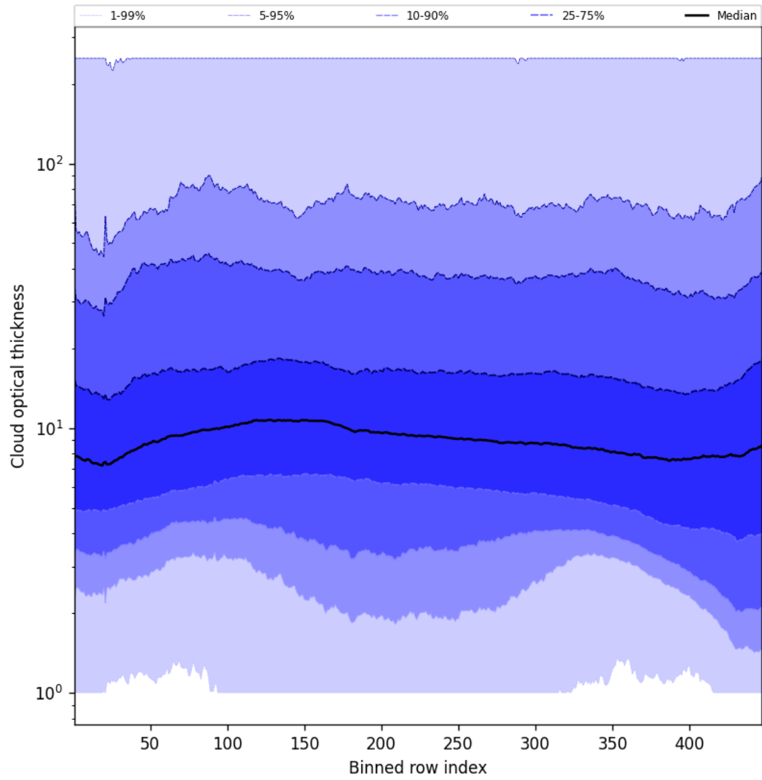
Figure 55: Along track statistics of “Cloud optical thickness” for 2024-12-06 to 2024-12-07
