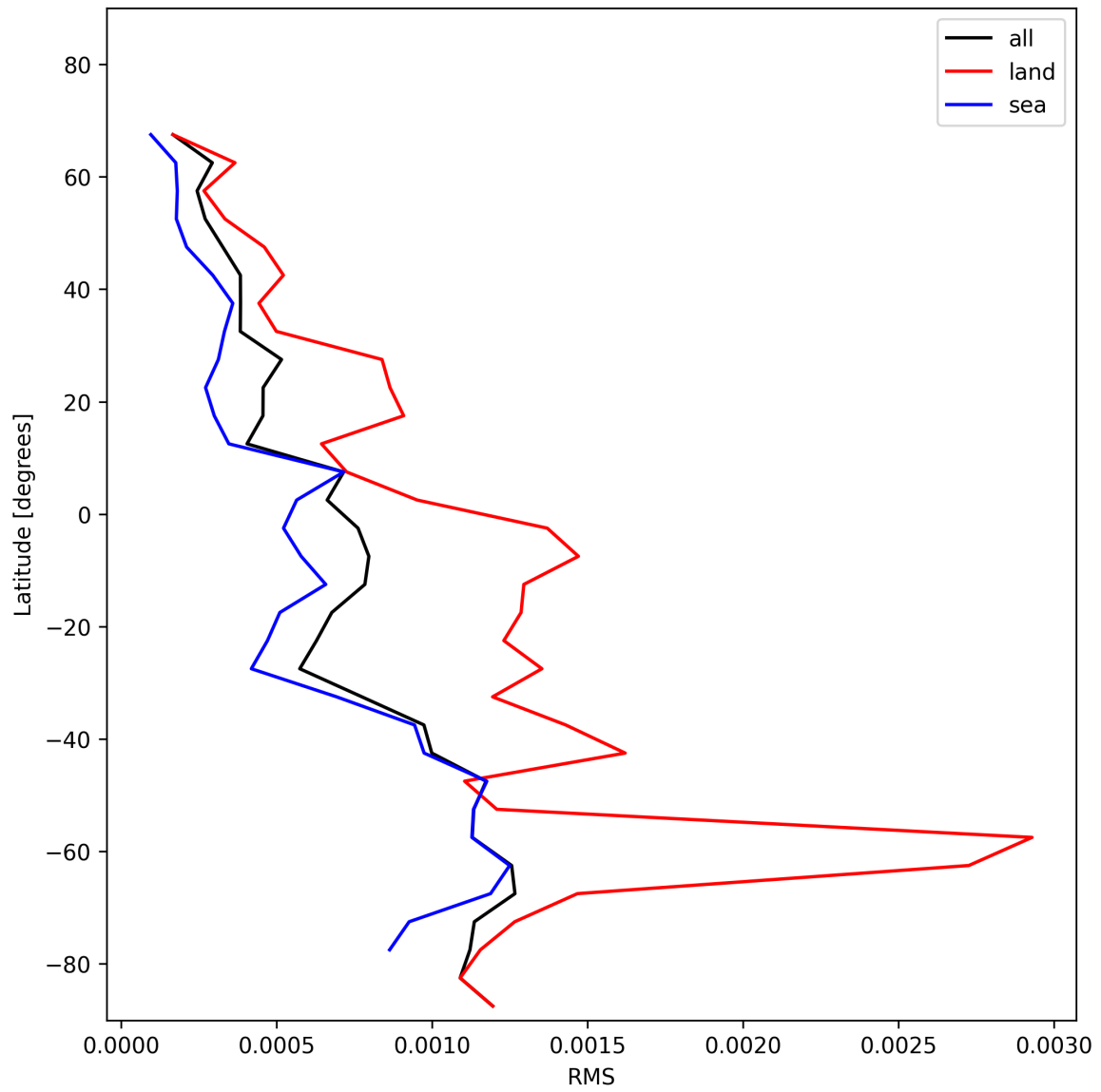
Figure 29: Zonal average of “RMS” for 2024-12-06 to 2024-12-07.
