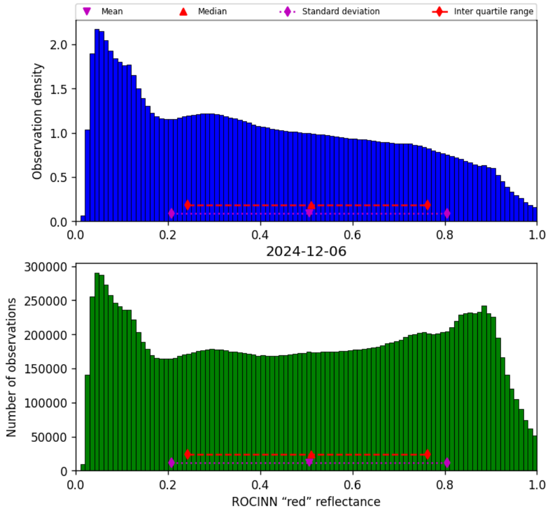
Figure 51: Histogram of “ROCINN “red” reflectance” for 2024-12-06 to 2024-12-07
