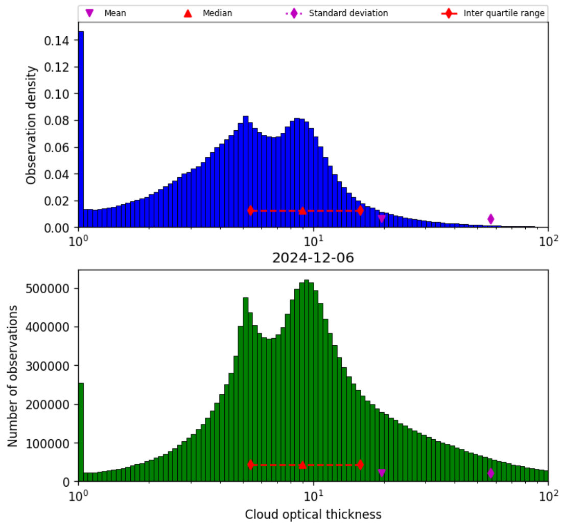
Figure 39: Histogram of “Cloud optical thickness” for 2024-12-06 to 2024-12-07
