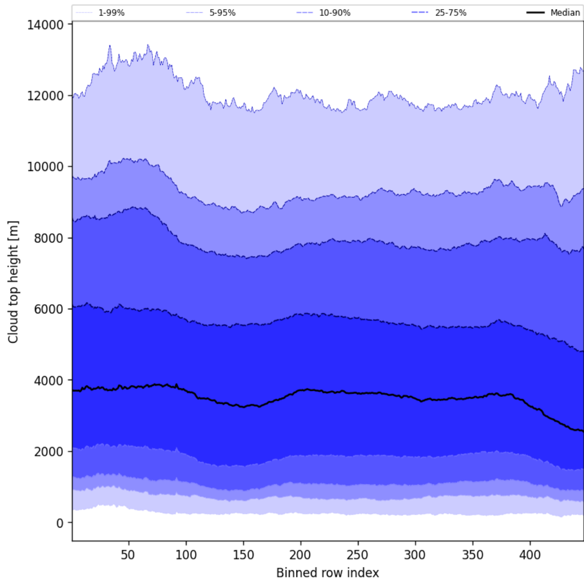
Figure 54: Along track statistics of “Cloud top height” for 2024-12-06 to 2024-12-07
