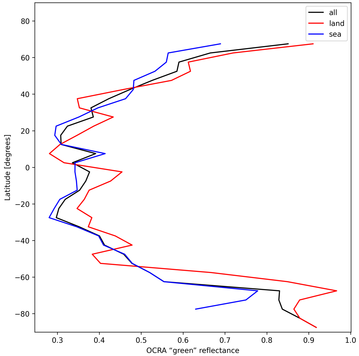
Figure 34: Zonal average of “OCRA “green” reflectance” for 2024-12-06 to 2024-12-07.
