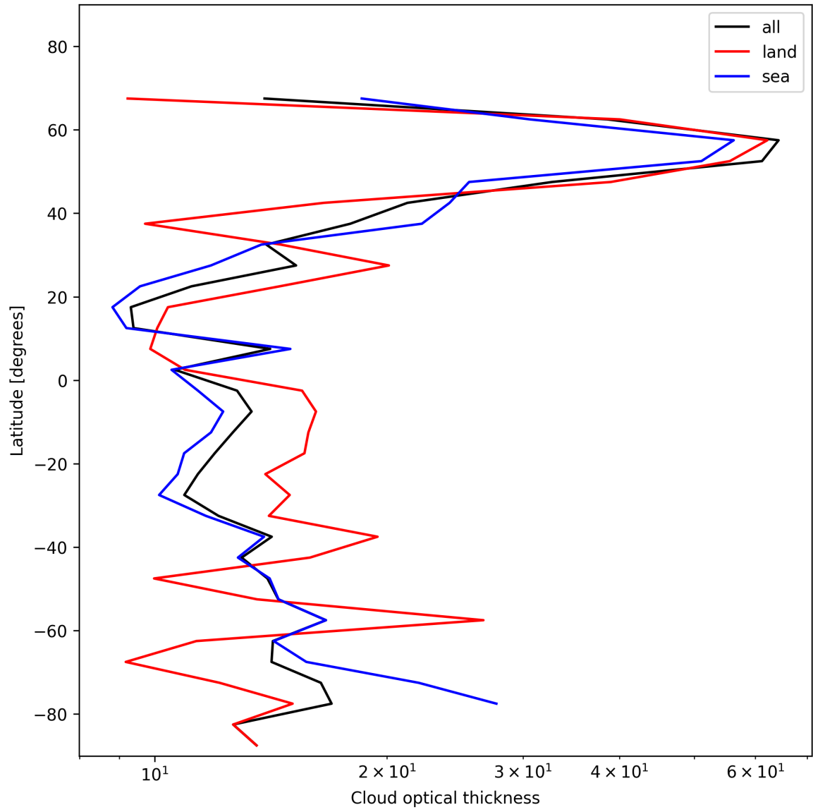
Figure 23: Zonal average of “Cloud optical thickness” for 2024-12-06 to 2024-12-07.
