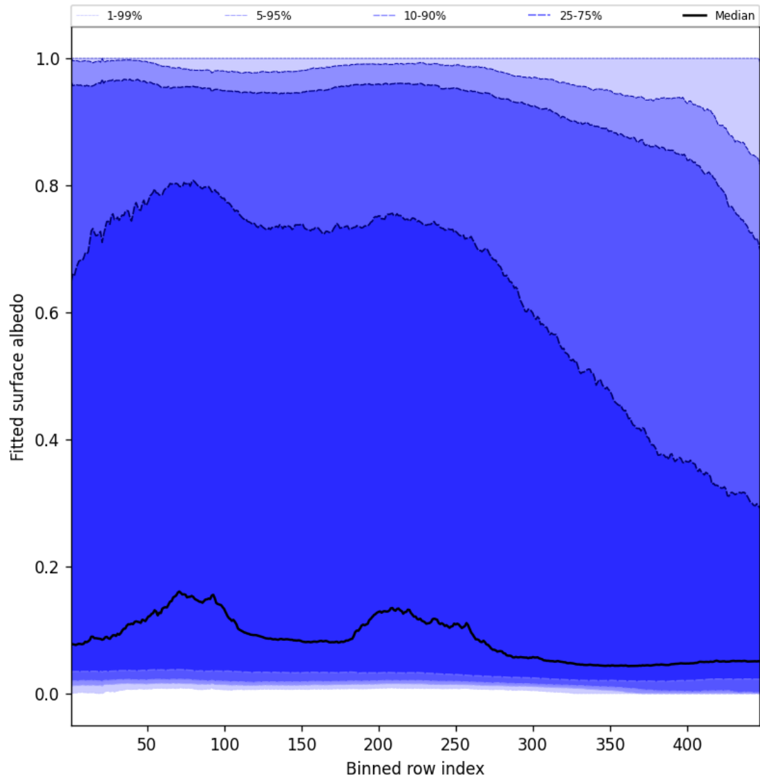
Figure 59: Along track statistics of “Fitted surface albedo” for 2024-12-06 to 2024-12-07
