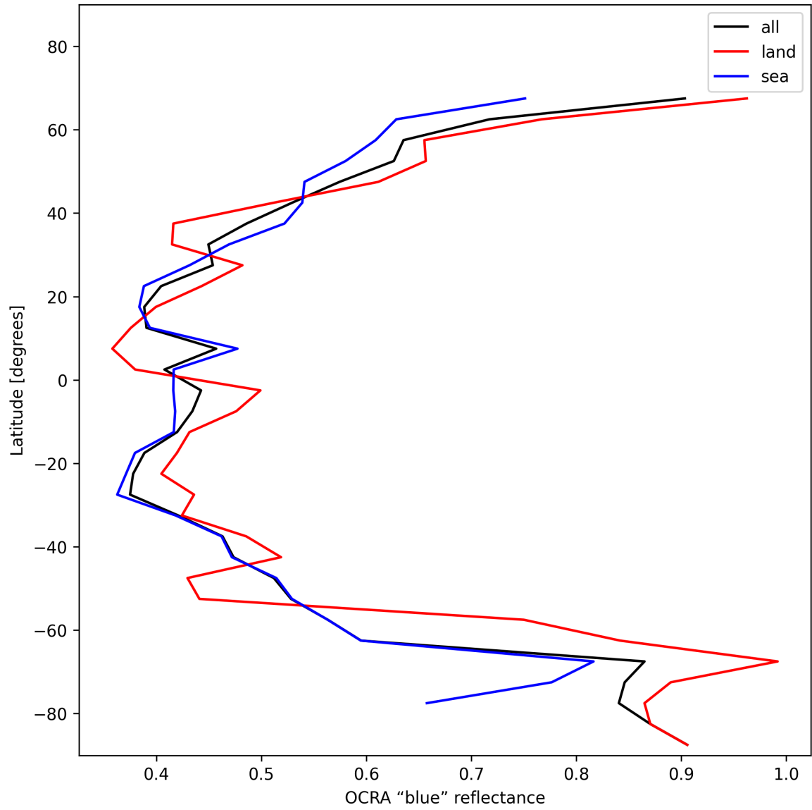
Figure 33: Zonal average of “OCRA “blue” reflectance” for 2024-12-06 to 2024-12-07.
