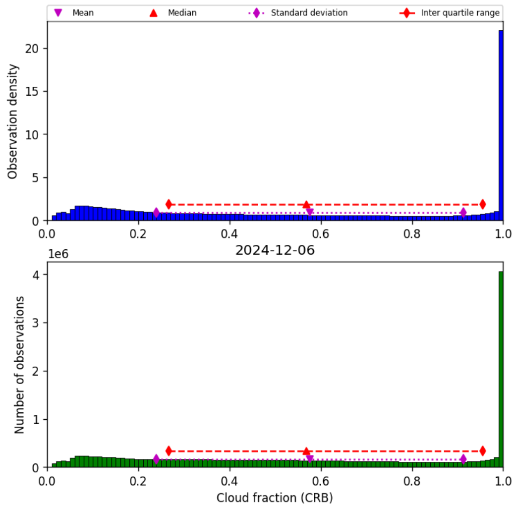
Figure 40: Histogram of “Cloud fraction (CRB)” for 2024-12-06 to 2024-12-07
