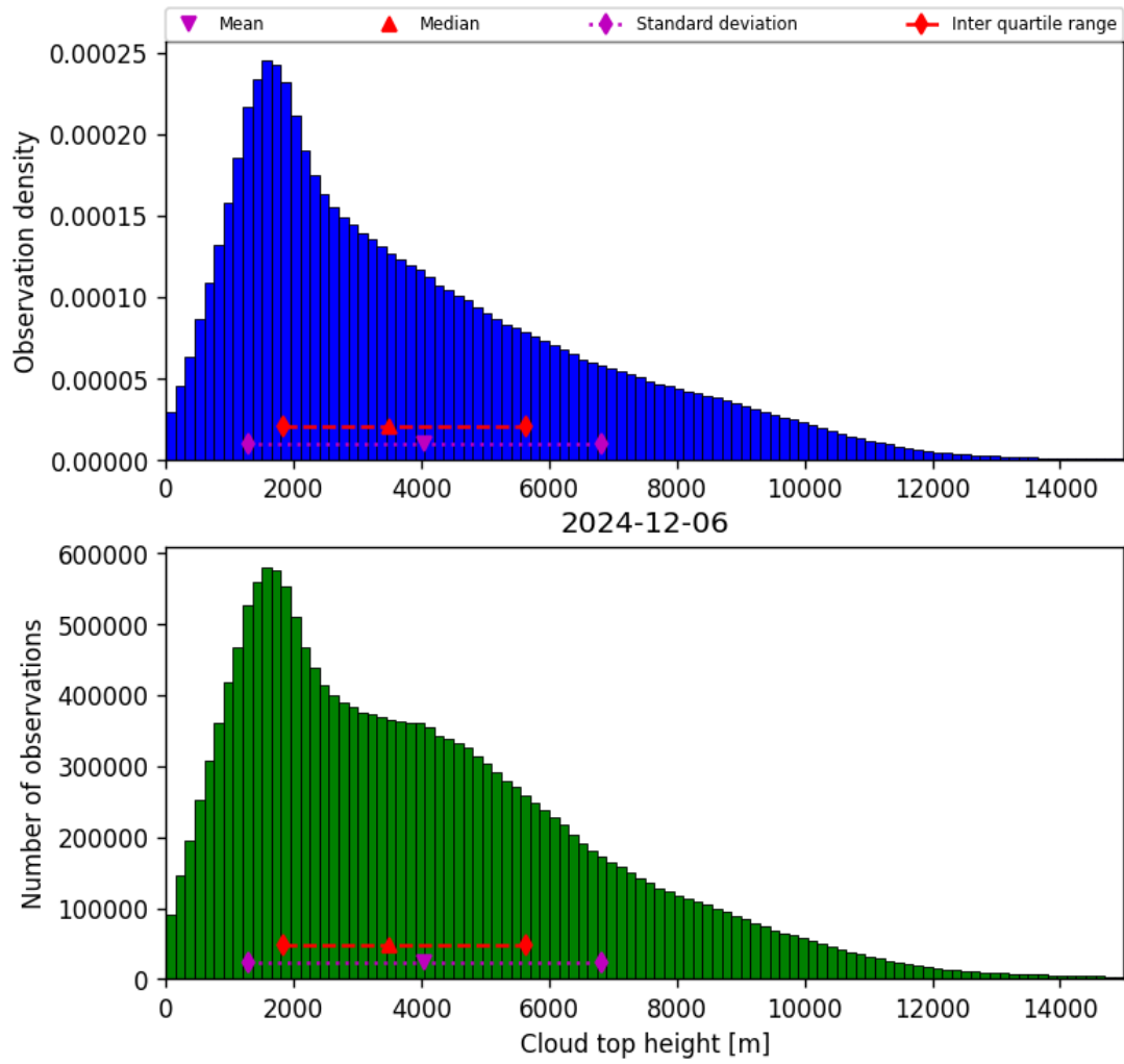
Figure 38: Histogram of “Cloud top height” for 2024-12-06 to 2024-12-07
