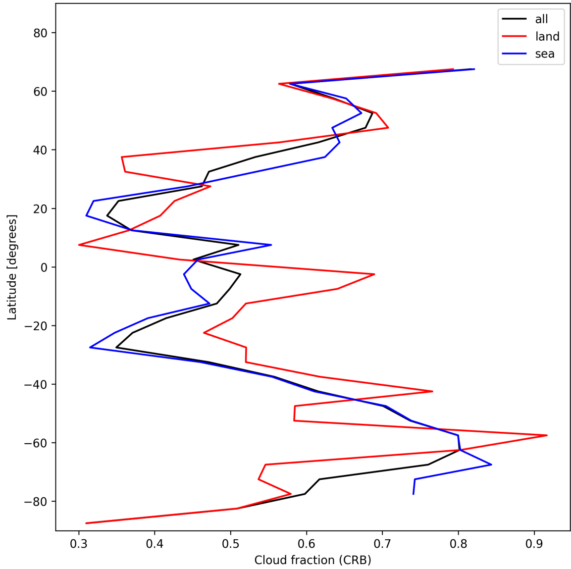
Figure 24: Zonal average of “Cloud fraction (CRB)” for 2024-12-06 to 2024-12-07.
