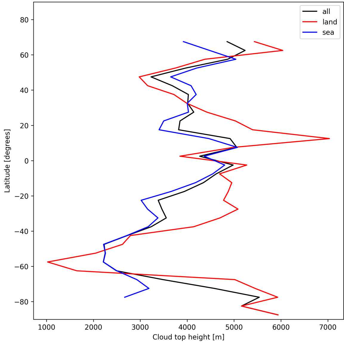
Figure 22: Zonal average of “Cloud top height” for 2024-12-06 to 2024-12-07.
