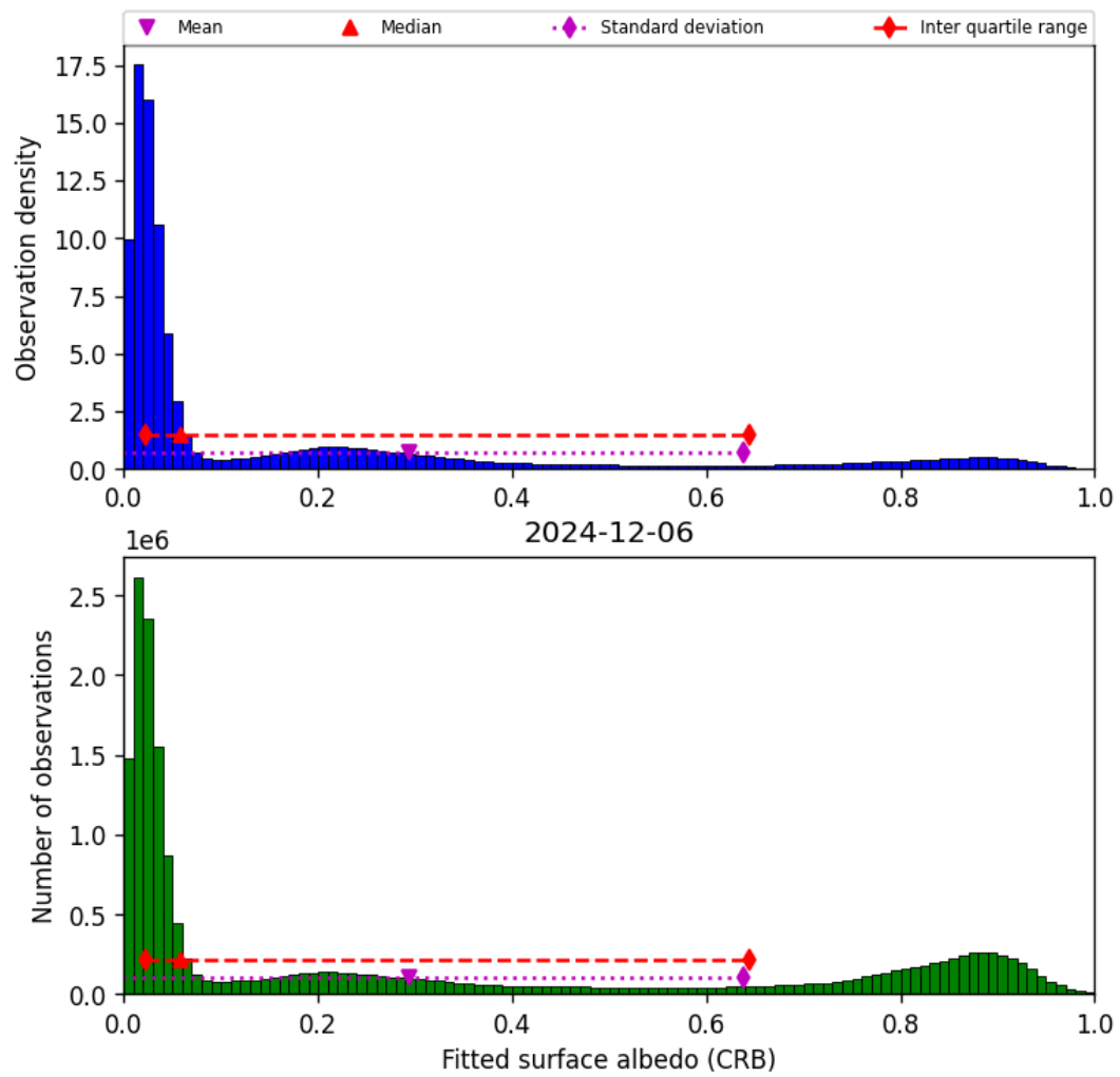
Figure 44: Histogram of “Fitted surface albedo (CRB)” for 2024-12-06 to 2024-12-07
