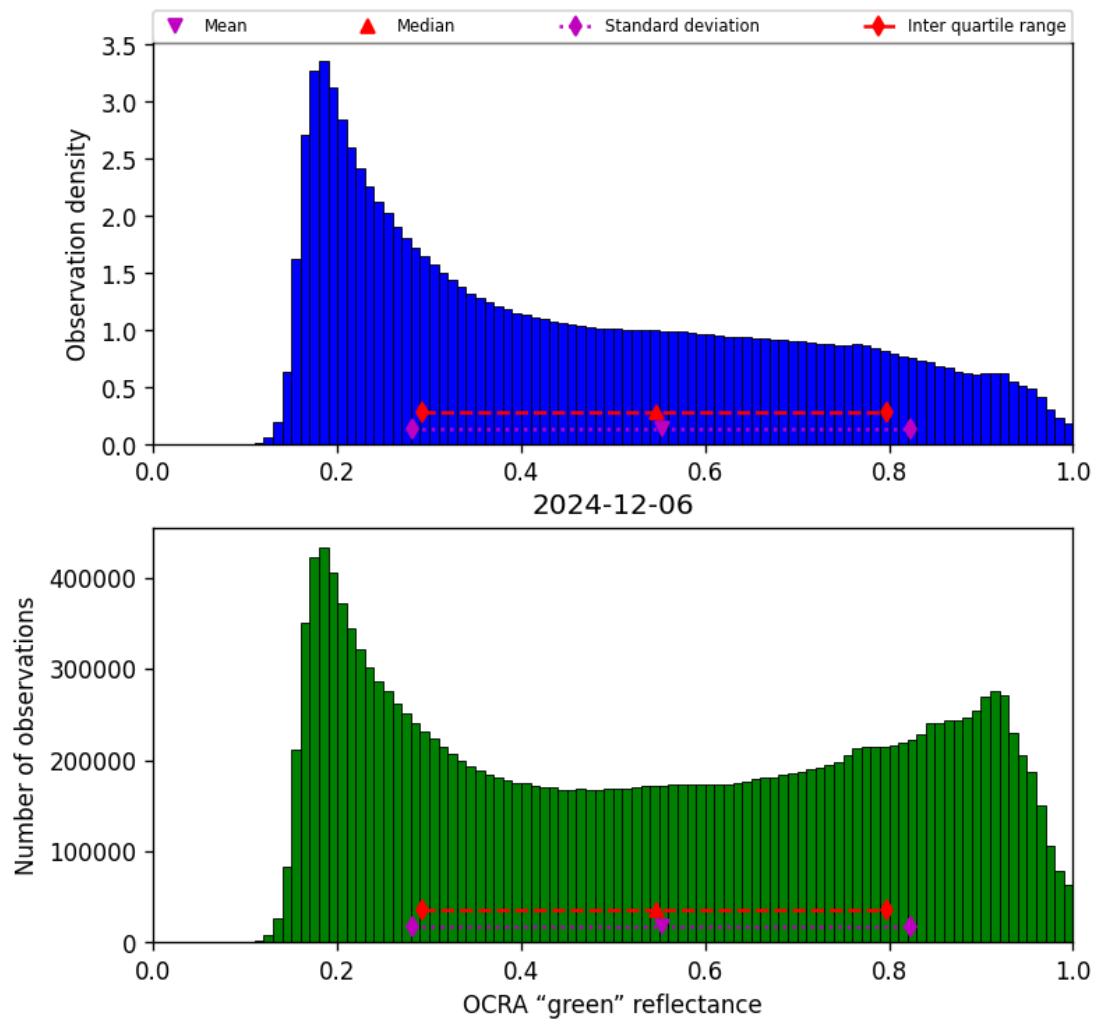
Figure 50: Histogram of “OCRA “green” reflectance” for 2024-12-06 to 2024-12-07
