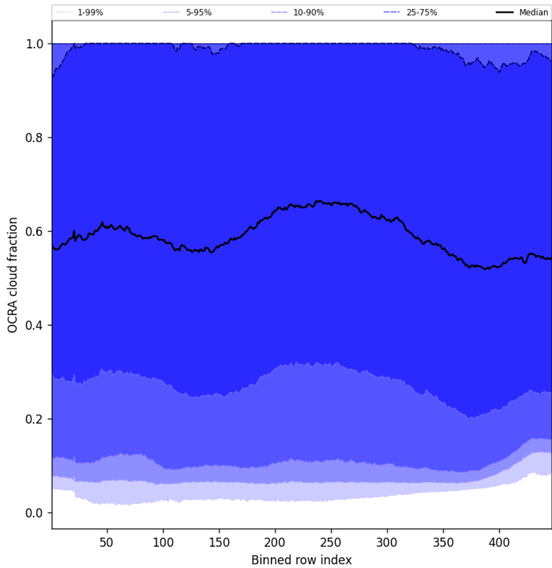
Figure 64: Along track statistics of “OCRA cloud fraction” for 2024-12-06 to 2024-12-07
