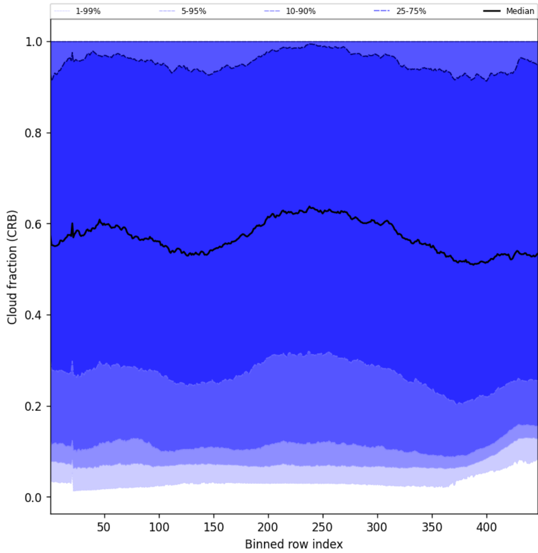
Figure 56: Along track statistics of “Cloud fraction (CRB)” for 2024-12-06 to 2024-12-07
