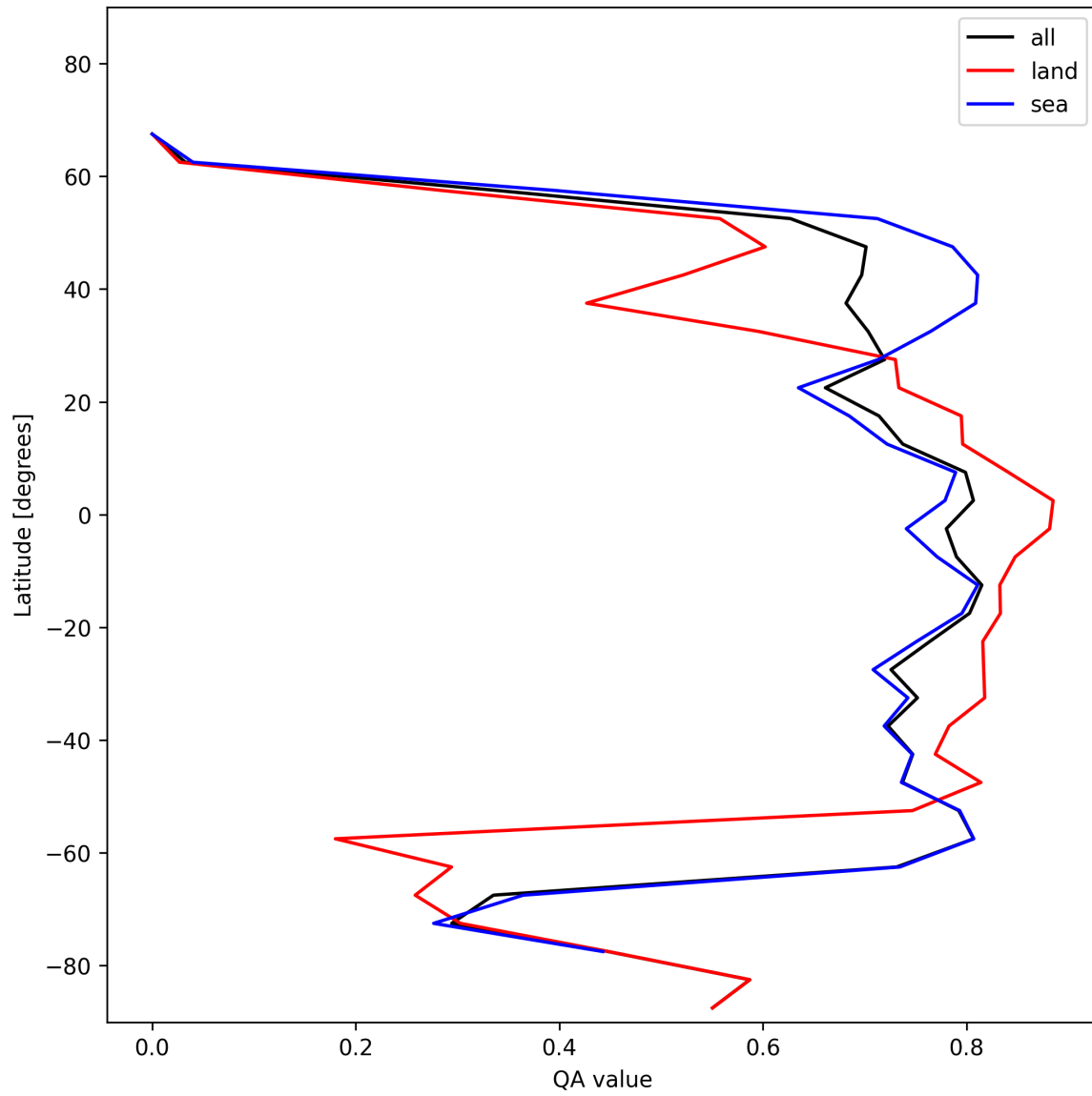
Figure 20: Zonal average of “QA value” for 2024-12-06 to 2024-12-07.
