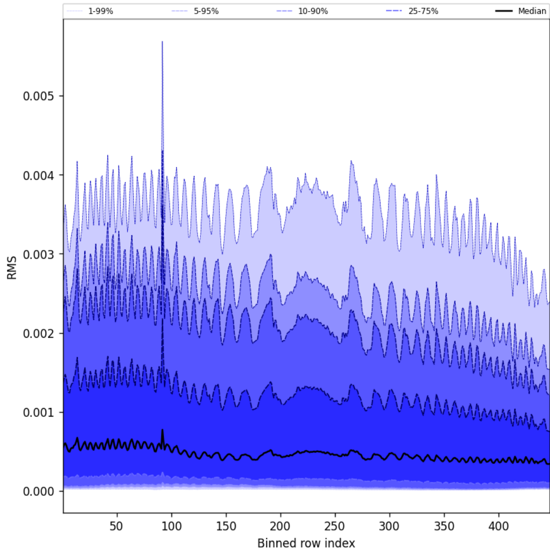
Figure 61: Along track statistics of “RMS” for 2024-12-06 to 2024-12-07
