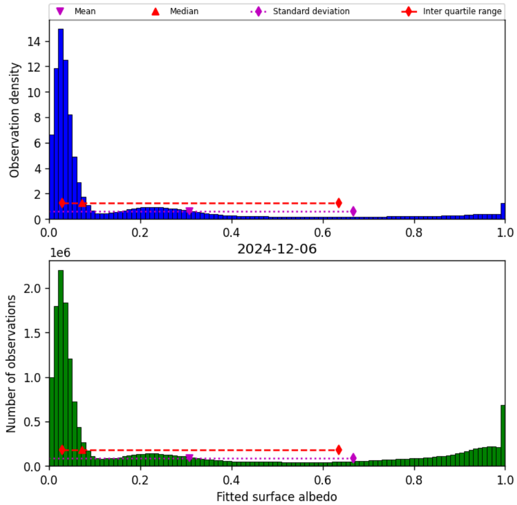
Figure 43: Histogram of “Fitted surface albedo” for 2024-12-06 to 2024-12-07
