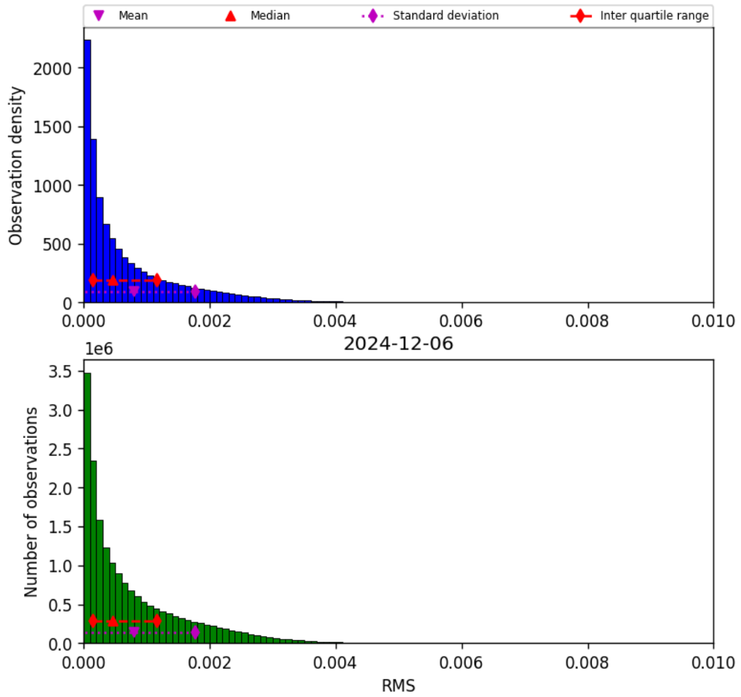
Figure 45: Histogram of “RMS” for 2024-12-06 to 2024-12-07
