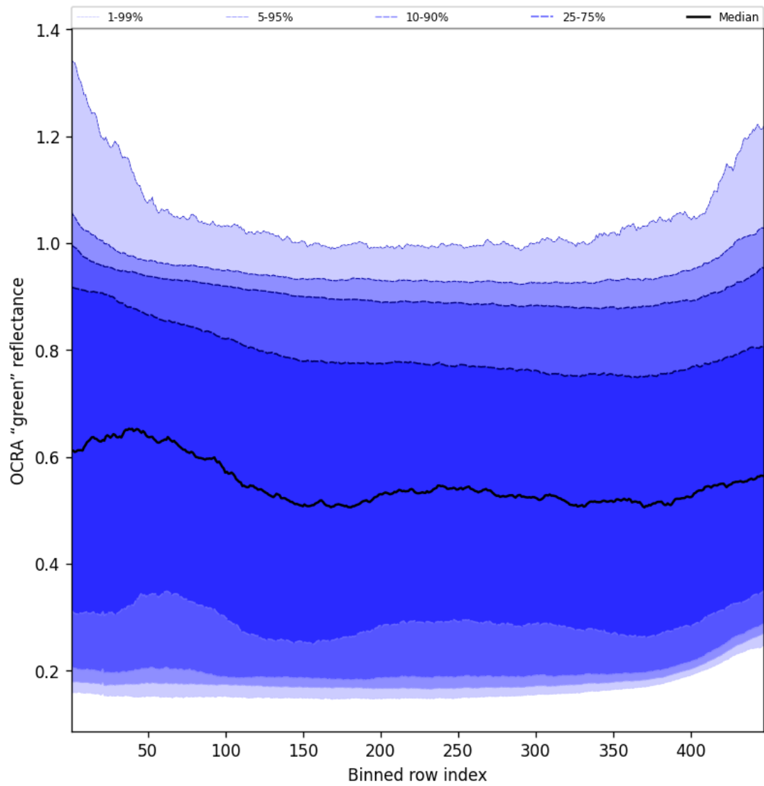
Figure 66: Along track statistics of “OCRA “green” reflectance” for 2024-12-06 to 2024-12-07
