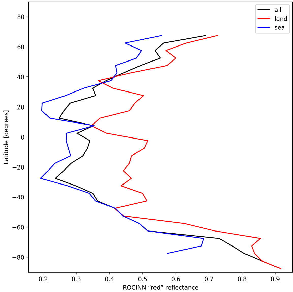
Figure 35: Zonal average of “ROCINN “red” reflectance” for 2024-12-06 to 2024-12-07.
