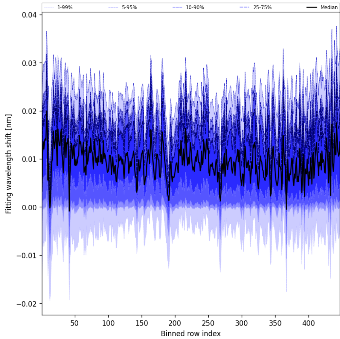
Figure 63: Along track statistics of “Fitting wavelength shift” for 2024-12-06 to 2024-12-07
