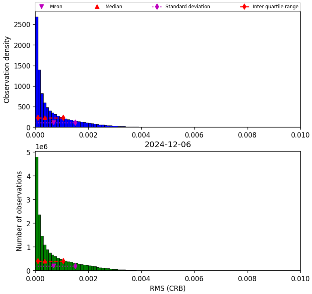
Figure 46: Histogram of “RMS (CRB)” for 2024-12-06 to 2024-12-07
