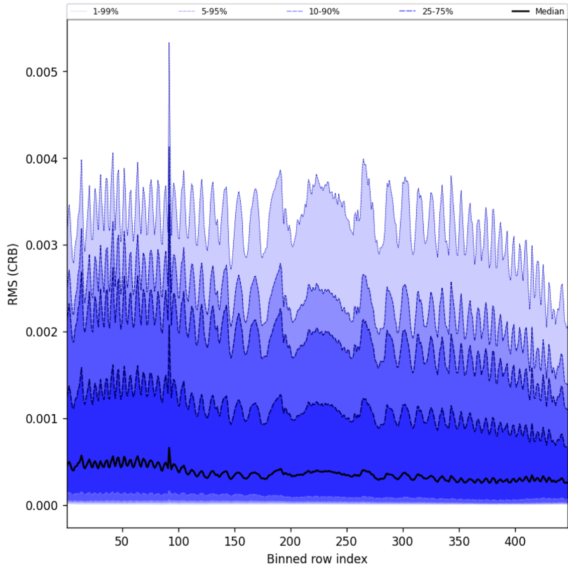
Figure 62: Along track statistics of “RMS (CRB)” for 2024-12-06 to 2024-12-07
