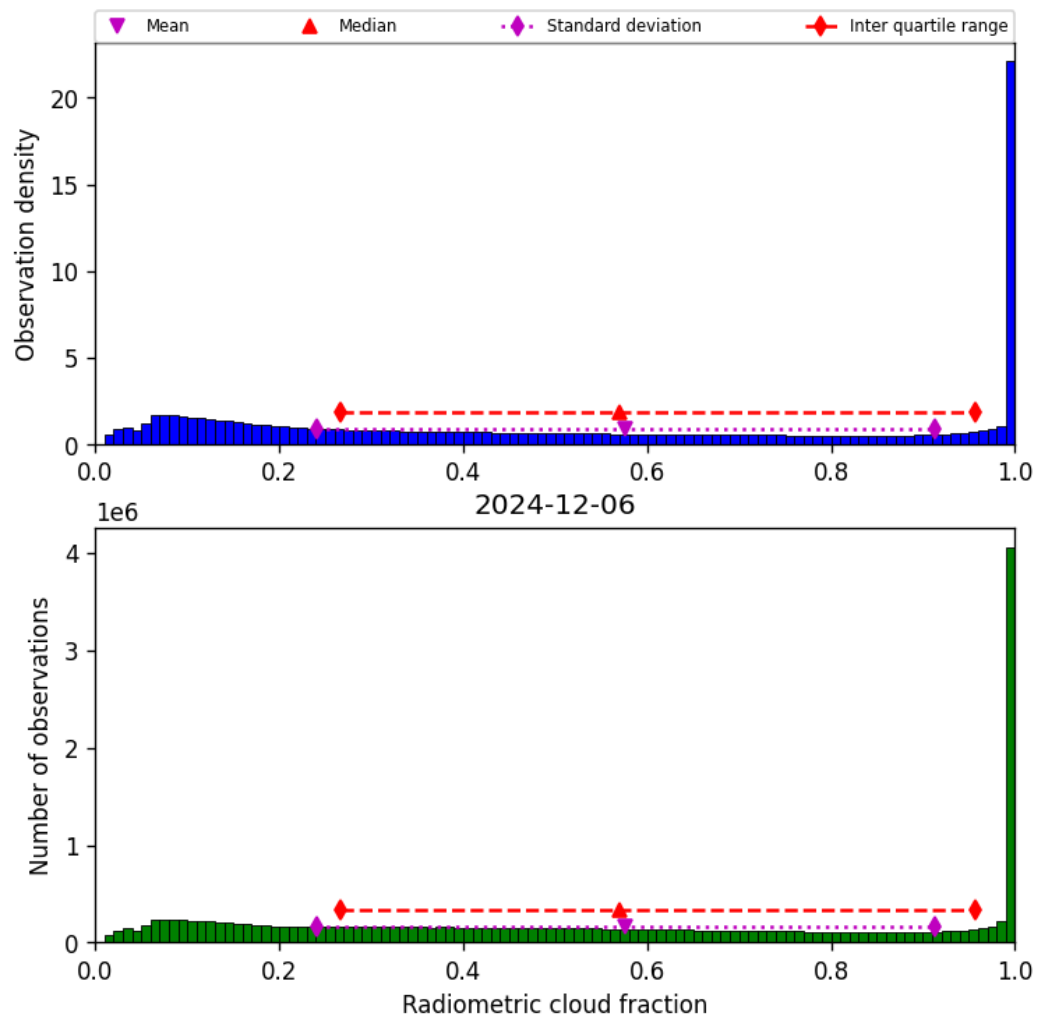
Figure 37: Histogram of “Radiometric cloud fraction” for 2024-12-06 to 2024-12-07
