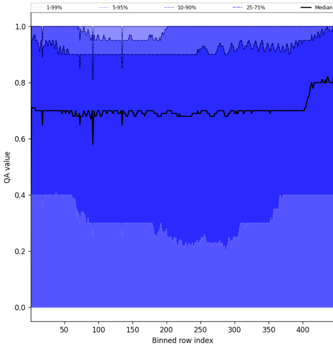
Figure 52: Along track statistics of “QA value” for 2024-12-06 to 2024-12-07
