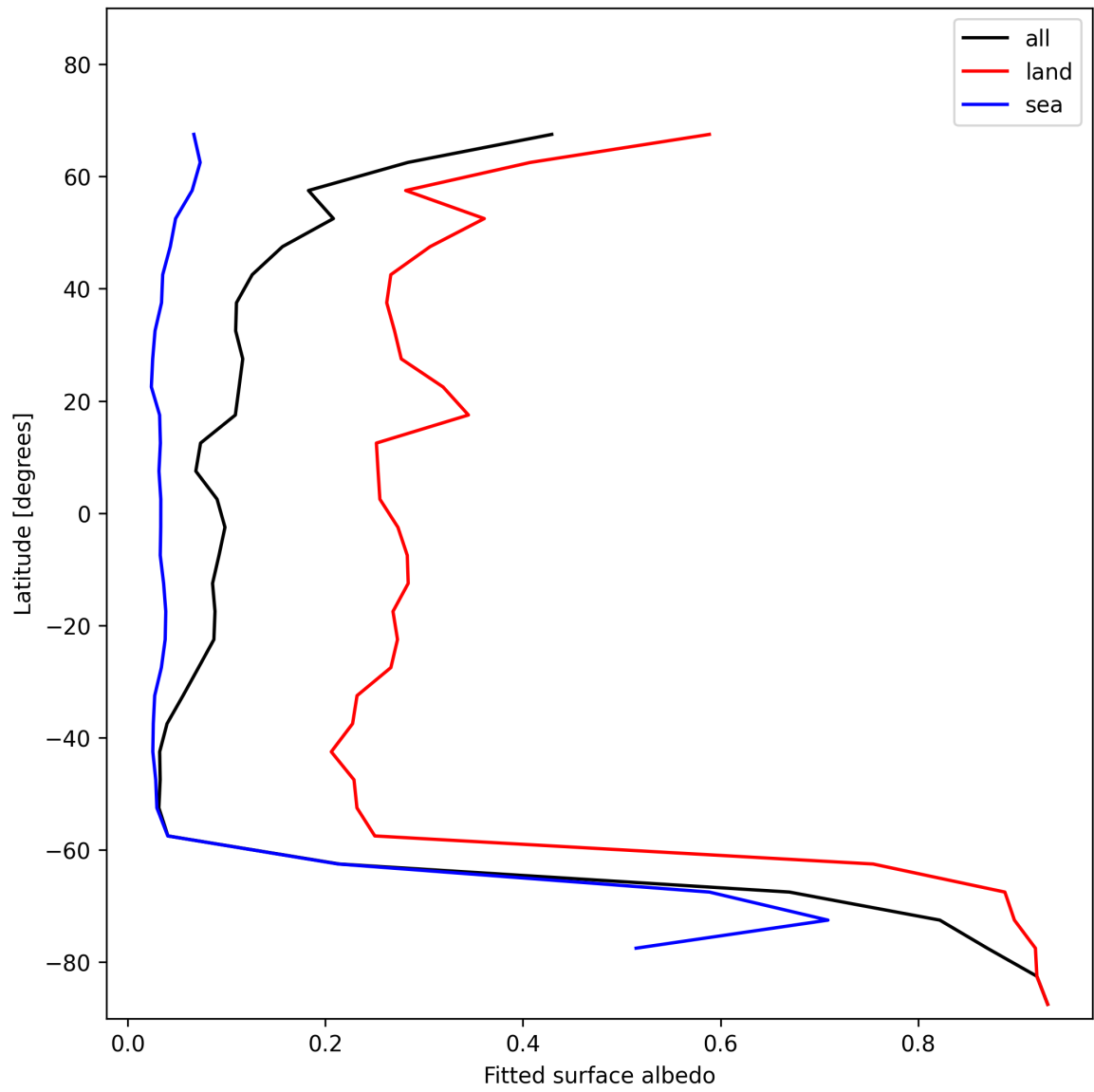
Figure 27: Zonal average of “Fitted surface albedo” for 2024-12-06 to 2024-12-07.
