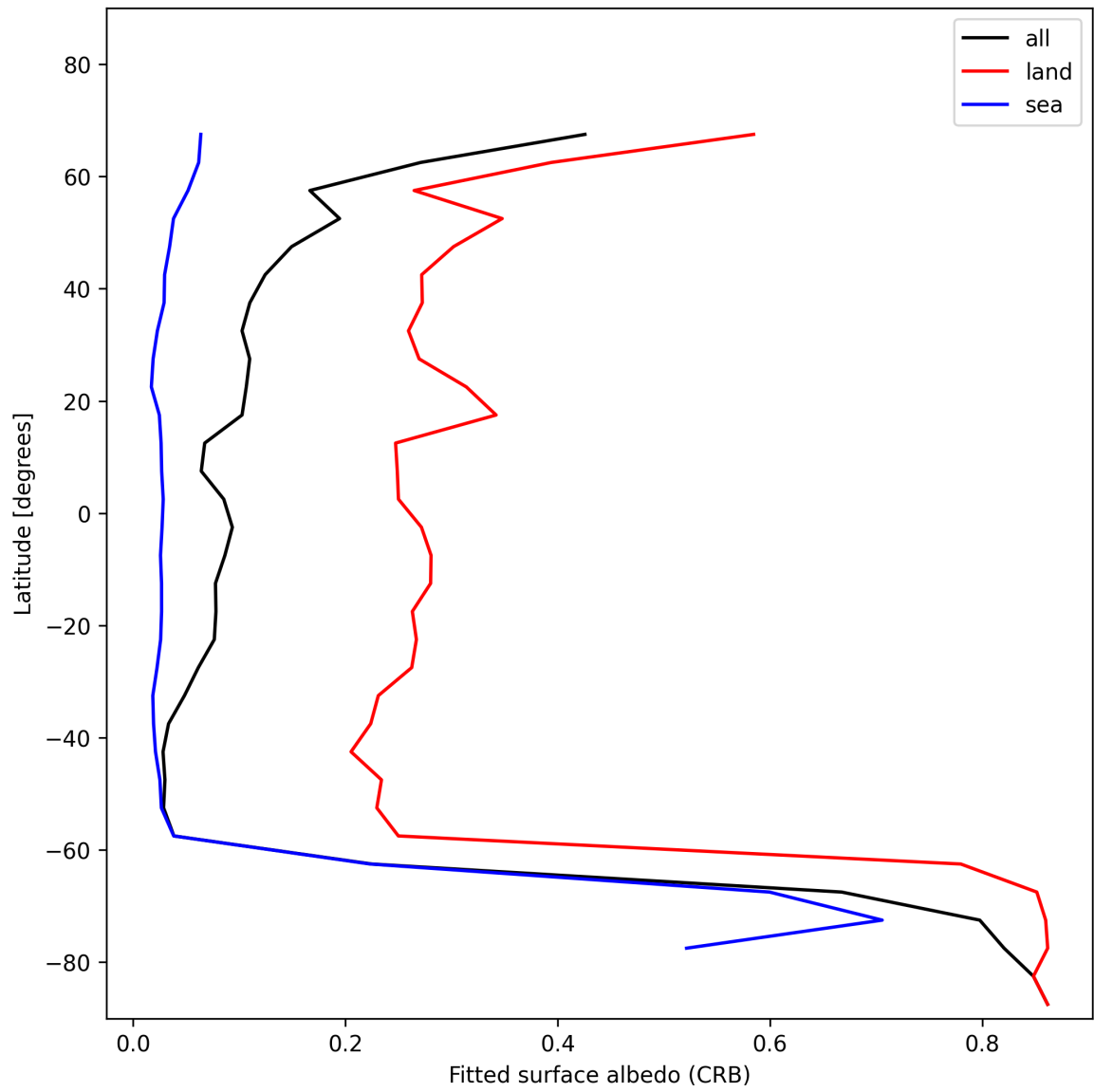
Figure 28: Zonal average of “Fitted surface albedo (CRB)” for 2024-12-06 to 2024-12-07.
