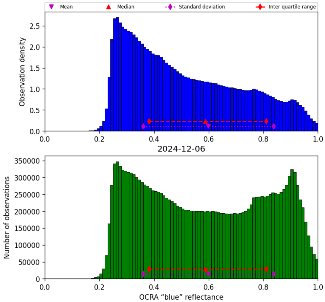
Figure 49: Histogram of “OCRA “blue” reflectance” for 2024-12-06 to 2024-12-07
