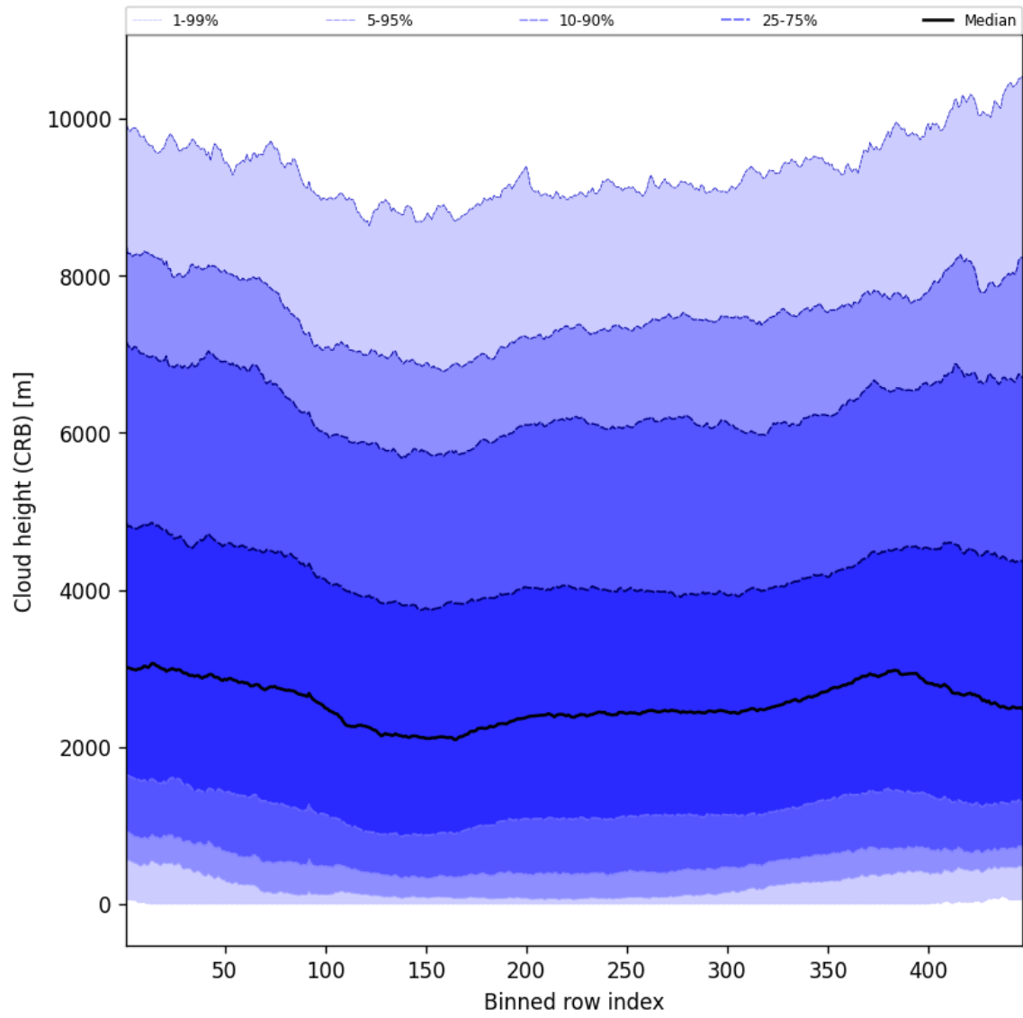
Figure 57: Along track statistics of “Cloud height (CRB)” for 2024-12-06 to 2024-12-07
