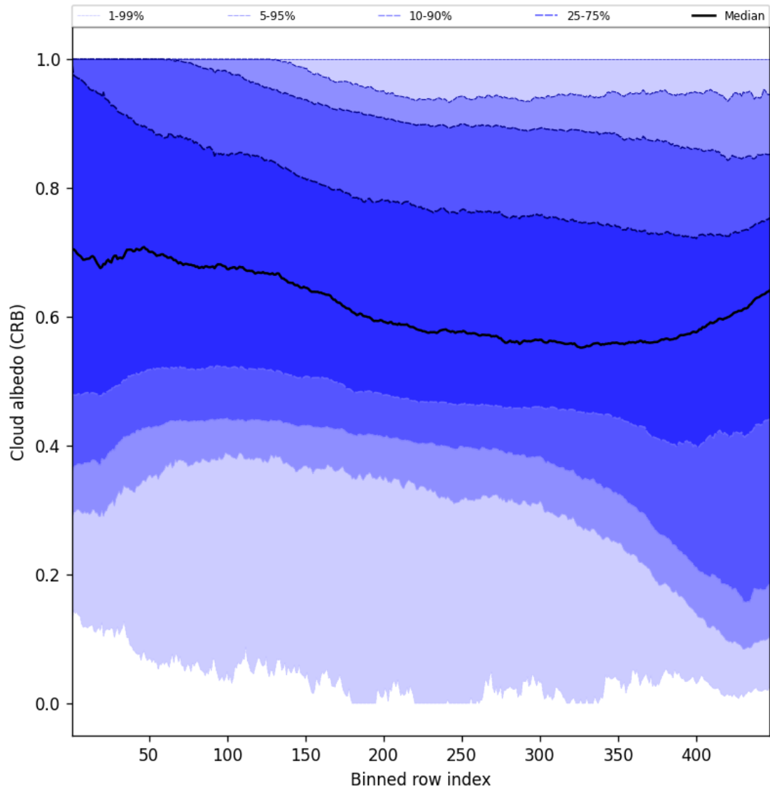
Figure 58: Along track statistics of “Cloud albedo (CRB)” for 2024-12-06 to 2024-12-07
