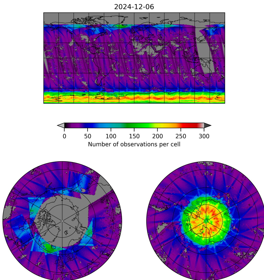
Figure 19: Map of the number of observations for 2024-12-06 to 2024-12-07
