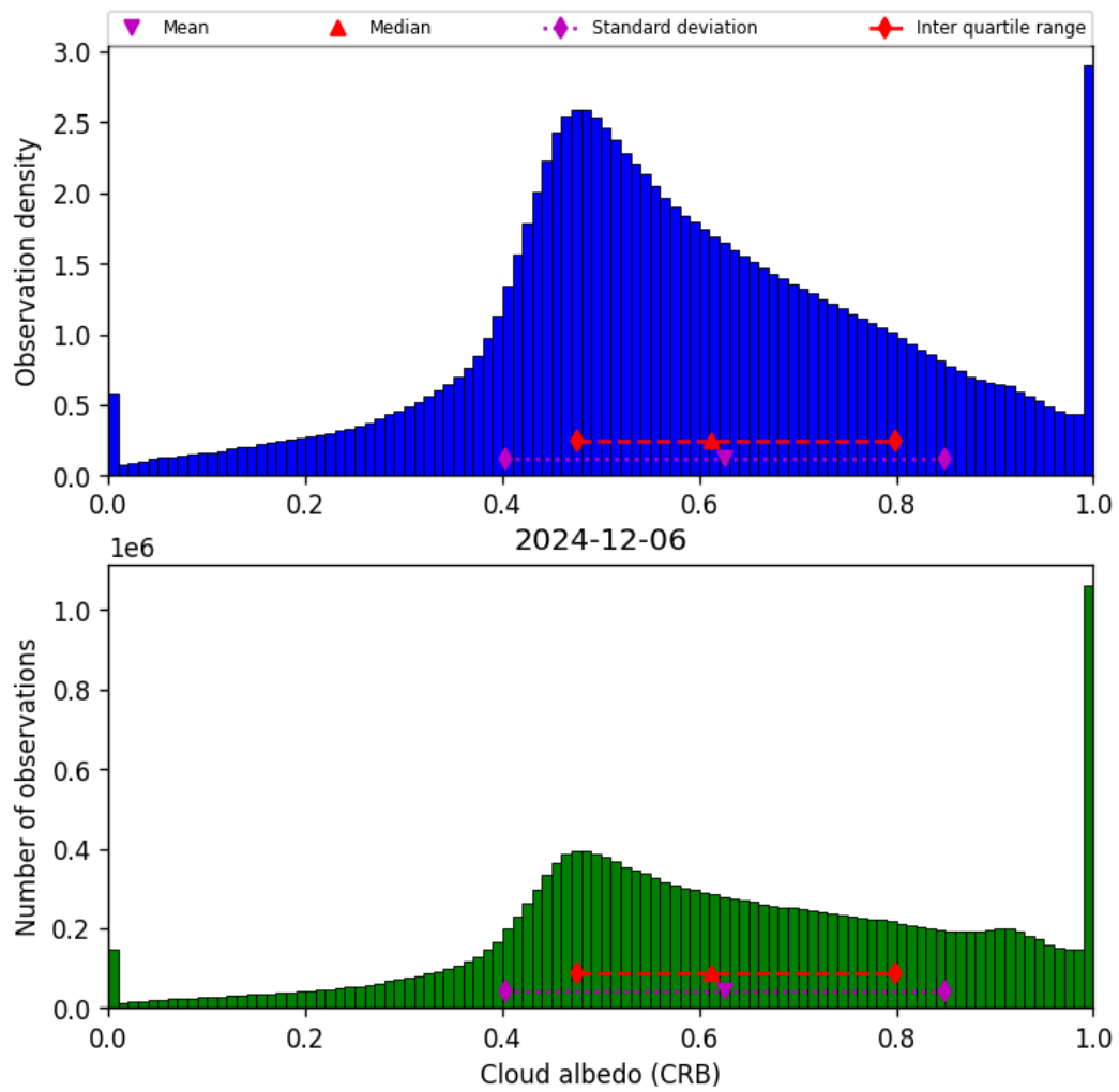
Figure 42: Histogram of “Cloud albedo (CRB)” for 2024-12-06 to 2024-12-07
