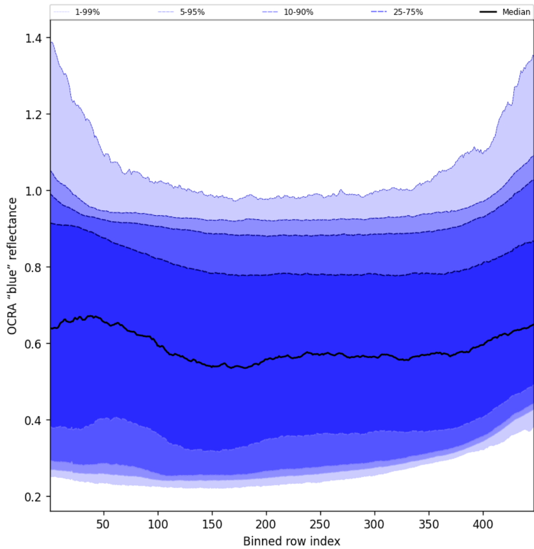
Figure 65: Along track statistics of “OCRA “blue” reflectance” for 2024-12-06 to 2024-12-07
