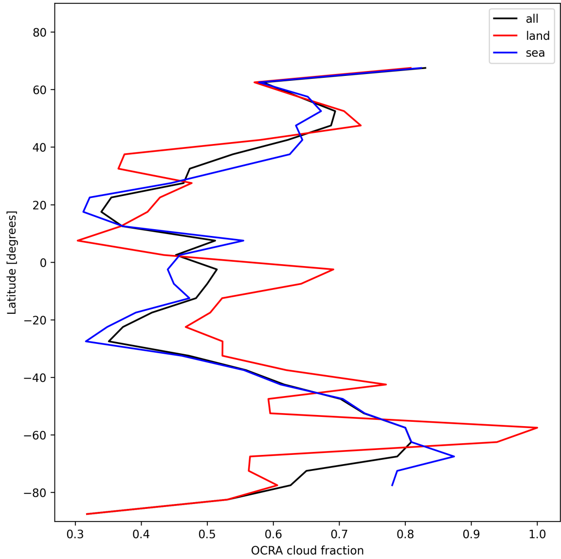
Figure 32: Zonal average of “OCRA cloud fraction” for 2024-12-06 to 2024-12-07.
