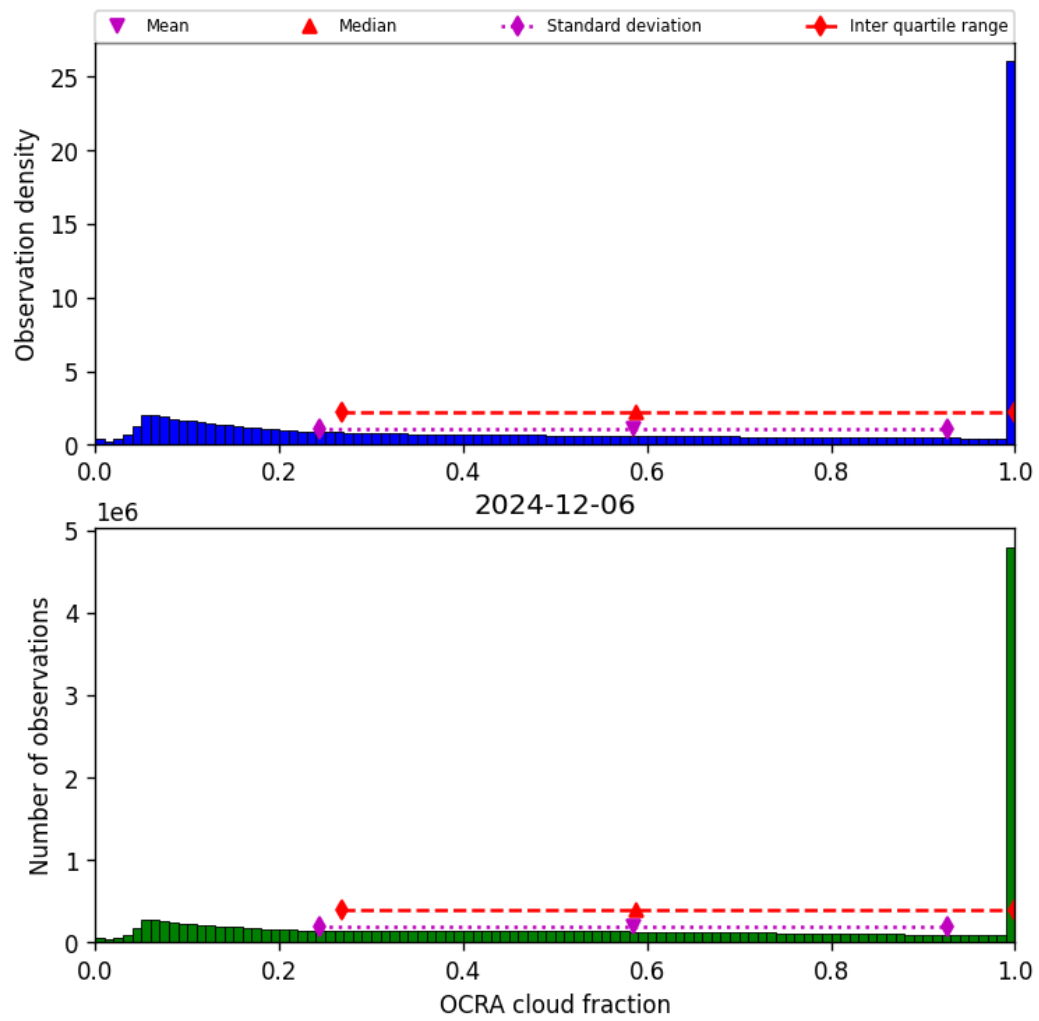
Figure 48: Histogram of “OCRA cloud fraction” for 2024-12-06 to 2024-12-07
