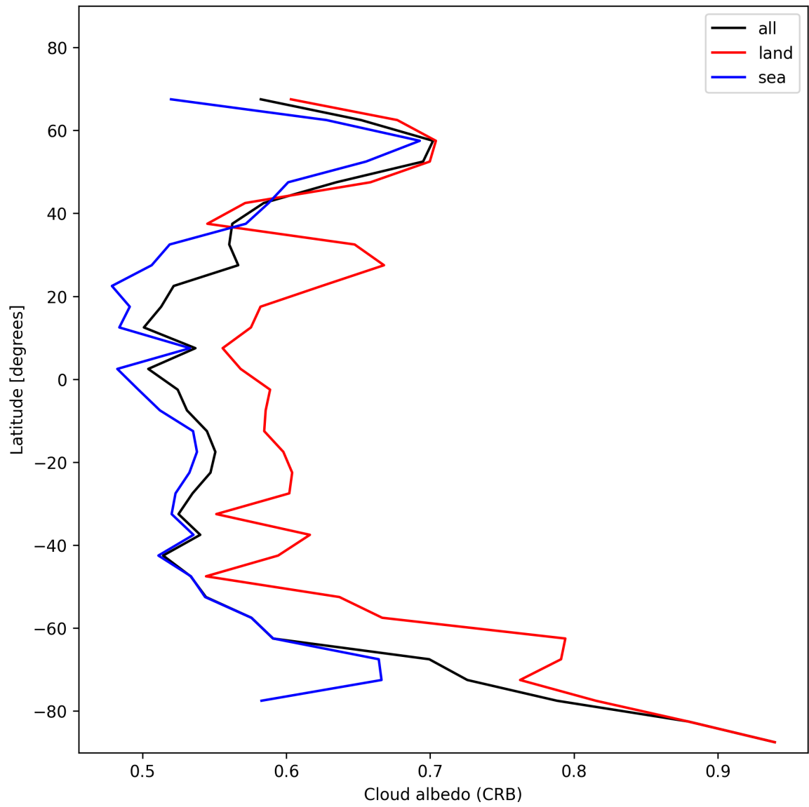
Figure 26: Zonal average of “Cloud albedo (CRB)” for 2024-12-06 to 2024-12-07.
