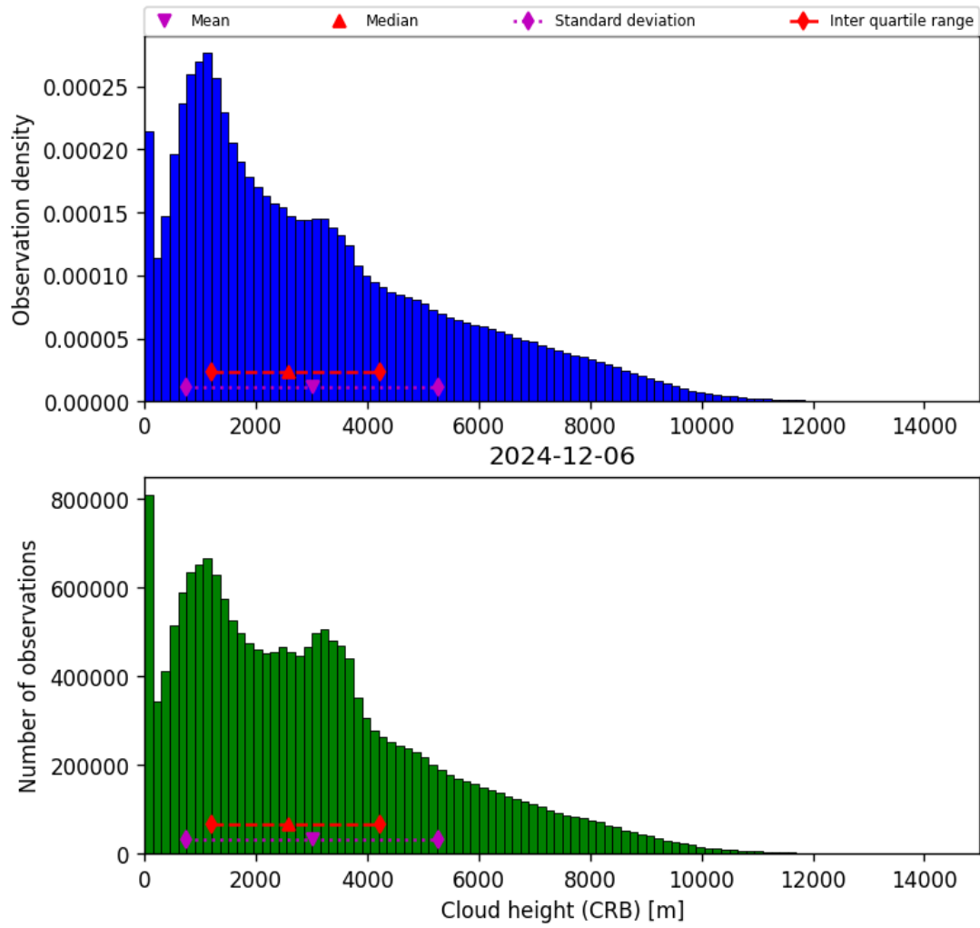
Figure 41: Histogram of “Cloud height (CRB)” for 2024-12-06 to 2024-12-07
