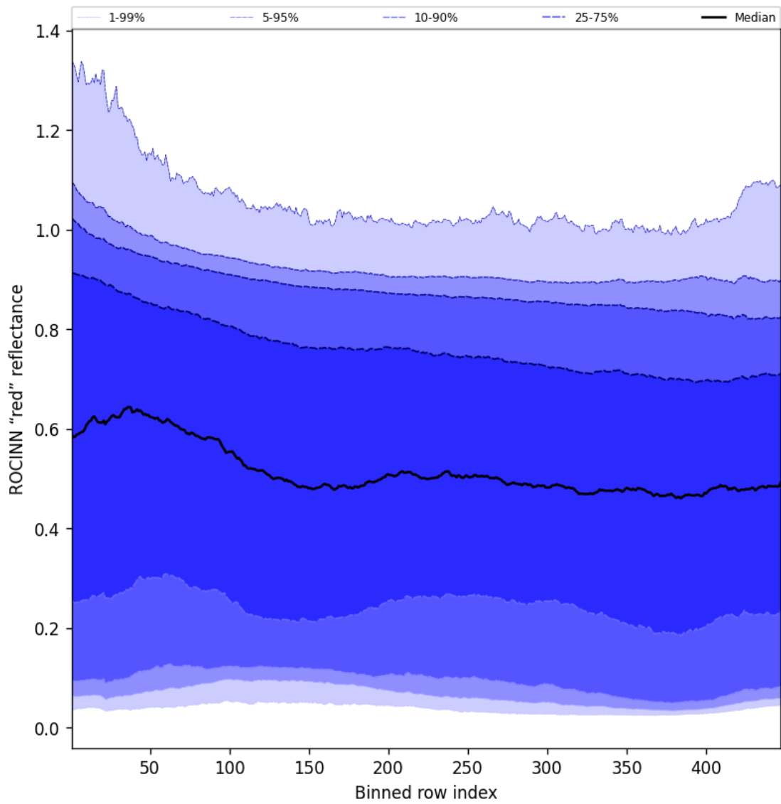
Figure 67: Along track statistics of "ROCINN "red" reflectance" for 2024-12-06 to 2024-12-07
