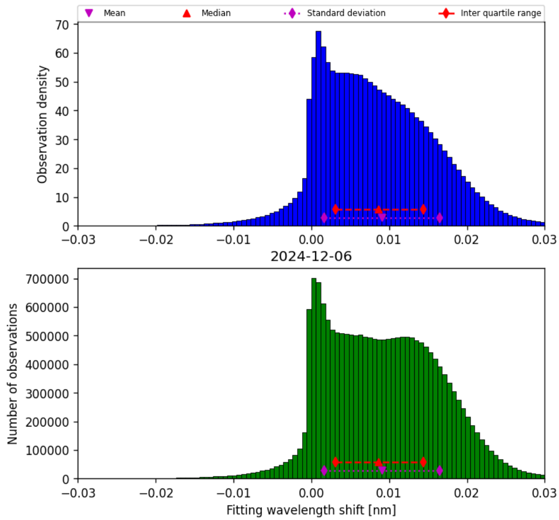
Figure 47: Histogram of “Fitting wavelength shift” for 2024-12-06 to 2024-12-07
