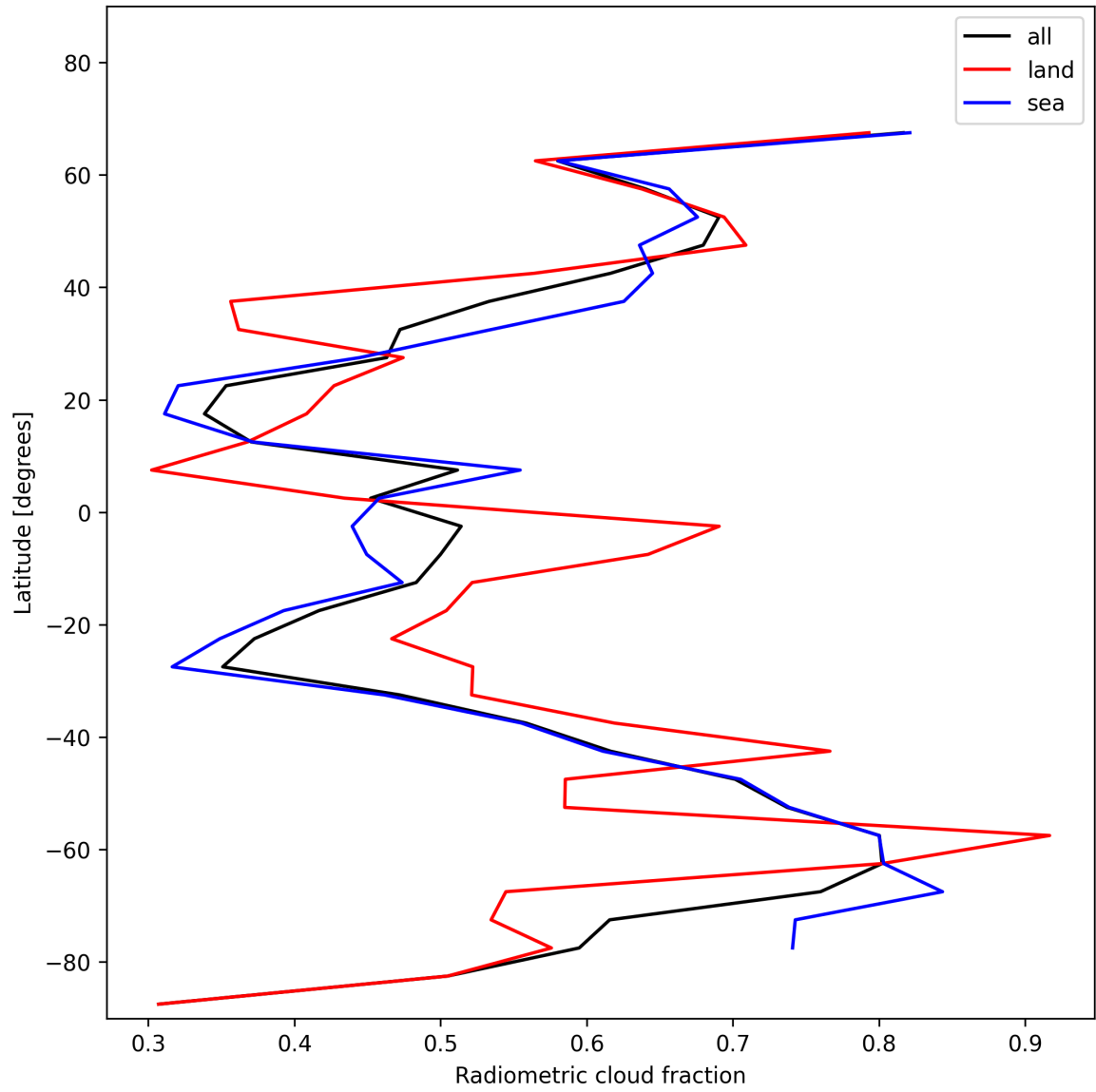
Figure 21: Zonal average of “Radiometric cloud fraction” for 2024-12-06 to 2024-12-07.
