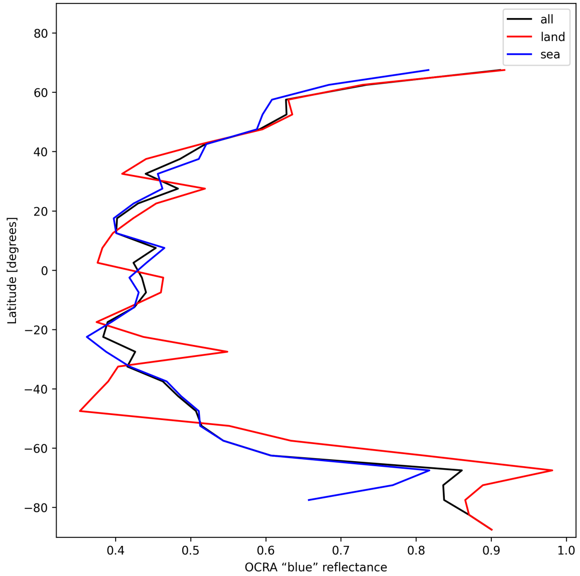
Figure 33: Zonal average of “OCRA “blue” reflectance” for 2024-12-07 to 2024-12-08.
