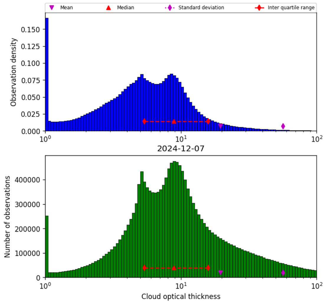
Figure 39: Histogram of “Cloud optical thickness” for 2024-12-07 to 2024-12-08
