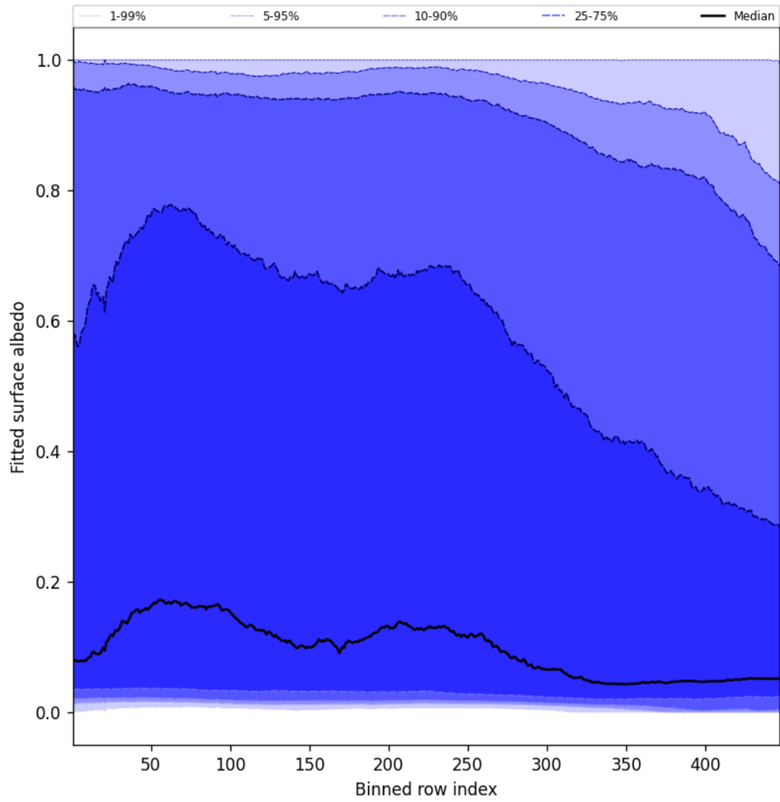
Figure 59: Along track statistics of “Fitted surface albedo” for 2024-12-07 to 2024-12-08
