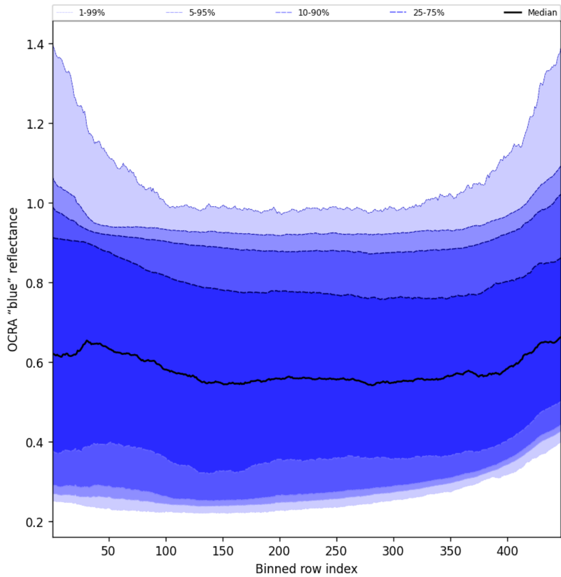
Figure 65: Along track statistics of “OCRA “blue” reflectance” for 2024-12-07 to 2024-12-08
