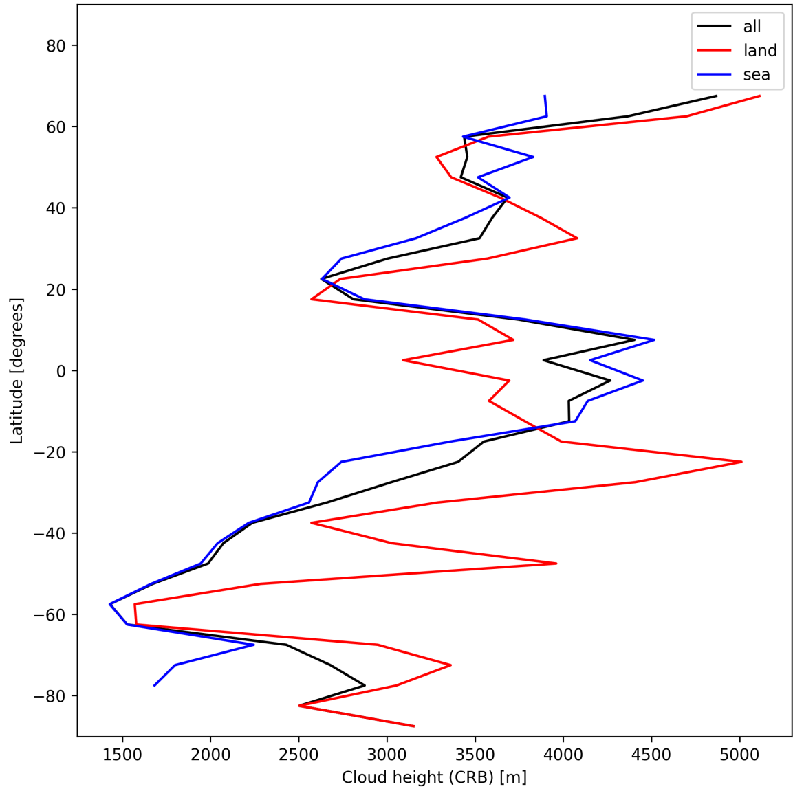
Figure 25: Zonal average of “Cloud height (CRB)” for 2024-12-07 to 2024-12-08.
