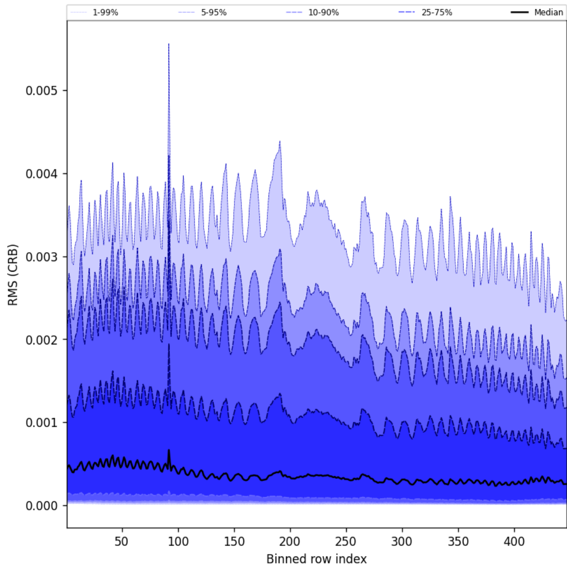
Figure 62: Along track statistics of “RMS (CRB)” for 2024-12-07 to 2024-12-08
