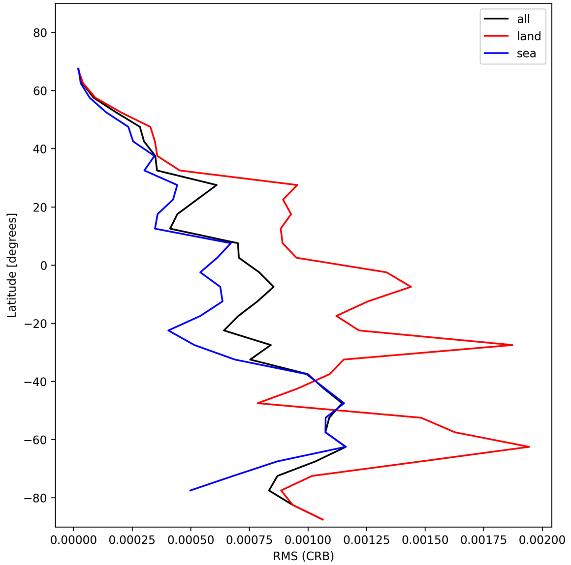
Figure 30: Zonal average of “RMS (CRB)” for 2024-12-07 to 2024-12-08.
