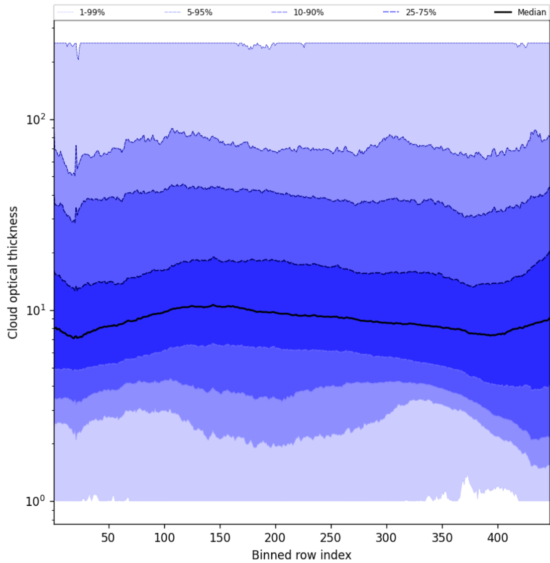
Figure 55: Along track statistics of “Cloud optical thickness” for 2024-12-07 to 2024-12-08
