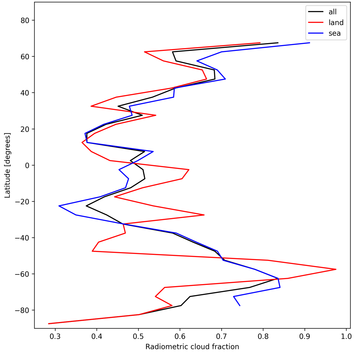
Figure 21: Zonal average of “Radiometric cloud fraction” for 2024-12-07 to 2024-12-08.
