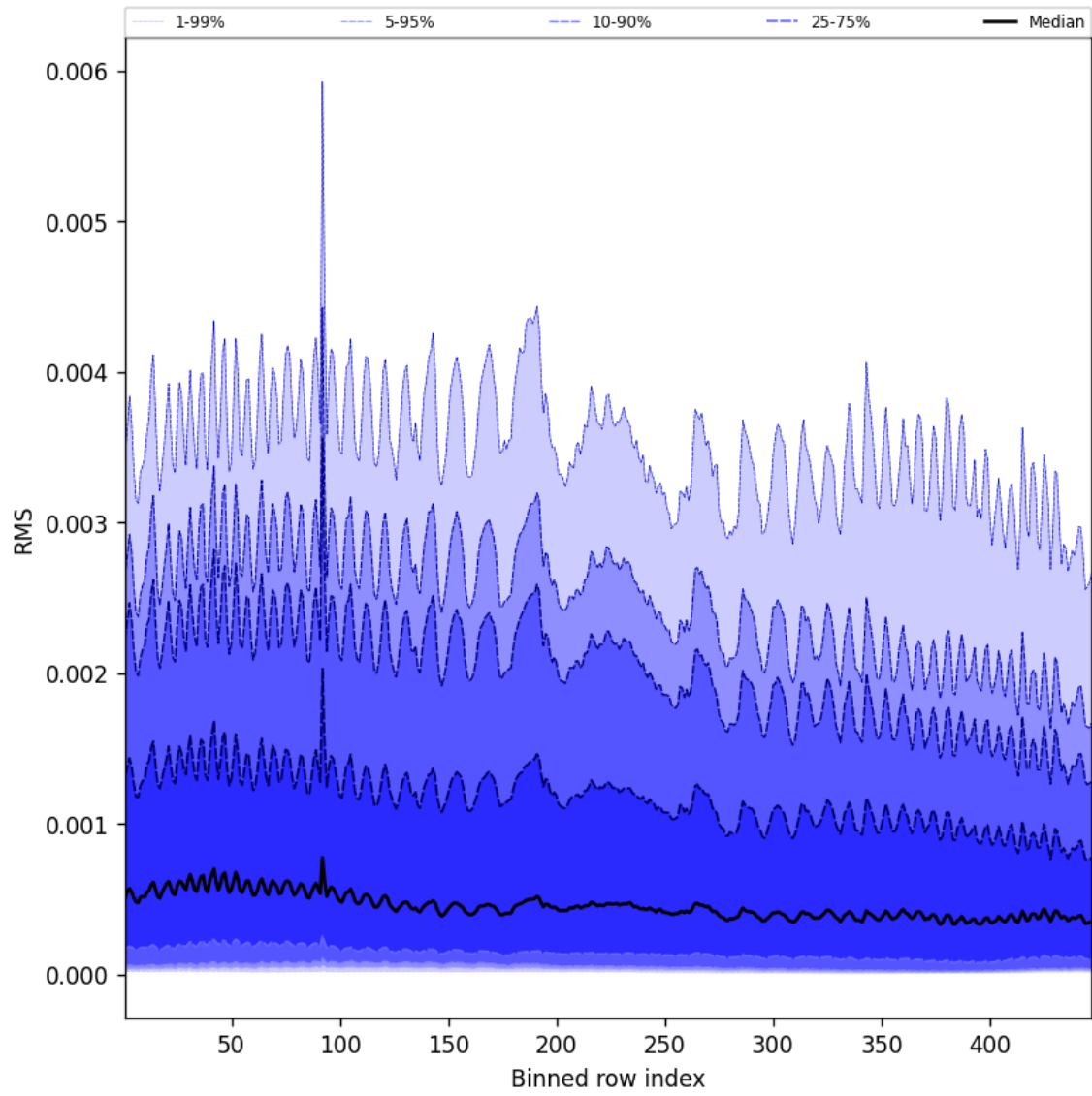
Figure 61: Along track statistics of “RMS” for 2024-12-07 to 2024-12-08
