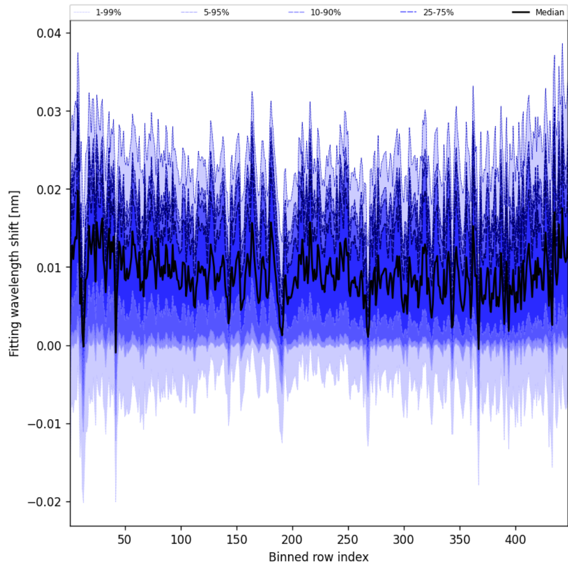
Figure 63: Along track statistics of “Fitting wavelength shift” for 2024-12-07 to 2024-12-08
