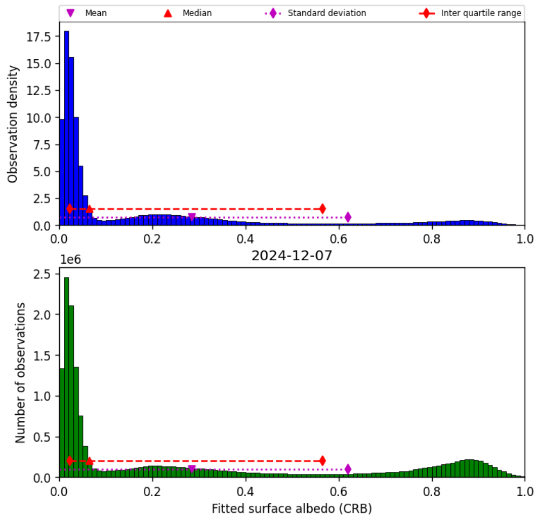
Figure 44: Histogram of “Fitted surface albedo (CRB)” for 2024-12-07 to 2024-12-08
