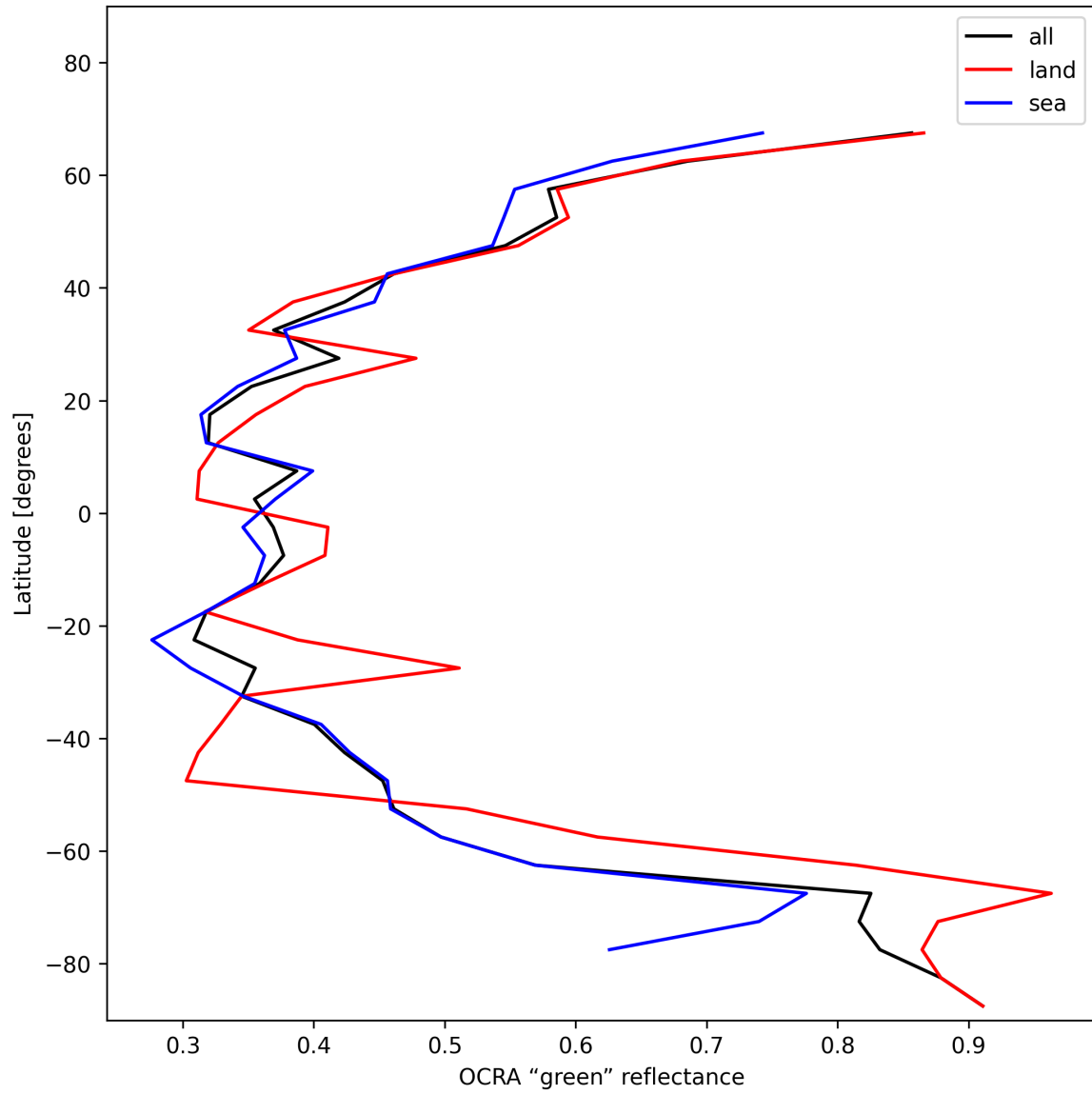
Figure 34: Zonal average of “OCRA “green” reflectance” for 2024-12-07 to 2024-12-08.
