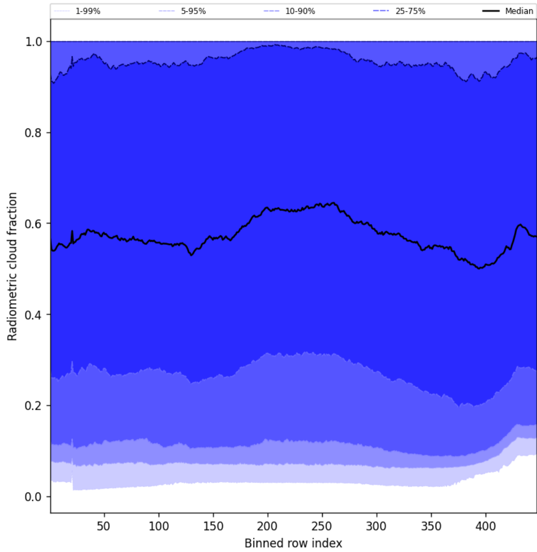
Figure 53: Along track statistics of “Radiometric cloud fraction” for 2024-12-07 to 2024-12-08
