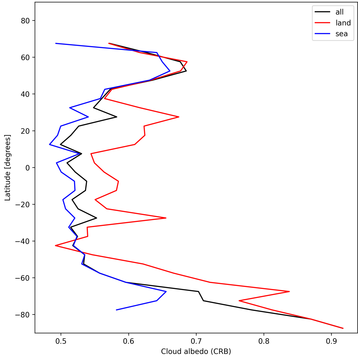
Figure 26: Zonal average of “Cloud albedo (CRB)” for 2024-12-07 to 2024-12-08.
