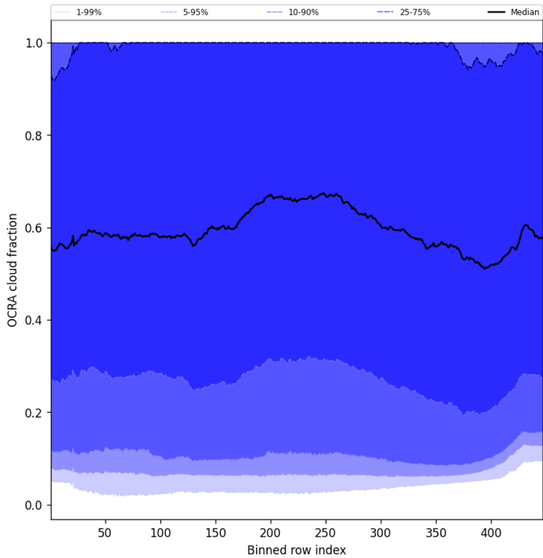
Figure 64: Along track statistics of “OCRA cloud fraction” for 2024-12-07 to 2024-12-08
