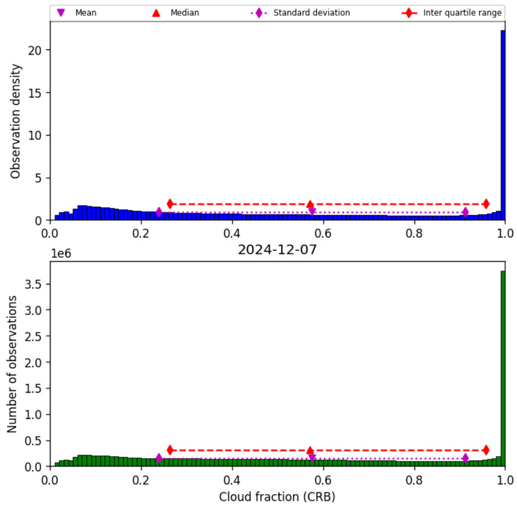
Figure 40: Histogram of “Cloud fraction (CRB)” for 2024-12-07 to 2024-12-08
