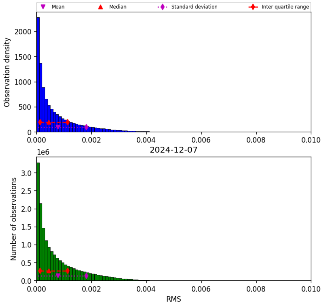
Figure 45: Histogram of “RMS” for 2024-12-07 to 2024-12-08
