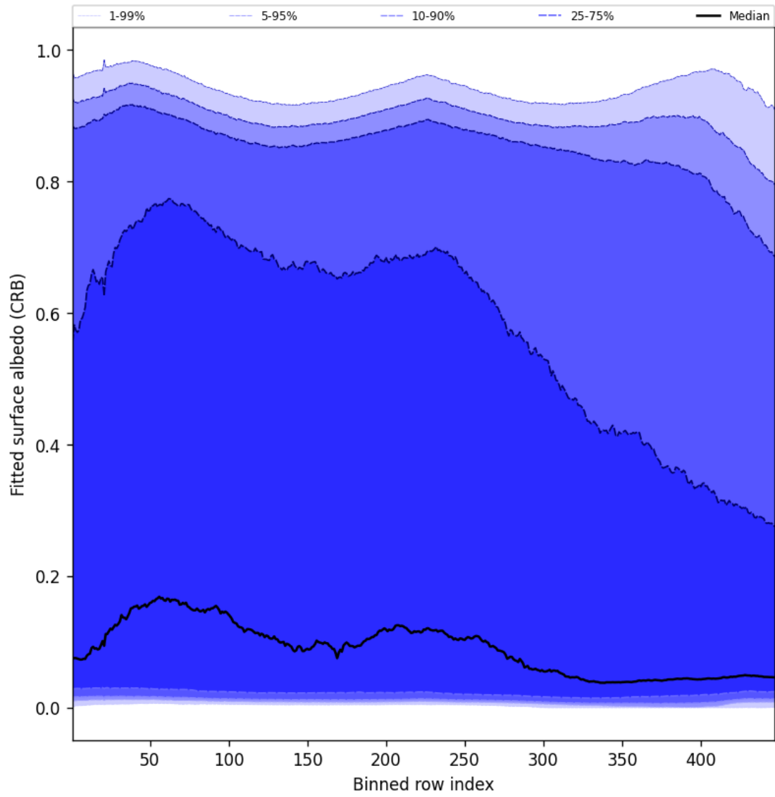
Figure 60: Along track statistics of “Fitted surface albedo (CRB)” for 2024-12-07 to 2024-12-08
