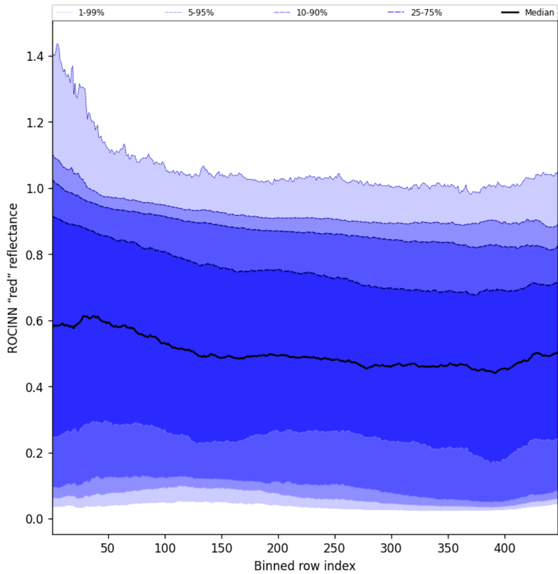
Figure 67: Along track statistics of "ROCINN "red" reflectance" for 2024-12-07 to 2024-12-08
