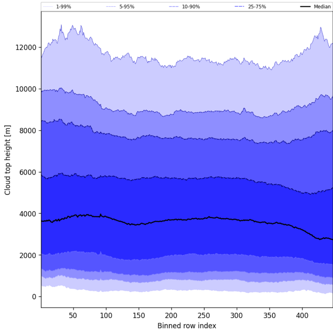
Figure 54: Along track statistics of “Cloud top height” for 2024-12-07 to 2024-12-08
