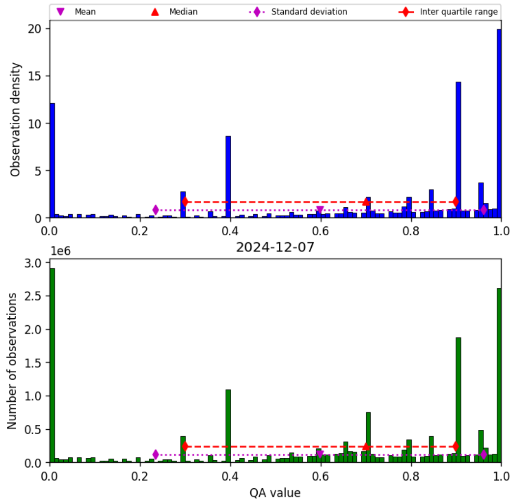
Figure 36: Histogram of “QA value” for 2024-12-07 to 2024-12-08
