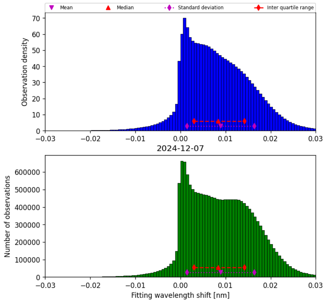
Figure 47: Histogram of “Fitting wavelength shift” for 2024-12-07 to 2024-12-08
