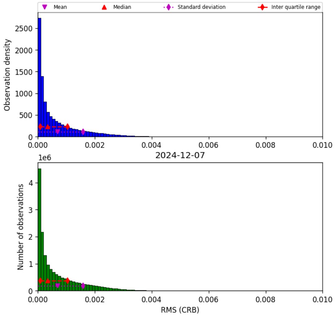
Figure 46: Histogram of “RMS (CRB)” for 2024-12-07 to 2024-12-08
