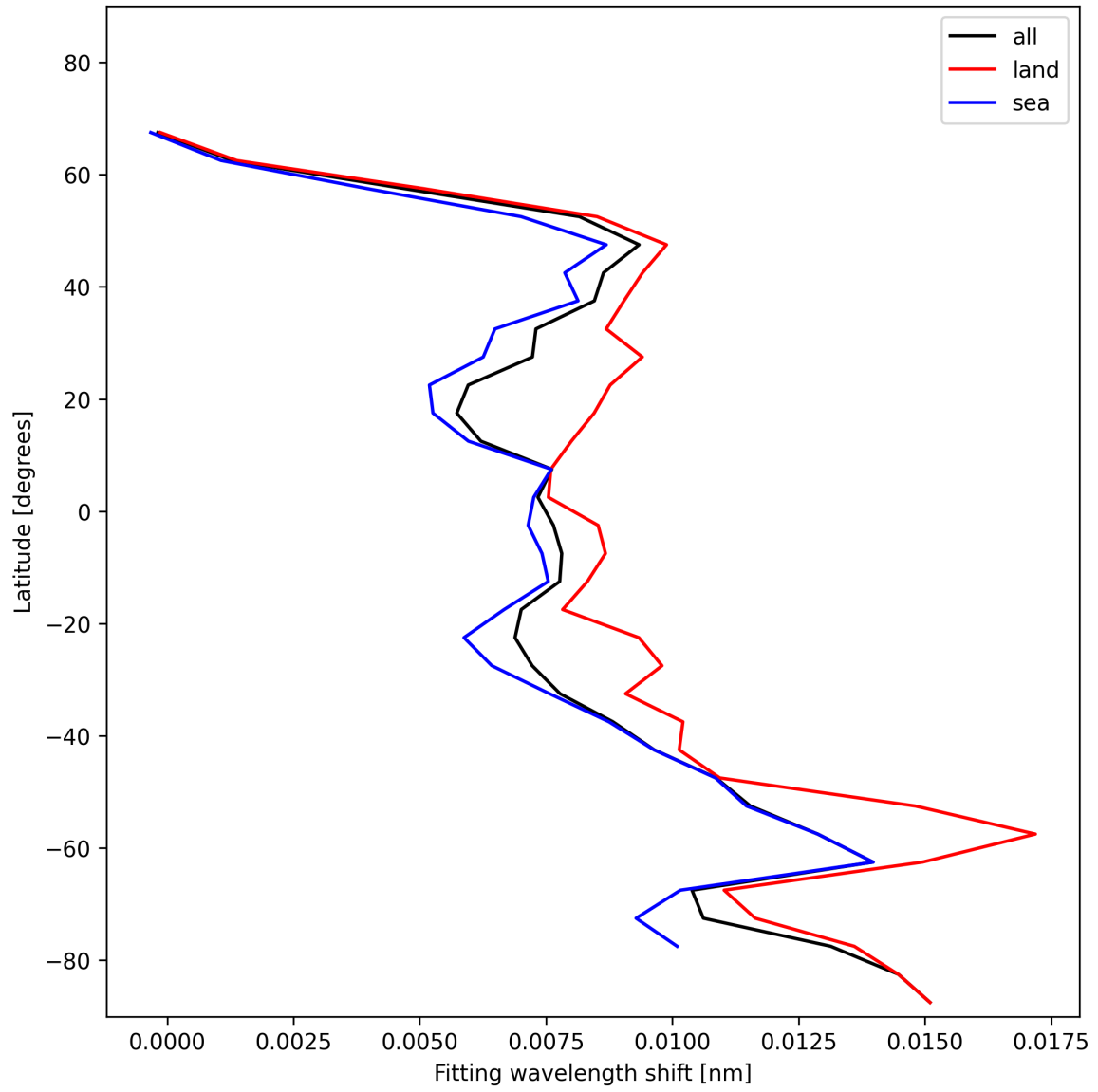
Figure 31: Zonal average of “Fitting wavelength shift” for 2024-12-07 to 2024-12-08.
