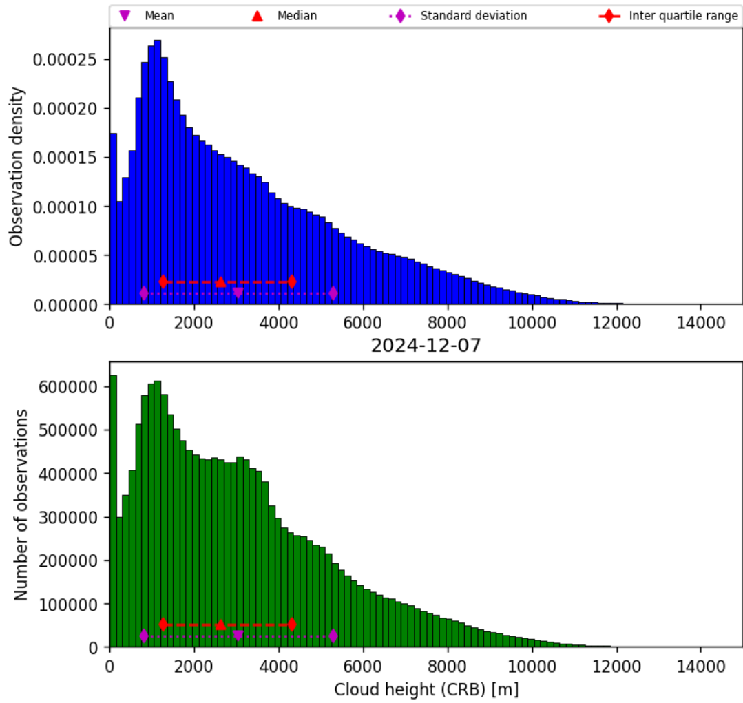
Figure 41: Histogram of “Cloud height (CRB)” for 2024-12-07 to 2024-12-08
