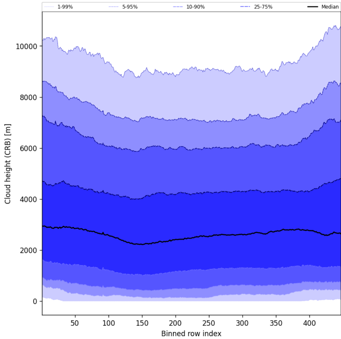
Figure 57: Along track statistics of “Cloud height (CRB)” for 2024-12-07 to 2024-12-08
