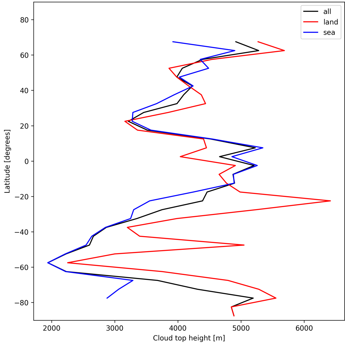
Figure 22: Zonal average of “Cloud top height” for 2024-12-07 to 2024-12-08.
