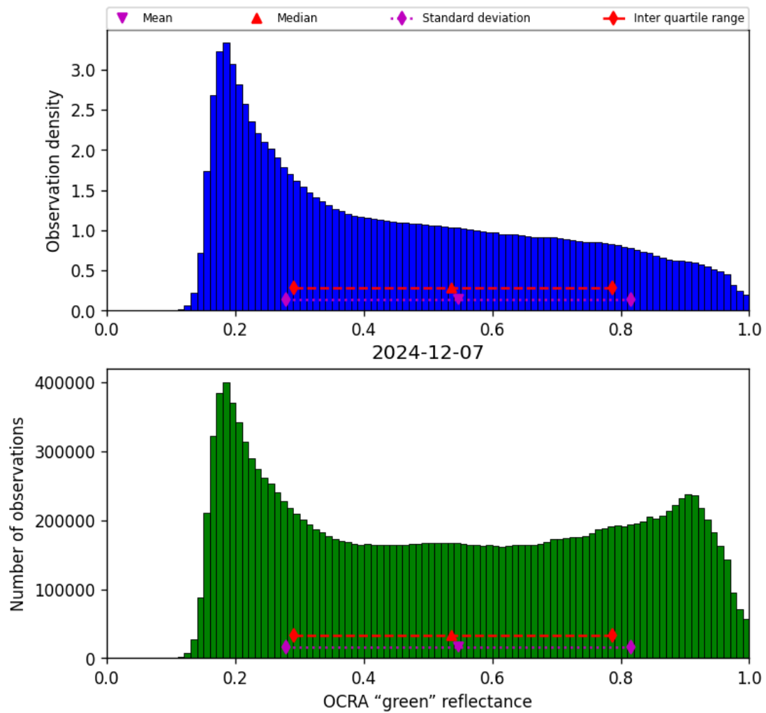
Figure 50: Histogram of “OCRA “green” reflectance” for 2024-12-07 to 2024-12-08
