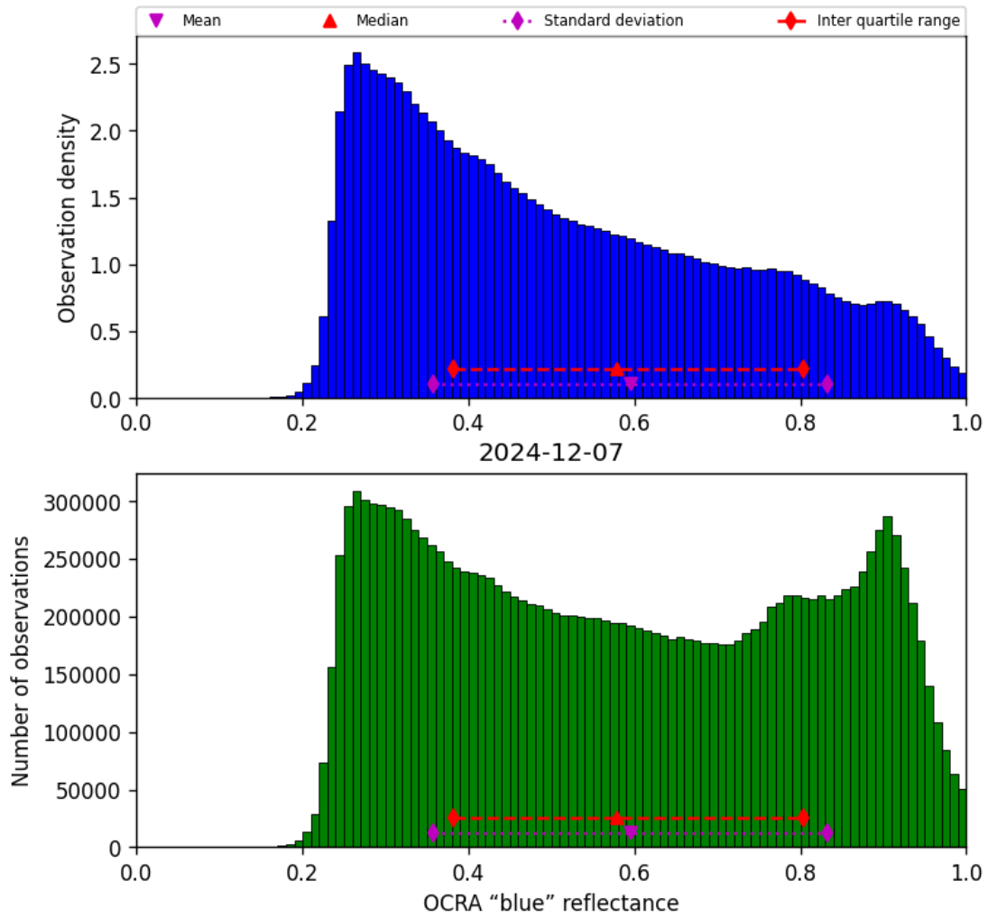
Figure 49: Histogram of “OCRA “blue” reflectance” for 2024-12-07 to 2024-12-08
