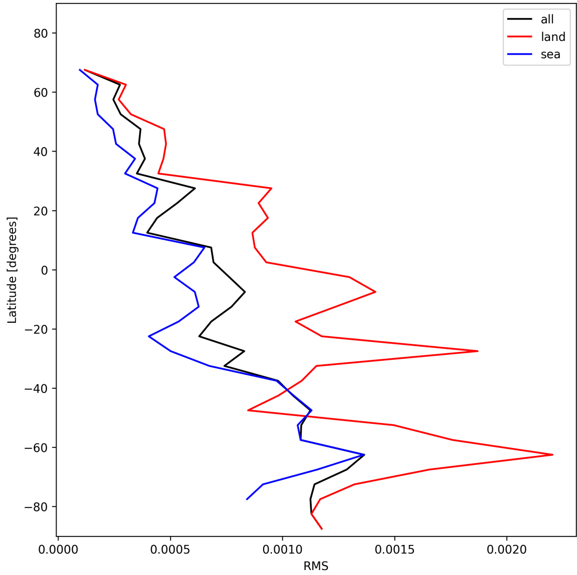
Figure 29: Zonal average of “RMS” for 2024-12-07 to 2024-12-08.
