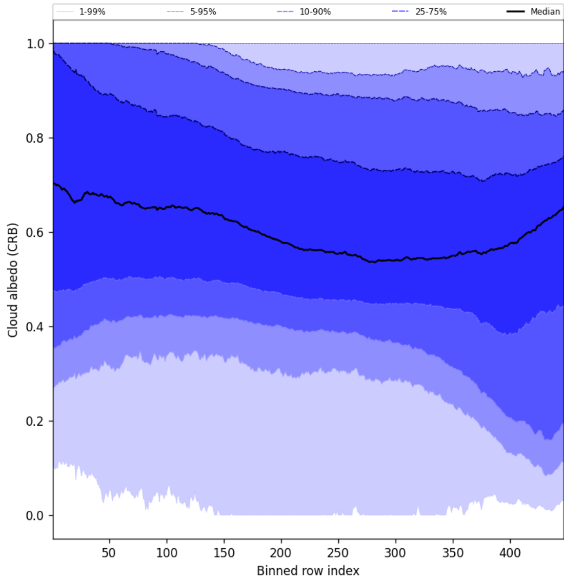
Figure 58: Along track statistics of “Cloud albedo (CRB)” for 2024-12-07 to 2024-12-08
