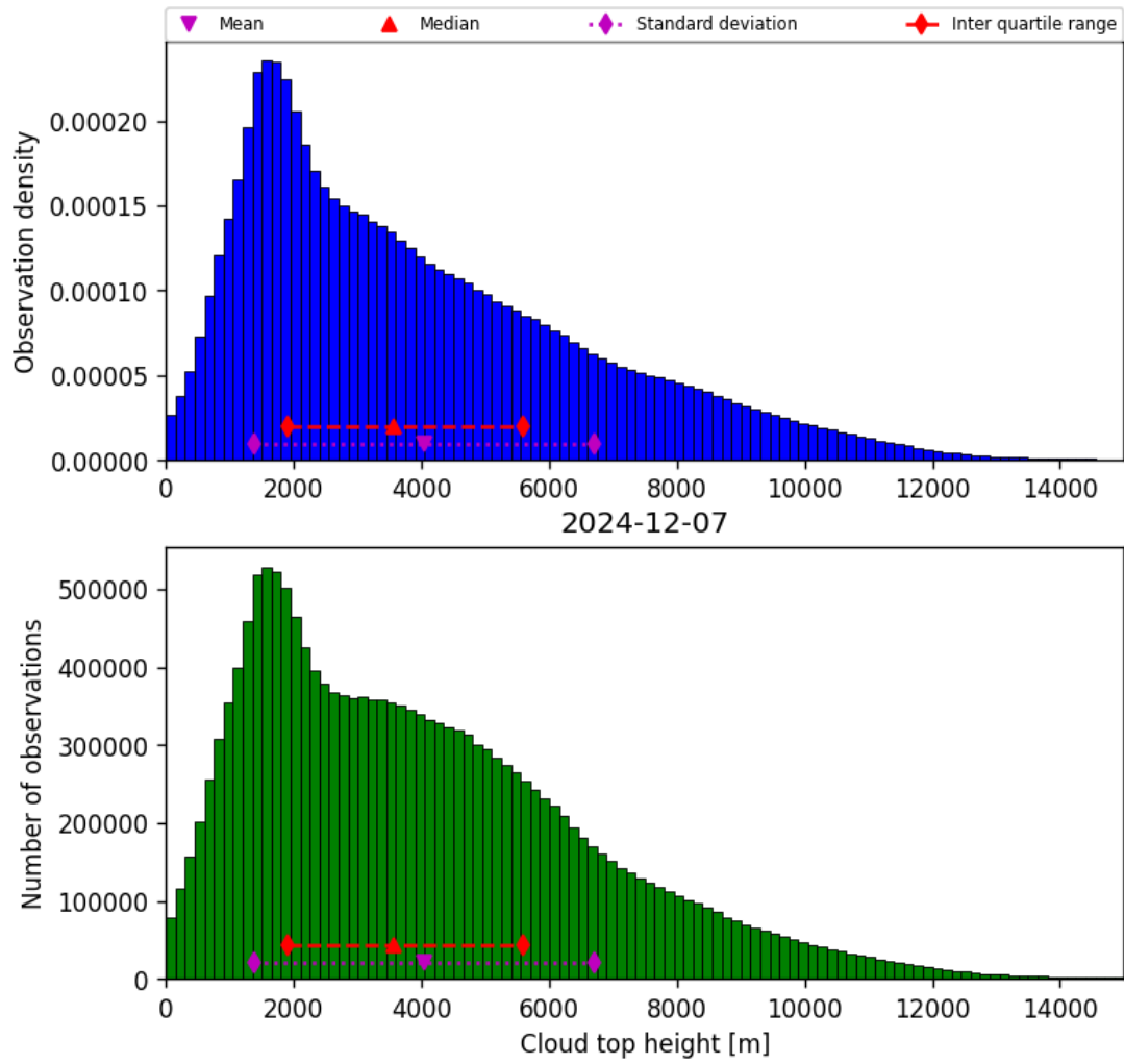
Figure 38: Histogram of “Cloud top height” for 2024-12-07 to 2024-12-08
