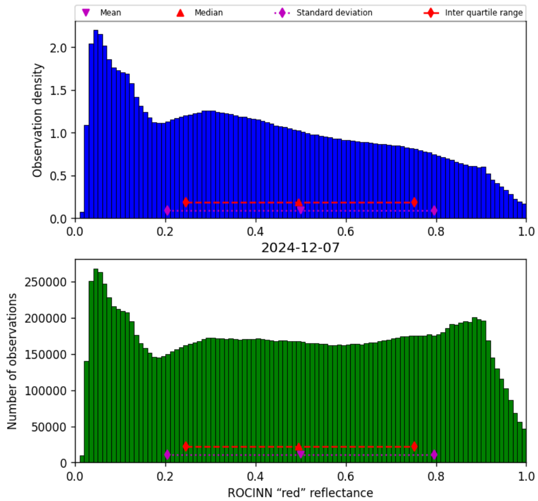
Figure 51: Histogram of “ROCINN “red” reflectance” for 2024-12-07 to 2024-12-08
