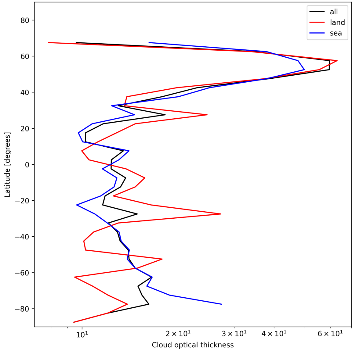
Figure 23: Zonal average of “Cloud optical thickness” for 2024-12-07 to 2024-12-08.
