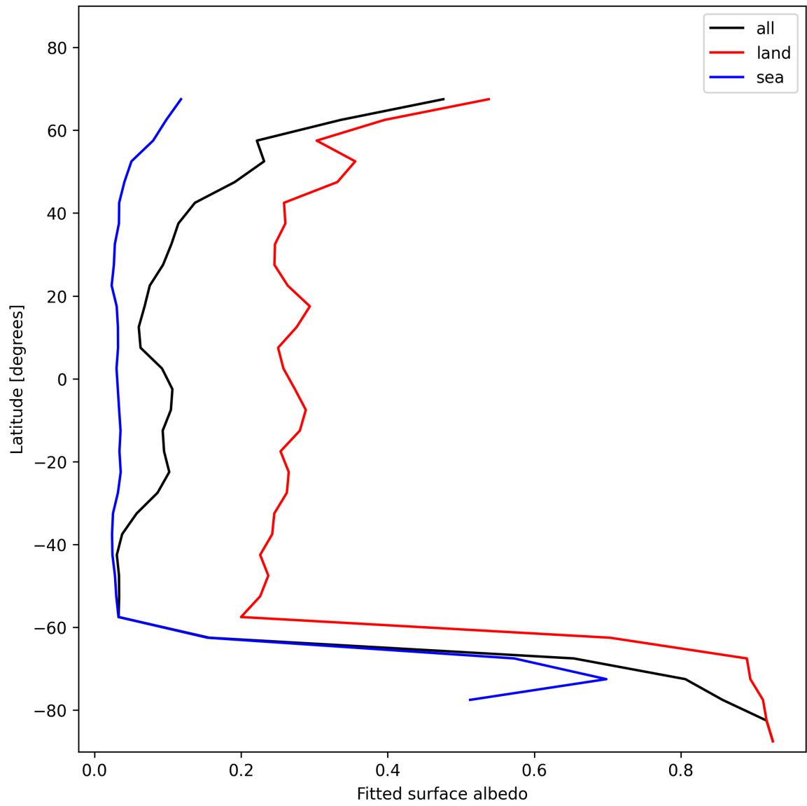
Figure 27: Zonal average of “Fitted surface albedo” for 2024-12-07 to 2024-12-08.
