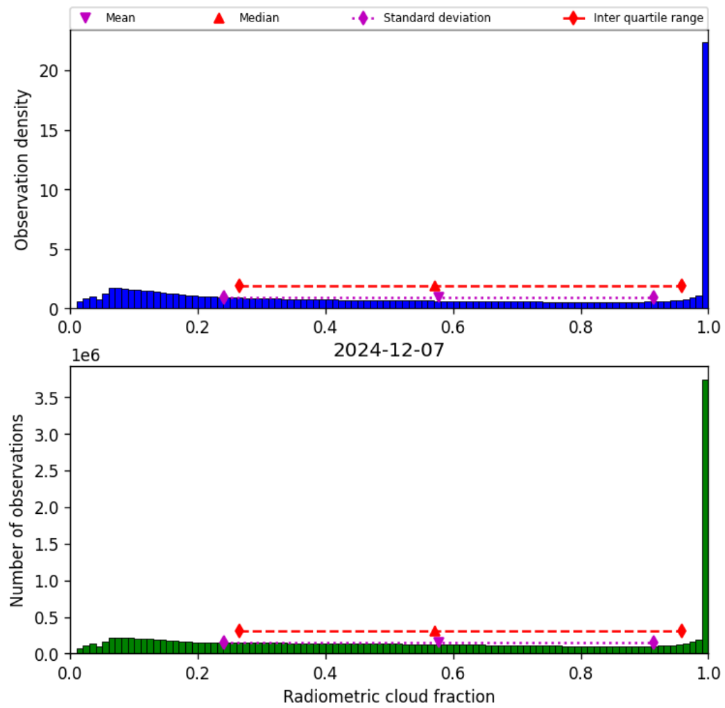
Figure 37: Histogram of “Radiometric cloud fraction” for 2024-12-07 to 2024-12-08
