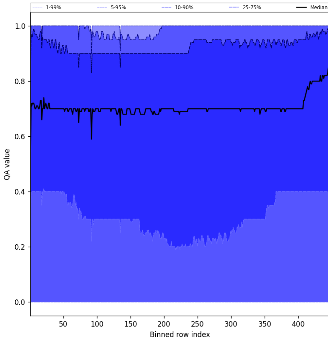
Figure 52: Along track statistics of “QA value” for 2024-12-07 to 2024-12-08
