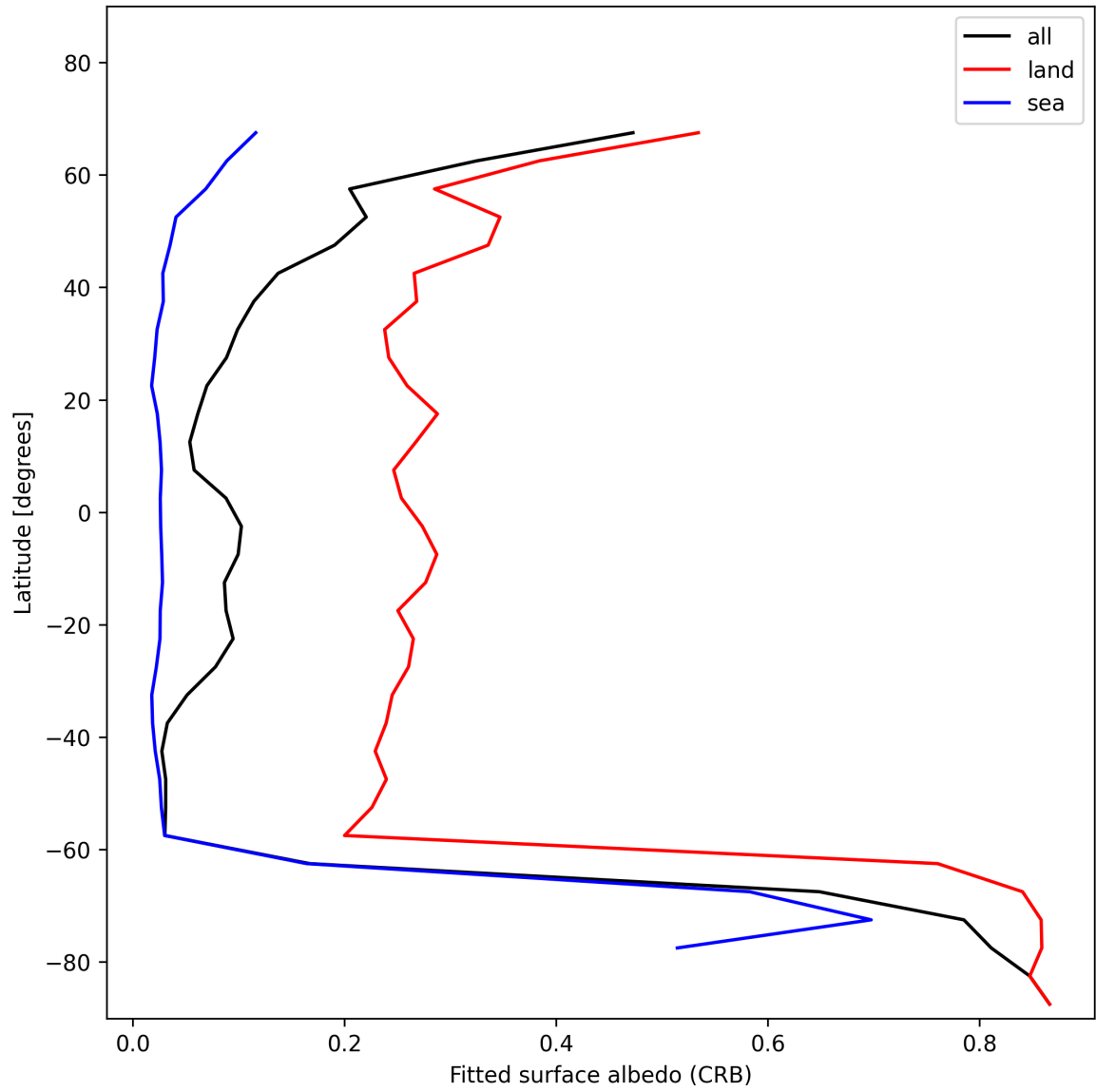
Figure 28: Zonal average of “Fitted surface albedo (CRB)” for 2024-12-07 to 2024-12-08.
