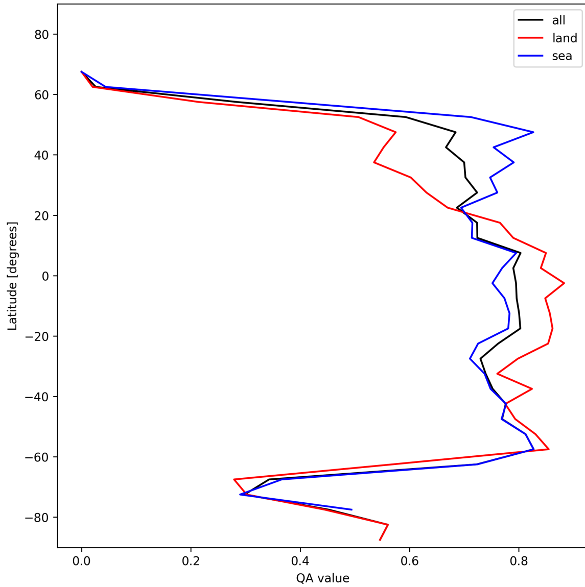
Figure 20: Zonal average of “QA value” for 2024-12-07 to 2024-12-08.
