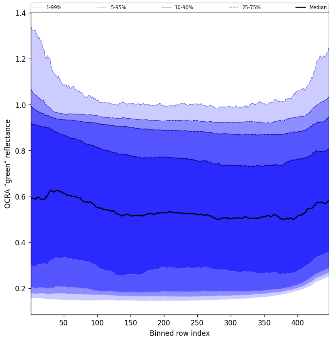
Figure 66: Along track statistics of “OCRA “green” reflectance” for 2024-12-07 to 2024-12-08
