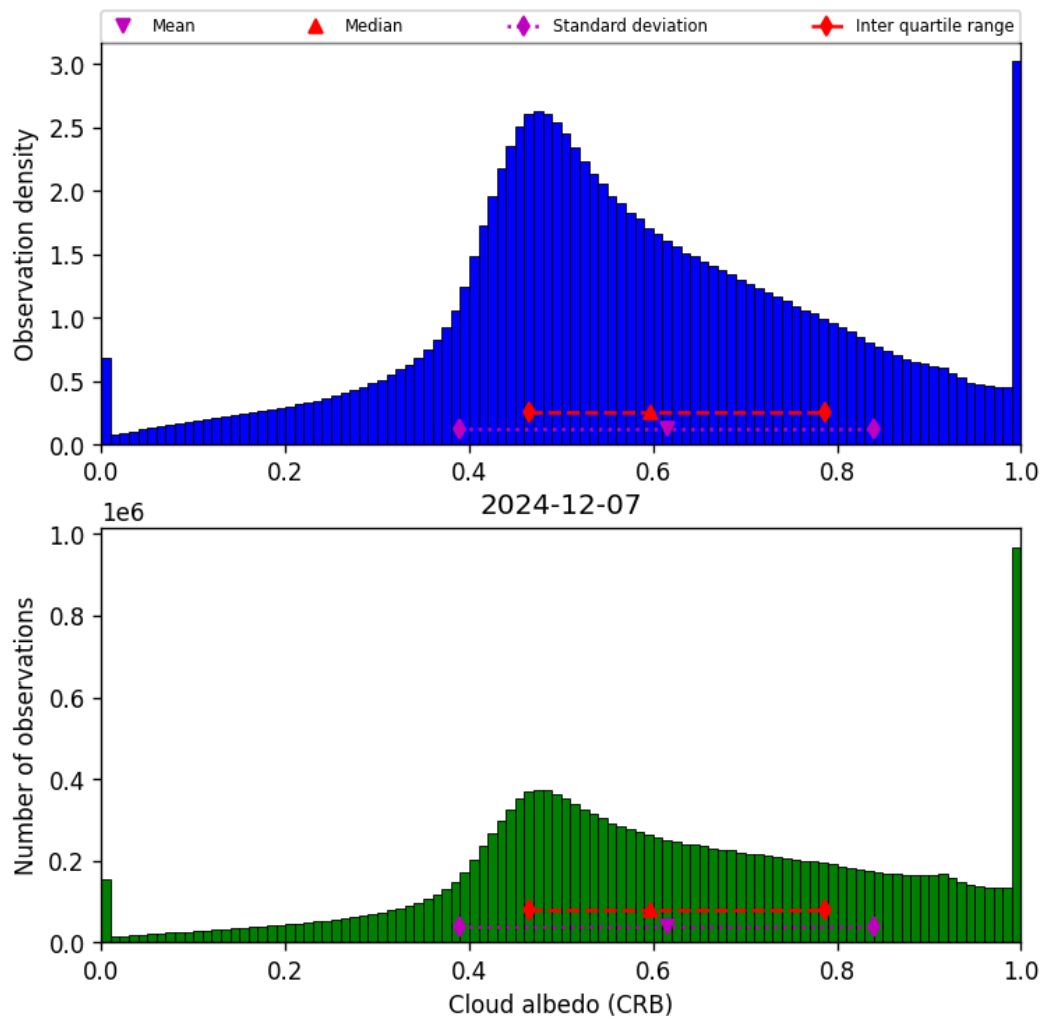
Figure 42: Histogram of “Cloud albedo (CRB)” for 2024-12-07 to 2024-12-08
