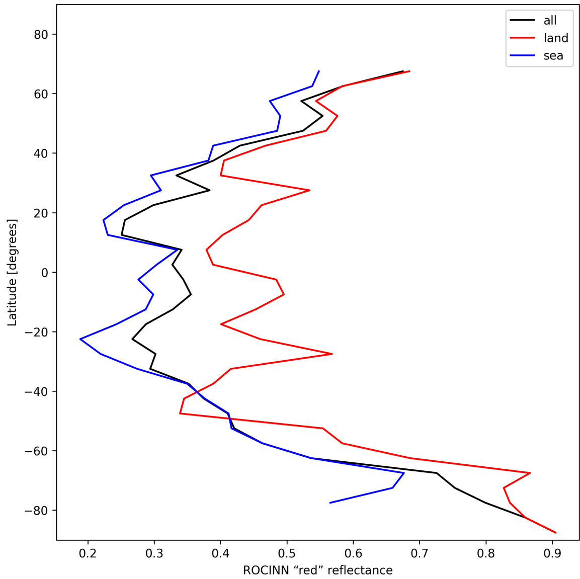
Figure 35: Zonal average of “ROCINN “red” reflectance” for 2024-12-07 to 2024-12-08.
