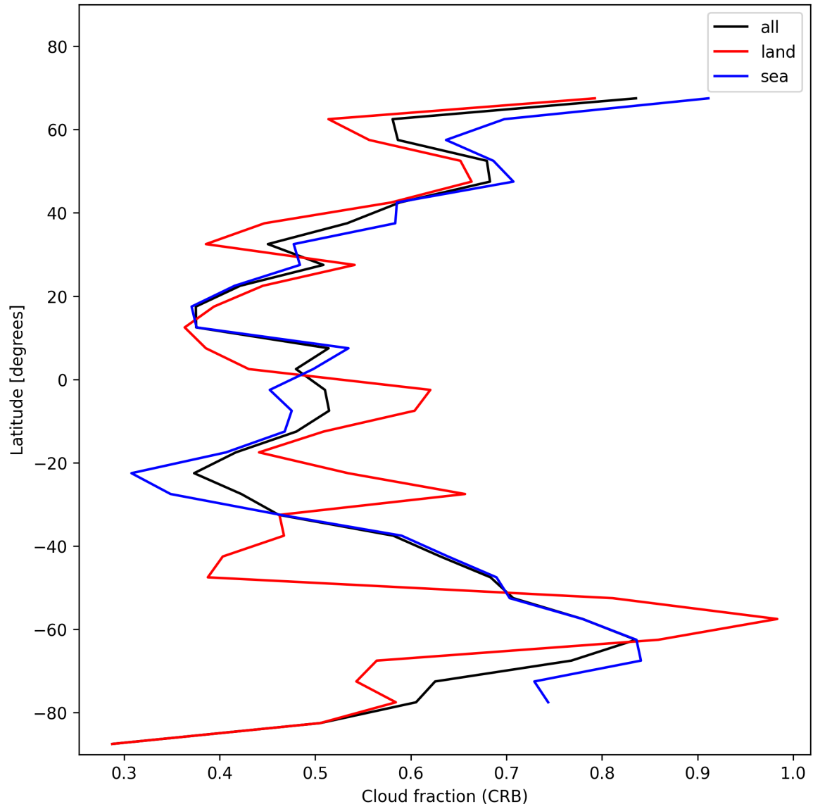
Figure 24: Zonal average of “Cloud fraction (CRB)” for 2024-12-07 to 2024-12-08.
