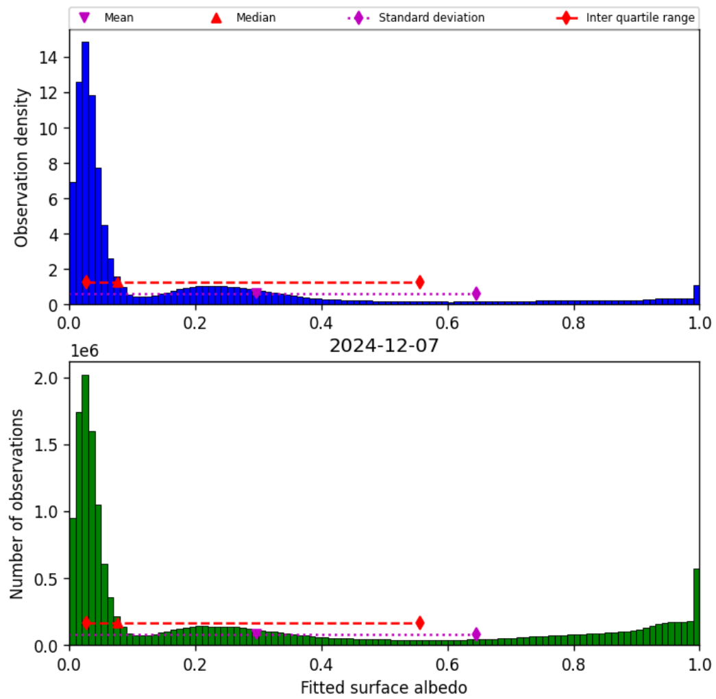
Figure 43: Histogram of “Fitted surface albedo” for 2024-12-07 to 2024-12-08
