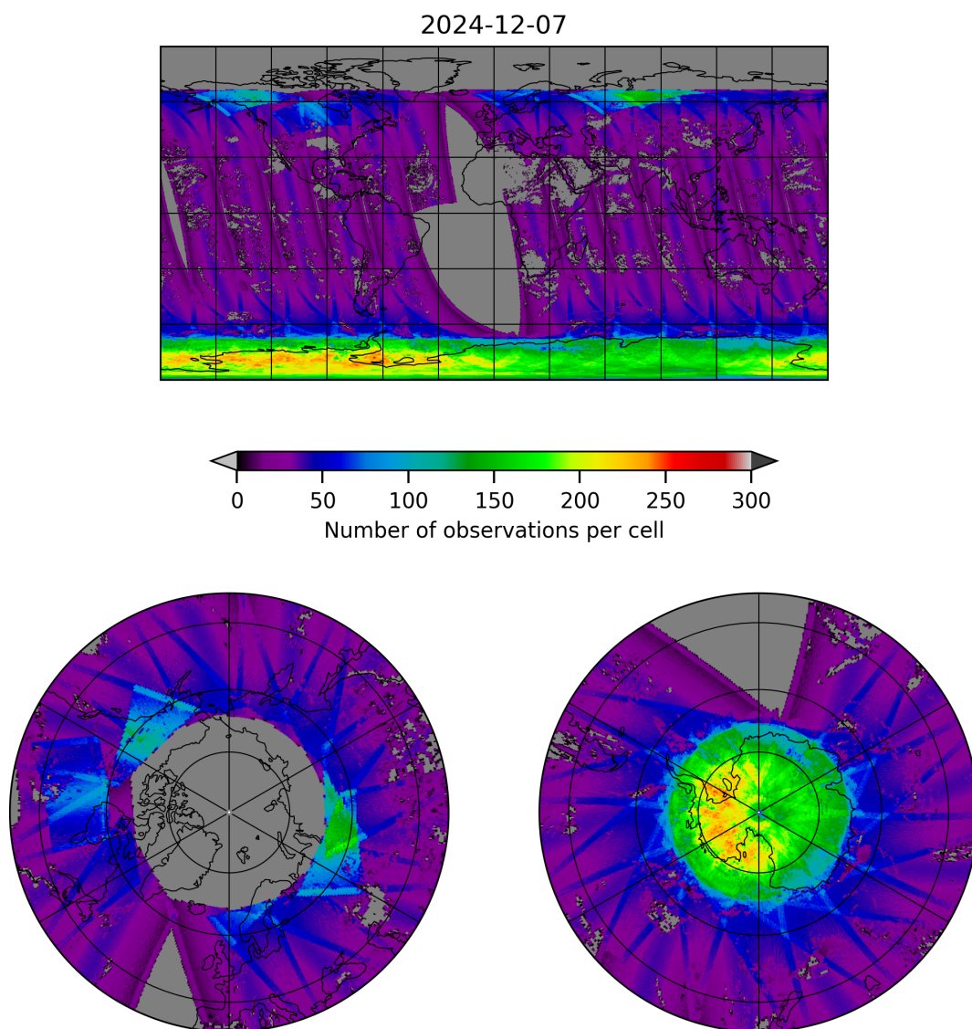
Figure 19: Map of the number of observations for 2024-12-07 to 2024-12-08
