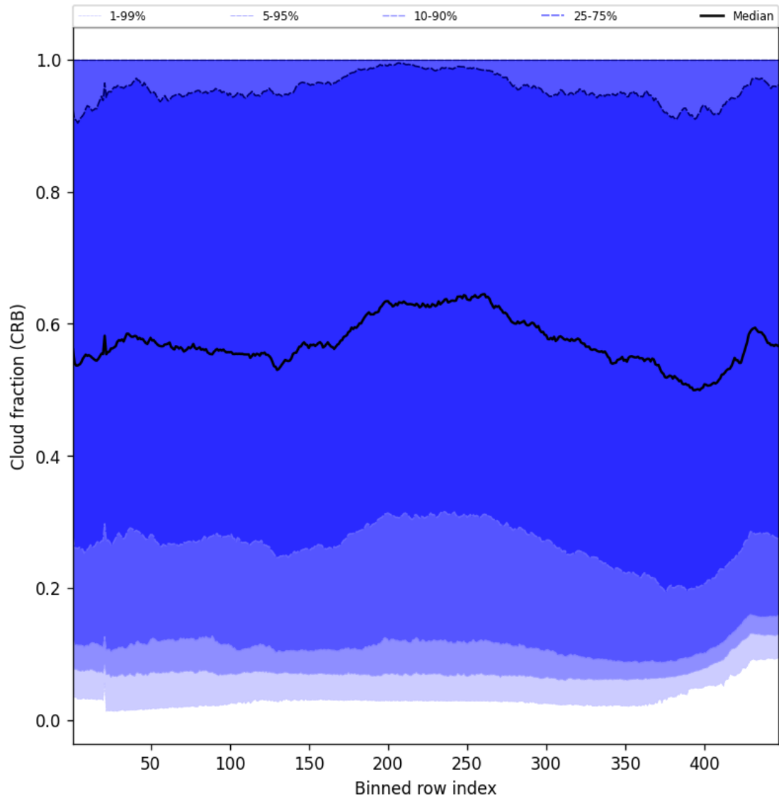
Figure 56: Along track statistics of “Cloud fraction (CRB)” for 2024-12-07 to 2024-12-08
