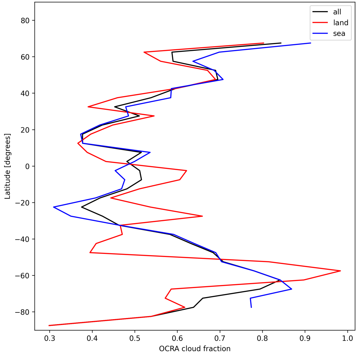
Figure 32: Zonal average of “OCRA cloud fraction” for 2024-12-07 to 2024-12-08.
