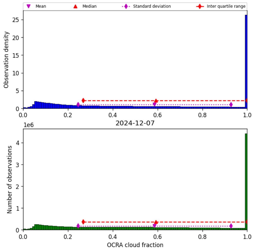
Figure 48: Histogram of “OCRA cloud fraction” for 2024-12-07 to 2024-12-08
