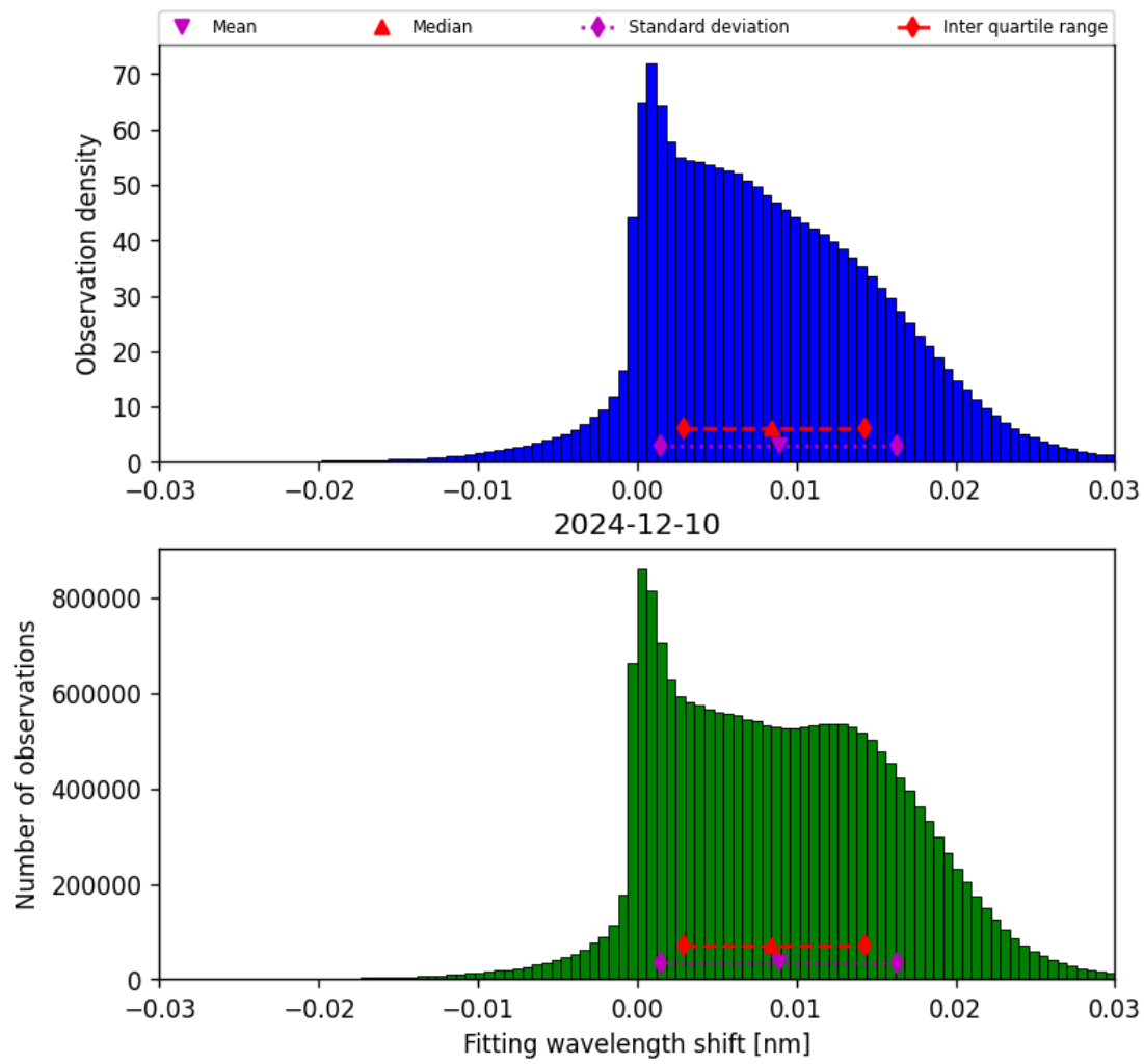
Figure 47: Histogram of “Fitting wavelength shift” for 2024-12-10 to 2024-12-11
