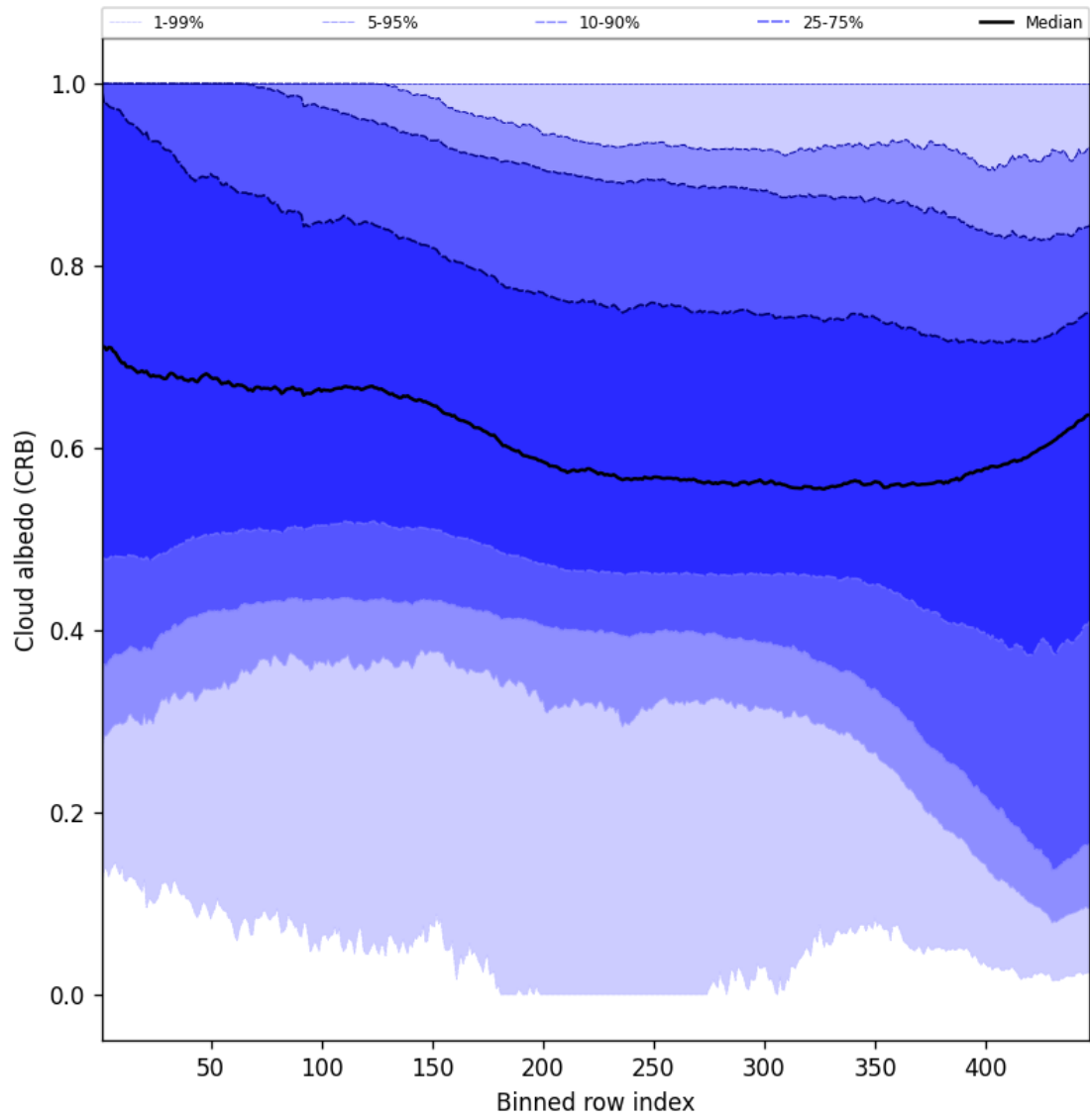
Figure 58: Along track statistics of “Cloud albedo (CRB)” for 2024-12-10 to 2024-12-11
