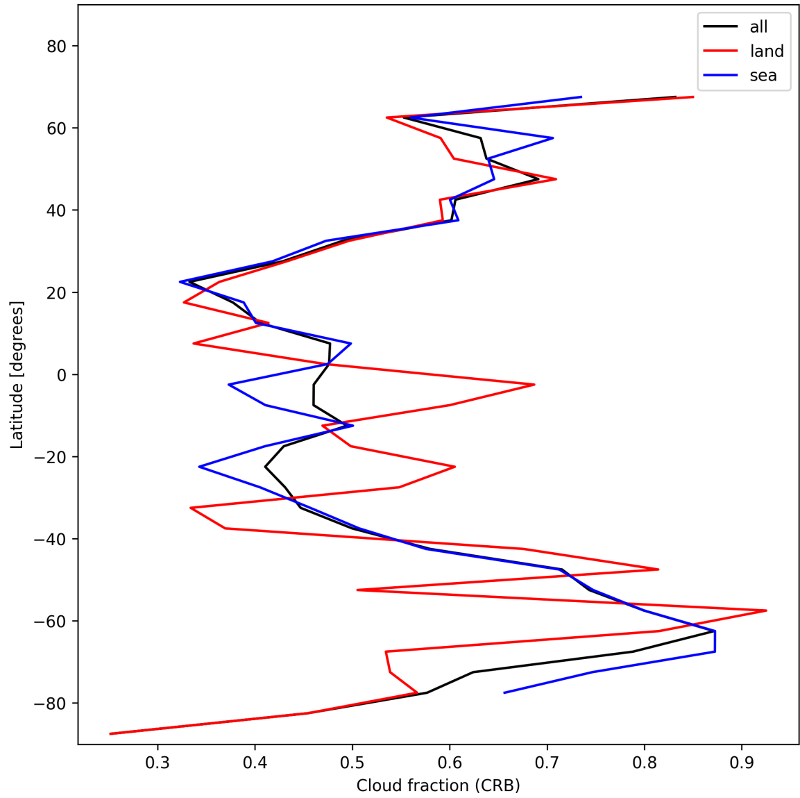
Figure 24: Zonal average of “Cloud fraction (CRB)” for 2024-12-10 to 2024-12-11.
