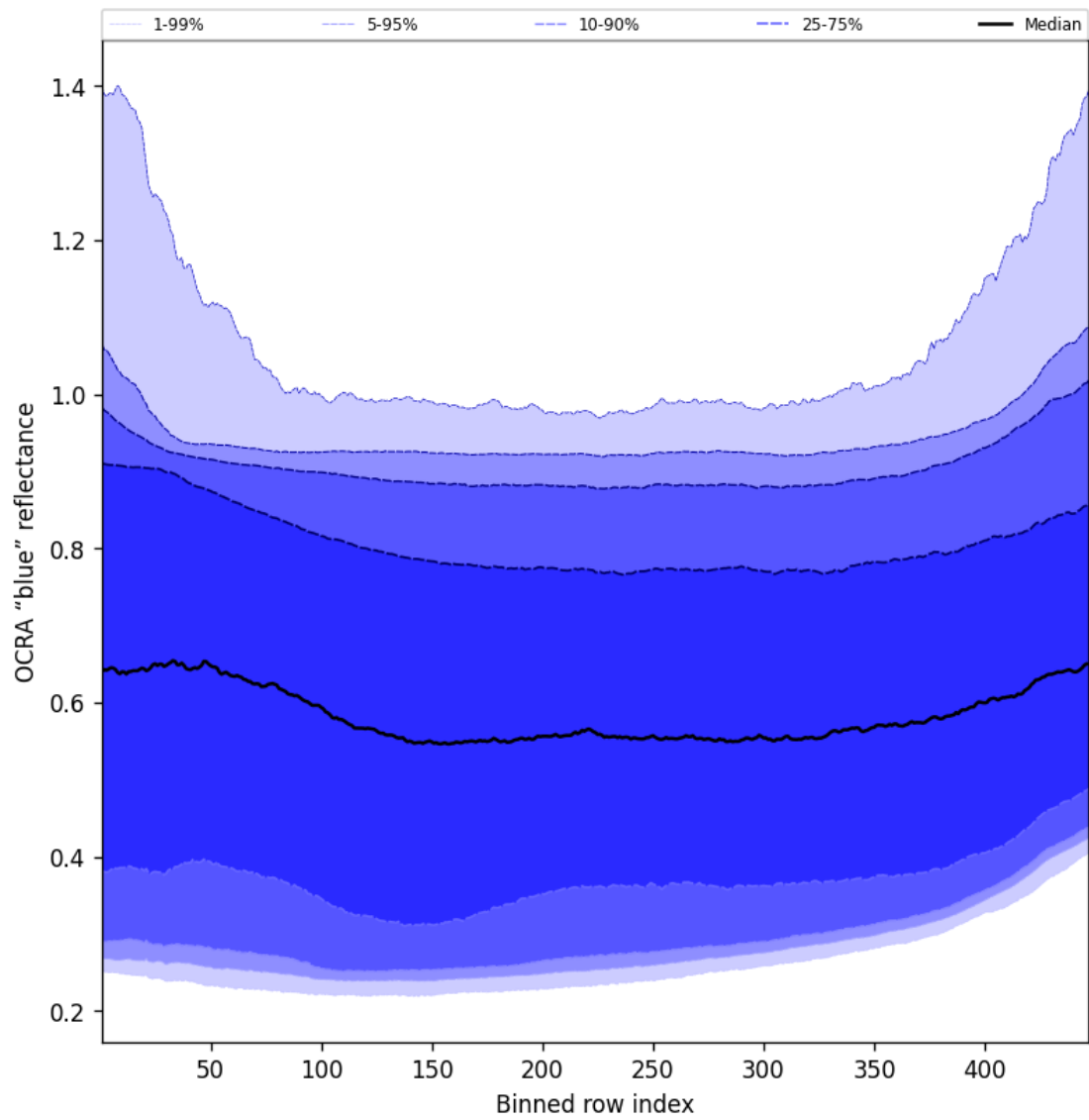
Figure 65: Along track statistics of “OCRA “blue” reflectance” for 2024-12-10 to 2024-12-11
