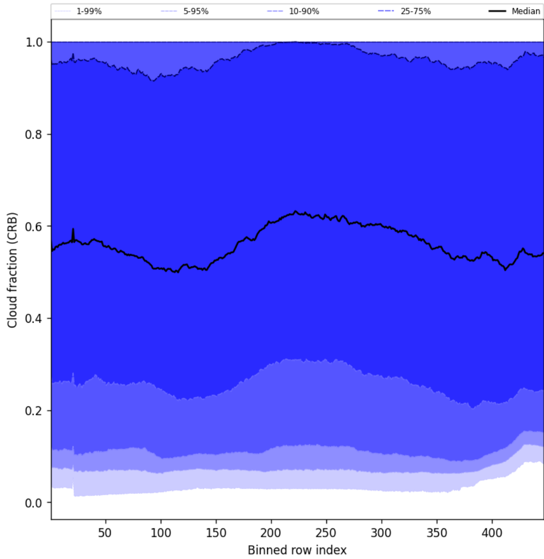
Figure 56: Along track statistics of “Cloud fraction (CRB)” for 2024-12-10 to 2024-12-11
