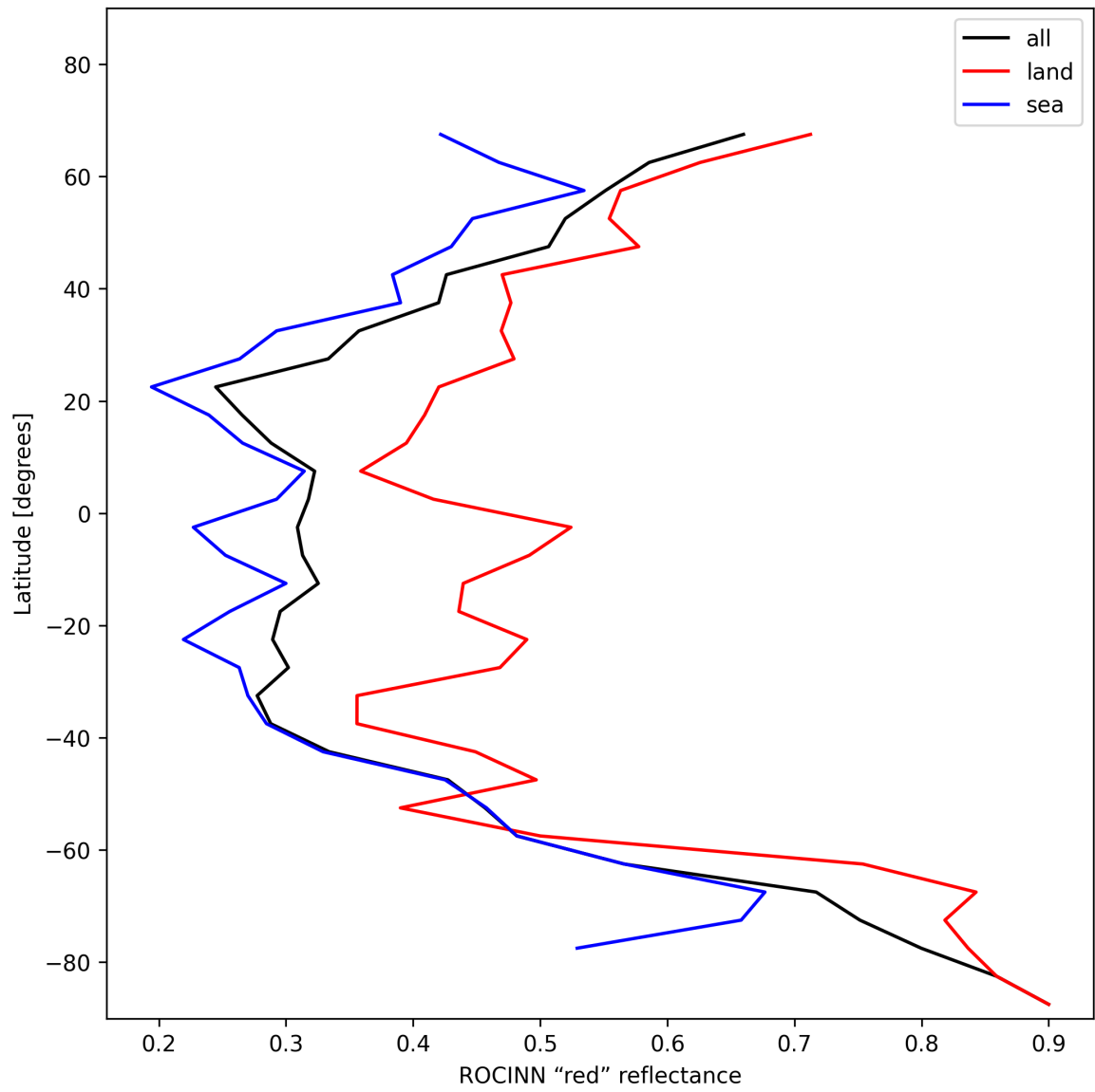
Figure 35: Zonal average of “ROCINN “red” reflectance” for 2024-12-10 to 2024-12-11.
