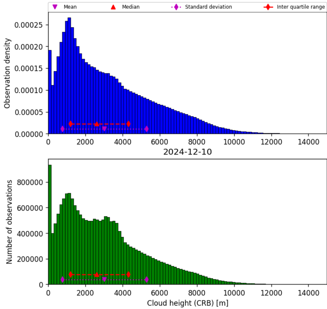
Figure 41: Histogram of “Cloud height (CRB)” for 2024-12-10 to 2024-12-11
