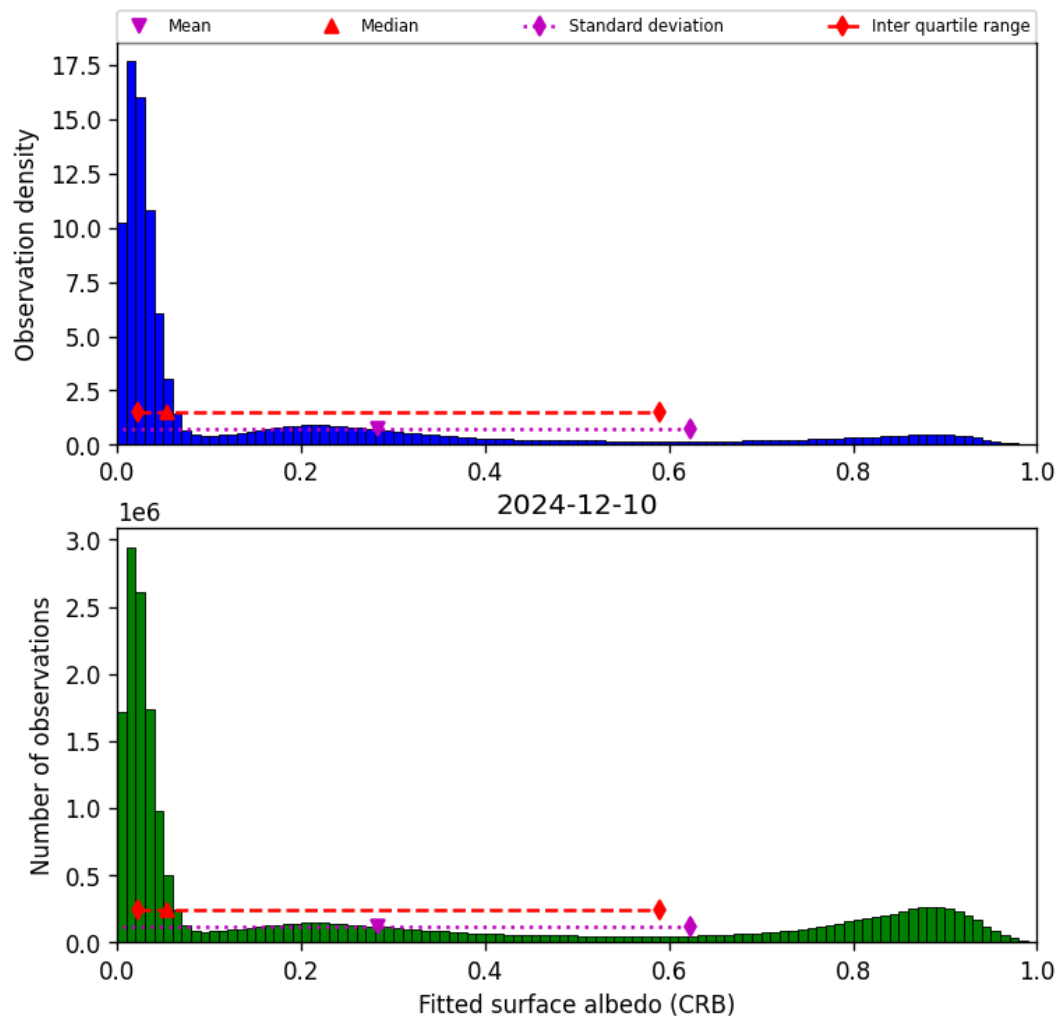
Figure 44: Histogram of “Fitted surface albedo (CRB)” for 2024-12-10 to 2024-12-11
