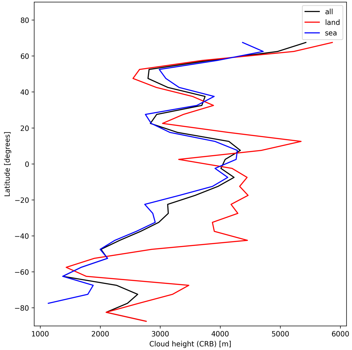
Figure 25: Zonal average of “Cloud height (CRB)” for 2024-12-10 to 2024-12-11.
