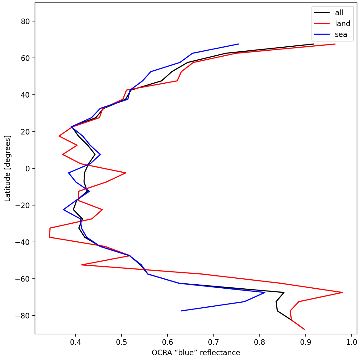
Figure 33: Zonal average of “OCRA “blue” reflectance” for 2024-12-10 to 2024-12-11.
