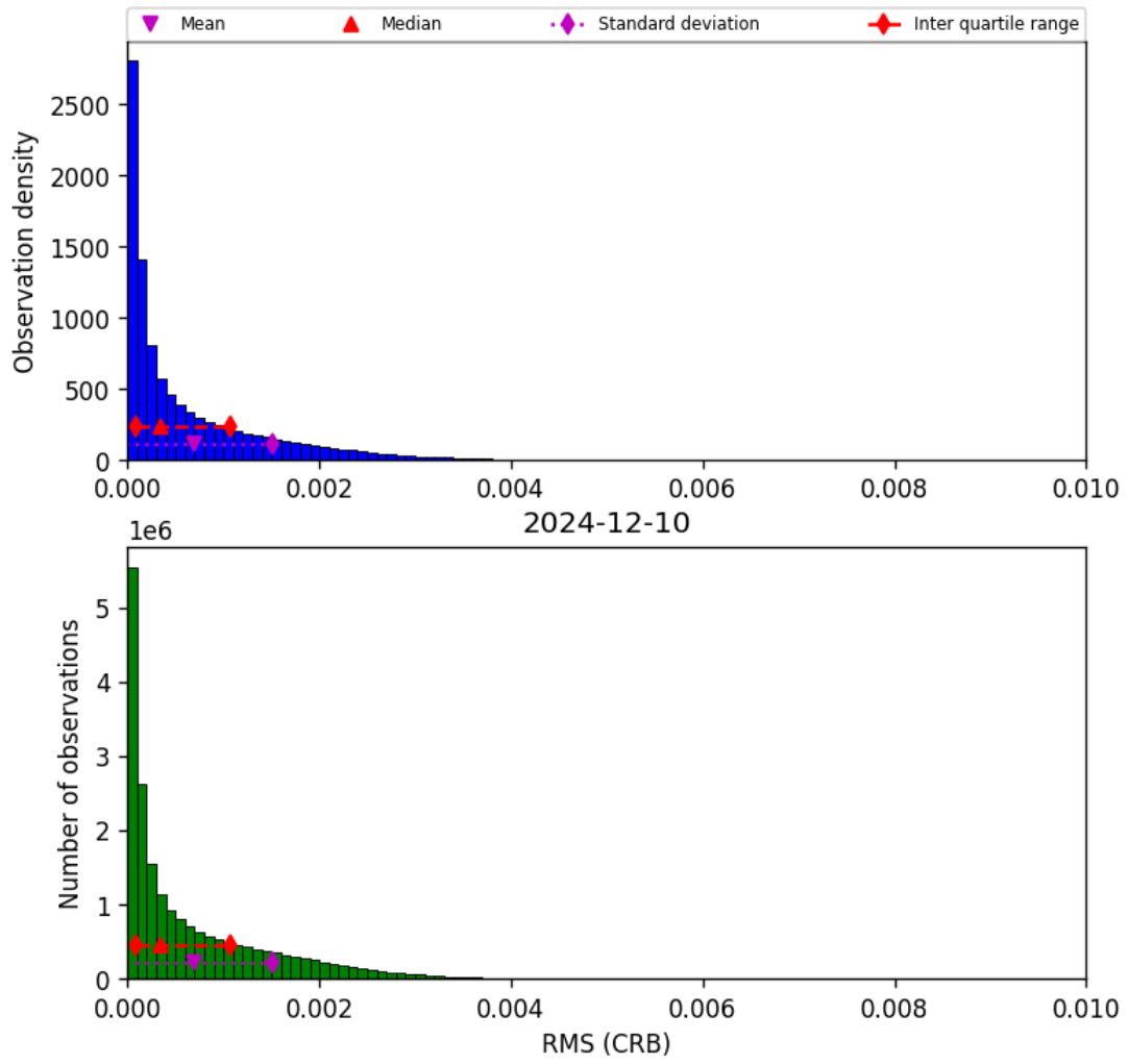
Figure 46: Histogram of "RMS (CRB)" for 2024-12-10 to 2024-12-11
