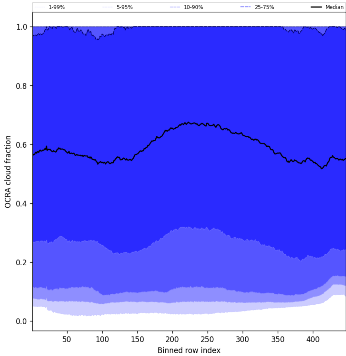
Figure 64: Along track statistics of “OCRA cloud fraction” for 2024-12-10 to 2024-12-11
