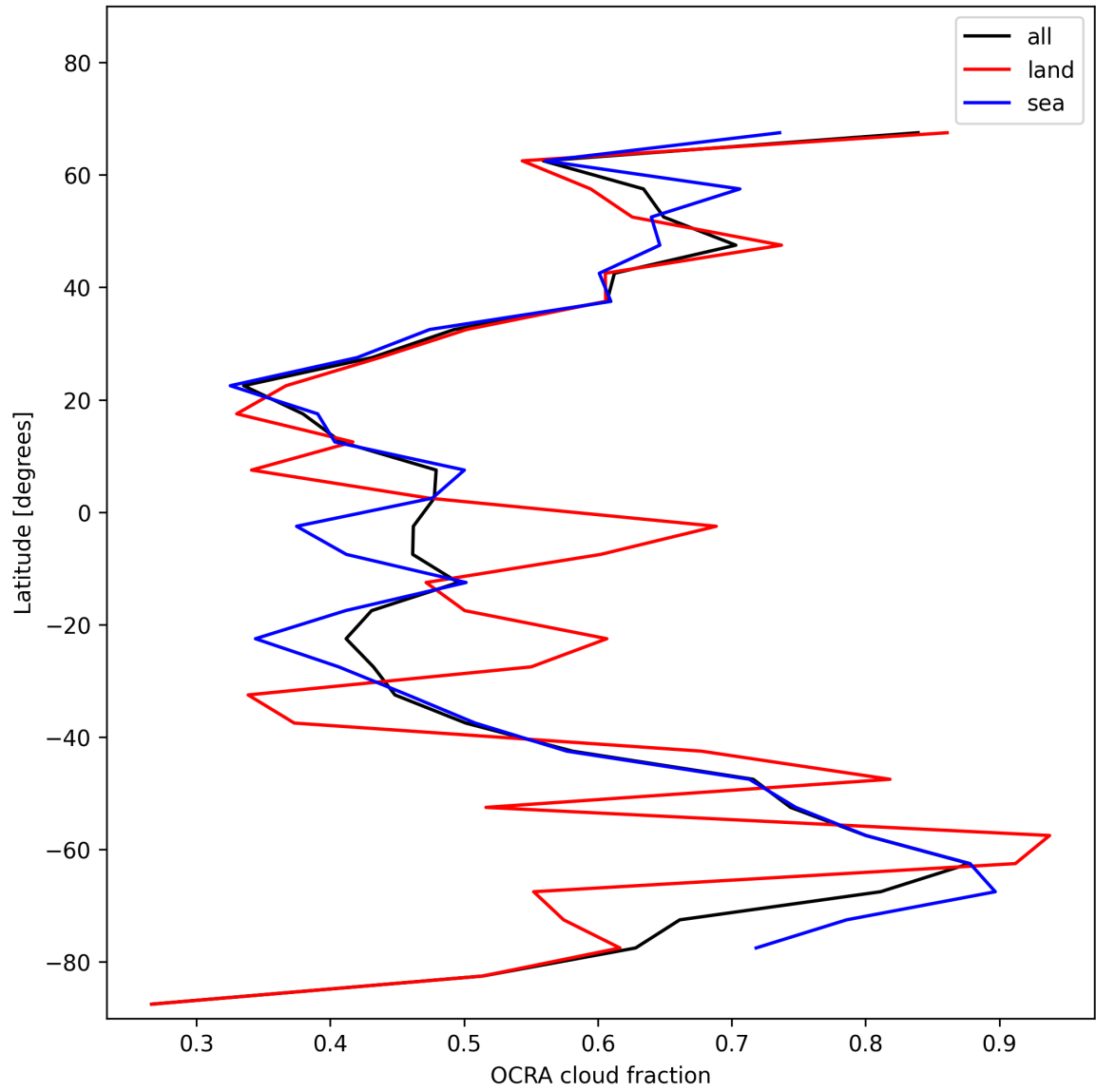
Figure 32: Zonal average of “OCRA cloud fraction” for 2024-12-10 to 2024-12-11.
