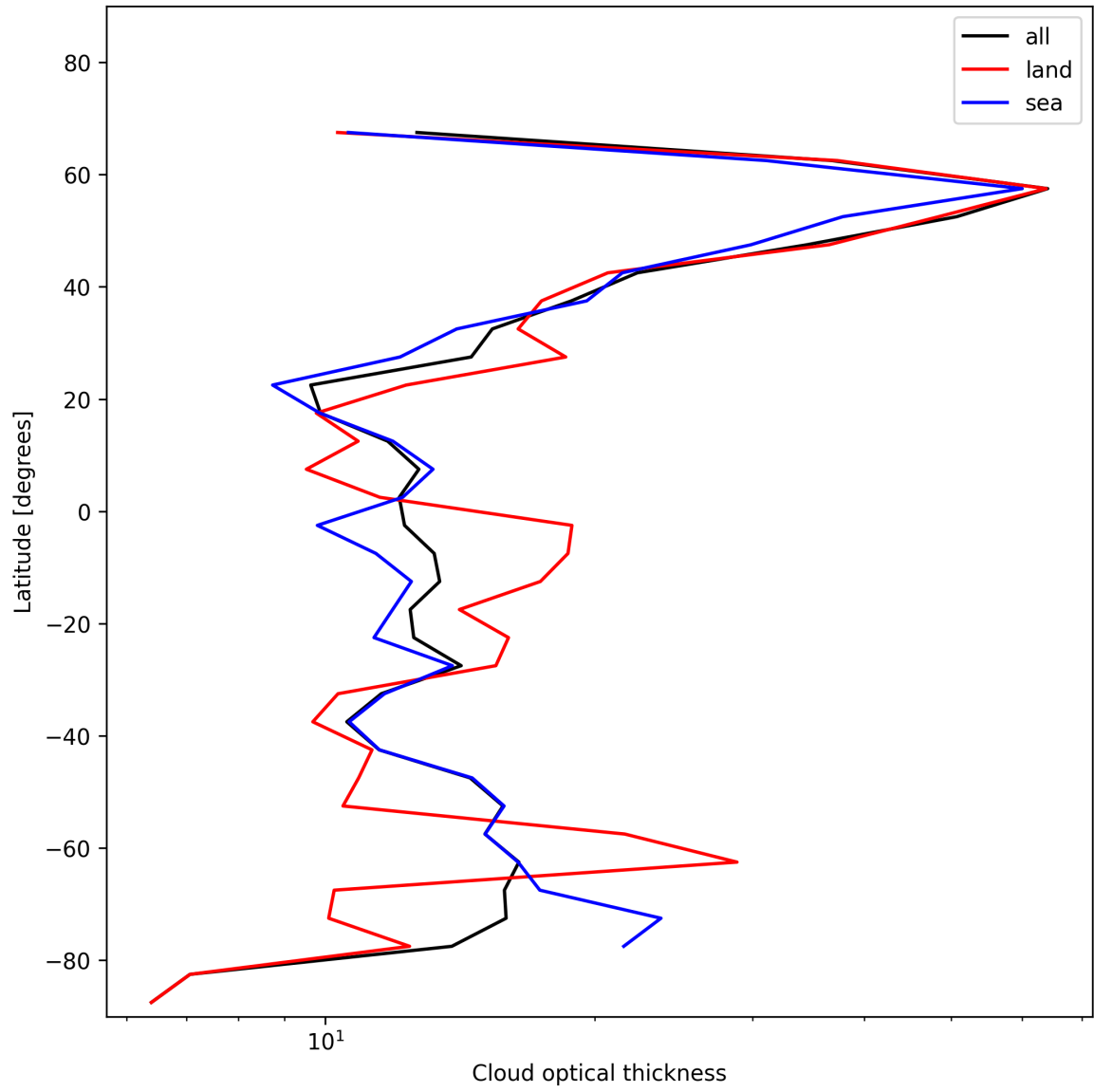
Figure 23: Zonal average of “Cloud optical thickness” for 2024-12-10 to 2024-12-11.
