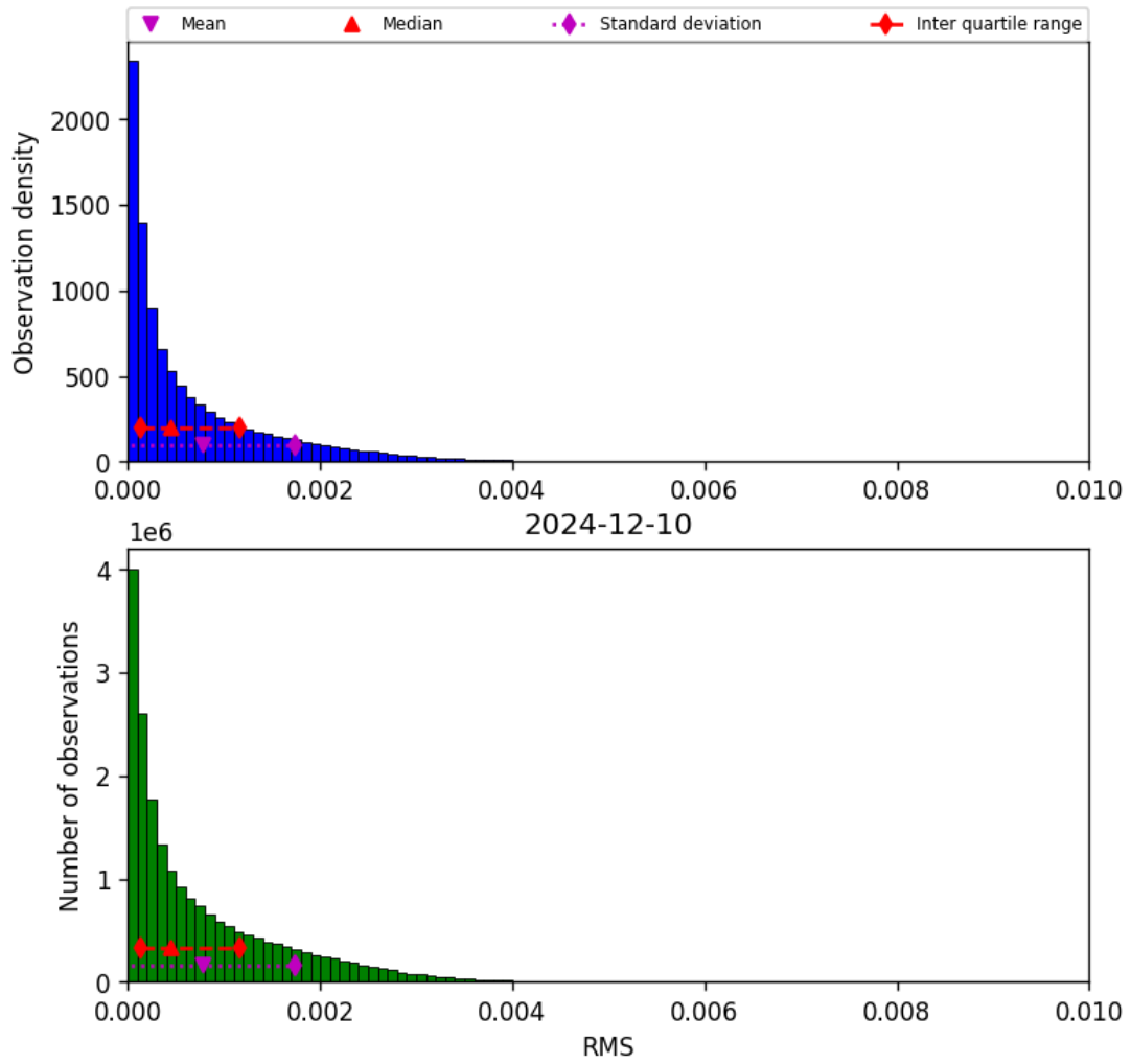
Figure 45: Histogram of “RMS” for 2024-12-10 to 2024-12-11
