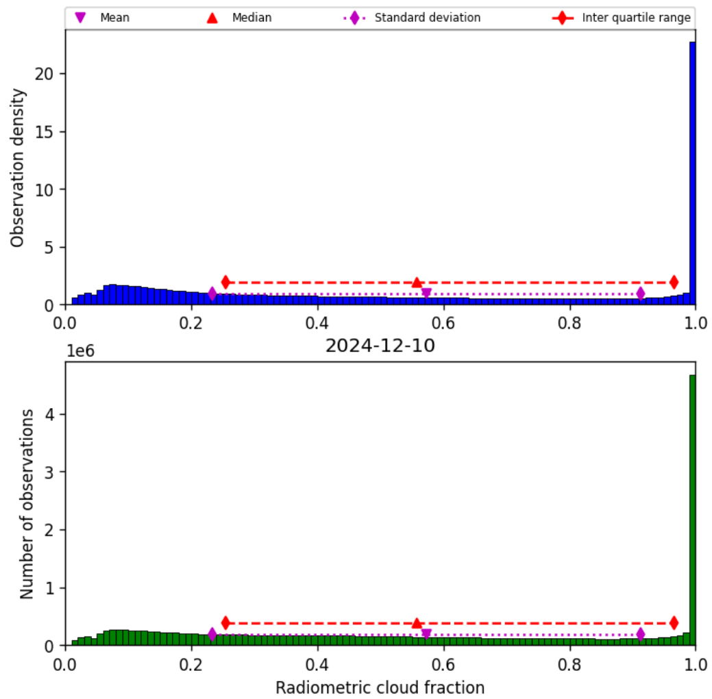
Figure 37: Histogram of “Radiometric cloud fraction” for 2024-12-10 to 2024-12-11
