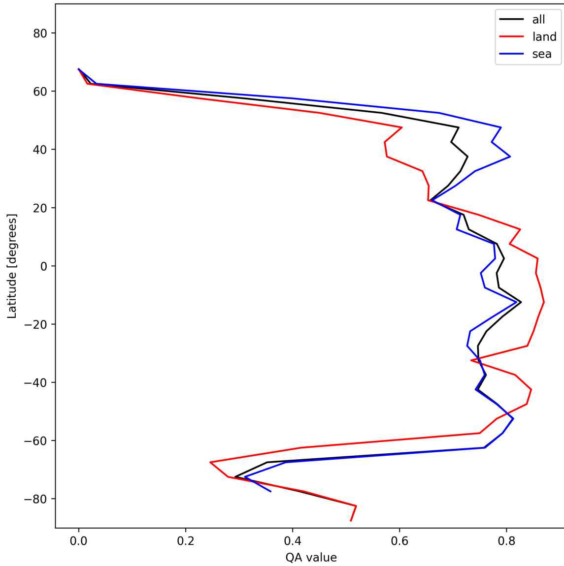
Figure 20: Zonal average of “QA value” for 2024-12-10 to 2024-12-11.
