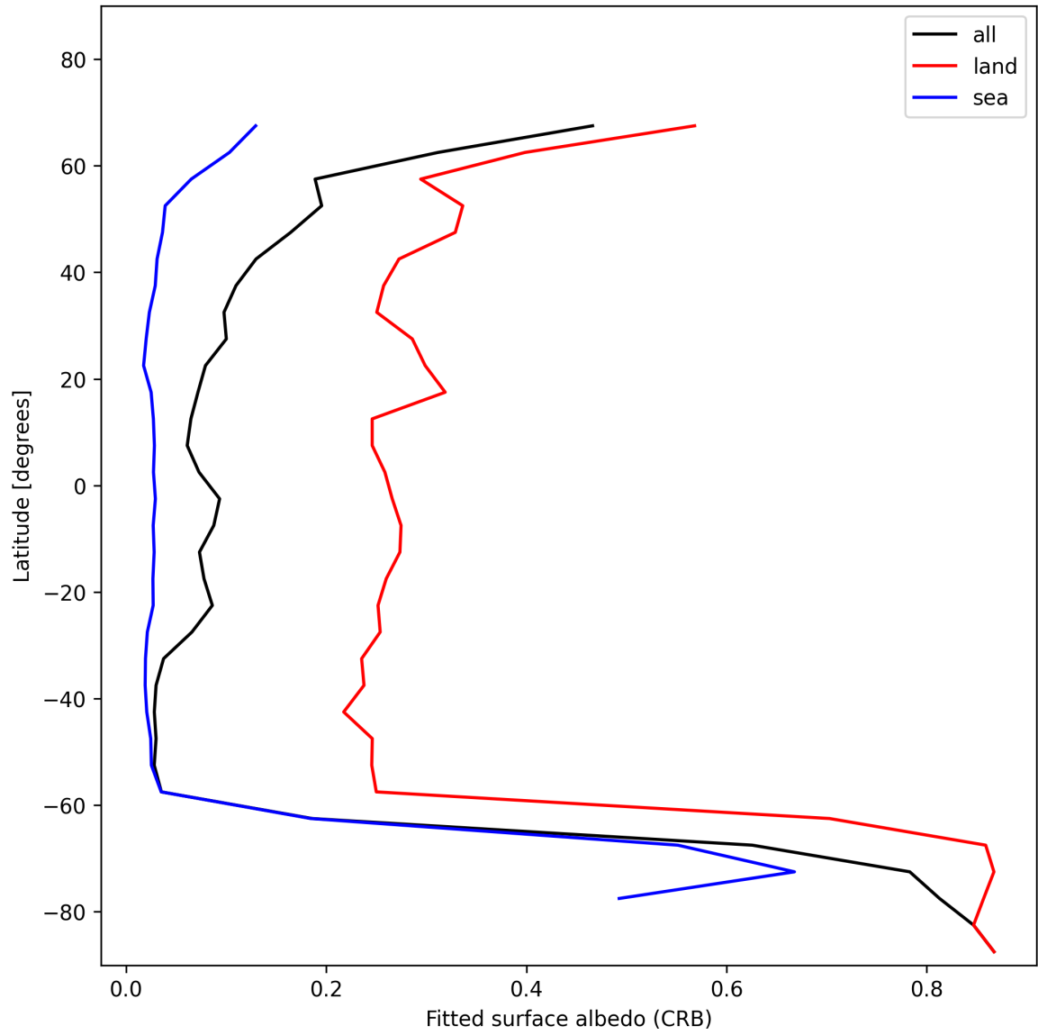
Figure 28: Zonal average of “Fitted surface albedo (CRB)” for 2024-12-10 to 2024-12-11.
