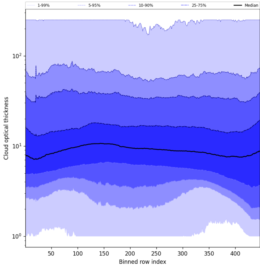
Figure 55: Along track statistics of “Cloud optical thickness” for 2024-12-10 to 2024-12-11
