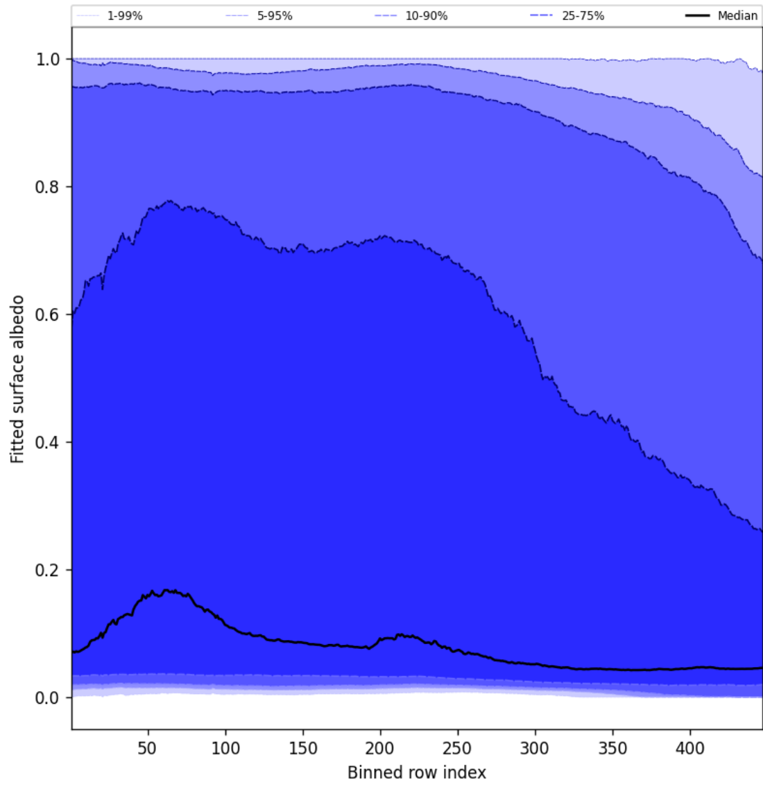
Figure 59: Along track statistics of “Fitted surface albedo” for 2024-12-10 to 2024-12-11
