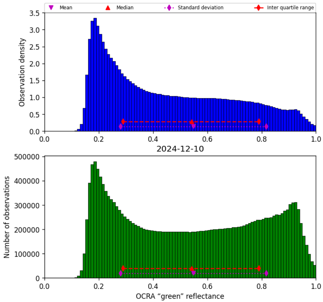
Figure 50: Histogram of “OCRA “green” reflectance” for 2024-12-10 to 2024-12-11
