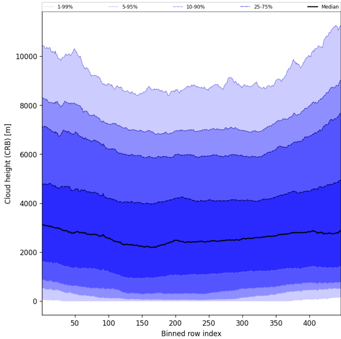
Figure 57: Along track statistics of “Cloud height (CRB)” for 2024-12-10 to 2024-12-11
