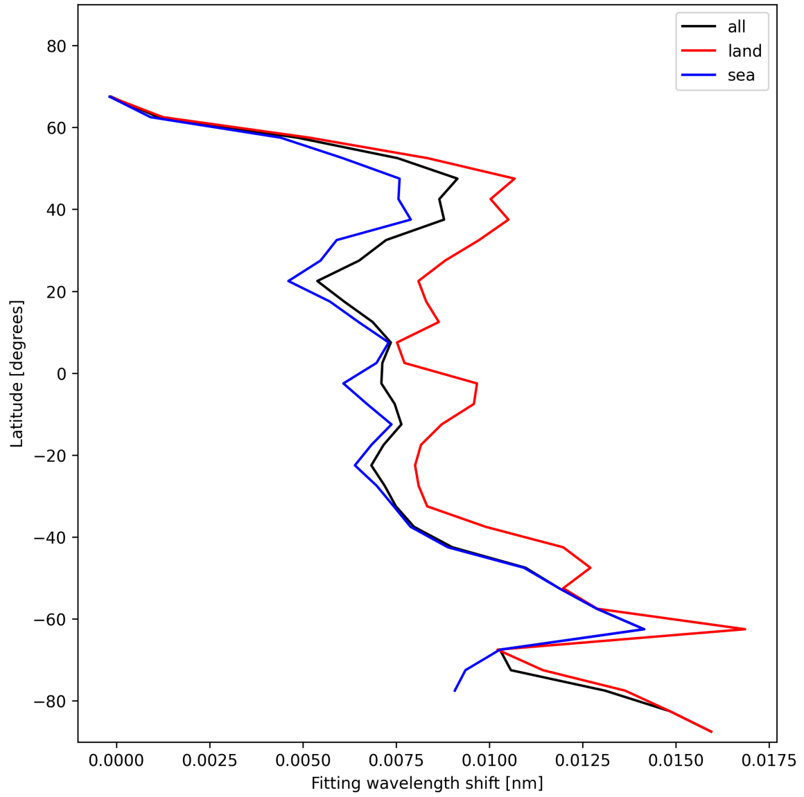
Figure 31: Zonal average of “Fitting wavelength shift” for 2024-12-10 to 2024-12-11.
