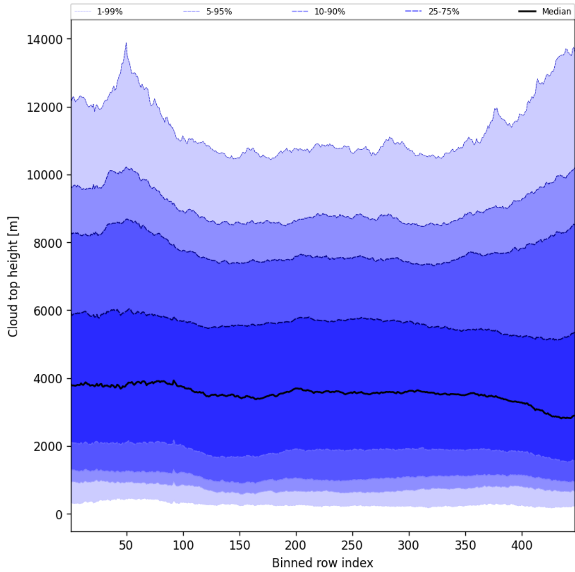
Figure 54: Along track statistics of “Cloud top height” for 2024-12-10 to 2024-12-11
