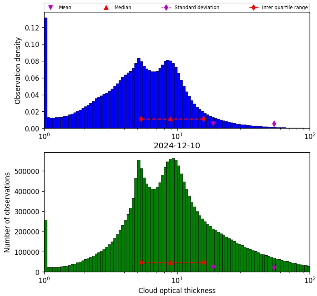
Figure 39: Histogram of “Cloud optical thickness” for 2024-12-10 to 2024-12-11
