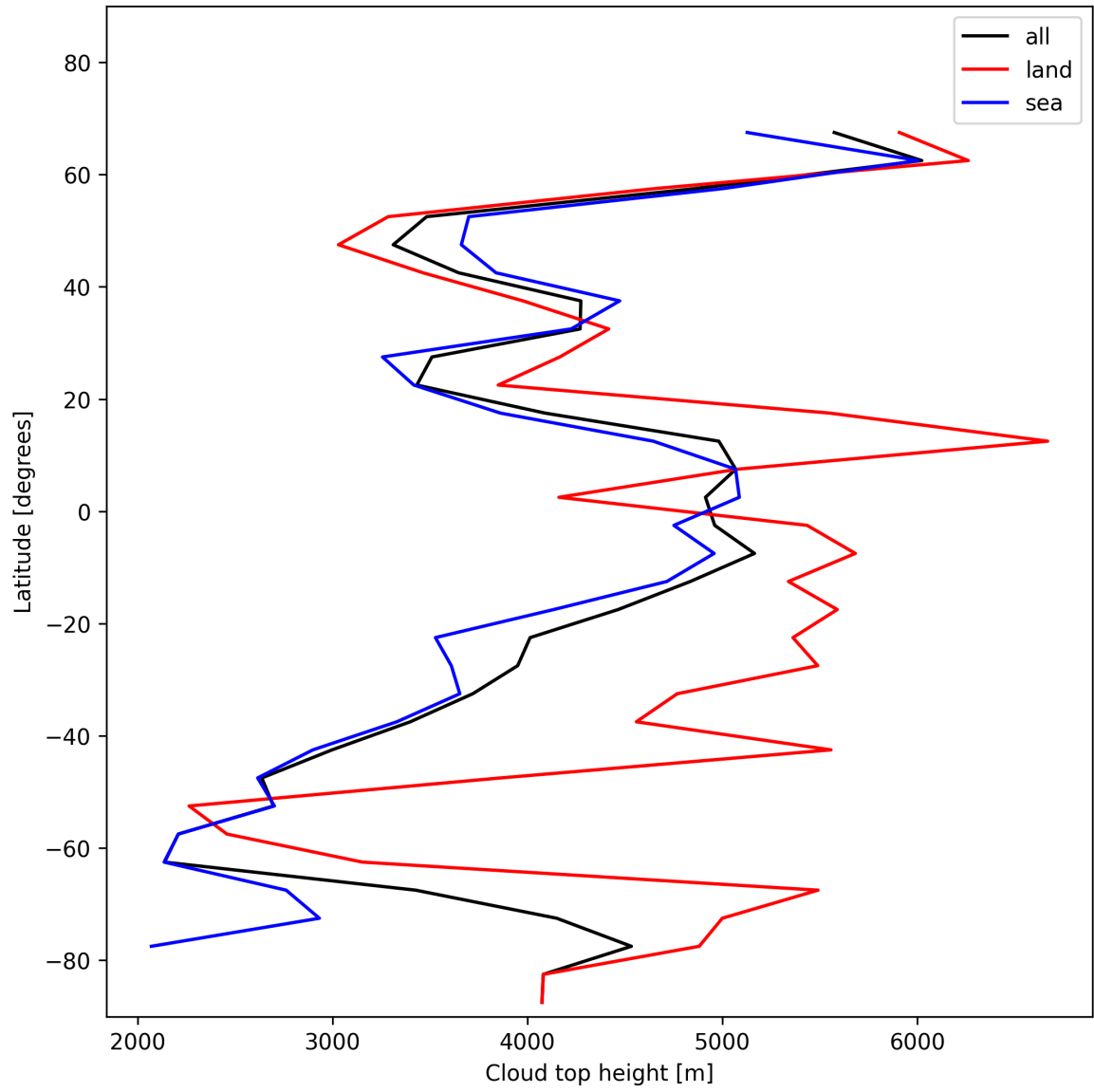
Figure 22: Zonal average of “Cloud top height” for 2024-12-10 to 2024-12-11.
