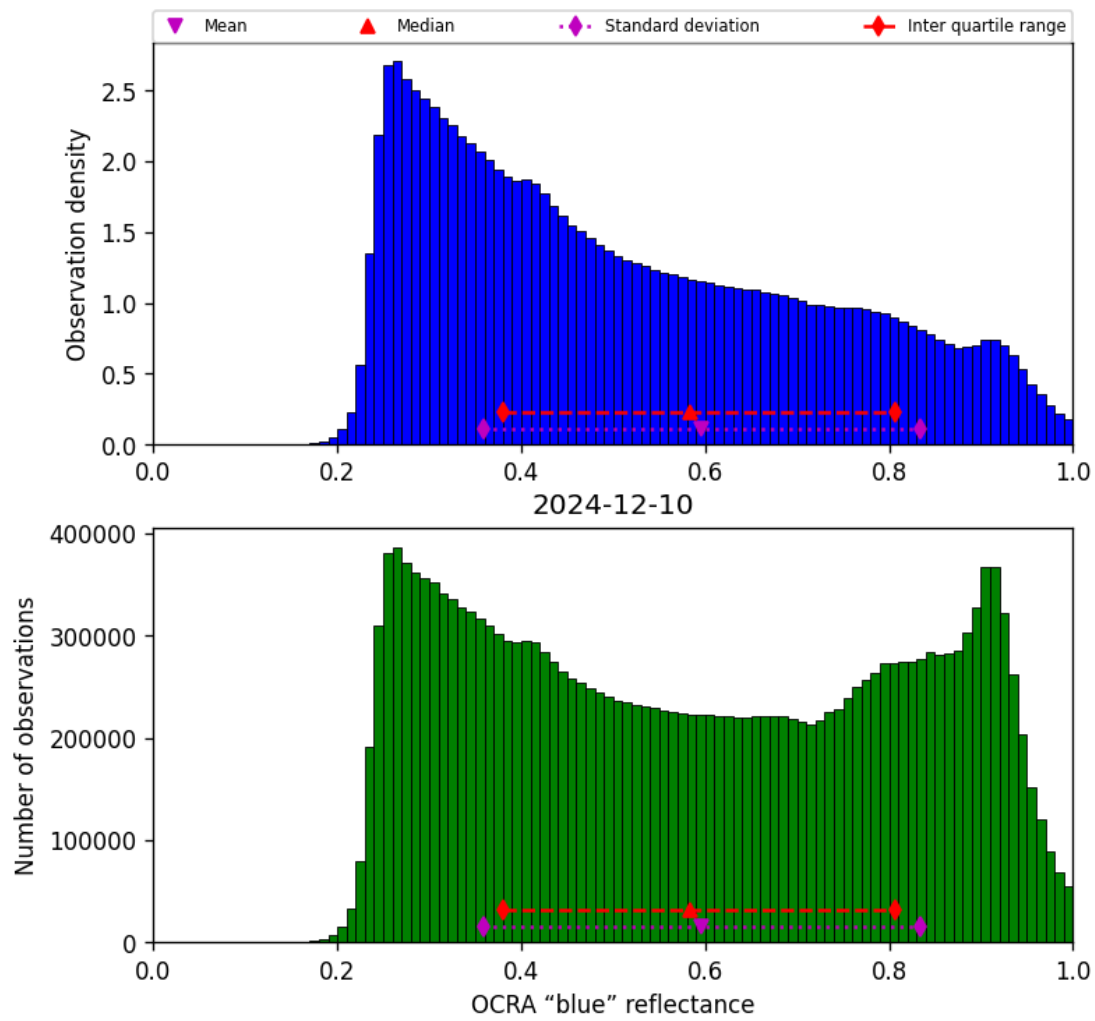
Figure 49: Histogram of "OCRA "blue" reflectance" for 2024-12-10 to 2024-12-11
