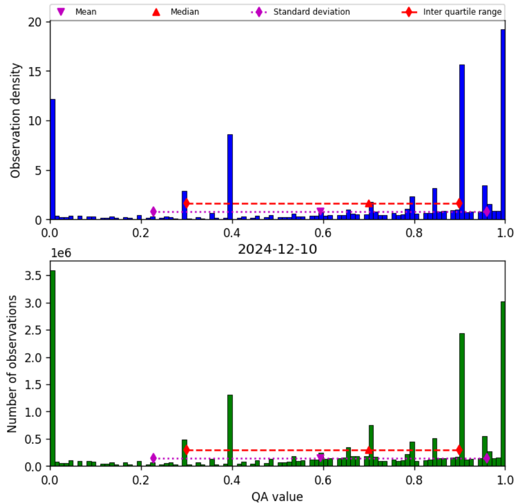
Figure 36: Histogram of “QA value” for 2024-12-10 to 2024-12-11
