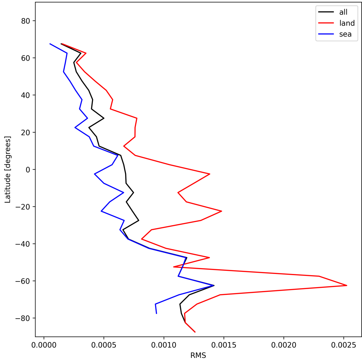
Figure 29: Zonal average of “RMS” for 2024-12-10 to 2024-12-11.
