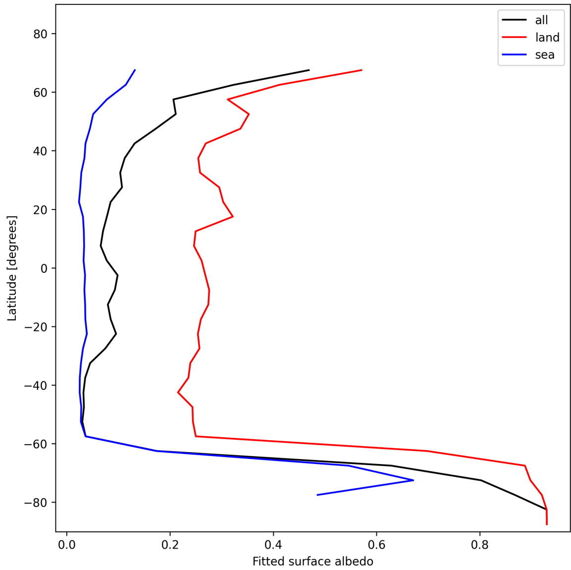
Figure 27: Zonal average of “Fitted surface albedo” for 2024-12-10 to 2024-12-11.
