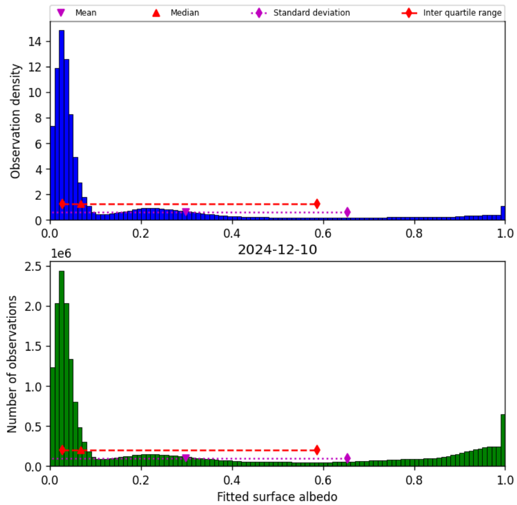
Figure 43: Histogram of “Fitted surface albedo” for 2024-12-10 to 2024-12-11
