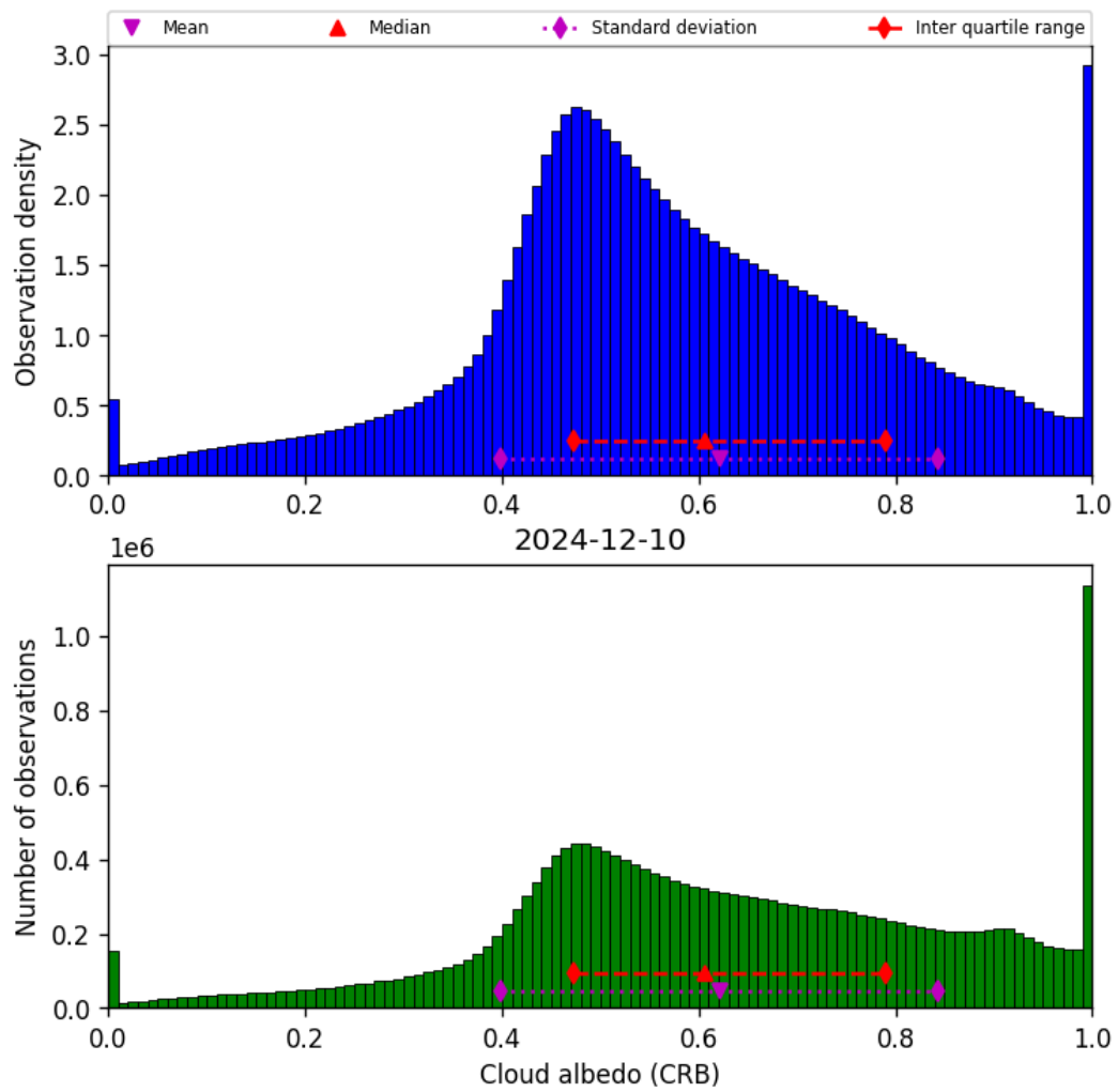
Figure 42: Histogram of “Cloud albedo (CRB)” for 2024-12-10 to 2024-12-11
