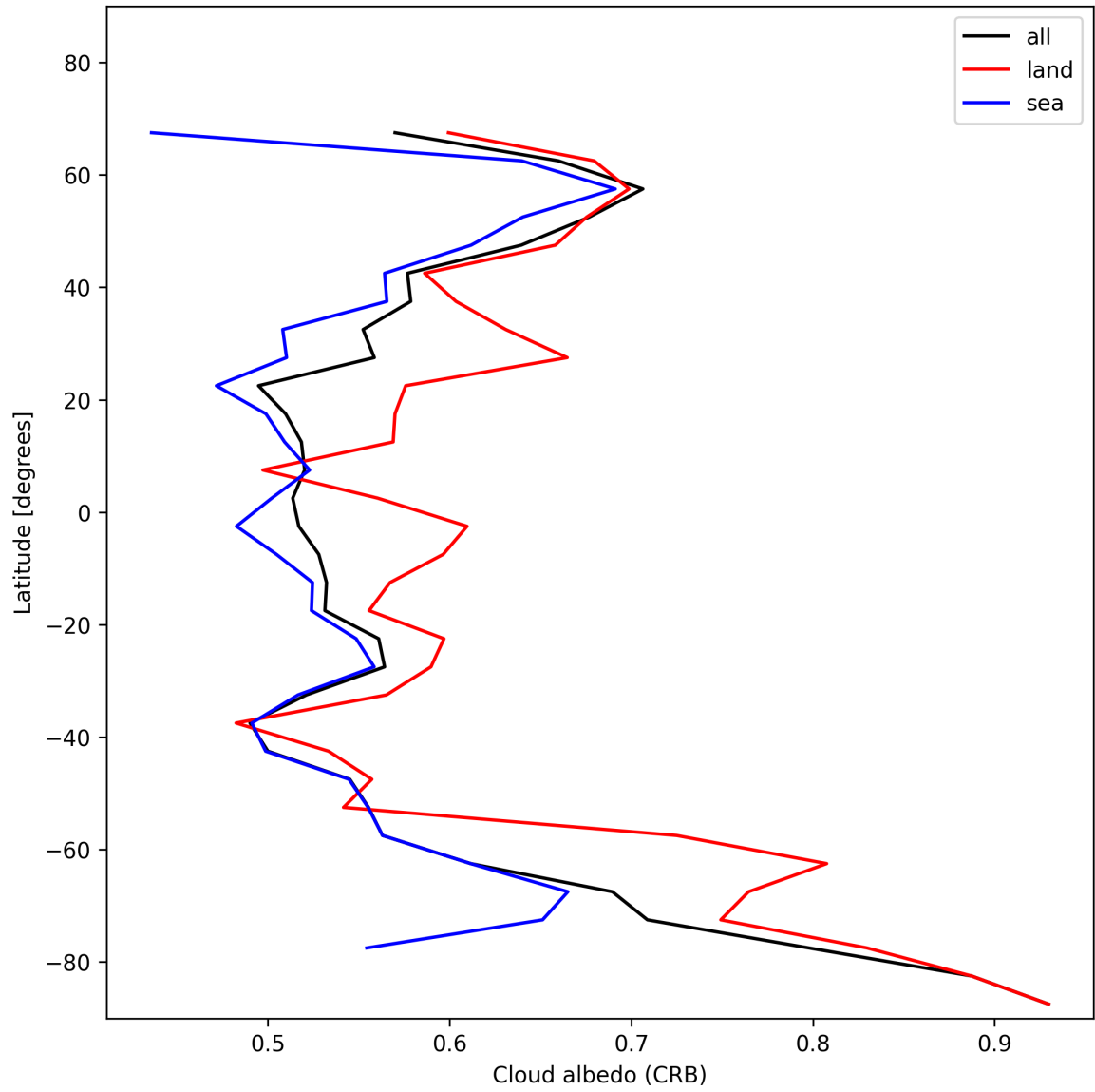
Figure 26: Zonal average of “Cloud albedo (CRB)” for 2024-12-10 to 2024-12-11.
