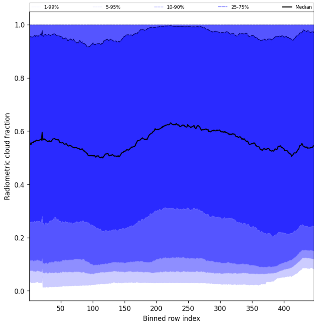
Figure 53: Along track statistics of “Radiometric cloud fraction” for 2024-12-10 to 2024-12-11
