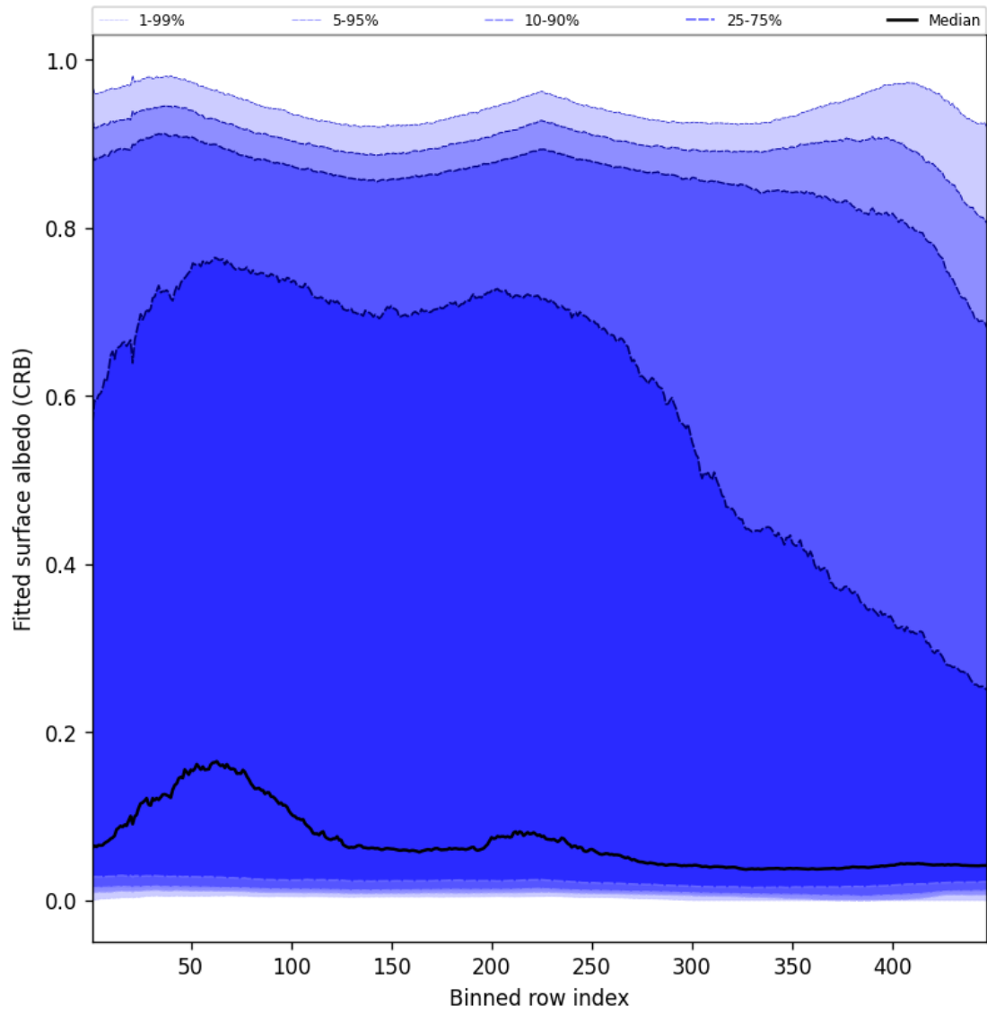
Figure 60: Along track statistics of “Fitted surface albedo (CRB)” for 2024-12-10 to 2024-12-11
