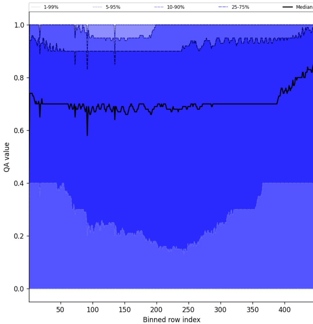
Figure 52: Along track statistics of “QA value” for 2024-12-10 to 2024-12-11
