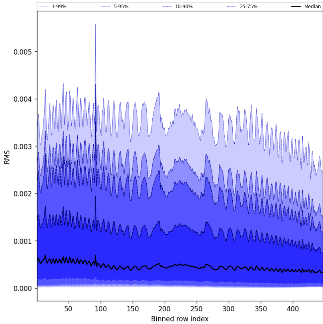
Figure 61: Along track statistics of “RMS” for 2024-12-10 to 2024-12-11
