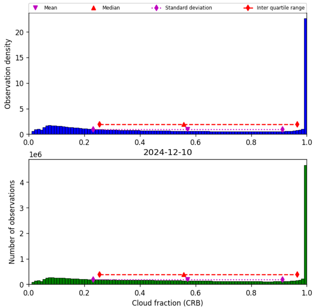
Figure 40: Histogram of “Cloud fraction (CRB)” for 2024-12-10 to 2024-12-11
