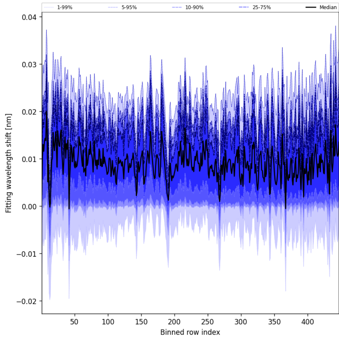
Figure 63: Along track statistics of “Fitting wavelength shift” for 2024-12-10 to 2024-12-11
