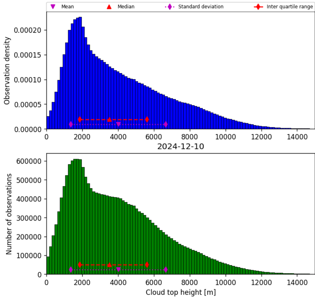
Figure 38: Histogram of “Cloud top height” for 2024-12-10 to 2024-12-11
