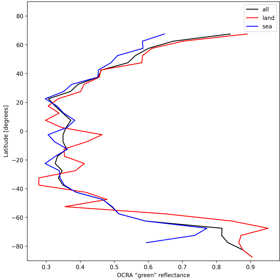
Figure 34: Zonal average of “OCRA “green” reflectance” for 2024-12-10 to 2024-12-11.
