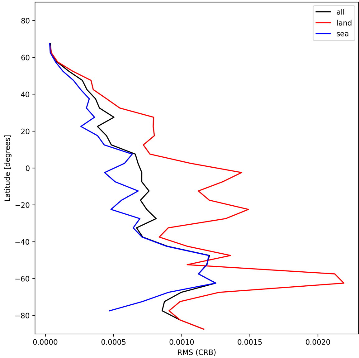
Figure 30: Zonal average of “RMS (CRB)” for 2024-12-10 to 2024-12-11.
