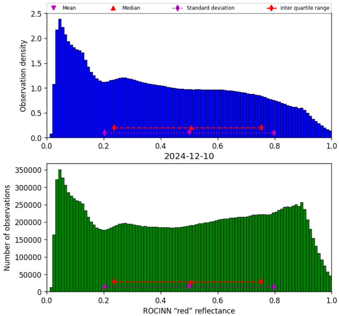
Figure 51: Histogram of “ROCINN “red” reflectance” for 2024-12-10 to 2024-12-11
