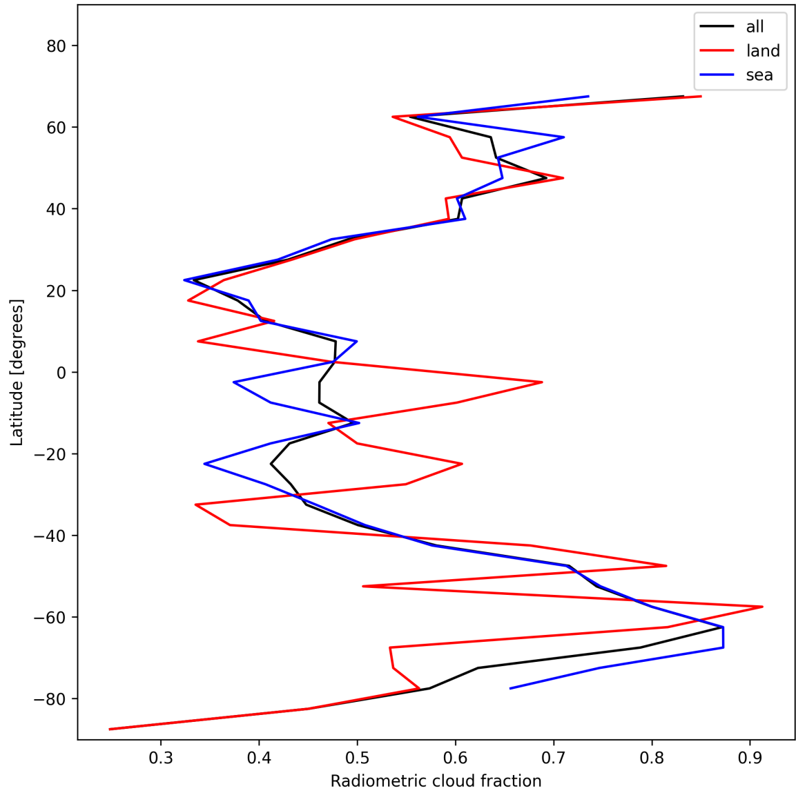
Figure 21: Zonal average of “Radiometric cloud fraction” for 2024-12-10 to 2024-12-11.
