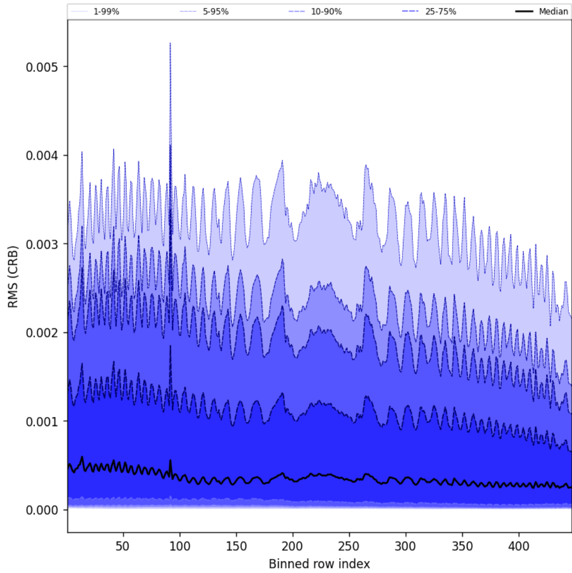
Figure 62: Along track statistics of “RMS (CRB)” for 2024-12-10 to 2024-12-11
