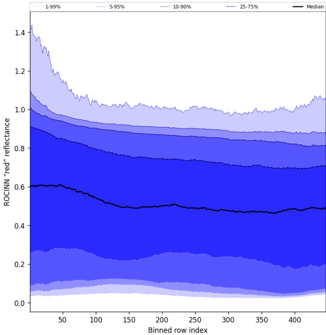
Figure 67: Along track statistics of “ROCINN “red” reflectance” for 2024-12-10 to 2024-12-11
