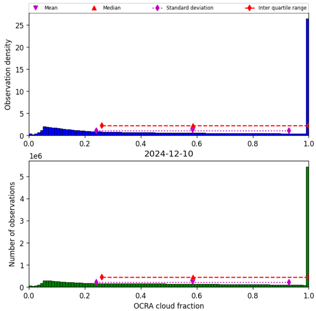
Figure 48: Histogram of “OCRA cloud fraction” for 2024-12-10 to 2024-12-11
