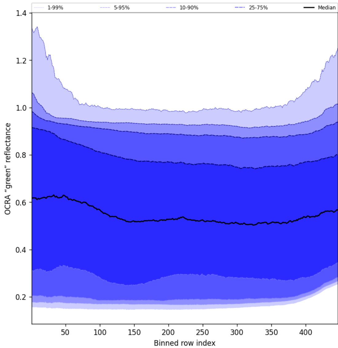
Figure 66: Along track statistics of “OCRA “green” reflectance” for 2024-12-10 to 2024-12-11
