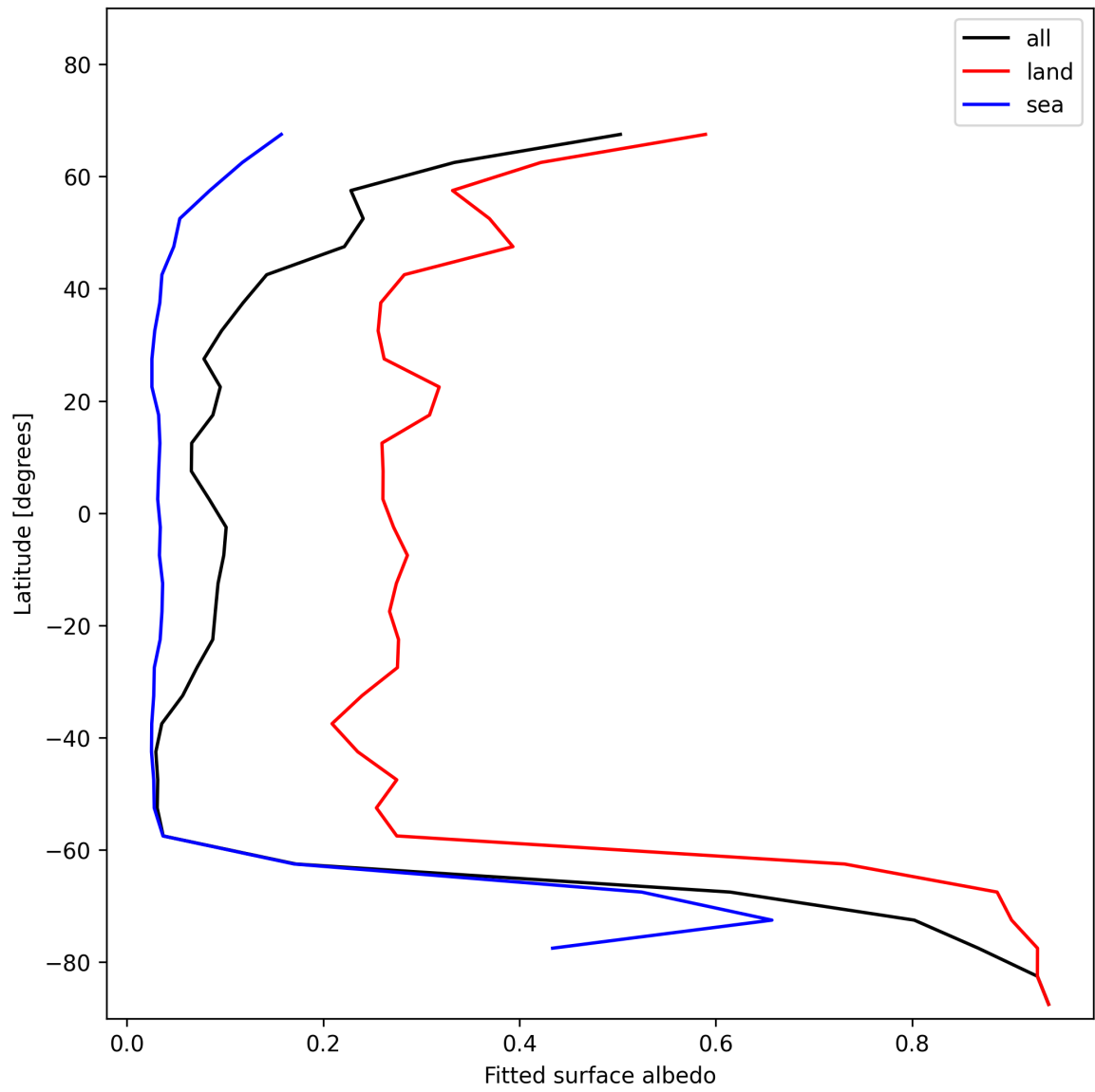
Figure 27: Zonal average of “Fitted surface albedo” for 2024-12-14 to 2024-12-14.
