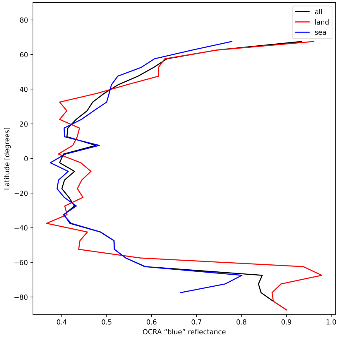
Figure 33: Zonal average of “OCRA “blue” reflectance” for 2024-12-14 to 2024-12-14.
