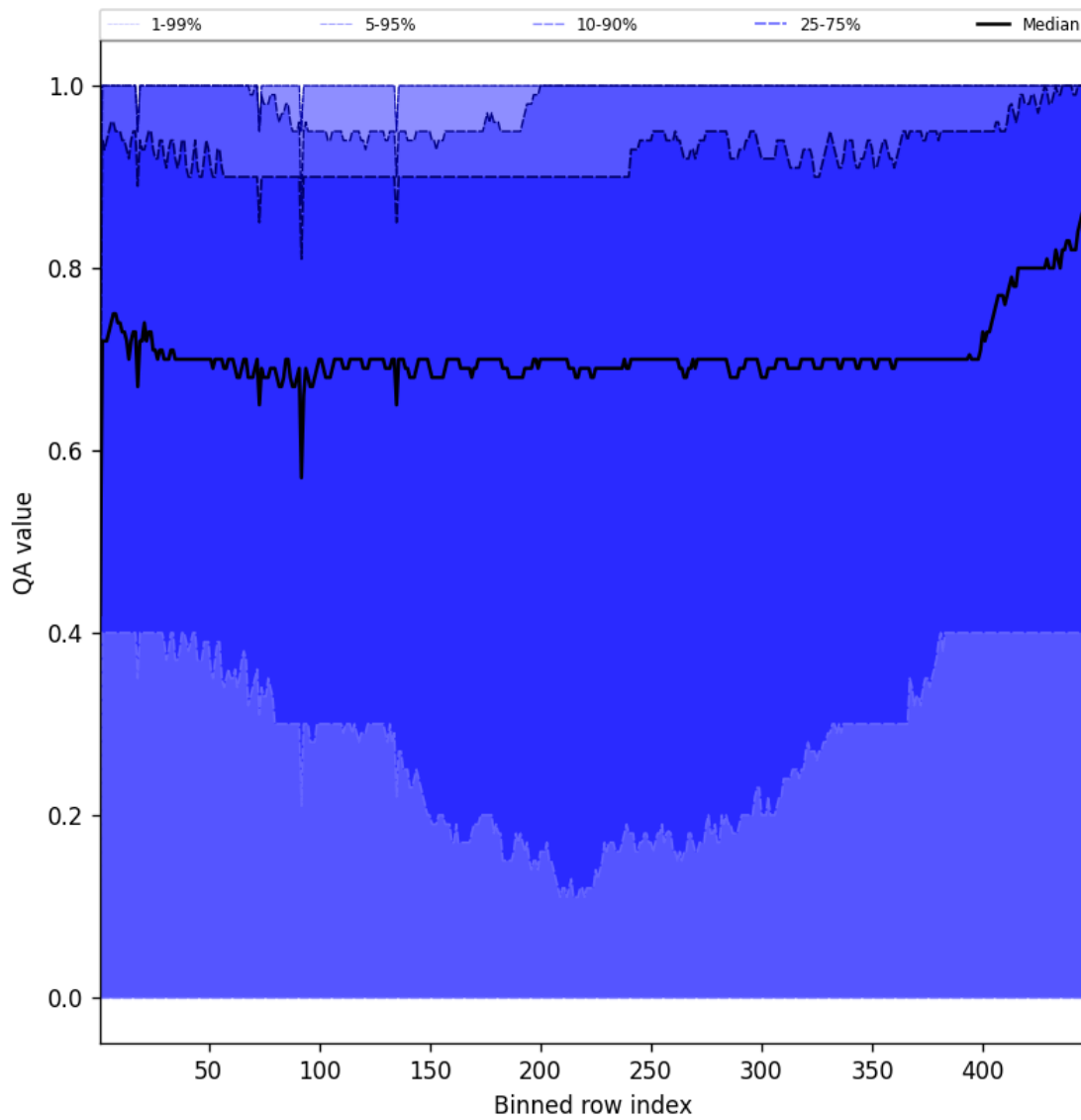
Figure 52: Along track statistics of “QA value” for 2024-12-14 to 2024-12-14
