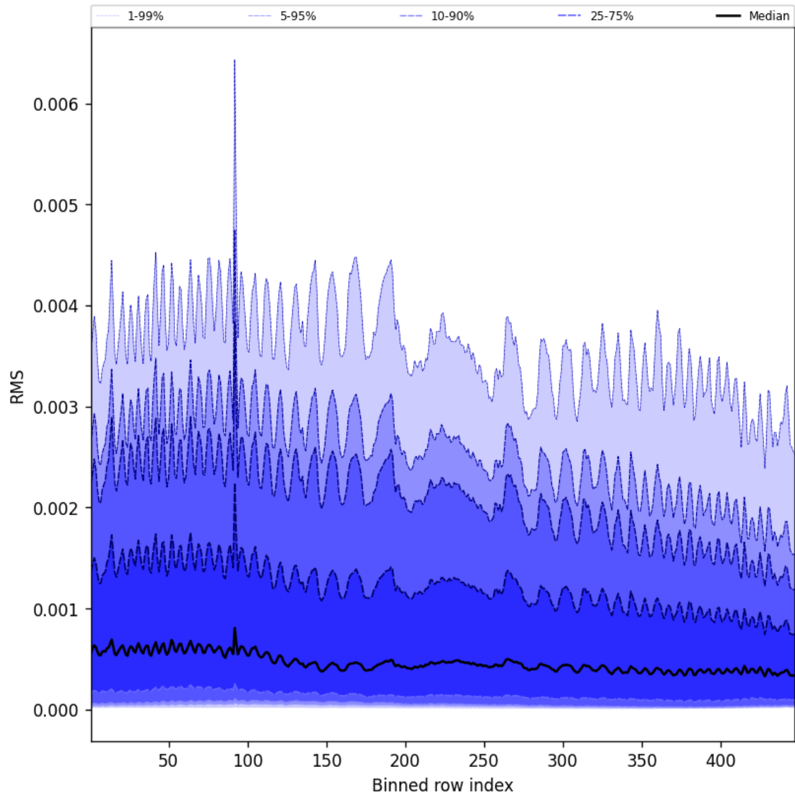
Figure 61: Along track statistics of “RMS” for 2024-12-14 to 2024-12-14
