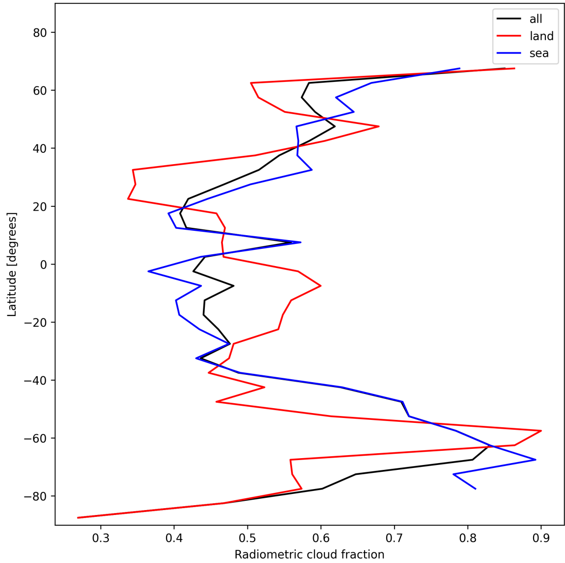
Figure 21: Zonal average of “Radiometric cloud fraction” for 2024-12-14 to 2024-12-14.
