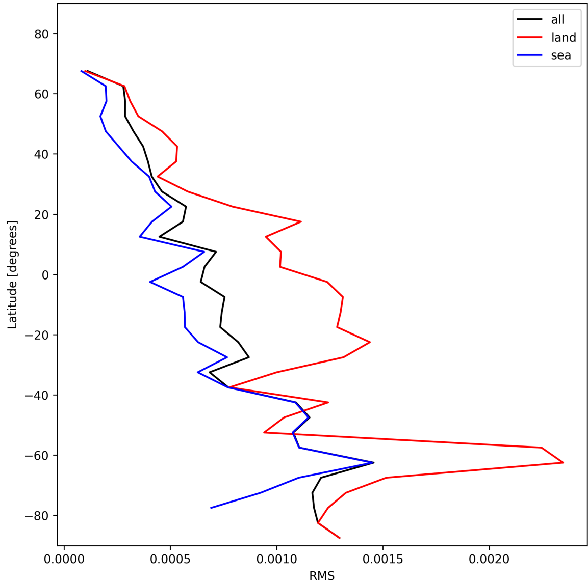
Figure 29: Zonal average of “RMS” for 2024-12-14 to 2024-12-14.
