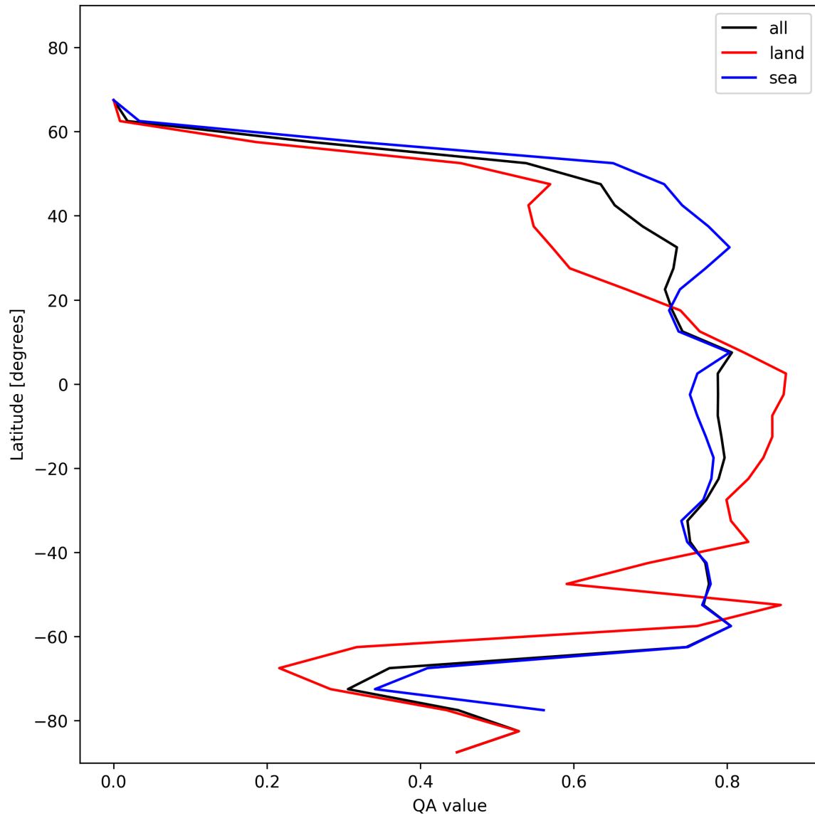
Figure 20: Zonal average of “QA value” for 2024-12-14 to 2024-12-14.
