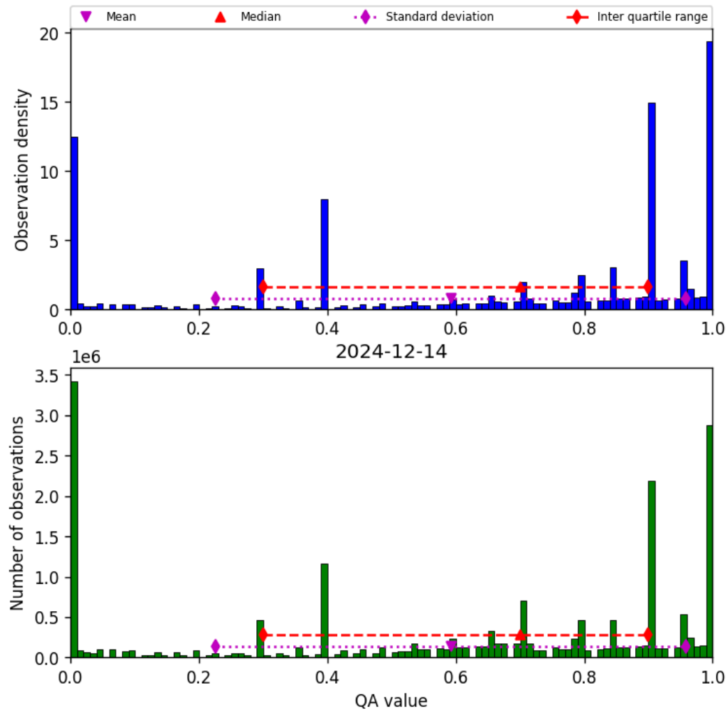
Figure 36: Histogram of “QA value” for 2024-12-14 to 2024-12-14
