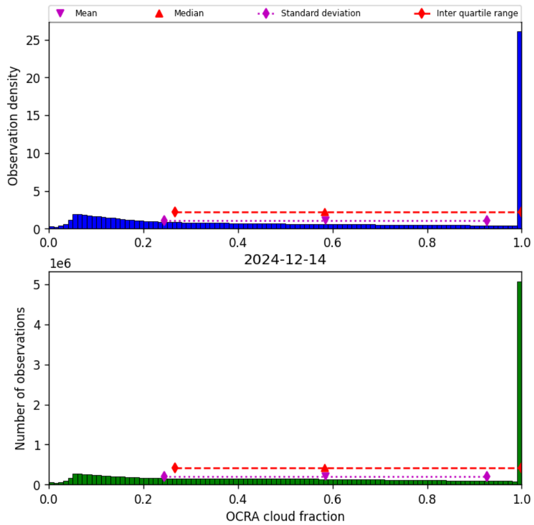
Figure 48: Histogram of “OCRA cloud fraction” for 2024-12-14 to 2024-12-14
