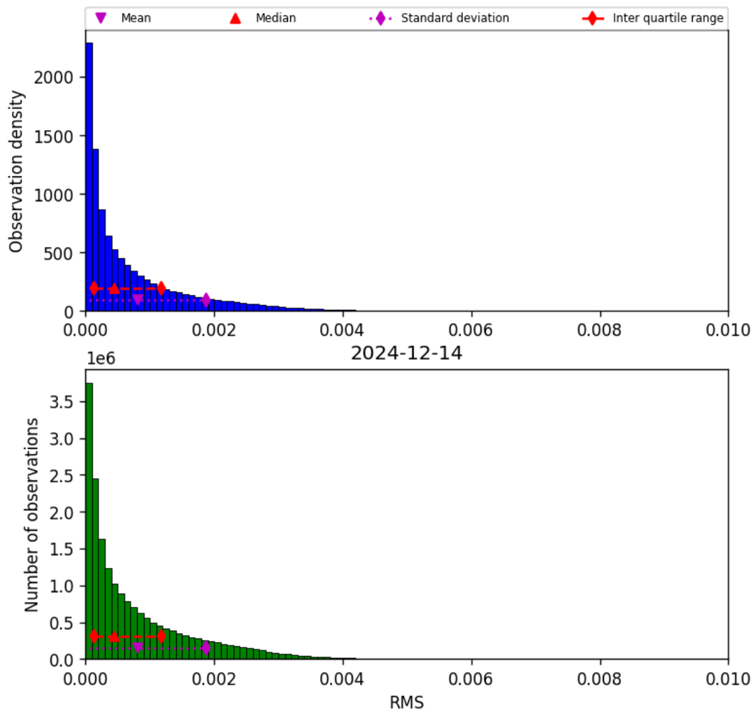
Figure 45: Histogram of “RMS” for 2024-12-14 to 2024-12-14
