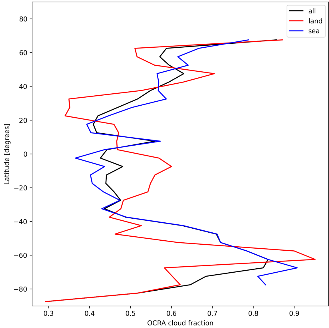
Figure 32: Zonal average of “OCRA cloud fraction” for 2024-12-14 to 2024-12-14.
