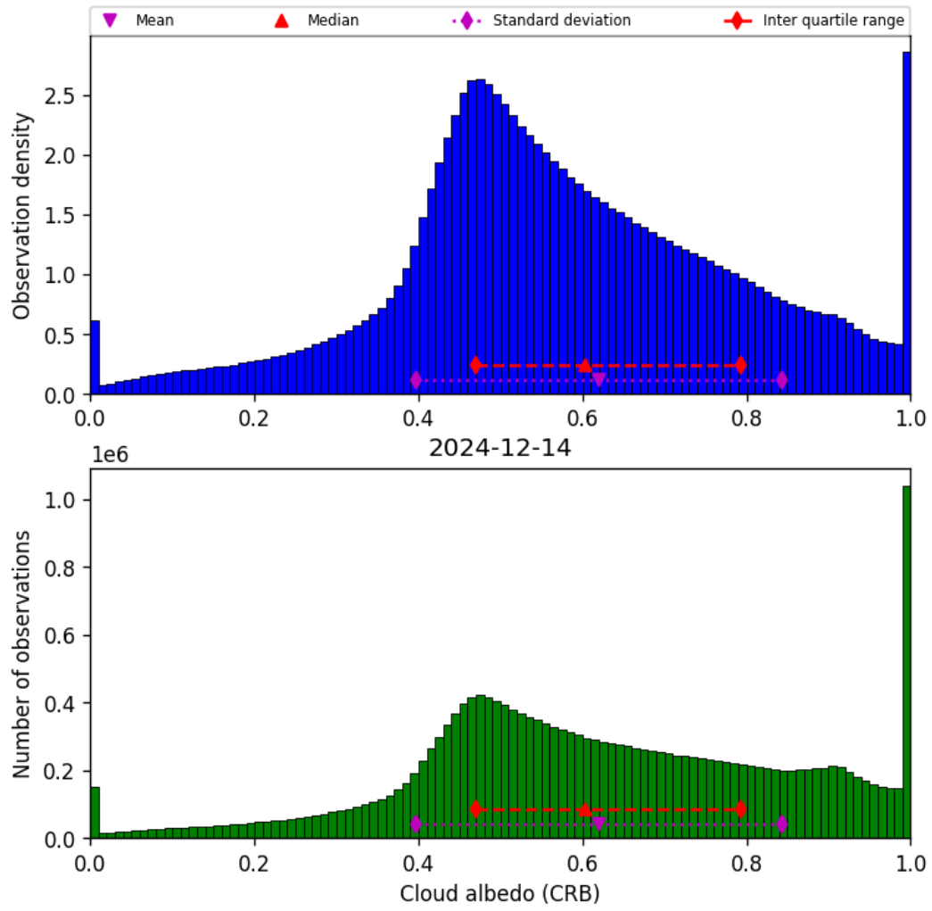
Figure 42: Histogram of “Cloud albedo (CRB)” for 2024-12-14 to 2024-12-14
