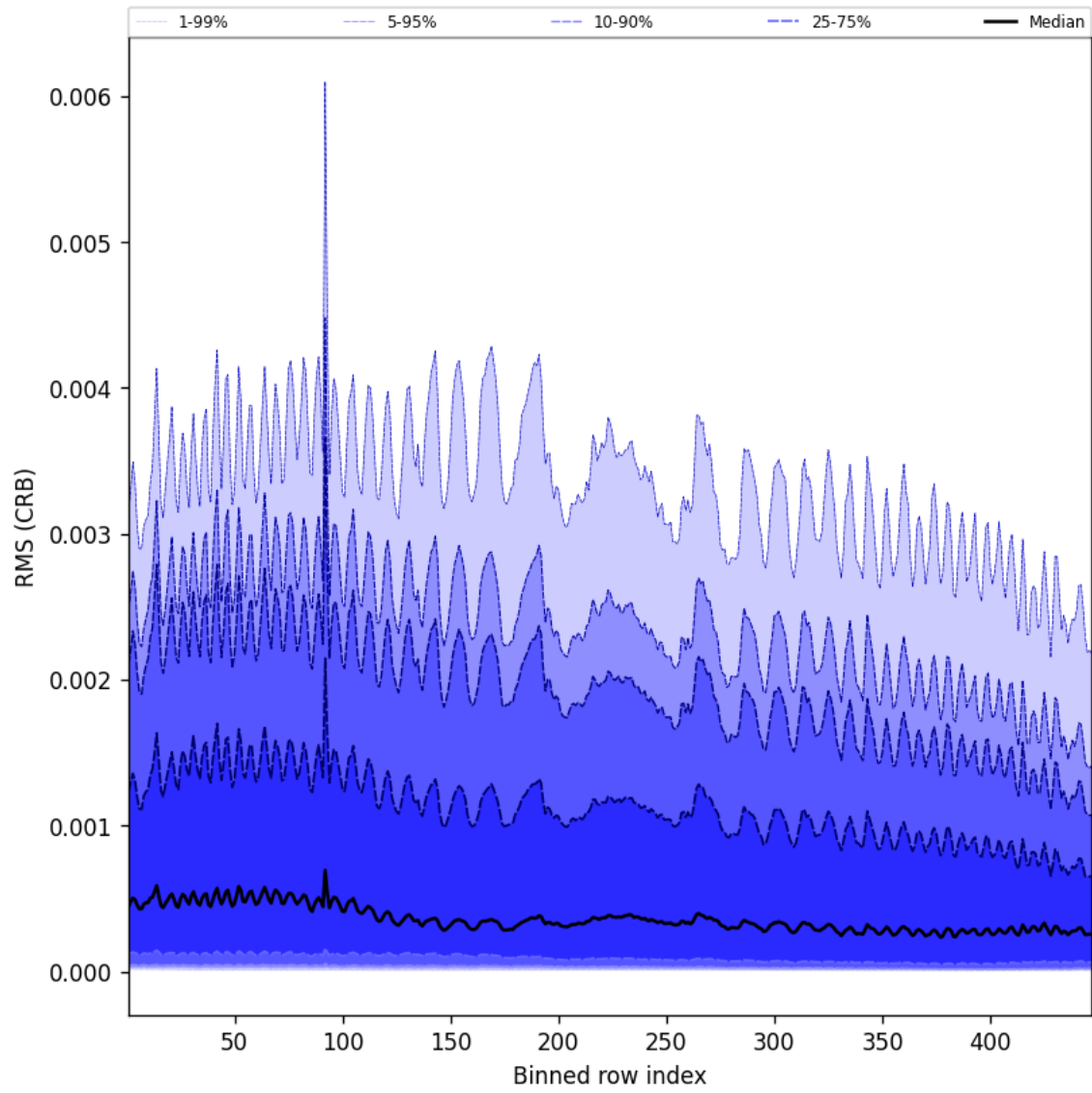
Figure 62: Along track statistics of “RMS (CRB)” for 2024-12-14 to 2024-12-14
