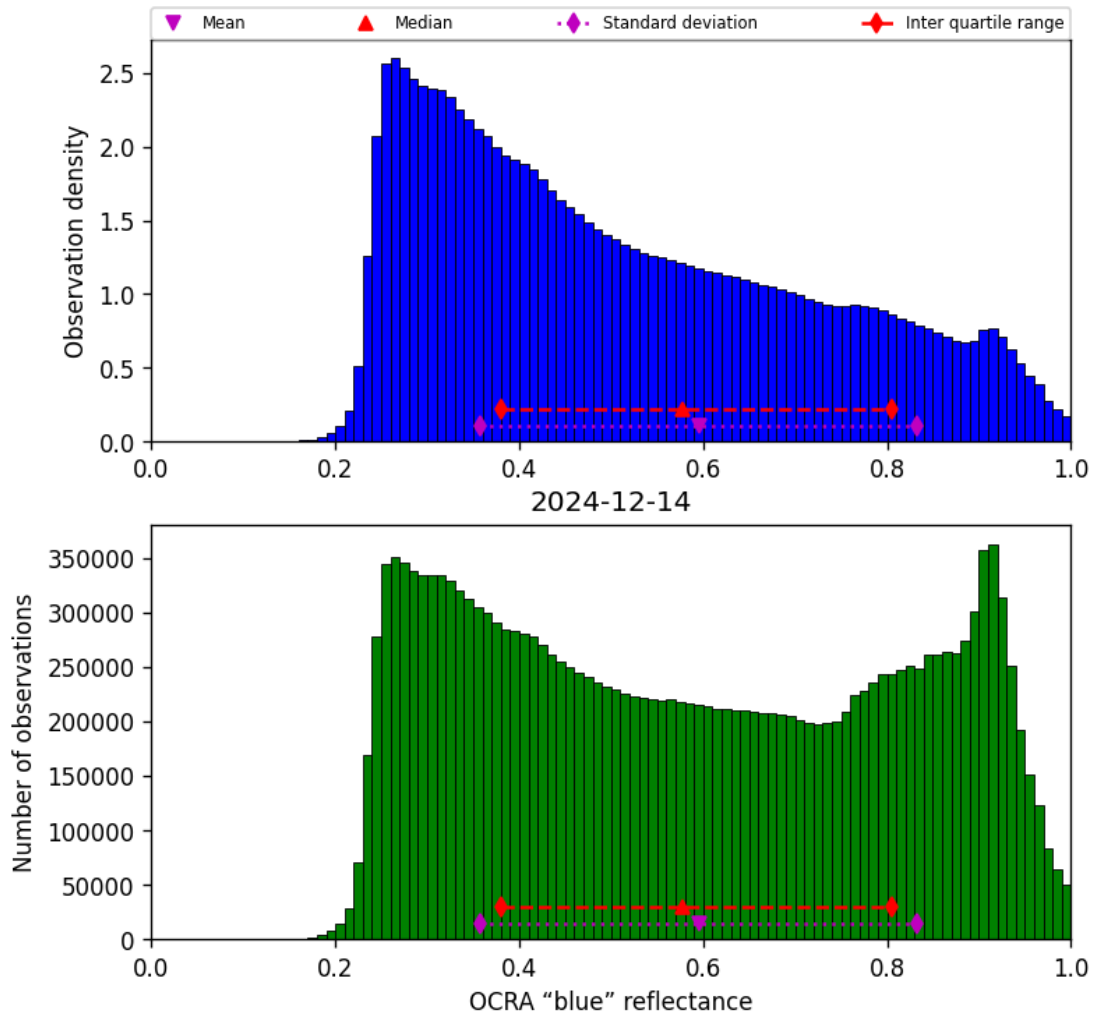
Figure 49: Histogram of "OCRA "blue" reflectance" for 2024-12-14 to 2024-12-14
