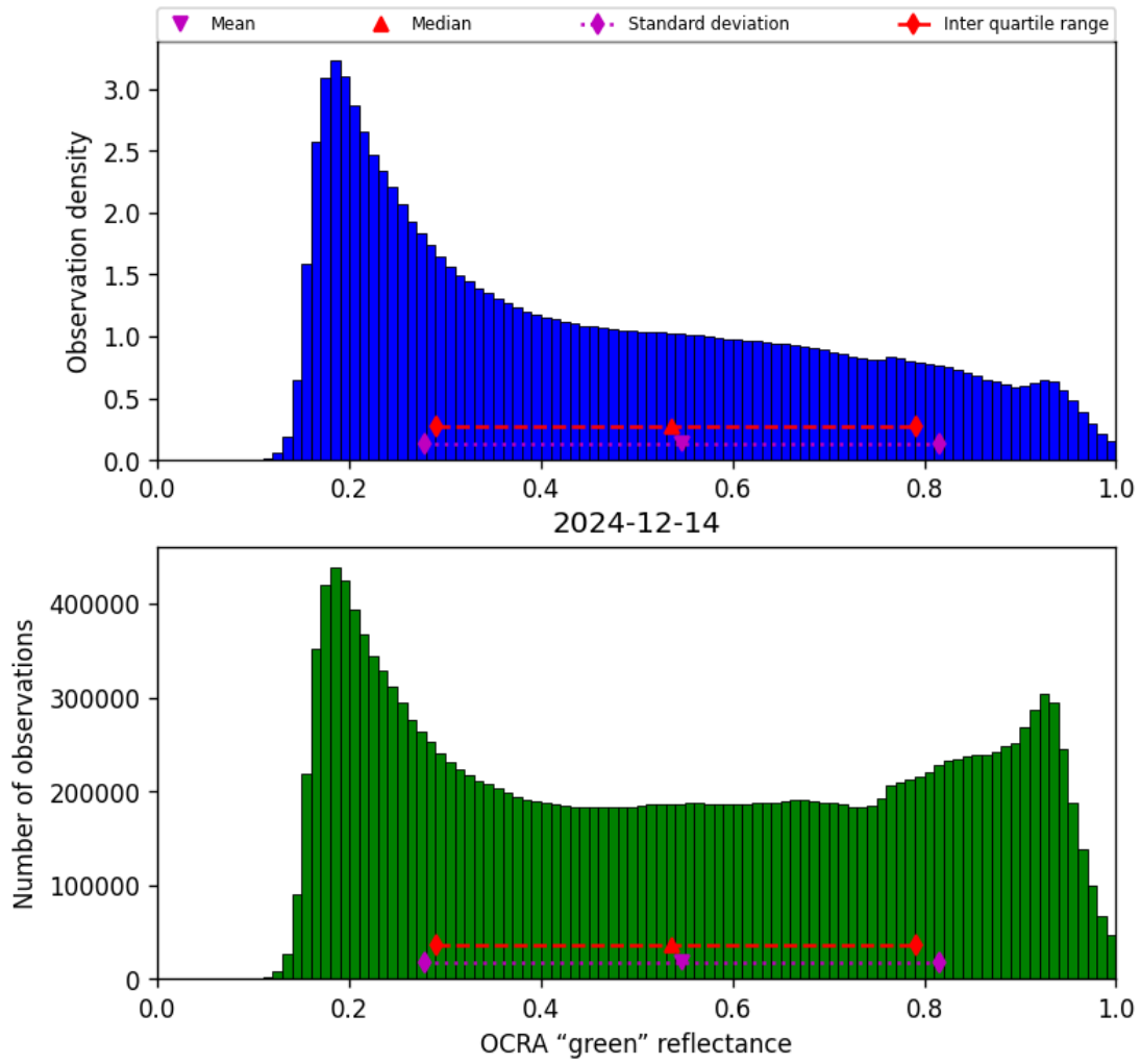
Figure 50: Histogram of “OCRA “green” reflectance” for 2024-12-14 to 2024-12-14
