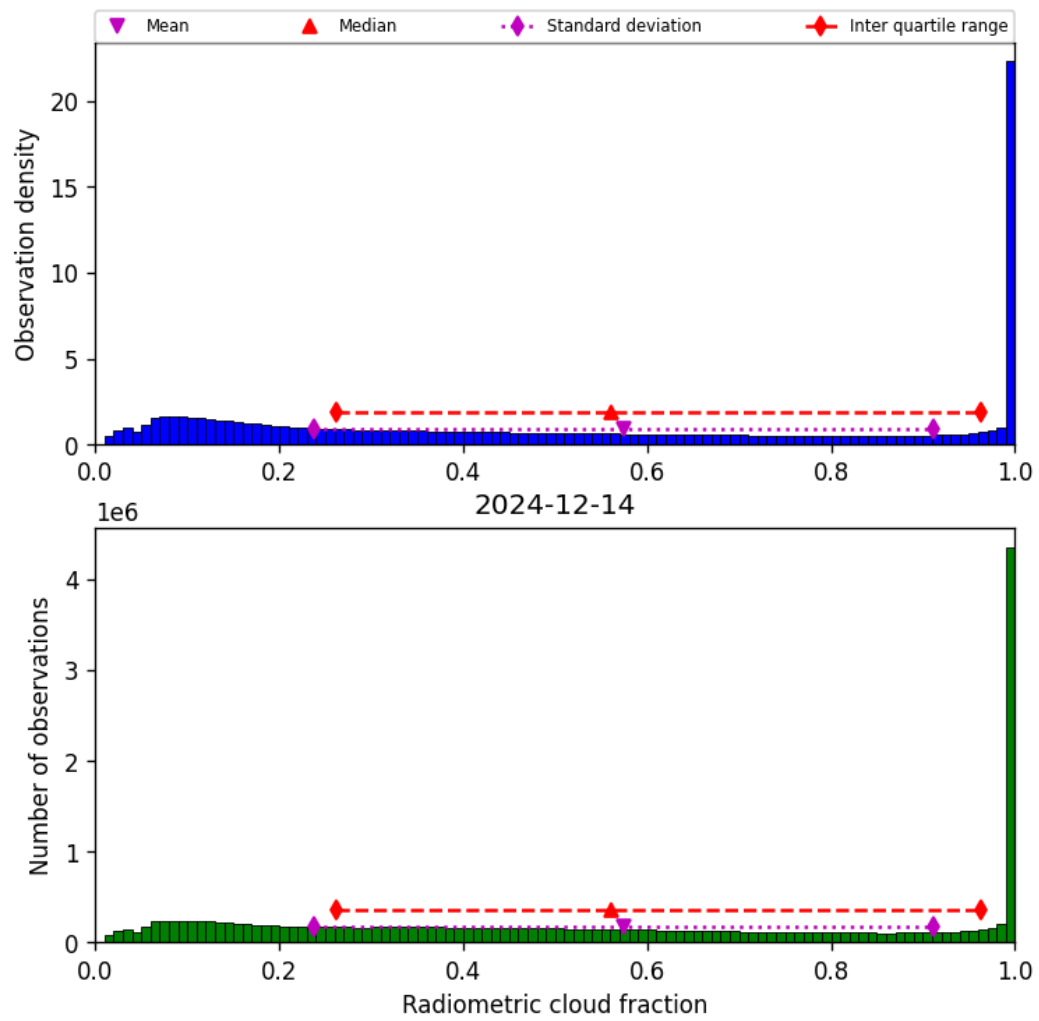
Figure 37: Histogram of “Radiometric cloud fraction” for 2024-12-14 to 2024-12-14
