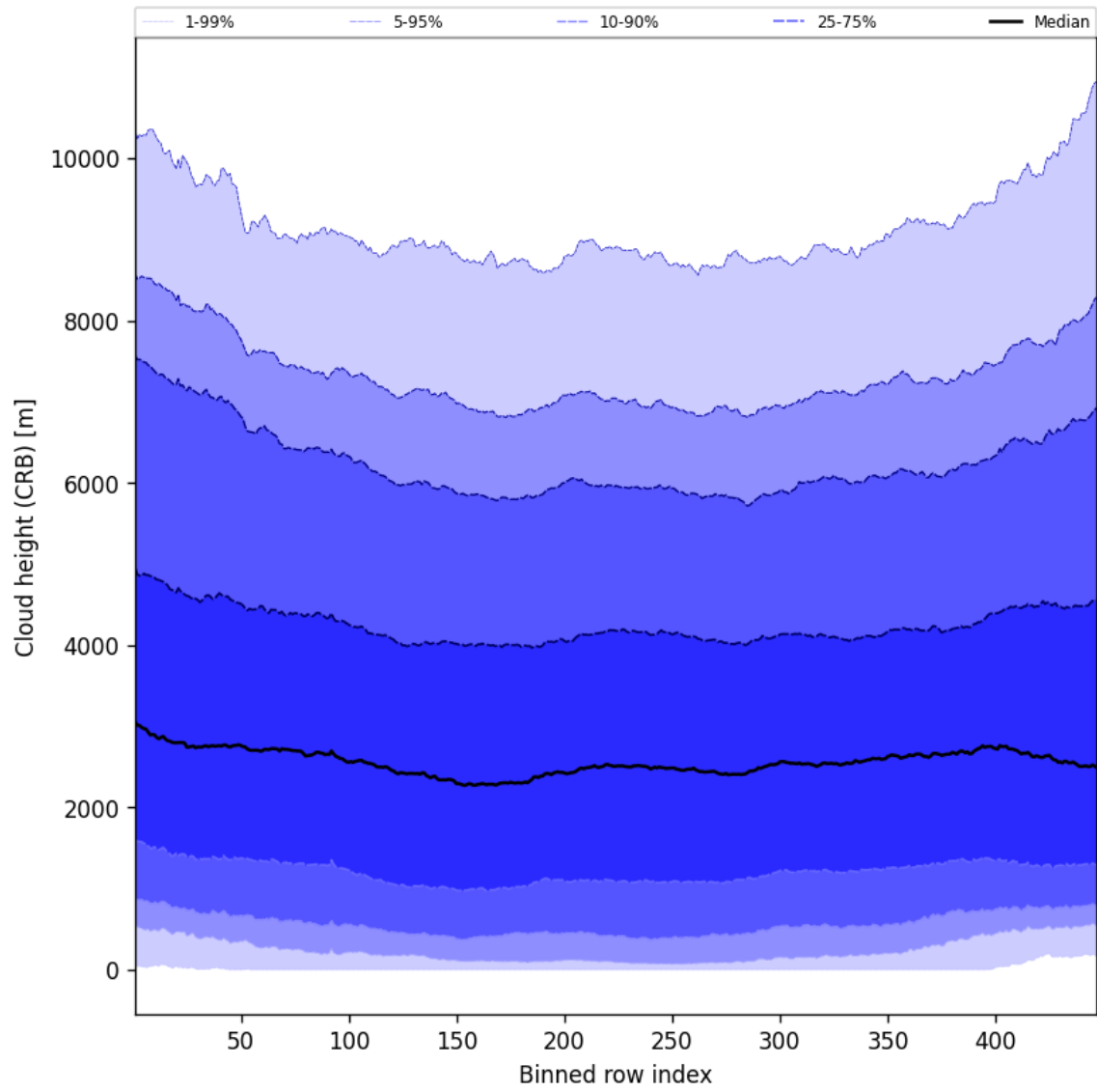
Figure 57: Along track statistics of “Cloud height (CRB)” for 2024-12-14 to 2024-12-14
