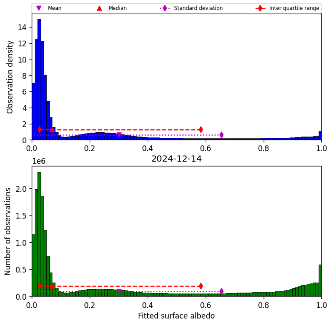
Figure 43: Histogram of “Fitted surface albedo” for 2024-12-14 to 2024-12-14
