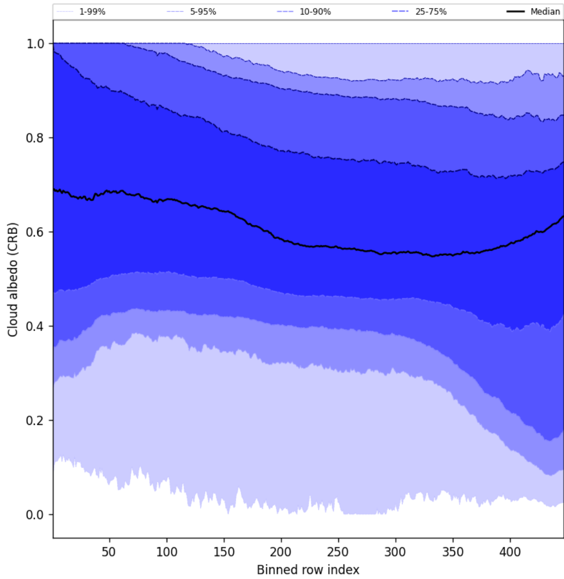
Figure 58: Along track statistics of “Cloud albedo (CRB)” for 2024-12-14 to 2024-12-14
