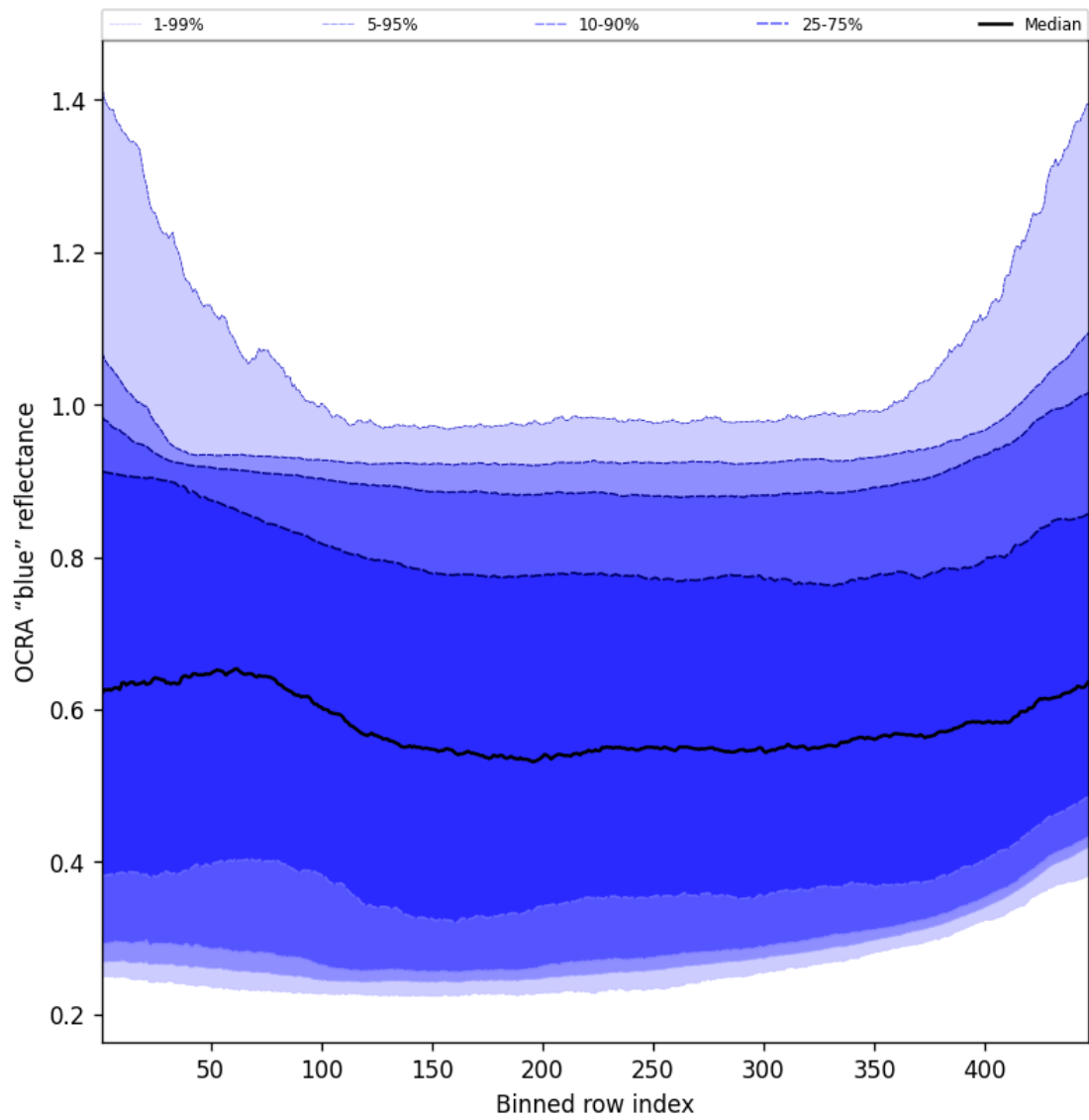
Figure 65: Along track statistics of "OCRA "blue" reflectance" for 2024-12-14 to 2024-12-14
