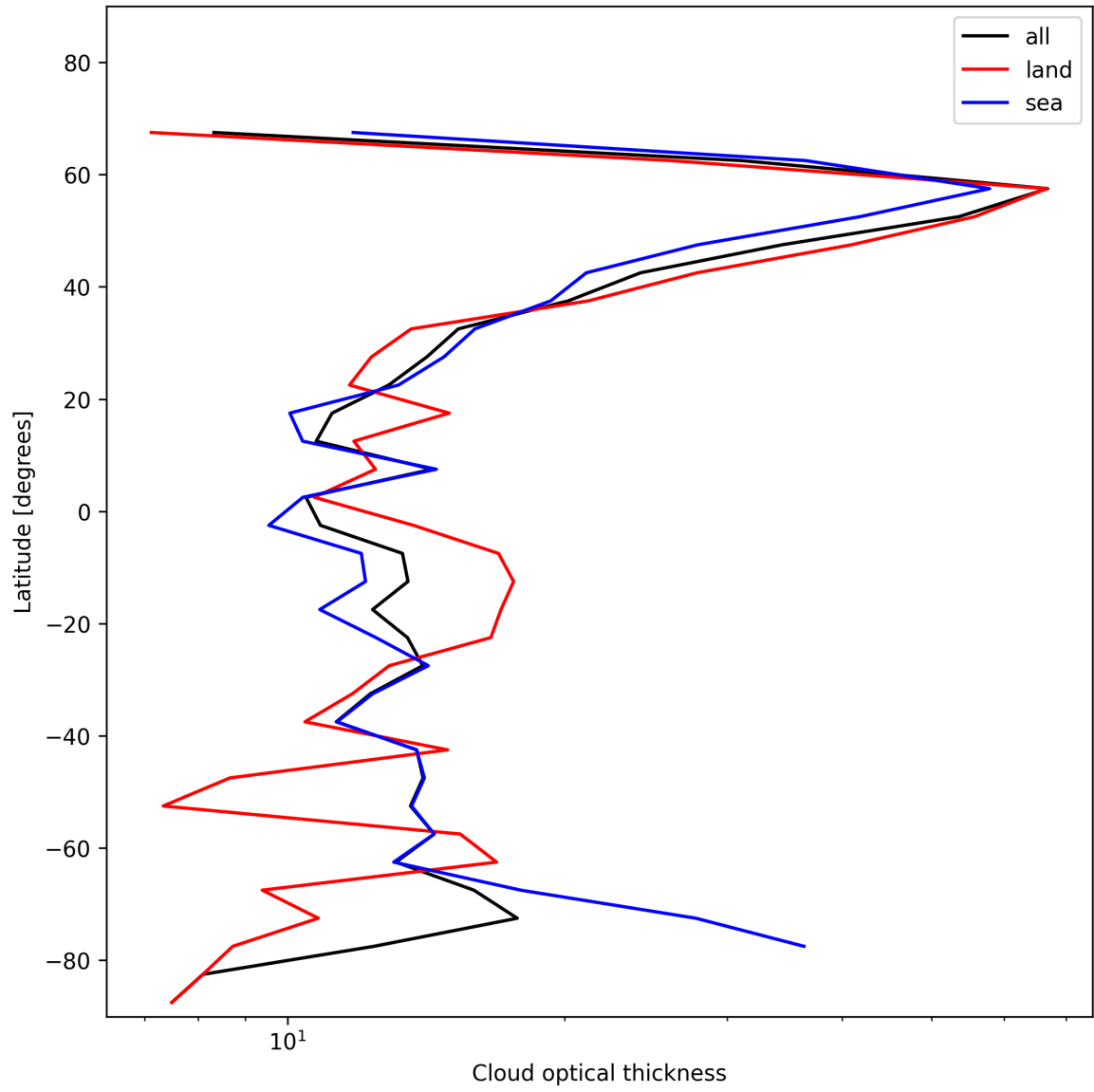
Figure 23: Zonal average of “Cloud optical thickness” for 2024-12-14 to 2024-12-14.
