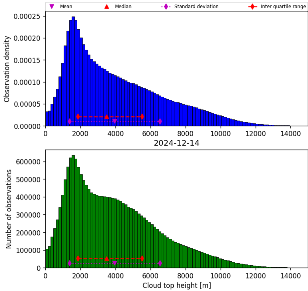
Figure 38: Histogram of “Cloud top height” for 2024-12-14 to 2024-12-14
