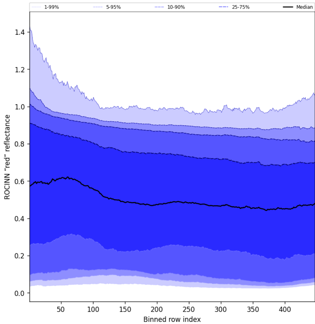
Figure 67: Along track statistics of “ROCINN “red” reflectance” for 2024-12-14 to 2024-12-14
