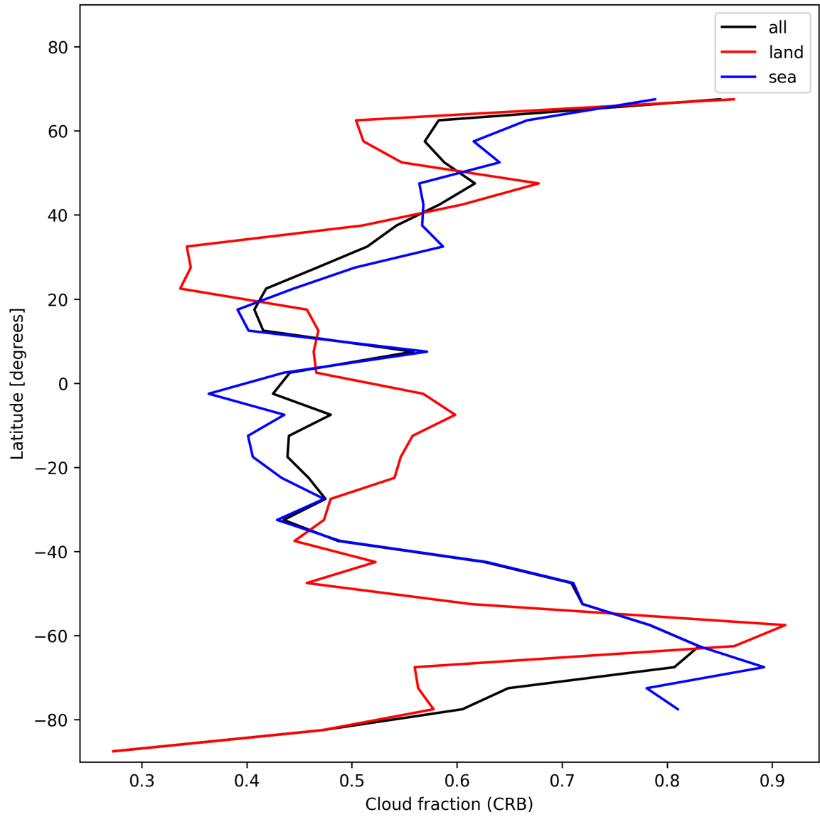
Figure 24: Zonal average of “Cloud fraction (CRB)” for 2024-12-14 to 2024-12-14.
