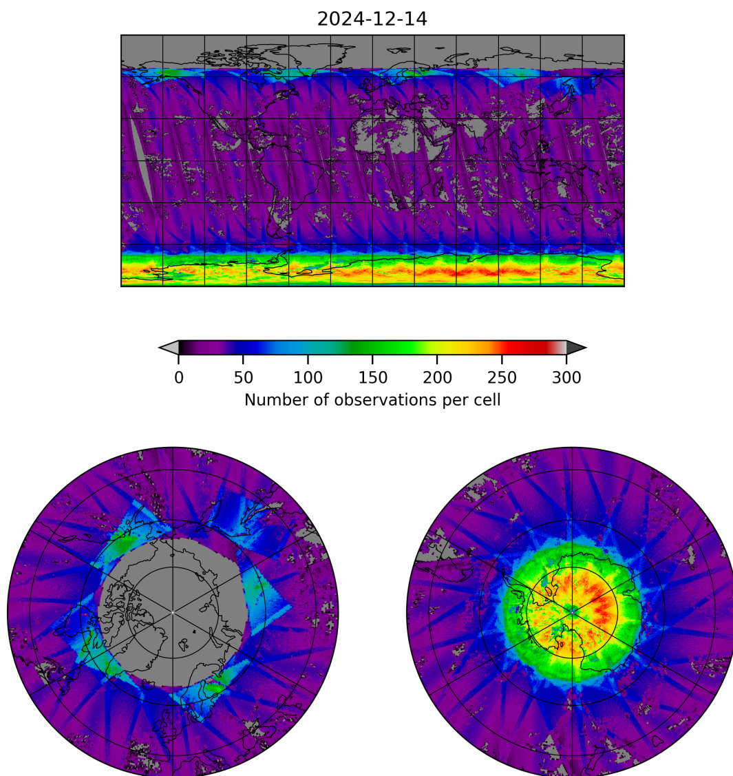
Figure 19: Map of the number of observations for 2024-12-14 to 2024-12-14
