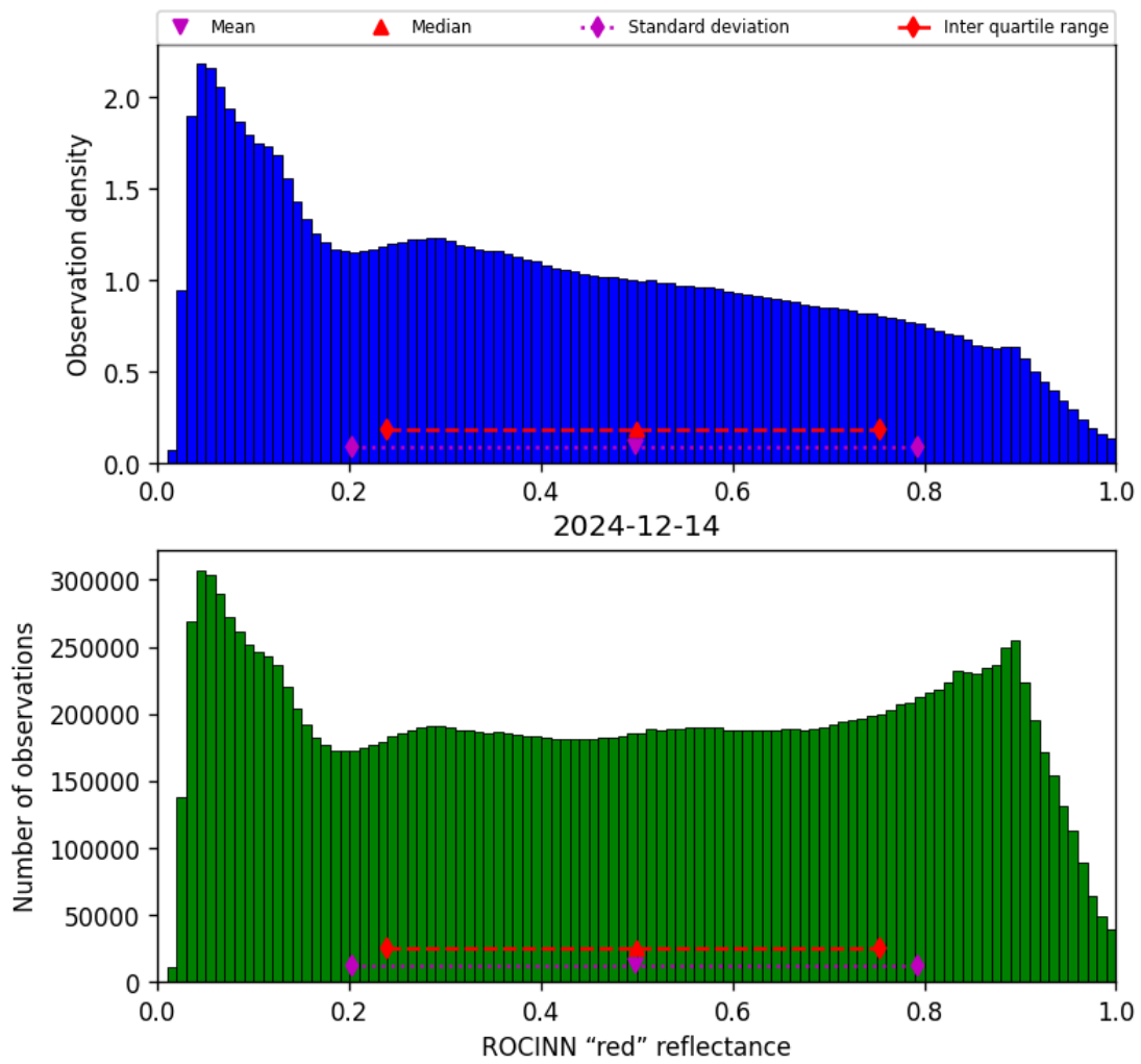
Figure 51: Histogram of “ROCINN “red” reflectance” for 2024-12-14 to 2024-12-14
