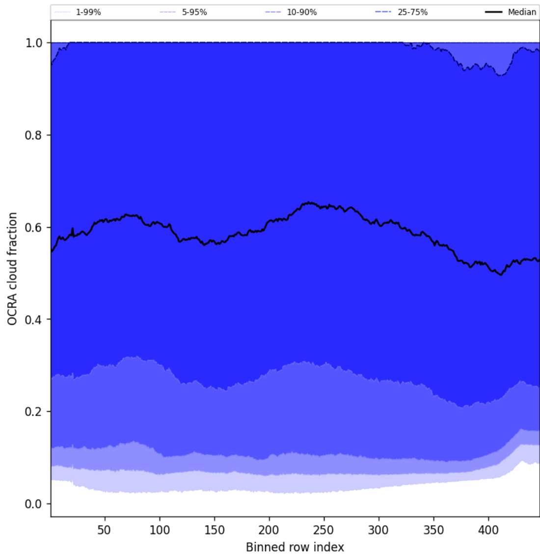
Figure 64: Along track statistics of “OCRA cloud fraction” for 2024-12-14 to 2024-12-14
