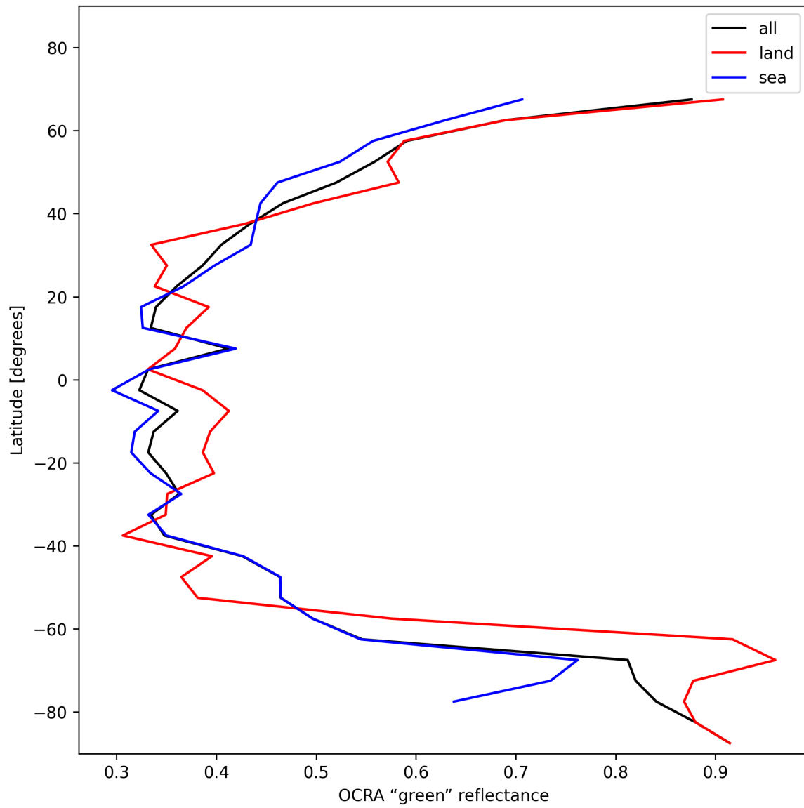
Figure 34: Zonal average of “OCRA “green” reflectance” for 2024-12-14 to 2024-12-14.
