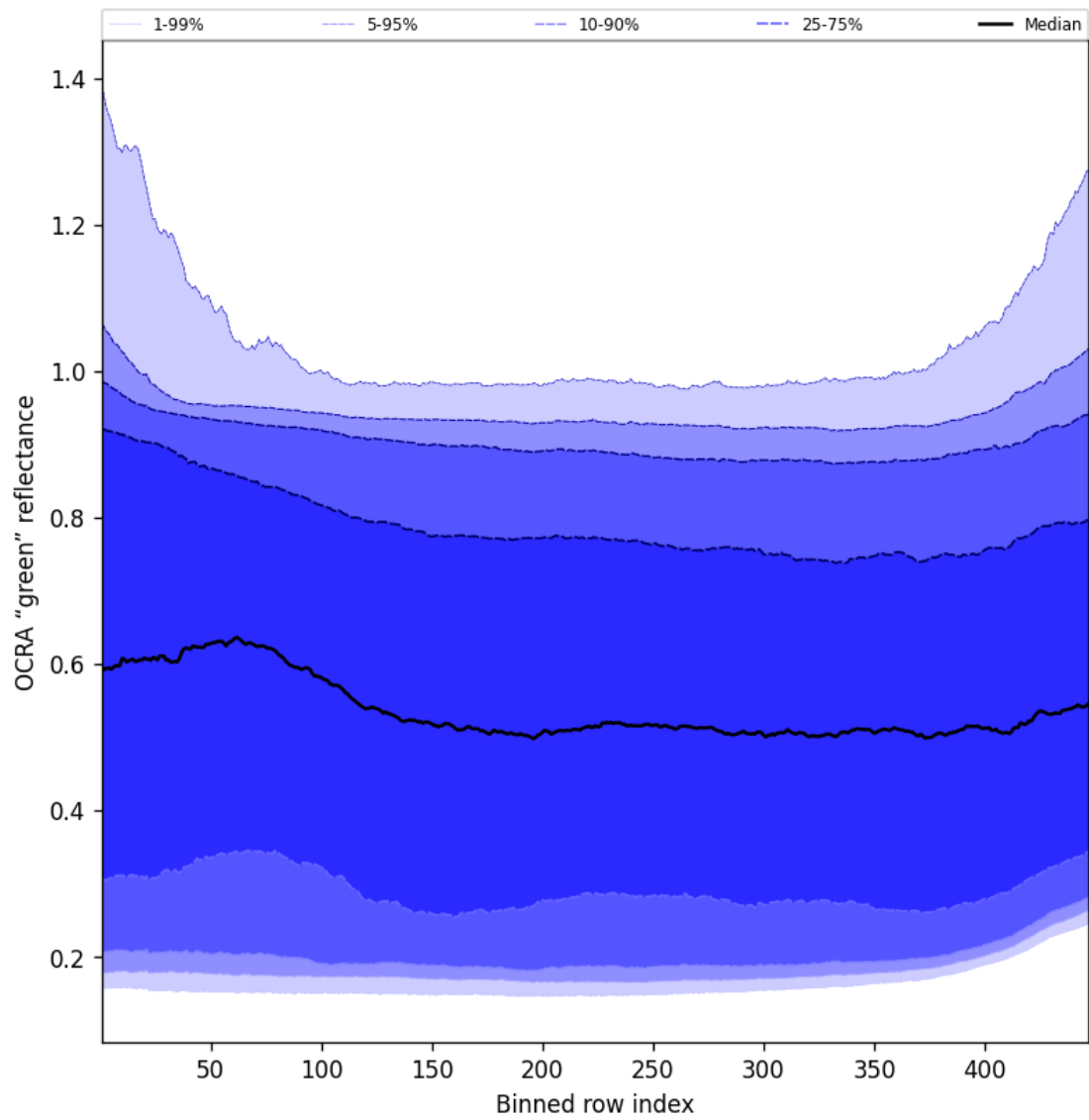
Figure 66: Along track statistics of "OCRA "green" reflectance" for 2024-12-14 to 2024-12-14
