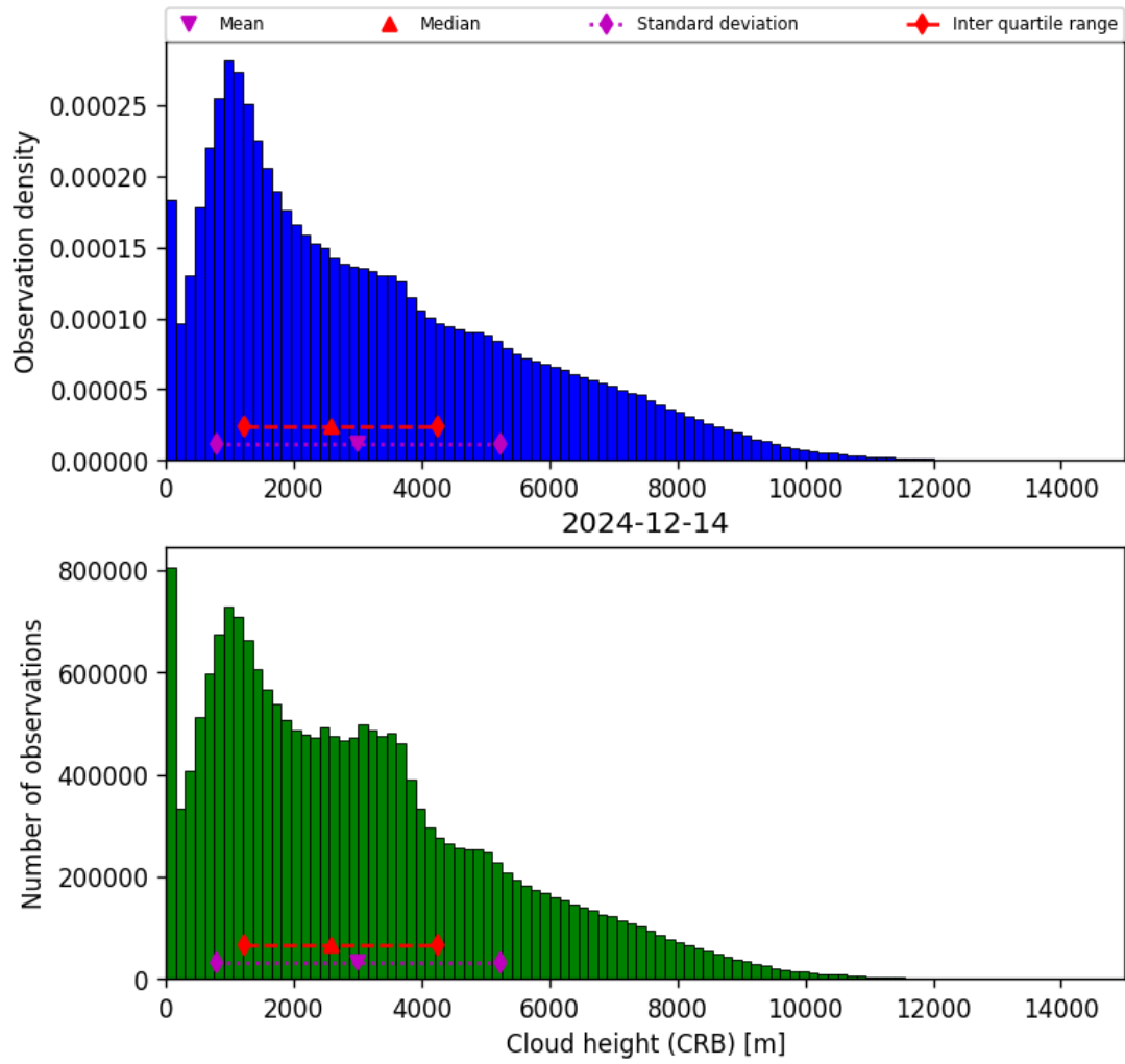
Figure 41: Histogram of “Cloud height (CRB)” for 2024-12-14 to 2024-12-14
