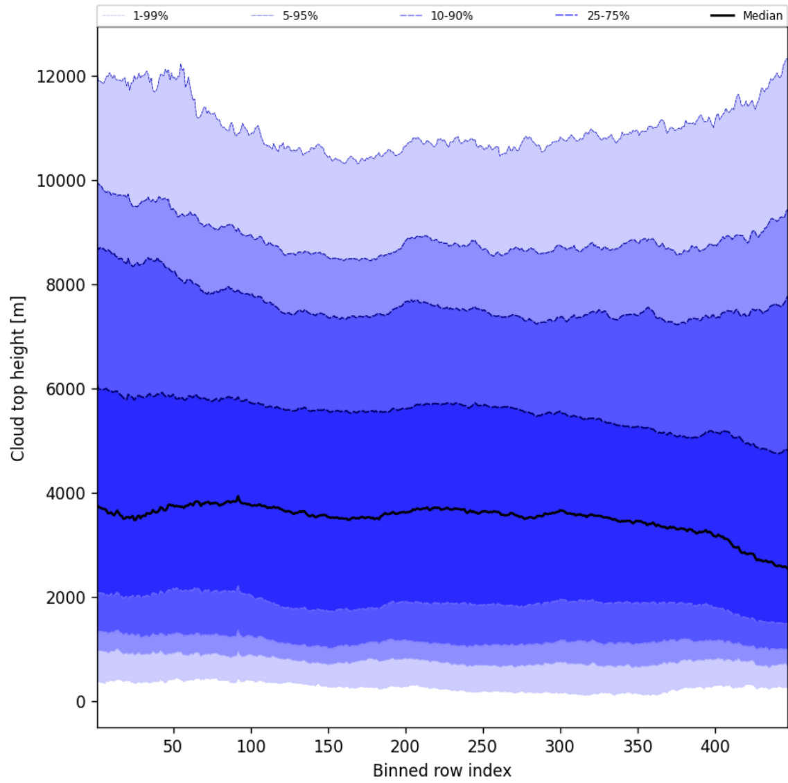
Figure 54: Along track statistics of “Cloud top height” for 2024-12-14 to 2024-12-14
