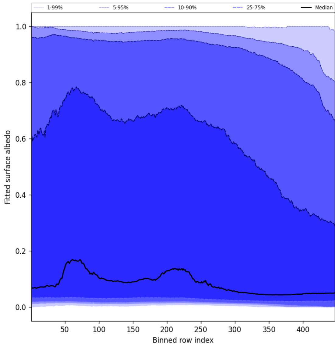
Figure 59: Along track statistics of “Fitted surface albedo” for 2024-12-14 to 2024-12-14
