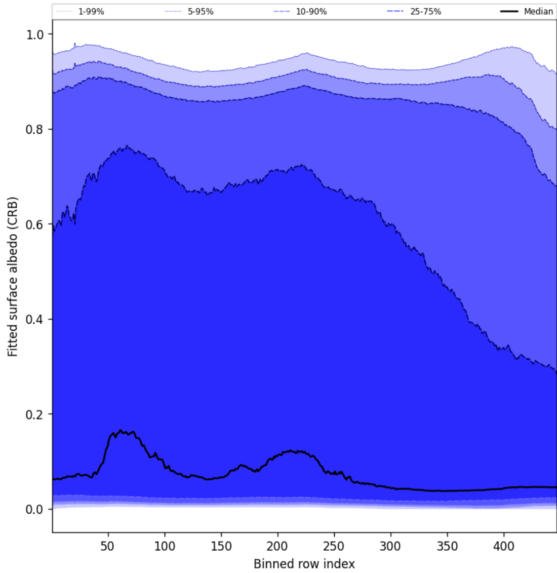
Figure 60: Along track statistics of “Fitted surface albedo (CRB)” for 2024-12-14 to 2024-12-14
