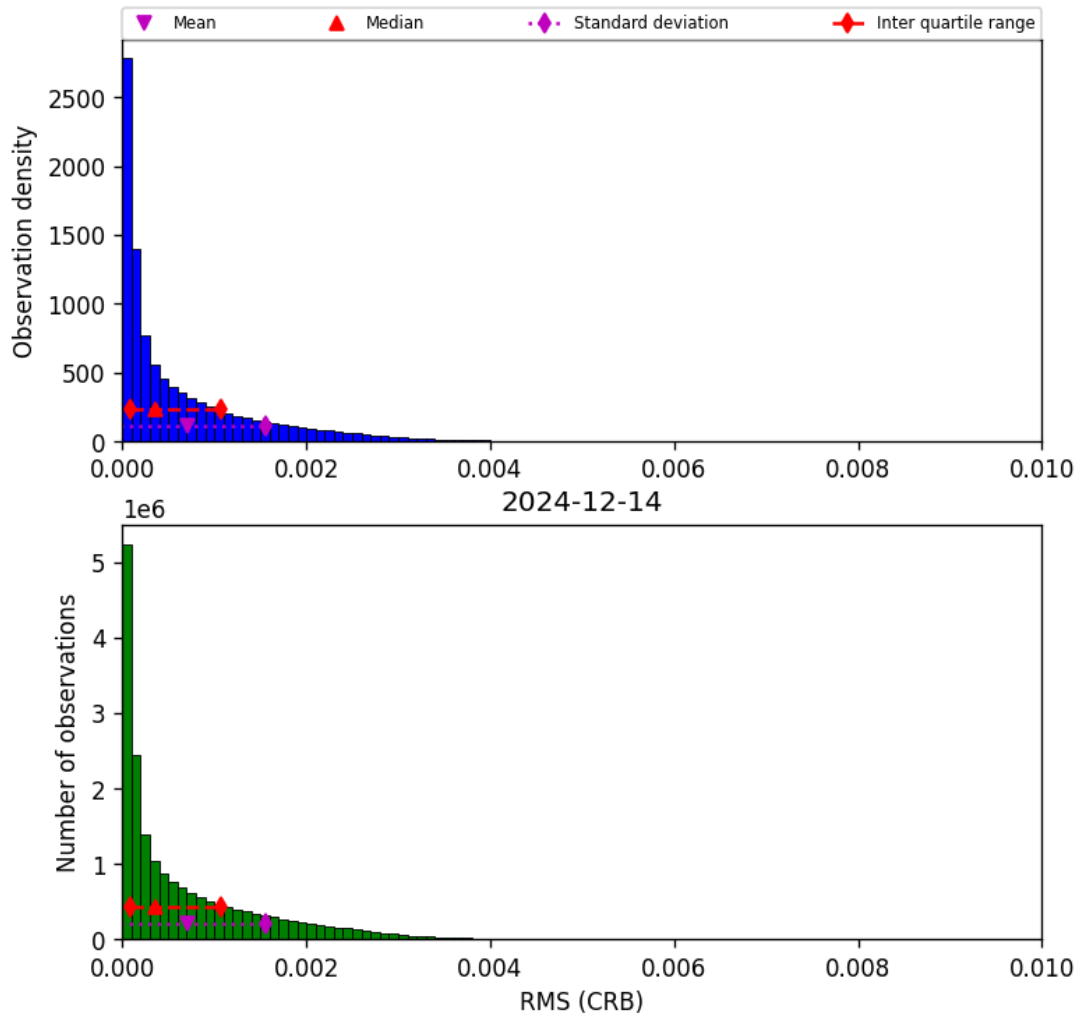
Figure 46: Histogram of “RMS (CRB)” for 2024-12-14 to 2024-12-14
