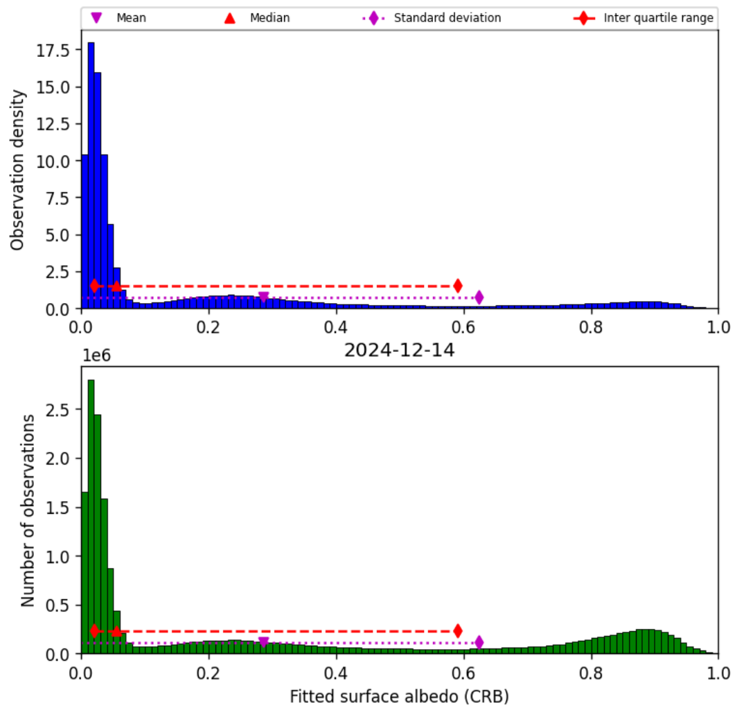
Figure 44: Histogram of “Fitted surface albedo (CRB)” for 2024-12-14 to 2024-12-14
