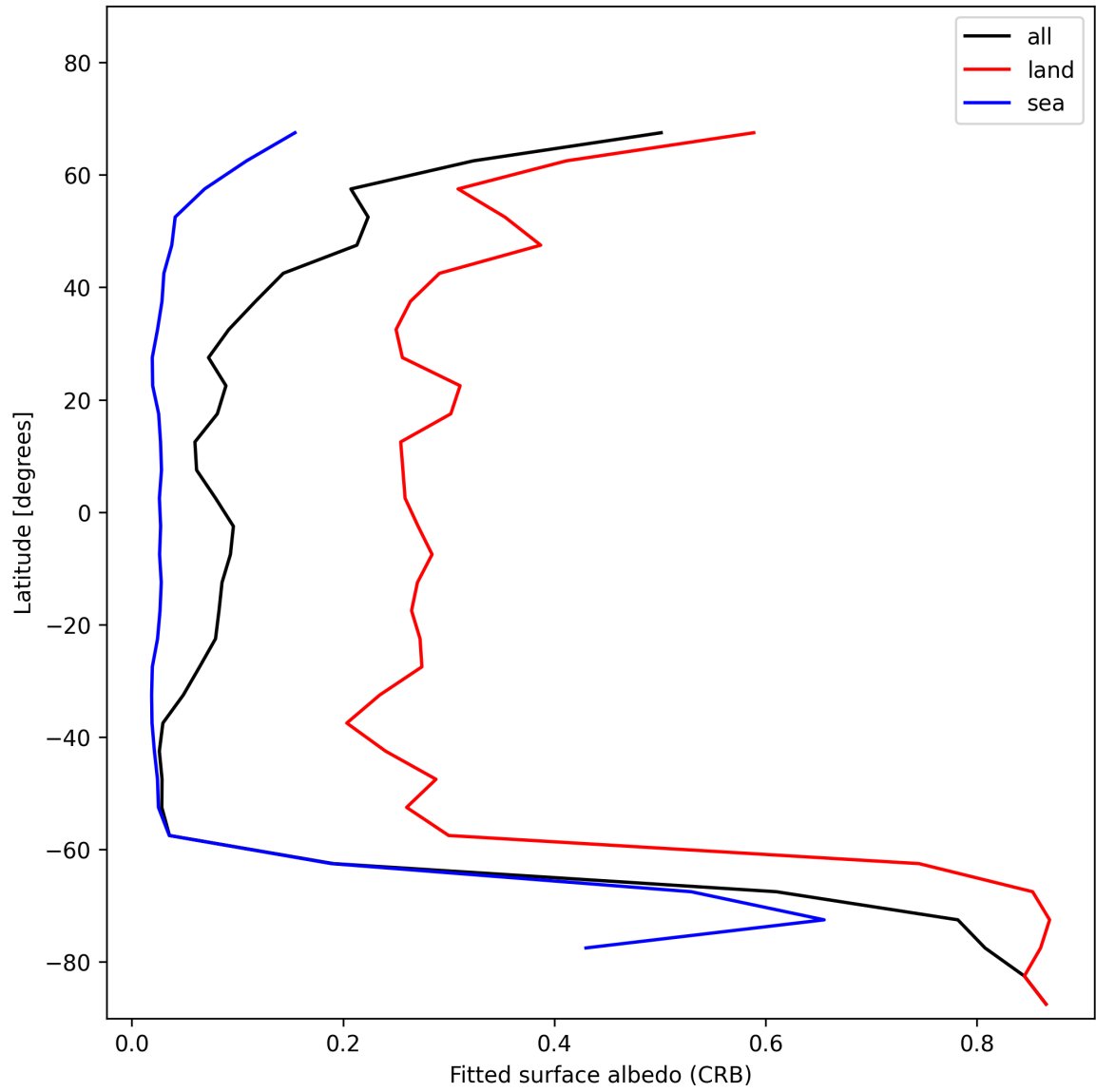
Figure 28: Zonal average of “Fitted surface albedo (CRB)” for 2024-12-14 to 2024-12-14.
