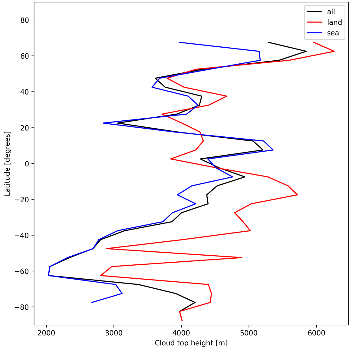
Figure 22: Zonal average of “Cloud top height” for 2024-12-14 to 2024-12-14.
