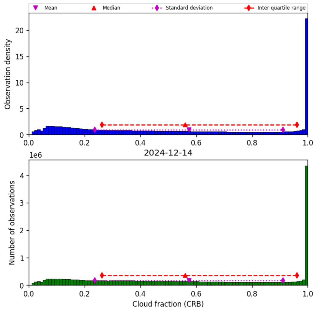
Figure 40: Histogram of “Cloud fraction (CRB)” for 2024-12-14 to 2024-12-14
