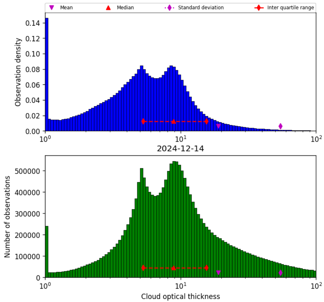
Figure 39: Histogram of “Cloud optical thickness” for 2024-12-14 to 2024-12-14
