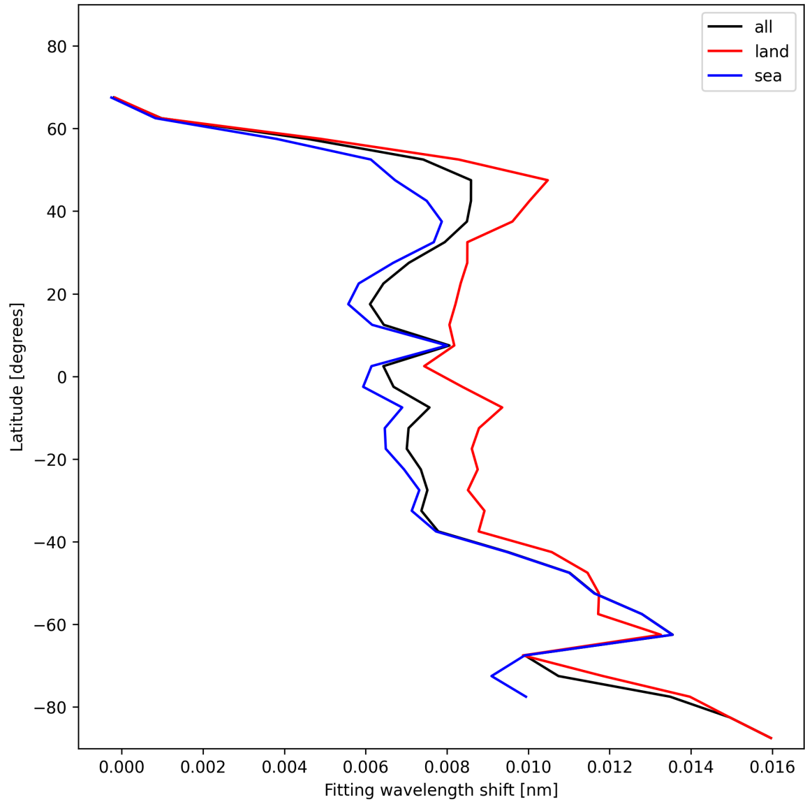
Figure 31: Zonal average of “Fitting wavelength shift” for 2024-12-14 to 2024-12-14.
