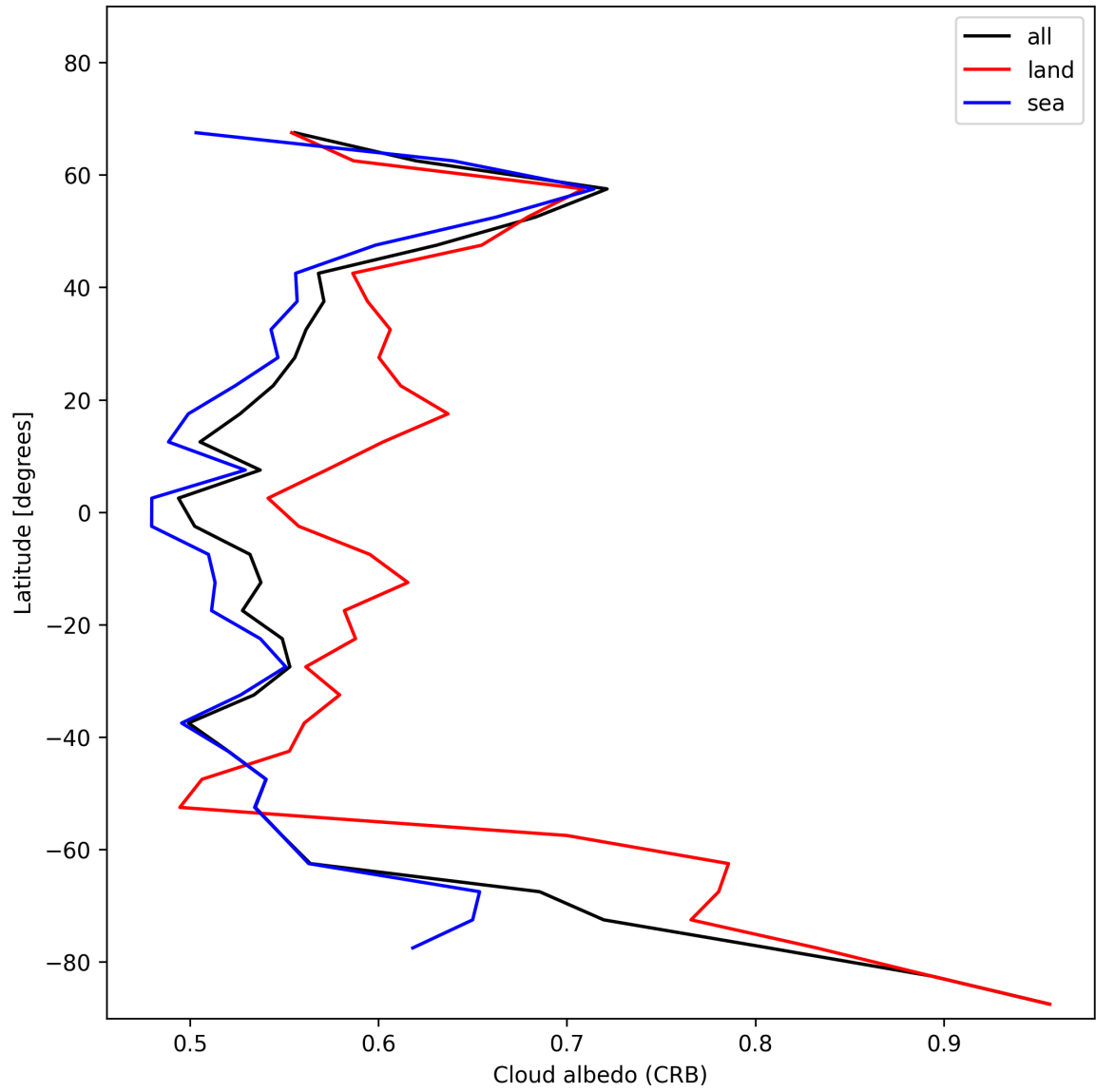
Figure 26: Zonal average of “Cloud albedo (CRB)” for 2024-12-14 to 2024-12-14.
