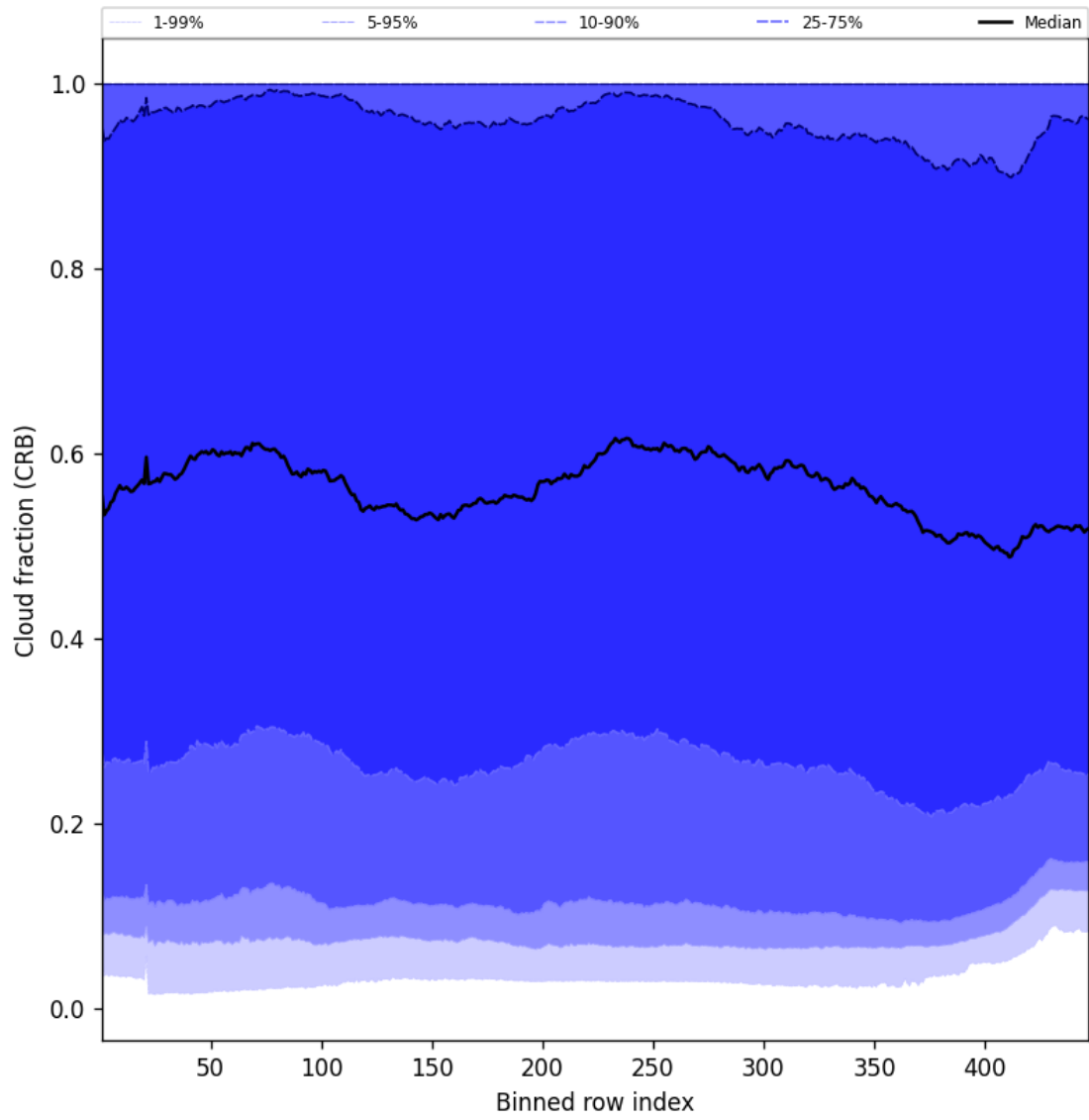
Figure 56: Along track statistics of “Cloud fraction (CRB)” for 2024-12-14 to 2024-12-14
