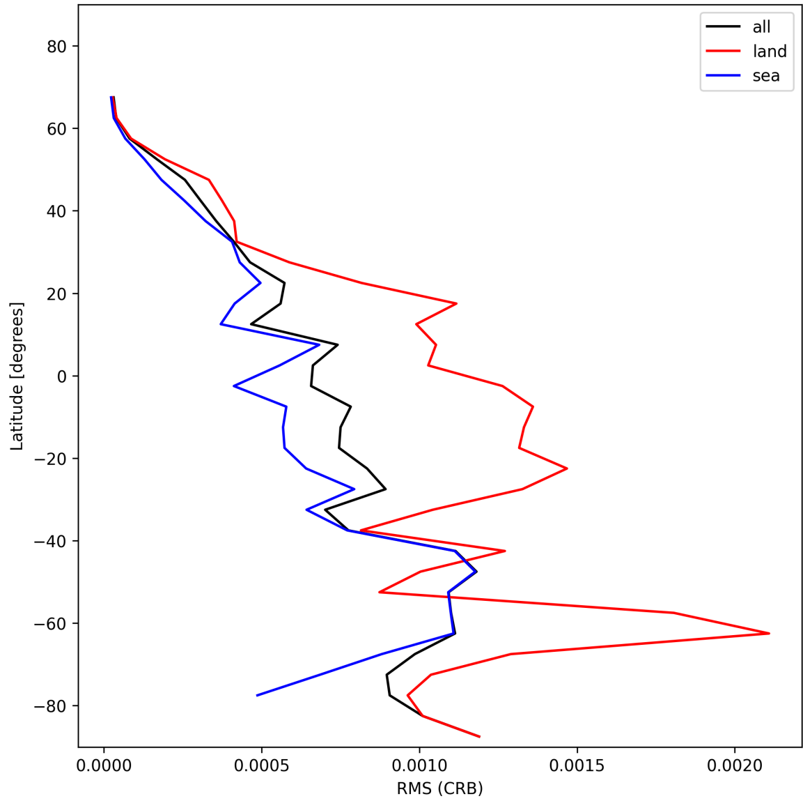
Figure 30: Zonal average of “RMS (CRB)” for 2024-12-14 to 2024-12-14.
