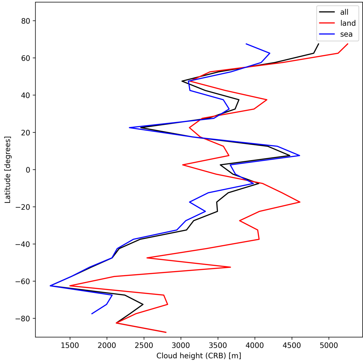
Figure 25: Zonal average of “Cloud height (CRB)” for 2024-12-14 to 2024-12-14.
