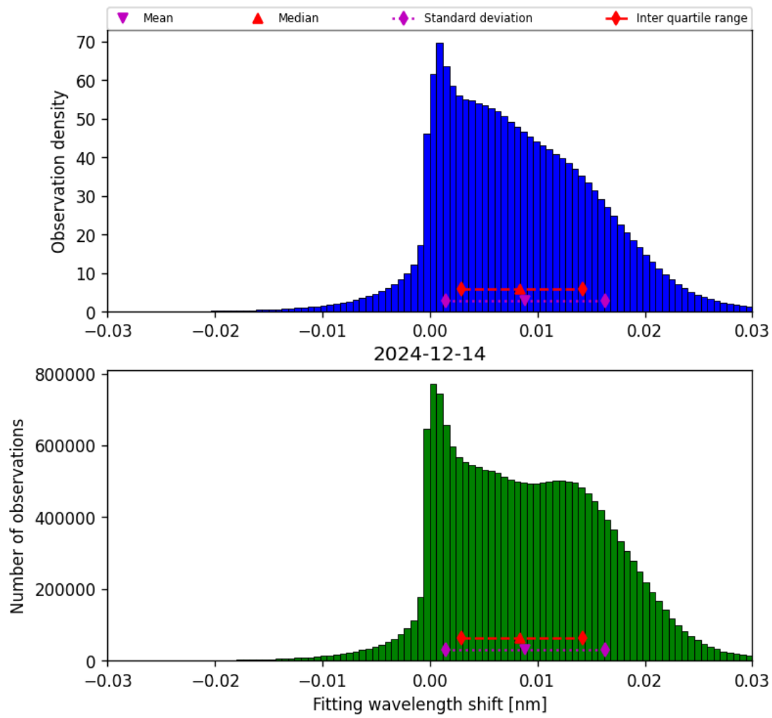
Figure 47: Histogram of “Fitting wavelength shift” for 2024-12-14 to 2024-12-14
