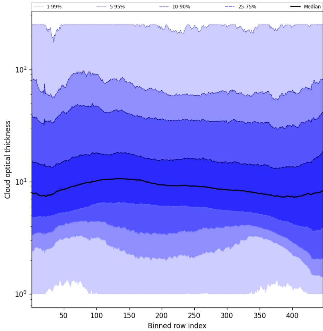
Figure 55: Along track statistics of “Cloud optical thickness” for 2024-12-14 to 2024-12-14
