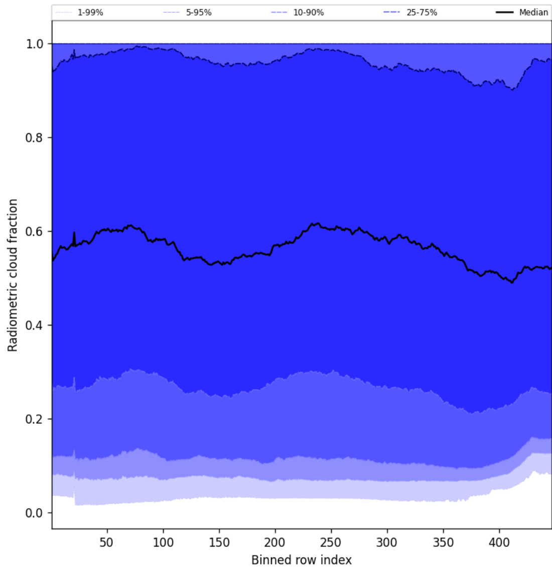
Figure 53: Along track statistics of “Radiometric cloud fraction” for 2024-12-14 to 2024-12-14
