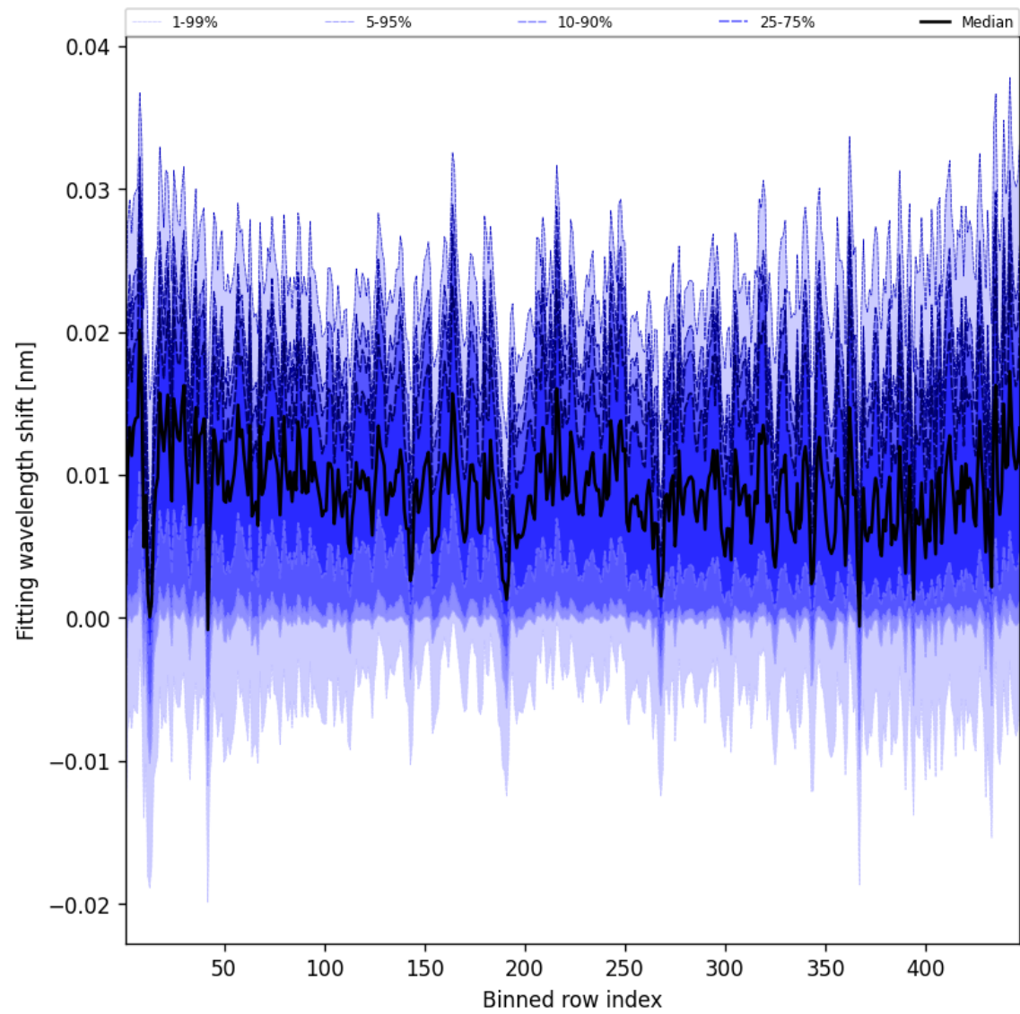
Figure 63: Along track statistics of “Fitting wavelength shift” for 2024-12-14 to 2024-12-14
