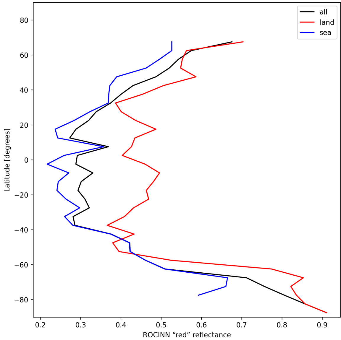
Figure 35: Zonal average of “ROCINN “red” reflectance” for 2024-12-14 to 2024-12-14.
