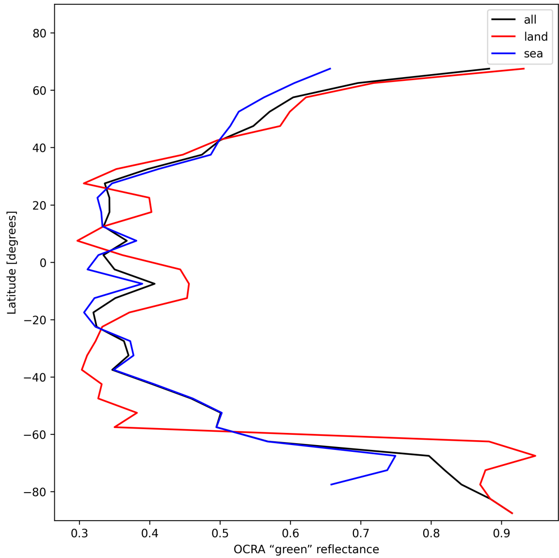
Figure 34: Zonal average of “OCRA “green” reflectance” for 2024-12-15 to 2024-12-16.
