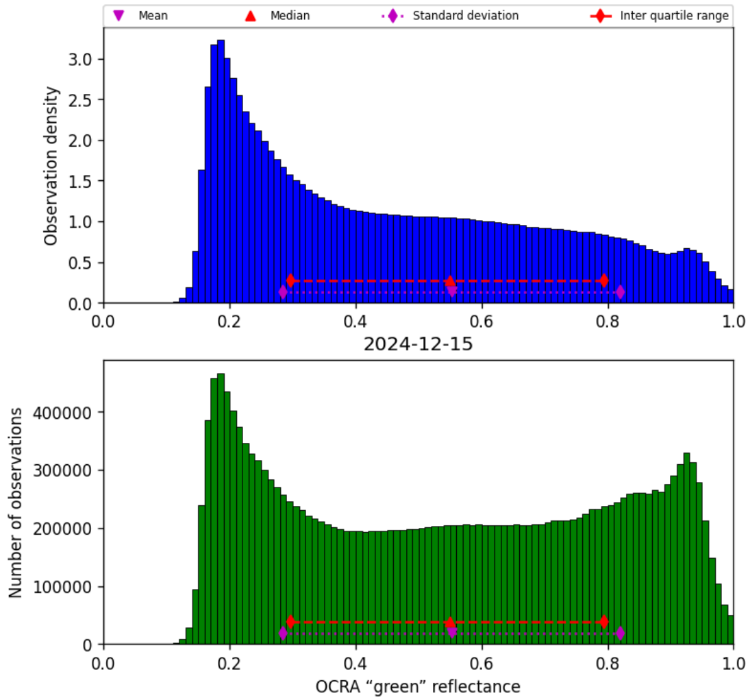
Figure 50: Histogram of “OCRA “green” reflectance” for 2024-12-15 to 2024-12-16
