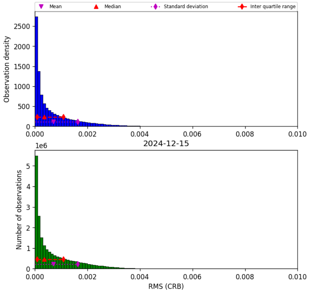
Figure 46: Histogram of “RMS (CRB)” for 2024-12-15 to 2024-12-16
