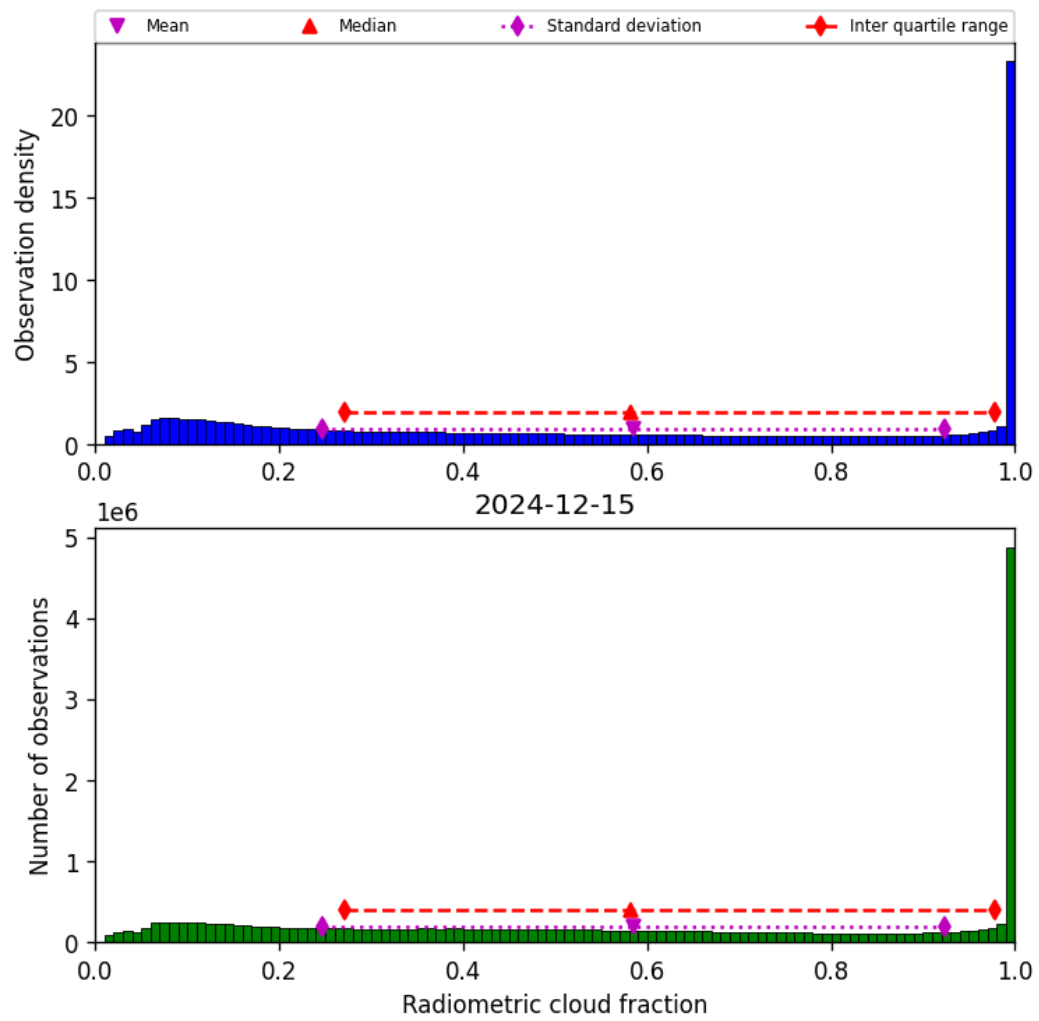
Figure 37: Histogram of “Radiometric cloud fraction” for 2024-12-15 to 2024-12-16
