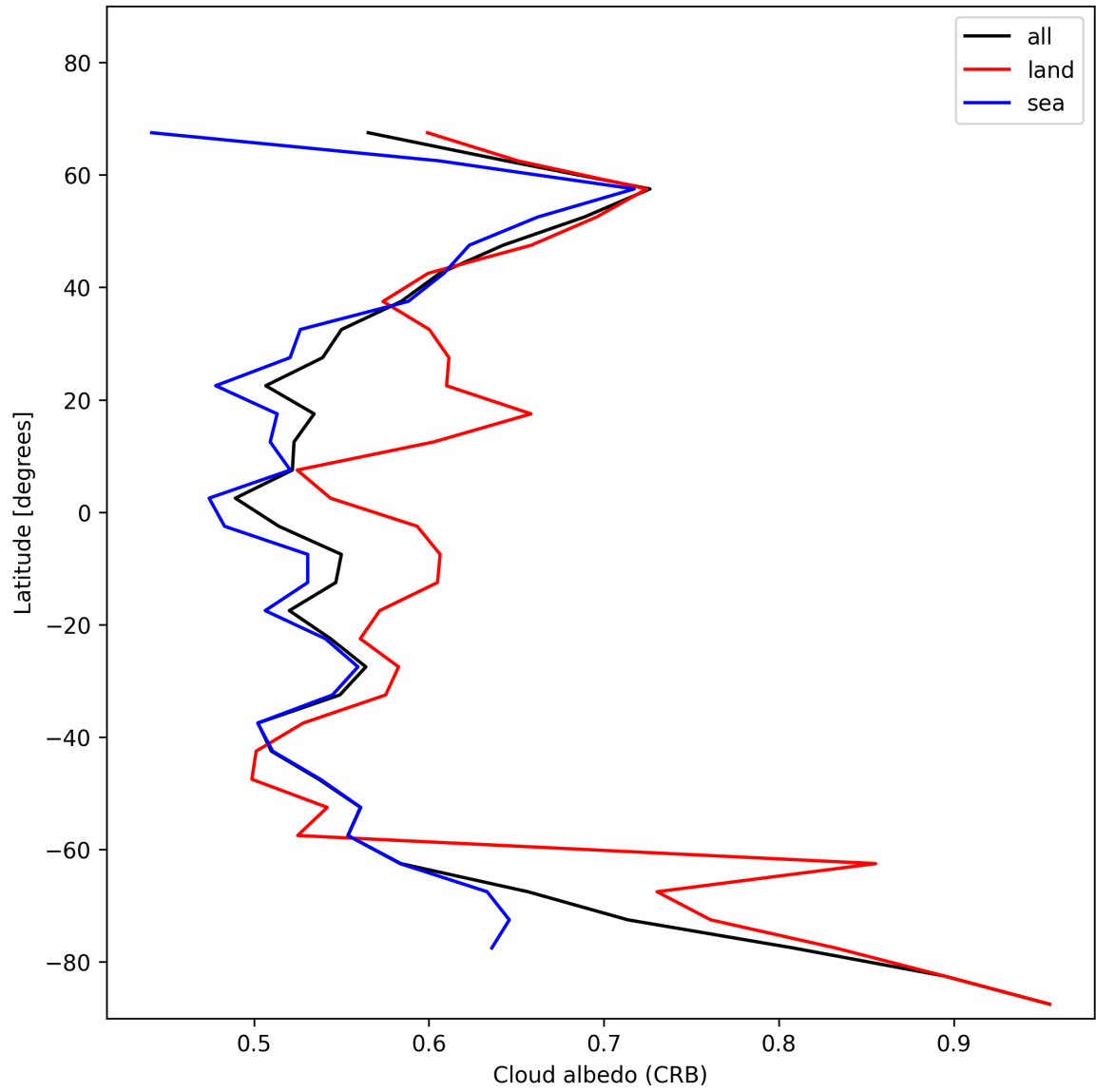
Figure 26: Zonal average of “Cloud albedo (CRB)” for 2024-12-15 to 2024-12-16.
