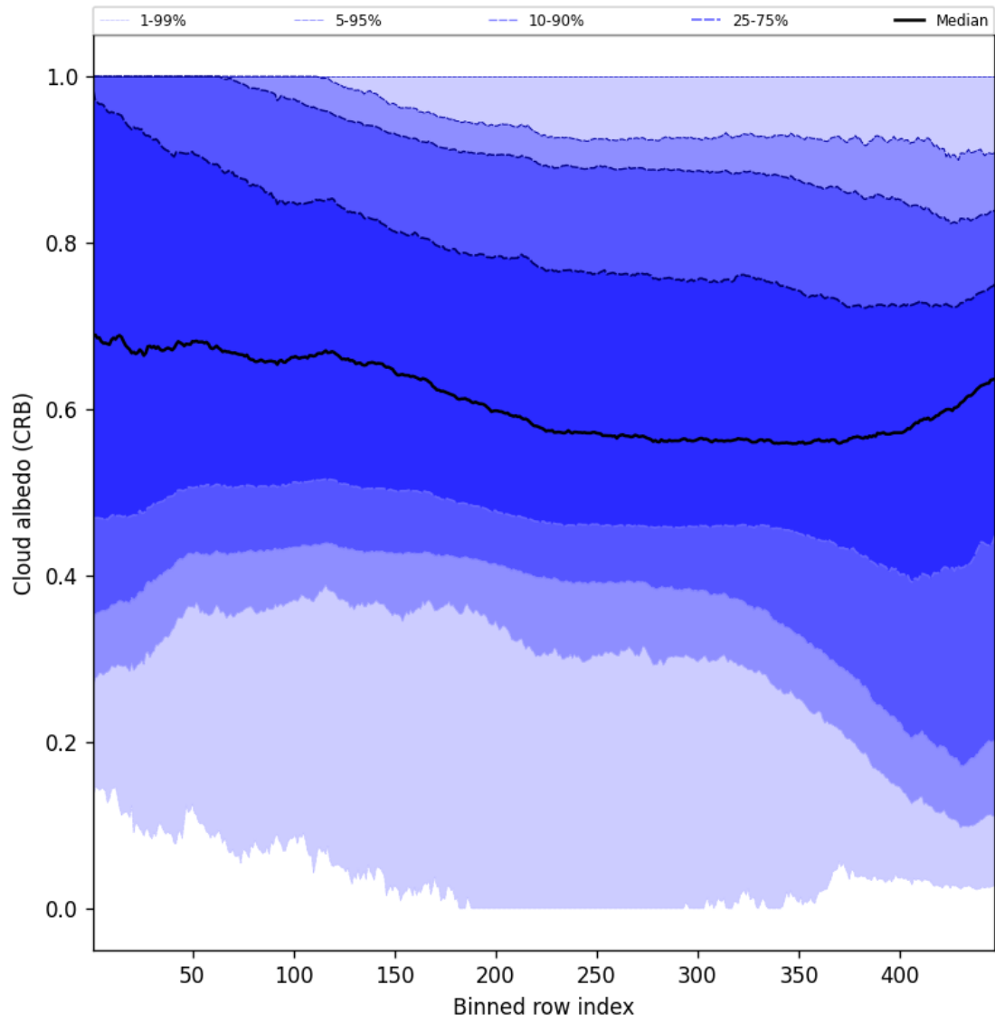
Figure 58: Along track statistics of “Cloud albedo (CRB)” for 2024-12-15 to 2024-12-16
