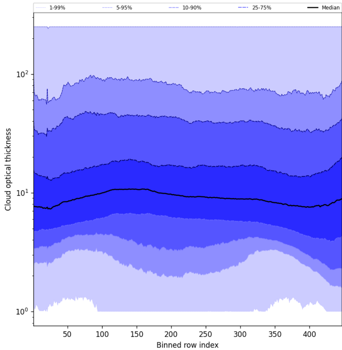
Figure 55: Along track statistics of “Cloud optical thickness” for 2024-12-15 to 2024-12-16
