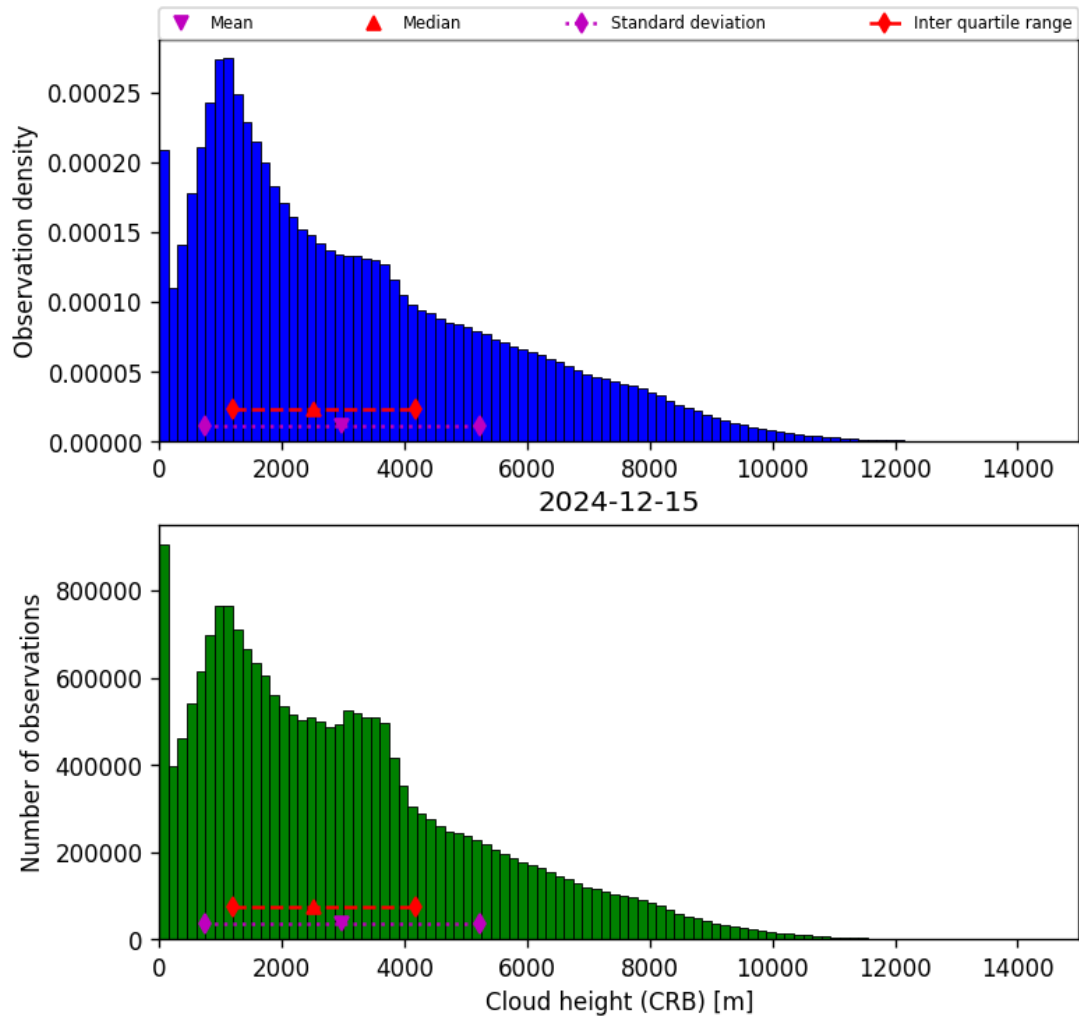
Figure 41: Histogram of “Cloud height (CRB)” for 2024-12-15 to 2024-12-16
