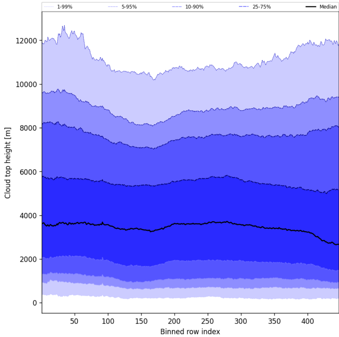
Figure 54: Along track statistics of “Cloud top height” for 2024-12-15 to 2024-12-16
