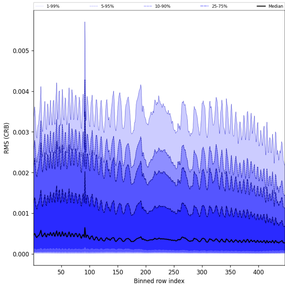
Figure 62: Along track statistics of “RMS (CRB)” for 2024-12-15 to 2024-12-16
