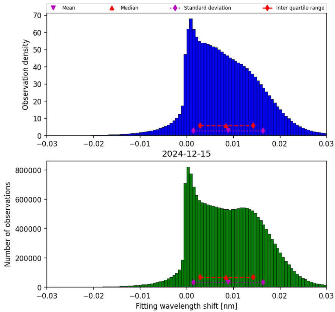
Figure 47: Histogram of “Fitting wavelength shift” for 2024-12-15 to 2024-12-16
