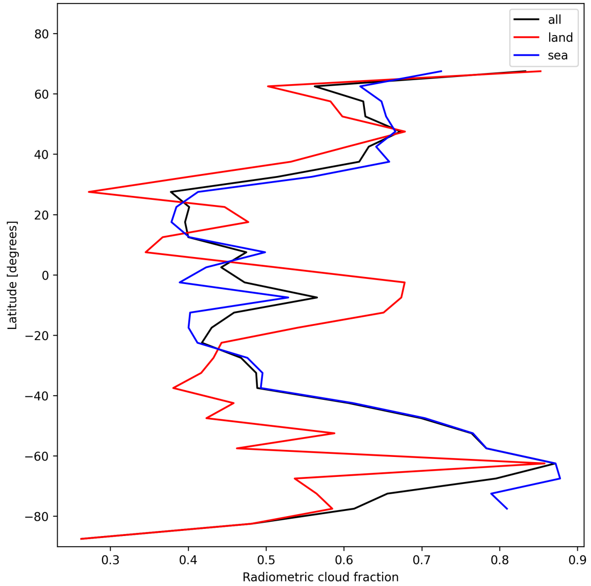
Figure 21: Zonal average of “Radiometric cloud fraction” for 2024-12-15 to 2024-12-16.
