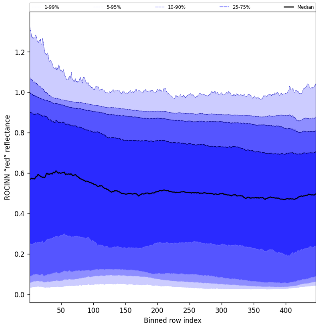
Figure 67: Along track statistics of “ROCINN “red” reflectance” for 2024-12-15 to 2024-12-16
