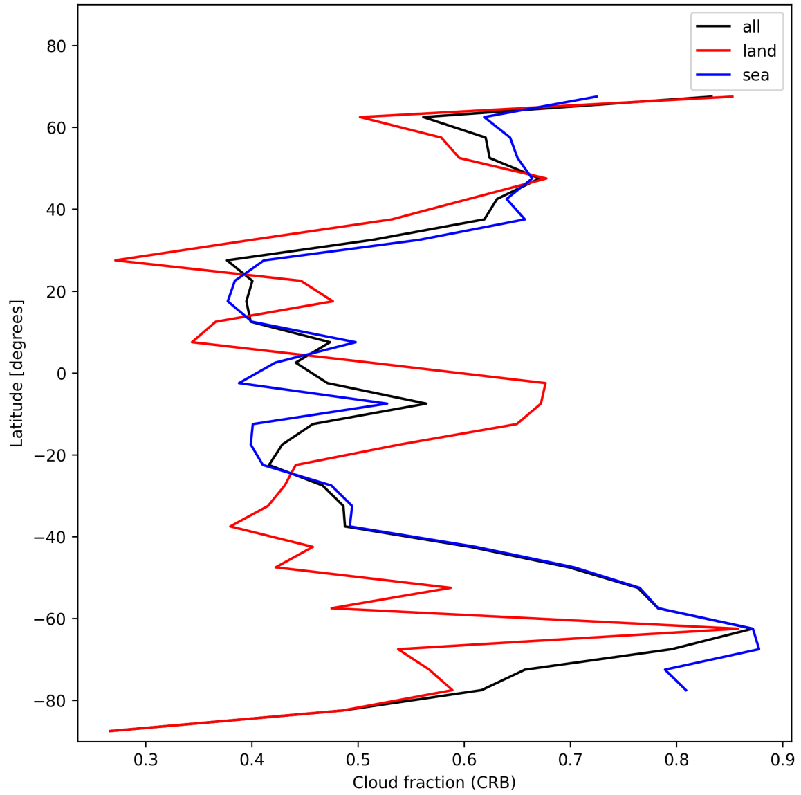
Figure 24: Zonal average of “Cloud fraction (CRB)” for 2024-12-15 to 2024-12-16.
