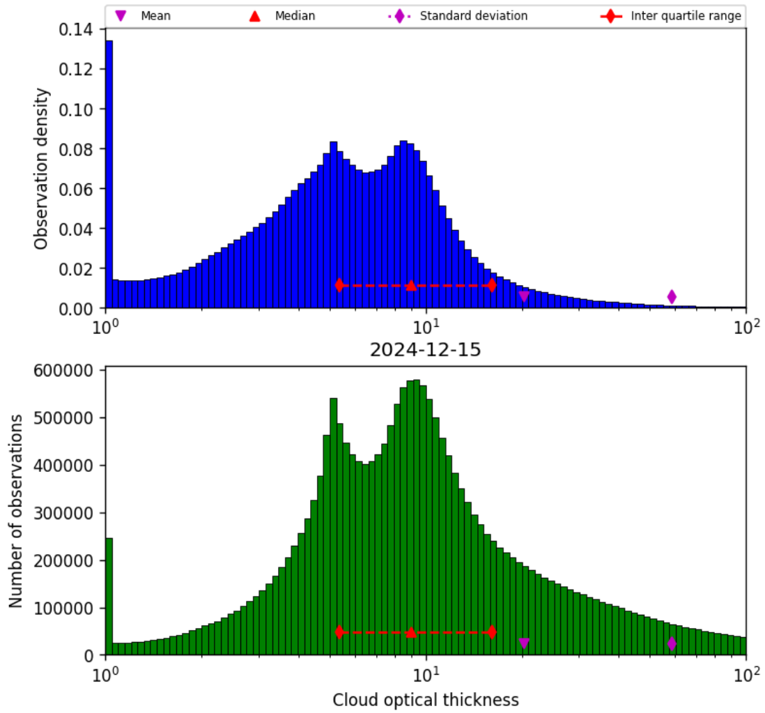
Figure 39: Histogram of “Cloud optical thickness” for 2024-12-15 to 2024-12-16
