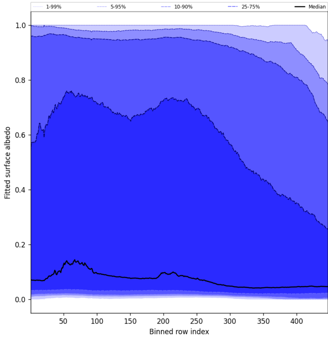
Figure 59: Along track statistics of “Fitted surface albedo” for 2024-12-15 to 2024-12-16
