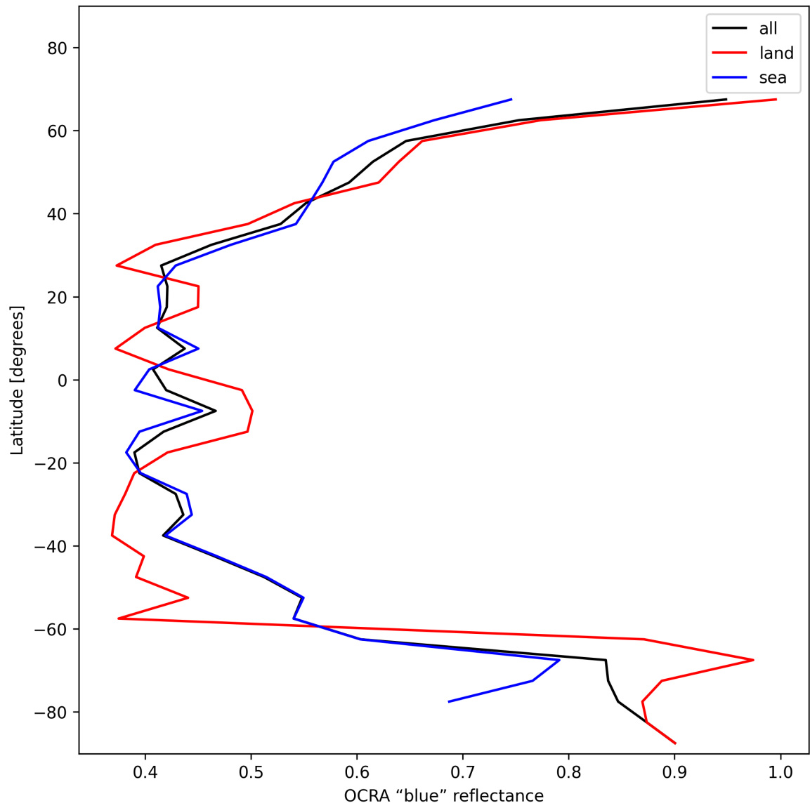
Figure 33: Zonal average of “OCRA “blue” reflectance” for 2024-12-15 to 2024-12-16.
