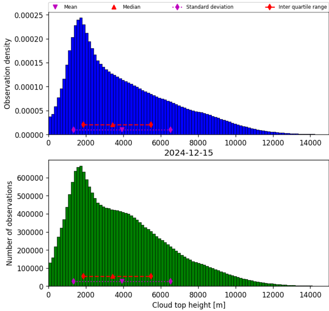
Figure 38: Histogram of “Cloud top height” for 2024-12-15 to 2024-12-16
