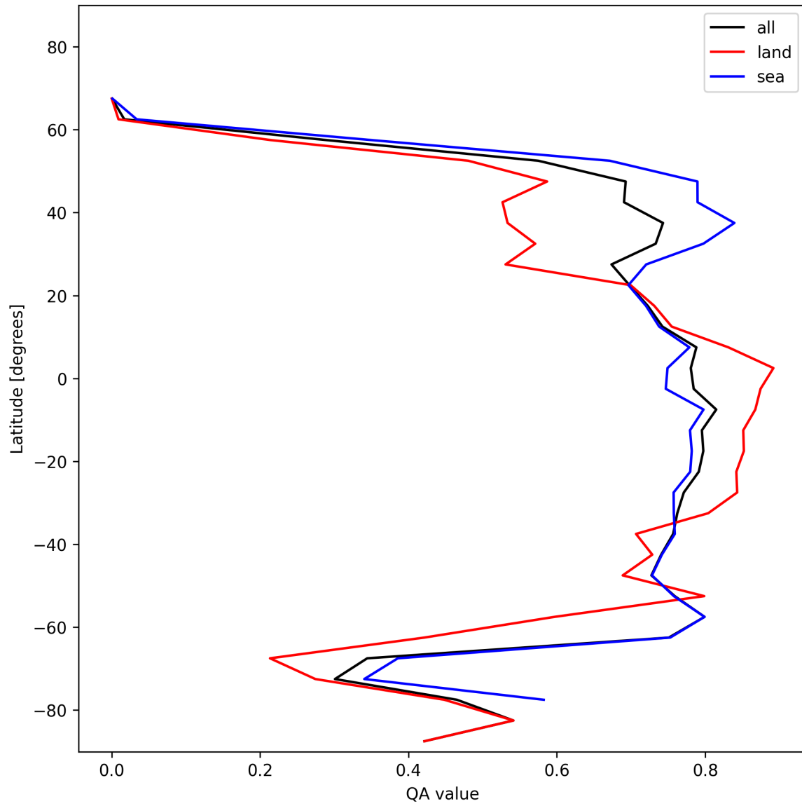
Figure 20: Zonal average of “QA value” for 2024-12-15 to 2024-12-16.
