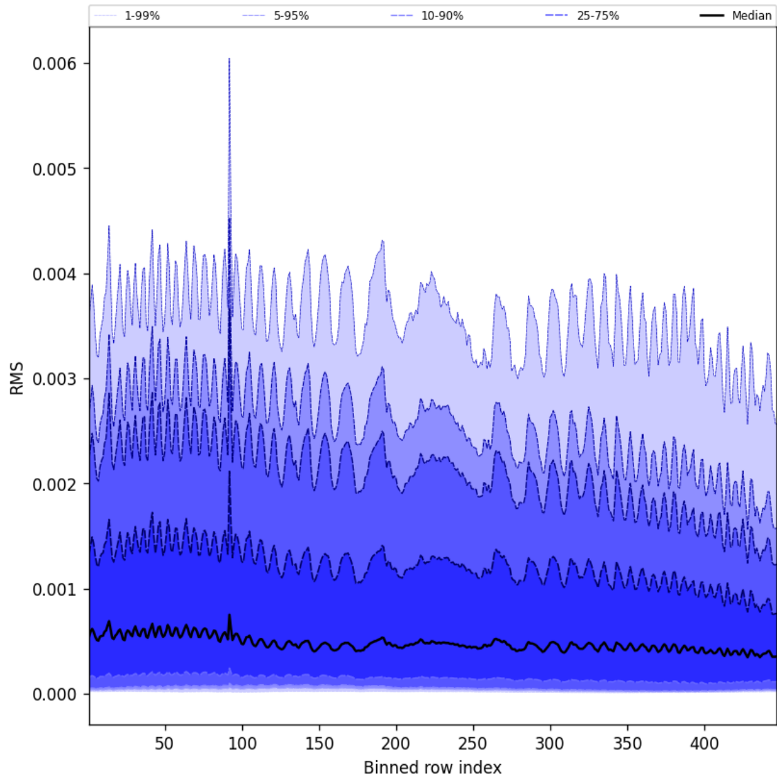
Figure 61: Along track statistics of “RMS” for 2024-12-15 to 2024-12-16
