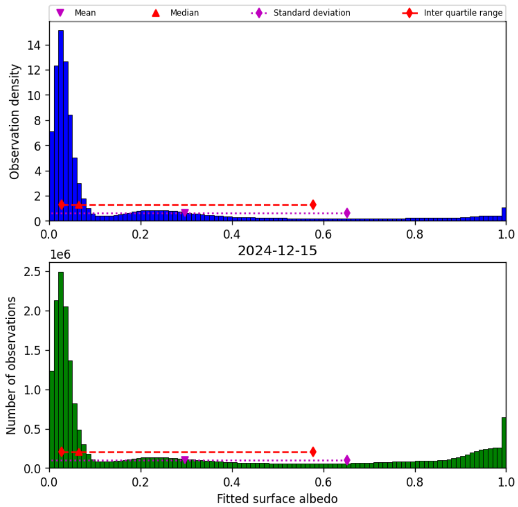
Figure 43: Histogram of “Fitted surface albedo” for 2024-12-15 to 2024-12-16
