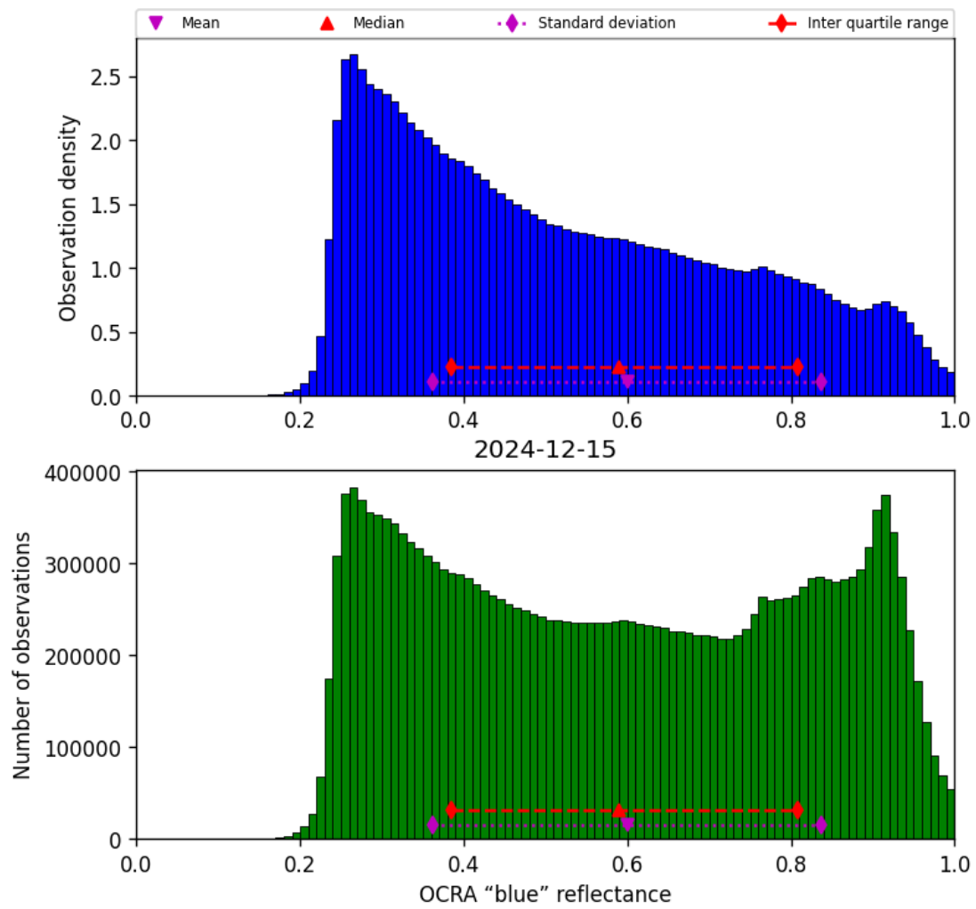
Figure 49: Histogram of "OCRA "blue" reflectance" for 2024-12-15 to 2024-12-16
