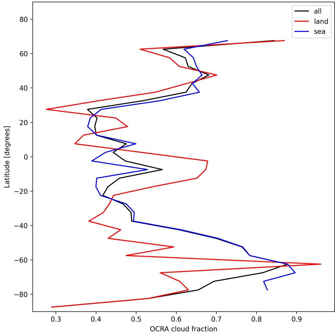
Figure 32: Zonal average of “OCRA cloud fraction” for 2024-12-15 to 2024-12-16.
