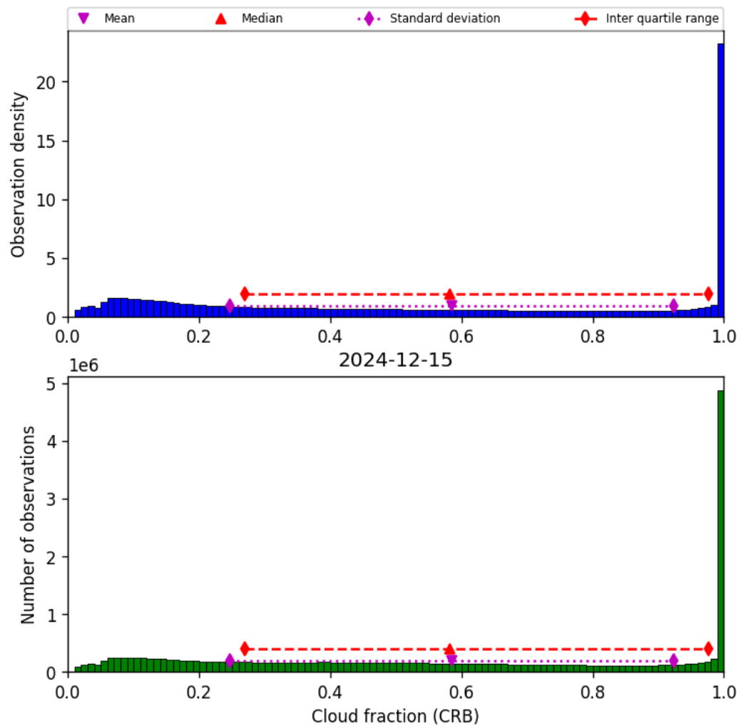
Figure 40: Histogram of “Cloud fraction (CRB)” for 2024-12-15 to 2024-12-16
