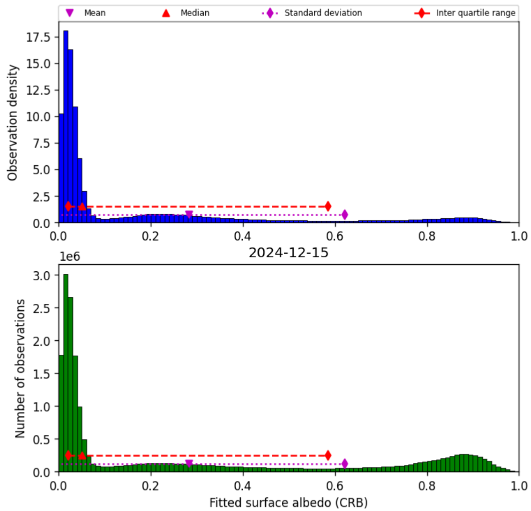
Figure 44: Histogram of “Fitted surface albedo (CRB)” for 2024-12-15 to 2024-12-16
