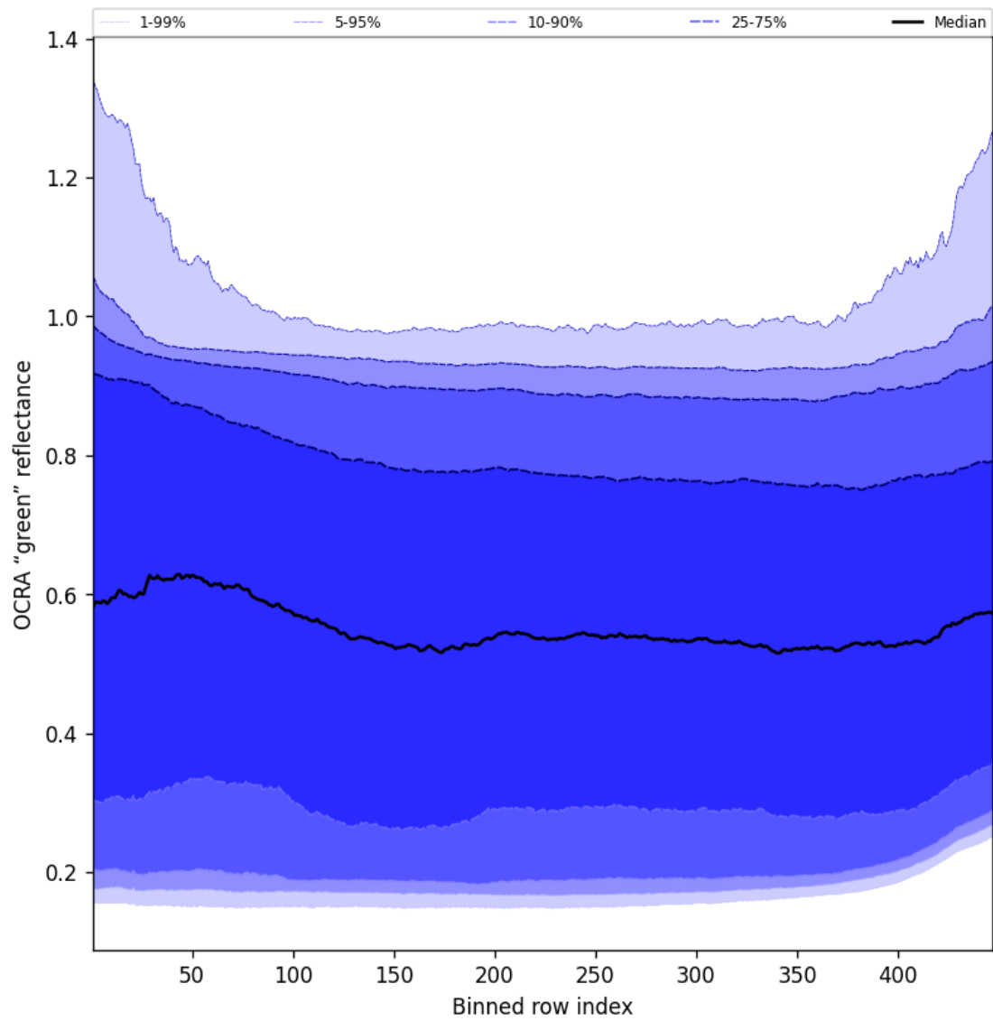
Figure 66: Along track statistics of "OCRA "green" reflectance" for 2024-12-15 to 2024-12-16
