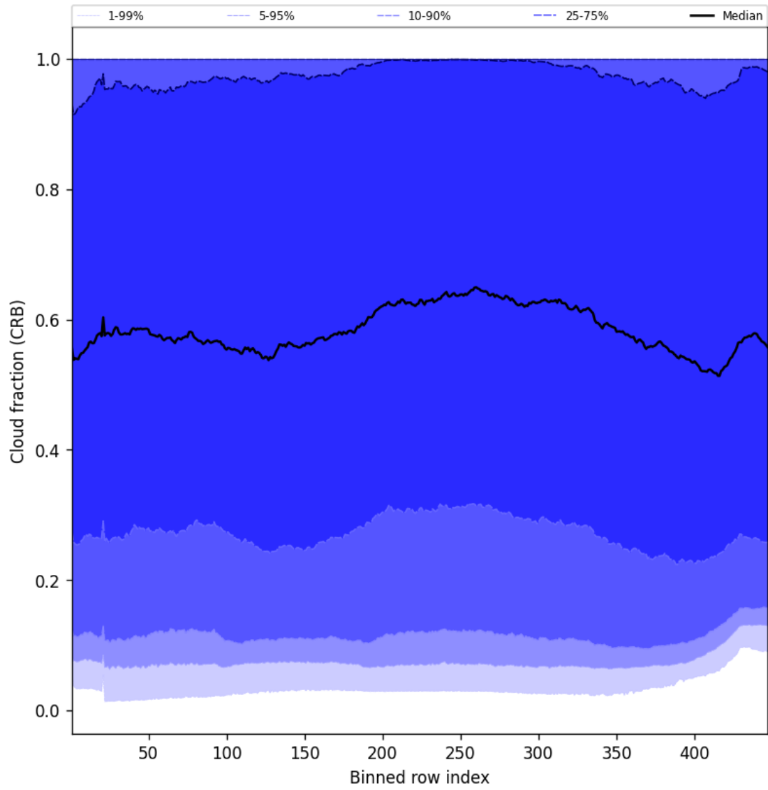
Figure 56: Along track statistics of “Cloud fraction (CRB)” for 2024-12-15 to 2024-12-16
