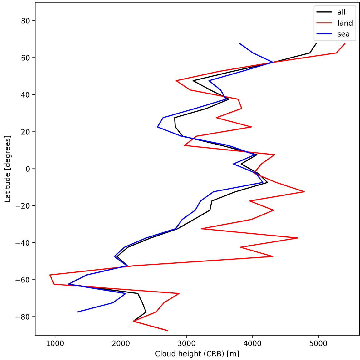
Figure 25: Zonal average of “Cloud height (CRB)” for 2024-12-15 to 2024-12-16.
