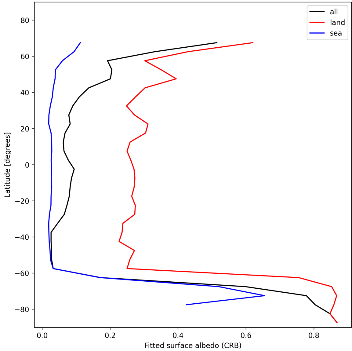
Figure 28: Zonal average of “Fitted surface albedo (CRB)” for 2024-12-15 to 2024-12-16.
