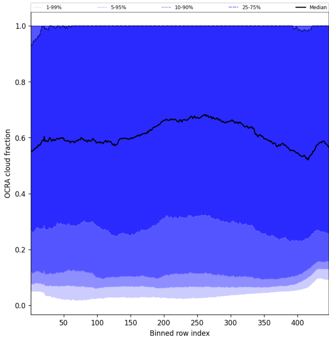
Figure 64: Along track statistics of “OCRA cloud fraction” for 2024-12-15 to 2024-12-16
