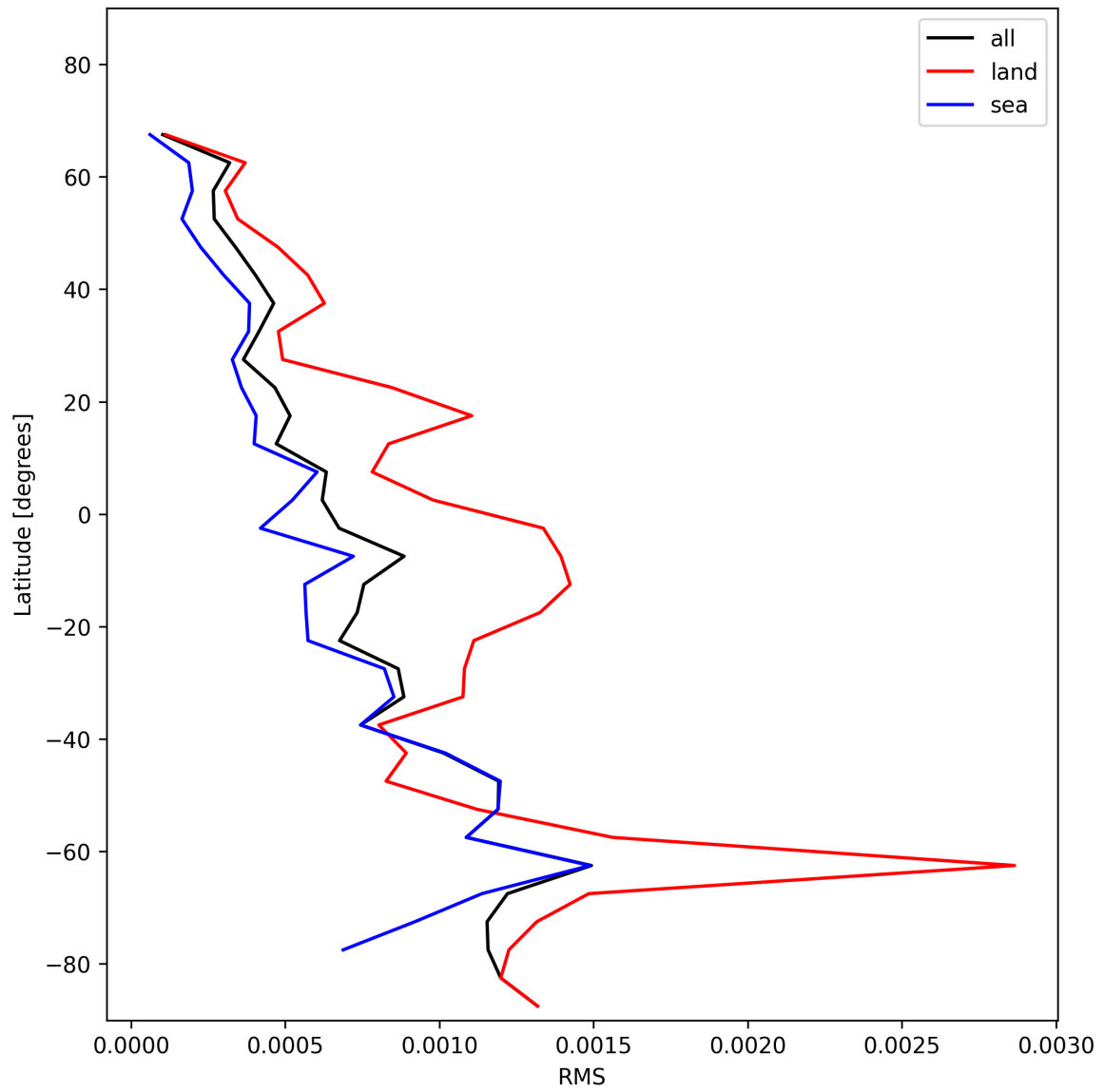
Figure 29: Zonal average of “RMS” for 2024-12-15 to 2024-12-16.
