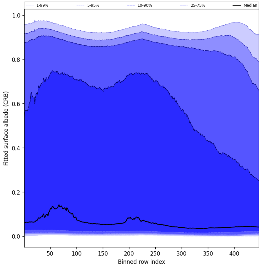
Figure 60: Along track statistics of “Fitted surface albedo (CRB)” for 2024-12-15 to 2024-12-16
