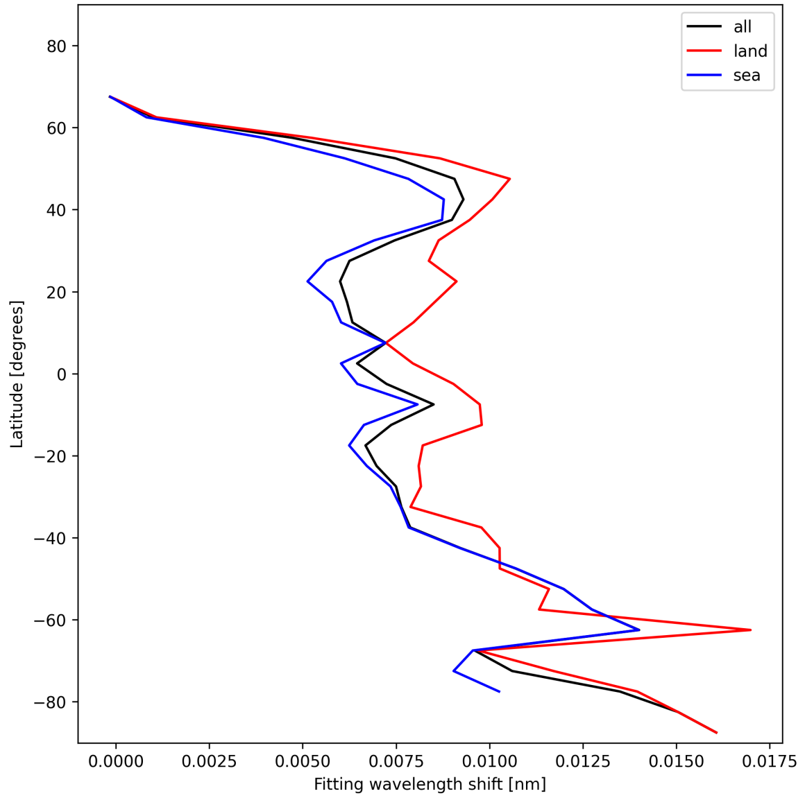
Figure 31: Zonal average of “Fitting wavelength shift” for 2024-12-15 to 2024-12-16.
