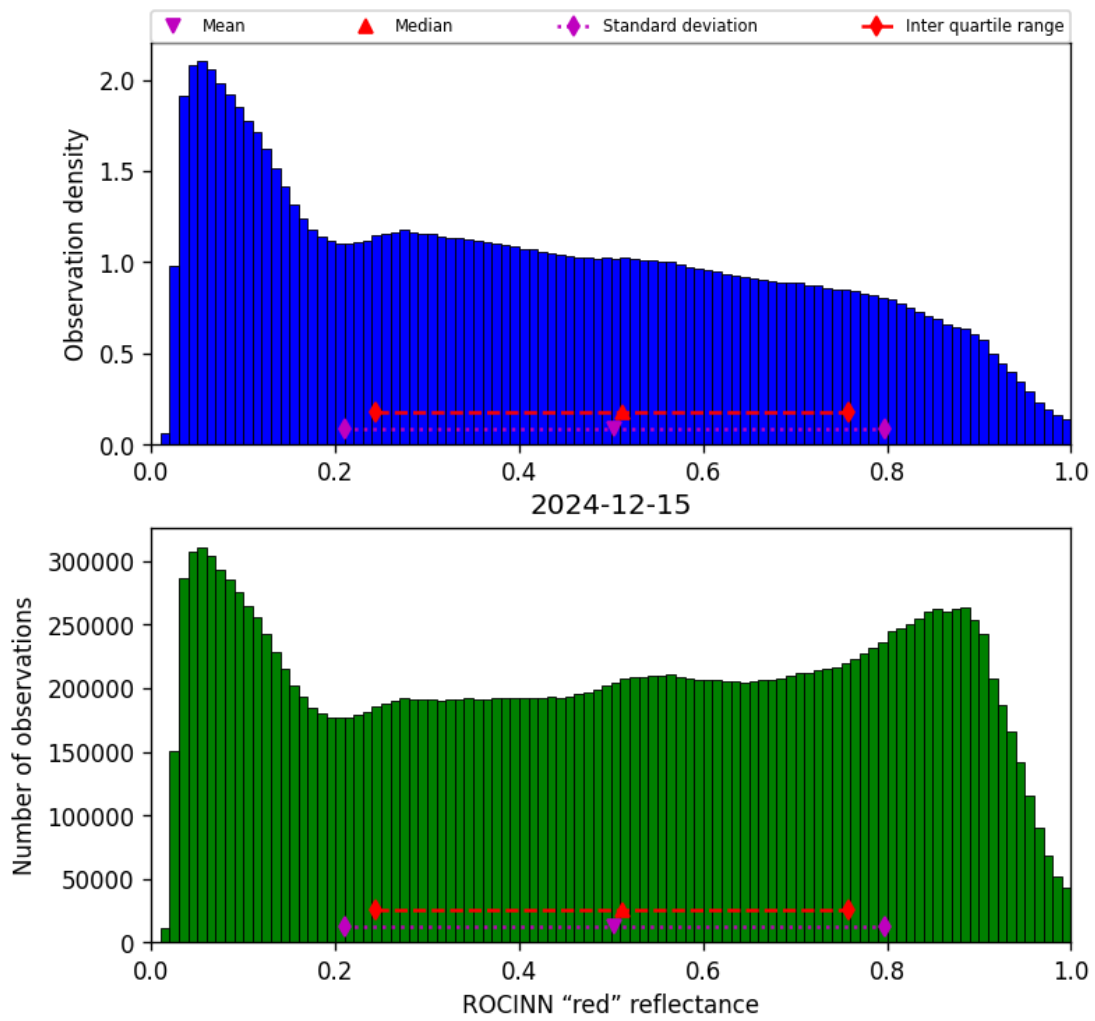
Figure 51: Histogram of “ROCINN “red” reflectance” for 2024-12-15 to 2024-12-16
