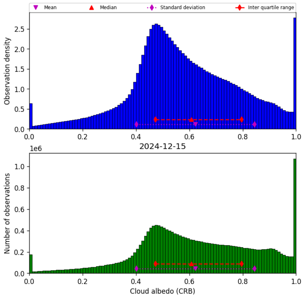
Figure 42: Histogram of “Cloud albedo (CRB)” for 2024-12-15 to 2024-12-16
