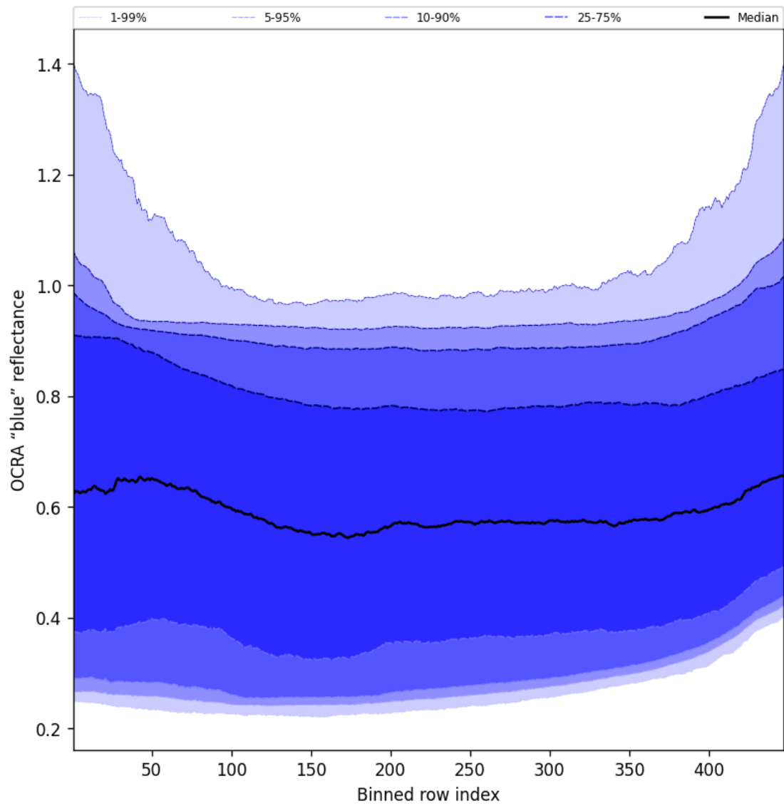
Figure 65: Along track statistics of “OCRA “blue” reflectance” for 2024-12-15 to 2024-12-16
