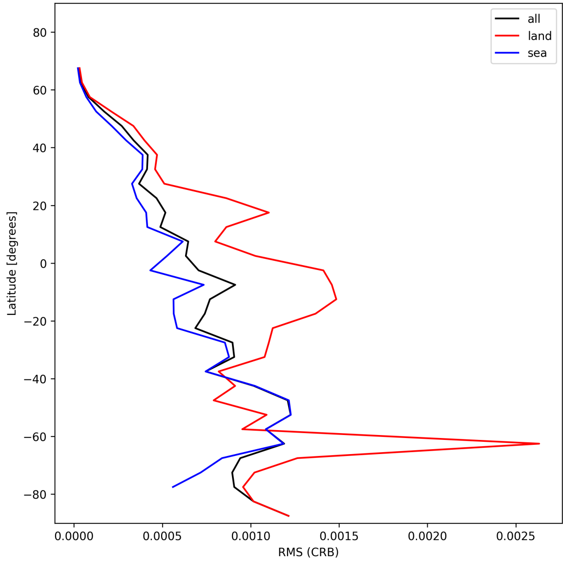
Figure 30: Zonal average of “RMS (CRB)” for 2024-12-15 to 2024-12-16.
