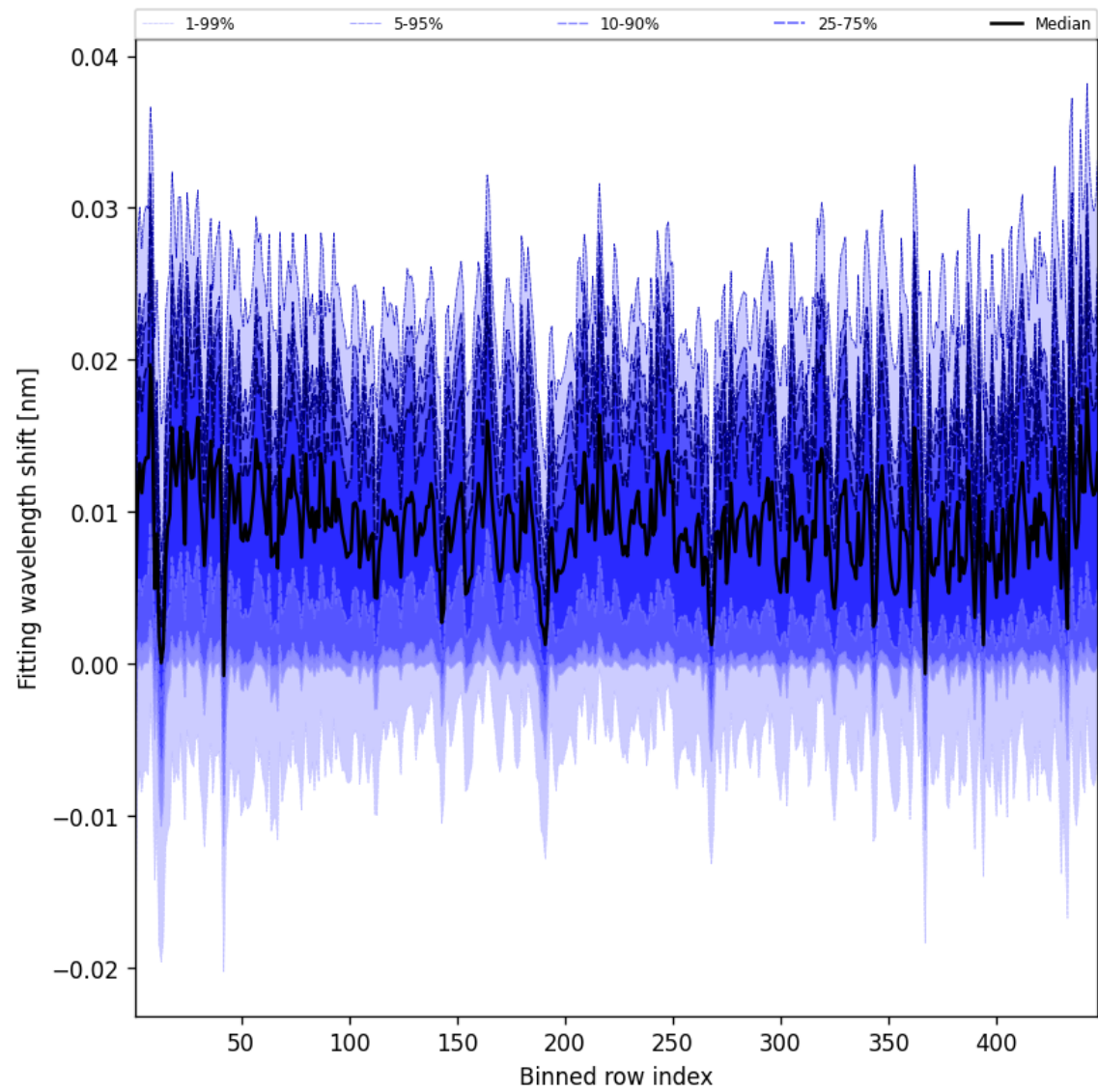
Figure 63: Along track statistics of “Fitting wavelength shift” for 2024-12-15 to 2024-12-16
