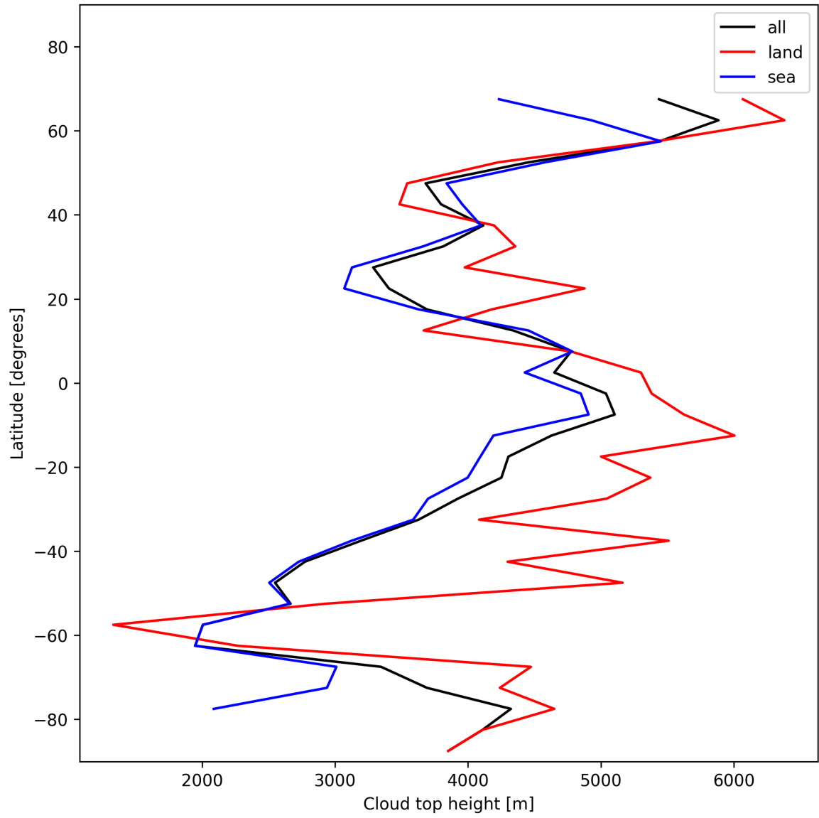
Figure 22: Zonal average of “Cloud top height” for 2024-12-15 to 2024-12-16.
