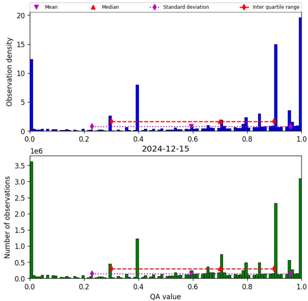
Figure 36: Histogram of “QA value” for 2024-12-15 to 2024-12-16
