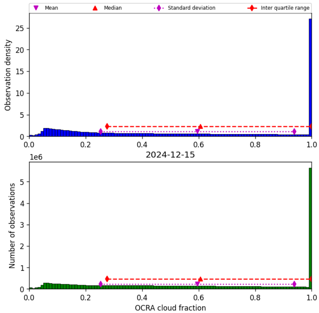
Figure 48: Histogram of “OCRA cloud fraction” for 2024-12-15 to 2024-12-16
