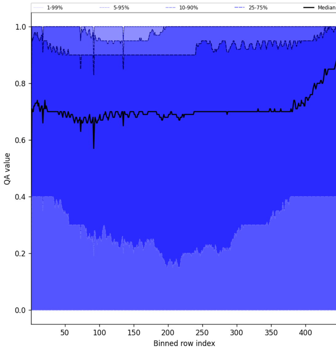
Figure 52: Along track statistics of “QA value” for 2024-12-15 to 2024-12-16
