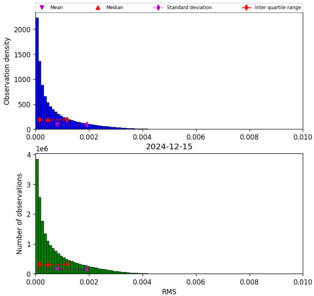
Figure 45: Histogram of “RMS” for 2024-12-15 to 2024-12-16
