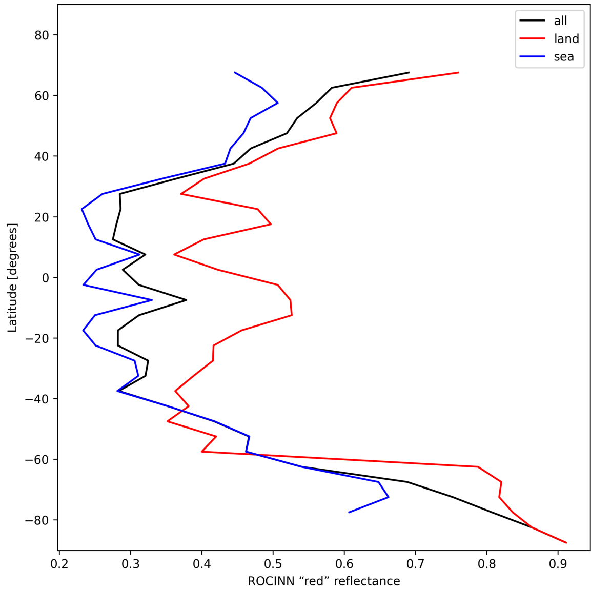
Figure 35: Zonal average of “ROCINN “red” reflectance” for 2024-12-15 to 2024-12-16.
