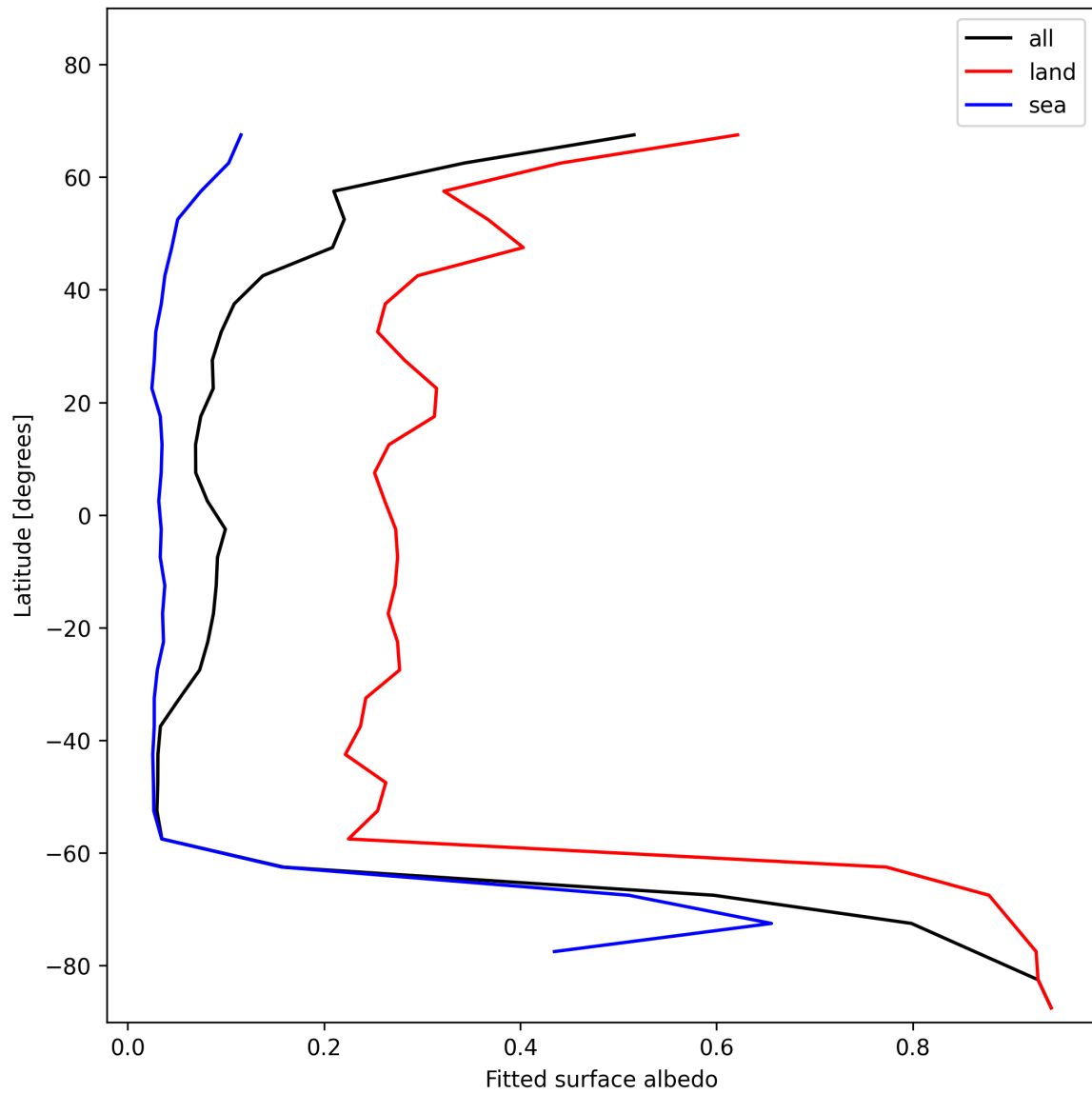
Figure 27: Zonal average of “Fitted surface albedo” for 2024-12-15 to 2024-12-16.
