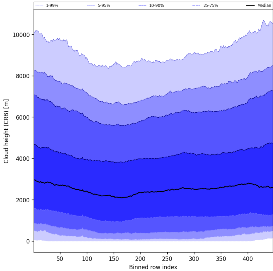
Figure 57: Along track statistics of “Cloud height (CRB)” for 2024-12-15 to 2024-12-16
