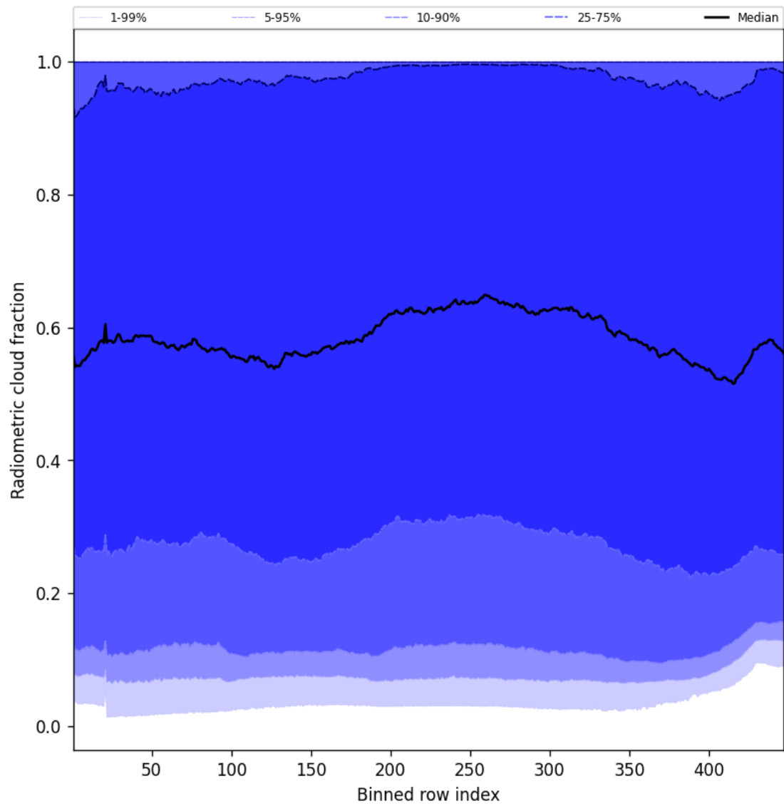
Figure 53: Along track statistics of “Radiometric cloud fraction” for 2024-12-15 to 2024-12-16
