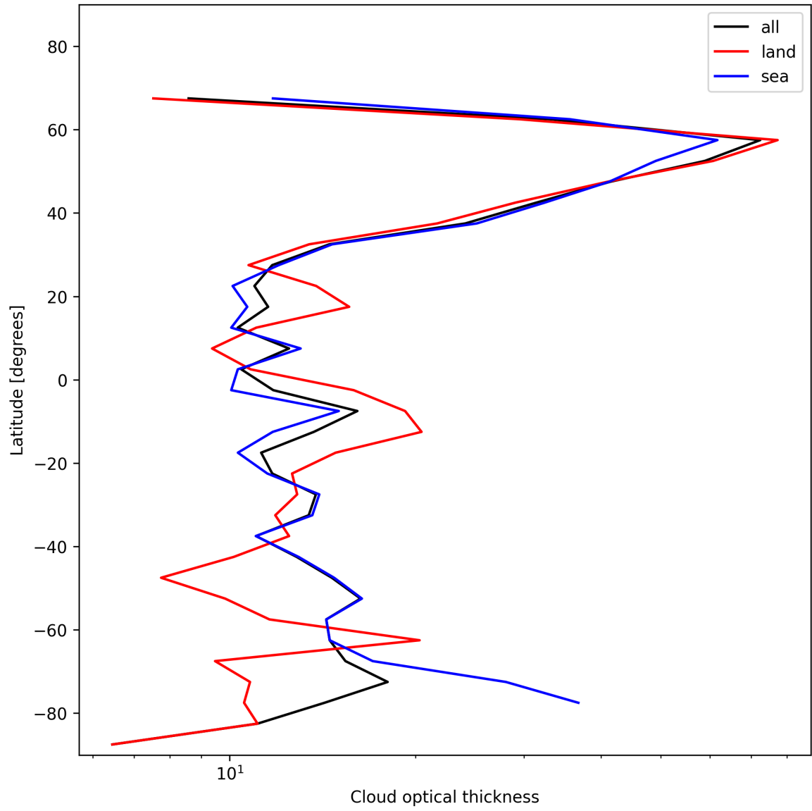
Figure 23: Zonal average of “Cloud optical thickness” for 2024-12-15 to 2024-12-16.
