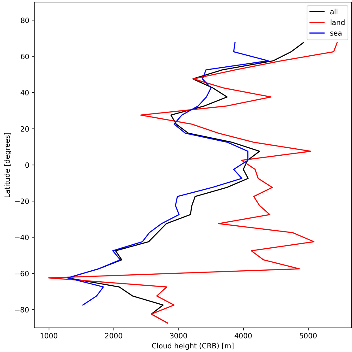
Figure 25: Zonal average of “Cloud height (CRB)” for 2024-12-16 to 2024-12-17.
