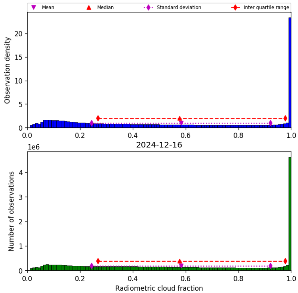
Figure 37: Histogram of “Radiometric cloud fraction” for 2024-12-16 to 2024-12-17
