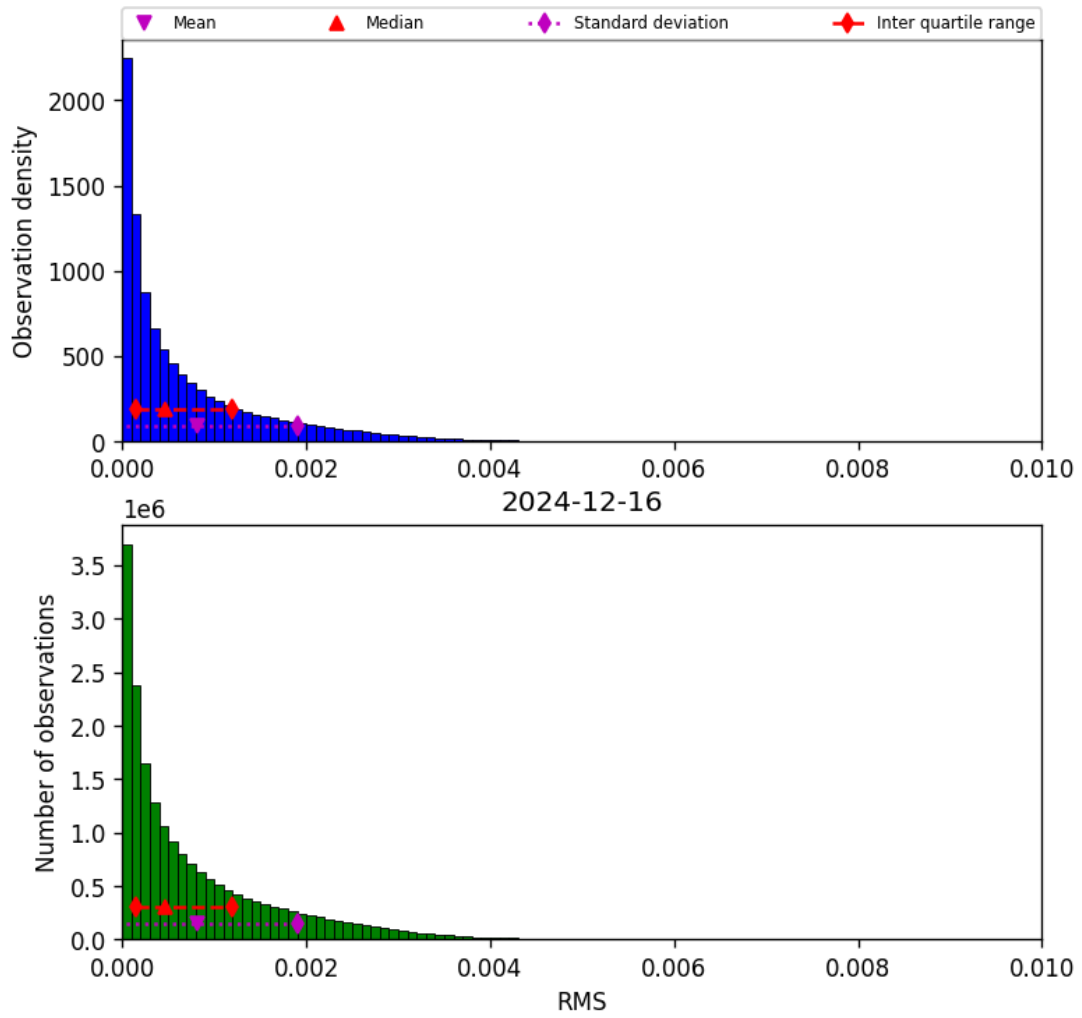
Figure 45: Histogram of “RMS” for 2024-12-16 to 2024-12-17
