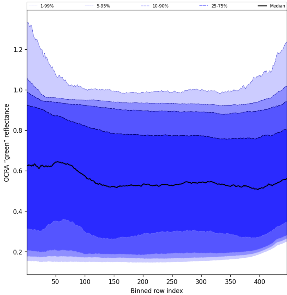
Figure 66: Along track statistics of "OCRA "green" reflectance" for 2024-12-16 to 2024-12-17
