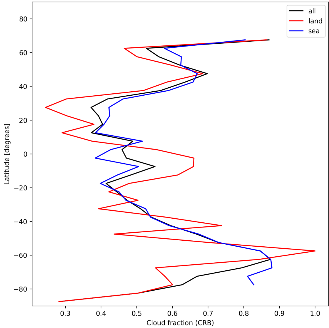
Figure 24: Zonal average of “Cloud fraction (CRB)” for 2024-12-16 to 2024-12-17.
