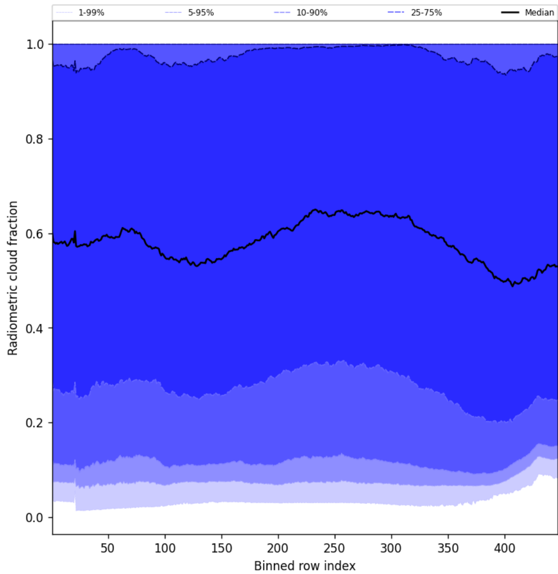
Figure 53: Along track statistics of “Radiometric cloud fraction” for 2024-12-16 to 2024-12-17
