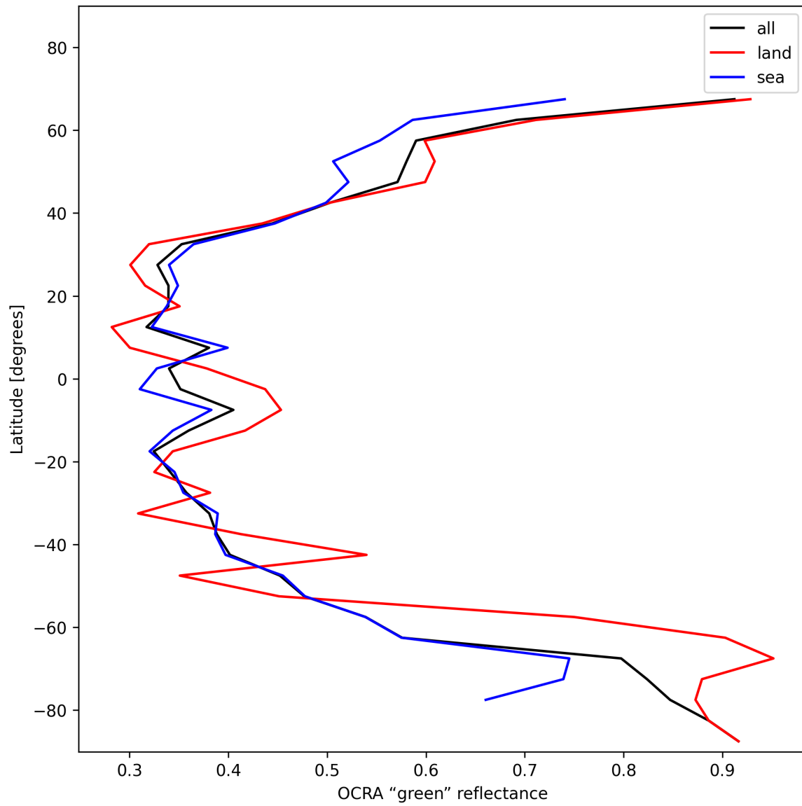
Figure 34: Zonal average of “OCRA “green” reflectance” for 2024-12-16 to 2024-12-17.
