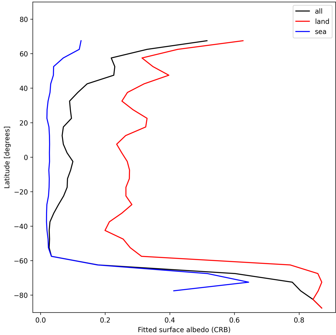
Figure 28: Zonal average of “Fitted surface albedo (CRB)” for 2024-12-16 to 2024-12-17.
