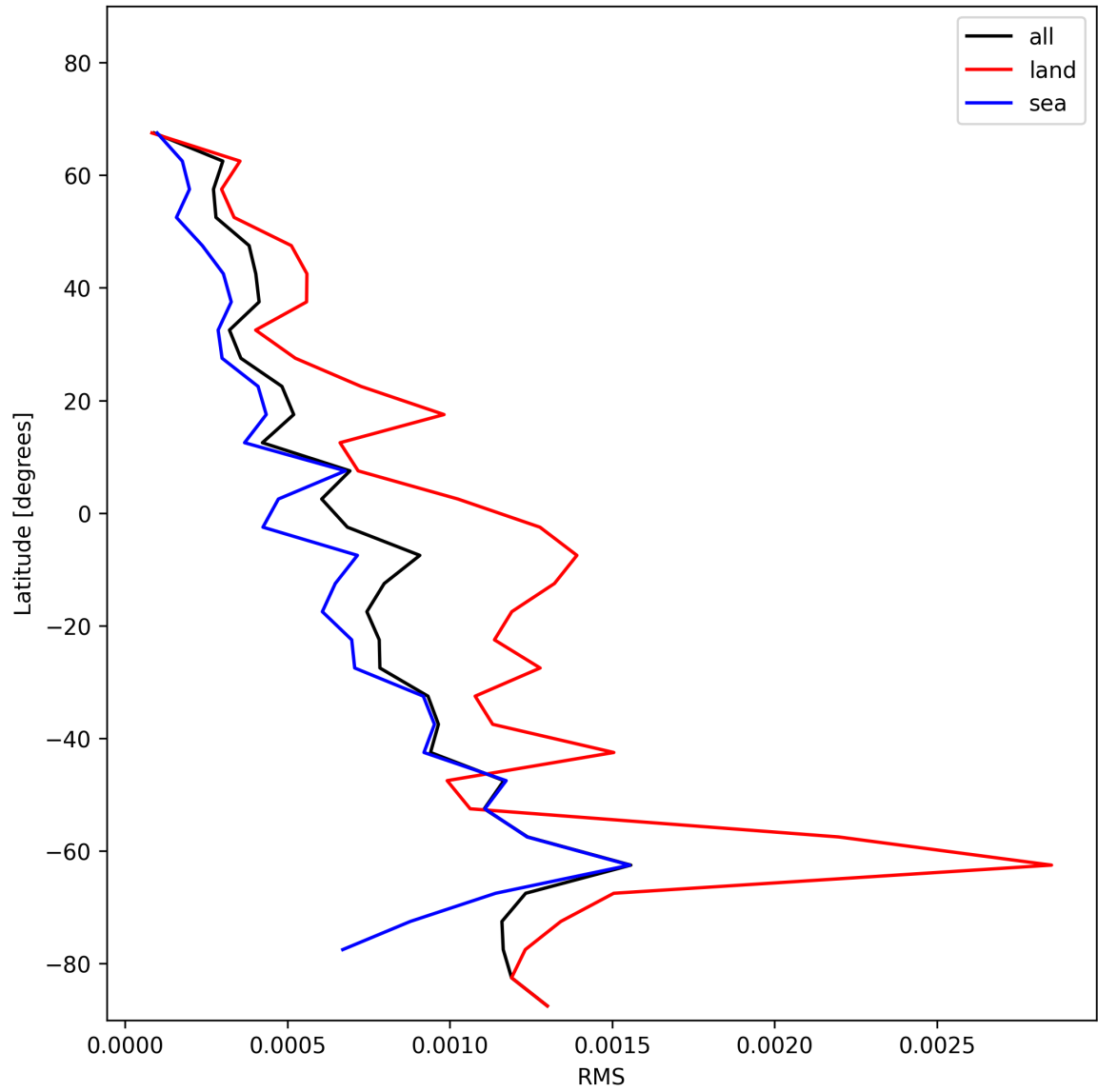
Figure 29: Zonal average of “RMS” for 2024-12-16 to 2024-12-17.
