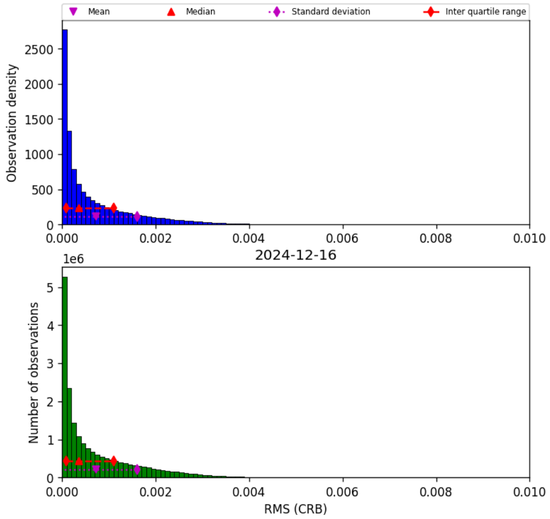
Figure 46: Histogram of “RMS (CRB)” for 2024-12-16 to 2024-12-17
