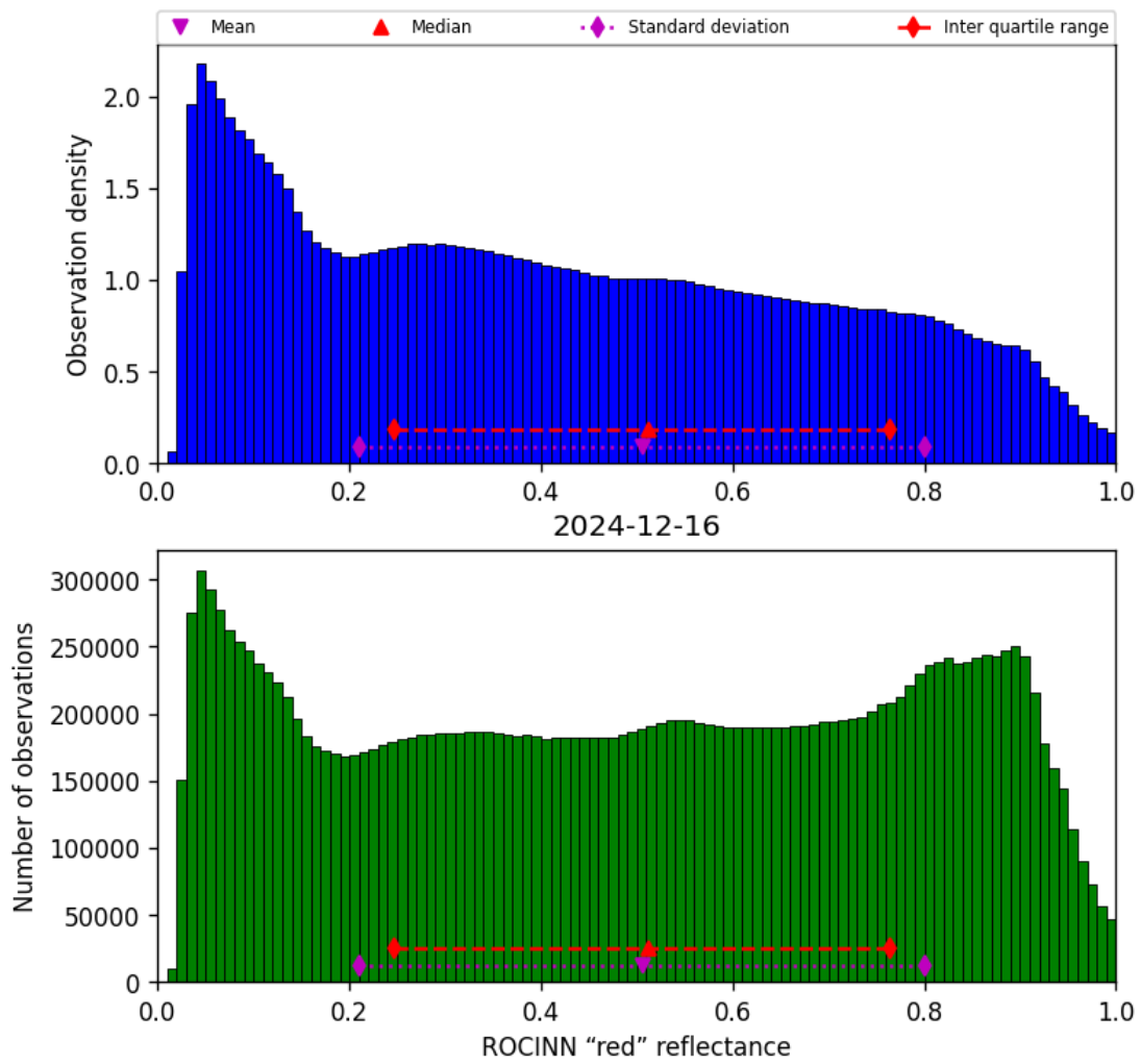
Figure 51: Histogram of “ROCINN “red” reflectance” for 2024-12-16 to 2024-12-17
