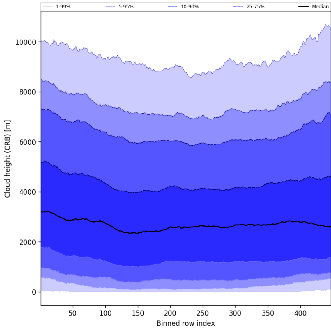
Figure 57: Along track statistics of “Cloud height (CRB)” for 2024-12-16 to 2024-12-17
