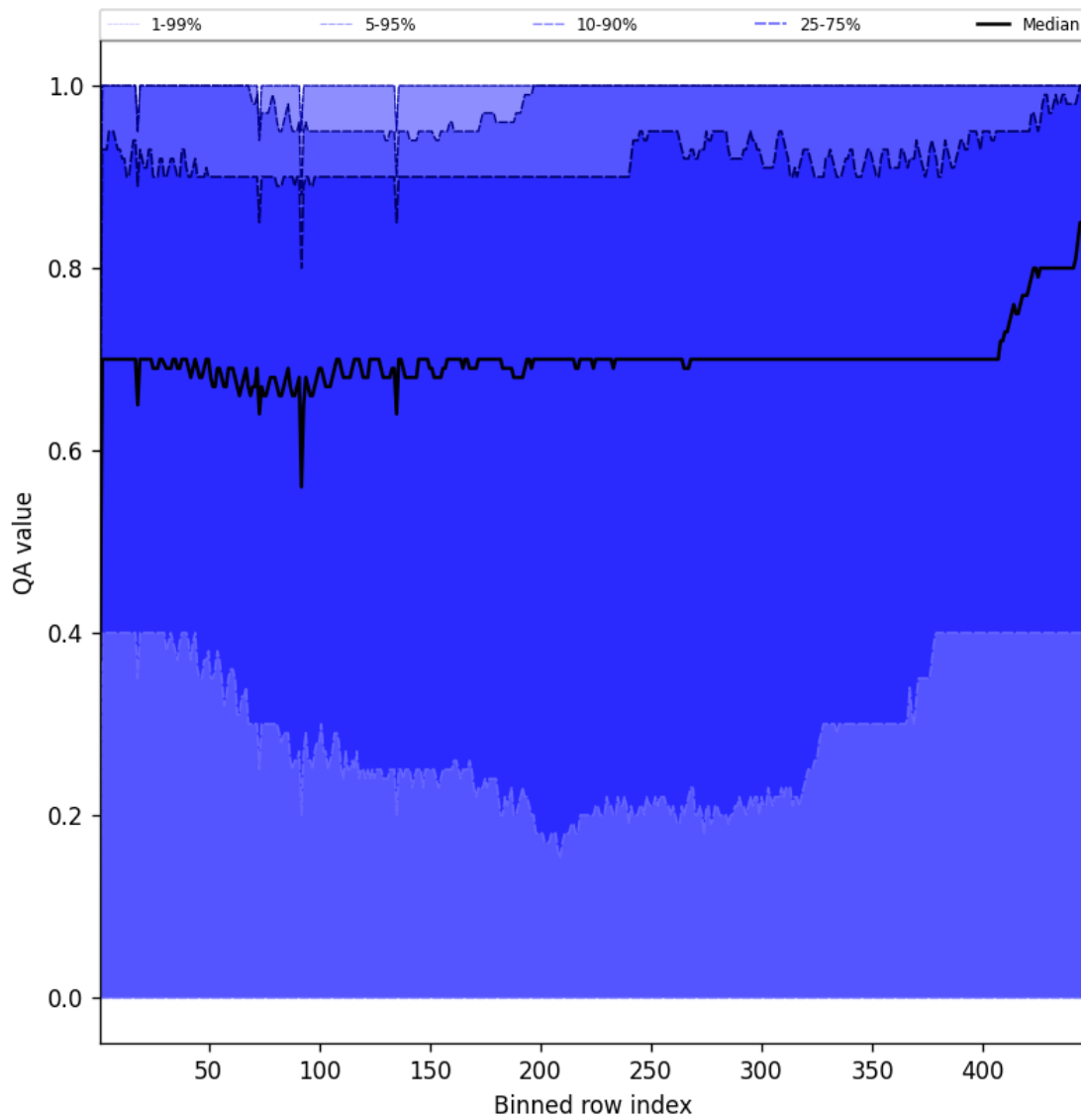
Figure 52: Along track statistics of “QA value” for 2024-12-16 to 2024-12-17
