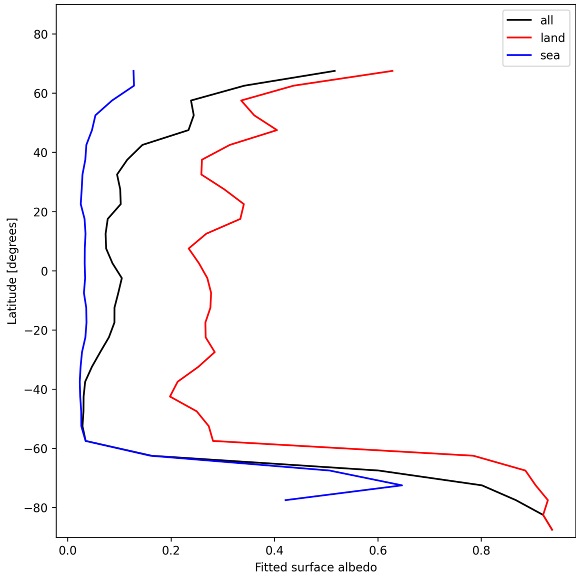
Figure 27: Zonal average of “Fitted surface albedo” for 2024-12-16 to 2024-12-17.
