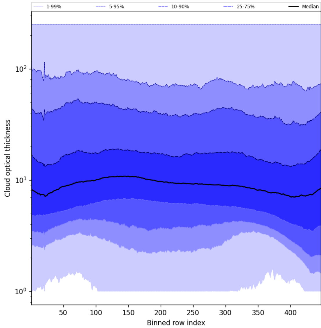
Figure 55: Along track statistics of “Cloud optical thickness” for 2024-12-16 to 2024-12-17
