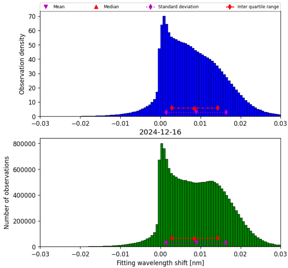
Figure 47: Histogram of “Fitting wavelength shift” for 2024-12-16 to 2024-12-17
