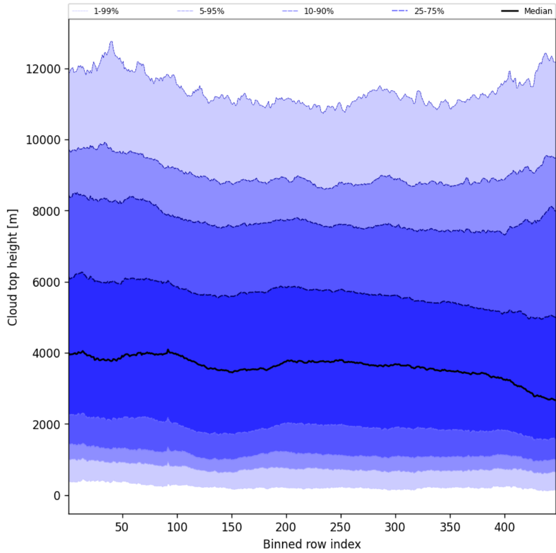
Figure 54: Along track statistics of "Cloud top height" for 2024-12-16 to 2024-12-17
