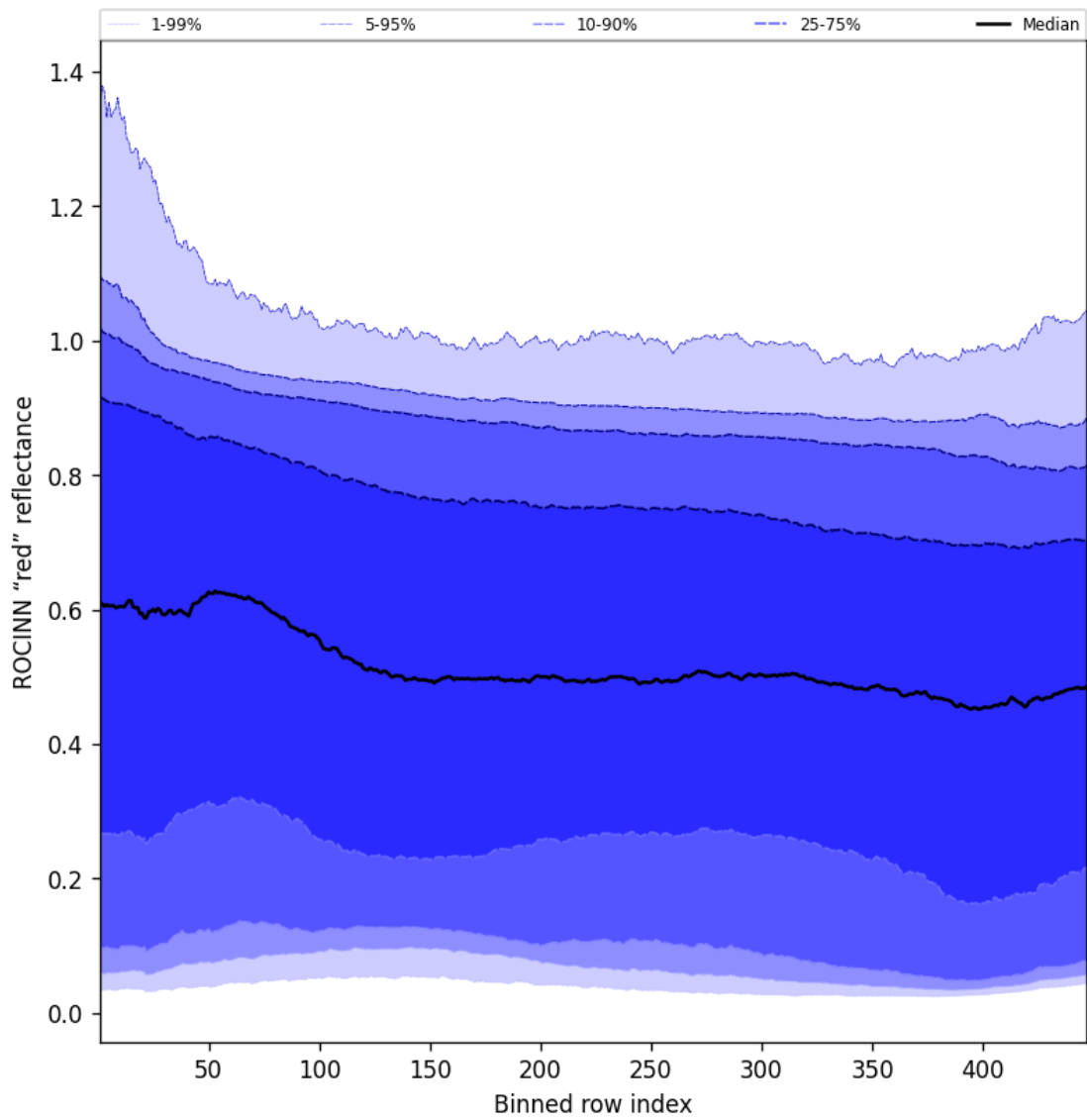
Figure 67: Along track statistics of “ROCINN “red” reflectance” for 2024-12-16 to 2024-12-17
