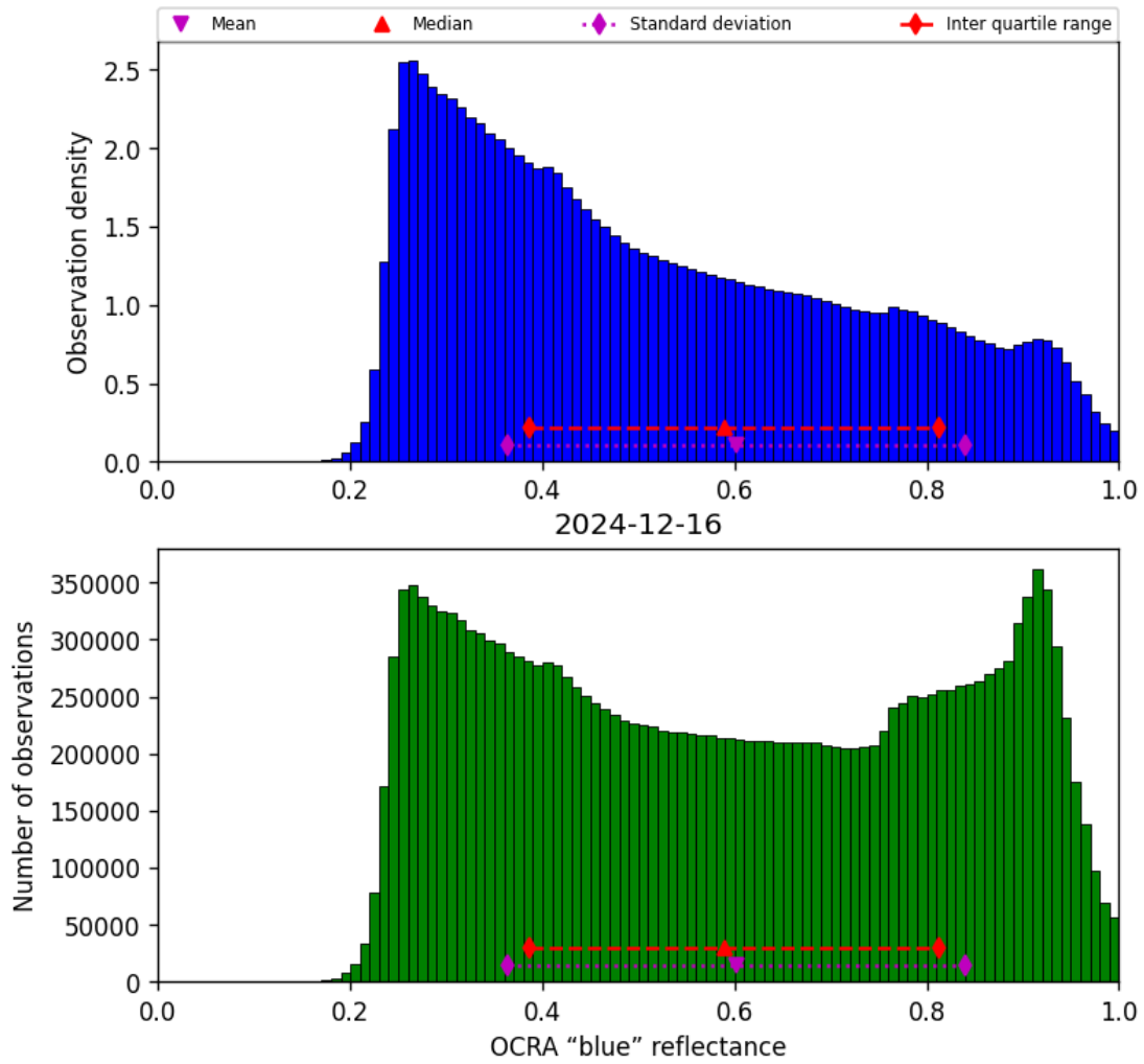
Figure 49: Histogram of “OCRA “blue” reflectance” for 2024-12-16 to 2024-12-17
