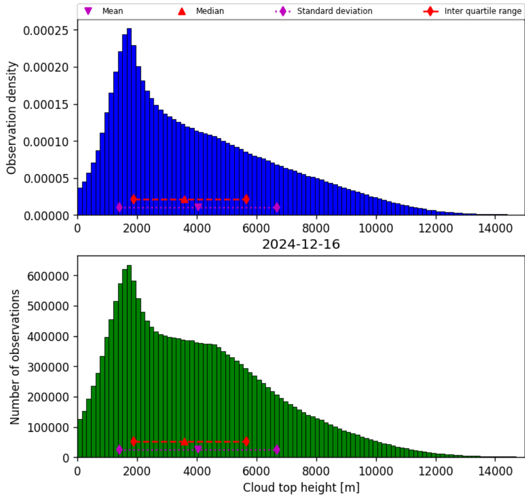
Figure 38: Histogram of “Cloud top height” for 2024-12-16 to 2024-12-17
