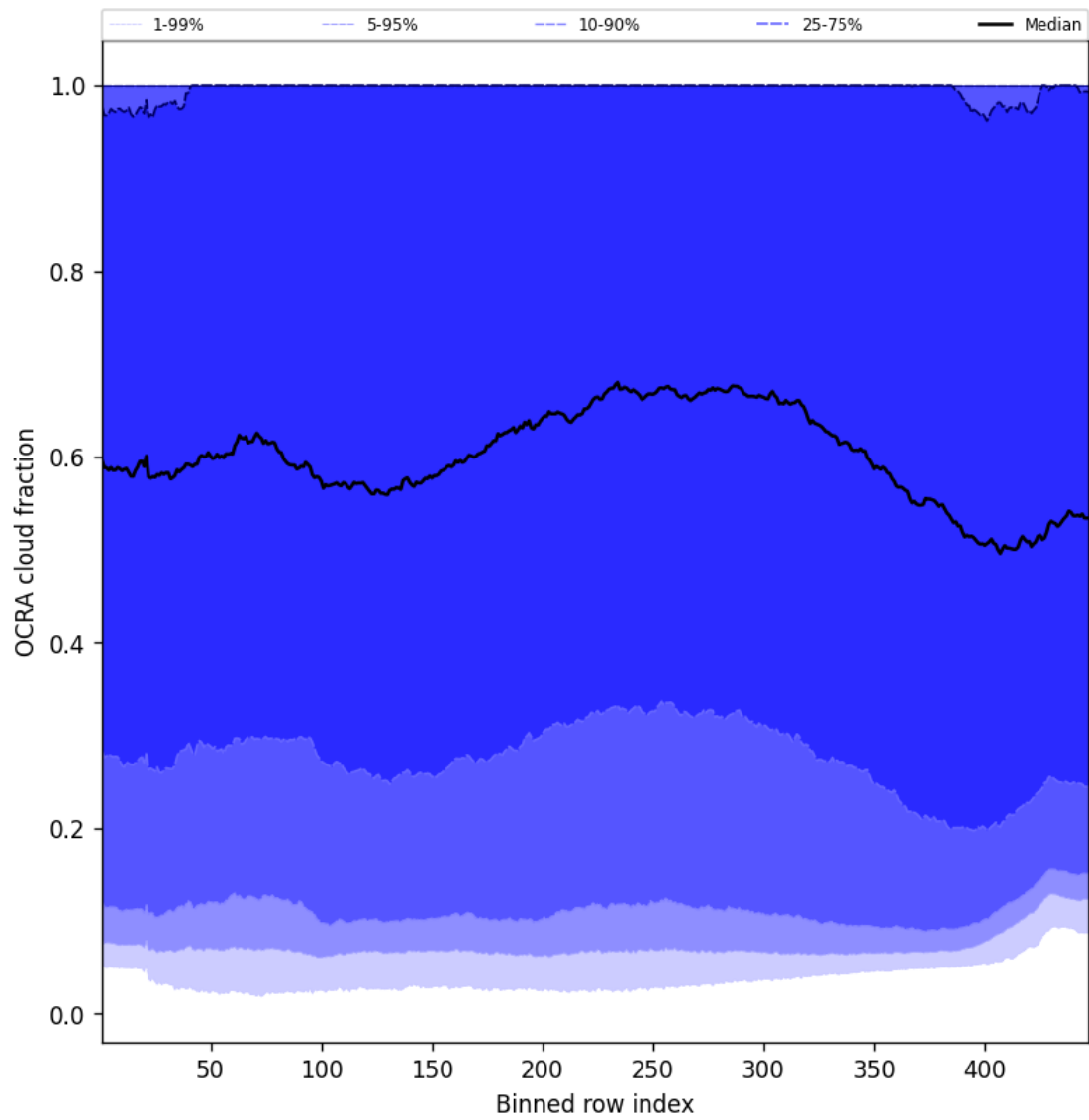
Figure 64: Along track statistics of “OCRA cloud fraction” for 2024-12-16 to 2024-12-17
