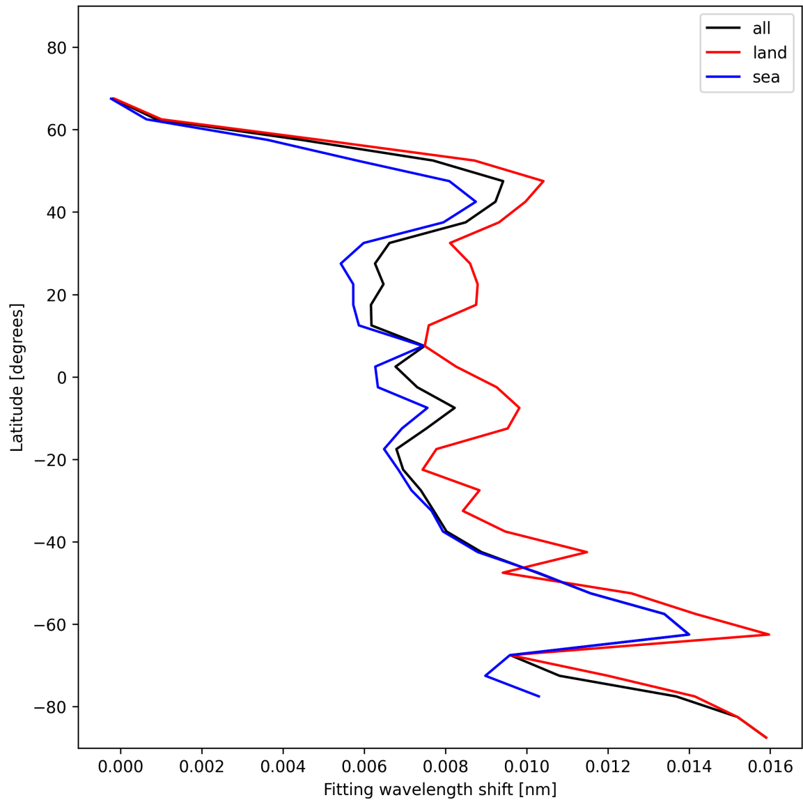
Figure 31: Zonal average of “Fitting wavelength shift” for 2024-12-16 to 2024-12-17.
