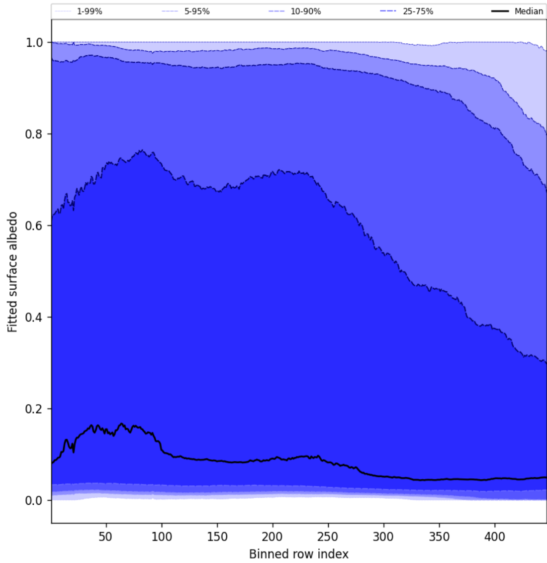
Figure 59: Along track statistics of “Fitted surface albedo” for 2024-12-16 to 2024-12-17
