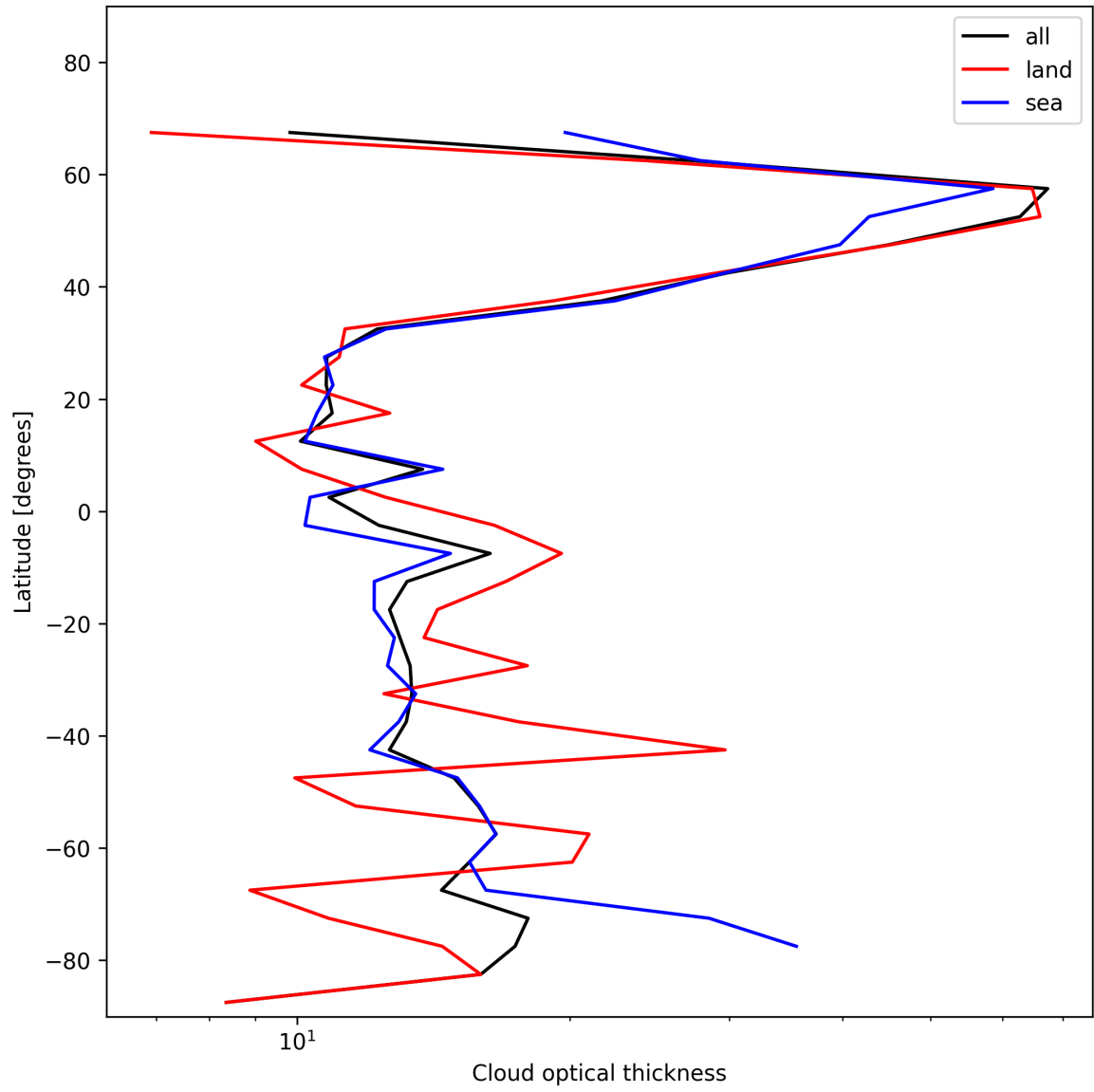
Figure 23: Zonal average of “Cloud optical thickness” for 2024-12-16 to 2024-12-17.
