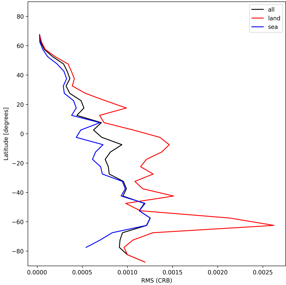
Figure 30: Zonal average of “RMS (CRB)” for 2024-12-16 to 2024-12-17.
