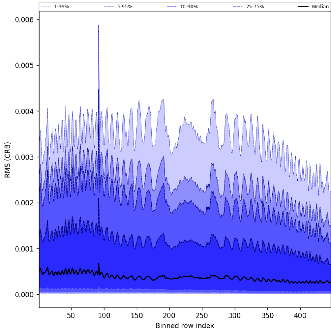
Figure 62: Along track statistics of “RMS (CRB)” for 2024-12-16 to 2024-12-17
