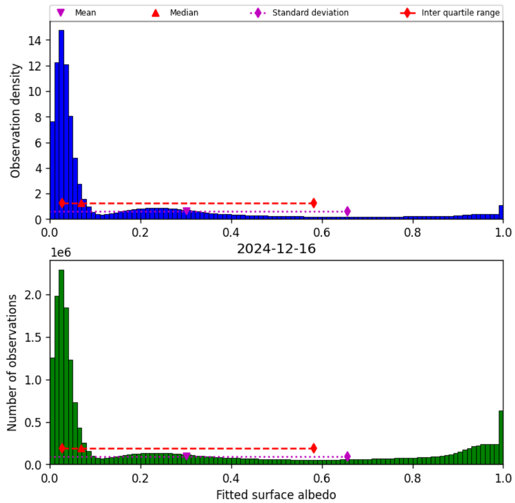
Figure 43: Histogram of “Fitted surface albedo” for 2024-12-16 to 2024-12-17
