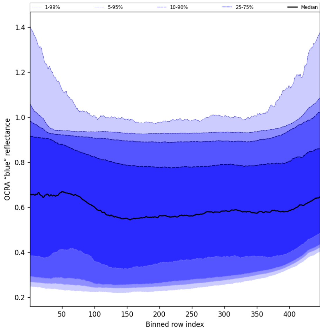
Figure 65: Along track statistics of "OCRA "blue" reflectance" for 2024-12-16 to 2024-12-17
