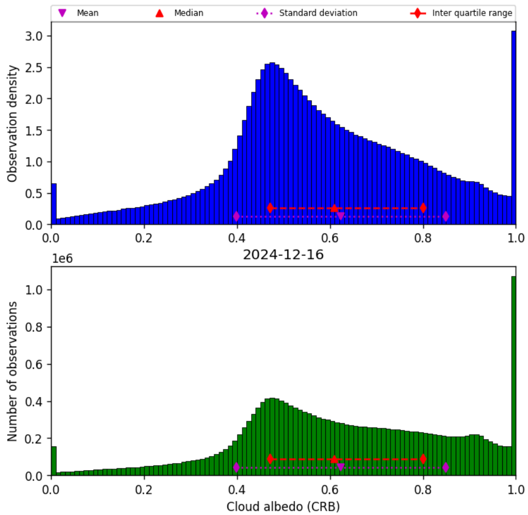
Figure 42: Histogram of “Cloud albedo (CRB)” for 2024-12-16 to 2024-12-17
