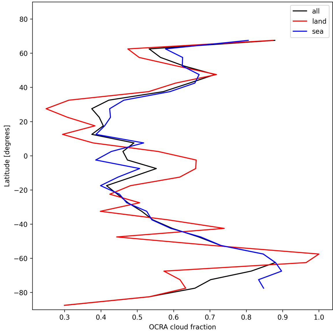
Figure 32: Zonal average of “OCRA cloud fraction” for 2024-12-16 to 2024-12-17.
