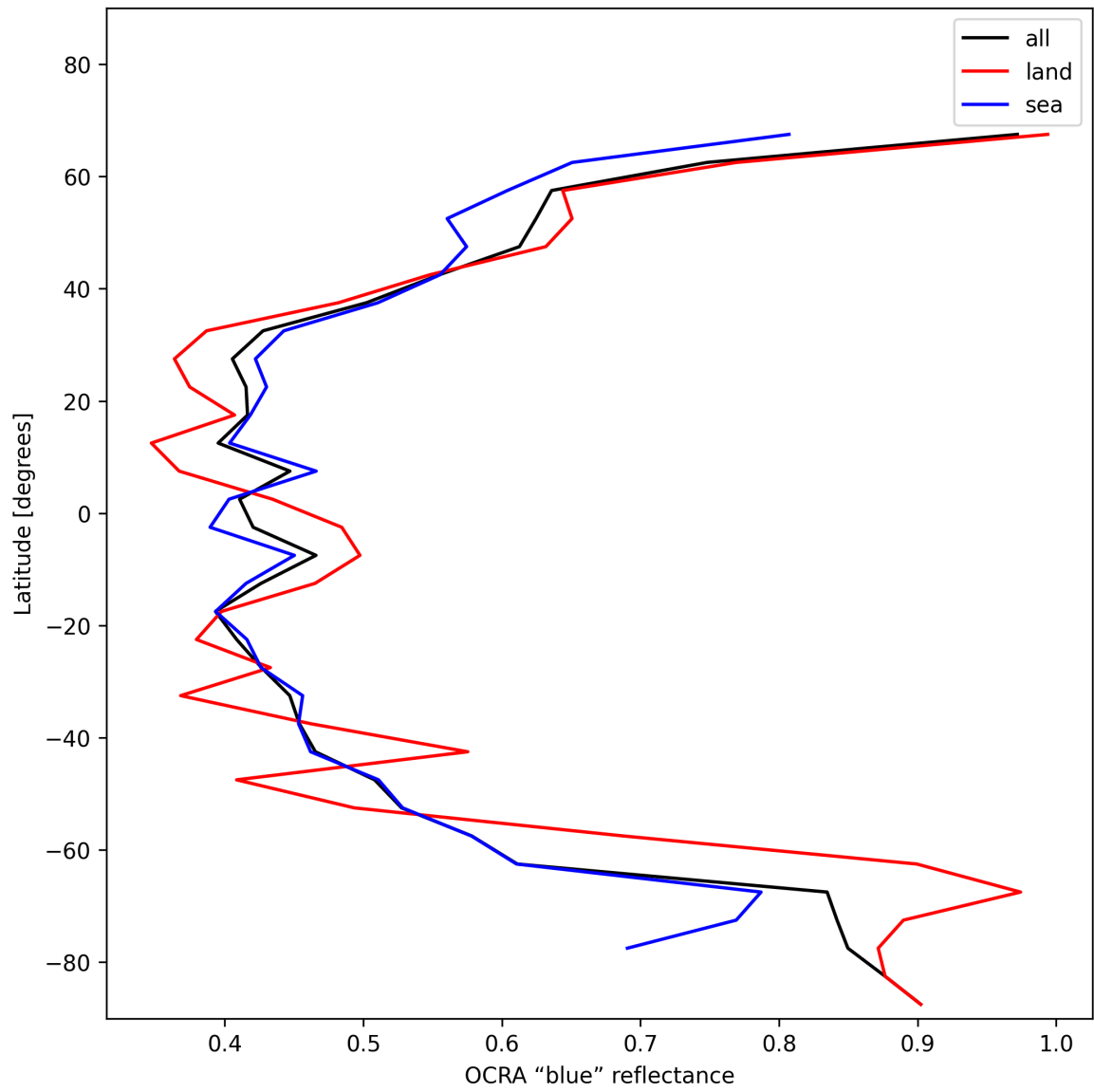
Figure 33: Zonal average of “OCRA “blue” reflectance” for 2024-12-16 to 2024-12-17.
