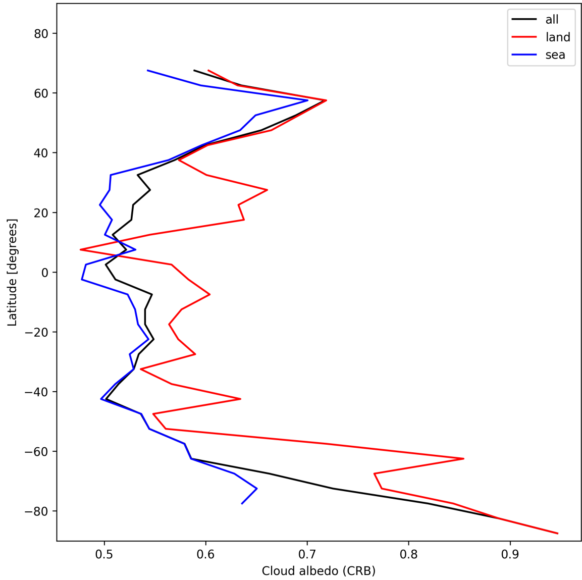
Figure 26: Zonal average of “Cloud albedo (CRB)” for 2024-12-16 to 2024-12-17.
