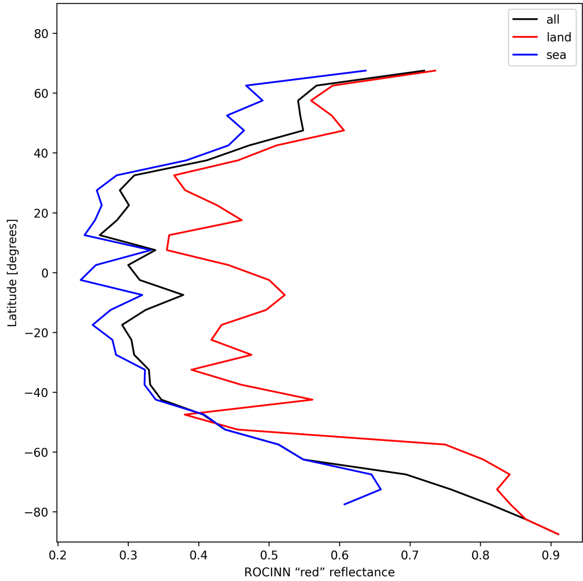
Figure 35: Zonal average of “ROCINN “red” reflectance” for 2024-12-16 to 2024-12-17.
