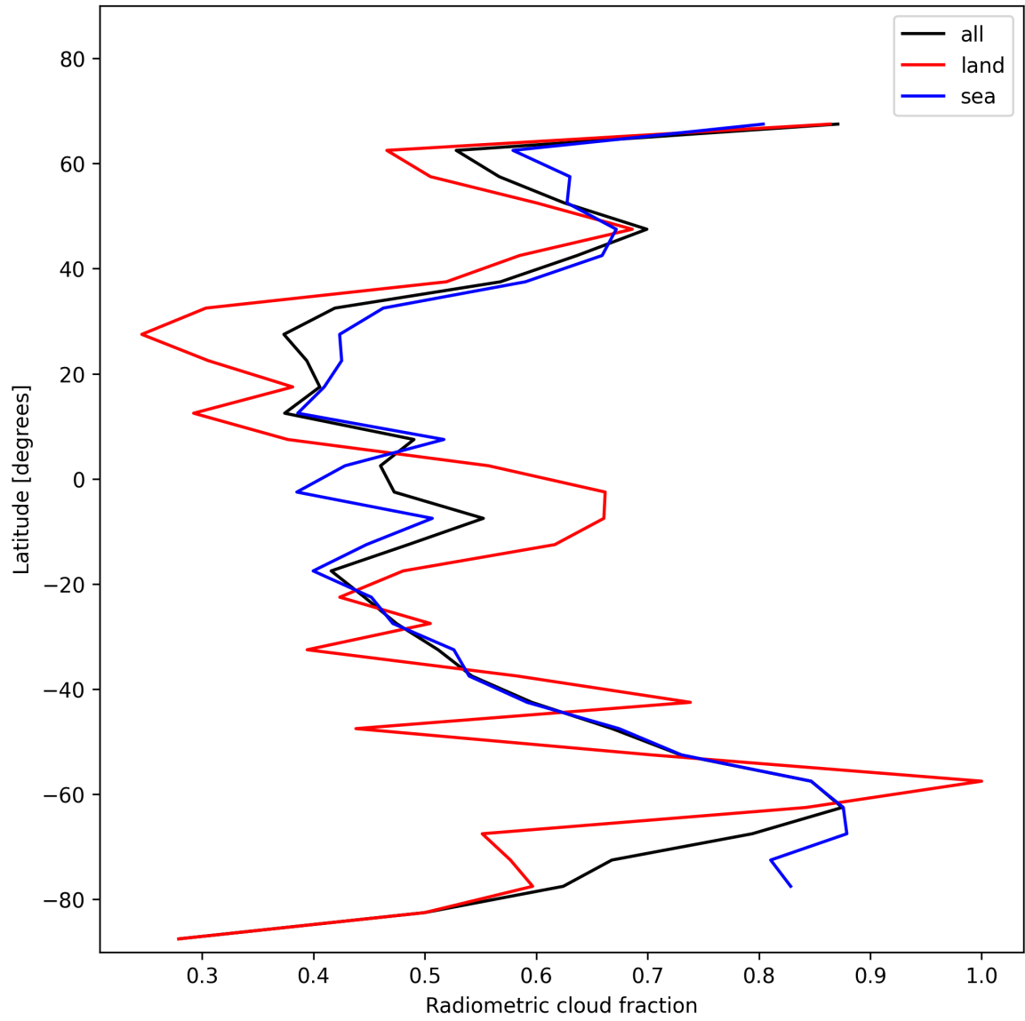
Figure 21: Zonal average of “Radiometric cloud fraction” for 2024-12-16 to 2024-12-17.
