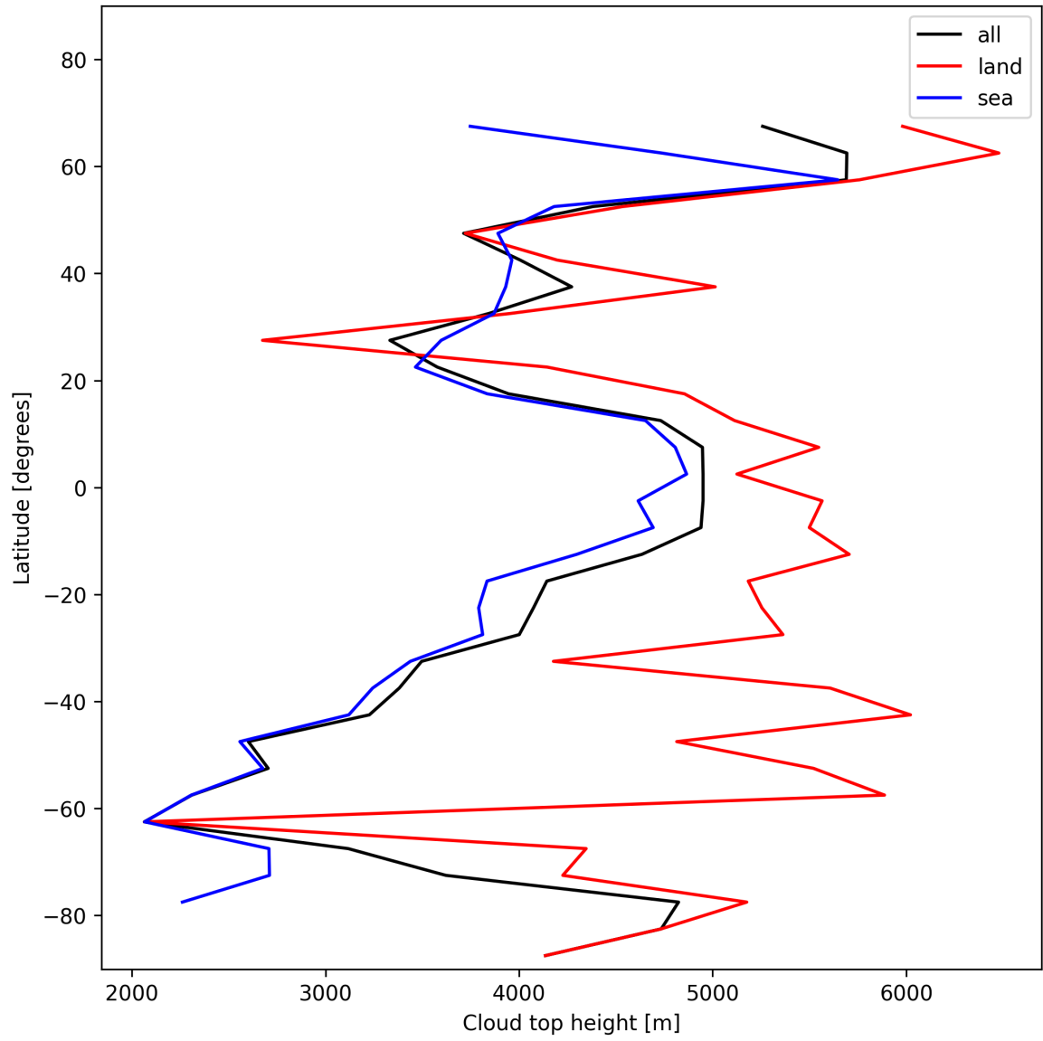
Figure 22: Zonal average of “Cloud top height” for 2024-12-16 to 2024-12-17.
