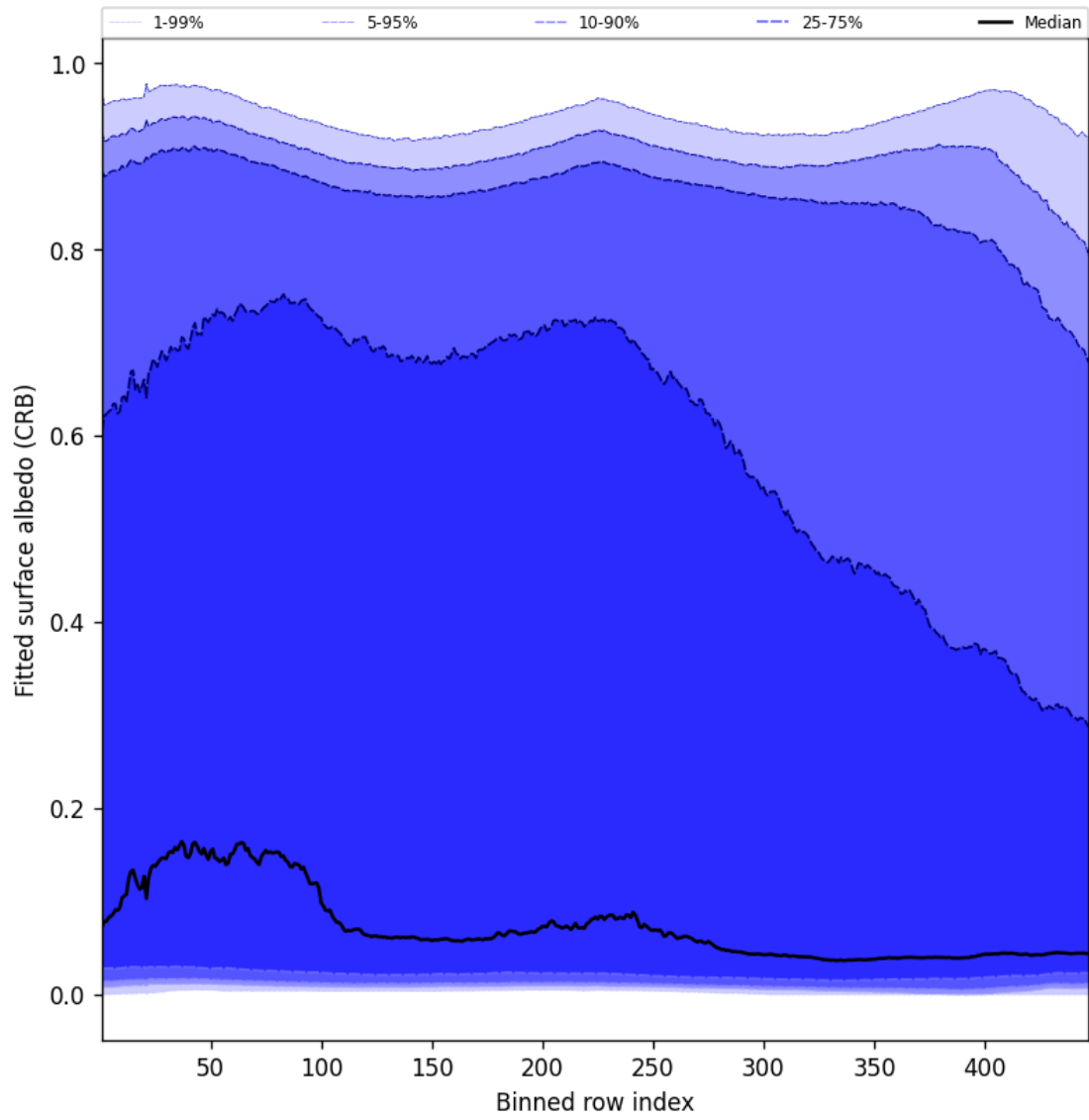
Figure 60: Along track statistics of “Fitted surface albedo (CRB)” for 2024-12-16 to 2024-12-17
