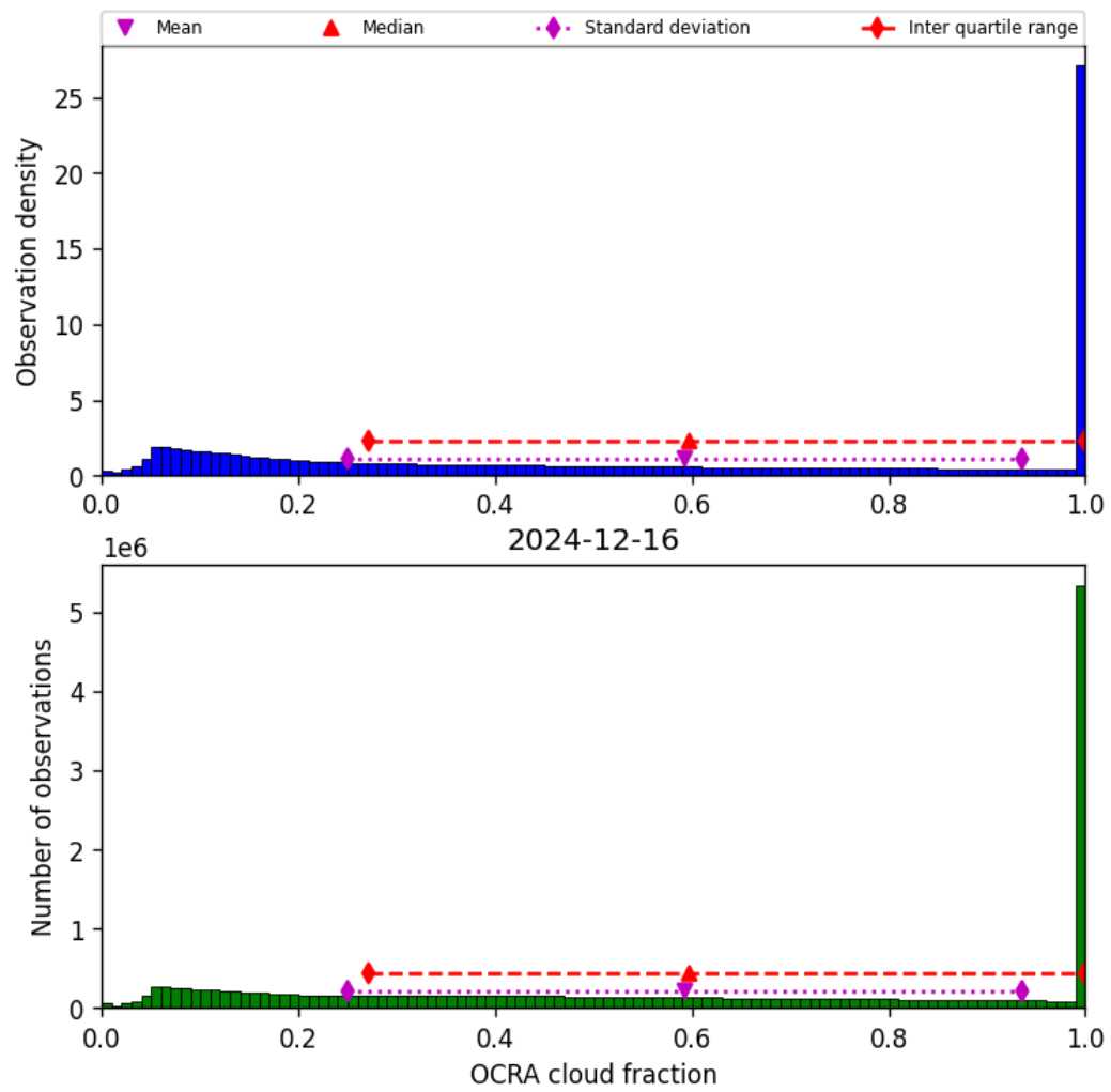
Figure 48: Histogram of “OCRA cloud fraction” for 2024-12-16 to 2024-12-17
