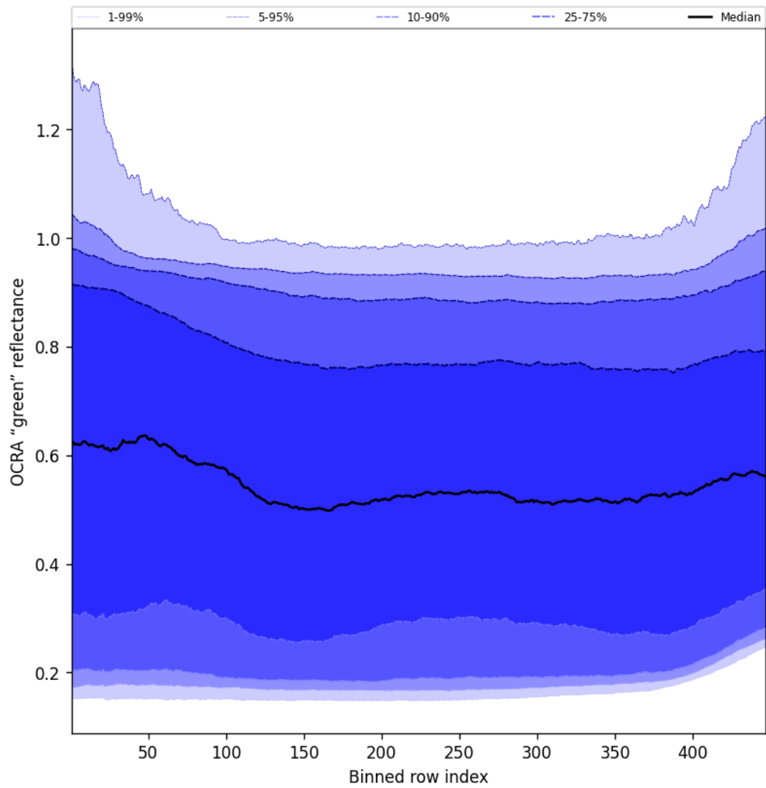
Figure 66: Along track statistics of "OCRA "green" reflectance" for 2024-12-18 to 2024-12-19
