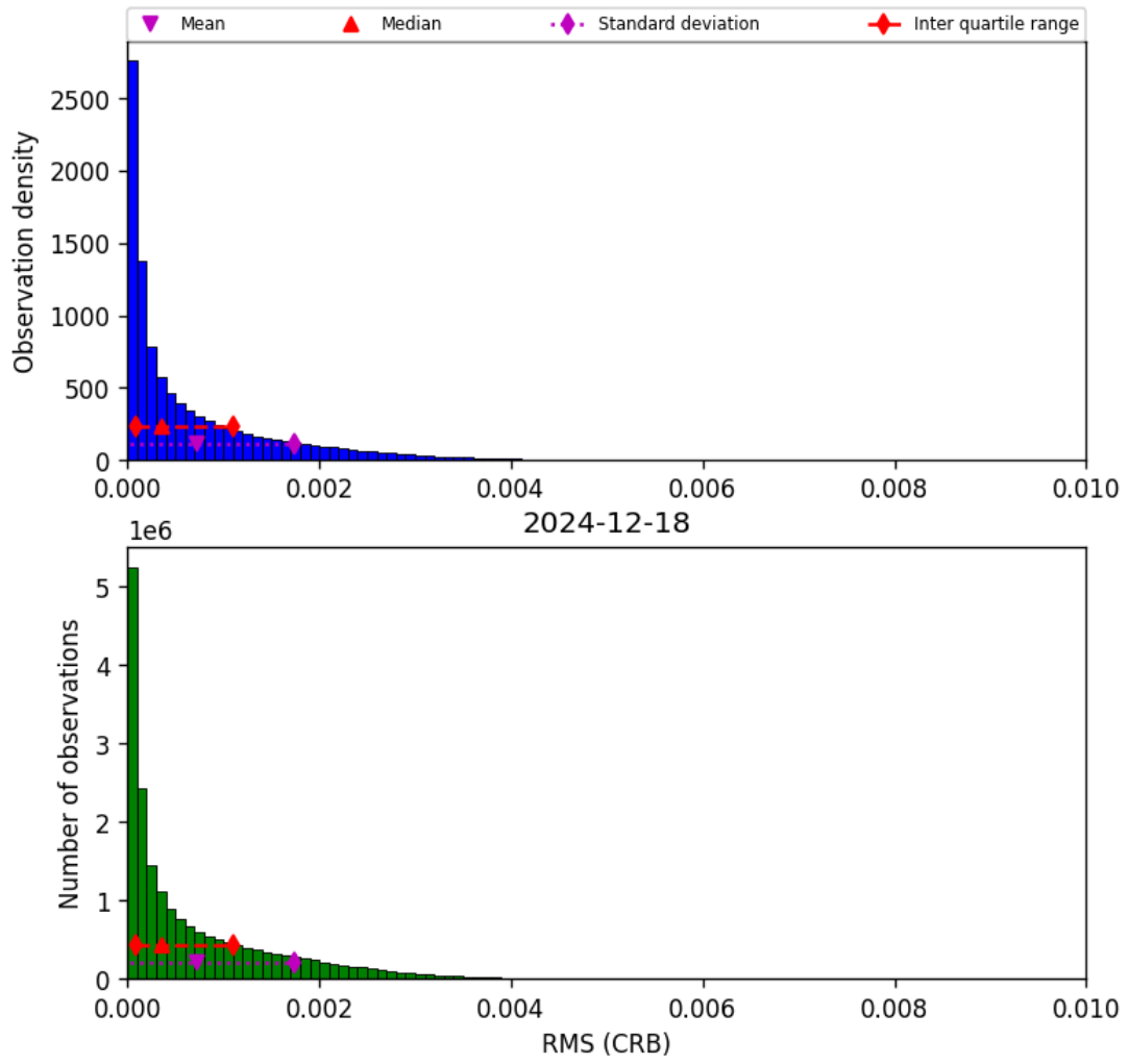
Figure 46: Histogram of “RMS (CRB)” for 2024-12-18 to 2024-12-19
