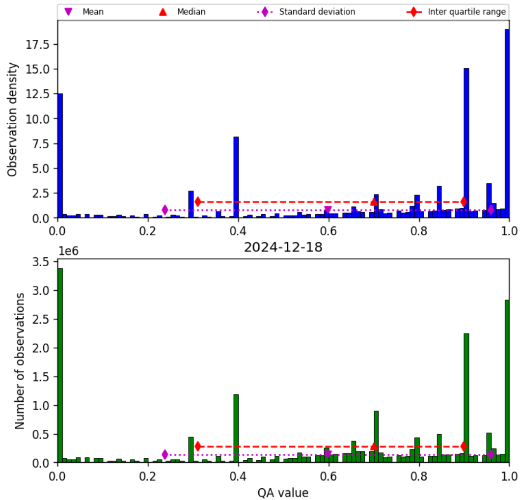
Figure 36: Histogram of “QA value” for 2024-12-18 to 2024-12-19
