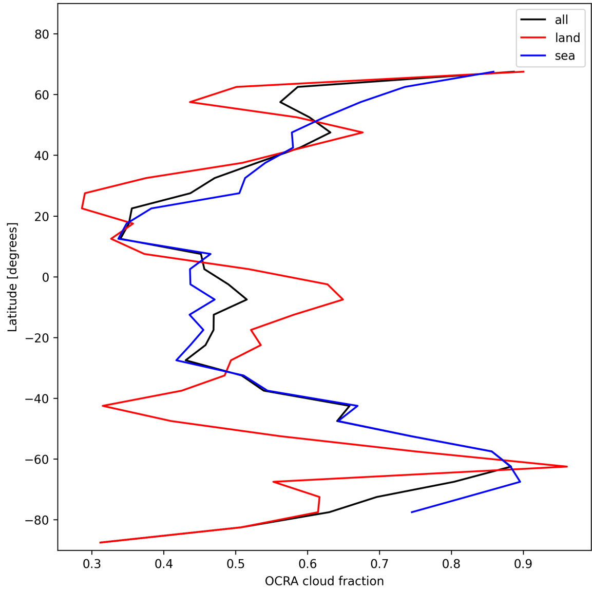
Figure 32: Zonal average of “OCRA cloud fraction” for 2024-12-18 to 2024-12-19.
