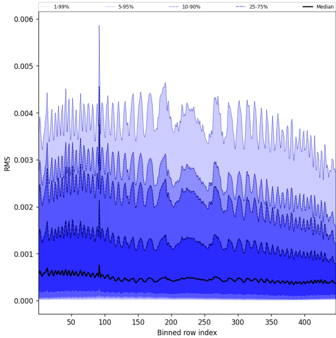
Figure 61: Along track statistics of “RMS” for 2024-12-18 to 2024-12-19
