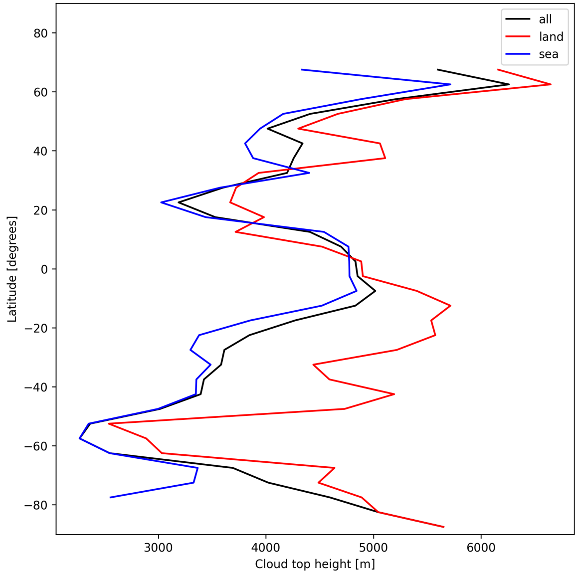
Figure 22: Zonal average of “Cloud top height” for 2024-12-18 to 2024-12-19.
