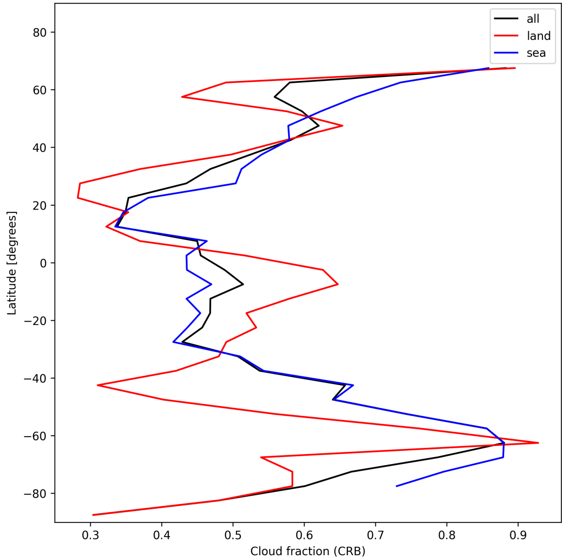
Figure 24: Zonal average of “Cloud fraction (CRB)” for 2024-12-18 to 2024-12-19.
