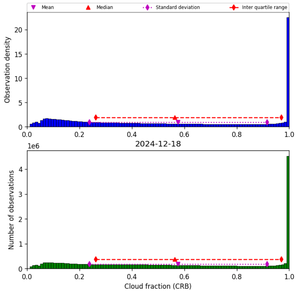
Figure 40: Histogram of “Cloud fraction (CRB)” for 2024-12-18 to 2024-12-19
