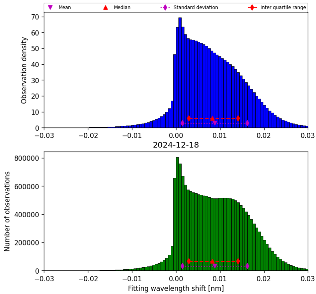
Figure 47: Histogram of “Fitting wavelength shift” for 2024-12-18 to 2024-12-19
