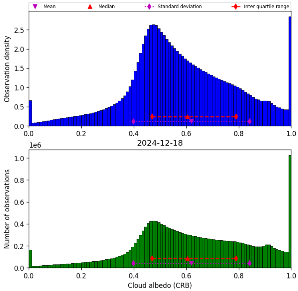
Figure 42: Histogram of “Cloud albedo (CRB)” for 2024-12-18 to 2024-12-19
