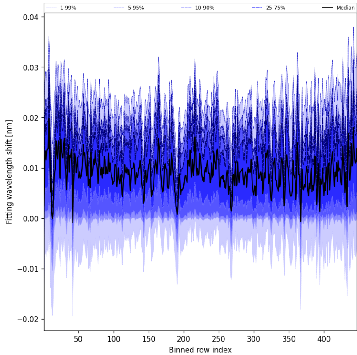
Figure 63: Along track statistics of “Fitting wavelength shift” for 2024-12-18 to 2024-12-19
