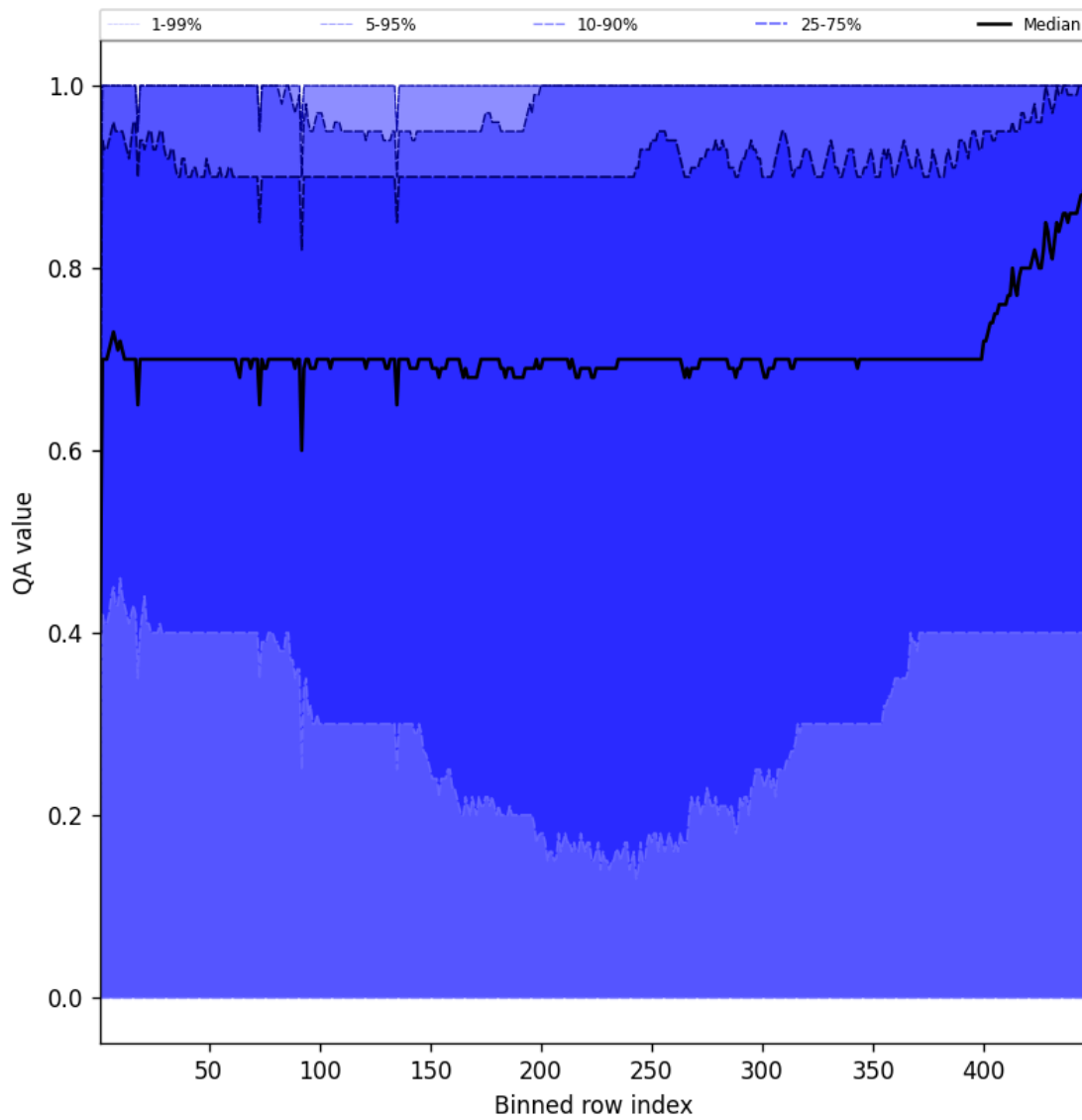
Figure 52: Along track statistics of “QA value” for 2024-12-18 to 2024-12-19
