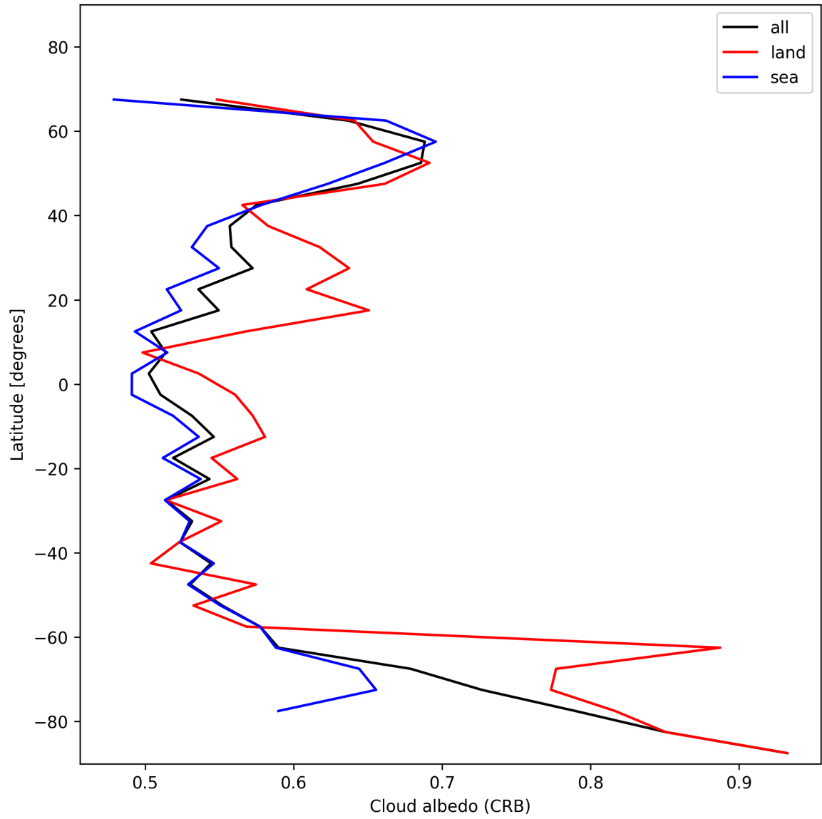
Figure 26: Zonal average of “Cloud albedo (CRB)” for 2024-12-18 to 2024-12-19.
