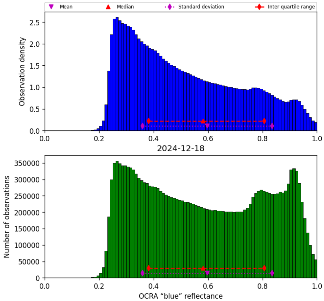
Figure 49: Histogram of "OCRA "blue" reflectance" for 2024-12-18 to 2024-12-19
