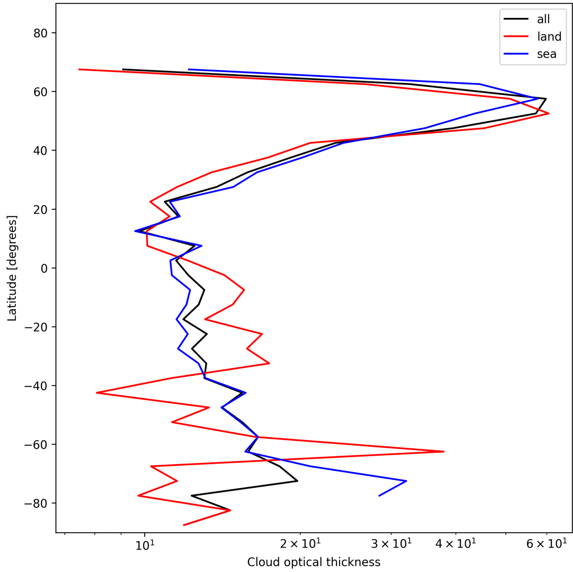
Figure 23: Zonal average of “Cloud optical thickness” for 2024-12-18 to 2024-12-19.
