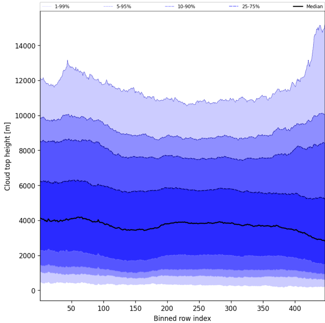
Figure 54: Along track statistics of “Cloud top height” for 2024-12-18 to 2024-12-19
