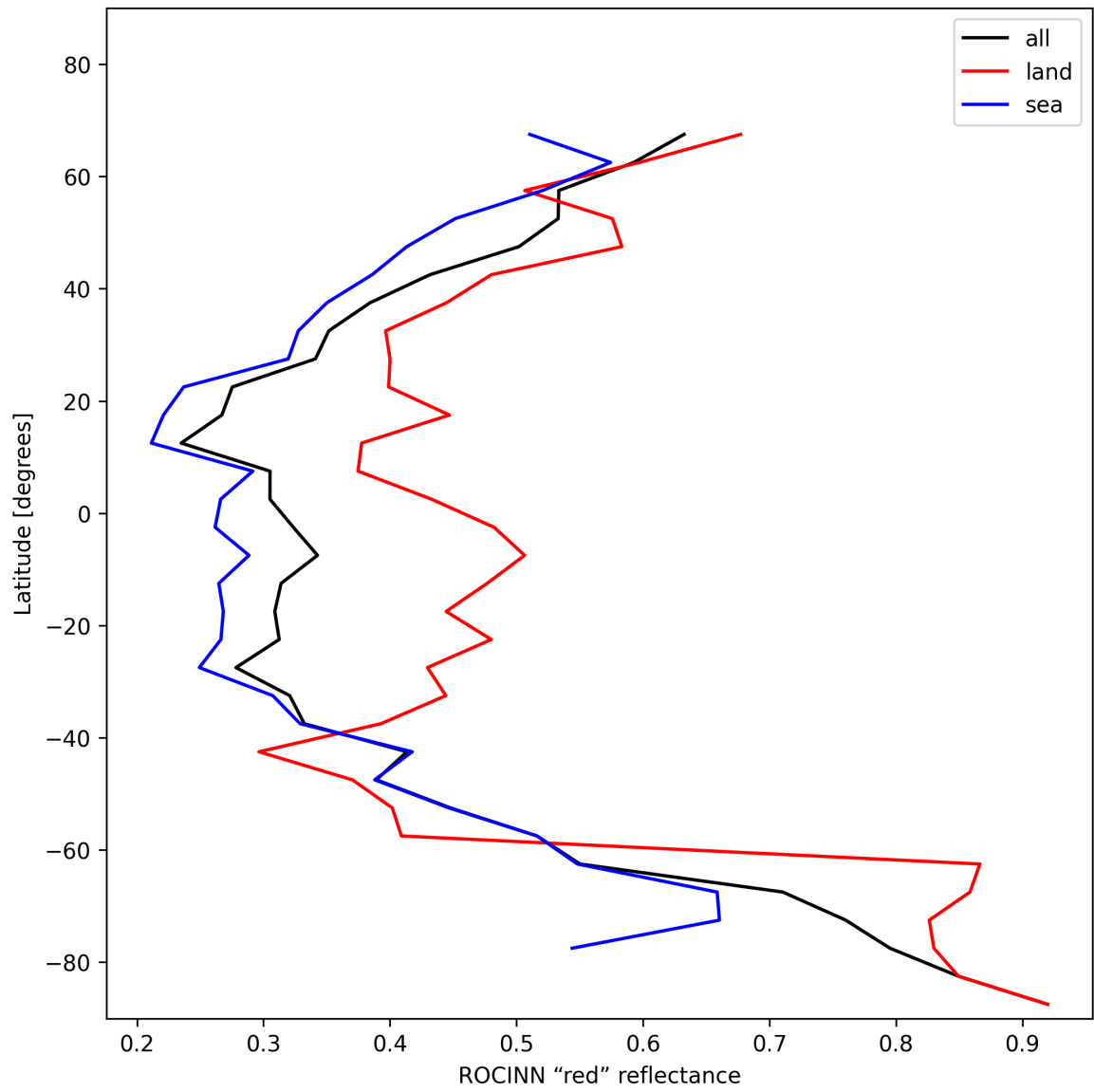
Figure 35: Zonal average of “ROCINN “red” reflectance” for 2024-12-18 to 2024-12-19.
