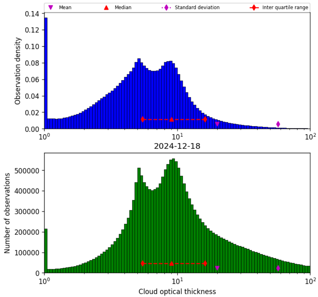
Figure 39: Histogram of “Cloud optical thickness” for 2024-12-18 to 2024-12-19
