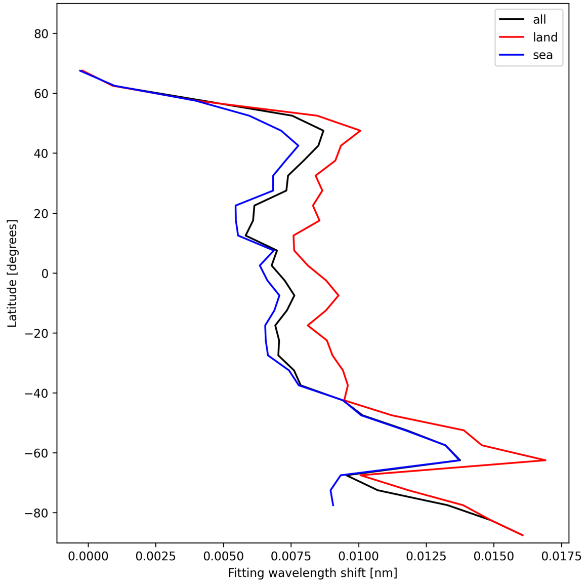
Figure 31: Zonal average of “Fitting wavelength shift” for 2024-12-18 to 2024-12-19.
