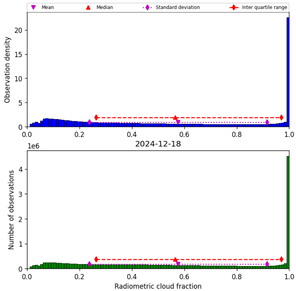
Figure 37: Histogram of “Radiometric cloud fraction” for 2024-12-18 to 2024-12-19
