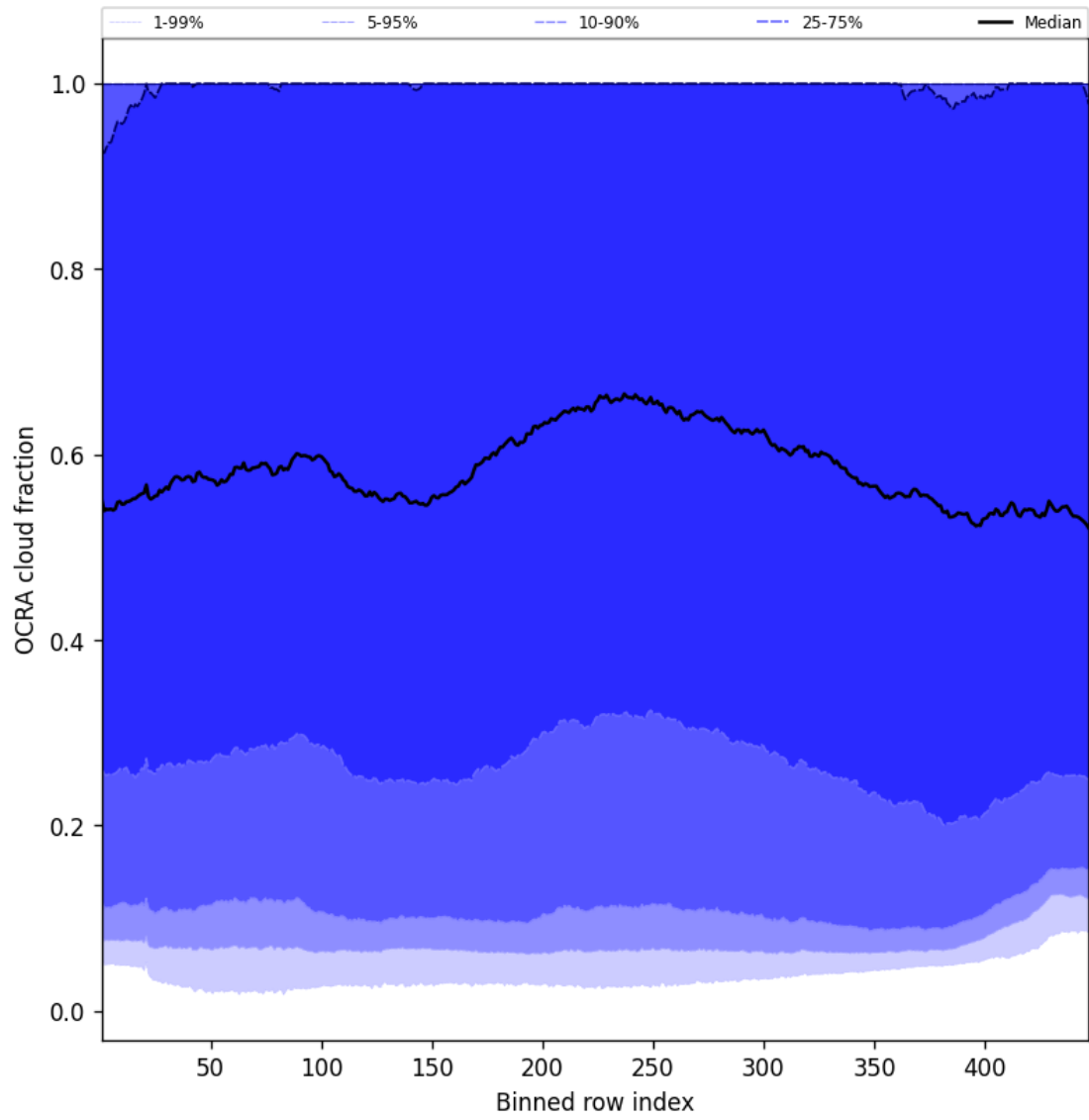
Figure 64: Along track statistics of “OCRA cloud fraction” for 2024-12-18 to 2024-12-19
