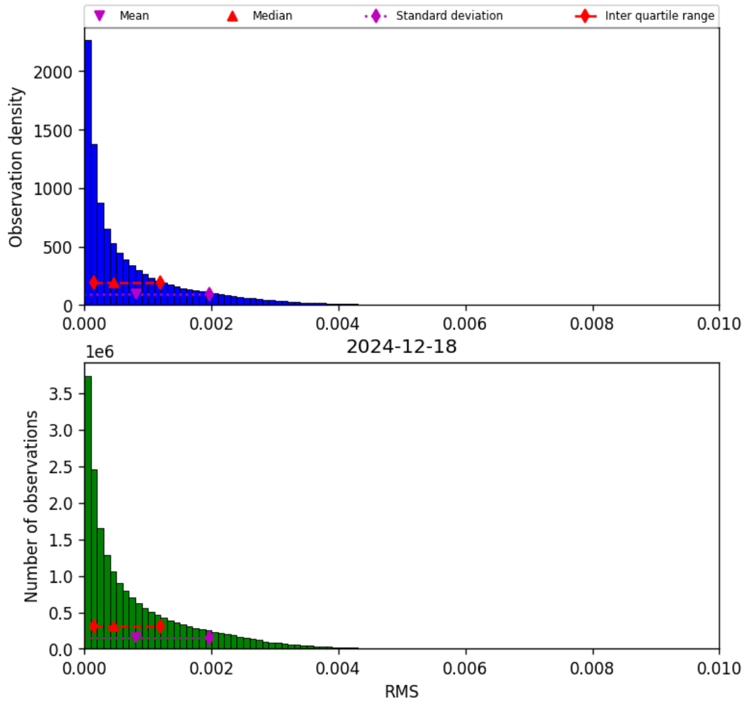
Figure 45: Histogram of “RMS” for 2024-12-18 to 2024-12-19
