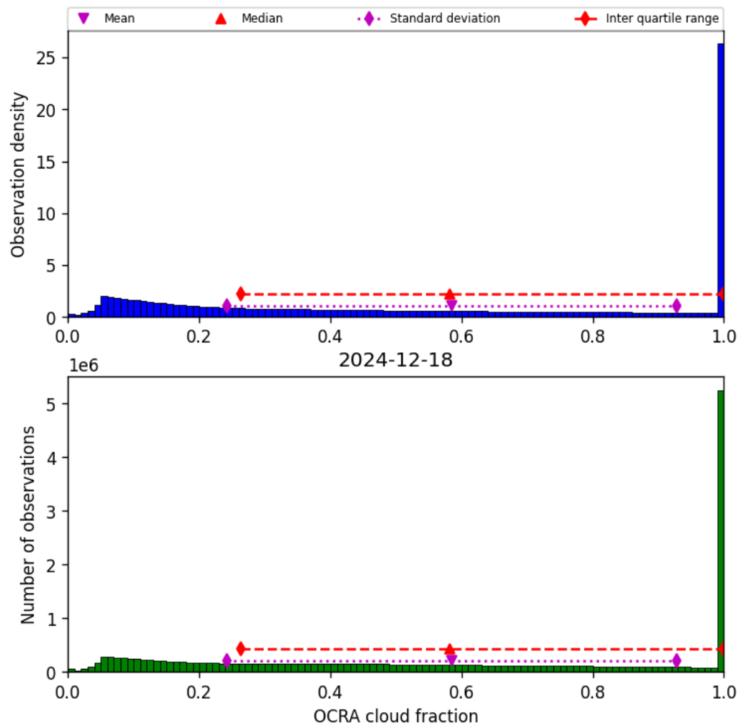
Figure 48: Histogram of “OCRA cloud fraction” for 2024-12-18 to 2024-12-19
