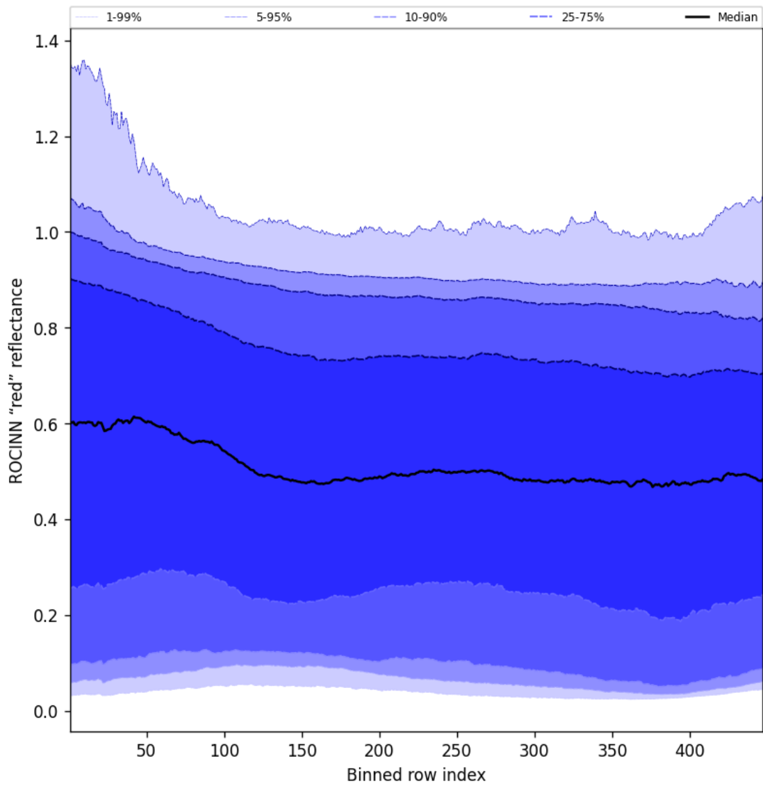
Figure 67: Along track statistics of "ROCINN "red" reflectance" for 2024-12-18 to 2024-12-19
