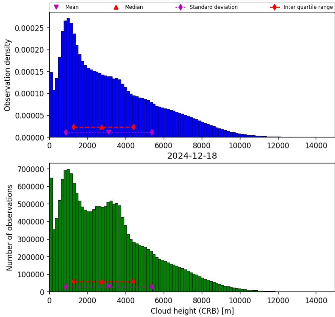
Figure 41: Histogram of “Cloud height (CRB)” for 2024-12-18 to 2024-12-19
