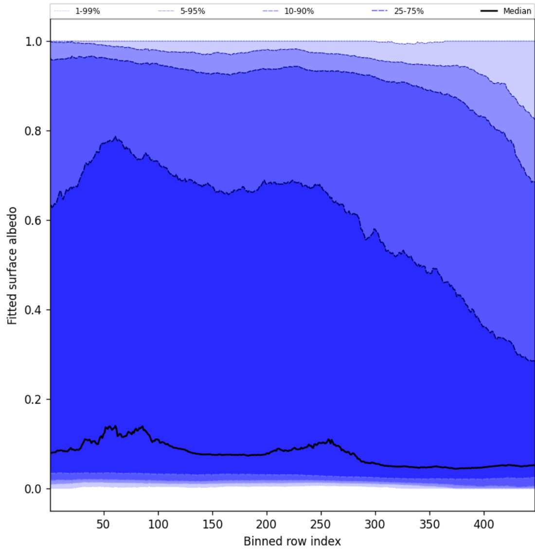
Figure 59: Along track statistics of “Fitted surface albedo” for 2024-12-18 to 2024-12-19
