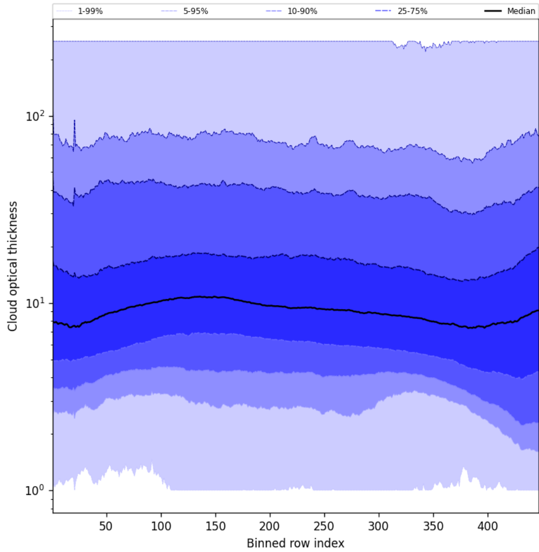
Figure 55: Along track statistics of “Cloud optical thickness” for 2024-12-18 to 2024-12-19
