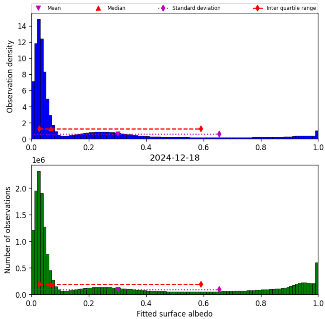
Figure 43: Histogram of “Fitted surface albedo” for 2024-12-18 to 2024-12-19
