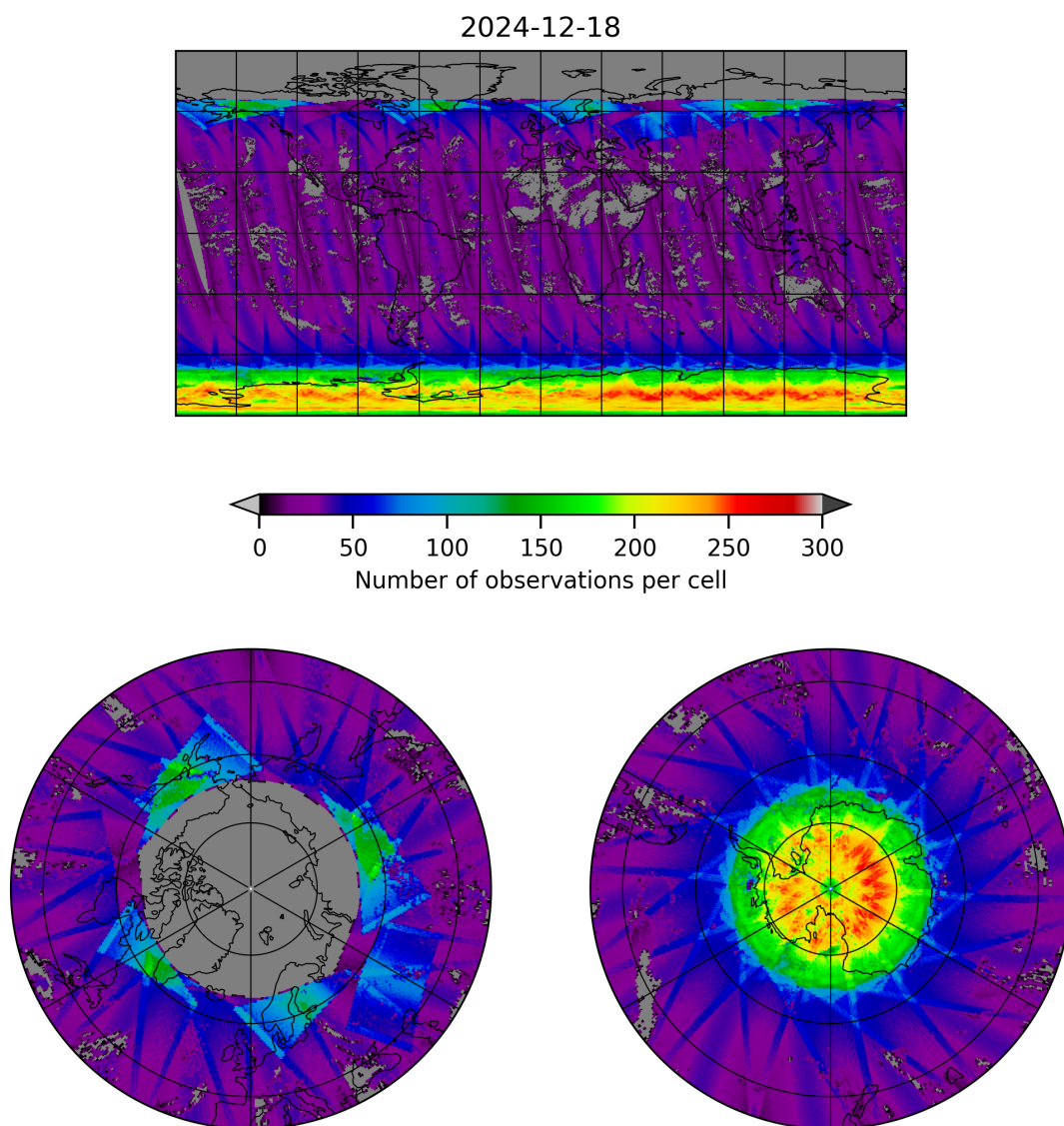
Figure 19: Map of the number of observations for 2024-12-18 to 2024-12-19
