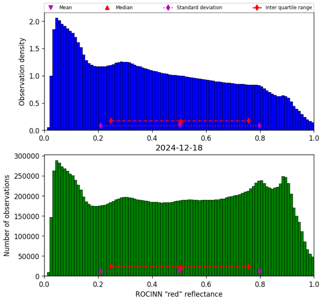
Figure 51: Histogram of “ROCINN “red” reflectance” for 2024-12-18 to 2024-12-19
