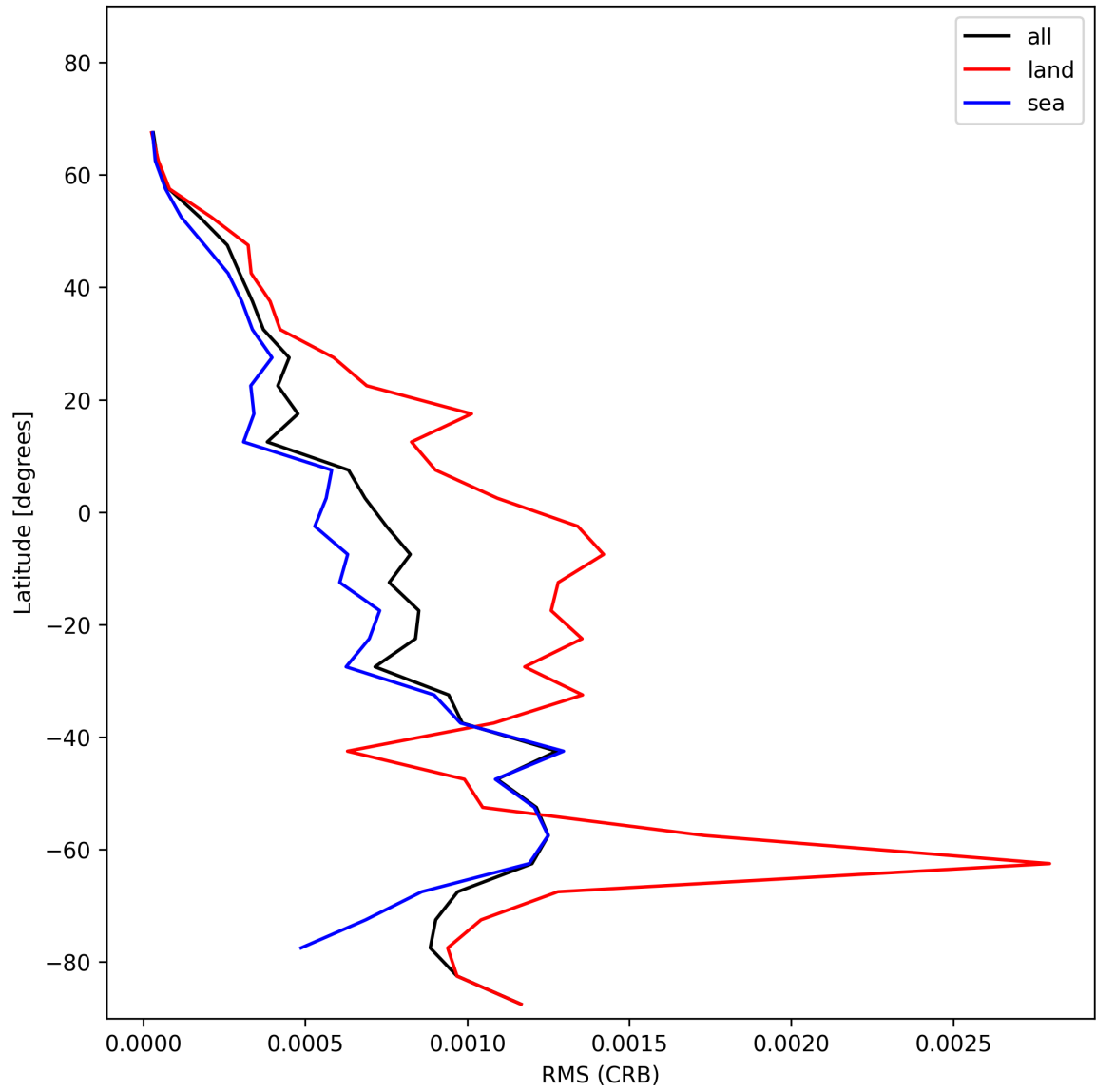
Figure 30: Zonal average of “RMS (CRB)” for 2024-12-18 to 2024-12-19.
