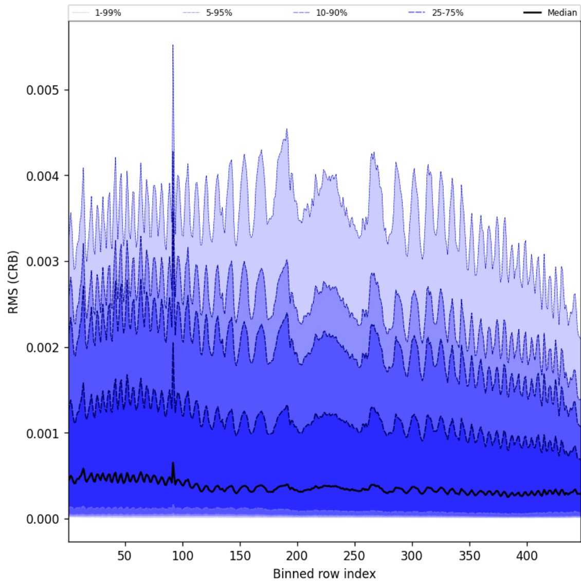
Figure 62: Along track statistics of “RMS (CRB)” for 2024-12-18 to 2024-12-19
