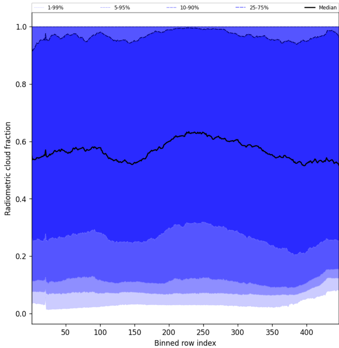
Figure 53: Along track statistics of “Radiometric cloud fraction” for 2024-12-18 to 2024-12-19
