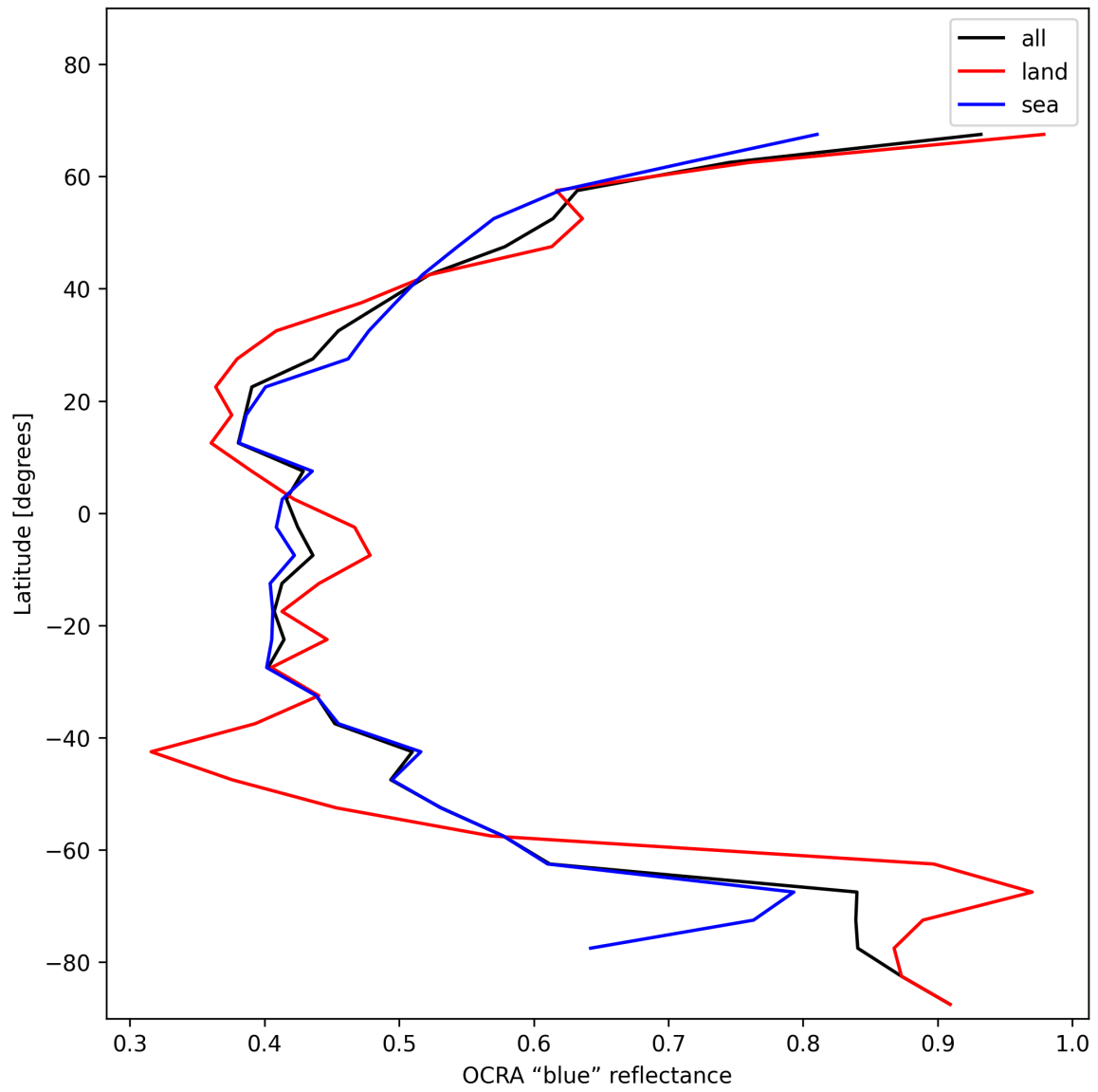
Figure 33: Zonal average of “OCRA “blue” reflectance” for 2024-12-18 to 2024-12-19.
