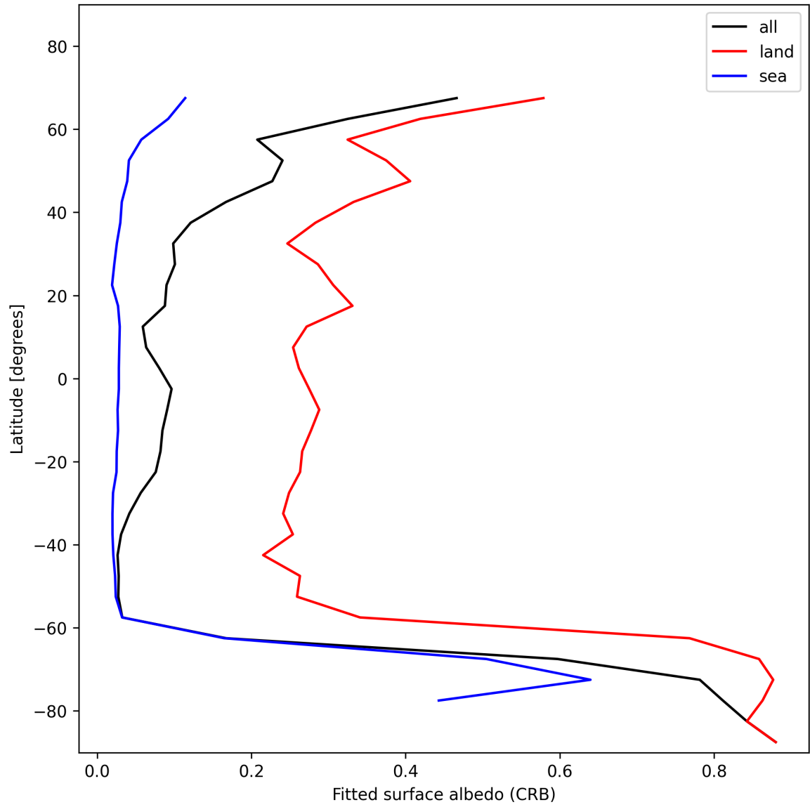
Figure 28: Zonal average of “Fitted surface albedo (CRB)” for 2024-12-18 to 2024-12-19.
