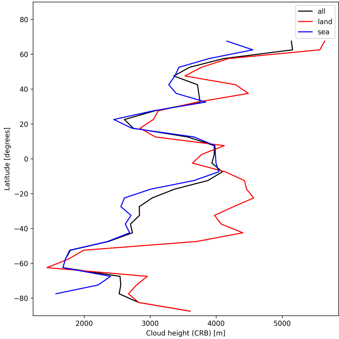
Figure 25: Zonal average of “Cloud height (CRB)” for 2024-12-18 to 2024-12-19.
