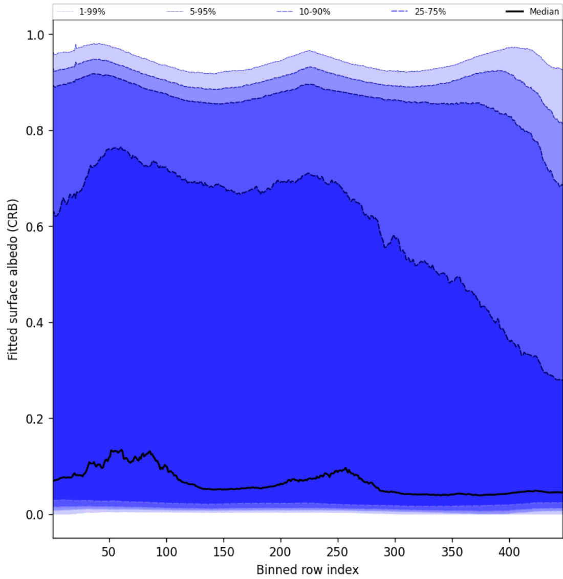
Figure 60: Along track statistics of “Fitted surface albedo (CRB)” for 2024-12-18 to 2024-12-19
