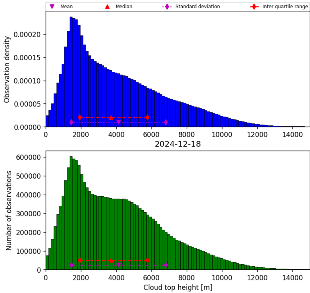
Figure 38: Histogram of “Cloud top height” for 2024-12-18 to 2024-12-19
