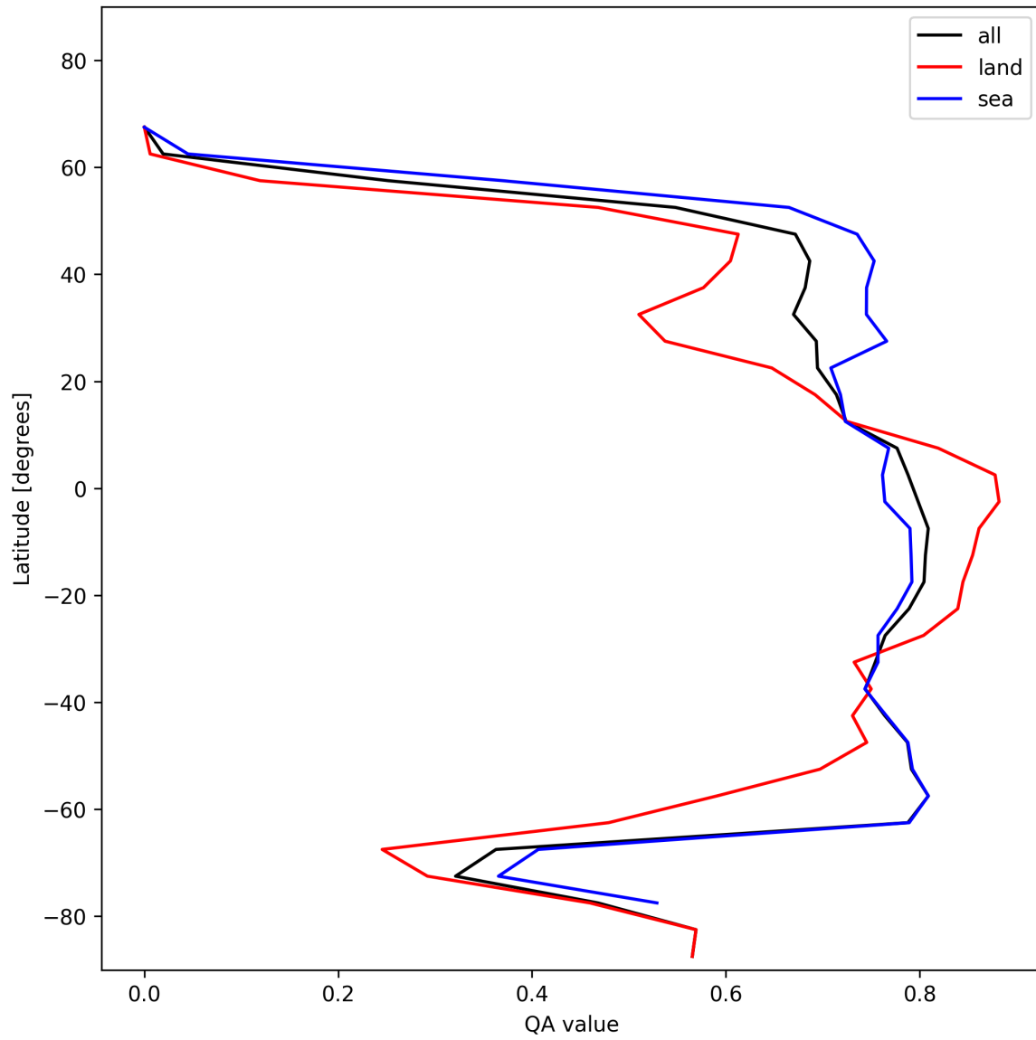
Figure 20: Zonal average of “QA value” for 2024-12-18 to 2024-12-19.
