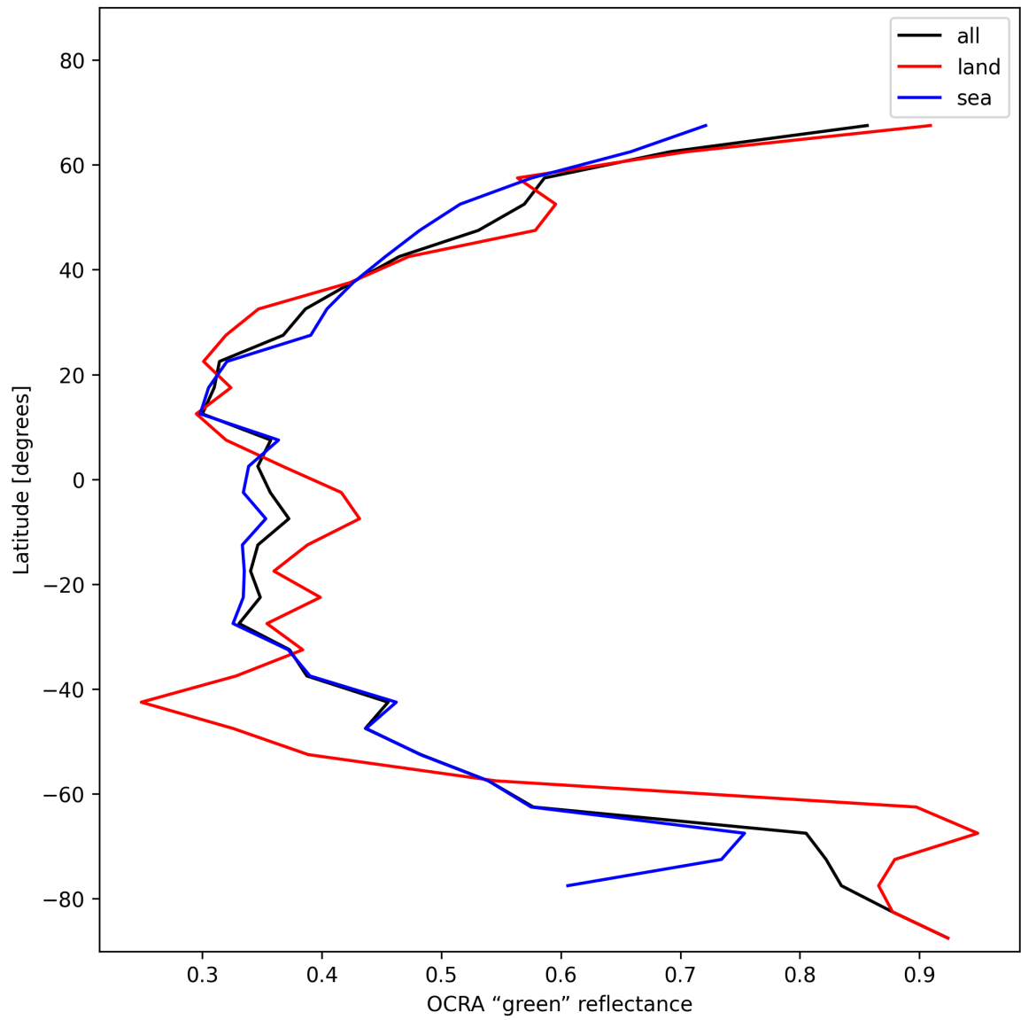
Figure 34: Zonal average of “OCRA “green” reflectance” for 2024-12-18 to 2024-12-19.
