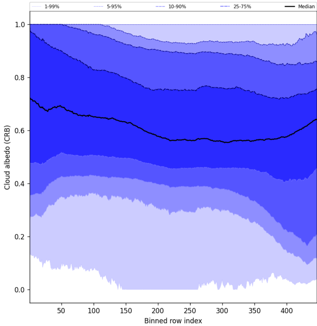
Figure 58: Along track statistics of “Cloud albedo (CRB)” for 2024-12-18 to 2024-12-19
