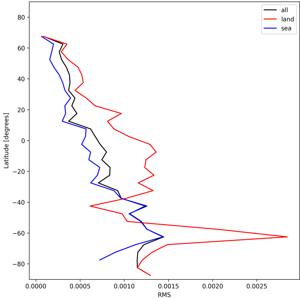
Figure 29: Zonal average of “RMS” for 2024-12-18 to 2024-12-19.
