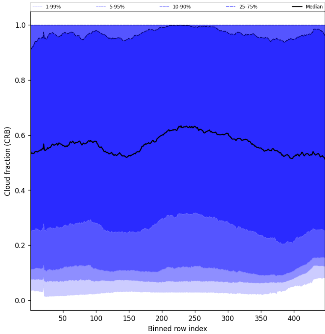
Figure 56: Along track statistics of “Cloud fraction (CRB)” for 2024-12-18 to 2024-12-19
