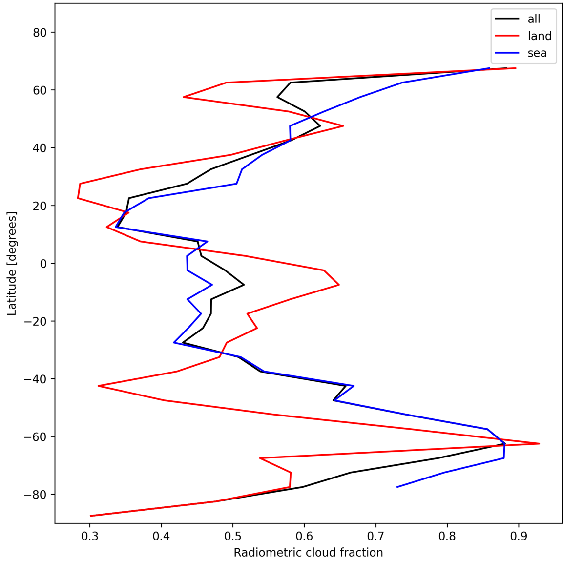
Figure 21: Zonal average of “Radiometric cloud fraction” for 2024-12-18 to 2024-12-19.
