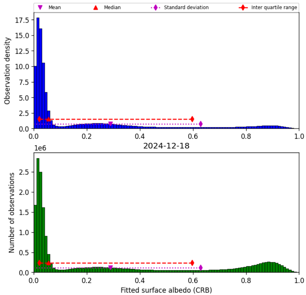
Figure 44: Histogram of “Fitted surface albedo (CRB)” for 2024-12-18 to 2024-12-19
