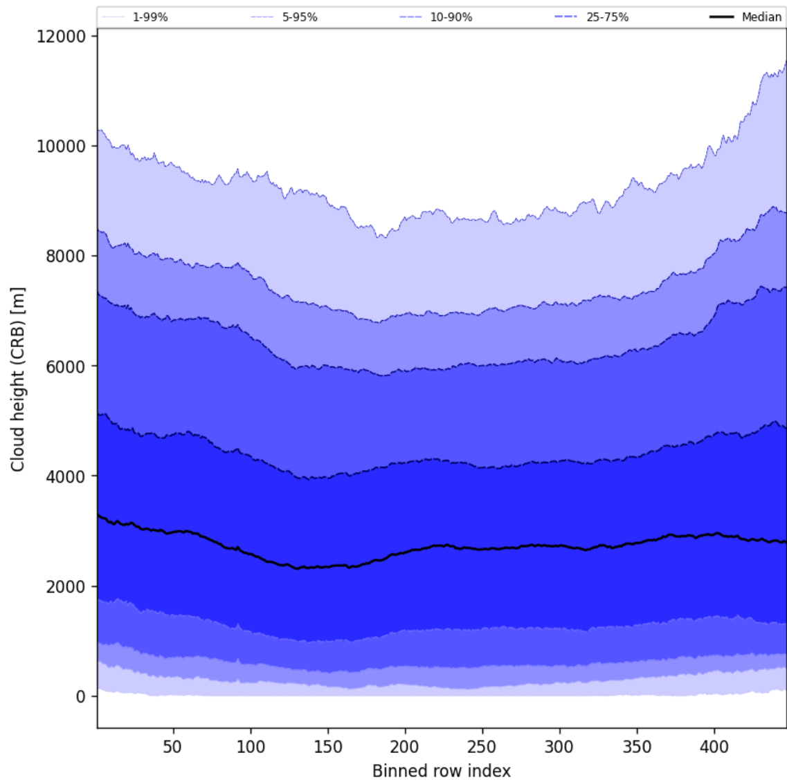
Figure 57: Along track statistics of “Cloud height (CRB)” for 2024-12-18 to 2024-12-19
