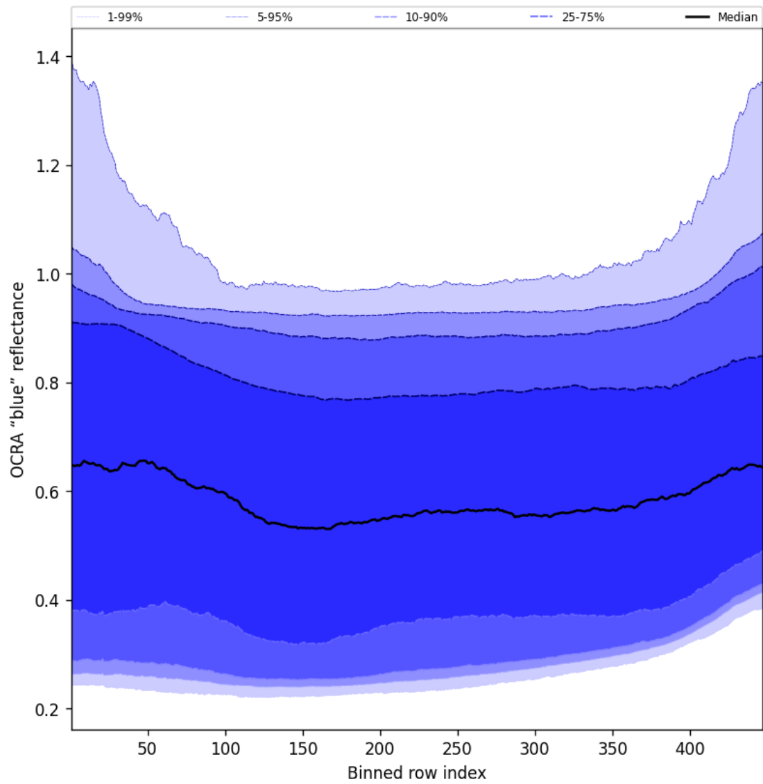
Figure 65: Along track statistics of “OCRA “blue” reflectance” for 2024-12-18 to 2024-12-19
