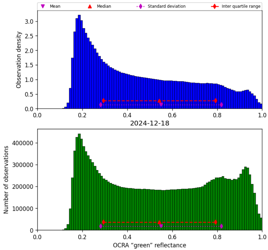
Figure 50: Histogram of “OCRA “green” reflectance” for 2024-12-18 to 2024-12-19
