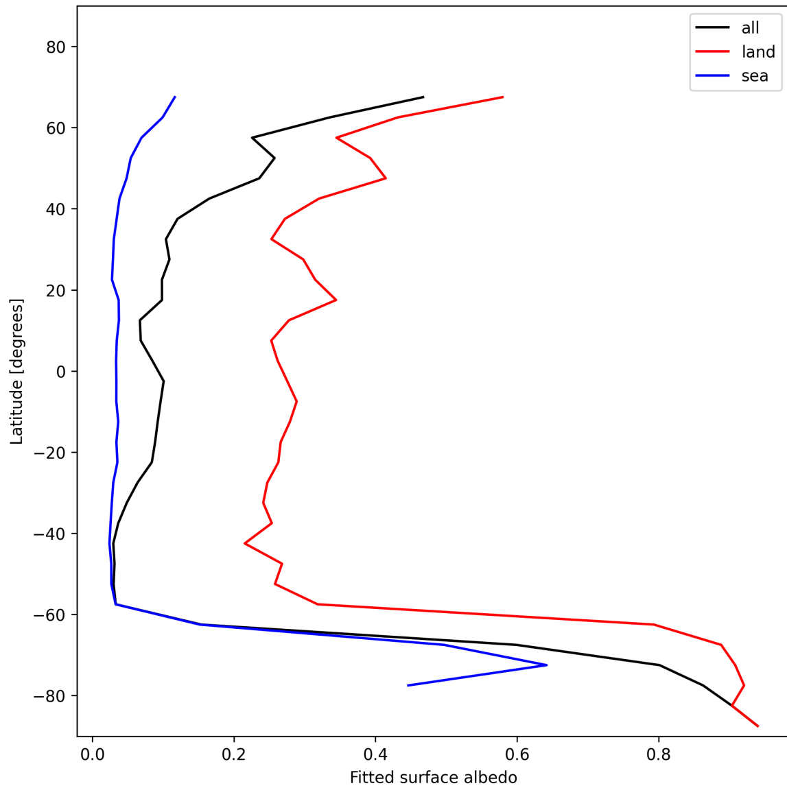
Figure 27: Zonal average of “Fitted surface albedo” for 2024-12-18 to 2024-12-19.
