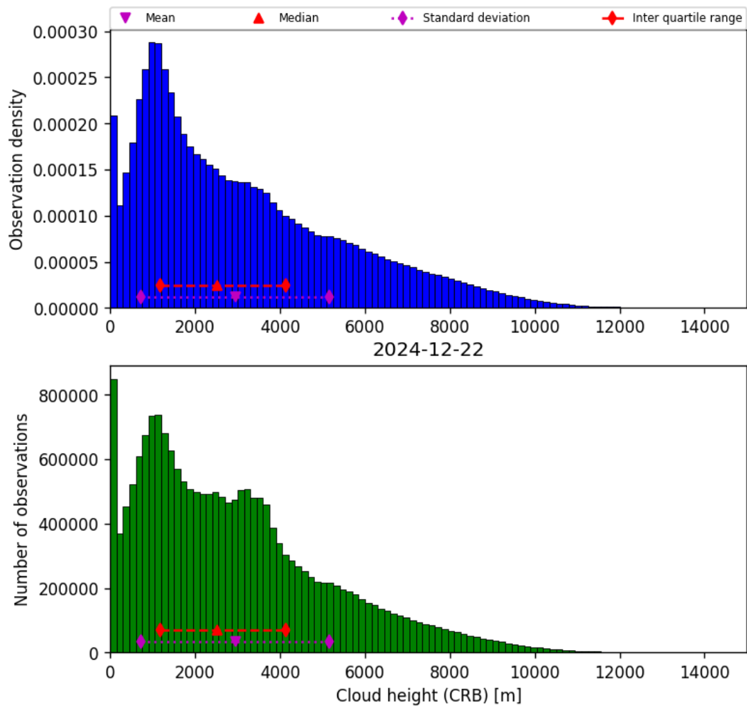
Figure 41: Histogram of “Cloud height (CRB)” for 2024-12-22 to 2024-12-23
