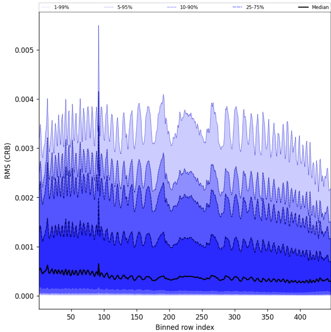
Figure 62: Along track statistics of “RMS (CRB)” for 2024-12-22 to 2024-12-23
