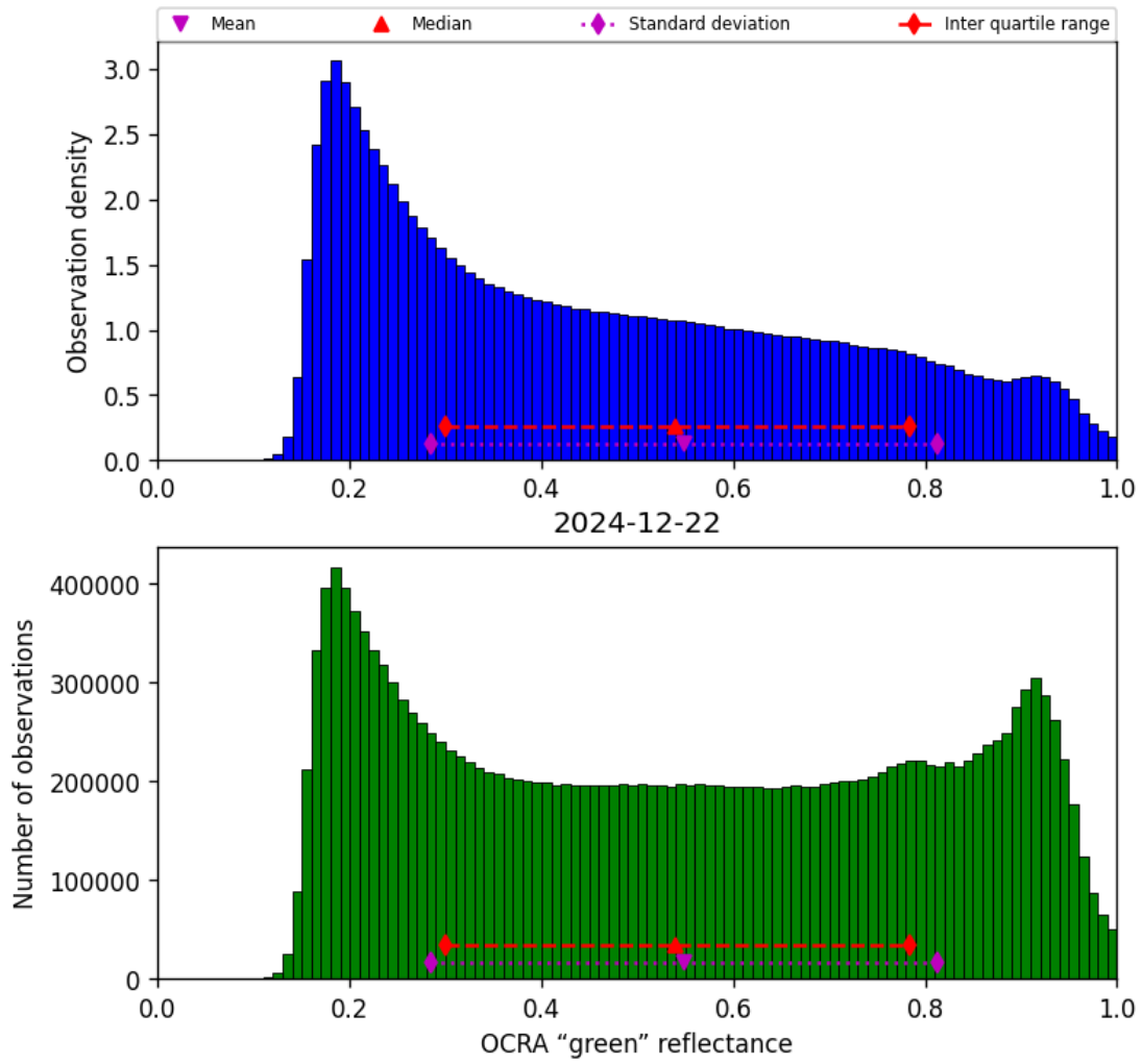
Figure 50: Histogram of “OCRA “green” reflectance” for 2024-12-22 to 2024-12-23
