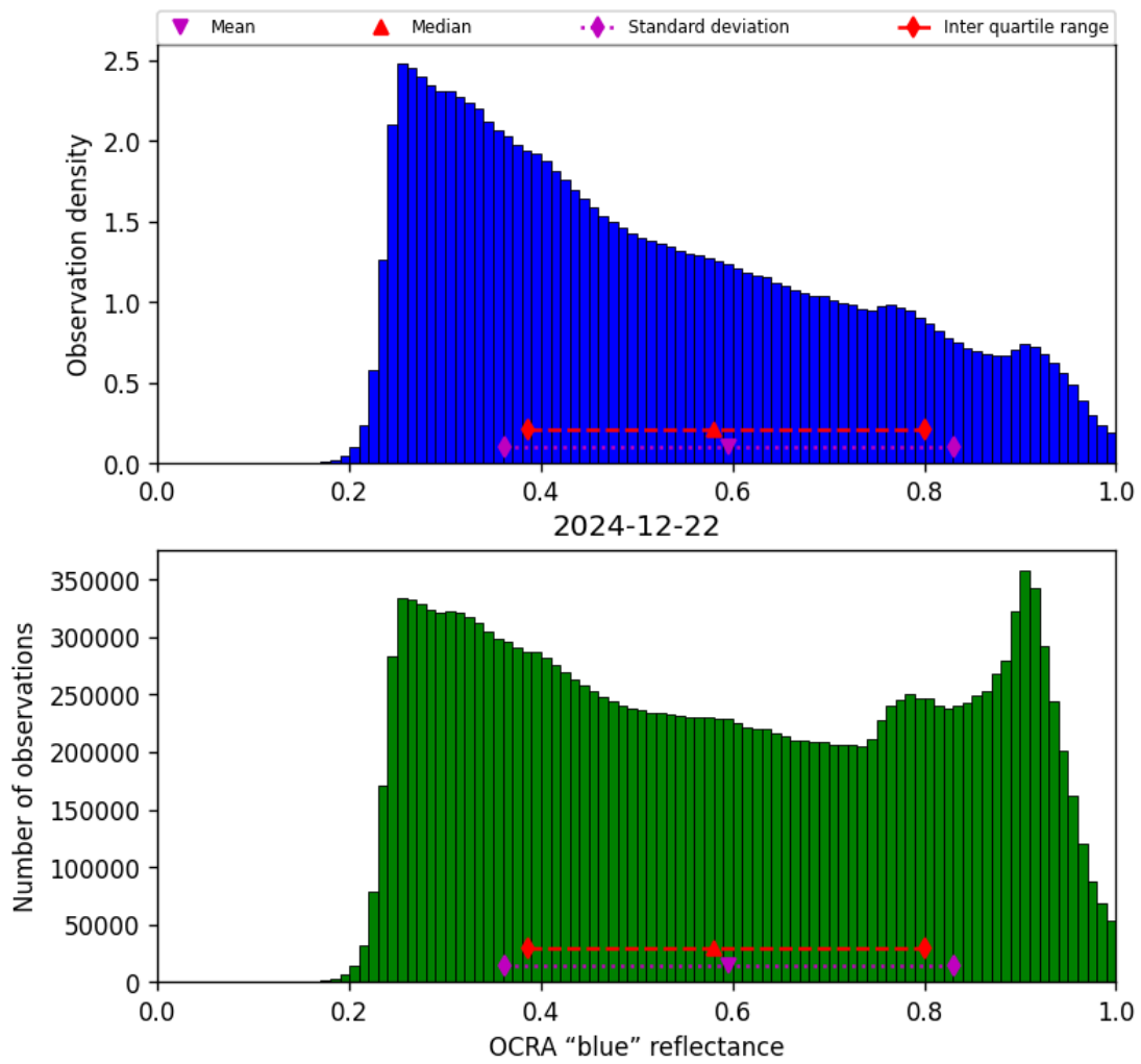
Figure 49: Histogram of “OCRA “blue” reflectance” for 2024-12-22 to 2024-12-23
