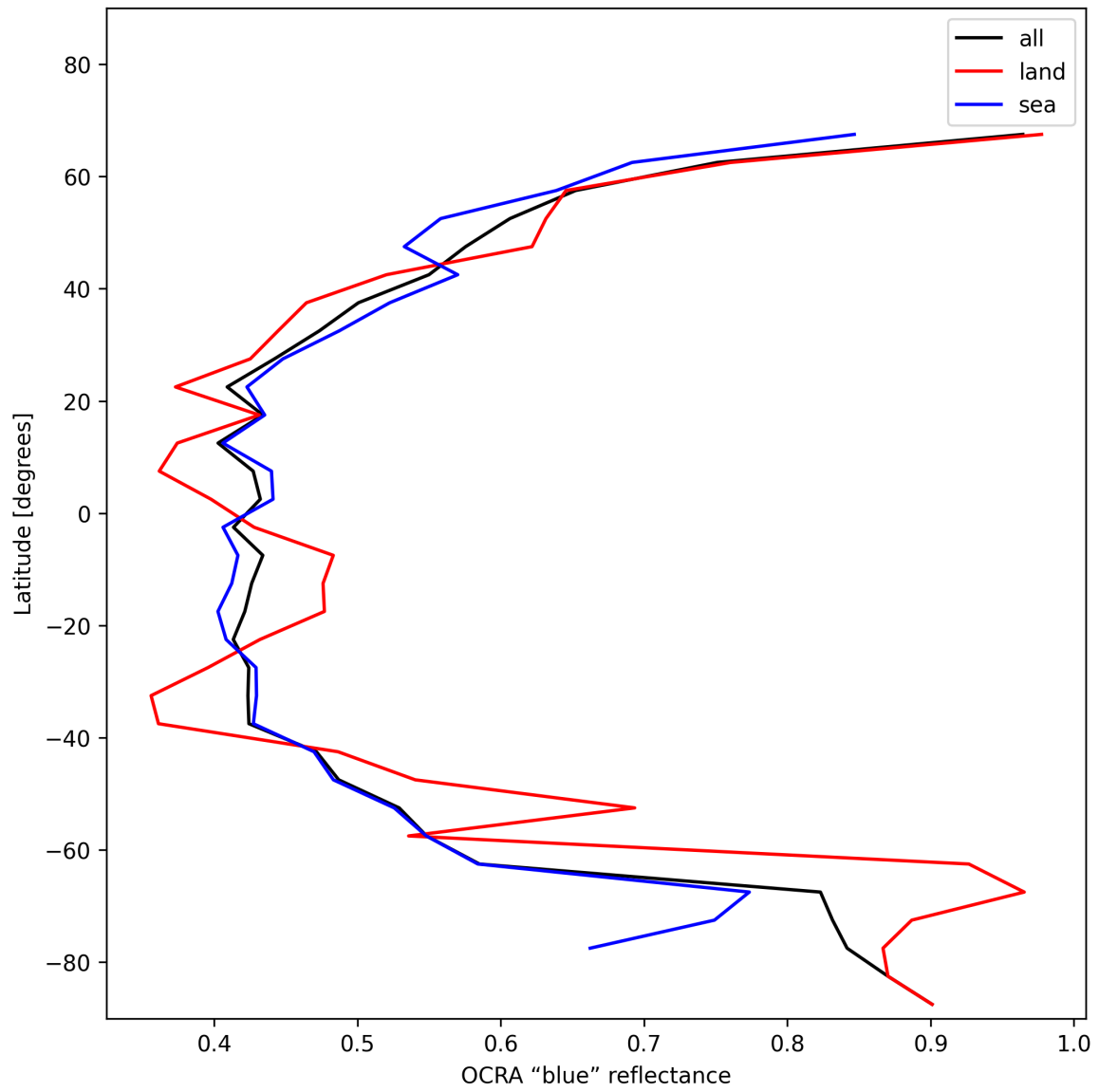
Figure 33: Zonal average of “OCRA “blue” reflectance” for 2024-12-22 to 2024-12-23.
