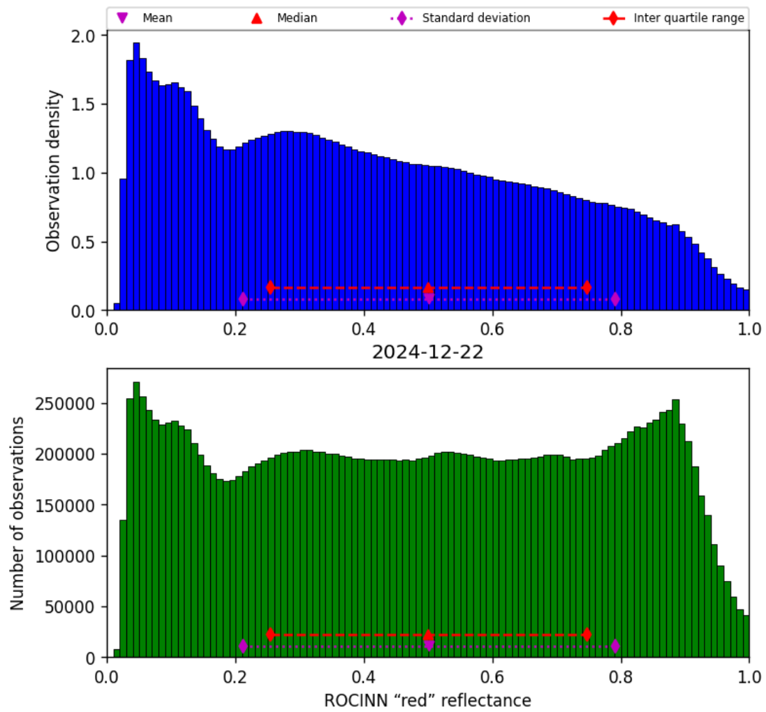
Figure 51: Histogram of “ROCINN “red” reflectance” for 2024-12-22 to 2024-12-23
