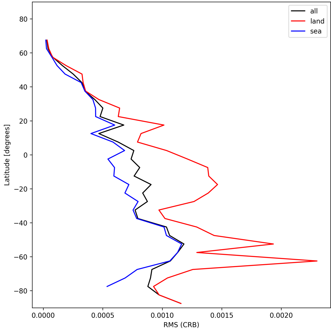
Figure 30: Zonal average of “RMS (CRB)” for 2024-12-22 to 2024-12-23.
