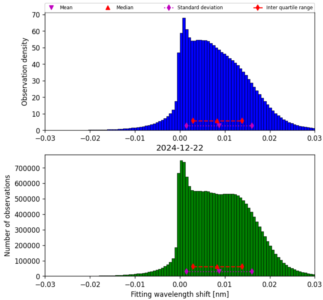
Figure 47: Histogram of “Fitting wavelength shift” for 2024-12-22 to 2024-12-23
