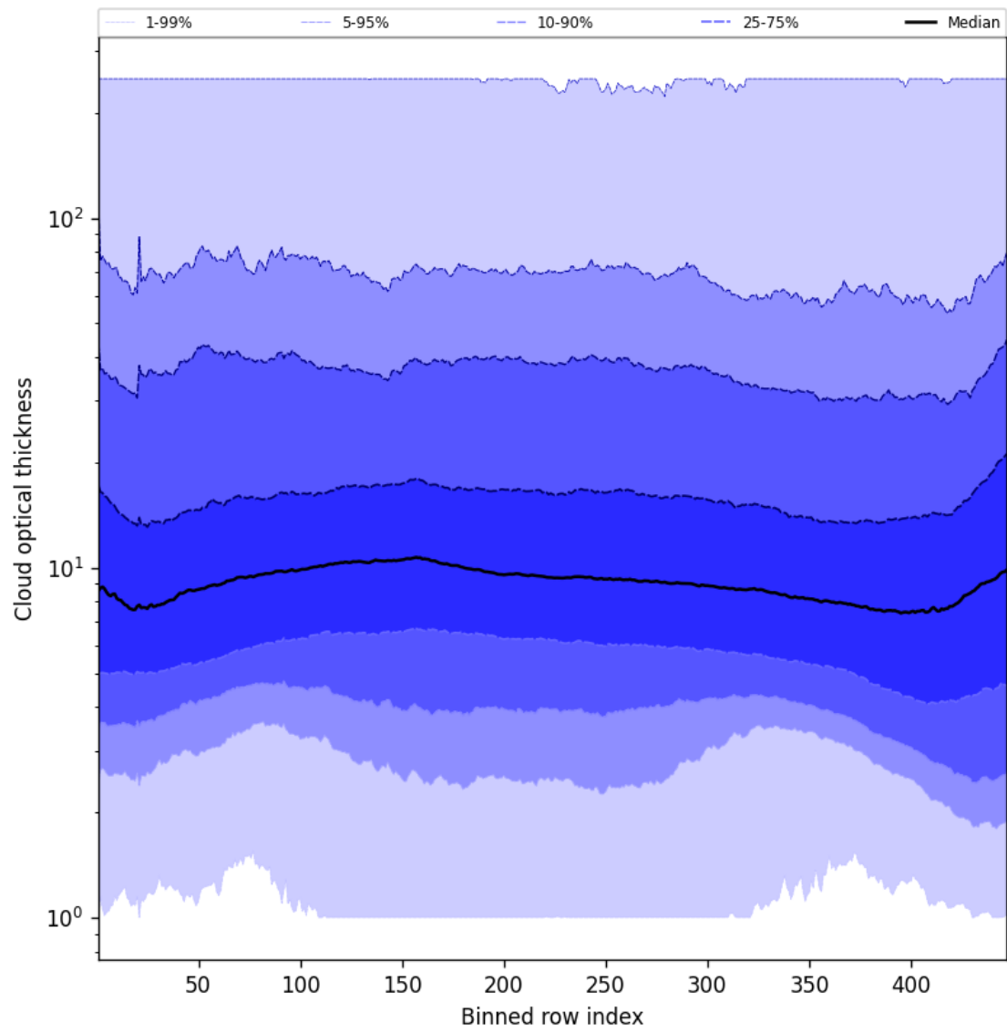
Figure 55: Along track statistics of “Cloud optical thickness” for 2024-12-22 to 2024-12-23
