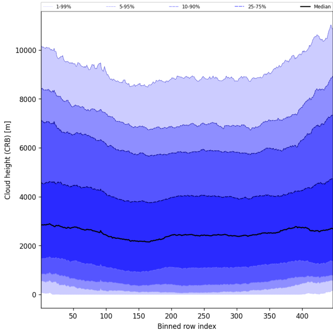
Figure 57: Along track statistics of “Cloud height (CRB)” for 2024-12-22 to 2024-12-23
