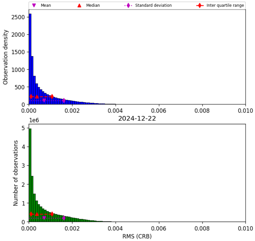
Figure 46: Histogram of “RMS (CRB)” for 2024-12-22 to 2024-12-23
