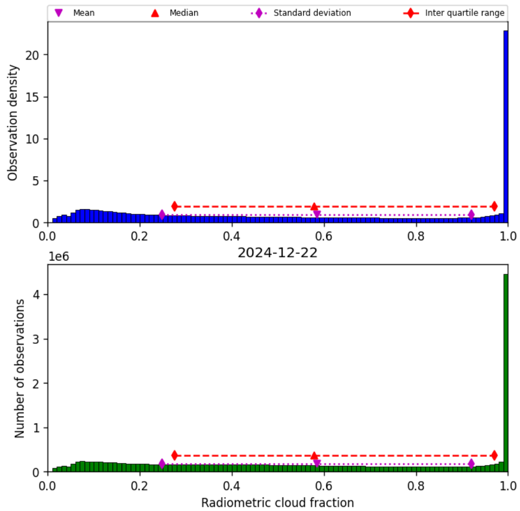
Figure 37: Histogram of “Radiometric cloud fraction” for 2024-12-22 to 2024-12-23
