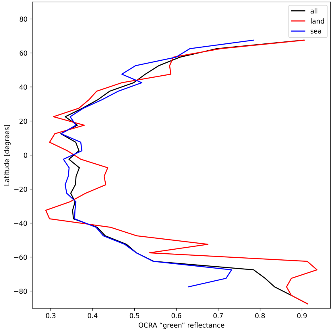
Figure 34: Zonal average of “OCRA “green” reflectance” for 2024-12-22 to 2024-12-23.
