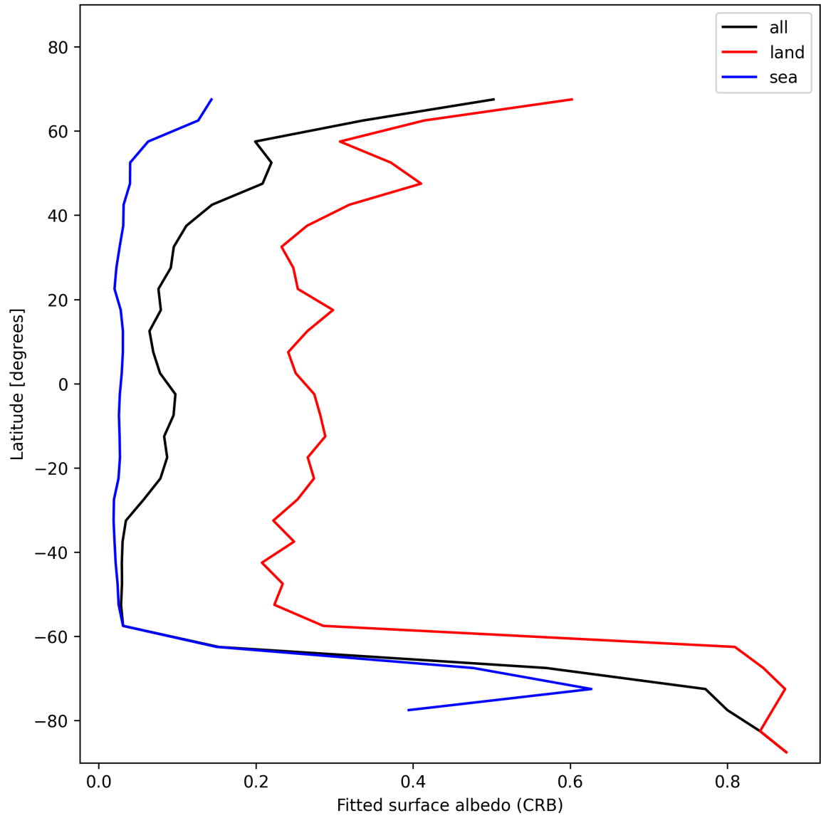
Figure 28: Zonal average of “Fitted surface albedo (CRB)” for 2024-12-22 to 2024-12-23.
