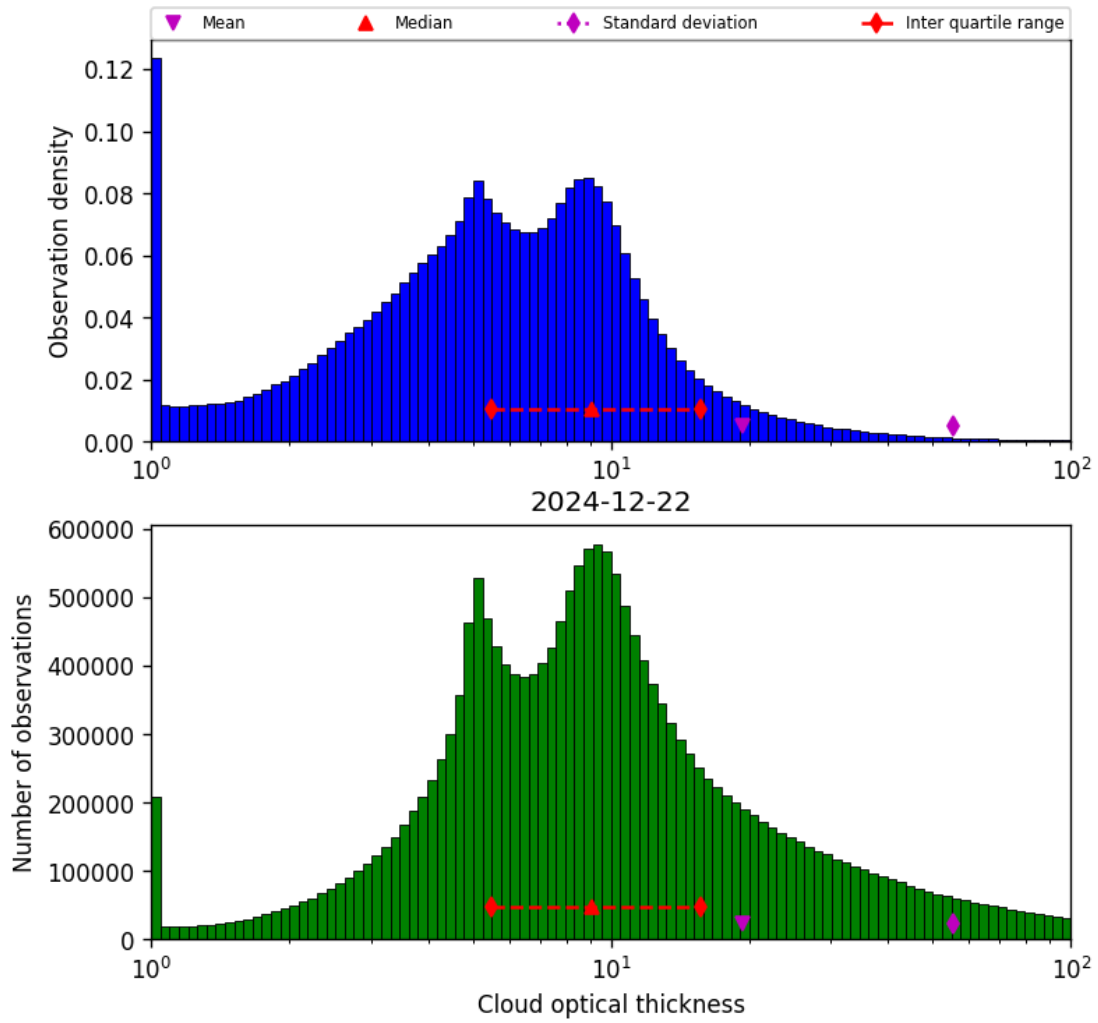
Figure 39: Histogram of “Cloud optical thickness” for 2024-12-22 to 2024-12-23
