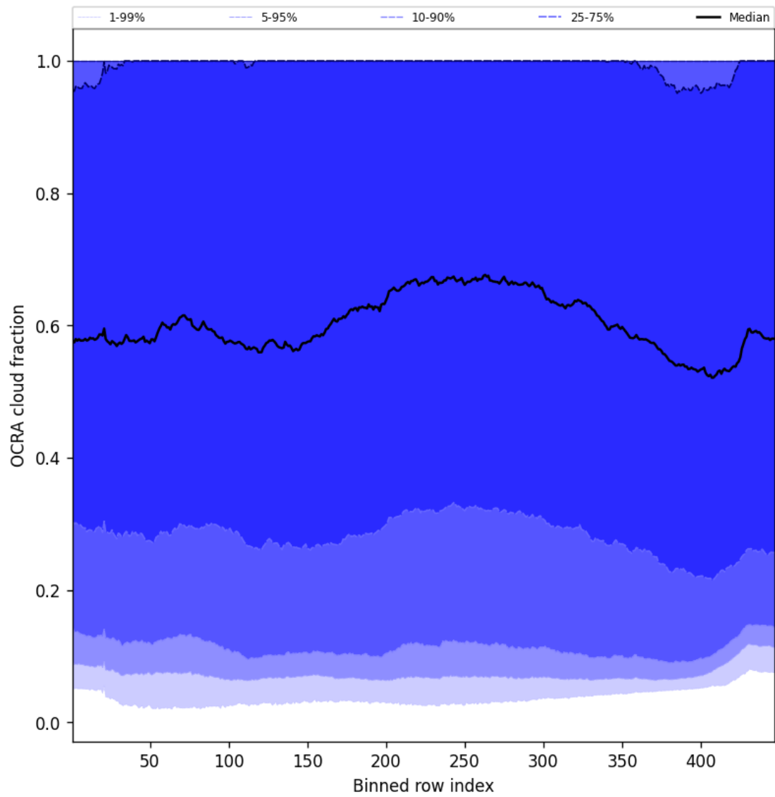
Figure 64: Along track statistics of “OCRA cloud fraction” for 2024-12-22 to 2024-12-23
