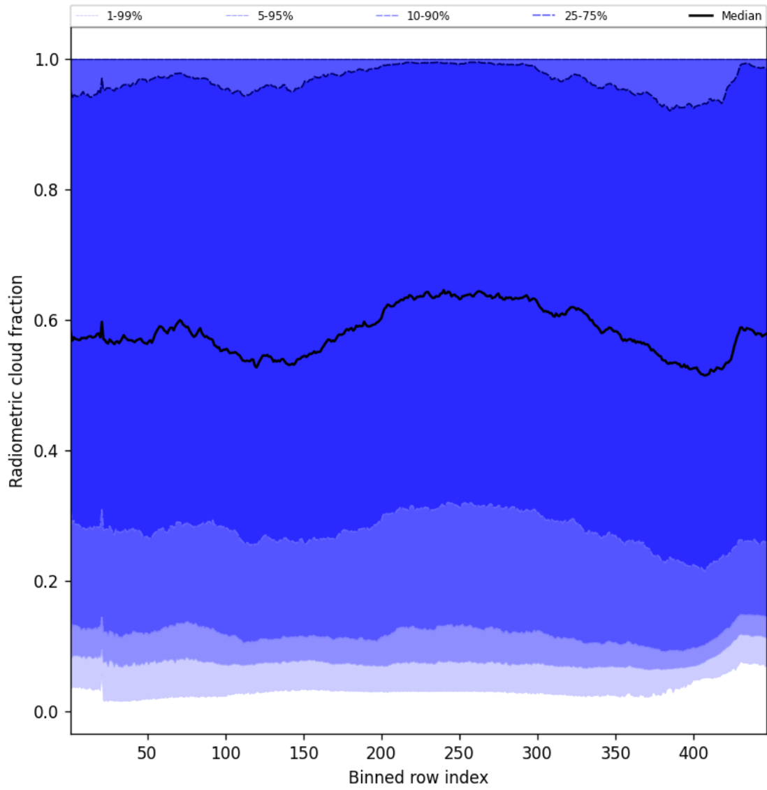
Figure 53: Along track statistics of “Radiometric cloud fraction” for 2024-12-22 to 2024-12-23
