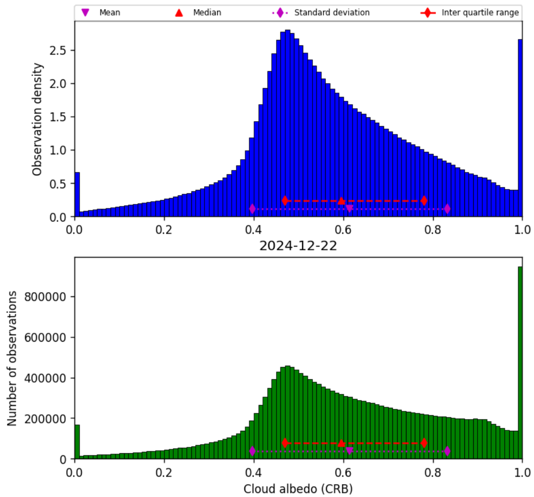
Figure 42: Histogram of “Cloud albedo (CRB)” for 2024-12-22 to 2024-12-23
