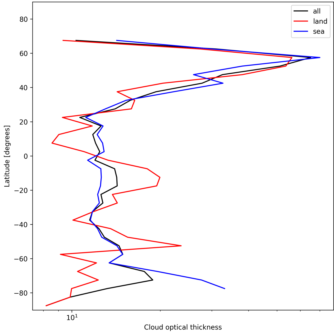
Figure 23: Zonal average of “Cloud optical thickness” for 2024-12-22 to 2024-12-23.
