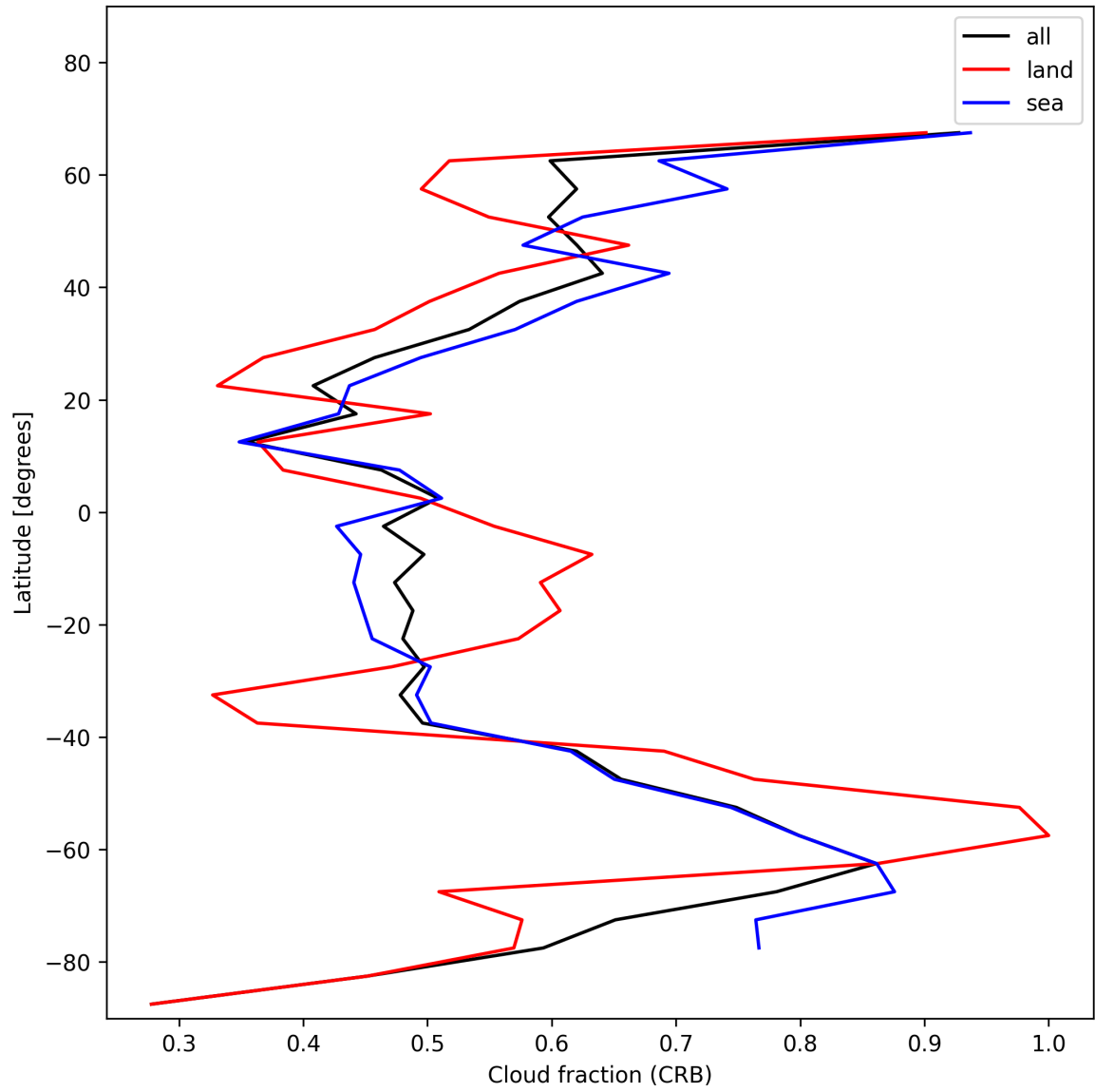
Figure 24: Zonal average of “Cloud fraction (CRB)” for 2024-12-22 to 2024-12-23.
