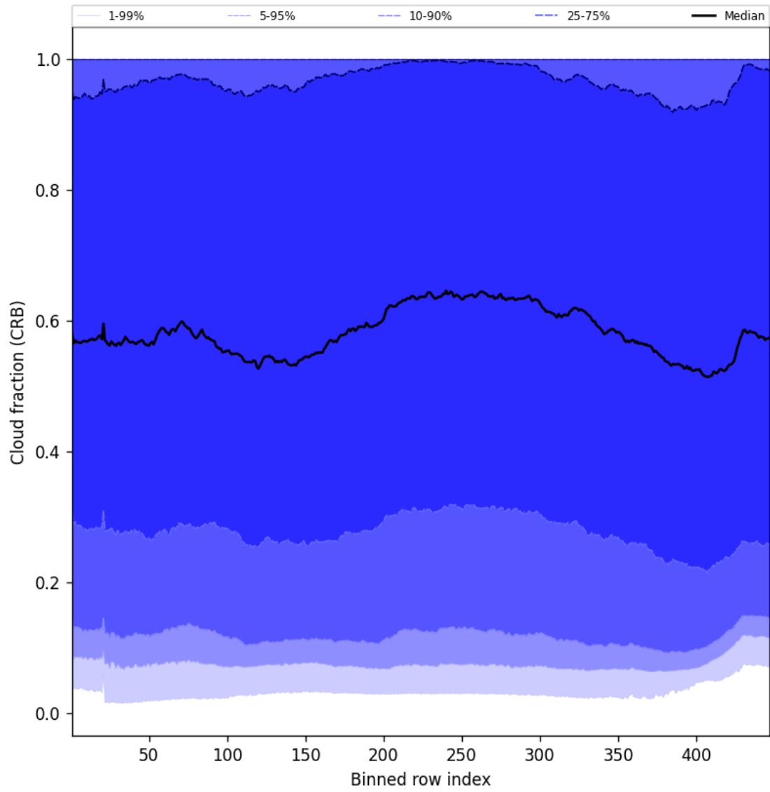
Figure 56: Along track statistics of “Cloud fraction (CRB)” for 2024-12-22 to 2024-12-23
