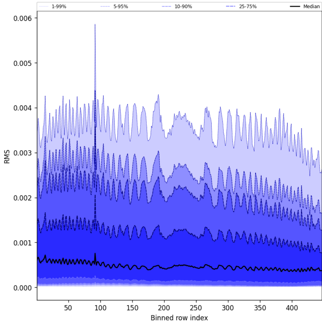
Figure 61: Along track statistics of “RMS” for 2024-12-22 to 2024-12-23
