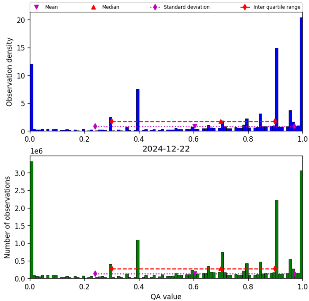
Figure 36: Histogram of “QA value” for 2024-12-22 to 2024-12-23
