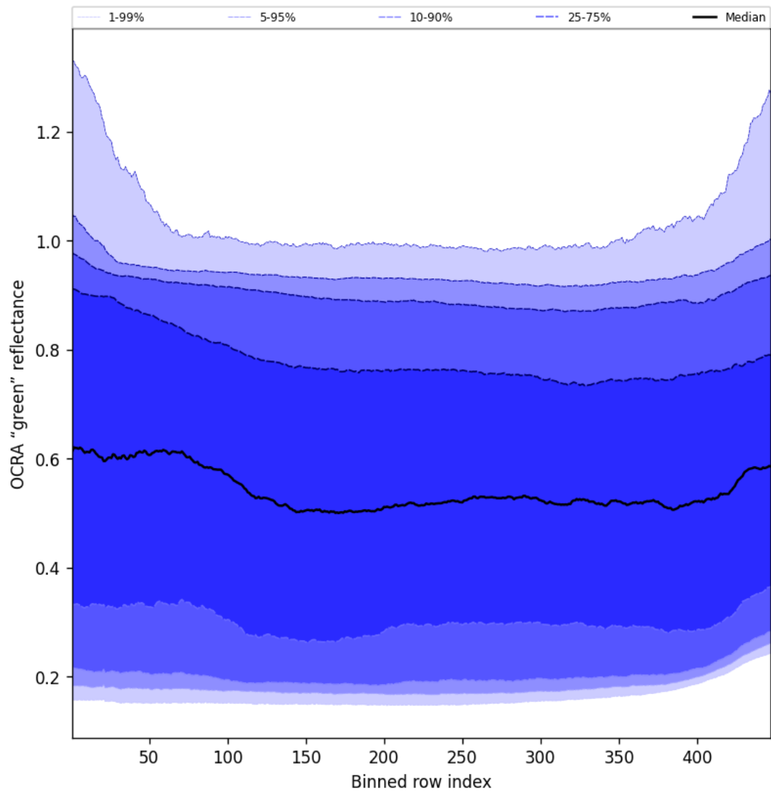
Figure 66: Along track statistics of "OCRA "green" reflectance" for 2024-12-22 to 2024-12-23
