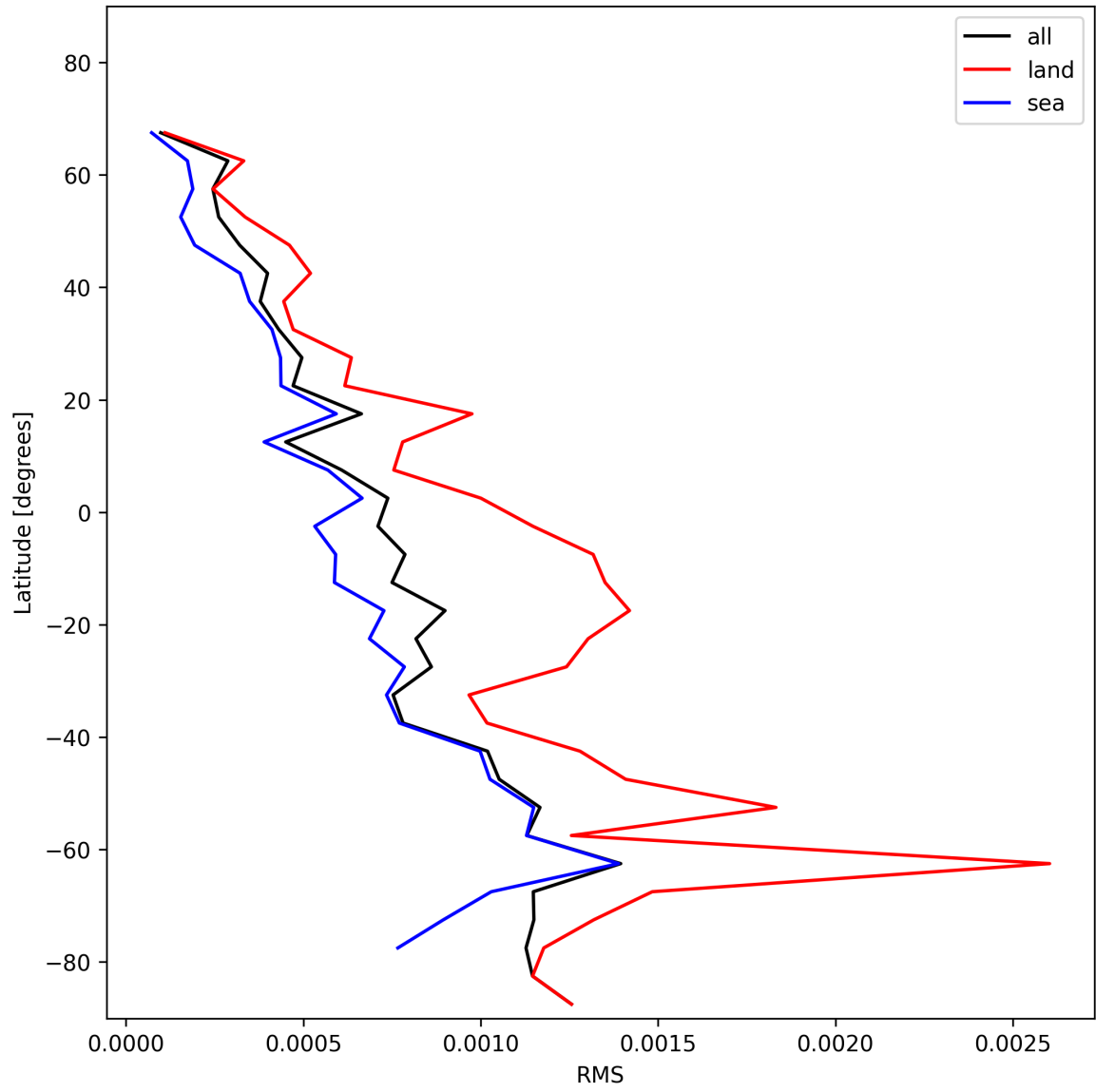
Figure 29: Zonal average of “RMS” for 2024-12-22 to 2024-12-23.
