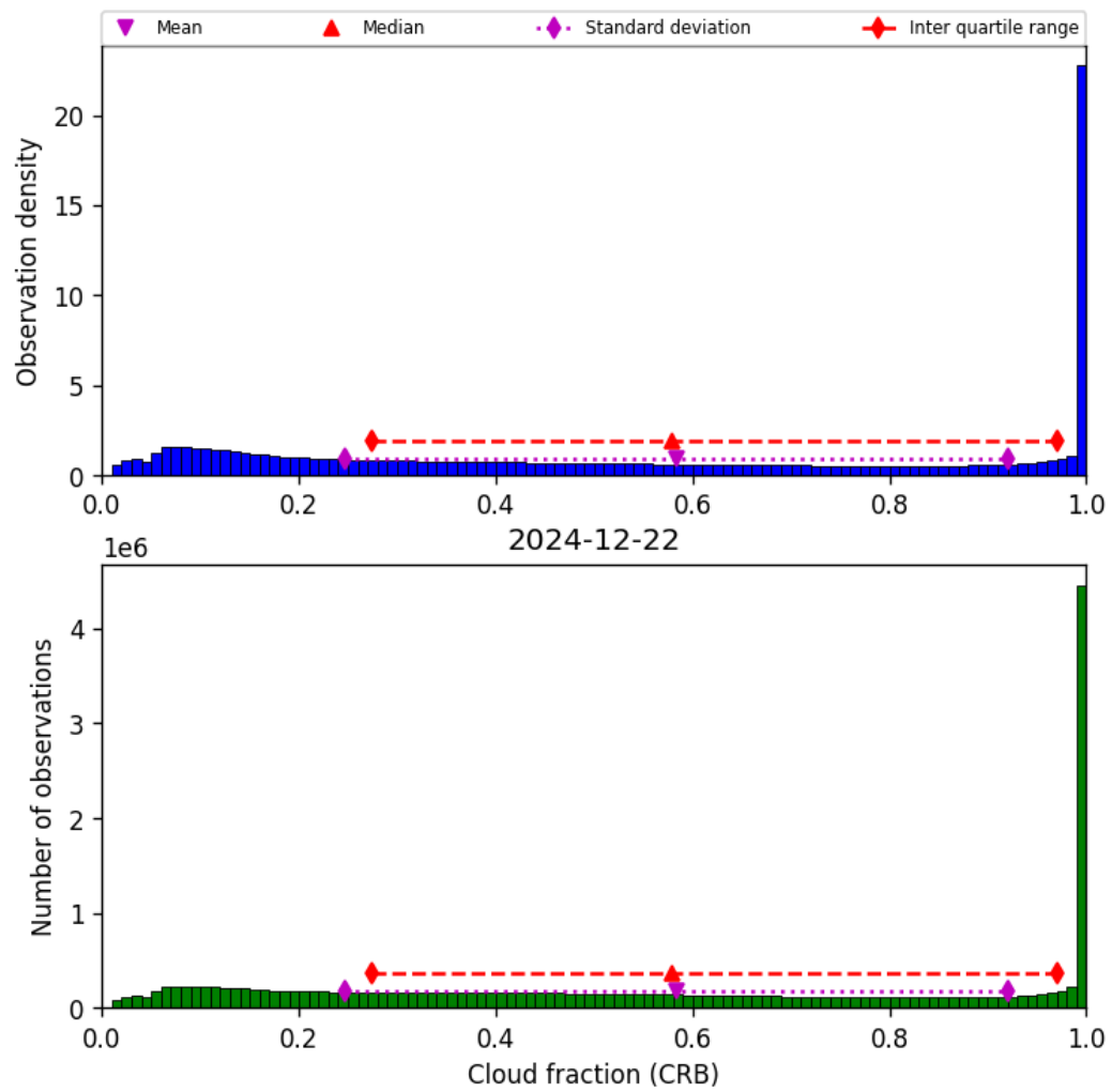
Figure 40: Histogram of “Cloud fraction (CRB)” for 2024-12-22 to 2024-12-23
