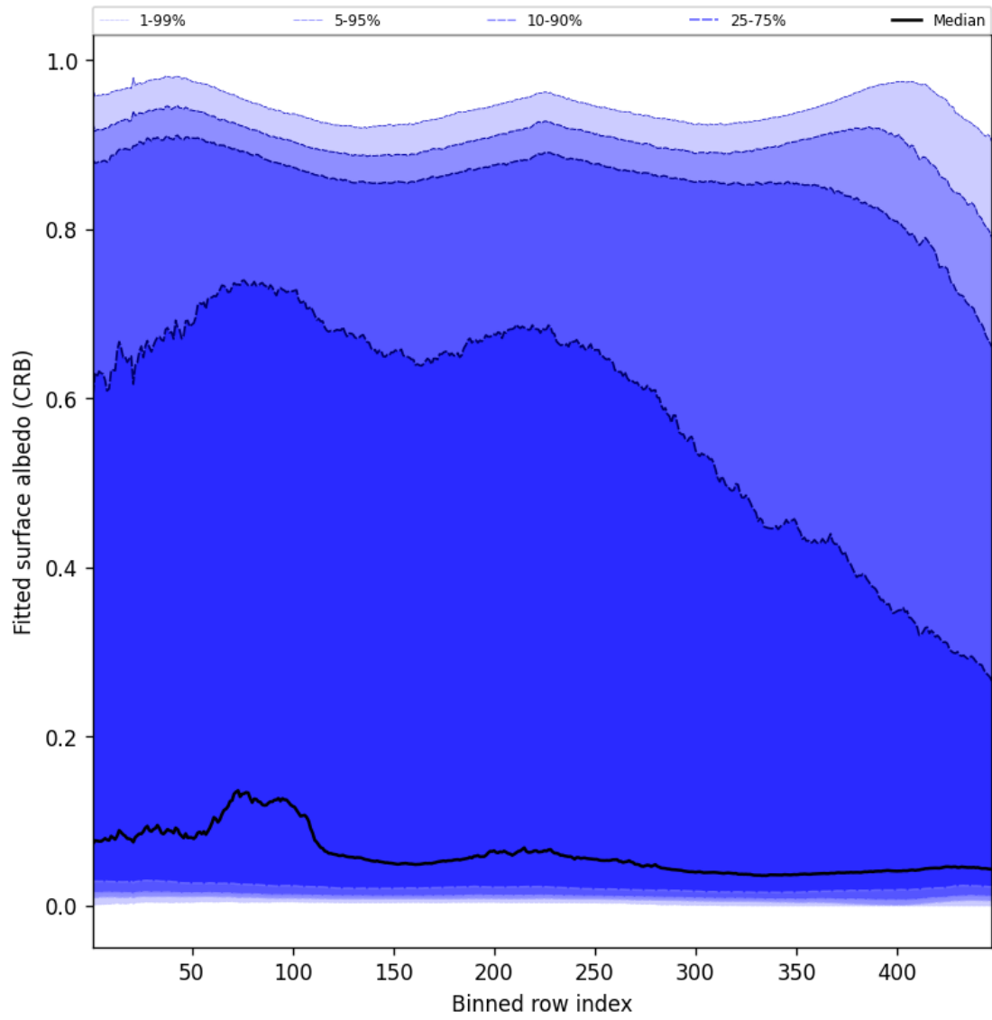
Figure 60: Along track statistics of “Fitted surface albedo (CRB)” for 2024-12-22 to 2024-12-23
