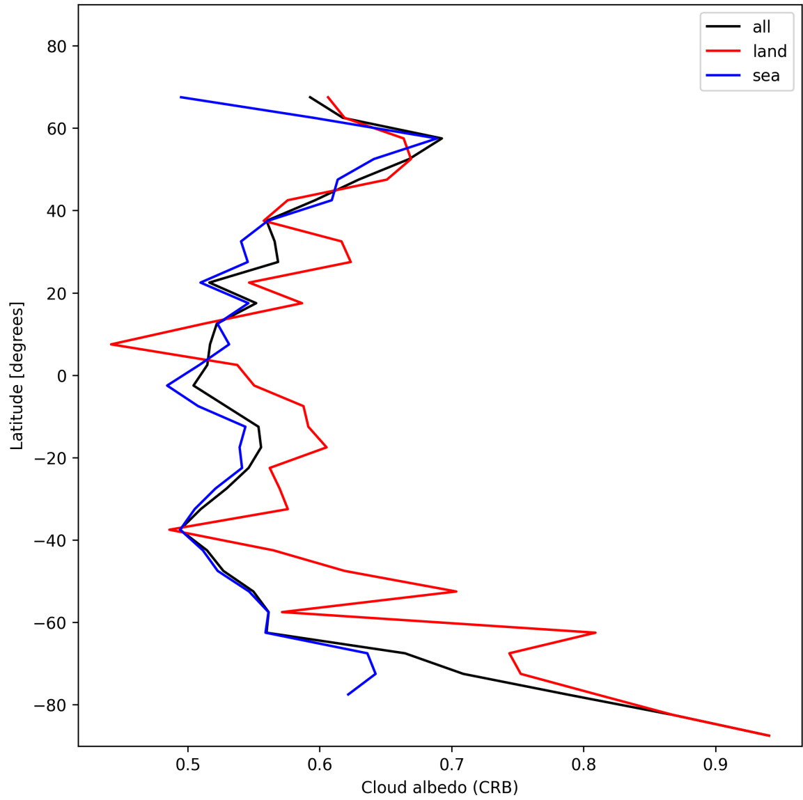
Figure 26: Zonal average of “Cloud albedo (CRB)” for 2024-12-22 to 2024-12-23.
