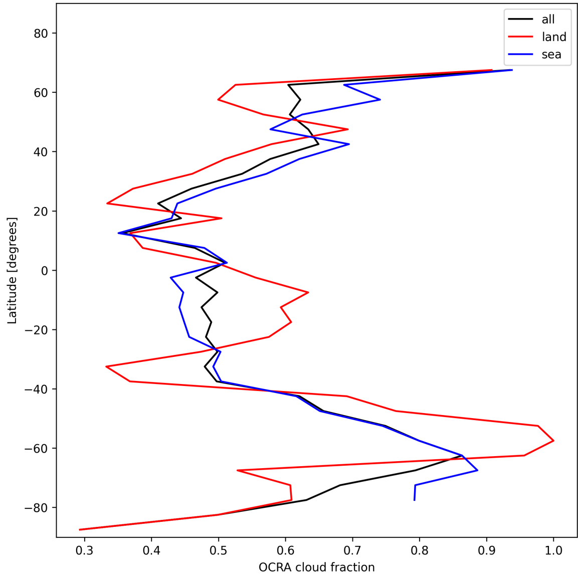
Figure 32: Zonal average of “OCRA cloud fraction” for 2024-12-22 to 2024-12-23.
