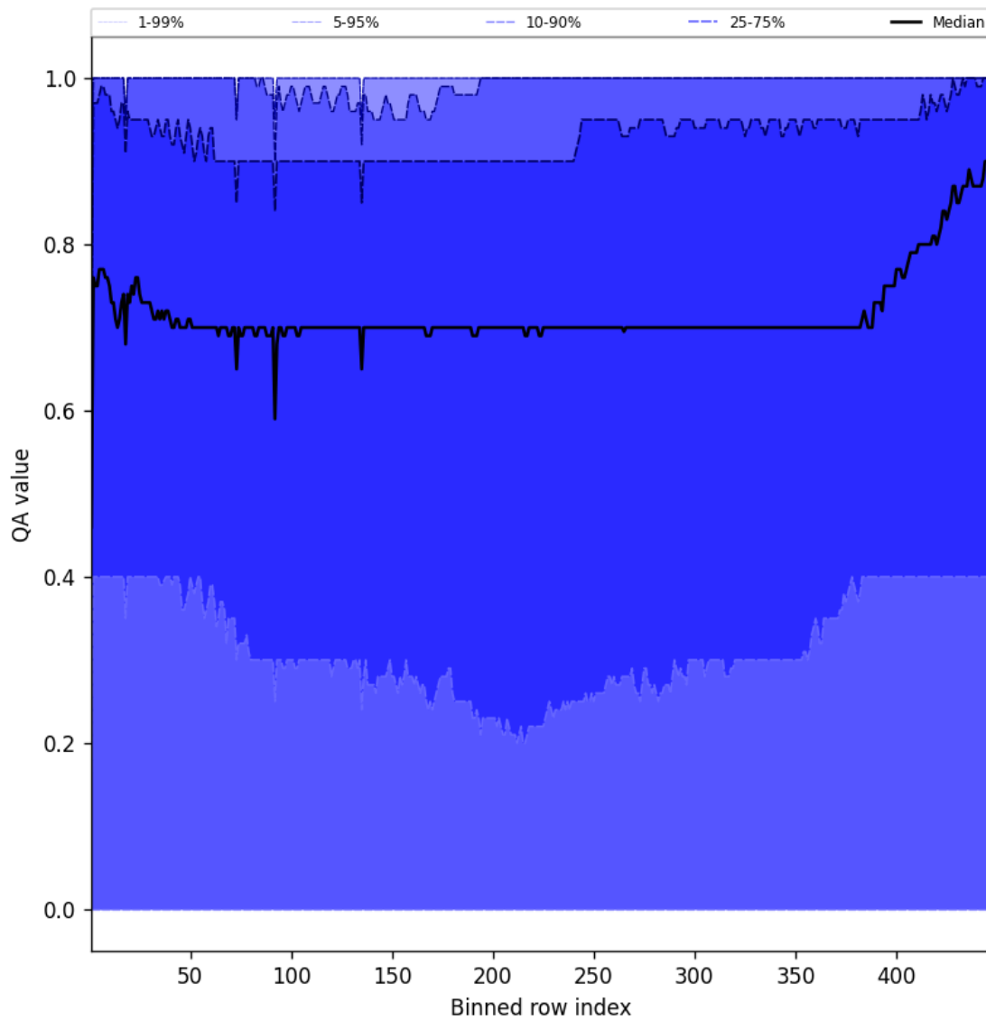
Figure 52: Along track statistics of “QA value” for 2024-12-22 to 2024-12-23
