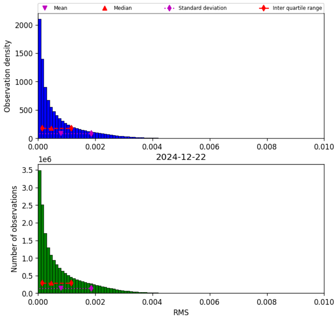
Figure 45: Histogram of “RMS” for 2024-12-22 to 2024-12-23
