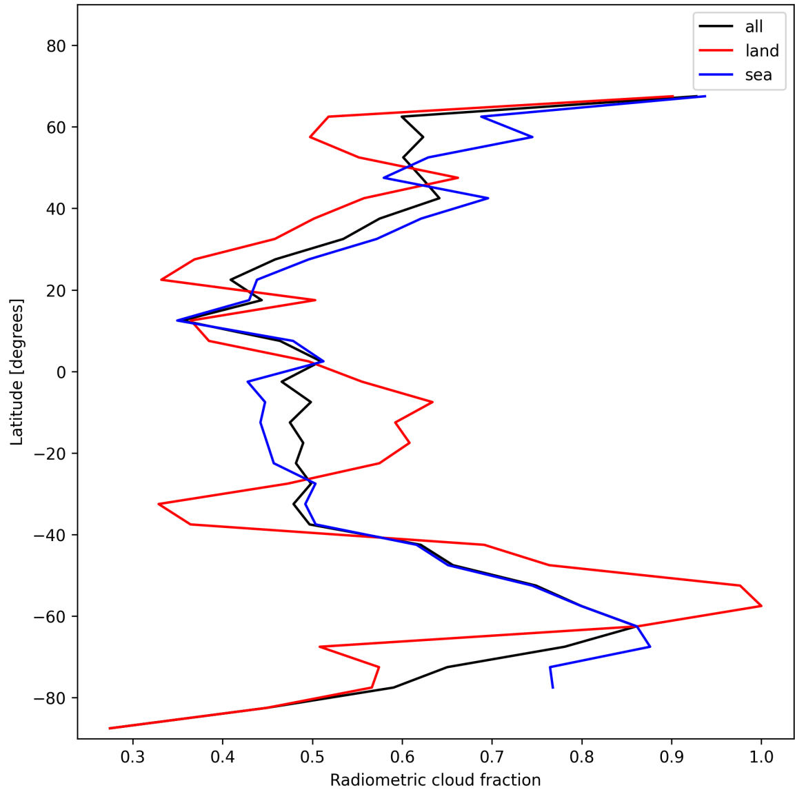
Figure 21: Zonal average of “Radiometric cloud fraction” for 2024-12-22 to 2024-12-23.
