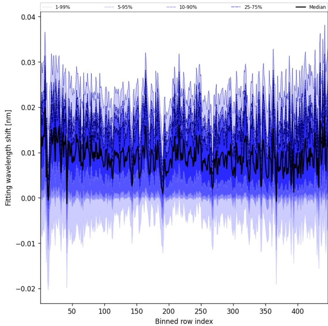
Figure 63: Along track statistics of “Fitting wavelength shift” for 2024-12-22 to 2024-12-23
