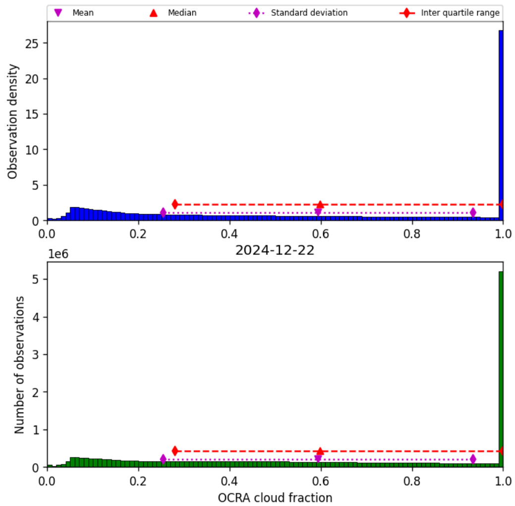
Figure 48: Histogram of “OCRA cloud fraction” for 2024-12-22 to 2024-12-23
