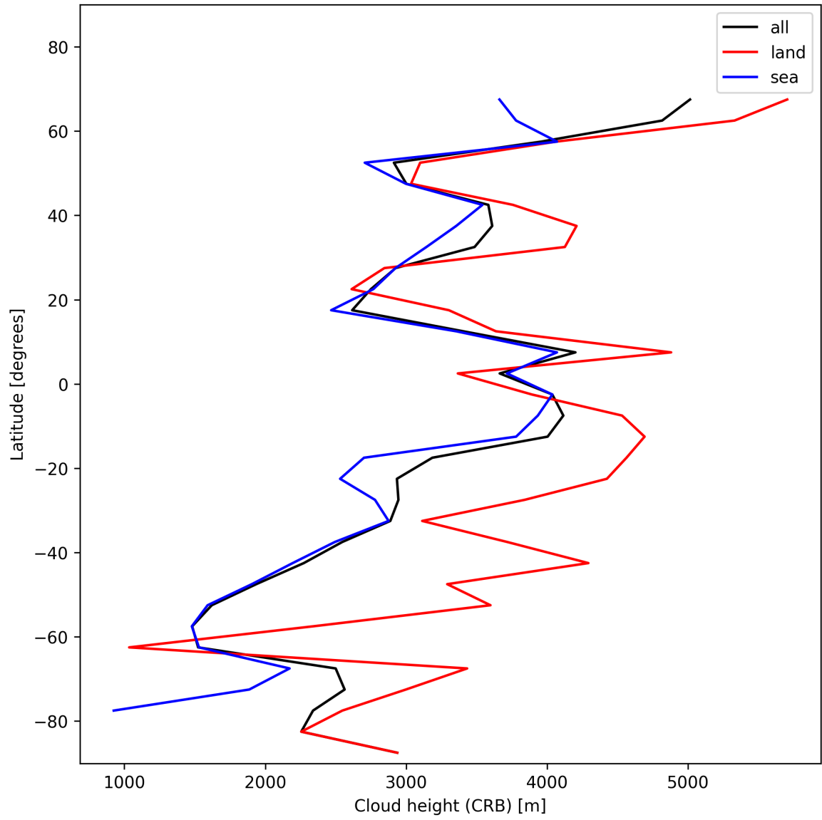
Figure 25: Zonal average of “Cloud height (CRB)” for 2024-12-22 to 2024-12-23.
