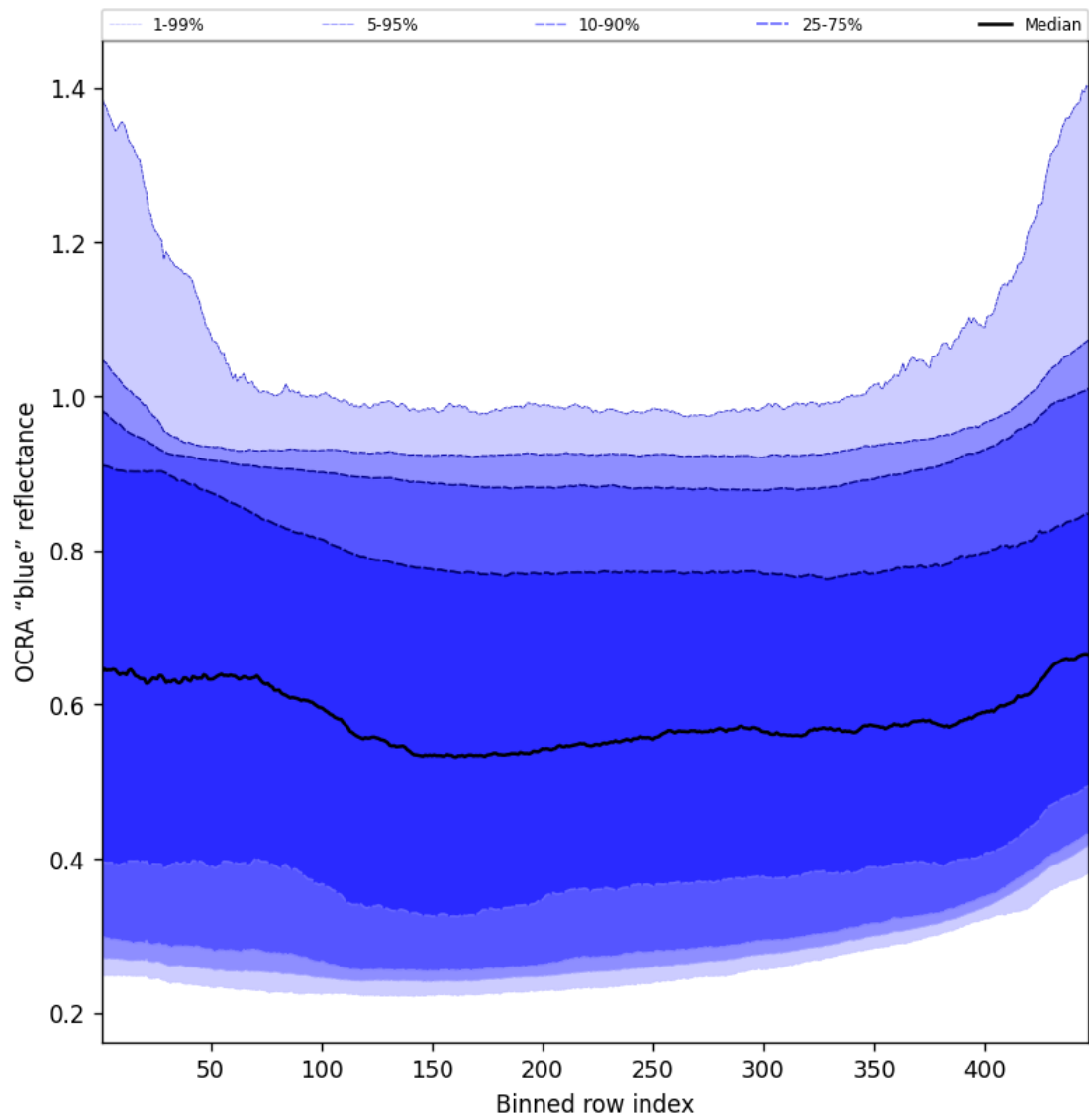
Figure 65: Along track statistics of “OCRA “blue” reflectance” for 2024-12-22 to 2024-12-23
