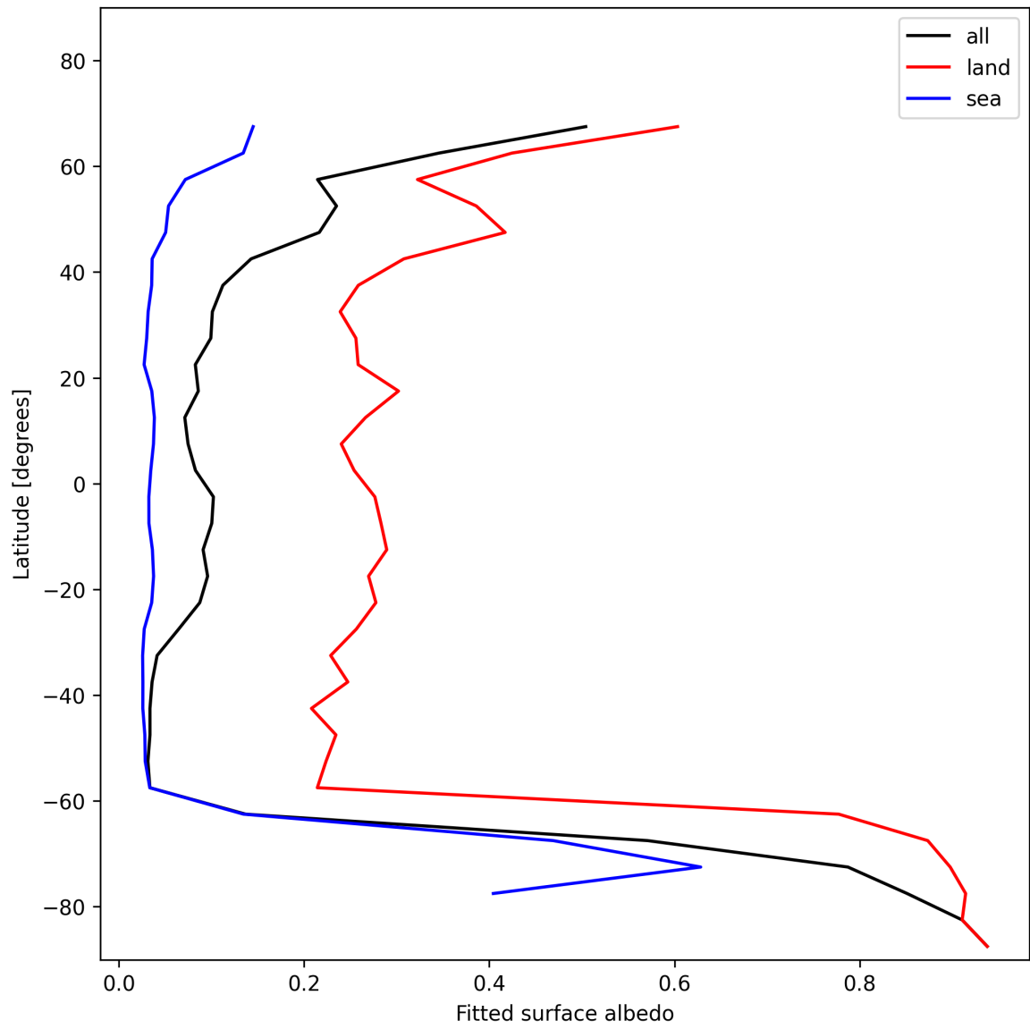
Figure 27: Zonal average of “Fitted surface albedo” for 2024-12-22 to 2024-12-23.
