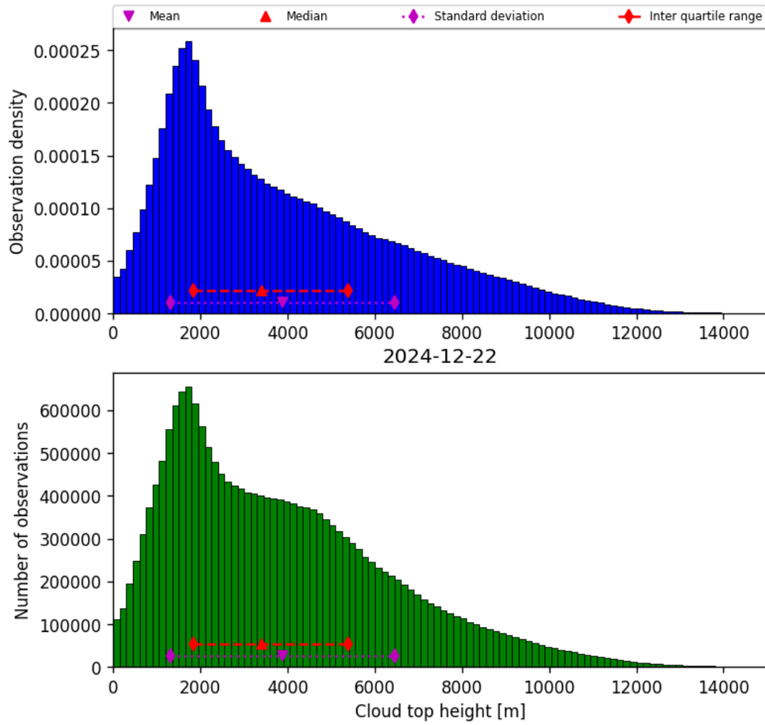
Figure 38: Histogram of “Cloud top height” for 2024-12-22 to 2024-12-23
