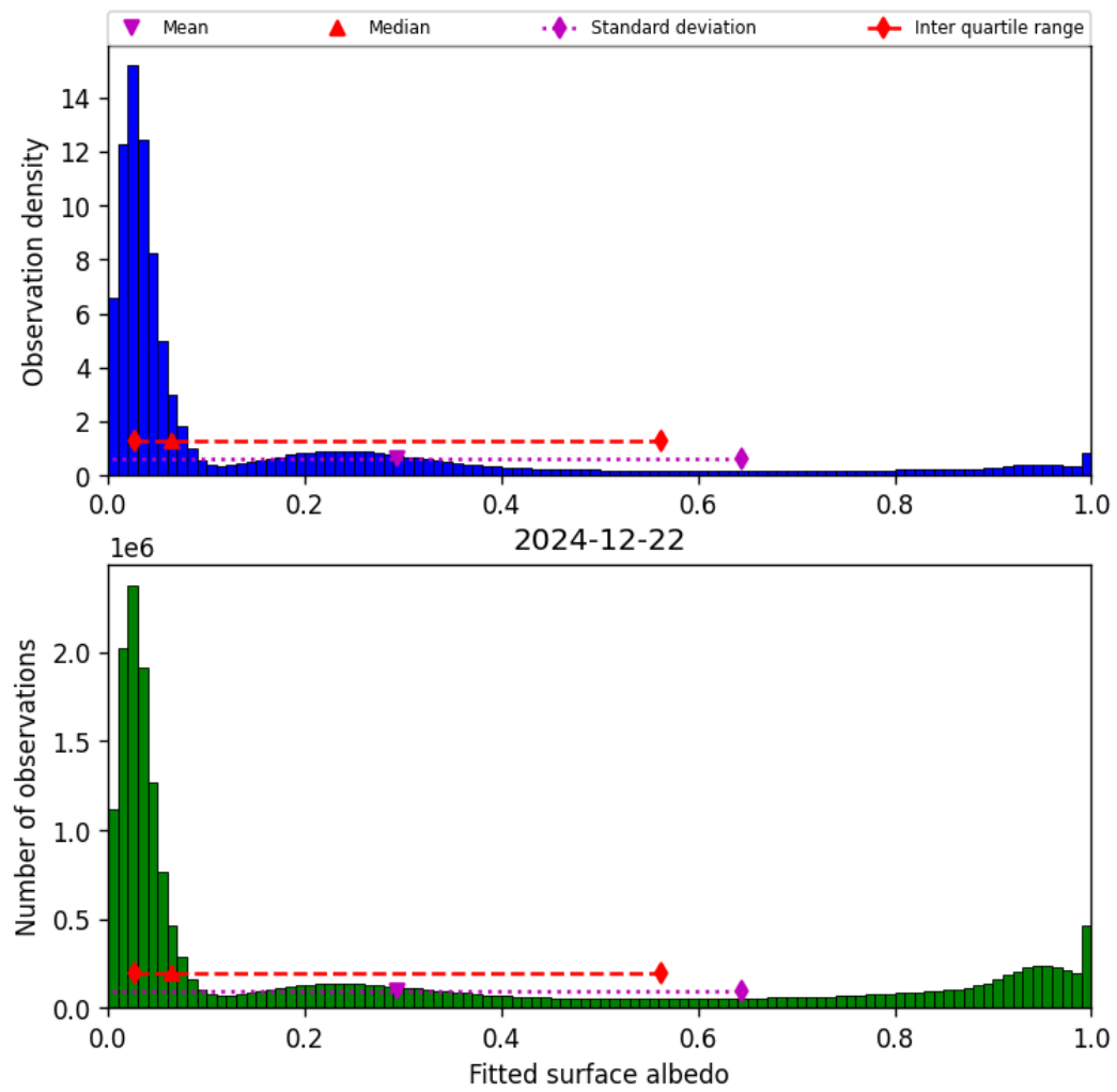
Figure 43: Histogram of “Fitted surface albedo” for 2024-12-22 to 2024-12-23
