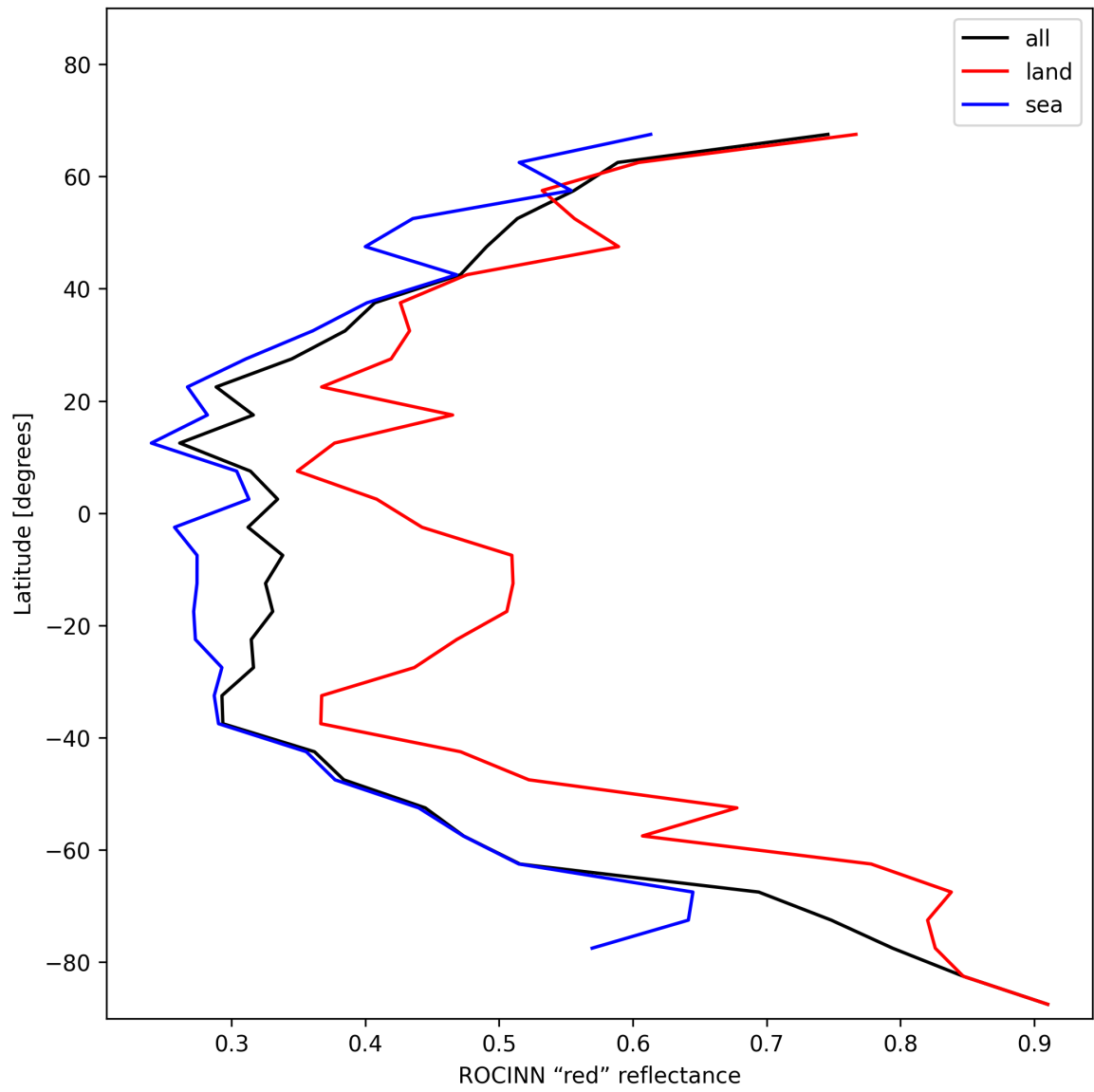
Figure 35: Zonal average of "ROCINN "red" reflectance" for 2024-12-22 to 2024-12-23.
