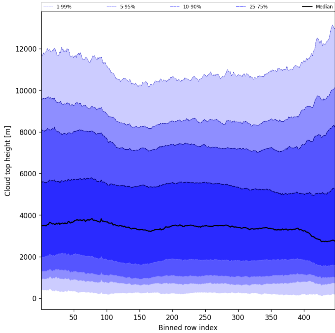
Figure 54: Along track statistics of “Cloud top height” for 2024-12-22 to 2024-12-23
