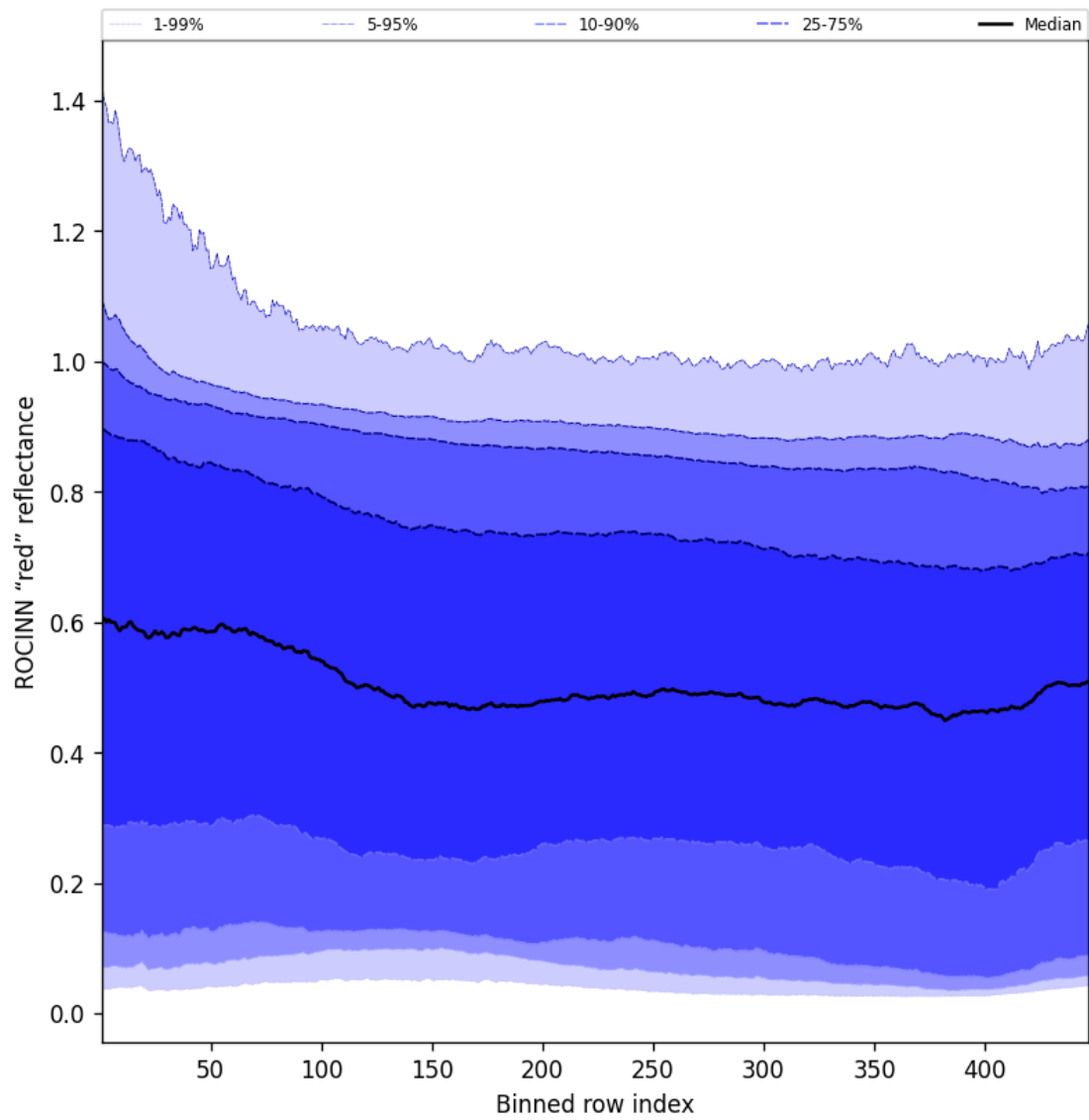
Figure 67: Along track statistics of “ROCINN “red” reflectance” for 2024-12-22 to 2024-12-23
