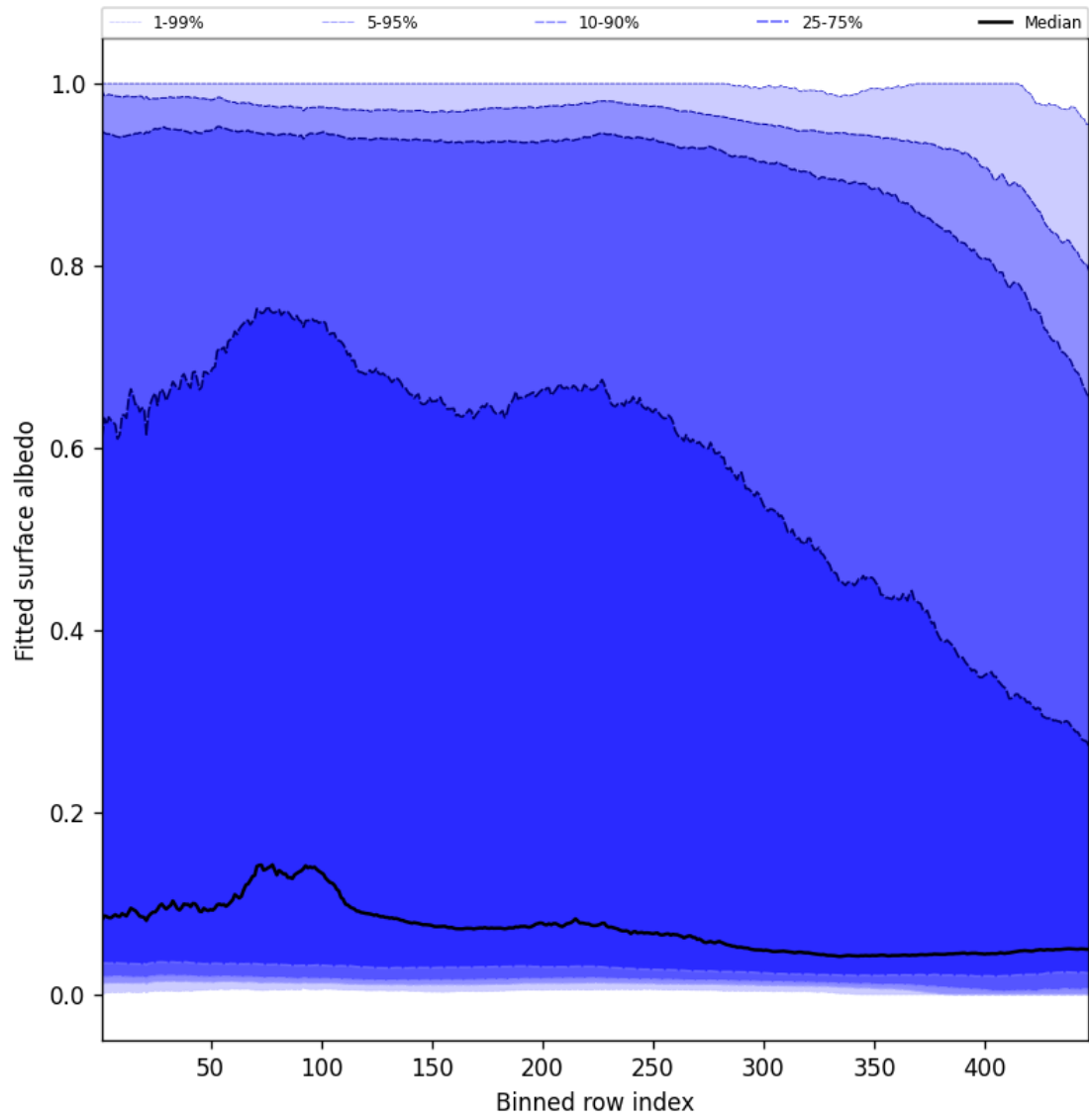
Figure 59: Along track statistics of “Fitted surface albedo” for 2024-12-22 to 2024-12-23
