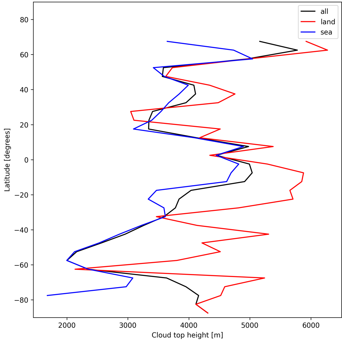
Figure 22: Zonal average of “Cloud top height” for 2024-12-22 to 2024-12-23.
