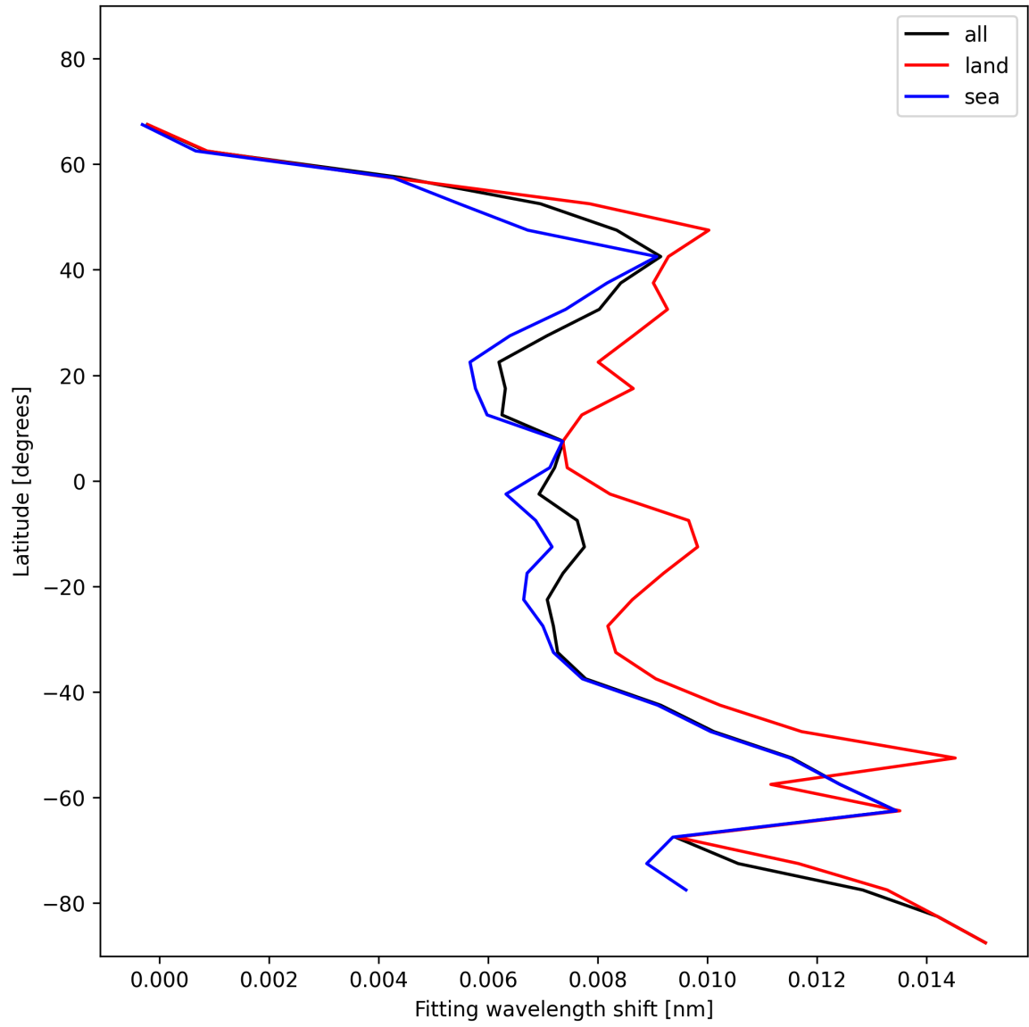
Figure 31: Zonal average of “Fitting wavelength shift” for 2024-12-22 to 2024-12-23.
