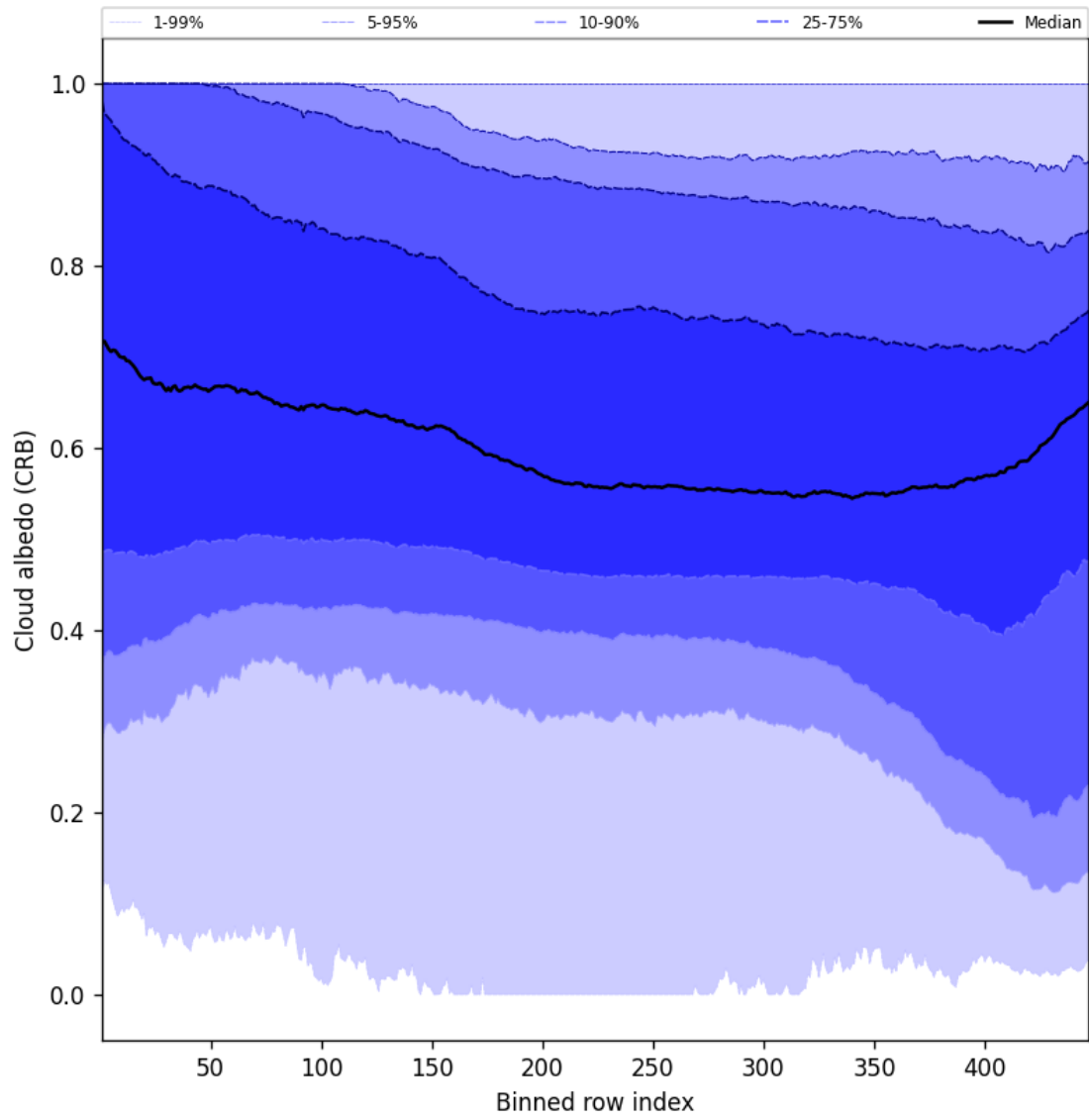
Figure 58: Along track statistics of “Cloud albedo (CRB)” for 2024-12-22 to 2024-12-23
