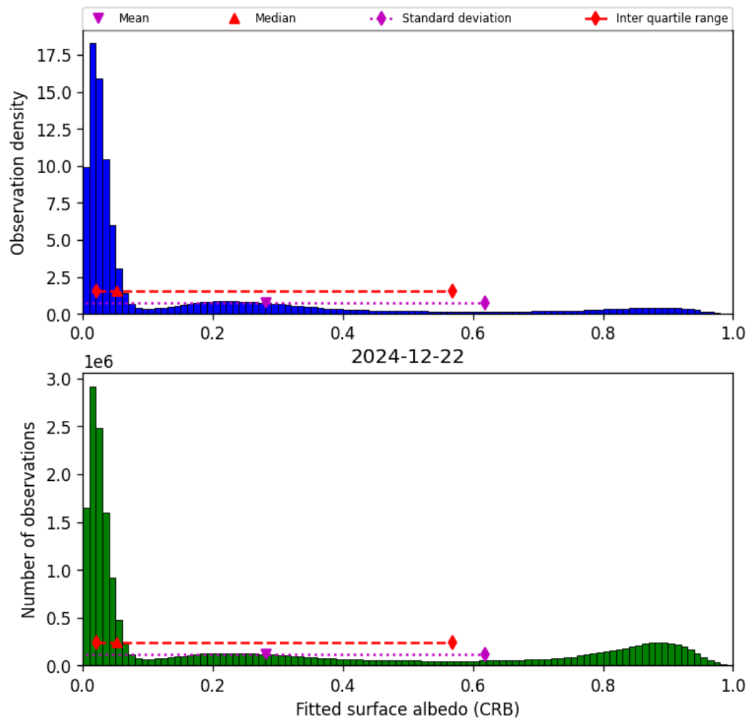
Figure 44: Histogram of “Fitted surface albedo (CRB)” for 2024-12-22 to 2024-12-23
