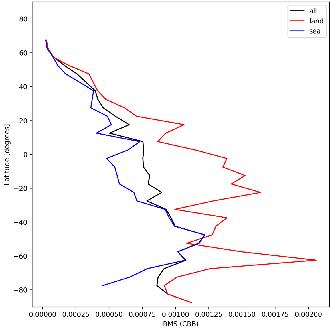
Figure 30: Zonal average of “RMS (CRB)” for 2024-12-25 to 2024-12-25.
