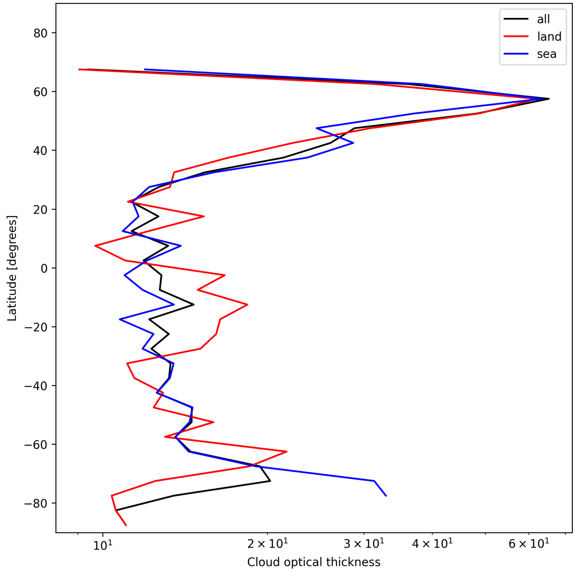
Figure 23: Zonal average of “Cloud optical thickness” for 2024-12-25 to 2024-12-25.
