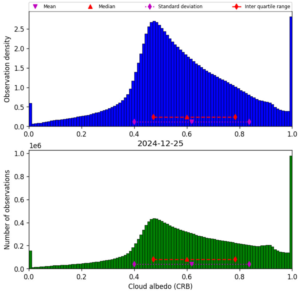
Figure 42: Histogram of “Cloud albedo (CRB)” for 2024-12-25 to 2024-12-25
