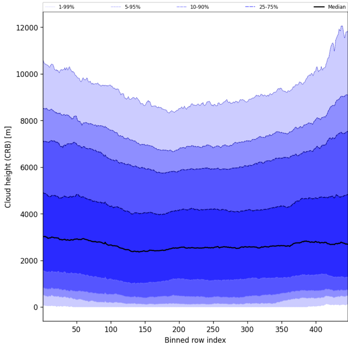
Figure 57: Along track statistics of “Cloud height (CRB)” for 2024-12-25 to 2024-12-25
