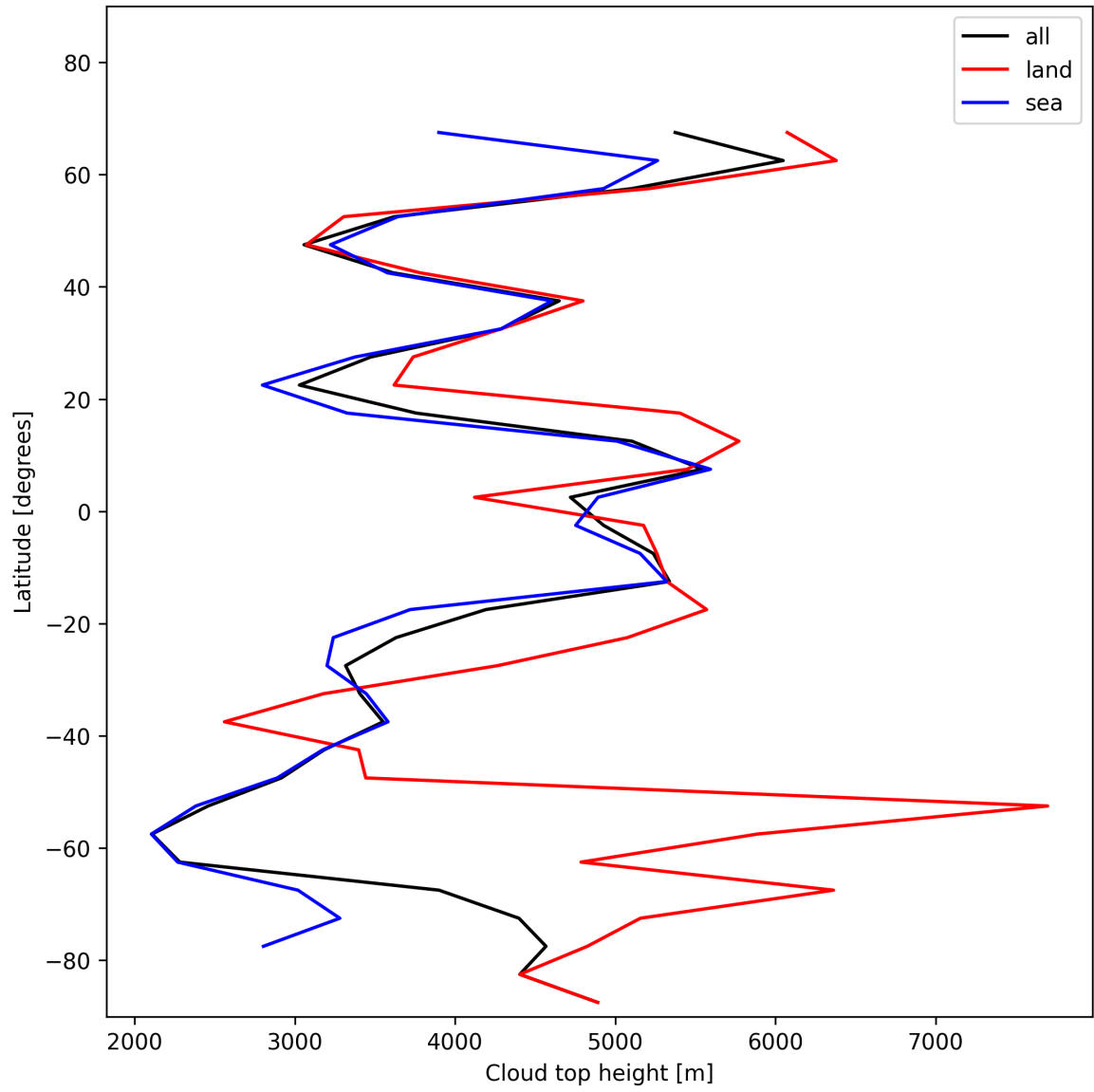
Figure 22: Zonal average of “Cloud top height” for 2024-12-25 to 2024-12-25.
