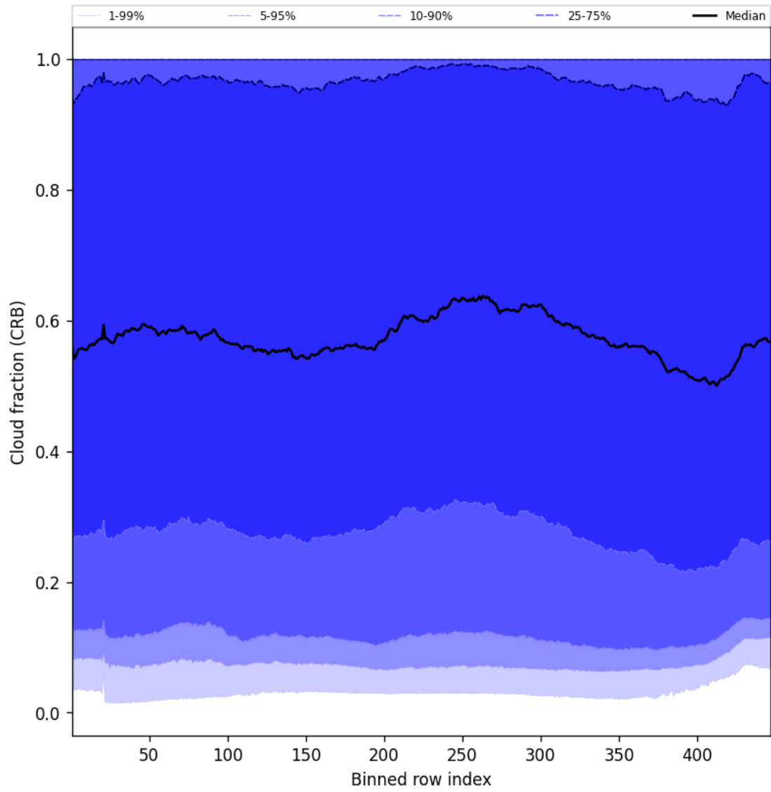
Figure 56: Along track statistics of “Cloud fraction (CRB)” for 2024-12-25 to 2024-12-25
