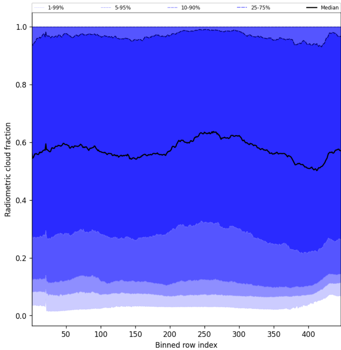
Figure 53: Along track statistics of “Radiometric cloud fraction” for 2024-12-25 to 2024-12-25
