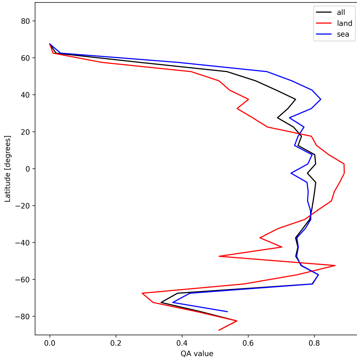
Figure 20: Zonal average of “QA value” for 2024-12-25 to 2024-12-25.
