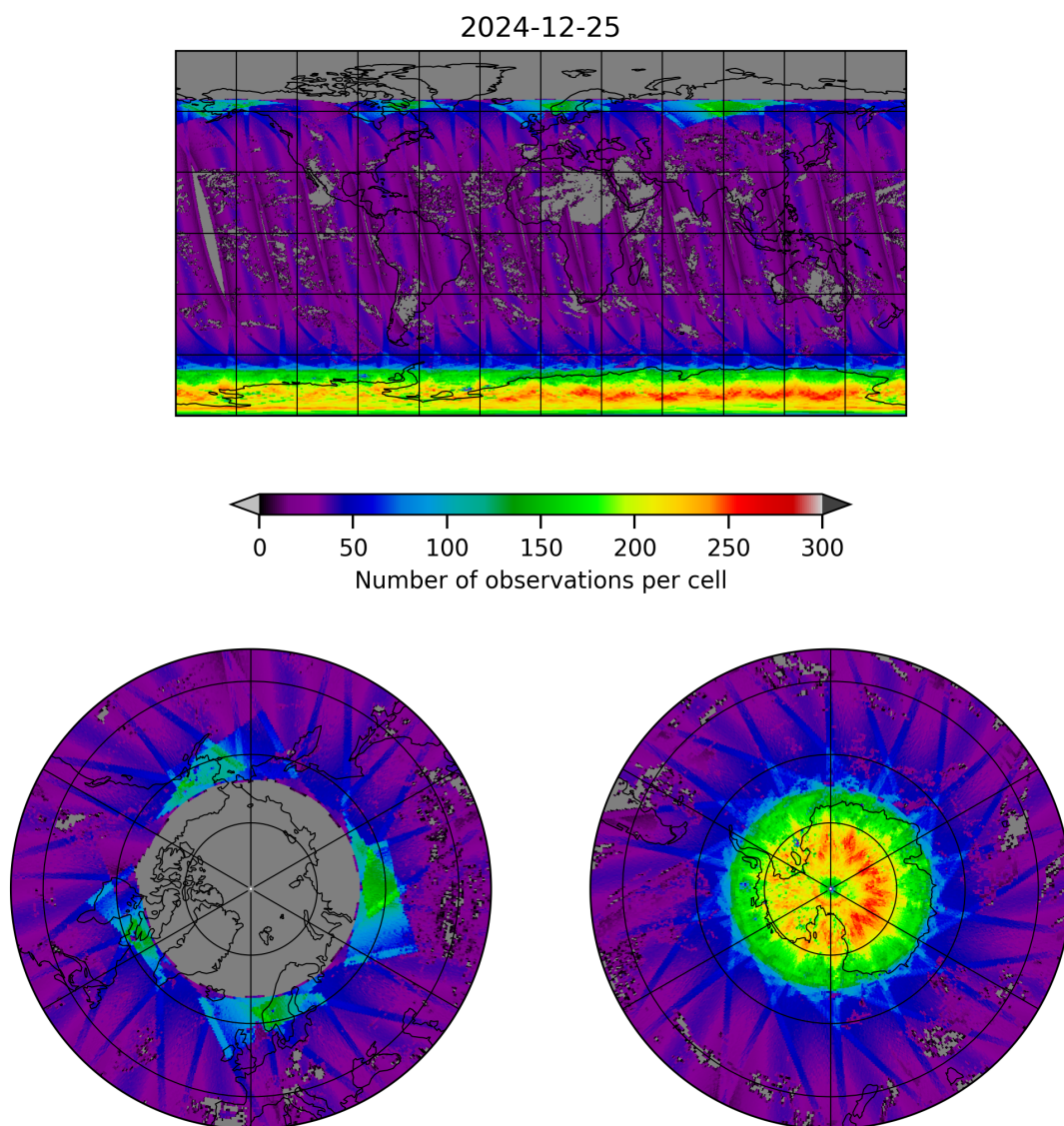
Figure 19: Map of the number of observations for 2024-12-25 to 2024-12-25
