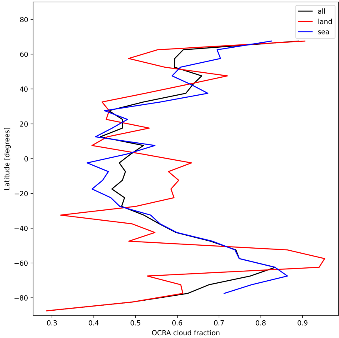
Figure 32: Zonal average of “OCRA cloud fraction” for 2024-12-25 to 2024-12-25.
