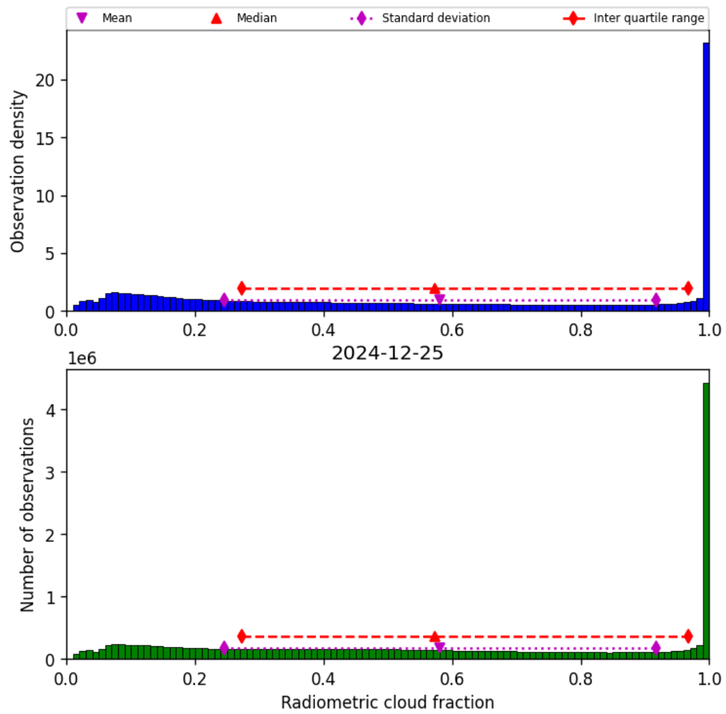
Figure 37: Histogram of “Radiometric cloud fraction” for 2024-12-25 to 2024-12-25
