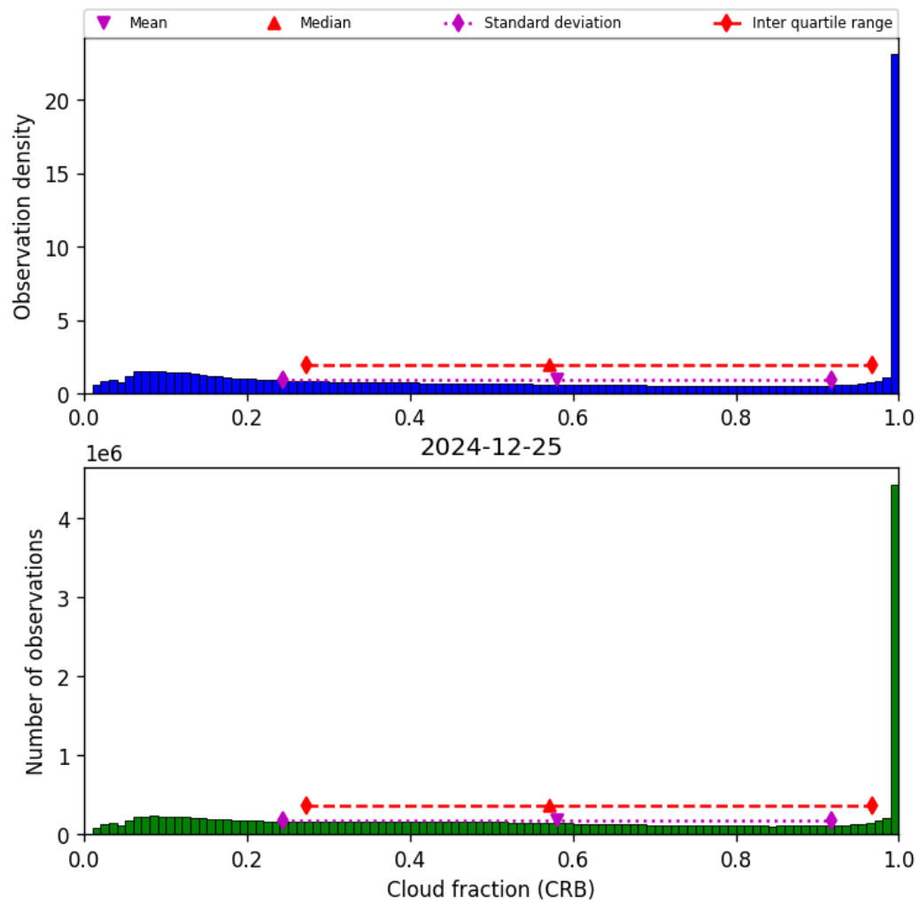
Figure 40: Histogram of “Cloud fraction (CRB)” for 2024-12-25 to 2024-12-25
