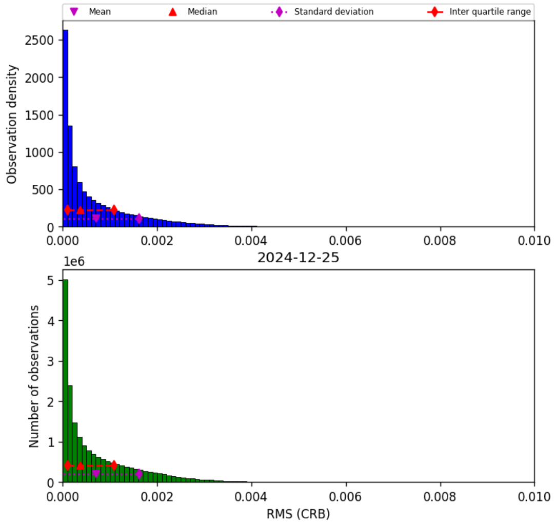
Figure 46: Histogram of “RMS (CRB)” for 2024-12-25 to 2024-12-25
