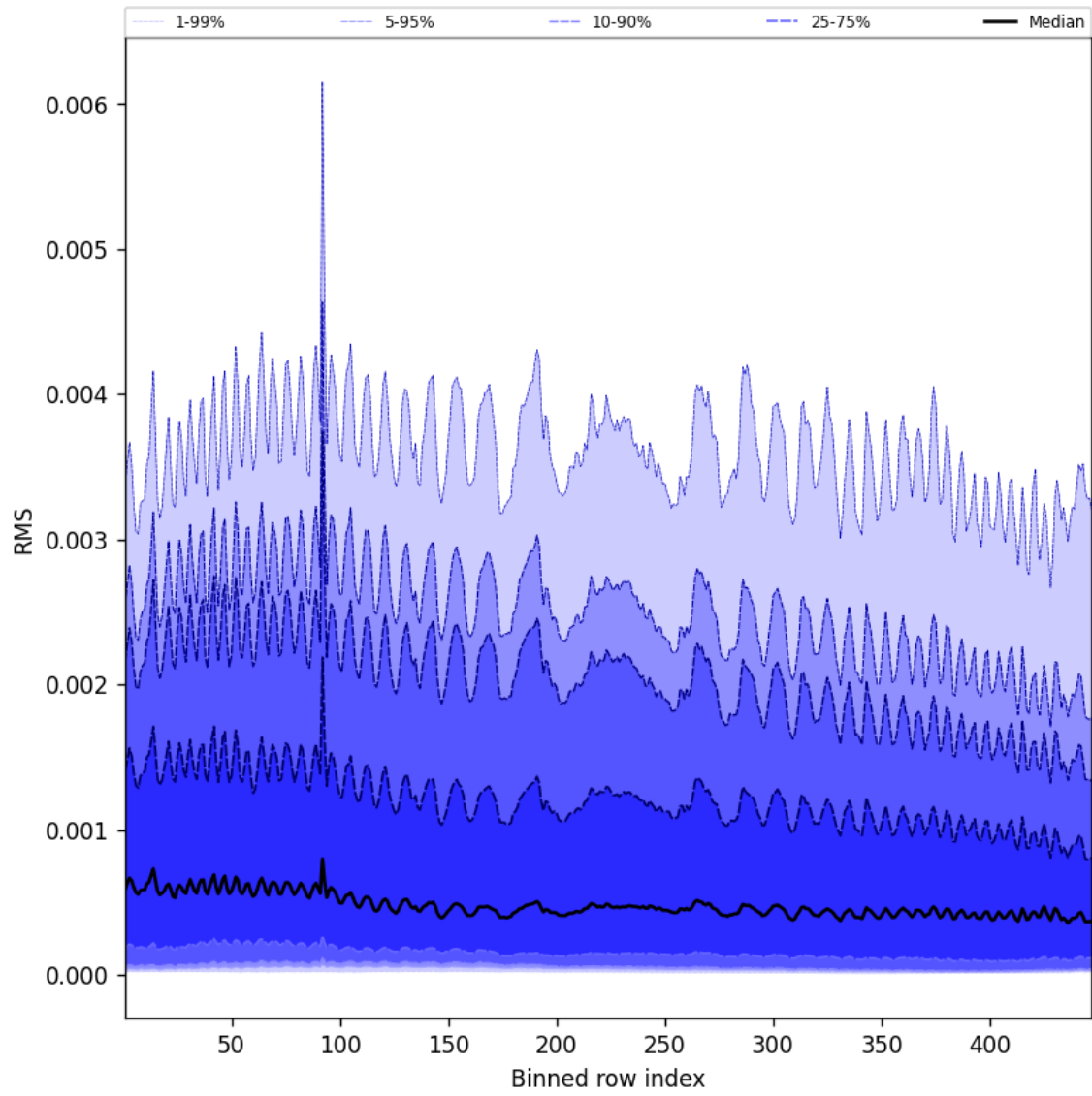
Figure 61: Along track statistics of “RMS” for 2024-12-25 to 2024-12-25
