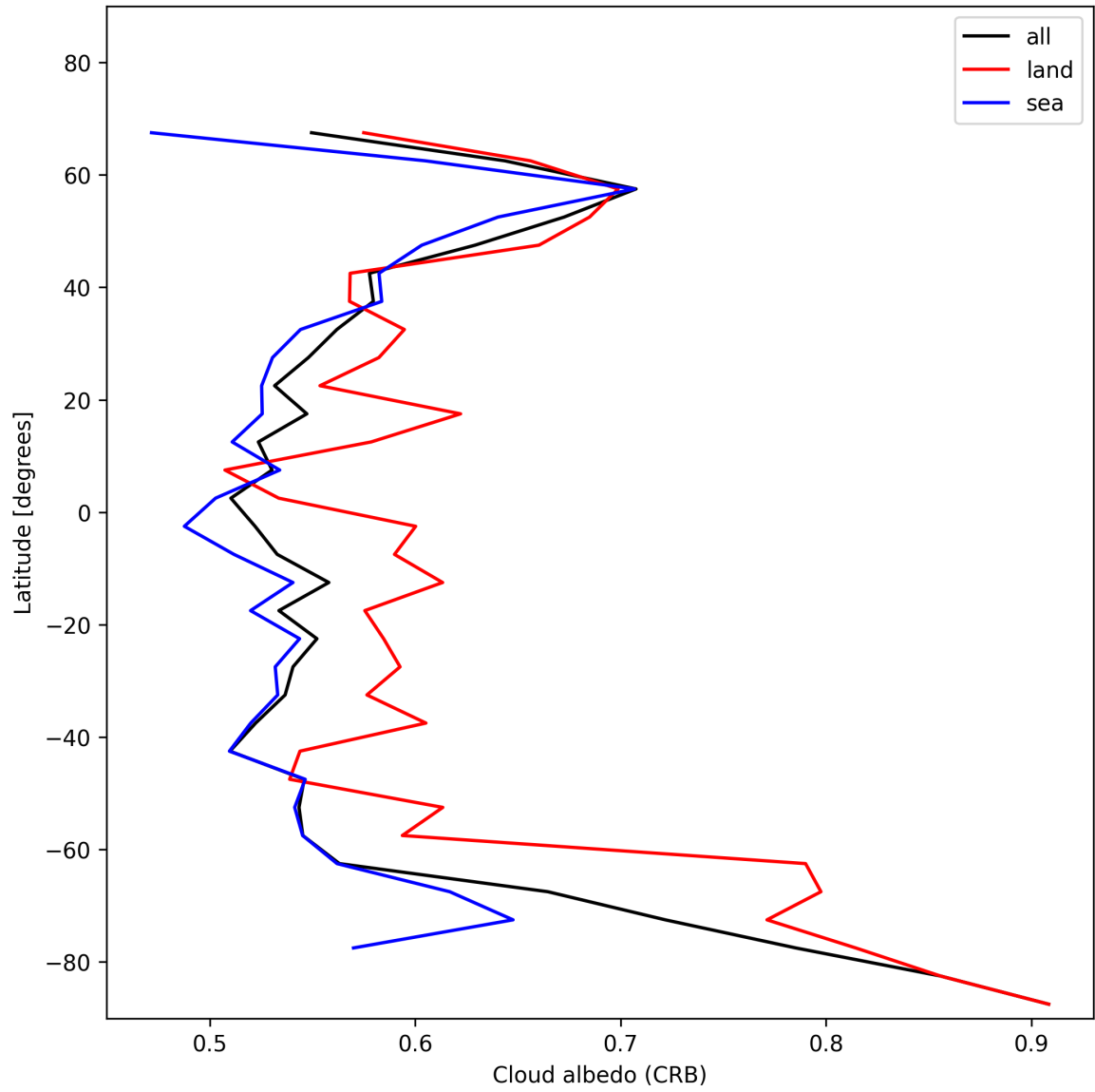
Figure 26: Zonal average of “Cloud albedo (CRB)” for 2024-12-25 to 2024-12-25.
