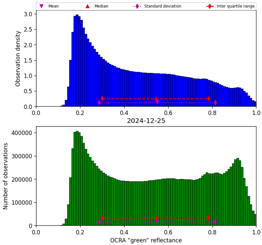
Figure 50: Histogram of “OCRA “green” reflectance” for 2024-12-25 to 2024-12-25
