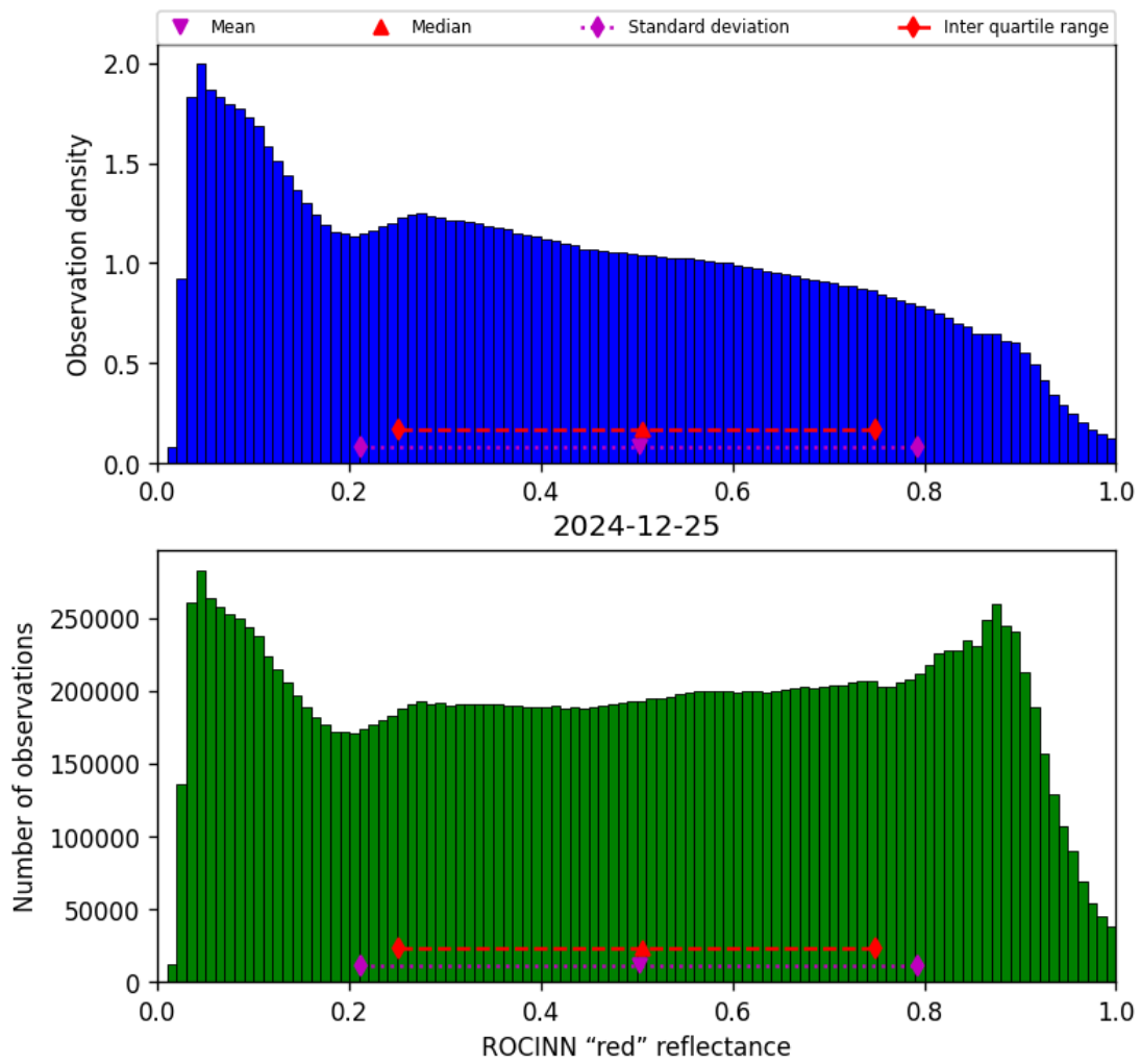
Figure 51: Histogram of “ROCINN “red” reflectance” for 2024-12-25 to 2024-12-25
