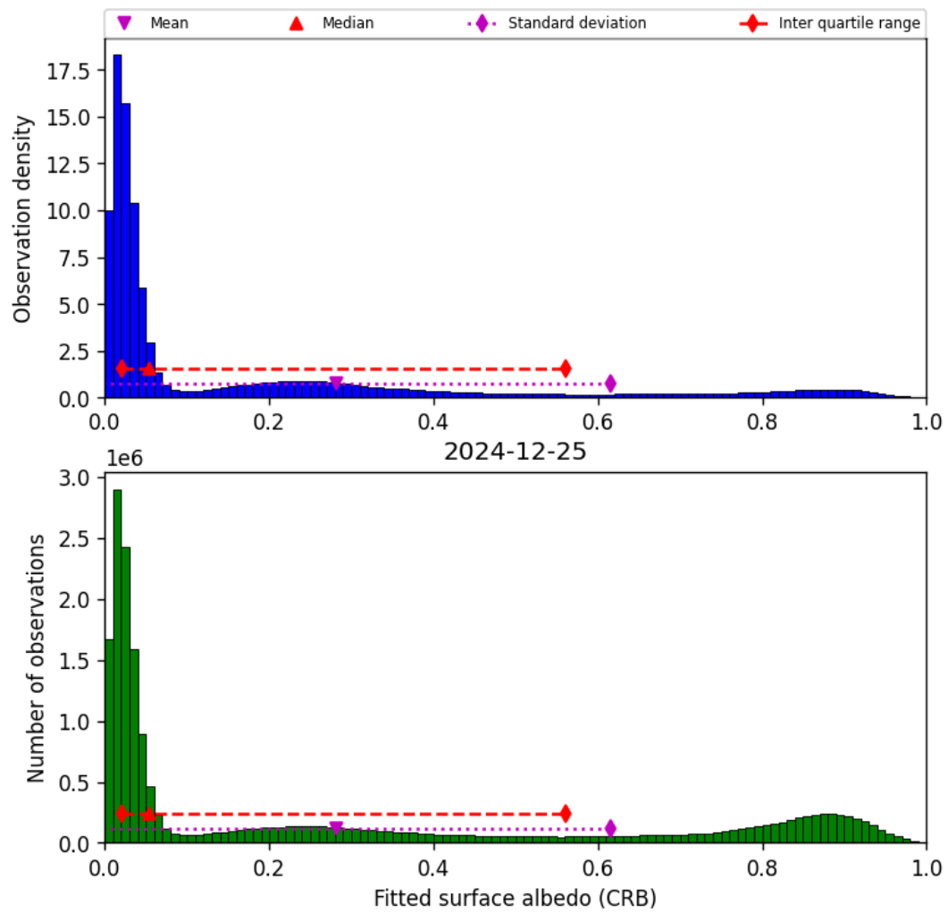
Figure 44: Histogram of “Fitted surface albedo (CRB)” for 2024-12-25 to 2024-12-25
