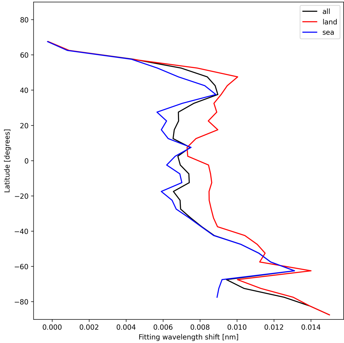
Figure 31: Zonal average of “Fitting wavelength shift” for 2024-12-25 to 2024-12-25.
