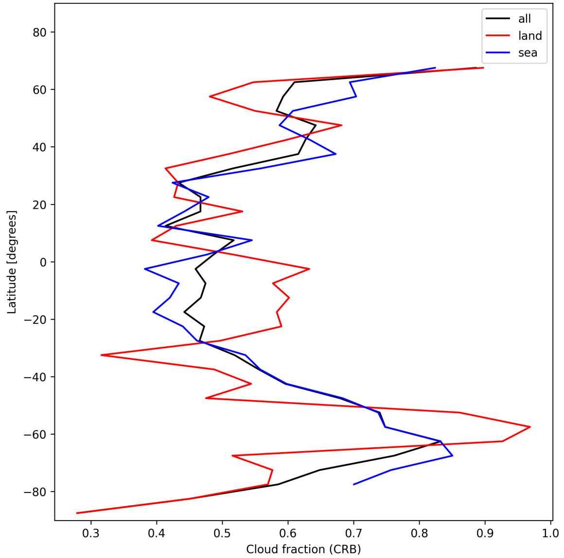
Figure 24: Zonal average of “Cloud fraction (CRB)” for 2024-12-25 to 2024-12-25.
