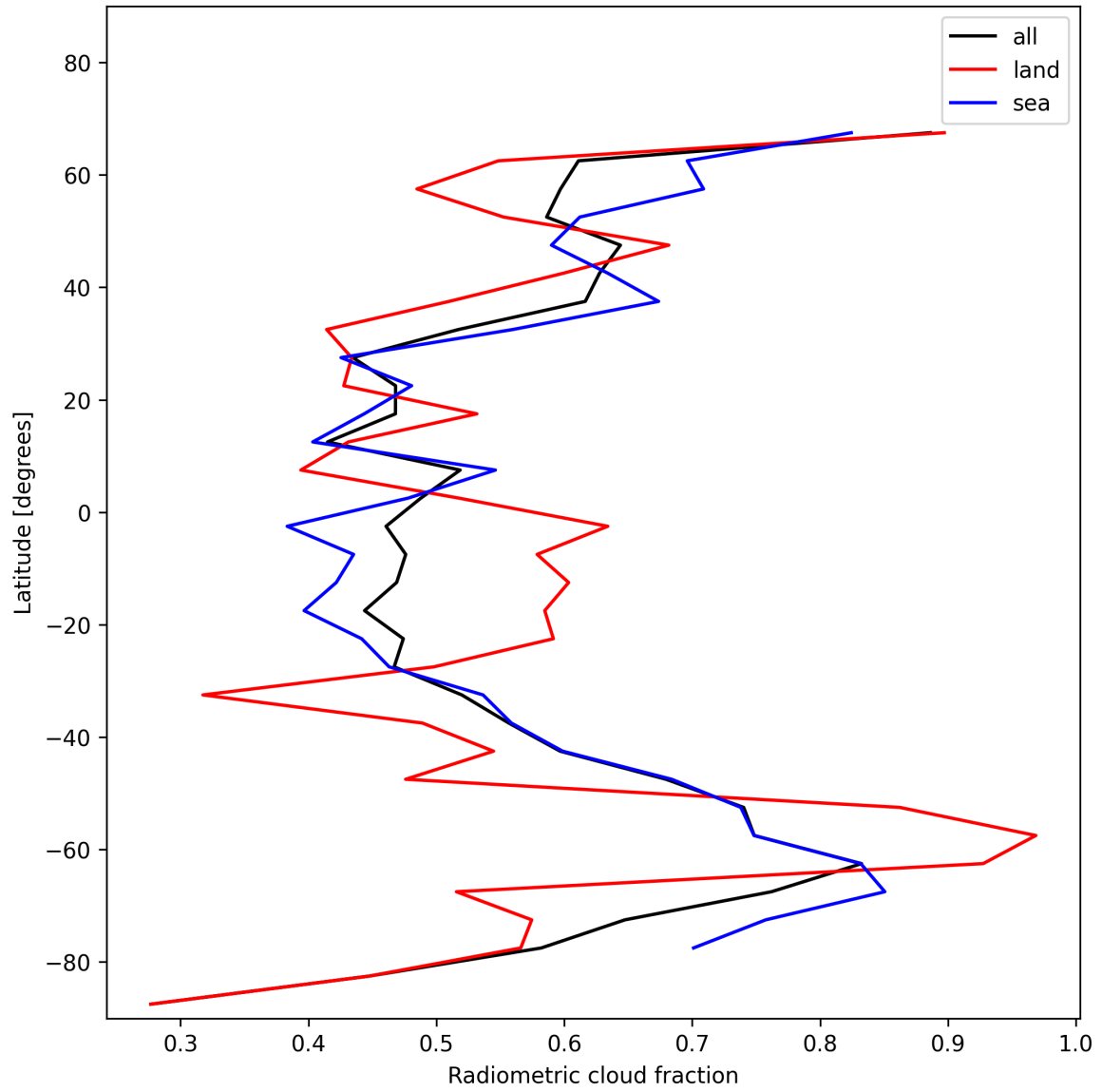
Figure 21: Zonal average of “Radiometric cloud fraction” for 2024-12-25 to 2024-12-25.
