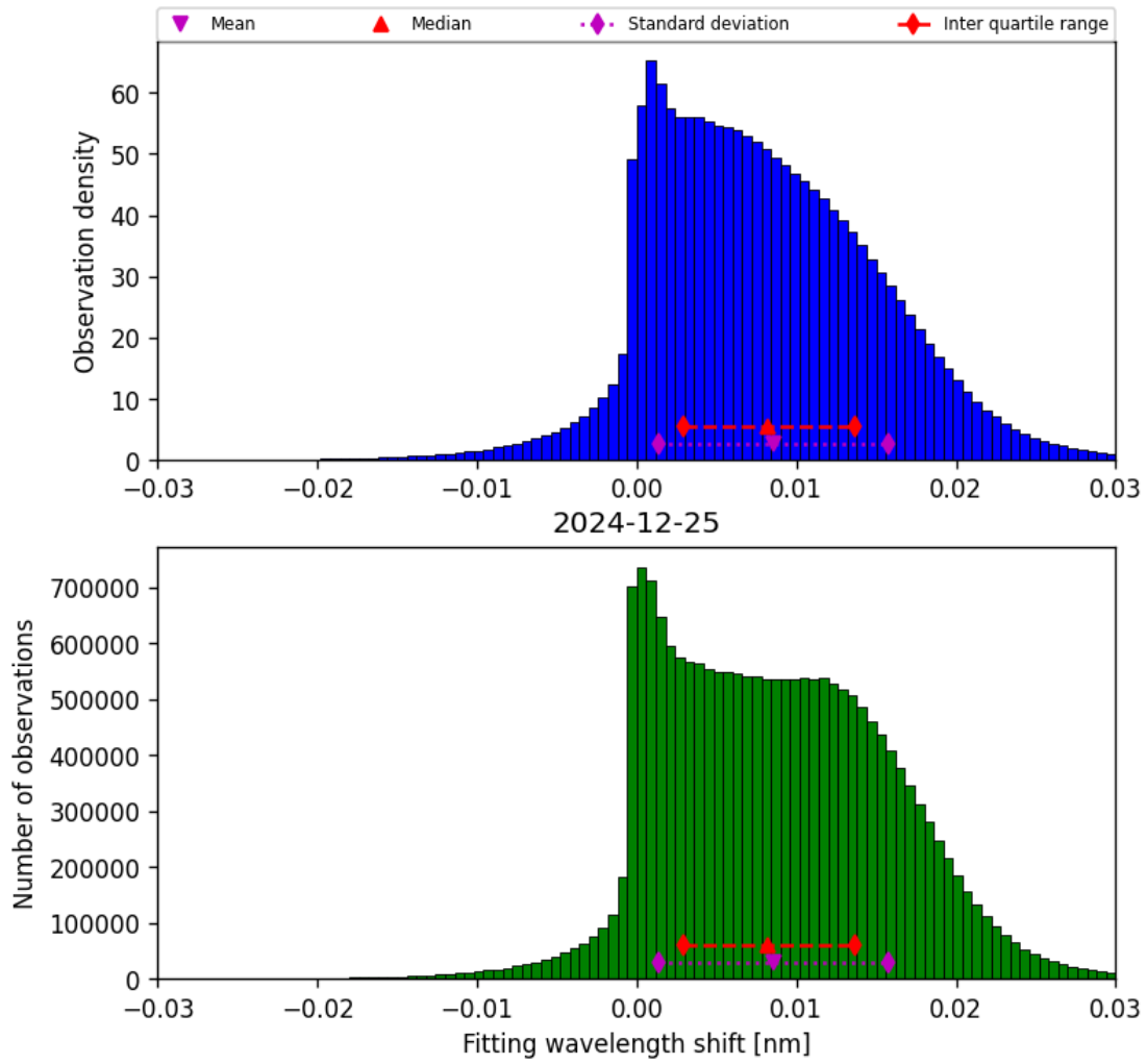
Figure 47: Histogram of “Fitting wavelength shift” for 2024-12-25 to 2024-12-25
