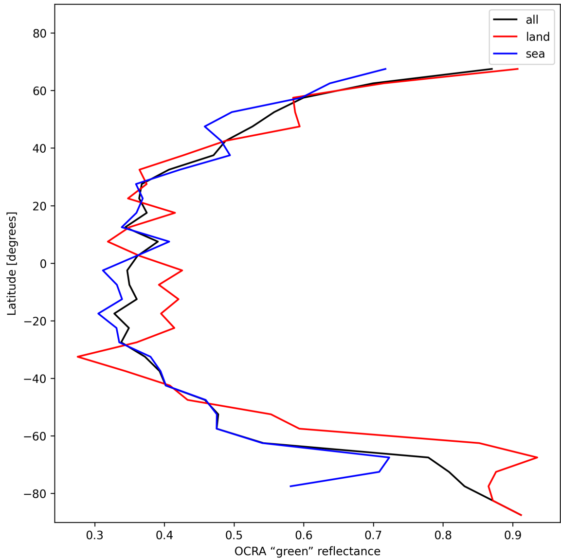
Figure 34: Zonal average of “OCRA “green” reflectance” for 2024-12-25 to 2024-12-25.
