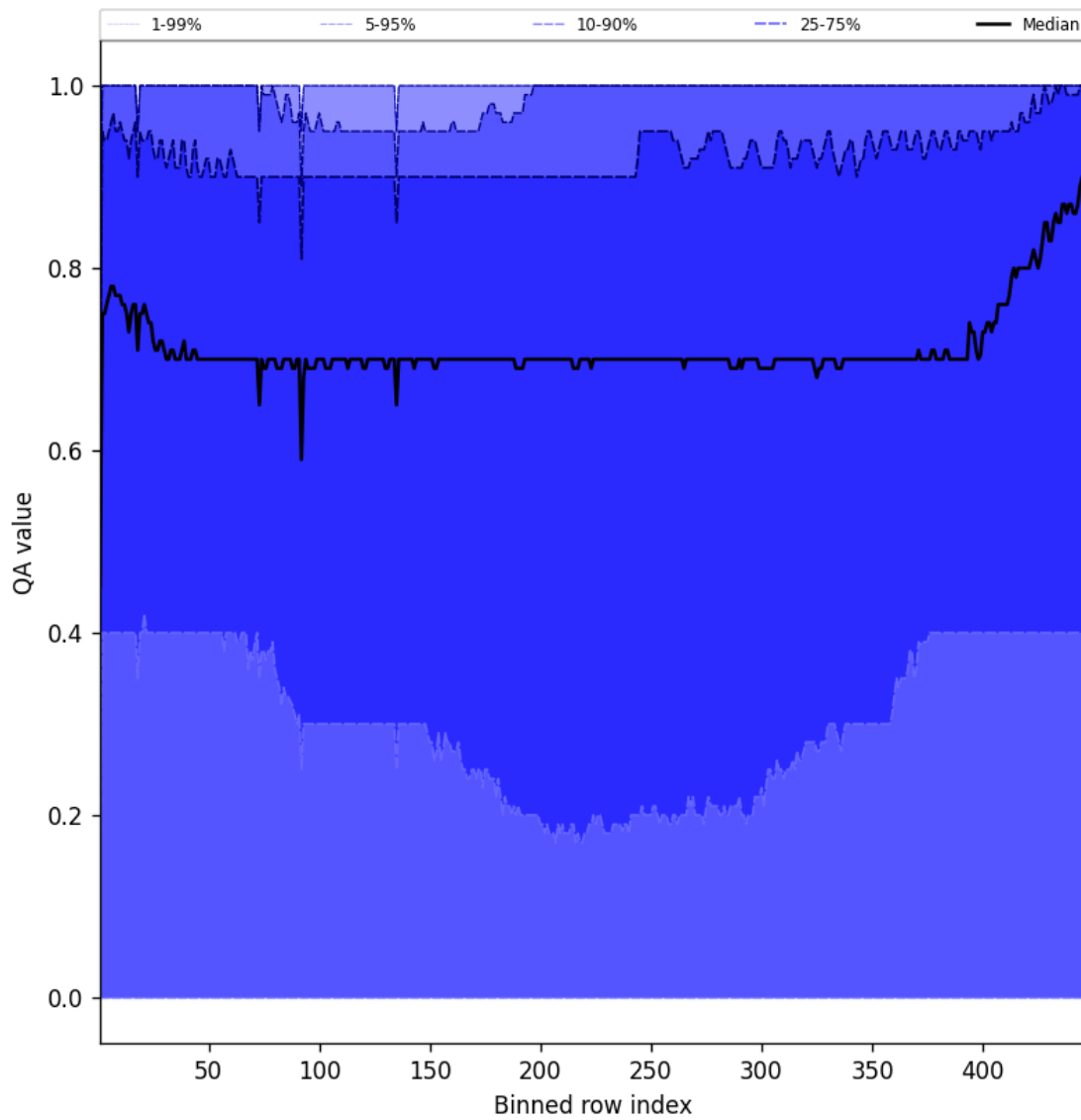
Figure 52: Along track statistics of “QA value” for 2024-12-25 to 2024-12-25
