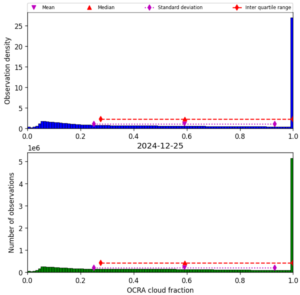
Figure 48: Histogram of “OCRA cloud fraction” for 2024-12-25 to 2024-12-25
