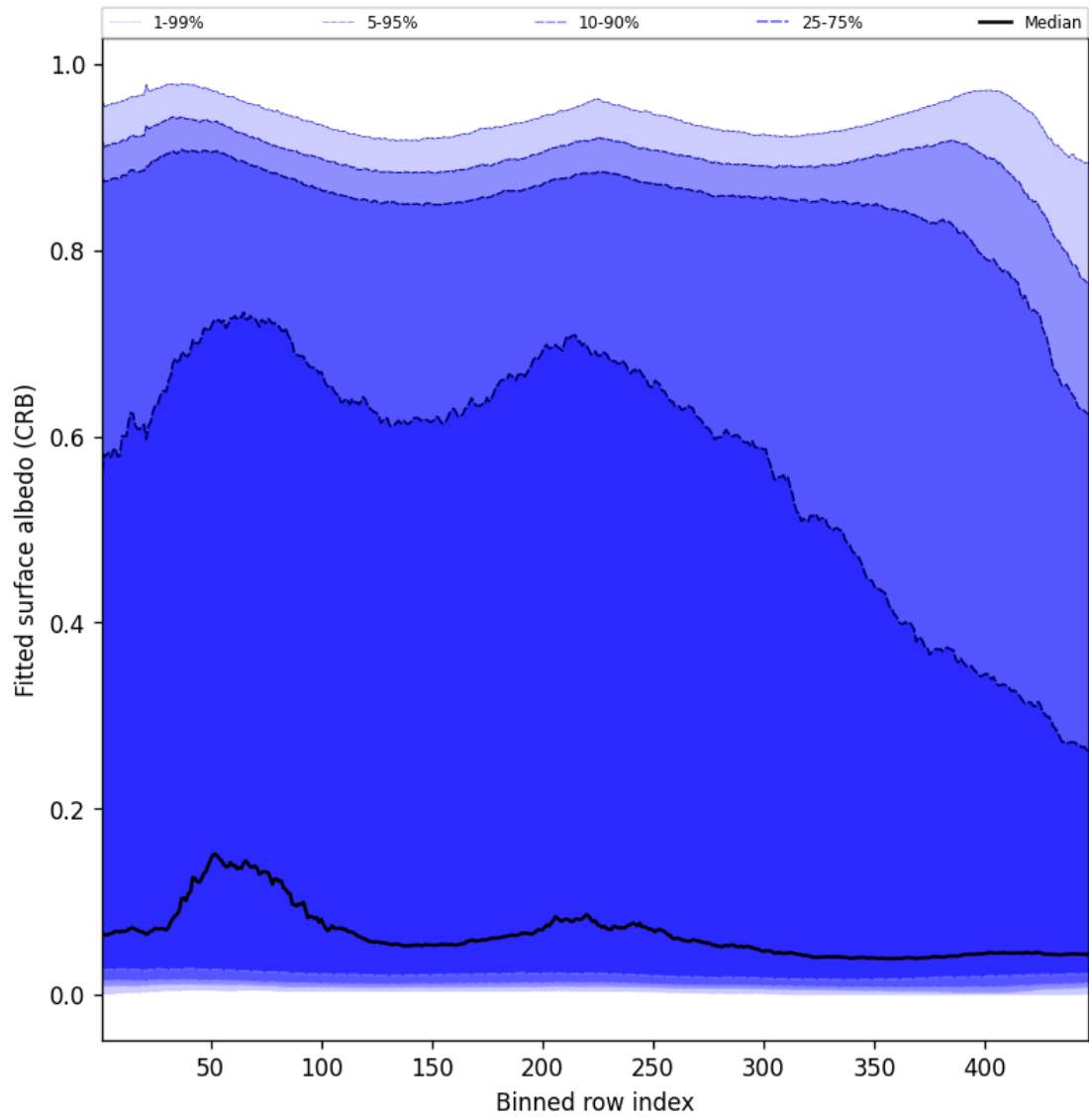
Figure 60: Along track statistics of “Fitted surface albedo (CRB)” for 2024-12-25 to 2024-12-25
