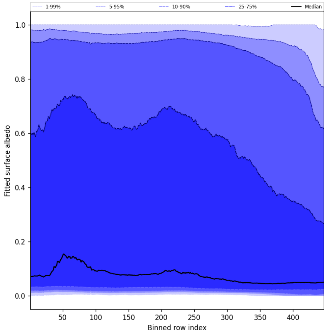
Figure 59: Along track statistics of “Fitted surface albedo” for 2024-12-25 to 2024-12-25
