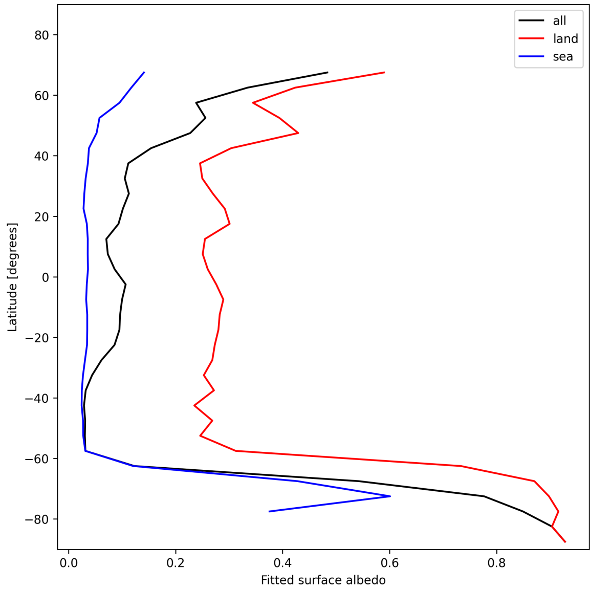
Figure 27: Zonal average of “Fitted surface albedo” for 2024-12-25 to 2024-12-25.
