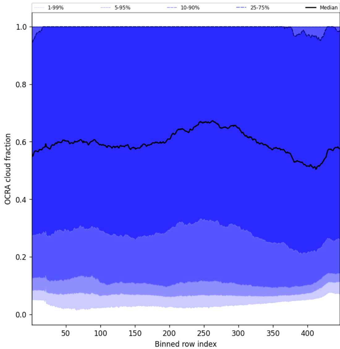
Figure 64: Along track statistics of “OCRA cloud fraction” for 2024-12-25 to 2024-12-25
