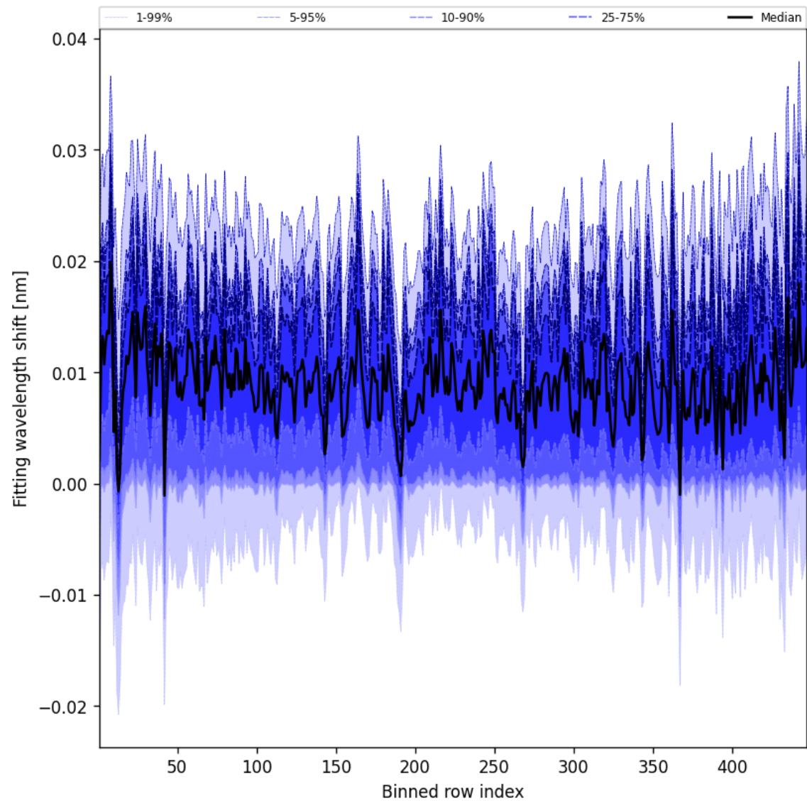
Figure 63: Along track statistics of “Fitting wavelength shift” for 2024-12-25 to 2024-12-25
