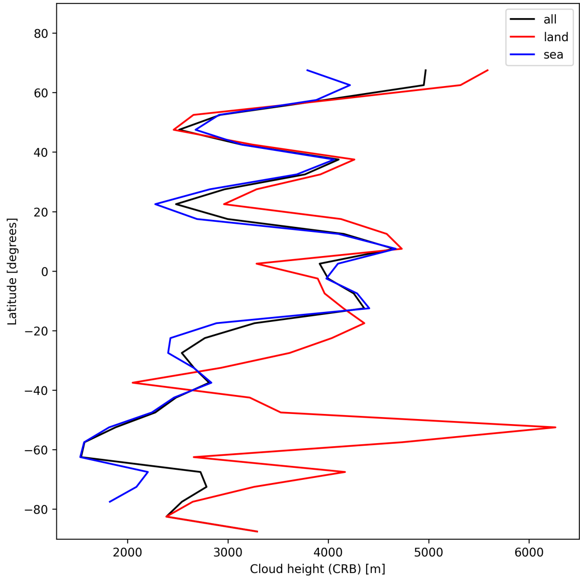
Figure 25: Zonal average of “Cloud height (CRB)” for 2024-12-25 to 2024-12-25.
