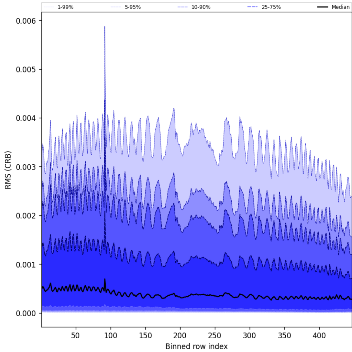
Figure 62: Along track statistics of “RMS (CRB)” for 2024-12-25 to 2024-12-25
