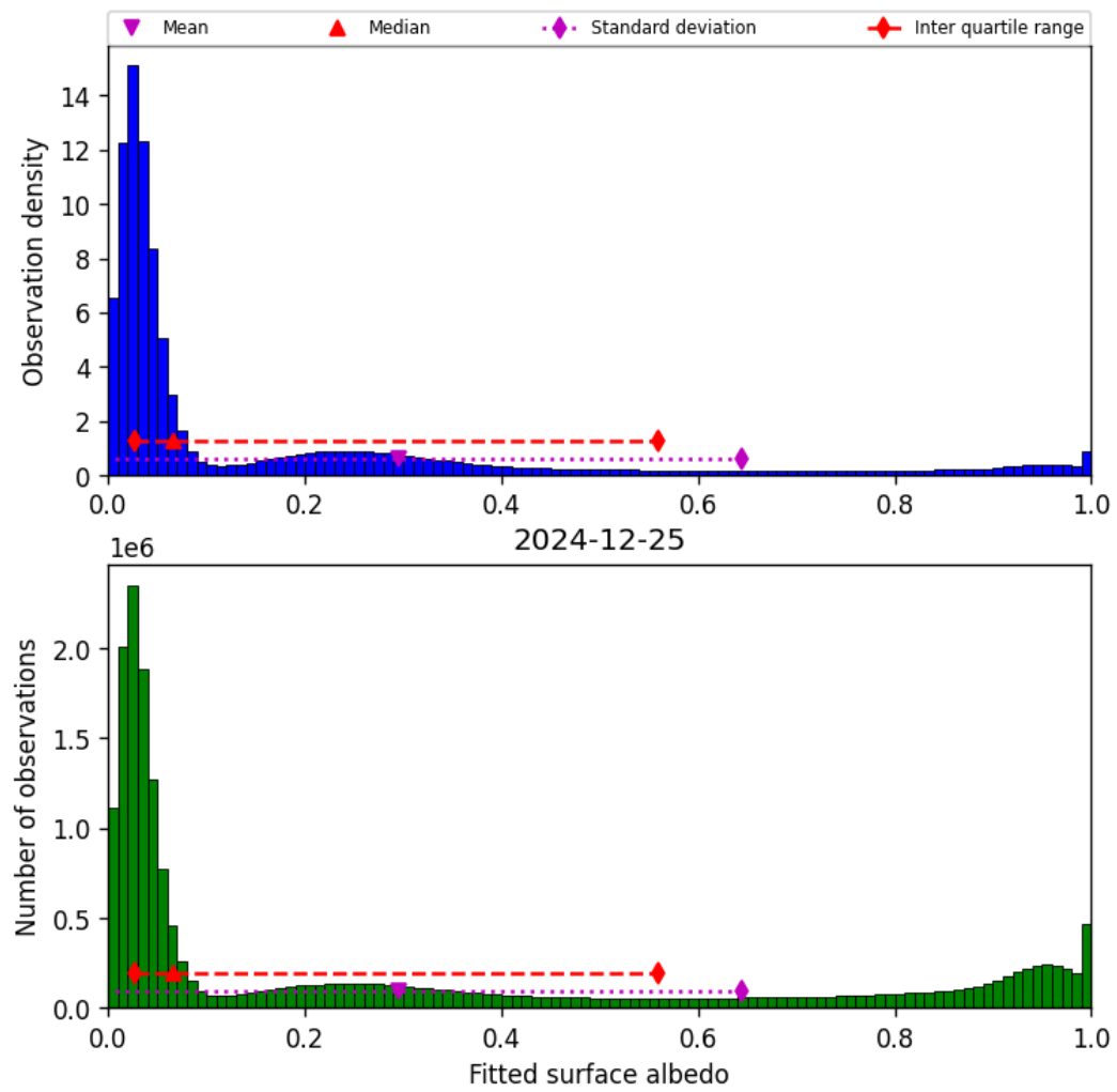
Figure 43: Histogram of “Fitted surface albedo” for 2024-12-25 to 2024-12-25
