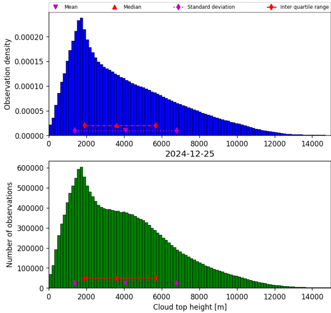
Figure 38: Histogram of “Cloud top height” for 2024-12-25 to 2024-12-25
