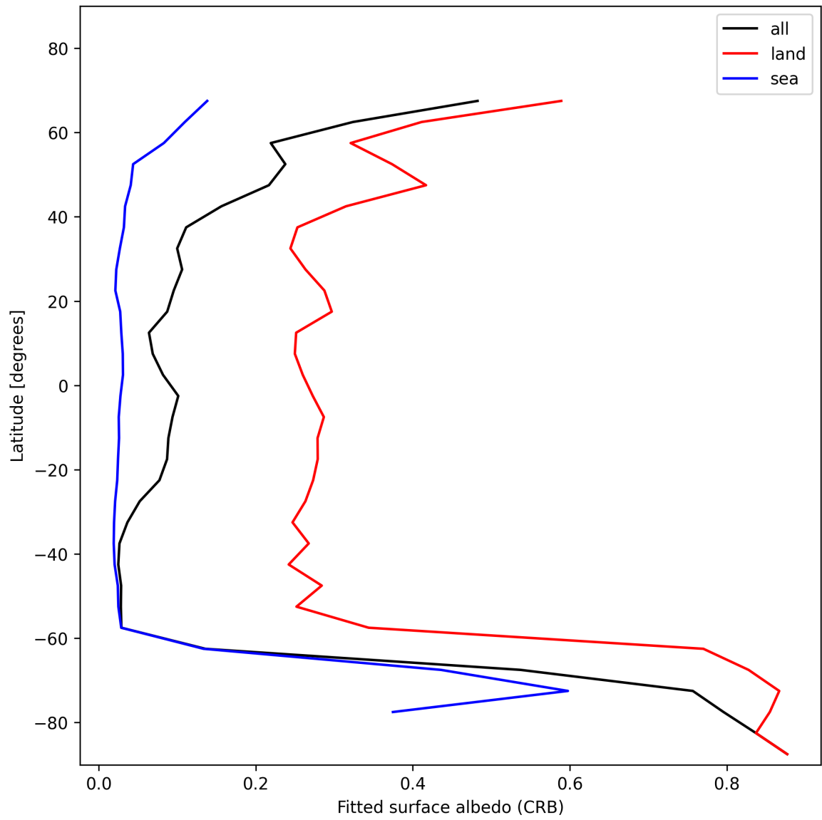
Figure 28: Zonal average of “Fitted surface albedo (CRB)” for 2024-12-25 to 2024-12-25.
