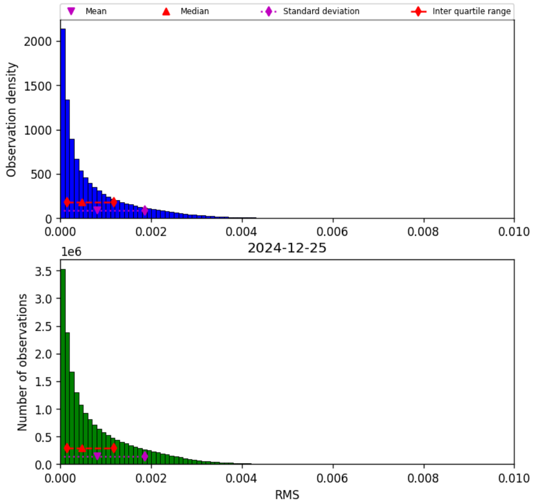
Figure 45: Histogram of “RMS” for 2024-12-25 to 2024-12-25
