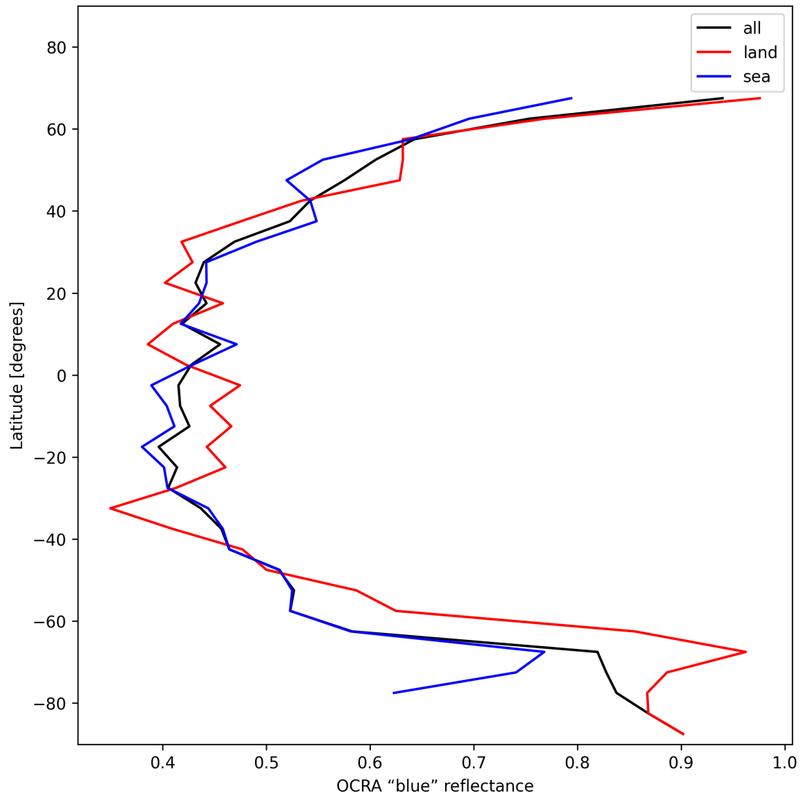
Figure 33: Zonal average of “OCRA “blue” reflectance” for 2024-12-25 to 2024-12-25.
