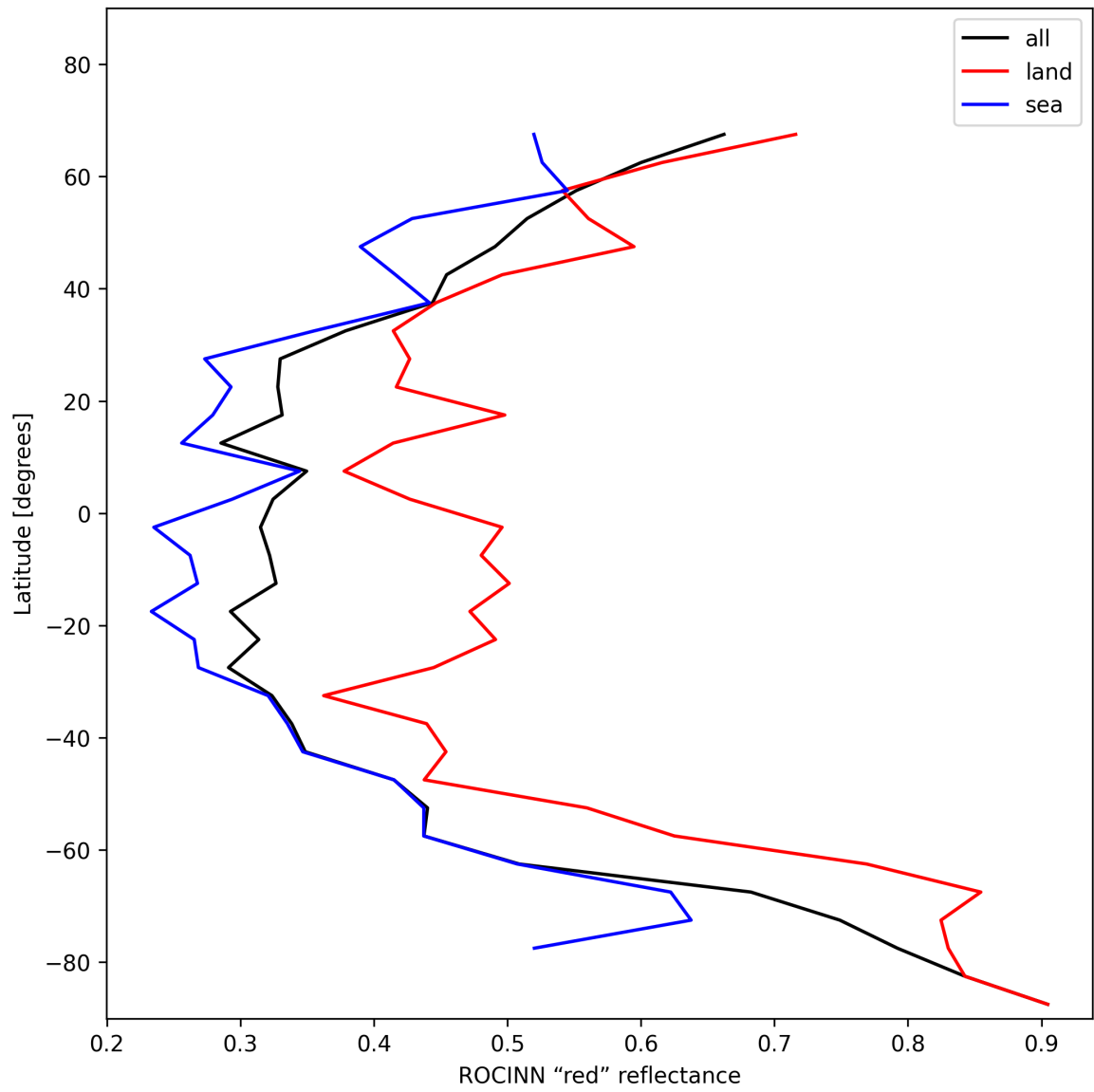
Figure 35: Zonal average of “ROCINN “red” reflectance” for 2024-12-25 to 2024-12-25.
