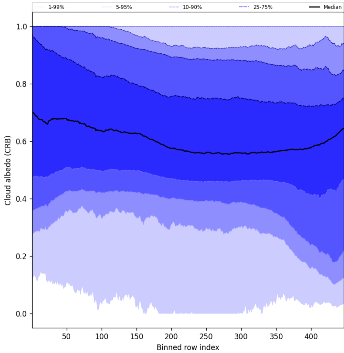
Figure 58: Along track statistics of “Cloud albedo (CRB)” for 2024-12-25 to 2024-12-25
