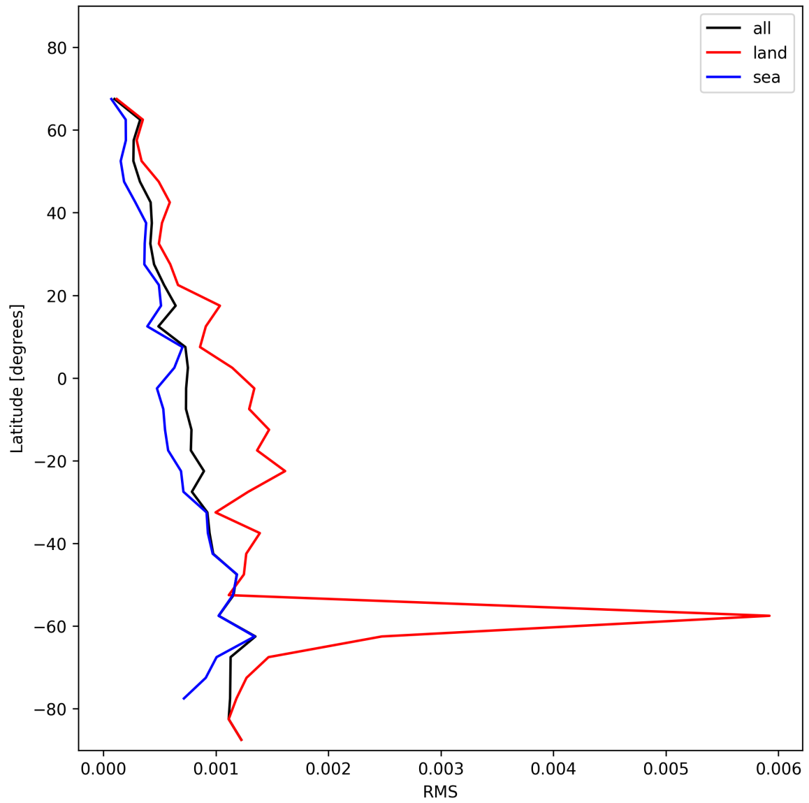
Figure 29: Zonal average of “RMS” for 2024-12-25 to 2024-12-25.
