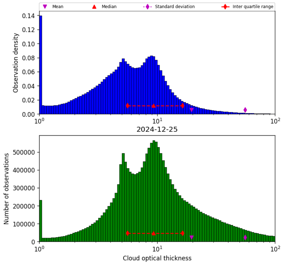
Figure 39: Histogram of “Cloud optical thickness” for 2024-12-25 to 2024-12-25
