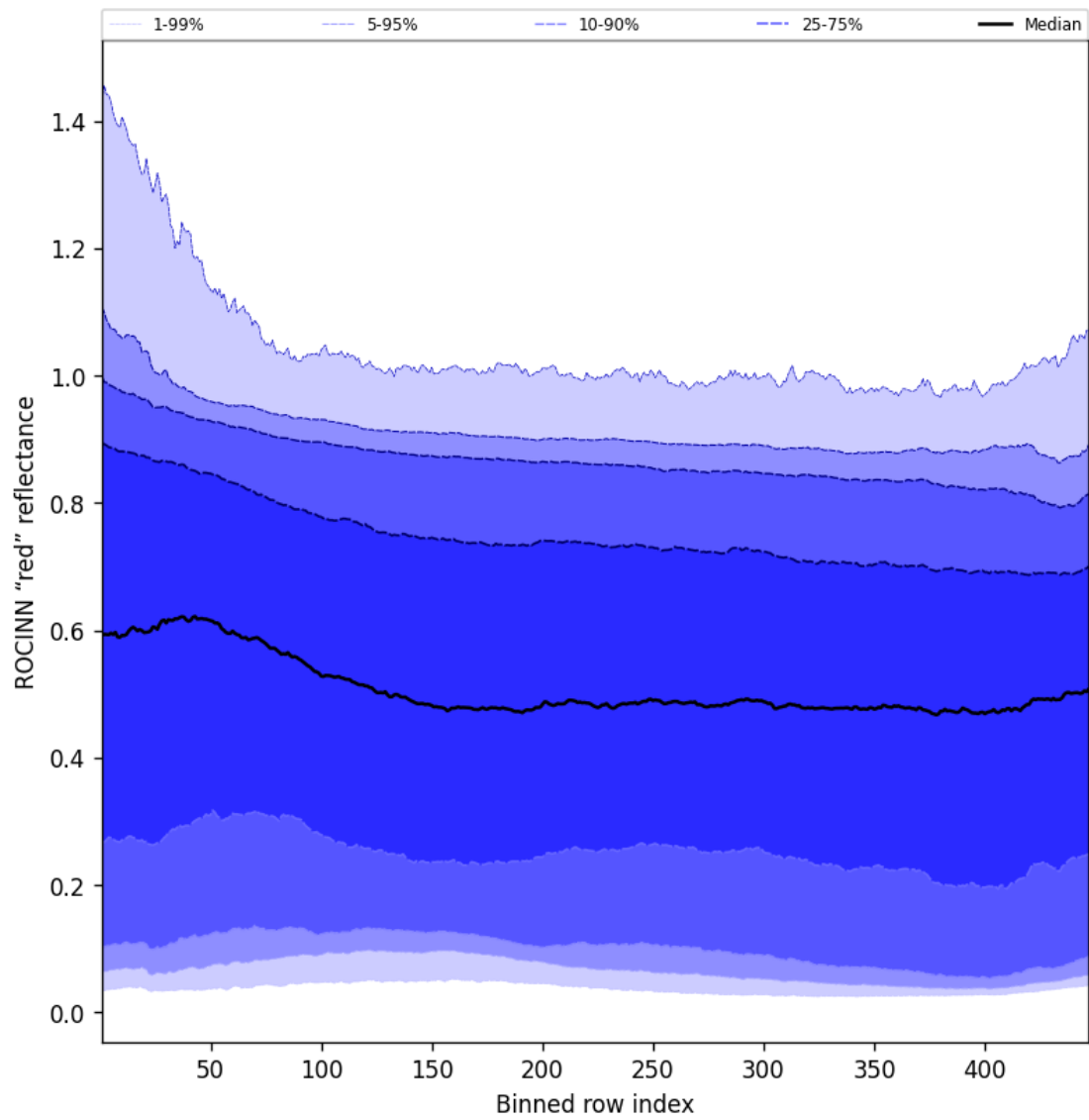
Figure 67: Along track statistics of “ROCINN “red” reflectance” for 2024-12-25 to 2024-12-25
