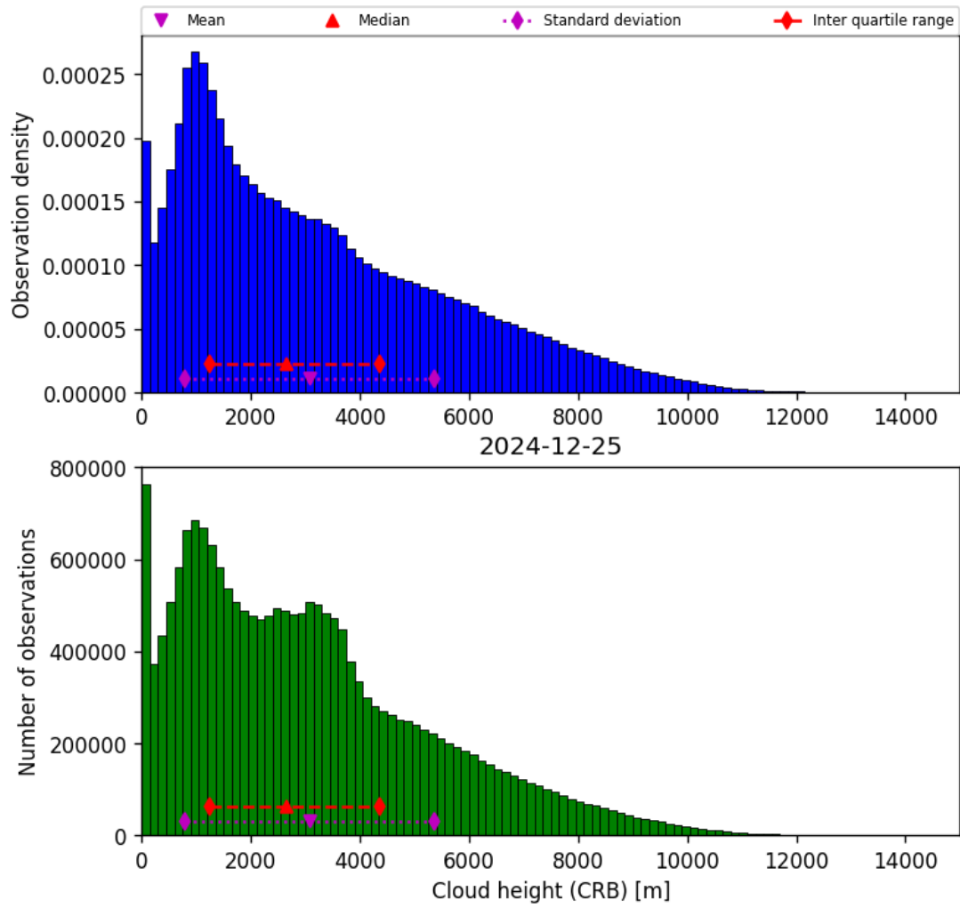
Figure 41: Histogram of “Cloud height (CRB)” for 2024-12-25 to 2024-12-25
