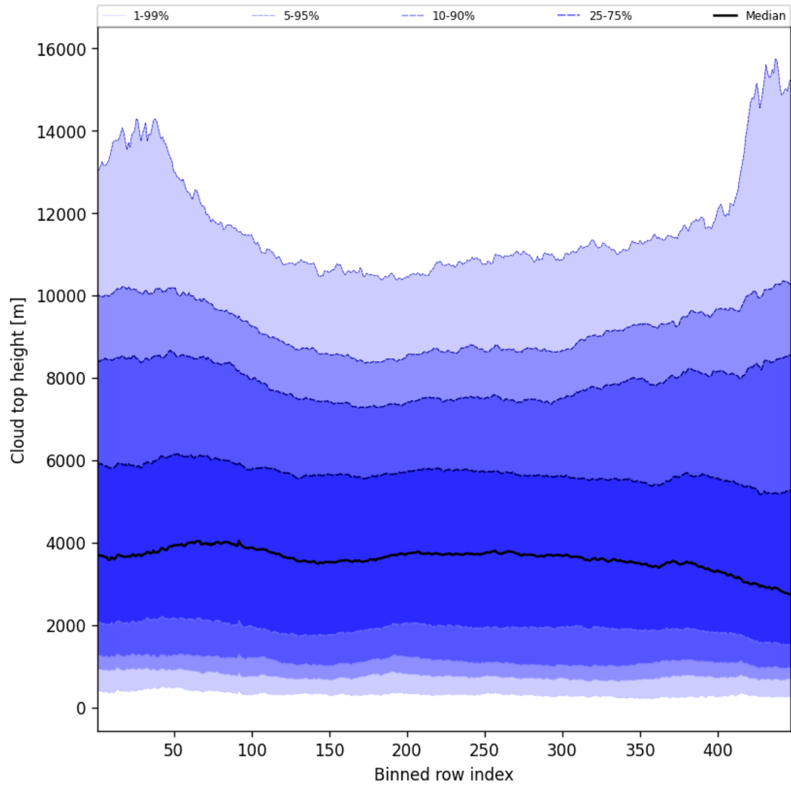
Figure 54: Along track statistics of “Cloud top height” for 2024-12-25 to 2024-12-25
