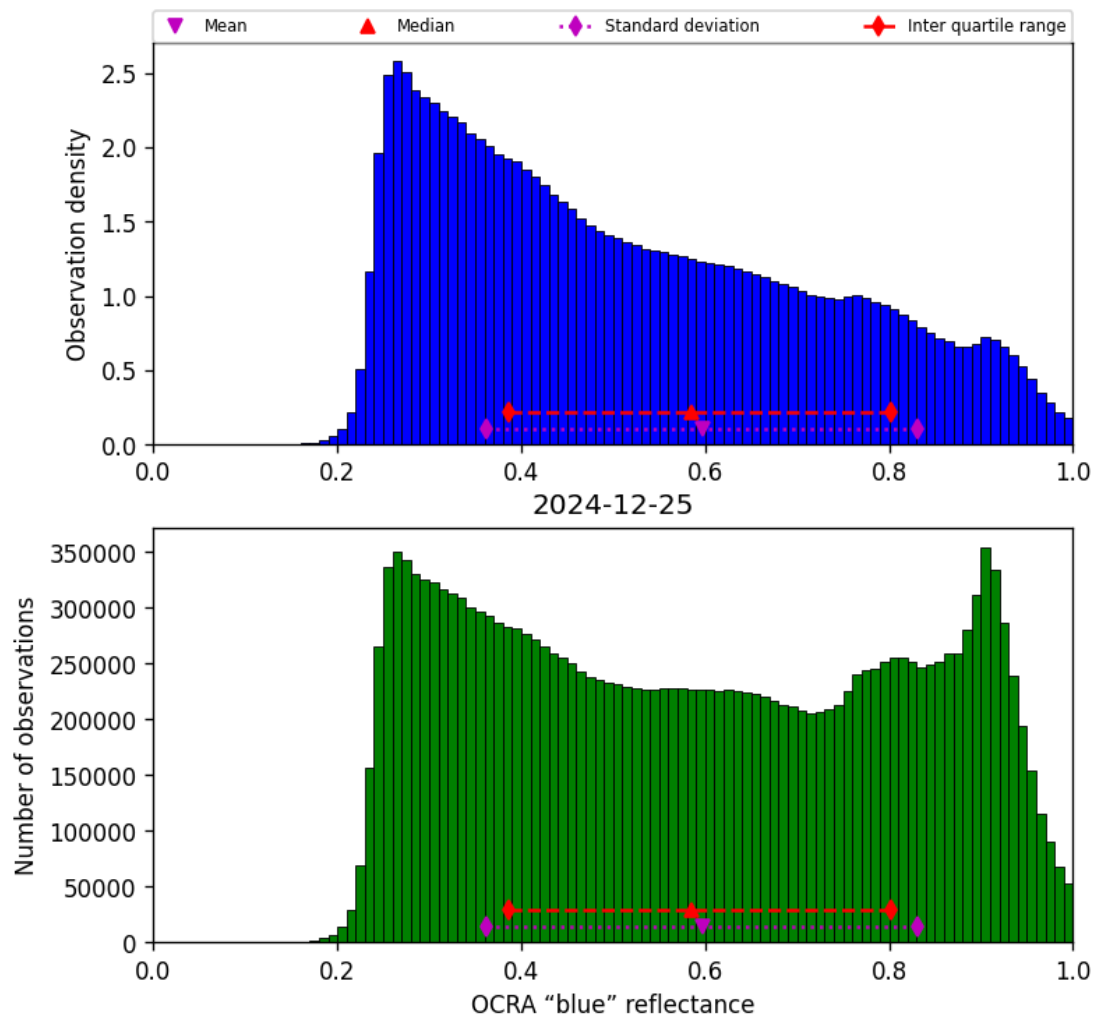
Figure 49: Histogram of “OCRA “blue” reflectance” for 2024-12-25 to 2024-12-25
