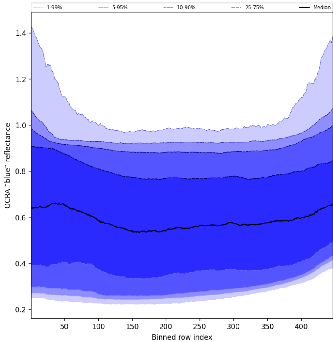
Figure 65: Along track statistics of “OCRA “blue” reflectance” for 2024-12-25 to 2024-12-25
