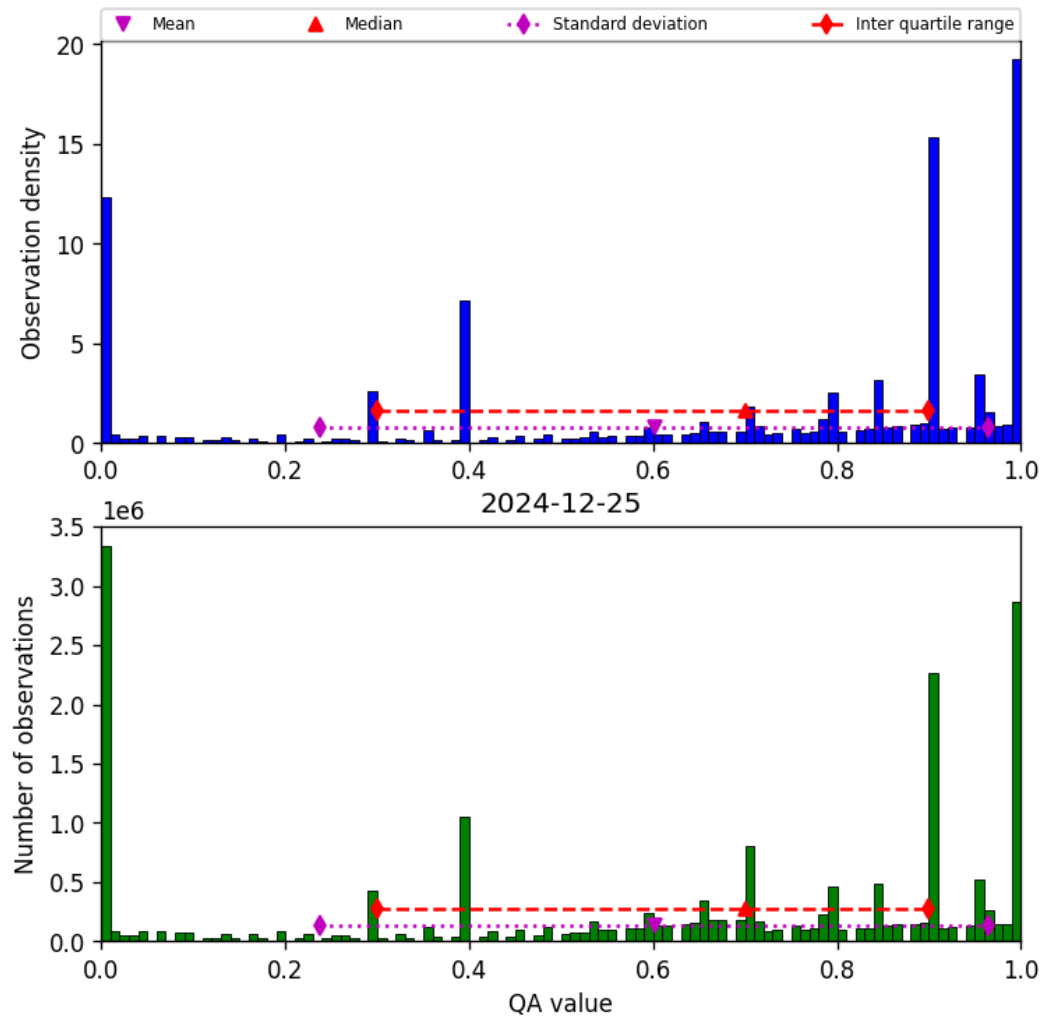
Figure 36: Histogram of “QA value” for 2024-12-25 to 2024-12-25
