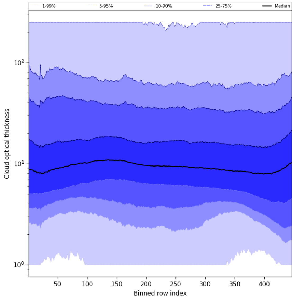
Figure 55: Along track statistics of “Cloud optical thickness” for 2024-12-25 to 2024-12-25
