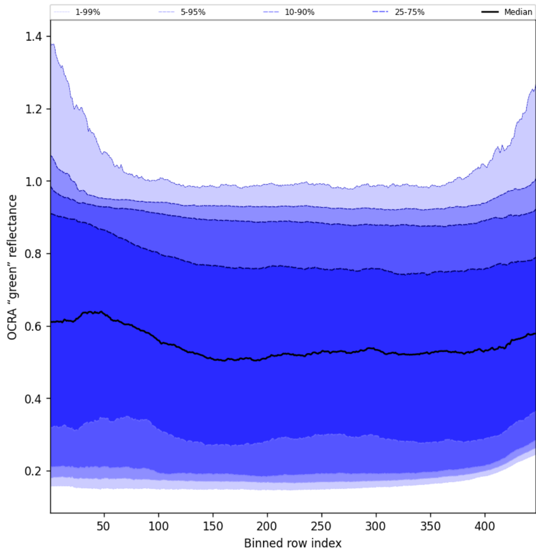
Figure 66: Along track statistics of “OCRA “green” reflectance” for 2024-12-25 to 2024-12-25
