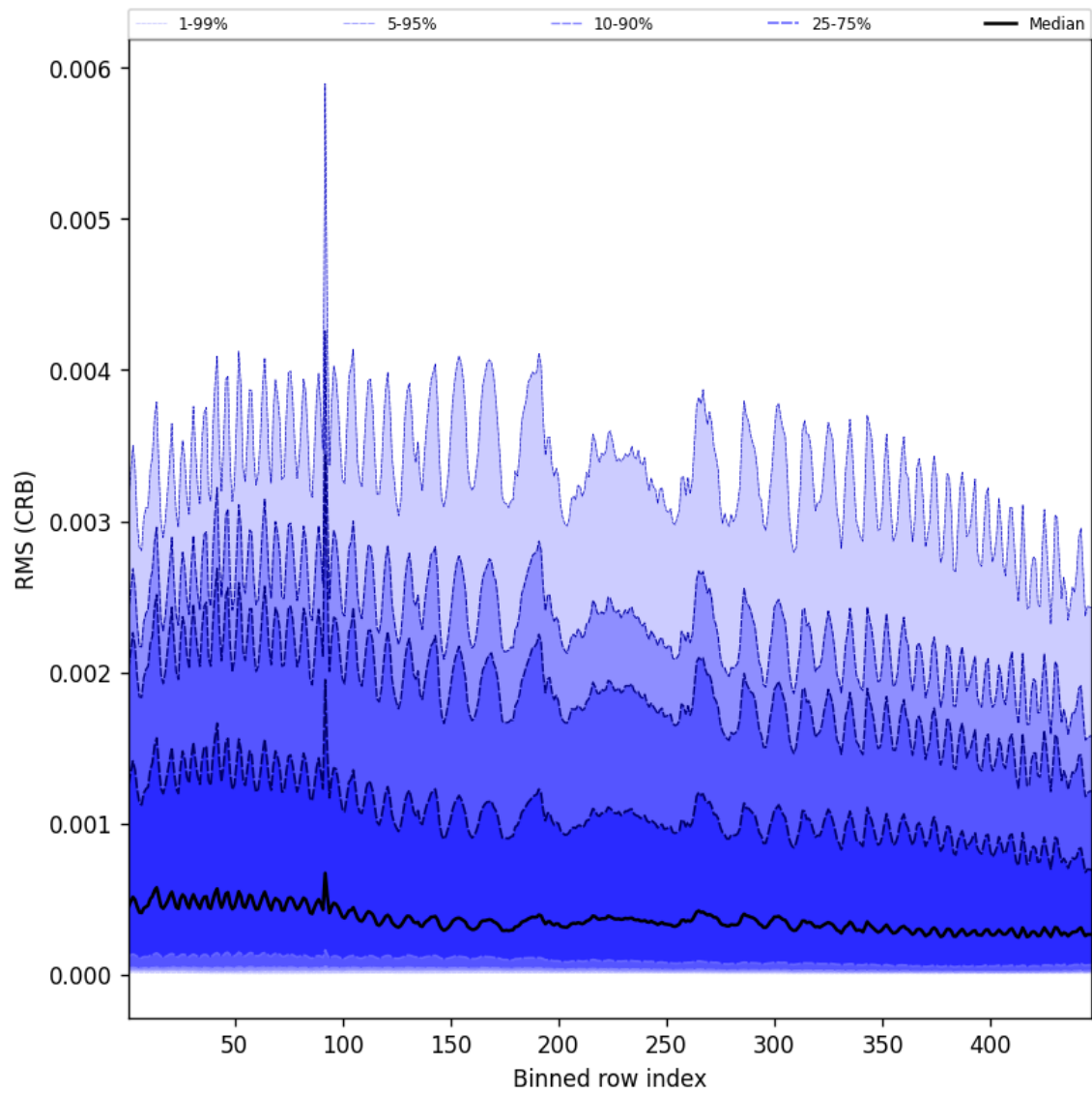
Figure 62: Along track statistics of “RMS (CRB)” for 2024-12-26 to 2024-12-27
