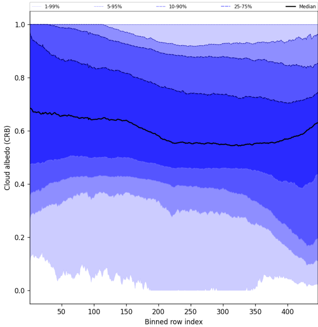
Figure 58: Along track statistics of “Cloud albedo (CRB)” for 2024-12-26 to 2024-12-27
