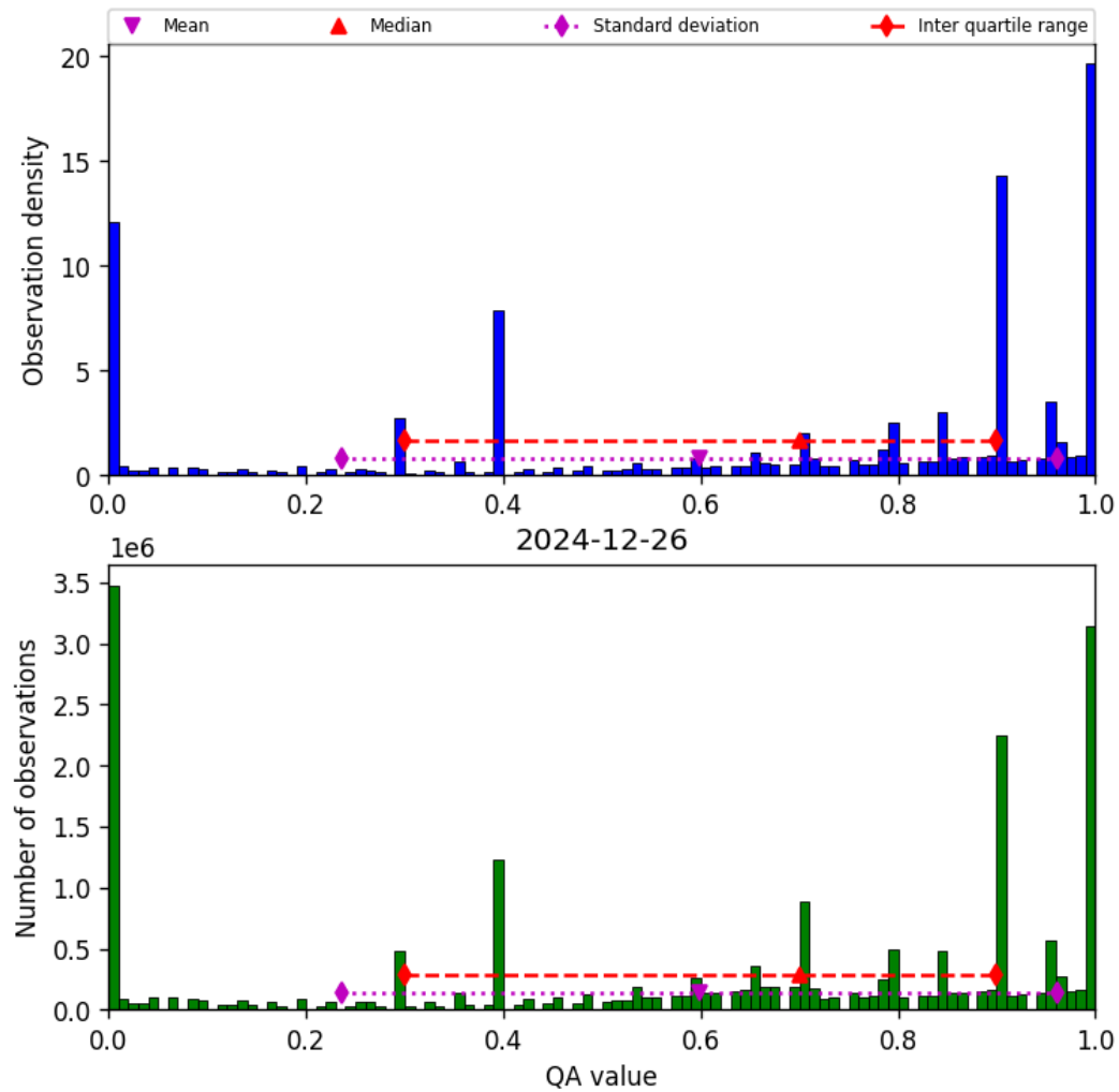
Figure 36: Histogram of “QA value” for 2024-12-26 to 2024-12-27
