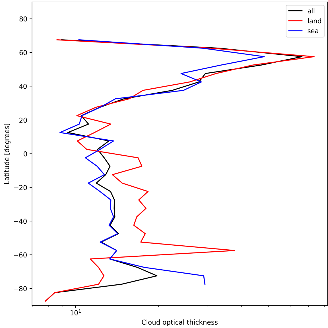
Figure 23: Zonal average of “Cloud optical thickness” for 2024-12-26 to 2024-12-27.
