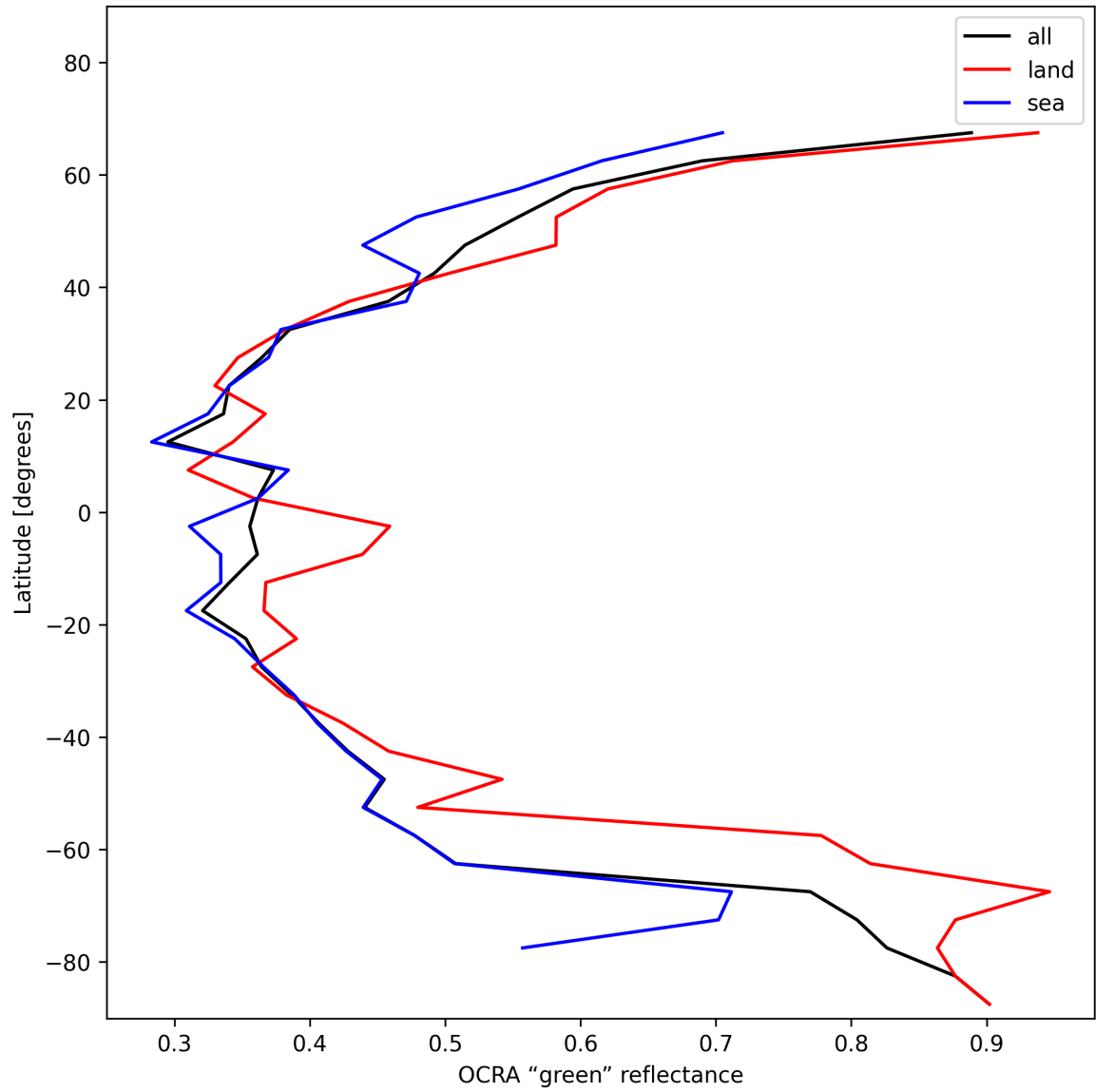
Figure 34: Zonal average of “OCRA “green” reflectance” for 2024-12-26 to 2024-12-27.
