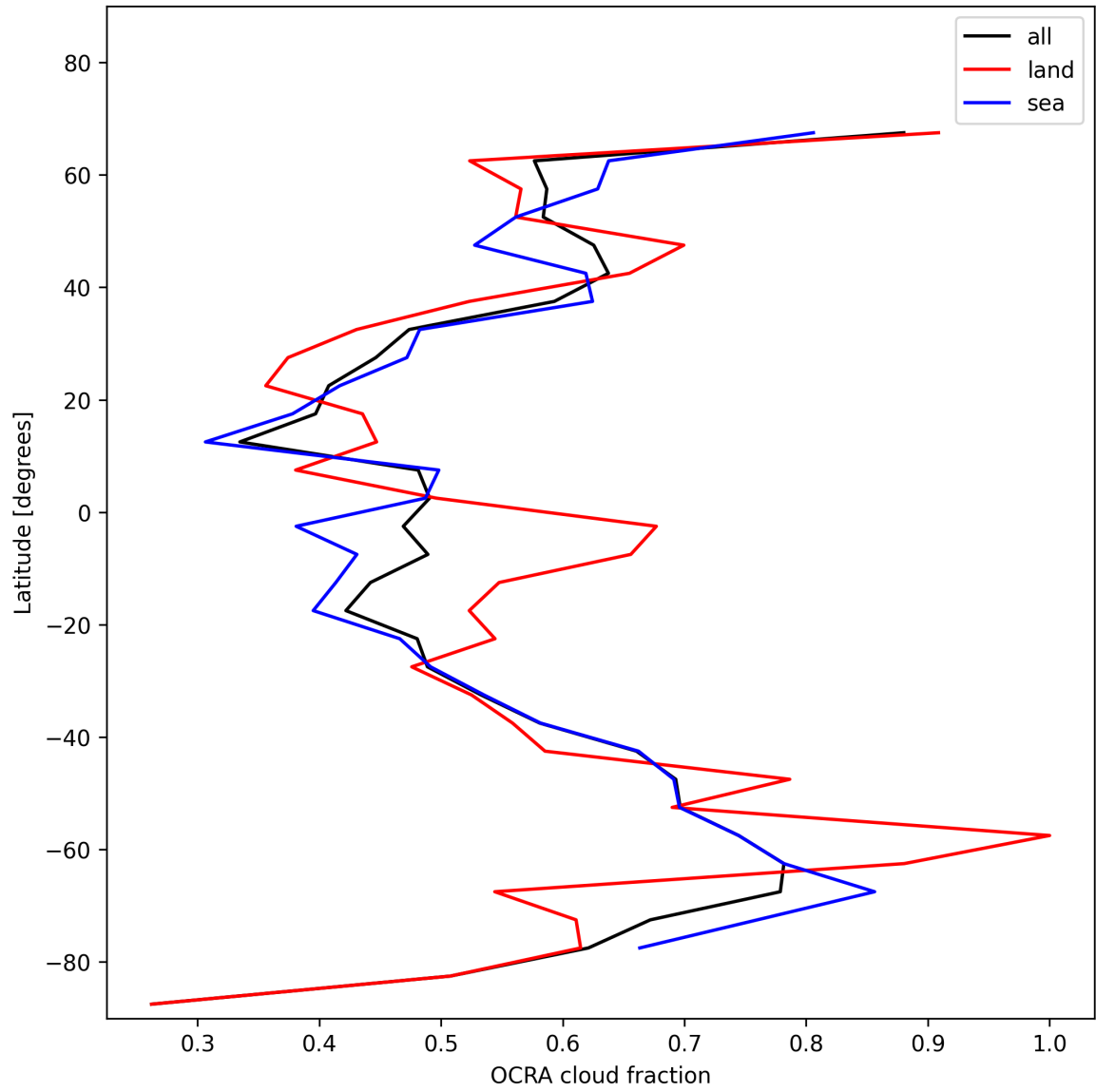
Figure 32: Zonal average of “OCRA cloud fraction” for 2024-12-26 to 2024-12-27.
