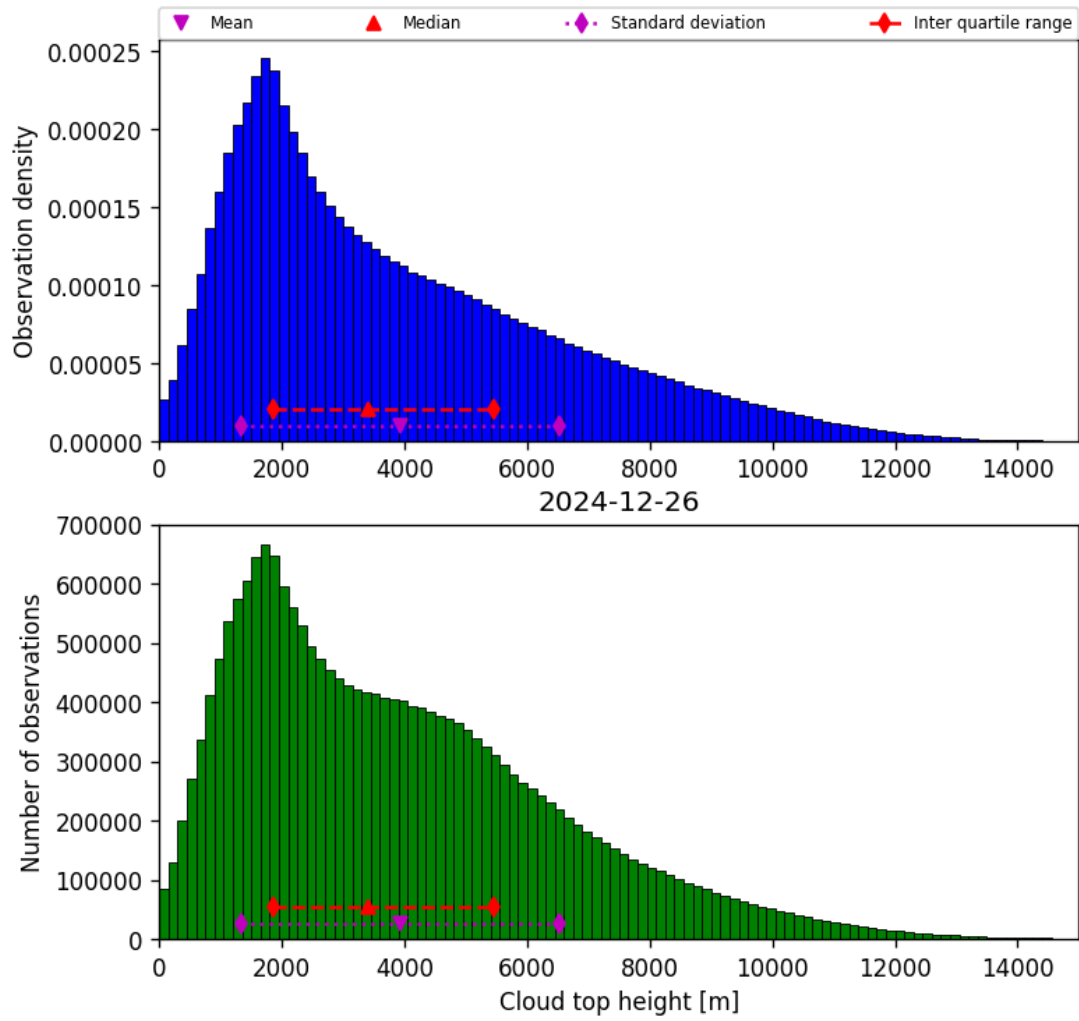
Figure 38: Histogram of “Cloud top height” for 2024-12-26 to 2024-12-27
