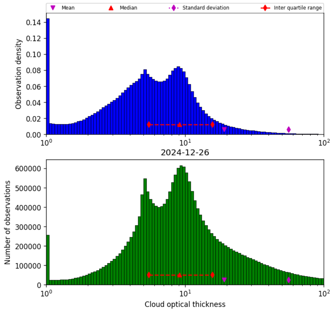
Figure 39: Histogram of “Cloud optical thickness” for 2024-12-26 to 2024-12-27
