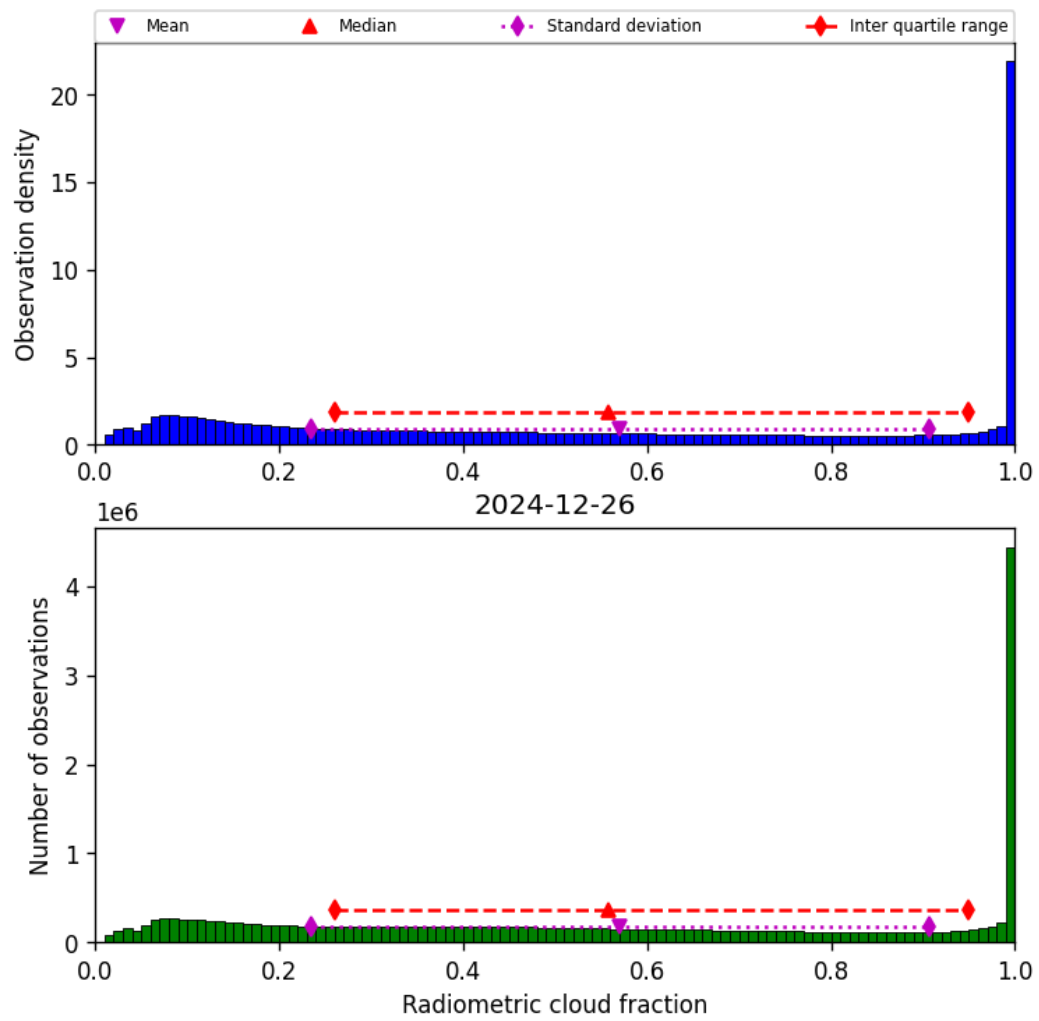
Figure 37: Histogram of “Radiometric cloud fraction” for 2024-12-26 to 2024-12-27
