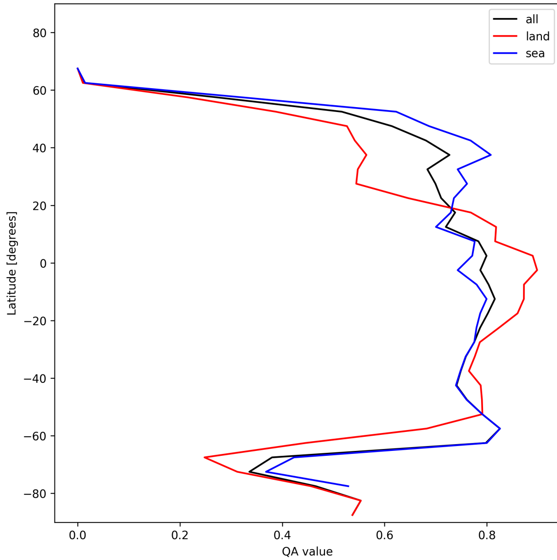
Figure 20: Zonal average of “QA value” for 2024-12-26 to 2024-12-27.
