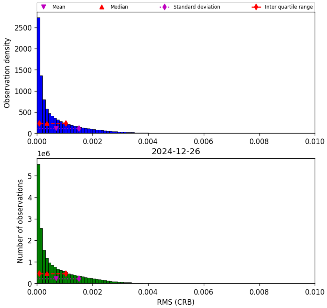
Figure 46: Histogram of “RMS (CRB)” for 2024-12-26 to 2024-12-27
