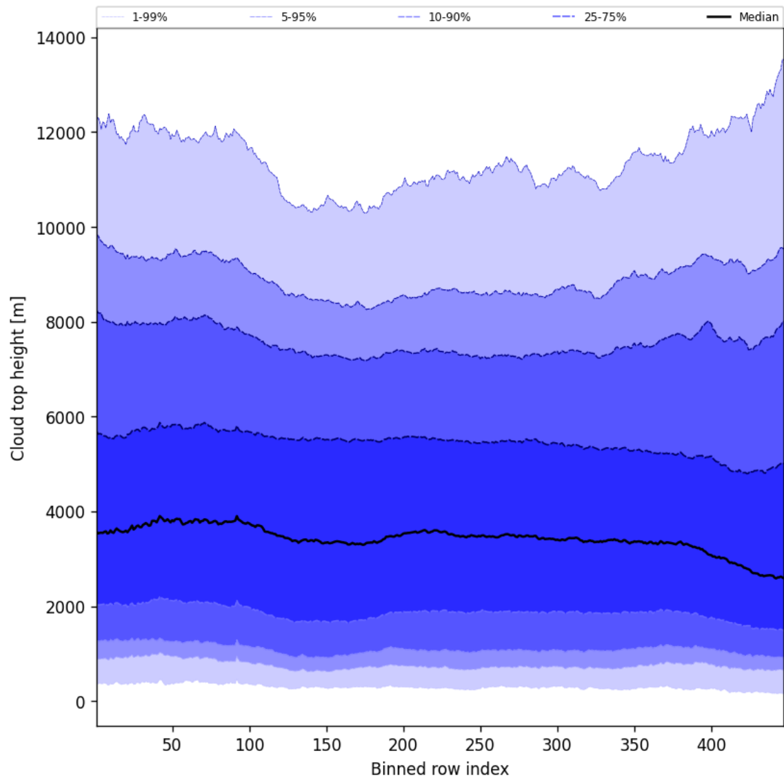
Figure 54: Along track statistics of “Cloud top height” for 2024-12-26 to 2024-12-27
