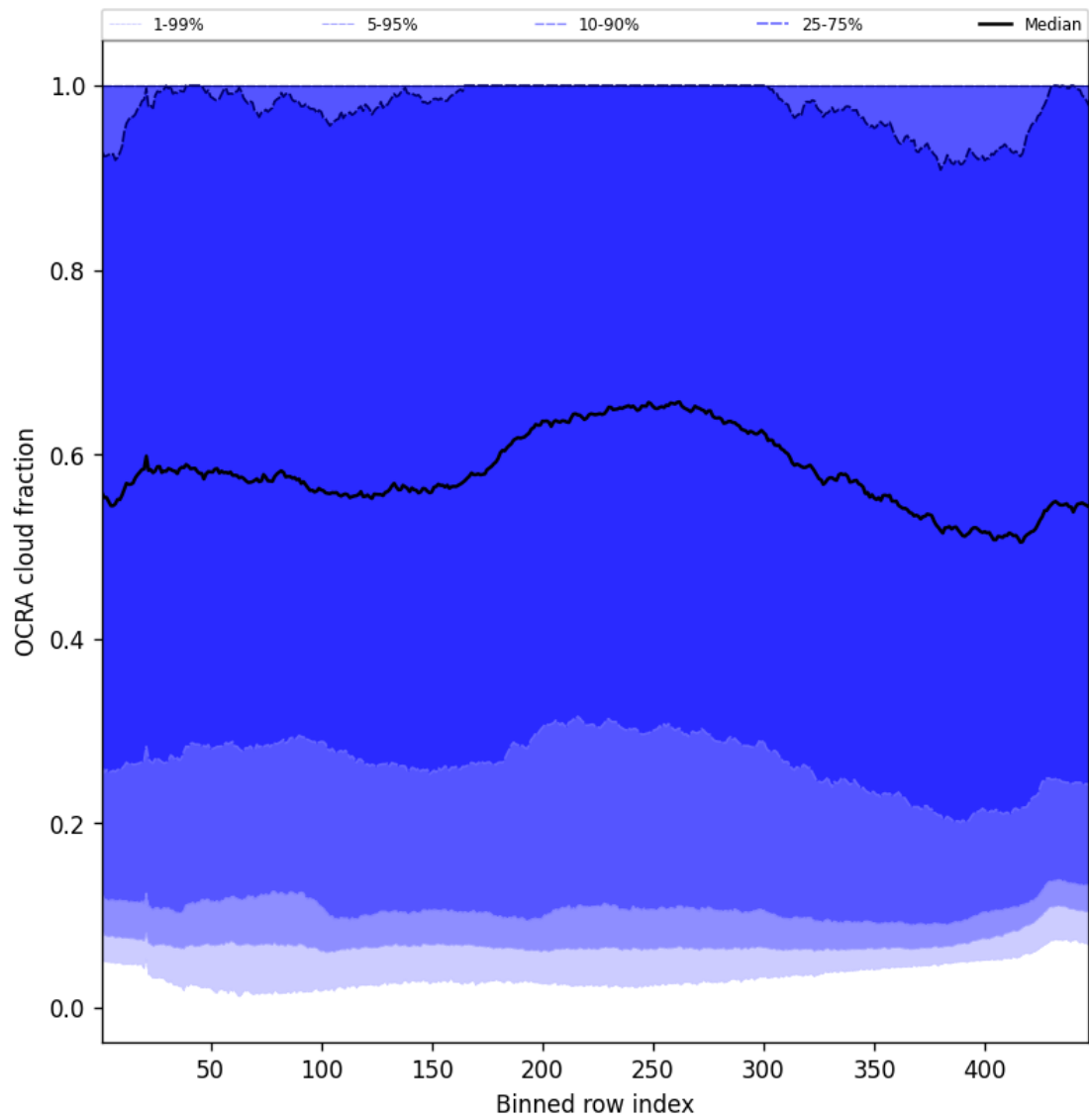
Figure 64: Along track statistics of “OCRA cloud fraction” for 2024-12-26 to 2024-12-27
