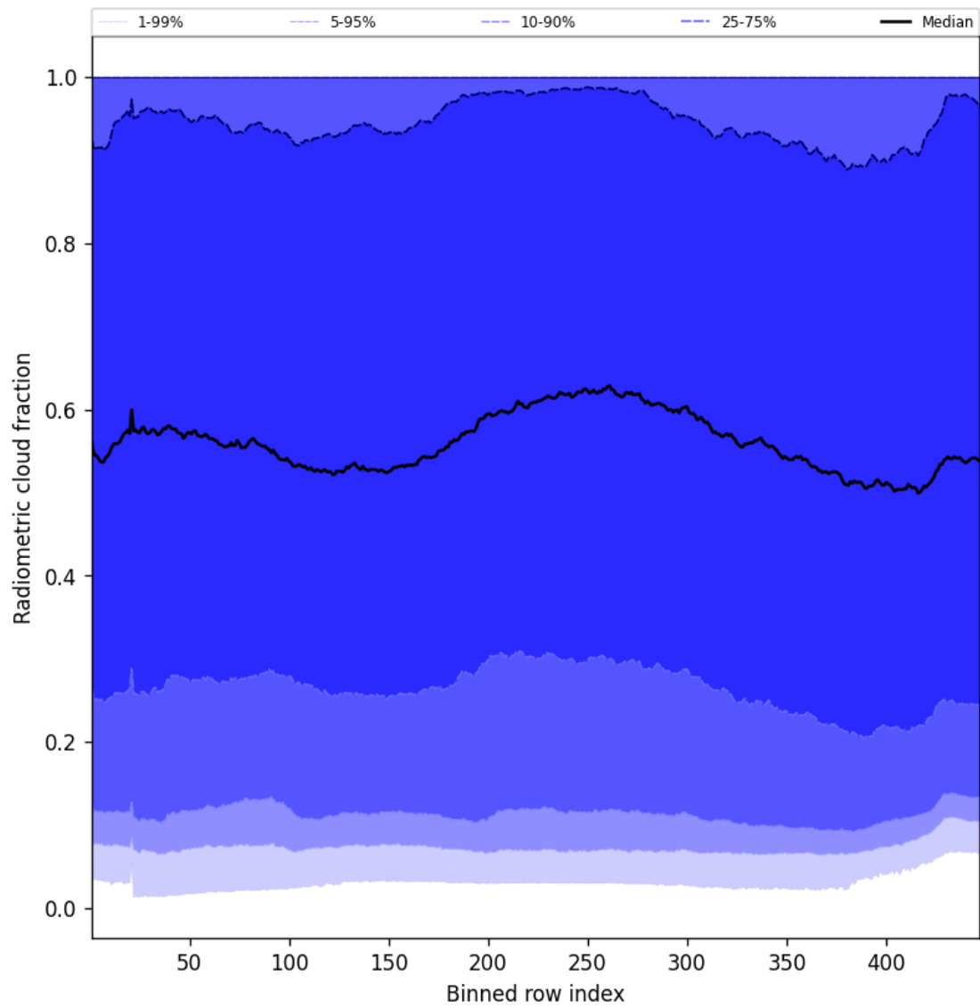
Figure 53: Along track statistics of “Radiometric cloud fraction” for 2024-12-26 to 2024-12-27
