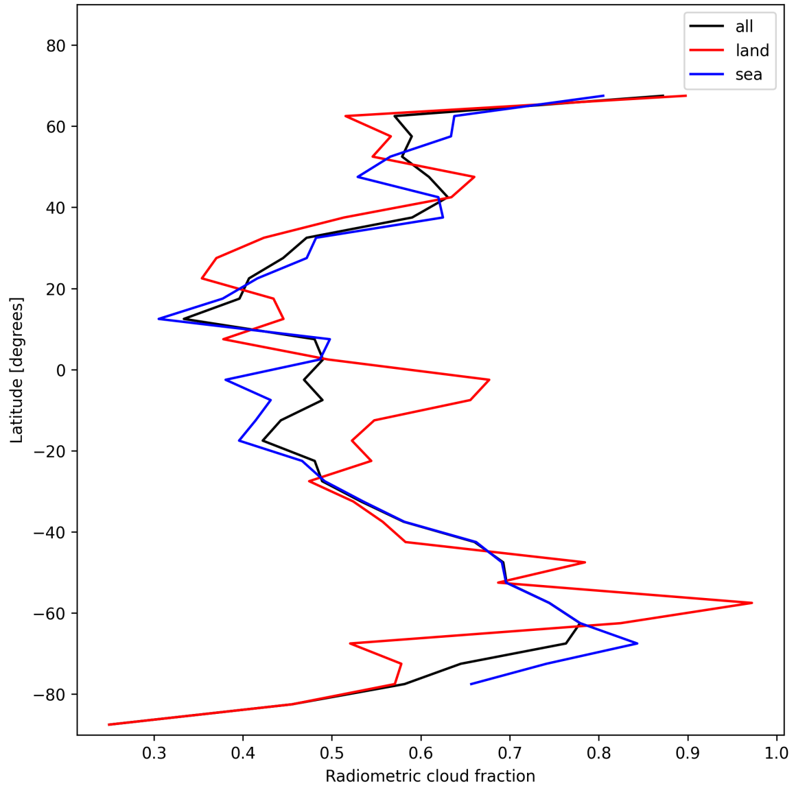
Figure 21: Zonal average of “Radiometric cloud fraction” for 2024-12-26 to 2024-12-27.
