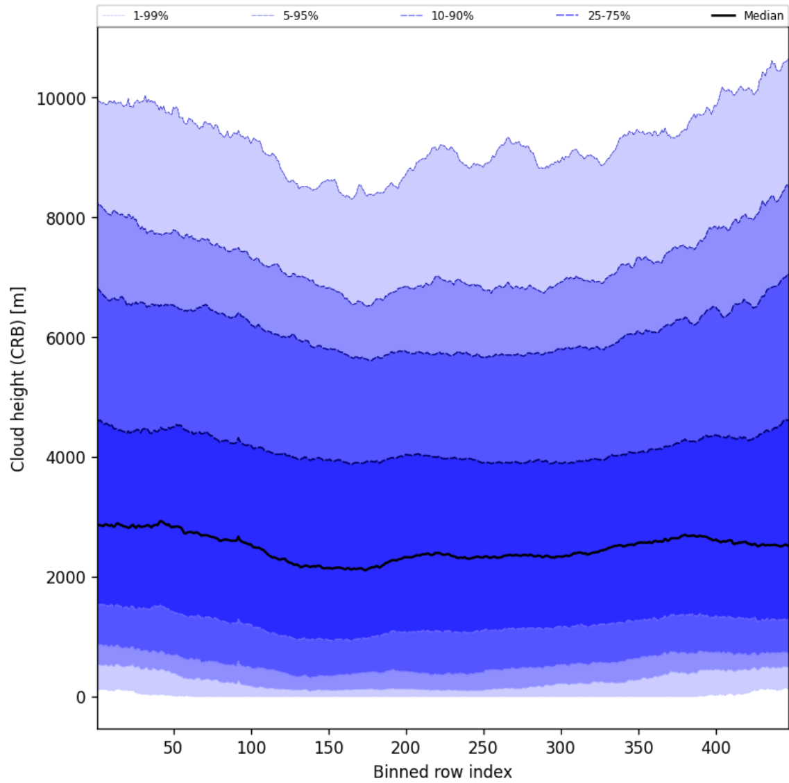
Figure 57: Along track statistics of “Cloud height (CRB)” for 2024-12-26 to 2024-12-27
