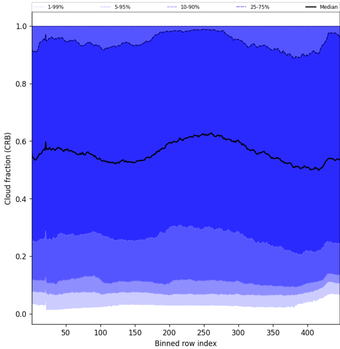
Figure 56: Along track statistics of “Cloud fraction (CRB)” for 2024-12-26 to 2024-12-27
