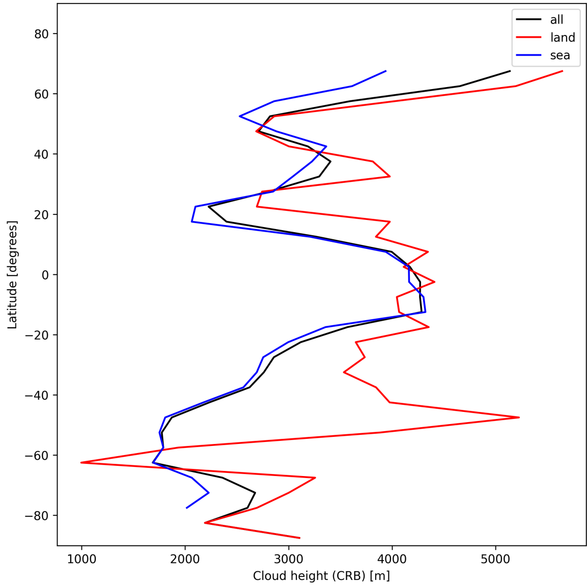
Figure 25: Zonal average of “Cloud height (CRB)” for 2024-12-26 to 2024-12-27.
