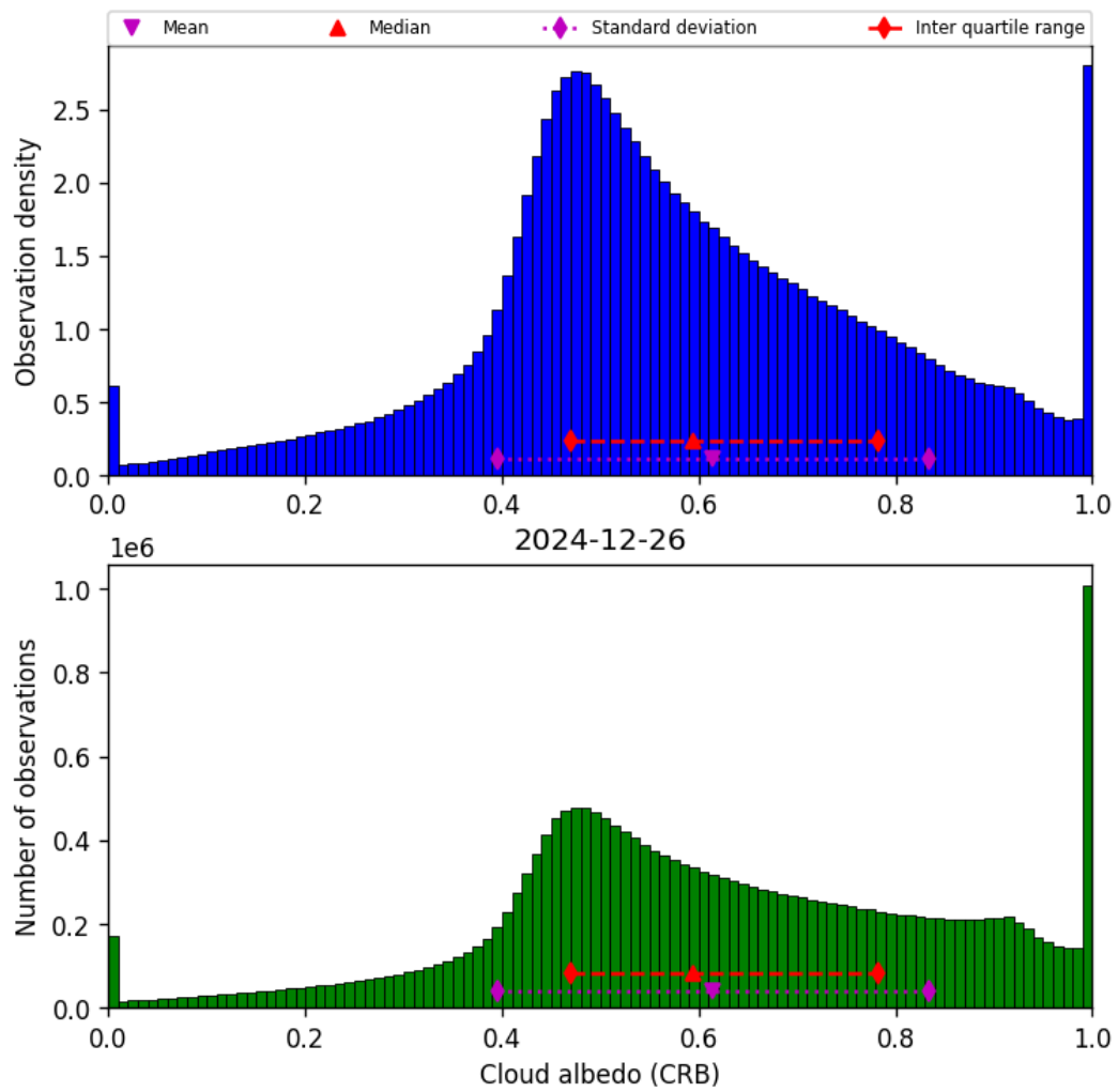
Figure 42: Histogram of “Cloud albedo (CRB)” for 2024-12-26 to 2024-12-27
