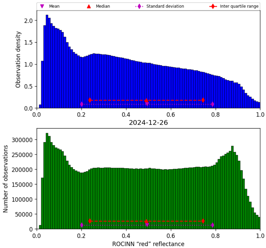
Figure 51: Histogram of “ROCINN “red” reflectance” for 2024-12-26 to 2024-12-27
