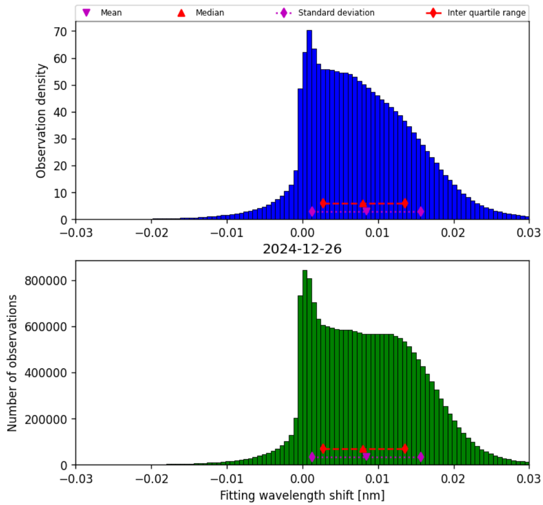
Figure 47: Histogram of “Fitting wavelength shift” for 2024-12-26 to 2024-12-27
