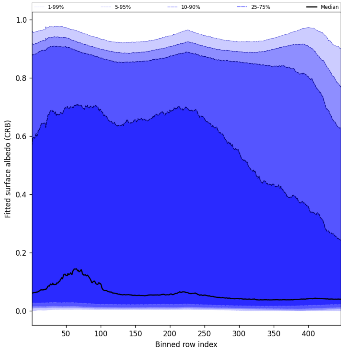
Figure 60: Along track statistics of “Fitted surface albedo (CRB)” for 2024-12-26 to 2024-12-27
