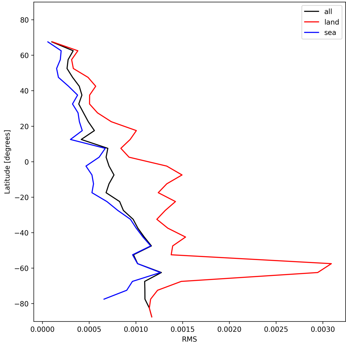
Figure 29: Zonal average of “RMS” for 2024-12-26 to 2024-12-27.
