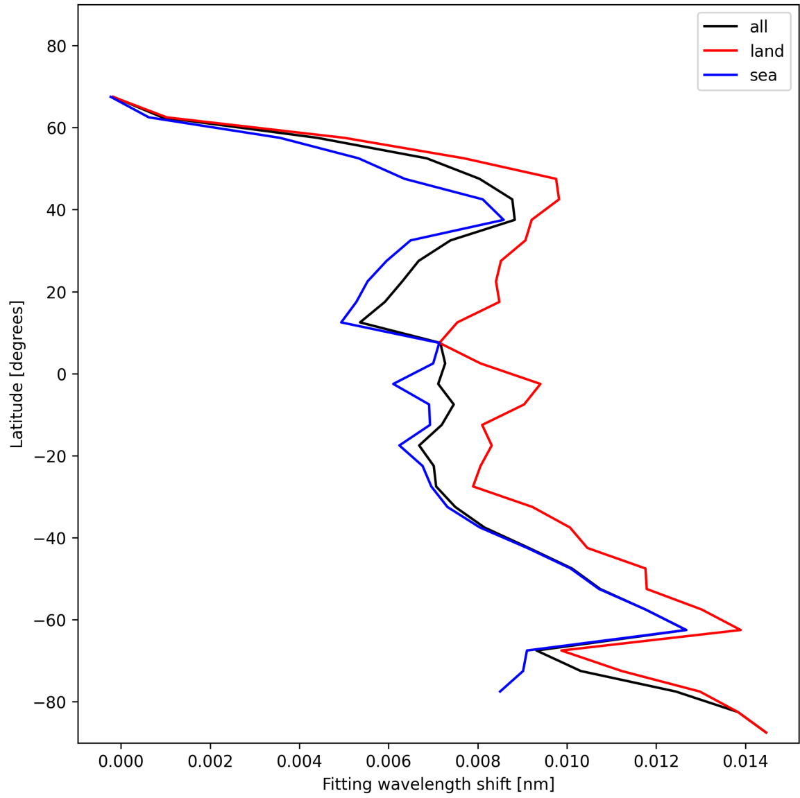
Figure 31: Zonal average of “Fitting wavelength shift” for 2024-12-26 to 2024-12-27.
