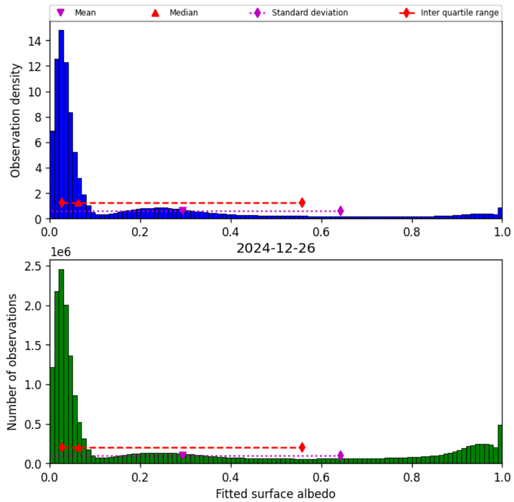
Figure 43: Histogram of “Fitted surface albedo” for 2024-12-26 to 2024-12-27
