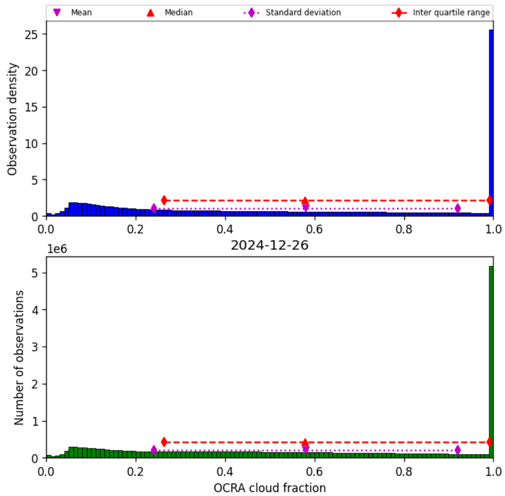
Figure 48: Histogram of “OCRA cloud fraction” for 2024-12-26 to 2024-12-27
