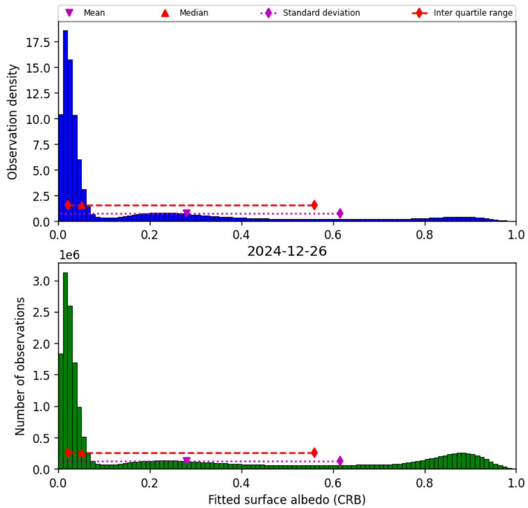
Figure 44: Histogram of “Fitted surface albedo (CRB)” for 2024-12-26 to 2024-12-27
