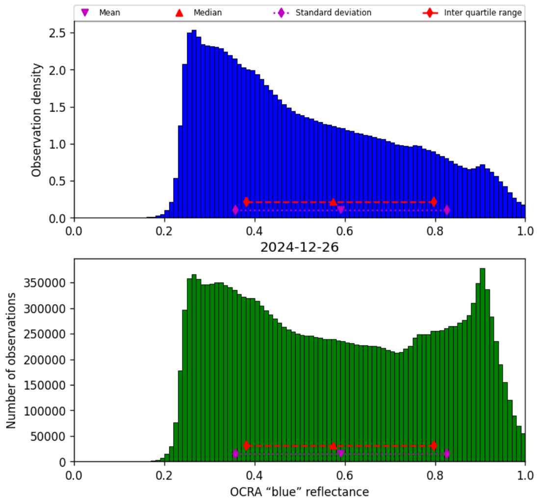
Figure 49: Histogram of “OCRA “blue” reflectance” for 2024-12-26 to 2024-12-27
