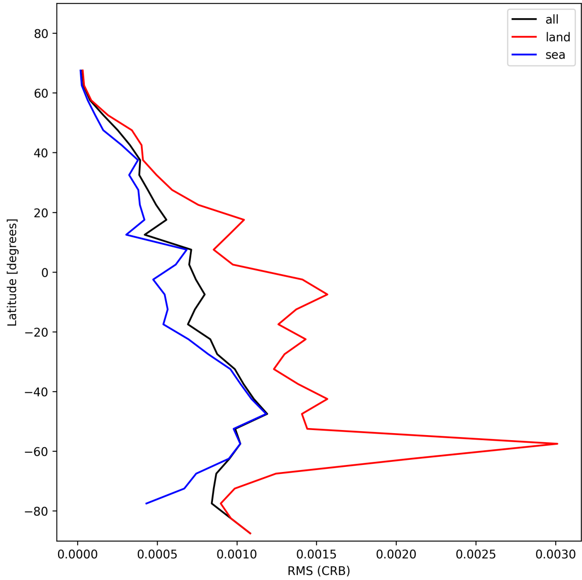
Figure 30: Zonal average of “RMS (CRB)” for 2024-12-26 to 2024-12-27.
