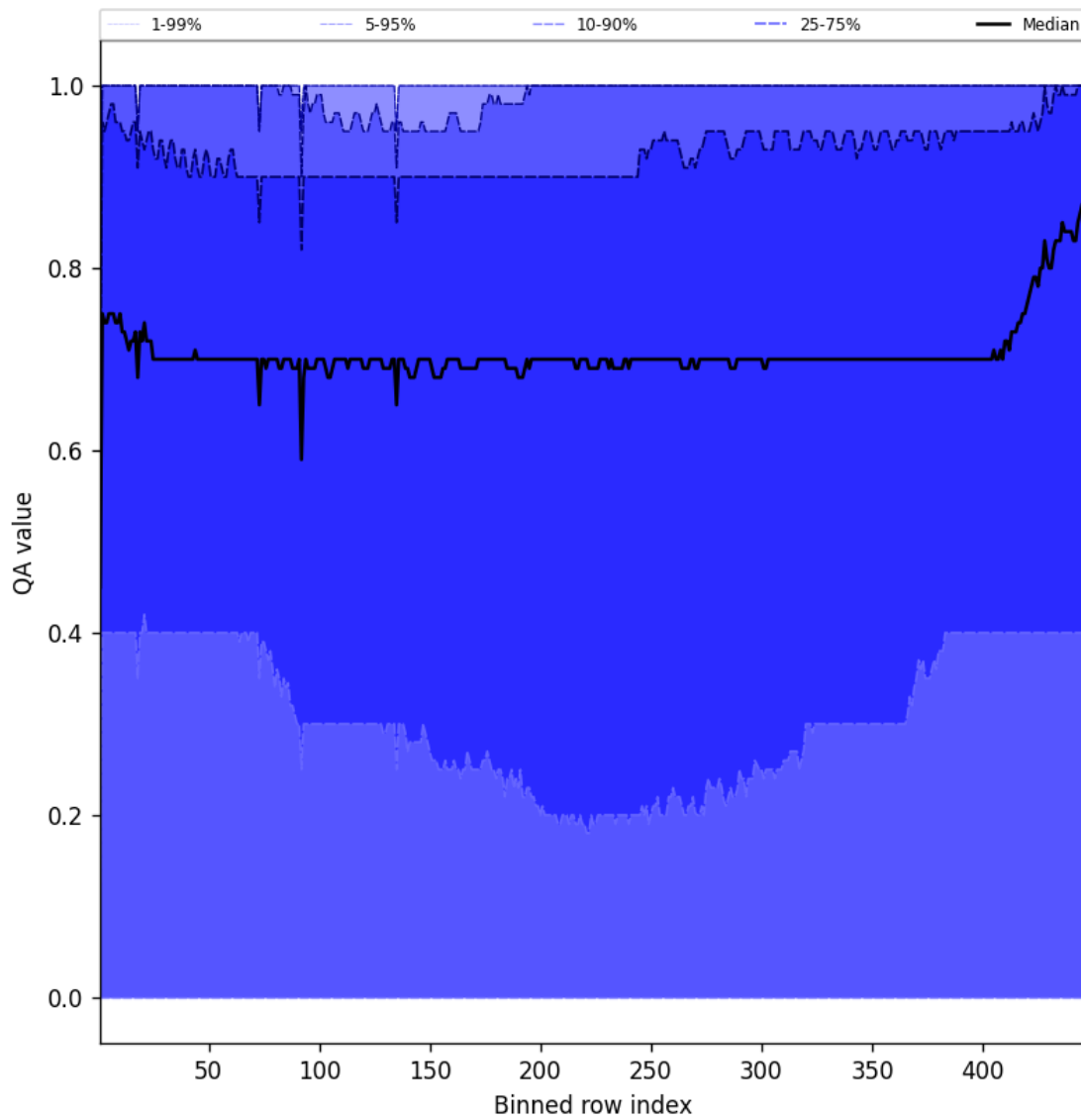
Figure 52: Along track statistics of “QA value” for 2024-12-26 to 2024-12-27
