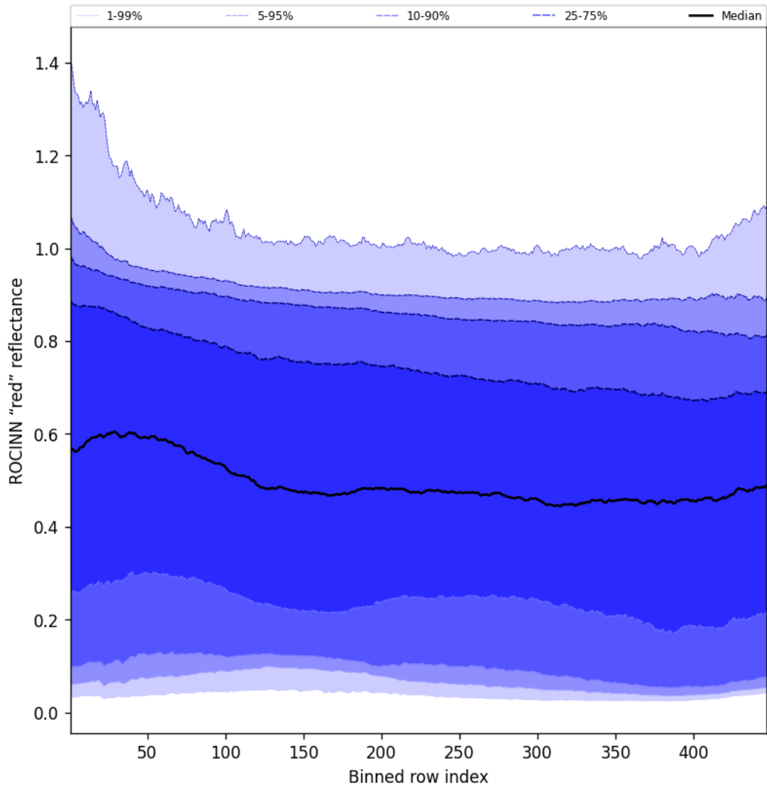
Figure 67: Along track statistics of "ROCINN "red" reflectance" for 2024-12-26 to 2024-12-27
