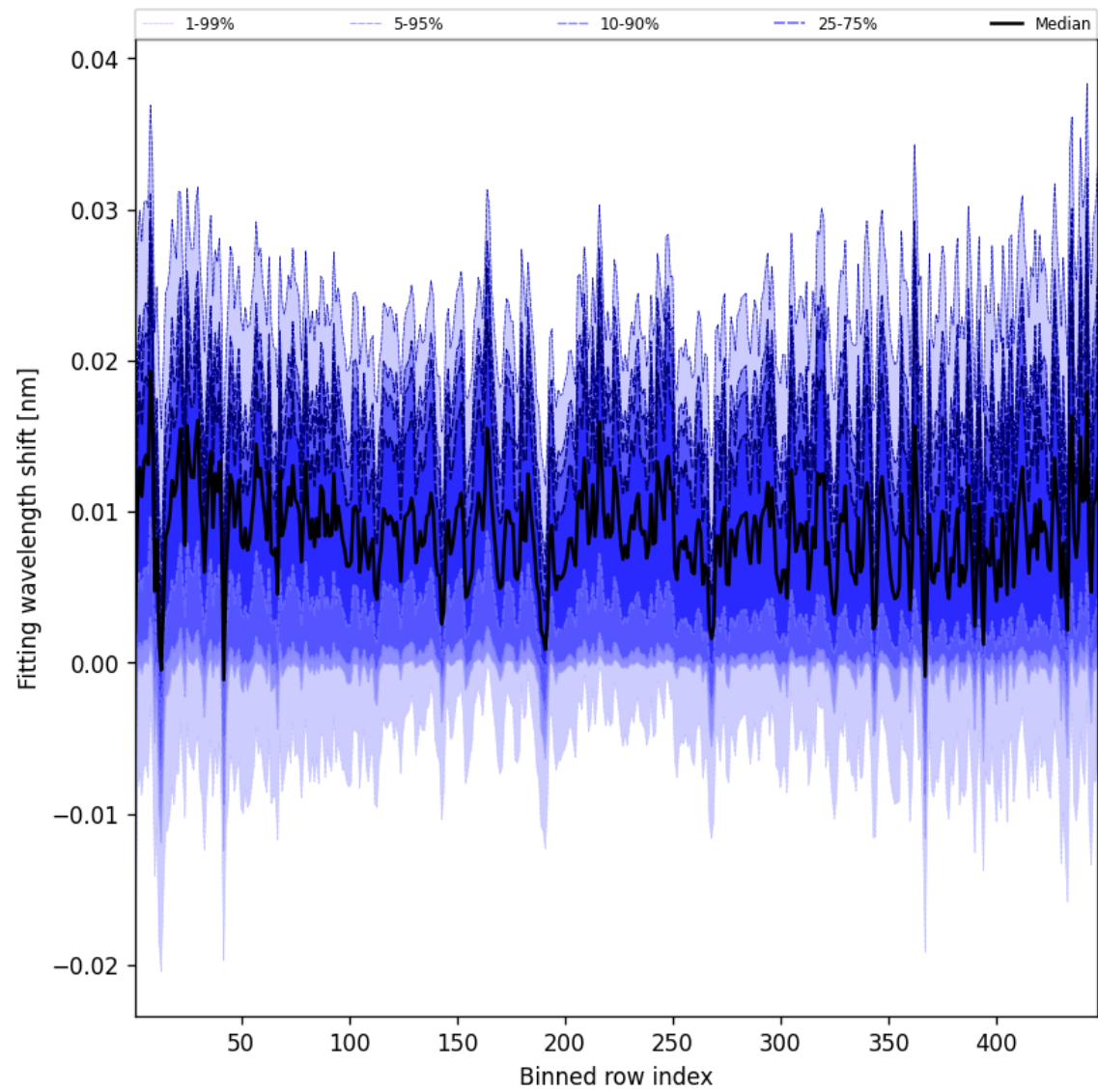
Figure 63: Along track statistics of “Fitting wavelength shift” for 2024-12-26 to 2024-12-27
