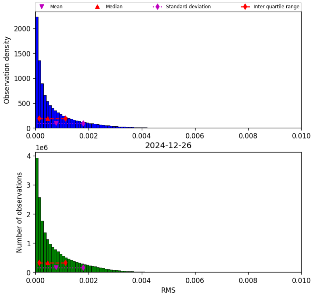
Figure 45: Histogram of “RMS” for 2024-12-26 to 2024-12-27
