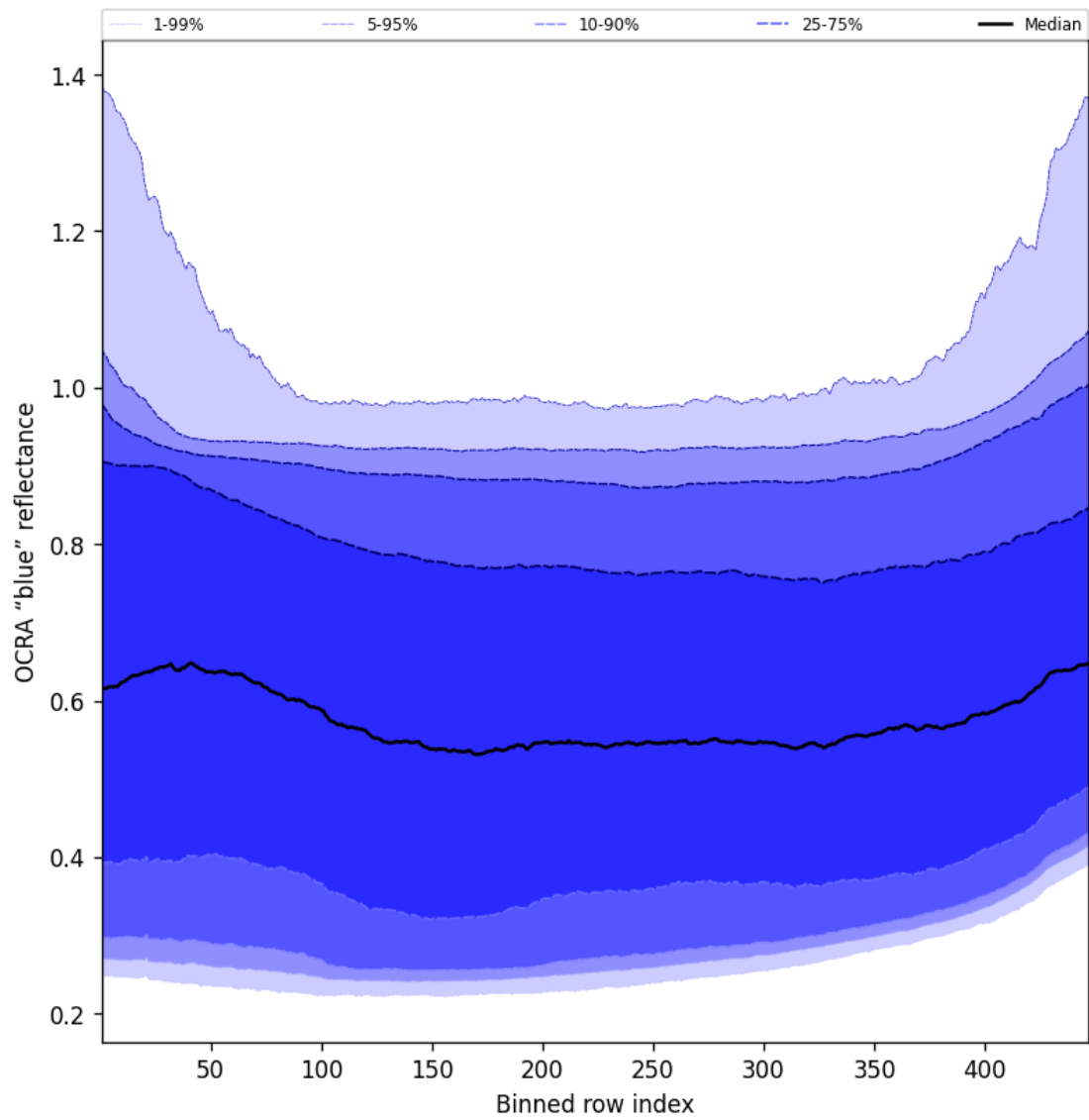
Figure 65: Along track statistics of "OCRA "blue" reflectance" for 2024-12-26 to 2024-12-27
