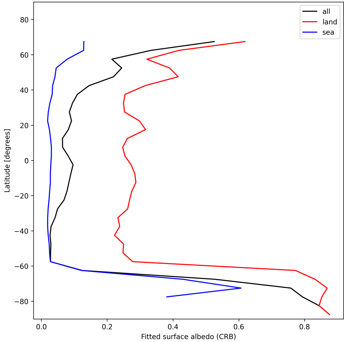
Figure 28: Zonal average of “Fitted surface albedo (CRB)” for 2024-12-26 to 2024-12-27.
