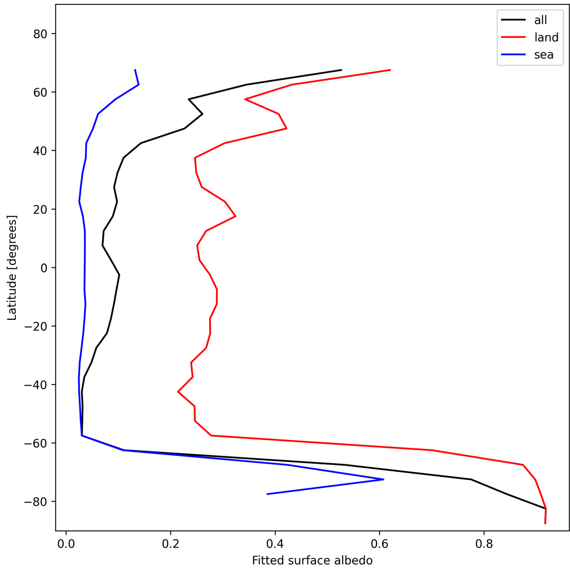
Figure 27: Zonal average of “Fitted surface albedo” for 2024-12-26 to 2024-12-27.
