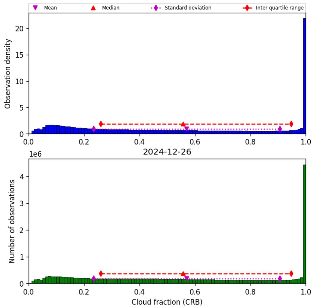
Figure 40: Histogram of “Cloud fraction (CRB)” for 2024-12-26 to 2024-12-27
