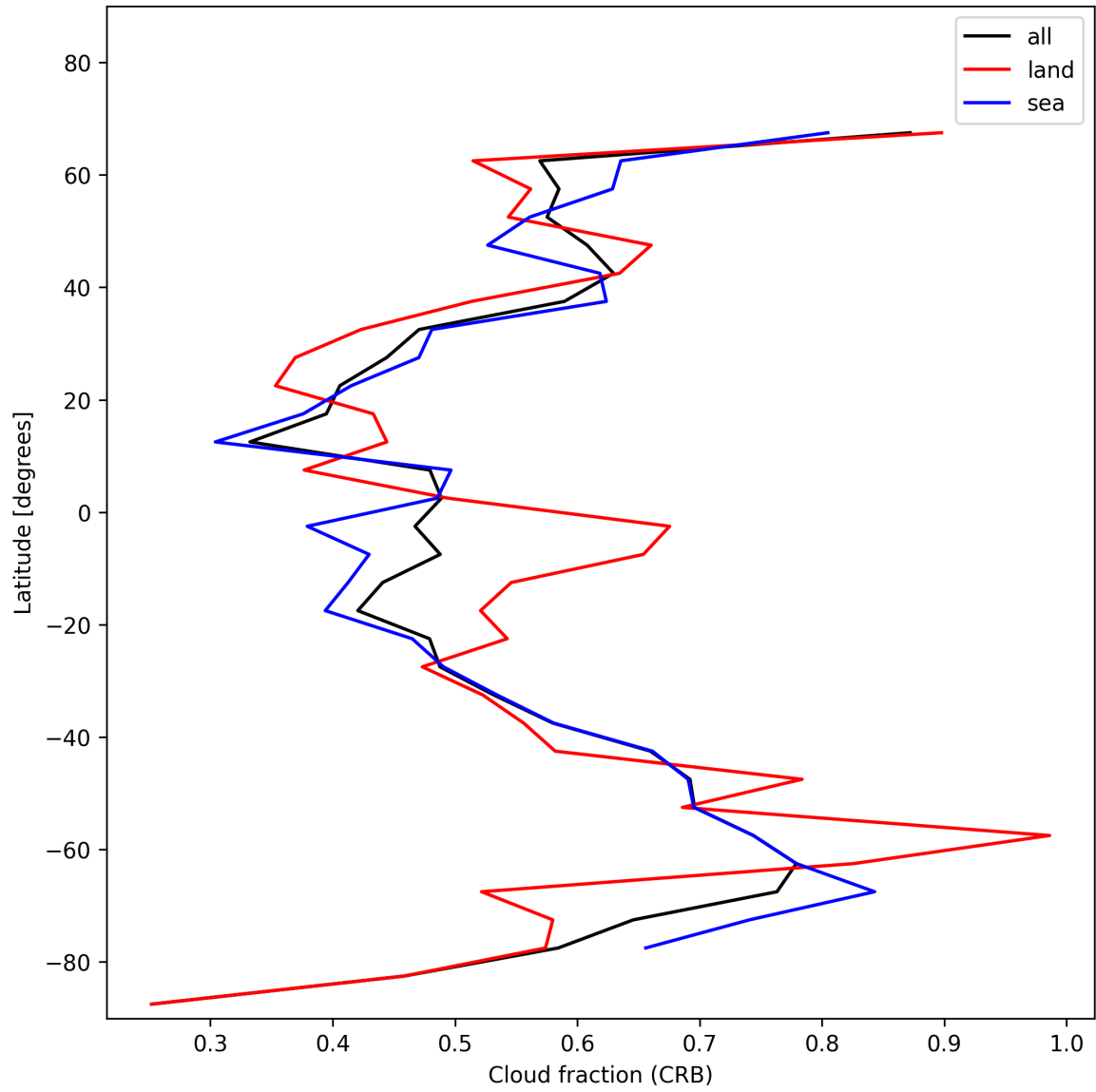
Figure 24: Zonal average of “Cloud fraction (CRB)” for 2024-12-26 to 2024-12-27.
