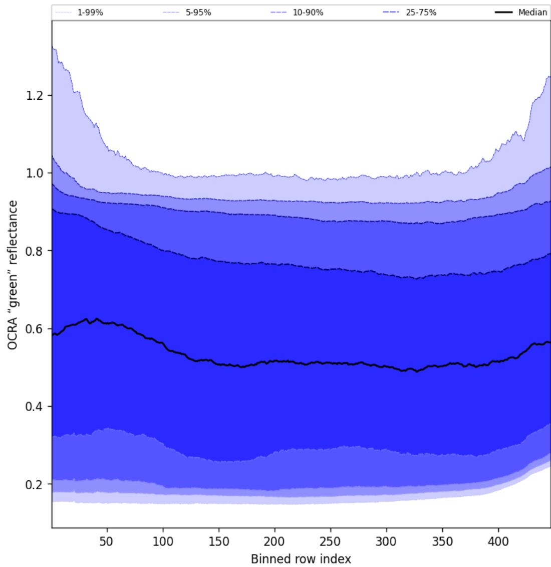
Figure 66: Along track statistics of "OCRA "green" reflectance" for 2024-12-26 to 2024-12-27
