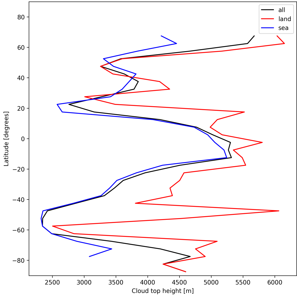
Figure 22: Zonal average of “Cloud top height” for 2024-12-26 to 2024-12-27.
