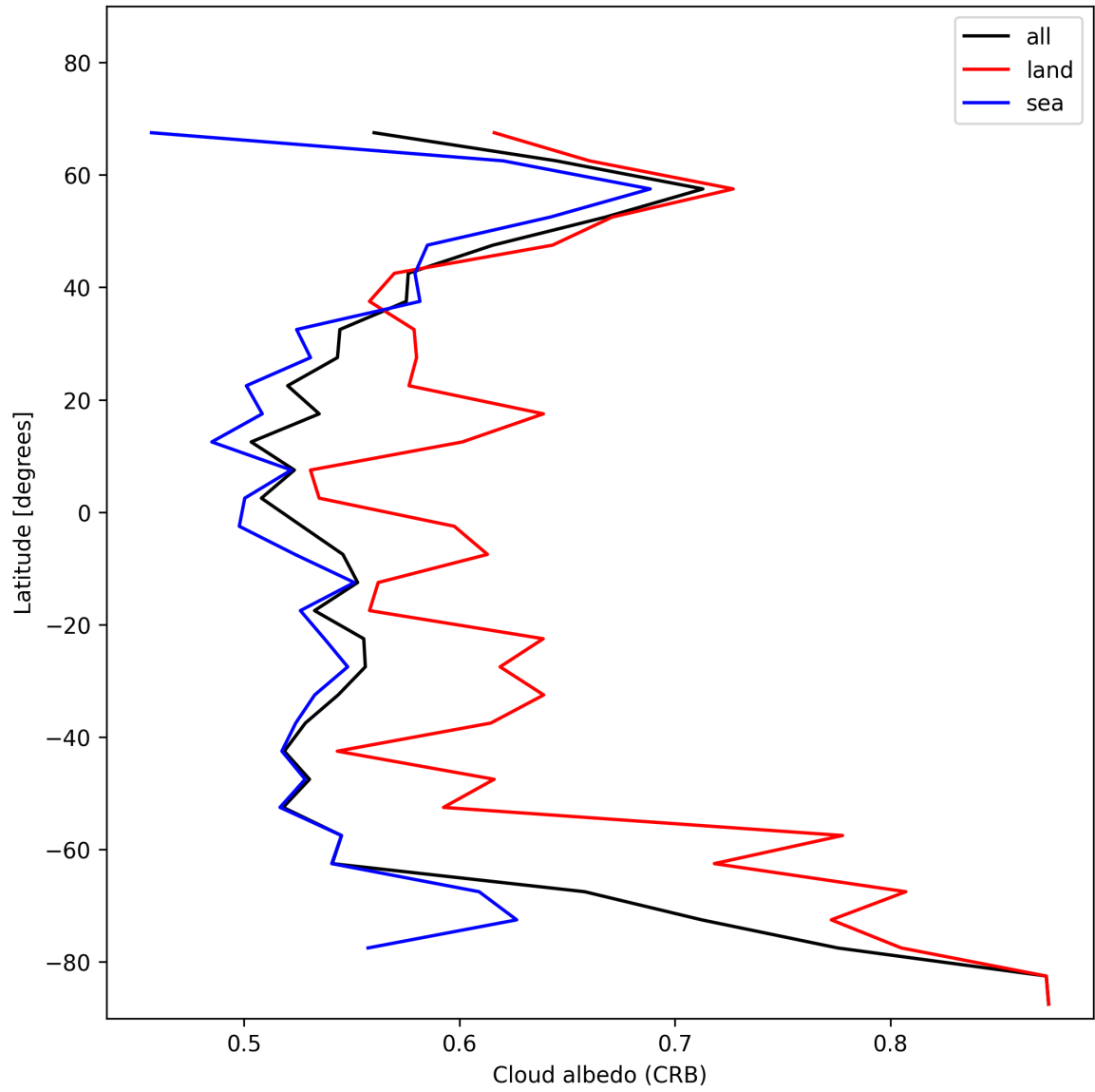
Figure 26: Zonal average of “Cloud albedo (CRB)” for 2024-12-26 to 2024-12-27.
