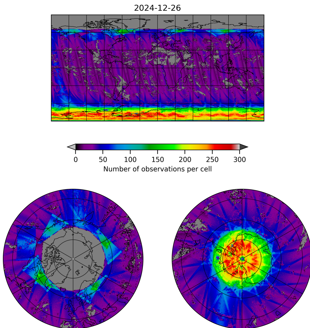
Figure 19: Map of the number of observations for 2024-12-26 to 2024-12-27
