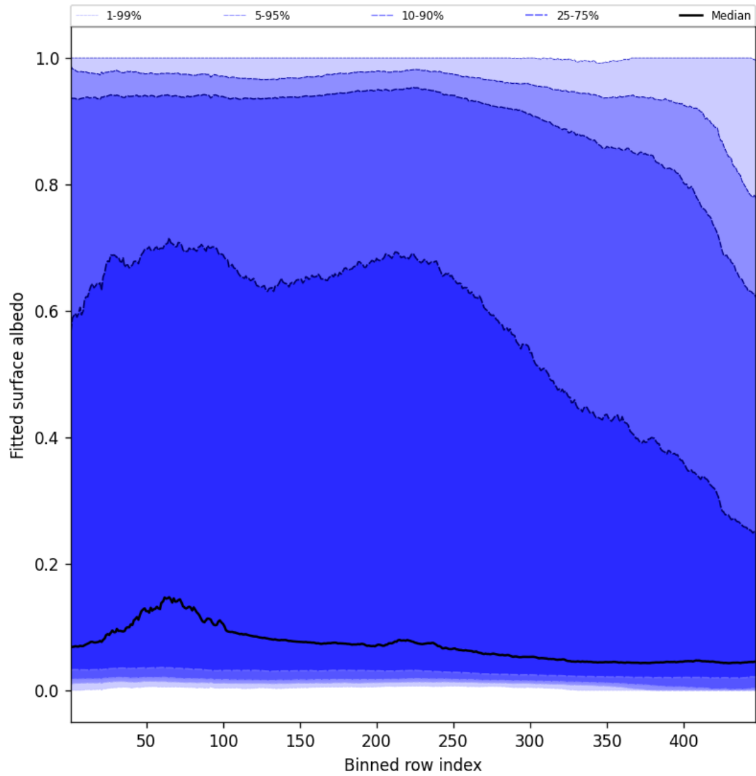
Figure 59: Along track statistics of “Fitted surface albedo” for 2024-12-26 to 2024-12-27
