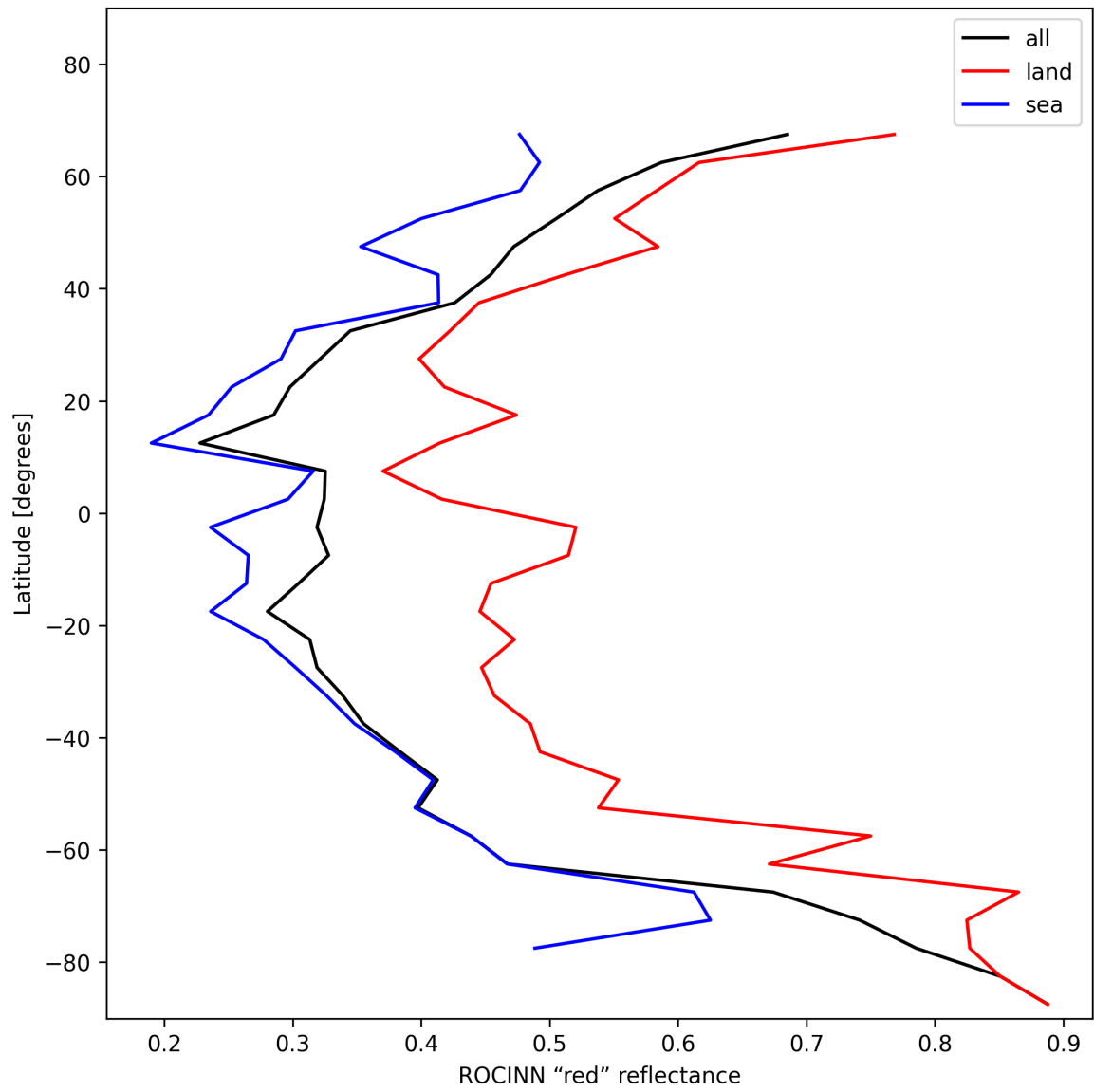
Figure 35: Zonal average of “ROCINN “red” reflectance” for 2024-12-26 to 2024-12-27.
