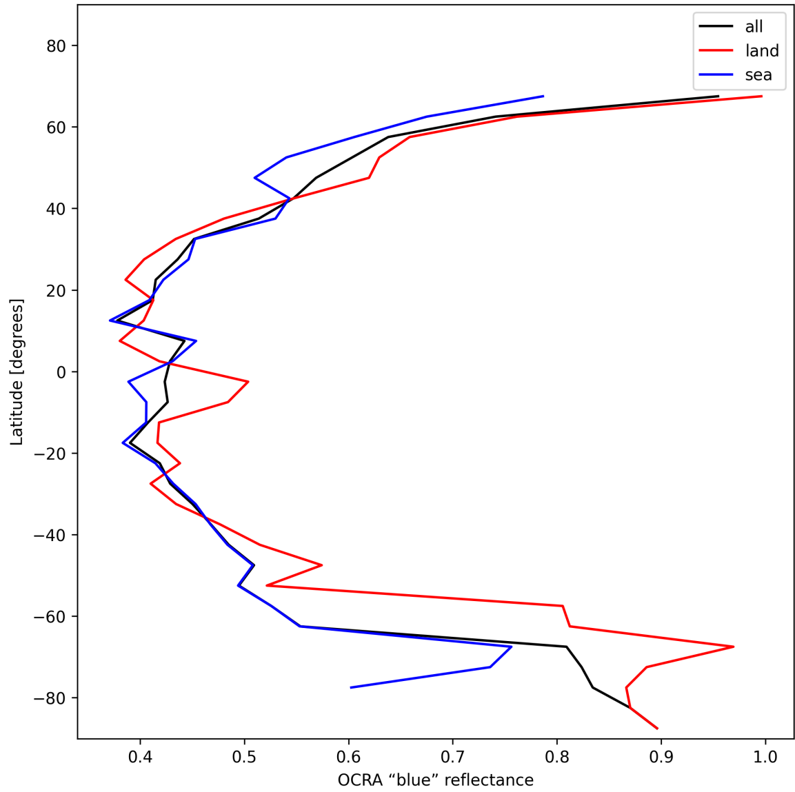
Figure 33: Zonal average of “OCRA “blue” reflectance” for 2024-12-26 to 2024-12-27.
