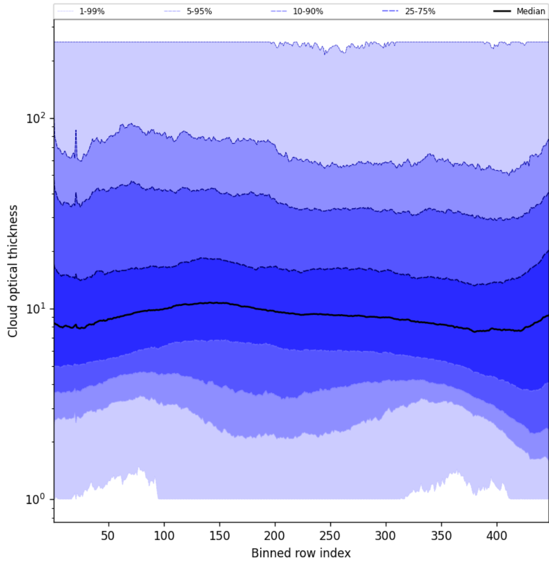
Figure 55: Along track statistics of “Cloud optical thickness” for 2024-12-26 to 2024-12-27
