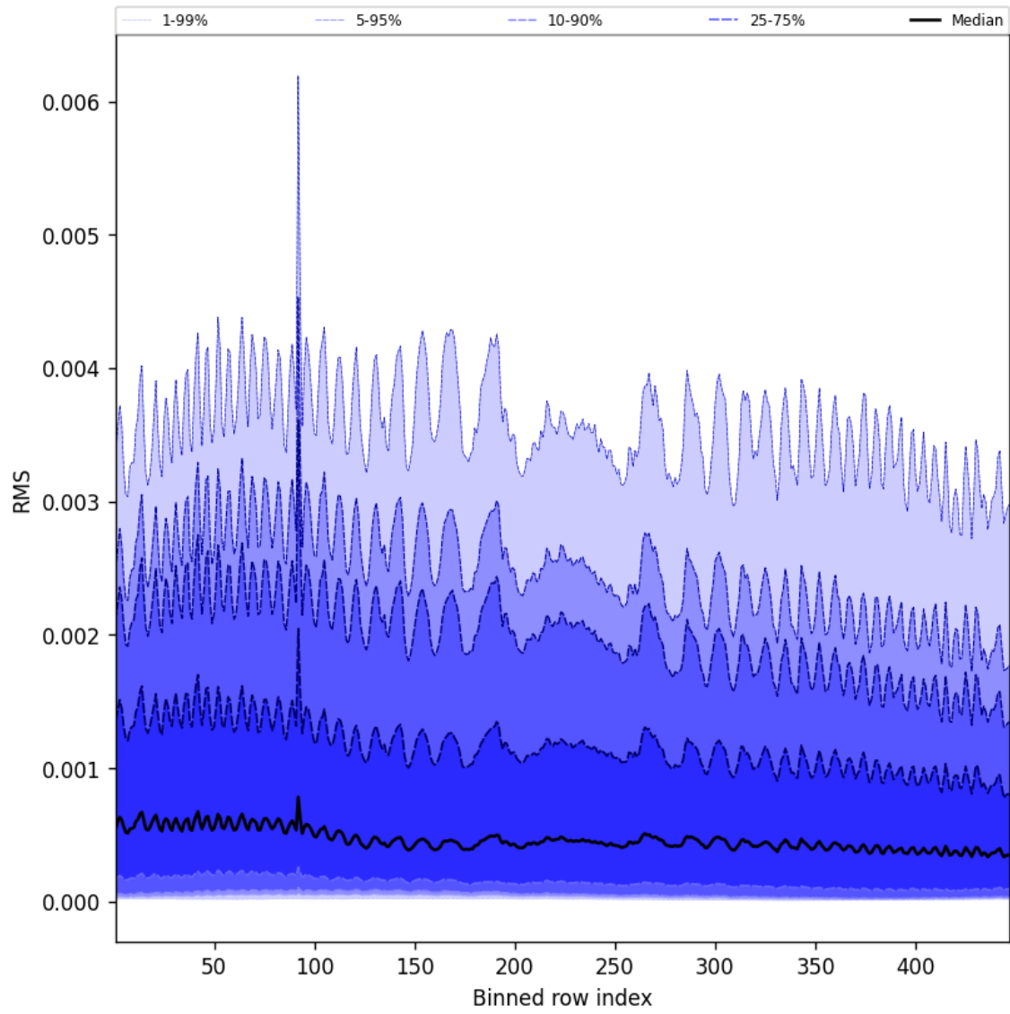
Figure 61: Along track statistics of “RMS” for 2024-12-26 to 2024-12-27
