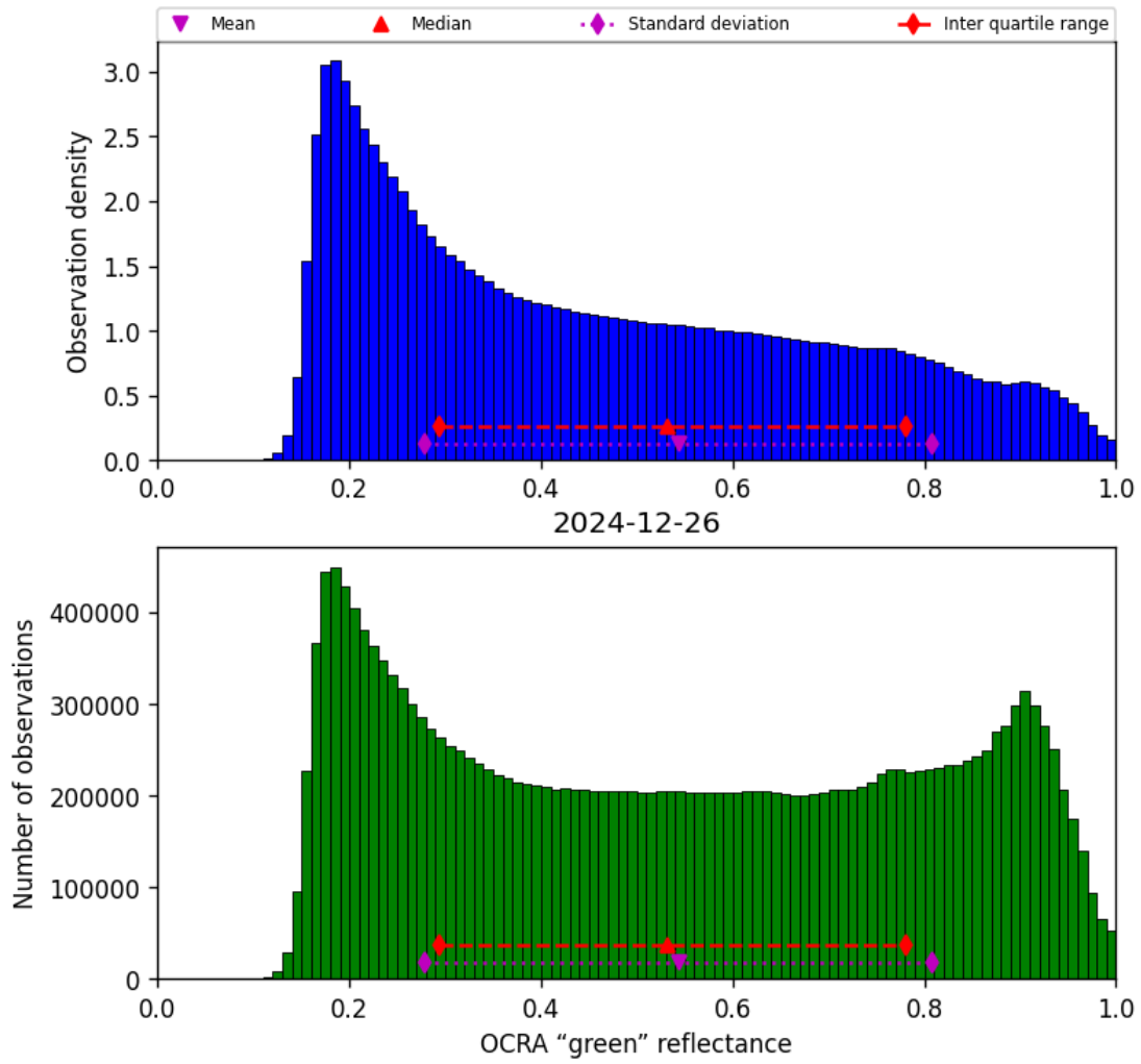
Figure 50: Histogram of “OCRA “green” reflectance” for 2024-12-26 to 2024-12-27
