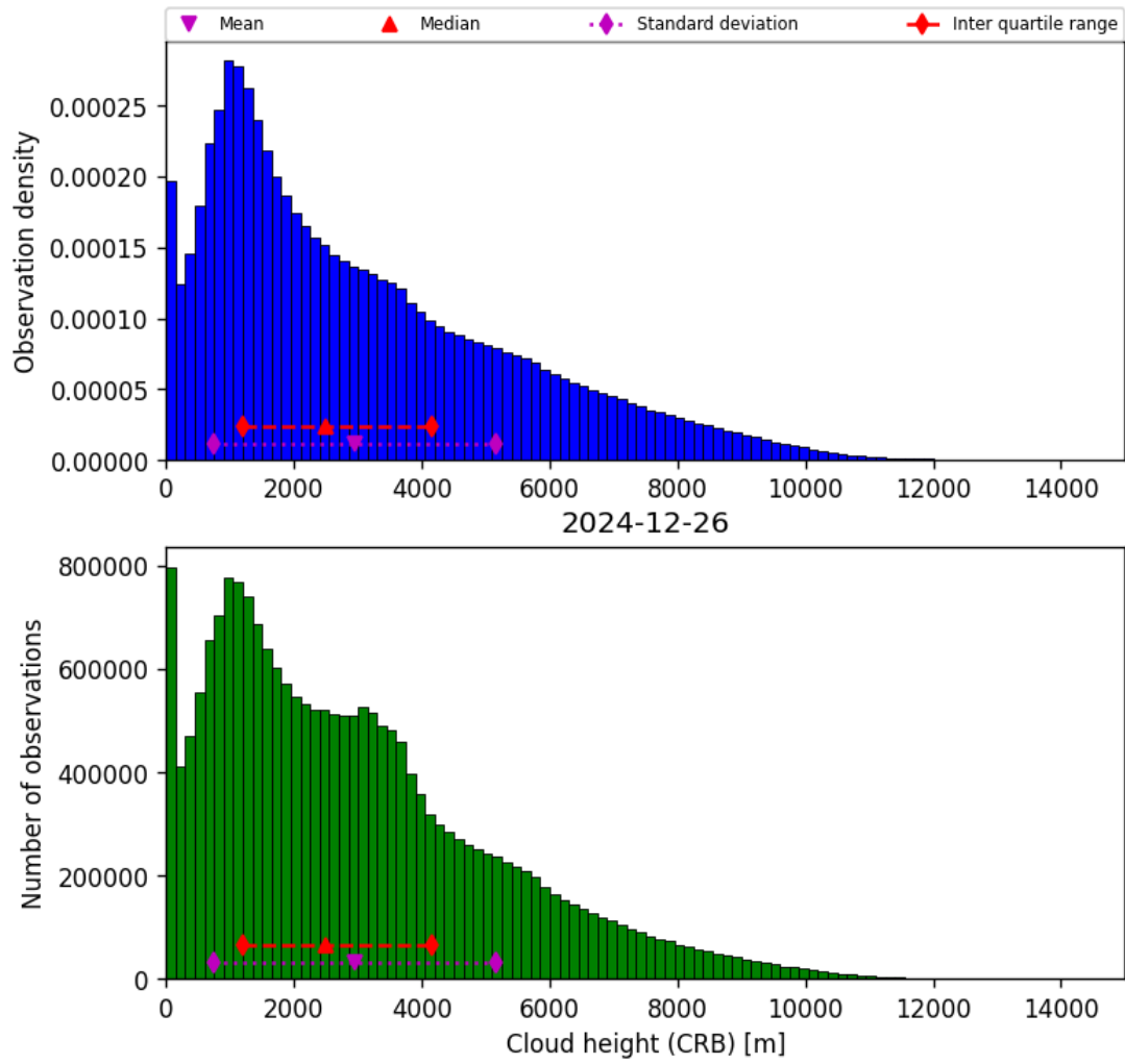
Figure 41: Histogram of “Cloud height (CRB)” for 2024-12-26 to 2024-12-27
