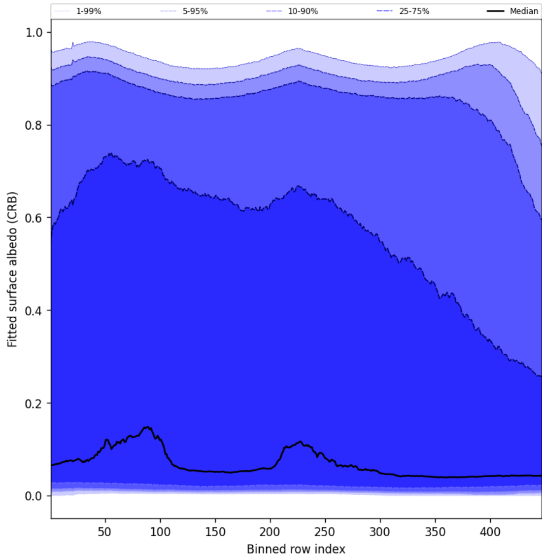
Figure 60: Along track statistics of “Fitted surface albedo (CRB)” for 2024-12-29 to 2024-12-30
