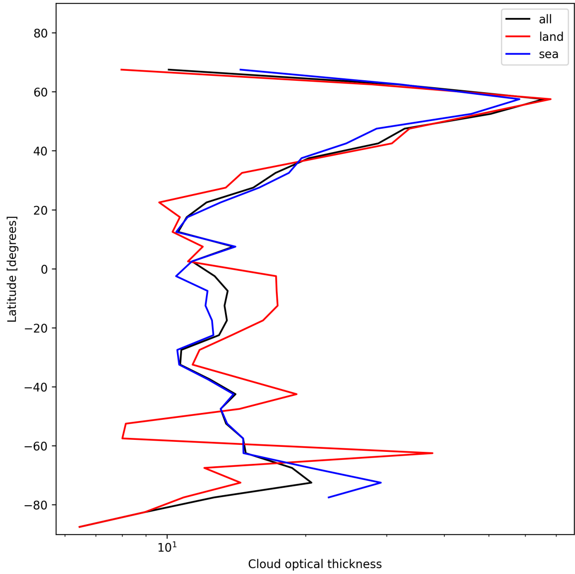
Figure 23: Zonal average of “Cloud optical thickness” for 2024-12-29 to 2024-12-30.
