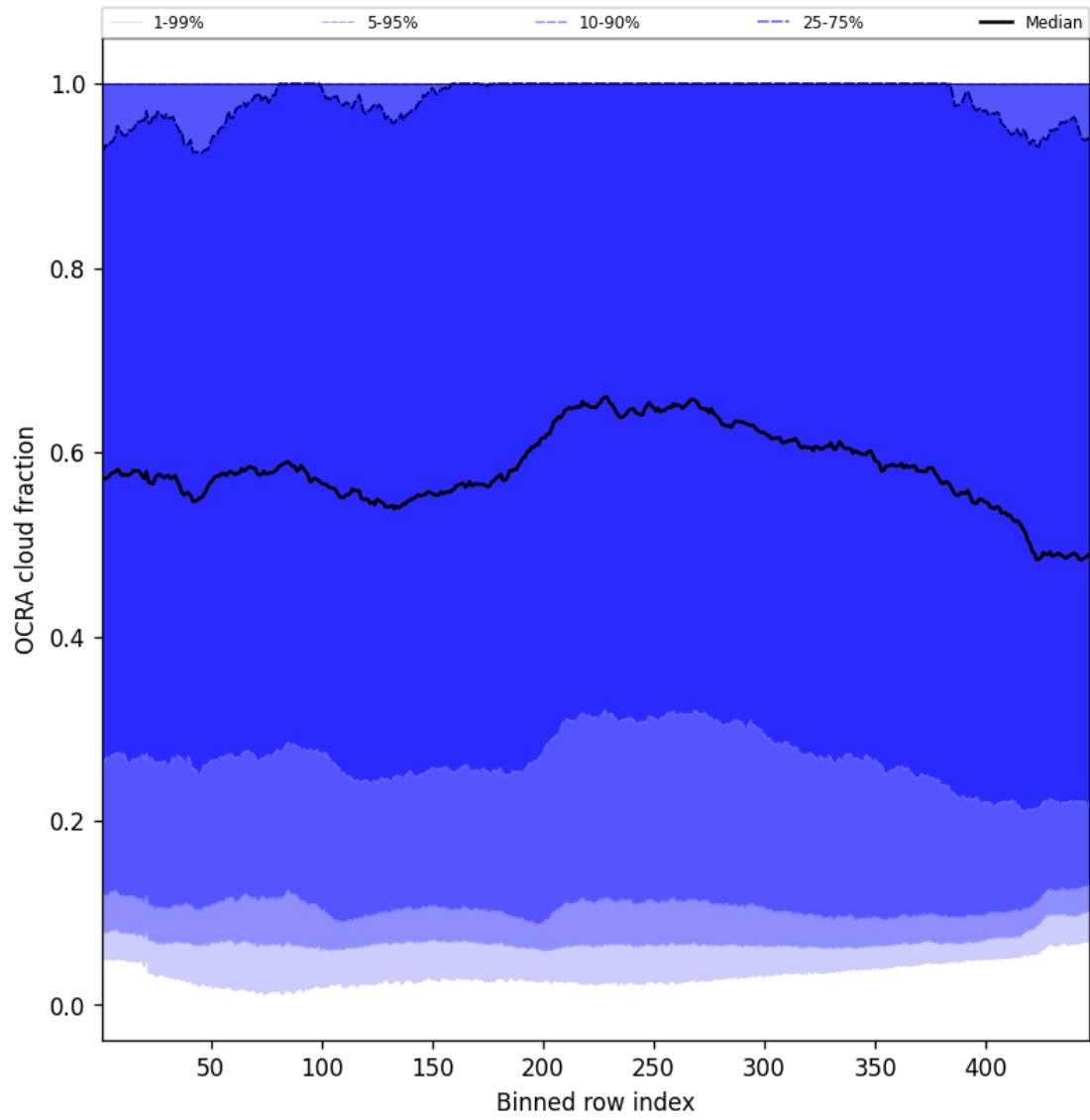
Figure 64: Along track statistics of “OCRA cloud fraction” for 2024-12-29 to 2024-12-30
