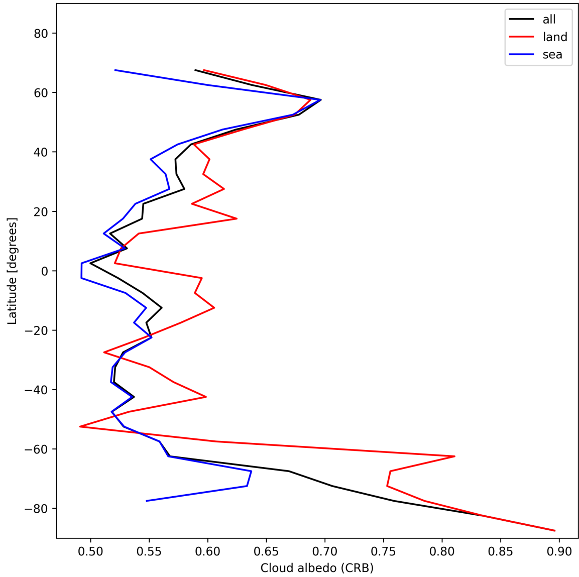
Figure 26: Zonal average of “Cloud albedo (CRB)” for 2024-12-29 to 2024-12-30.
