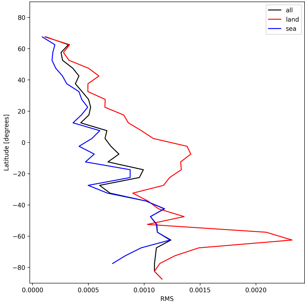
Figure 29: Zonal average of “RMS” for 2024-12-29 to 2024-12-30.
