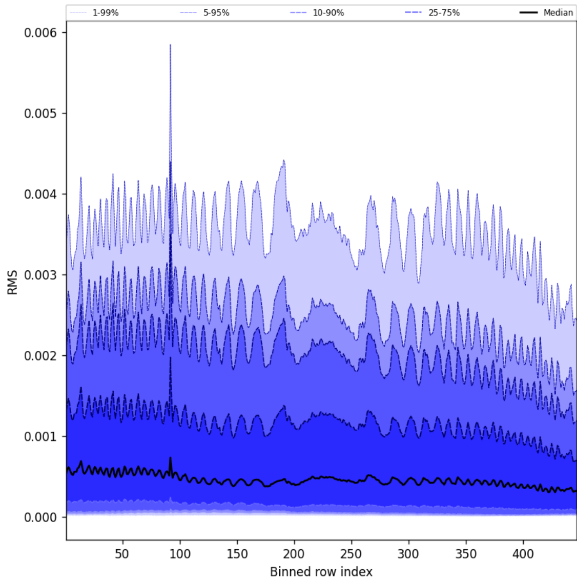
Figure 61: Along track statistics of “RMS” for 2024-12-29 to 2024-12-30
