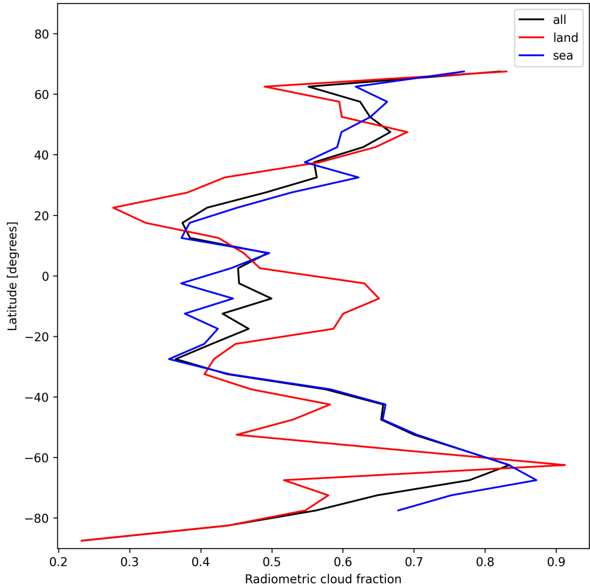
Figure 21: Zonal average of “Radiometric cloud fraction” for 2024-12-29 to 2024-12-30.
