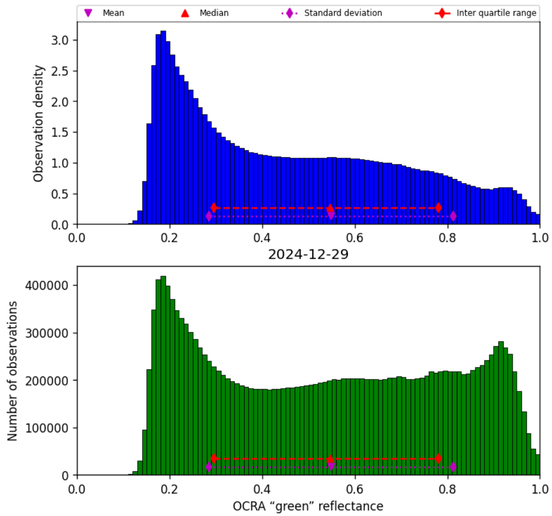
Figure 50: Histogram of “OCRA “green” reflectance” for 2024-12-29 to 2024-12-30
