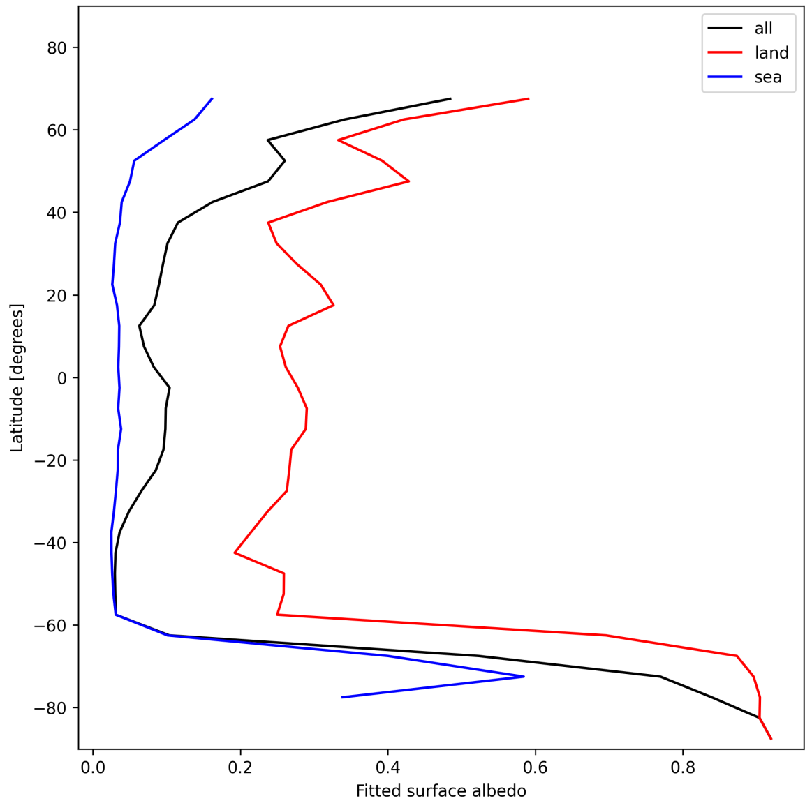
Figure 27: Zonal average of “Fitted surface albedo” for 2024-12-29 to 2024-12-30.
