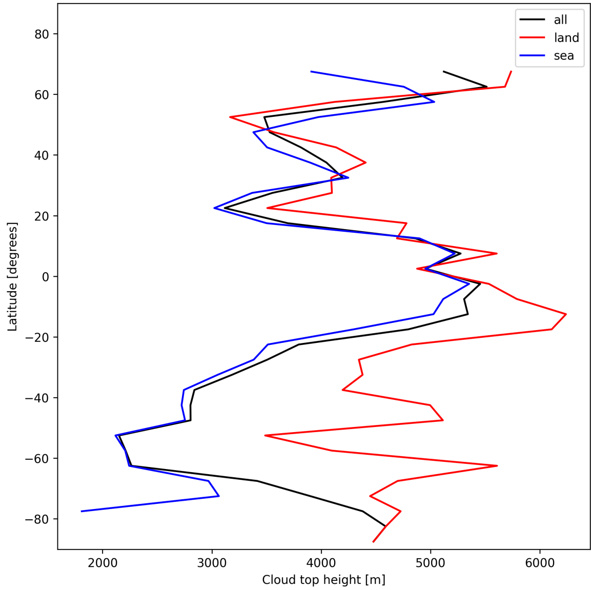
Figure 22: Zonal average of “Cloud top height” for 2024-12-29 to 2024-12-30.
