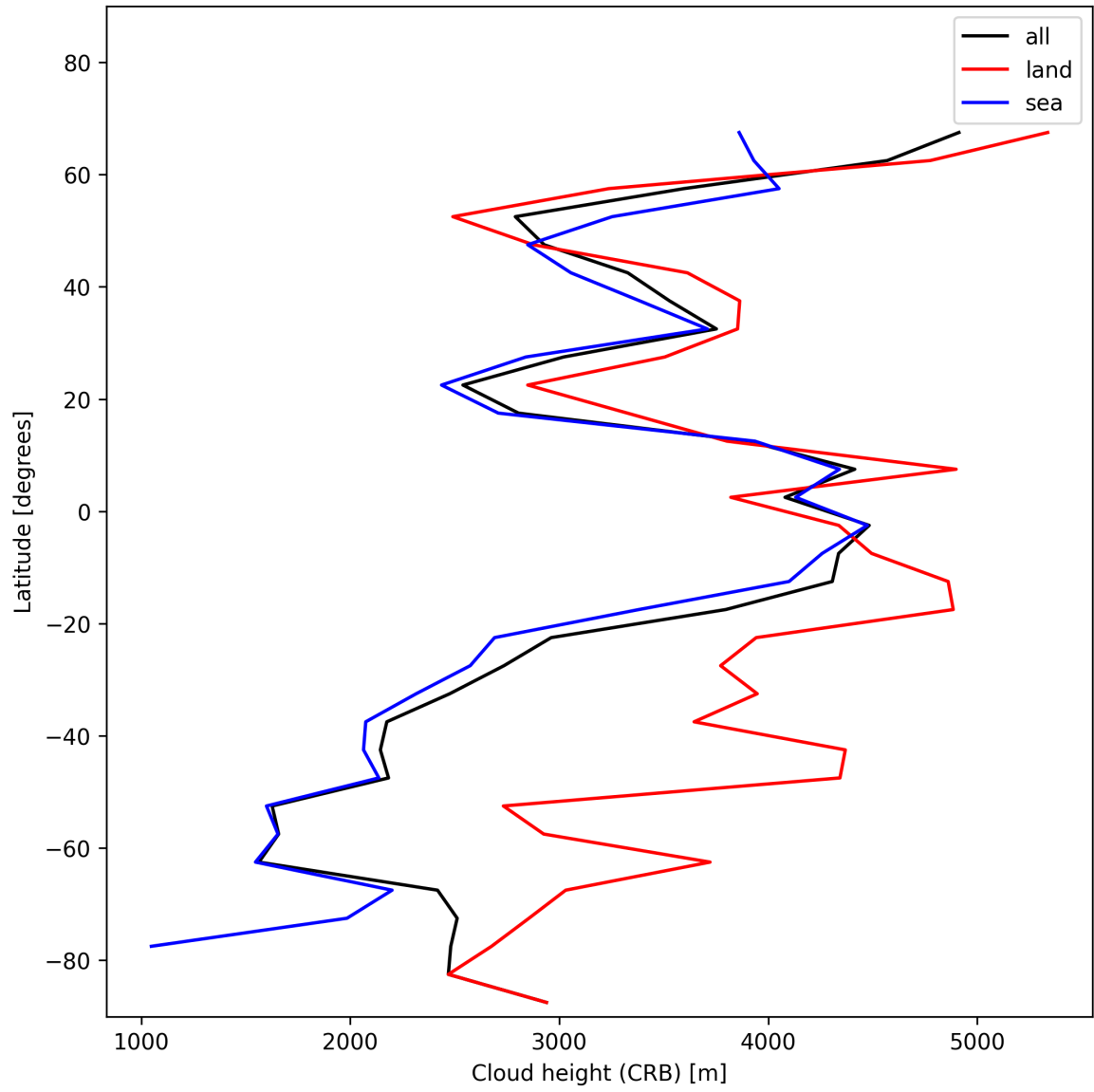
Figure 25: Zonal average of “Cloud height (CRB)” for 2024-12-29 to 2024-12-30.
