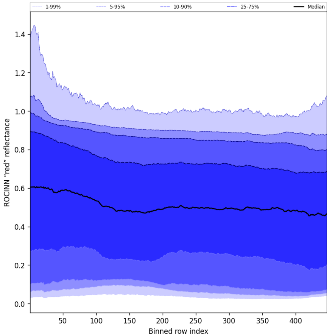
Figure 67: Along track statistics of "ROCINN "red" reflectance" for 2024-12-29 to 2024-12-30
