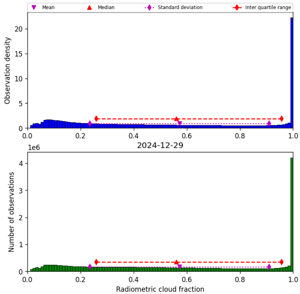
Figure 37: Histogram of “Radiometric cloud fraction” for 2024-12-29 to 2024-12-30
