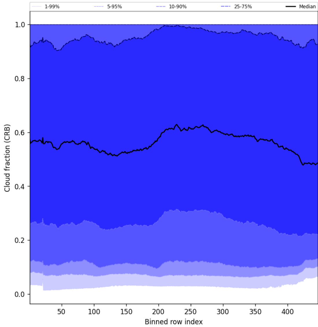
Figure 56: Along track statistics of “Cloud fraction (CRB)” for 2024-12-29 to 2024-12-30
