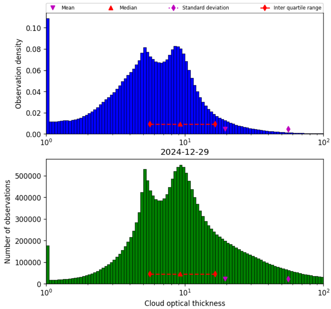
Figure 39: Histogram of “Cloud optical thickness” for 2024-12-29 to 2024-12-30
