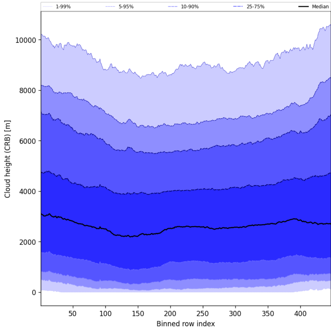
Figure 57: Along track statistics of “Cloud height (CRB)” for 2024-12-29 to 2024-12-30
