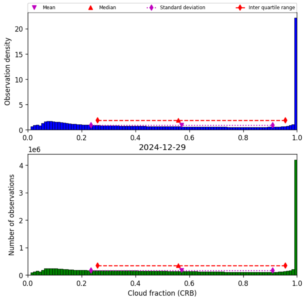
Figure 40: Histogram of “Cloud fraction (CRB)” for 2024-12-29 to 2024-12-30
