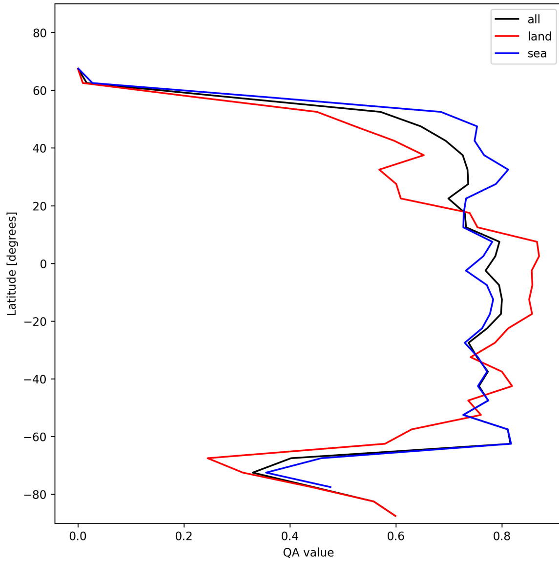
Figure 20: Zonal average of “QA value” for 2024-12-29 to 2024-12-30.
