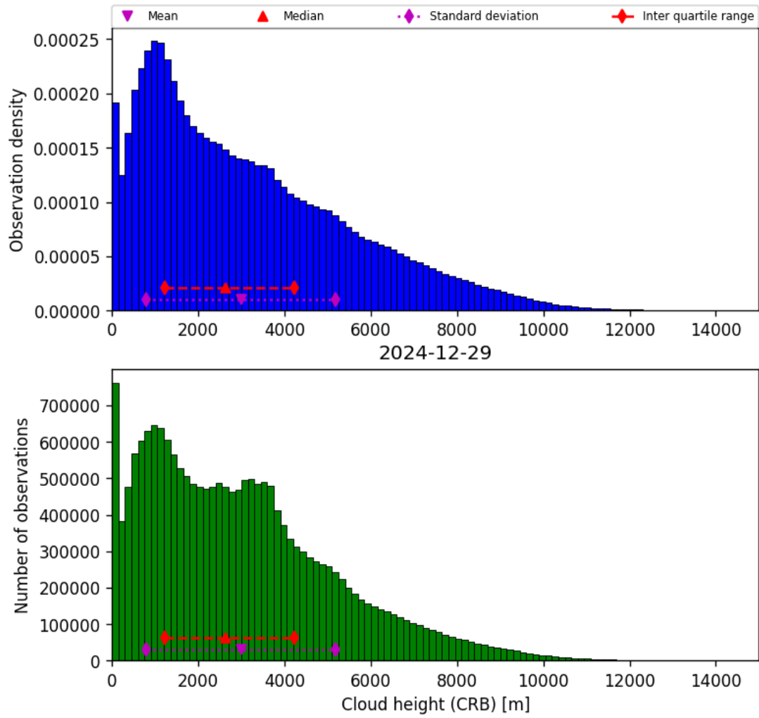
Figure 41: Histogram of “Cloud height (CRB)” for 2024-12-29 to 2024-12-30
