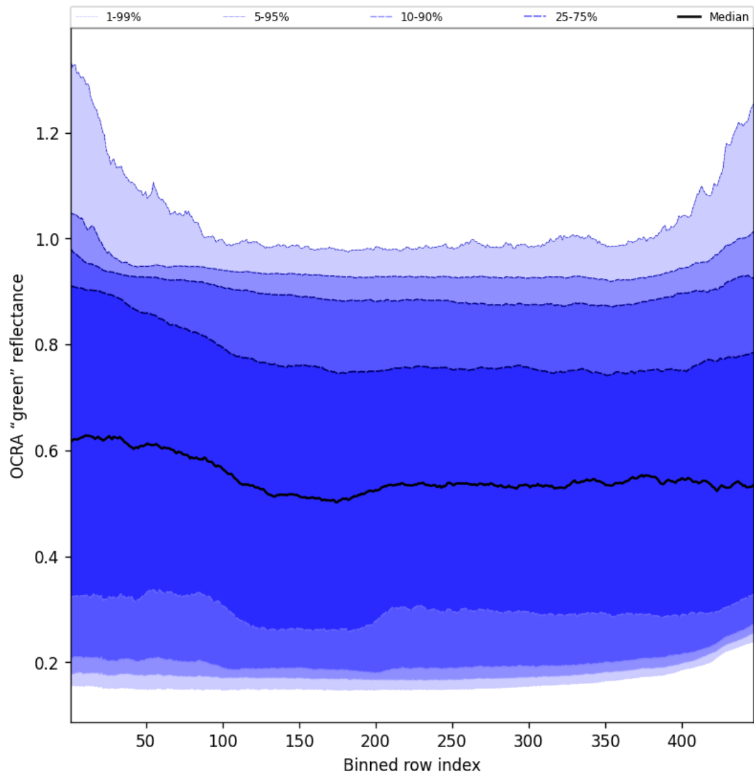
Figure 66: Along track statistics of "OCRA "green" reflectance" for 2024-12-29 to 2024-12-30
