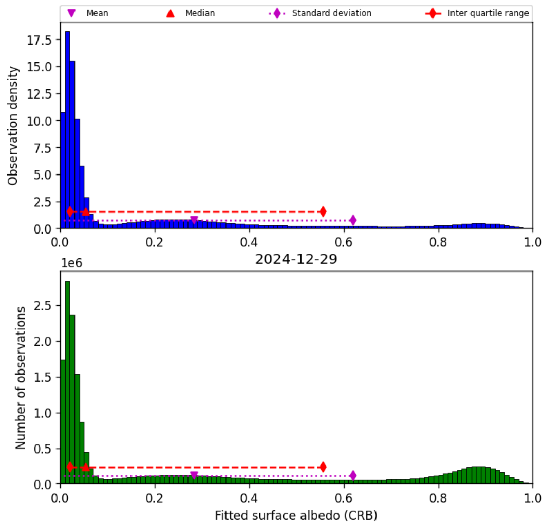
Figure 44: Histogram of “Fitted surface albedo (CRB)” for 2024-12-29 to 2024-12-30
