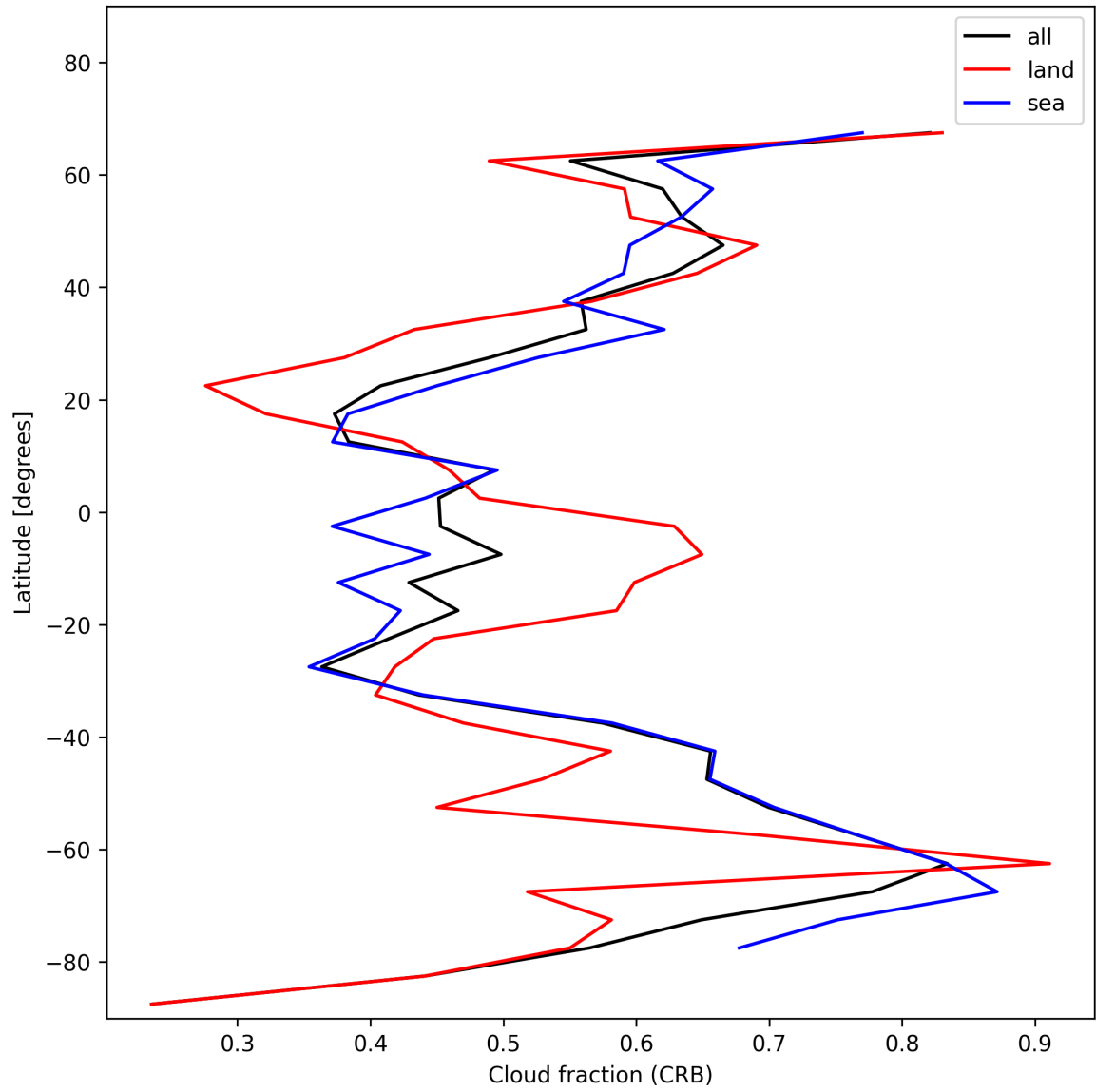
Figure 24: Zonal average of “Cloud fraction (CRB)” for 2024-12-29 to 2024-12-30.
