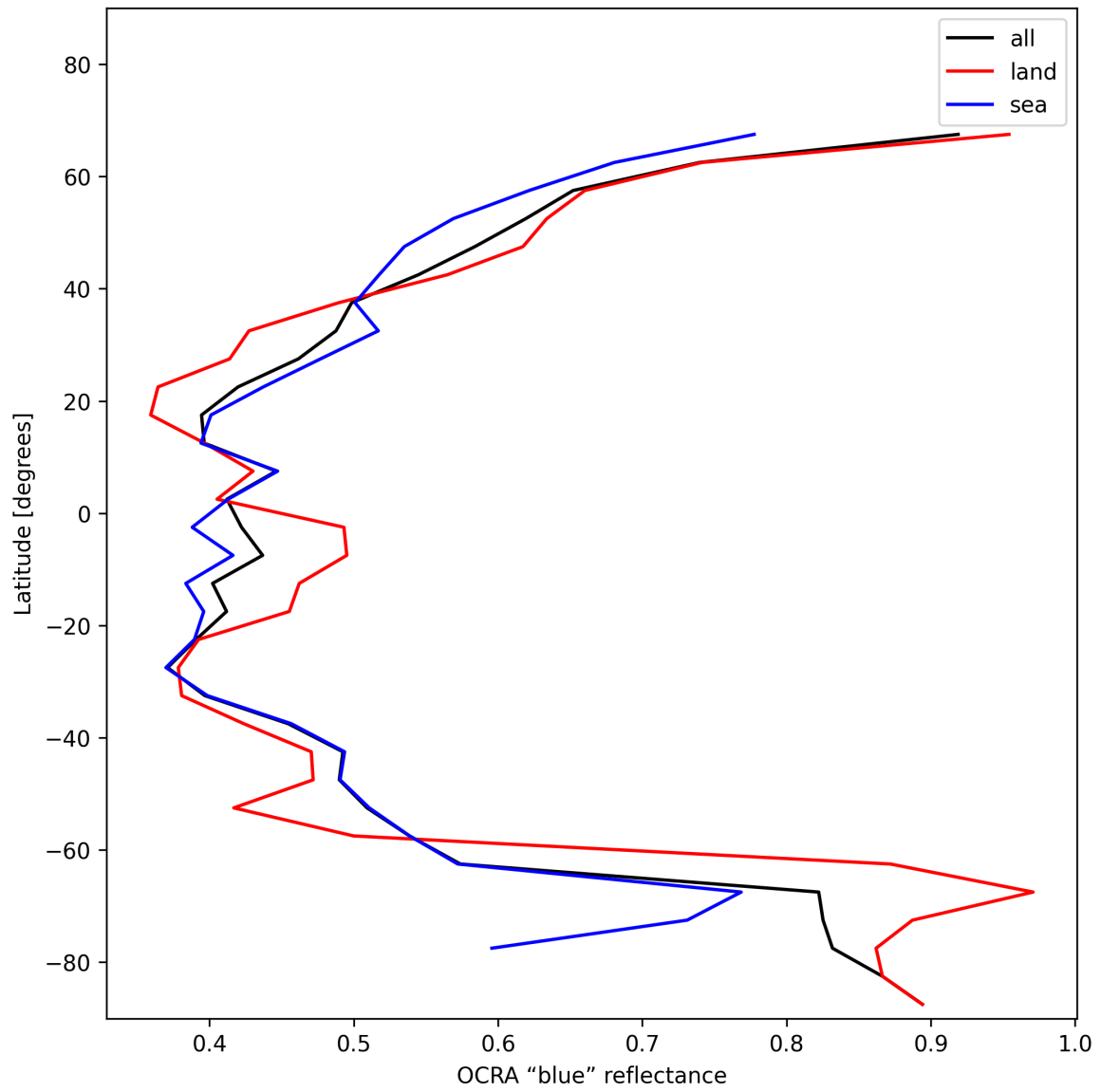
Figure 33: Zonal average of “OCRA “blue” reflectance” for 2024-12-29 to 2024-12-30.
