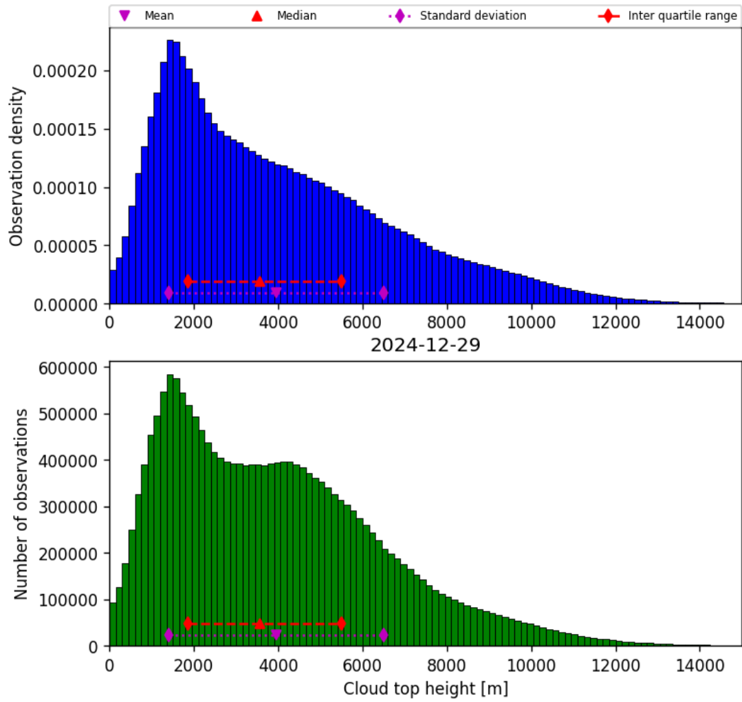
Figure 38: Histogram of “Cloud top height” for 2024-12-29 to 2024-12-30
