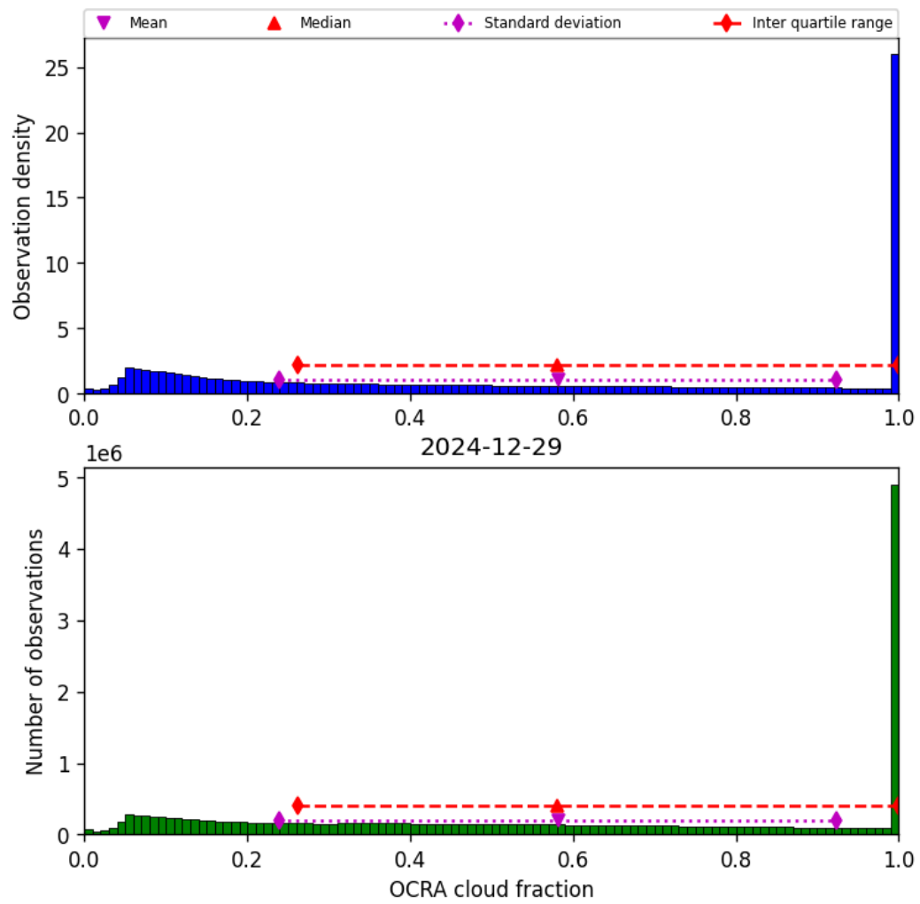
Figure 48: Histogram of “OCRA cloud fraction” for 2024-12-29 to 2024-12-30
