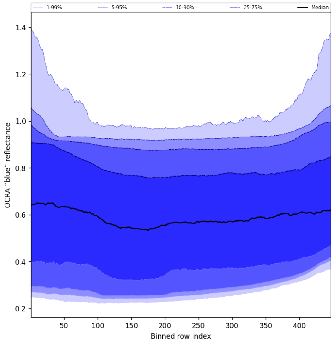
Figure 65: Along track statistics of “OCRA “blue” reflectance” for 2024-12-29 to 2024-12-30
