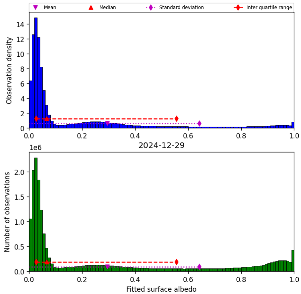
Figure 43: Histogram of “Fitted surface albedo” for 2024-12-29 to 2024-12-30
