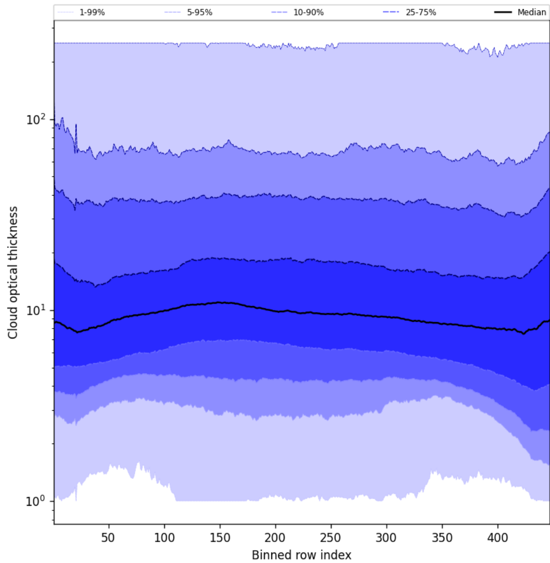
Figure 55: Along track statistics of “Cloud optical thickness” for 2024-12-29 to 2024-12-30
