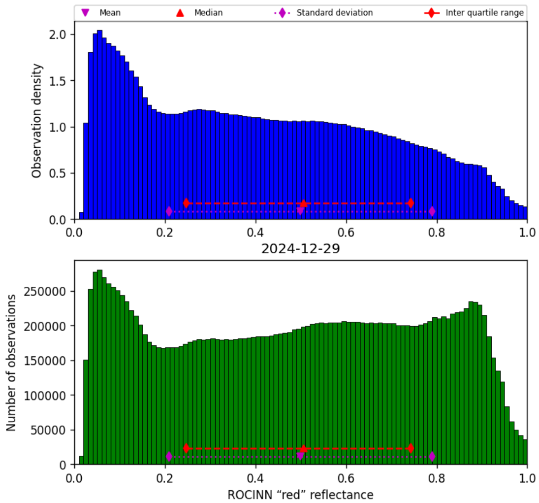
Figure 51: Histogram of “ROCINN “red” reflectance” for 2024-12-29 to 2024-12-30
