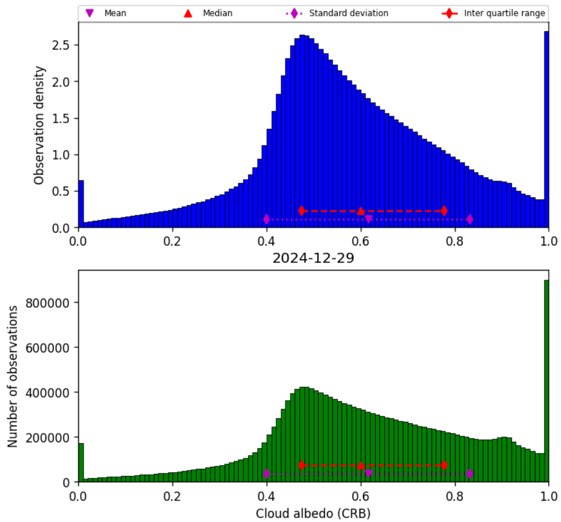
Figure 42: Histogram of “Cloud albedo (CRB)” for 2024-12-29 to 2024-12-30
