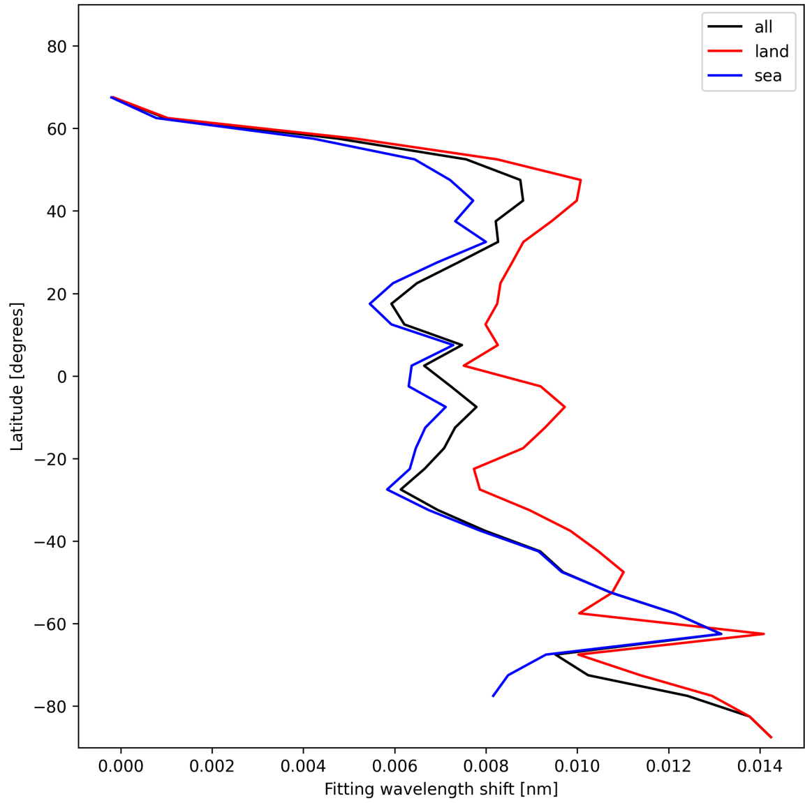
Figure 31: Zonal average of “Fitting wavelength shift” for 2024-12-29 to 2024-12-30.
