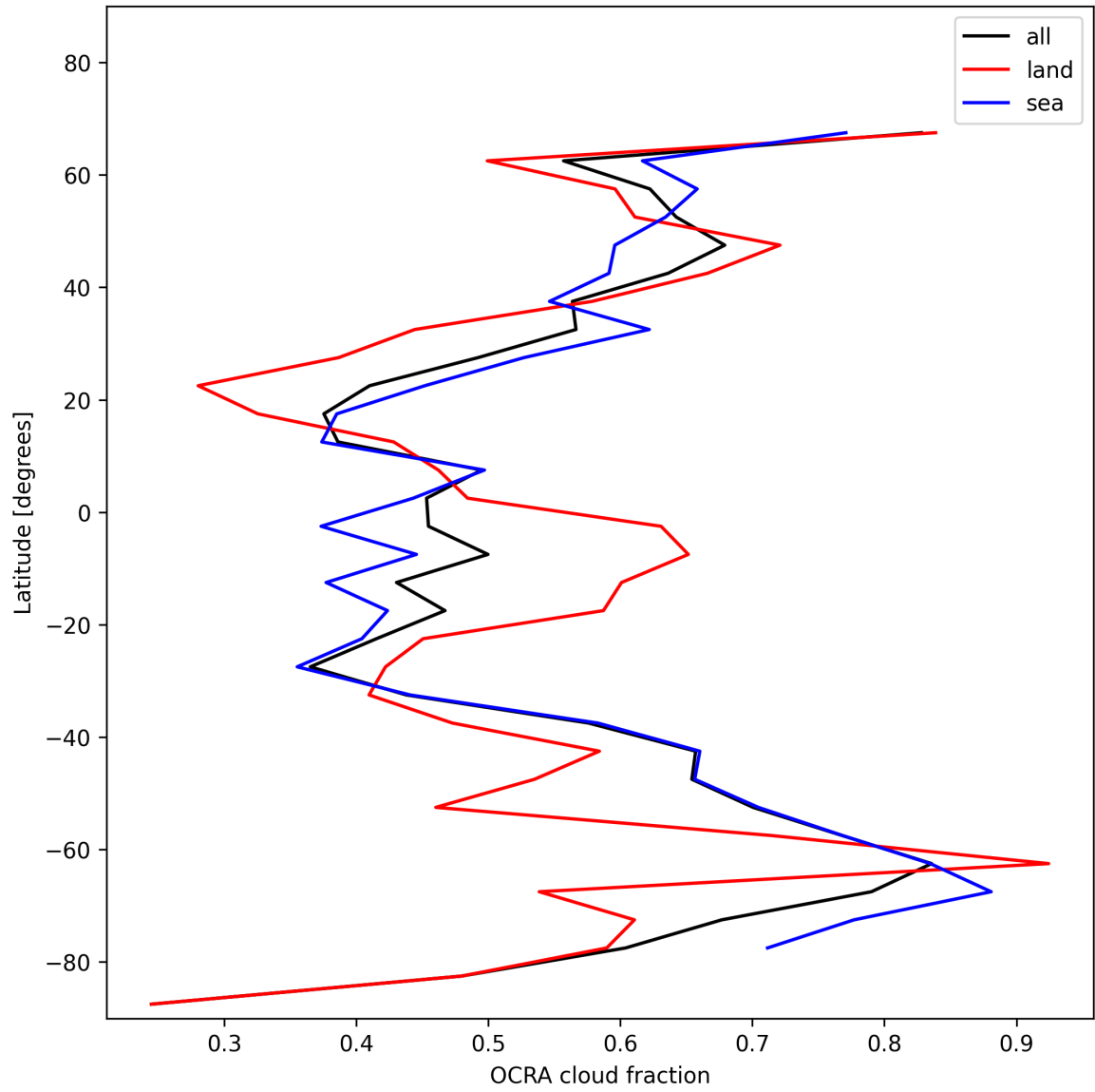
Figure 32: Zonal average of “OCRA cloud fraction” for 2024-12-29 to 2024-12-30.
