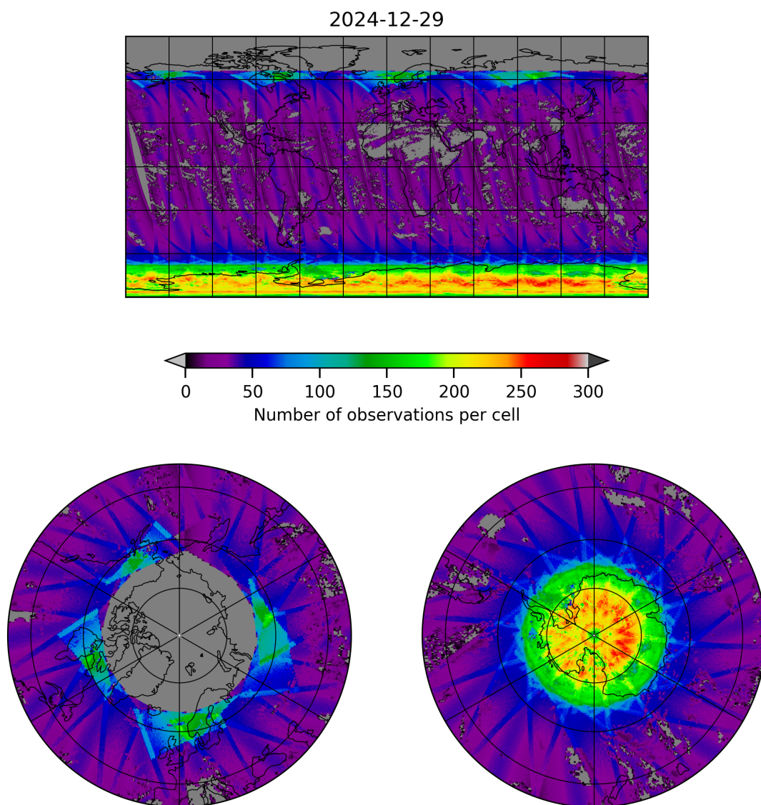
Figure 19: Map of the number of observations for 2024-12-29 to 2024-12-30
