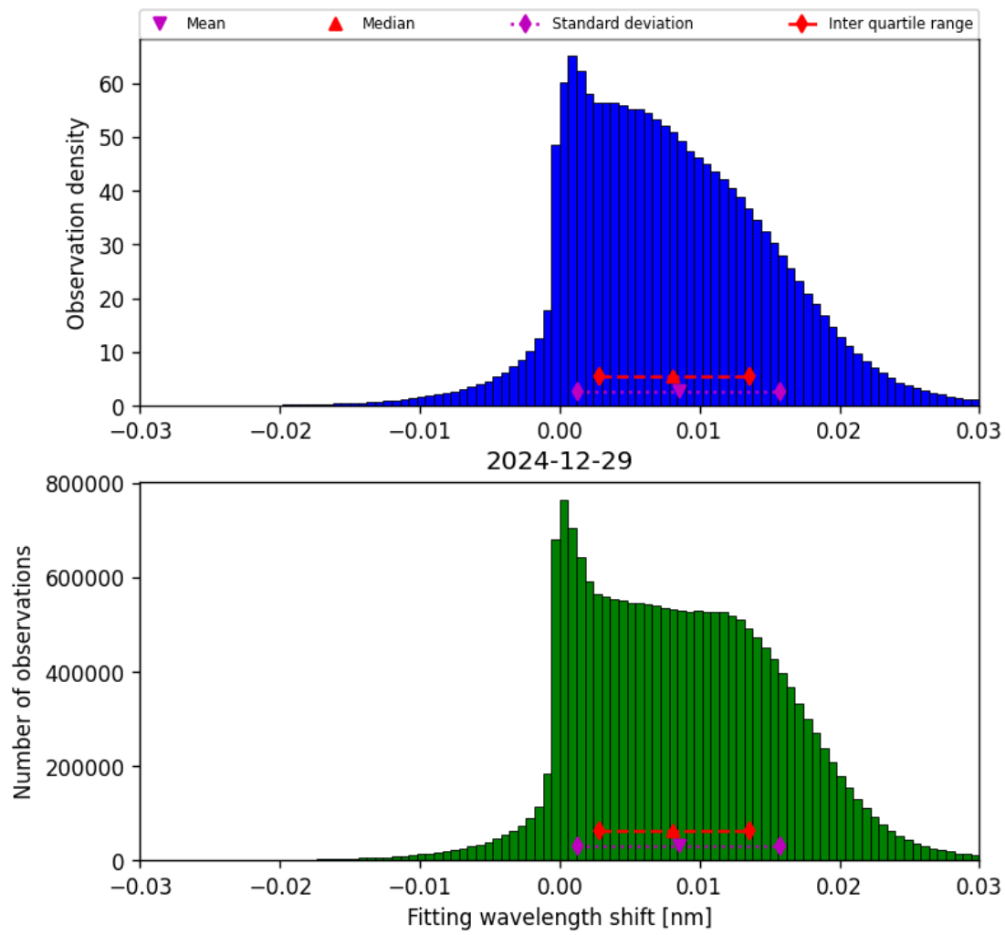
Figure 47: Histogram of “Fitting wavelength shift” for 2024-12-29 to 2024-12-30
