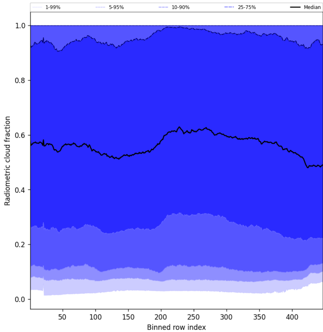
Figure 53: Along track statistics of “Radiometric cloud fraction” for 2024-12-29 to 2024-12-30
