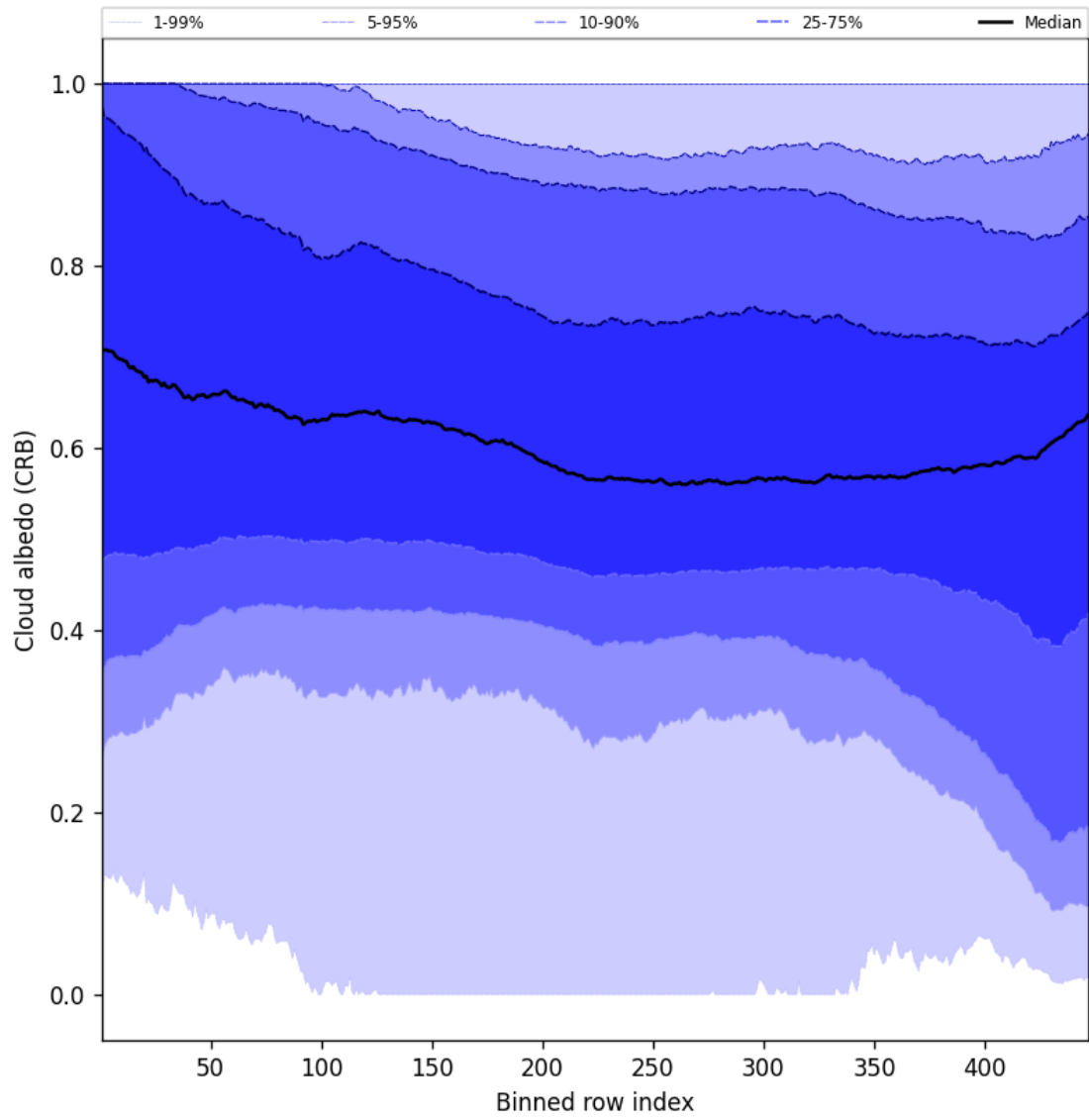
Figure 58: Along track statistics of “Cloud albedo (CRB)” for 2024-12-29 to 2024-12-30
