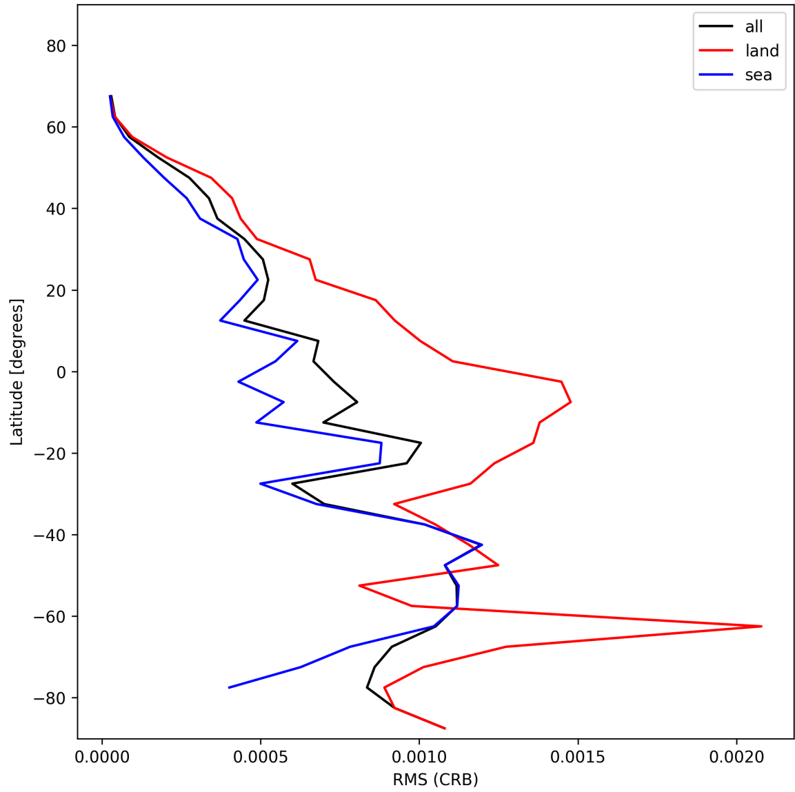
Figure 30: Zonal average of “RMS (CRB)” for 2024-12-29 to 2024-12-30.
