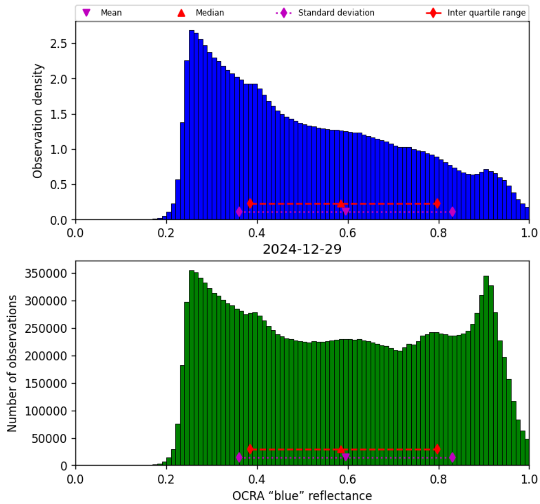
Figure 49: Histogram of “OCRA “blue” reflectance” for 2024-12-29 to 2024-12-30
