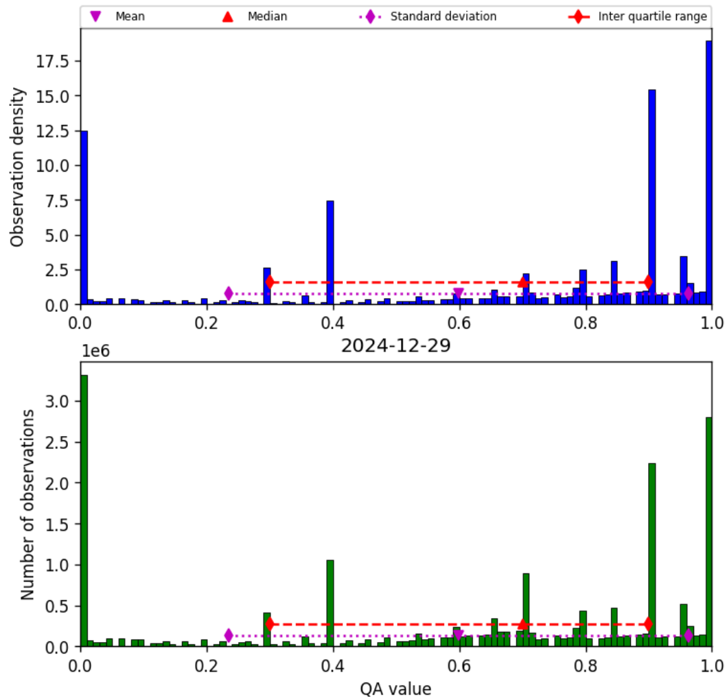
Figure 36: Histogram of “QA value” for 2024-12-29 to 2024-12-30
