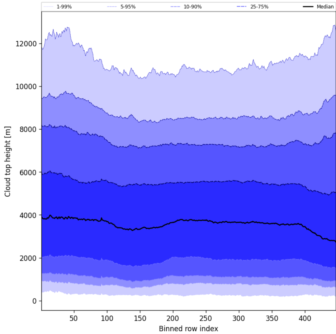
Figure 54: Along track statistics of “Cloud top height” for 2024-12-29 to 2024-12-30
