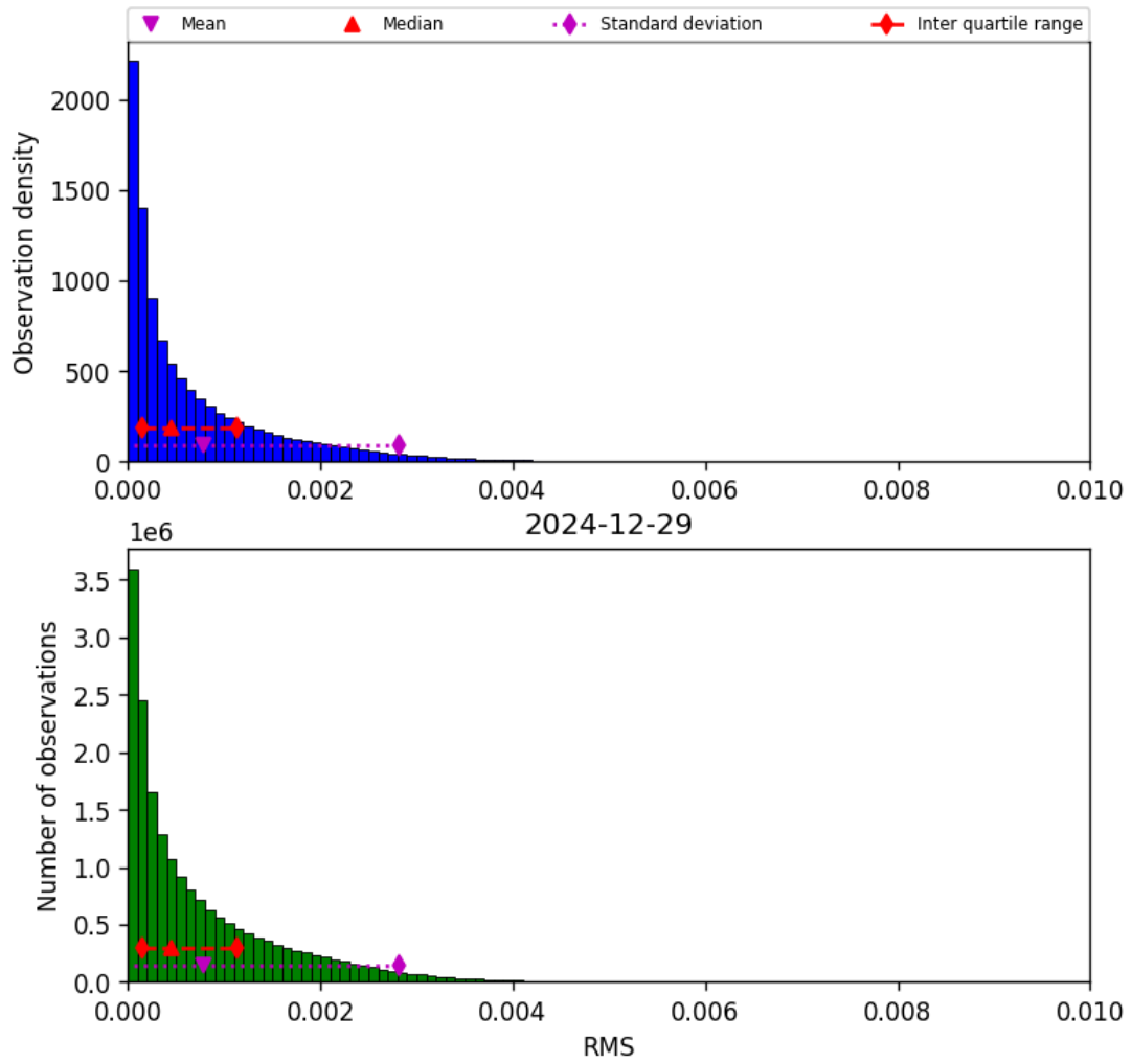
Figure 45: Histogram of “RMS” for 2024-12-29 to 2024-12-30
