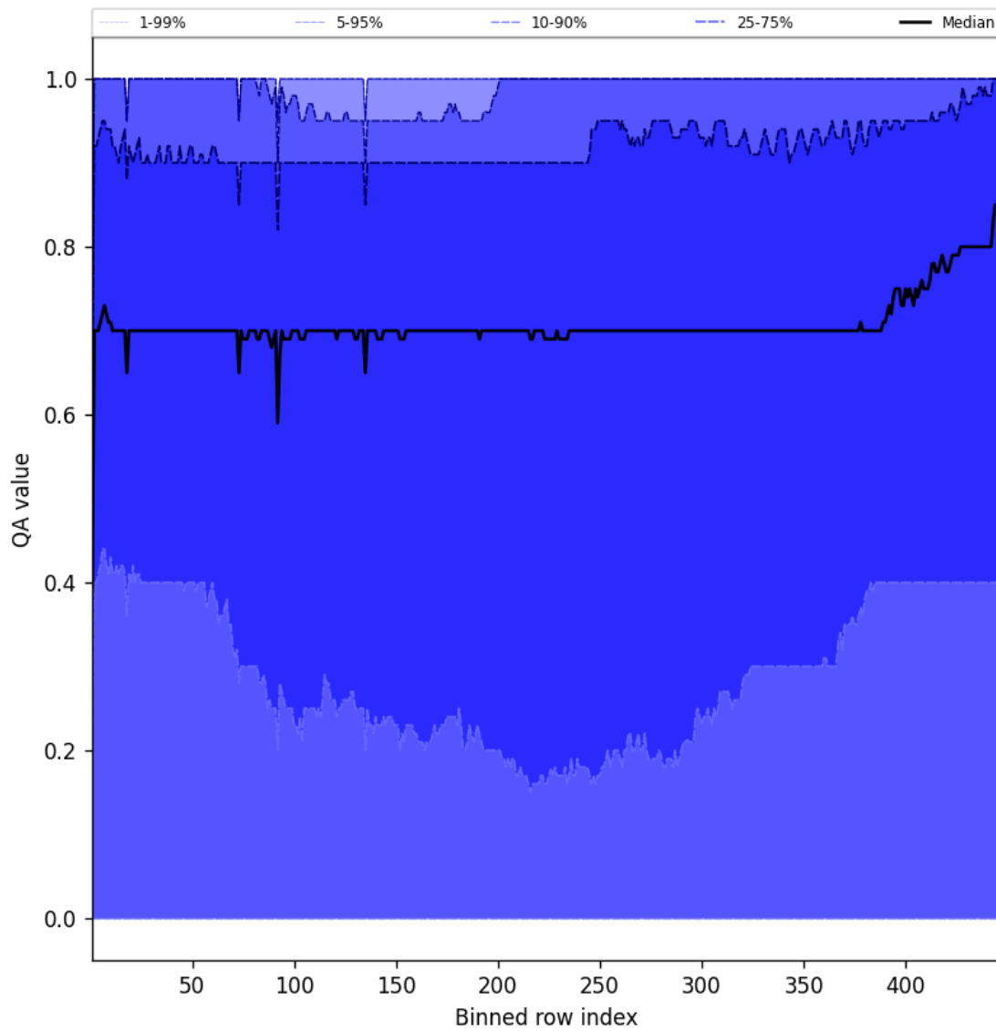
Figure 52: Along track statistics of “QA value” for 2024-12-29 to 2024-12-30
