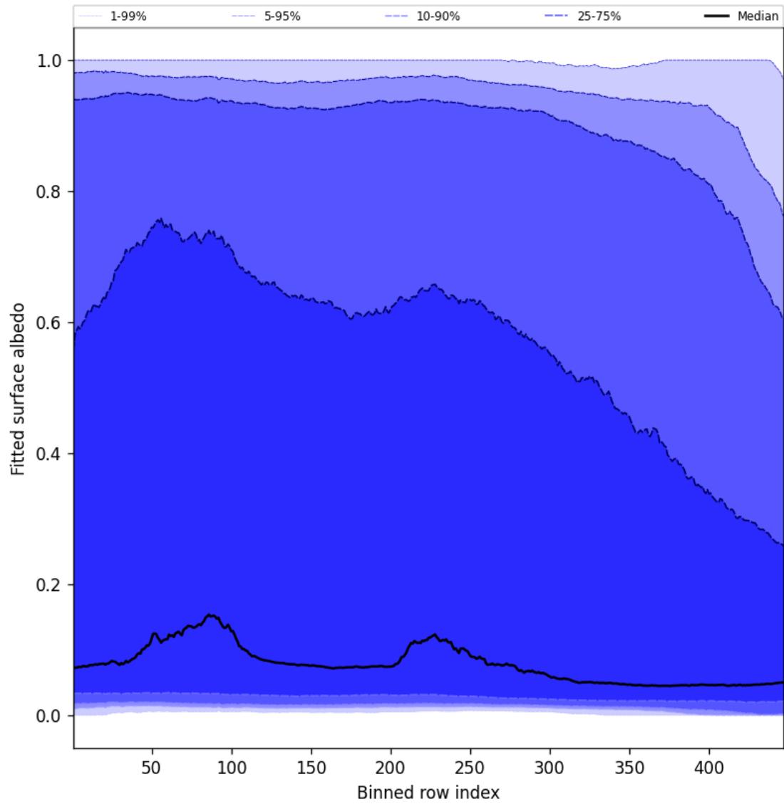
Figure 59: Along track statistics of “Fitted surface albedo” for 2024-12-29 to 2024-12-30
