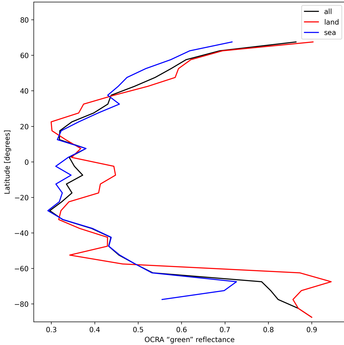
Figure 34: Zonal average of “OCRA “green” reflectance” for 2024-12-29 to 2024-12-30.
