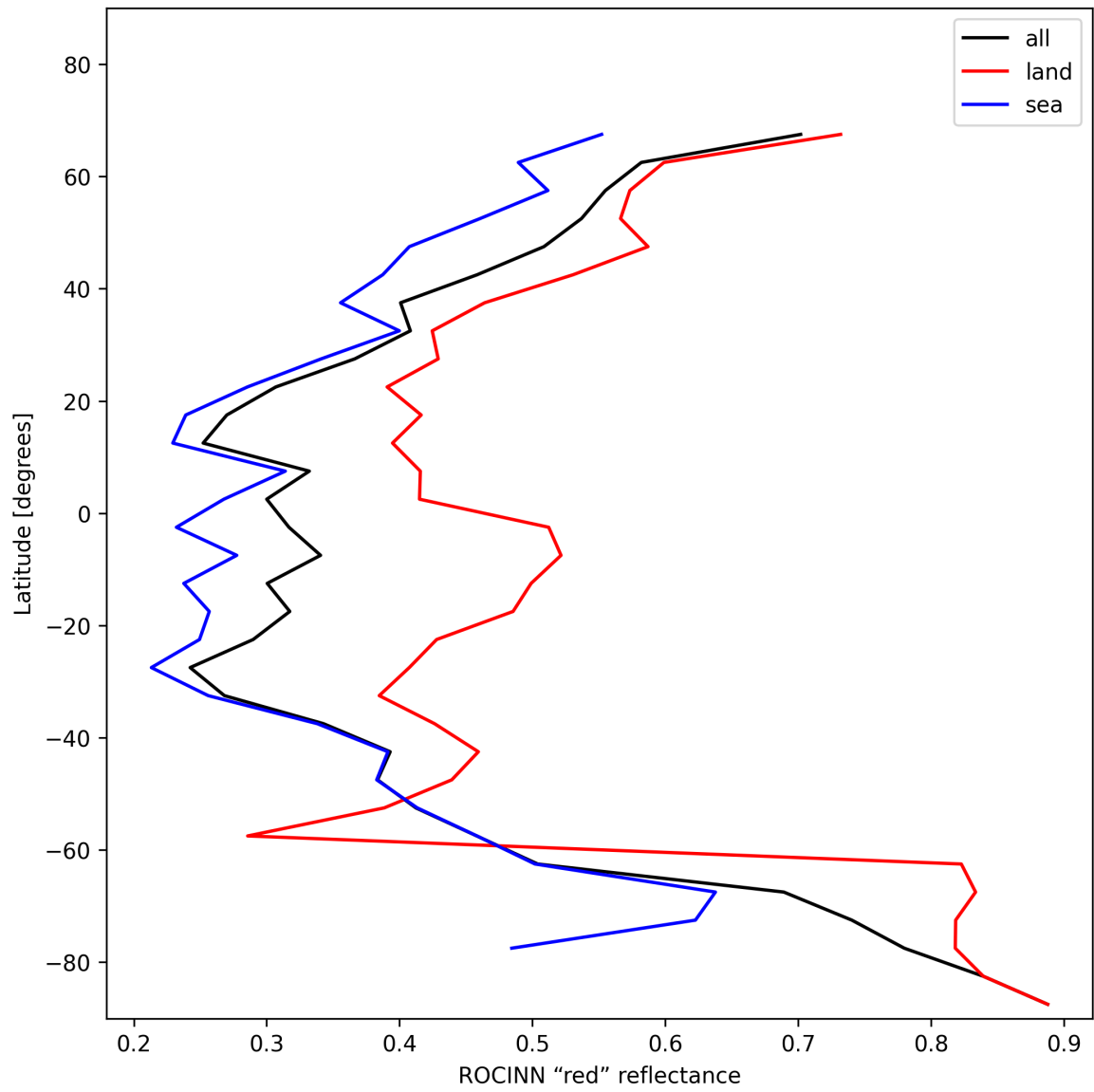
Figure 35: Zonal average of “ROCINN “red” reflectance” for 2024-12-29 to 2024-12-30.
