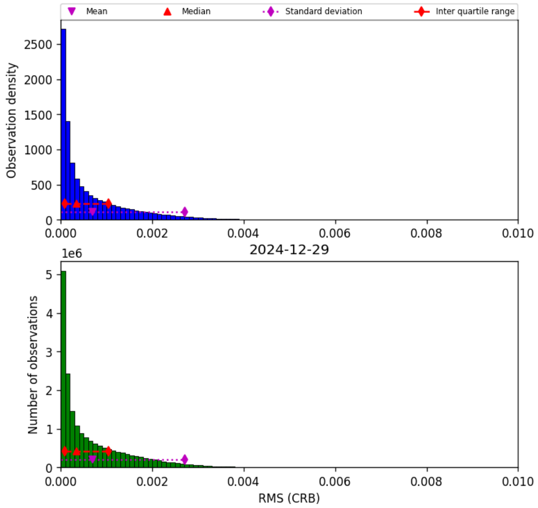
Figure 46: Histogram of “RMS (CRB)” for 2024-12-29 to 2024-12-30
