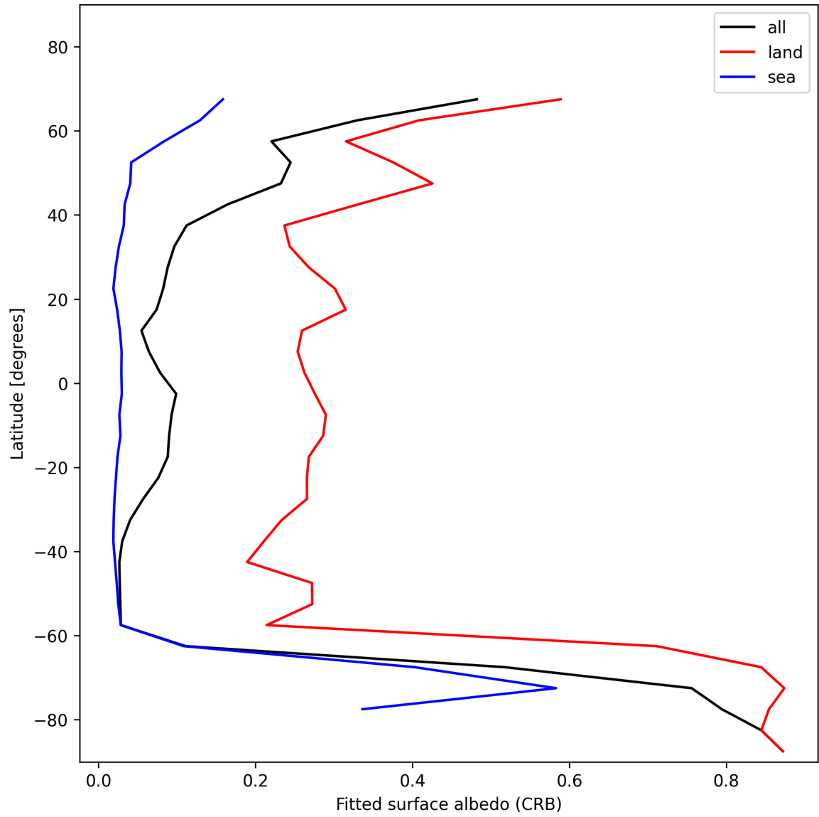
Figure 28: Zonal average of “Fitted surface albedo (CRB)” for 2024-12-29 to 2024-12-30.
