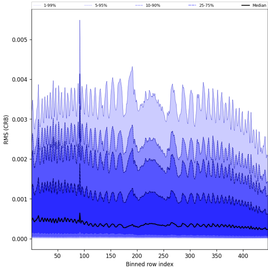
Figure 62: Along track statistics of “RMS (CRB)” for 2024-12-29 to 2024-12-30
