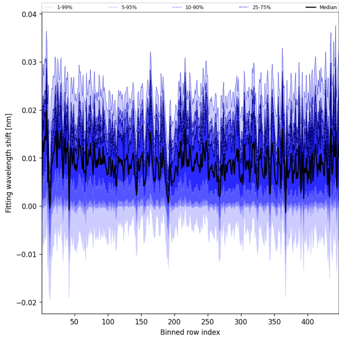
Figure 63: Along track statistics of “Fitting wavelength shift” for 2024-12-29 to 2024-12-30
