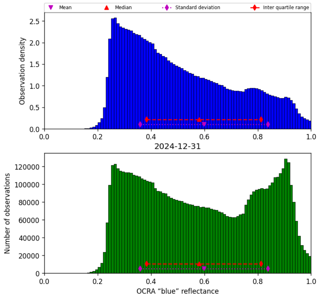
Figure 49: Histogram of “OCRA “blue” reflectance” for 2024-12-31 to 2024-12-31
