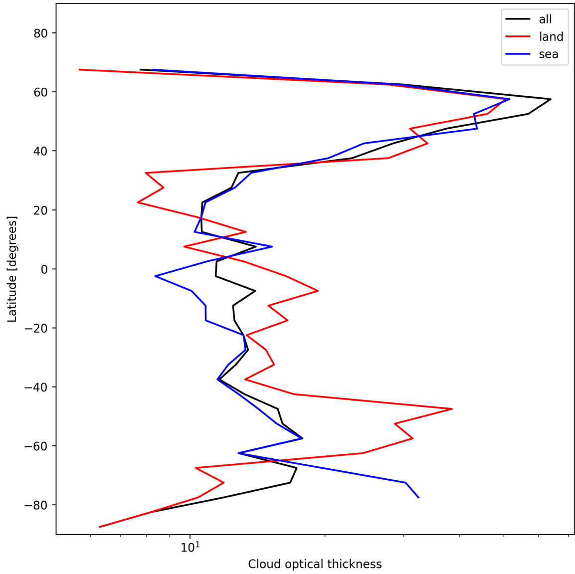
Figure 23: Zonal average of “Cloud optical thickness” for 2024-12-31 to 2024-12-31.
