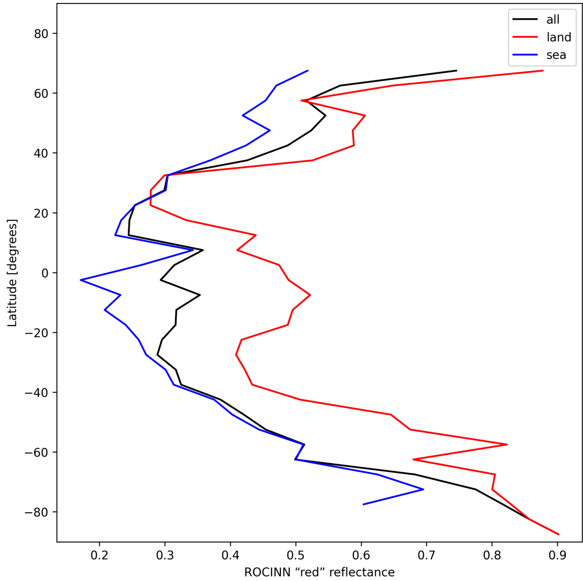
Figure 35: Zonal average of "ROCINN "red" reflectance" for 2024-12-31 to 2024-12-31.
