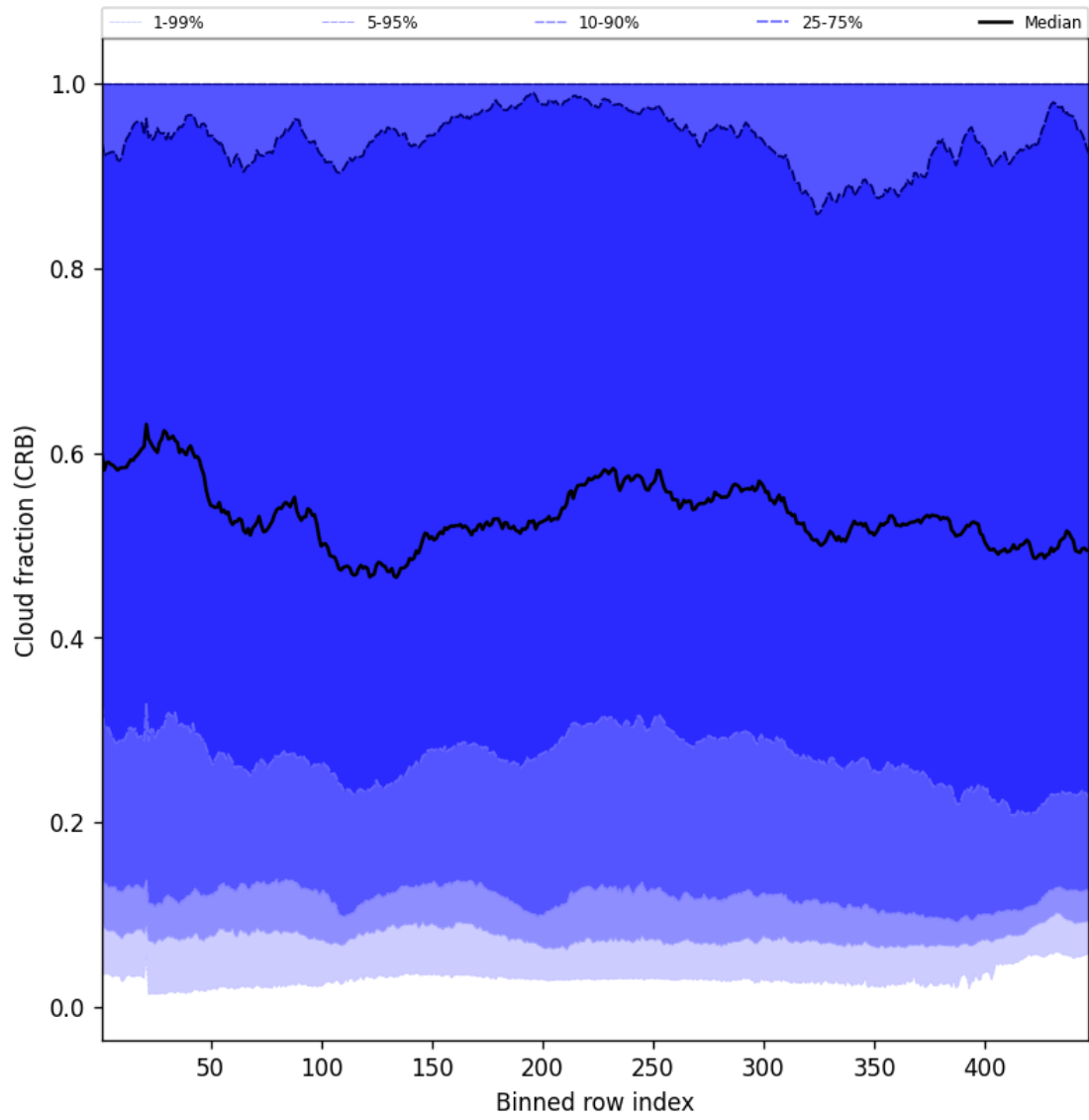
Figure 56: Along track statistics of “Cloud fraction (CRB)” for 2024-12-31 to 2024-12-31
