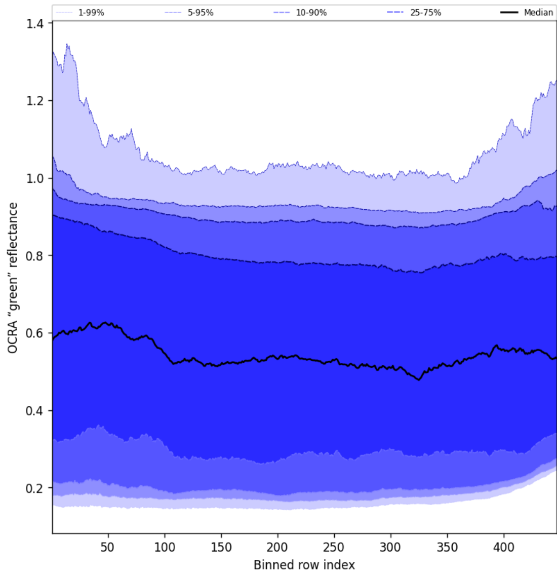
Figure 66: Along track statistics of “OCRA “green” reflectance” for 2024-12-31 to 2024-12-31
