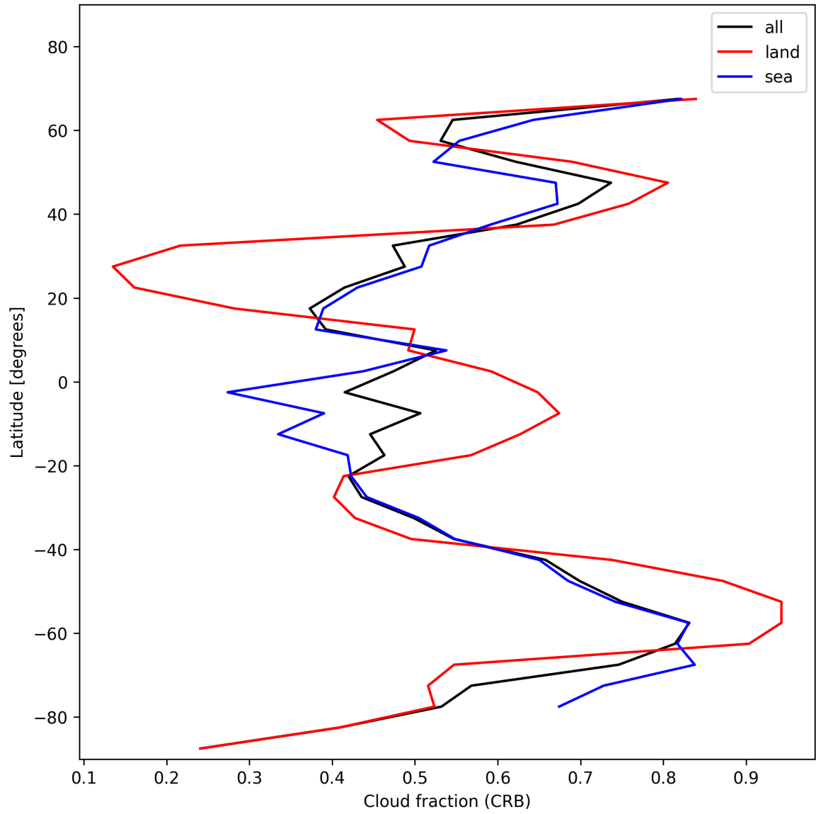
Figure 24: Zonal average of “Cloud fraction (CRB)” for 2024-12-31 to 2024-12-31.
