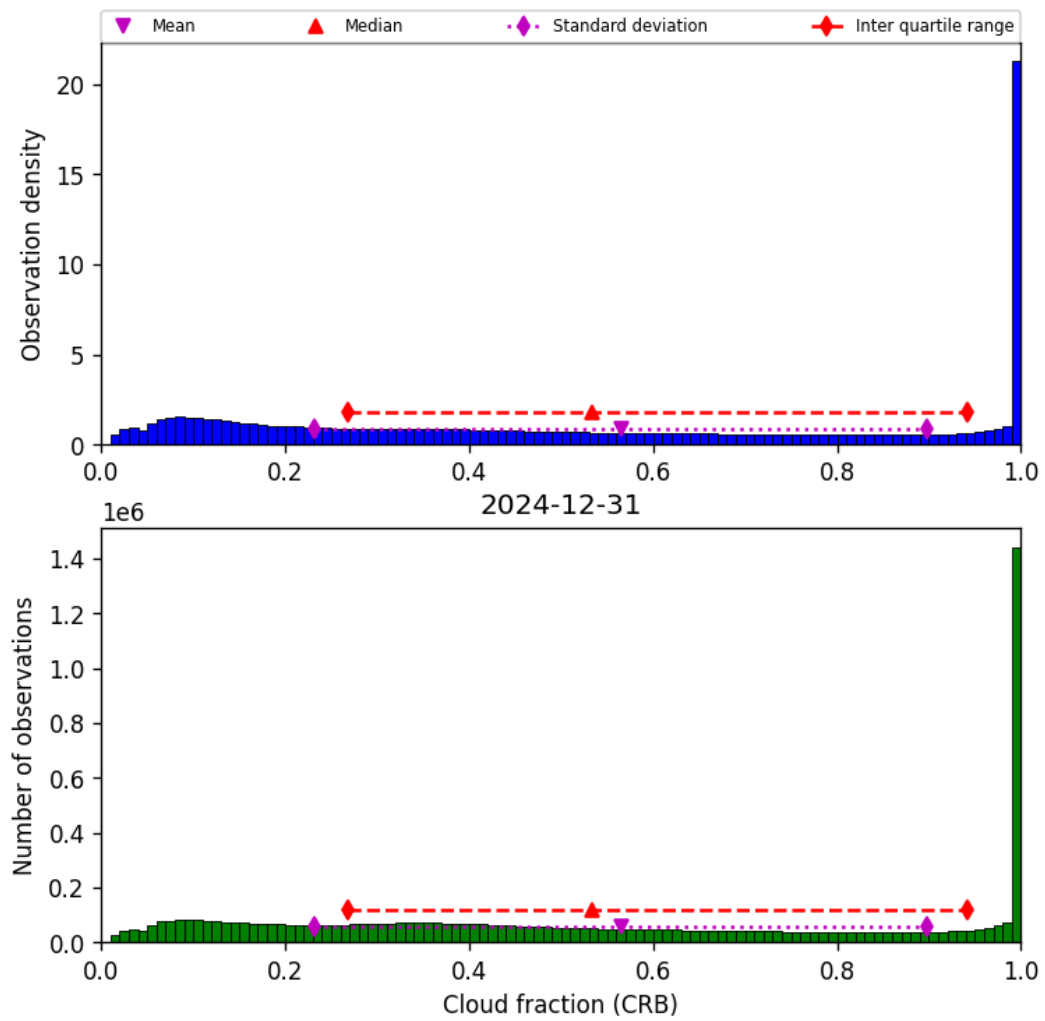
Figure 40: Histogram of “Cloud fraction (CRB)” for 2024-12-31 to 2024-12-31
