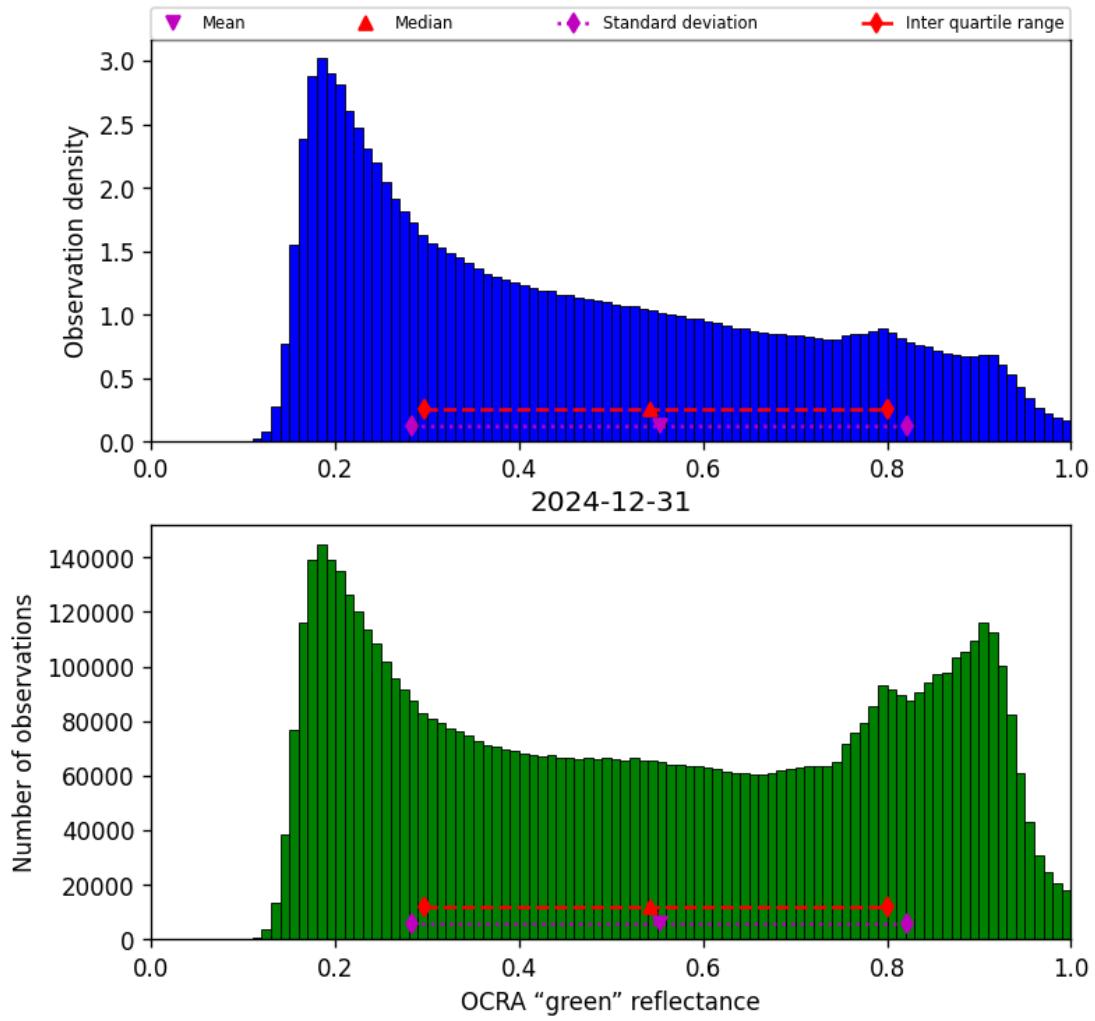
Figure 50: Histogram of “OCRA “green” reflectance” for 2024-12-31 to 2024-12-31
