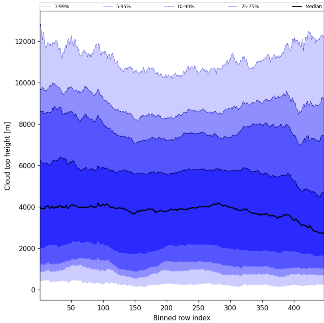
Figure 54: Along track statistics of “Cloud top height” for 2024-12-31 to 2024-12-31
