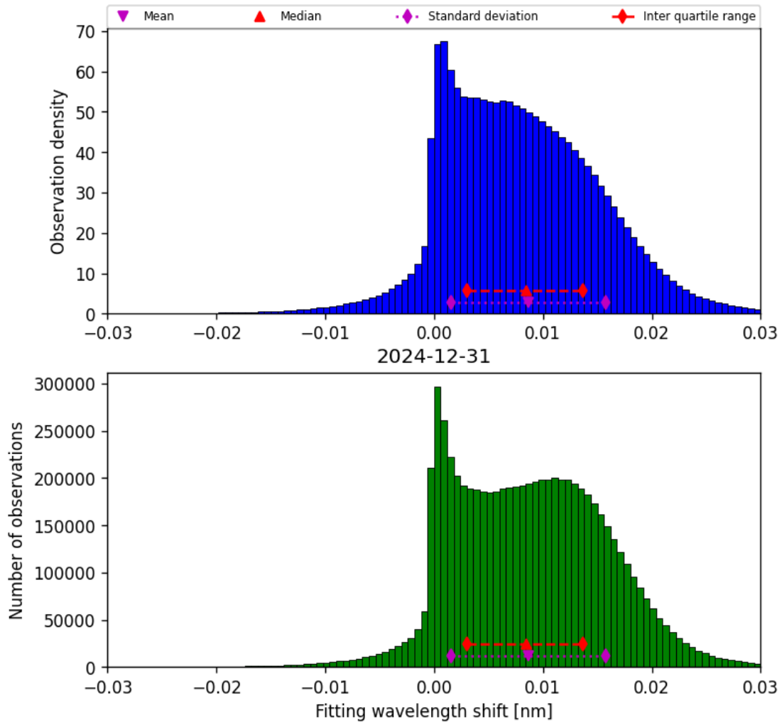
Figure 47: Histogram of “Fitting wavelength shift” for 2024-12-31 to 2024-12-31
