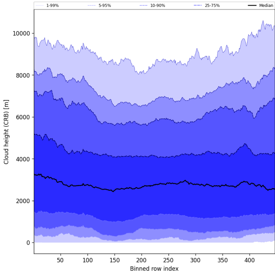
Figure 57: Along track statistics of “Cloud height (CRB)” for 2024-12-31 to 2024-12-31
