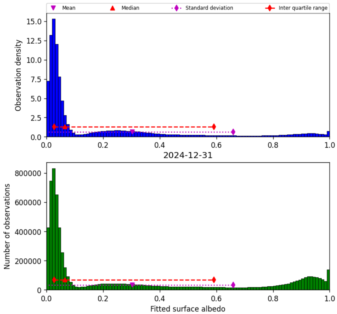
Figure 43: Histogram of “Fitted surface albedo” for 2024-12-31 to 2024-12-31
