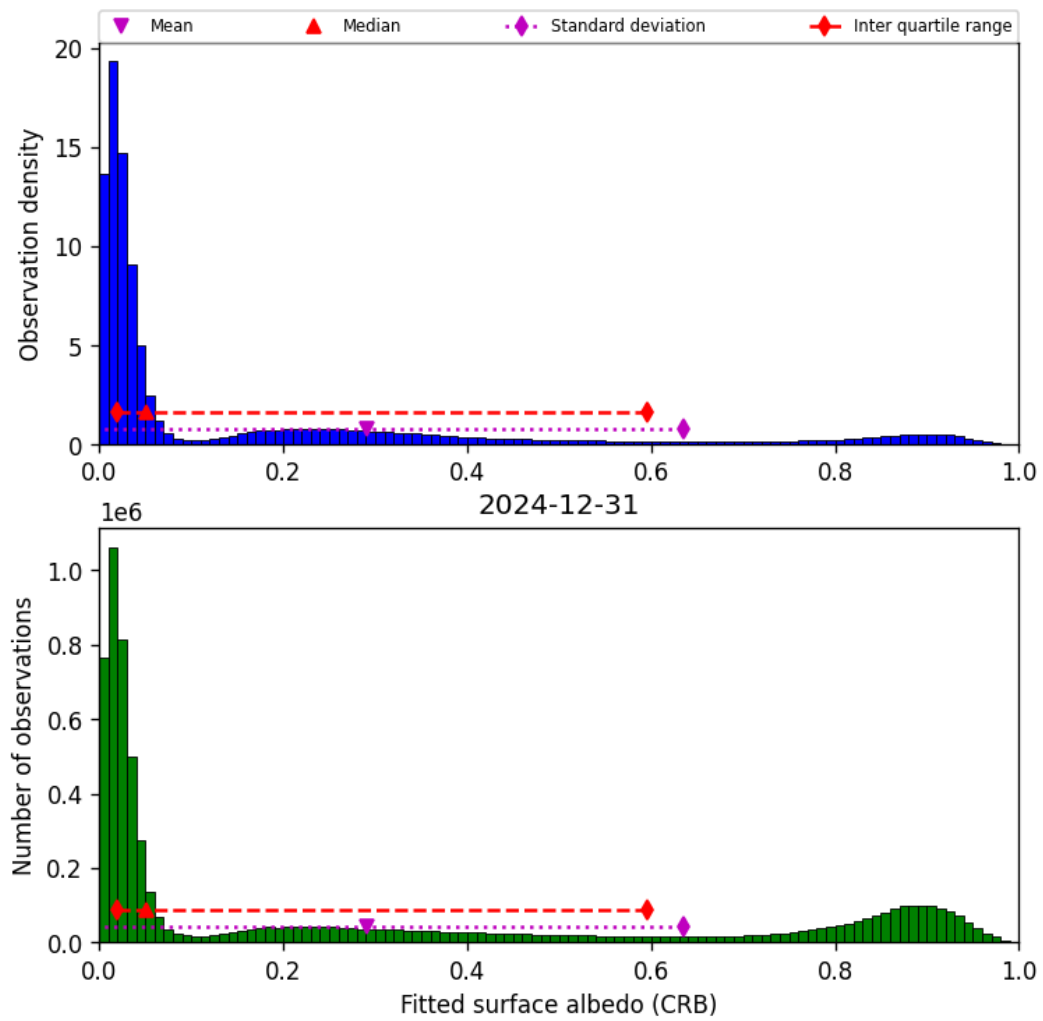
Figure 44: Histogram of “Fitted surface albedo (CRB)” for 2024-12-31 to 2024-12-31
