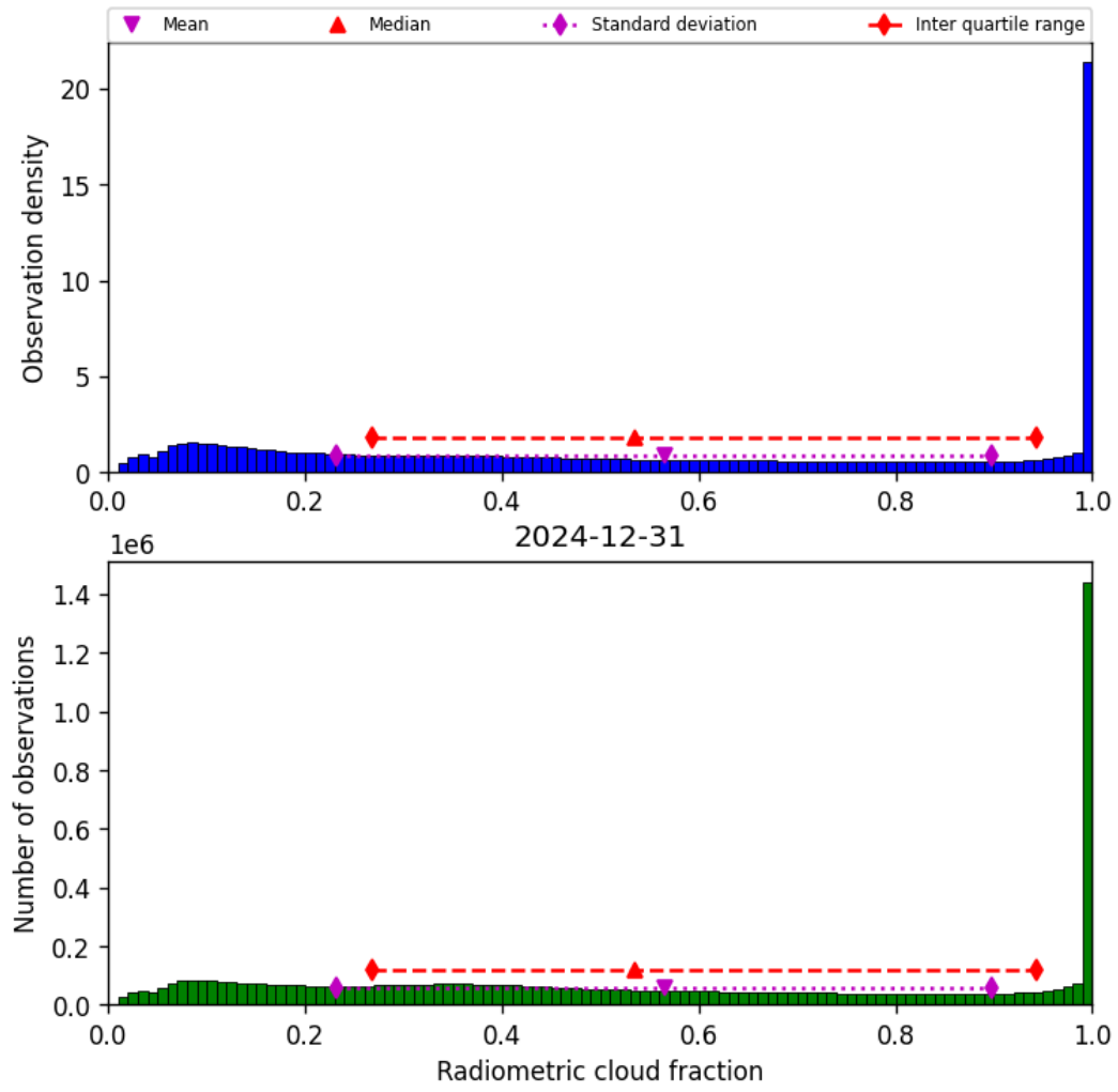
Figure 37: Histogram of “Radiometric cloud fraction” for 2024-12-31 to 2024-12-31
