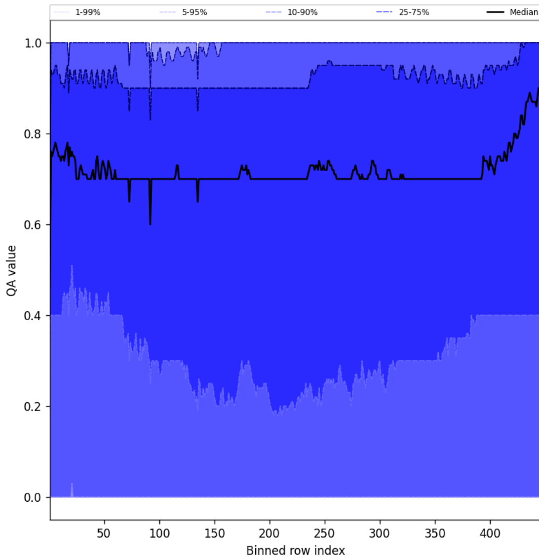
Figure 52: Along track statistics of “QA value” for 2024-12-31 to 2024-12-31
