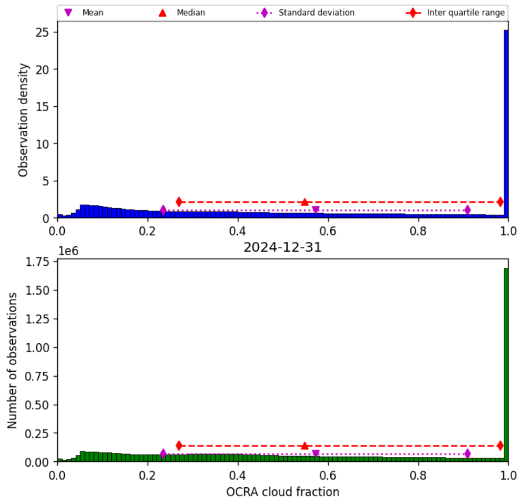
Figure 48: Histogram of “OCRA cloud fraction” for 2024-12-31 to 2024-12-31
