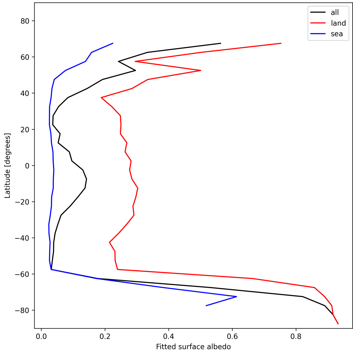
Figure 27: Zonal average of “Fitted surface albedo” for 2024-12-31 to 2024-12-31.
