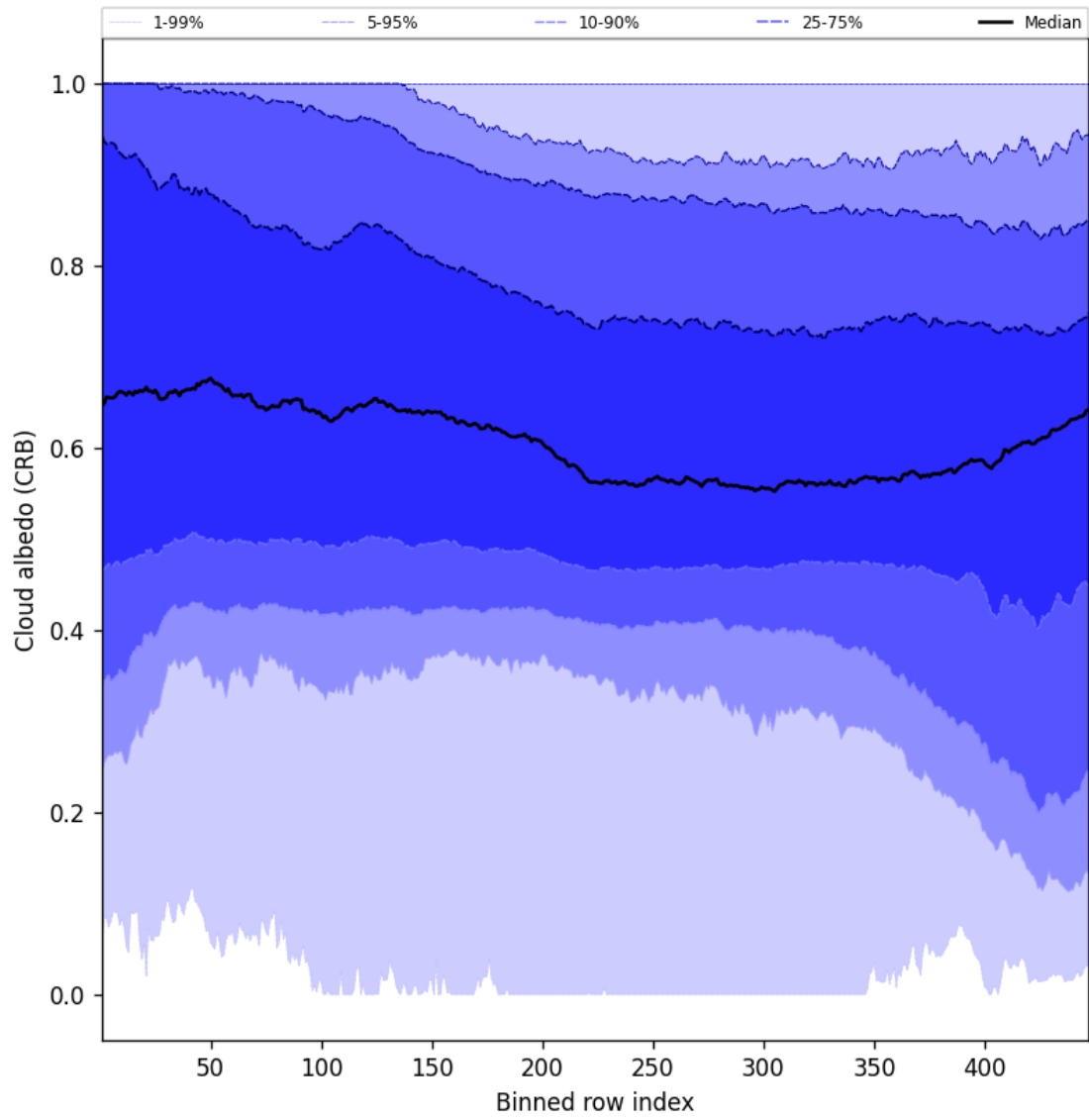
Figure 58: Along track statistics of “Cloud albedo (CRB)” for 2024-12-31 to 2024-12-31
