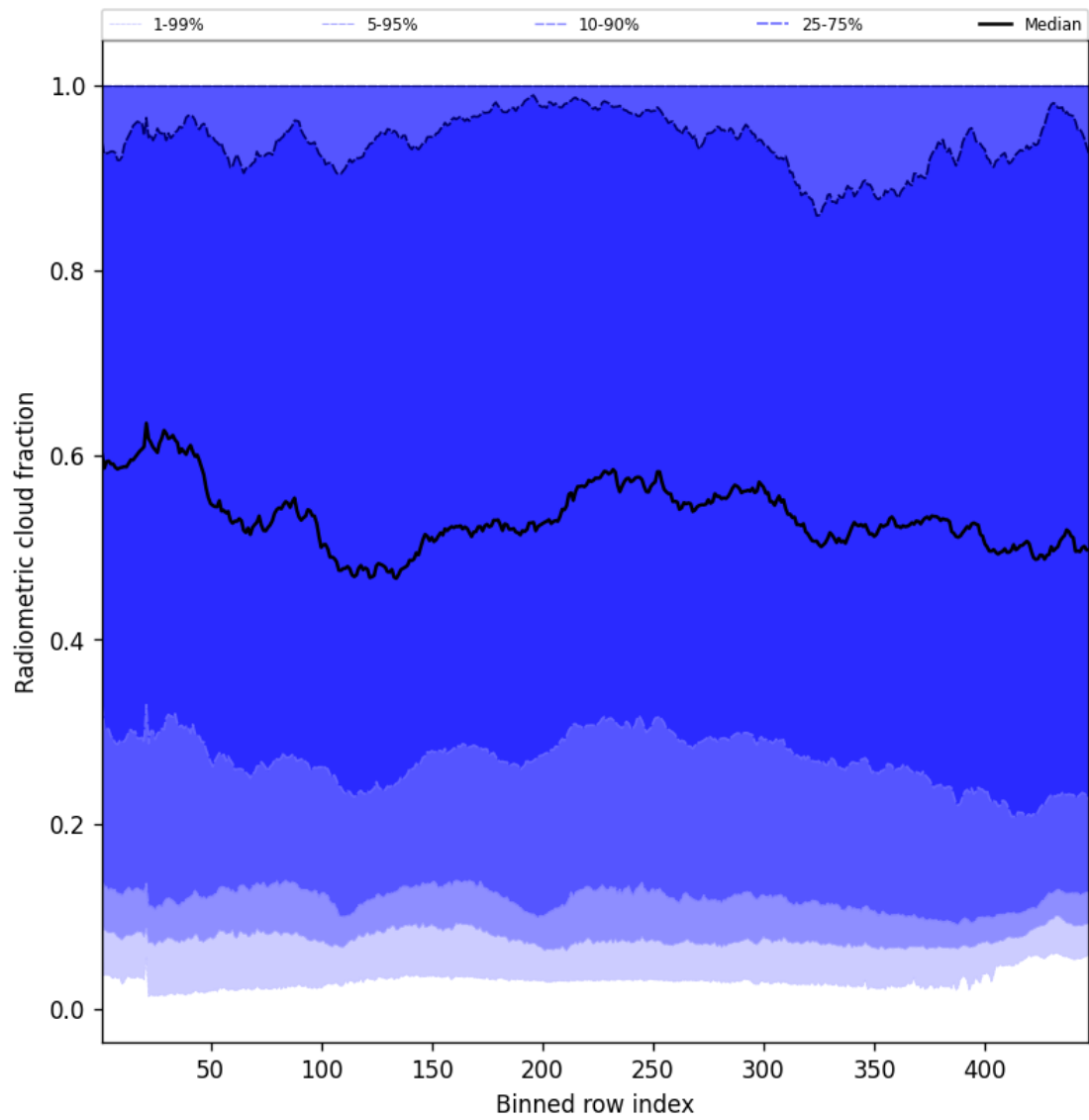
Figure 53: Along track statistics of “Radiometric cloud fraction” for 2024-12-31 to 2024-12-31
