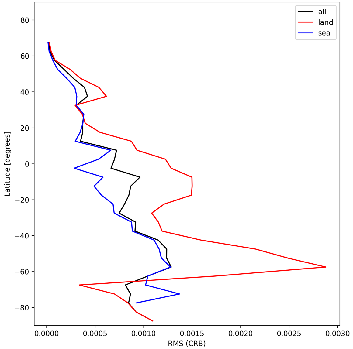
Figure 30: Zonal average of “RMS (CRB)” for 2024-12-31 to 2024-12-31.
