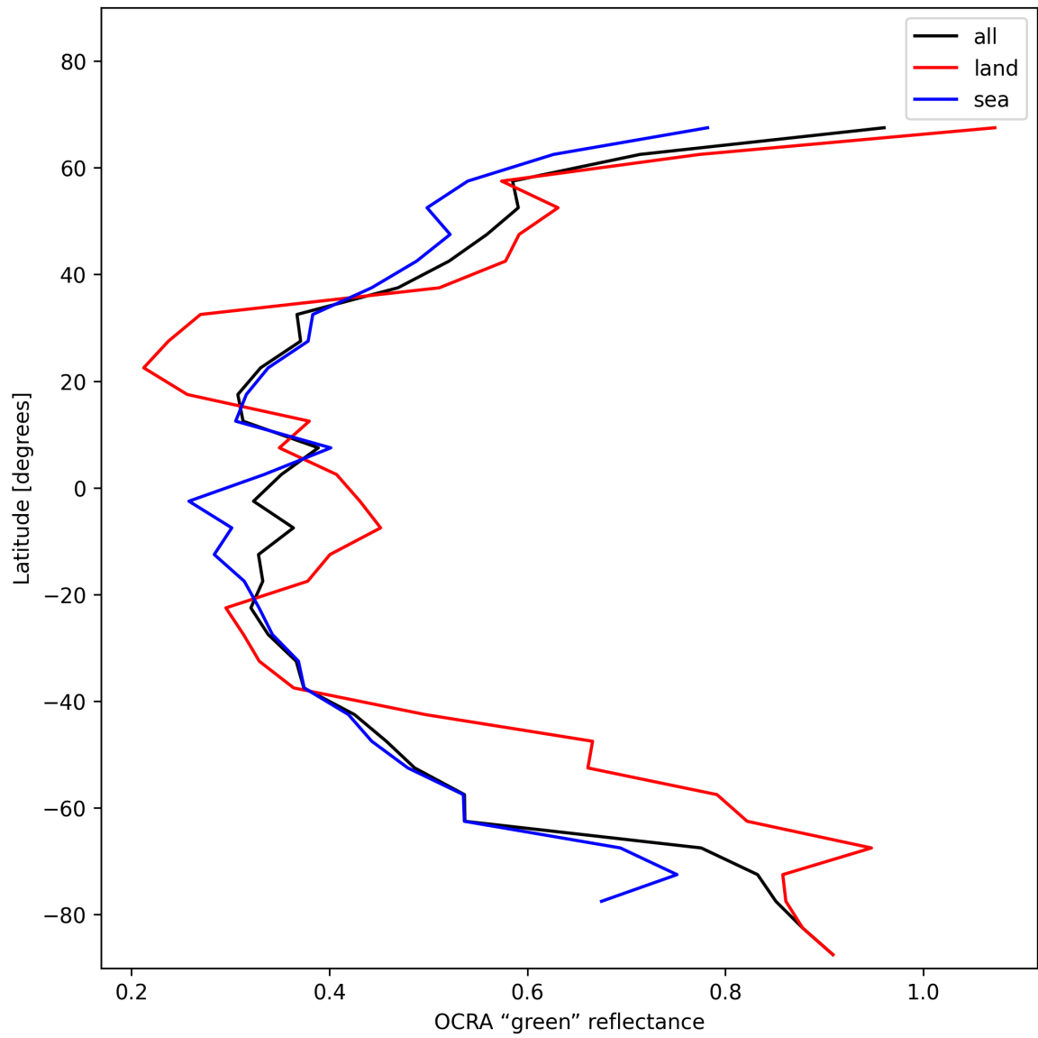
Figure 34: Zonal average of “OCRA “green” reflectance” for 2024-12-31 to 2024-12-31.
