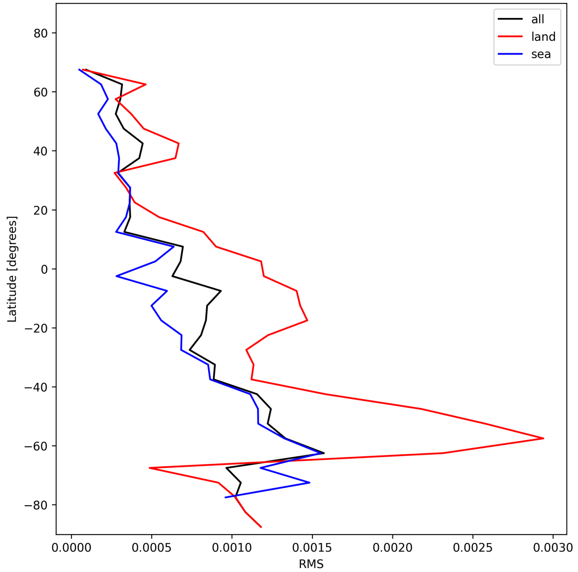
Figure 29: Zonal average of “RMS” for 2024-12-31 to 2024-12-31.
