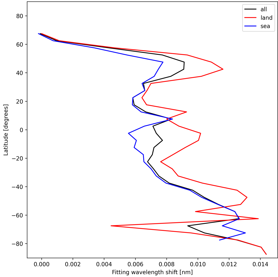
Figure 31: Zonal average of “Fitting wavelength shift” for 2024-12-31 to 2024-12-31.
