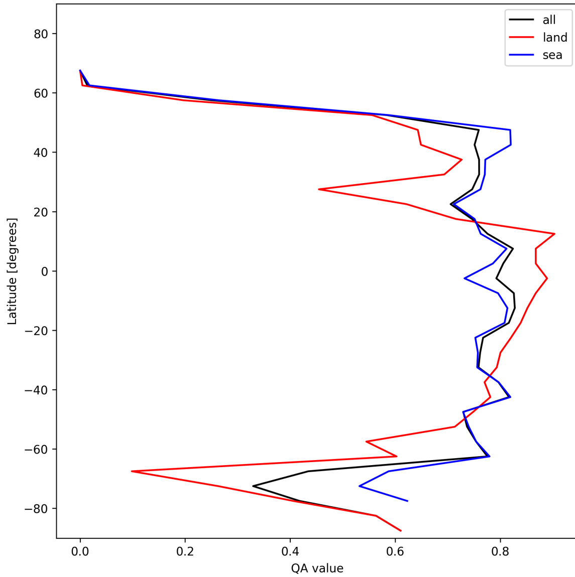
Figure 20: Zonal average of “QA value” for 2024-12-31 to 2024-12-31.
