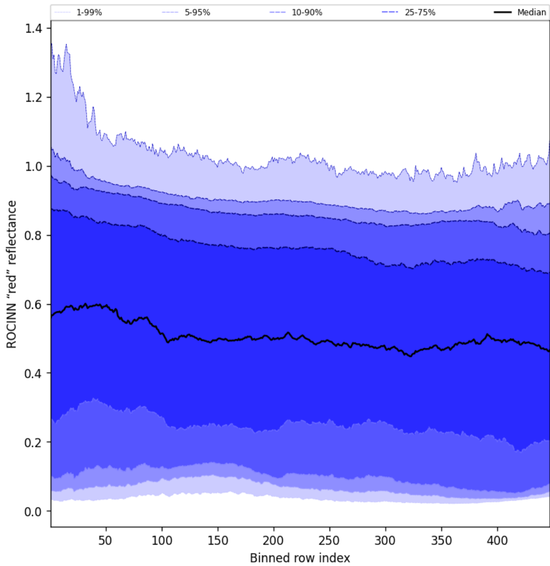
Figure 67: Along track statistics of “ROCINN “red” reflectance” for 2024-12-31 to 2024-12-31
