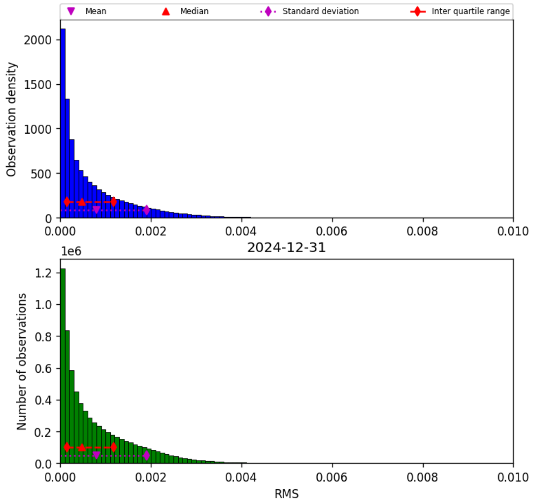
Figure 45: Histogram of “RMS” for 2024-12-31 to 2024-12-31
