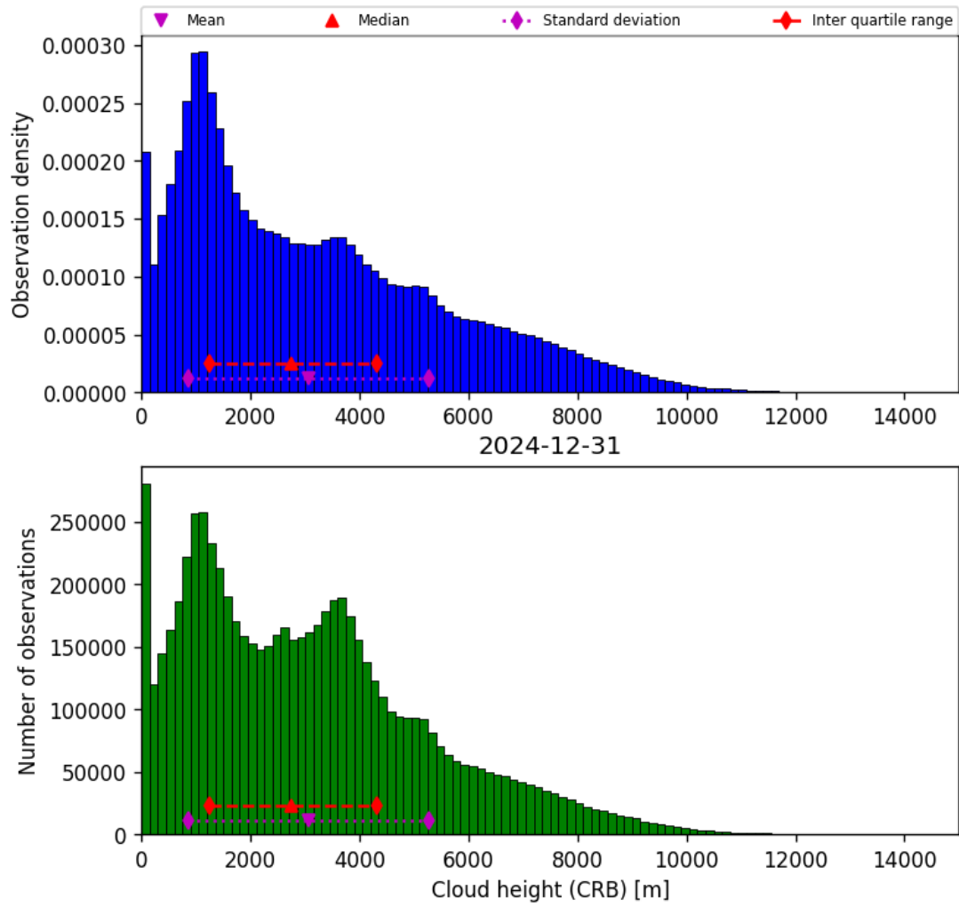
Figure 41: Histogram of “Cloud height (CRB)” for 2024-12-31 to 2024-12-31
