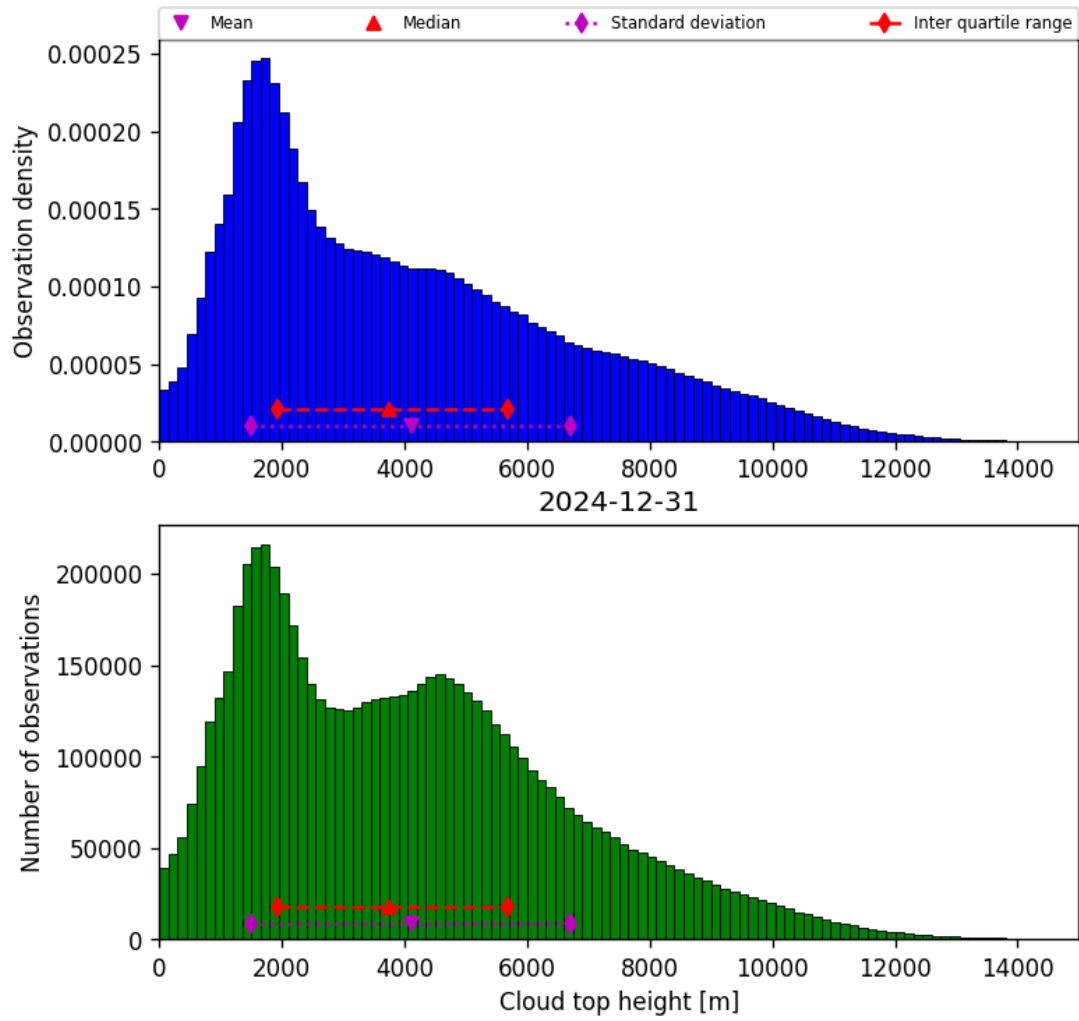
Figure 38: Histogram of “Cloud top height” for 2024-12-31 to 2024-12-31
