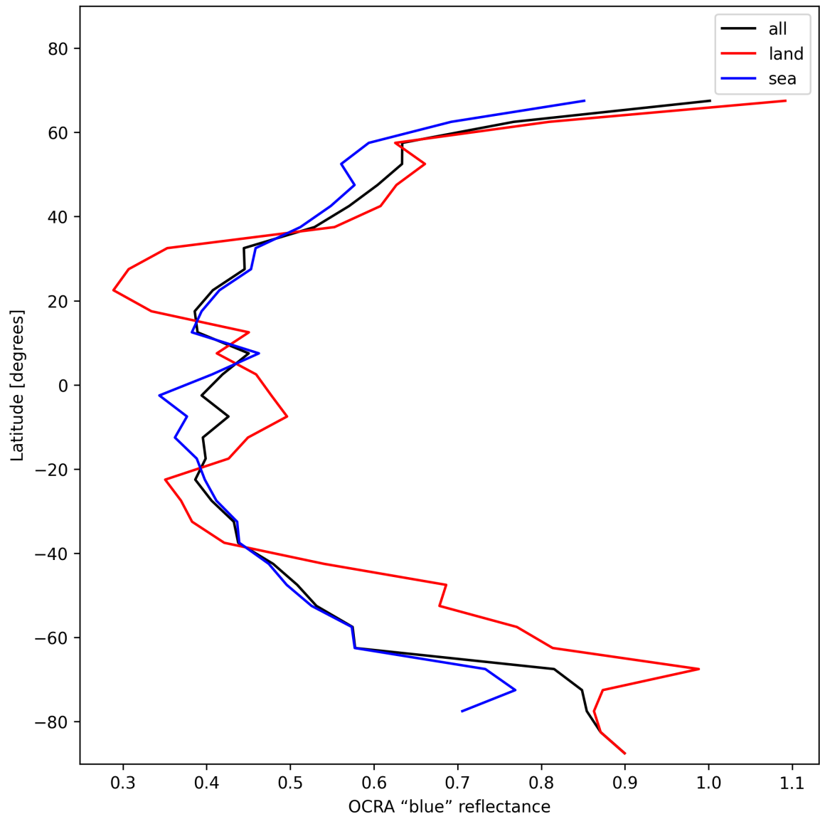
Figure 33: Zonal average of “OCRA “blue” reflectance” for 2024-12-31 to 2024-12-31.
