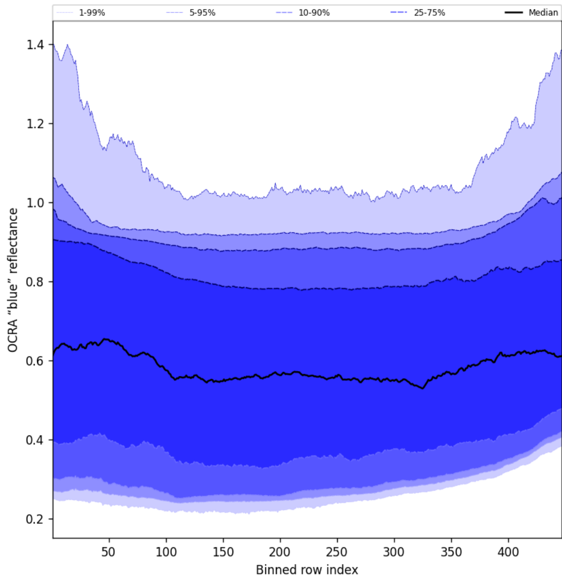
Figure 65: Along track statistics of “OCRA “blue” reflectance” for 2024-12-31 to 2024-12-31
