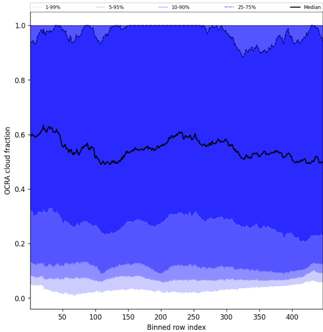
Figure 64: Along track statistics of “OCRA cloud fraction” for 2024-12-31 to 2024-12-31
