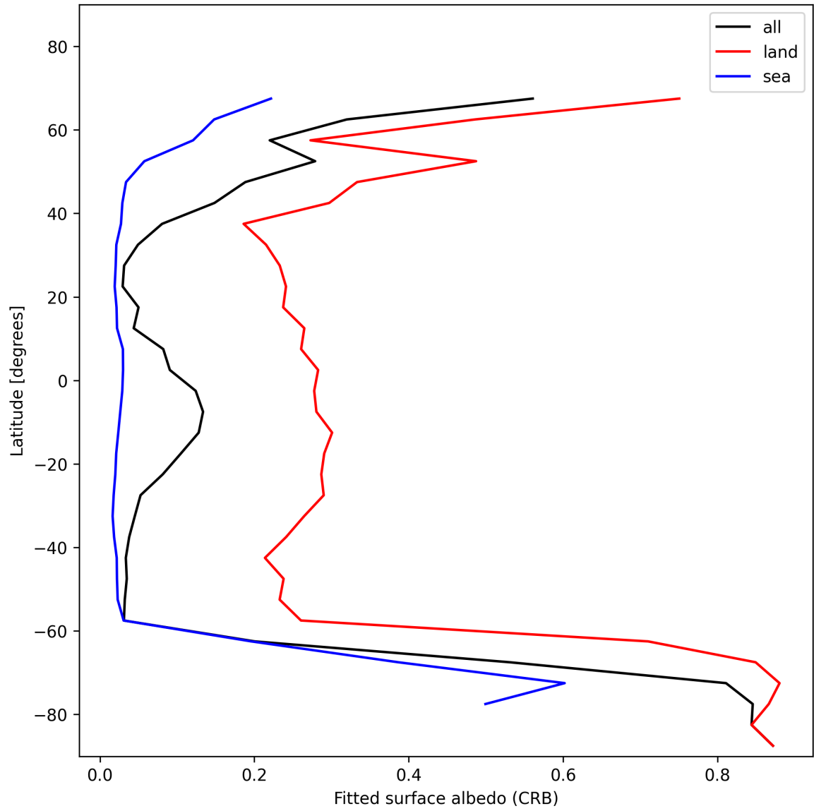
Figure 28: Zonal average of “Fitted surface albedo (CRB)” for 2024-12-31 to 2024-12-31.
