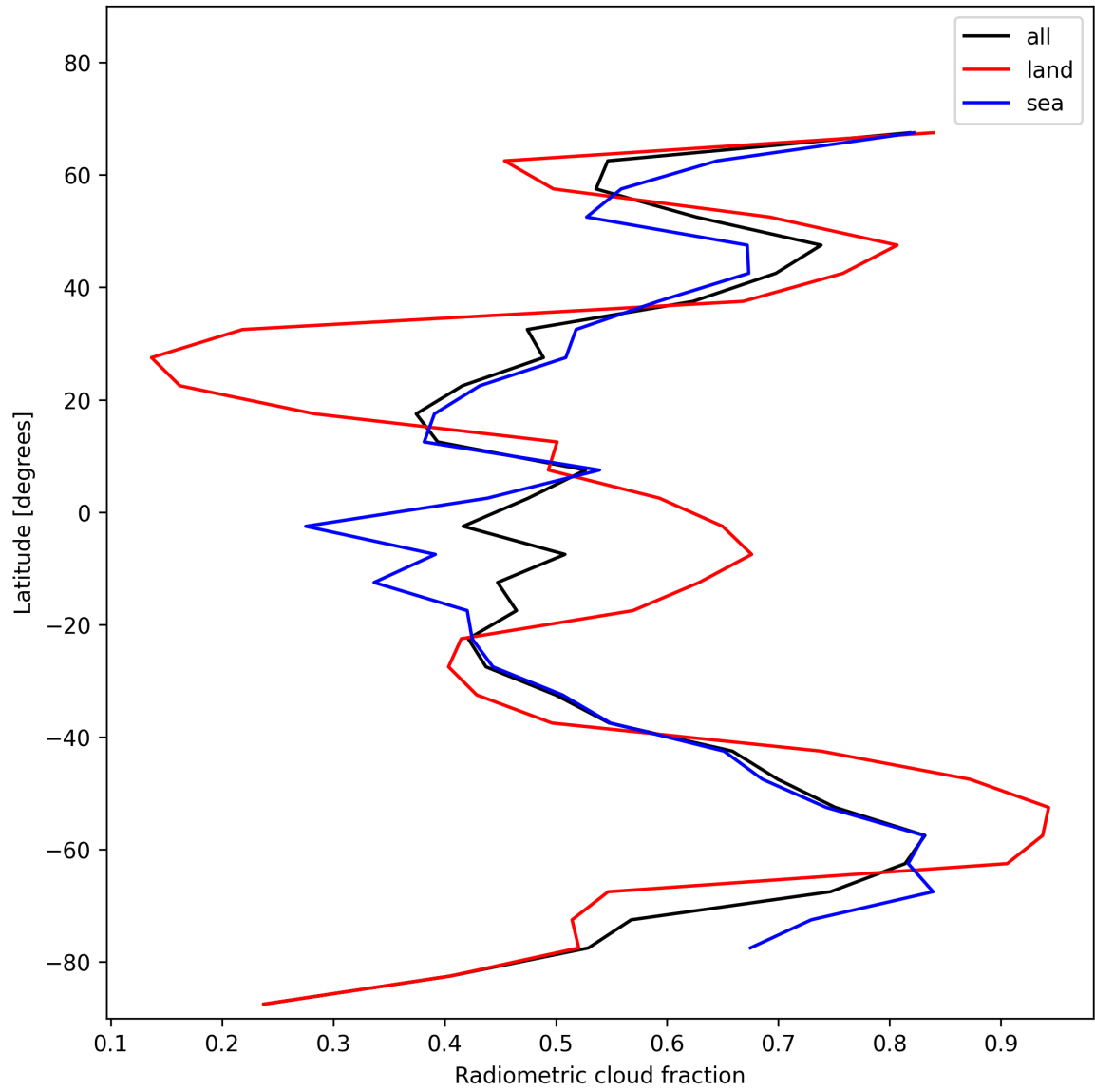
Figure 21: Zonal average of “Radiometric cloud fraction” for 2024-12-31 to 2024-12-31.
