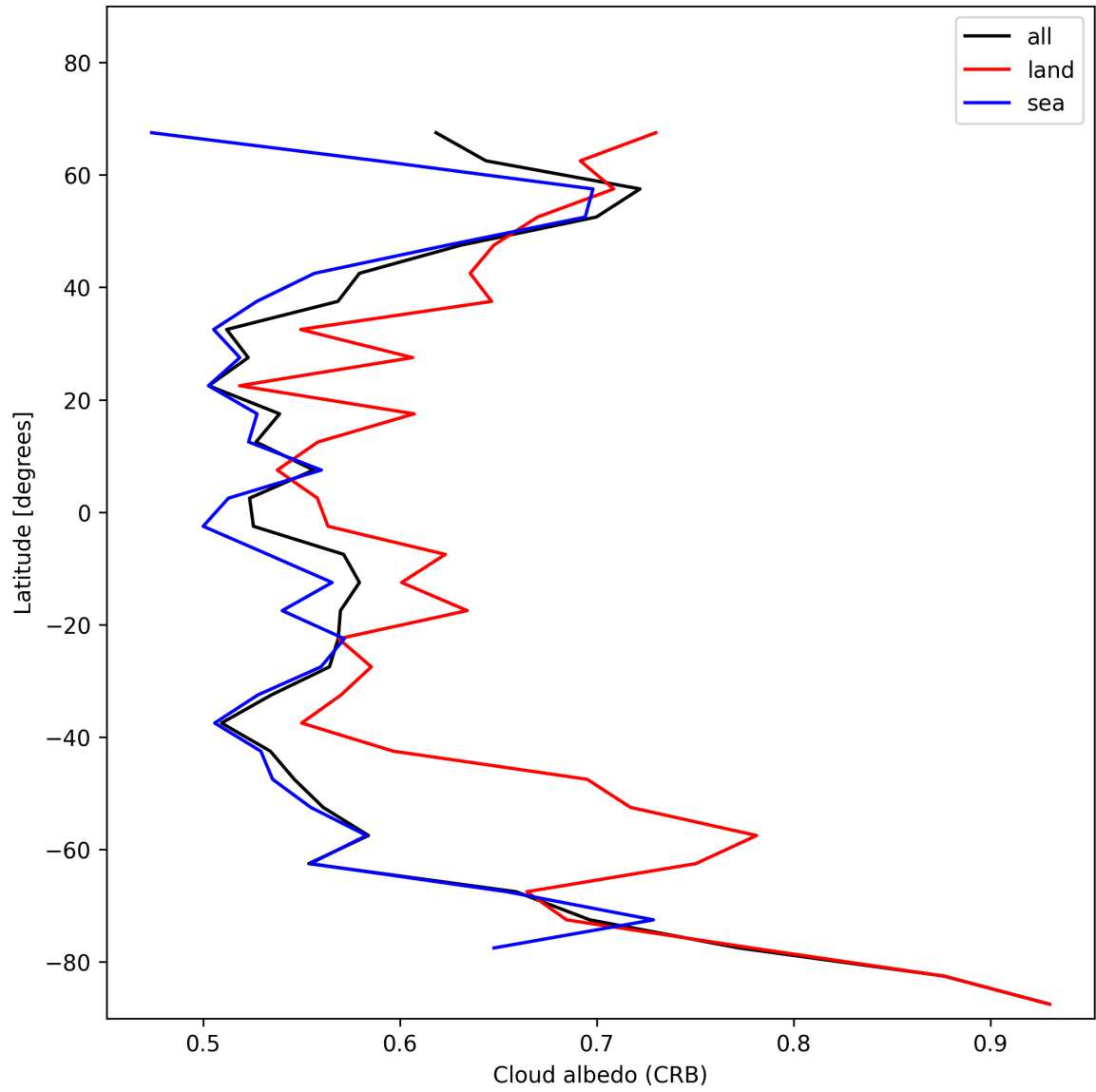
Figure 26: Zonal average of “Cloud albedo (CRB)” for 2024-12-31 to 2024-12-31.
