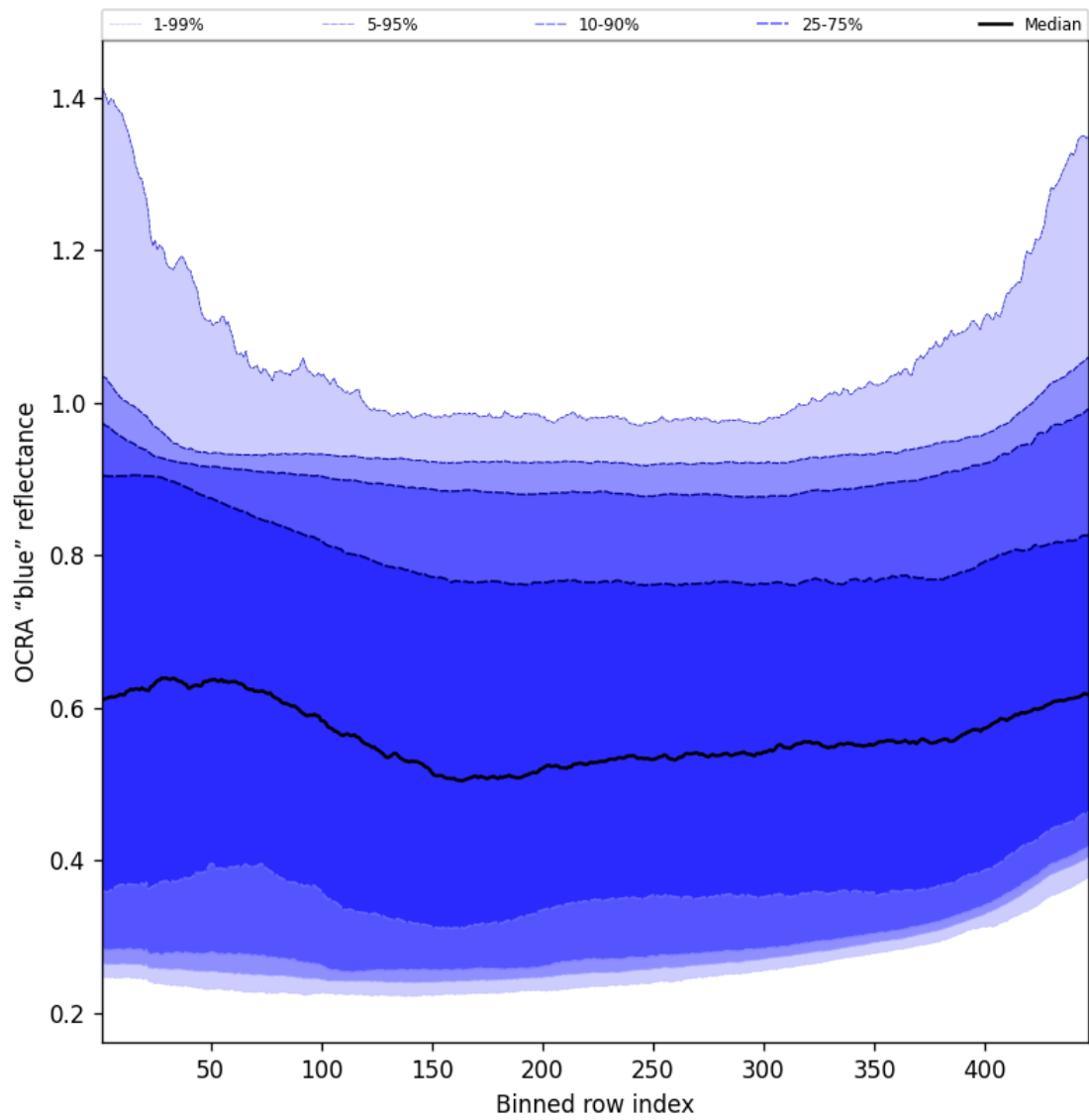
Figure 65: Along track statistics of “OCRA “blue” reflectance” for 2025-01-02 to 2025-01-03
