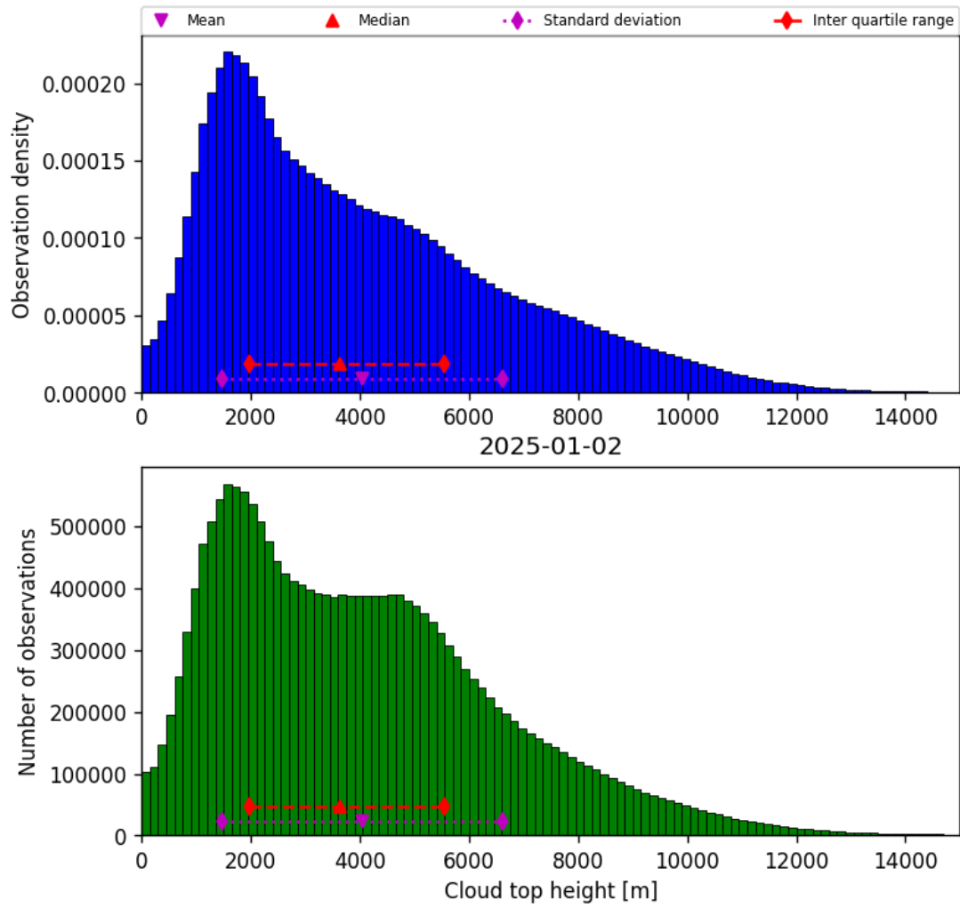
Figure 38: Histogram of “Cloud top height” for 2025-01-02 to 2025-01-03
