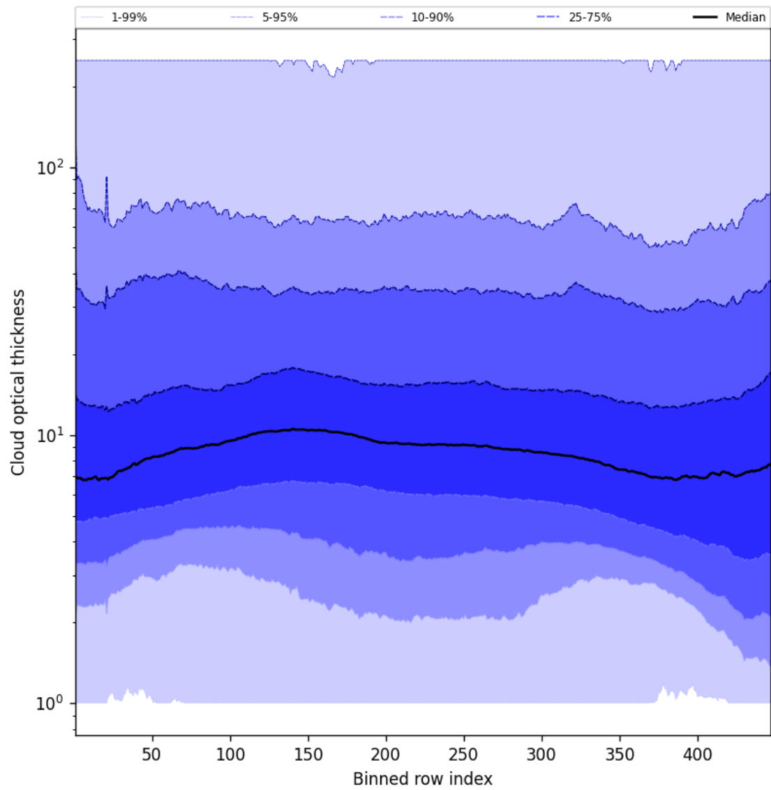
Figure 55: Along track statistics of “Cloud optical thickness” for 2025-01-02 to 2025-01-03
