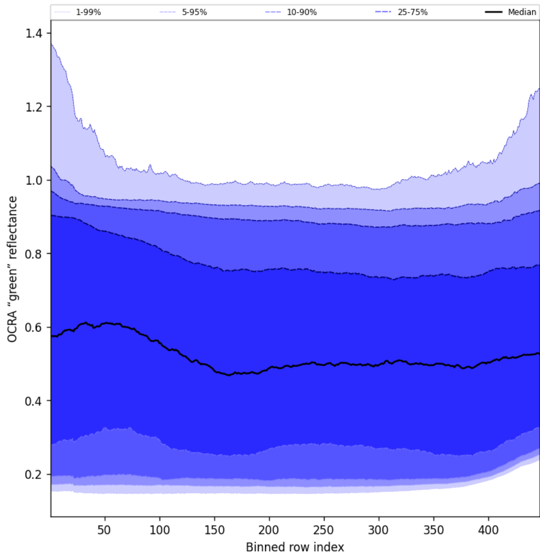
Figure 66: Along track statistics of "OCRA "green" reflectance" for 2025-01-02 to 2025-01-03
