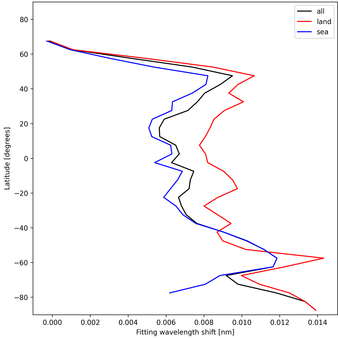
Figure 31: Zonal average of “Fitting wavelength shift” for 2025-01-02 to 2025-01-03.
