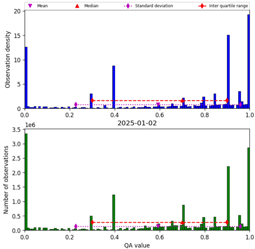
Figure 36: Histogram of “QA value” for 2025-01-02 to 2025-01-03
