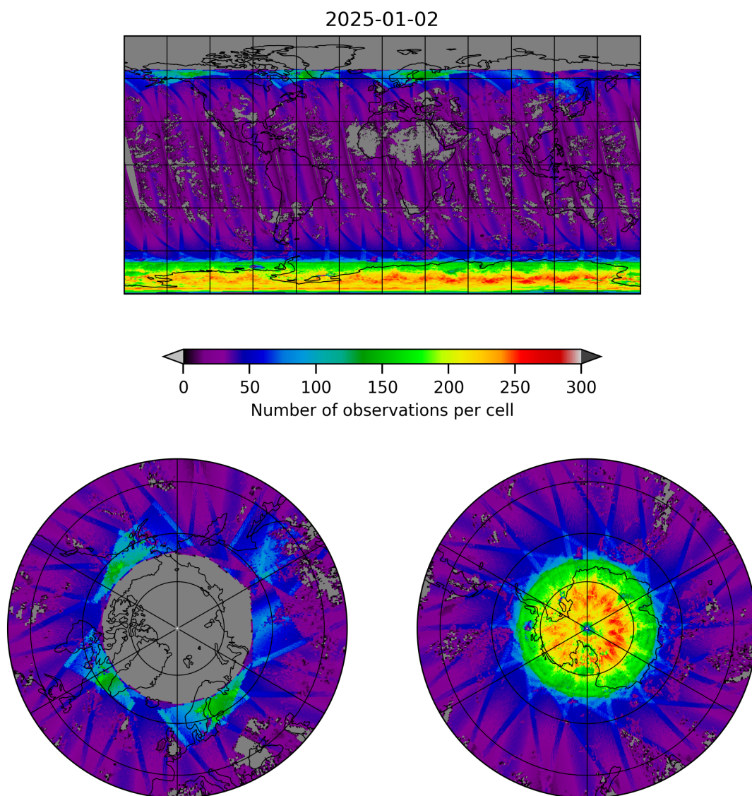
Figure 19: Map of the number of observations for 2025-01-02 to 2025-01-03
