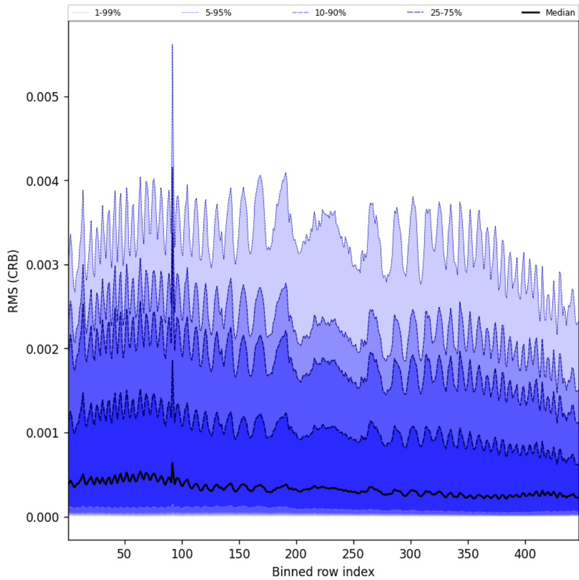
Figure 62: Along track statistics of “RMS (CRB)” for 2025-01-02 to 2025-01-03
