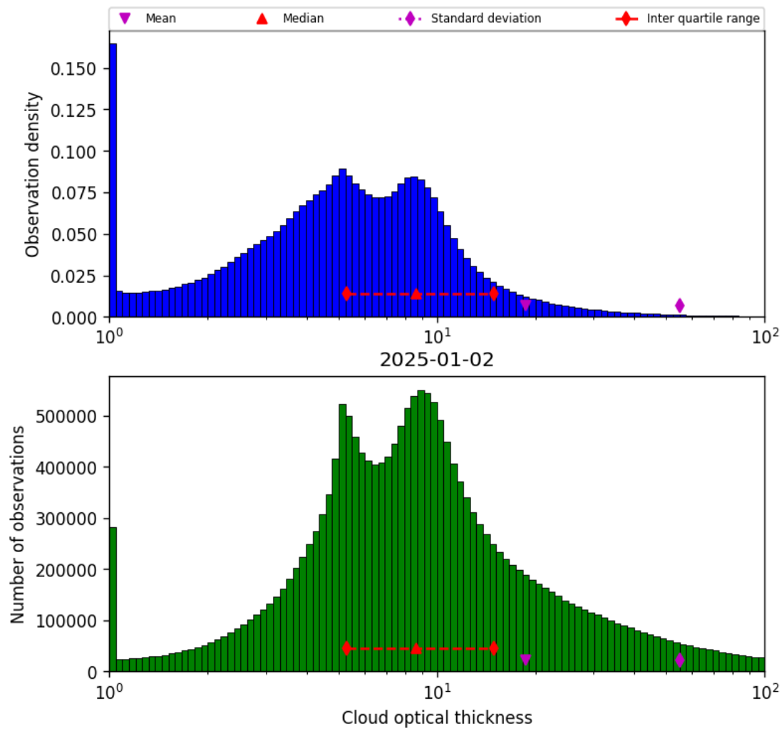
Figure 39: Histogram of “Cloud optical thickness” for 2025-01-02 to 2025-01-03
