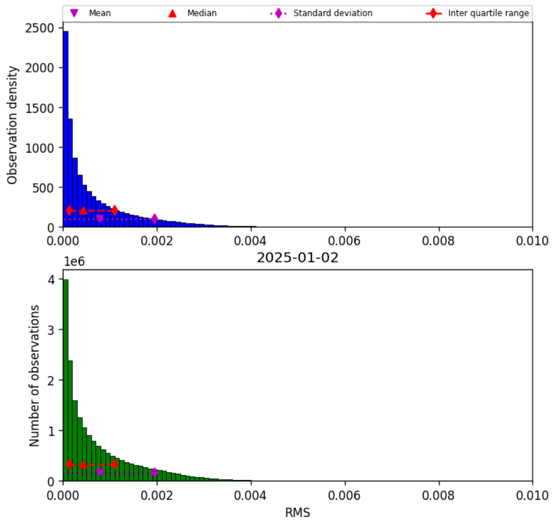
Figure 45: Histogram of “RMS” for 2025-01-02 to 2025-01-03
