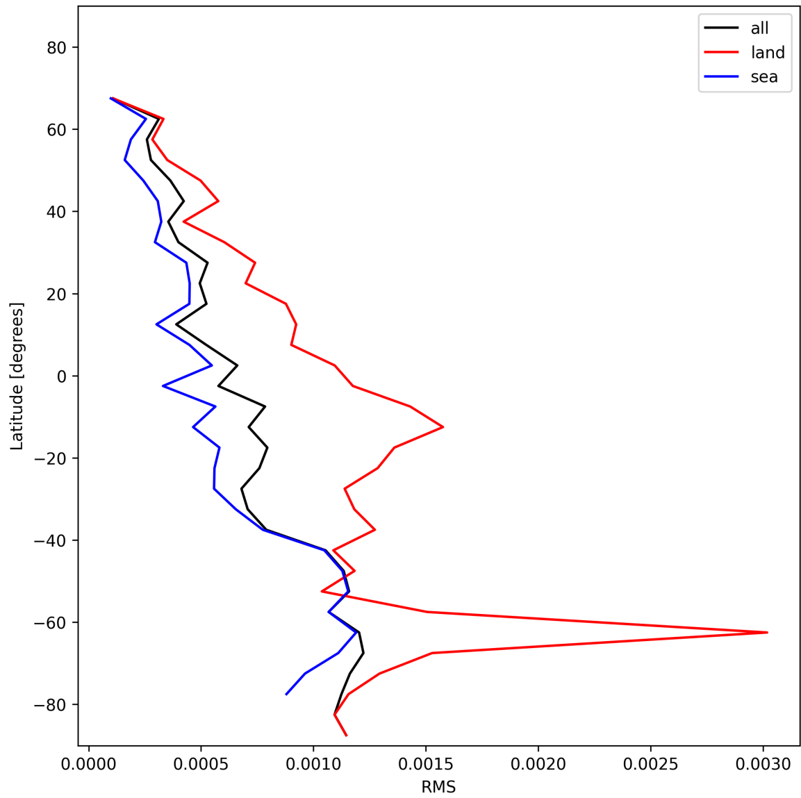
Figure 29: Zonal average of “RMS” for 2025-01-02 to 2025-01-03.
