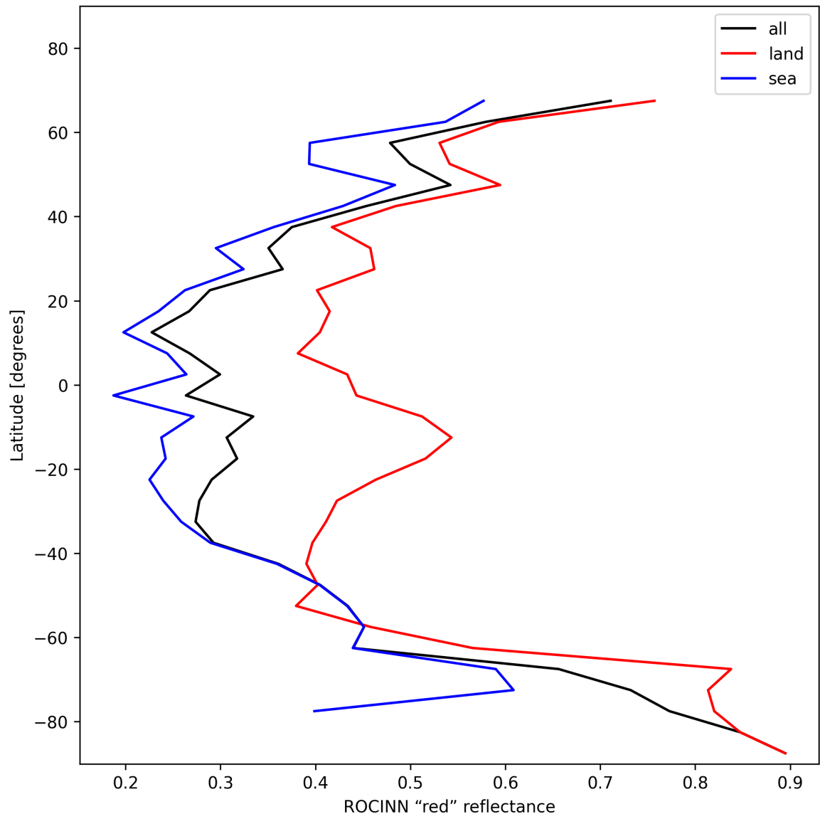
Figure 35: Zonal average of "ROCINN "red" reflectance" for 2025-01-02 to 2025-01-03.
