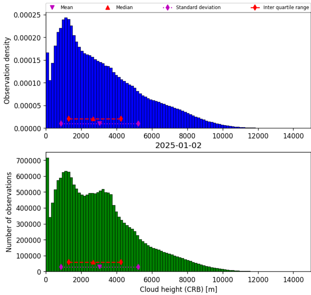
Figure 41: Histogram of “Cloud height (CRB)” for 2025-01-02 to 2025-01-03
