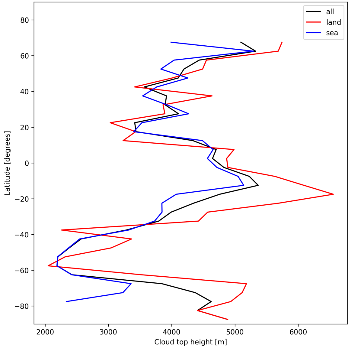
Figure 22: Zonal average of “Cloud top height” for 2025-01-02 to 2025-01-03.
