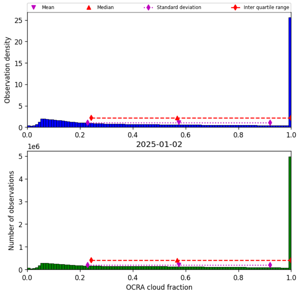
Figure 48: Histogram of “OCRA cloud fraction” for 2025-01-02 to 2025-01-03
