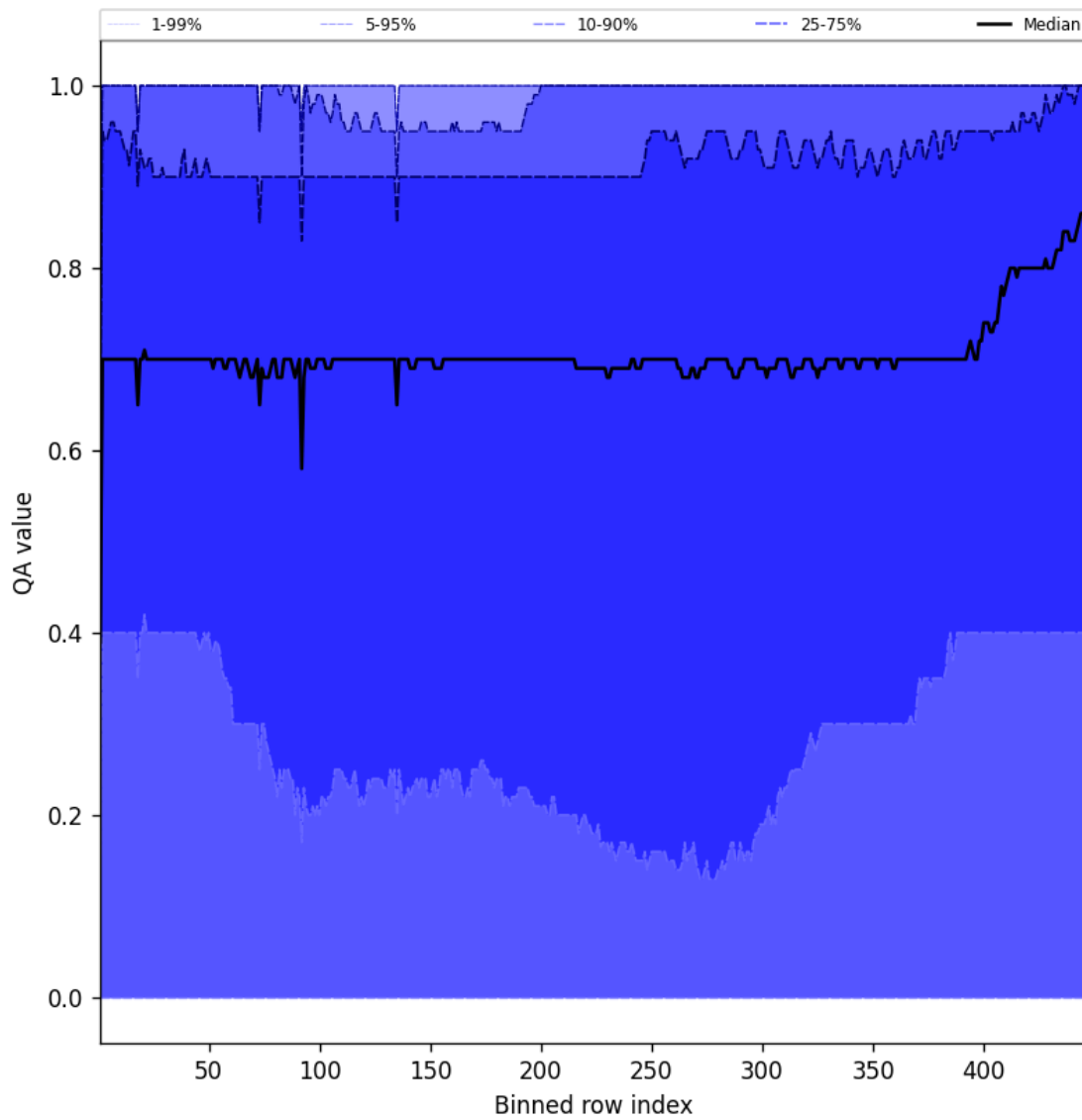
Figure 52: Along track statistics of “QA value” for 2025-01-02 to 2025-01-03
