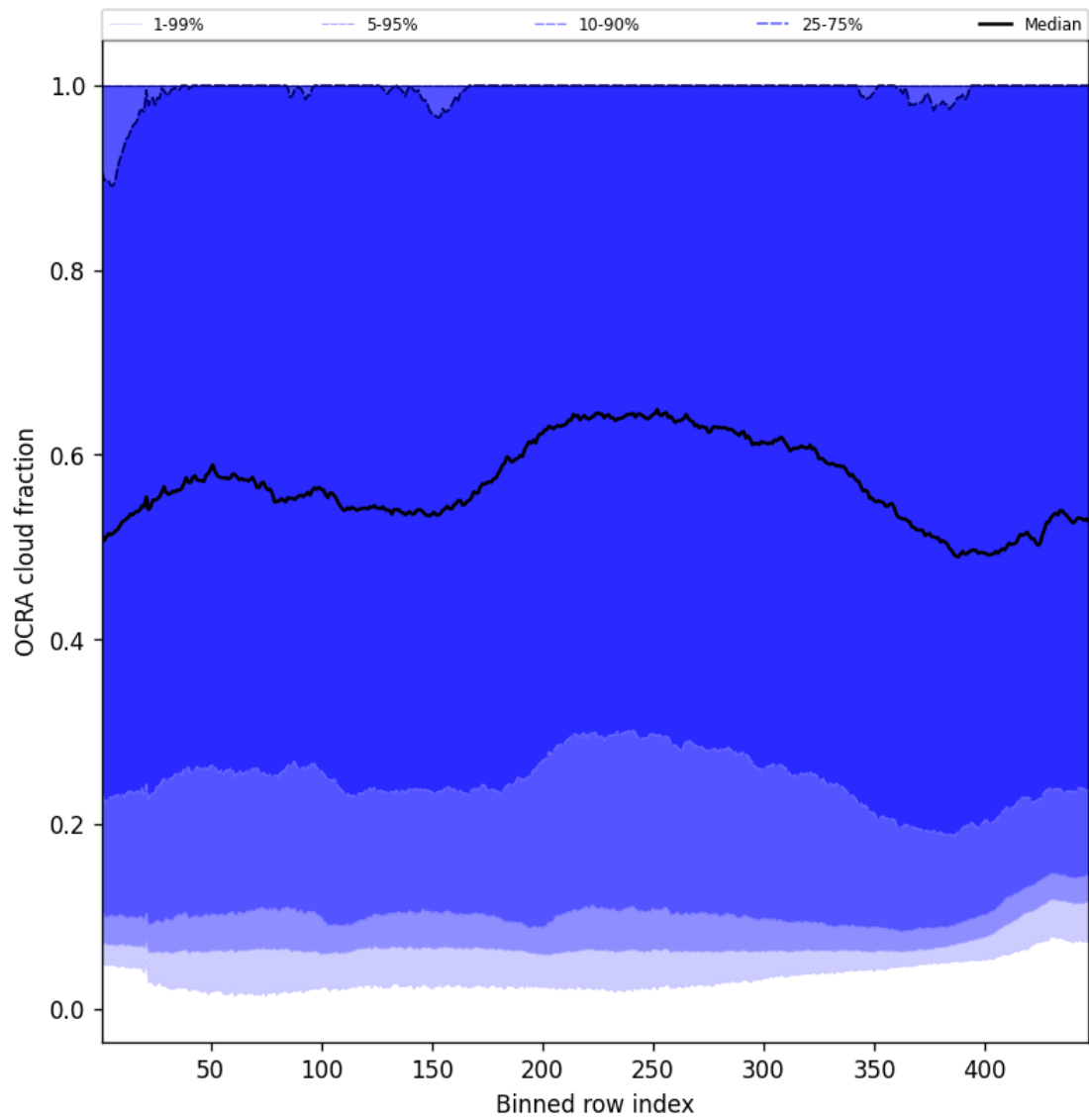
Figure 64: Along track statistics of “OCRA cloud fraction” for 2025-01-02 to 2025-01-03
