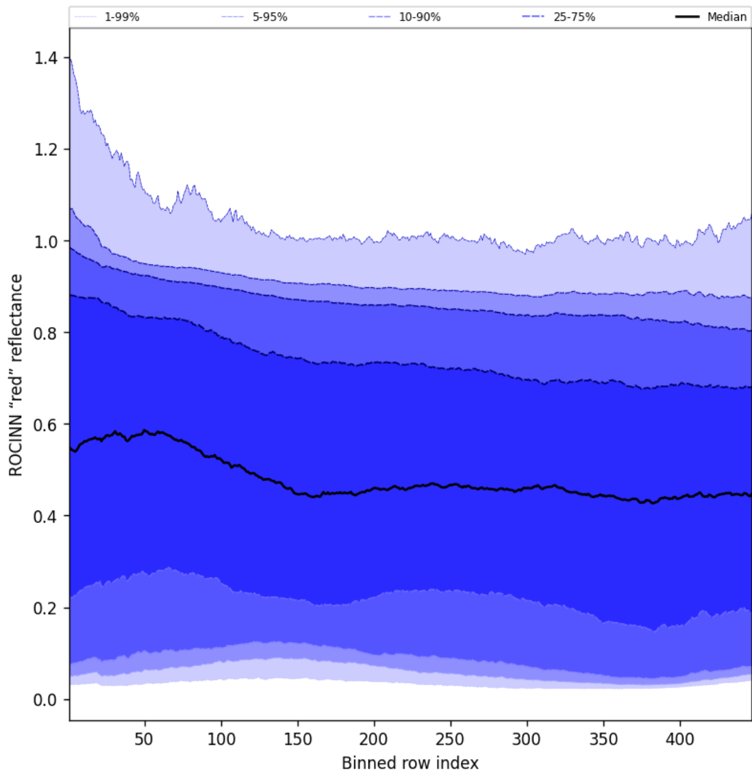
Figure 67: Along track statistics of “ROCINN “red” reflectance” for 2025-01-02 to 2025-01-03
