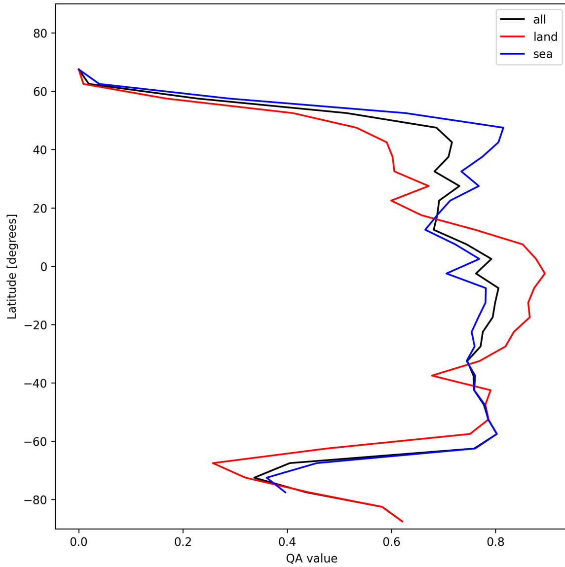
Figure 20: Zonal average of “QA value” for 2025-01-02 to 2025-01-03.
