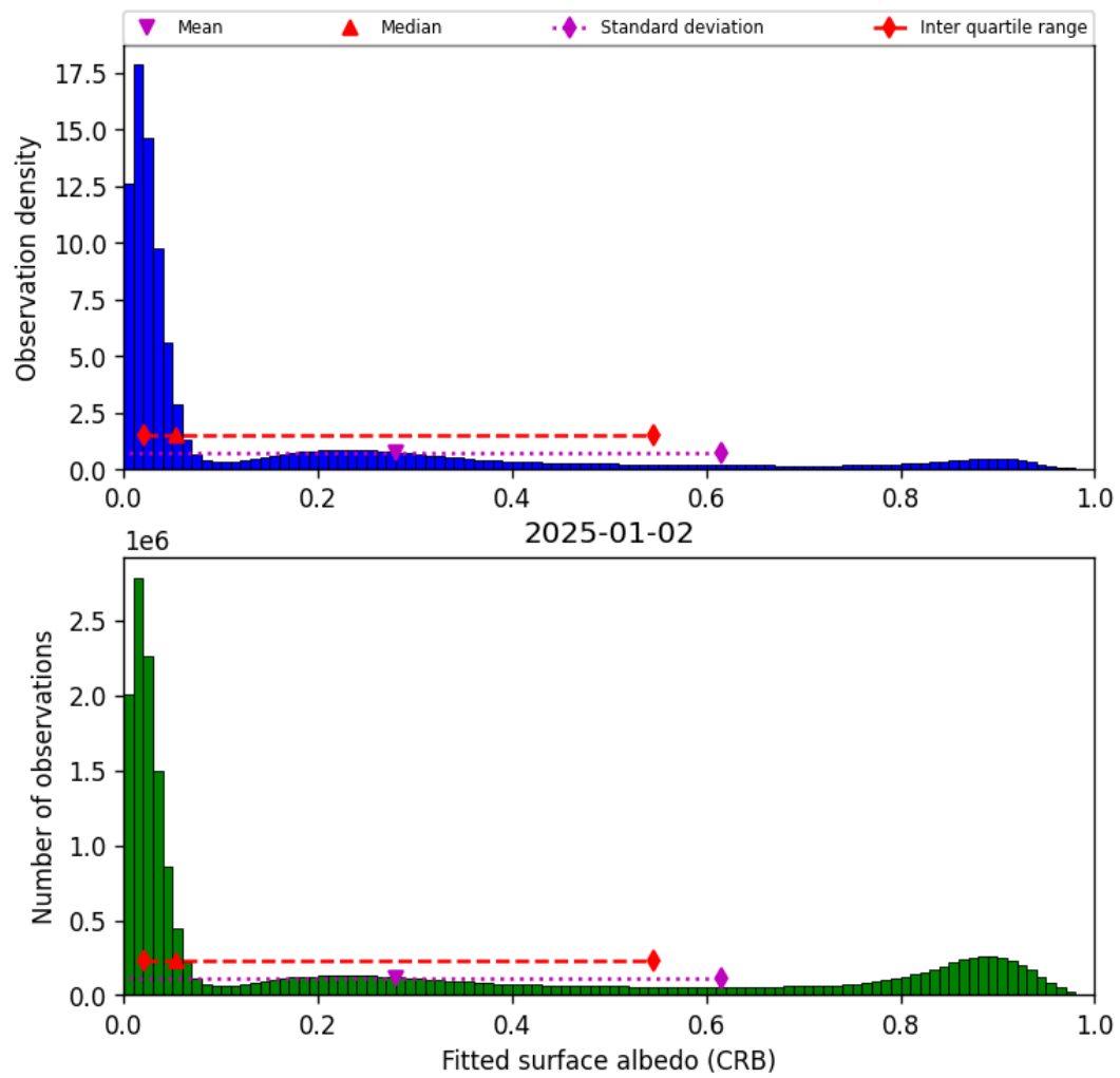
Figure 44: Histogram of “Fitted surface albedo (CRB)” for 2025-01-02 to 2025-01-03
