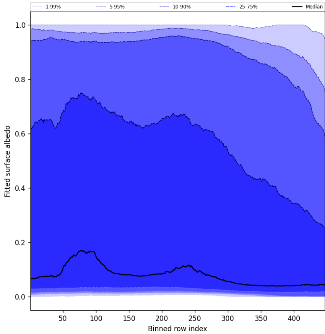
Figure 59: Along track statistics of “Fitted surface albedo” for 2025-01-02 to 2025-01-03
