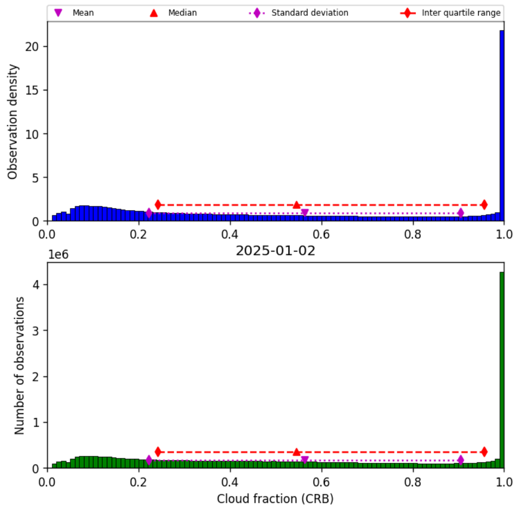
Figure 40: Histogram of “Cloud fraction (CRB)” for 2025-01-02 to 2025-01-03
