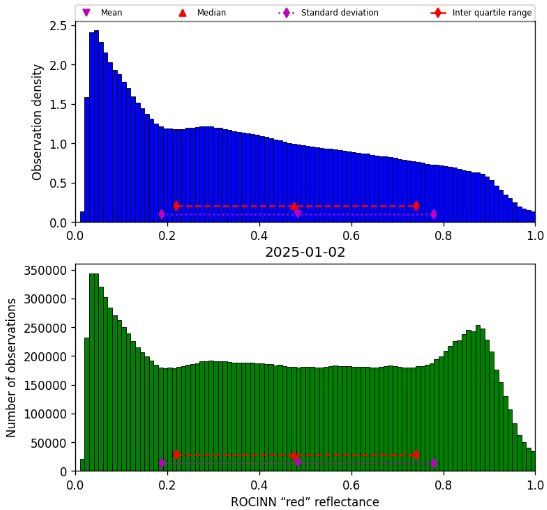
Figure 51: Histogram of “ROCINN “red” reflectance” for 2025-01-02 to 2025-01-03
