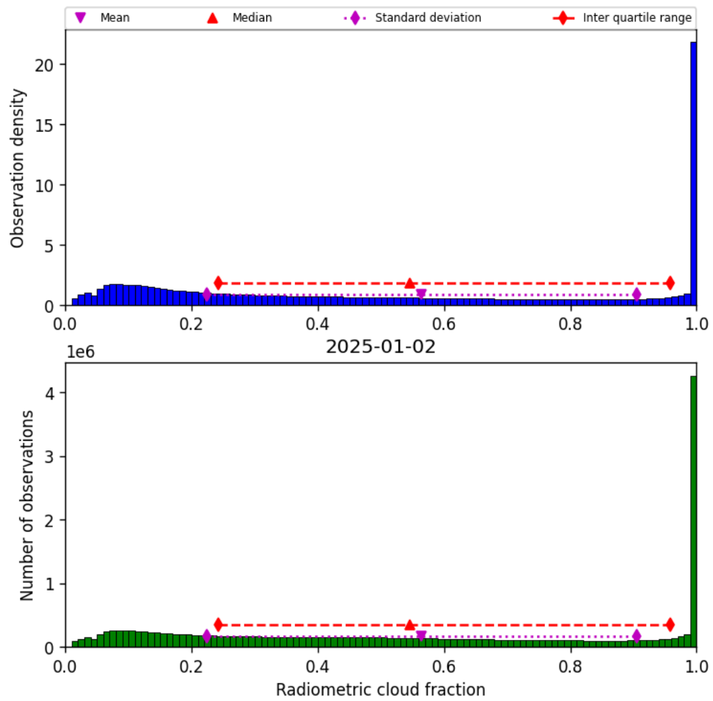
Figure 37: Histogram of “Radiometric cloud fraction” for 2025-01-02 to 2025-01-03
