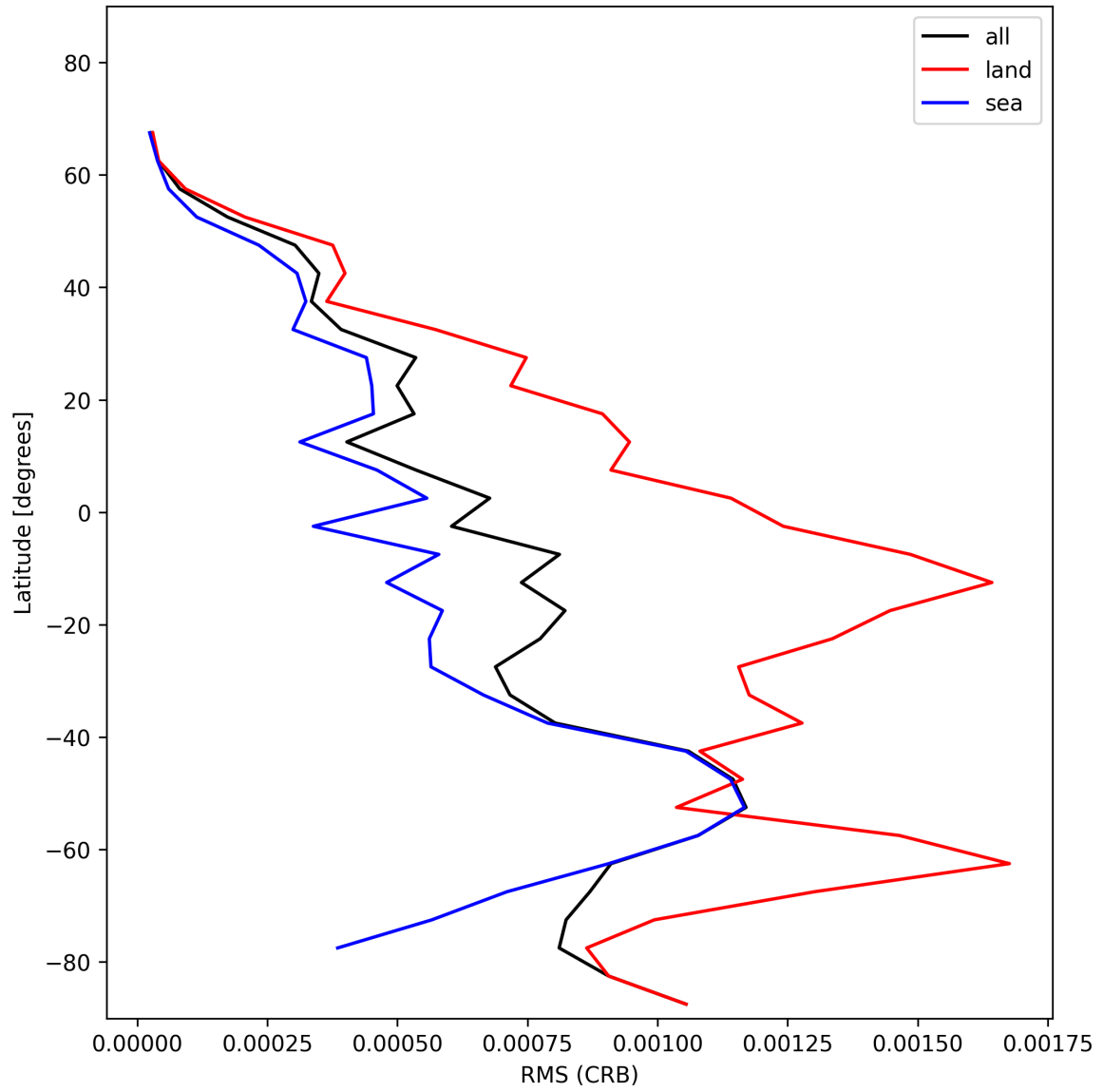
Figure 30: Zonal average of “RMS (CRB)” for 2025-01-02 to 2025-01-03.
