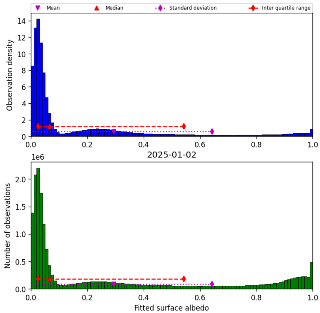
Figure 43: Histogram of “Fitted surface albedo” for 2025-01-02 to 2025-01-03
