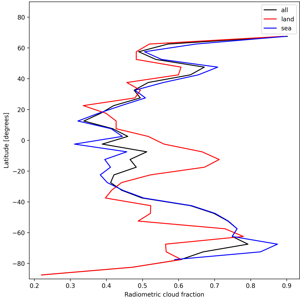
Figure 21: Zonal average of “Radiometric cloud fraction” for 2025-01-02 to 2025-01-03.
