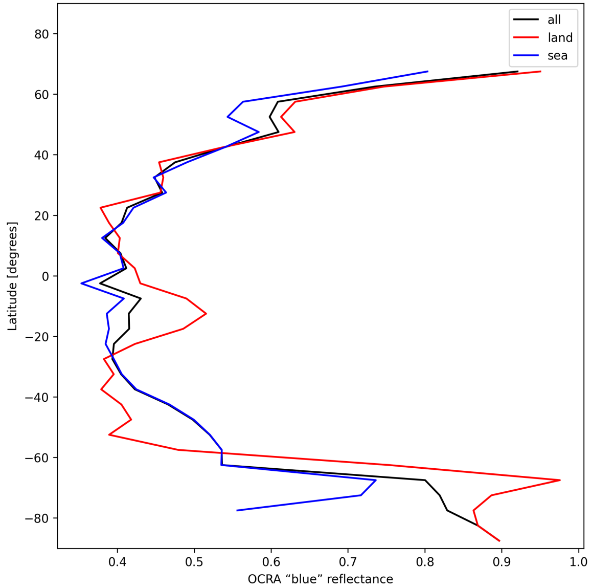
Figure 33: Zonal average of “OCRA “blue” reflectance” for 2025-01-02 to 2025-01-03.
