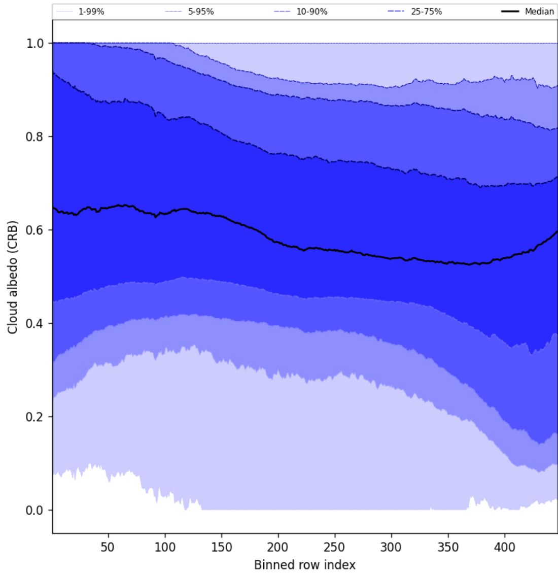
Figure 58: Along track statistics of “Cloud albedo (CRB)” for 2025-01-02 to 2025-01-03
