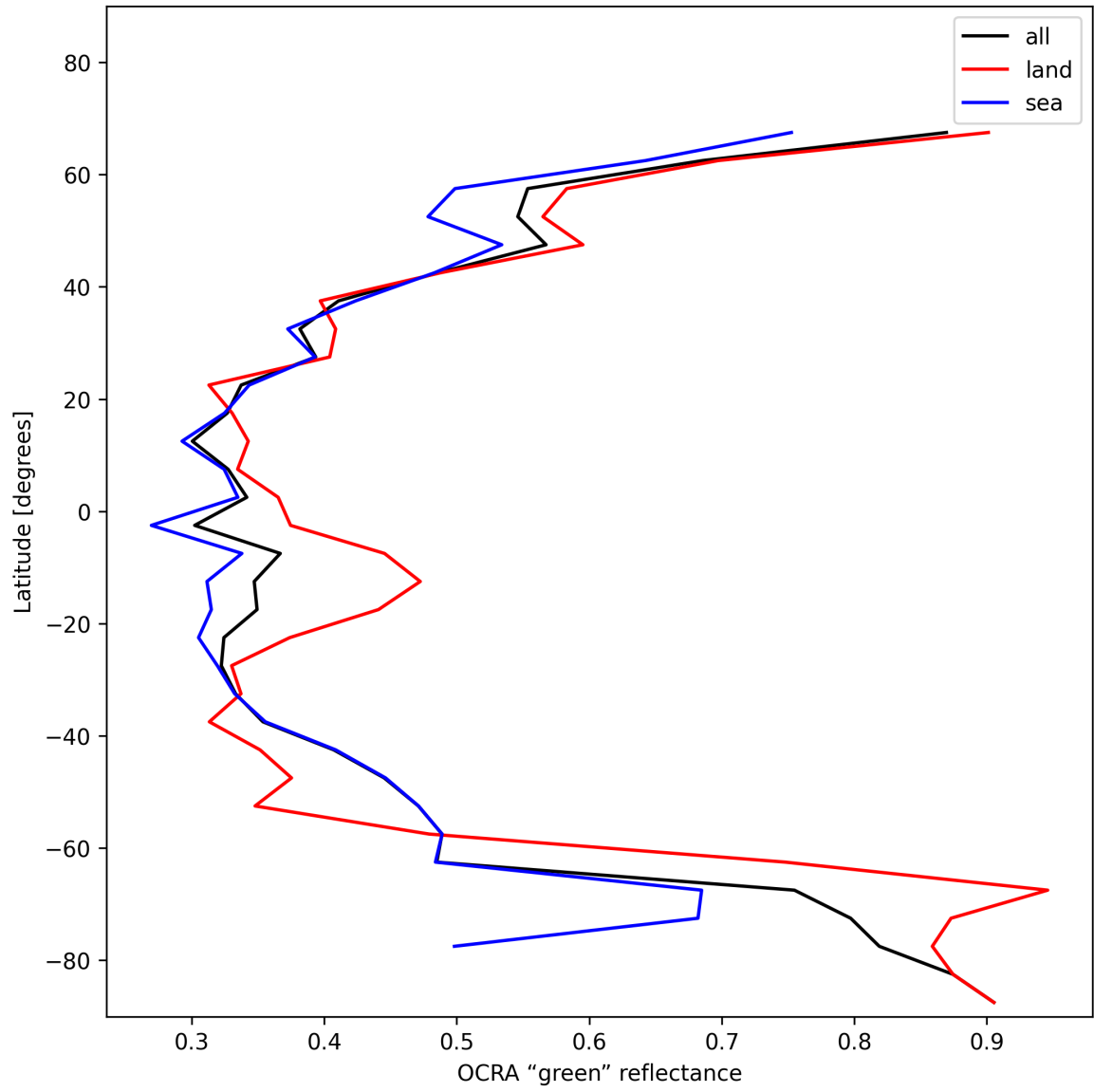
Figure 34: Zonal average of “OCRA “green” reflectance” for 2025-01-02 to 2025-01-03.
