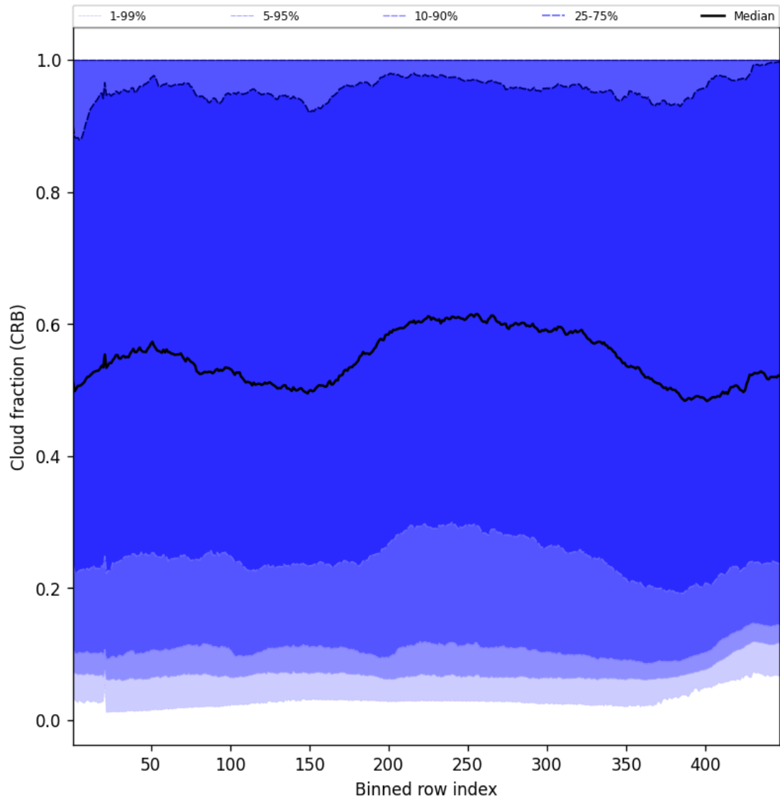
Figure 56: Along track statistics of “Cloud fraction (CRB)” for 2025-01-02 to 2025-01-03
