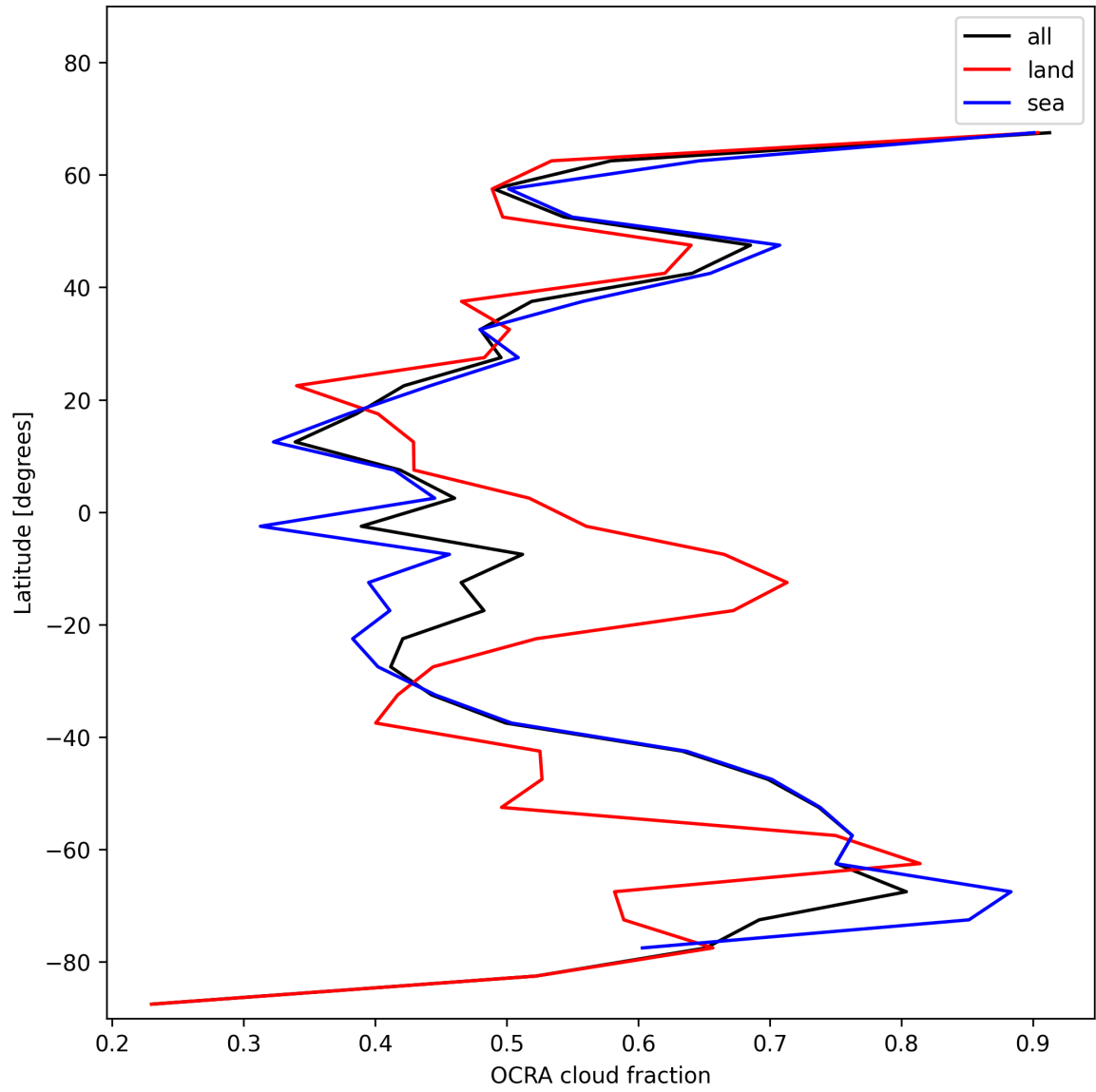
Figure 32: Zonal average of “OCRA cloud fraction” for 2025-01-02 to 2025-01-03.
