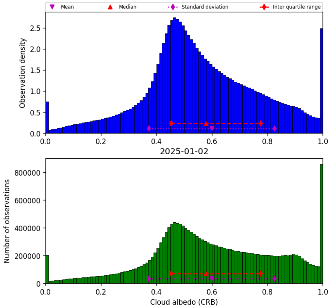
Figure 42: Histogram of “Cloud albedo (CRB)” for 2025-01-02 to 2025-01-03
