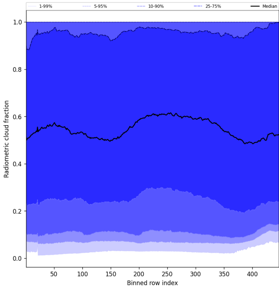
Figure 53: Along track statistics of “Radiometric cloud fraction” for 2025-01-02 to 2025-01-03
