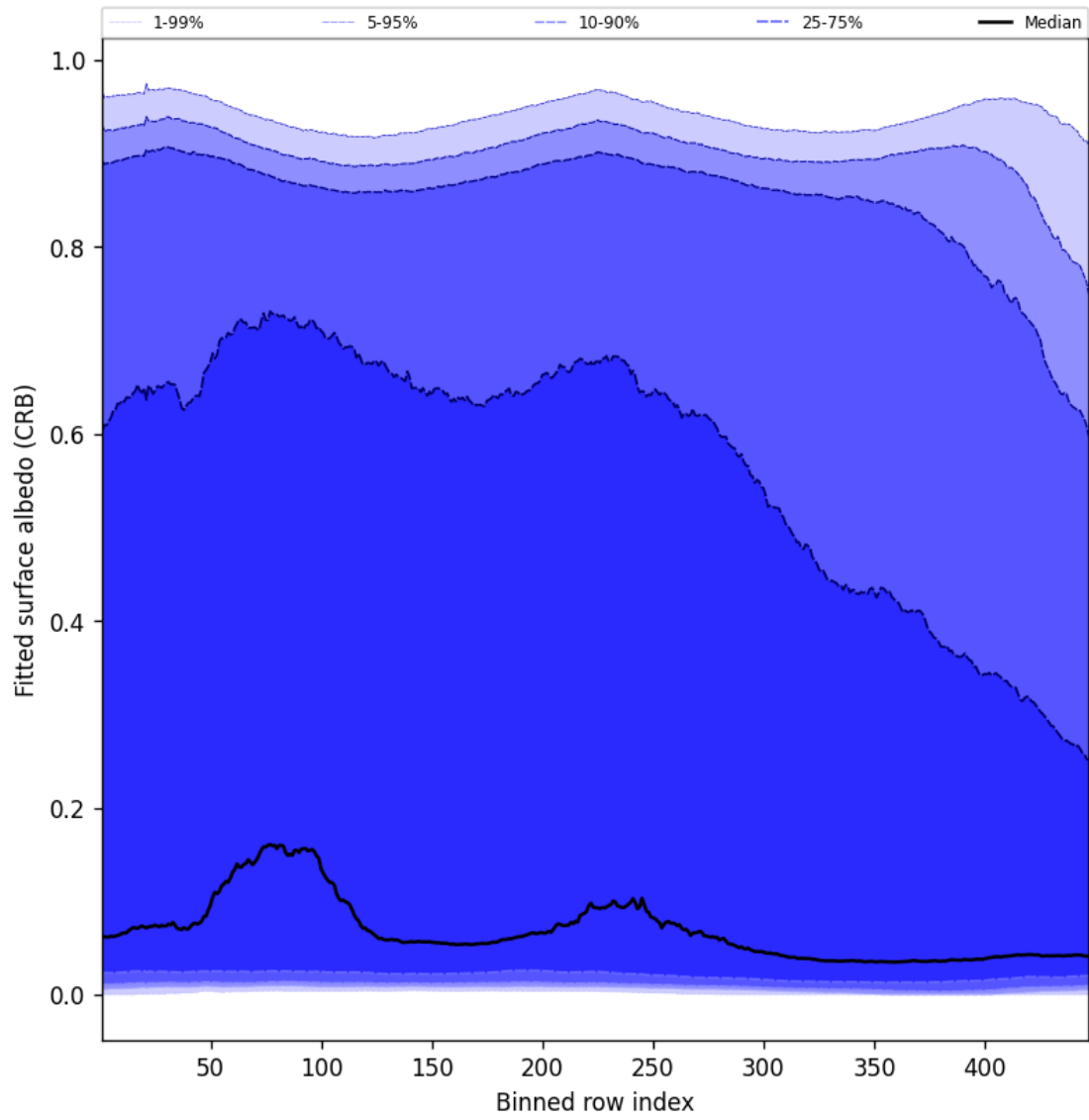
Figure 60: Along track statistics of “Fitted surface albedo (CRB)” for 2025-01-02 to 2025-01-03
