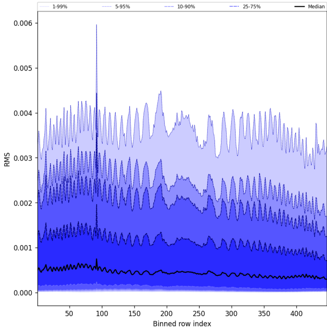
Figure 61: Along track statistics of “RMS” for 2025-01-02 to 2025-01-03
