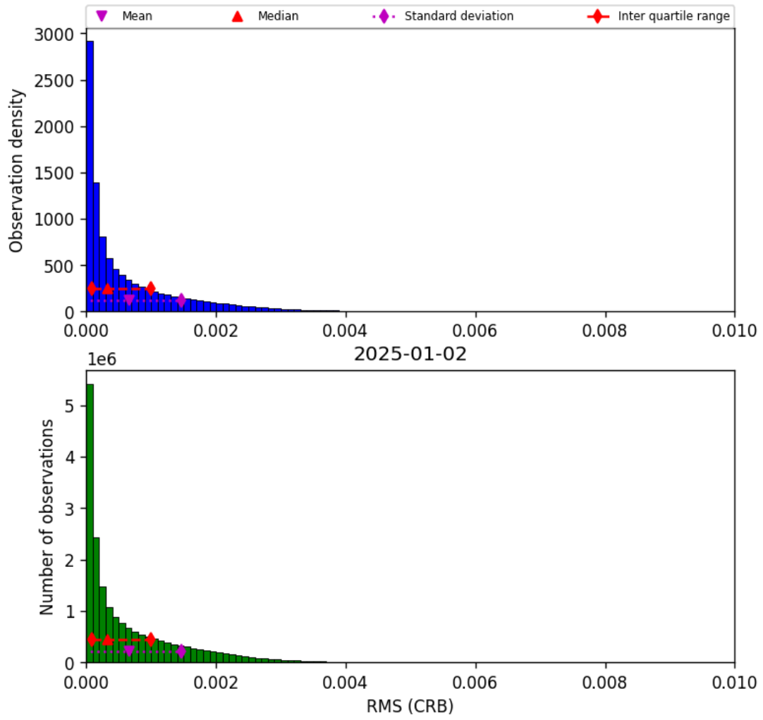
Figure 46: Histogram of “RMS (CRB)” for 2025-01-02 to 2025-01-03
