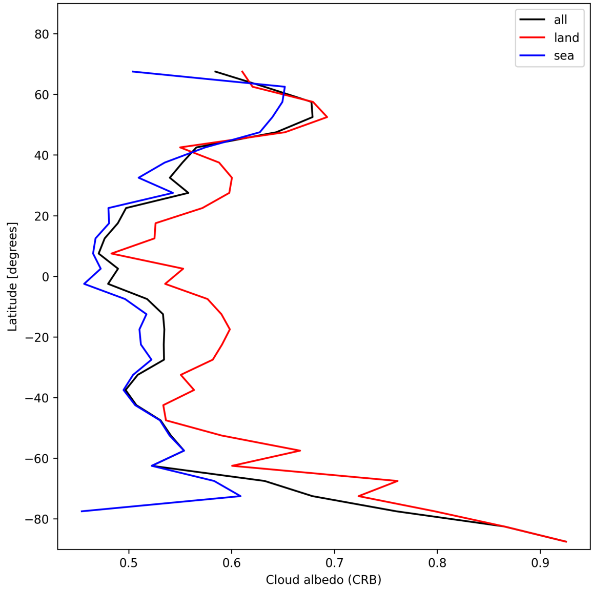
Figure 26: Zonal average of “Cloud albedo (CRB)” for 2025-01-02 to 2025-01-03.
