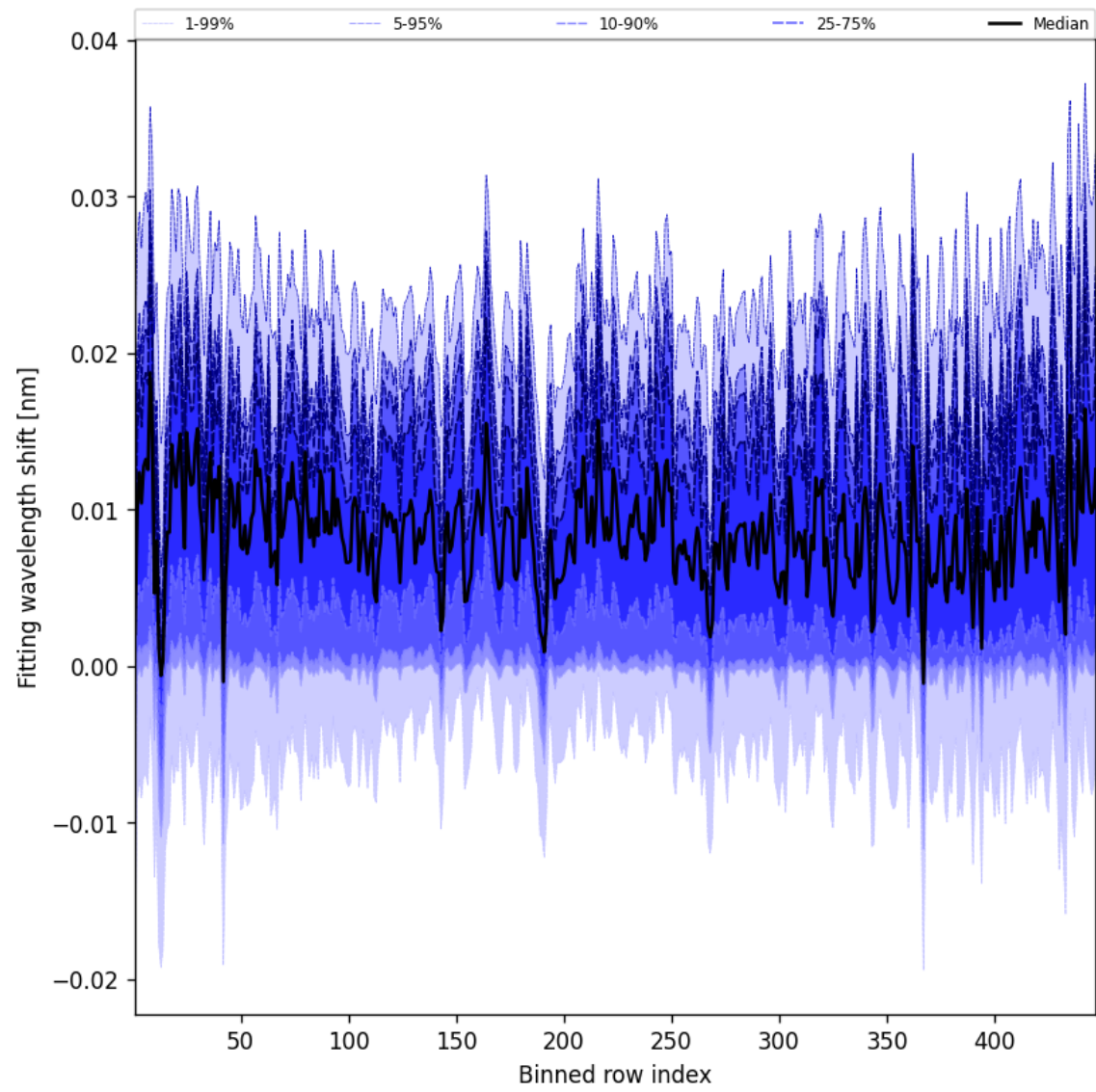
Figure 63: Along track statistics of “Fitting wavelength shift” for 2025-01-02 to 2025-01-03
