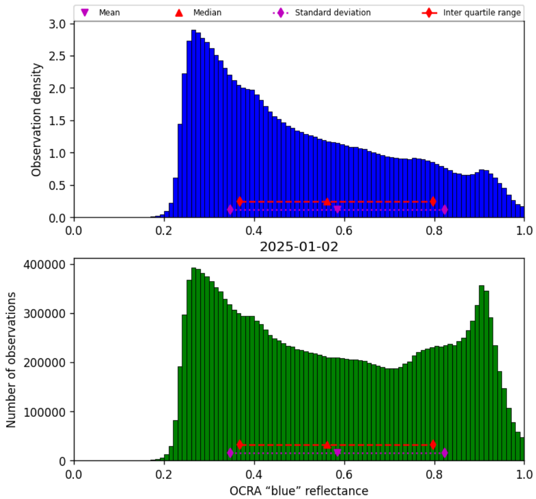
Figure 49: Histogram of “OCRA “blue” reflectance” for 2025-01-02 to 2025-01-03
