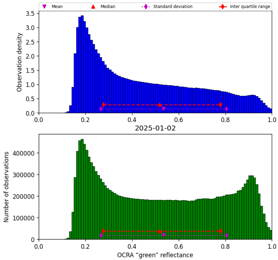
Figure 50: Histogram of “OCRA “green” reflectance” for 2025-01-02 to 2025-01-03
