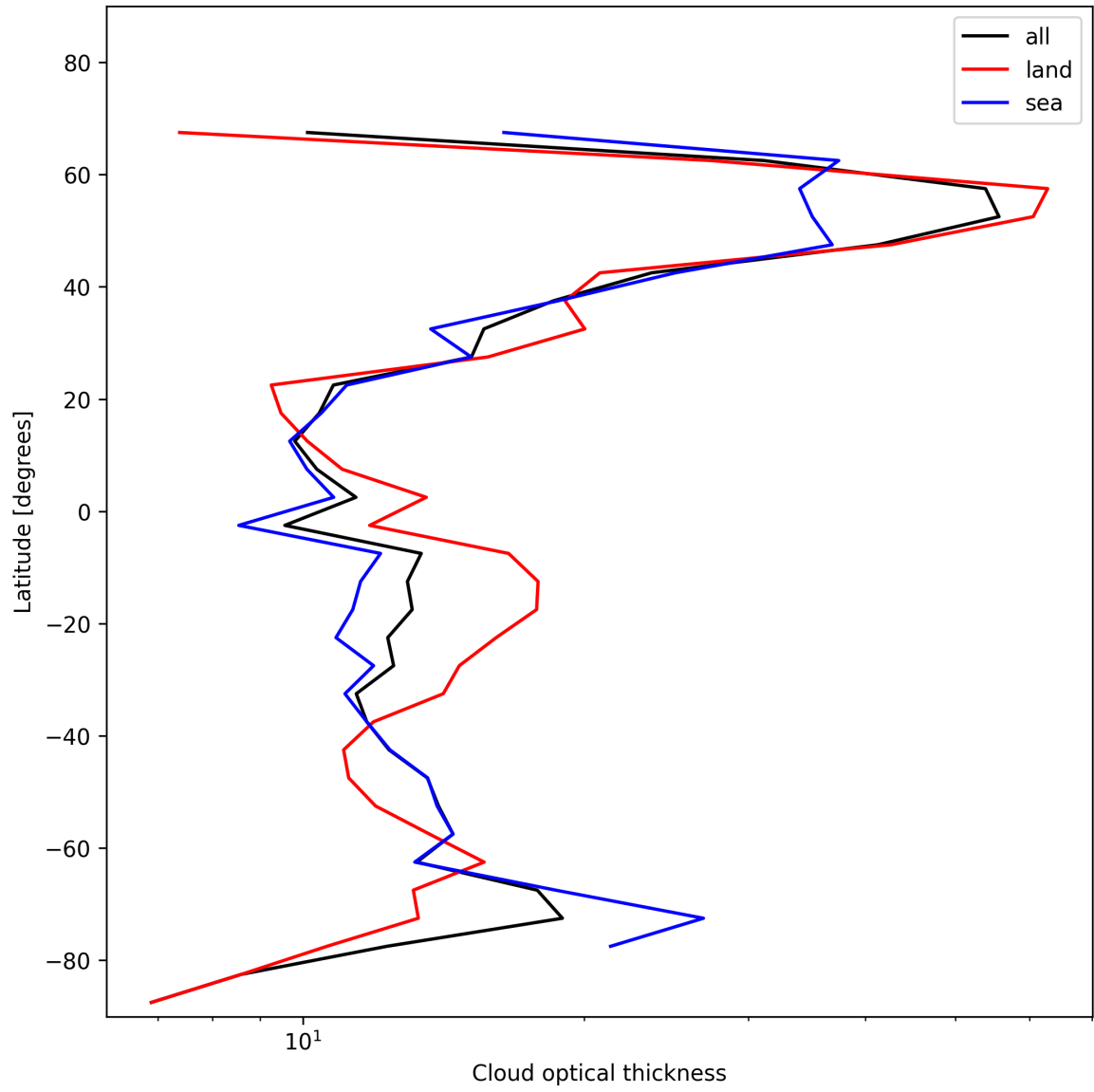
Figure 23: Zonal average of “Cloud optical thickness” for 2025-01-02 to 2025-01-03.
