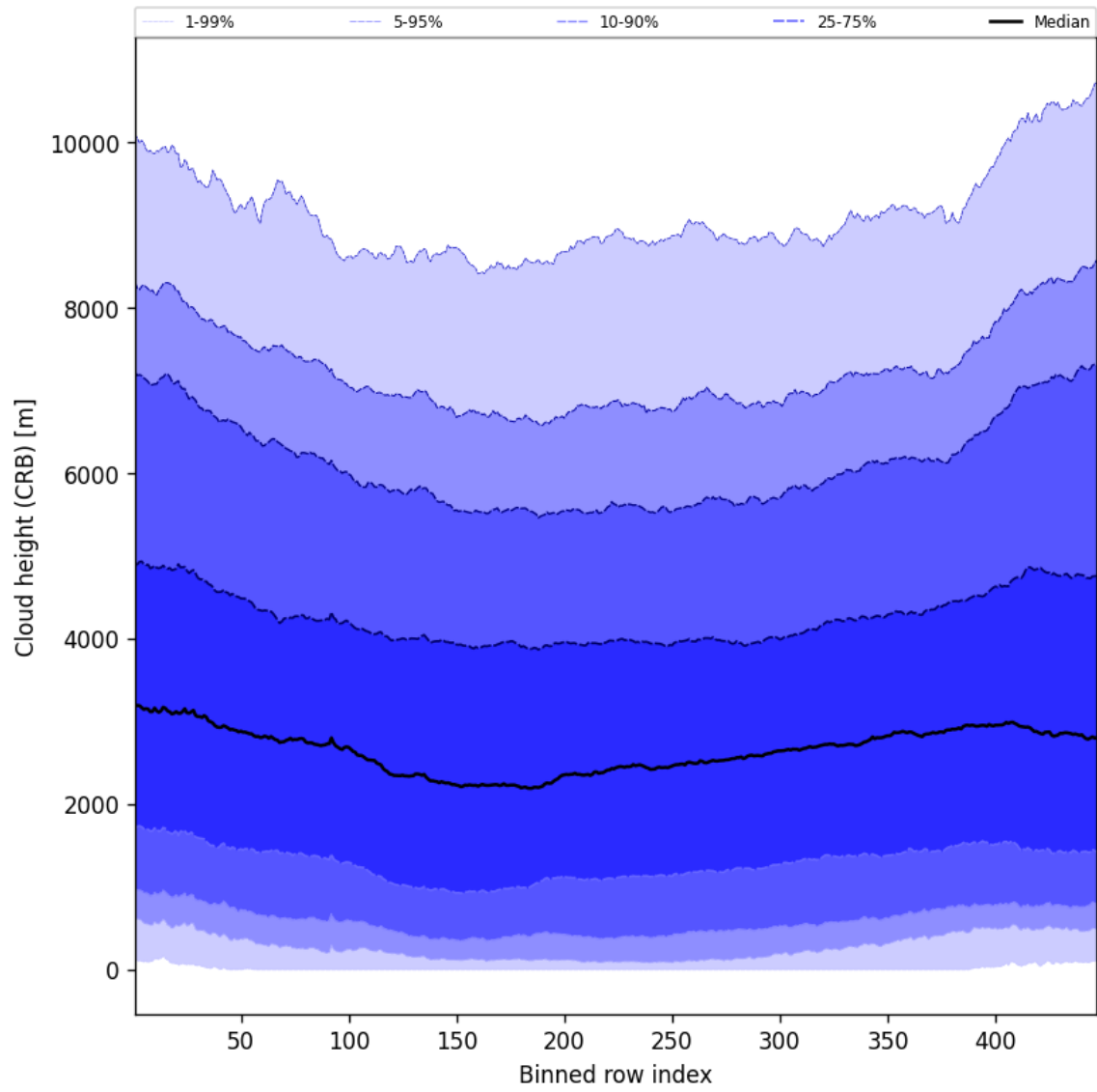
Figure 57: Along track statistics of “Cloud height (CRB)” for 2025-01-02 to 2025-01-03
