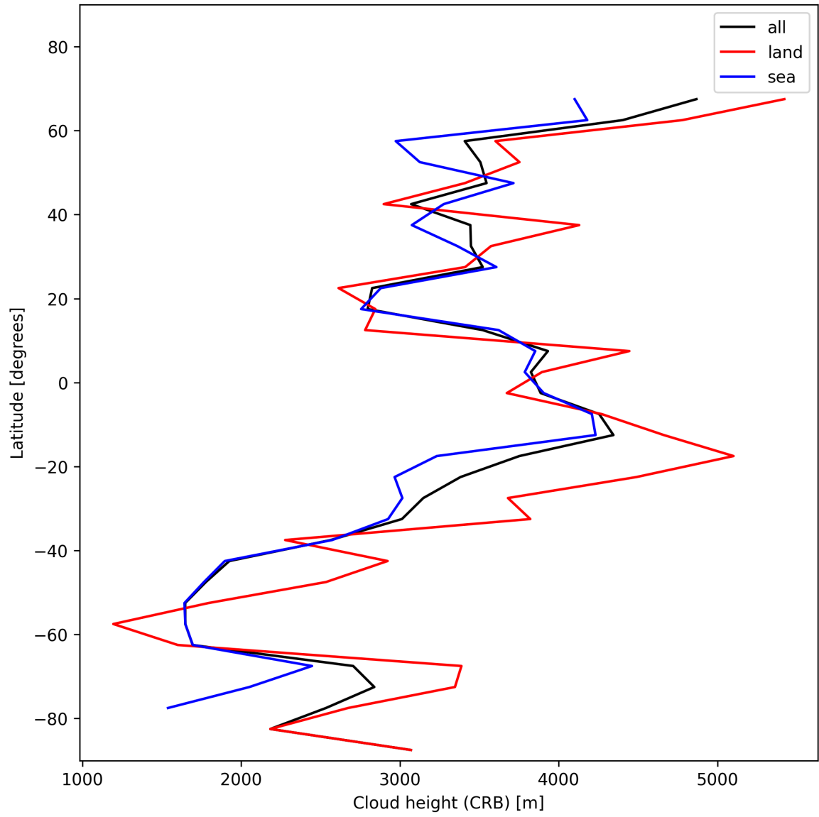
Figure 25: Zonal average of “Cloud height (CRB)” for 2025-01-02 to 2025-01-03.
