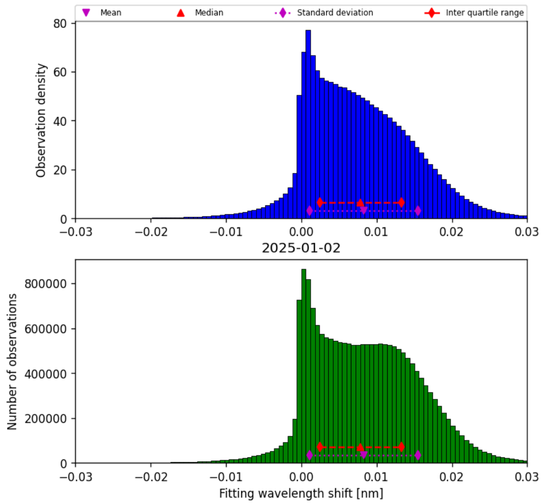
Figure 47: Histogram of “Fitting wavelength shift” for 2025-01-02 to 2025-01-03
