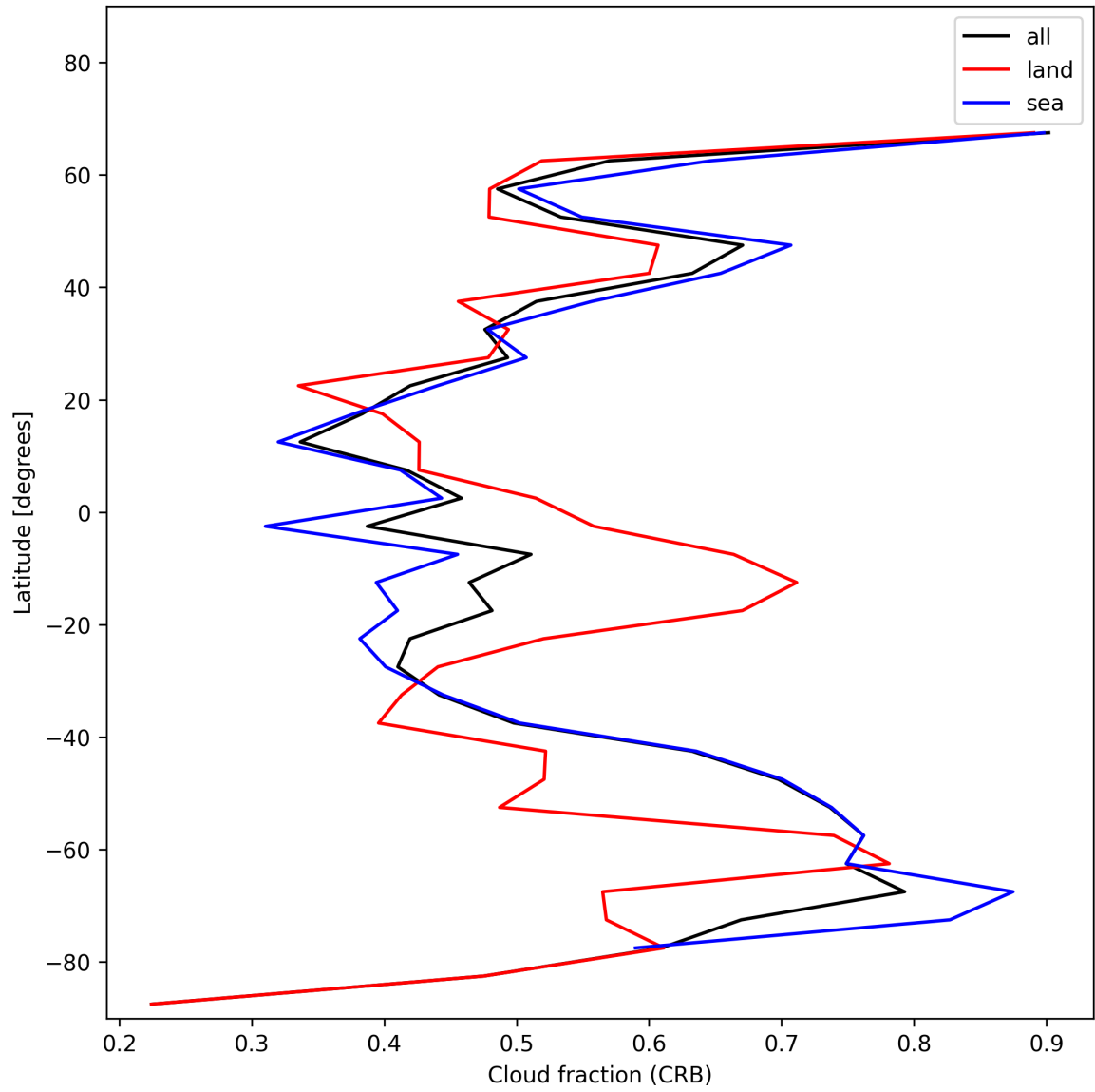
Figure 24: Zonal average of “Cloud fraction (CRB)” for 2025-01-02 to 2025-01-03.
