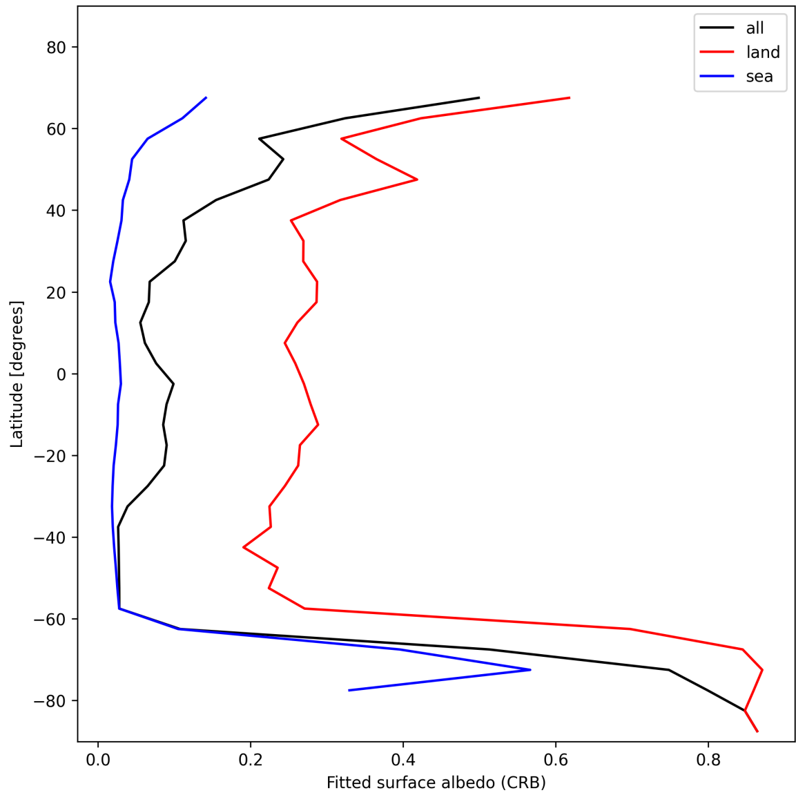
Figure 28: Zonal average of “Fitted surface albedo (CRB)” for 2025-01-02 to 2025-01-03.
