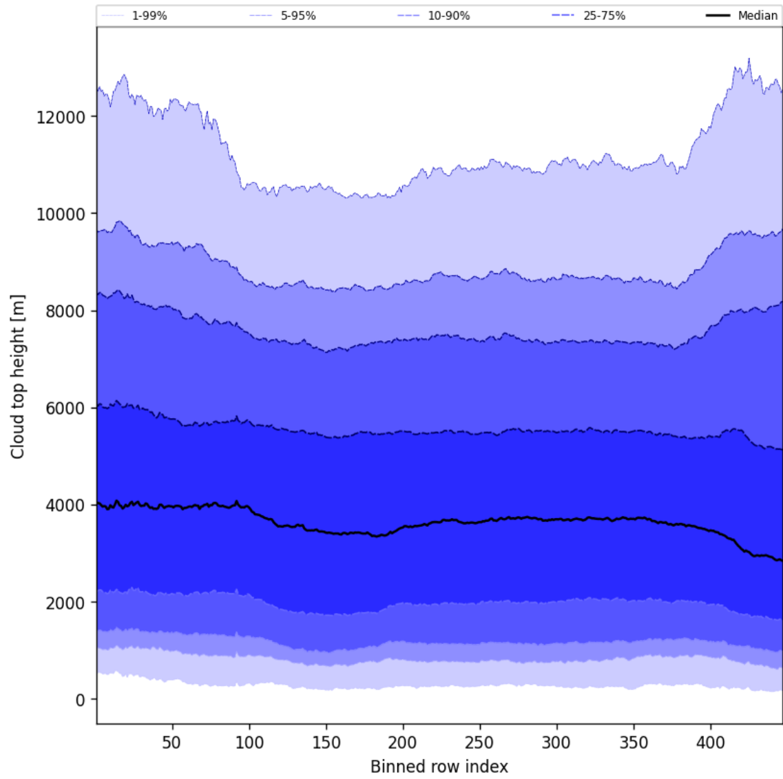
Figure 54: Along track statistics of “Cloud top height” for 2025-01-02 to 2025-01-03
