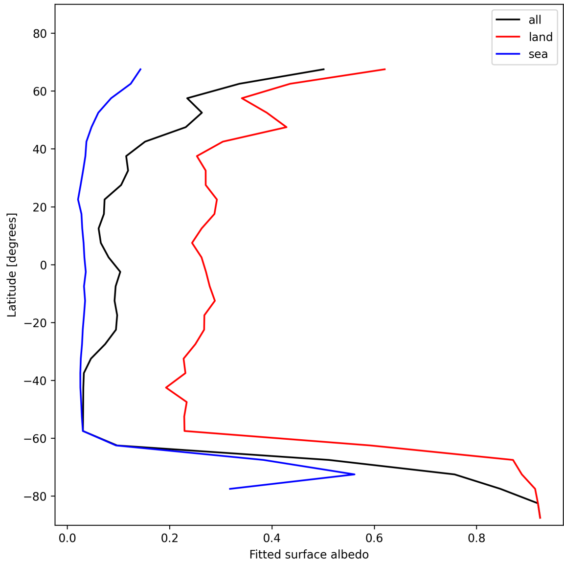
Figure 27: Zonal average of “Fitted surface albedo” for 2025-01-02 to 2025-01-03.
