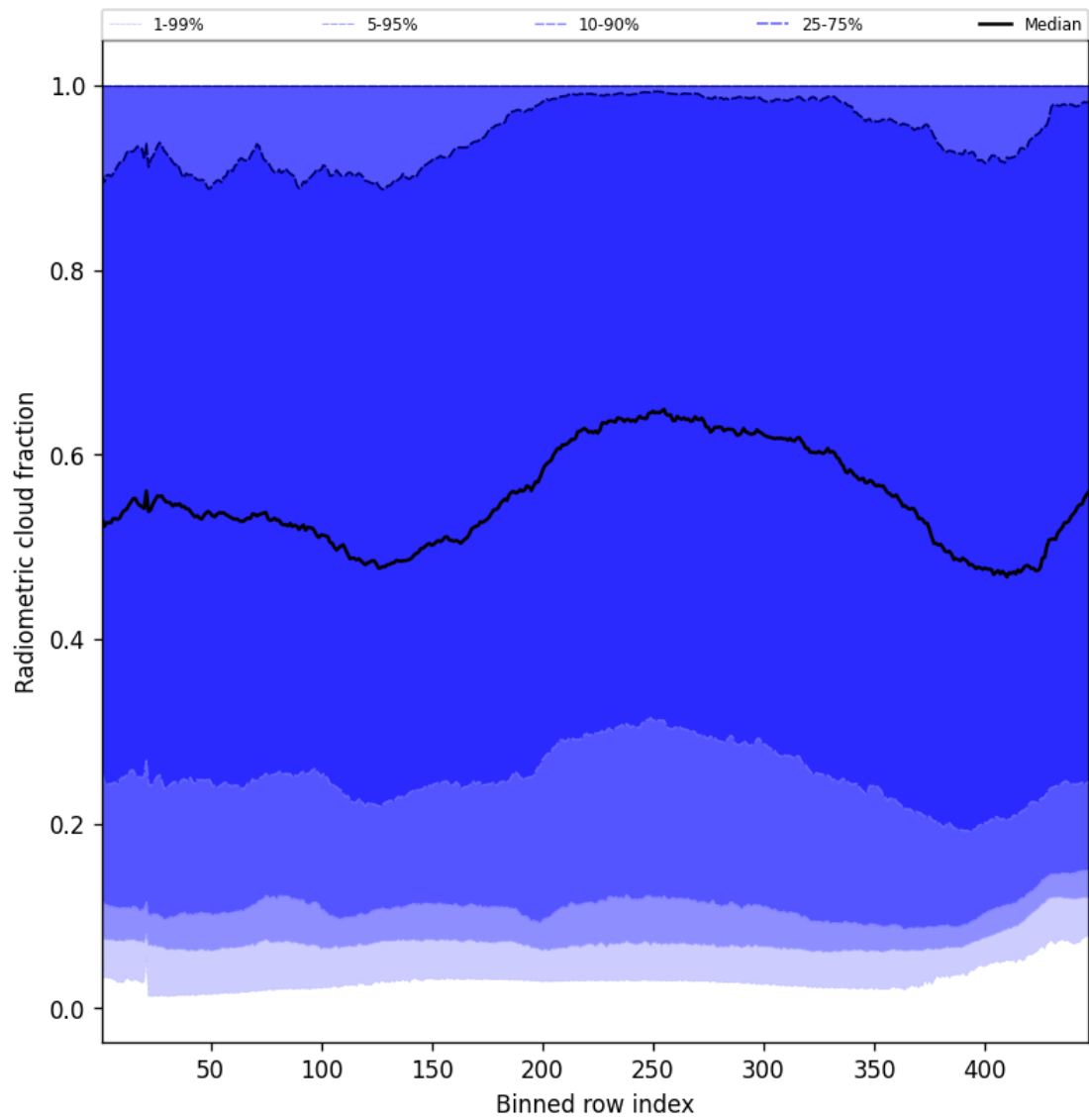
Figure 53: Along track statistics of “Radiometric cloud fraction” for 2025-01-03 to 2025-01-04
