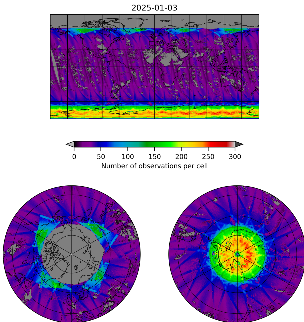
Figure 19: Map of the number of observations for 2025-01-03 to 2025-01-04
