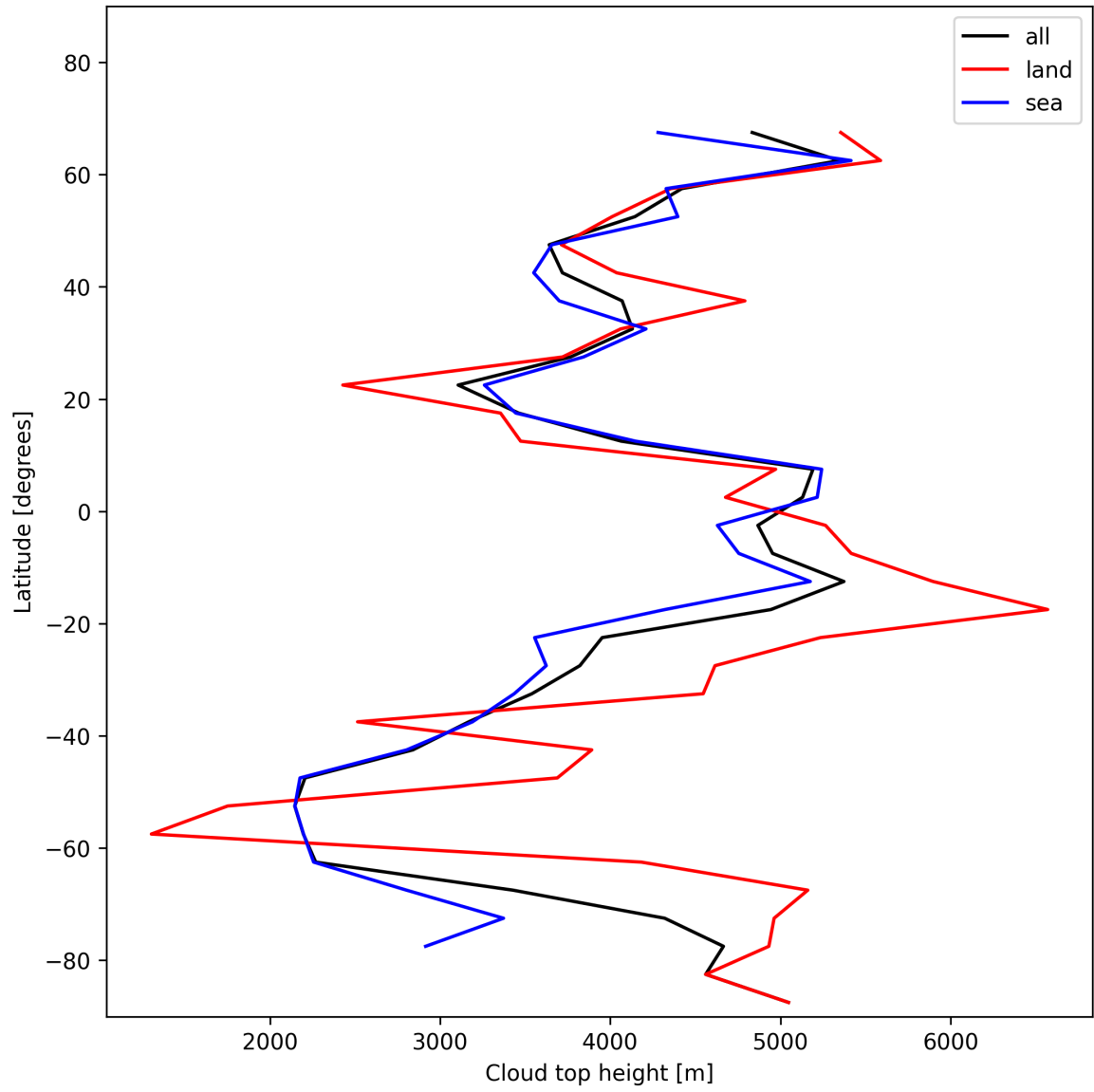
Figure 22: Zonal average of “Cloud top height” for 2025-01-03 to 2025-01-04.
