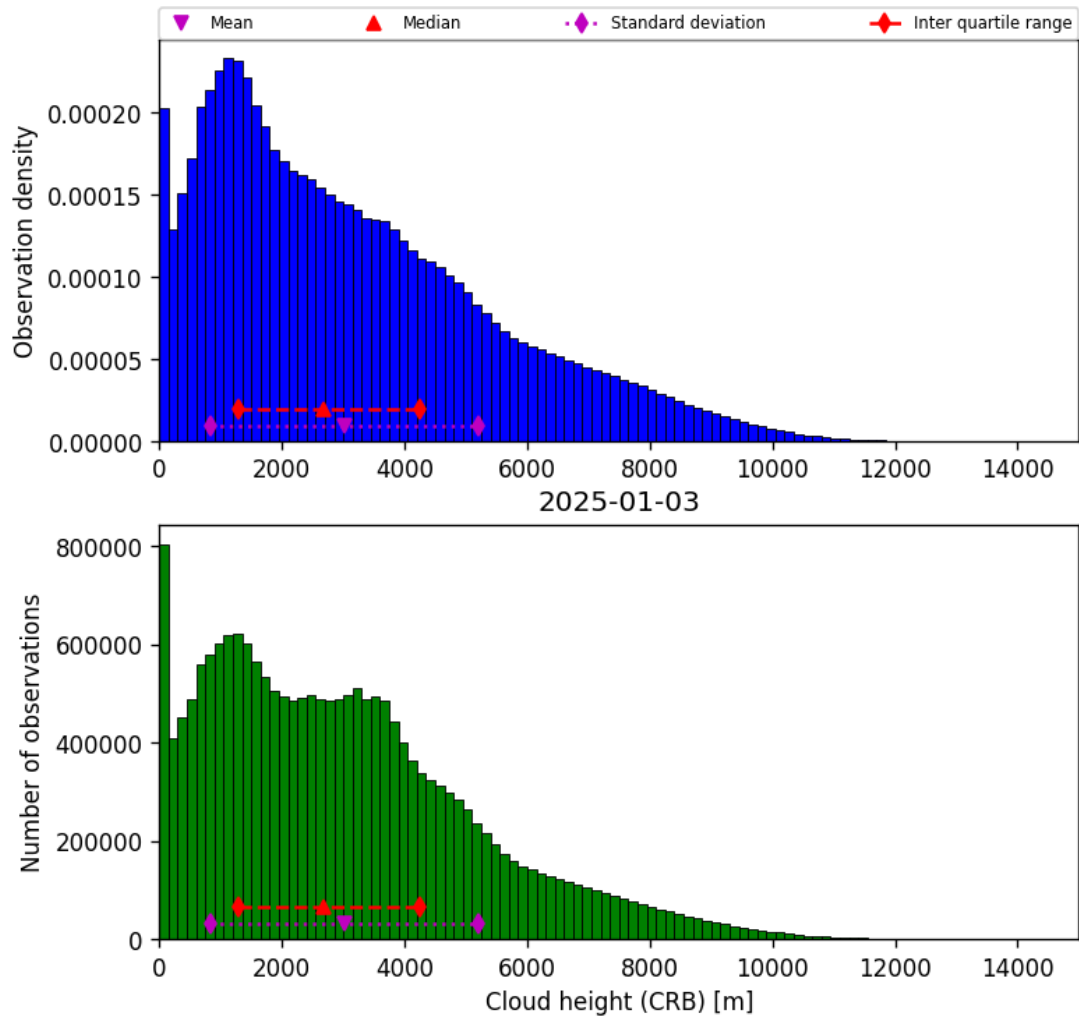
Figure 41: Histogram of “Cloud height (CRB)” for 2025-01-03 to 2025-01-04
