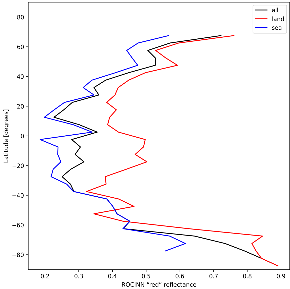
Figure 35: Zonal average of “ROCINN “red” reflectance” for 2025-01-03 to 2025-01-04.
