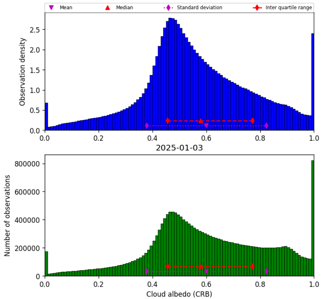
Figure 42: Histogram of “Cloud albedo (CRB)” for 2025-01-03 to 2025-01-04
