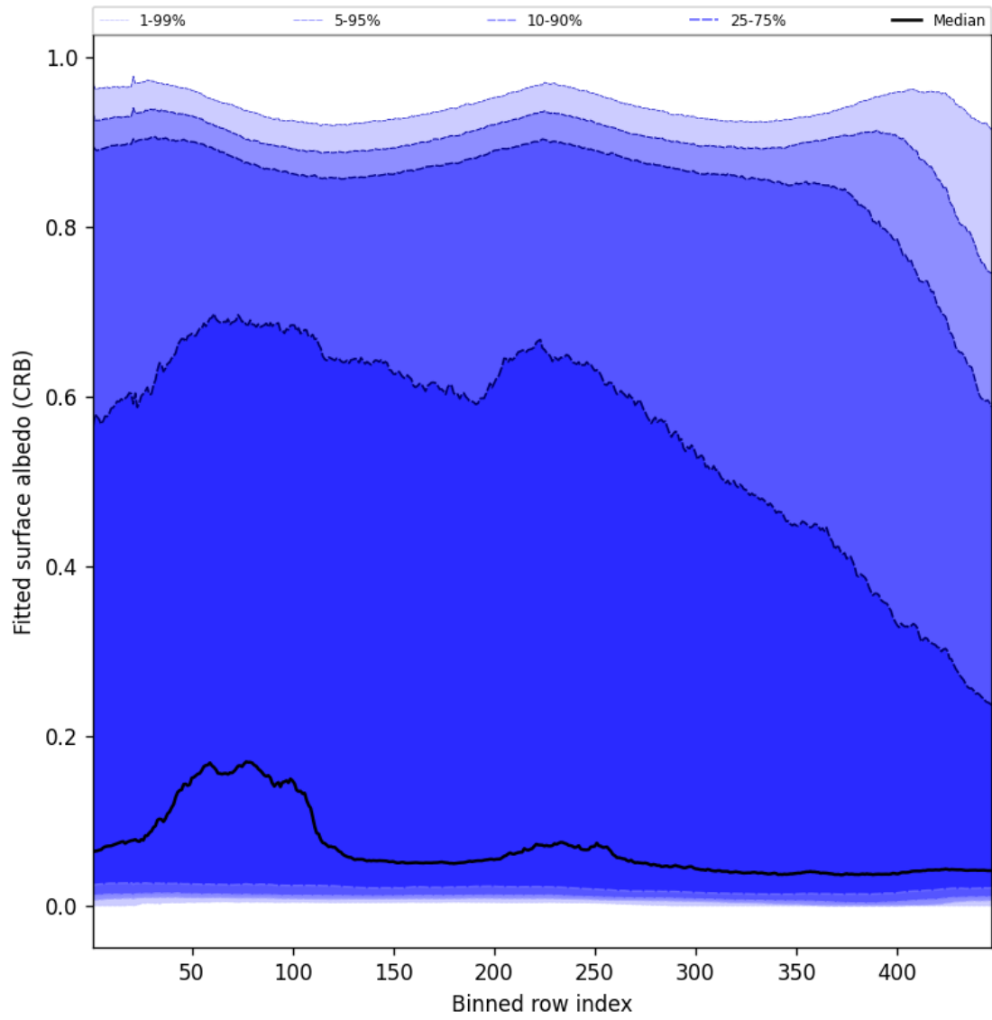
Figure 60: Along track statistics of “Fitted surface albedo (CRB)” for 2025-01-03 to 2025-01-04
