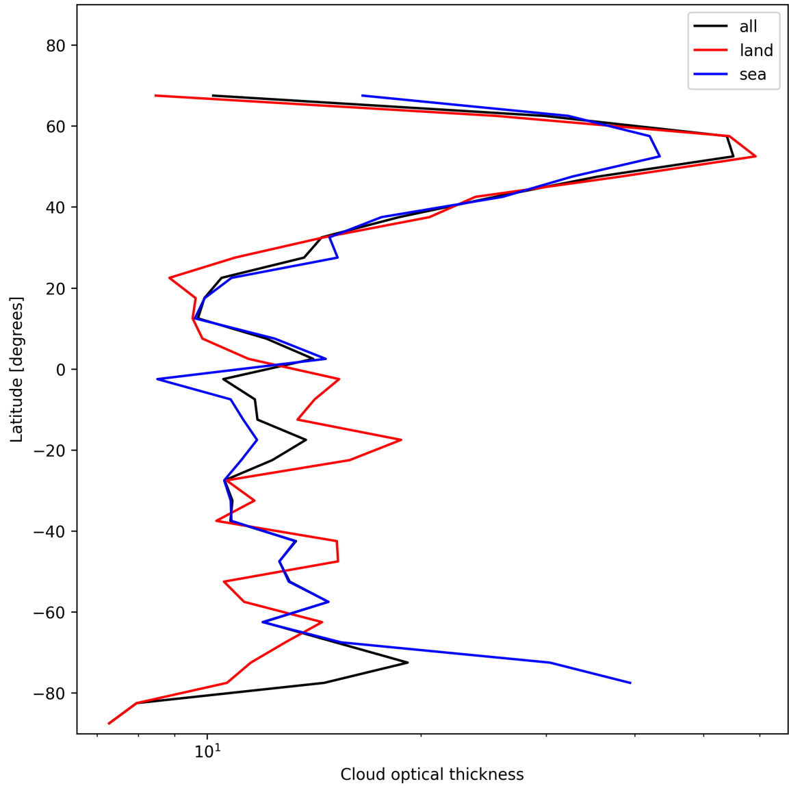
Figure 23: Zonal average of “Cloud optical thickness” for 2025-01-03 to 2025-01-04.
