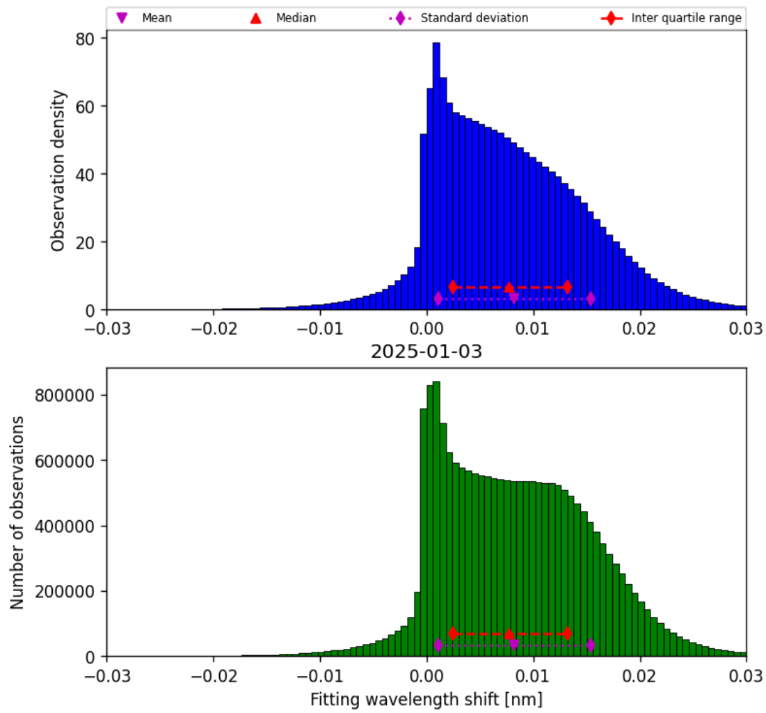
Figure 47: Histogram of “Fitting wavelength shift” for 2025-01-03 to 2025-01-04
