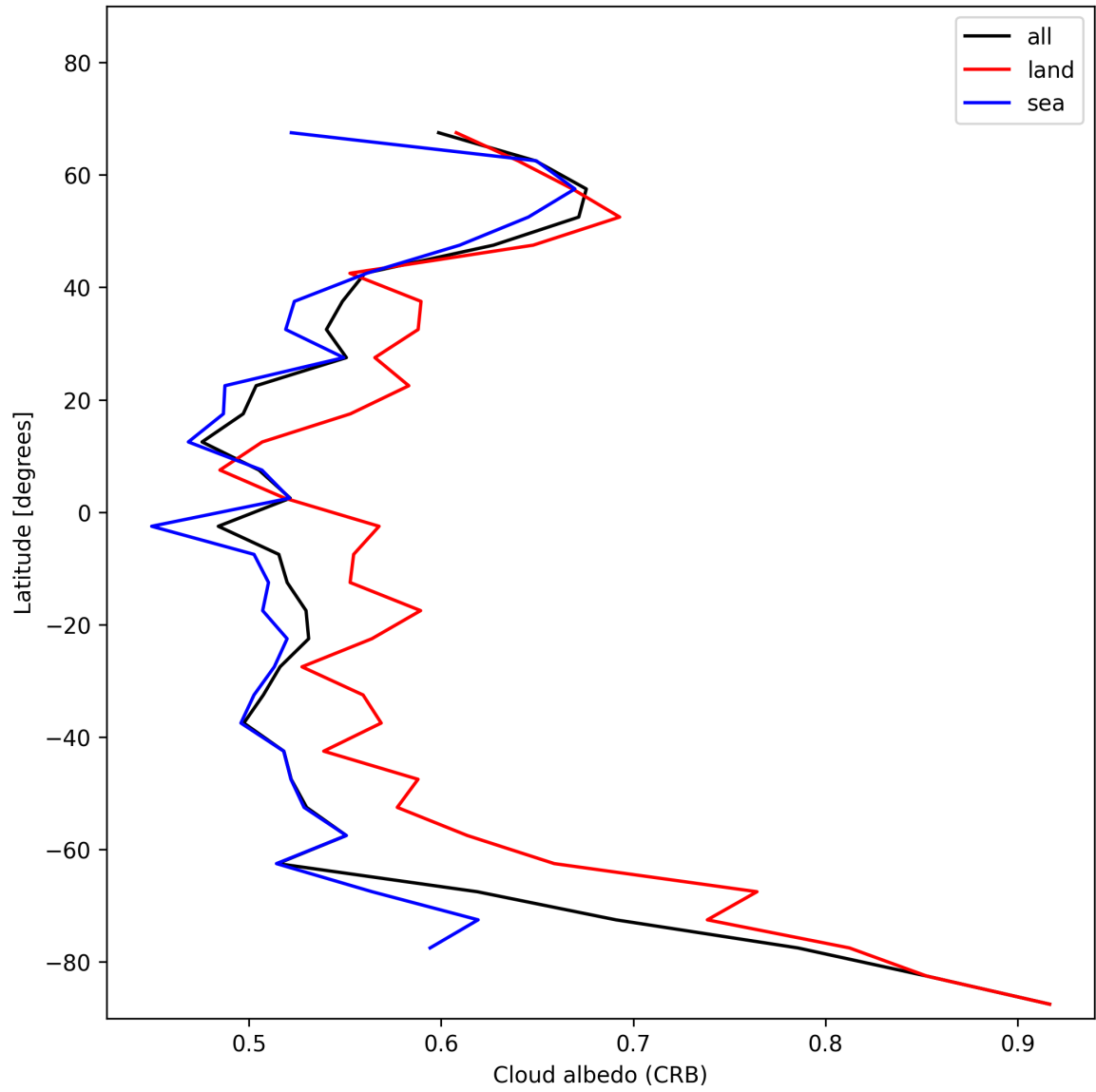
Figure 26: Zonal average of “Cloud albedo (CRB)” for 2025-01-03 to 2025-01-04.
