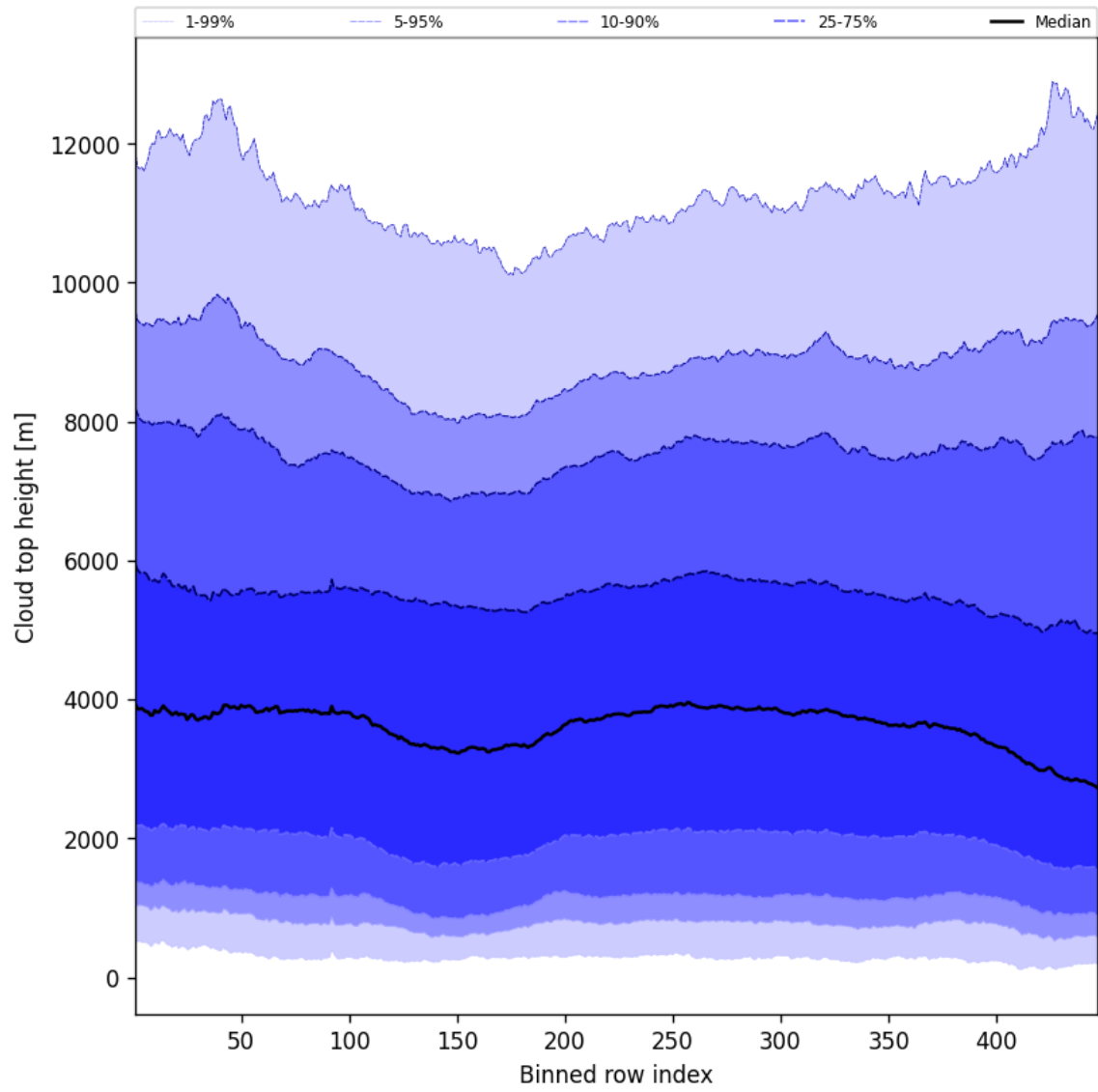
Figure 54: Along track statistics of “Cloud top height” for 2025-01-03 to 2025-01-04
