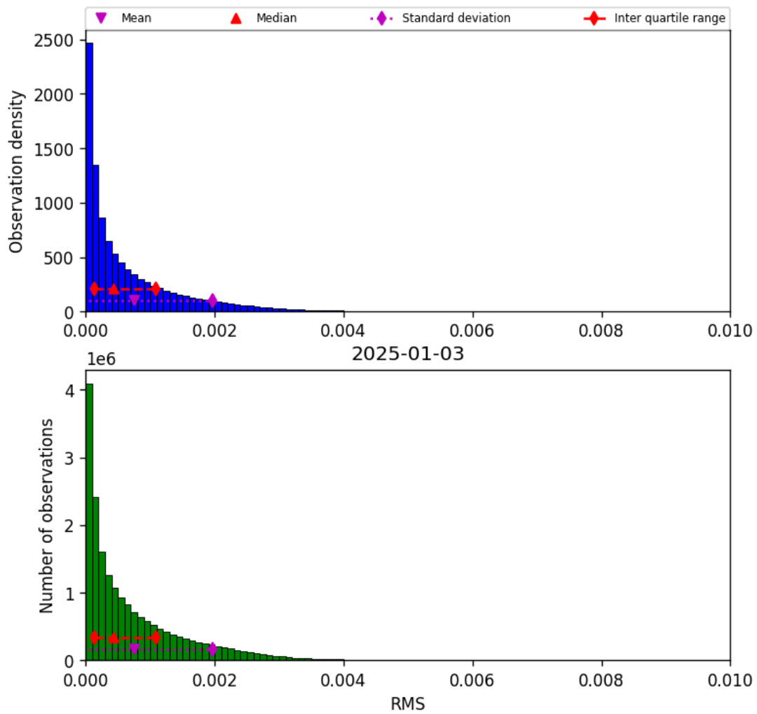
Figure 45: Histogram of “RMS” for 2025-01-03 to 2025-01-04
