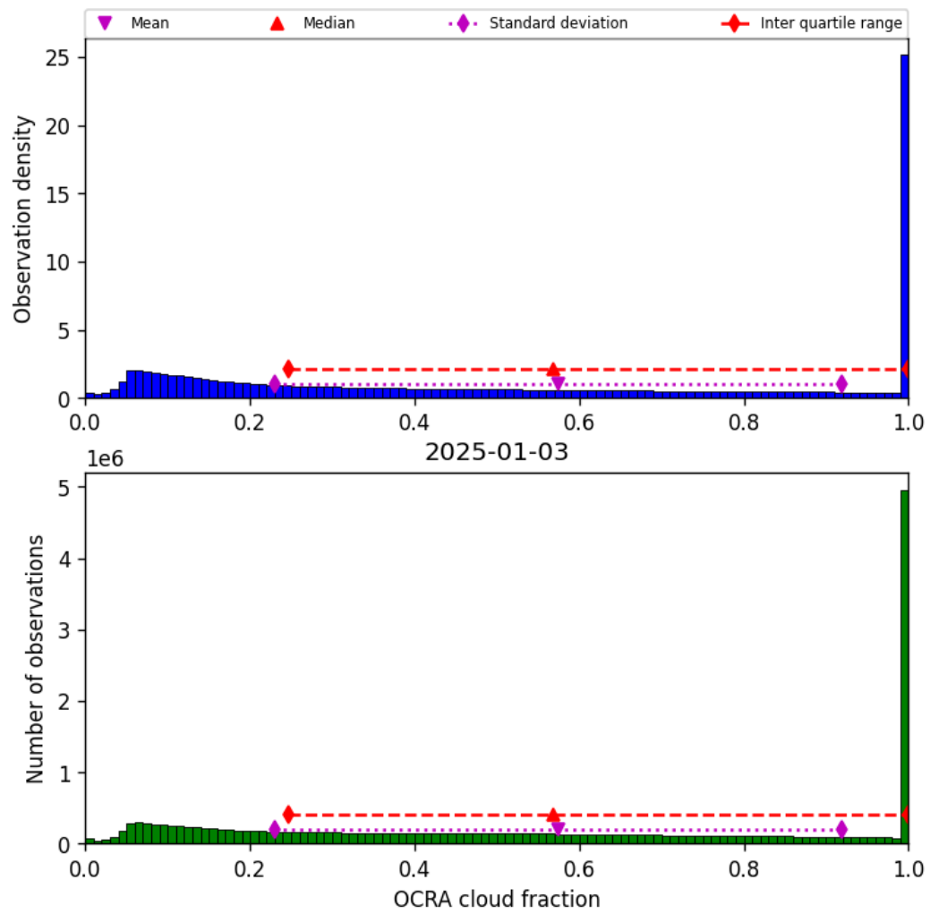
Figure 48: Histogram of “OCRA cloud fraction” for 2025-01-03 to 2025-01-04
