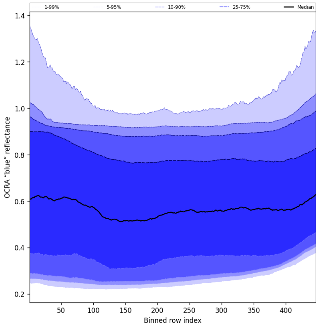
Figure 65: Along track statistics of “OCRA “blue” reflectance” for 2025-01-03 to 2025-01-04
