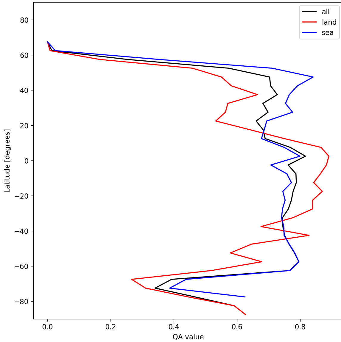
Figure 20: Zonal average of “QA value” for 2025-01-03 to 2025-01-04.
