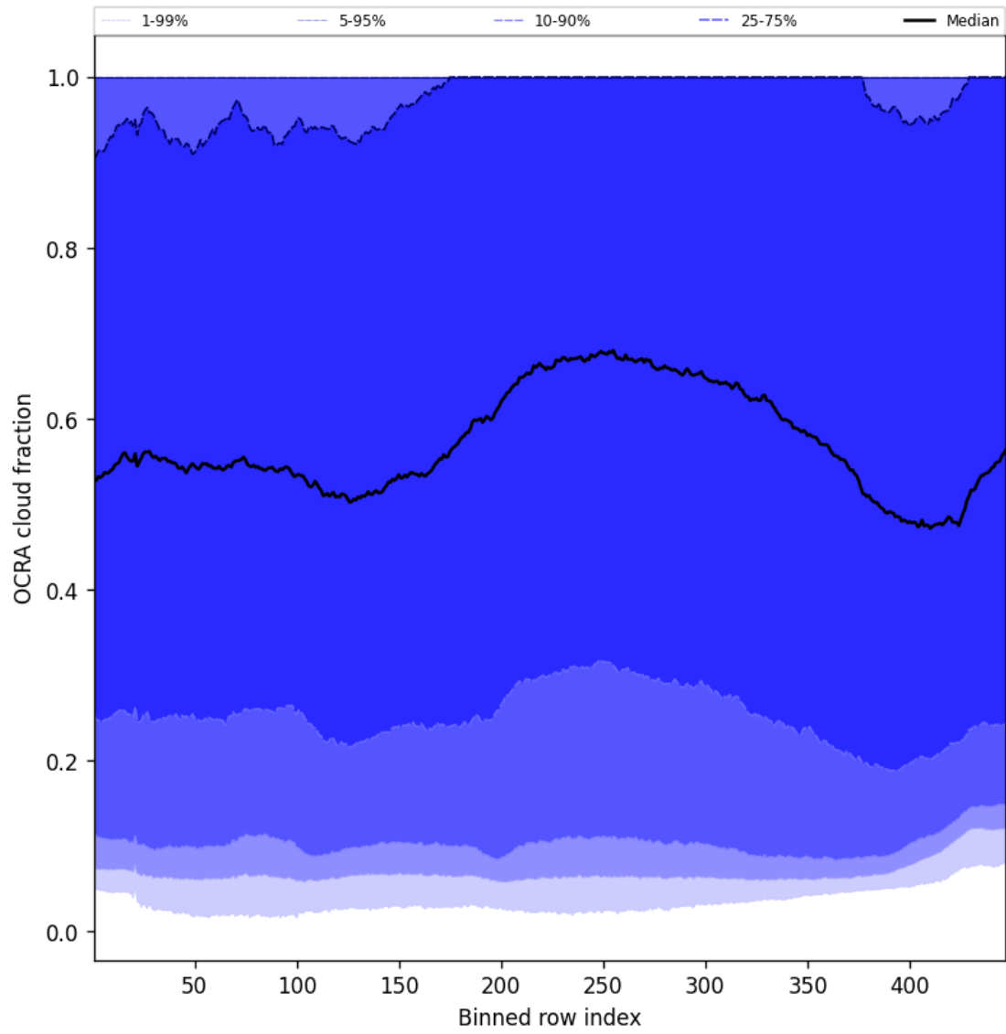
Figure 64: Along track statistics of “OCRA cloud fraction” for 2025-01-03 to 2025-01-04
