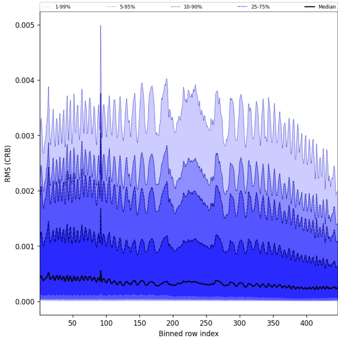
Figure 62: Along track statistics of “RMS (CRB)” for 2025-01-03 to 2025-01-04
