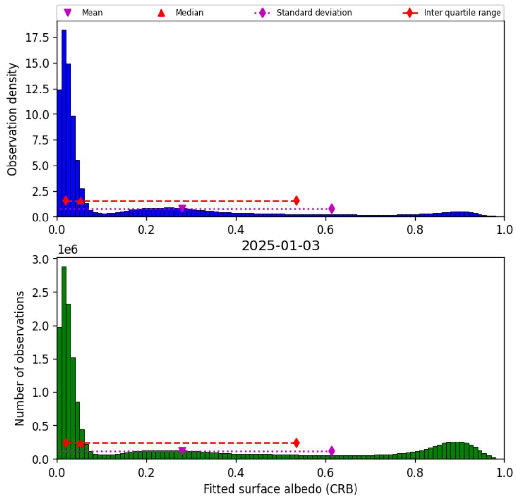
Figure 44: Histogram of “Fitted surface albedo (CRB)” for 2025-01-03 to 2025-01-04
