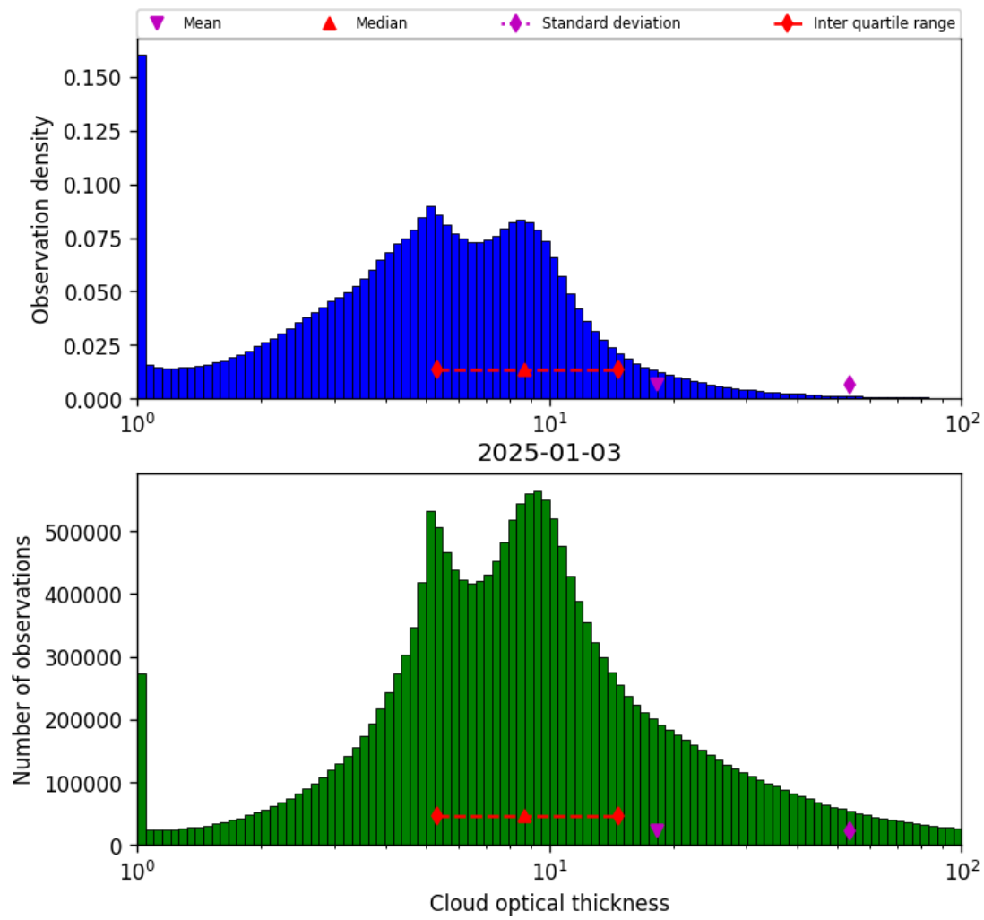
Figure 39: Histogram of “Cloud optical thickness” for 2025-01-03 to 2025-01-04
