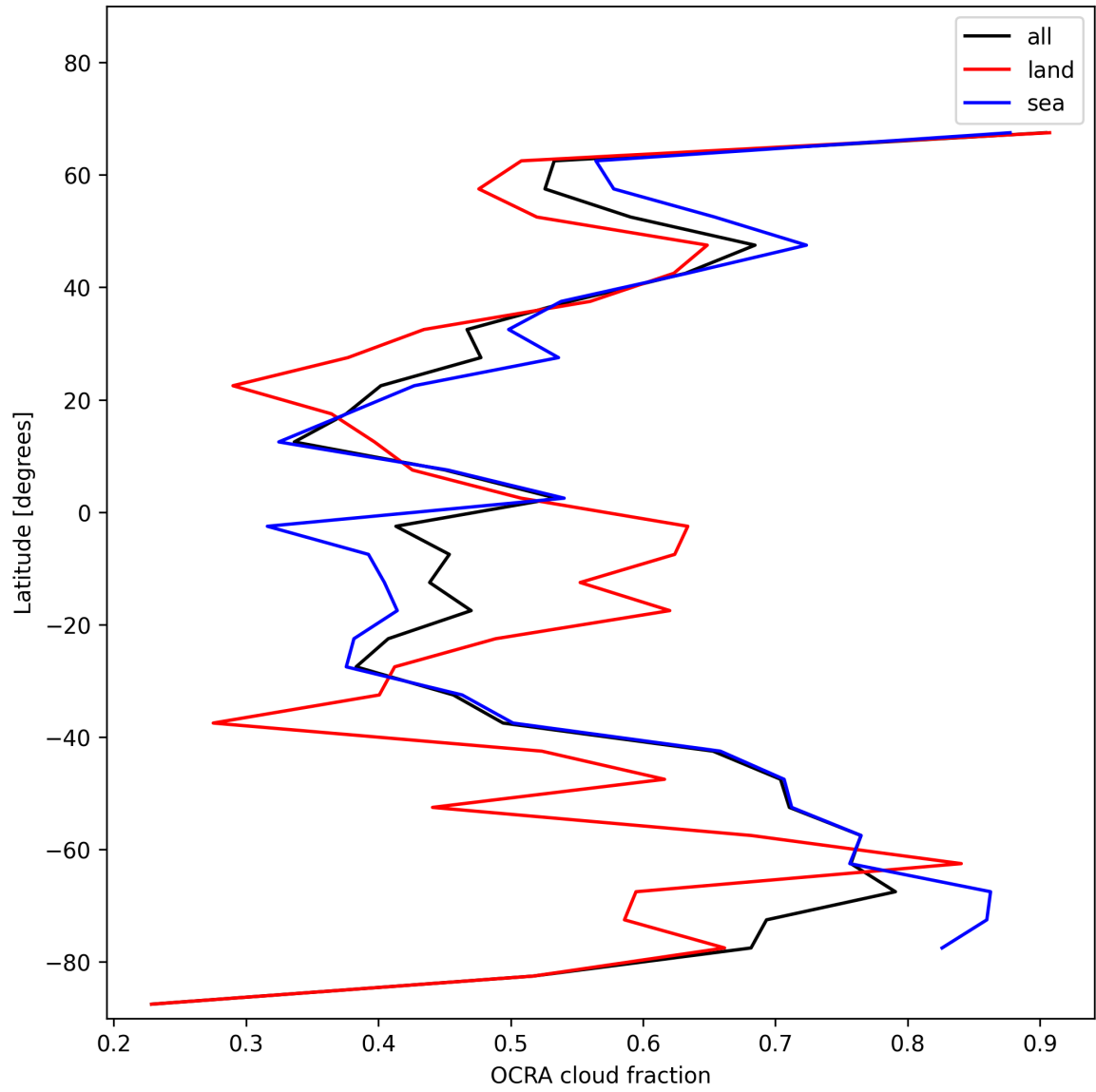
Figure 32: Zonal average of “OCRA cloud fraction” for 2025-01-03 to 2025-01-04.
