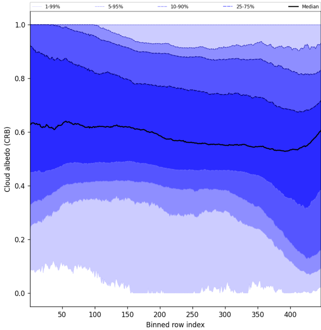
Figure 58: Along track statistics of “Cloud albedo (CRB)” for 2025-01-03 to 2025-01-04
