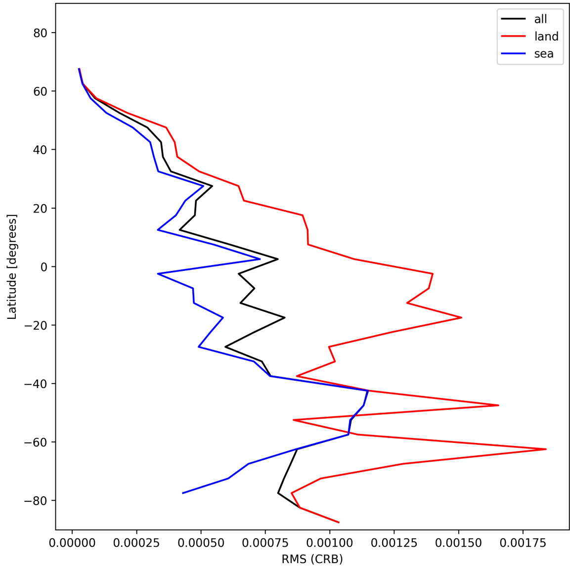
Figure 30: Zonal average of “RMS (CRB)” for 2025-01-03 to 2025-01-04.
