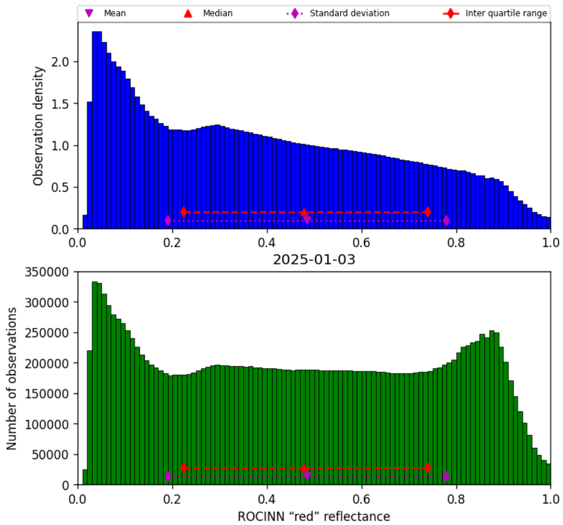
Figure 51: Histogram of “ROCINN “red” reflectance” for 2025-01-03 to 2025-01-04
