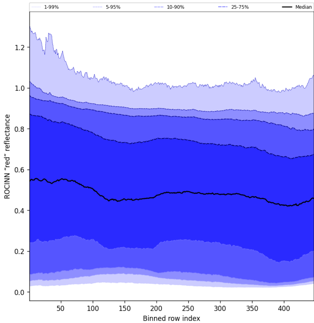
Figure 67: Along track statistics of "ROCINN "red" reflectance" for 2025-01-03 to 2025-01-04
