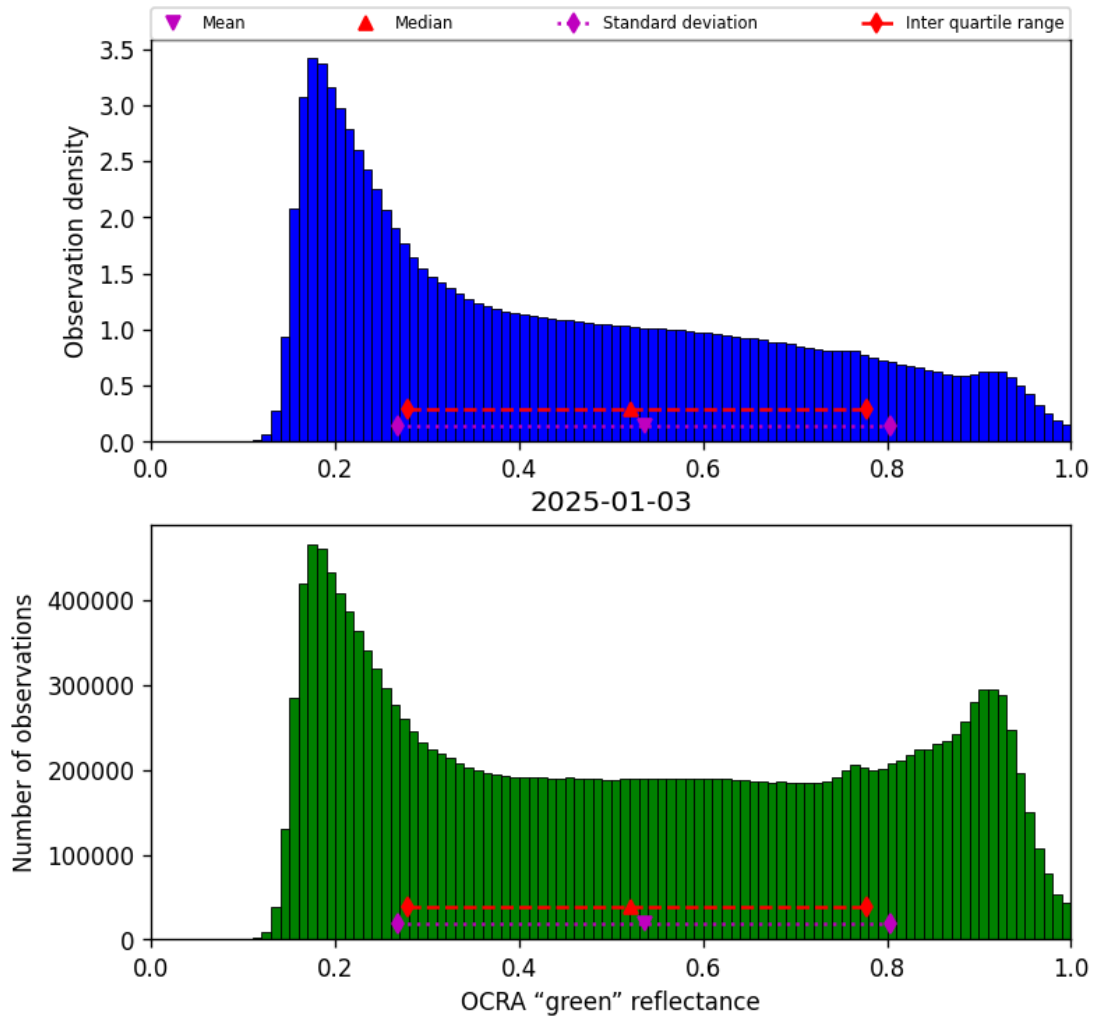
Figure 50: Histogram of “OCRA “green” reflectance” for 2025-01-03 to 2025-01-04
