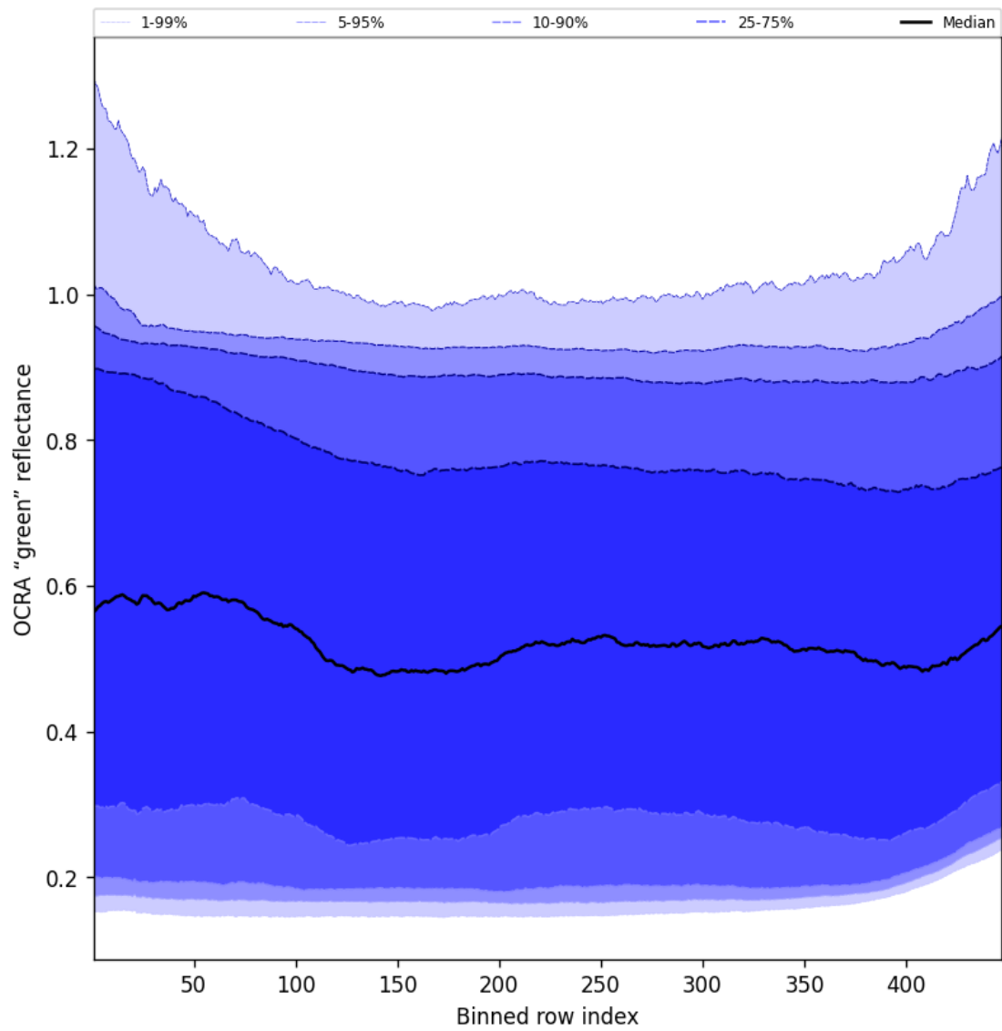
Figure 66: Along track statistics of “OCRA “green” reflectance” for 2025-01-03 to 2025-01-04
