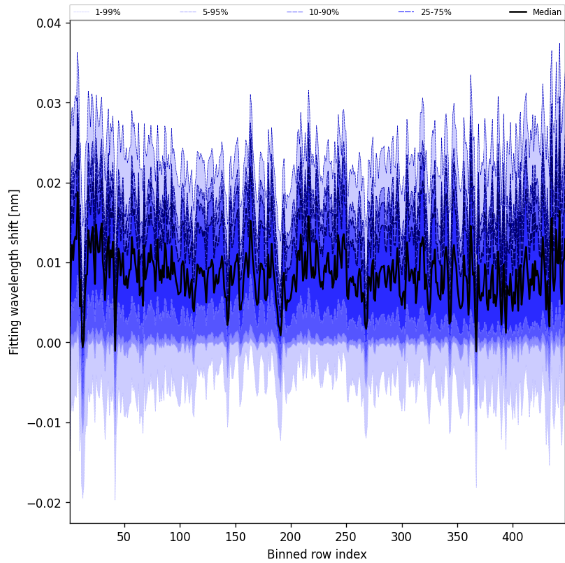
Figure 63: Along track statistics of “Fitting wavelength shift” for 2025-01-03 to 2025-01-04
