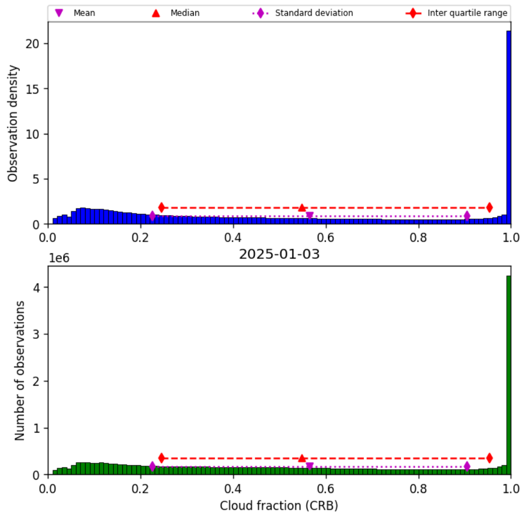
Figure 40: Histogram of “Cloud fraction (CRB)” for 2025-01-03 to 2025-01-04
