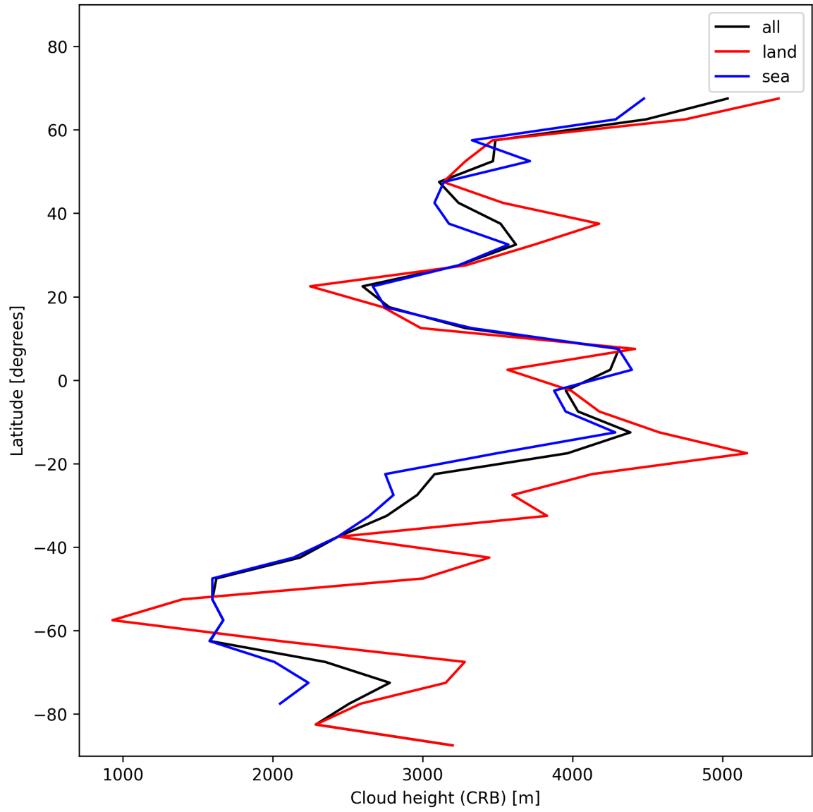
Figure 25: Zonal average of “Cloud height (CRB)” for 2025-01-03 to 2025-01-04.
