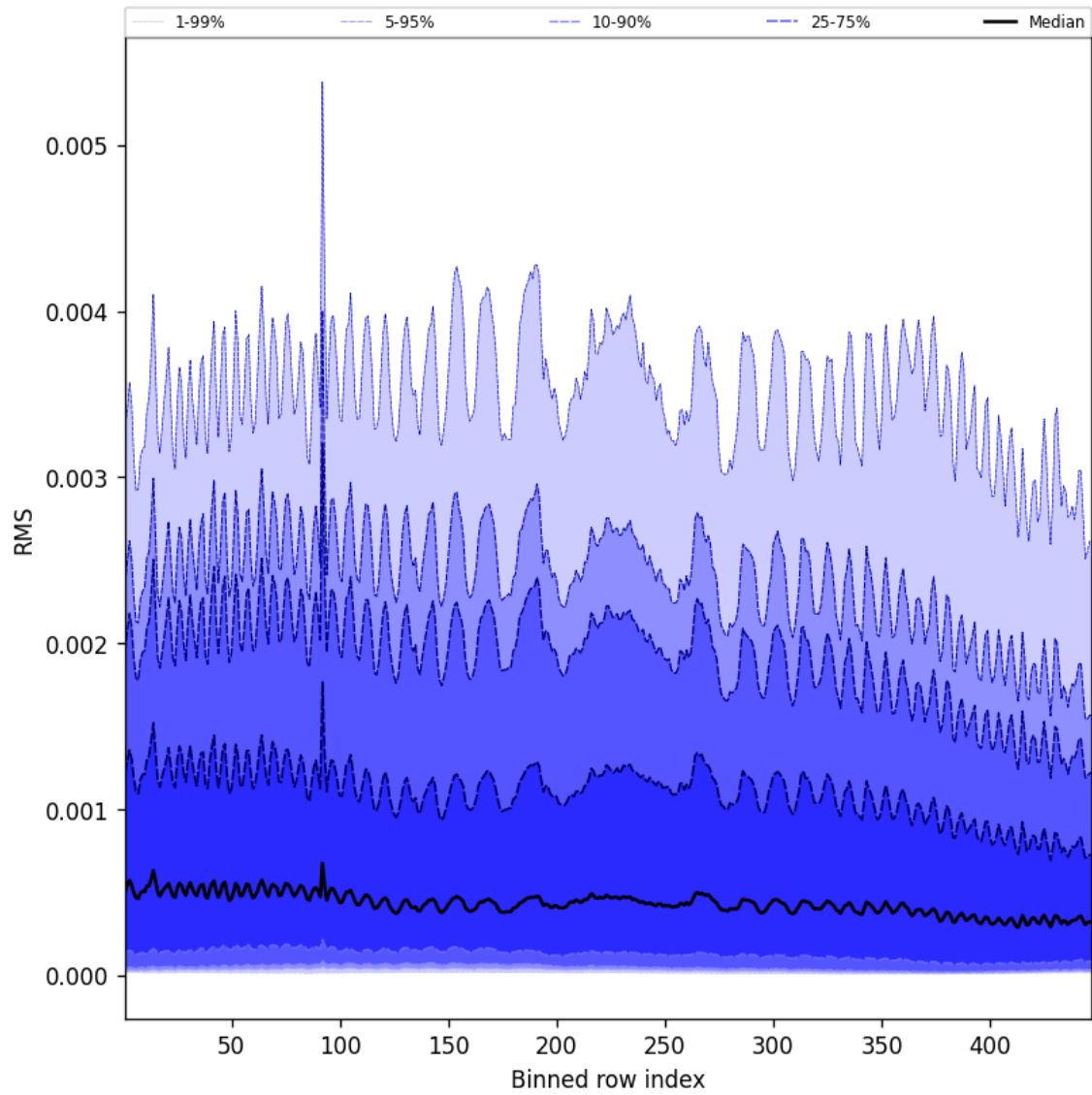
Figure 61: Along track statistics of “RMS” for 2025-01-03 to 2025-01-04
