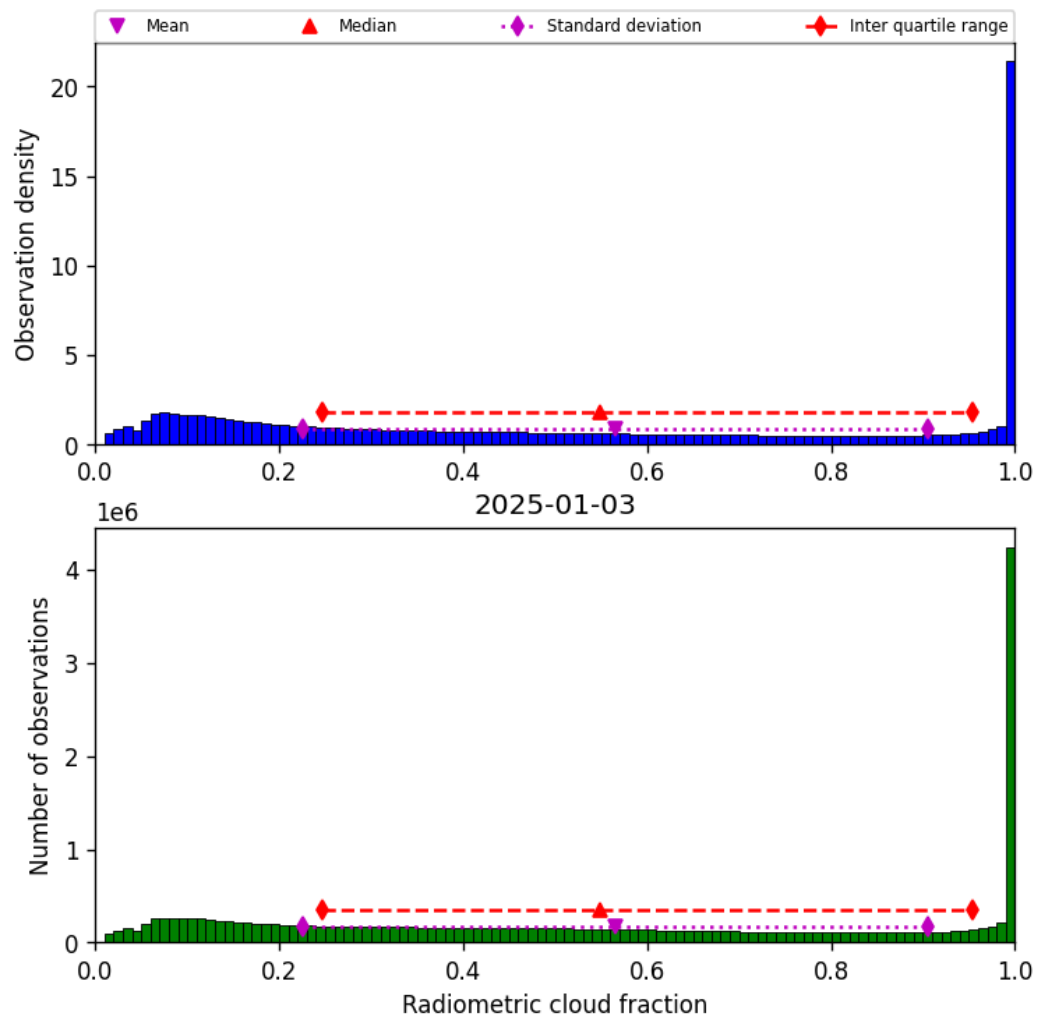
Figure 37: Histogram of “Radiometric cloud fraction” for 2025-01-03 to 2025-01-04
