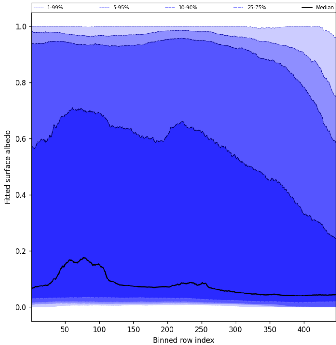
Figure 59: Along track statistics of “Fitted surface albedo” for 2025-01-03 to 2025-01-04
