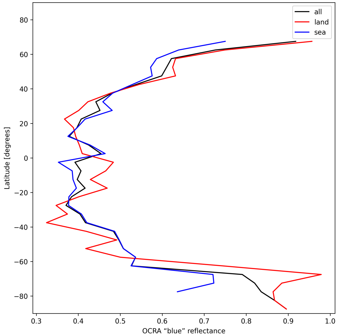
Figure 33: Zonal average of “OCRA “blue” reflectance” for 2025-01-03 to 2025-01-04.
