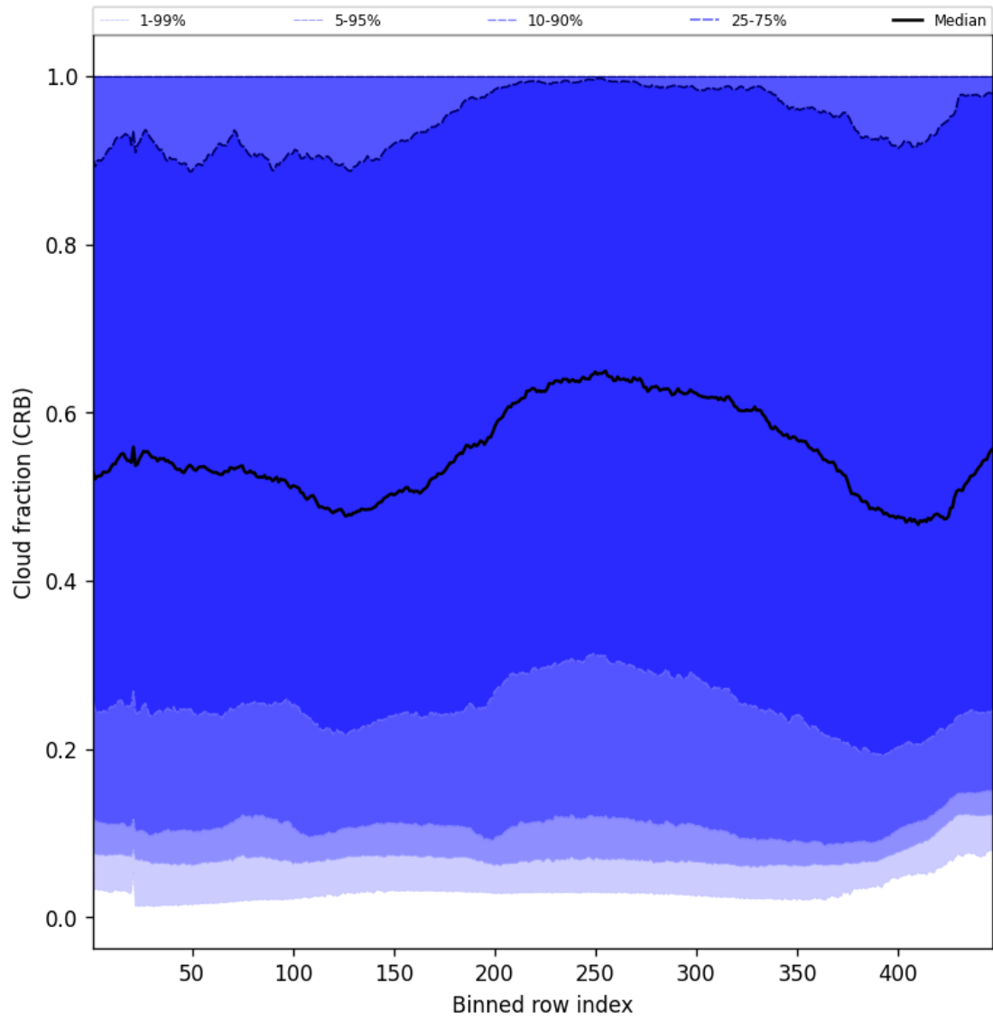
Figure 56: Along track statistics of “Cloud fraction (CRB)” for 2025-01-03 to 2025-01-04
