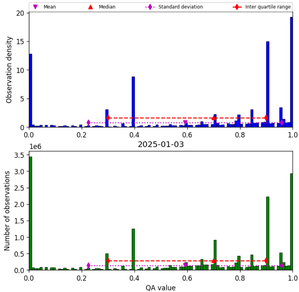
Figure 36: Histogram of “QA value” for 2025-01-03 to 2025-01-04
