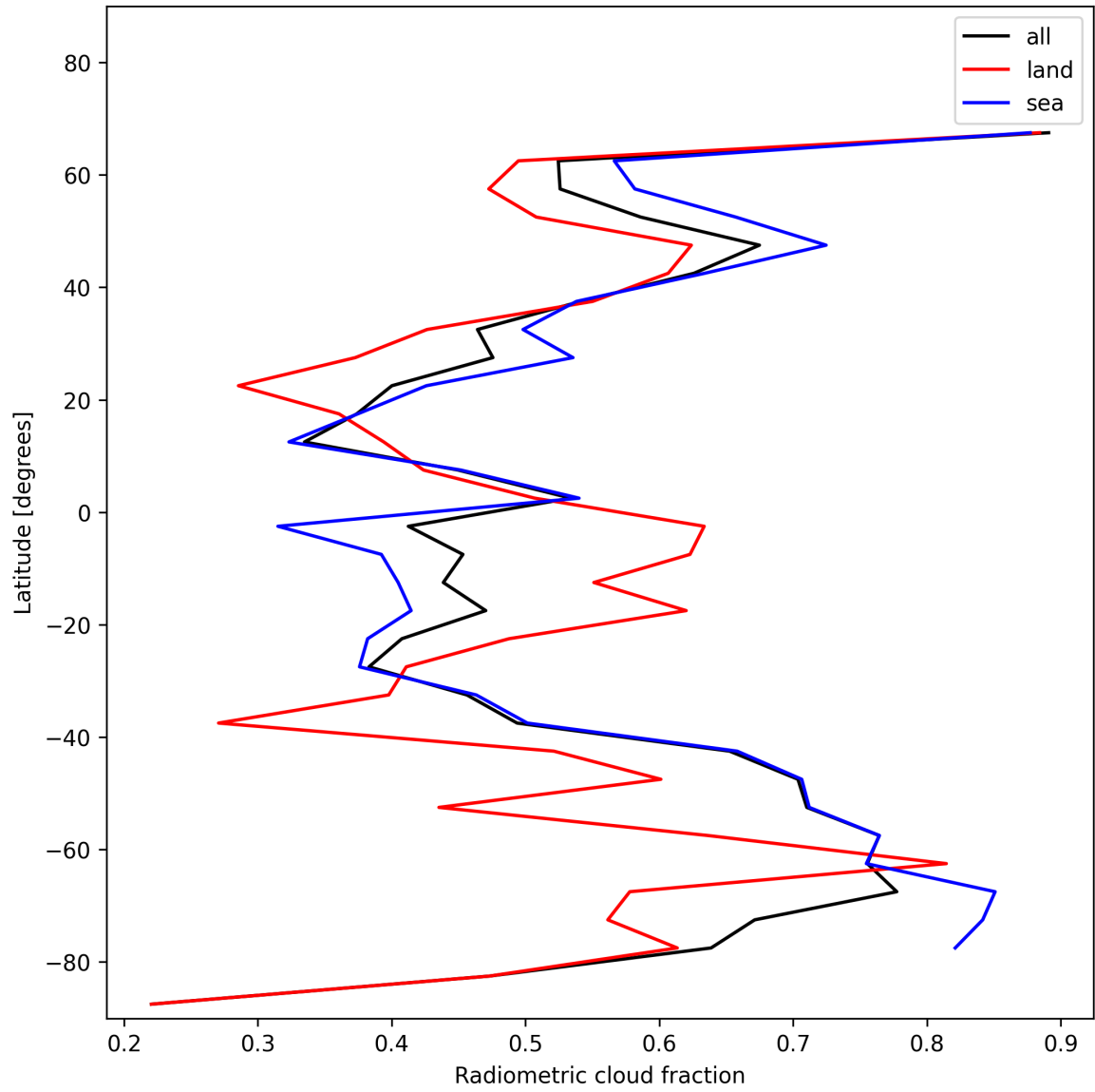
Figure 21: Zonal average of “Radiometric cloud fraction” for 2025-01-03 to 2025-01-04.
