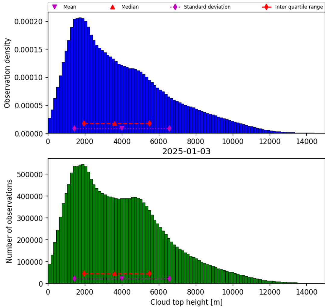
Figure 38: Histogram of “Cloud top height” for 2025-01-03 to 2025-01-04
