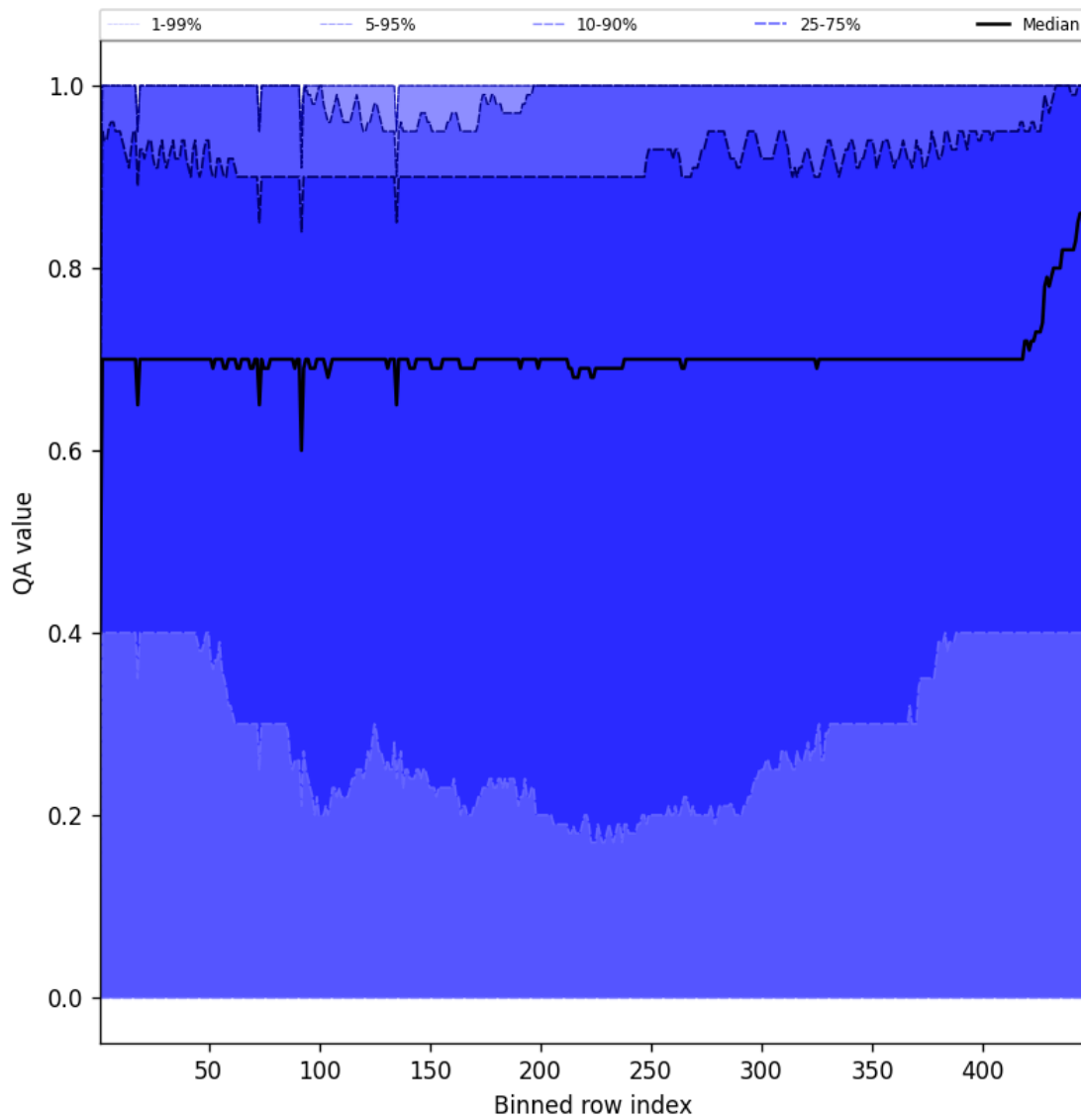
Figure 52: Along track statistics of “QA value” for 2025-01-03 to 2025-01-04
