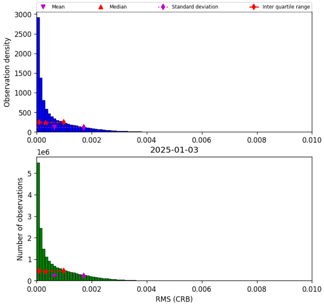
Figure 46: Histogram of “RMS (CRB)” for 2025-01-03 to 2025-01-04
