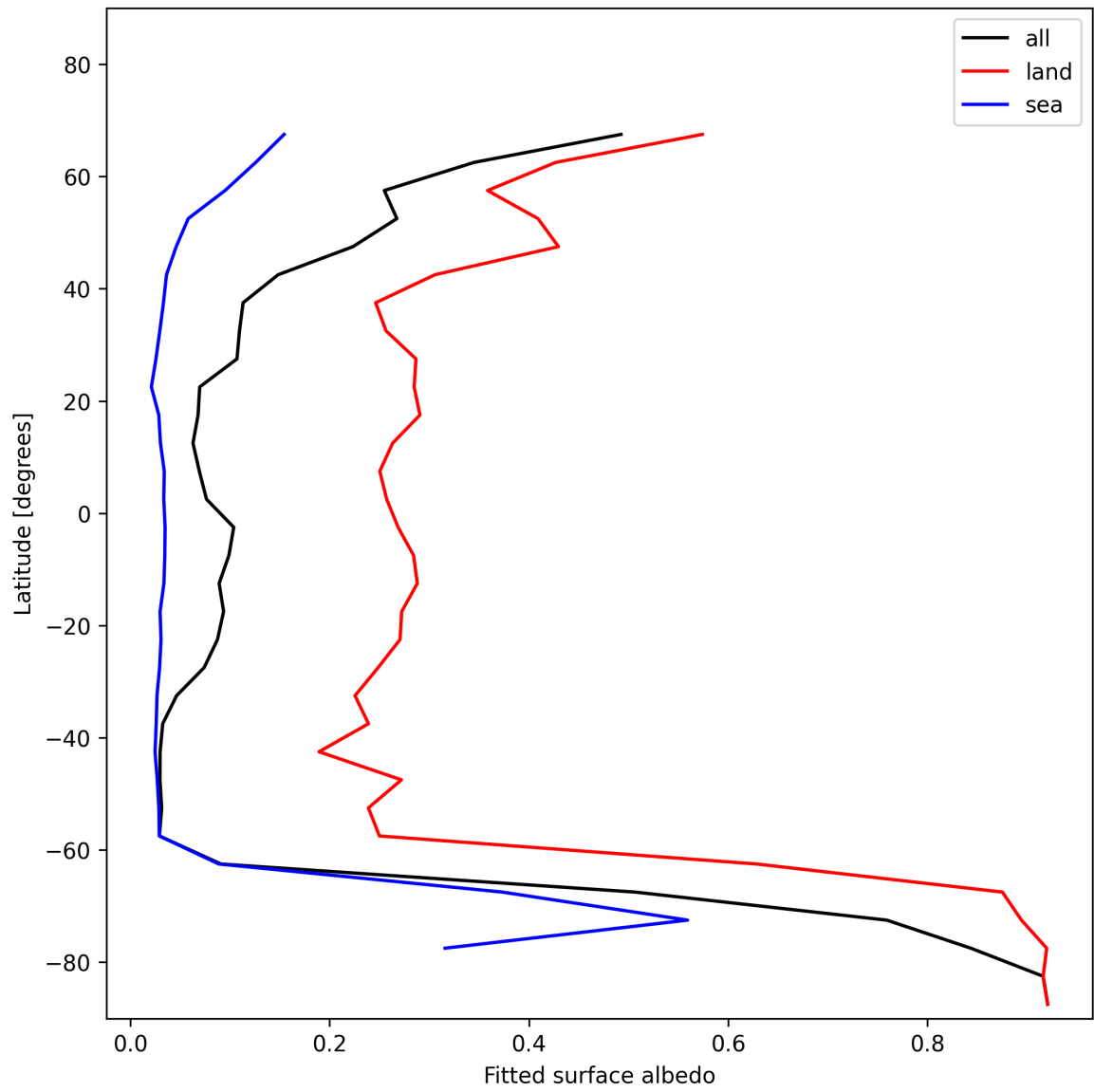
Figure 27: Zonal average of “Fitted surface albedo” for 2025-01-03 to 2025-01-04.
