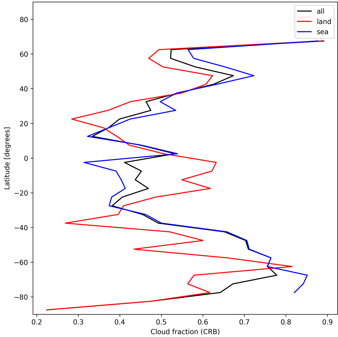
Figure 24: Zonal average of “Cloud fraction (CRB)” for 2025-01-03 to 2025-01-04.
