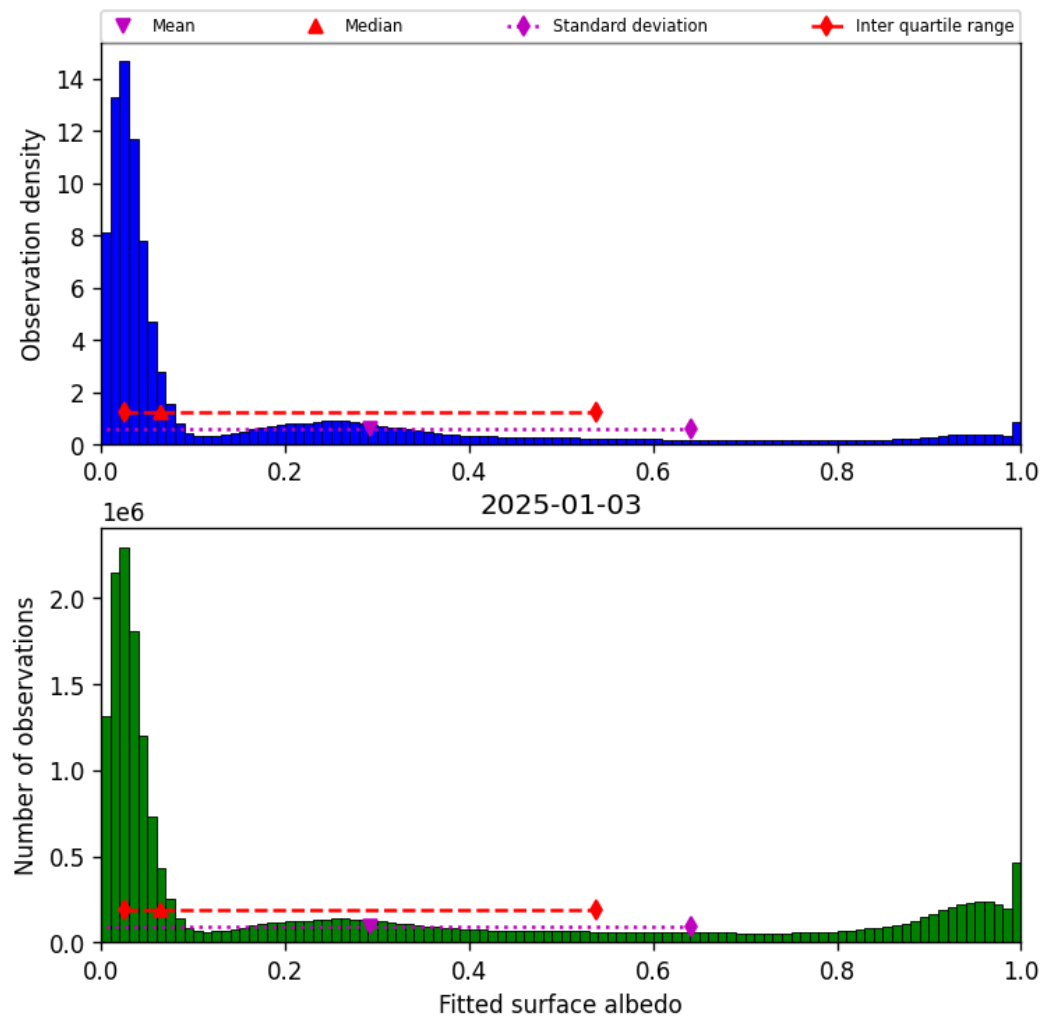
Figure 43: Histogram of “Fitted surface albedo” for 2025-01-03 to 2025-01-04
