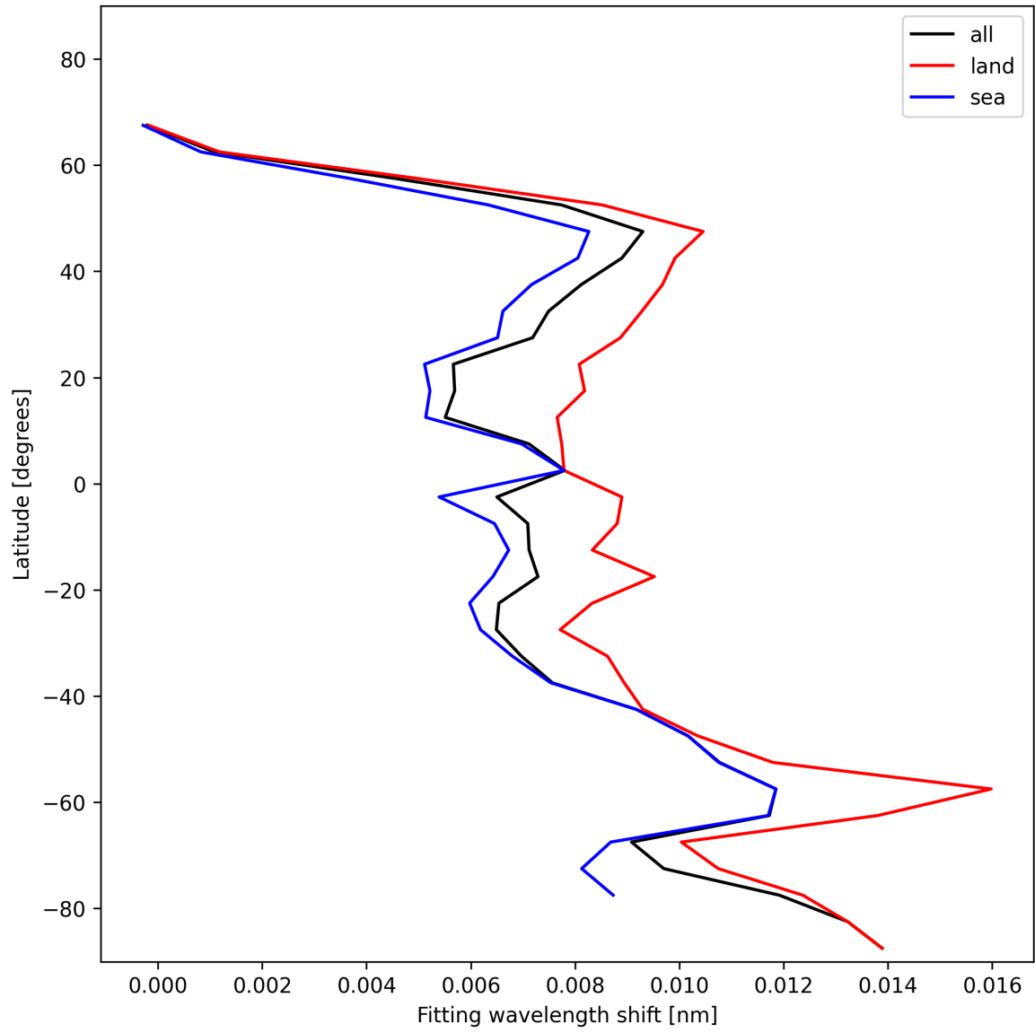
Figure 31: Zonal average of “Fitting wavelength shift” for 2025-01-03 to 2025-01-04.
