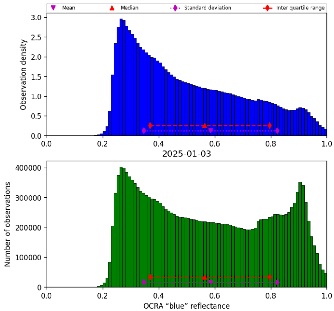
Figure 49: Histogram of “OCRA “blue” reflectance” for 2025-01-03 to 2025-01-04
