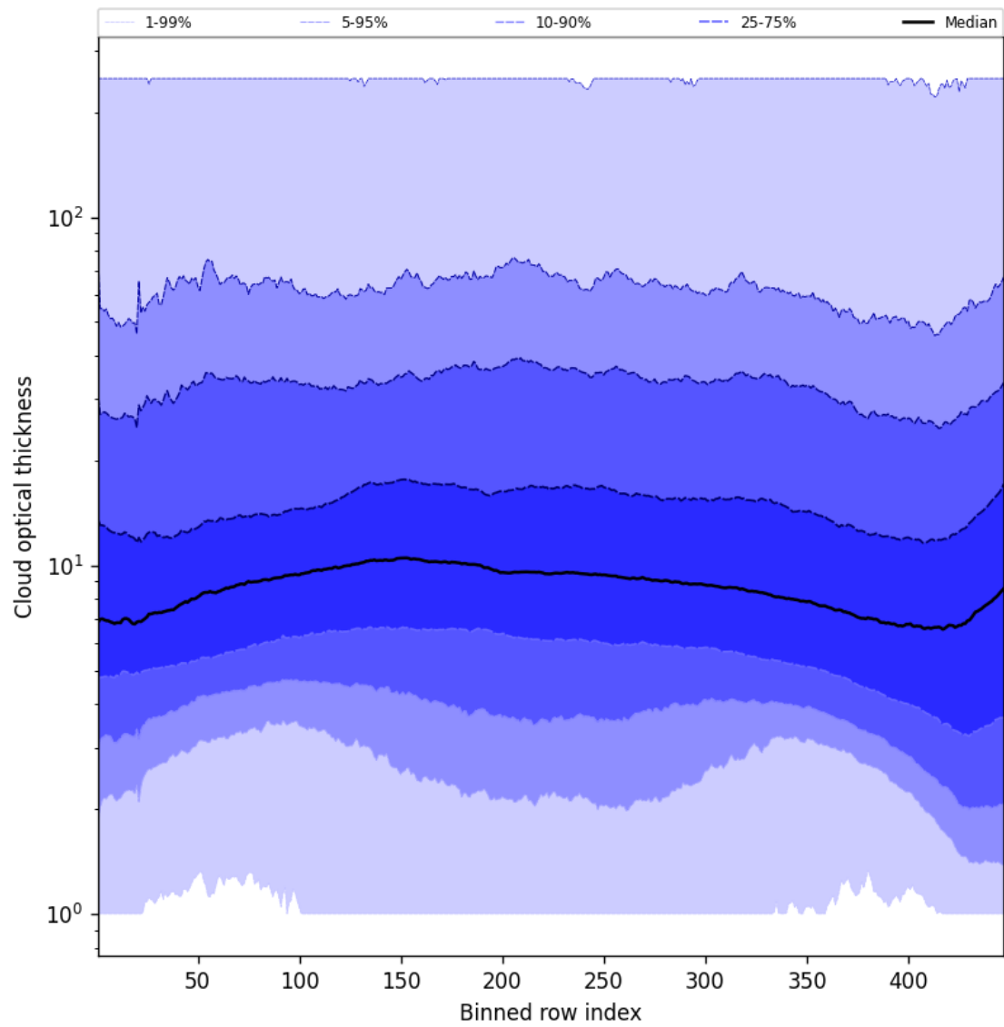
Figure 55: Along track statistics of “Cloud optical thickness” for 2025-01-03 to 2025-01-04
