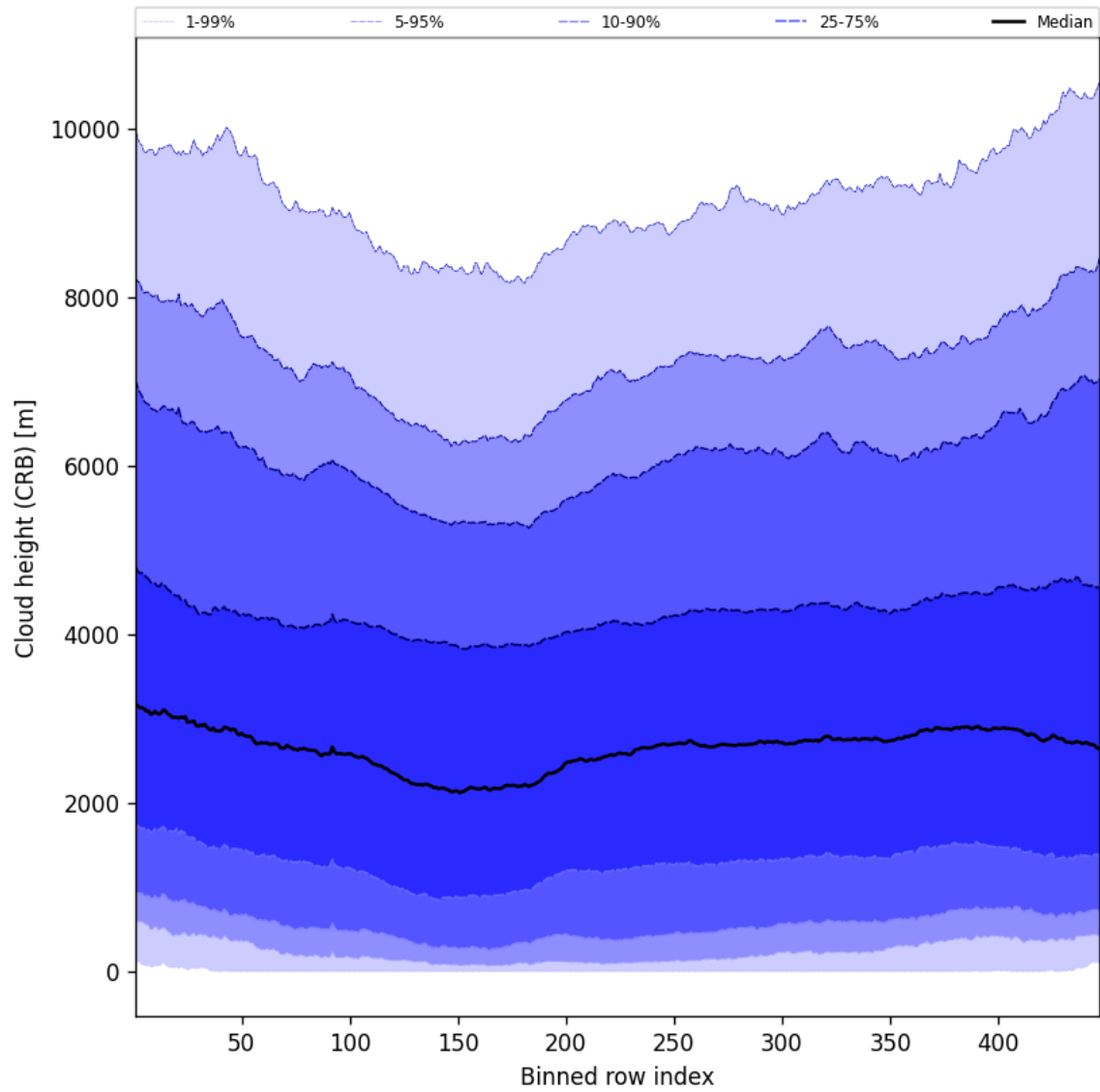
Figure 57: Along track statistics of “Cloud height (CRB)” for 2025-01-03 to 2025-01-04
