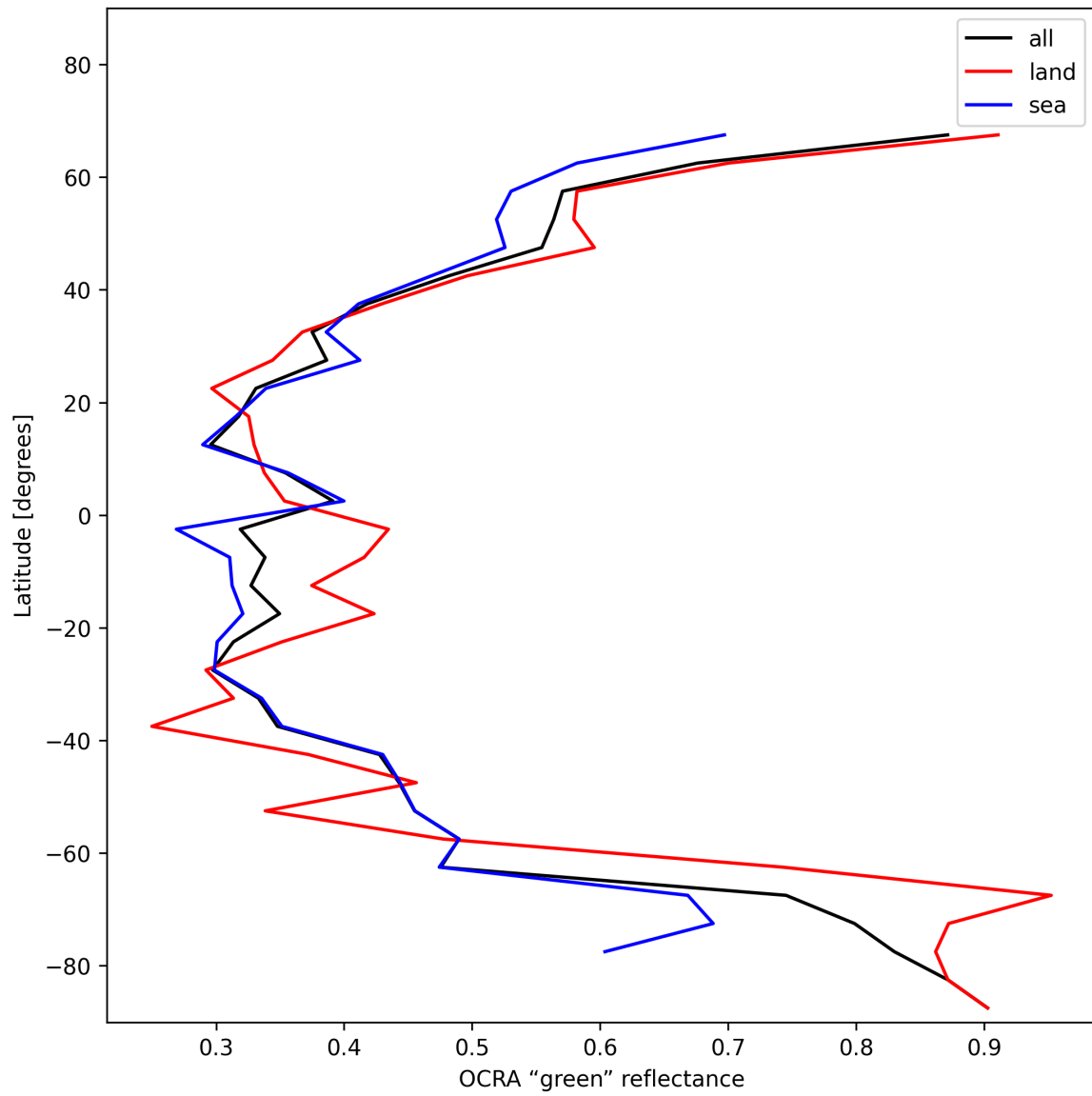
Figure 34: Zonal average of “OCRA “green” reflectance” for 2025-01-03 to 2025-01-04.
