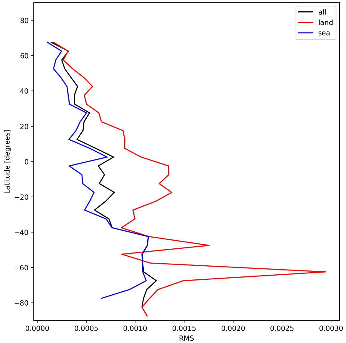
Figure 29: Zonal average of “RMS” for 2025-01-03 to 2025-01-04.
