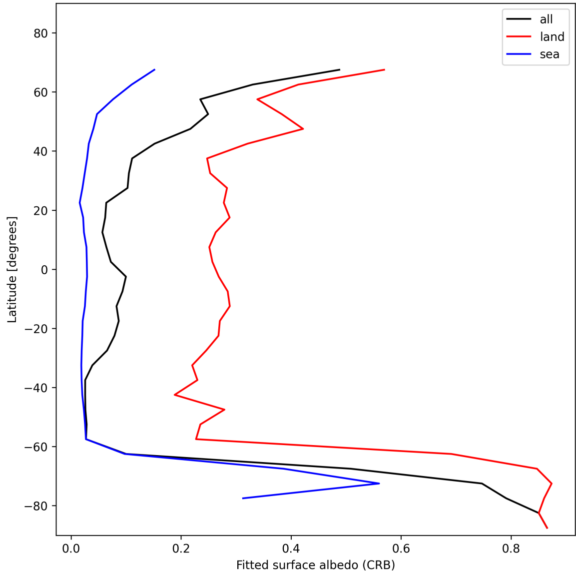
Figure 28: Zonal average of “Fitted surface albedo (CRB)” for 2025-01-03 to 2025-01-04.
