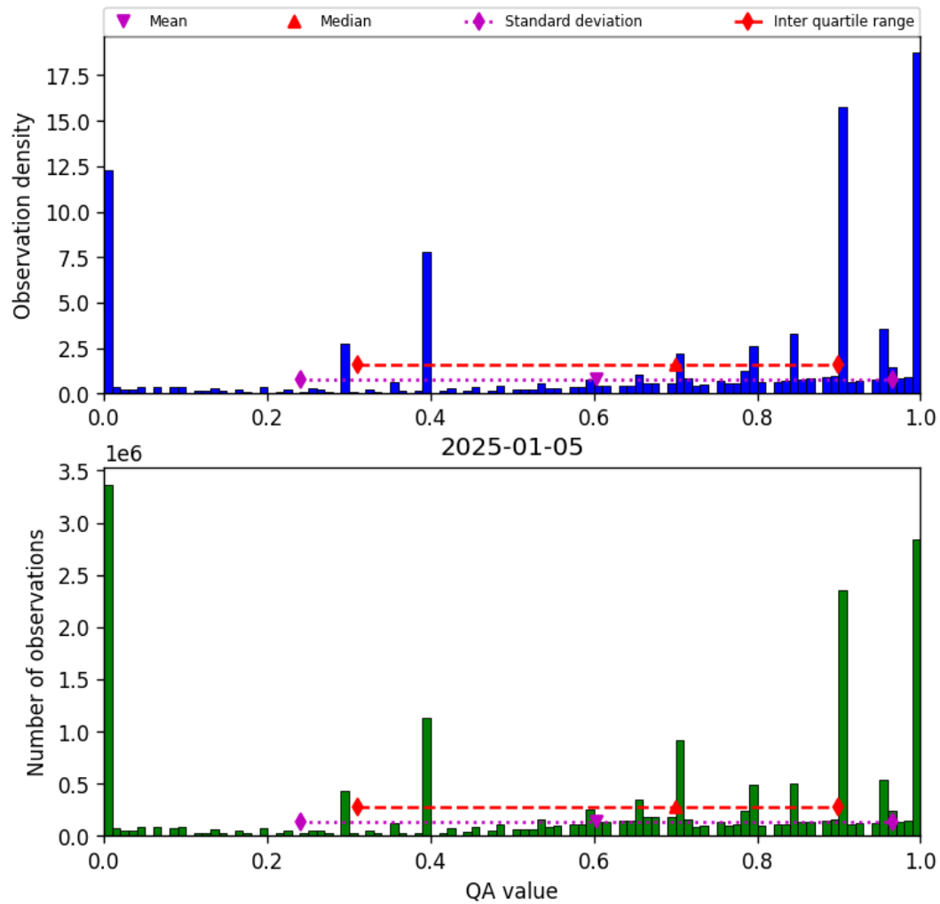
Figure 36: Histogram of “QA value” for 2025-01-05 to 2025-01-05
