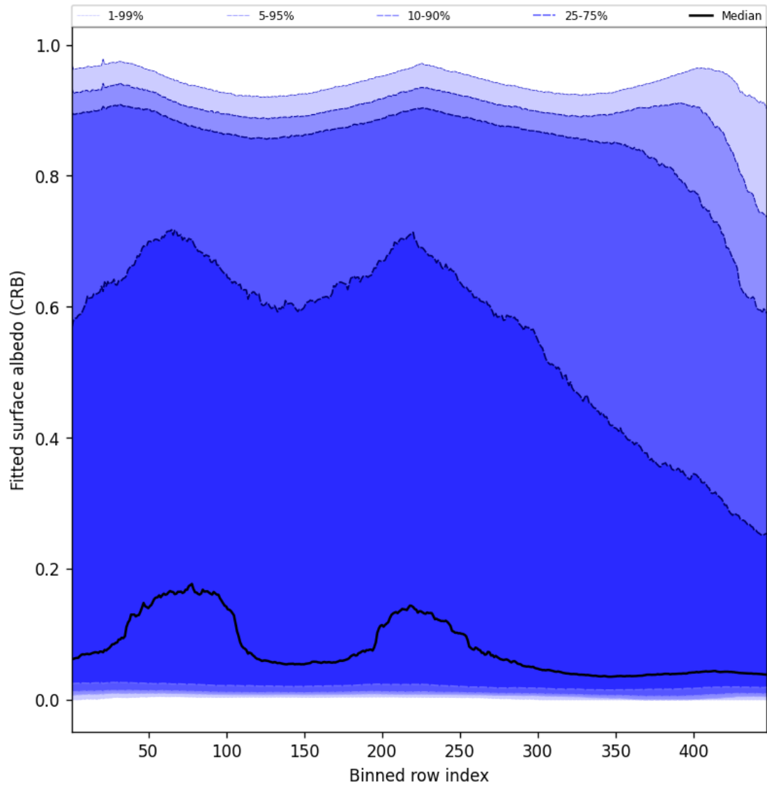
Figure 60: Along track statistics of “Fitted surface albedo (CRB)” for 2025-01-05 to 2025-01-05
