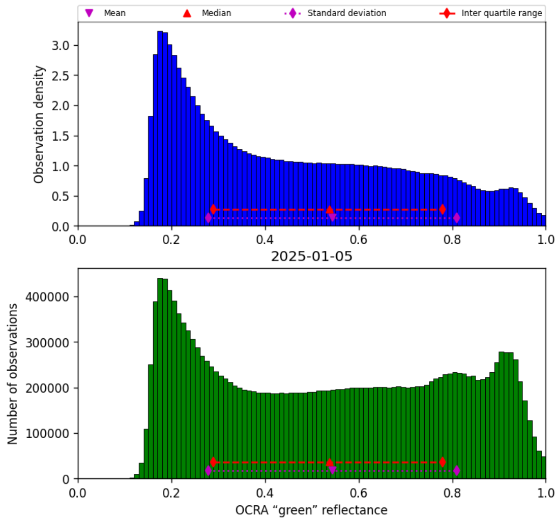
Figure 50: Histogram of “OCRA “green” reflectance” for 2025-01-05 to 2025-01-05
