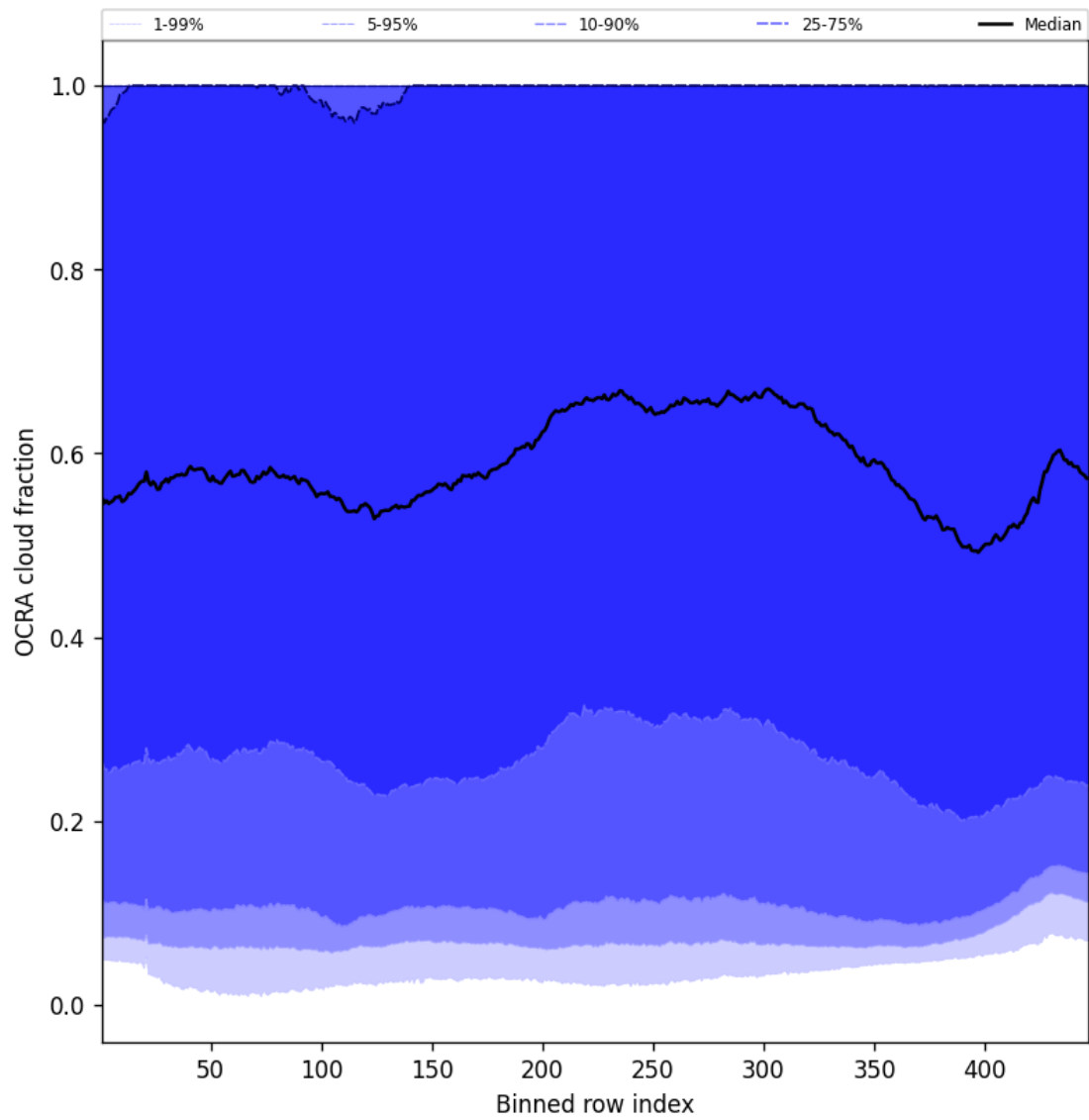
Figure 64: Along track statistics of “OCRA cloud fraction” for 2025-01-05 to 2025-01-05
