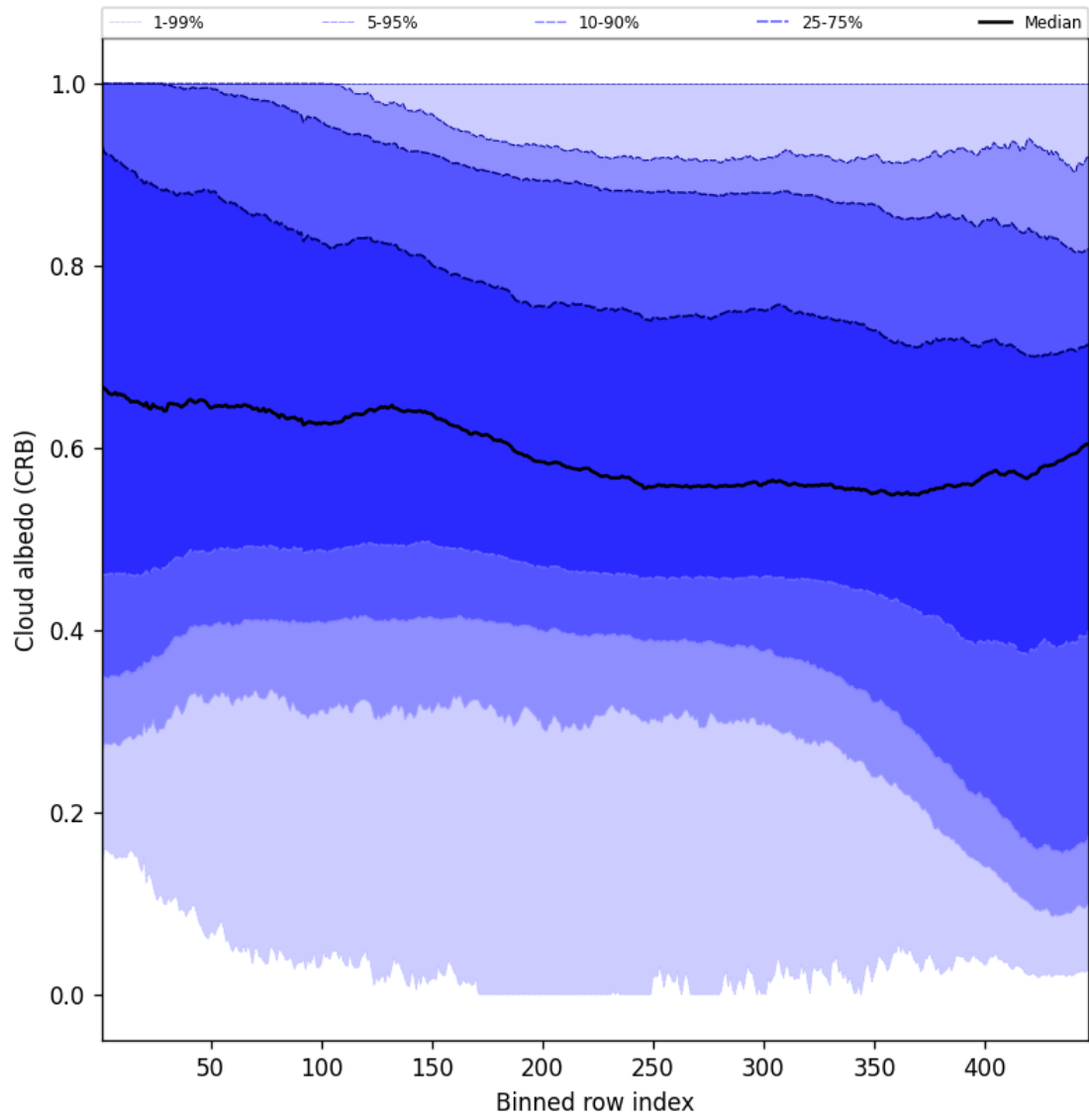
Figure 58: Along track statistics of “Cloud albedo (CRB)” for 2025-01-05 to 2025-01-05
