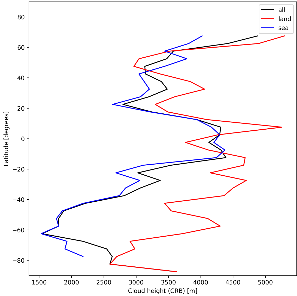
Figure 25: Zonal average of “Cloud height (CRB)” for 2025-01-05 to 2025-01-05.
