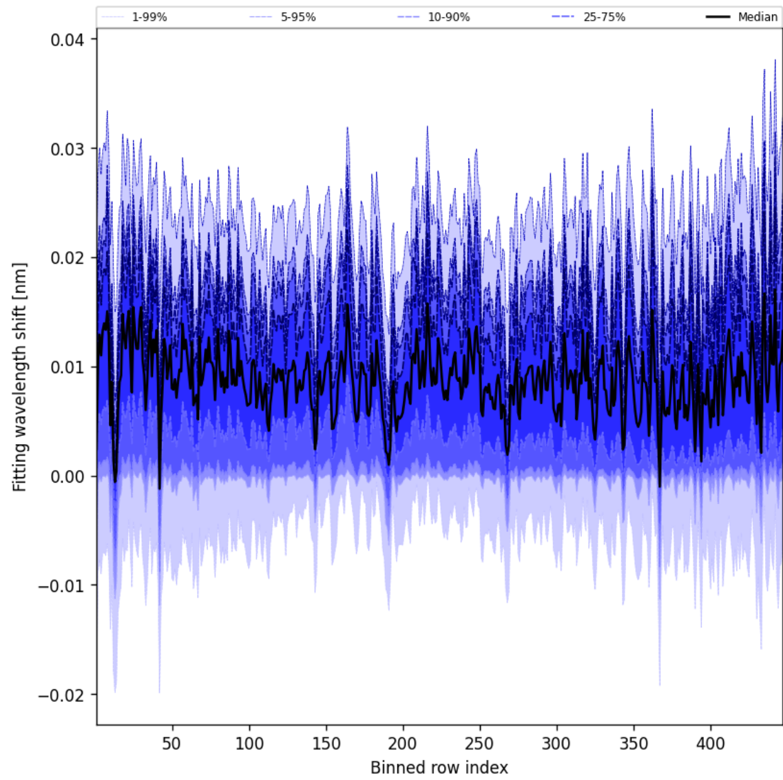
Figure 63: Along track statistics of “Fitting wavelength shift” for 2025-01-05 to 2025-01-05
