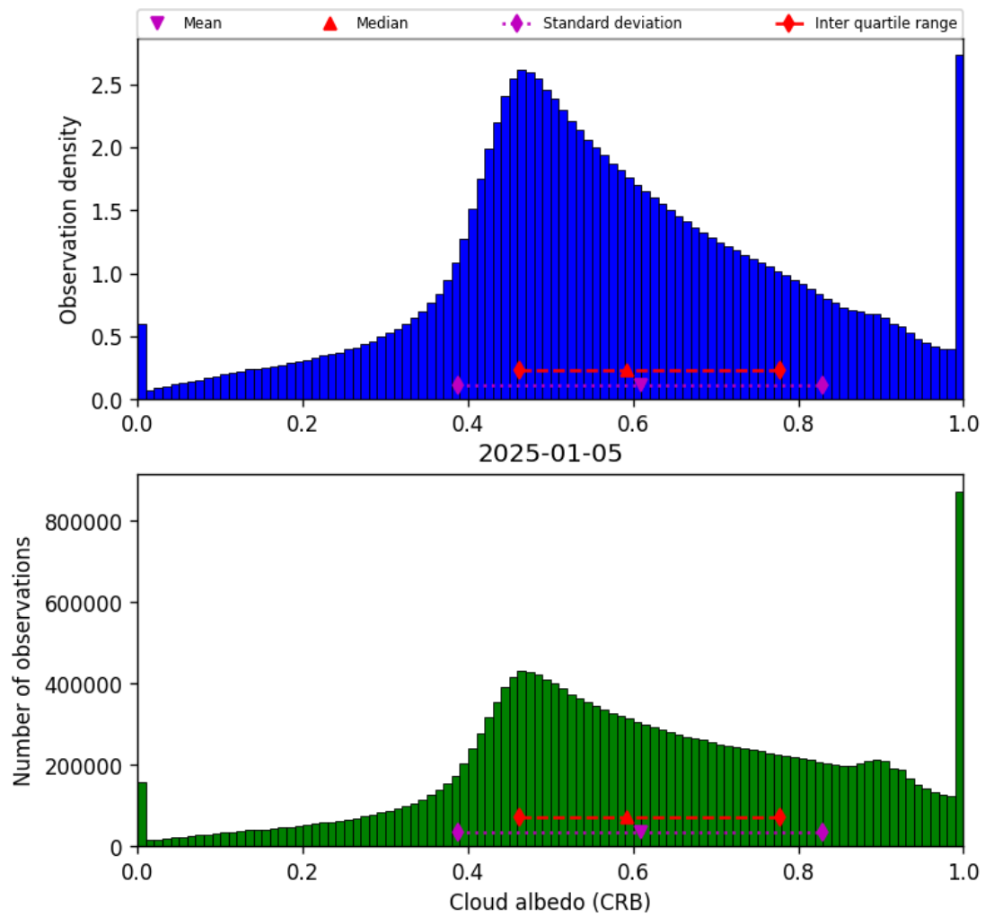
Figure 42: Histogram of “Cloud albedo (CRB)” for 2025-01-05 to 2025-01-05
