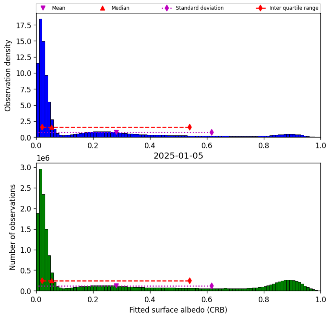
Figure 44: Histogram of “Fitted surface albedo (CRB)” for 2025-01-05 to 2025-01-05
