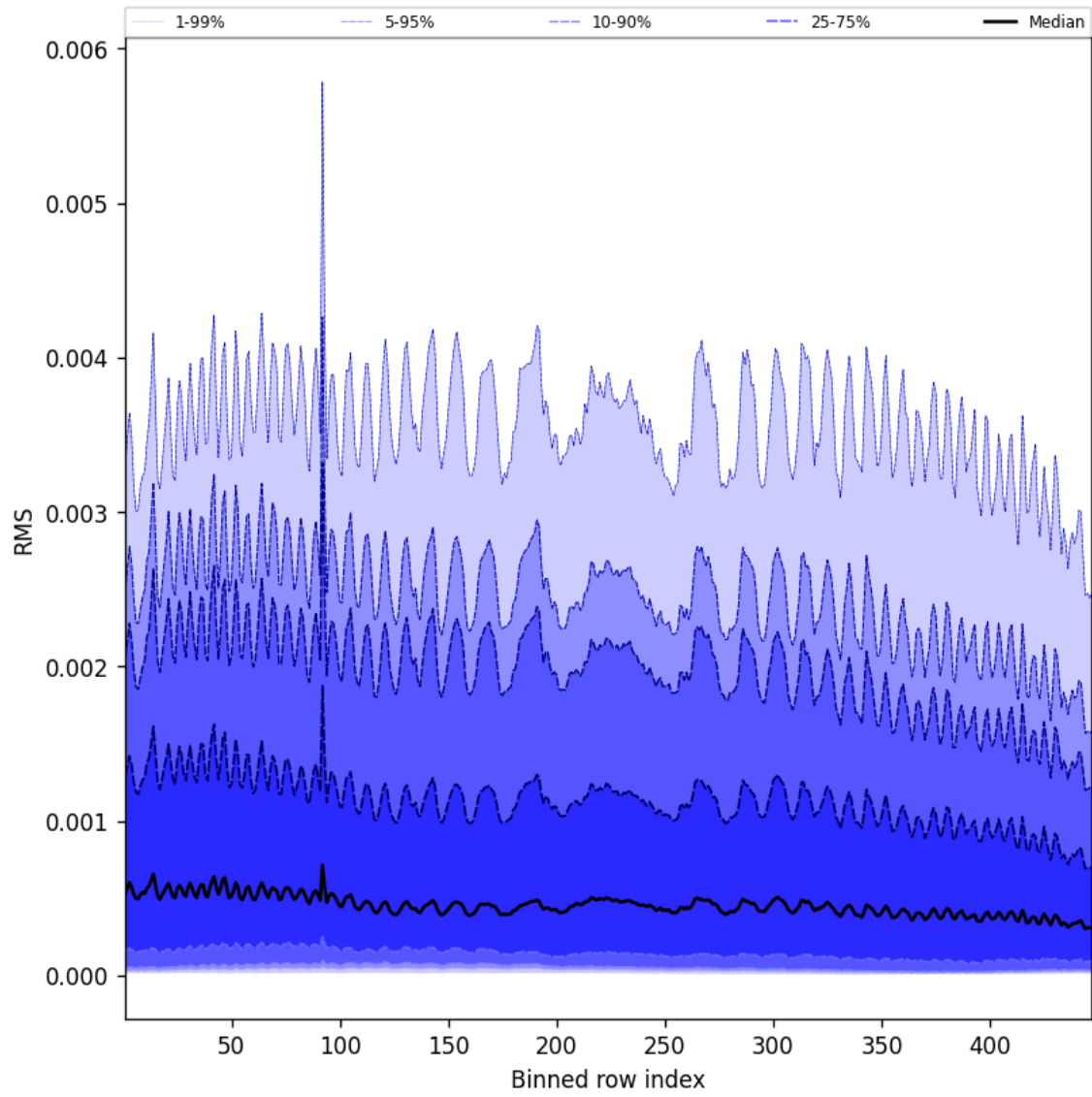
Figure 61: Along track statistics of “RMS” for 2025-01-05 to 2025-01-05
