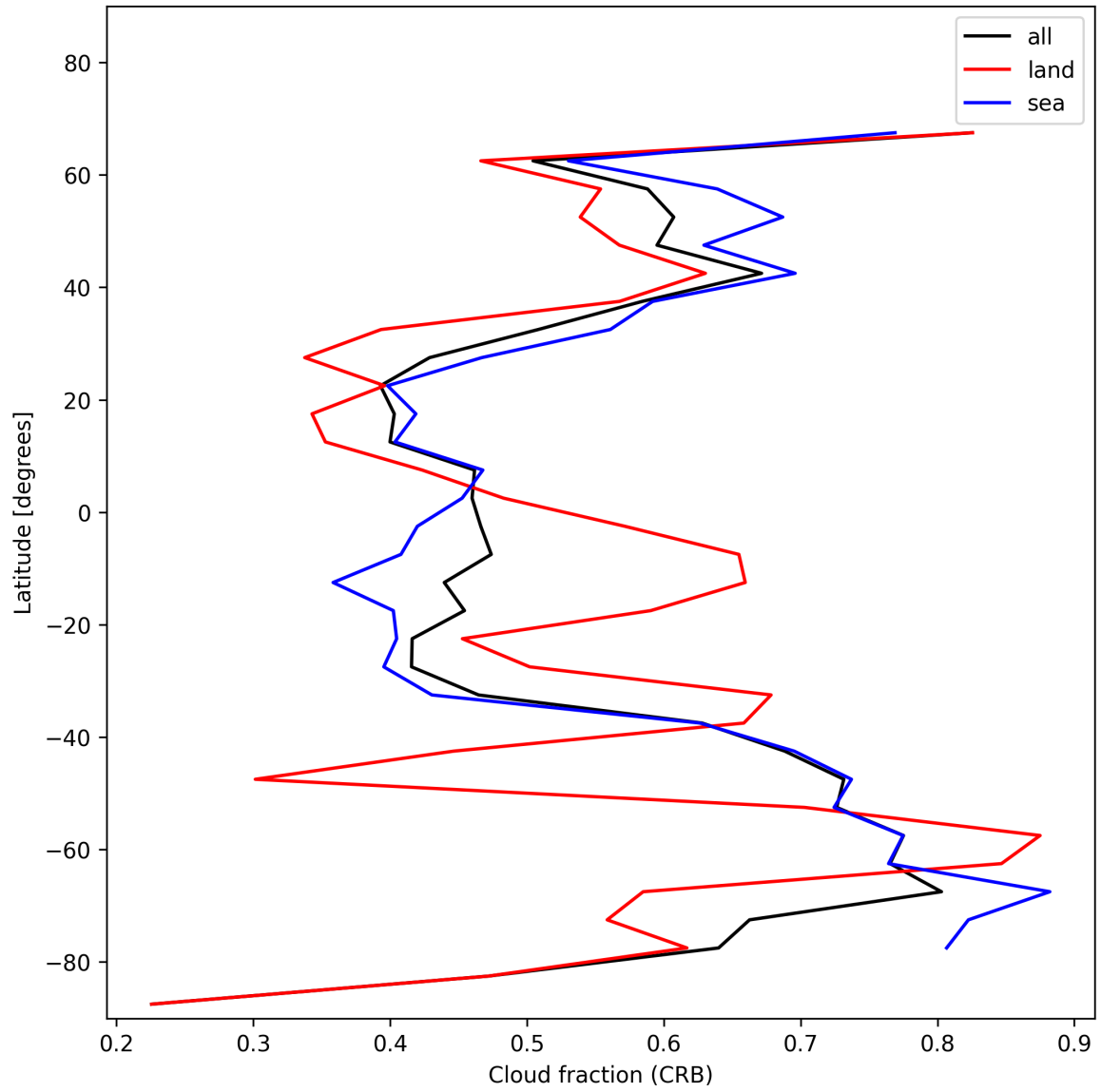
Figure 24: Zonal average of “Cloud fraction (CRB)” for 2025-01-05 to 2025-01-05.
