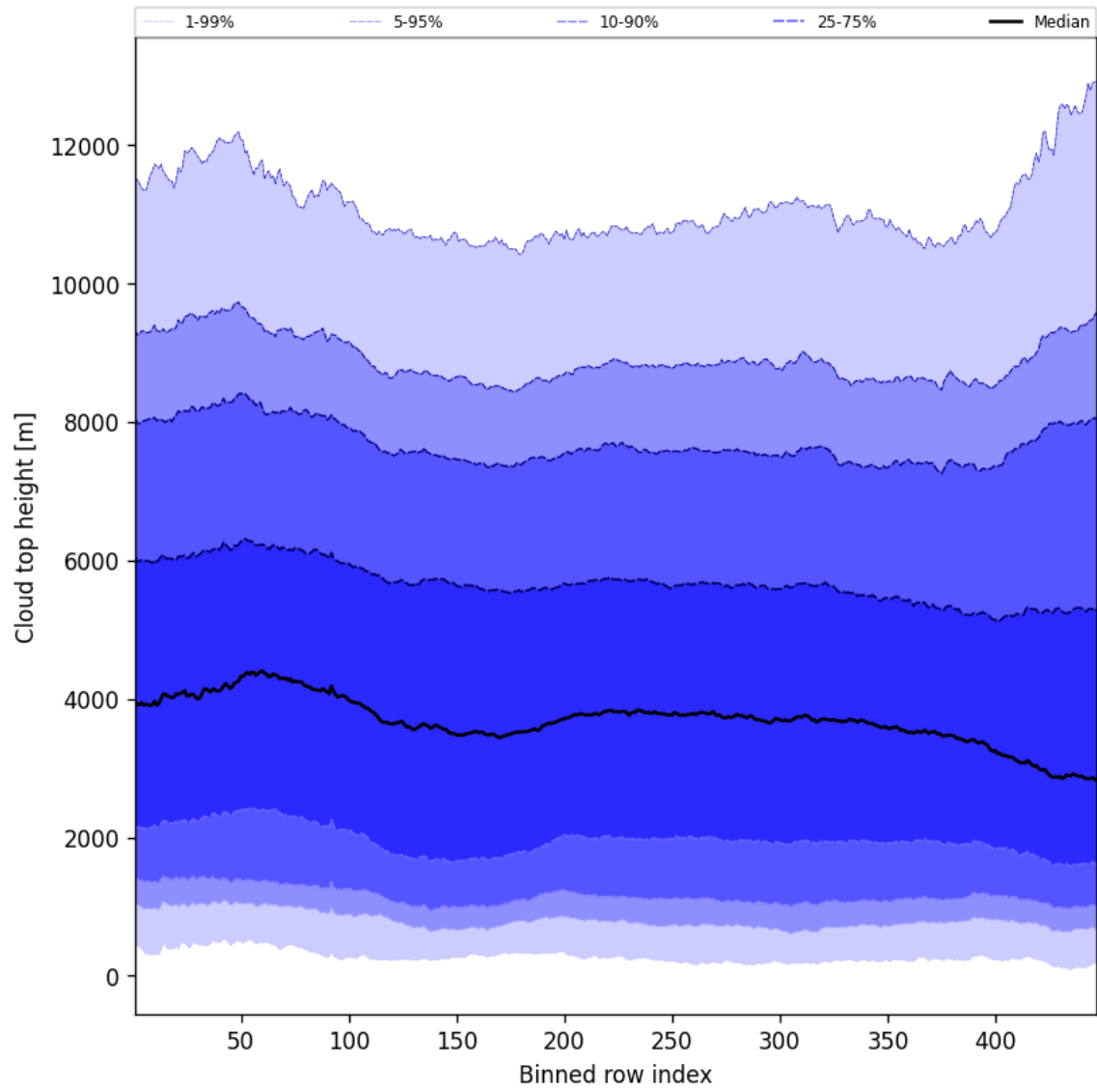
Figure 54: Along track statistics of “Cloud top height” for 2025-01-05 to 2025-01-05
