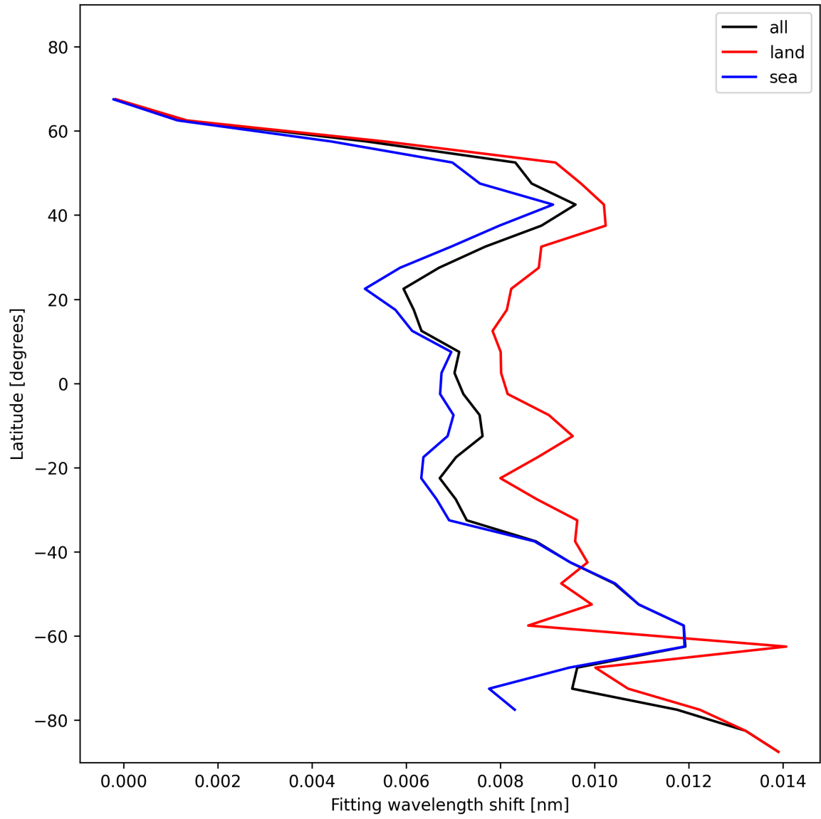
Figure 31: Zonal average of “Fitting wavelength shift” for 2025-01-05 to 2025-01-05.
