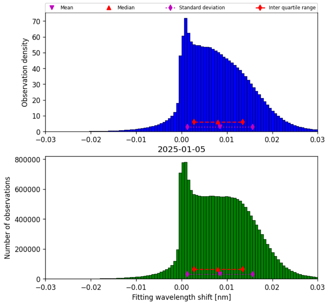
Figure 47: Histogram of “Fitting wavelength shift” for 2025-01-05 to 2025-01-05
