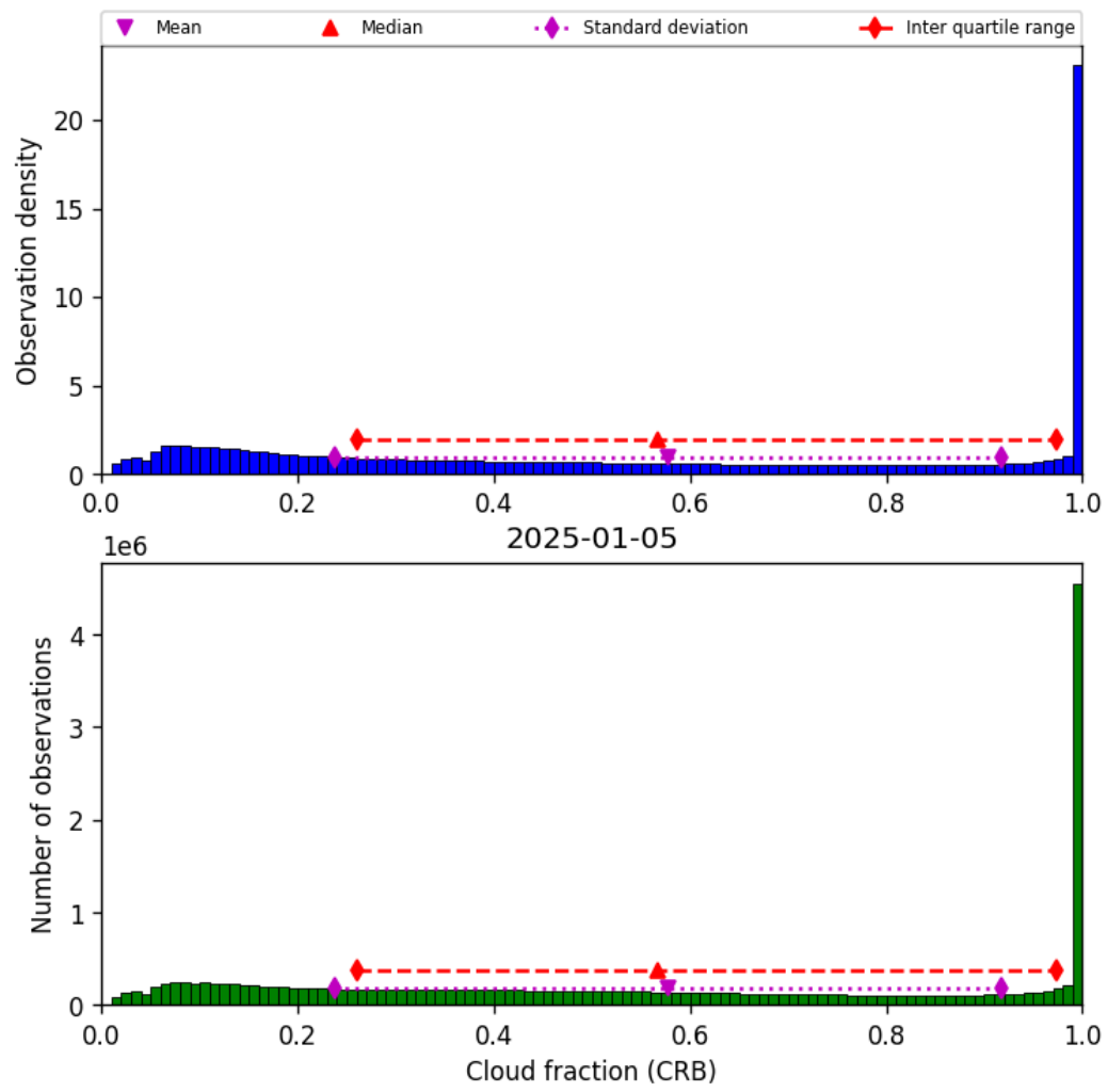
Figure 40: Histogram of "Cloud fraction (CRB)" for 2025-01-05 to 2025-01-05
