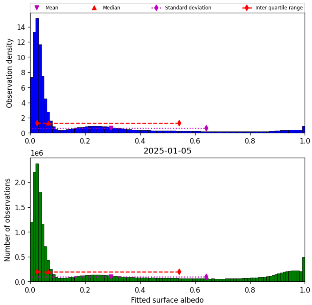
Figure 43: Histogram of “Fitted surface albedo” for 2025-01-05 to 2025-01-05
