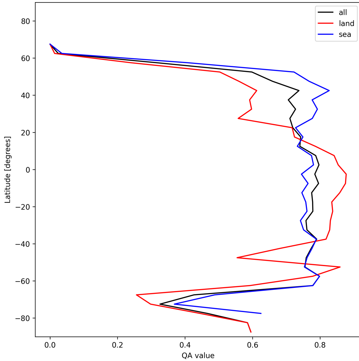
Figure 20: Zonal average of “QA value” for 2025-01-05 to 2025-01-05.
