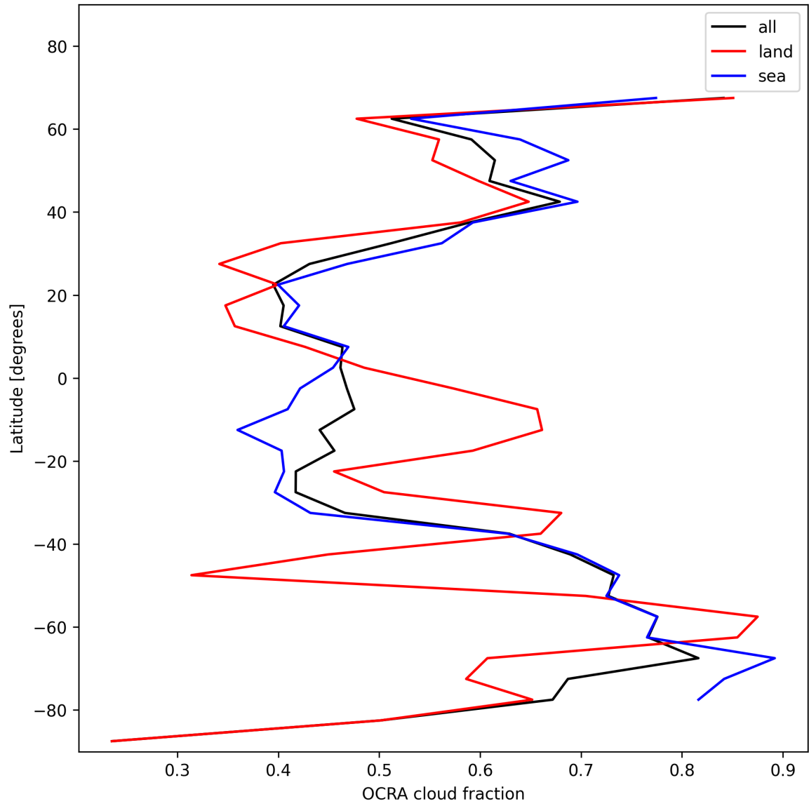
Figure 32: Zonal average of “OCRA cloud fraction” for 2025-01-05 to 2025-01-05.
