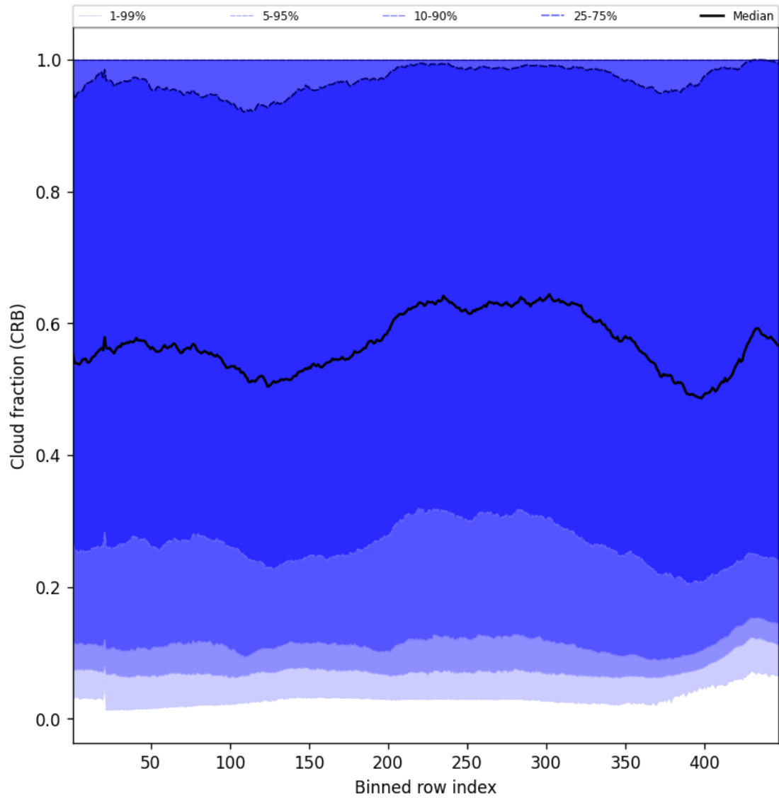
Figure 56: Along track statistics of “Cloud fraction (CRB)” for 2025-01-05 to 2025-01-05
