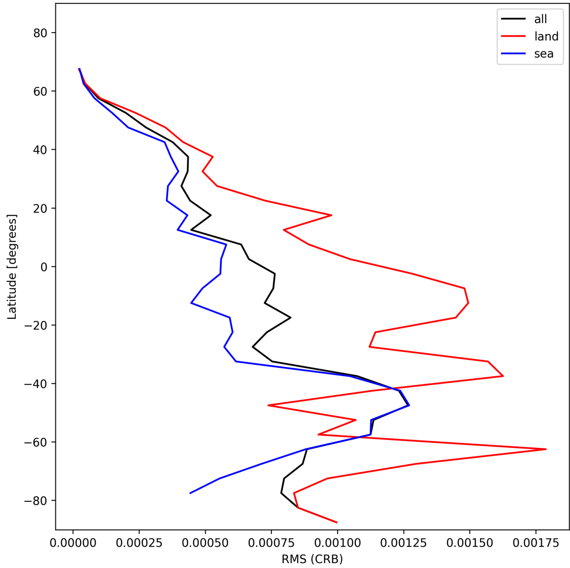
Figure 30: Zonal average of “RMS (CRB)” for 2025-01-05 to 2025-01-05.
