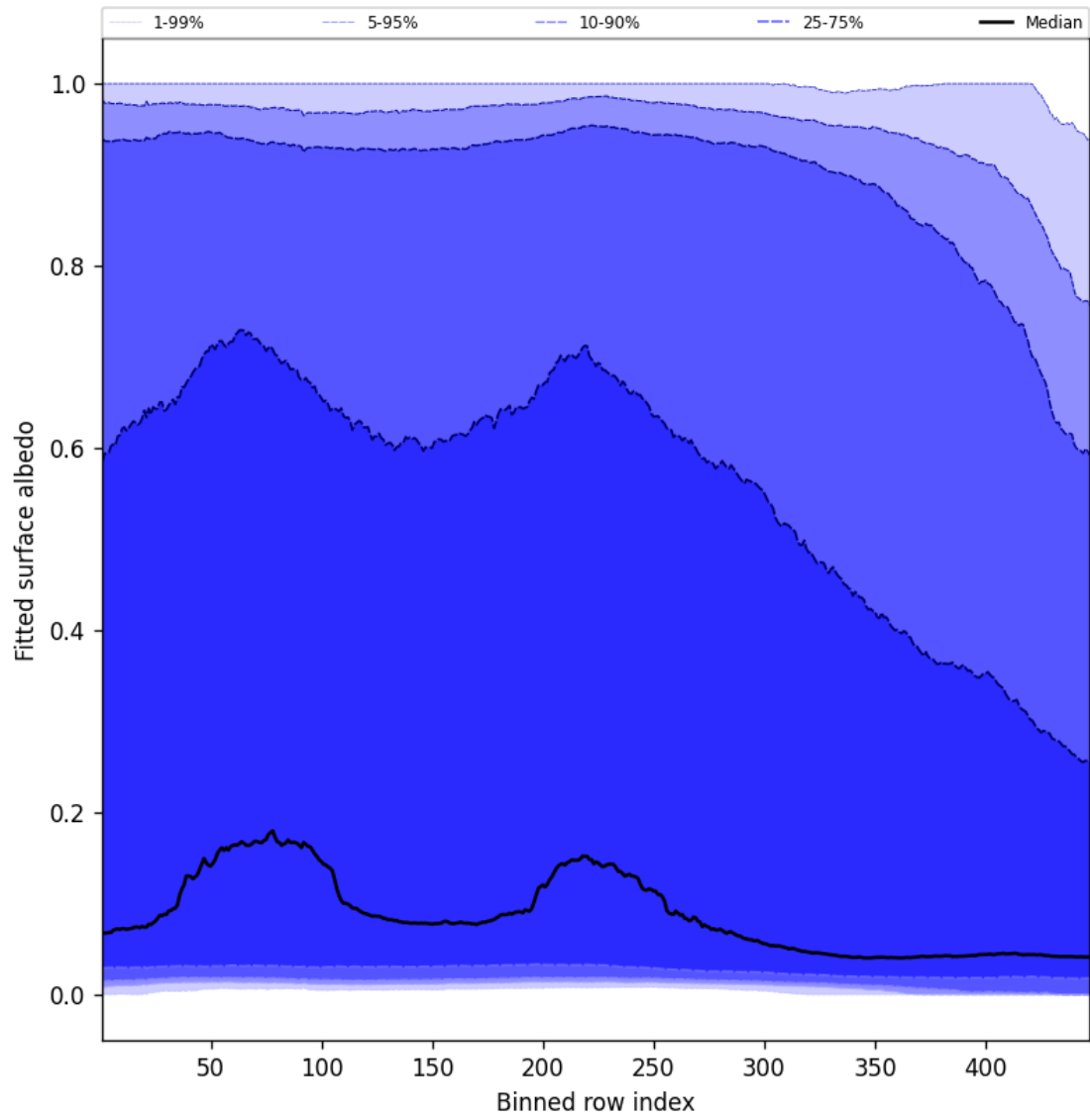
Figure 59: Along track statistics of “Fitted surface albedo” for 2025-01-05 to 2025-01-05
