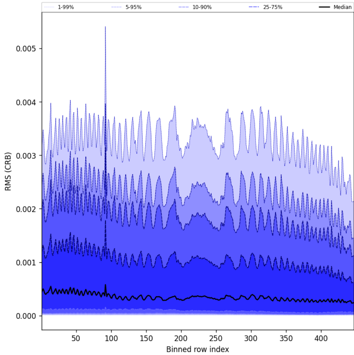
Figure 62: Along track statistics of “RMS (CRB)” for 2025-01-05 to 2025-01-05
