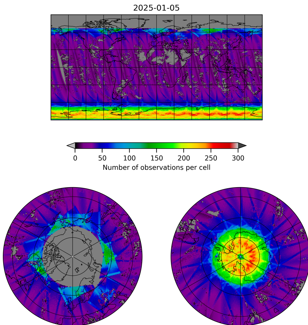
Figure 19: Map of the number of observations for 2025-01-05 to 2025-01-05
