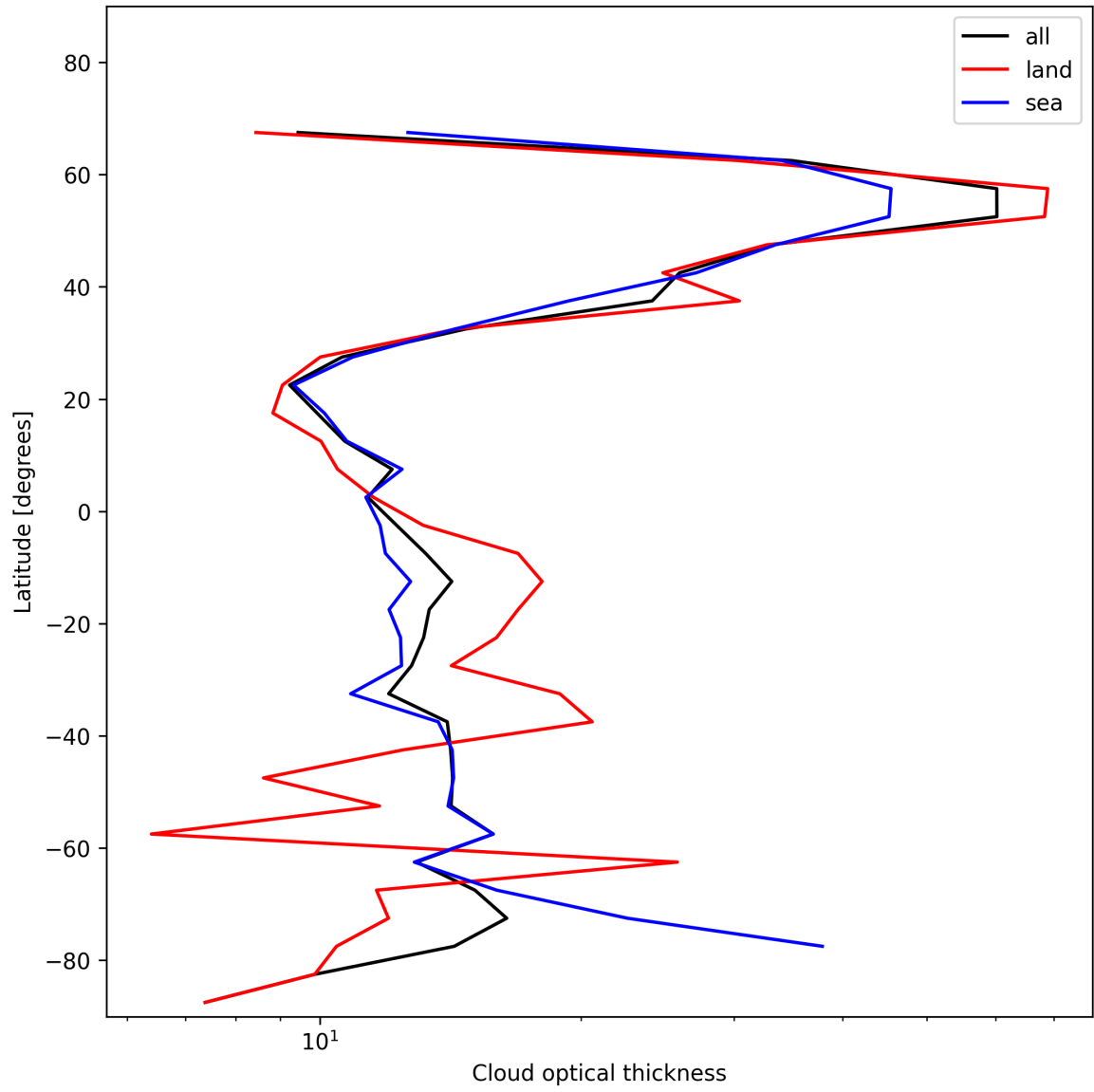
Figure 23: Zonal average of “Cloud optical thickness” for 2025-01-05 to 2025-01-05.
