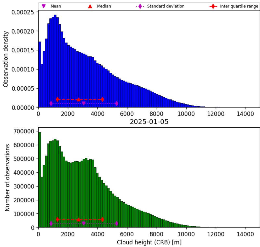
Figure 41: Histogram of “Cloud height (CRB)” for 2025-01-05 to 2025-01-05
