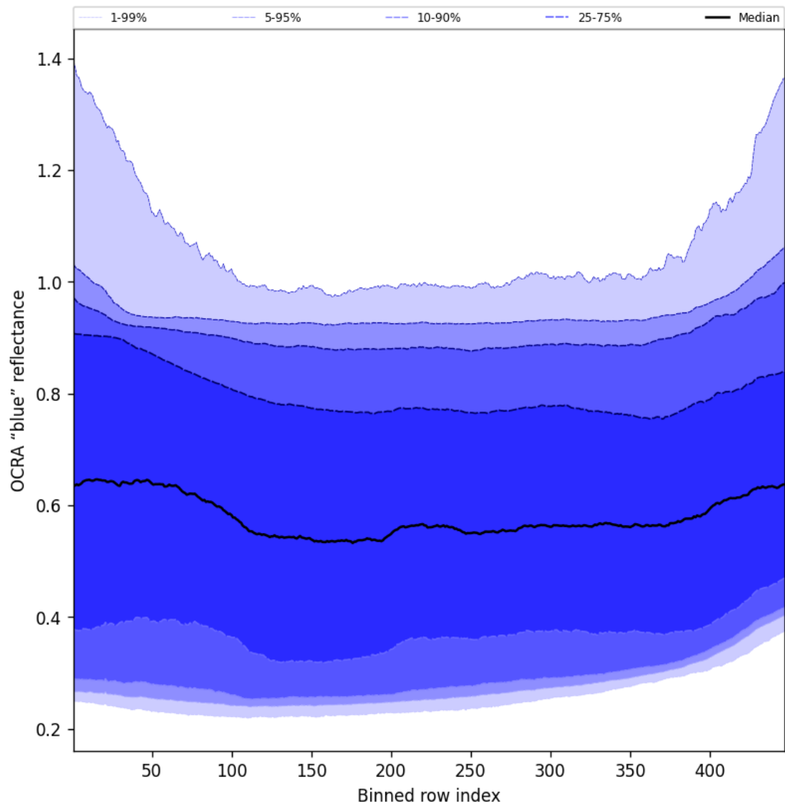
Figure 65: Along track statistics of “OCRA “blue” reflectance” for 2025-01-05 to 2025-01-05
