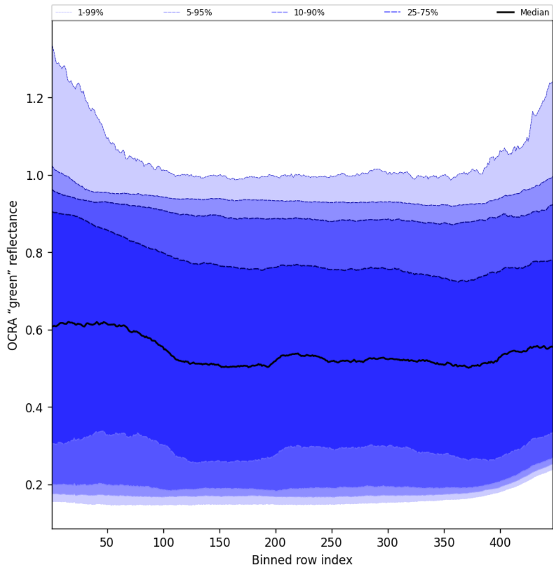
Figure 66: Along track statistics of "OCRA "green" reflectance" for 2025-01-05 to 2025-01-05
