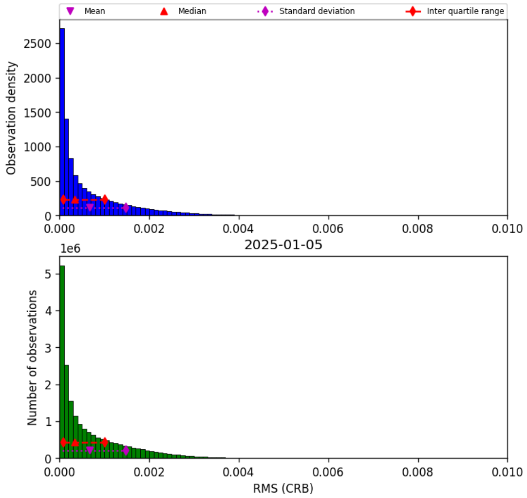
Figure 46: Histogram of “RMS (CRB)” for 2025-01-05 to 2025-01-05
