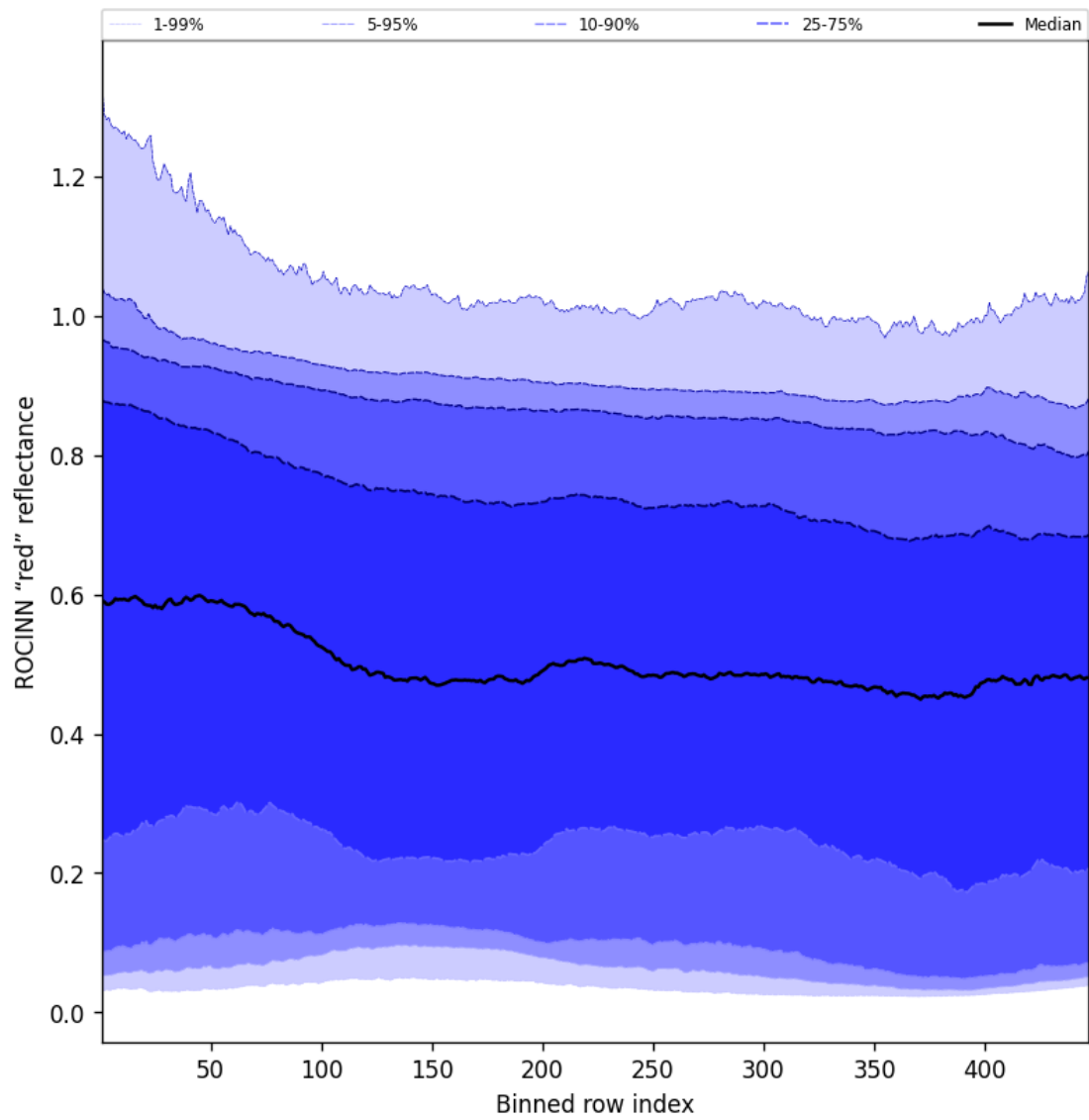
Figure 67: Along track statistics of “ROCINN “red” reflectance” for 2025-01-05 to 2025-01-05
