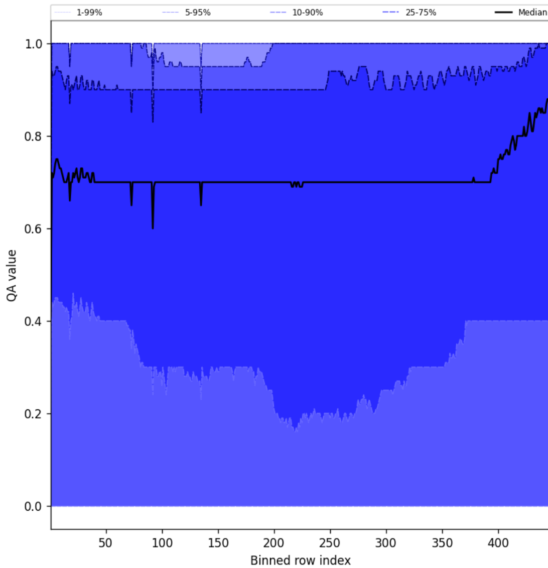
Figure 52: Along track statistics of “QA value” for 2025-01-05 to 2025-01-05
