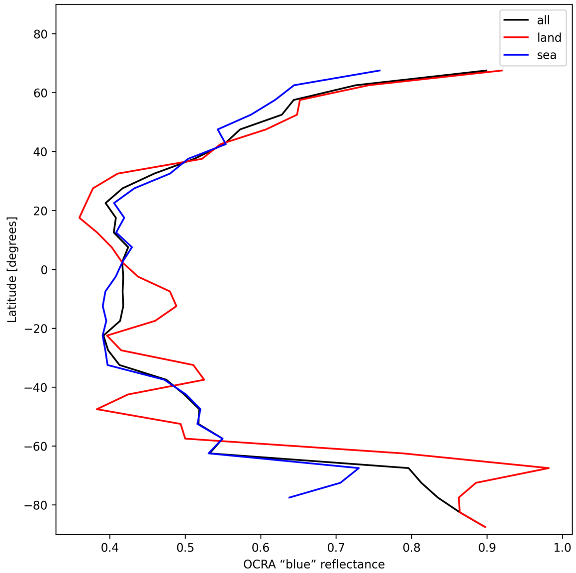
Figure 33: Zonal average of “OCRA “blue” reflectance” for 2025-01-05 to 2025-01-05.
