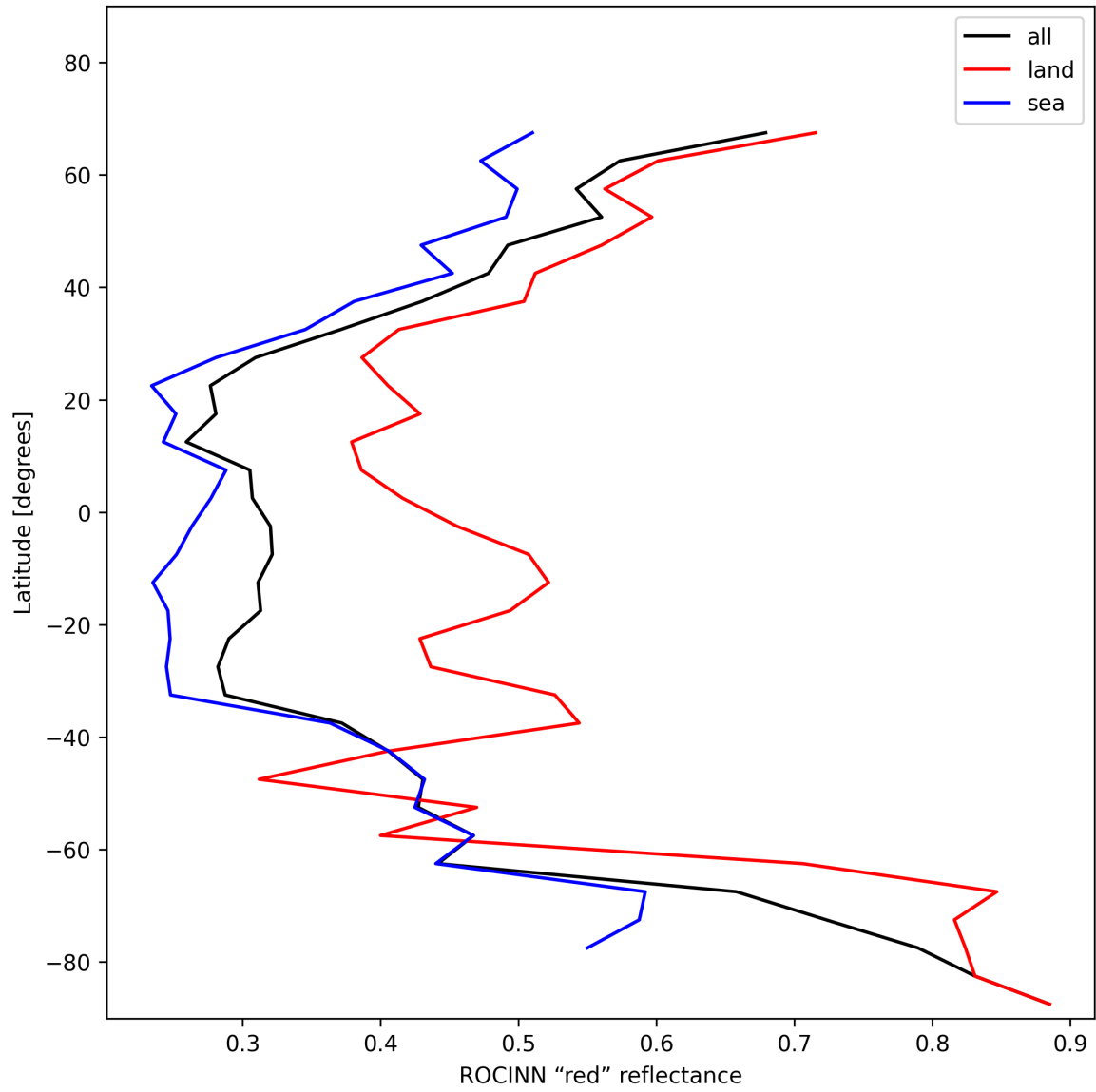
Figure 35: Zonal average of "ROCINN "red" reflectance" for 2025-01-05 to 2025-01-05.
