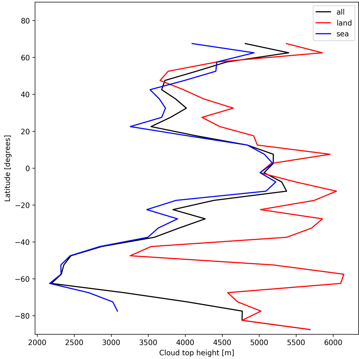
Figure 22: Zonal average of “Cloud top height” for 2025-01-05 to 2025-01-05.
