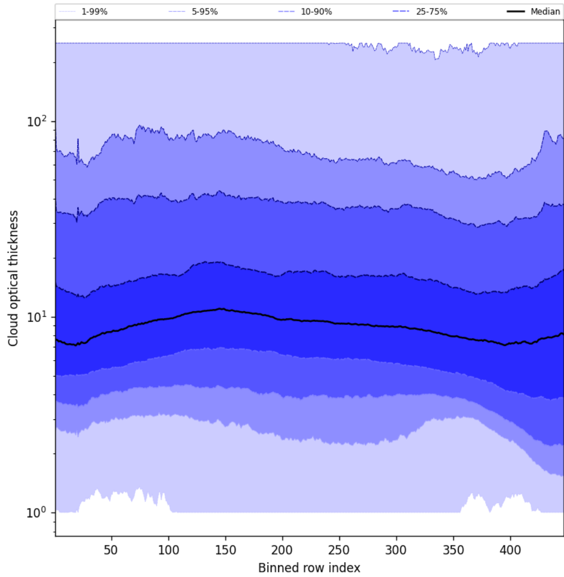
Figure 55: Along track statistics of “Cloud optical thickness” for 2025-01-05 to 2025-01-05
