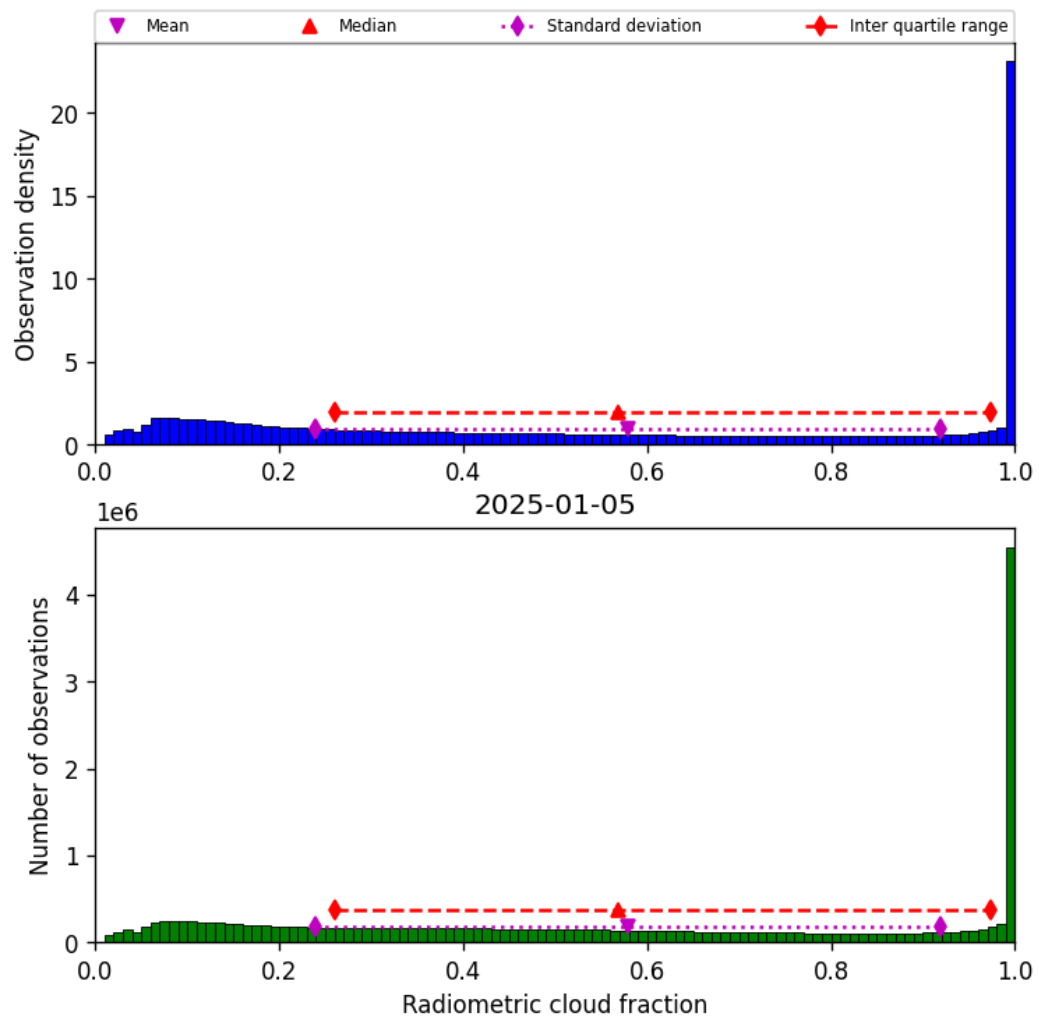
Figure 37: Histogram of "Radiometric cloud fraction" for 2025-01-05 to 2025-01-05
