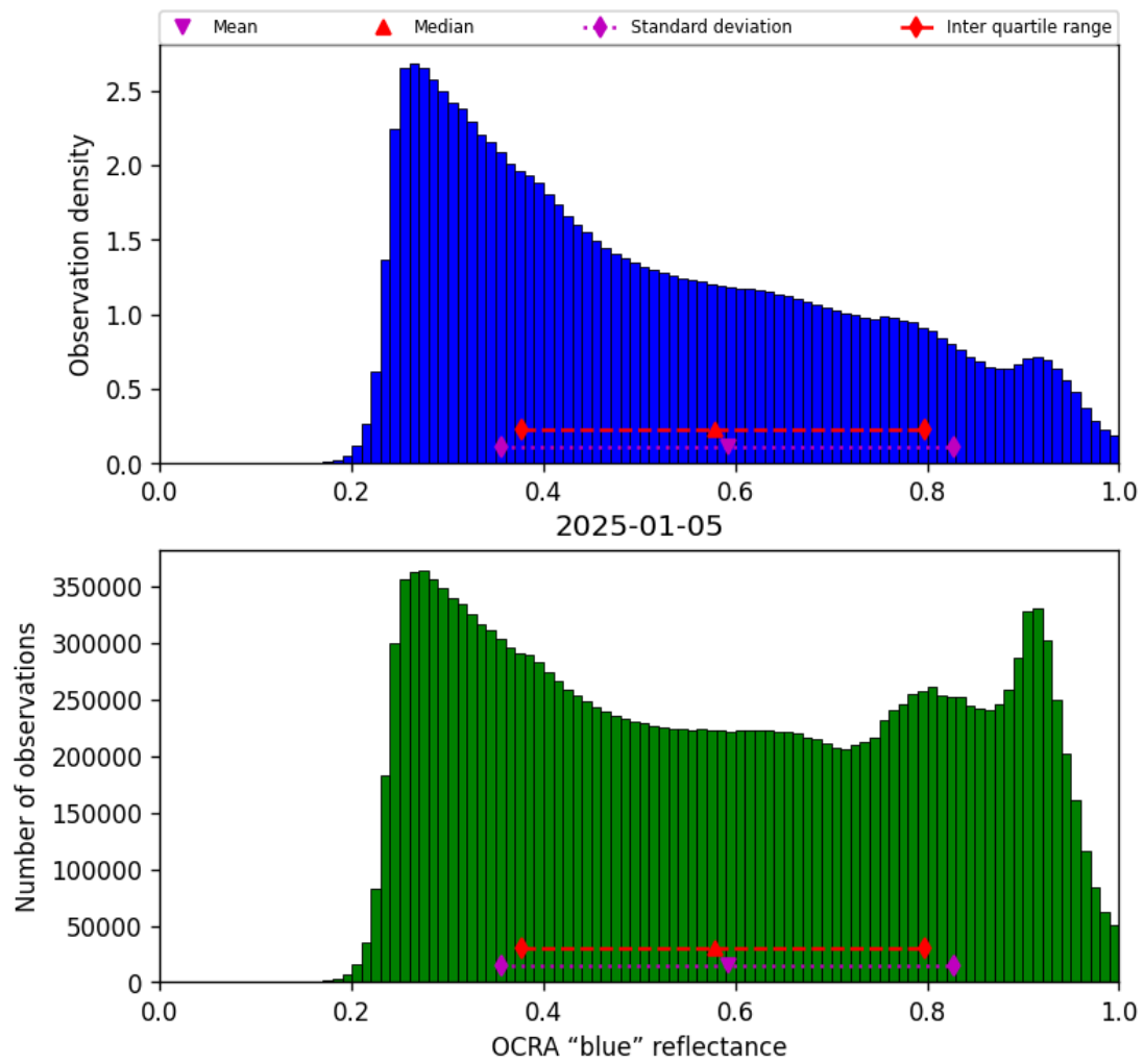
Figure 49: Histogram of “OCRA “blue” reflectance” for 2025-01-05 to 2025-01-05
