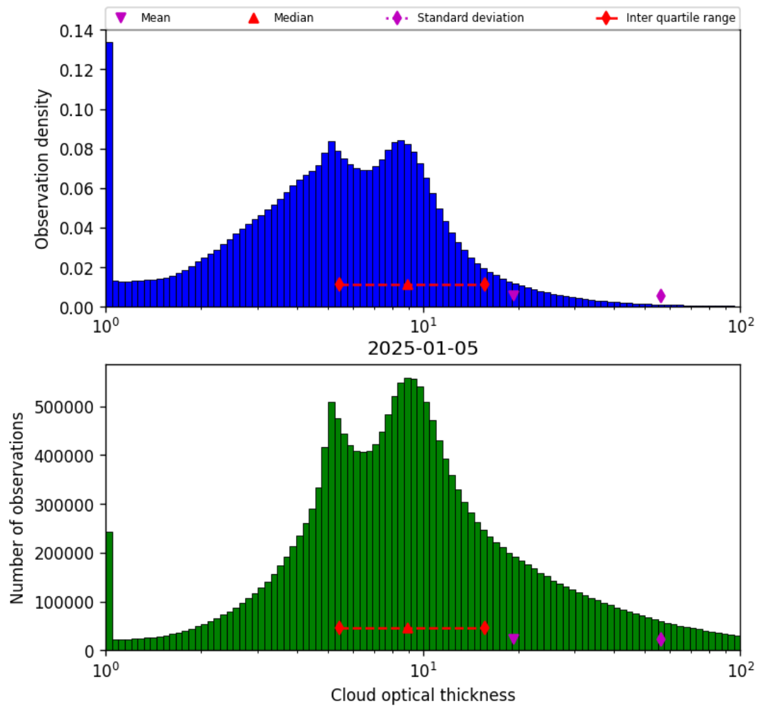
Figure 39: Histogram of “Cloud optical thickness” for 2025-01-05 to 2025-01-05
