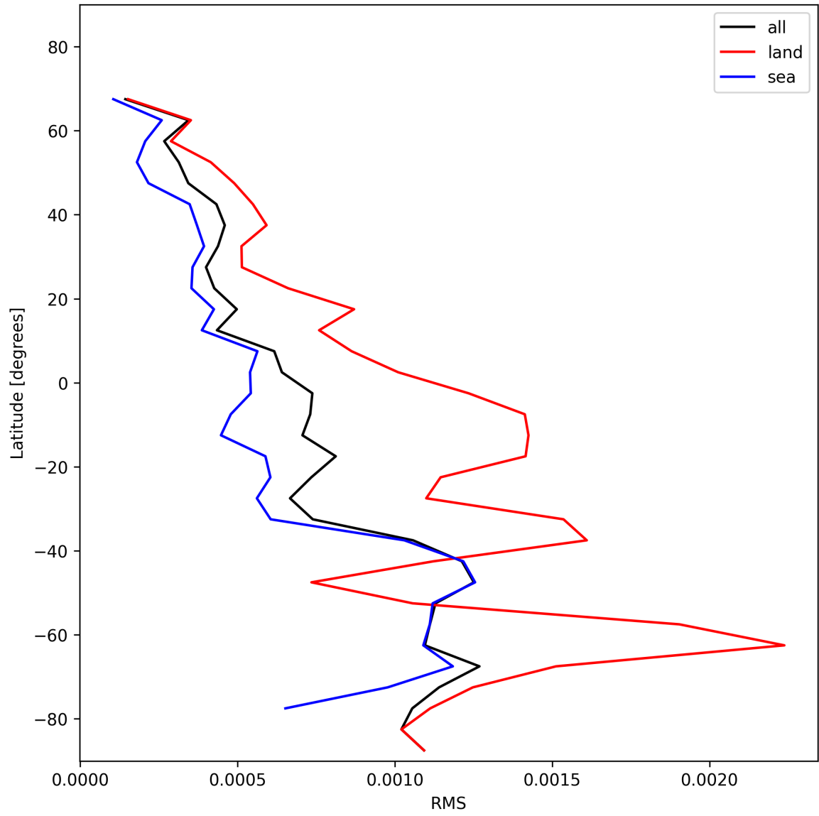
Figure 29: Zonal average of “RMS” for 2025-01-05 to 2025-01-05.
