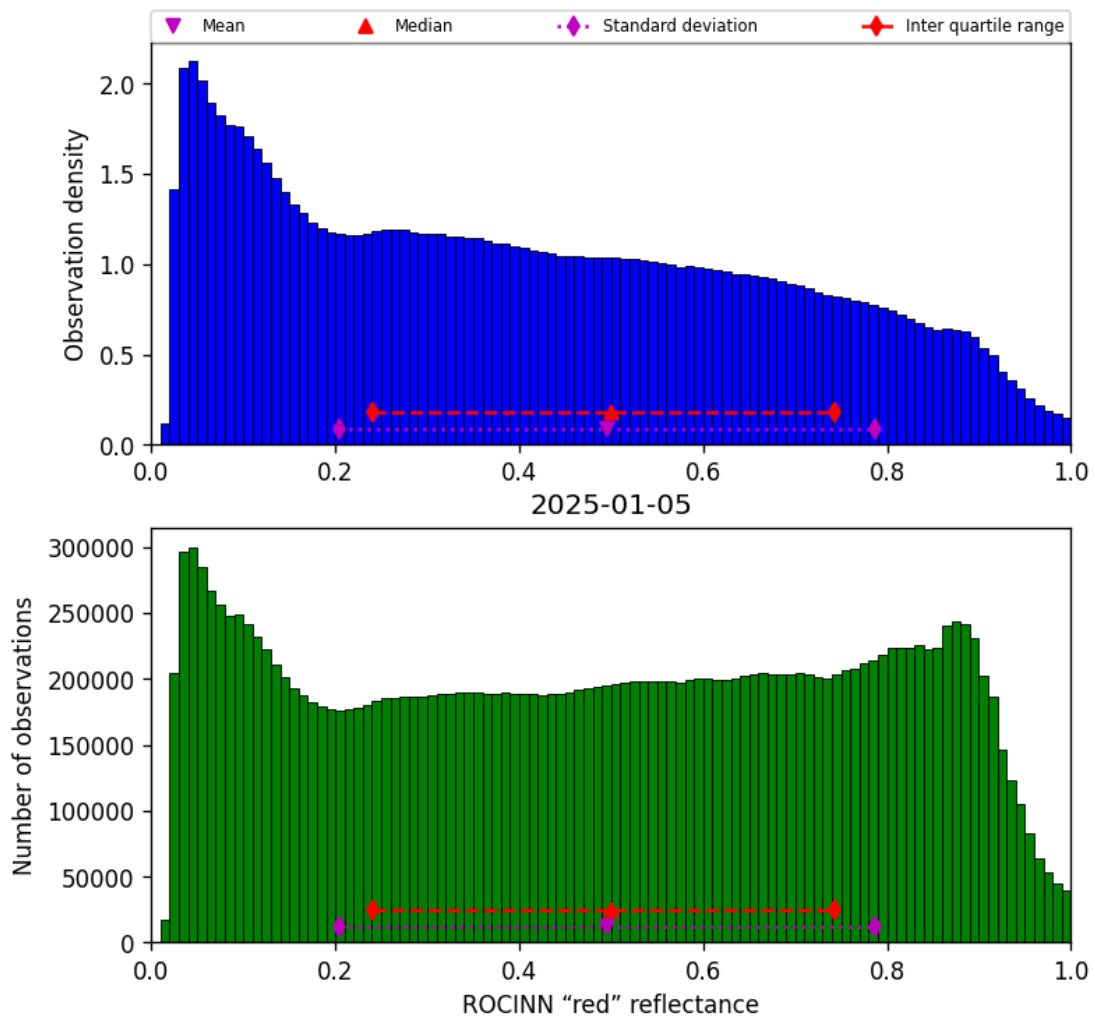
Figure 51: Histogram of “ROCINN “red” reflectance” for 2025-01-05 to 2025-01-05
