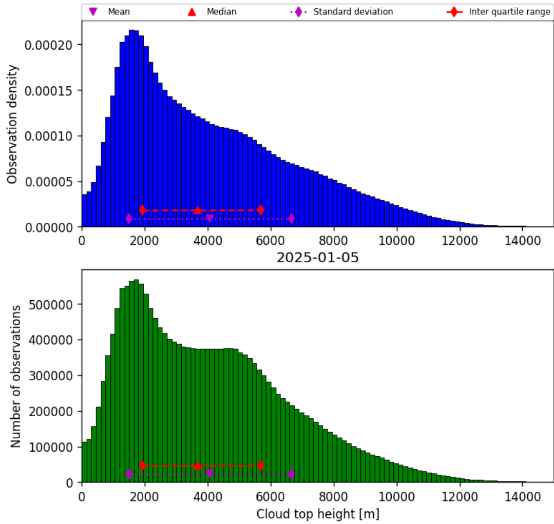
Figure 38: Histogram of “Cloud top height” for 2025-01-05 to 2025-01-05
