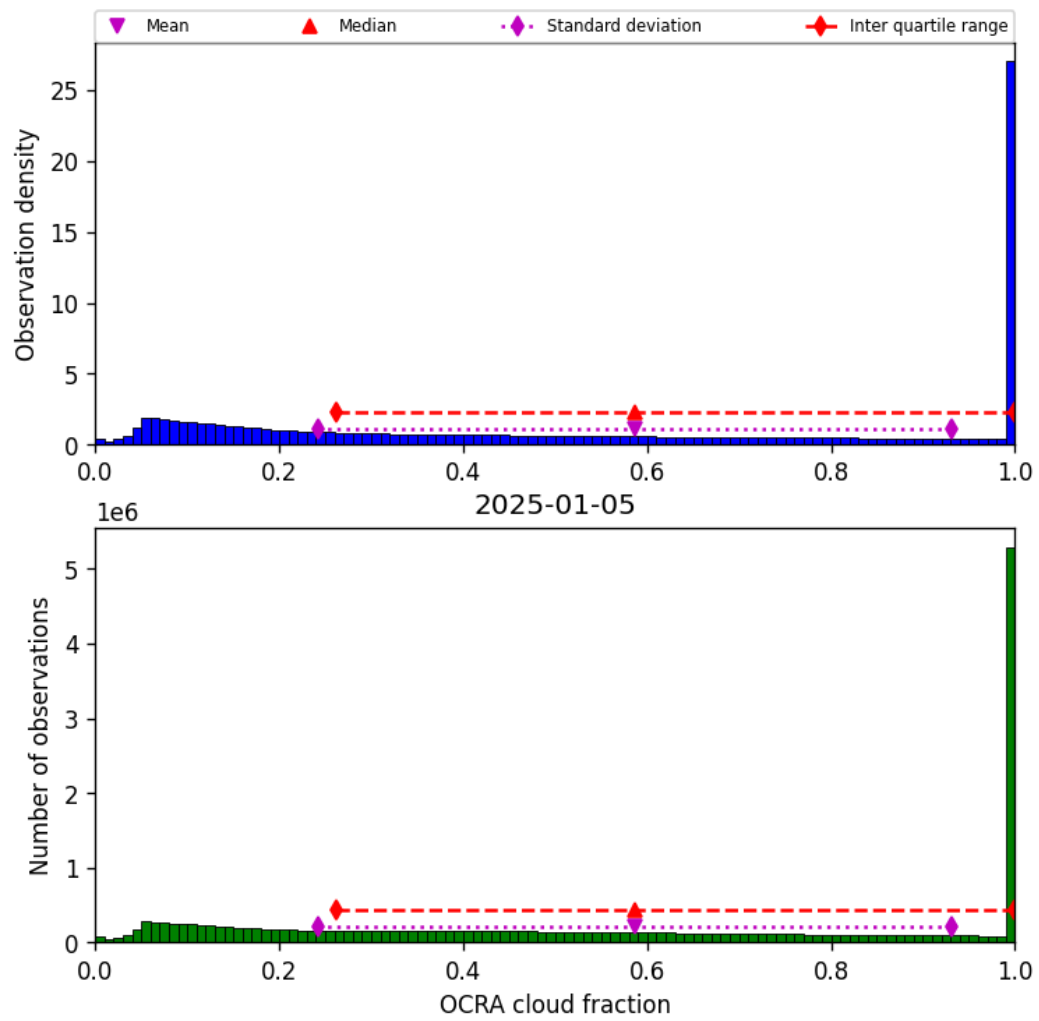
Figure 48: Histogram of “OCRA cloud fraction” for 2025-01-05 to 2025-01-05
