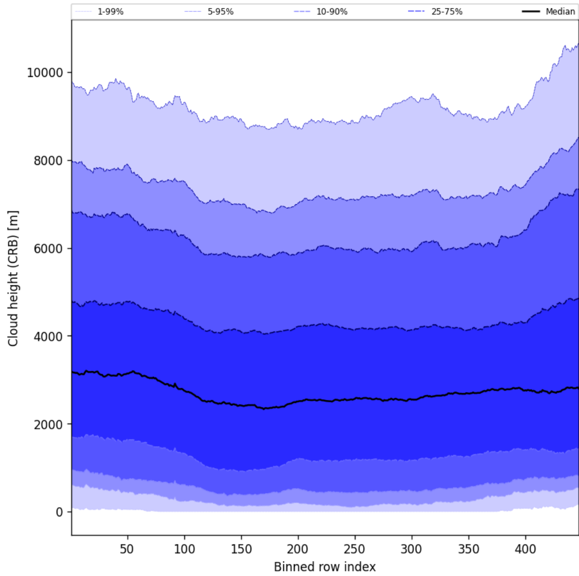
Figure 57: Along track statistics of “Cloud height (CRB)” for 2025-01-05 to 2025-01-05
