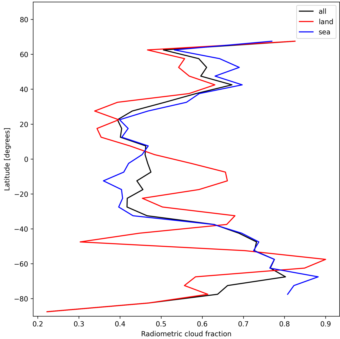
Figure 21: Zonal average of “Radiometric cloud fraction” for 2025-01-05 to 2025-01-05.
