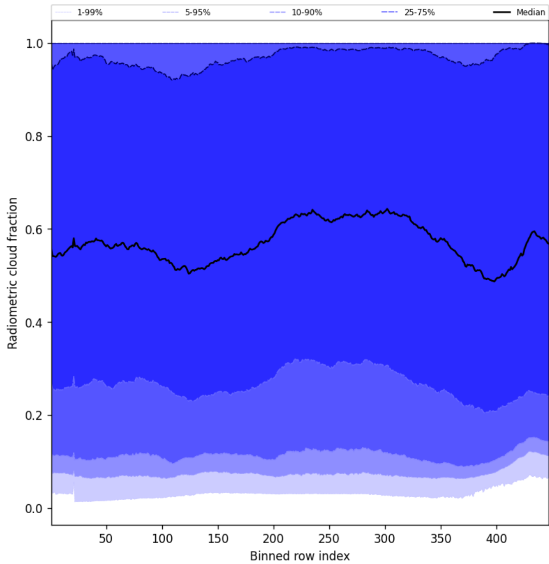
Figure 53: Along track statistics of “Radiometric cloud fraction” for 2025-01-05 to 2025-01-05
