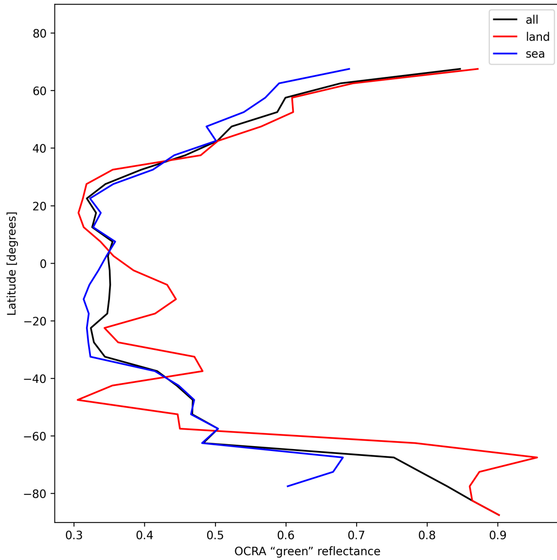
Figure 34: Zonal average of “OCRA “green” reflectance” for 2025-01-05 to 2025-01-05.
