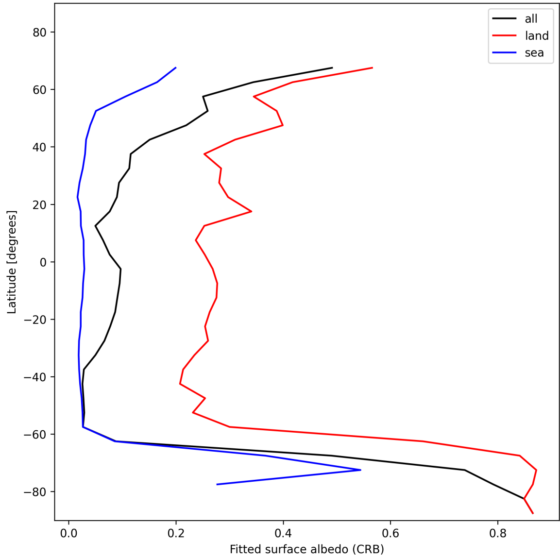
Figure 28: Zonal average of “Fitted surface albedo (CRB)” for 2025-01-05 to 2025-01-05.
