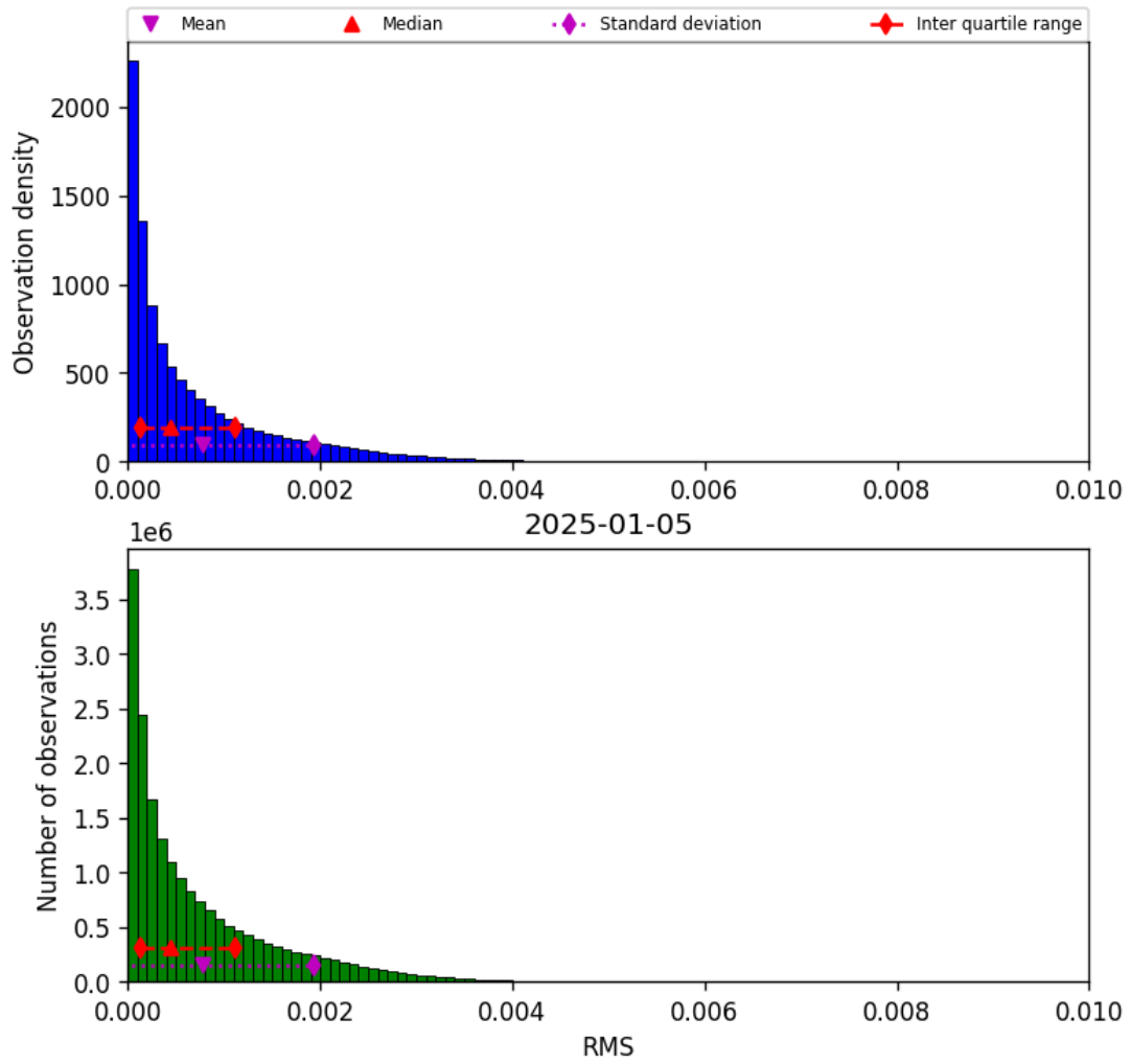
Figure 45: Histogram of “RMS” for 2025-01-05 to 2025-01-05
