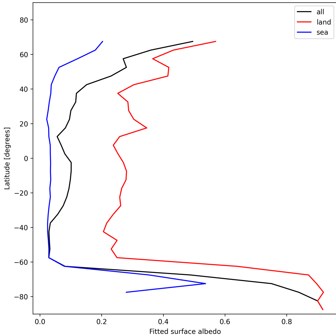
Figure 27: Zonal average of “Fitted surface albedo” for 2025-01-05 to 2025-01-05.
