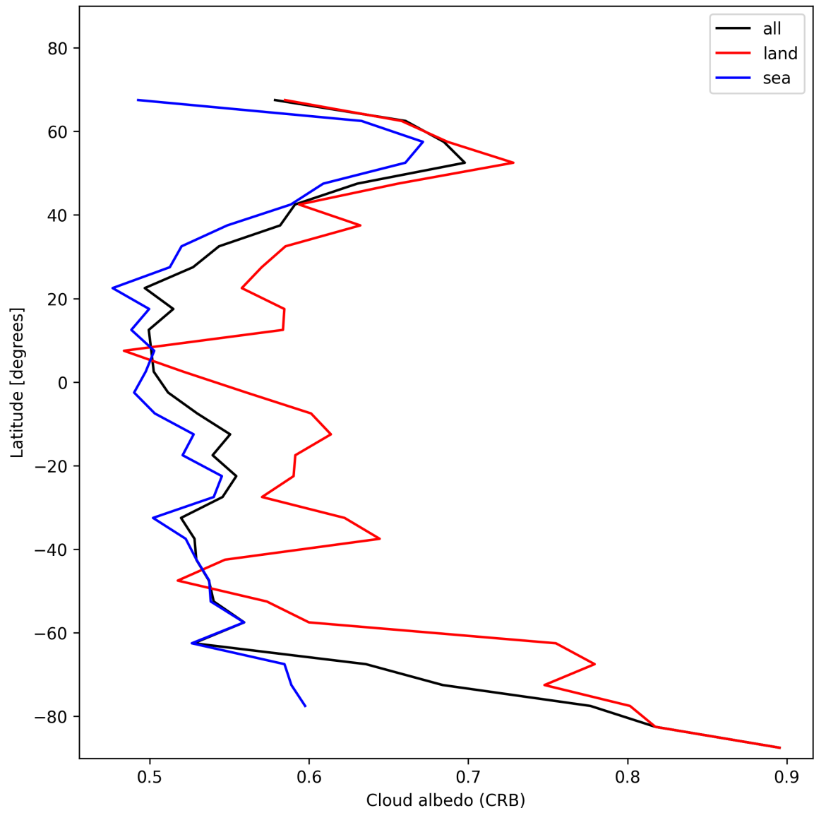
Figure 26: Zonal average of “Cloud albedo (CRB)” for 2025-01-05 to 2025-01-05.
