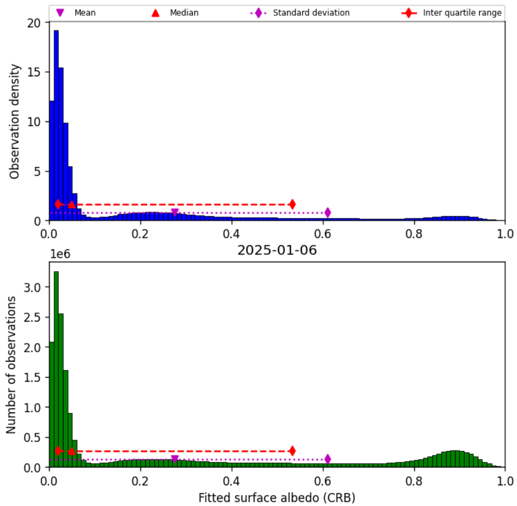
Figure 44: Histogram of “Fitted surface albedo (CRB)” for 2025-01-06 to 2025-01-07
