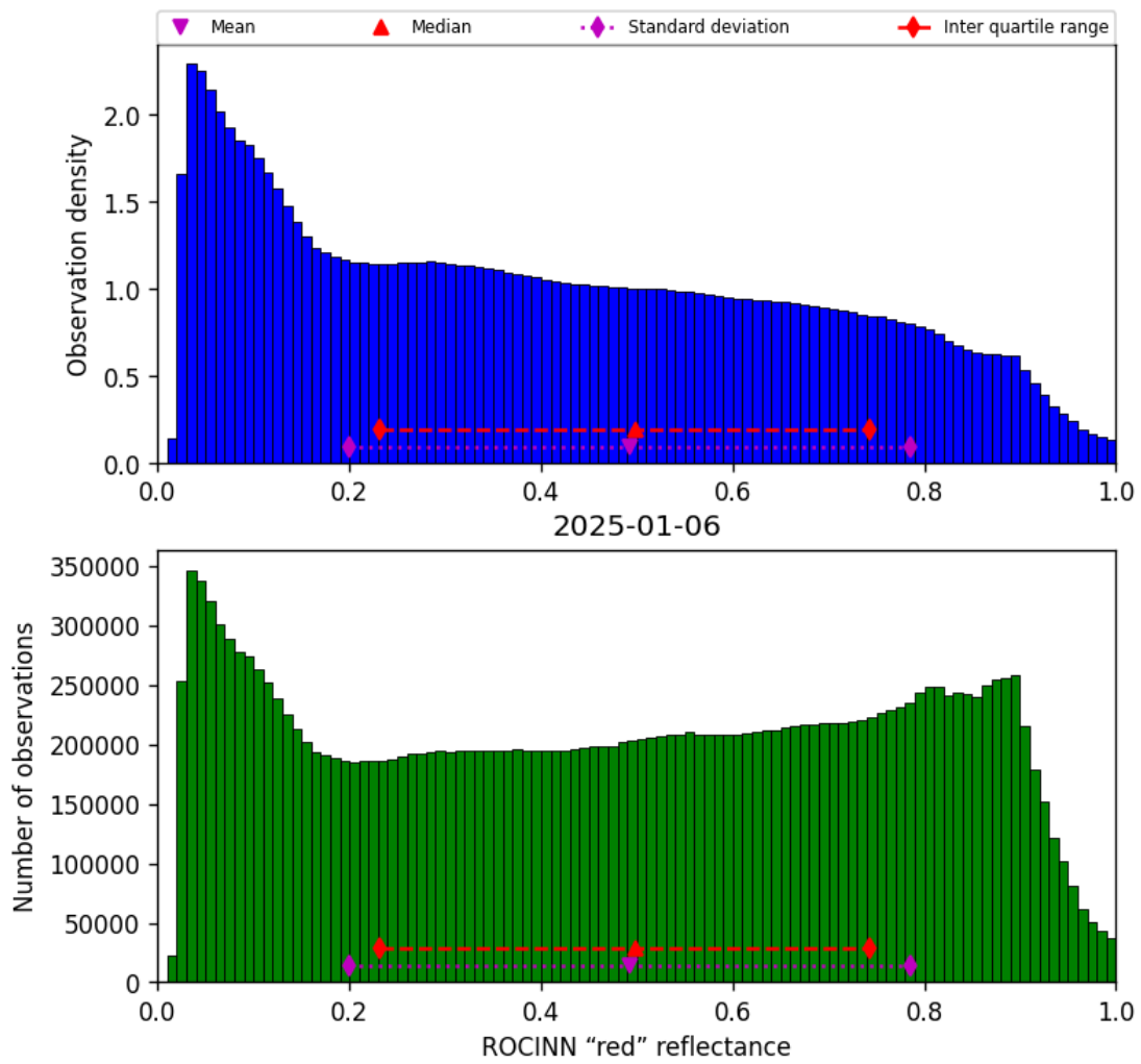
Figure 51: Histogram of “ROCINN “red” reflectance” for 2025-01-06 to 2025-01-07
