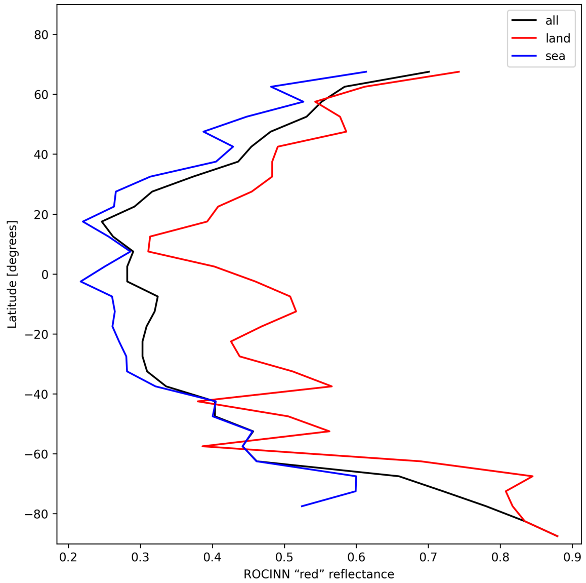
Figure 35: Zonal average of “ROCINN “red” reflectance” for 2025-01-06 to 2025-01-07.
