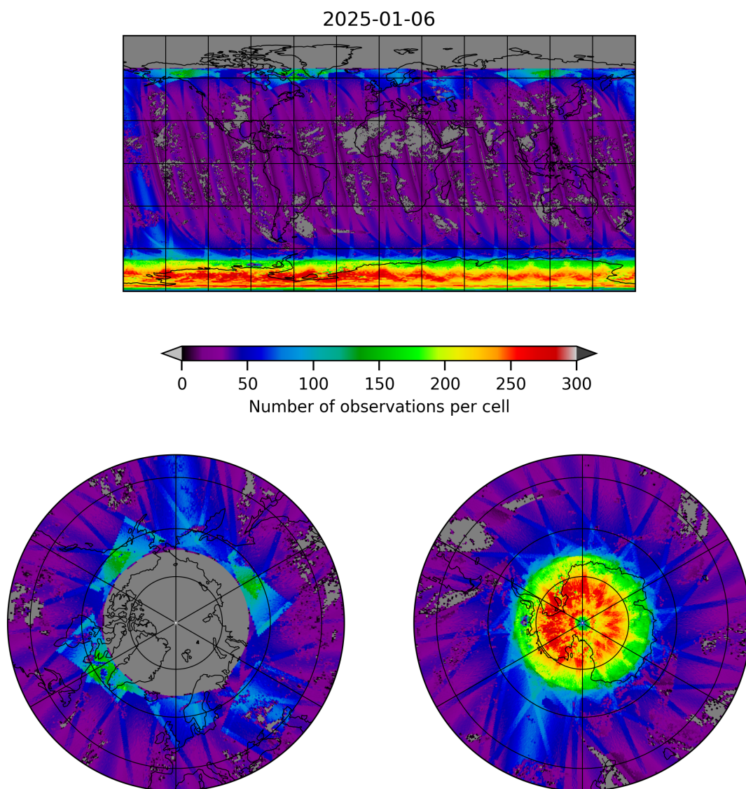
Figure 19: Map of the number of observations for 2025-01-06 to 2025-01-07
