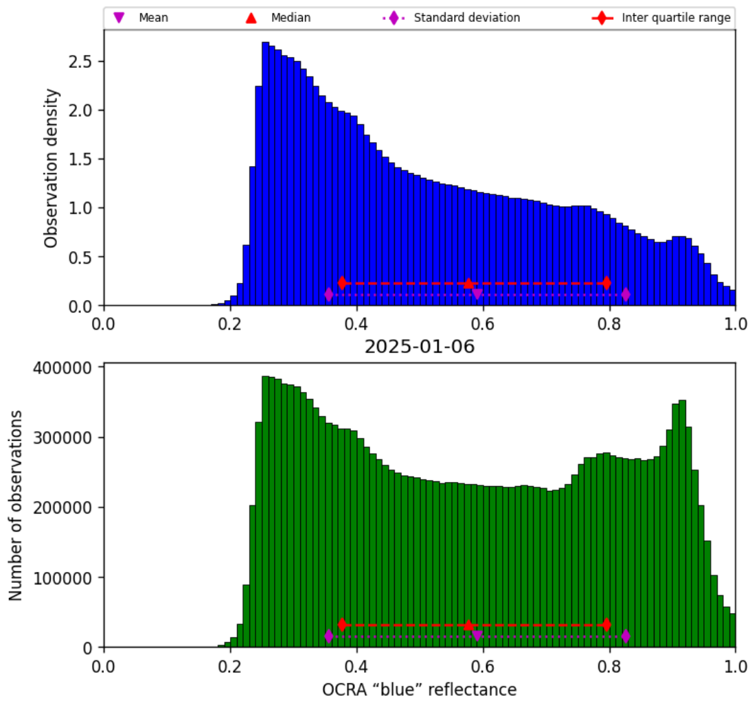
Figure 49: Histogram of “OCRA “blue” reflectance” for 2025-01-06 to 2025-01-07
