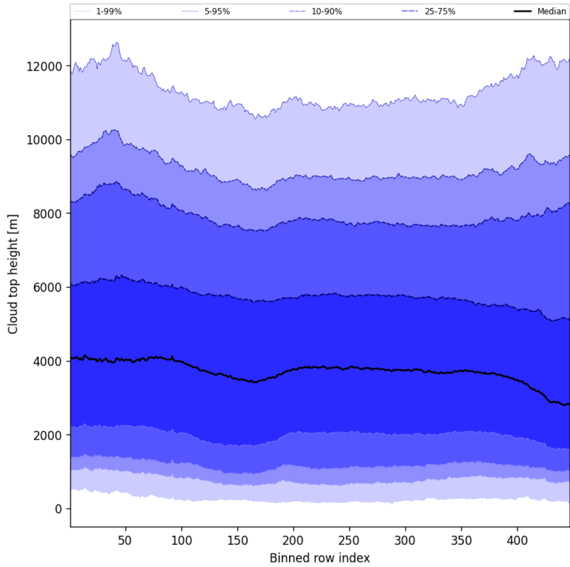
Figure 54: Along track statistics of “Cloud top height” for 2025-01-06 to 2025-01-07
