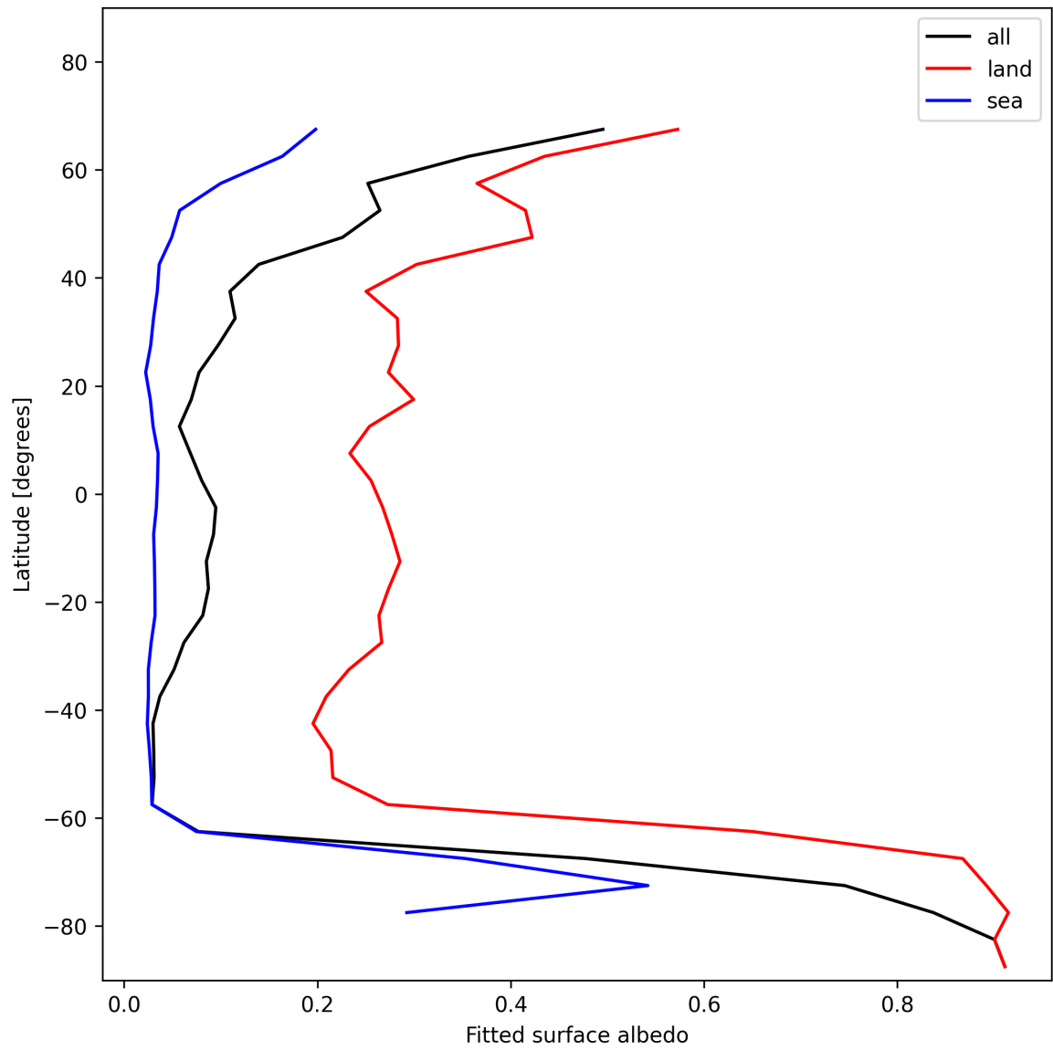
Figure 27: Zonal average of “Fitted surface albedo” for 2025-01-06 to 2025-01-07.
