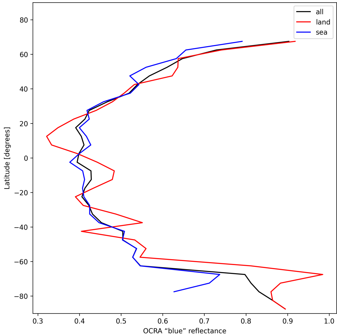
Figure 33: Zonal average of “OCRA “blue” reflectance” for 2025-01-06 to 2025-01-07.
