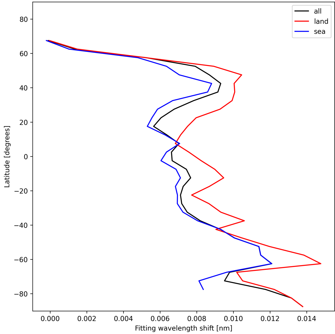
Figure 31: Zonal average of “Fitting wavelength shift” for 2025-01-06 to 2025-01-07.
