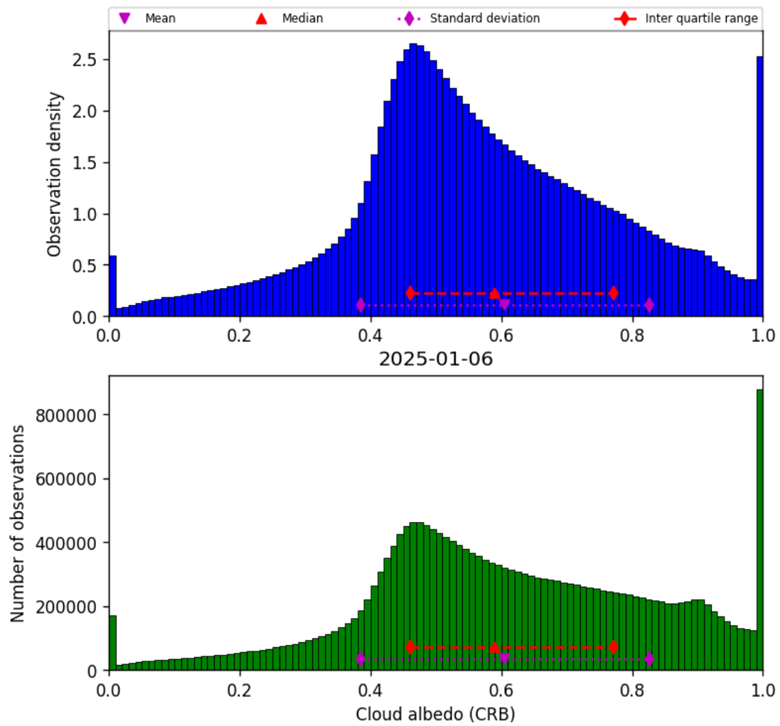
Figure 42: Histogram of “Cloud albedo (CRB)” for 2025-01-06 to 2025-01-07
