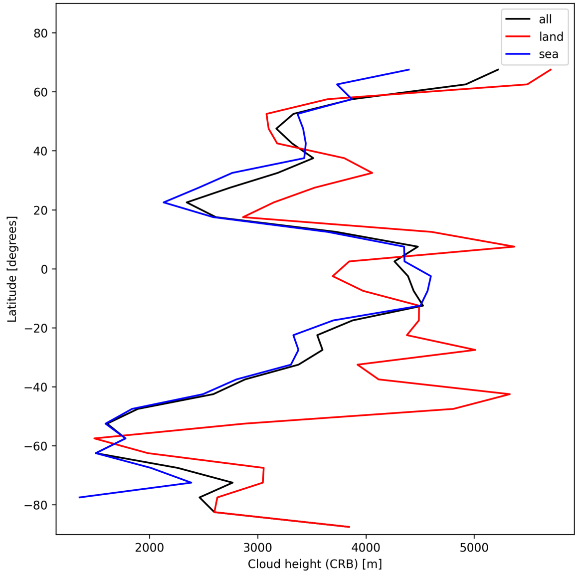
Figure 25: Zonal average of “Cloud height (CRB)” for 2025-01-06 to 2025-01-07.
