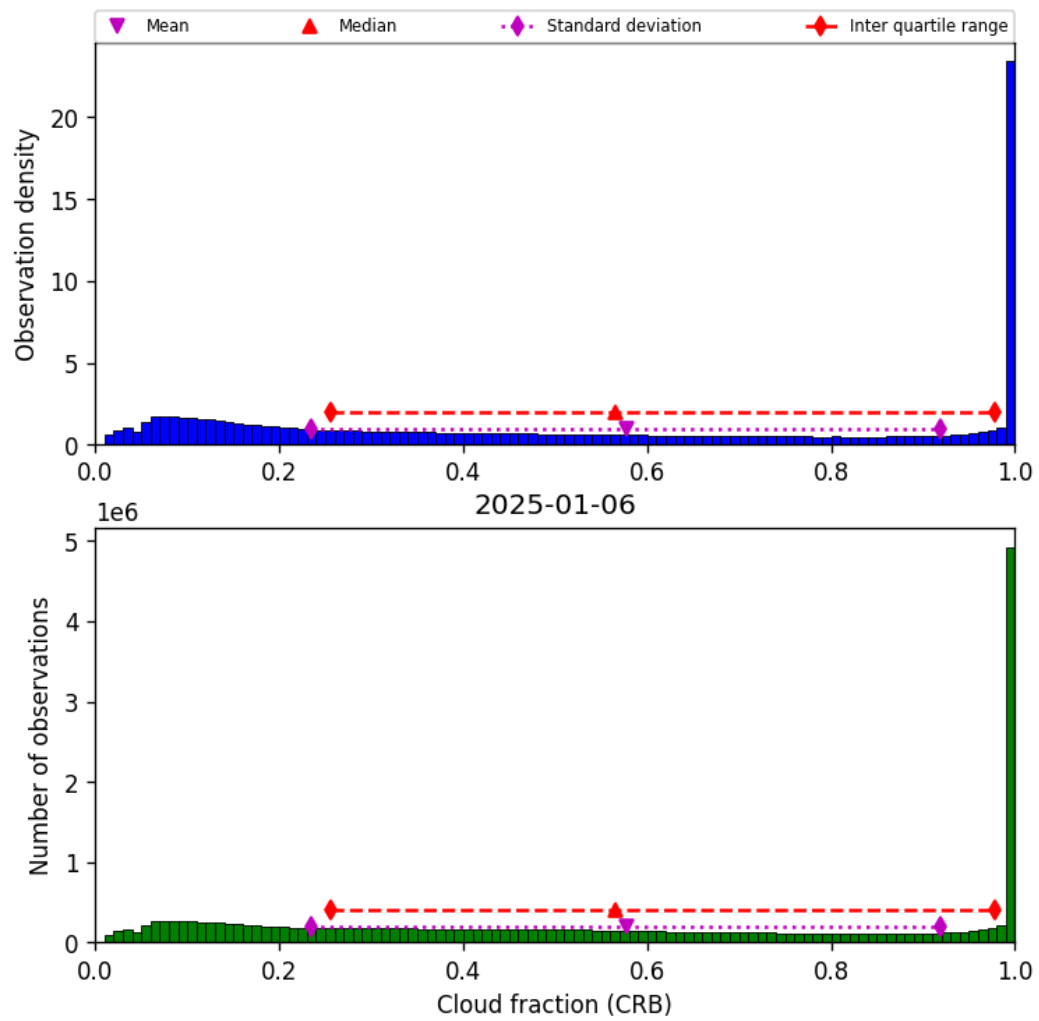
Figure 40: Histogram of “Cloud fraction (CRB)” for 2025-01-06 to 2025-01-07
