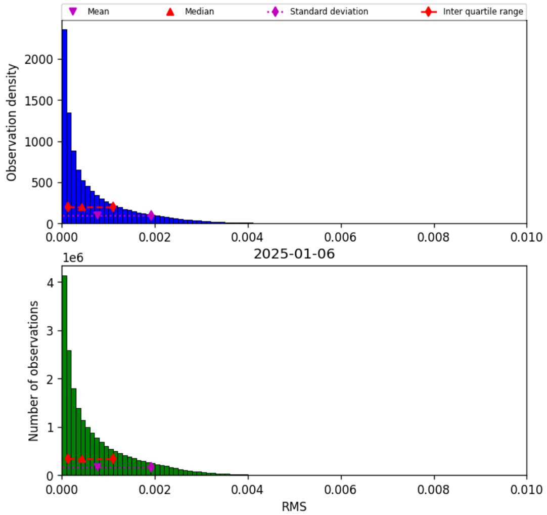
Figure 45: Histogram of “RMS” for 2025-01-06 to 2025-01-07
