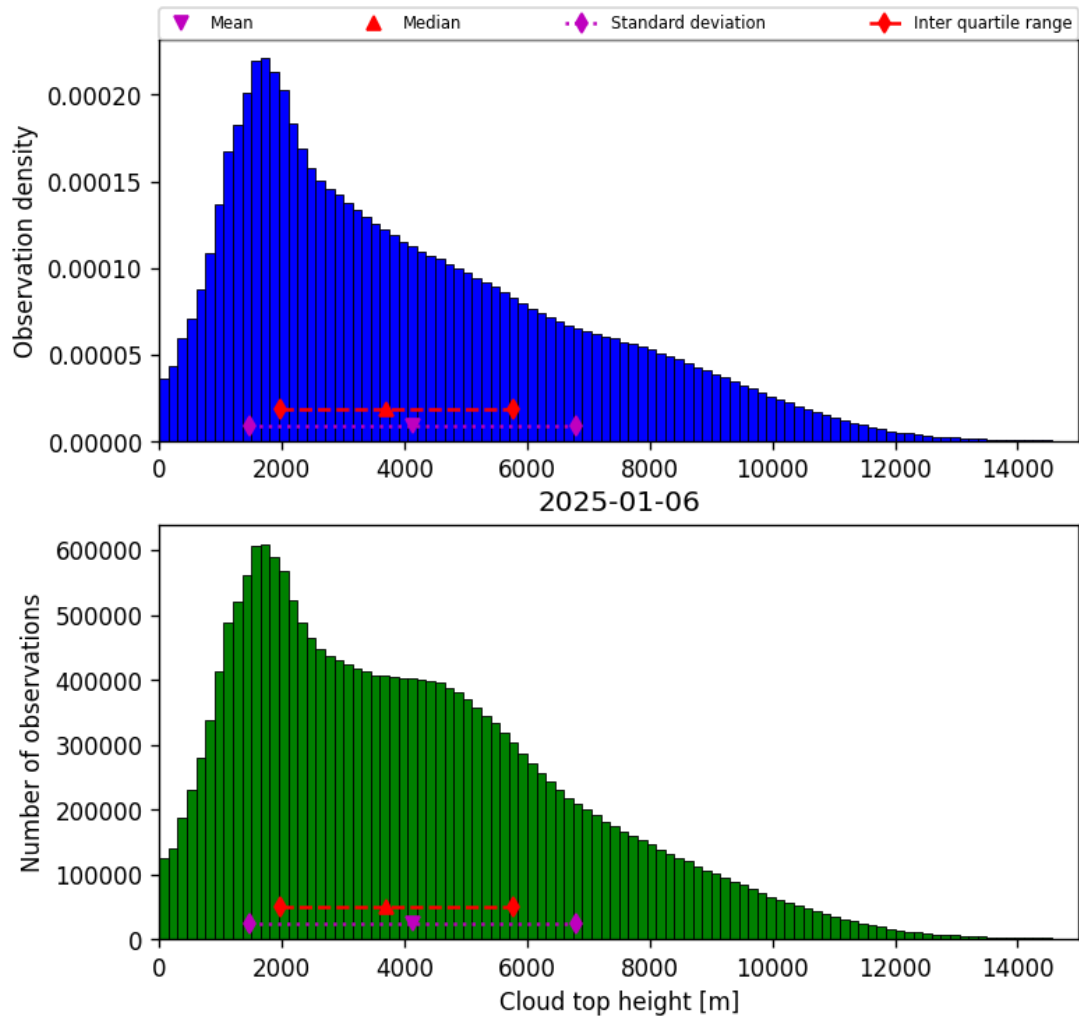
Figure 38: Histogram of “Cloud top height” for 2025-01-06 to 2025-01-07
