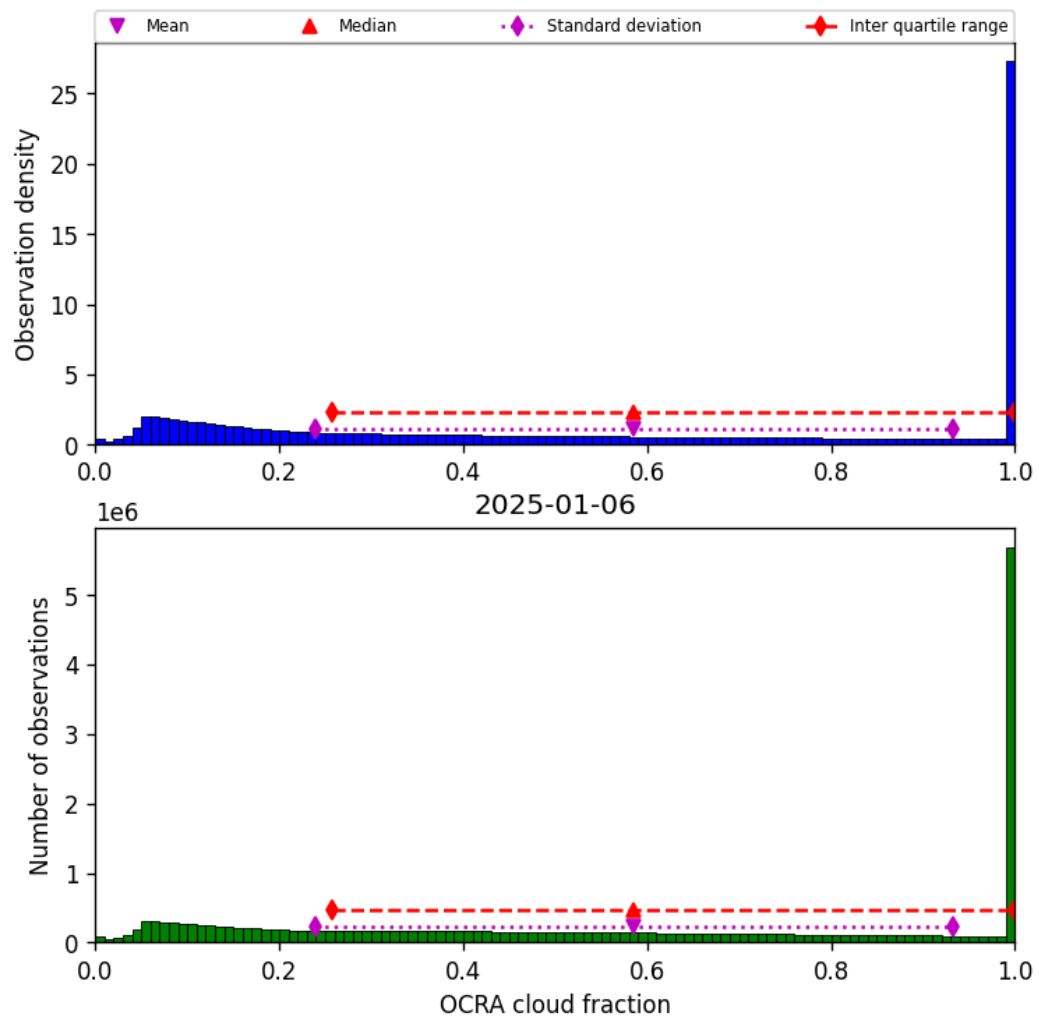
Figure 48: Histogram of “OCRA cloud fraction” for 2025-01-06 to 2025-01-07
