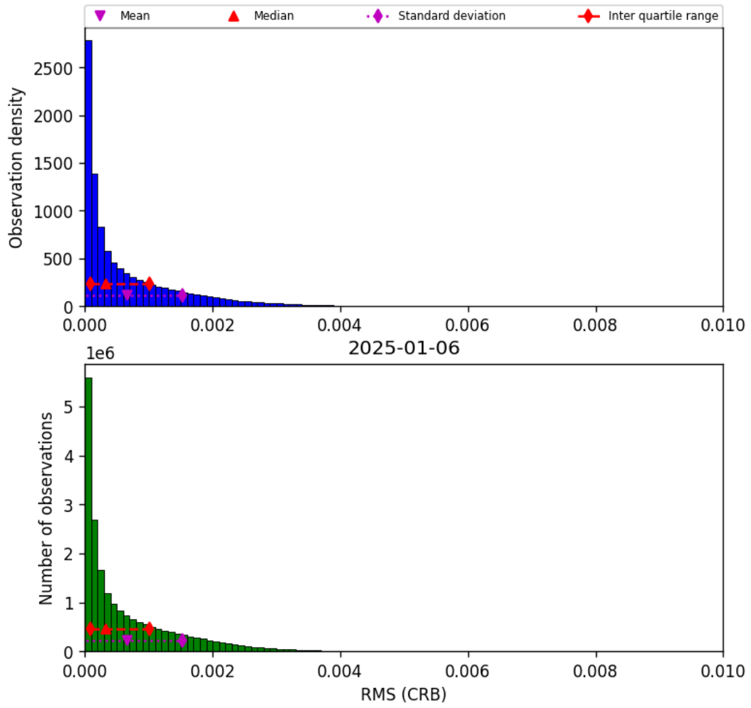
Figure 46: Histogram of "RMS (CRB)" for 2025-01-06 to 2025-01-07
