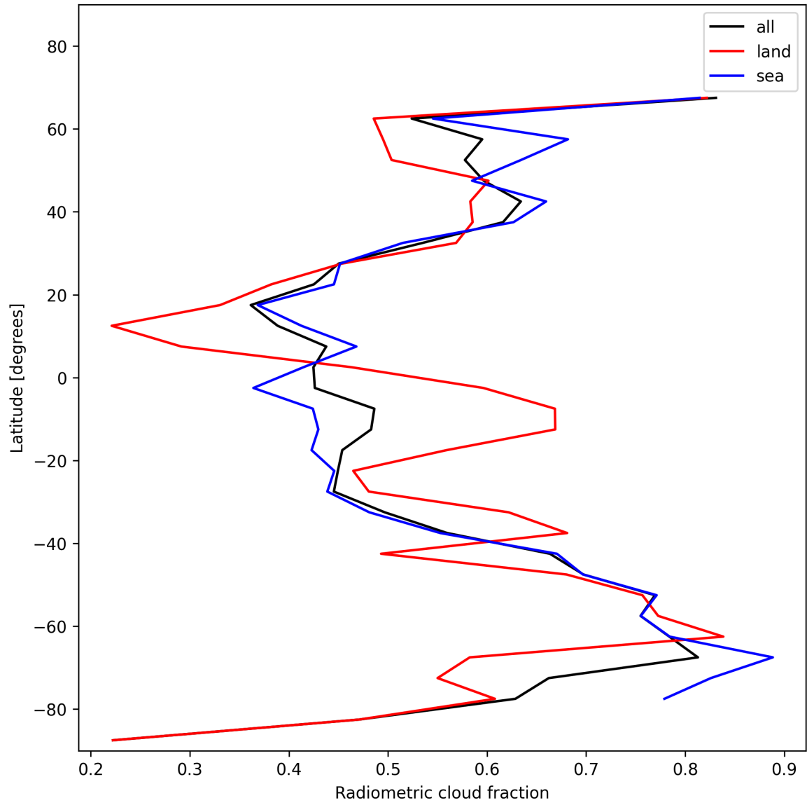
Figure 21: Zonal average of “Radiometric cloud fraction” for 2025-01-06 to 2025-01-07.
