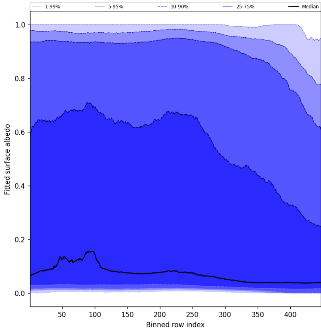
Figure 59: Along track statistics of “Fitted surface albedo” for 2025-01-06 to 2025-01-07
