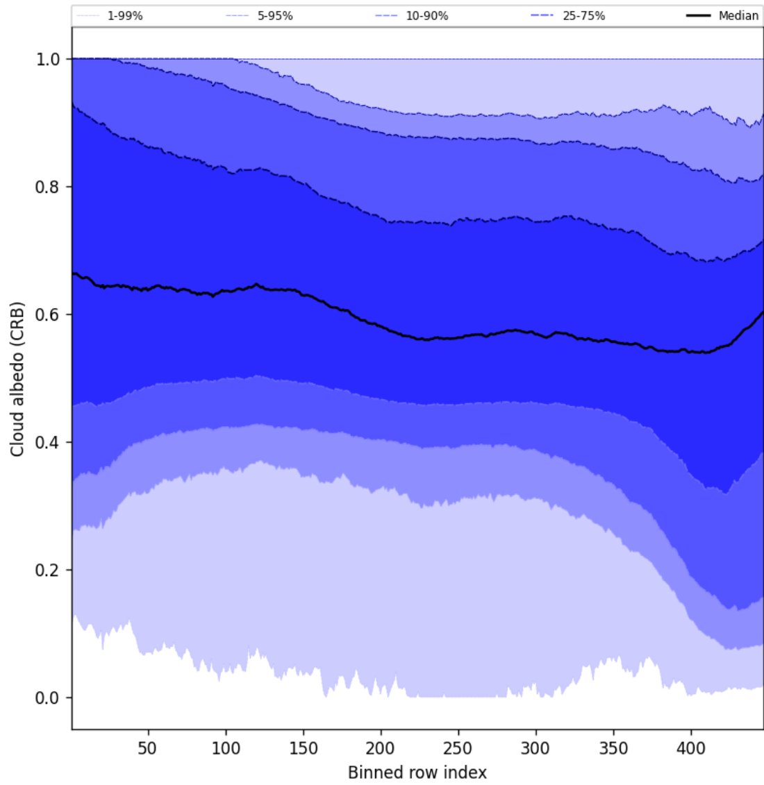
Figure 58: Along track statistics of “Cloud albedo (CRB)” for 2025-01-06 to 2025-01-07
