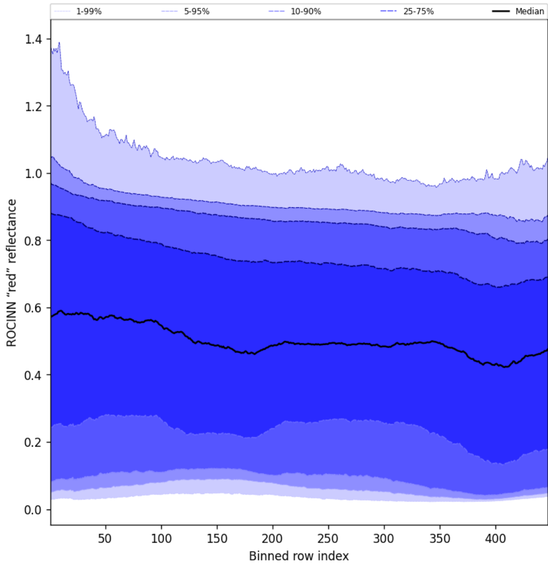
Figure 67: Along track statistics of “ROCINN “red” reflectance” for 2025-01-06 to 2025-01-07
