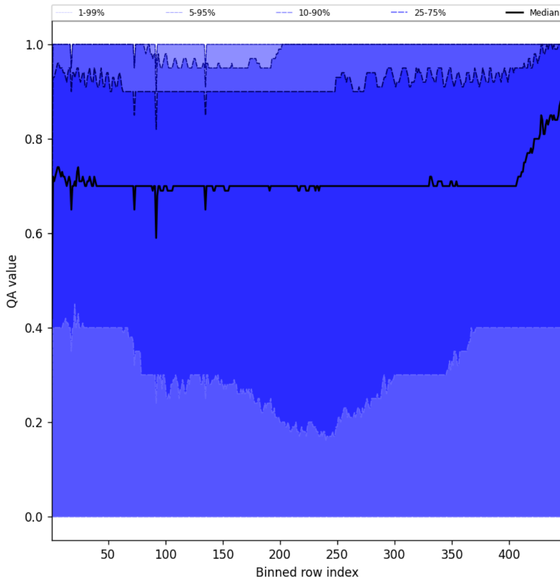
Figure 52: Along track statistics of “QA value” for 2025-01-06 to 2025-01-07
