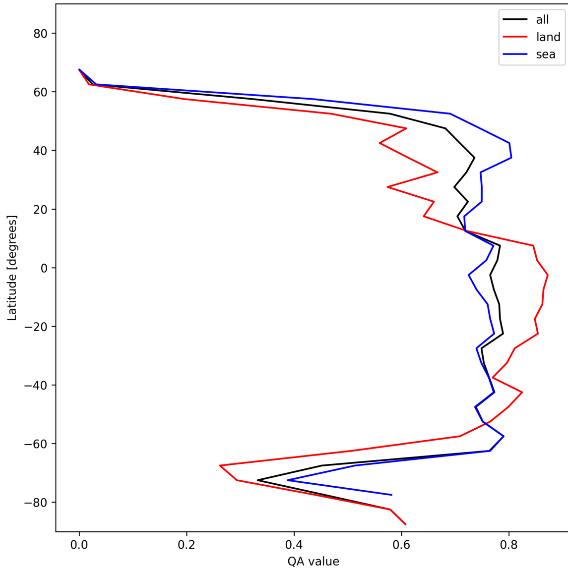
Figure 20: Zonal average of “QA value” for 2025-01-06 to 2025-01-07.
