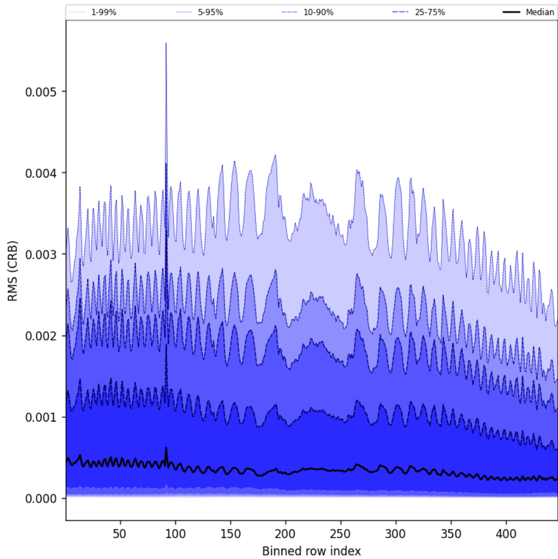
Figure 62: Along track statistics of “RMS (CRB)” for 2025-01-06 to 2025-01-07
