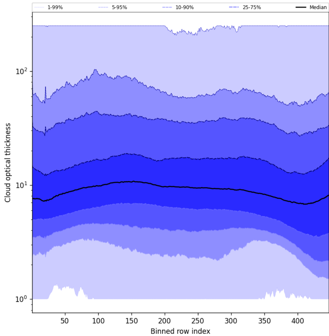
Figure 55: Along track statistics of “Cloud optical thickness” for 2025-01-06 to 2025-01-07
