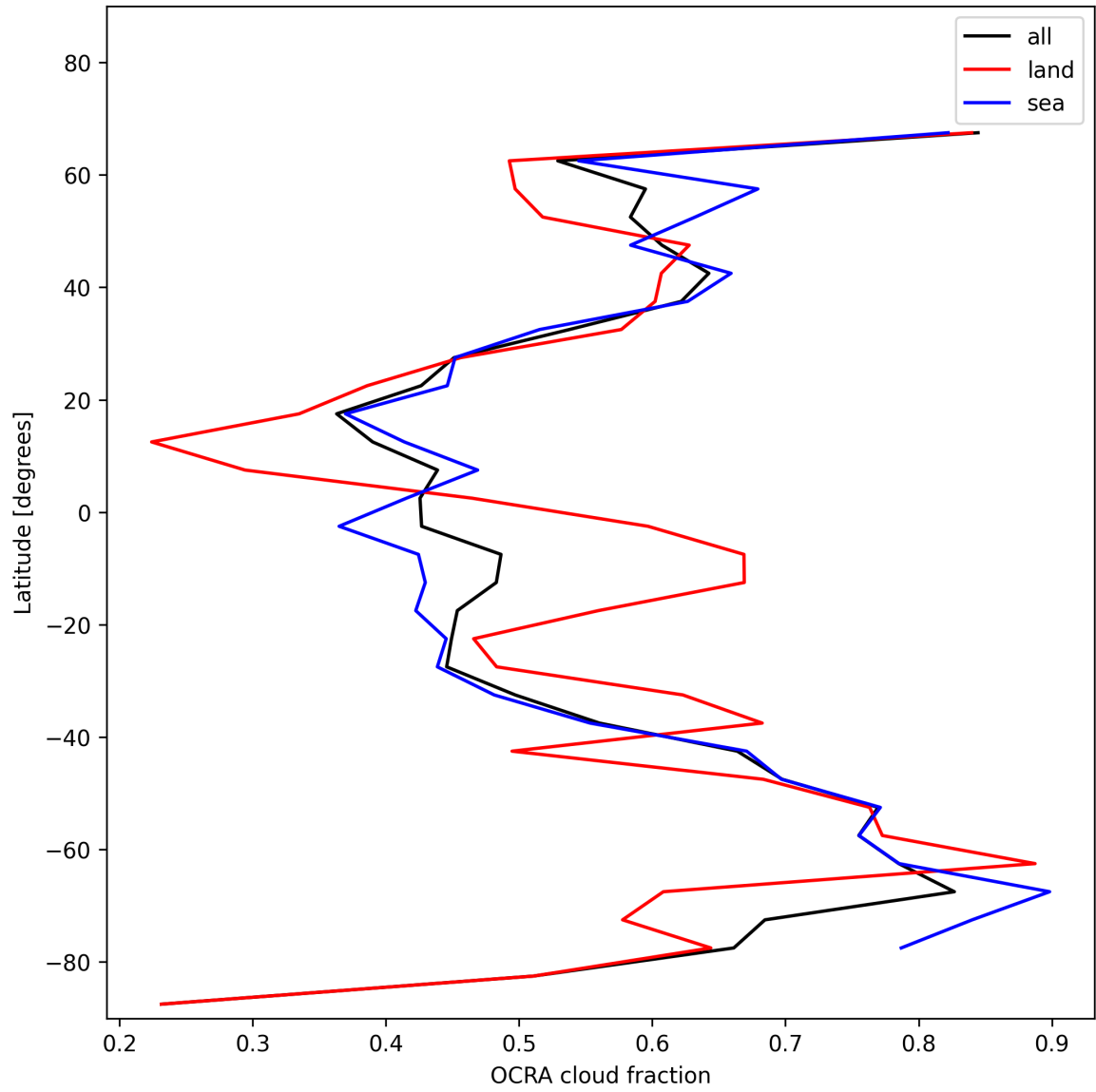
Figure 32: Zonal average of “OCRA cloud fraction” for 2025-01-06 to 2025-01-07.
