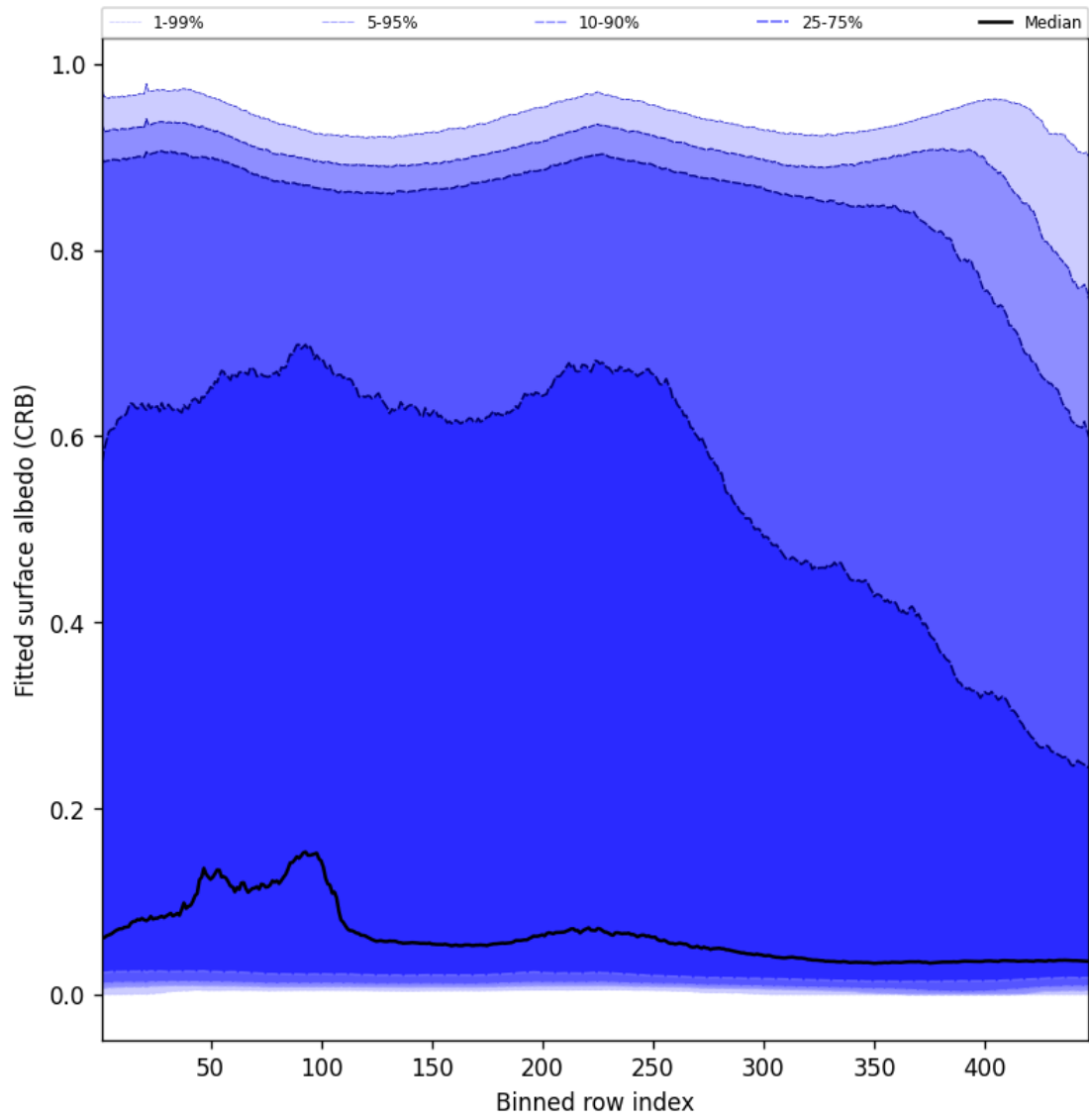
Figure 60: Along track statistics of “Fitted surface albedo (CRB)” for 2025-01-06 to 2025-01-07
