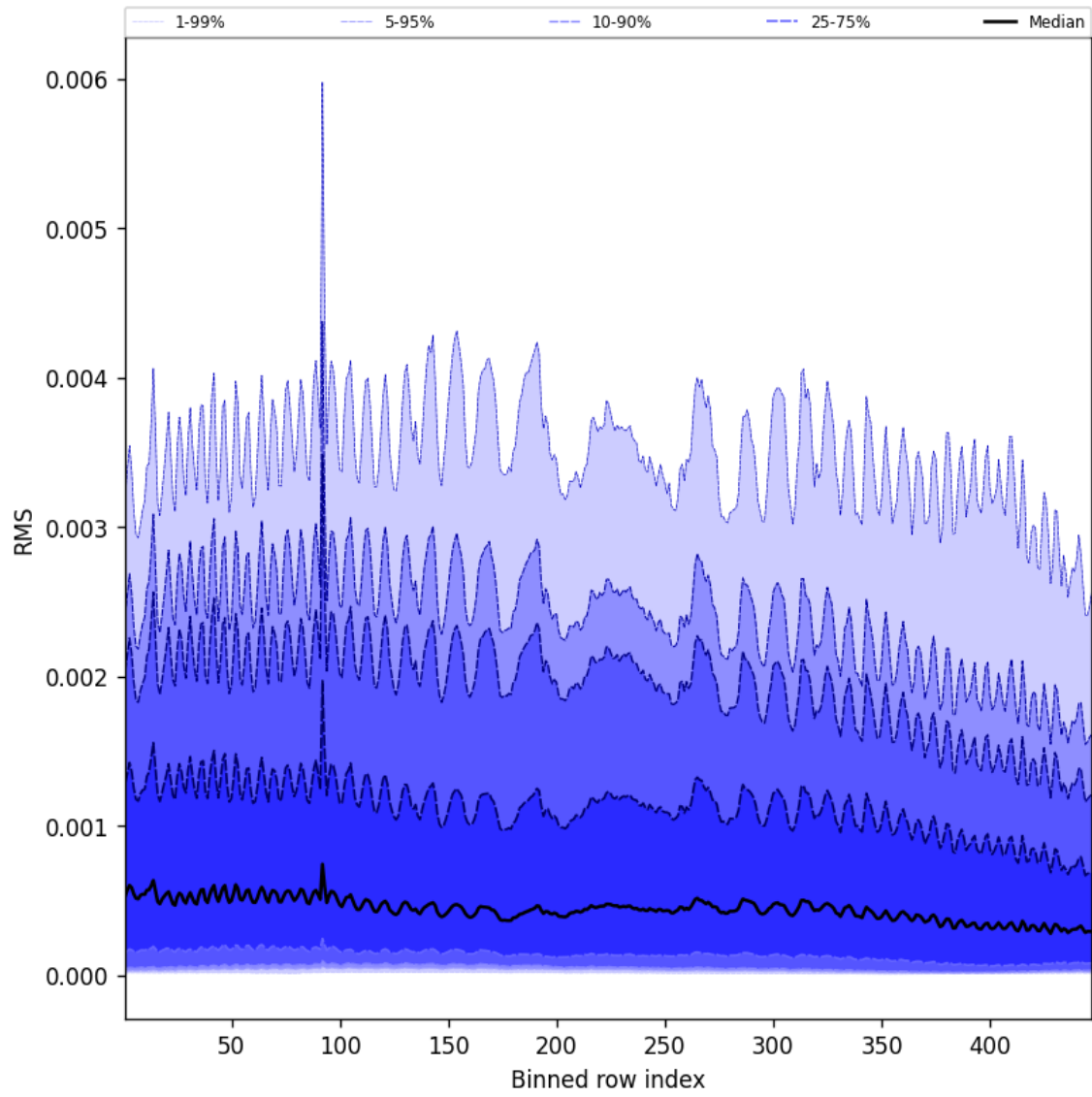
Figure 61: Along track statistics of “RMS” for 2025-01-06 to 2025-01-07
