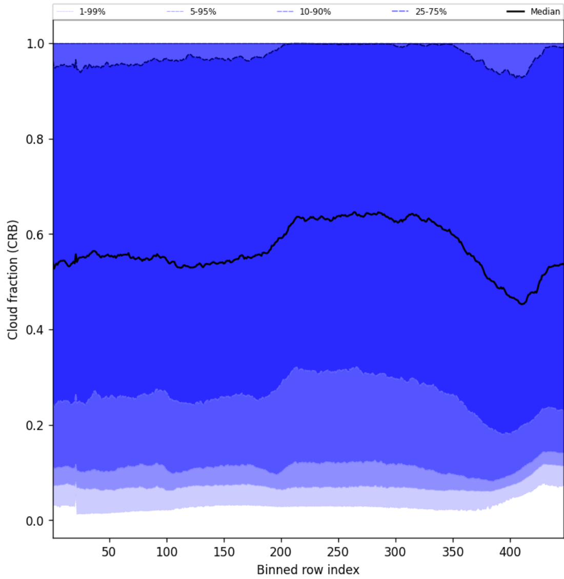
Figure 56: Along track statistics of “Cloud fraction (CRB)” for 2025-01-06 to 2025-01-07
