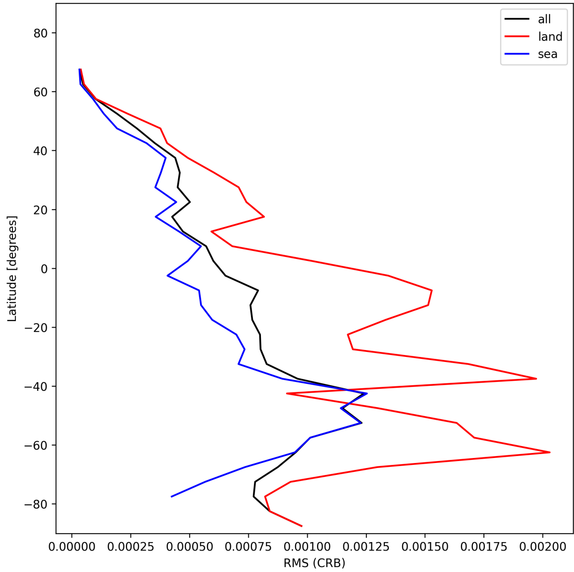
Figure 30: Zonal average of “RMS (CRB)” for 2025-01-06 to 2025-01-07.
