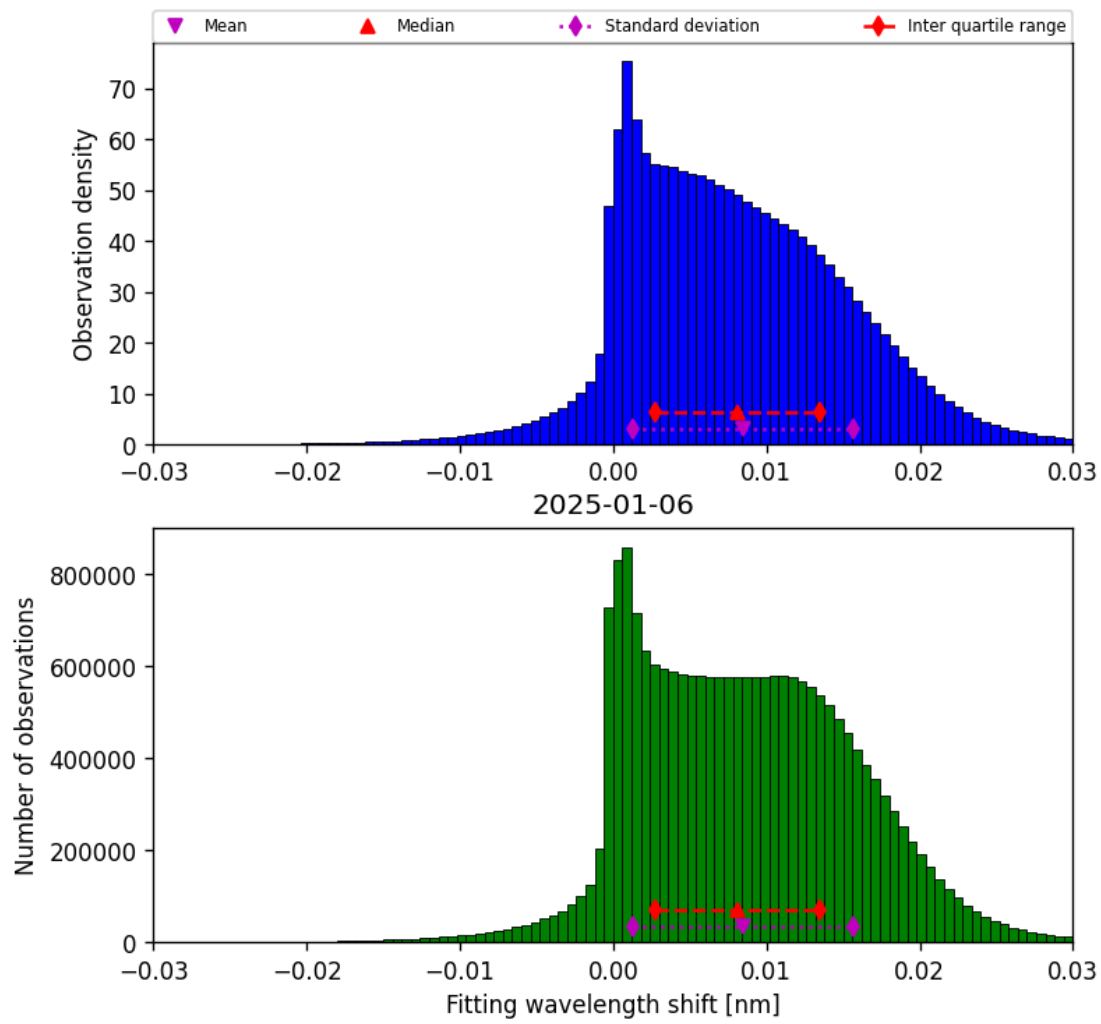
Figure 47: Histogram of “Fitting wavelength shift” for 2025-01-06 to 2025-01-07
