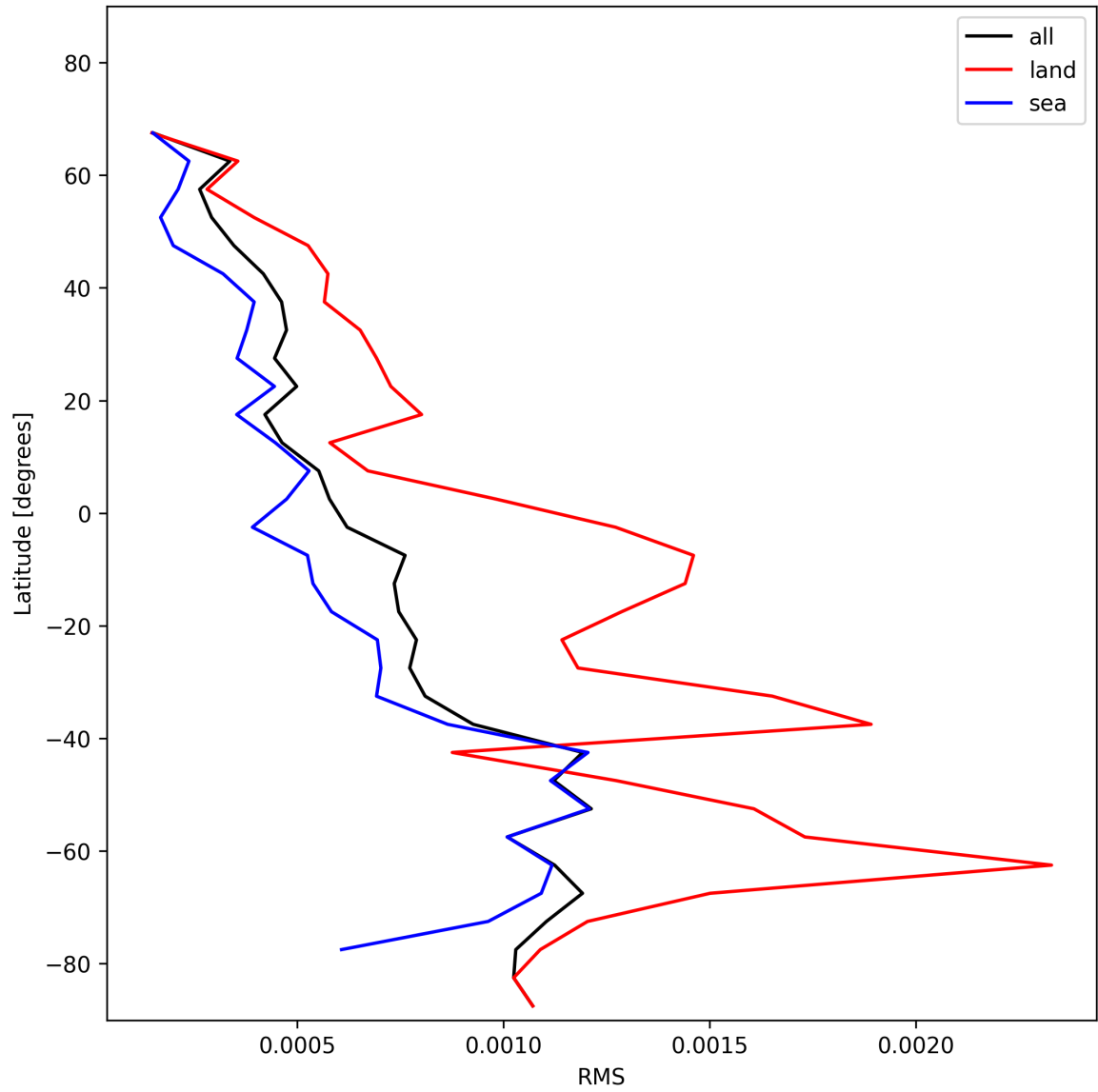
Figure 29: Zonal average of “RMS” for 2025-01-06 to 2025-01-07.
