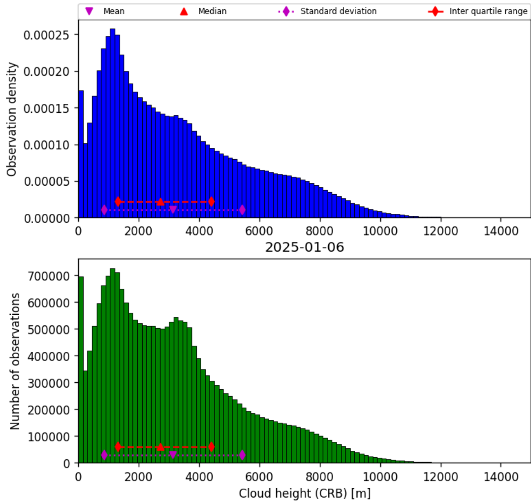
Figure 41: Histogram of “Cloud height (CRB)” for 2025-01-06 to 2025-01-07
