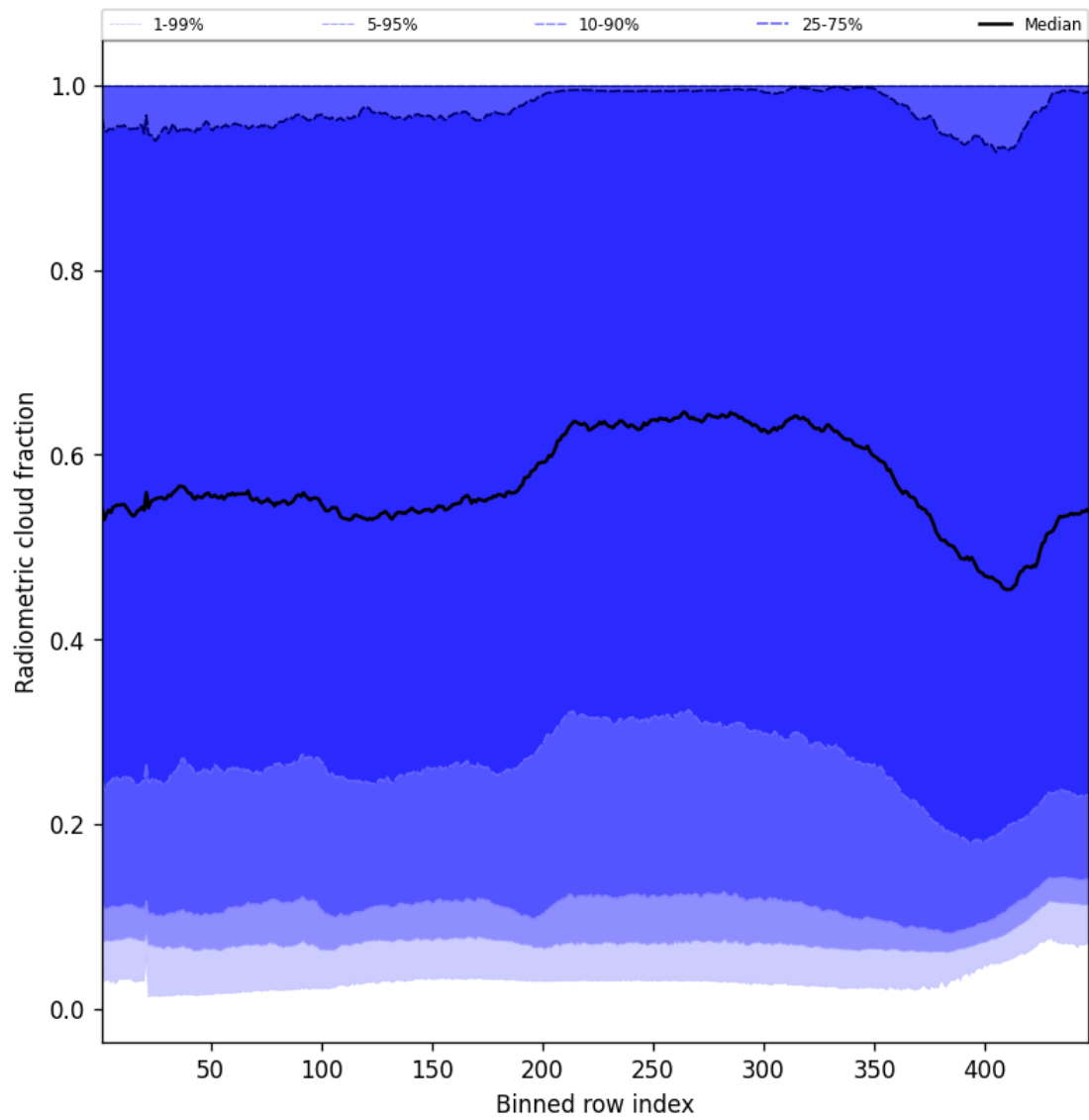
Figure 53: Along track statistics of “Radiometric cloud fraction” for 2025-01-06 to 2025-01-07
