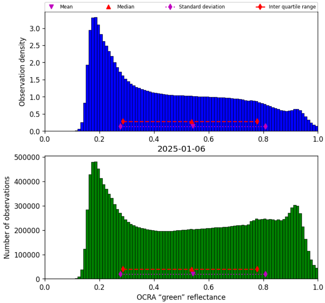
Figure 50: Histogram of “OCRA “green” reflectance” for 2025-01-06 to 2025-01-07
