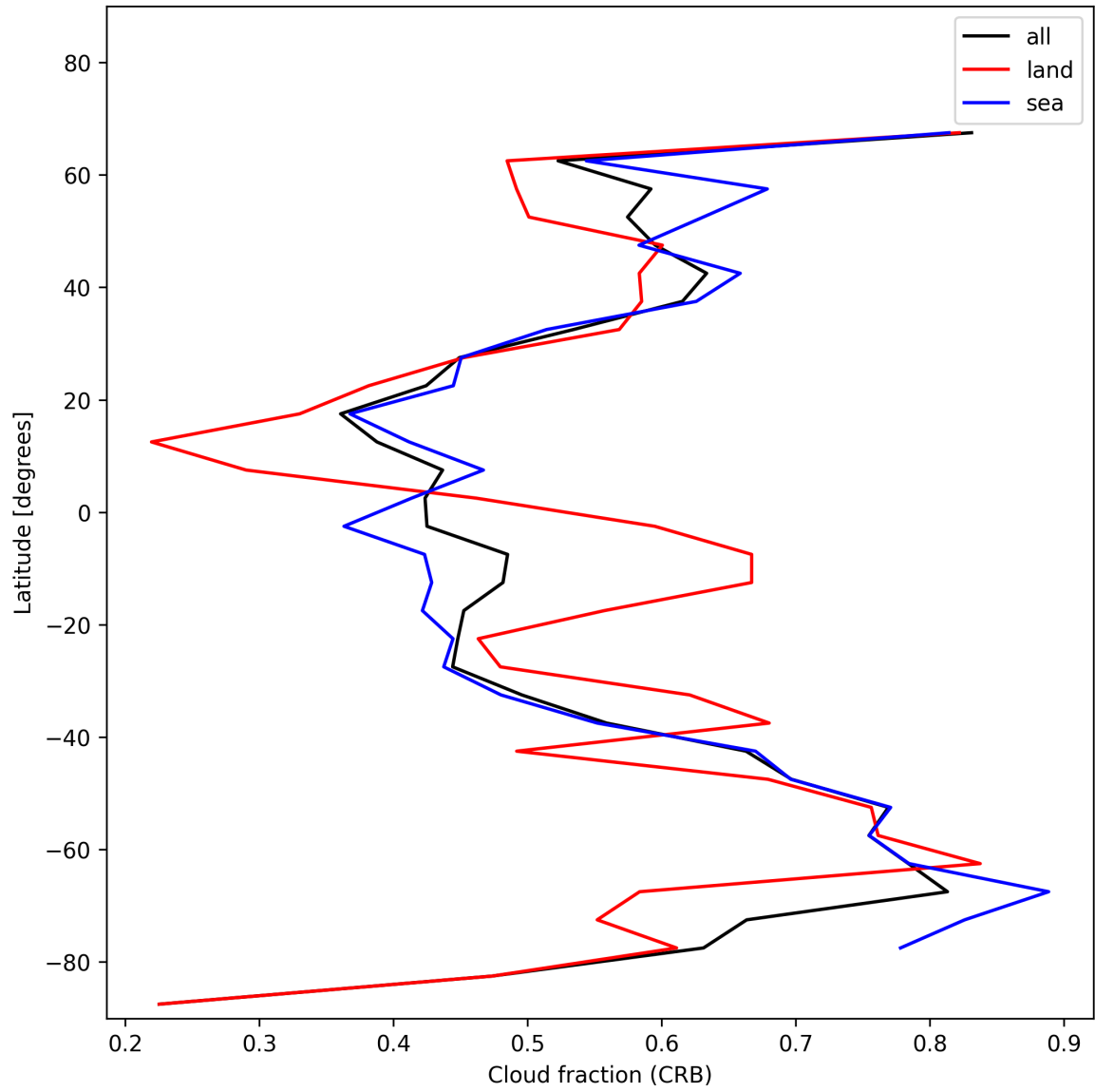
Figure 24: Zonal average of “Cloud fraction (CRB)” for 2025-01-06 to 2025-01-07.
