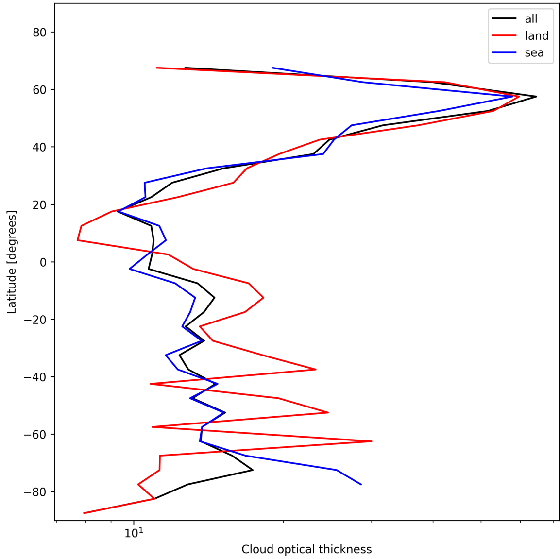
Figure 23: Zonal average of “Cloud optical thickness” for 2025-01-06 to 2025-01-07.
