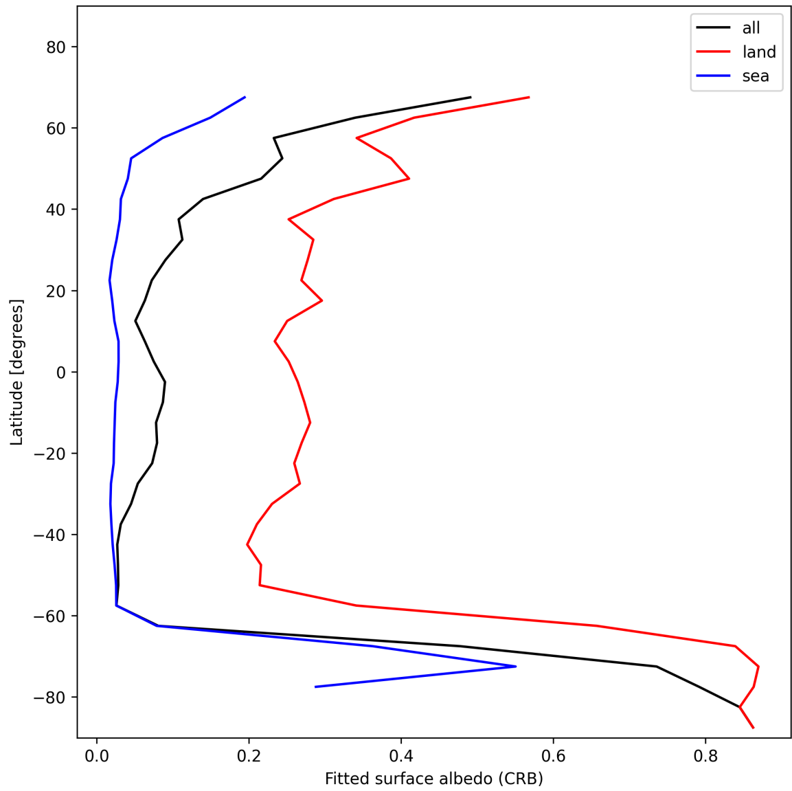
Figure 28: Zonal average of “Fitted surface albedo (CRB)” for 2025-01-06 to 2025-01-07.
