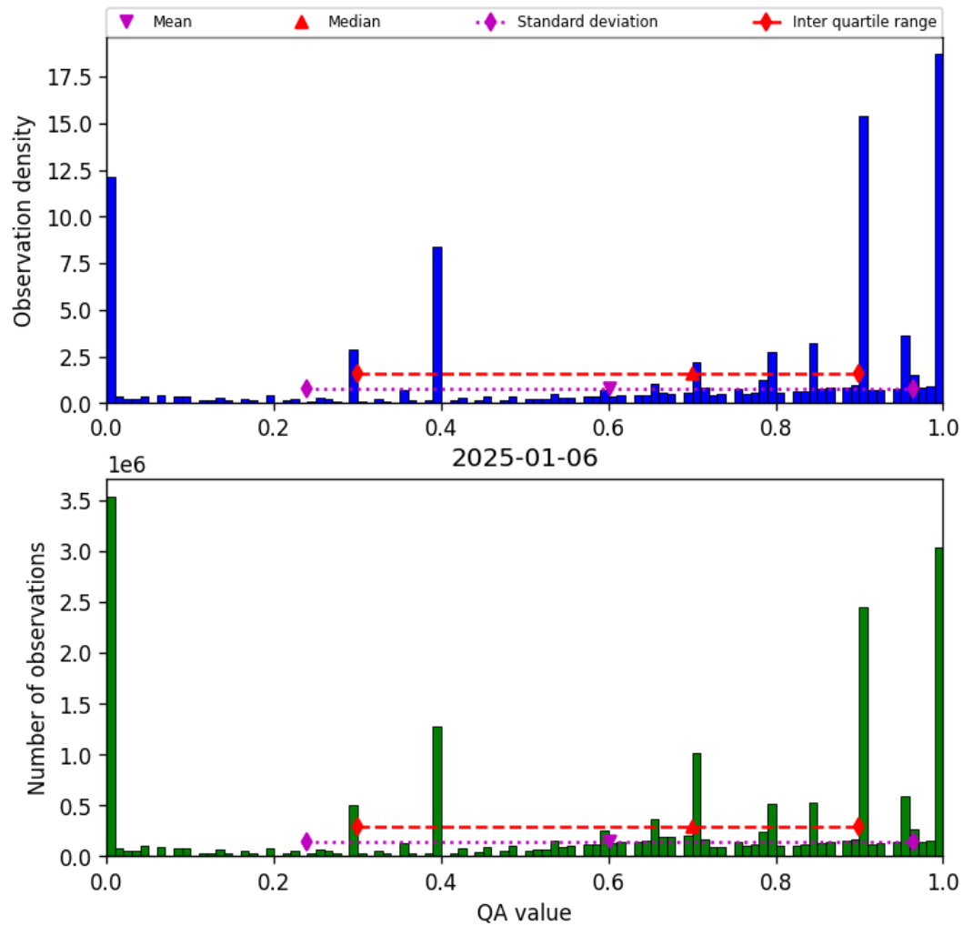
Figure 36: Histogram of “QA value” for 2025-01-06 to 2025-01-07
