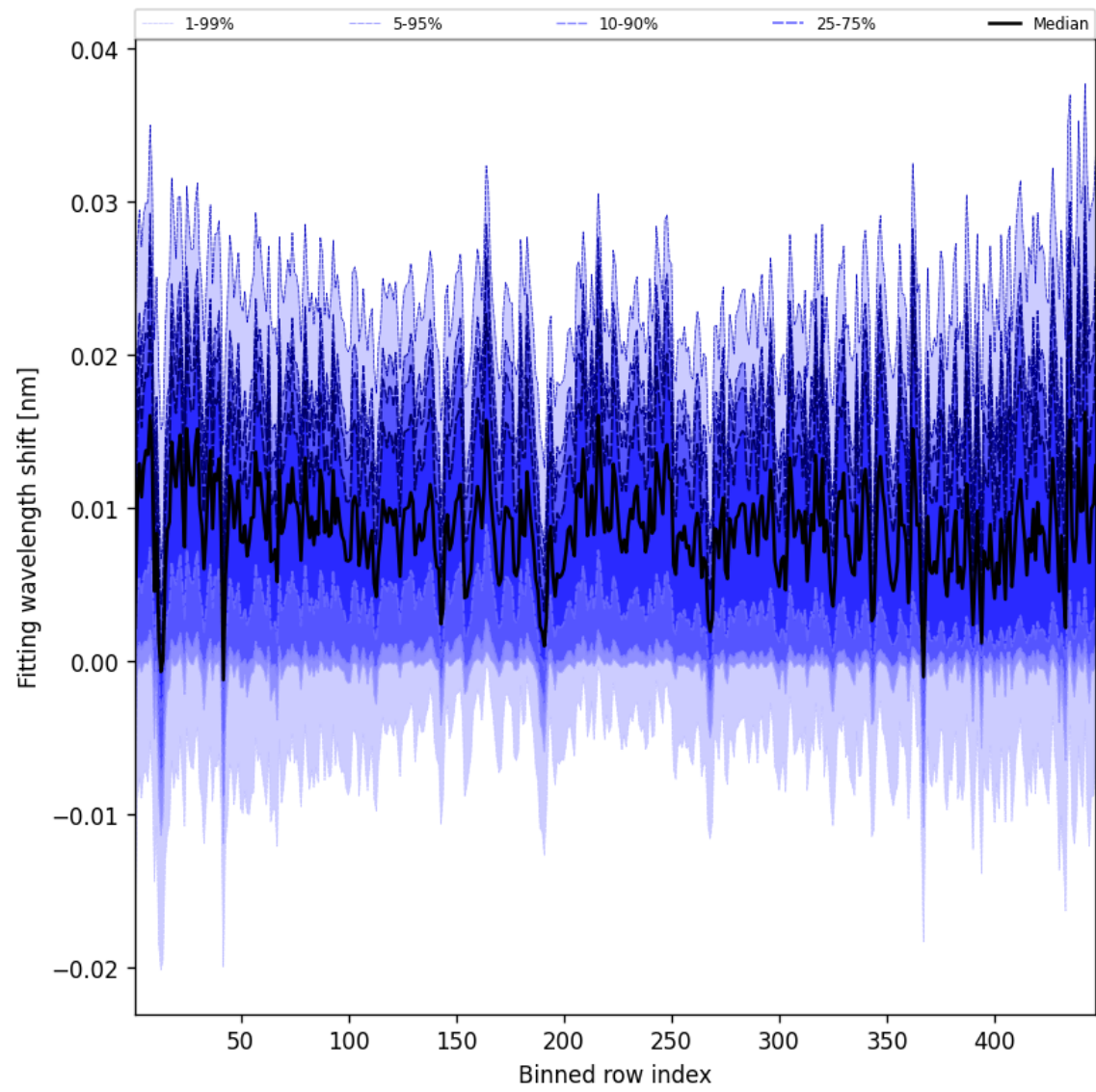
Figure 63: Along track statistics of “Fitting wavelength shift” for 2025-01-06 to 2025-01-07
