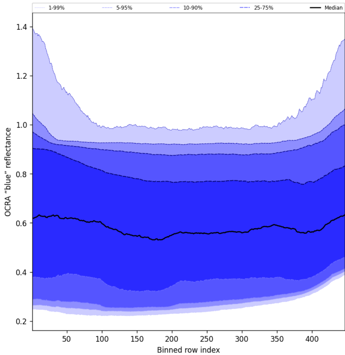
Figure 65: Along track statistics of “OCRA “blue” reflectance” for 2025-01-06 to 2025-01-07
