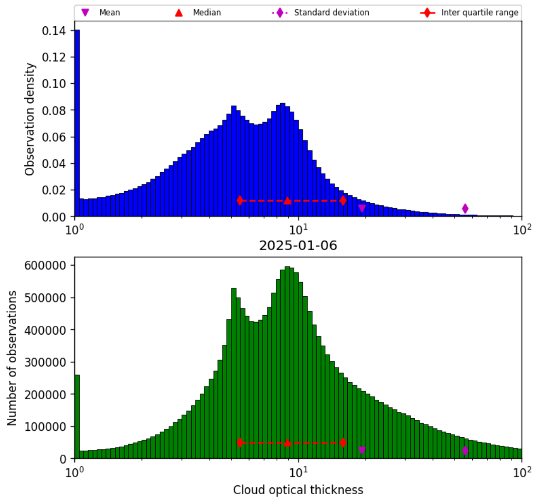
Figure 39: Histogram of “Cloud optical thickness” for 2025-01-06 to 2025-01-07
