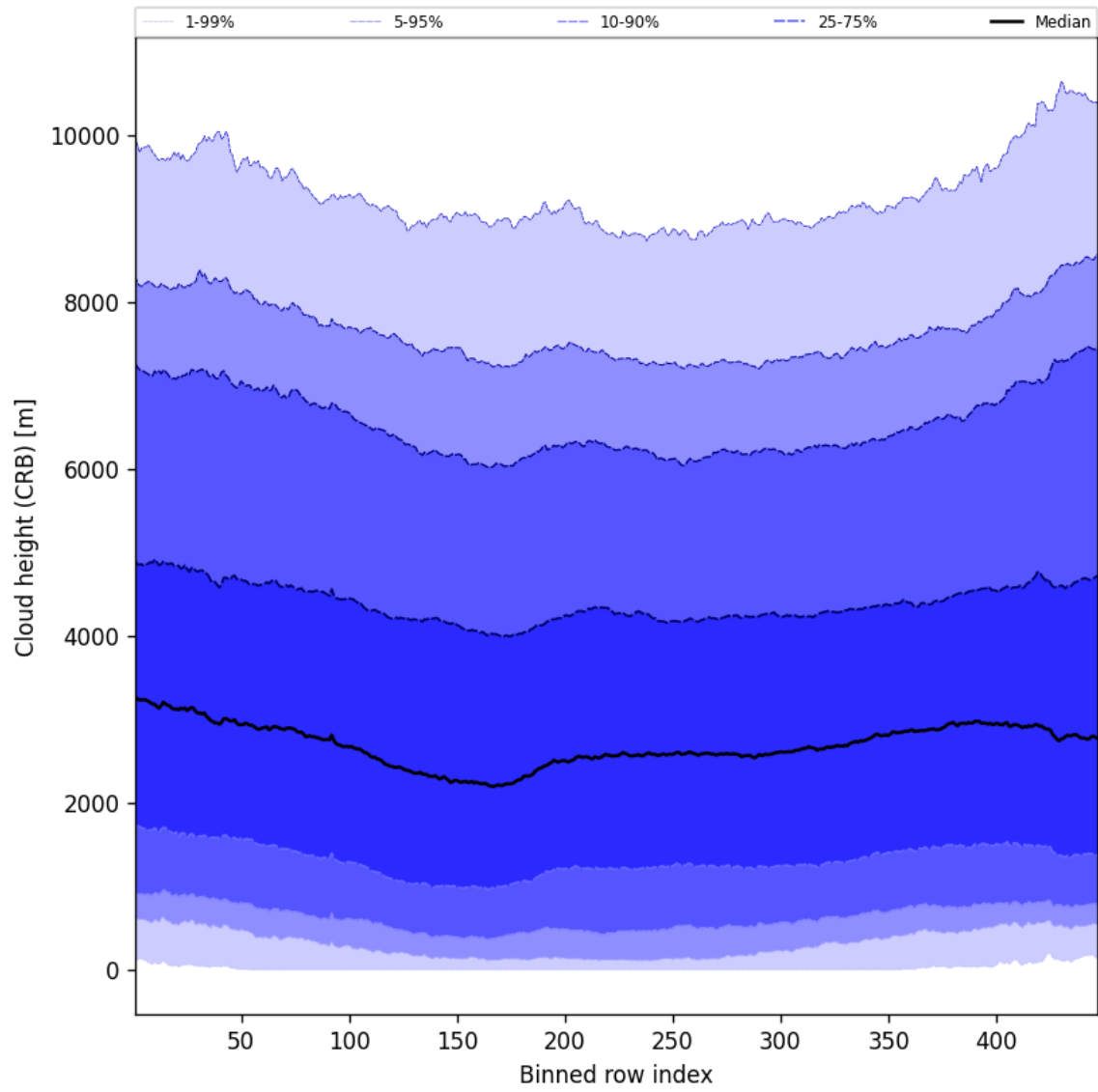
Figure 57: Along track statistics of “Cloud height (CRB)” for 2025-01-06 to 2025-01-07
