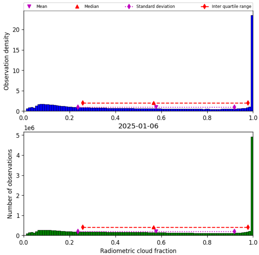
Figure 37: Histogram of “Radiometric cloud fraction” for 2025-01-06 to 2025-01-07
