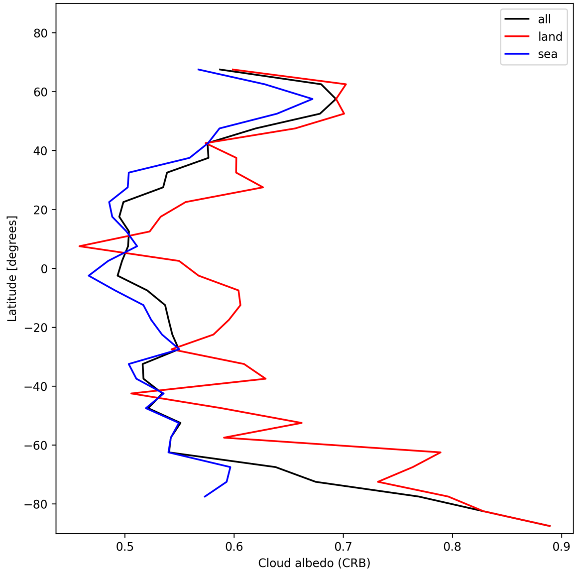
Figure 26: Zonal average of “Cloud albedo (CRB)” for 2025-01-06 to 2025-01-07.
