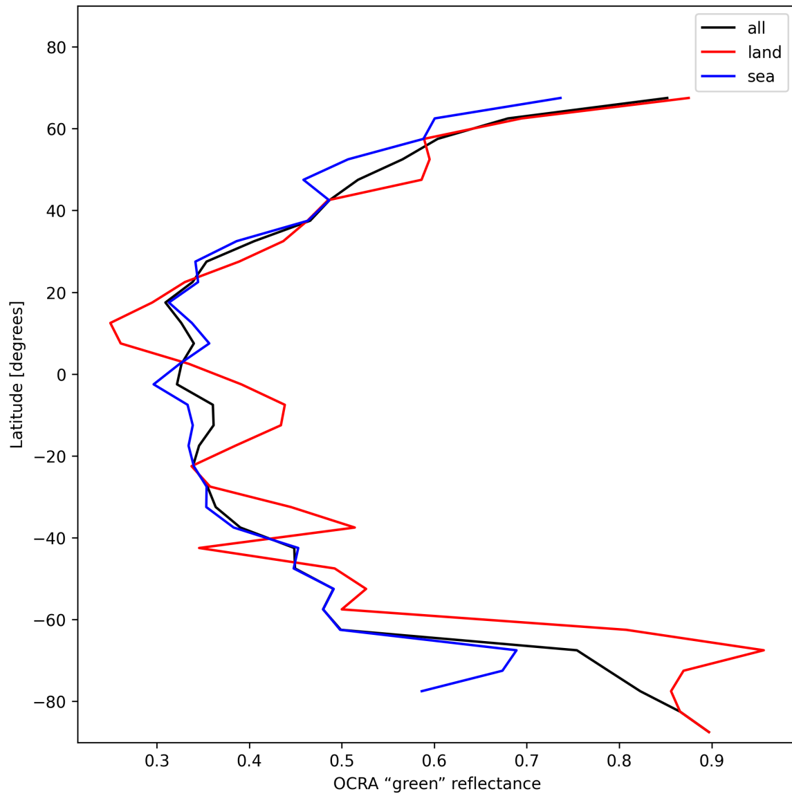
Figure 34: Zonal average of “OCRA “green” reflectance” for 2025-01-06 to 2025-01-07.
