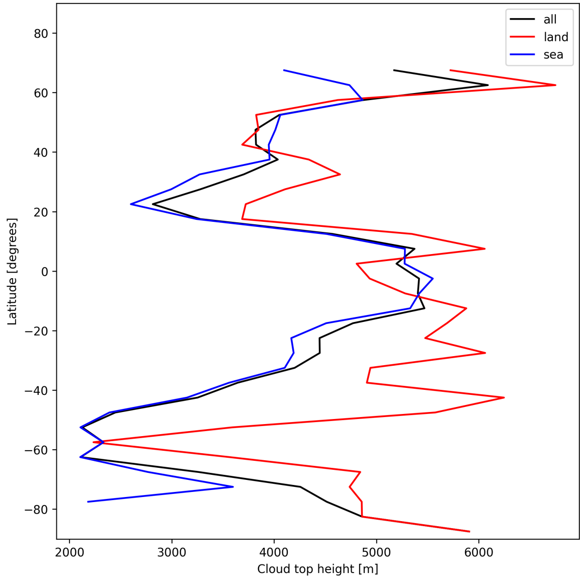
Figure 22: Zonal average of “Cloud top height” for 2025-01-06 to 2025-01-07.
