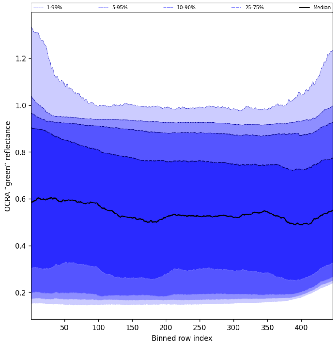
Figure 66: Along track statistics of "OCRA "green" reflectance" for 2025-01-06 to 2025-01-07
