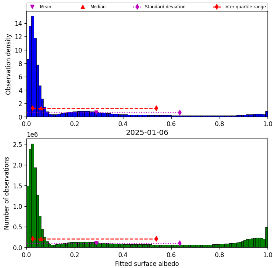
Figure 43: Histogram of “Fitted surface albedo” for 2025-01-06 to 2025-01-07
