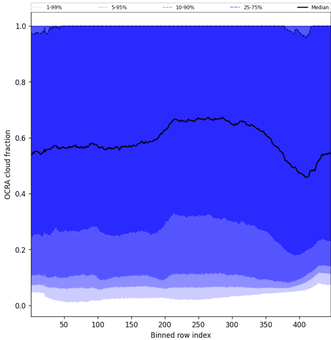
Figure 64: Along track statistics of “OCRA cloud fraction” for 2025-01-06 to 2025-01-07
