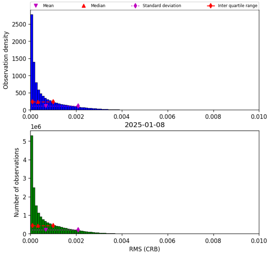
Figure 46: Histogram of “RMS (CRB)” for 2025-01-08 to 2025-01-09
