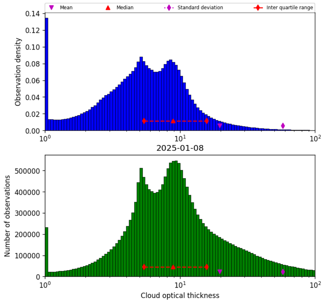
Figure 39: Histogram of “Cloud optical thickness” for 2025-01-08 to 2025-01-09
