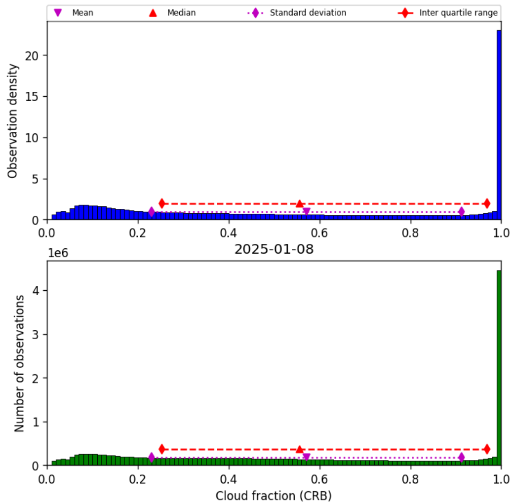
Figure 40: Histogram of “Cloud fraction (CRB)” for 2025-01-08 to 2025-01-09
