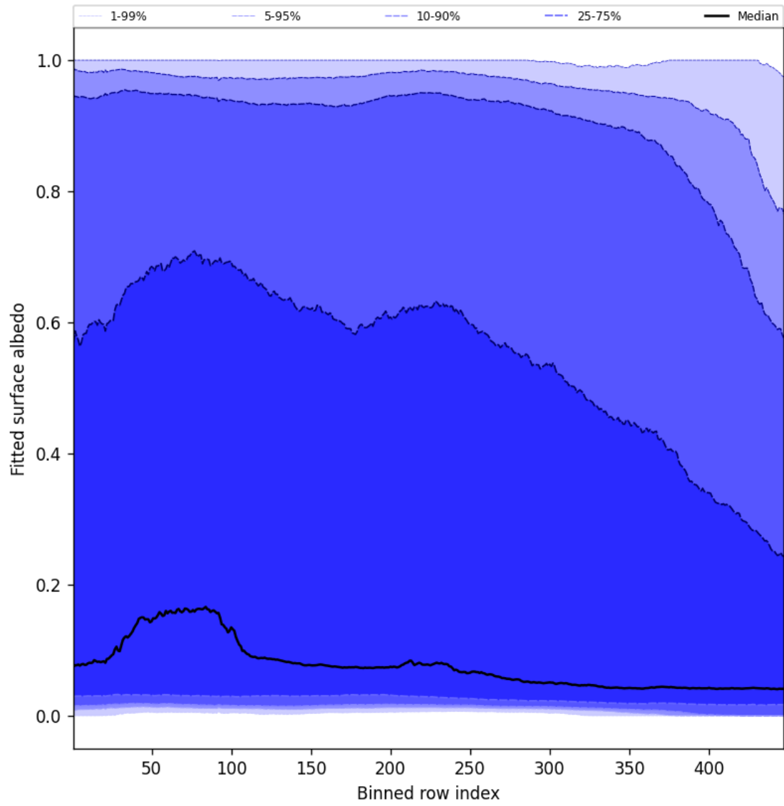
Figure 59: Along track statistics of “Fitted surface albedo” for 2025-01-08 to 2025-01-09
