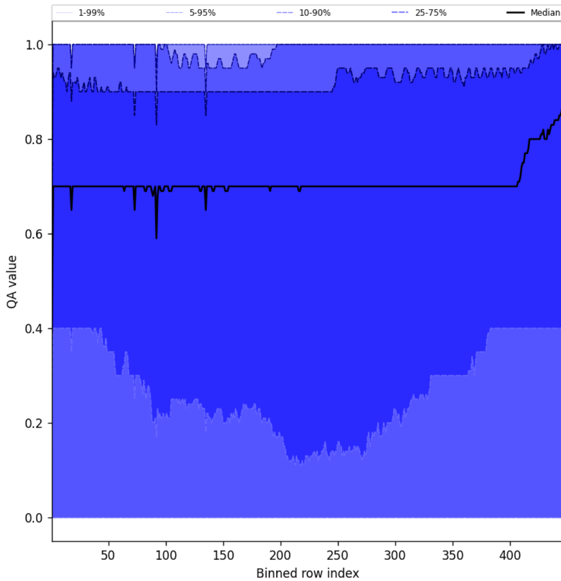
Figure 52: Along track statistics of “QA value” for 2025-01-08 to 2025-01-09
