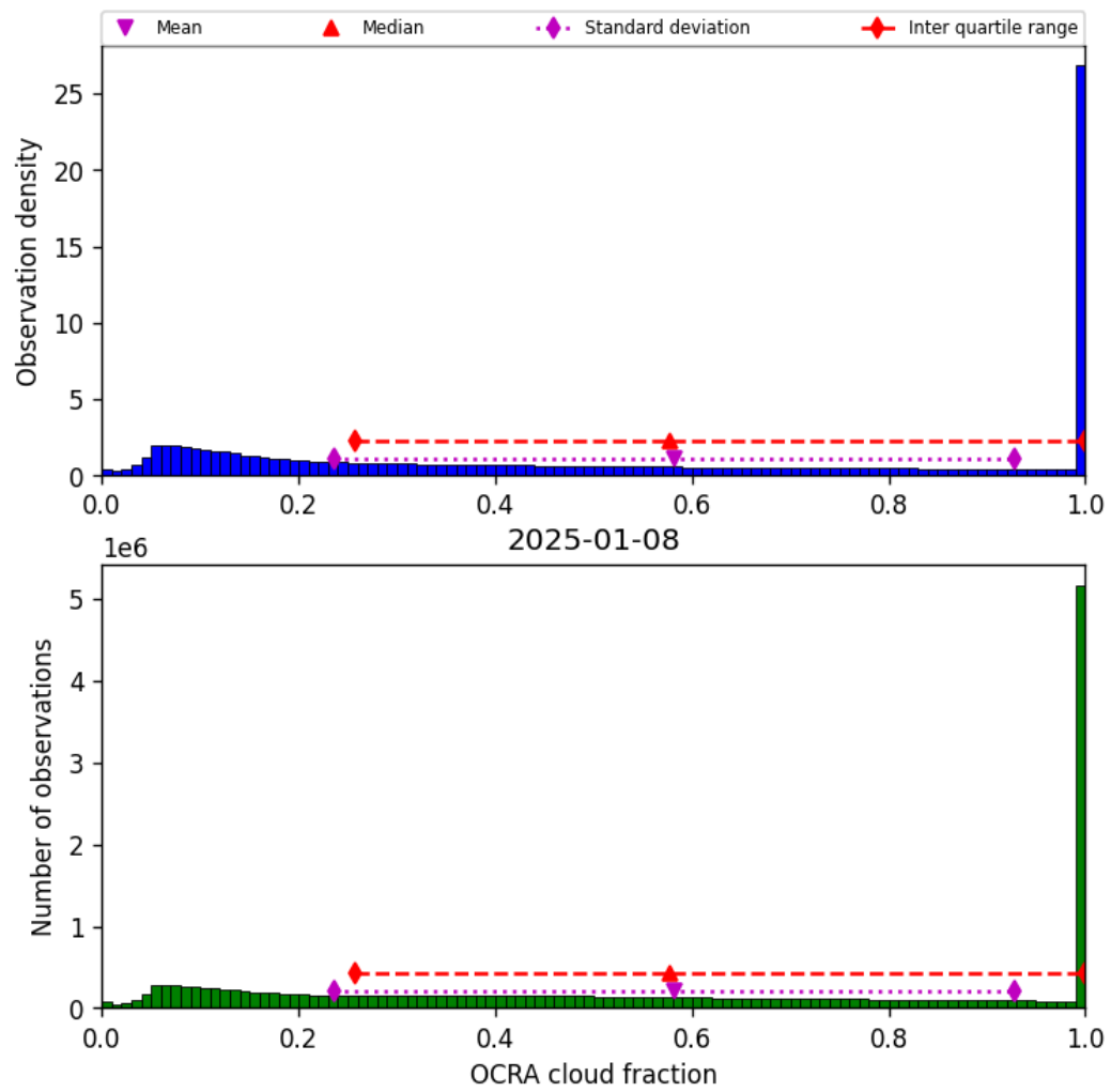
Figure 48: Histogram of “OCRA cloud fraction” for 2025-01-08 to 2025-01-09
