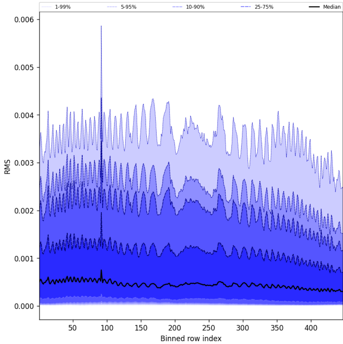
Figure 61: Along track statistics of “RMS” for 2025-01-08 to 2025-01-09
