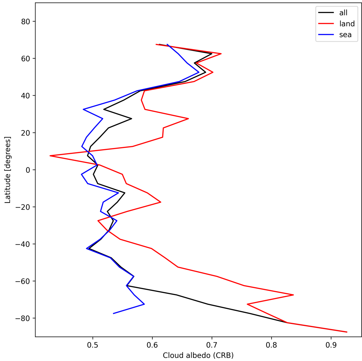
Figure 26: Zonal average of “Cloud albedo (CRB)” for 2025-01-08 to 2025-01-09.
