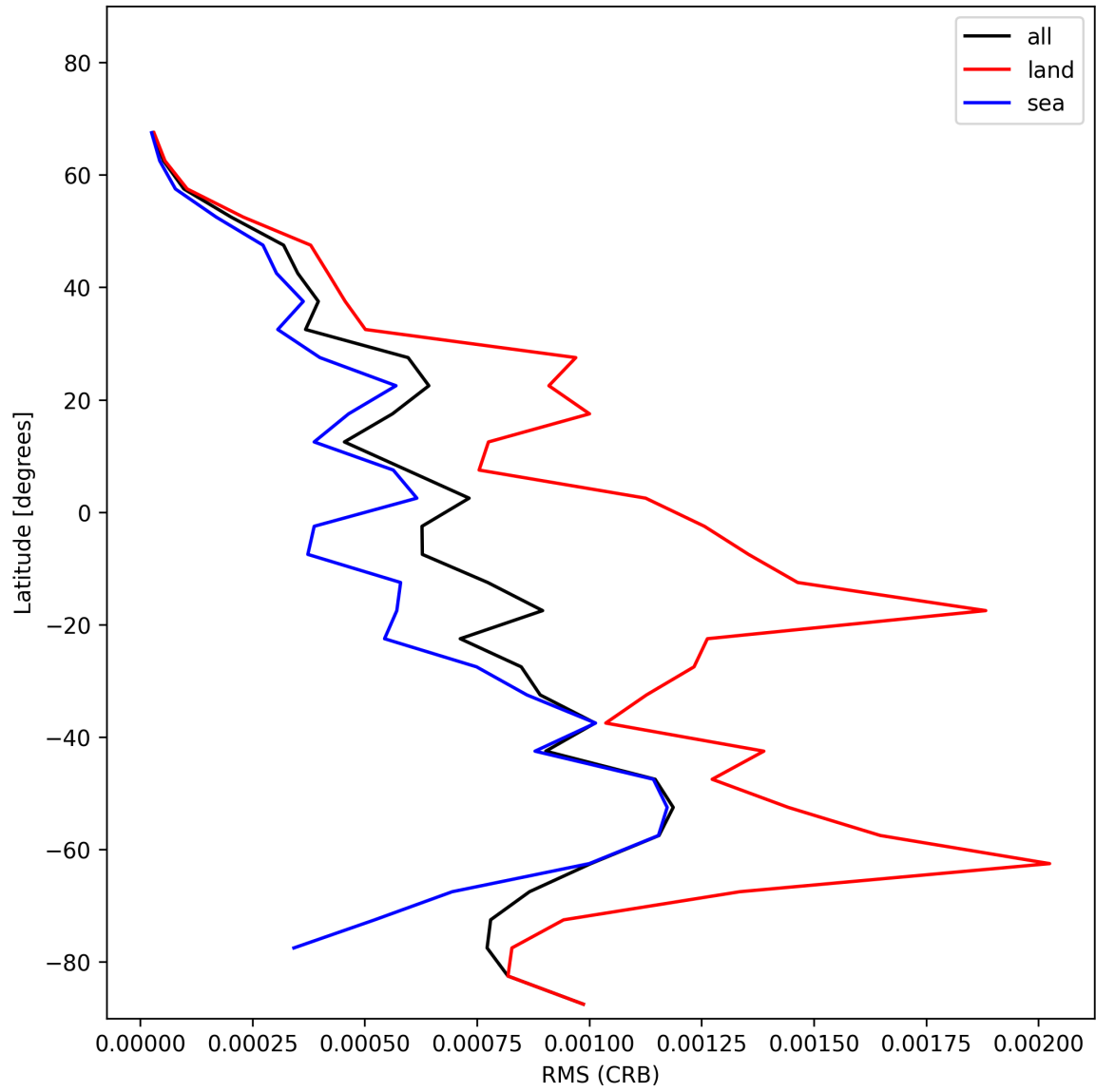
Figure 30: Zonal average of “RMS (CRB)” for 2025-01-08 to 2025-01-09.
