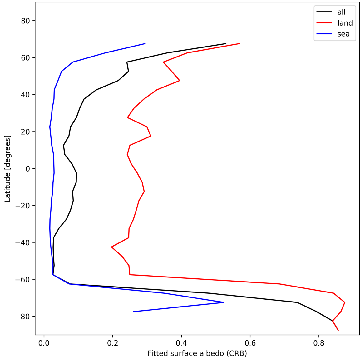
Figure 28: Zonal average of “Fitted surface albedo (CRB)” for 2025-01-08 to 2025-01-09.
