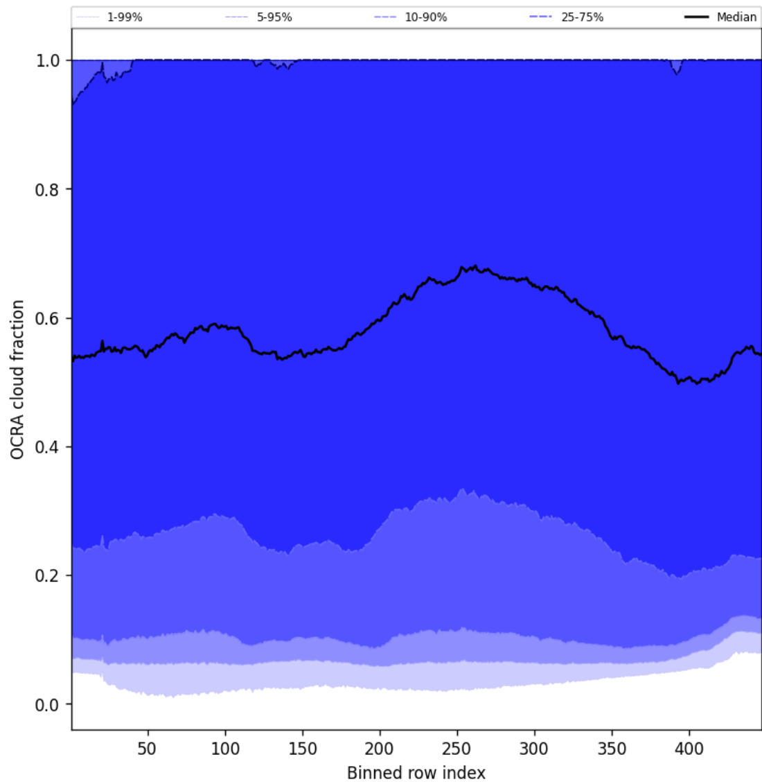
Figure 64: Along track statistics of “OCRA cloud fraction” for 2025-01-08 to 2025-01-09
