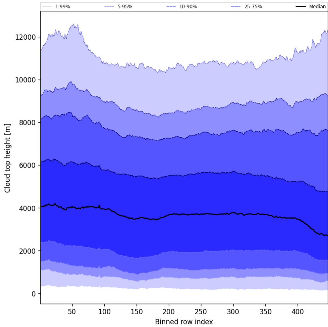
Figure 54: Along track statistics of “Cloud top height” for 2025-01-08 to 2025-01-09
