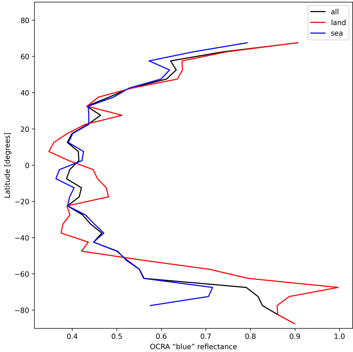
Figure 33: Zonal average of "OCRA "blue" reflectance" for 2025-01-08 to 2025-01-09.
