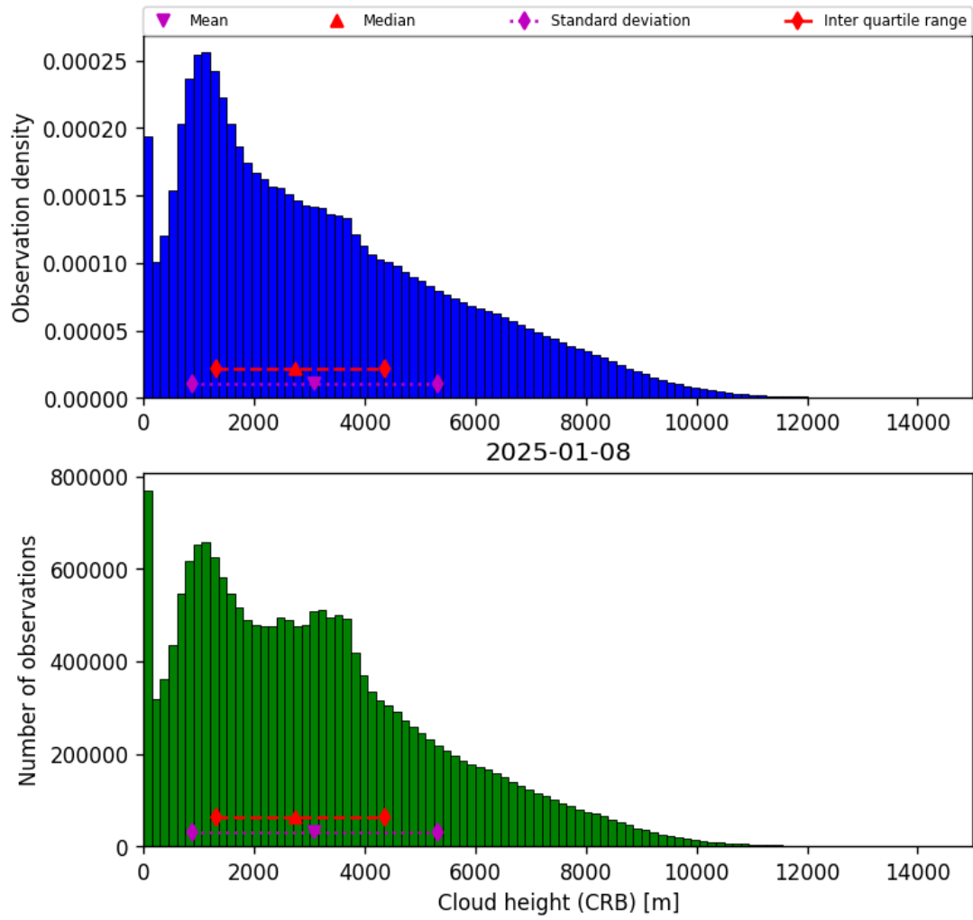
Figure 41: Histogram of “Cloud height (CRB)” for 2025-01-08 to 2025-01-09
