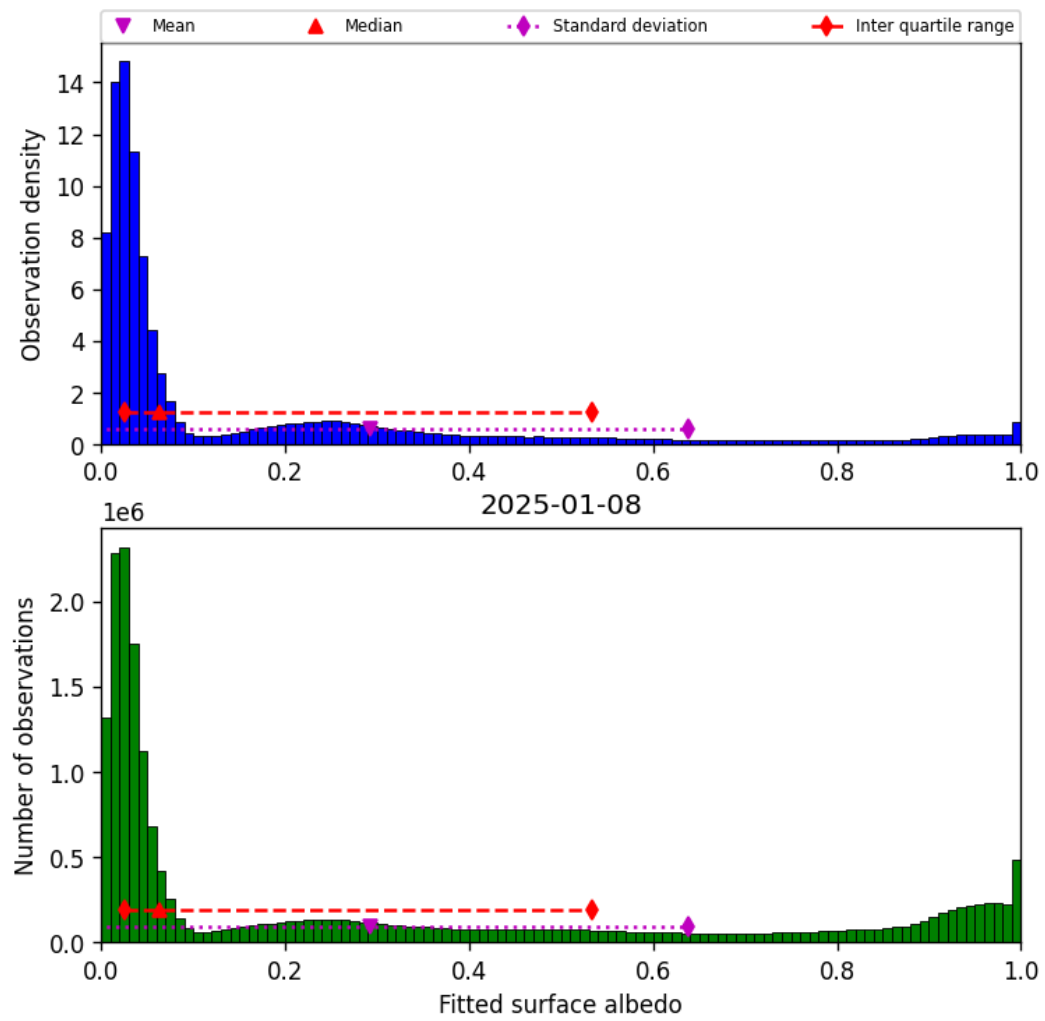
Figure 43: Histogram of “Fitted surface albedo” for 2025-01-08 to 2025-01-09
