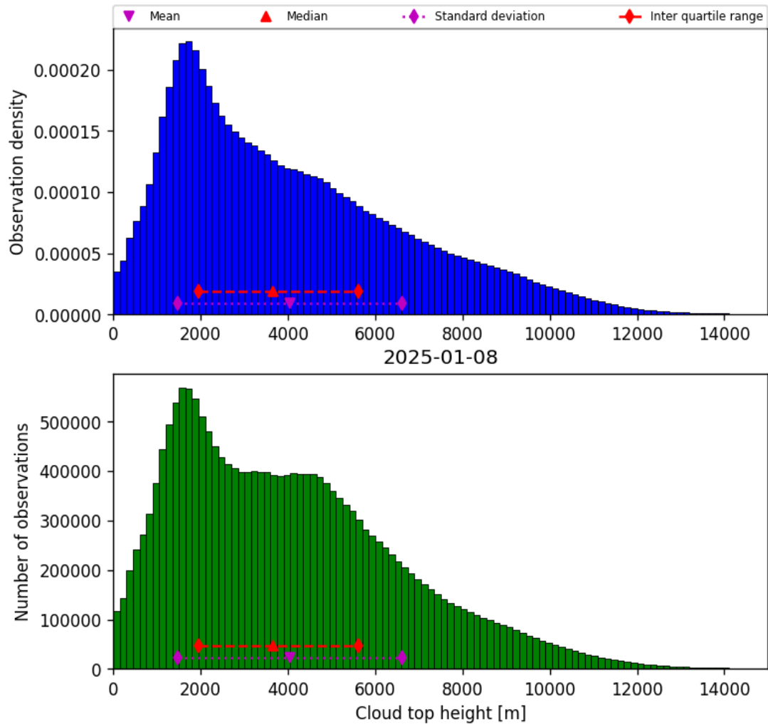
Figure 38: Histogram of “Cloud top height” for 2025-01-08 to 2025-01-09
