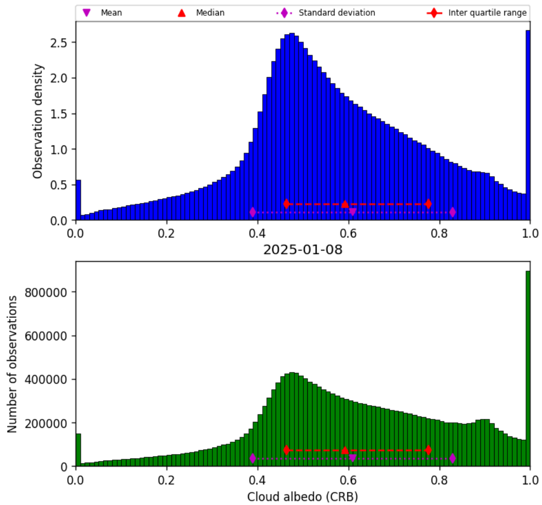
Figure 42: Histogram of “Cloud albedo (CRB)” for 2025-01-08 to 2025-01-09
