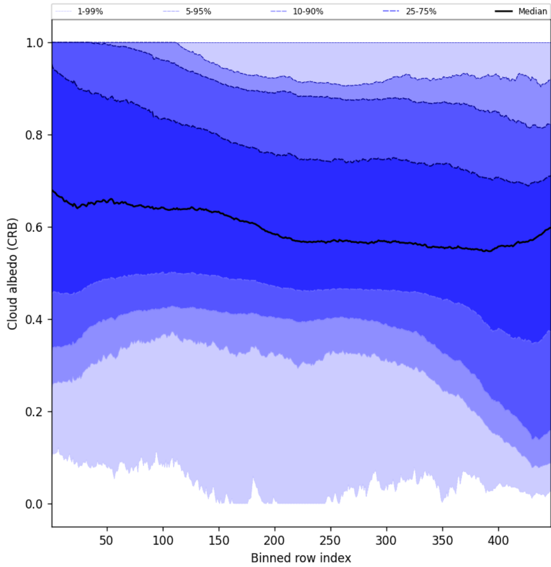
Figure 58: Along track statistics of “Cloud albedo (CRB)” for 2025-01-08 to 2025-01-09
