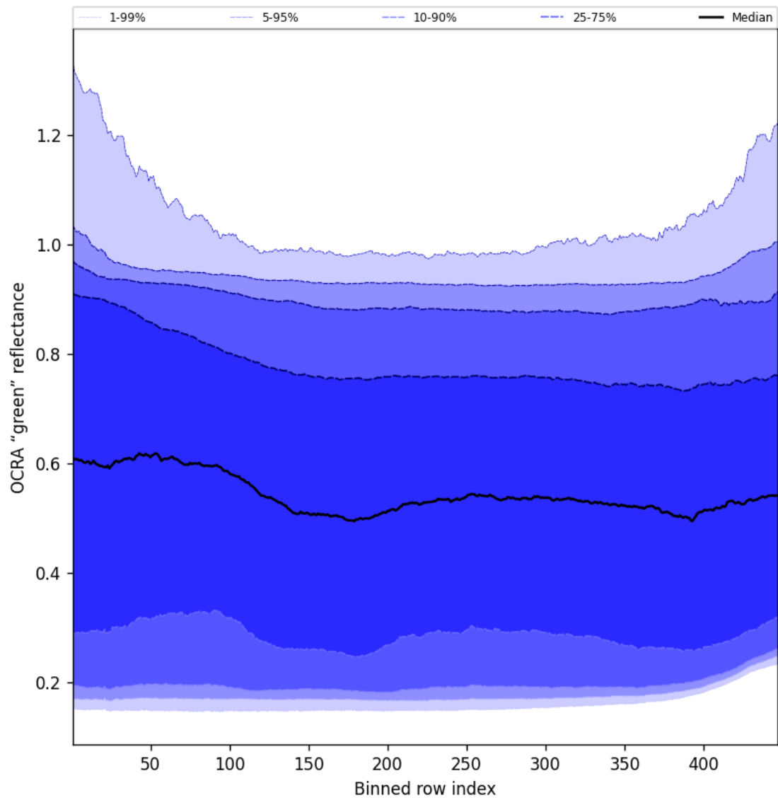
Figure 66: Along track statistics of “OCRA “green” reflectance” for 2025-01-08 to 2025-01-09
