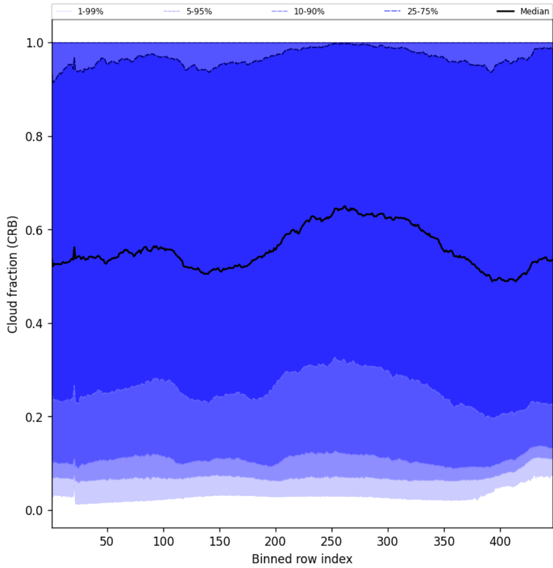
Figure 56: Along track statistics of “Cloud fraction (CRB)” for 2025-01-08 to 2025-01-09
