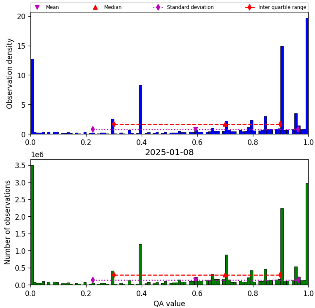
Figure 36: Histogram of “QA value” for 2025-01-08 to 2025-01-09
