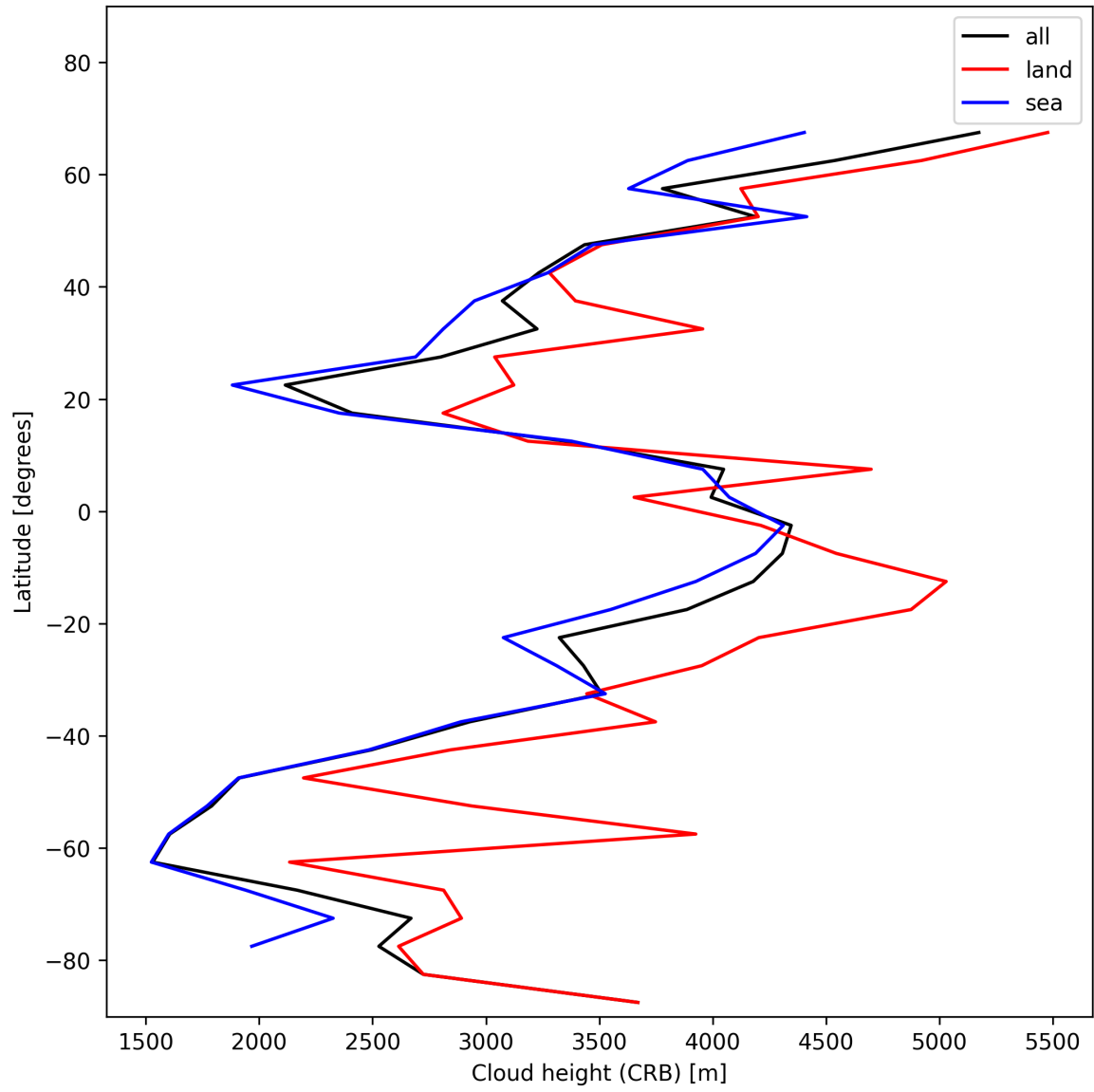
Figure 25: Zonal average of “Cloud height (CRB)” for 2025-01-08 to 2025-01-09.
