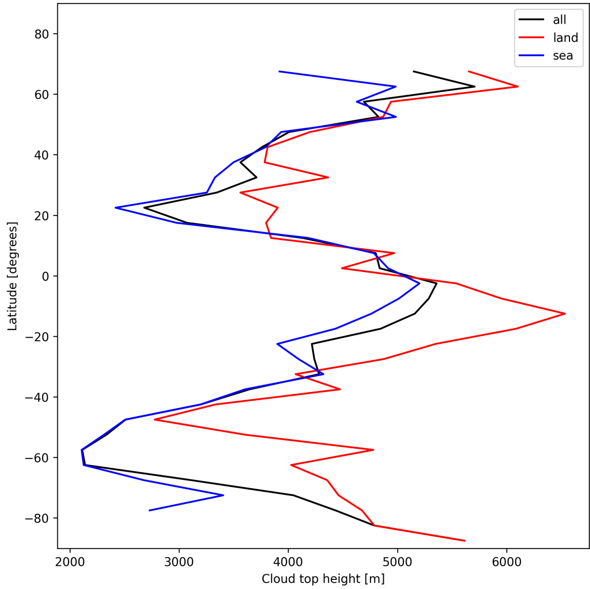
Figure 22: Zonal average of “Cloud top height” for 2025-01-08 to 2025-01-09.
