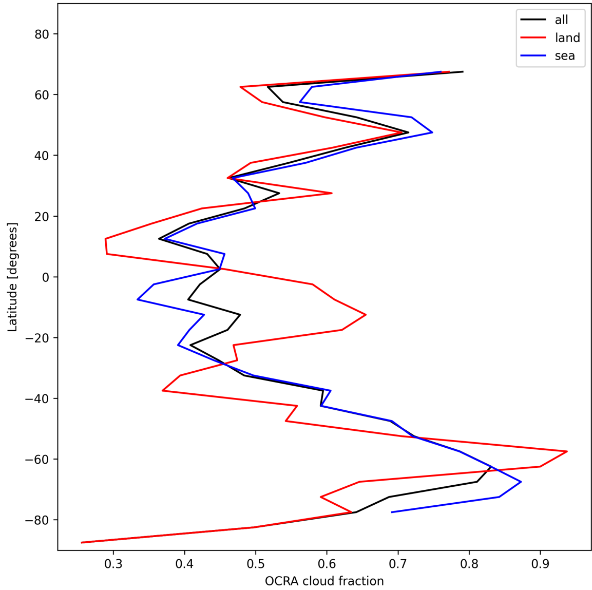
Figure 32: Zonal average of “OCRA cloud fraction” for 2025-01-08 to 2025-01-09.
