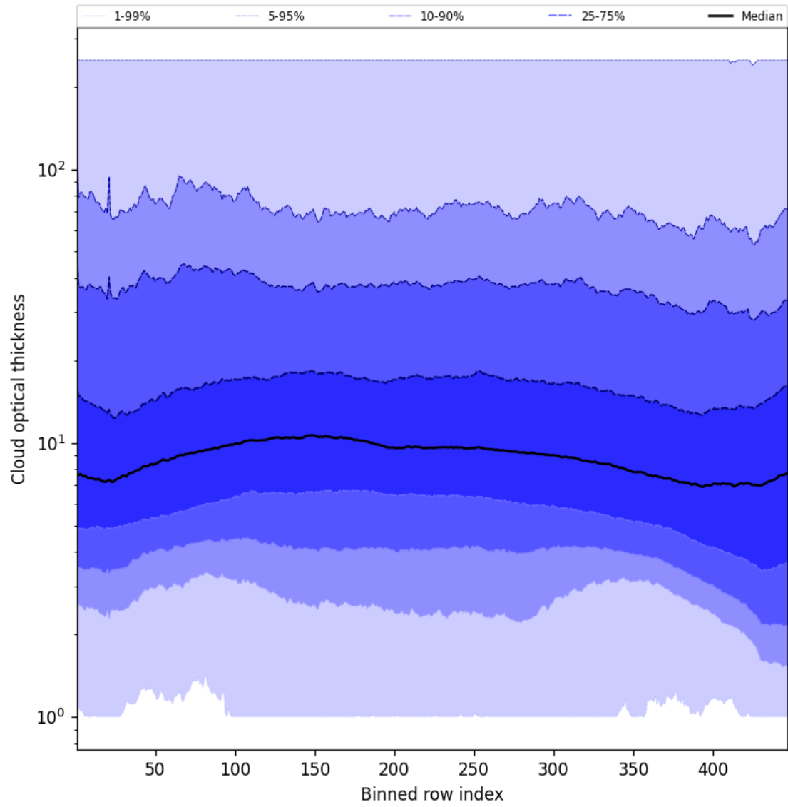
Figure 55: Along track statistics of “Cloud optical thickness” for 2025-01-08 to 2025-01-09
