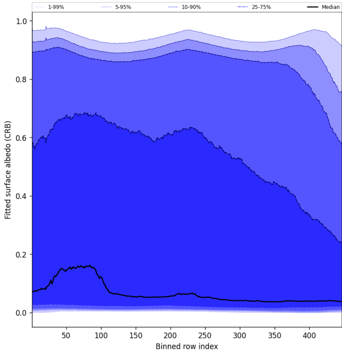
Figure 60: Along track statistics of “Fitted surface albedo (CRB)” for 2025-01-08 to 2025-01-09
