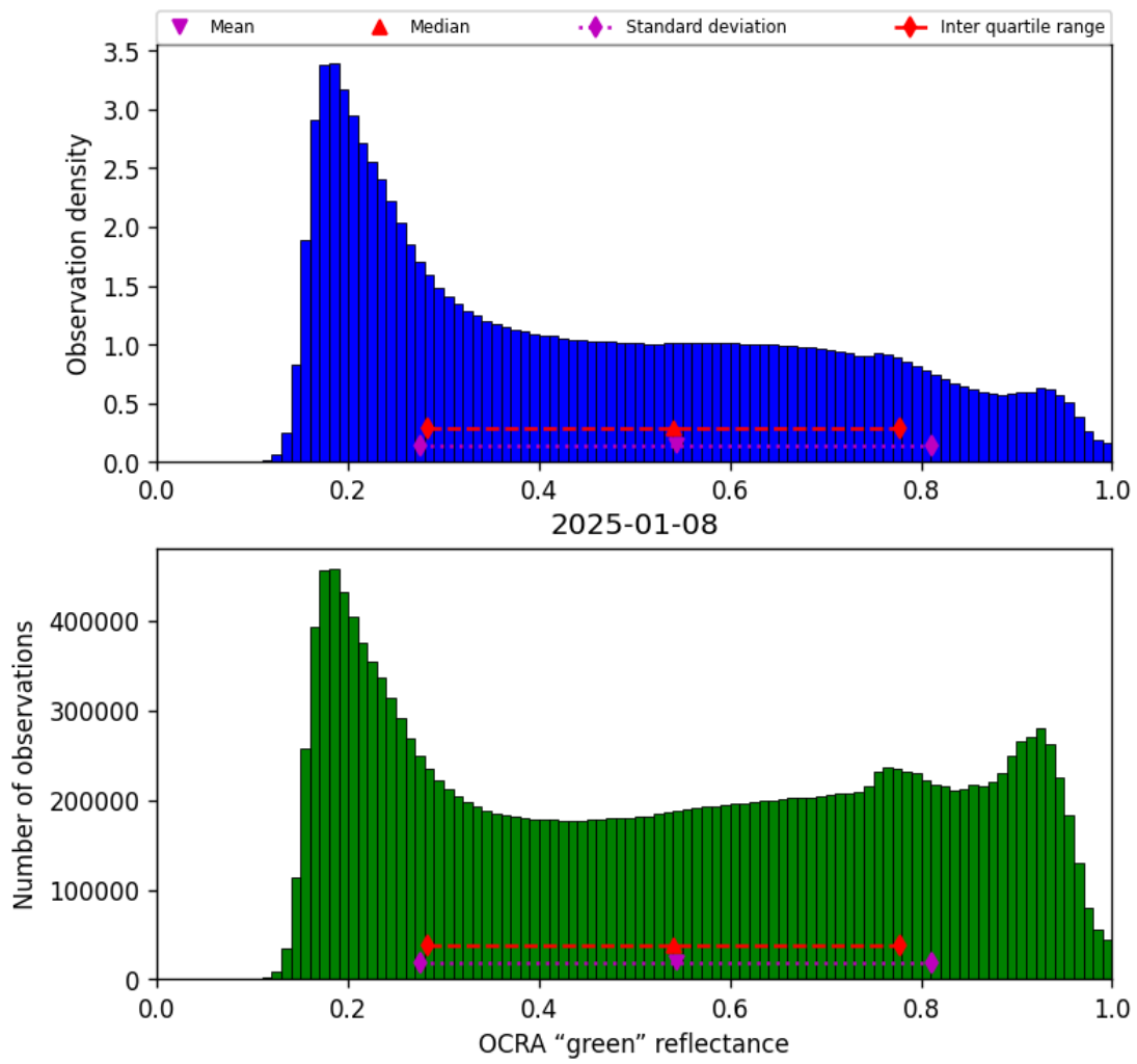
Figure 50: Histogram of “OCRA “green” reflectance” for 2025-01-08 to 2025-01-09
