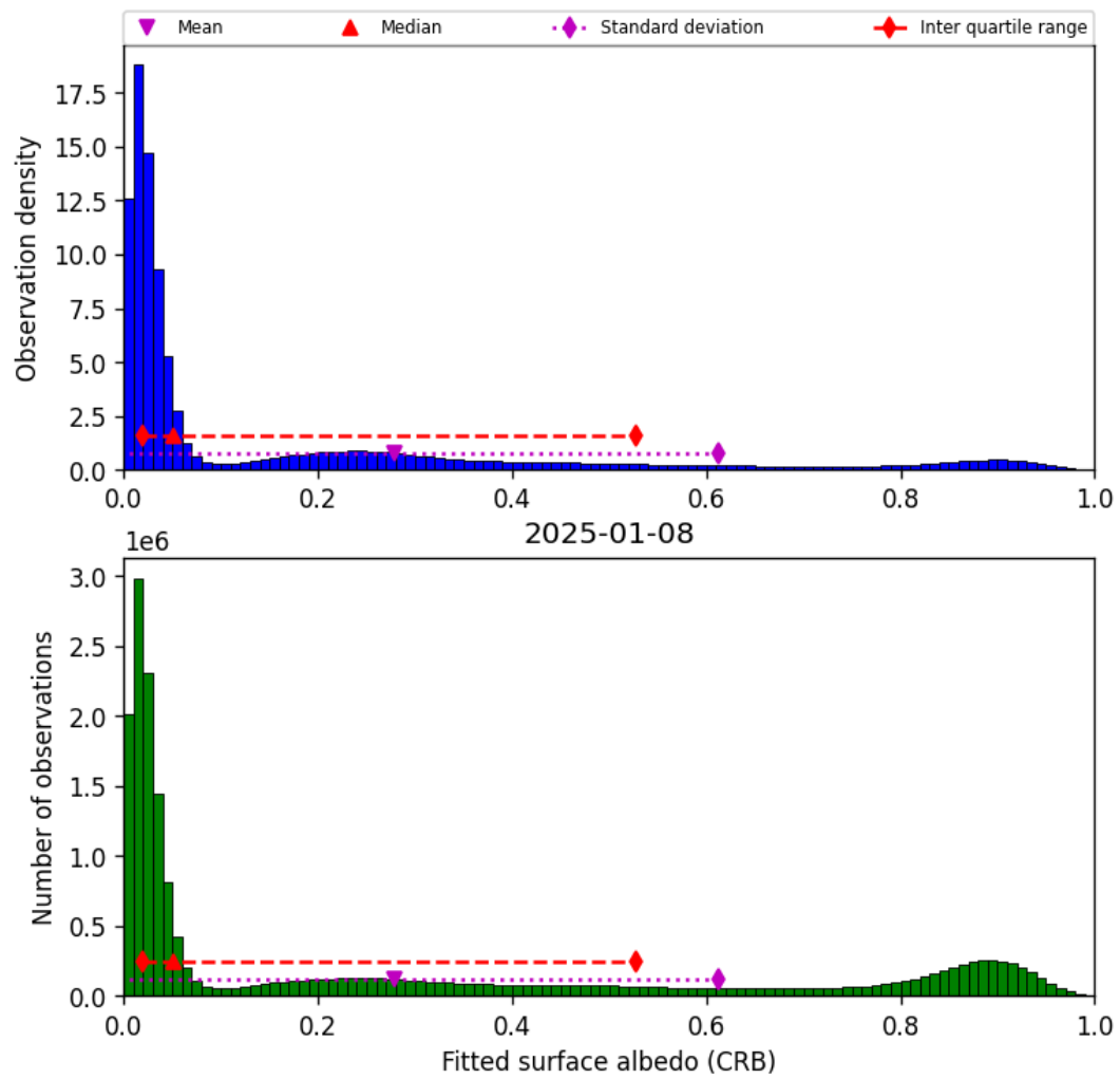
Figure 44: Histogram of “Fitted surface albedo (CRB)” for 2025-01-08 to 2025-01-09
