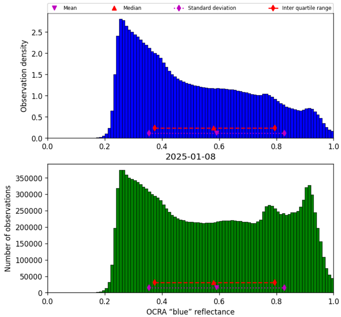
Figure 49: Histogram of “OCRA “blue” reflectance” for 2025-01-08 to 2025-01-09
