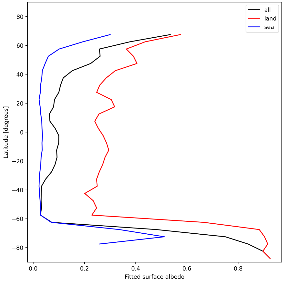
Figure 27: Zonal average of “Fitted surface albedo” for 2025-01-08 to 2025-01-09.
