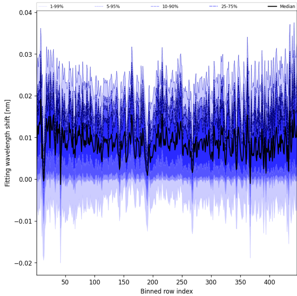
Figure 63: Along track statistics of “Fitting wavelength shift” for 2025-01-08 to 2025-01-09
