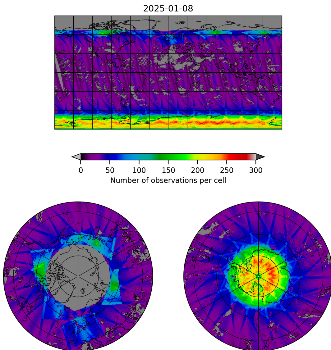
Figure 19: Map of the number of observations for 2025-01-08 to 2025-01-09
