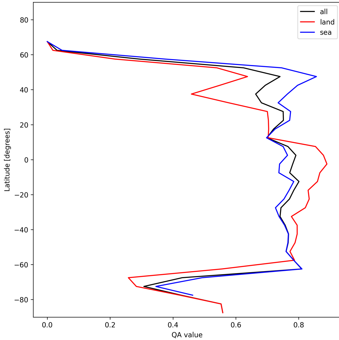
Figure 20: Zonal average of “QA value” for 2025-01-08 to 2025-01-09.
