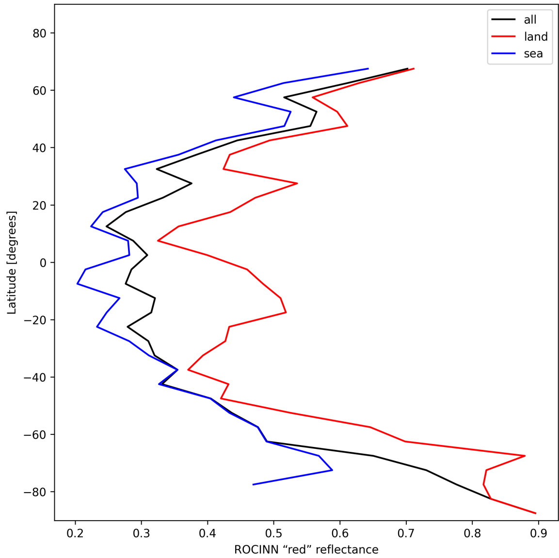
Figure 35: Zonal average of "ROCINN "red" reflectance" for 2025-01-08 to 2025-01-09.
