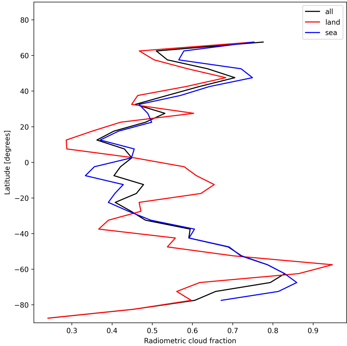
Figure 21: Zonal average of “Radiometric cloud fraction” for 2025-01-08 to 2025-01-09.
