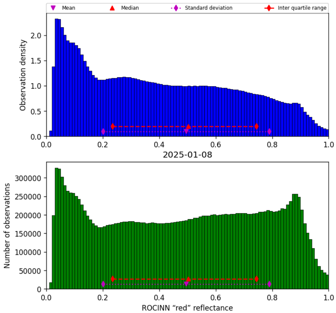
Figure 51: Histogram of “ROCINN “red” reflectance” for 2025-01-08 to 2025-01-09
