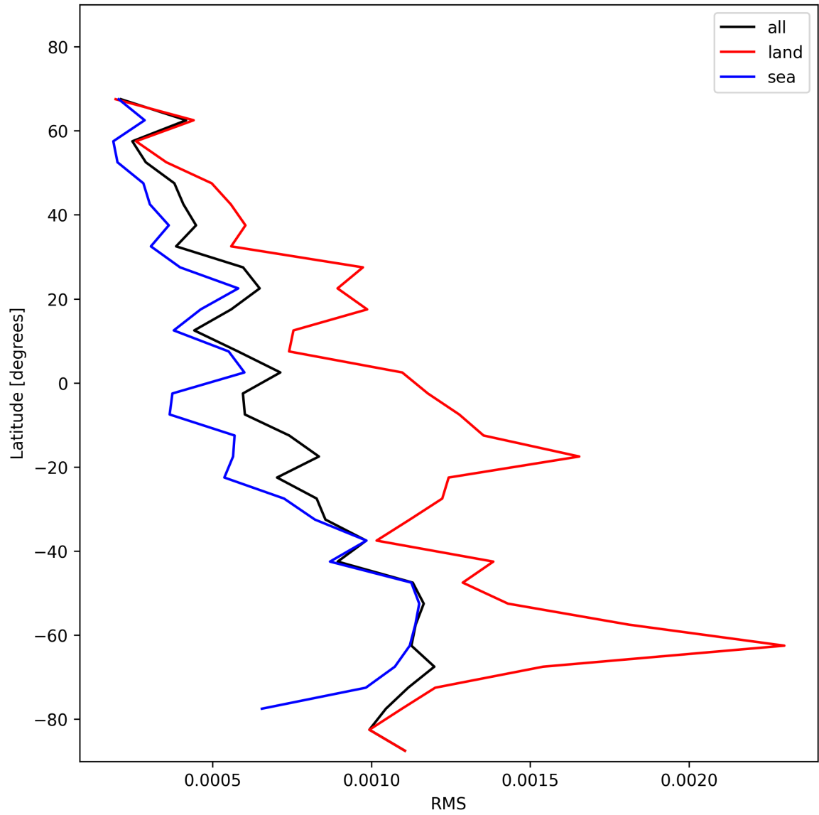
Figure 29: Zonal average of “RMS” for 2025-01-08 to 2025-01-09.
