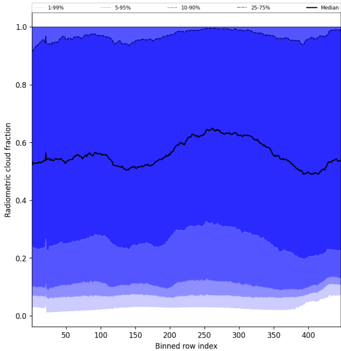
Figure 53: Along track statistics of “Radiometric cloud fraction” for 2025-01-08 to 2025-01-09
