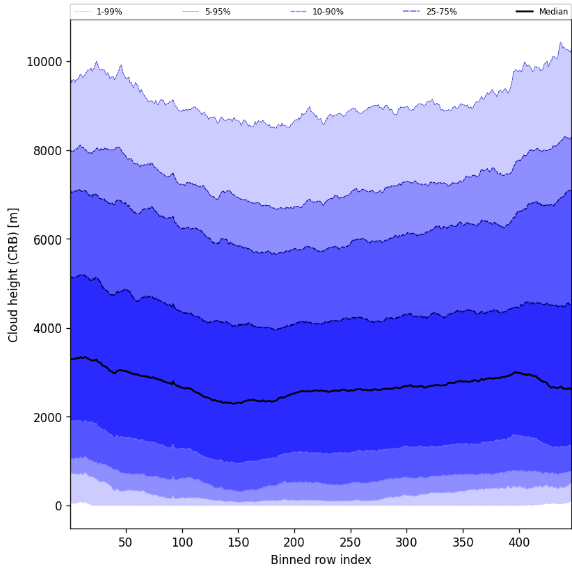
Figure 57: Along track statistics of “Cloud height (CRB)” for 2025-01-08 to 2025-01-09
