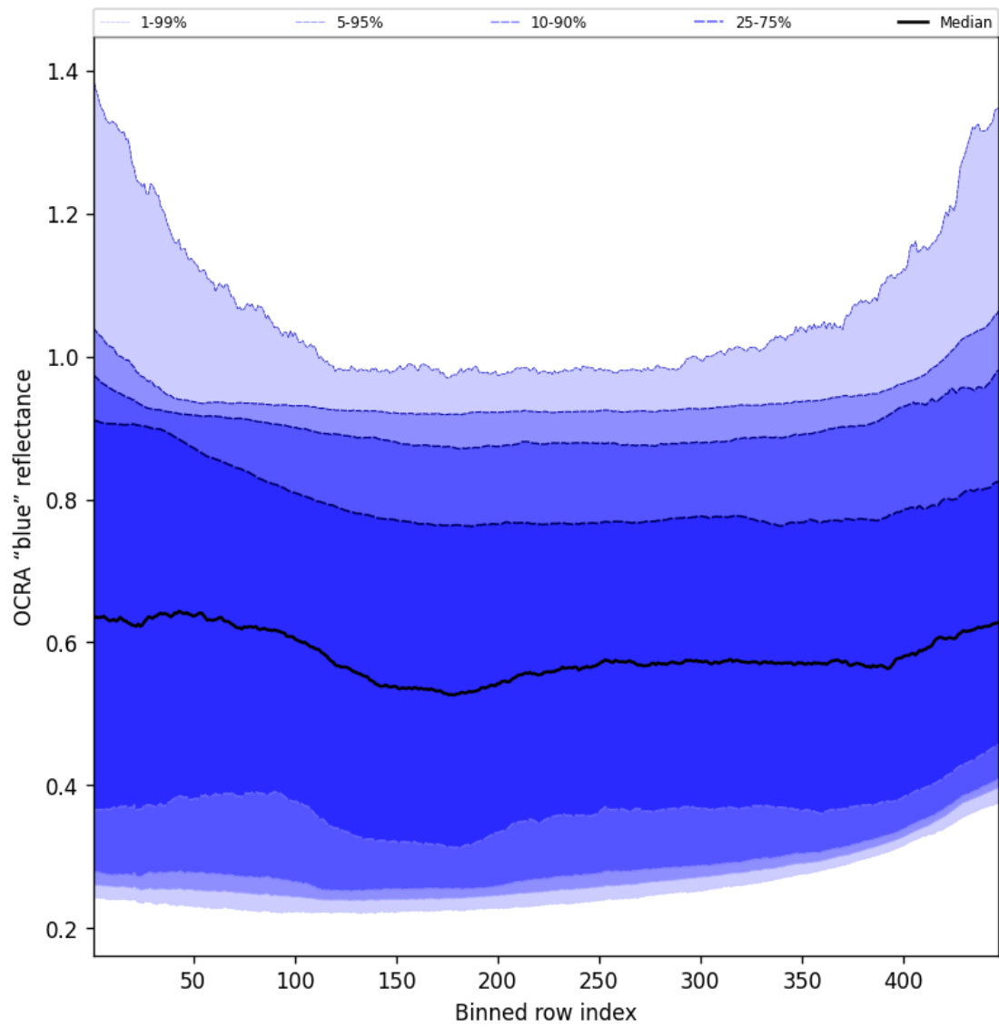
Figure 65: Along track statistics of “OCRA “blue” reflectance” for 2025-01-08 to 2025-01-09
