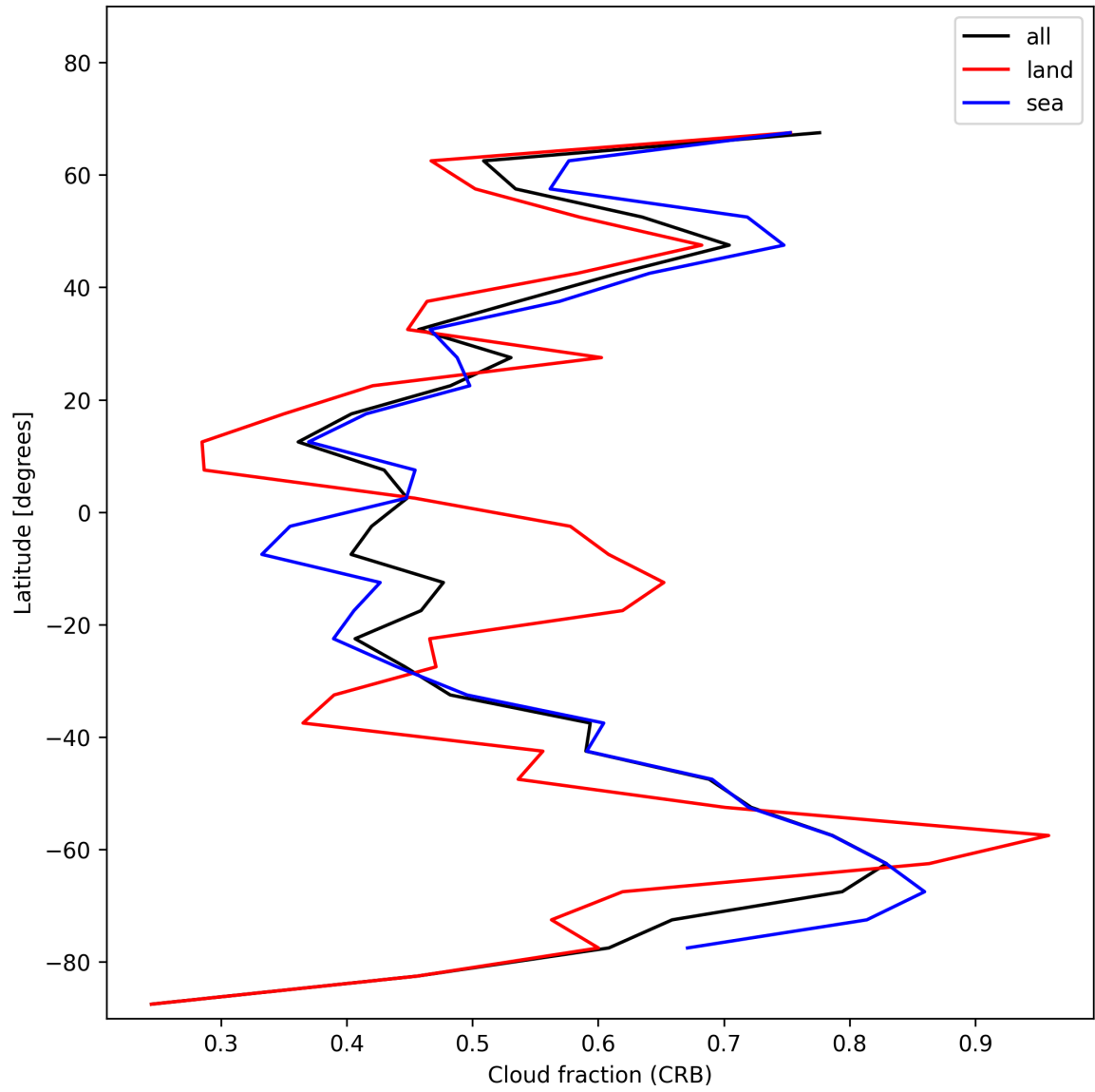
Figure 24: Zonal average of “Cloud fraction (CRB)” for 2025-01-08 to 2025-01-09.
