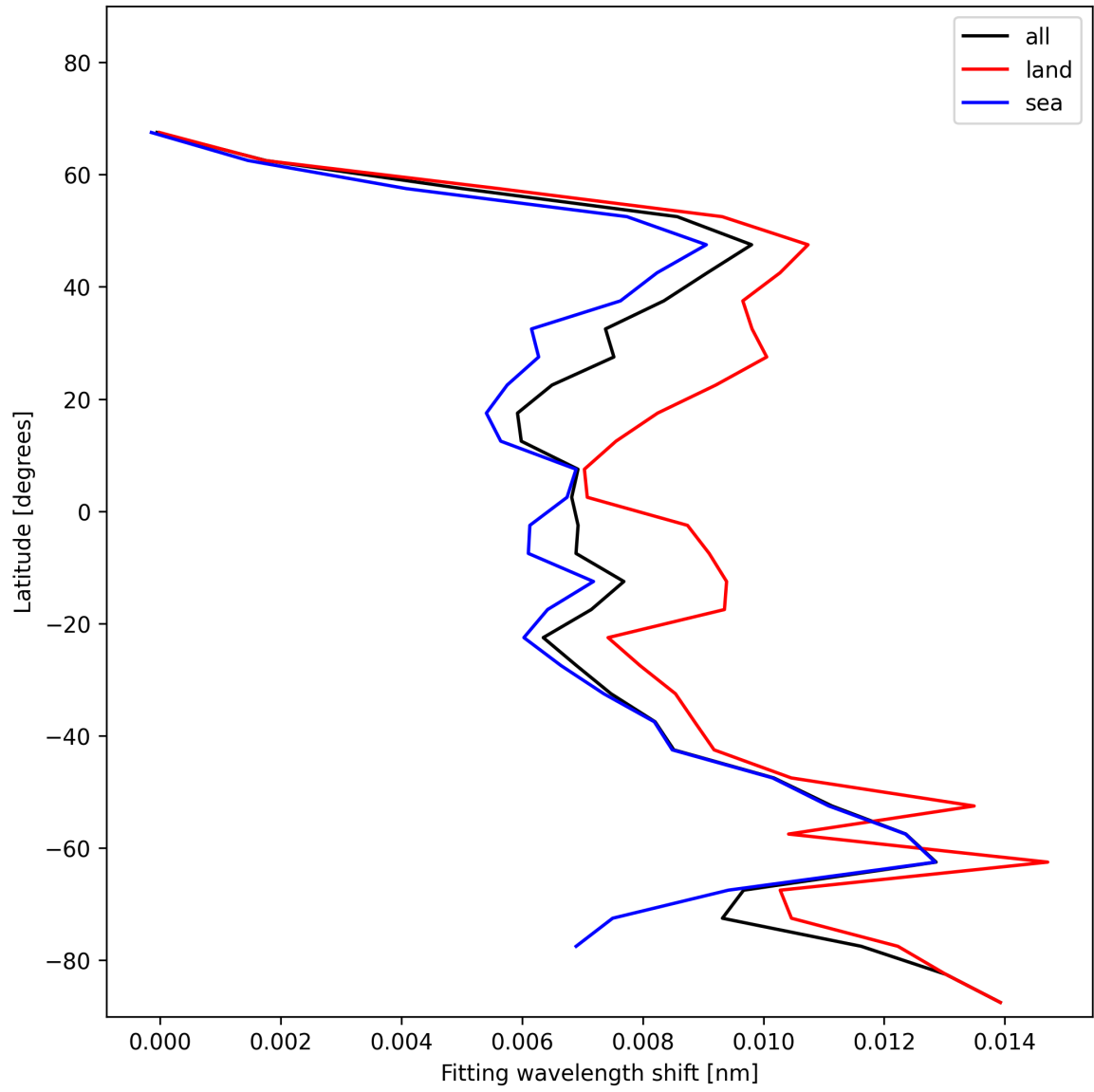
Figure 31: Zonal average of “Fitting wavelength shift” for 2025-01-08 to 2025-01-09.
