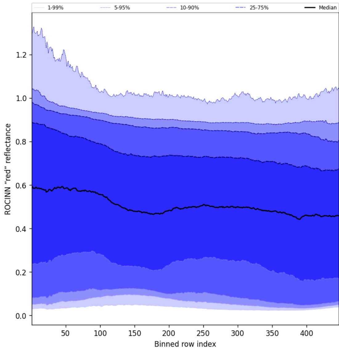
Figure 67: Along track statistics of “ROCINN “red” reflectance” for 2025-01-08 to 2025-01-09
