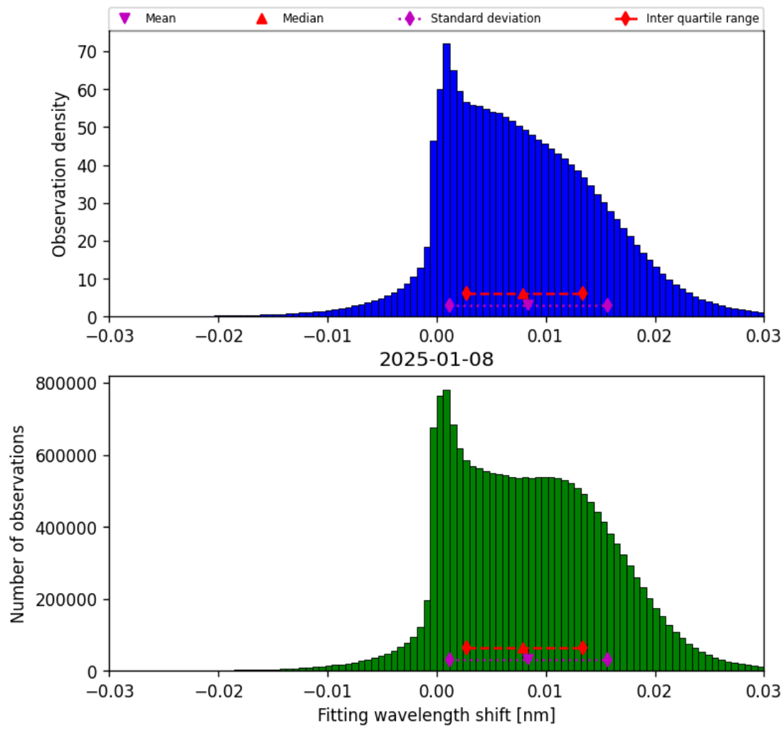
Figure 47: Histogram of “Fitting wavelength shift” for 2025-01-08 to 2025-01-09
