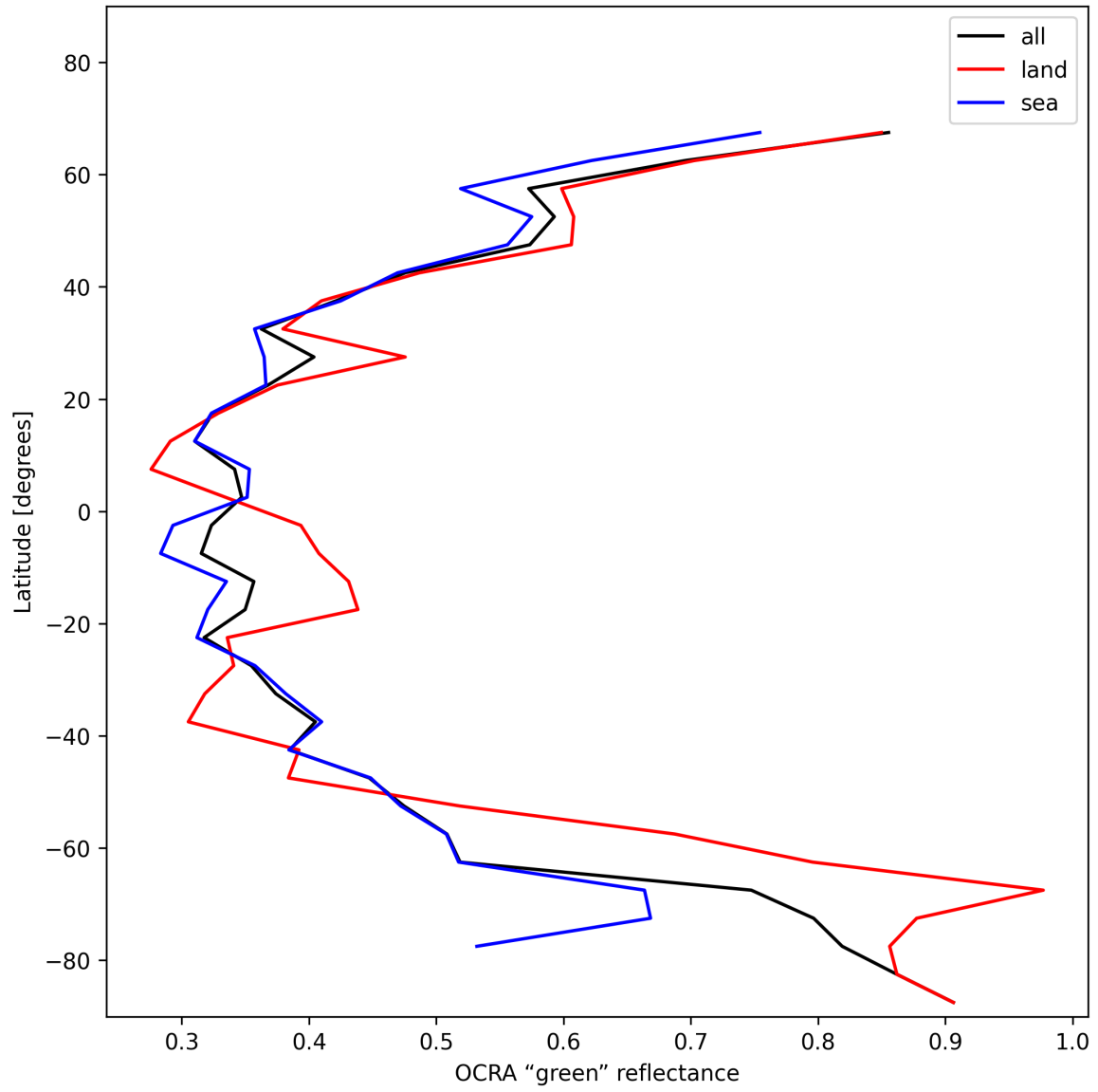
Figure 34: Zonal average of “OCRA “green” reflectance” for 2025-01-08 to 2025-01-09.
