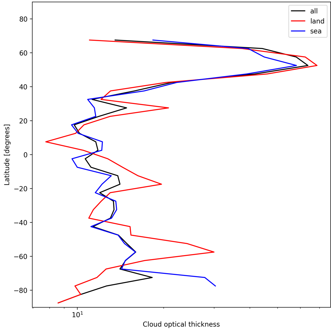
Figure 23: Zonal average of “Cloud optical thickness” for 2025-01-08 to 2025-01-09.
