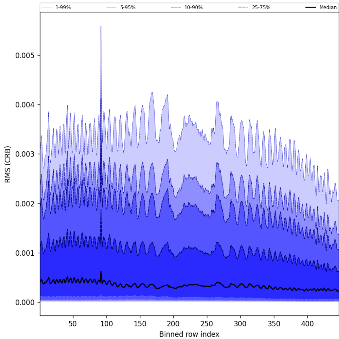
Figure 62: Along track statistics of “RMS (CRB)” for 2025-01-08 to 2025-01-09
