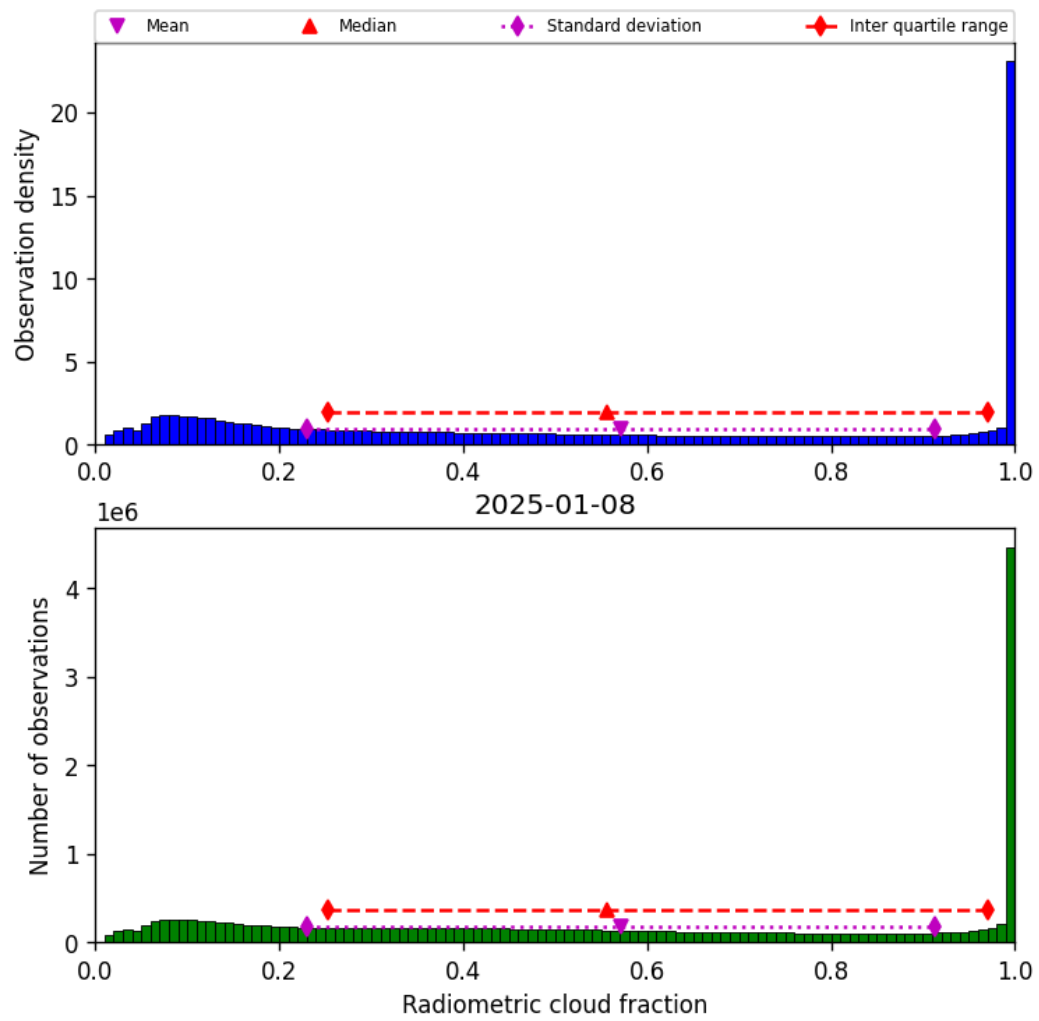
Figure 37: Histogram of “Radiometric cloud fraction” for 2025-01-08 to 2025-01-09
