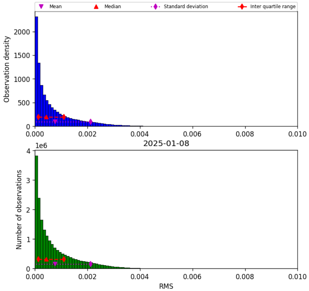
Figure 45: Histogram of “RMS” for 2025-01-08 to 2025-01-09
