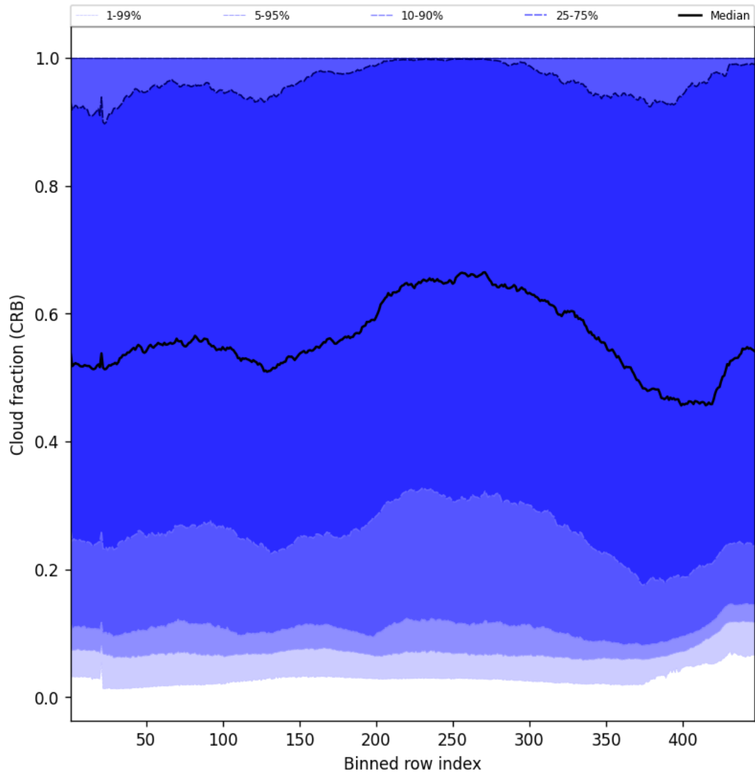
Figure 56: Along track statistics of “Cloud fraction (CRB)” for 2025-01-09 to 2025-01-10
