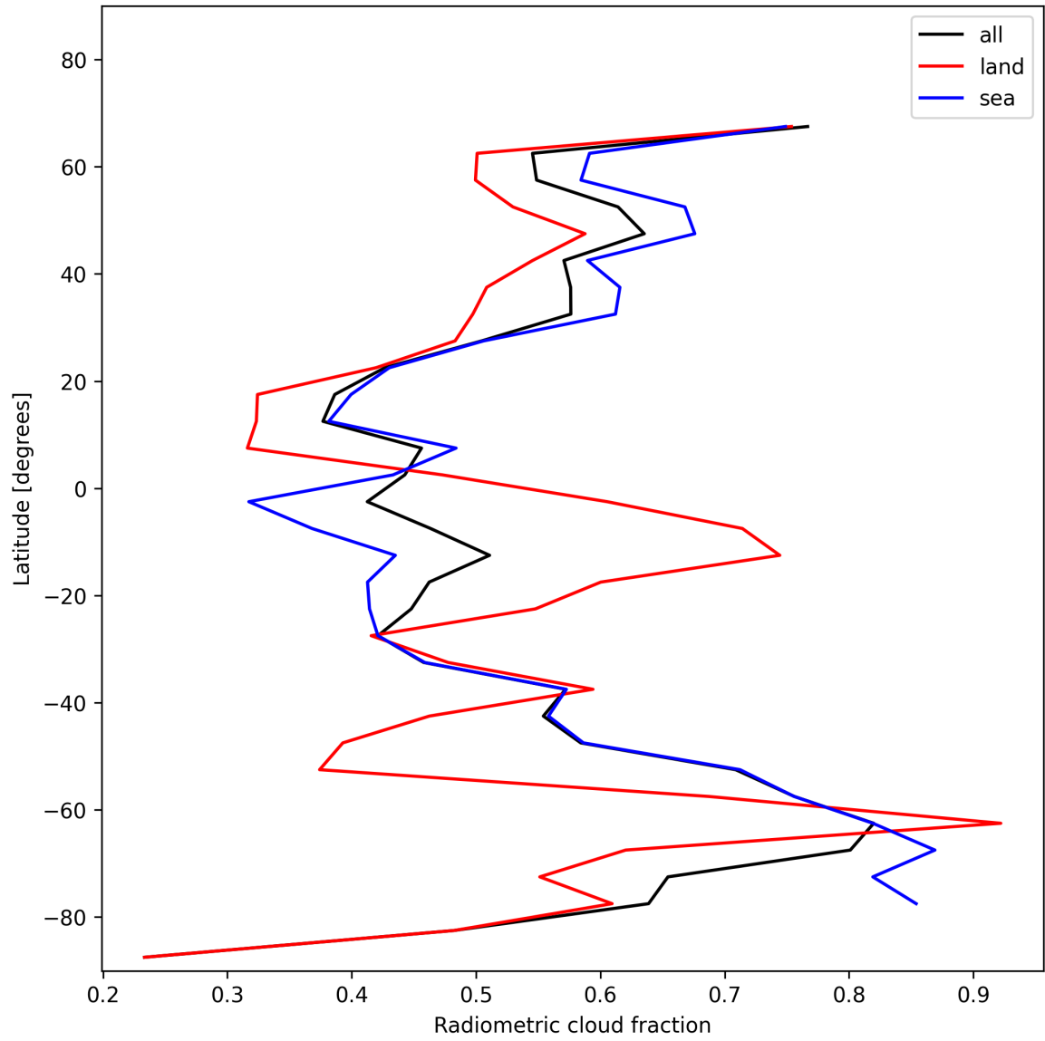
Figure 21: Zonal average of “Radiometric cloud fraction” for 2025-01-09 to 2025-01-10.
