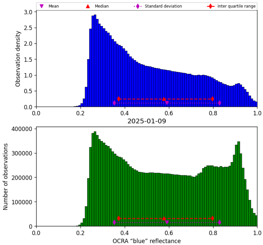
Figure 49: Histogram of “OCRA “blue” reflectance” for 2025-01-09 to 2025-01-10
