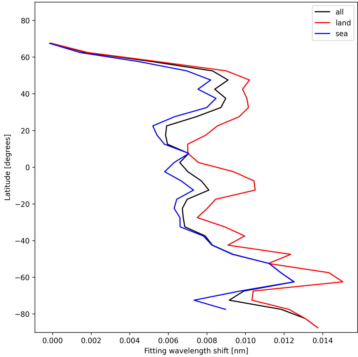
Figure 31: Zonal average of “Fitting wavelength shift” for 2025-01-09 to 2025-01-10.
