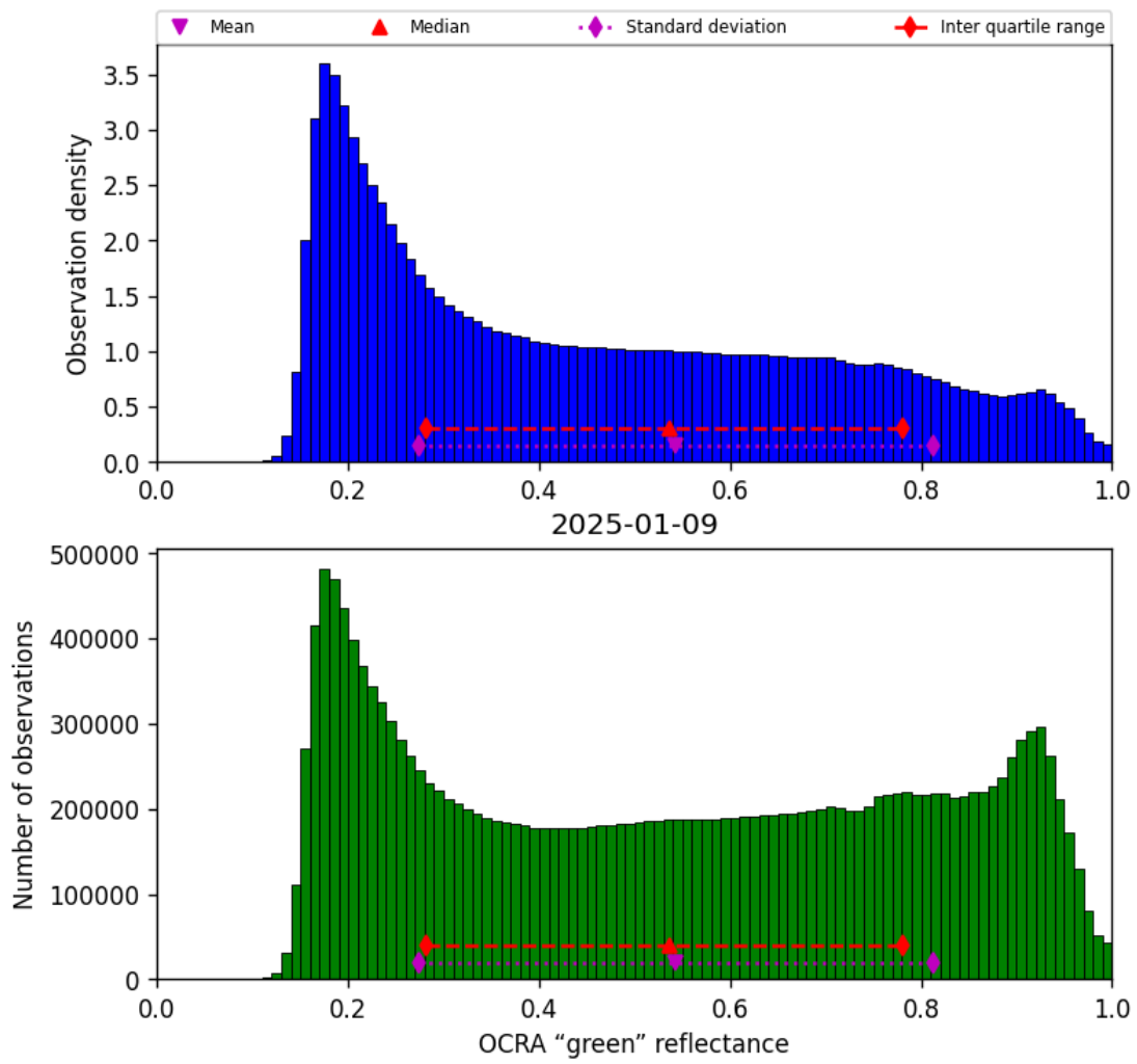
Figure 50: Histogram of “OCRA “green” reflectance” for 2025-01-09 to 2025-01-10
