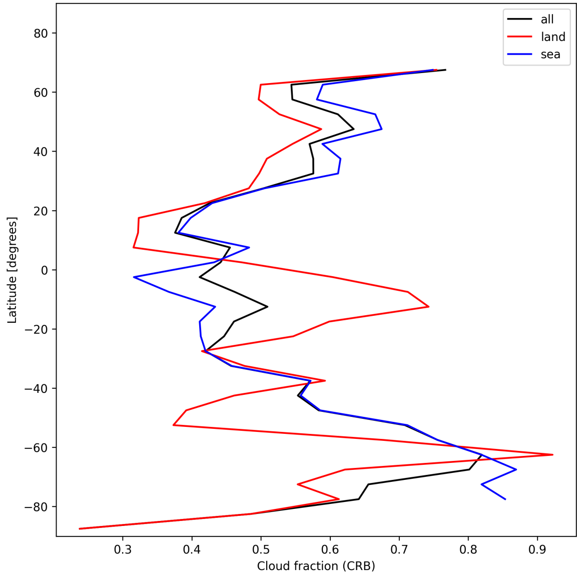
Figure 24: Zonal average of “Cloud fraction (CRB)” for 2025-01-09 to 2025-01-10.
