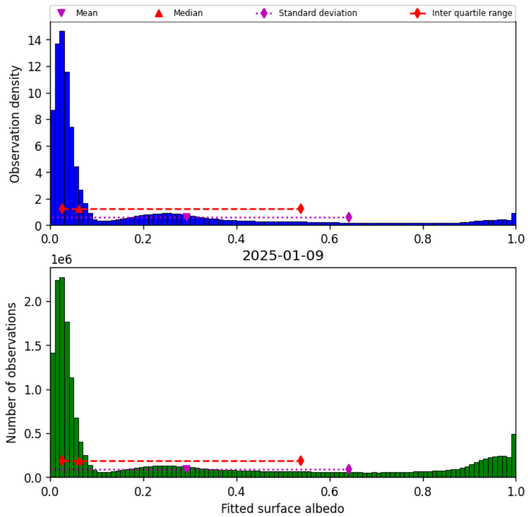
Figure 43: Histogram of “Fitted surface albedo” for 2025-01-09 to 2025-01-10
