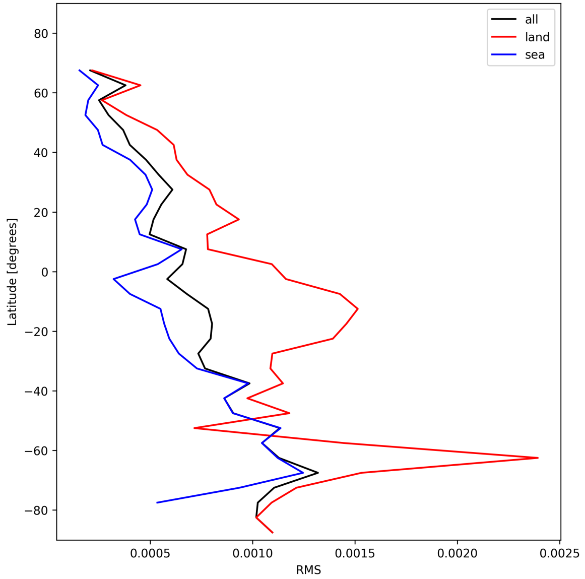
Figure 29: Zonal average of “RMS” for 2025-01-09 to 2025-01-10.
