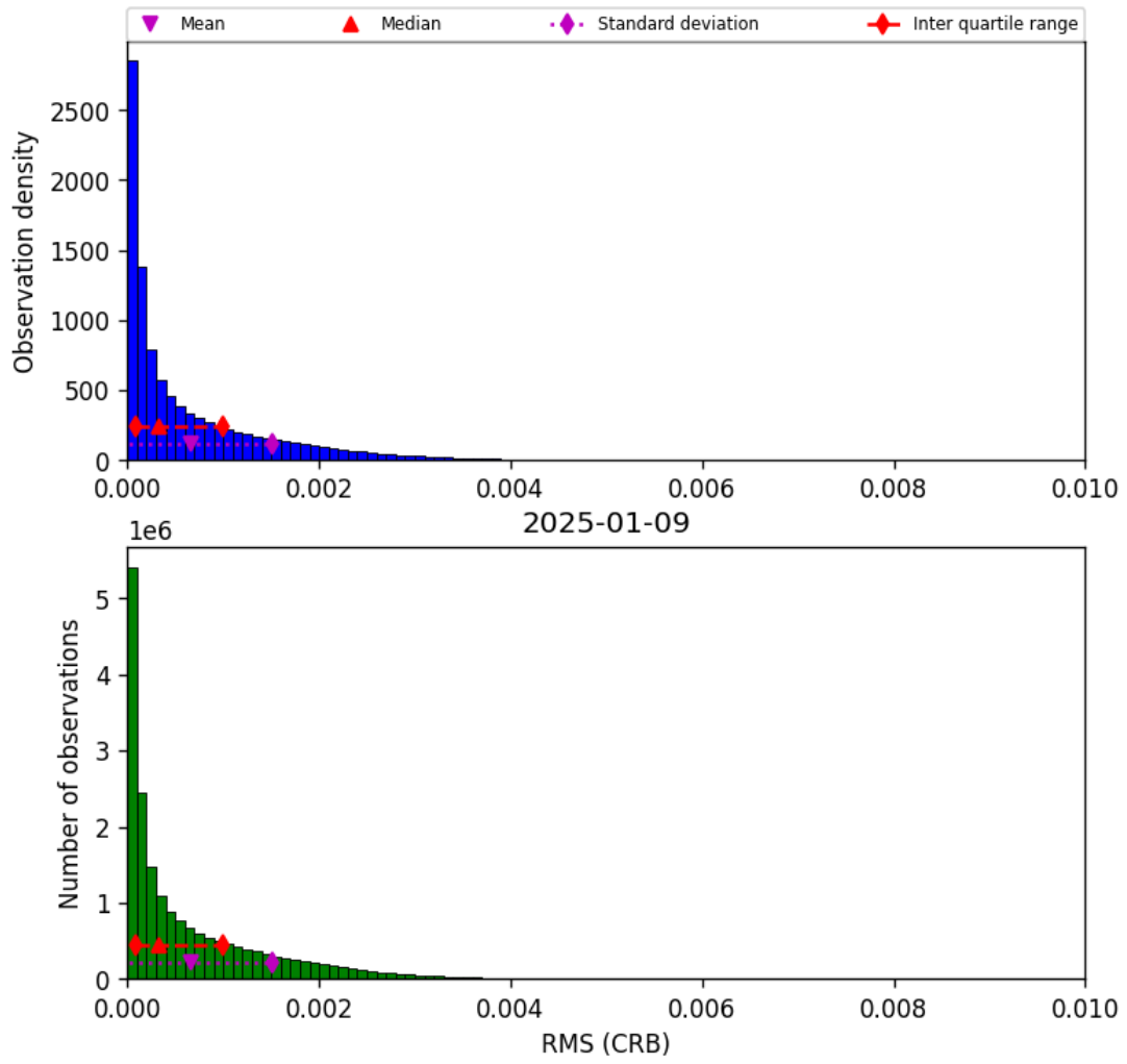
Figure 46: Histogram of “RMS (CRB)” for 2025-01-09 to 2025-01-10
