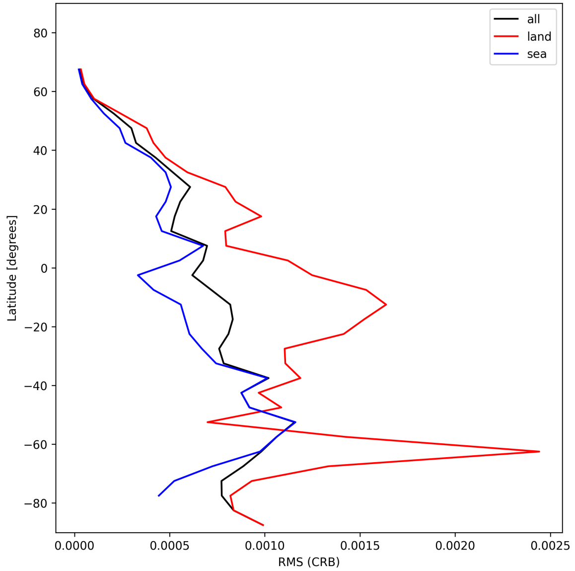
Figure 30: Zonal average of “RMS (CRB)” for 2025-01-09 to 2025-01-10.
