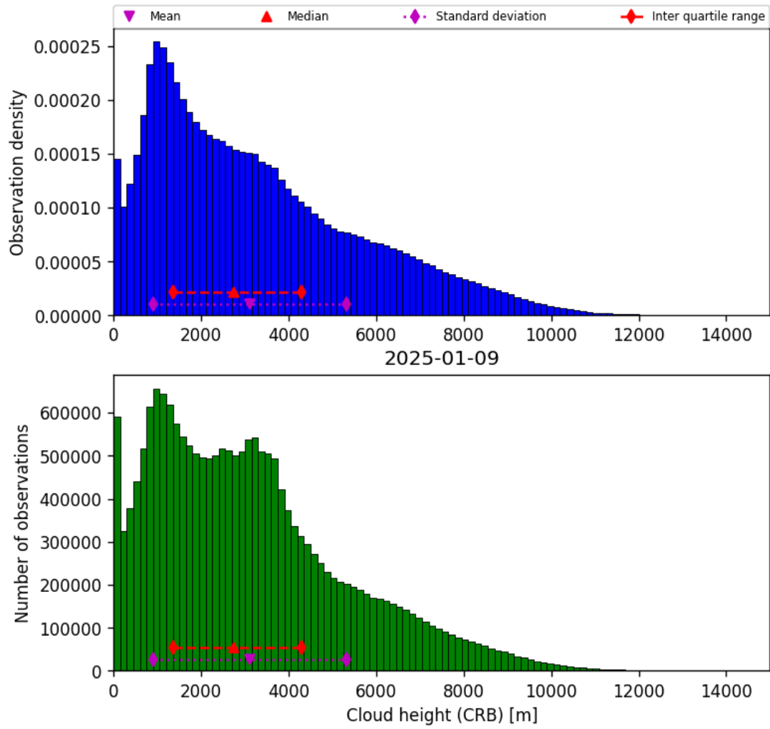
Figure 41: Histogram of “Cloud height (CRB)” for 2025-01-09 to 2025-01-10
