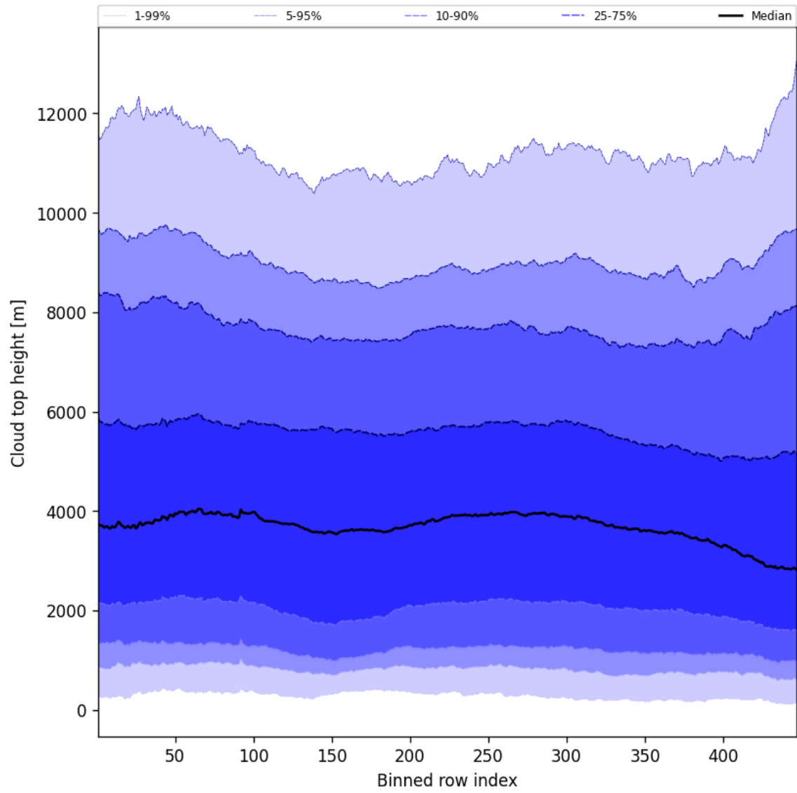
Figure 54: Along track statistics of “Cloud top height” for 2025-01-09 to 2025-01-10
