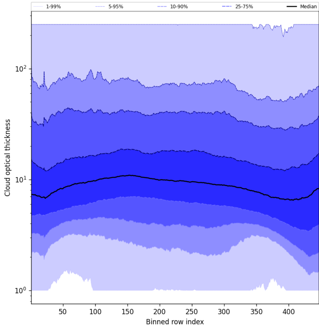
Figure 55: Along track statistics of “Cloud optical thickness” for 2025-01-09 to 2025-01-10
