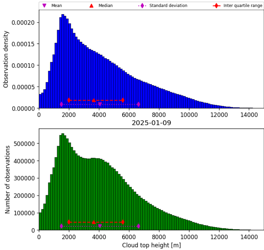
Figure 38: Histogram of “Cloud top height” for 2025-01-09 to 2025-01-10
