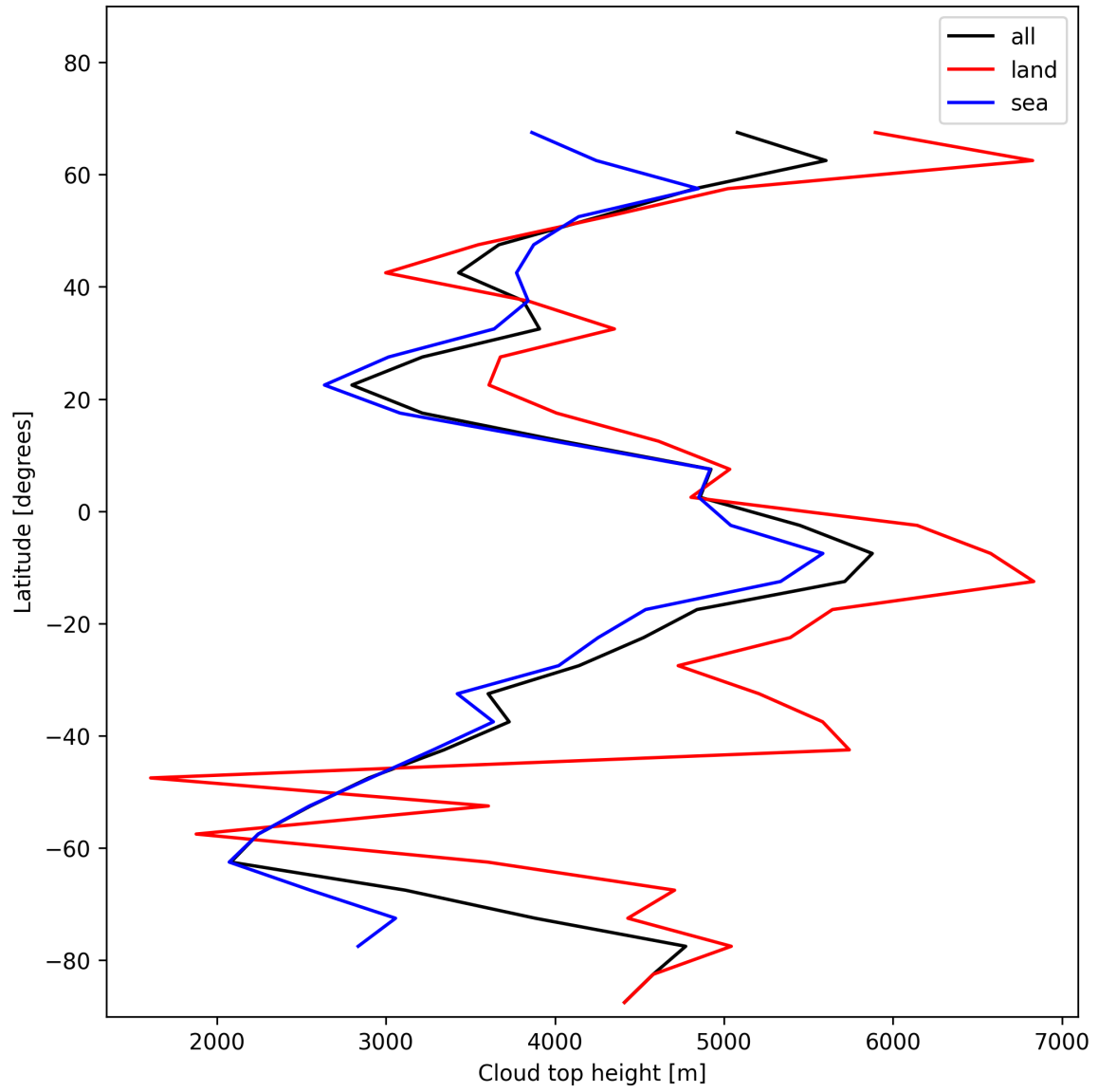
Figure 22: Zonal average of “Cloud top height” for 2025-01-09 to 2025-01-10.
