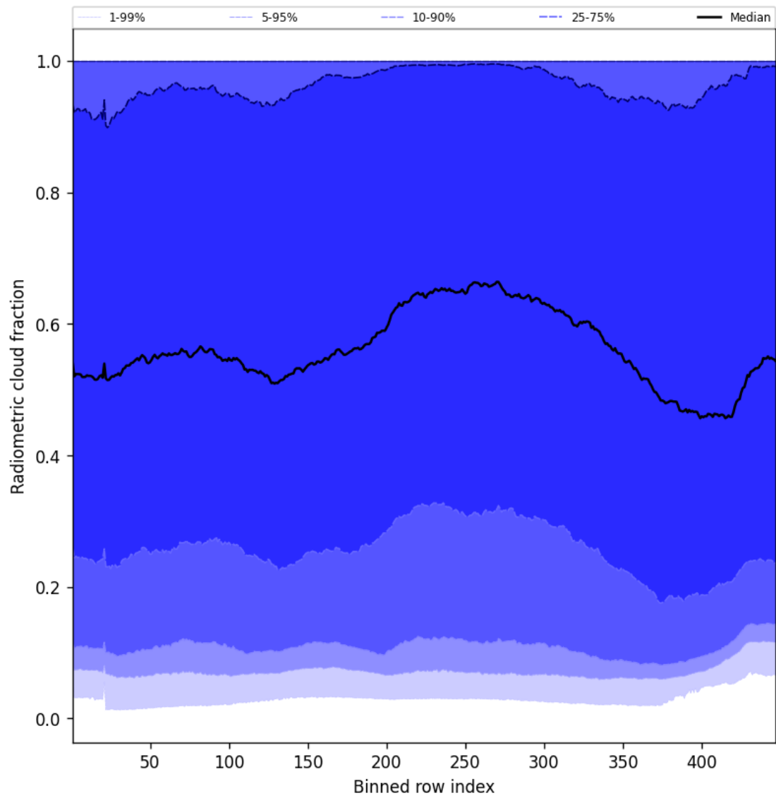
Figure 53: Along track statistics of “Radiometric cloud fraction” for 2025-01-09 to 2025-01-10
