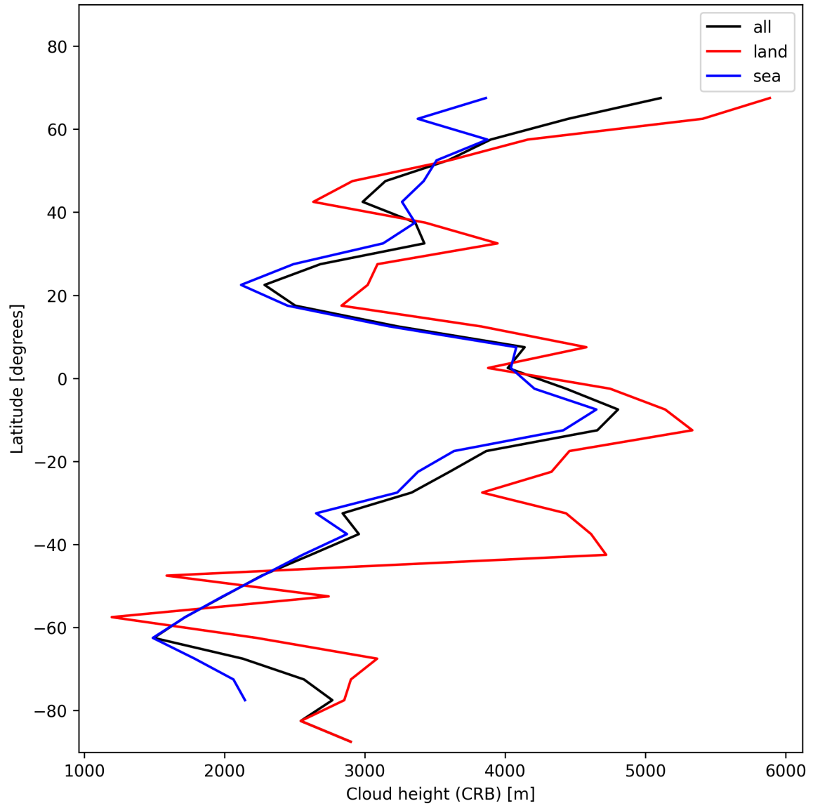
Figure 25: Zonal average of “Cloud height (CRB)” for 2025-01-09 to 2025-01-10.
