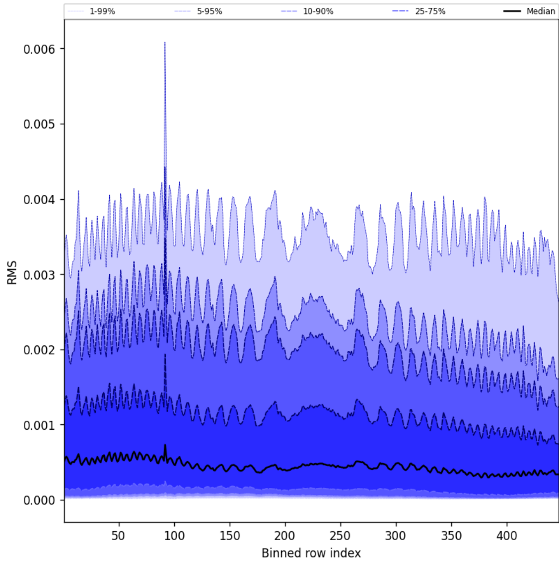
Figure 61: Along track statistics of “RMS” for 2025-01-09 to 2025-01-10
