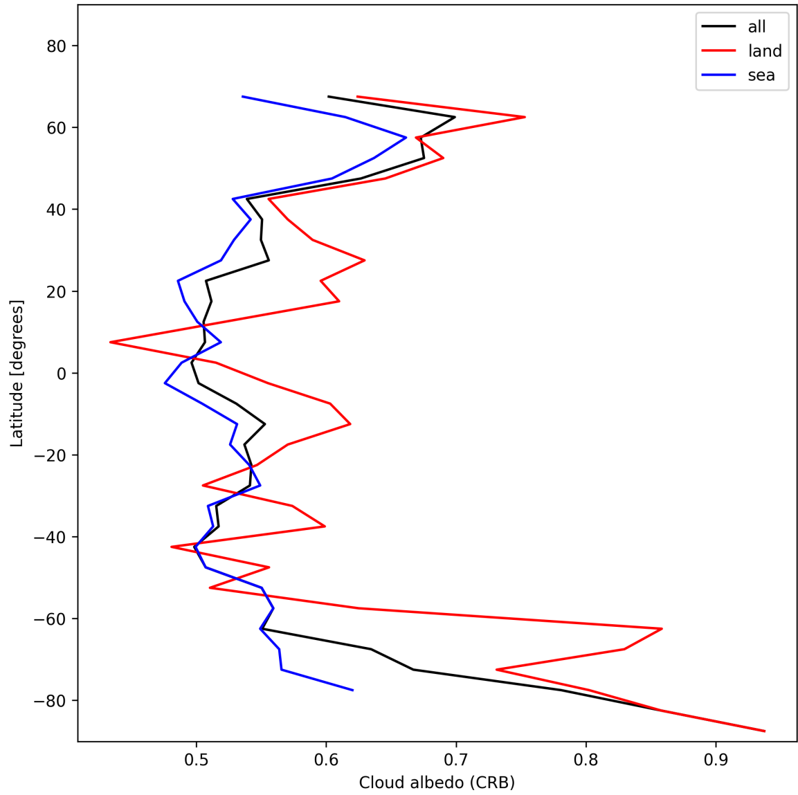
Figure 26: Zonal average of “Cloud albedo (CRB)” for 2025-01-09 to 2025-01-10.
