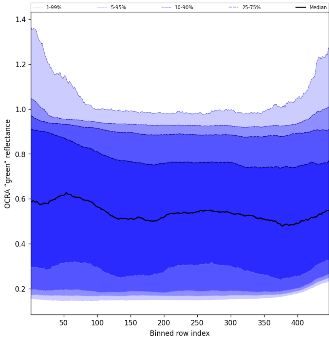
Figure 66: Along track statistics of "OCRA "green" reflectance" for 2025-01-09 to 2025-01-10
