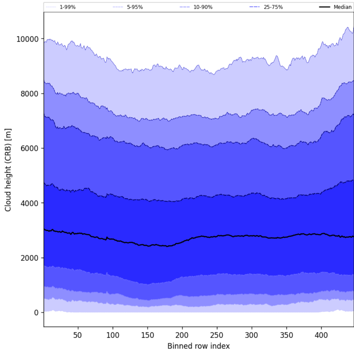
Figure 57: Along track statistics of “Cloud height (CRB)” for 2025-01-09 to 2025-01-10
