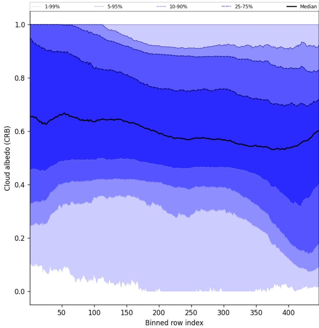
Figure 58: Along track statistics of “Cloud albedo (CRB)” for 2025-01-09 to 2025-01-10
