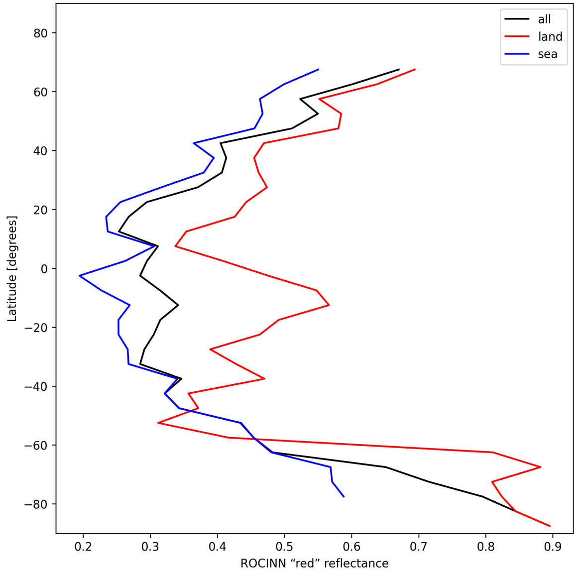
Figure 35: Zonal average of “ROCINN “red” reflectance” for 2025-01-09 to 2025-01-10.
