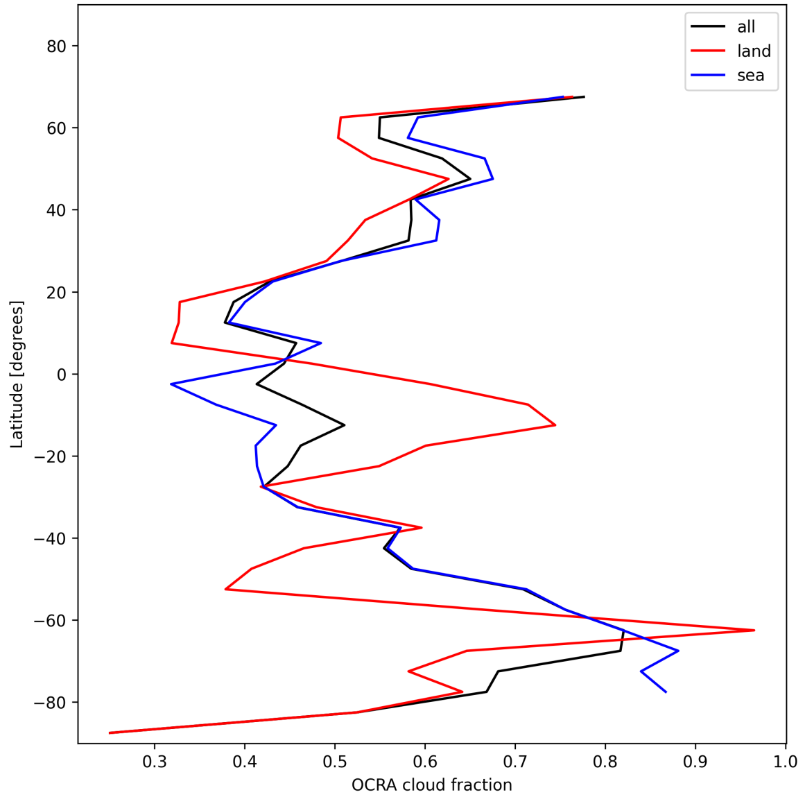
Figure 32: Zonal average of “OCRA cloud fraction” for 2025-01-09 to 2025-01-10.
