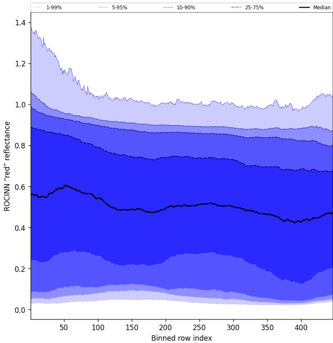
Figure 67: Along track statistics of "ROCINN "red" reflectance" for 2025-01-09 to 2025-01-10
