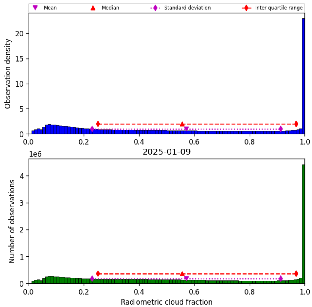
Figure 37: Histogram of “Radiometric cloud fraction” for 2025-01-09 to 2025-01-10
