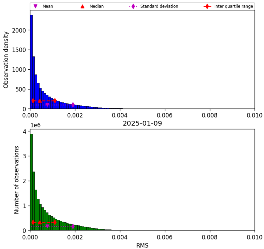
Figure 45: Histogram of “RMS” for 2025-01-09 to 2025-01-10
