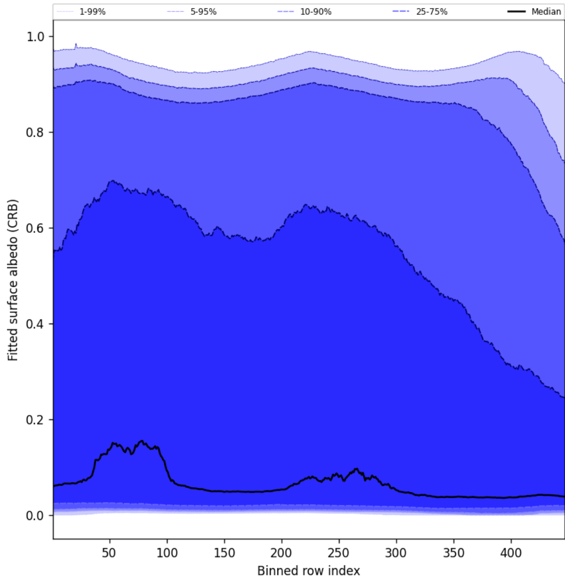
Figure 60: Along track statistics of “Fitted surface albedo (CRB)” for 2025-01-09 to 2025-01-10
