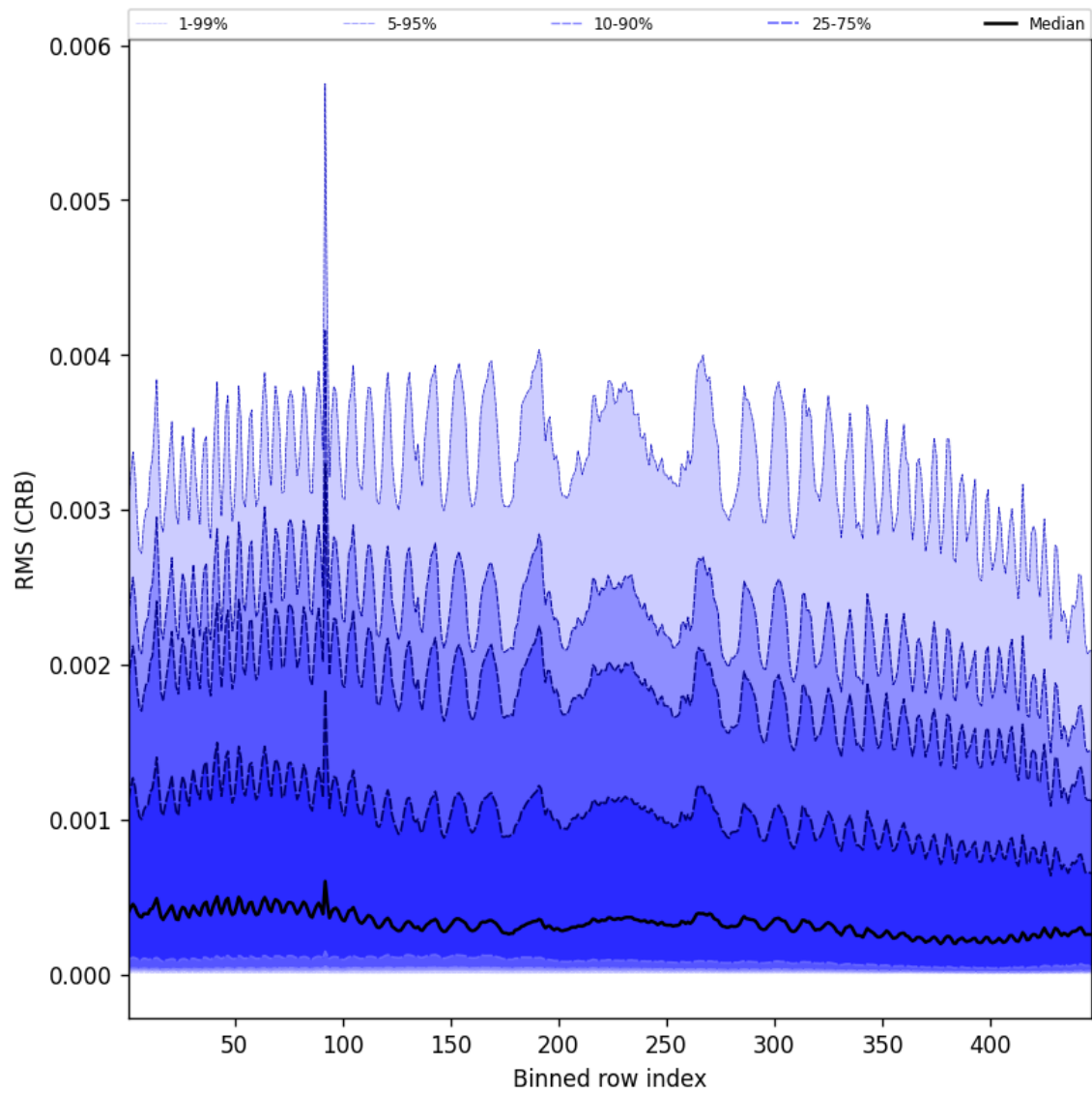
Figure 62: Along track statistics of “RMS (CRB)” for 2025-01-09 to 2025-01-10
