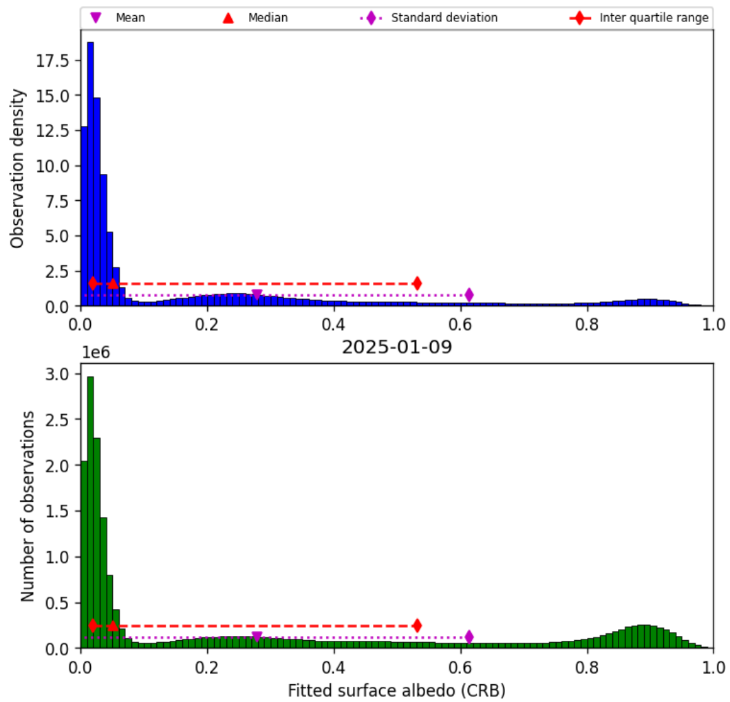
Figure 44: Histogram of “Fitted surface albedo (CRB)” for 2025-01-09 to 2025-01-10
