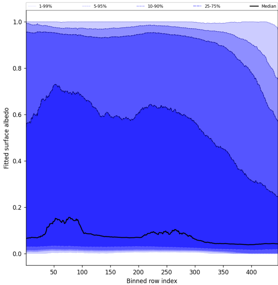
Figure 59: Along track statistics of “Fitted surface albedo” for 2025-01-09 to 2025-01-10
