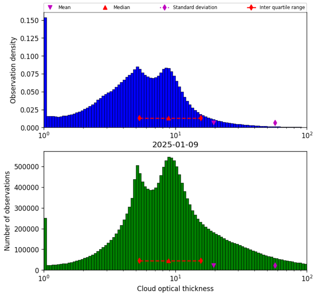
Figure 39: Histogram of “Cloud optical thickness” for 2025-01-09 to 2025-01-10
