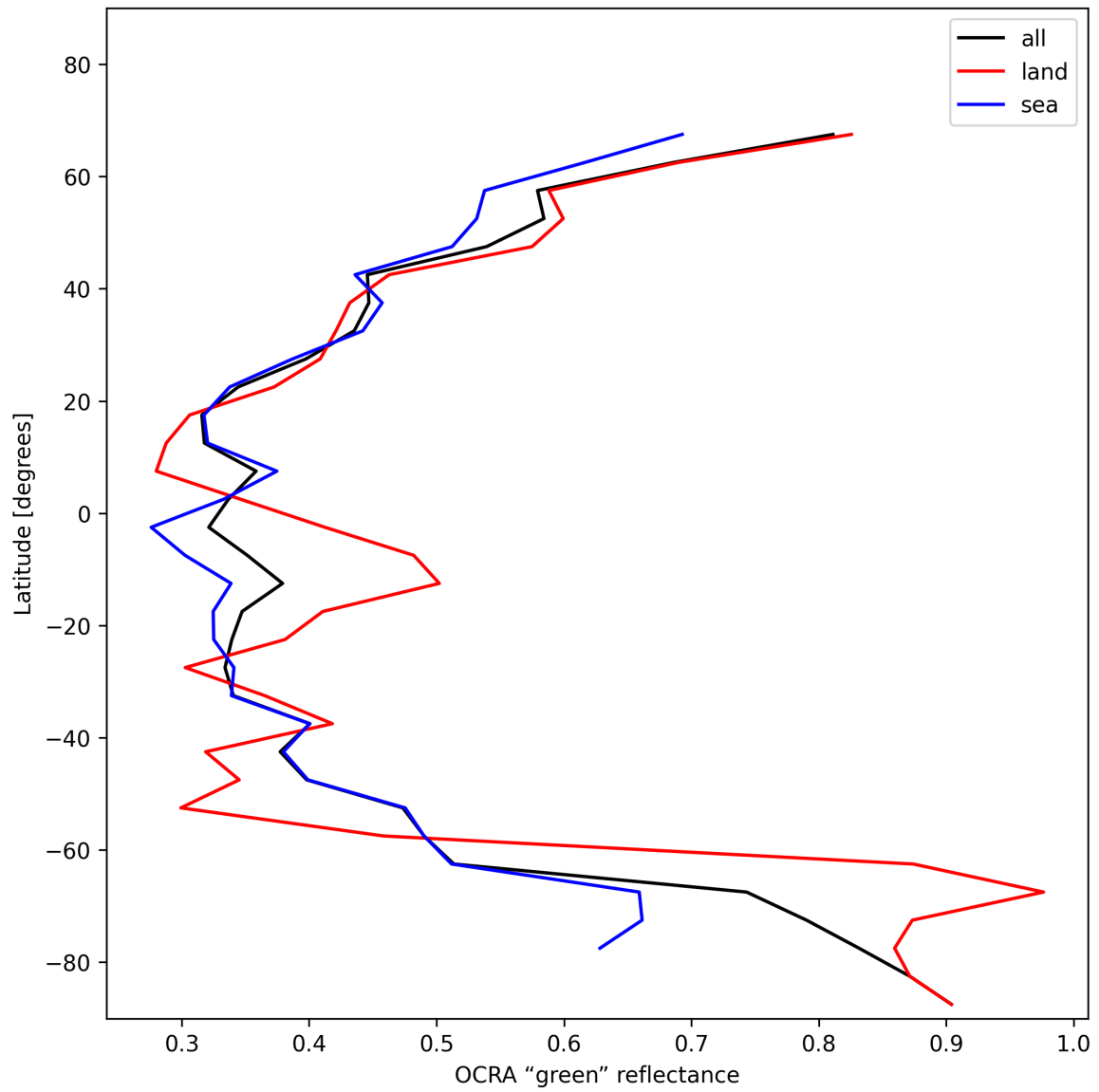
Figure 34: Zonal average of “OCRA “green” reflectance” for 2025-01-09 to 2025-01-10.
