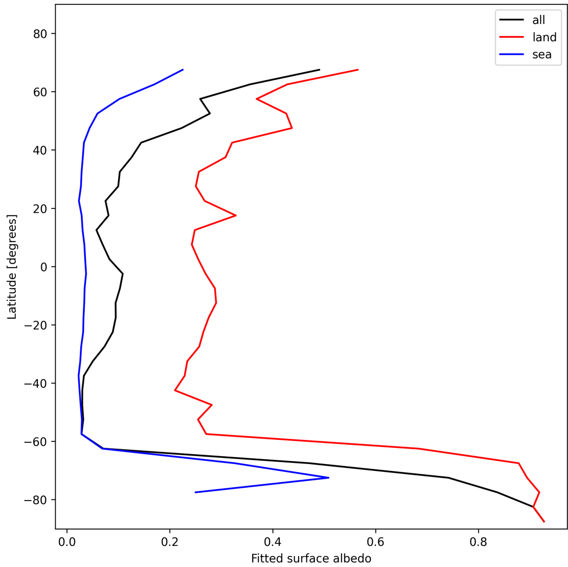
Figure 27: Zonal average of “Fitted surface albedo” for 2025-01-09 to 2025-01-10.
