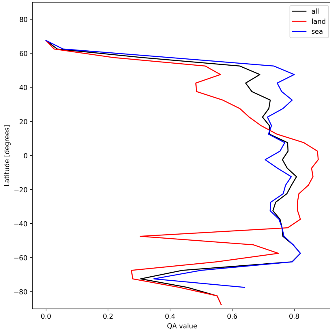
Figure 20: Zonal average of “QA value” for 2025-01-09 to 2025-01-10.
