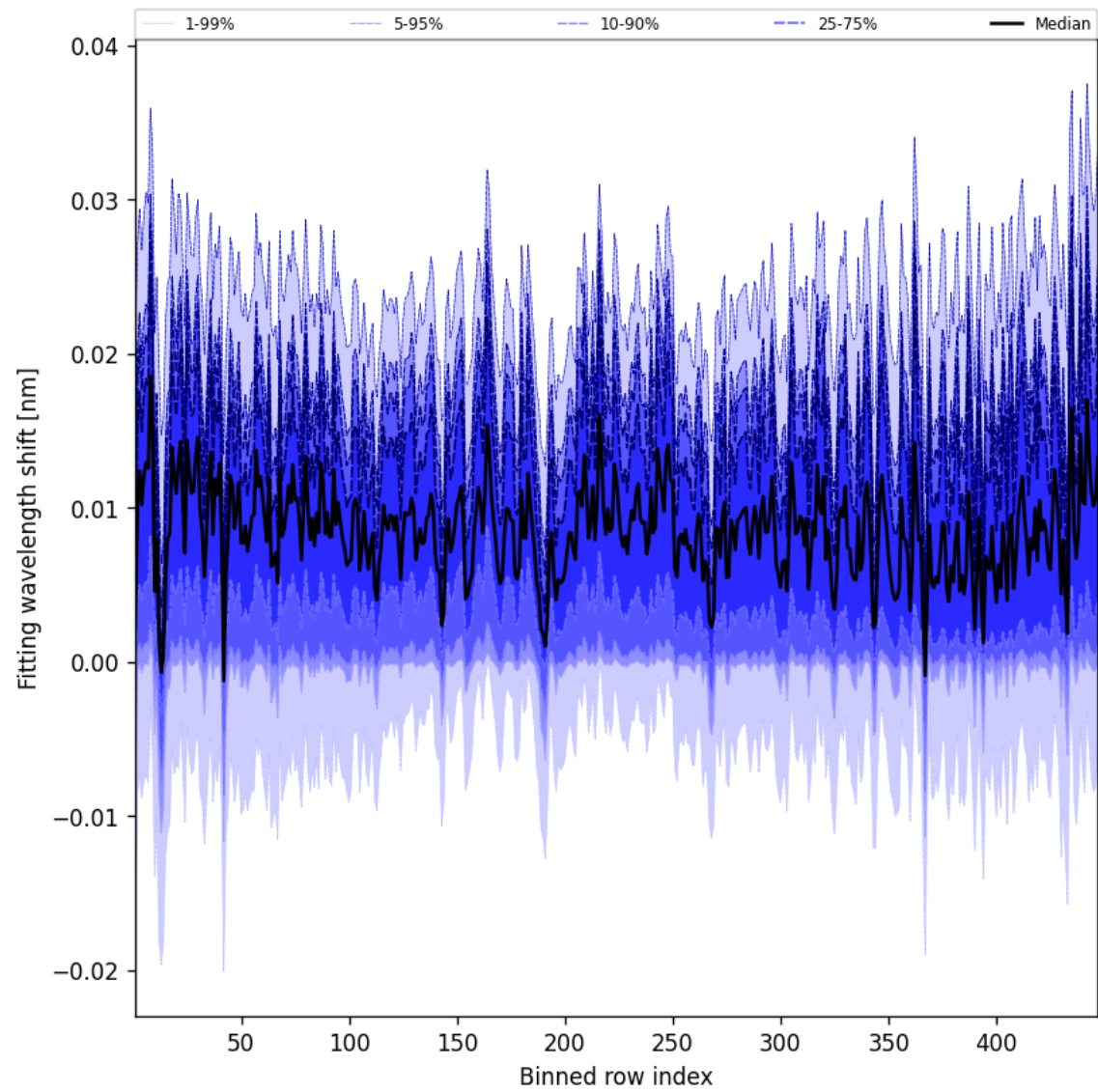
Figure 63: Along track statistics of “Fitting wavelength shift” for 2025-01-09 to 2025-01-10
