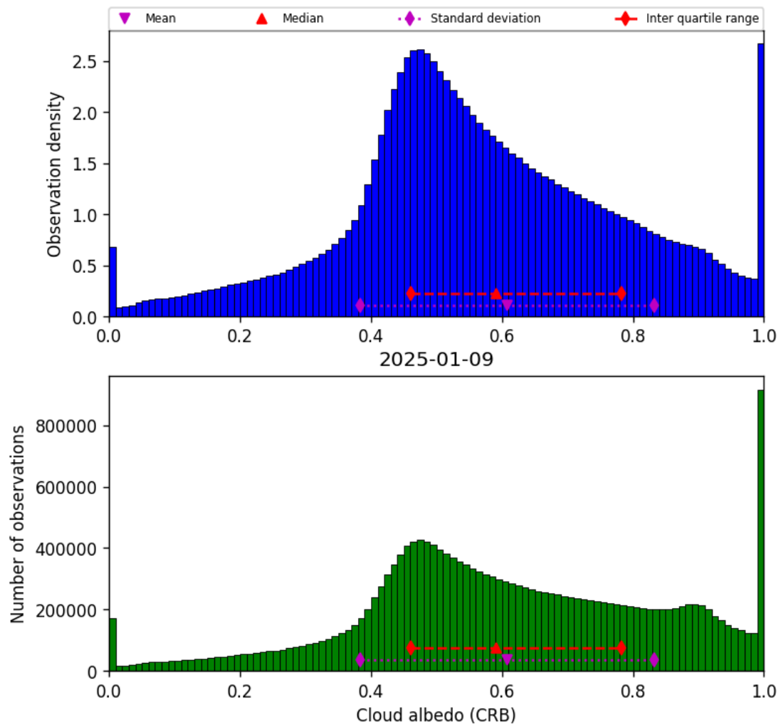
Figure 42: Histogram of “Cloud albedo (CRB)” for 2025-01-09 to 2025-01-10
