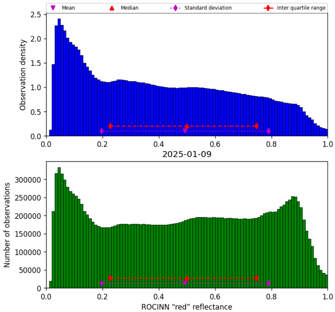
Figure 51: Histogram of “ROCINN “red” reflectance” for 2025-01-09 to 2025-01-10
