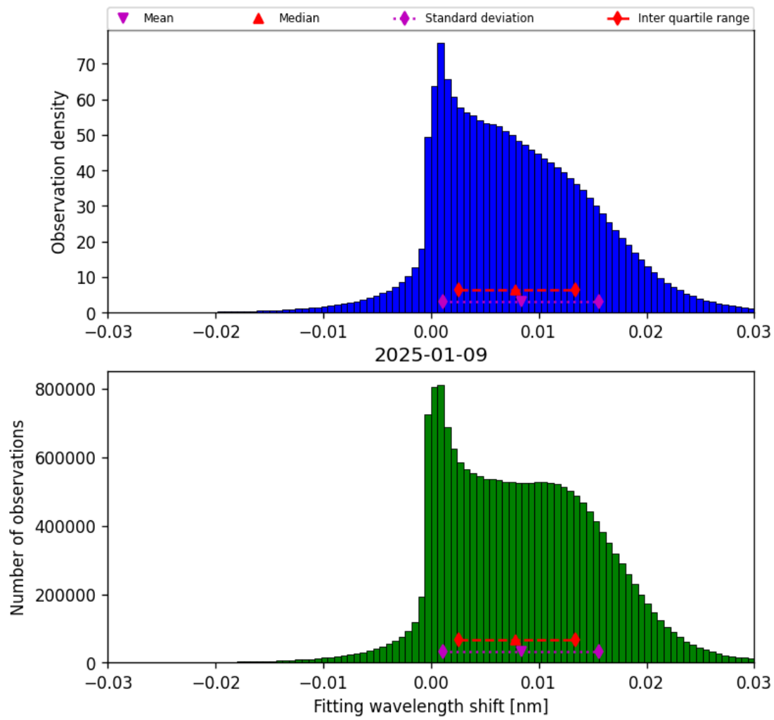
Figure 47: Histogram of “Fitting wavelength shift” for 2025-01-09 to 2025-01-10
