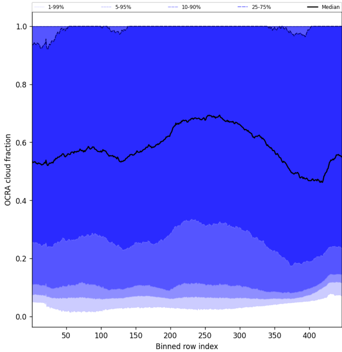
Figure 64: Along track statistics of “OCRA cloud fraction” for 2025-01-09 to 2025-01-10
