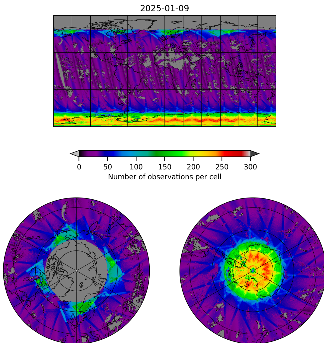
Figure 19: Map of the number of observations for 2025-01-09 to 2025-01-10
