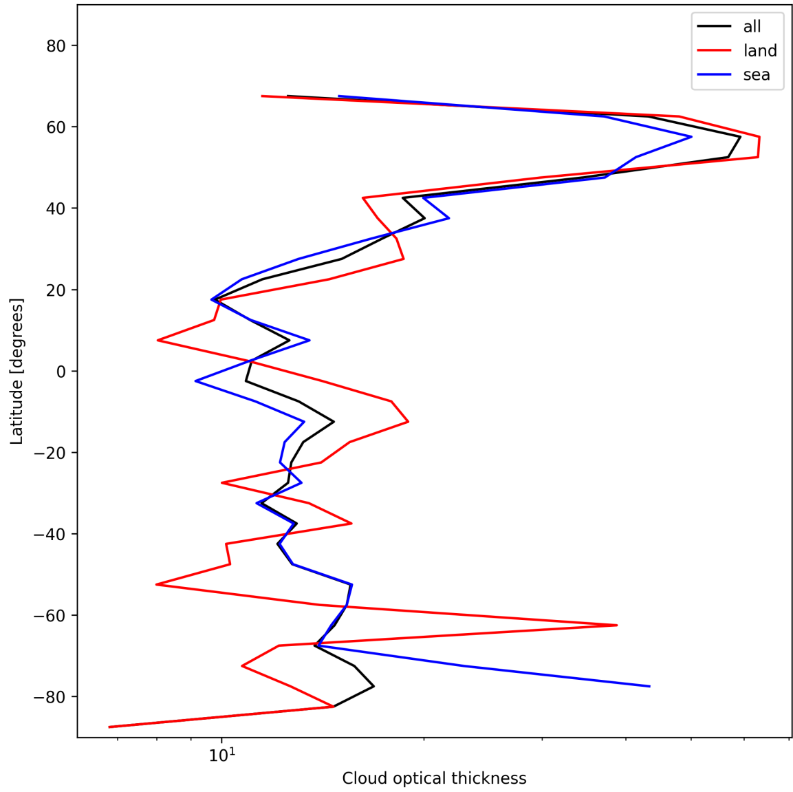
Figure 23: Zonal average of “Cloud optical thickness” for 2025-01-09 to 2025-01-10.
