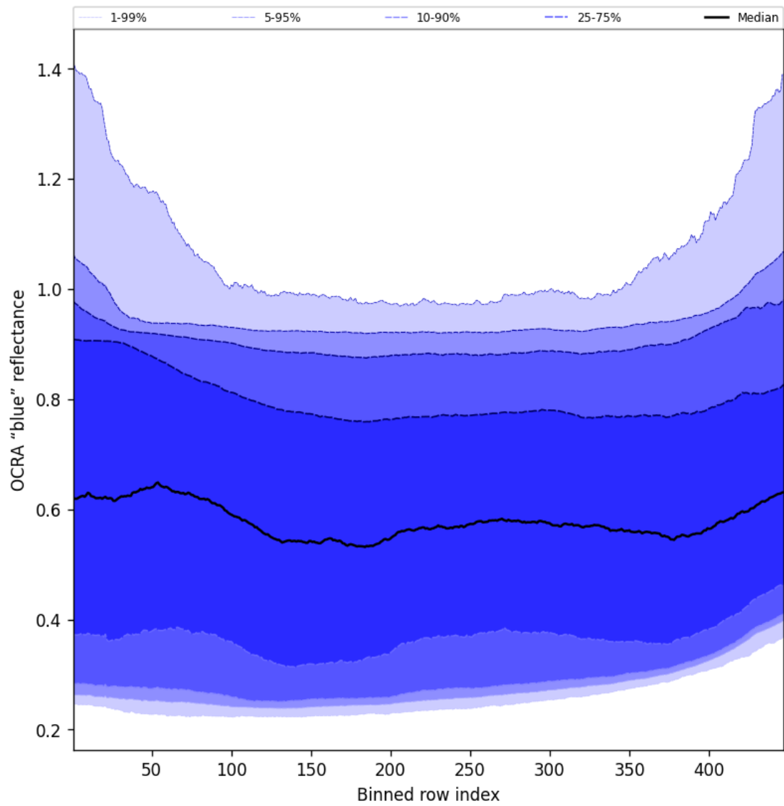
Figure 65: Along track statistics of “OCRA “blue” reflectance” for 2025-01-09 to 2025-01-10
