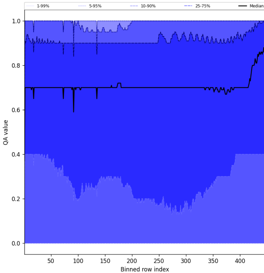
Figure 52: Along track statistics of “QA value” for 2025-01-09 to 2025-01-10
