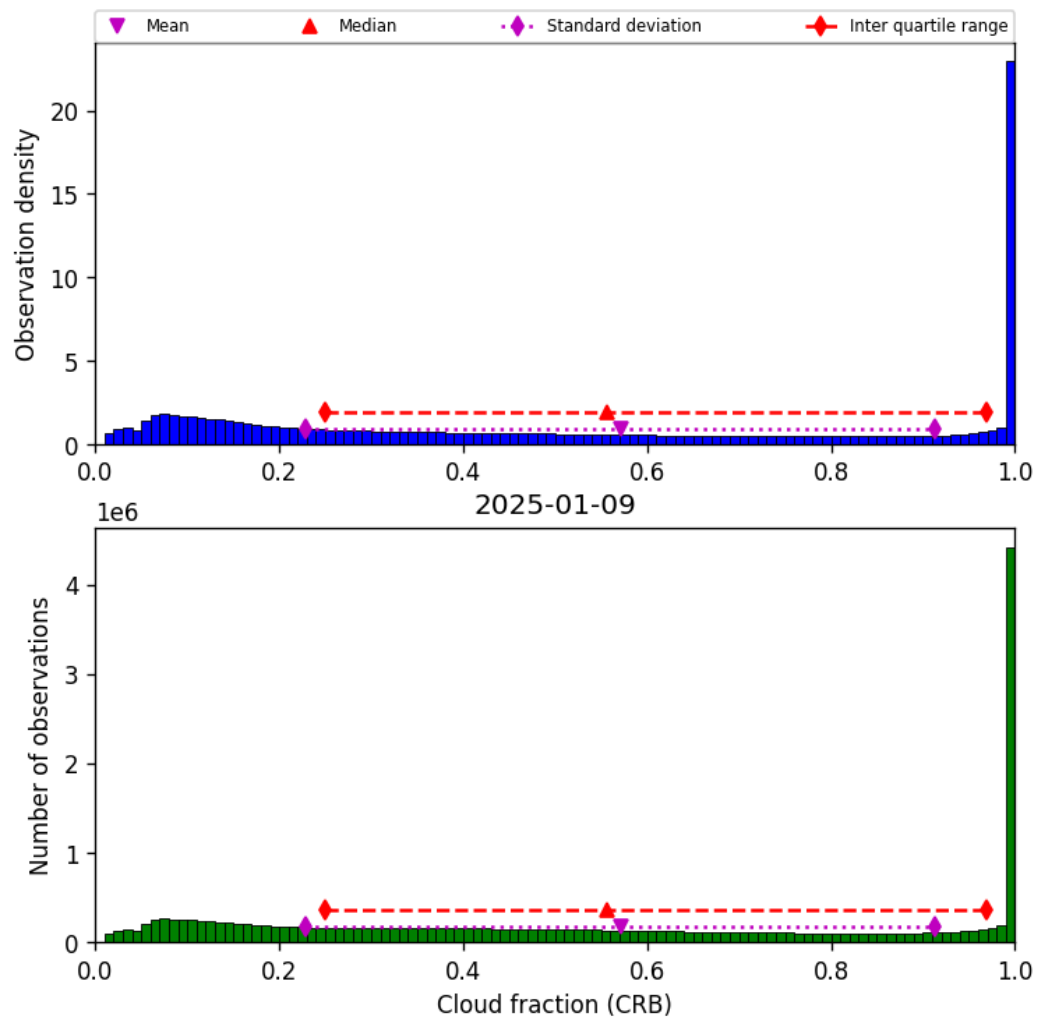
Figure 40: Histogram of “Cloud fraction (CRB)” for 2025-01-09 to 2025-01-10
