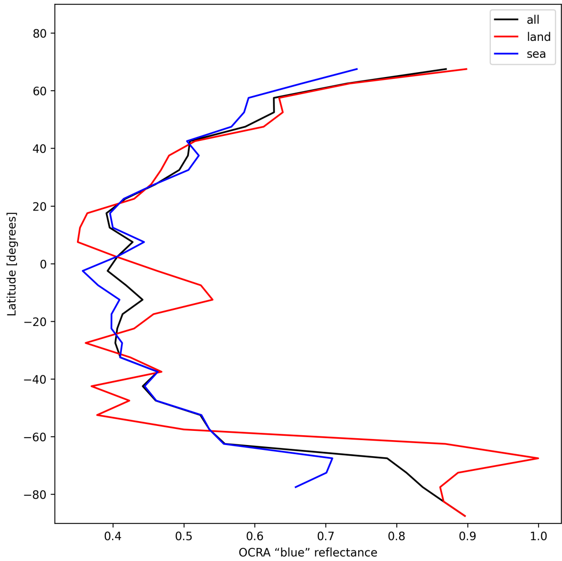
Figure 33: Zonal average of “OCRA “blue” reflectance” for 2025-01-09 to 2025-01-10.
