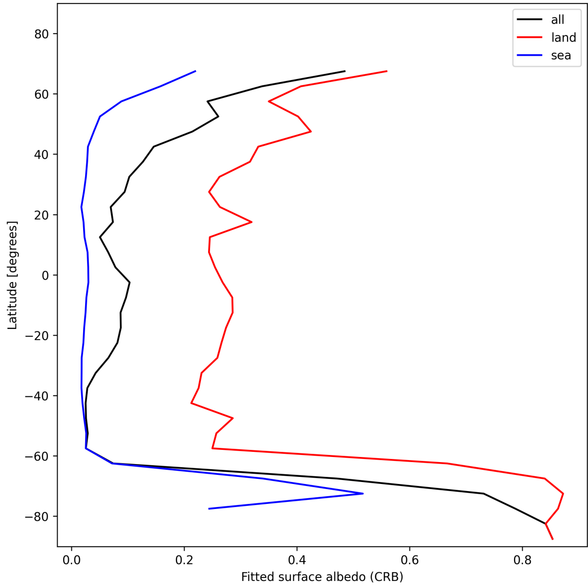
Figure 28: Zonal average of “Fitted surface albedo (CRB)” for 2025-01-09 to 2025-01-10.
