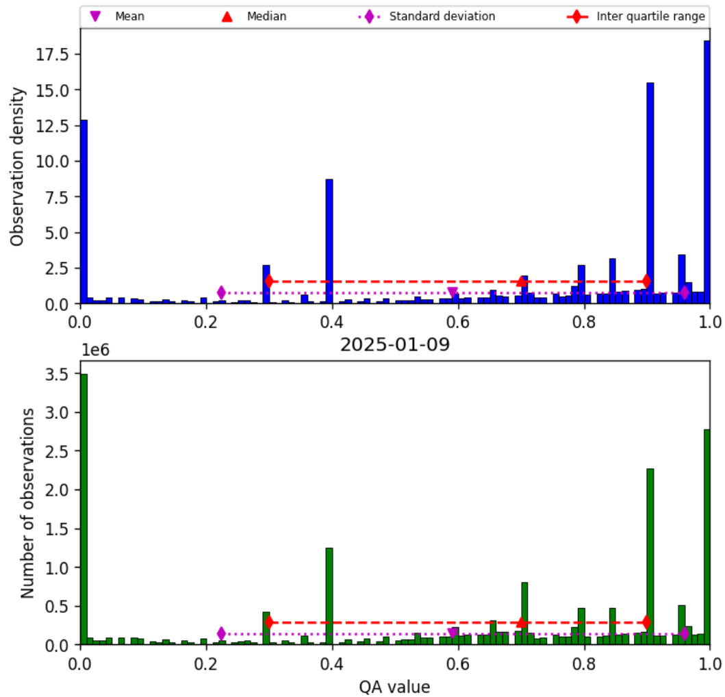
Figure 36: Histogram of “QA value” for 2025-01-09 to 2025-01-10
