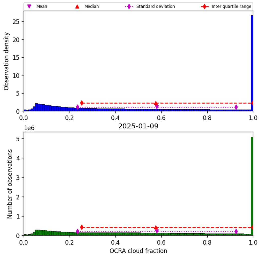
Figure 48: Histogram of “OCRA cloud fraction” for 2025-01-09 to 2025-01-10
