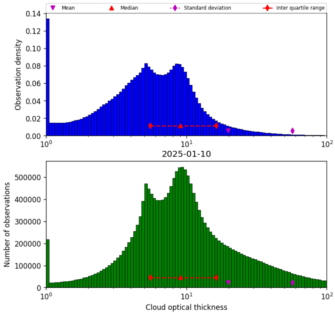
Figure 39: Histogram of “Cloud optical thickness” for 2025-01-10 to 2025-01-10
