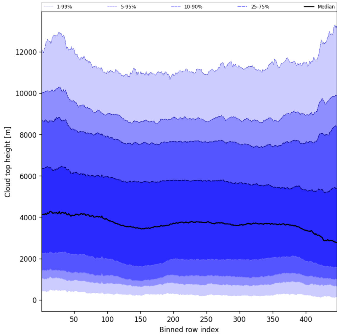
Figure 54: Along track statistics of “Cloud top height” for 2025-01-10 to 2025-01-10
