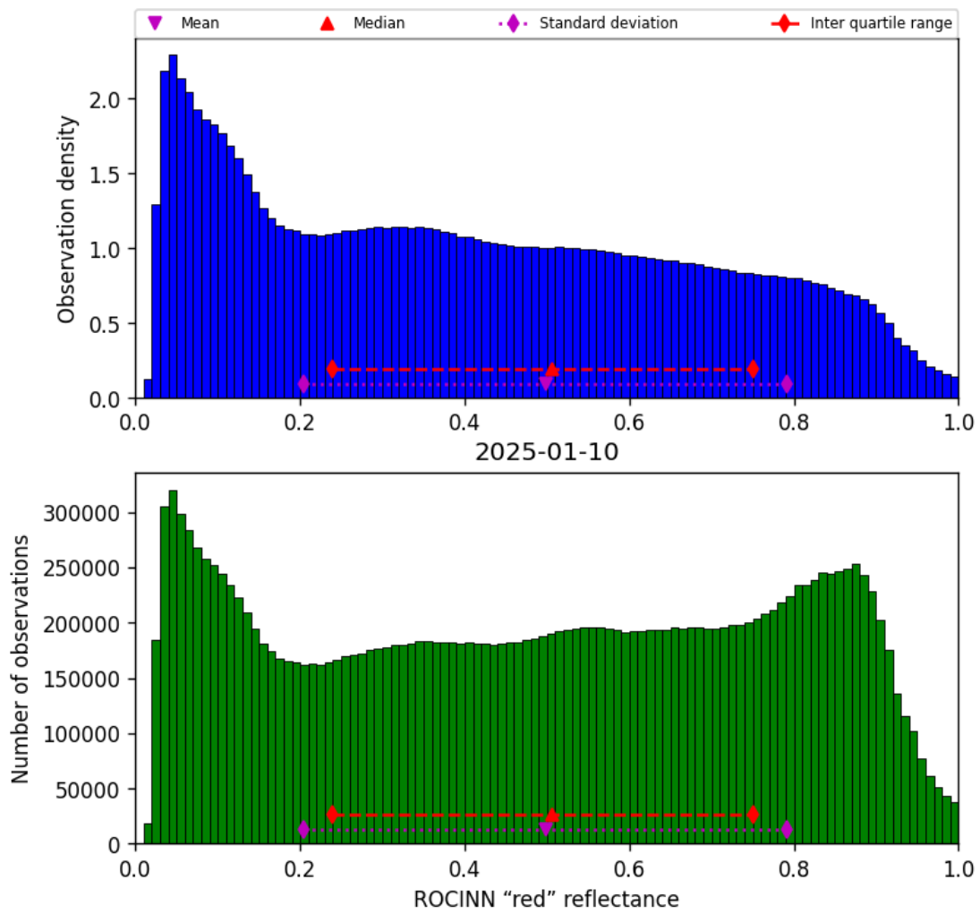
Figure 51: Histogram of “ROCINN “red” reflectance” for 2025-01-10 to 2025-01-10
