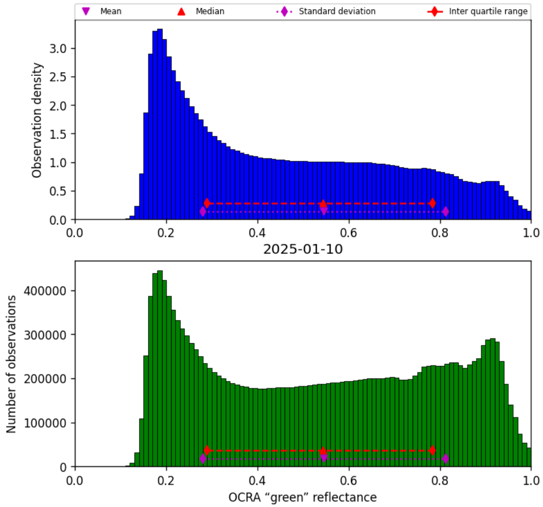
Figure 50: Histogram of “OCRA “green” reflectance” for 2025-01-10 to 2025-01-10
