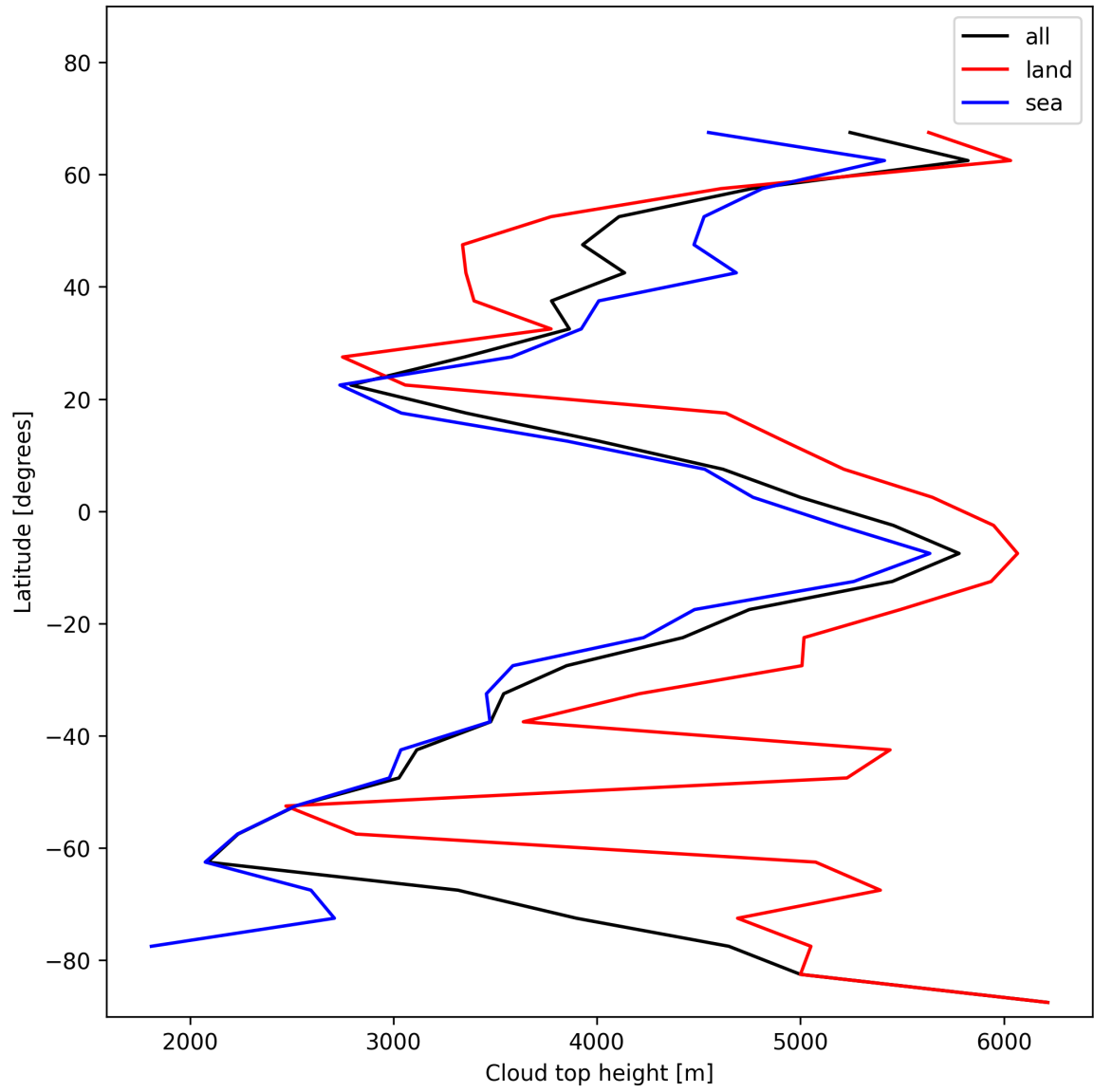
Figure 22: Zonal average of “Cloud top height” for 2025-01-10 to 2025-01-10.
