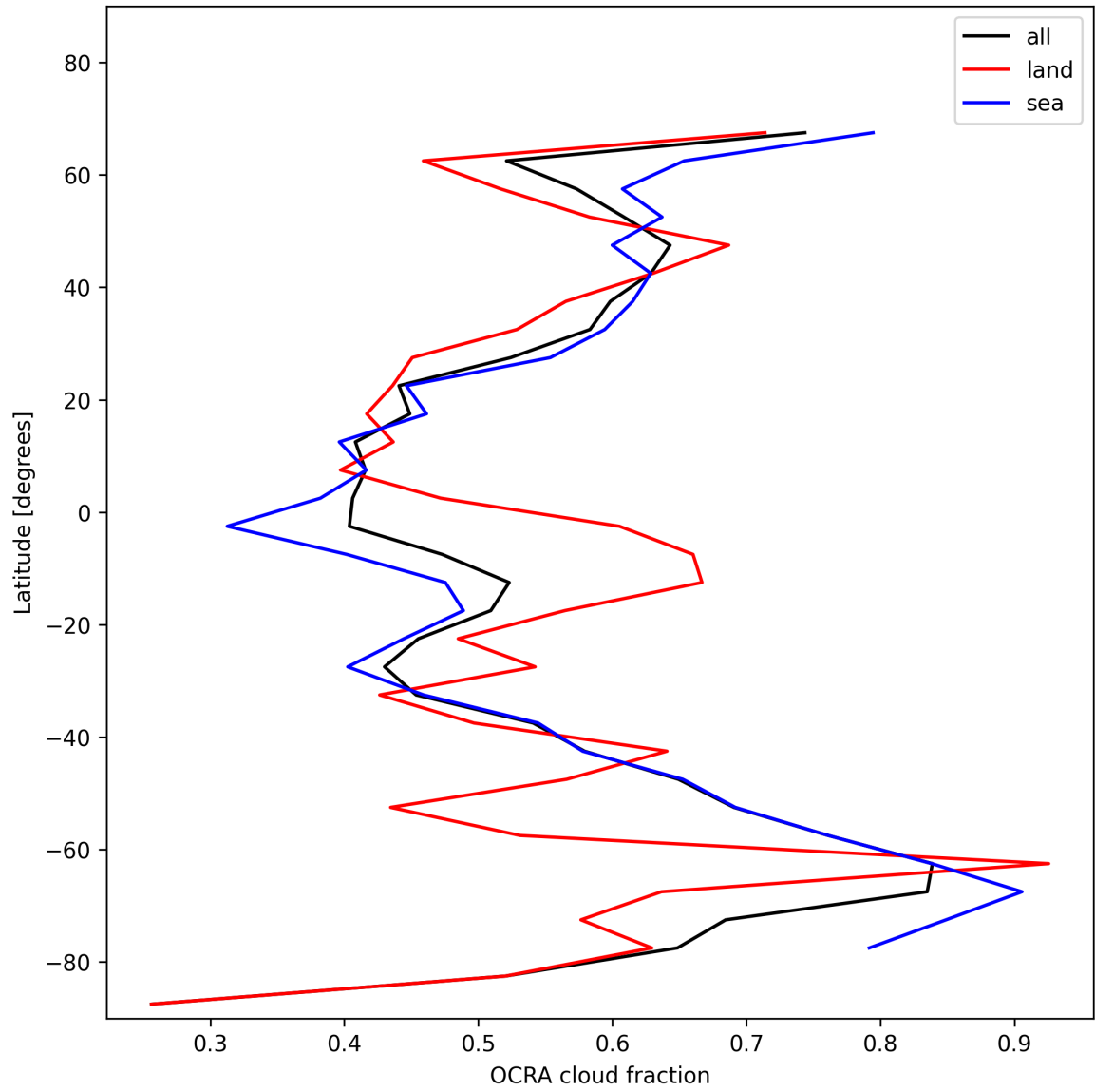
Figure 32: Zonal average of “OCRA cloud fraction” for 2025-01-10 to 2025-01-10.
