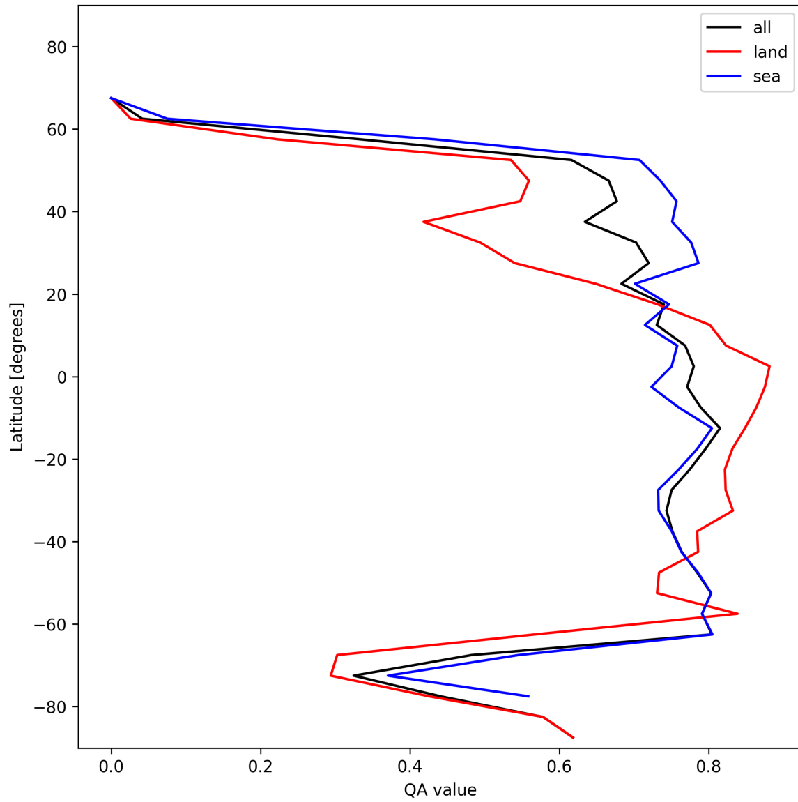
Figure 20: Zonal average of “QA value” for 2025-01-10 to 2025-01-10.
