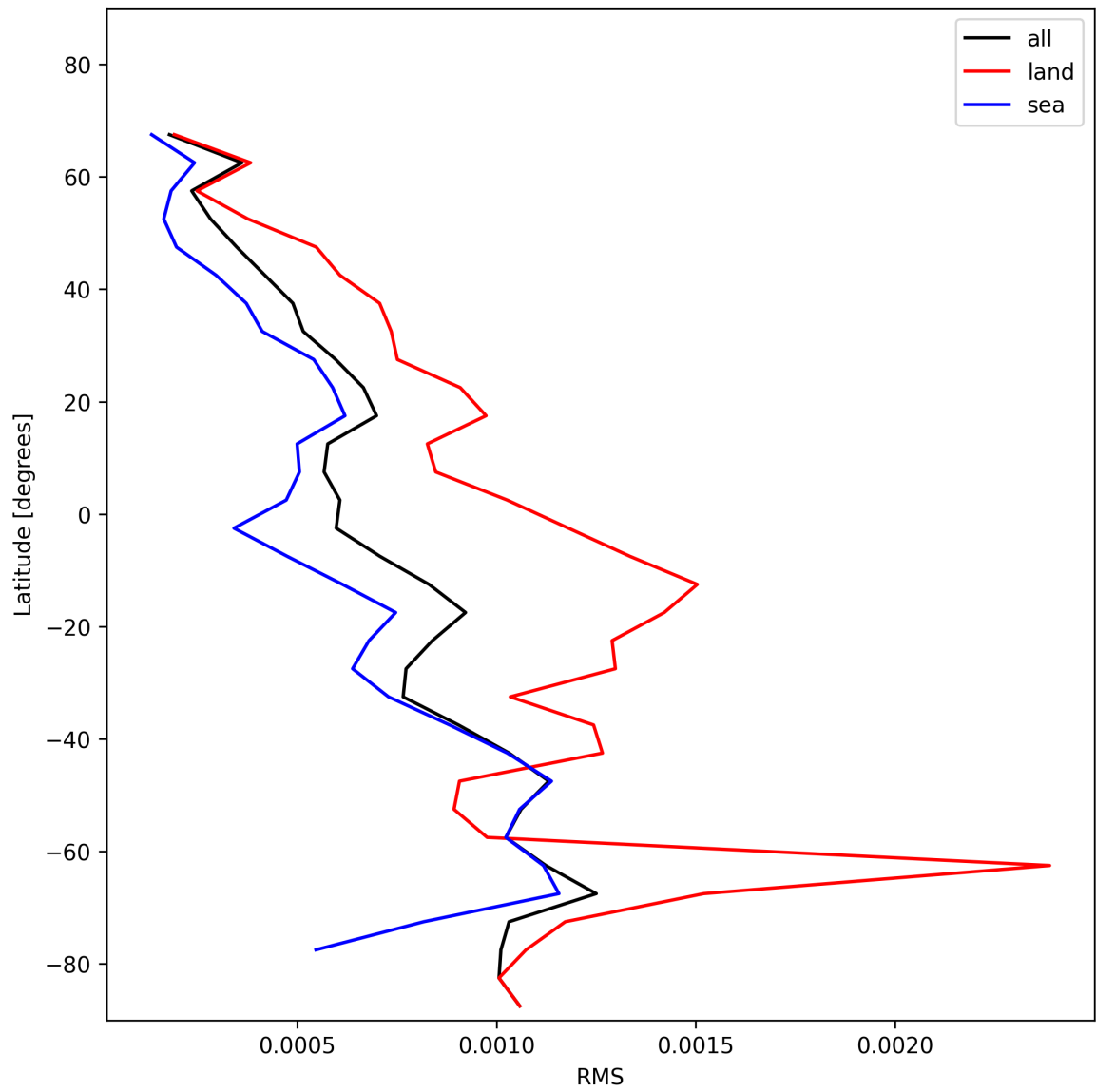
Figure 29: Zonal average of “RMS” for 2025-01-10 to 2025-01-10.
