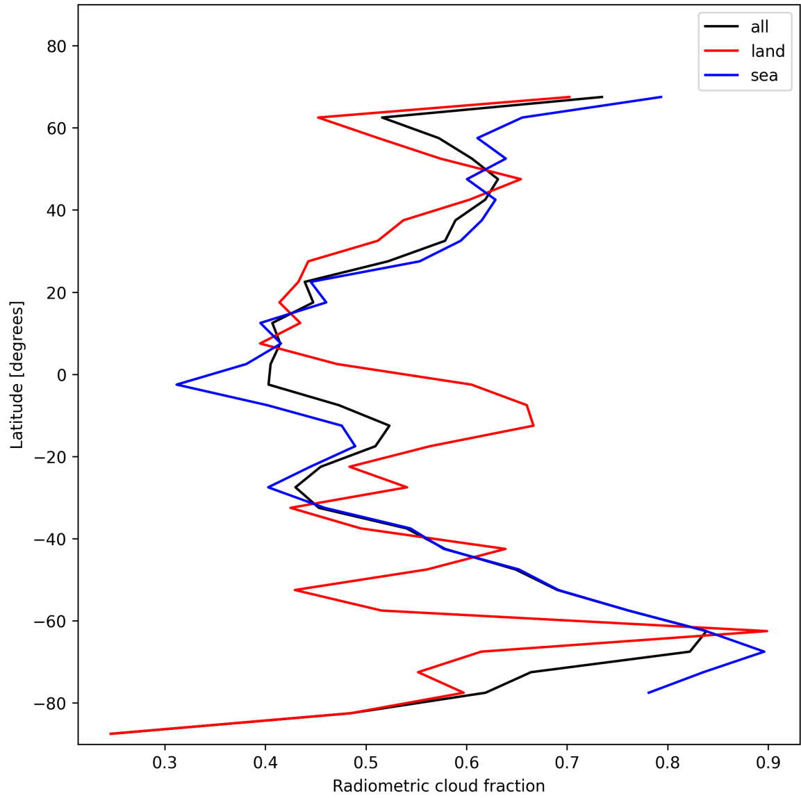
Figure 21: Zonal average of “Radiometric cloud fraction” for 2025-01-10 to 2025-01-10.
