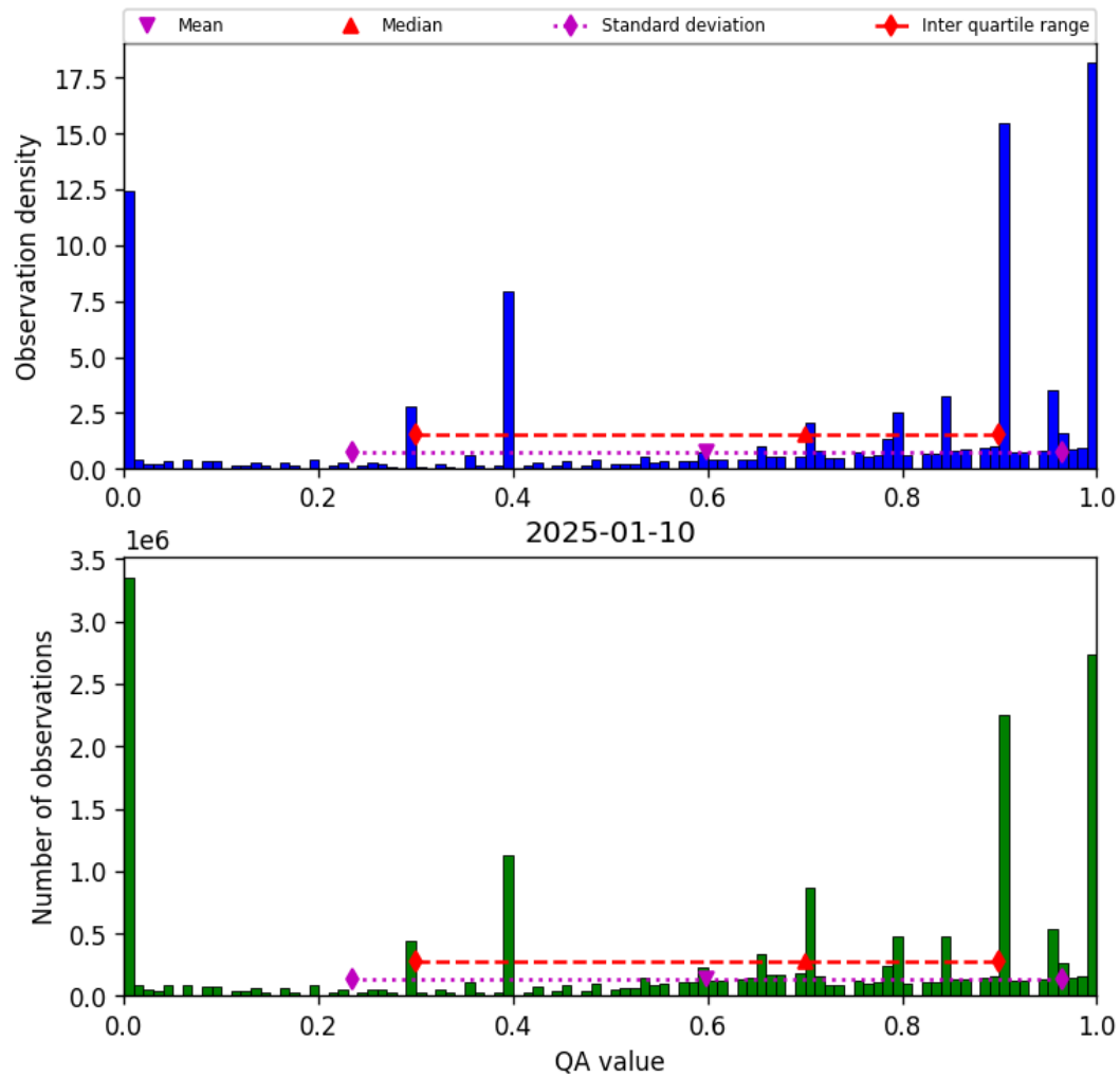
Figure 36: Histogram of “QA value” for 2025-01-10 to 2025-01-10
