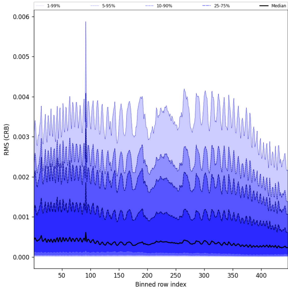
Figure 62: Along track statistics of “RMS (CRB)” for 2025-01-10 to 2025-01-10
