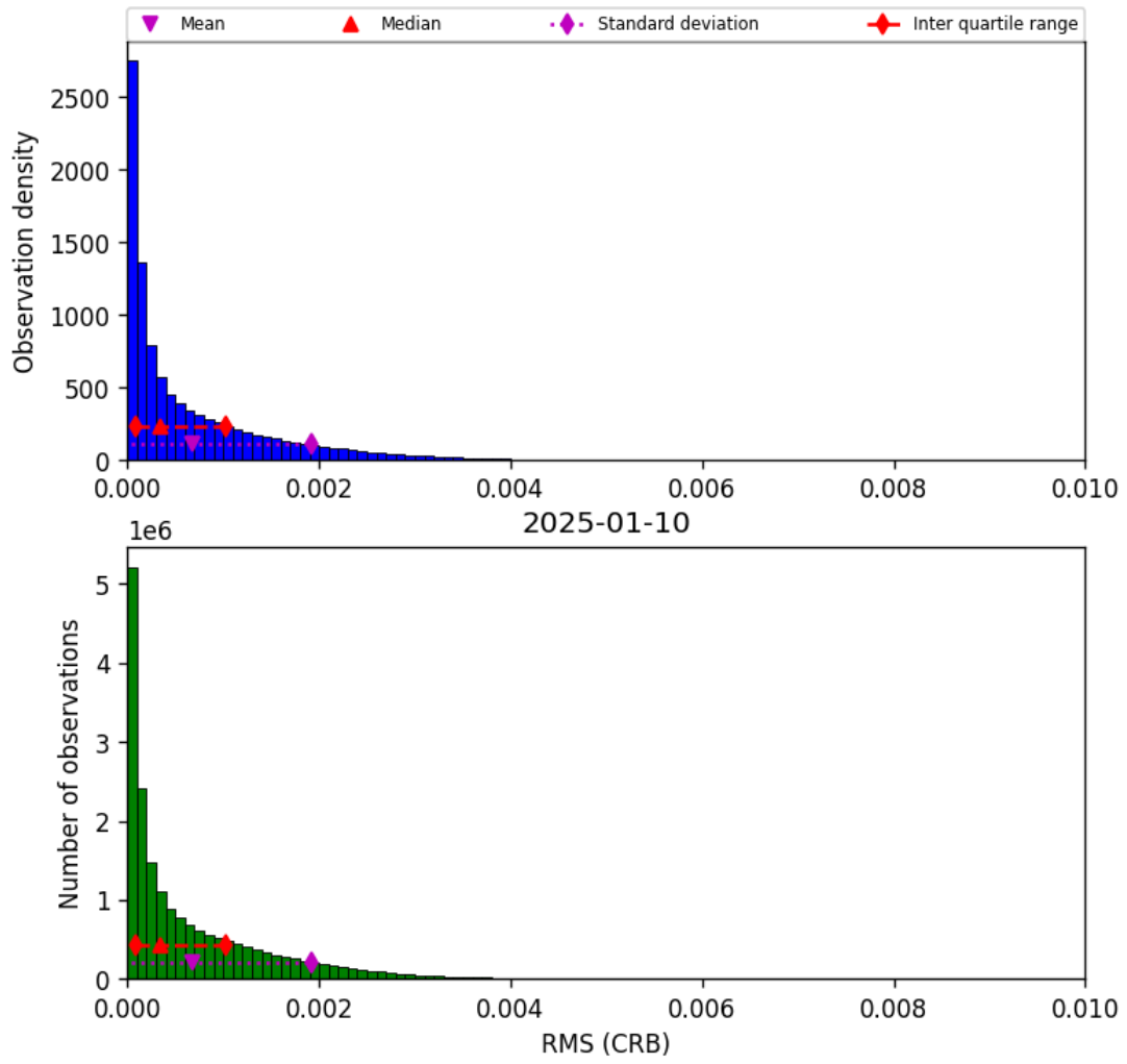
Figure 46: Histogram of “RMS (CRB)” for 2025-01-10 to 2025-01-10
