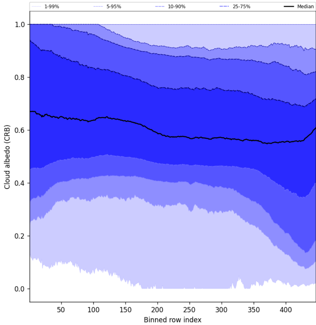
Figure 58: Along track statistics of “Cloud albedo (CRB)” for 2025-01-10 to 2025-01-10
