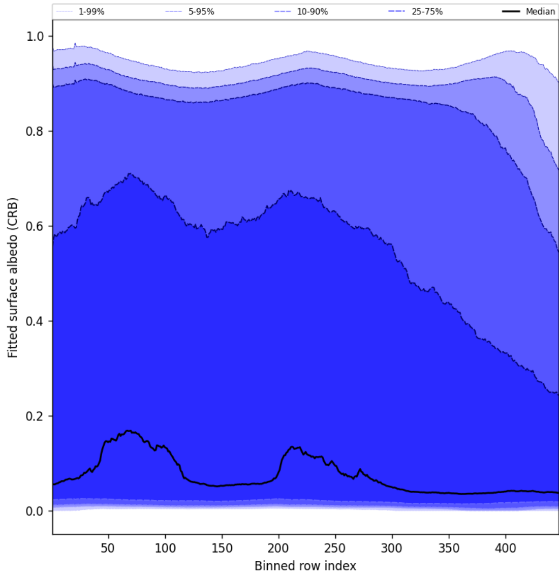
Figure 60: Along track statistics of “Fitted surface albedo (CRB)” for 2025-01-10 to 2025-01-10
