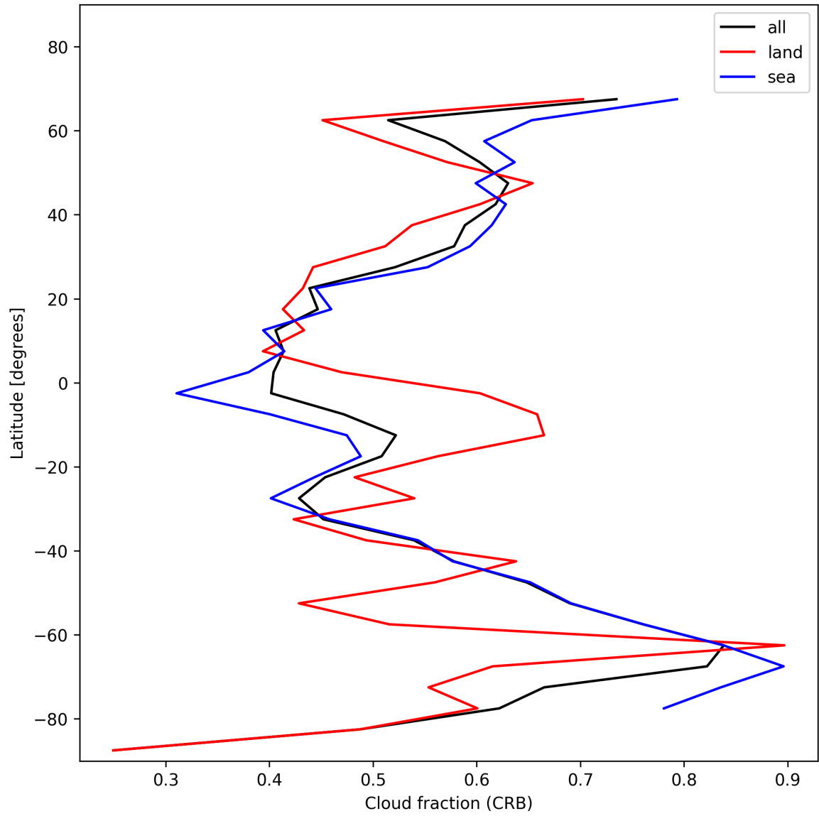
Figure 24: Zonal average of “Cloud fraction (CRB)” for 2025-01-10 to 2025-01-10.
