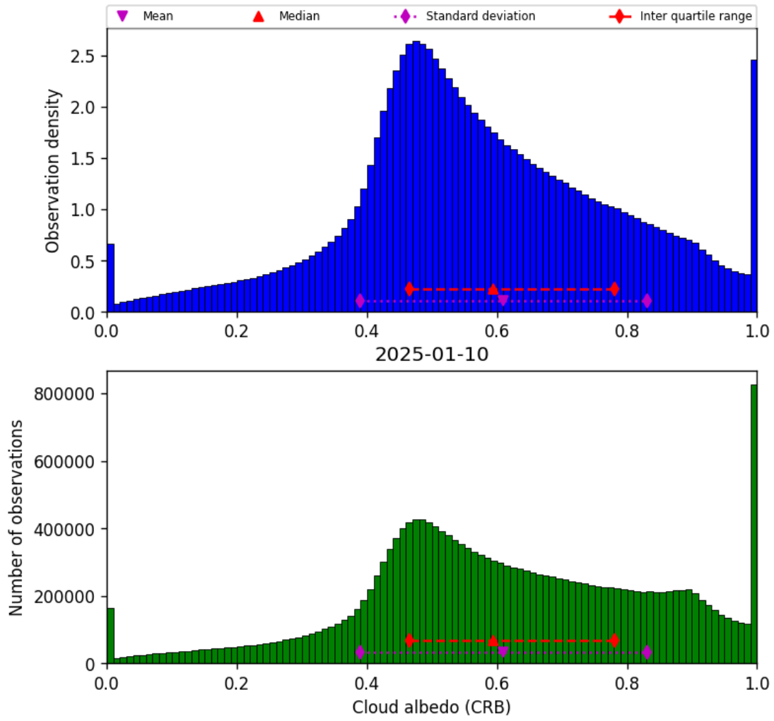
Figure 42: Histogram of “Cloud albedo (CRB)” for 2025-01-10 to 2025-01-10
