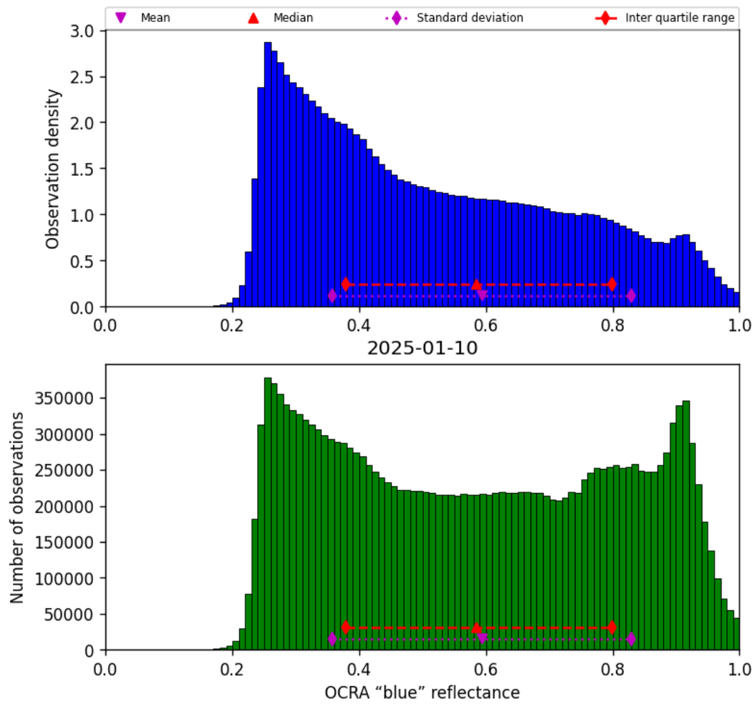
Figure 49: Histogram of "OCRA "blue" reflectance" for 2025-01-10 to 2025-01-10
