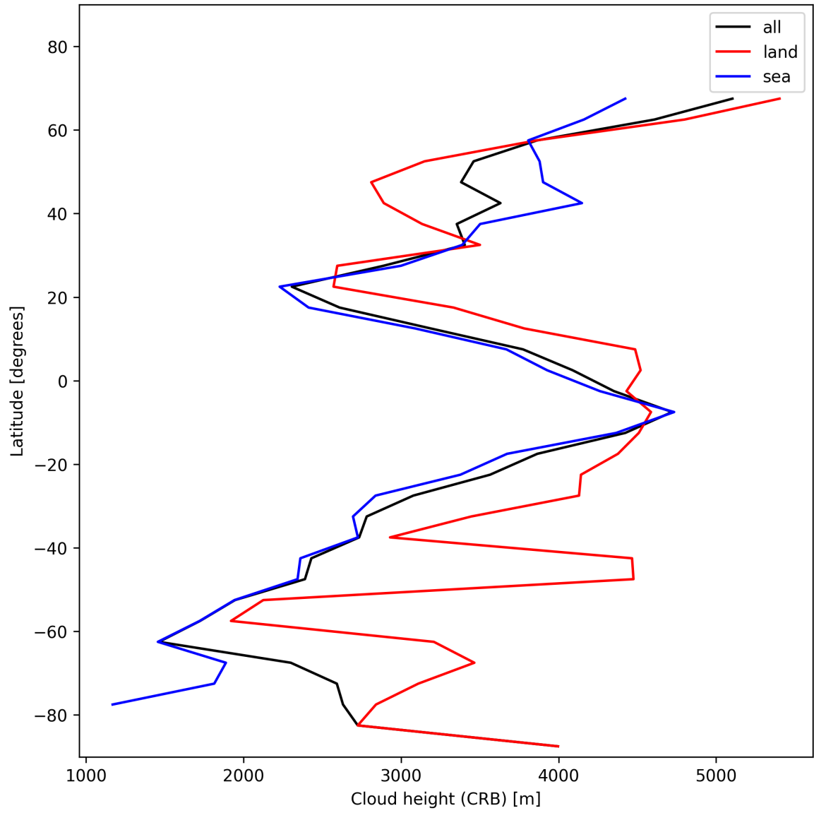
Figure 25: Zonal average of “Cloud height (CRB)” for 2025-01-10 to 2025-01-10.
