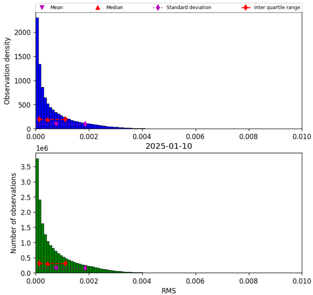
Figure 45: Histogram of “RMS” for 2025-01-10 to 2025-01-10
