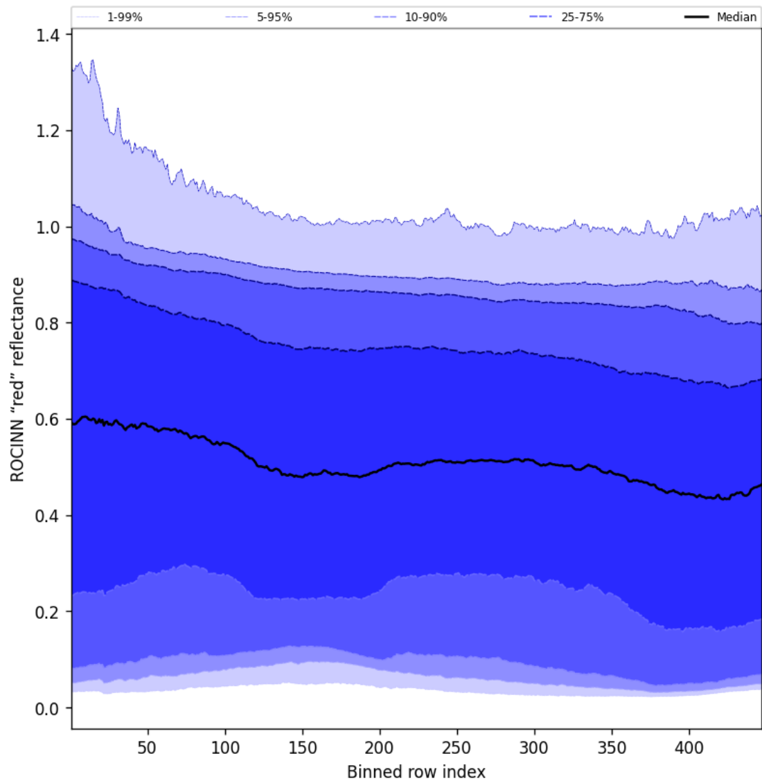
Figure 67: Along track statistics of “ROCINN “red” reflectance” for 2025-01-10 to 2025-01-10
