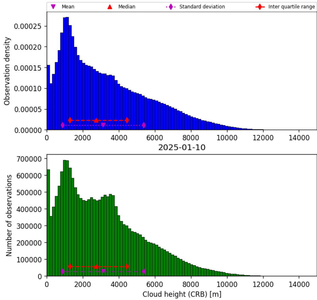
Figure 41: Histogram of “Cloud height (CRB)” for 2025-01-10 to 2025-01-10
