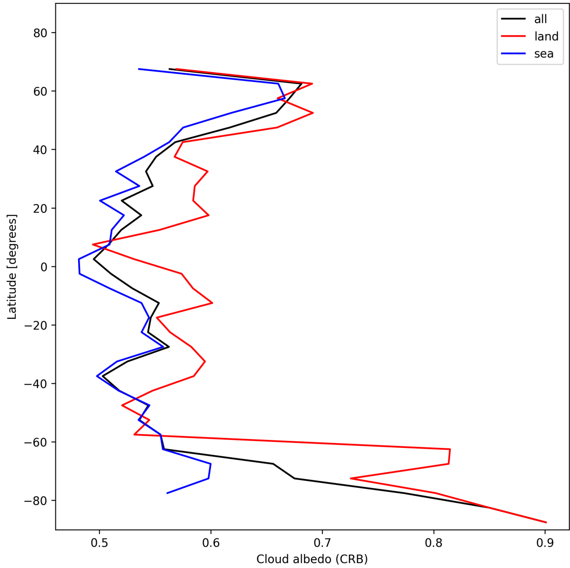
Figure 26: Zonal average of “Cloud albedo (CRB)” for 2025-01-10 to 2025-01-10.
