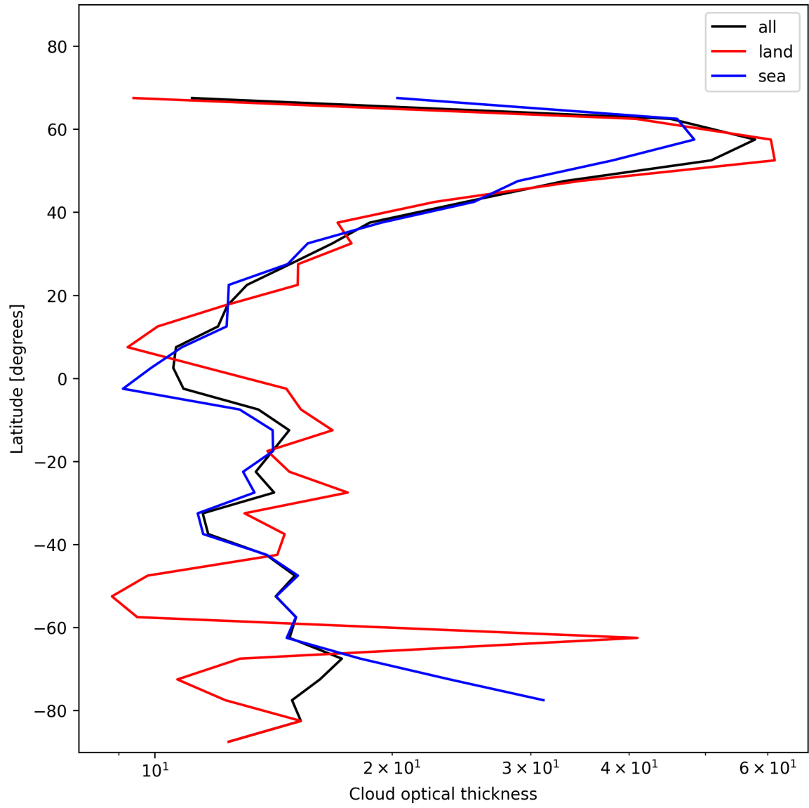
Figure 23: Zonal average of “Cloud optical thickness” for 2025-01-10 to 2025-01-10.
