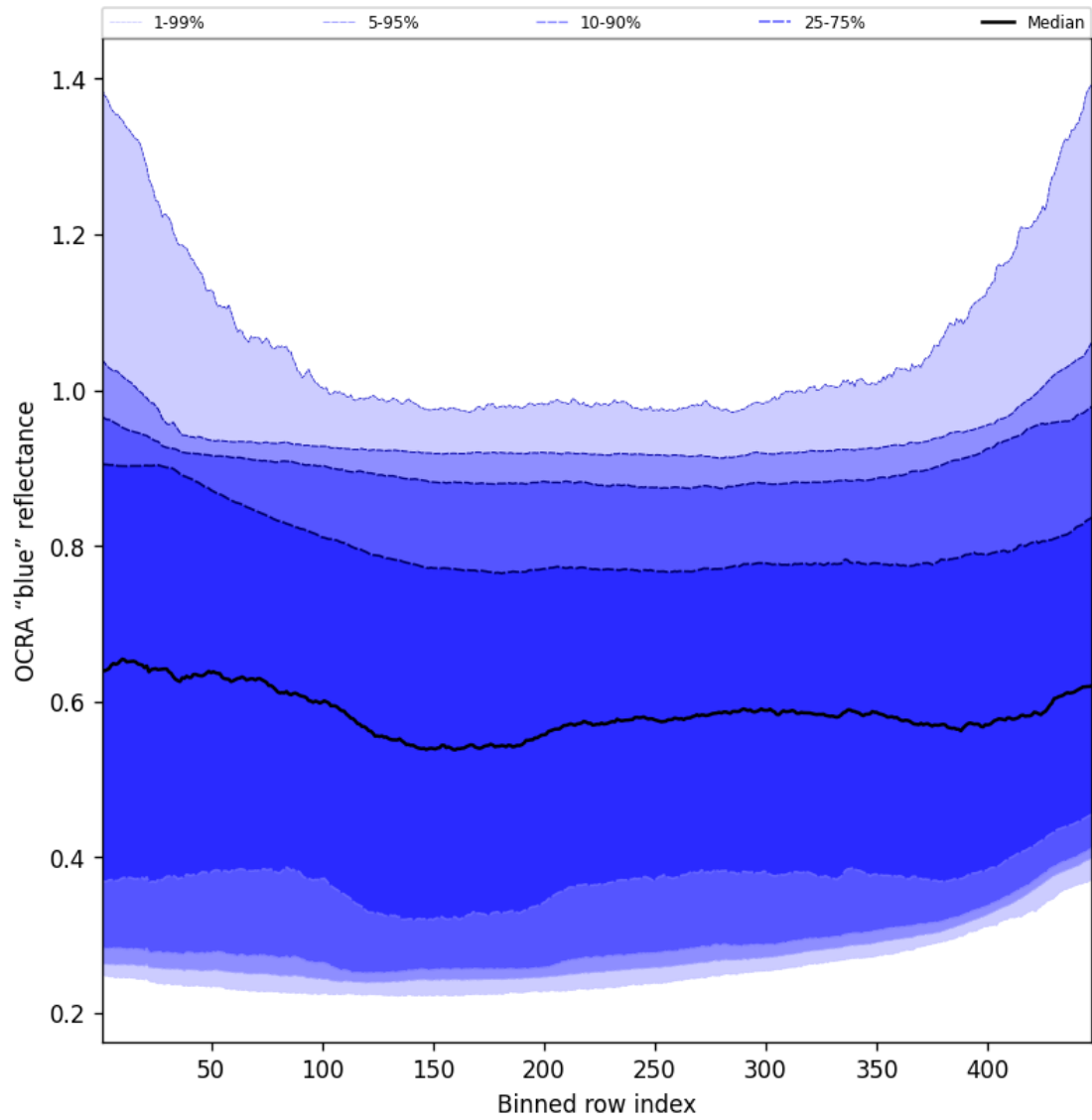
Figure 65: Along track statistics of “OCRA “blue” reflectance” for 2025-01-10 to 2025-01-10
