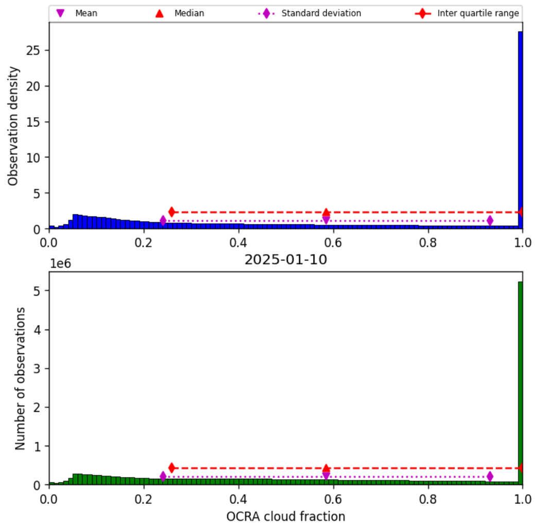
Figure 48: Histogram of “OCRA cloud fraction” for 2025-01-10 to 2025-01-10
