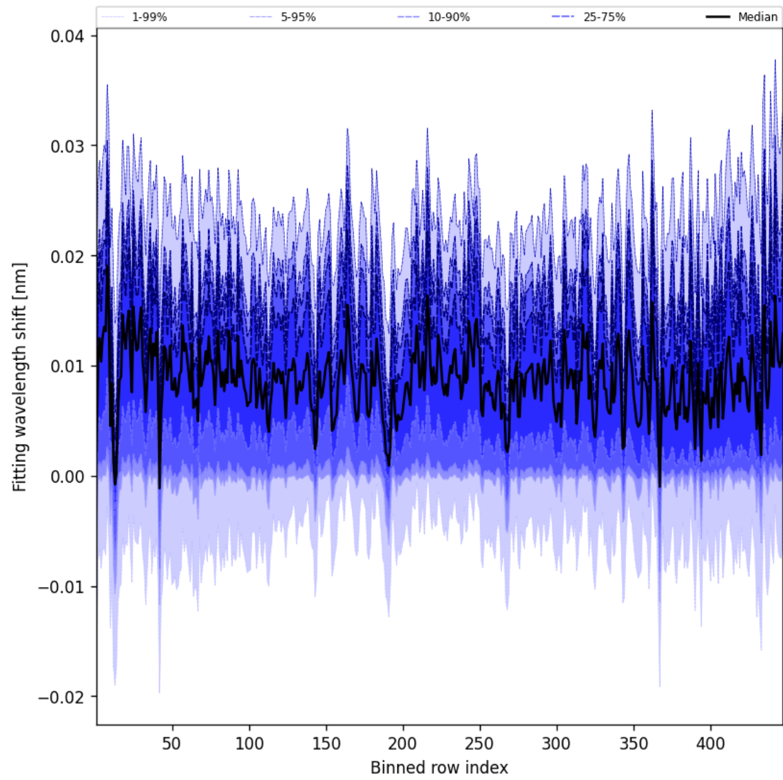
Figure 63: Along track statistics of “Fitting wavelength shift” for 2025-01-10 to 2025-01-10
