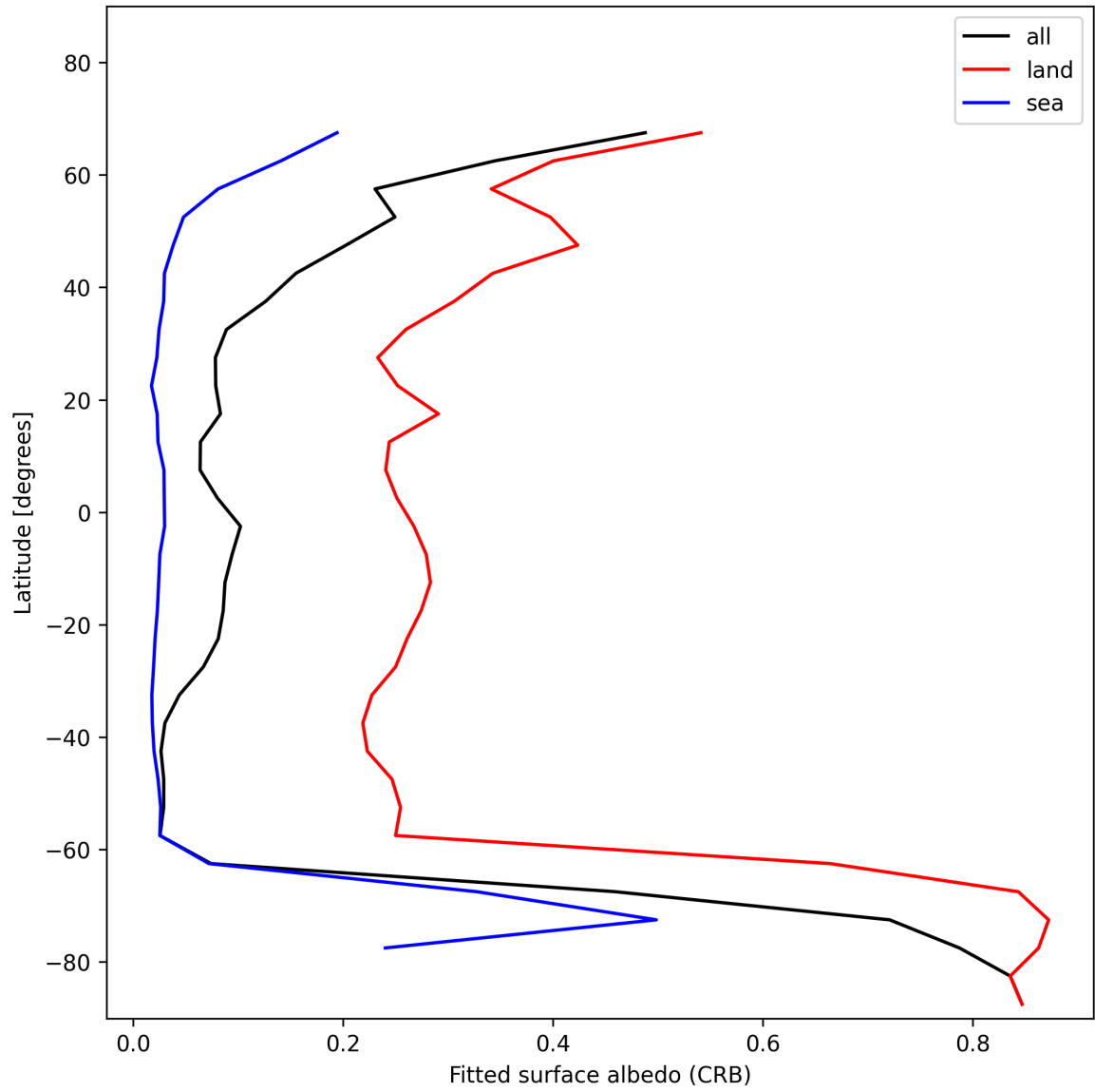
Figure 28: Zonal average of “Fitted surface albedo (CRB)” for 2025-01-10 to 2025-01-10.
