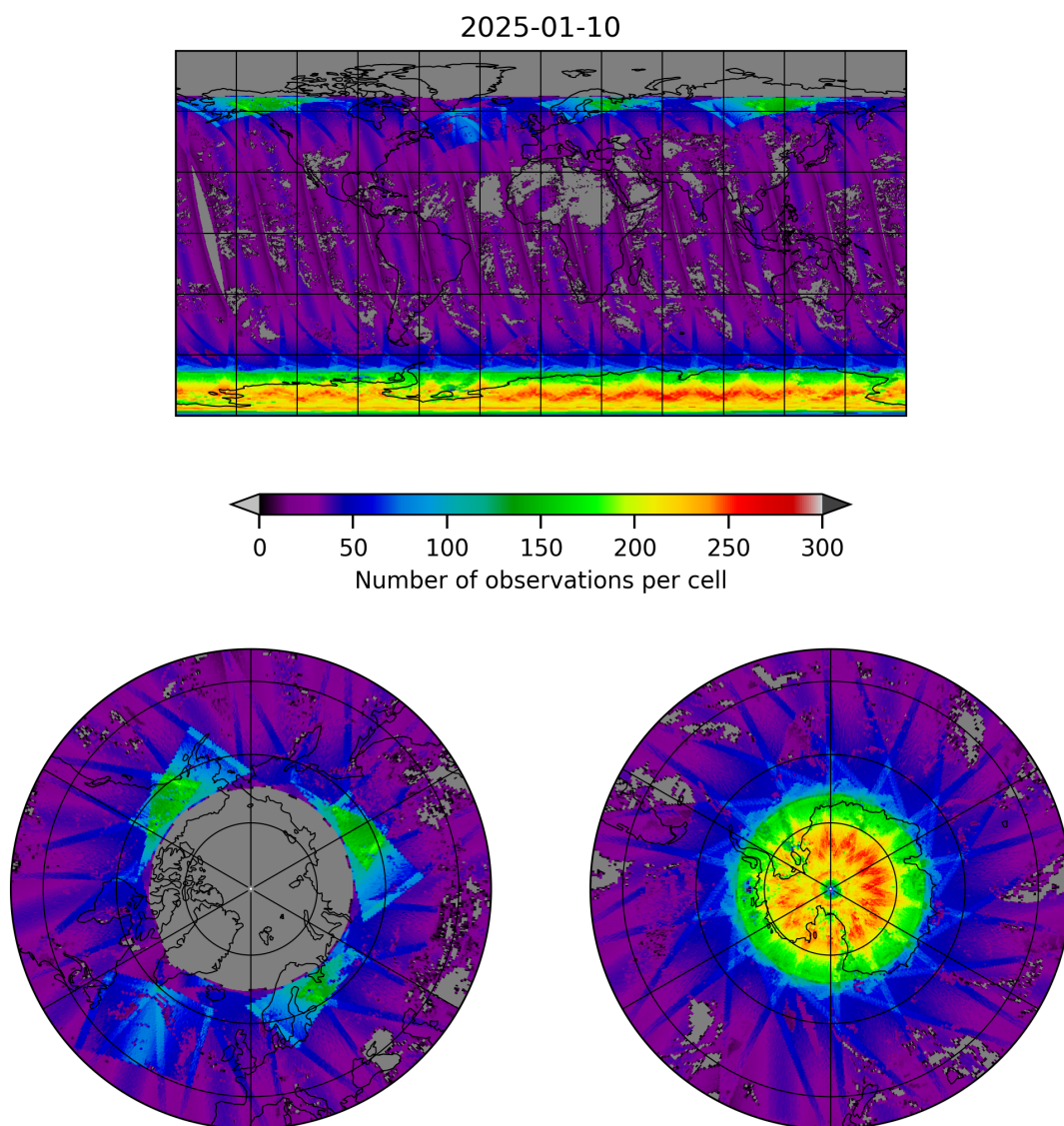
Figure 19: Map of the number of observations for 2025-01-10 to 2025-01-10
