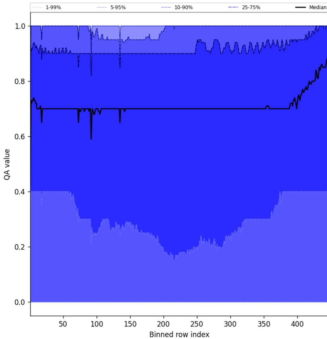
Figure 52: Along track statistics of “QA value” for 2025-01-10 to 2025-01-10
