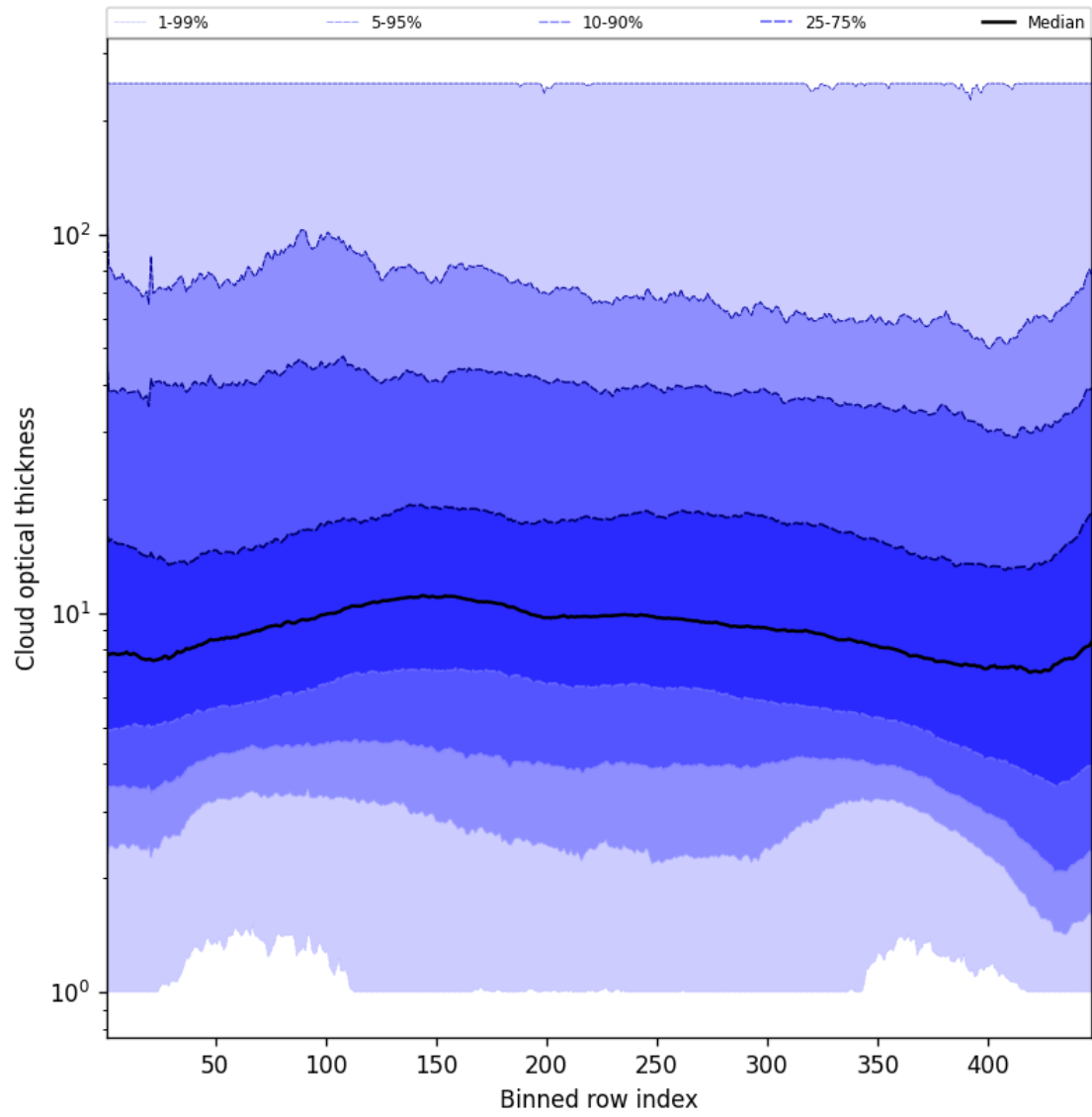
Figure 55: Along track statistics of “Cloud optical thickness” for 2025-01-10 to 2025-01-10
