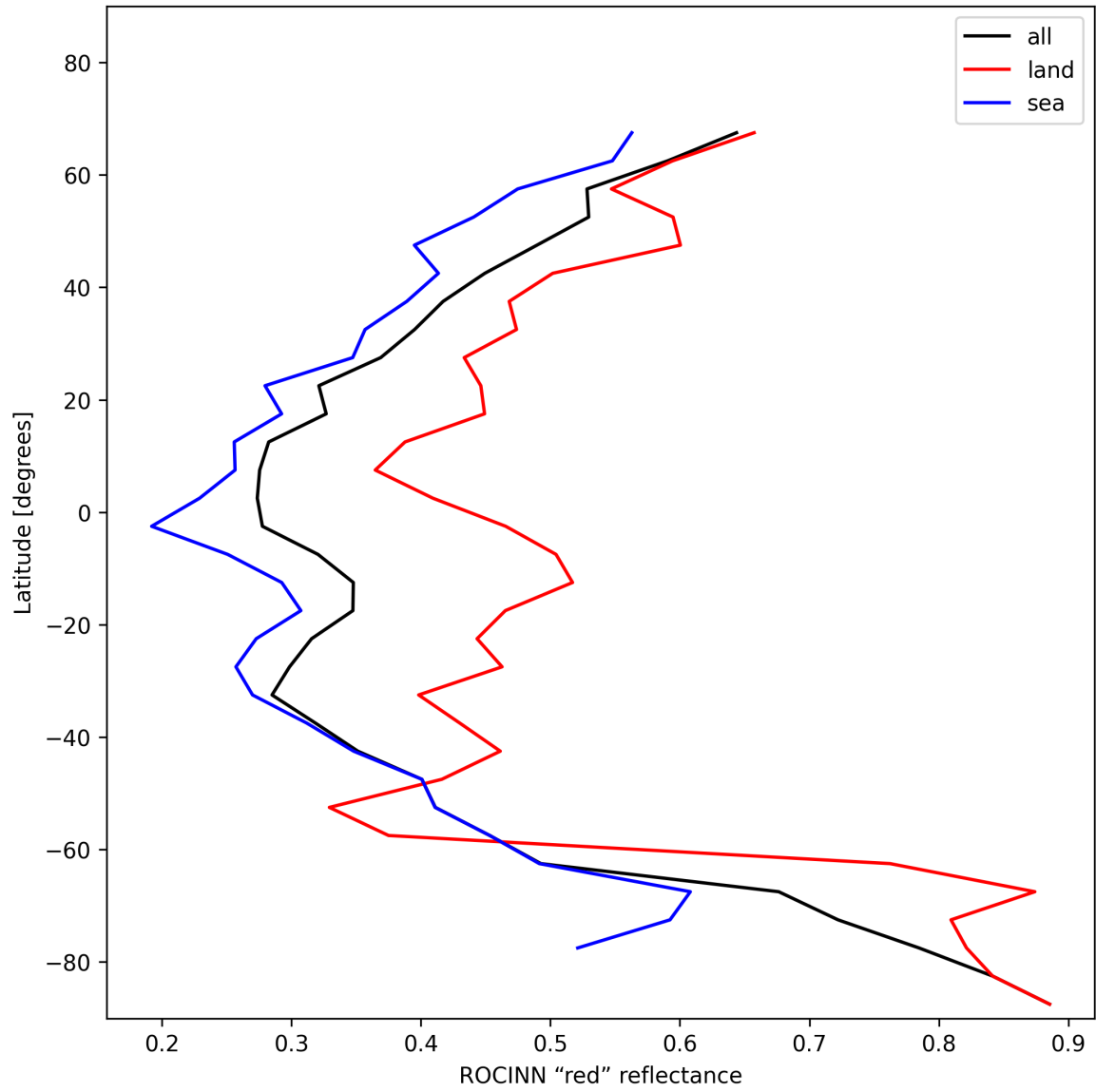
Figure 35: Zonal average of “ROCINN “red” reflectance” for 2025-01-10 to 2025-01-10.
