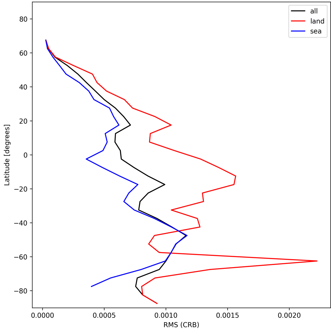
Figure 30: Zonal average of “RMS (CRB)” for 2025-01-10 to 2025-01-10.
