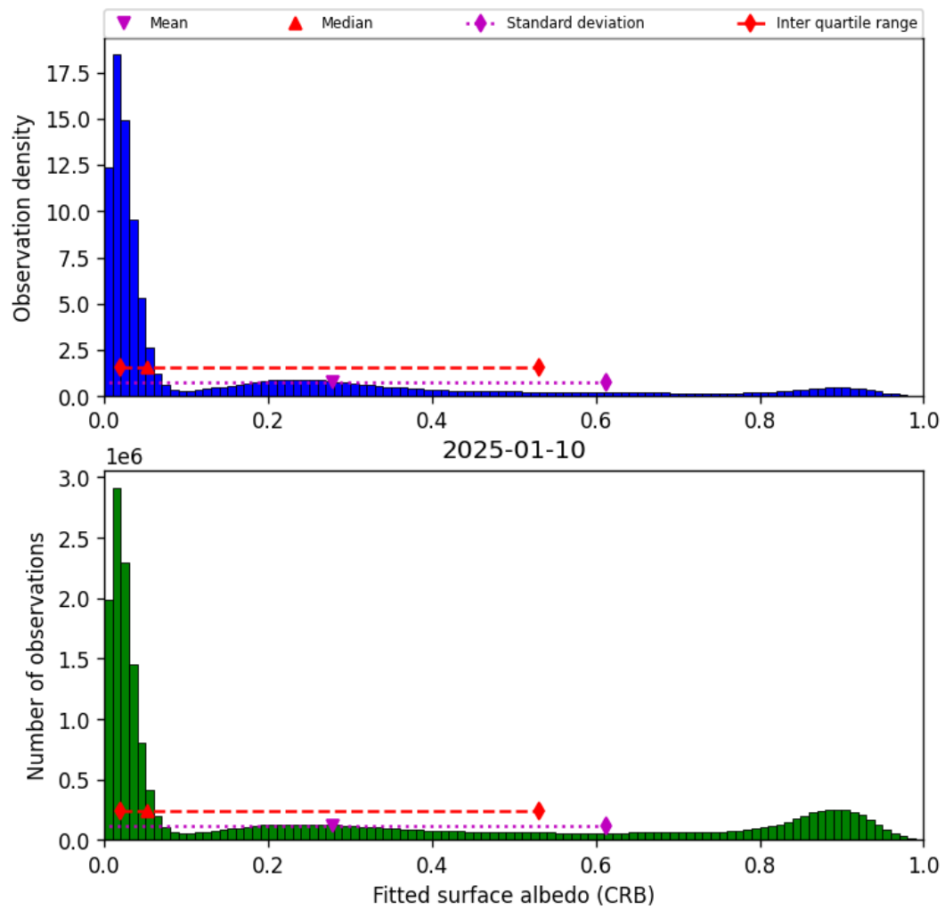
Figure 44: Histogram of “Fitted surface albedo (CRB)” for 2025-01-10 to 2025-01-10
