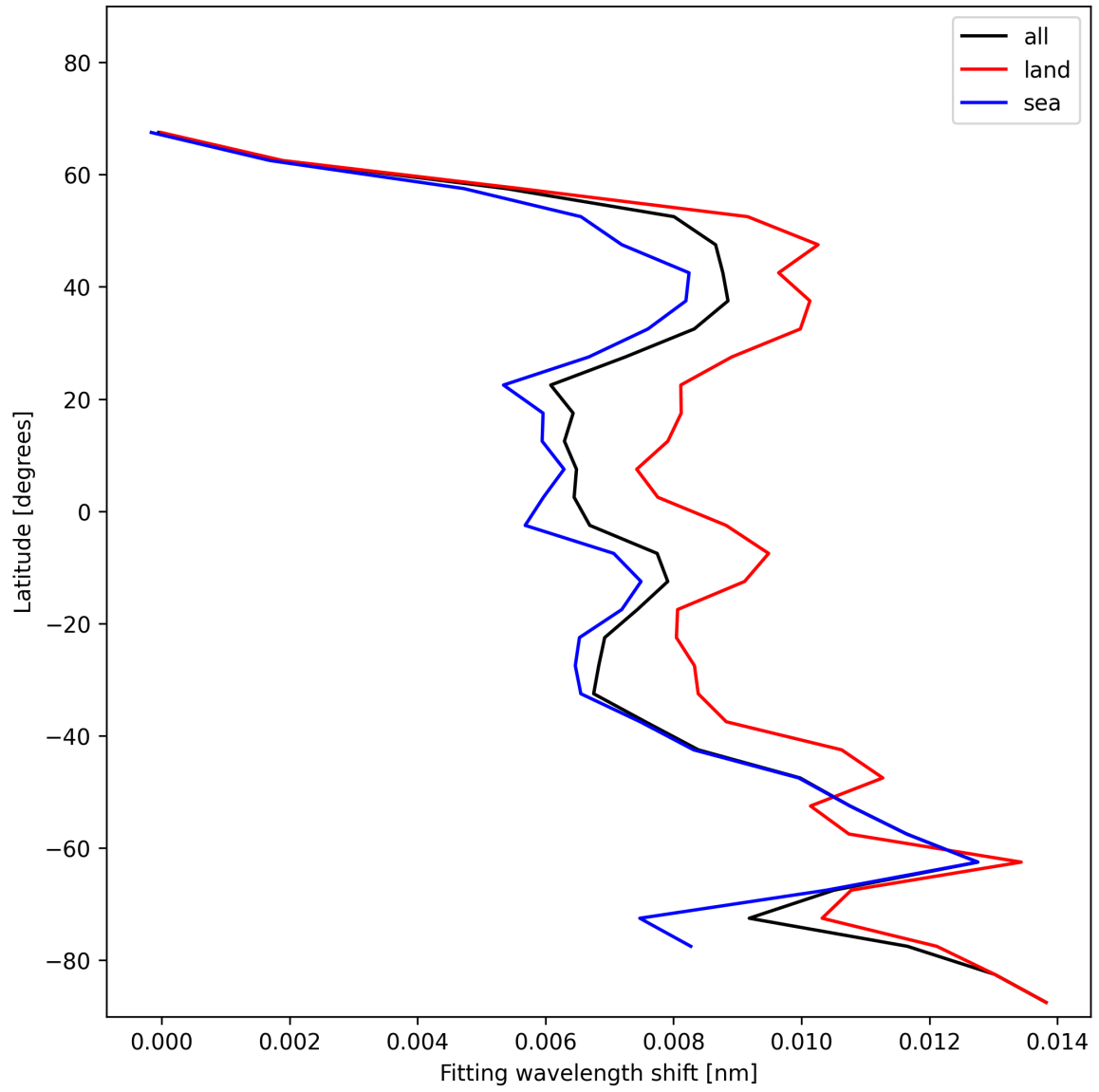
Figure 31: Zonal average of “Fitting wavelength shift” for 2025-01-10 to 2025-01-10.
