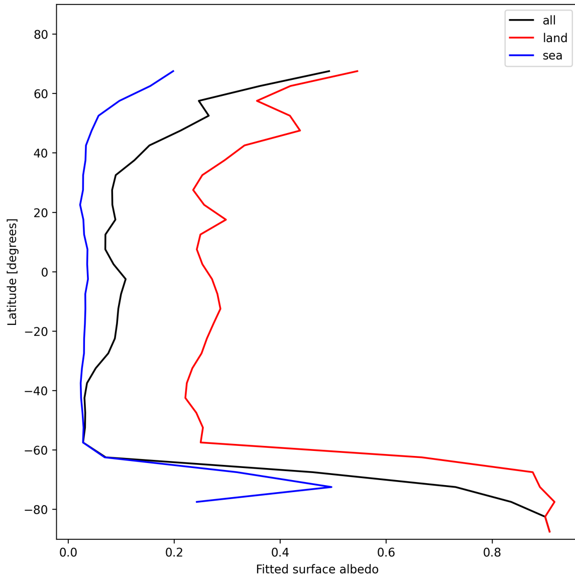
Figure 27: Zonal average of “Fitted surface albedo” for 2025-01-10 to 2025-01-10.
