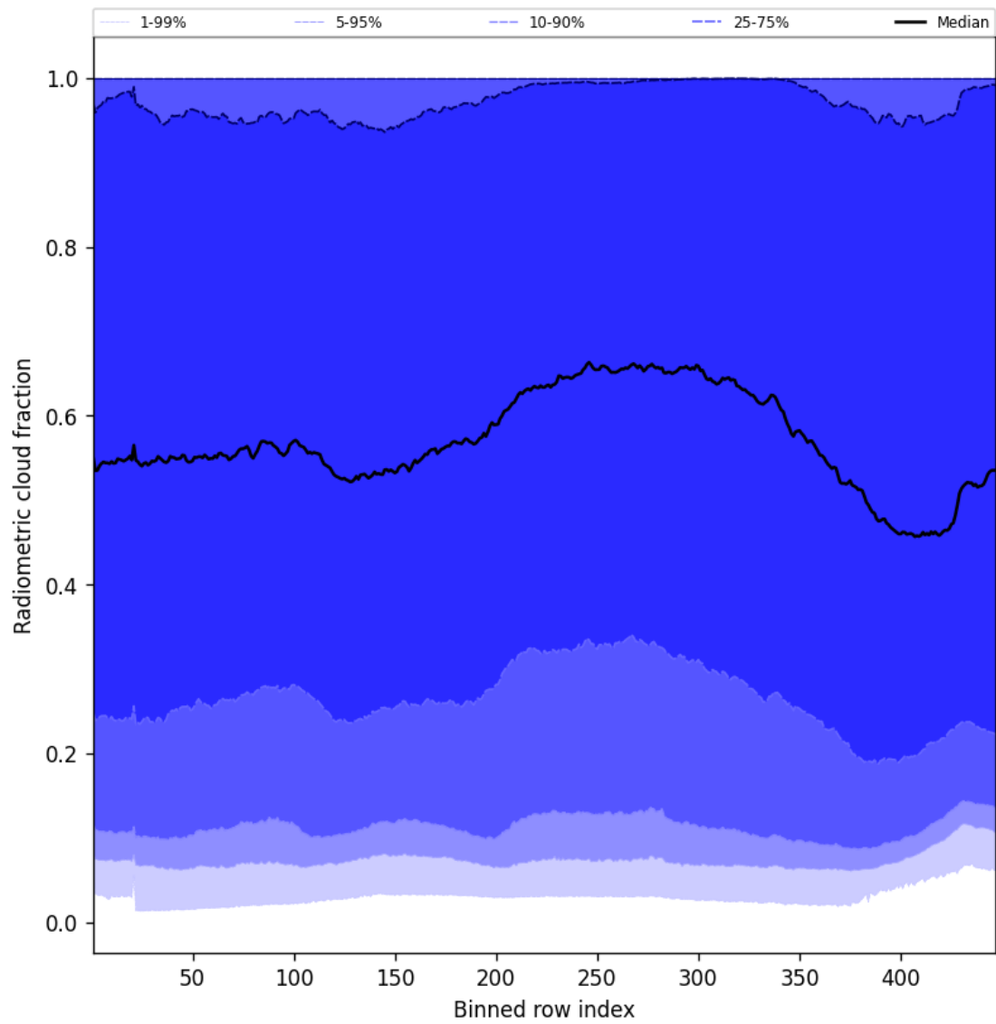
Figure 53: Along track statistics of “Radiometric cloud fraction” for 2025-01-10 to 2025-01-10
