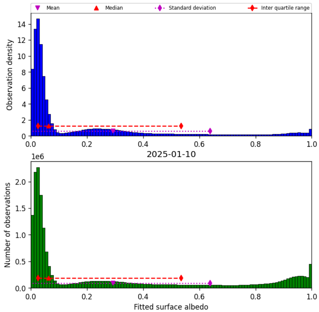
Figure 43: Histogram of “Fitted surface albedo” for 2025-01-10 to 2025-01-10
