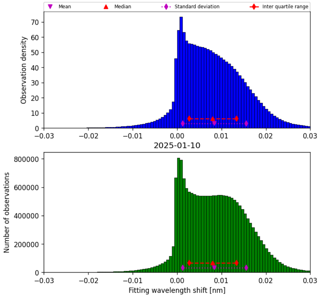
Figure 47: Histogram of “Fitting wavelength shift” for 2025-01-10 to 2025-01-10
