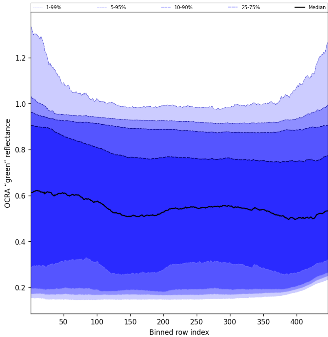
Figure 66: Along track statistics of “OCRA “green” reflectance” for 2025-01-10 to 2025-01-10
