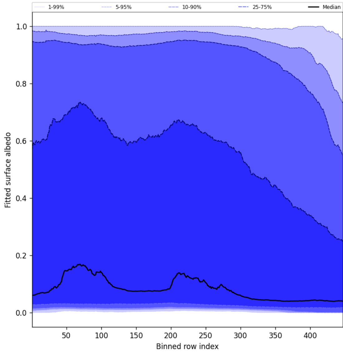
Figure 59: Along track statistics of “Fitted surface albedo” for 2025-01-10 to 2025-01-10
