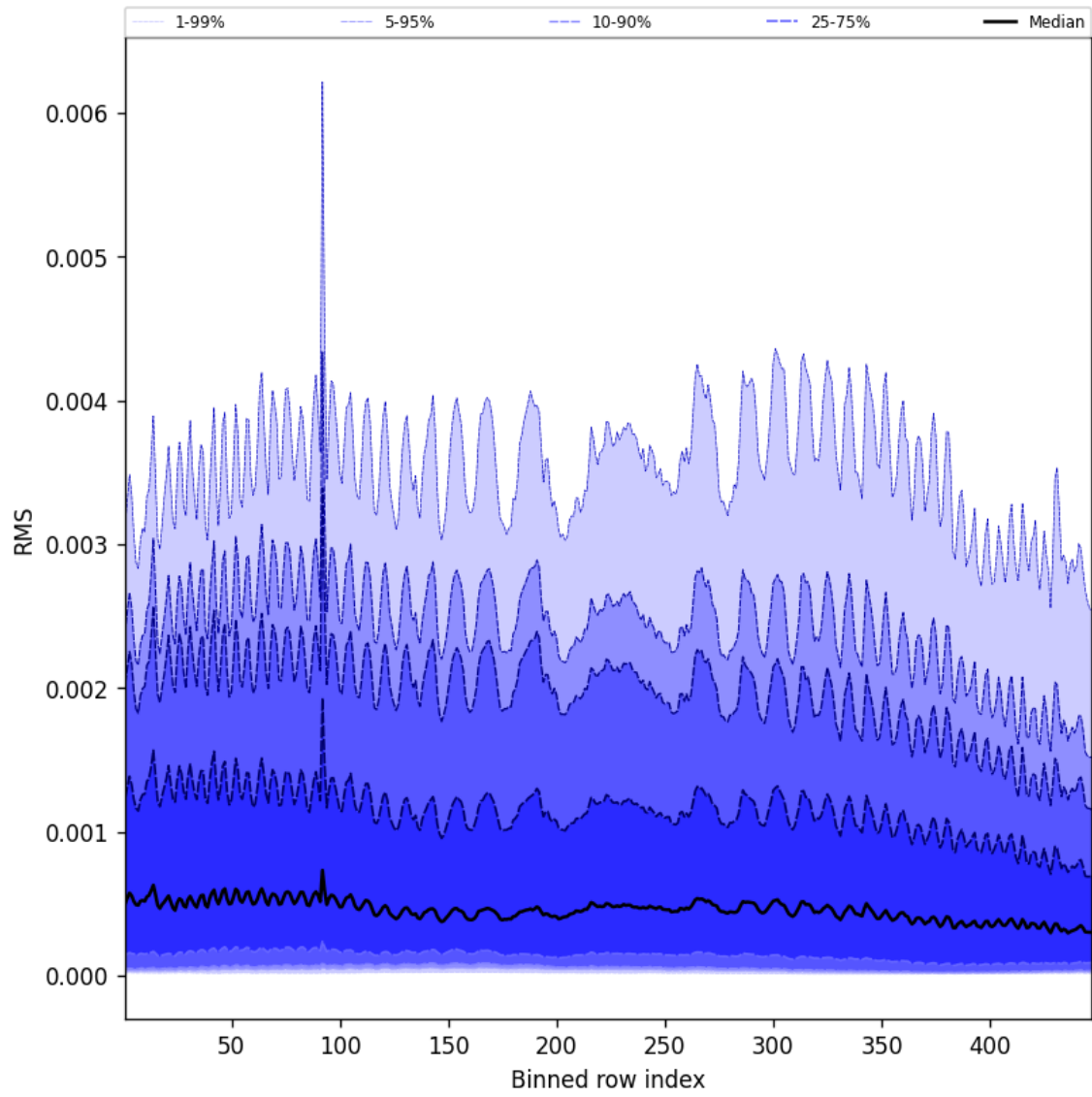
Figure 61: Along track statistics of “RMS” for 2025-01-10 to 2025-01-10
