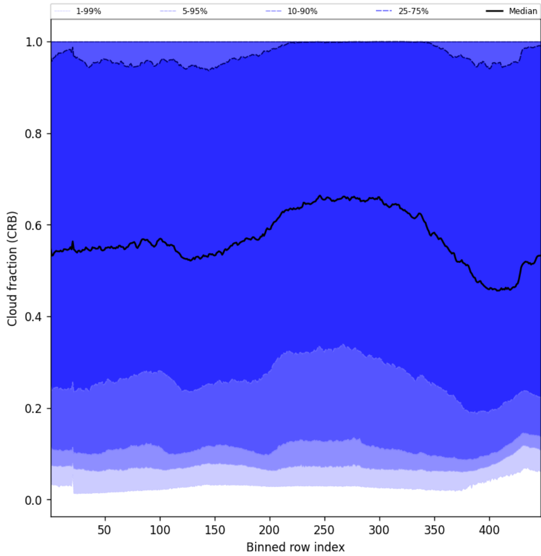
Figure 56: Along track statistics of “Cloud fraction (CRB)” for 2025-01-10 to 2025-01-10
