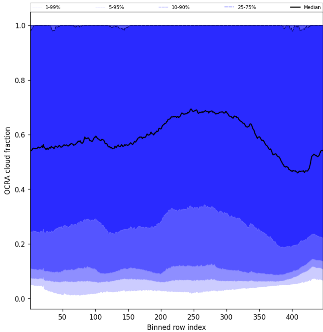
Figure 64: Along track statistics of “OCRA cloud fraction” for 2025-01-10 to 2025-01-10
