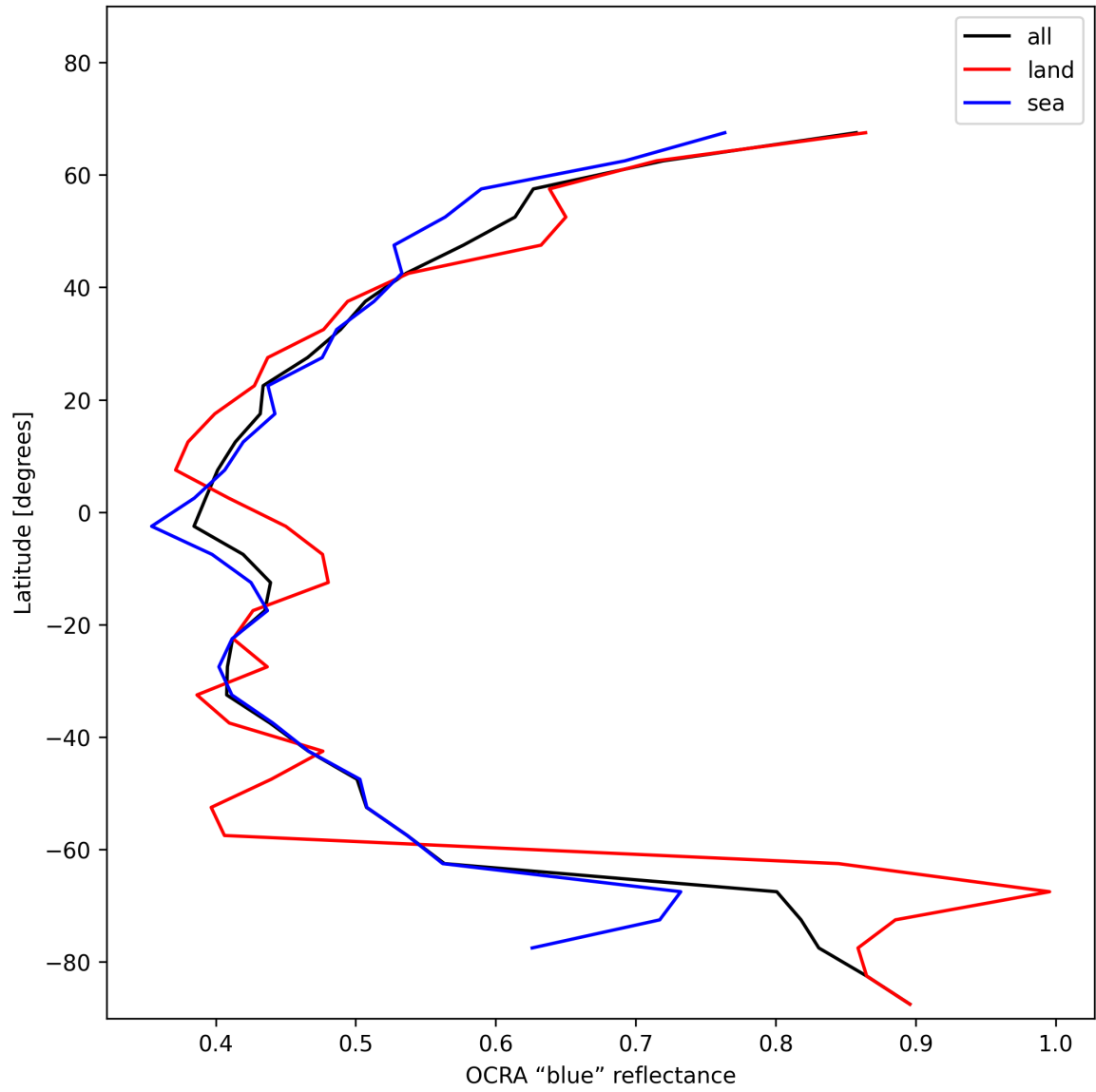
Figure 33: Zonal average of “OCRA “blue” reflectance” for 2025-01-10 to 2025-01-10.
