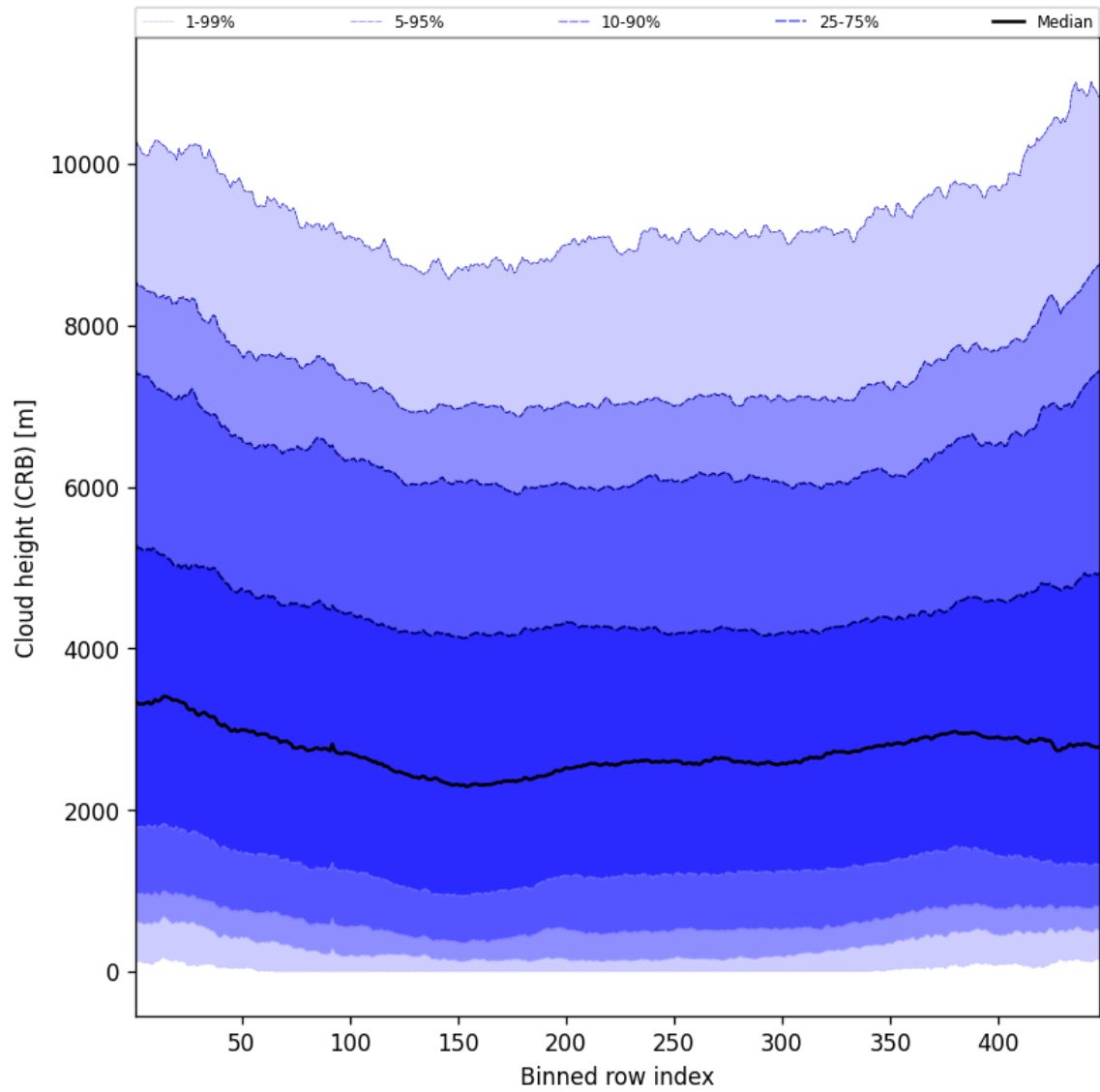
Figure 57: Along track statistics of “Cloud height (CRB)” for 2025-01-10 to 2025-01-10
