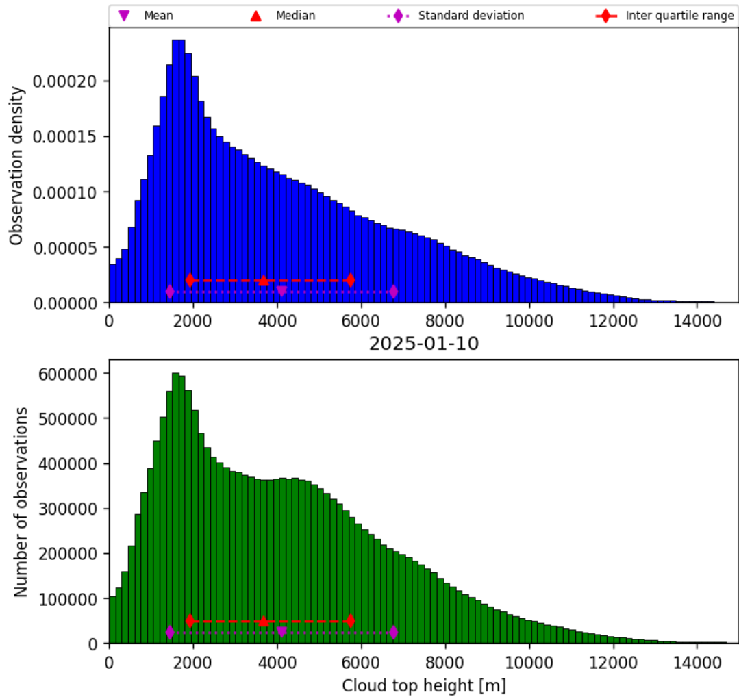
Figure 38: Histogram of “Cloud top height” for 2025-01-10 to 2025-01-10
