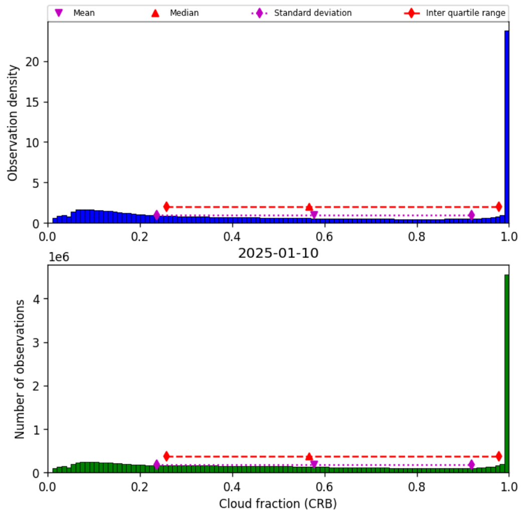
Figure 40: Histogram of “Cloud fraction (CRB)” for 2025-01-10 to 2025-01-10
