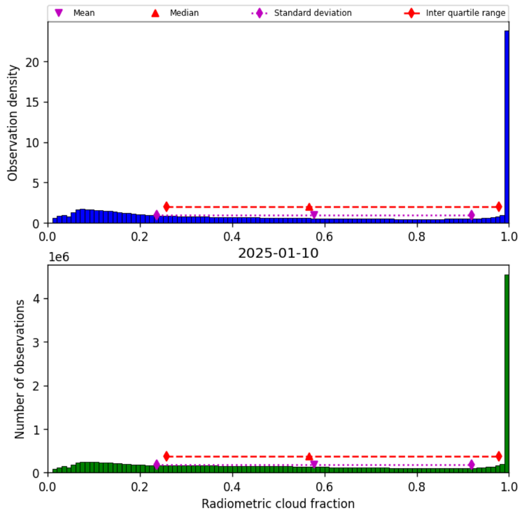
Figure 37: Histogram of “Radiometric cloud fraction” for 2025-01-10 to 2025-01-10
