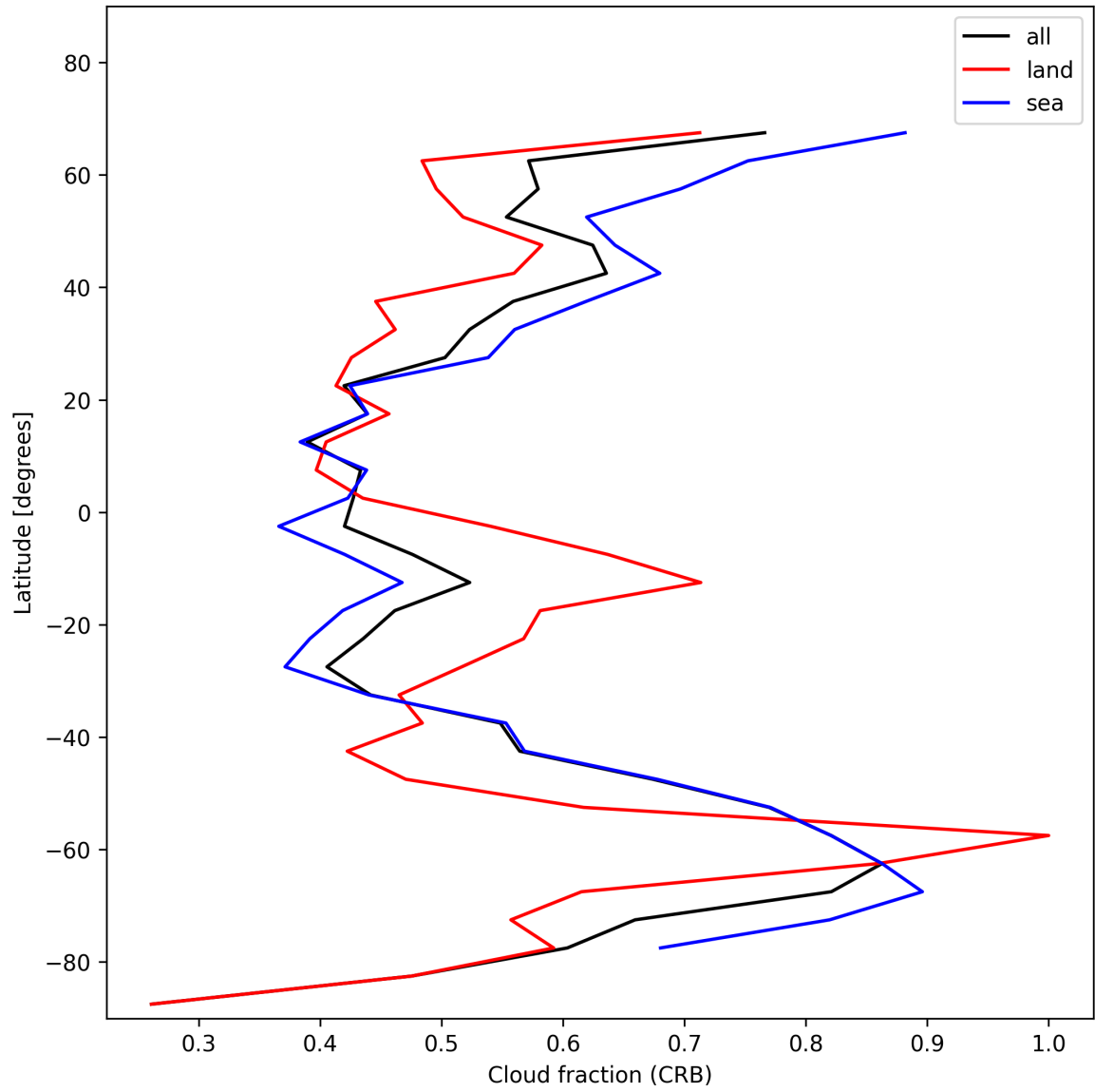
Figure 24: Zonal average of “Cloud fraction (CRB)” for 2025-01-12 to 2025-01-13.
