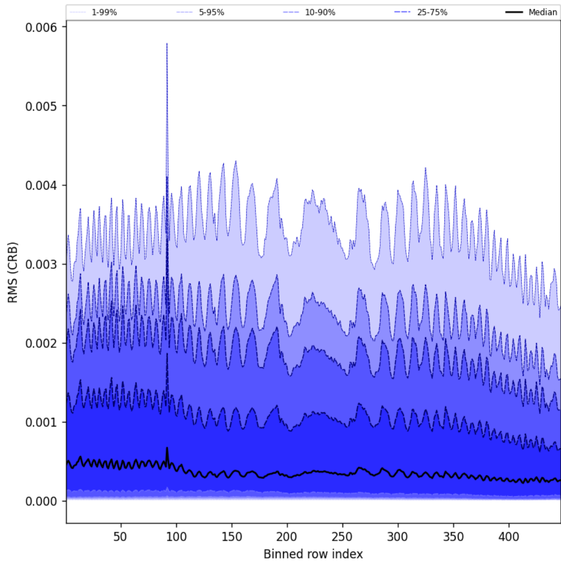
Figure 62: Along track statistics of “RMS (CRB)” for 2025-01-12 to 2025-01-13
