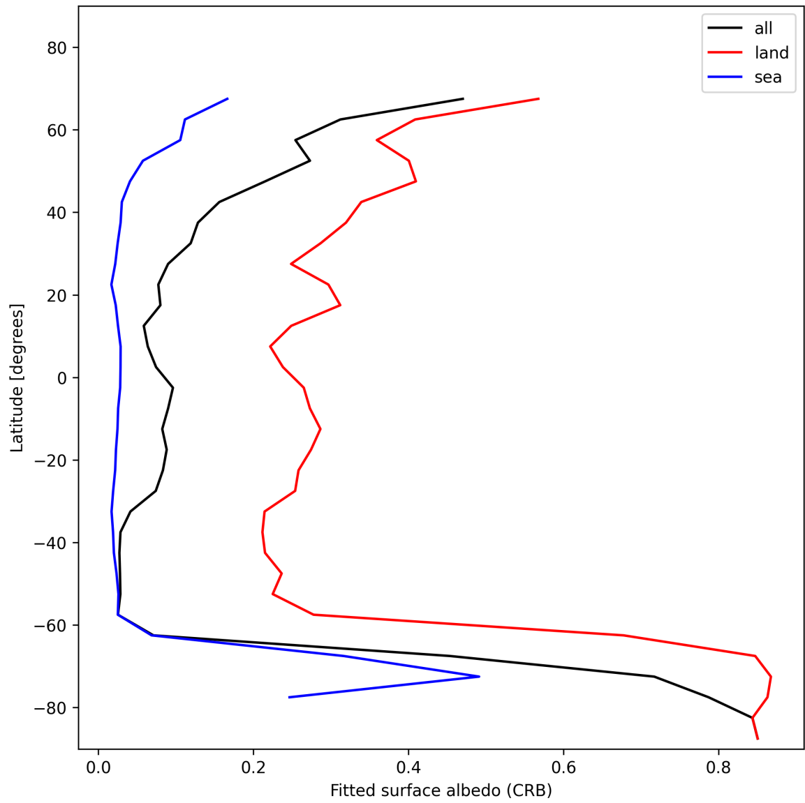
Figure 28: Zonal average of “Fitted surface albedo (CRB)” for 2025-01-12 to 2025-01-13.
