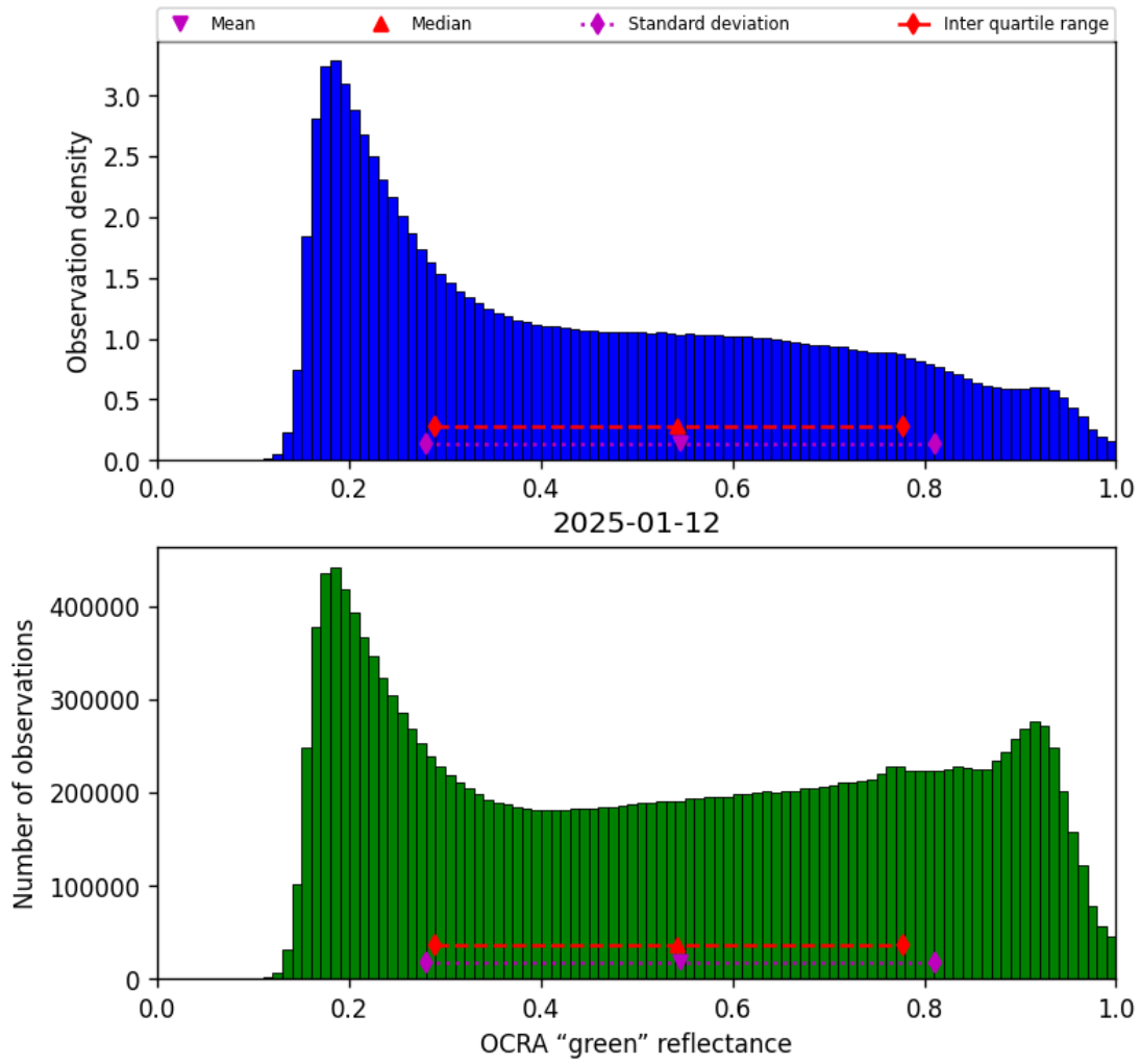
Figure 50: Histogram of “OCRA “green” reflectance” for 2025-01-12 to 2025-01-13
