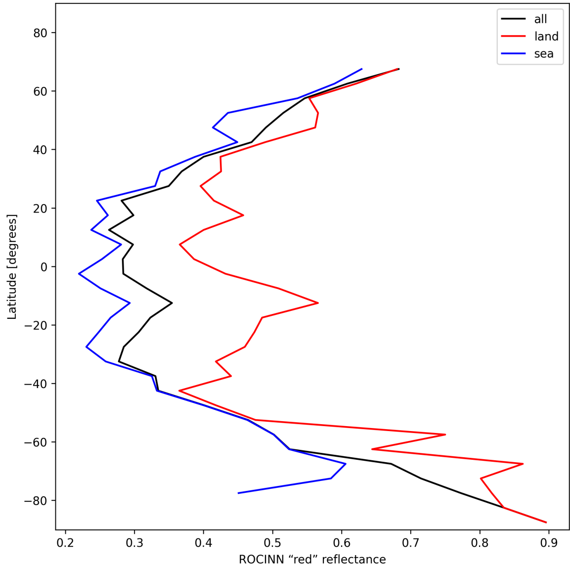
Figure 35: Zonal average of “ROCINN “red” reflectance” for 2025-01-12 to 2025-01-13.
