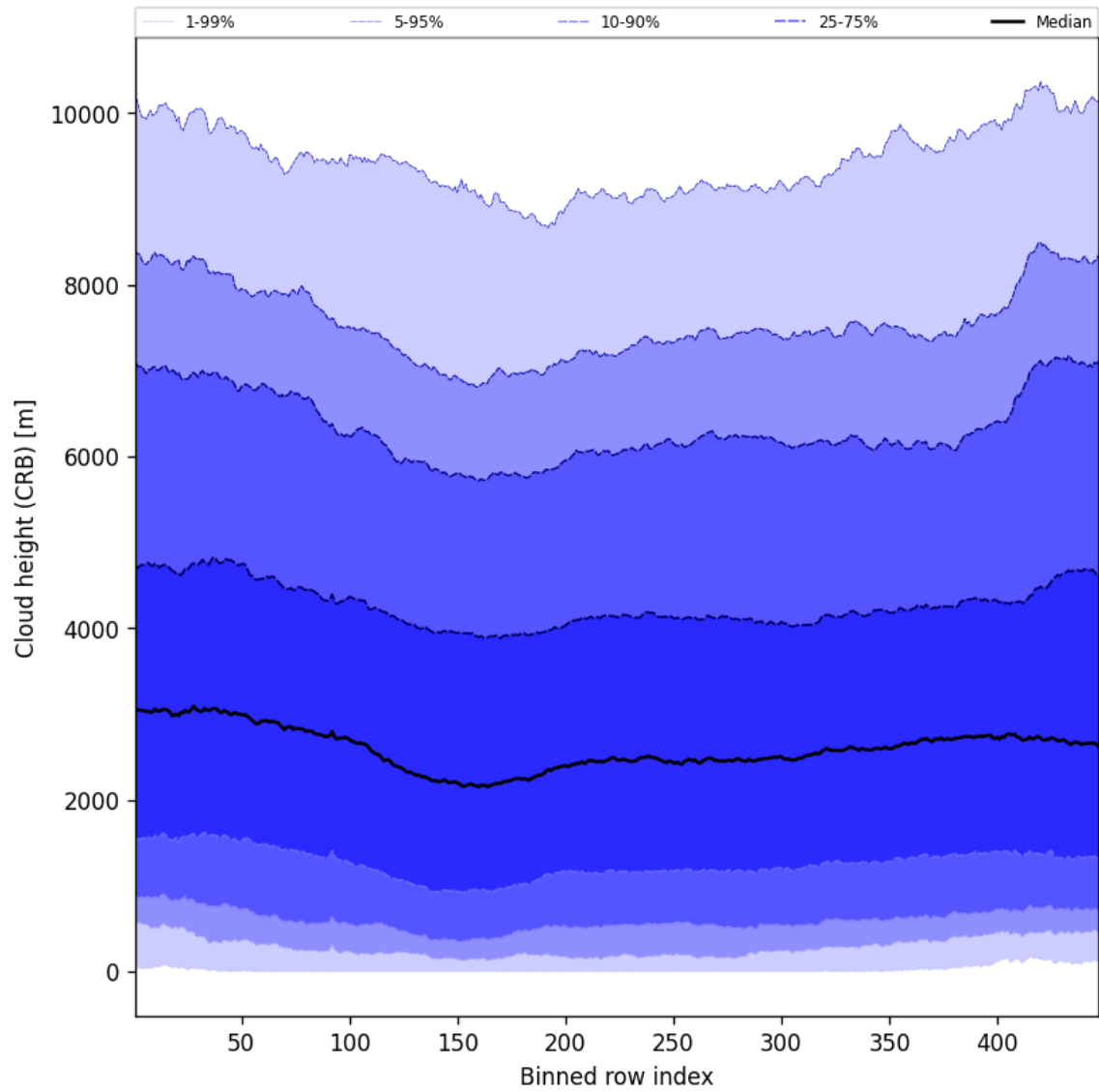
Figure 57: Along track statistics of “Cloud height (CRB)” for 2025-01-12 to 2025-01-13
