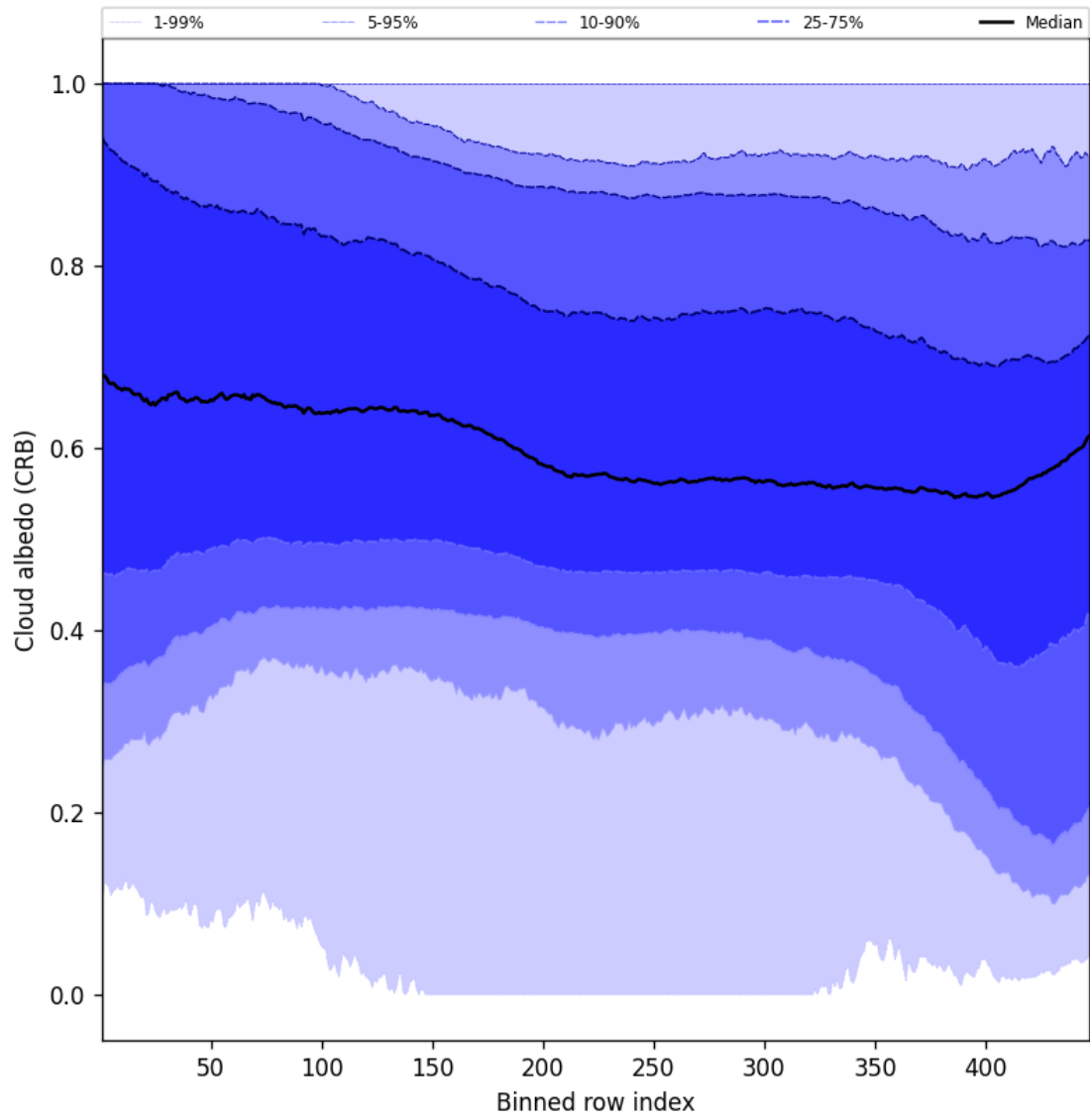
Figure 58: Along track statistics of “Cloud albedo (CRB)” for 2025-01-12 to 2025-01-13
