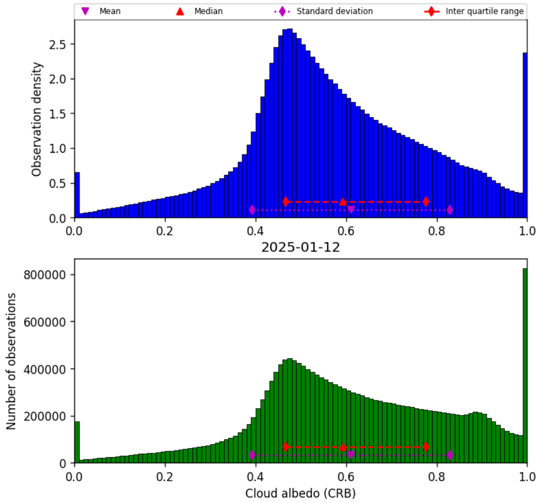
Figure 42: Histogram of “Cloud albedo (CRB)” for 2025-01-12 to 2025-01-13
