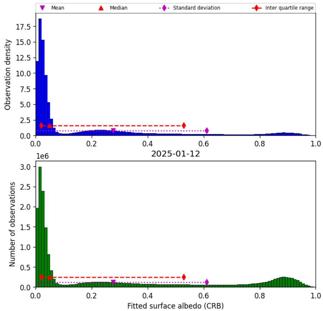
Figure 44: Histogram of “Fitted surface albedo (CRB)” for 2025-01-12 to 2025-01-13
