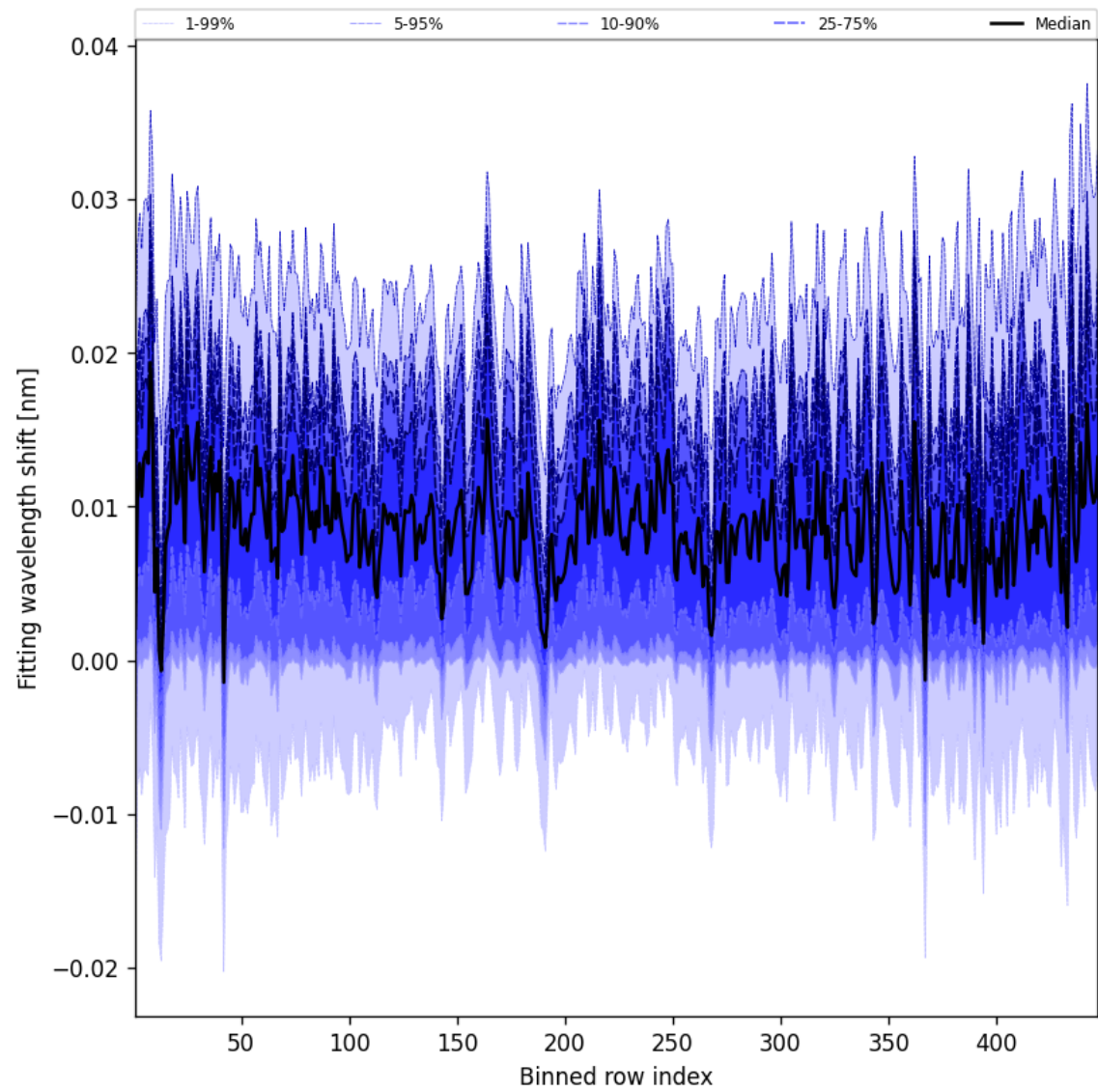
Figure 63: Along track statistics of “Fitting wavelength shift” for 2025-01-12 to 2025-01-13
