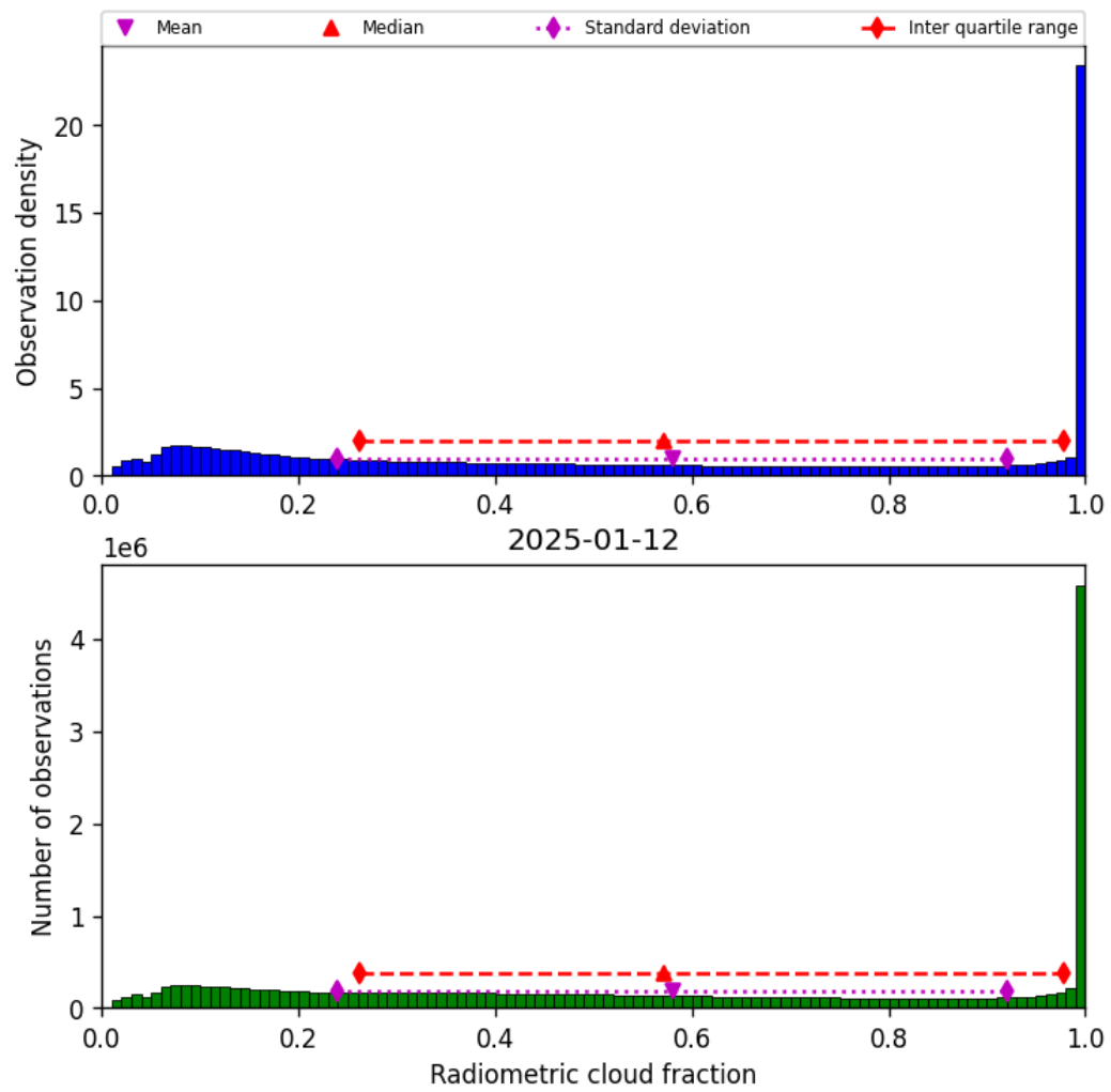
Figure 37: Histogram of “Radiometric cloud fraction” for 2025-01-12 to 2025-01-13
