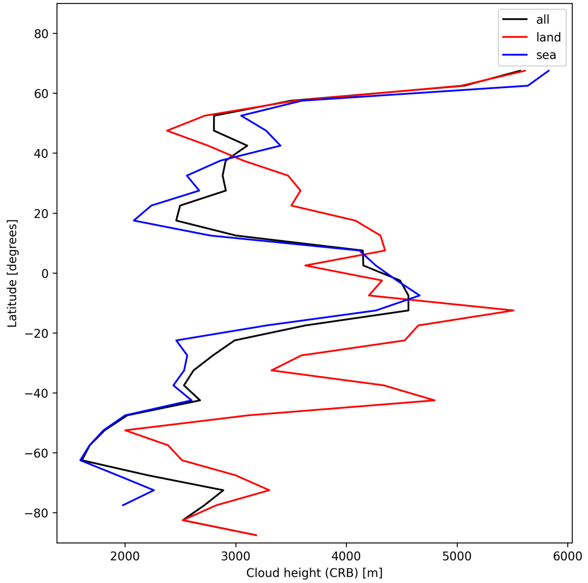
Figure 25: Zonal average of “Cloud height (CRB)” for 2025-01-12 to 2025-01-13.
