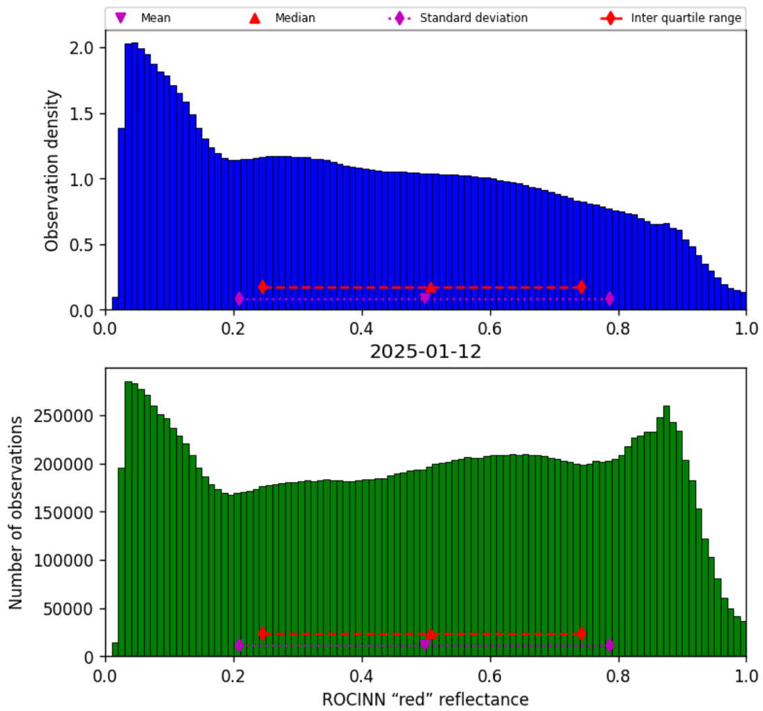
Figure 51: Histogram of “ROCINN “red” reflectance” for 2025-01-12 to 2025-01-13
