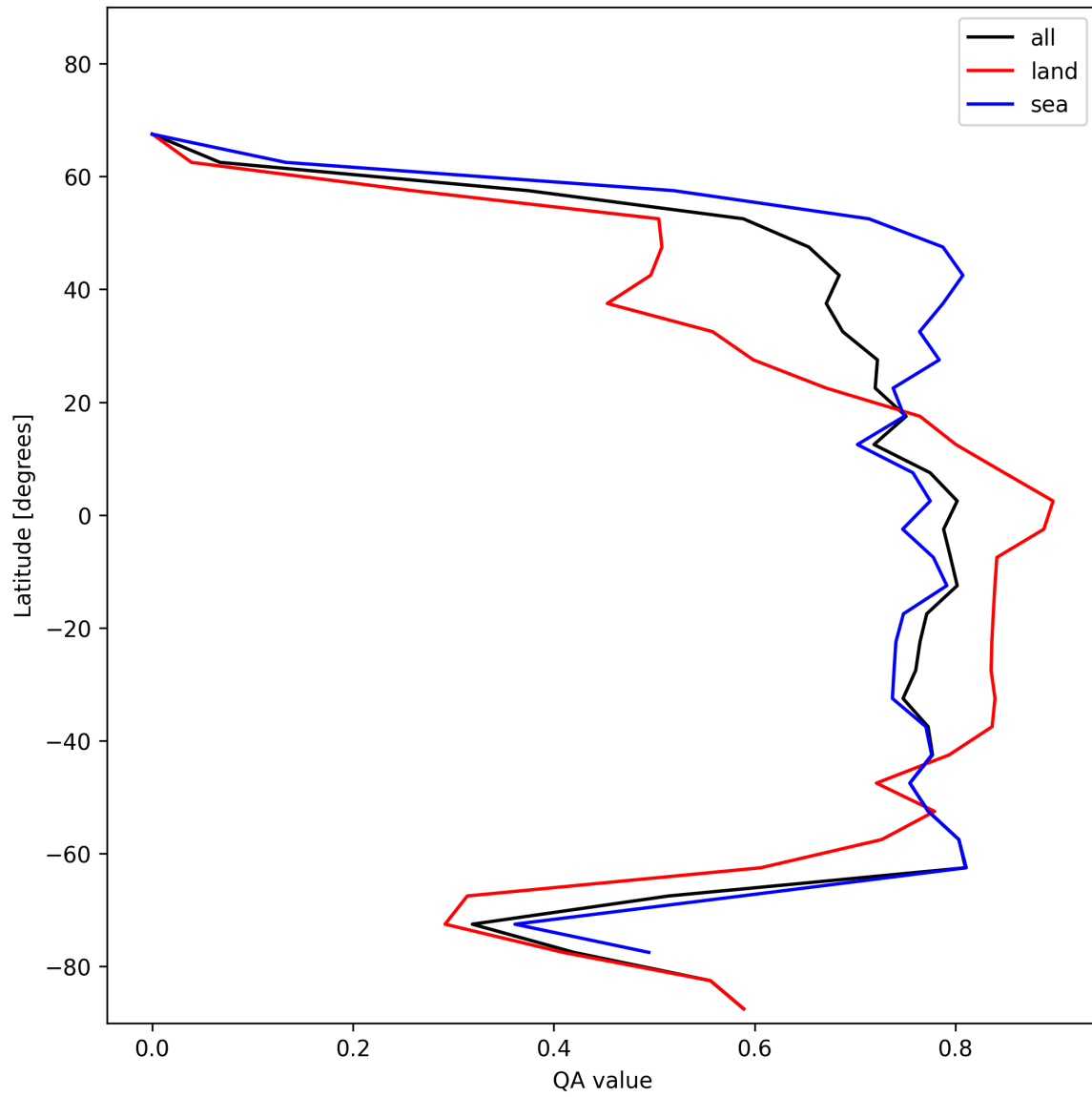
Figure 20: Zonal average of “QA value” for 2025-01-12 to 2025-01-13.
