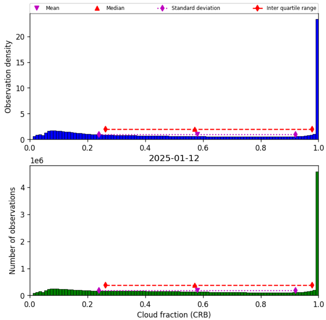
Figure 40: Histogram of “Cloud fraction (CRB)” for 2025-01-12 to 2025-01-13
