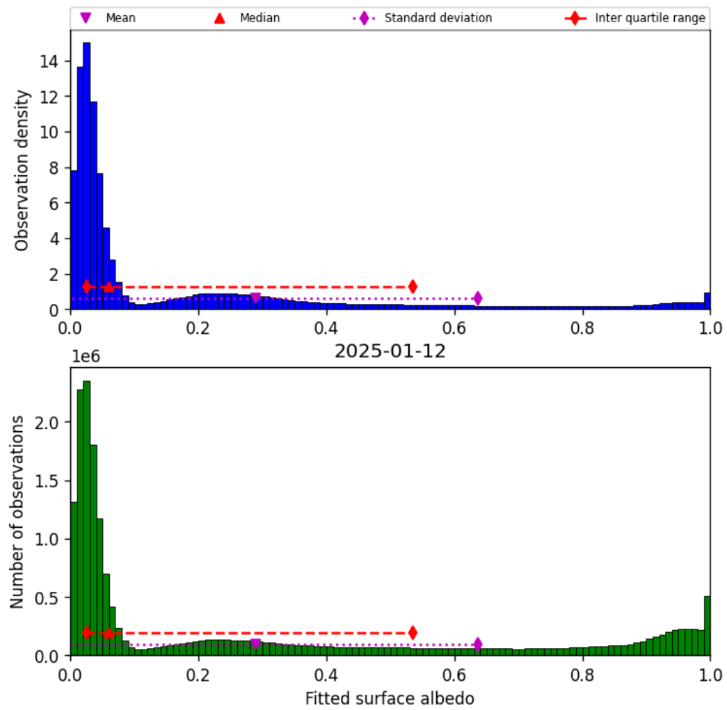
Figure 43: Histogram of “Fitted surface albedo” for 2025-01-12 to 2025-01-13
