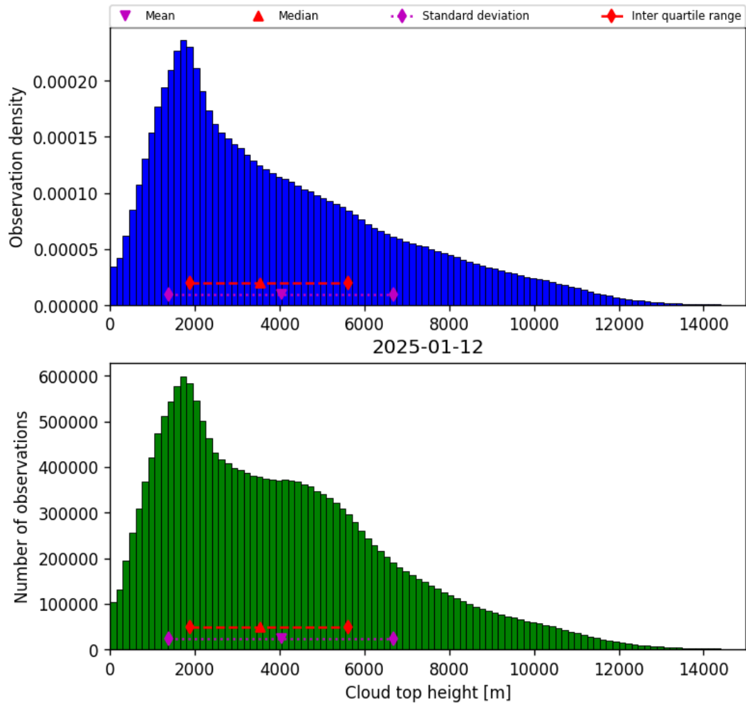
Figure 38: Histogram of “Cloud top height” for 2025-01-12 to 2025-01-13
