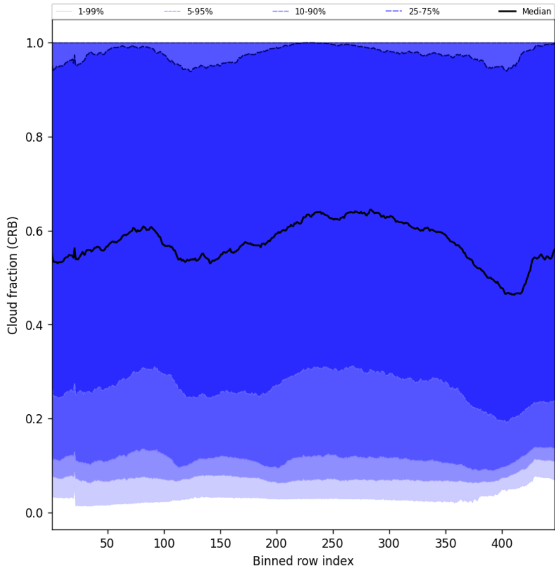
Figure 56: Along track statistics of “Cloud fraction (CRB)” for 2025-01-12 to 2025-01-13
