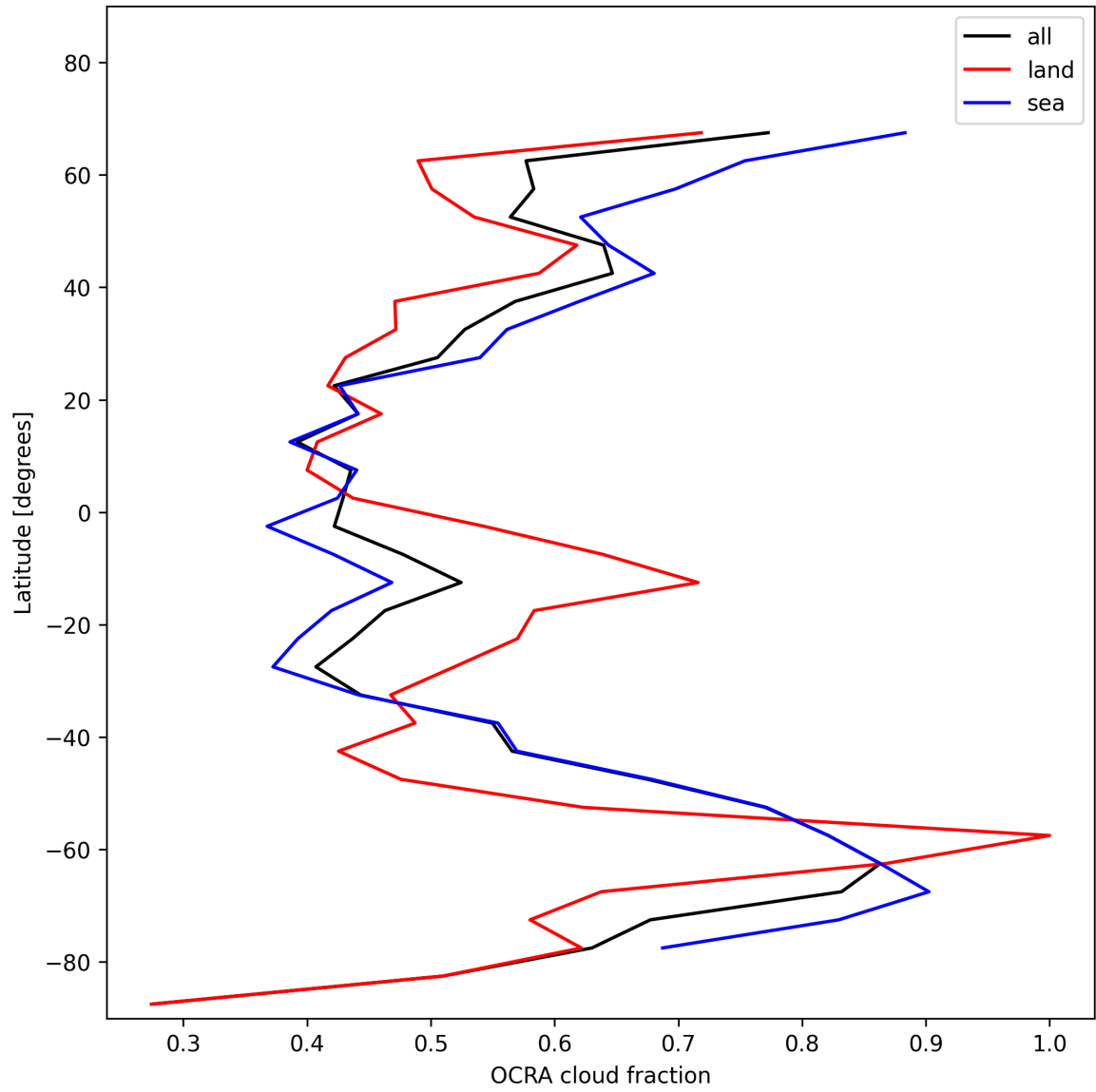
Figure 32: Zonal average of “OCRA cloud fraction” for 2025-01-12 to 2025-01-13.
