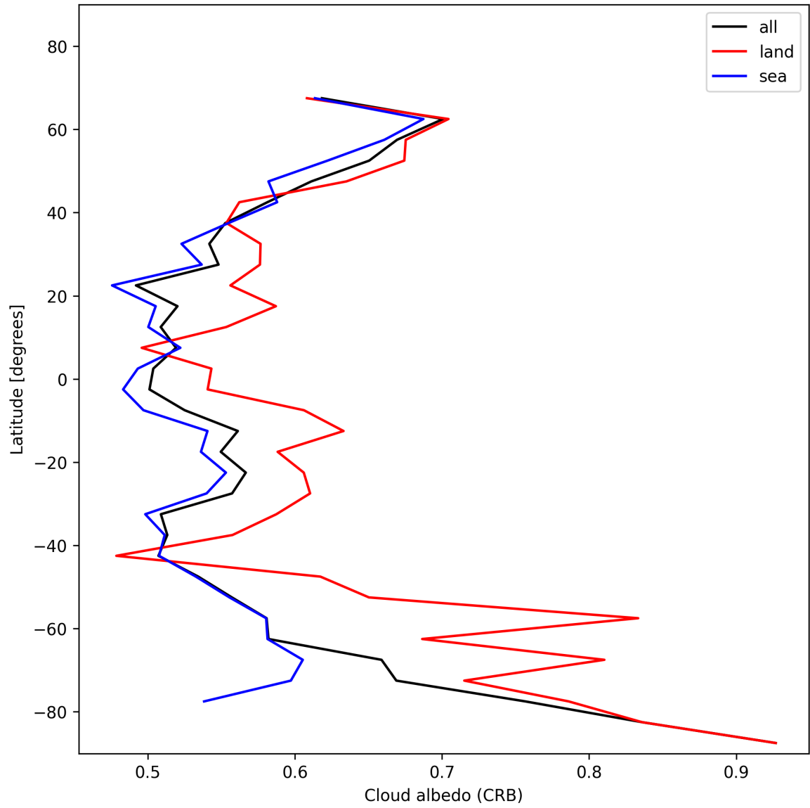
Figure 26: Zonal average of “Cloud albedo (CRB)” for 2025-01-12 to 2025-01-13.
