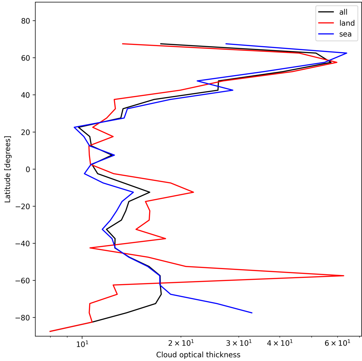
Figure 23: Zonal average of “Cloud optical thickness” for 2025-01-12 to 2025-01-13.
