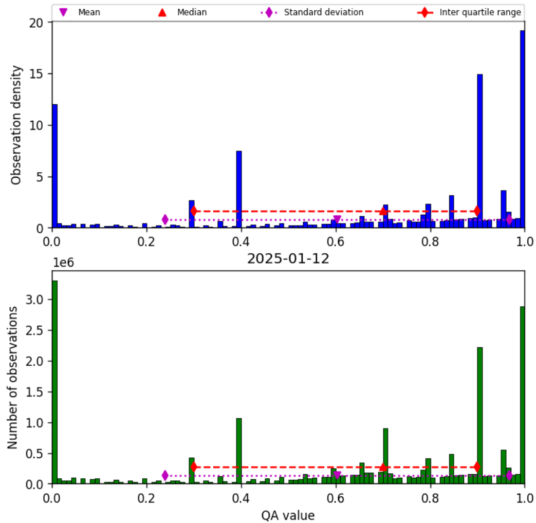
Figure 36: Histogram of “QA value” for 2025-01-12 to 2025-01-13
