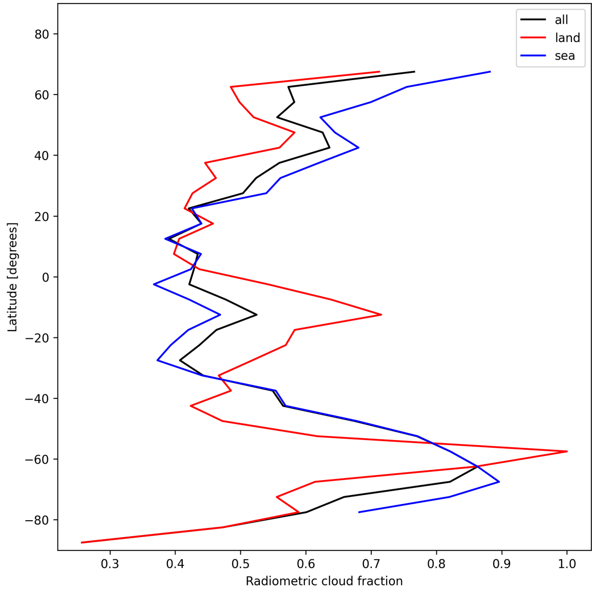
Figure 21: Zonal average of “Radiometric cloud fraction” for 2025-01-12 to 2025-01-13.
