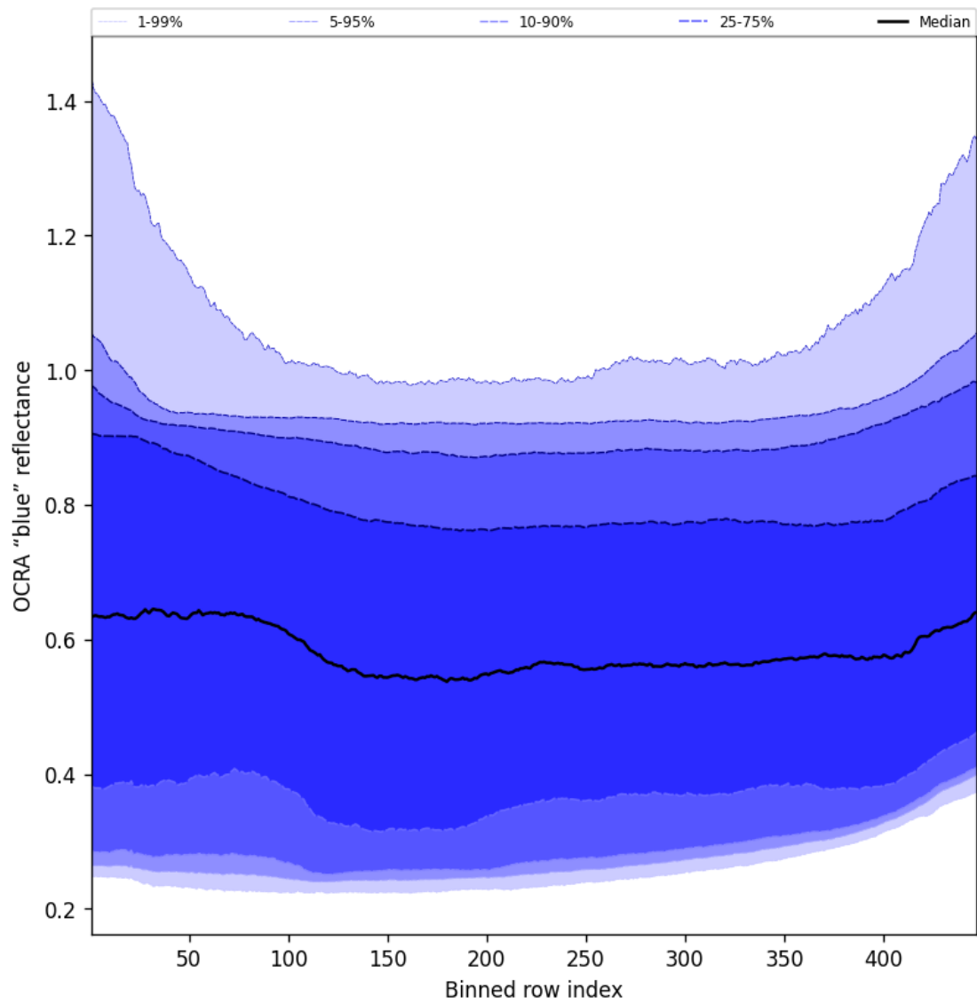
Figure 65: Along track statistics of "OCRA "blue" reflectance" for 2025-01-12 to 2025-01-13
