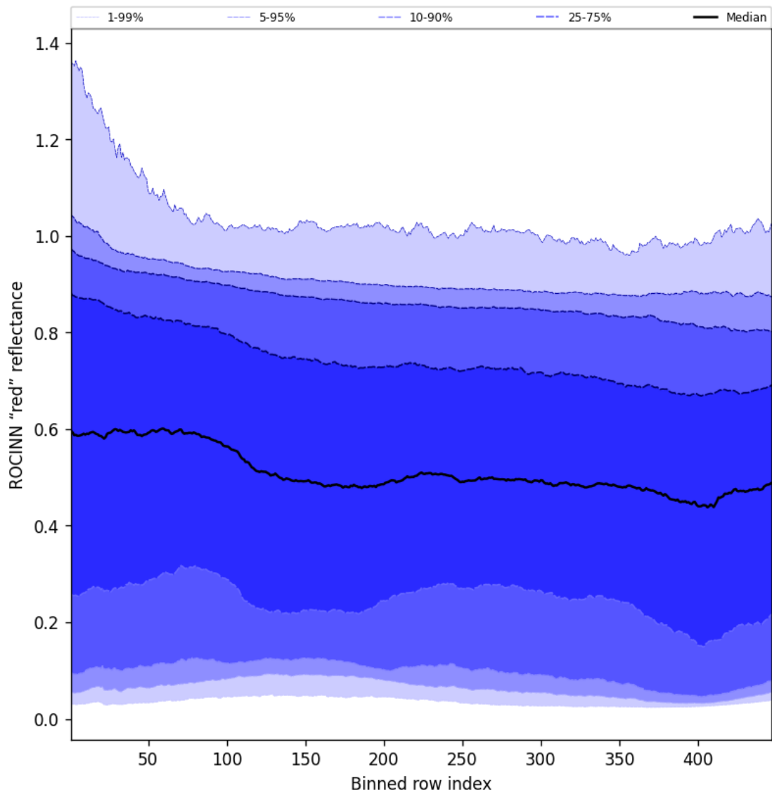
Figure 67: Along track statistics of “ROCINN “red” reflectance” for 2025-01-12 to 2025-01-13
