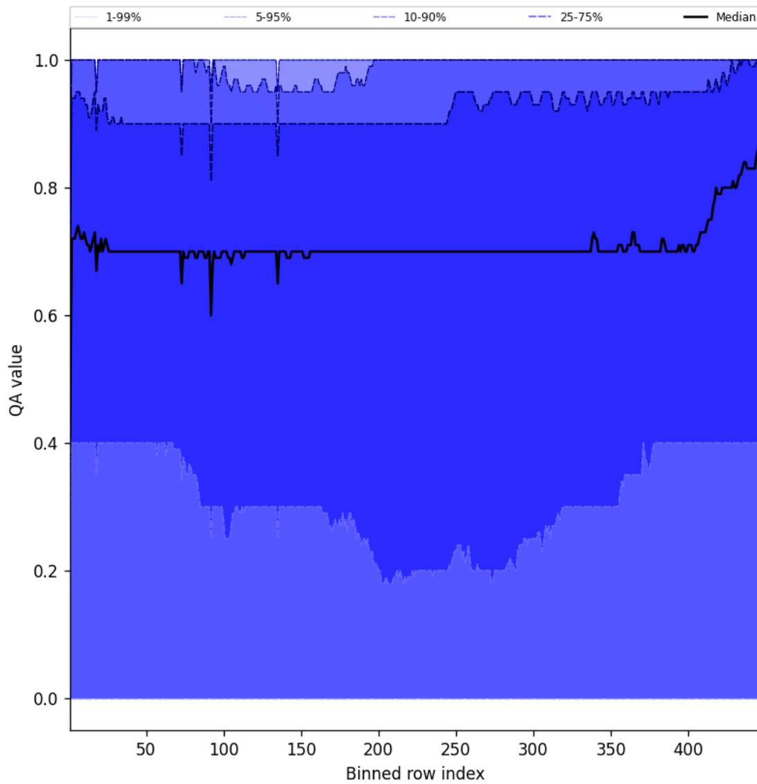
Figure 52: Along track statistics of “QA value” for 2025-01-12 to 2025-01-13
