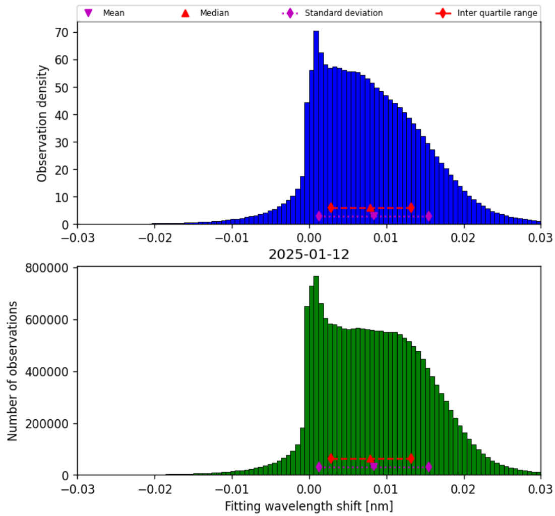
Figure 47: Histogram of “Fitting wavelength shift” for 2025-01-12 to 2025-01-13
