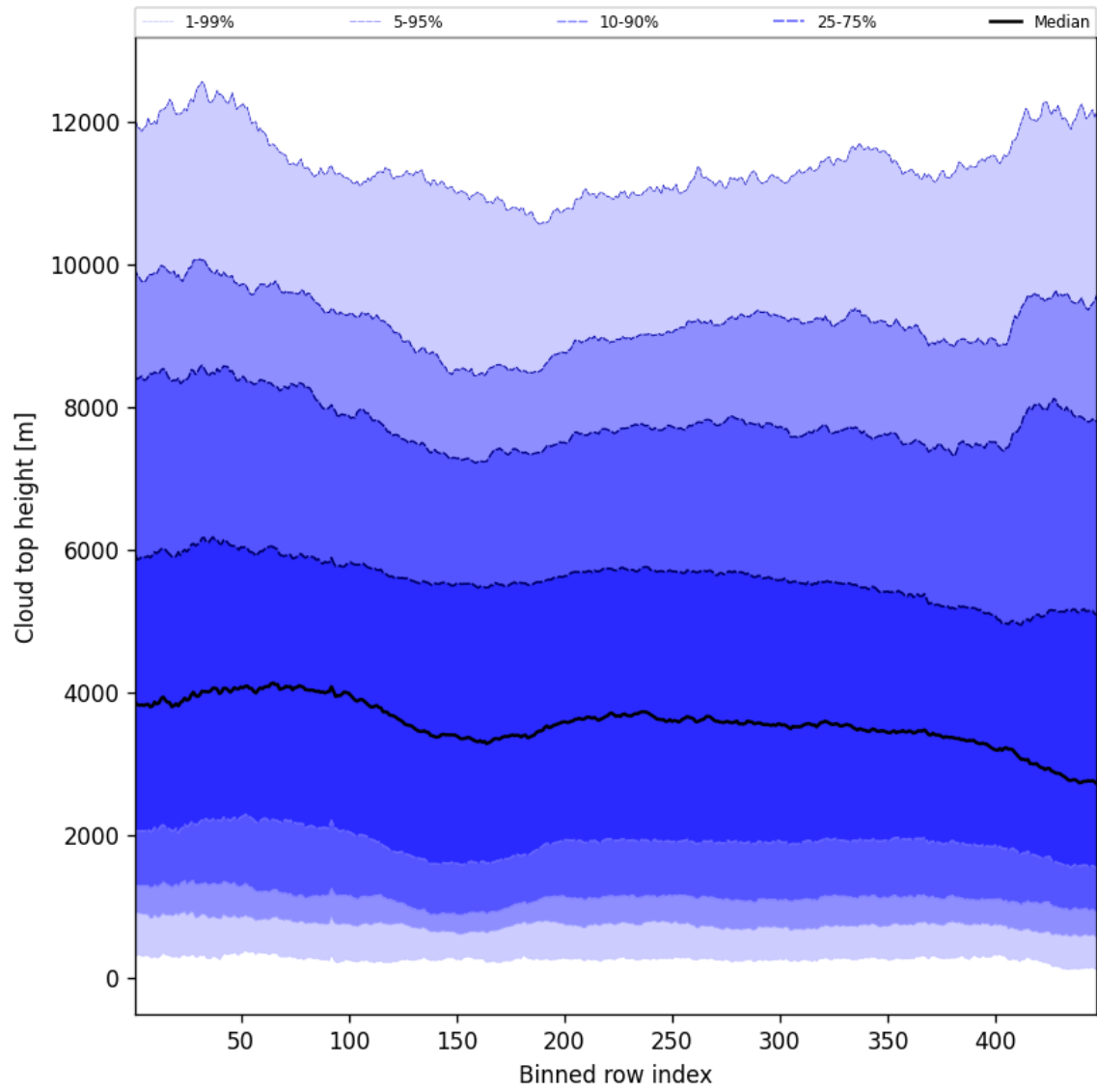
Figure 54: Along track statistics of “Cloud top height” for 2025-01-12 to 2025-01-13
