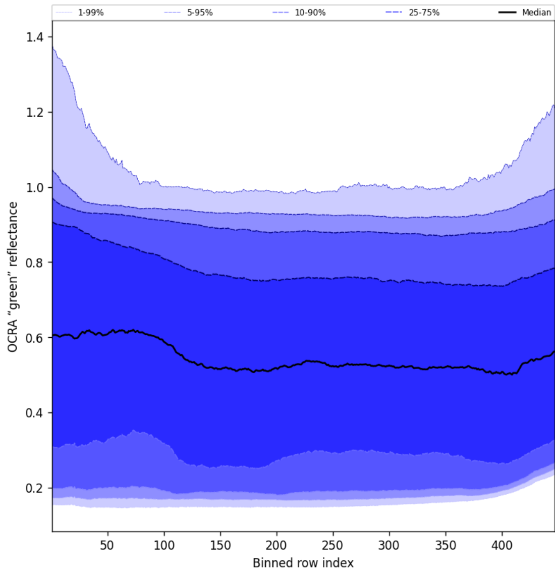
Figure 66: Along track statistics of “OCRA “green” reflectance” for 2025-01-12 to 2025-01-13
