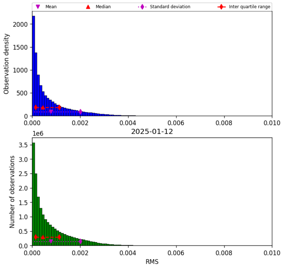
Figure 45: Histogram of “RMS” for 2025-01-12 to 2025-01-13
