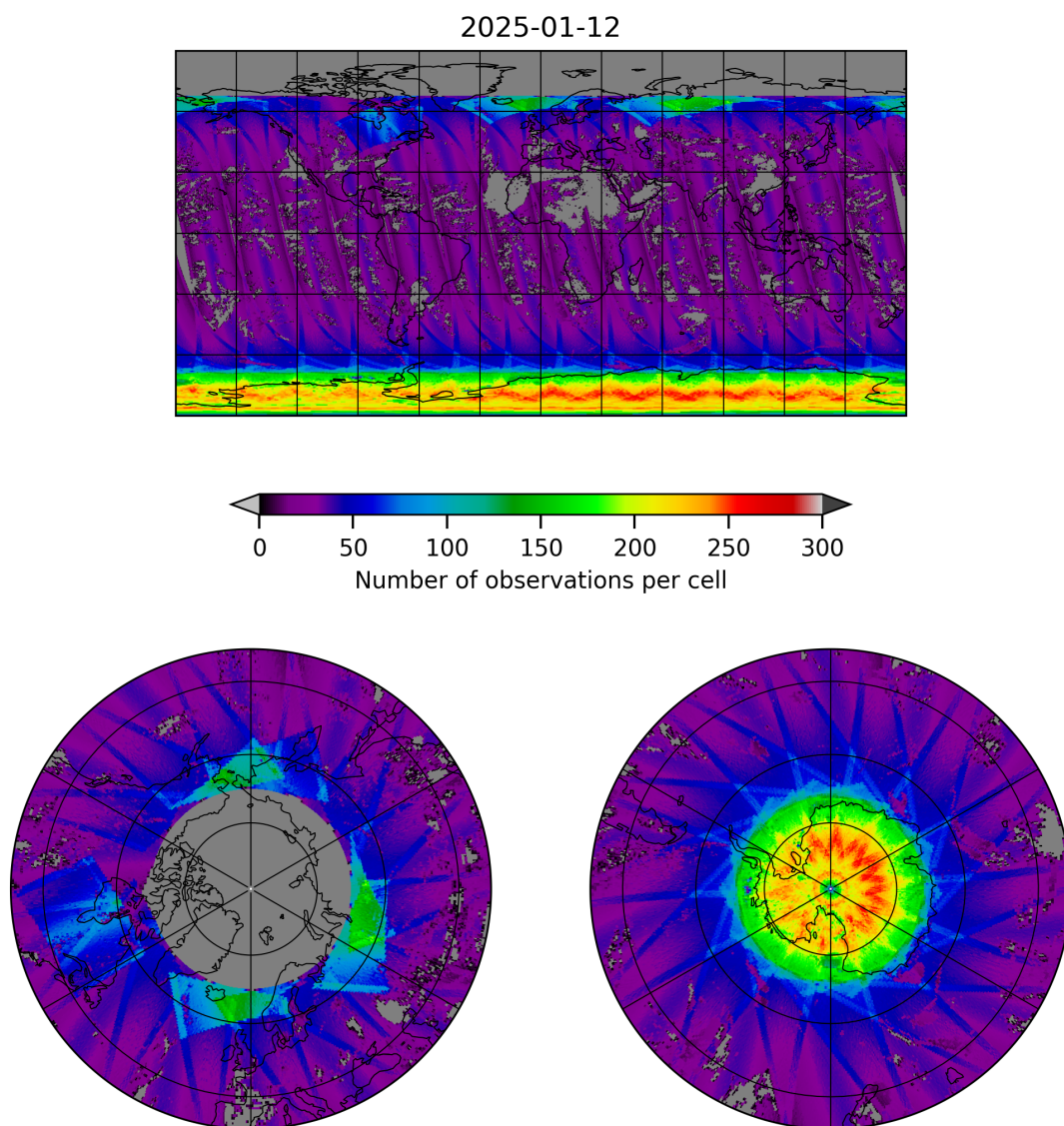
Figure 19: Map of the number of observations for 2025-01-12 to 2025-01-13
