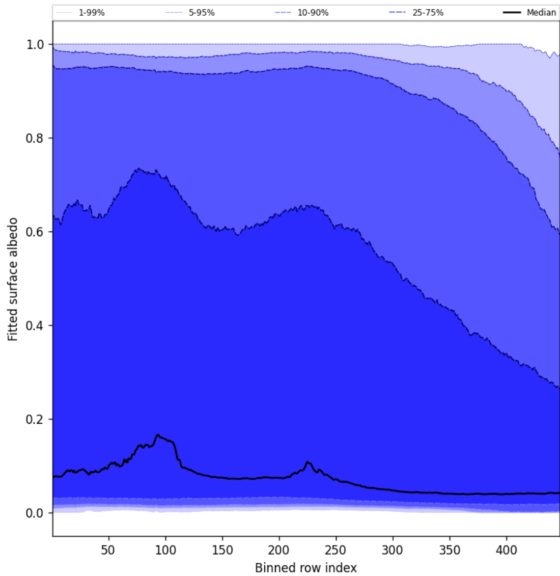
Figure 59: Along track statistics of “Fitted surface albedo” for 2025-01-12 to 2025-01-13
