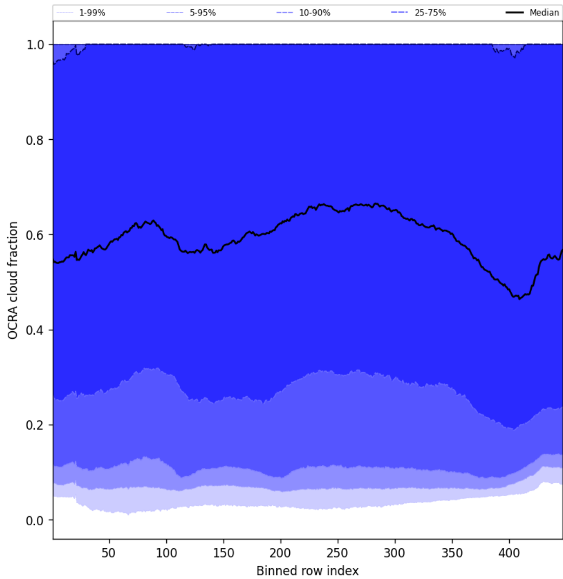
Figure 64: Along track statistics of “OCRA cloud fraction” for 2025-01-12 to 2025-01-13
