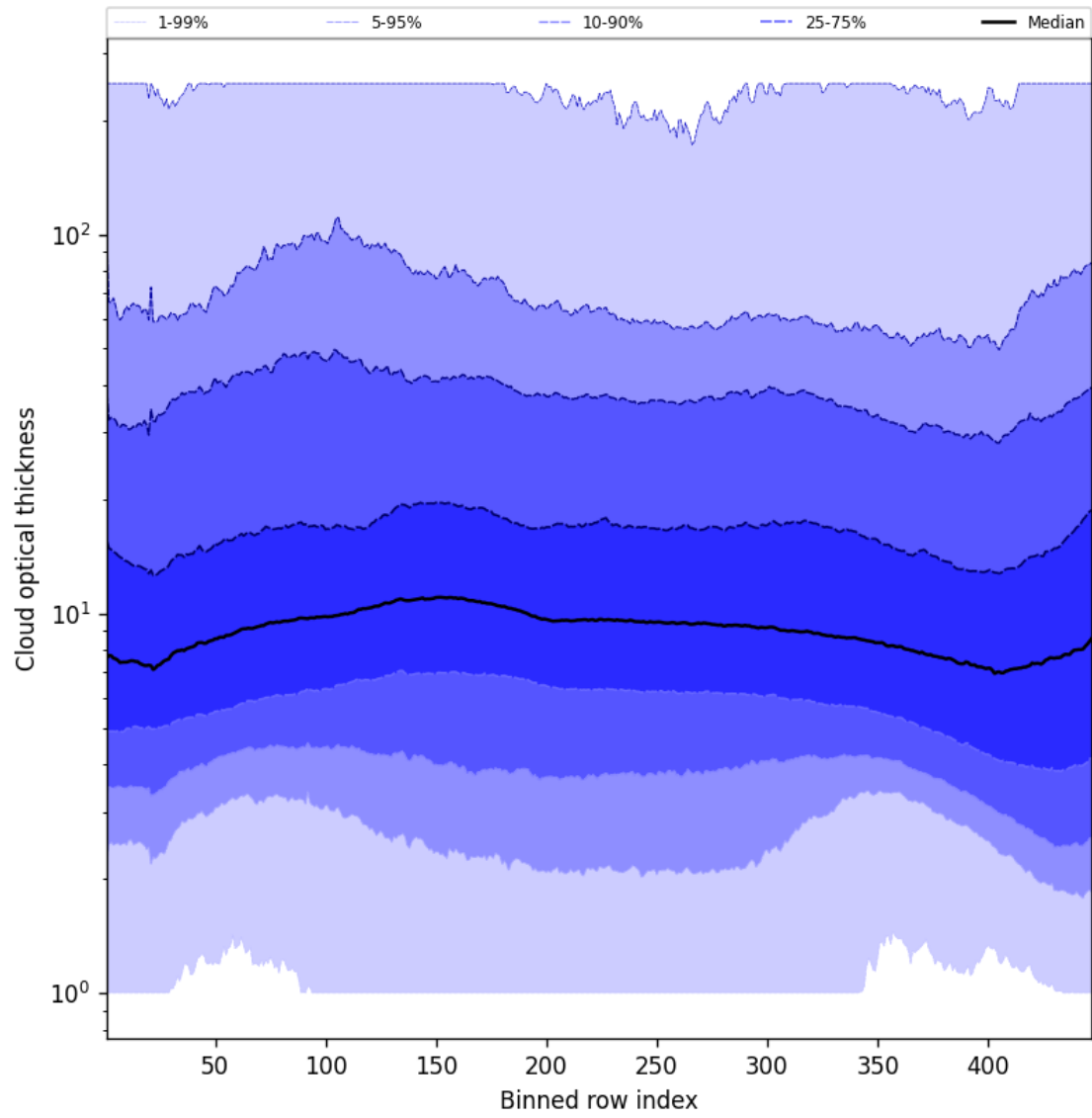
Figure 55: Along track statistics of “Cloud optical thickness” for 2025-01-12 to 2025-01-13
