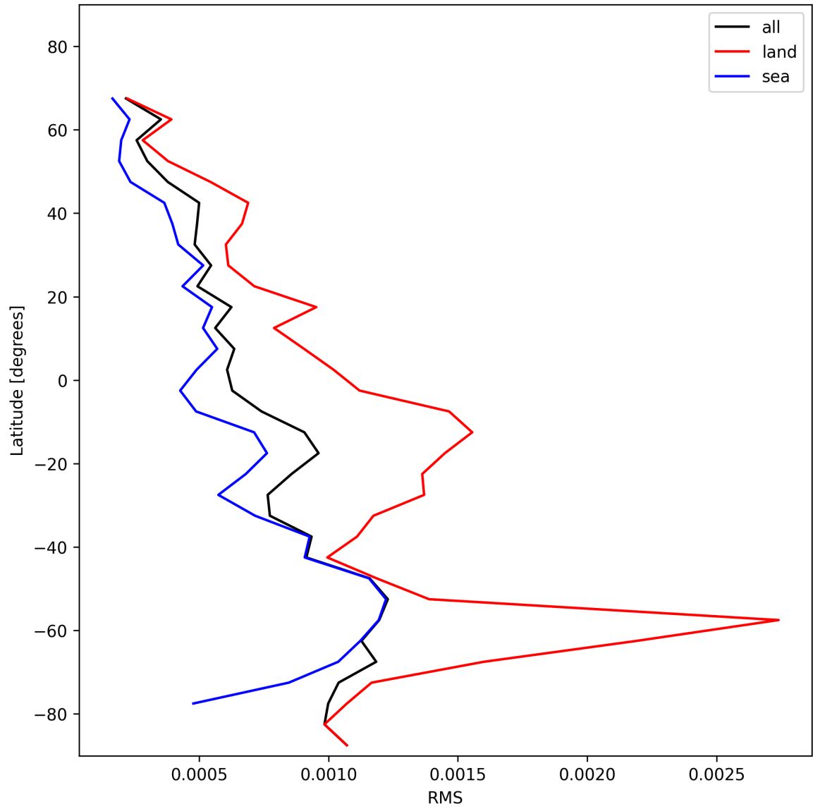
Figure 29: Zonal average of “RMS” for 2025-01-12 to 2025-01-13.
