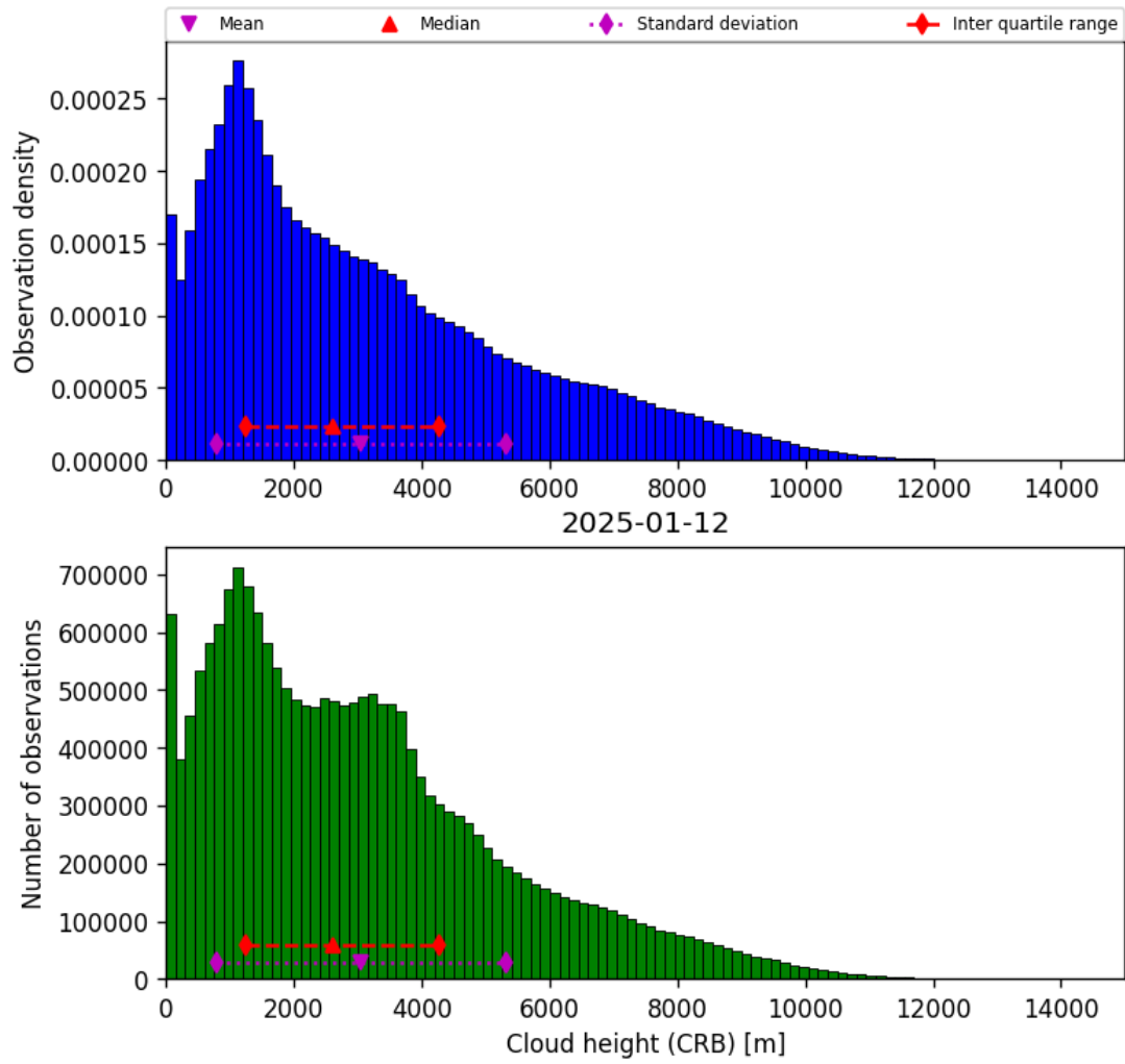
Figure 41: Histogram of “Cloud height (CRB)” for 2025-01-12 to 2025-01-13
