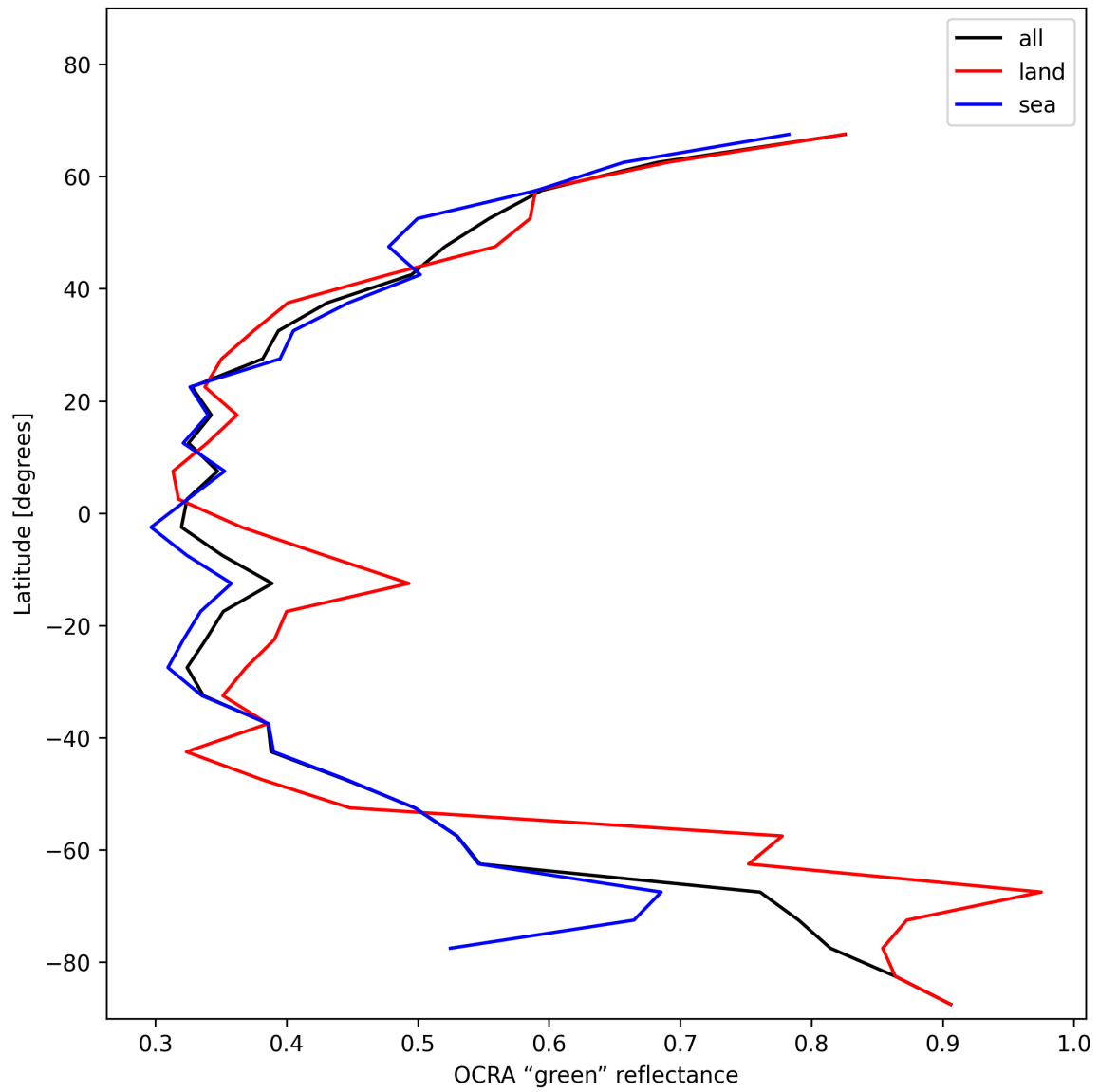
Figure 34: Zonal average of “OCRA “green” reflectance” for 2025-01-12 to 2025-01-13.
