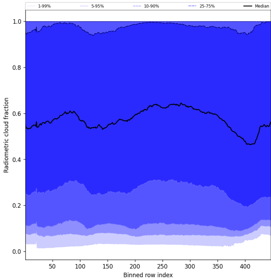
Figure 53: Along track statistics of “Radiometric cloud fraction” for 2025-01-12 to 2025-01-13
