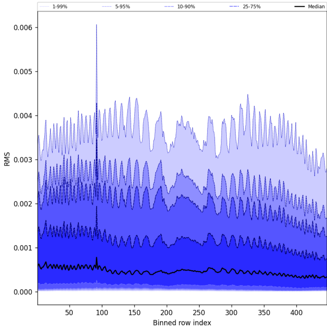
Figure 61: Along track statistics of “RMS” for 2025-01-12 to 2025-01-13
