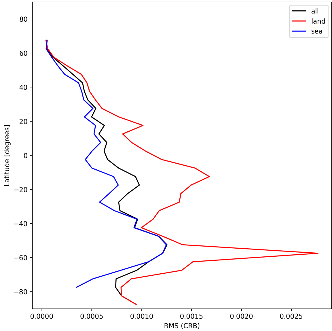
Figure 30: Zonal average of “RMS (CRB)” for 2025-01-12 to 2025-01-13.
