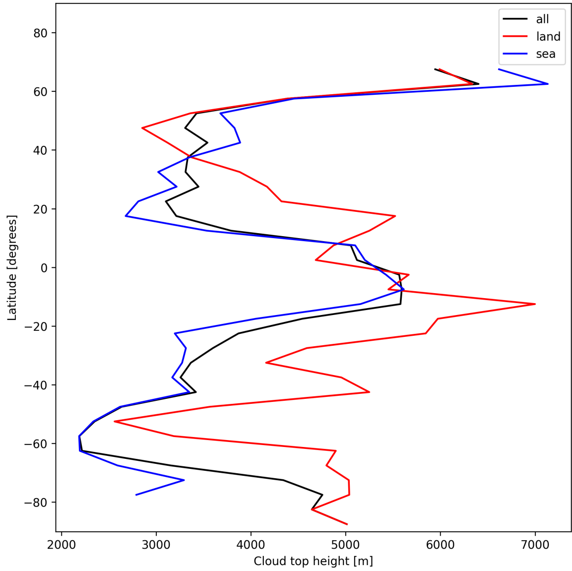
Figure 22: Zonal average of “Cloud top height” for 2025-01-12 to 2025-01-13.
