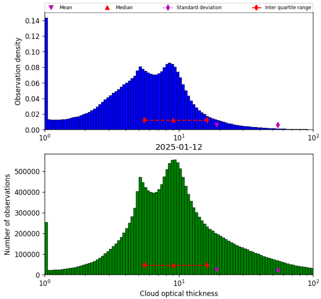
Figure 39: Histogram of “Cloud optical thickness” for 2025-01-12 to 2025-01-13
