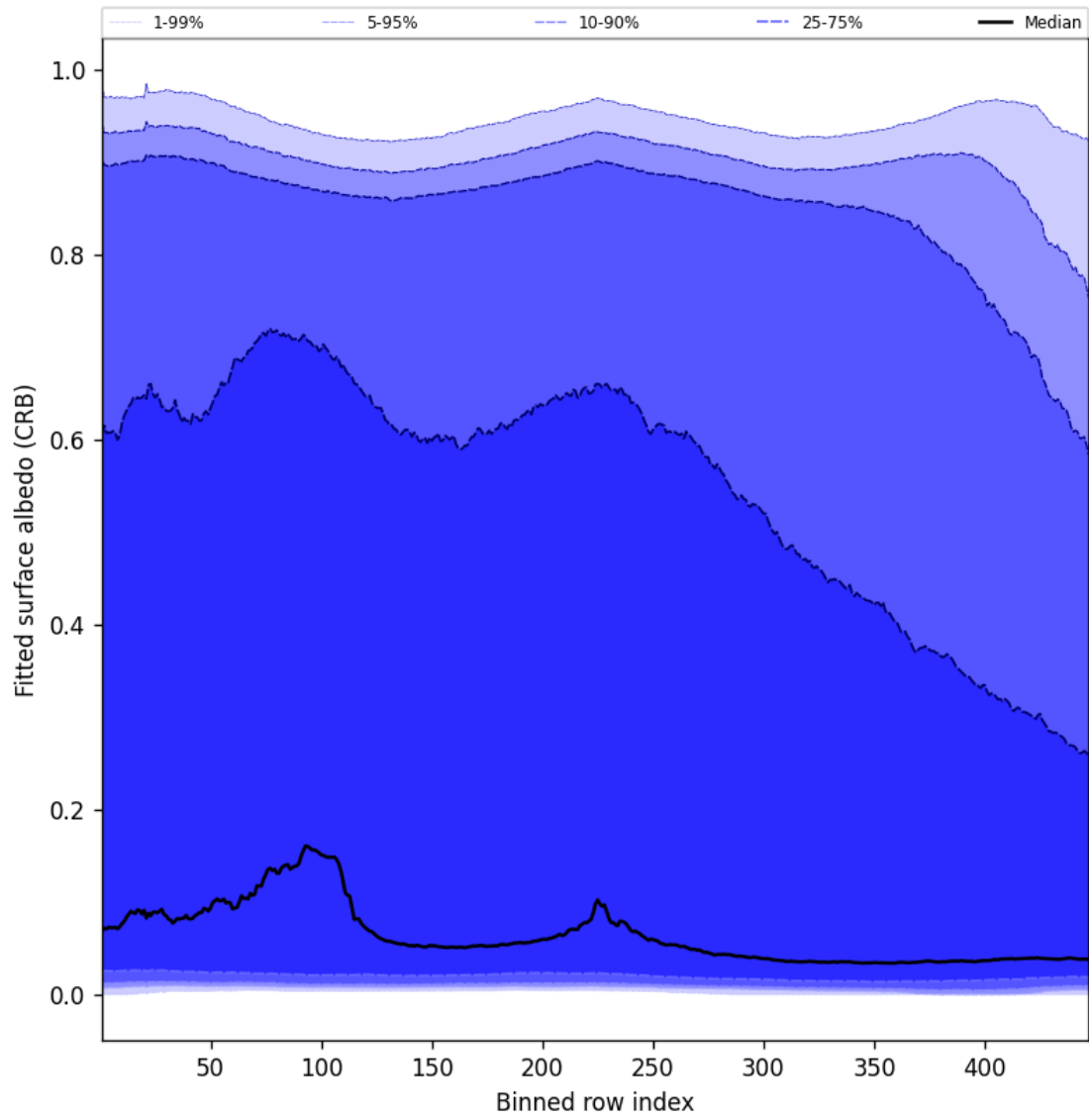
Figure 60: Along track statistics of “Fitted surface albedo (CRB)” for 2025-01-12 to 2025-01-13
