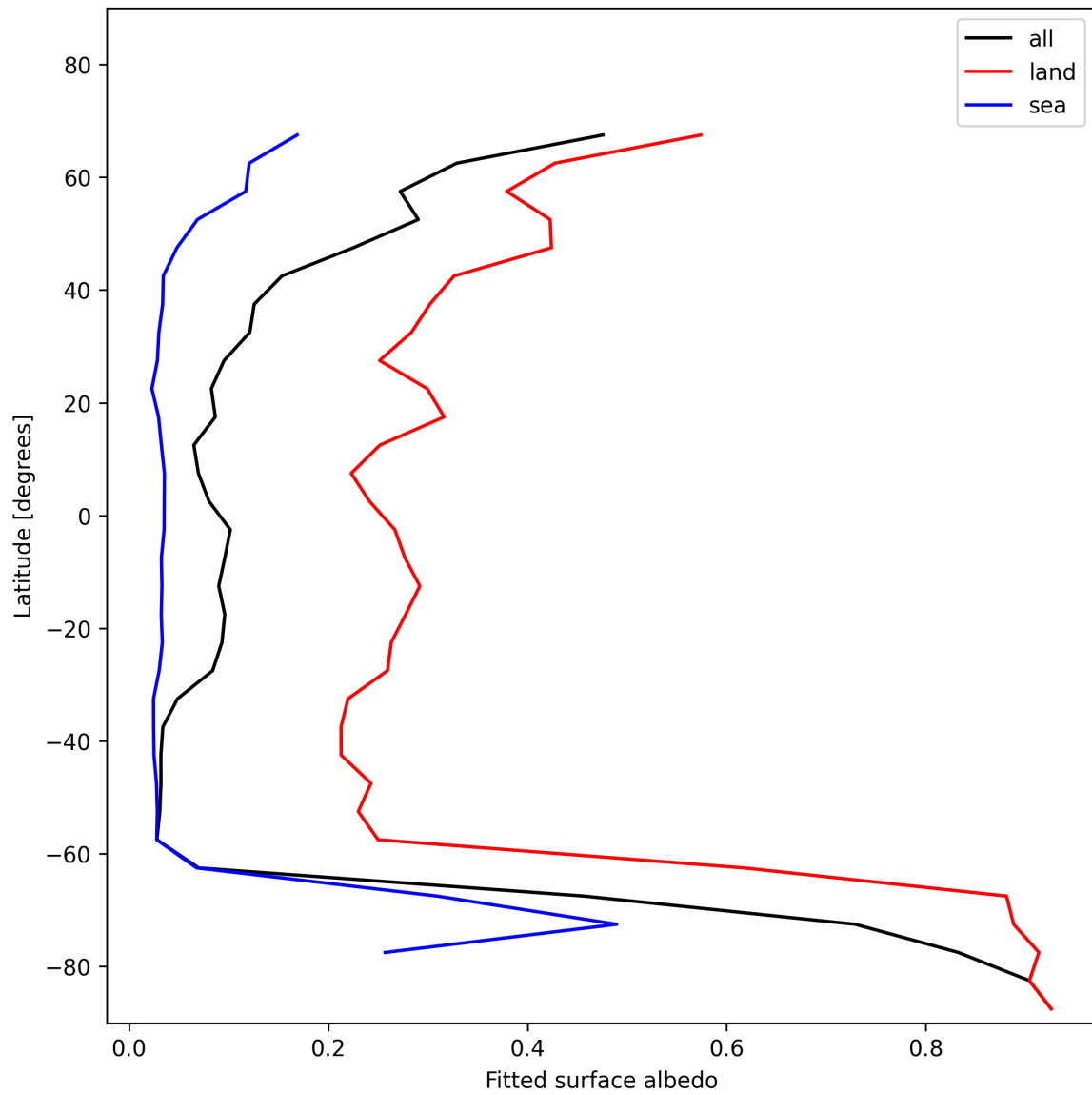
Figure 27: Zonal average of “Fitted surface albedo” for 2025-01-12 to 2025-01-13.
