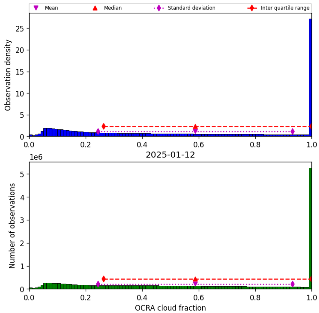
Figure 48: Histogram of “OCRA cloud fraction” for 2025-01-12 to 2025-01-13
