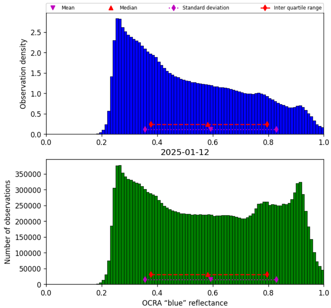
Figure 49: Histogram of "OCRA "blue" reflectance" for 2025-01-12 to 2025-01-13
