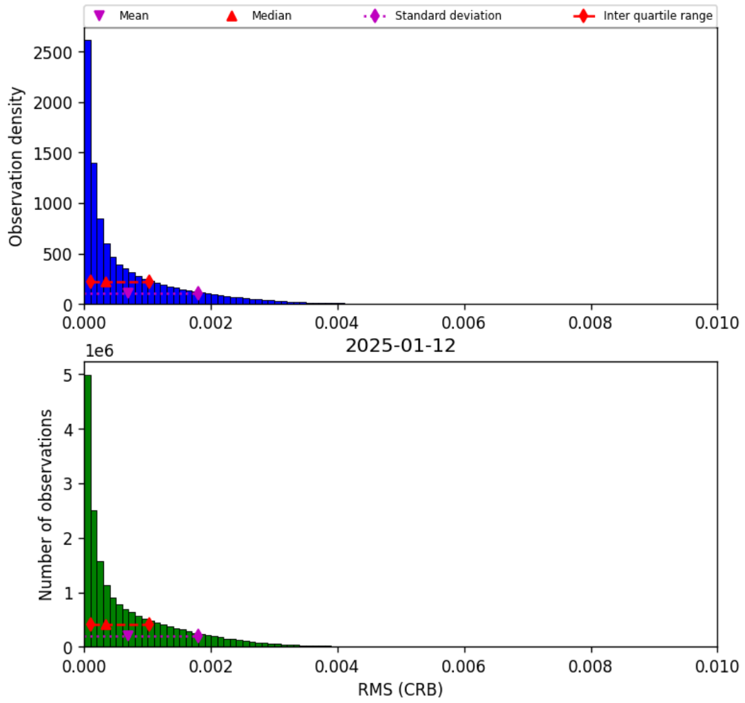
Figure 46: Histogram of “RMS (CRB)” for 2025-01-12 to 2025-01-13
