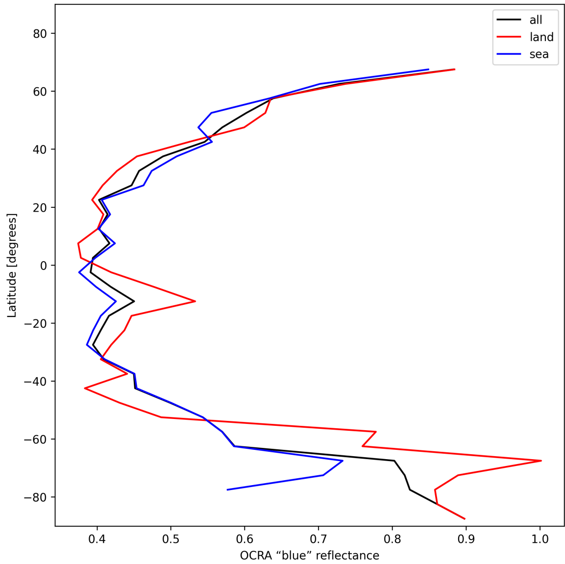
Figure 33: Zonal average of “OCRA “blue” reflectance” for 2025-01-12 to 2025-01-13.
