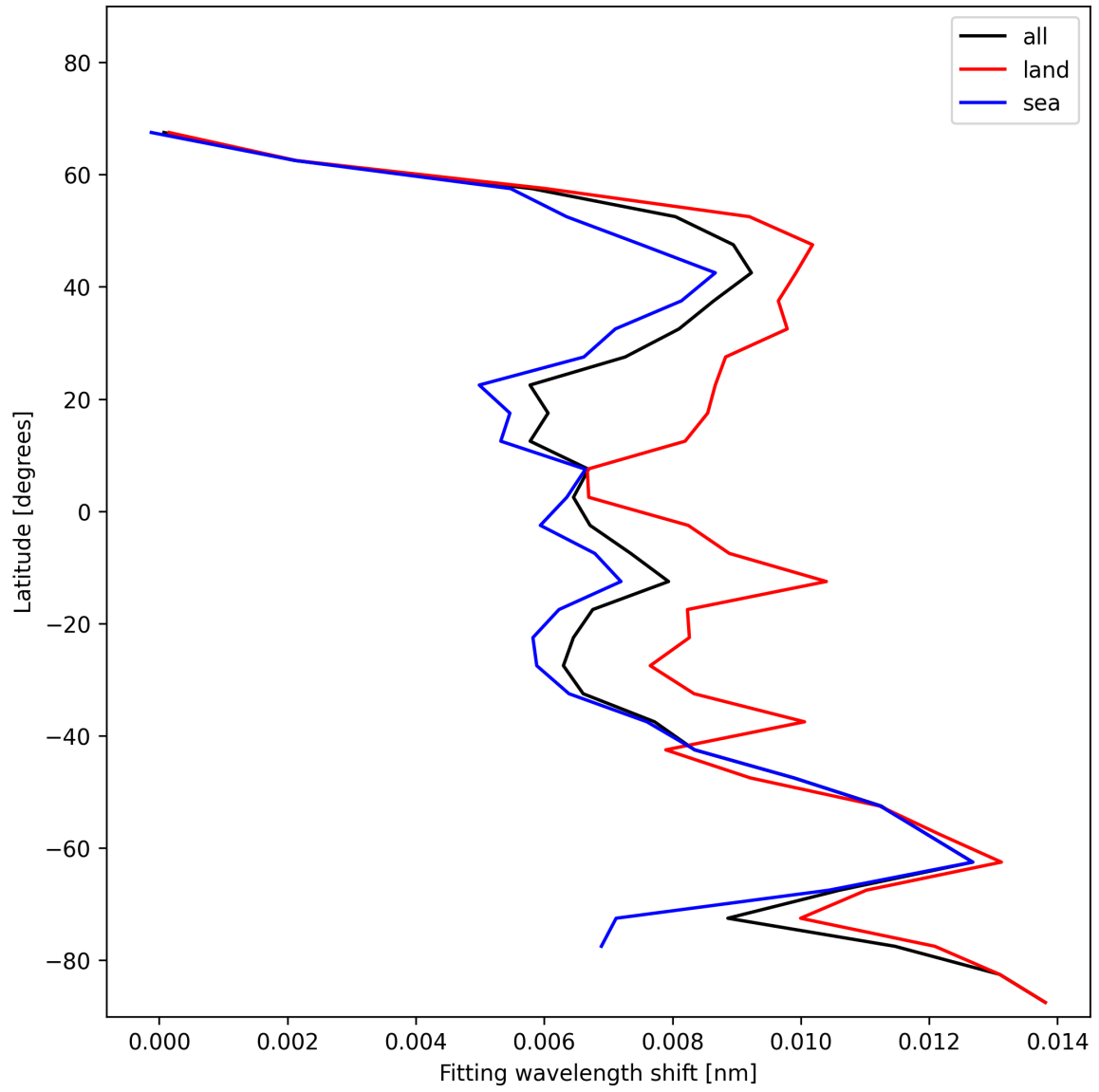
Figure 31: Zonal average of “Fitting wavelength shift” for 2025-01-12 to 2025-01-13.
