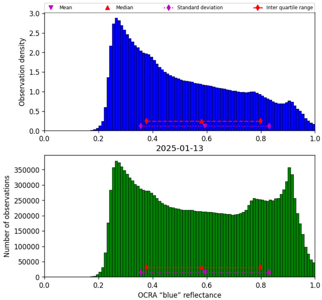
Figure 49: Histogram of “OCRA “blue” reflectance” for 2025-01-13 to 2025-01-14
