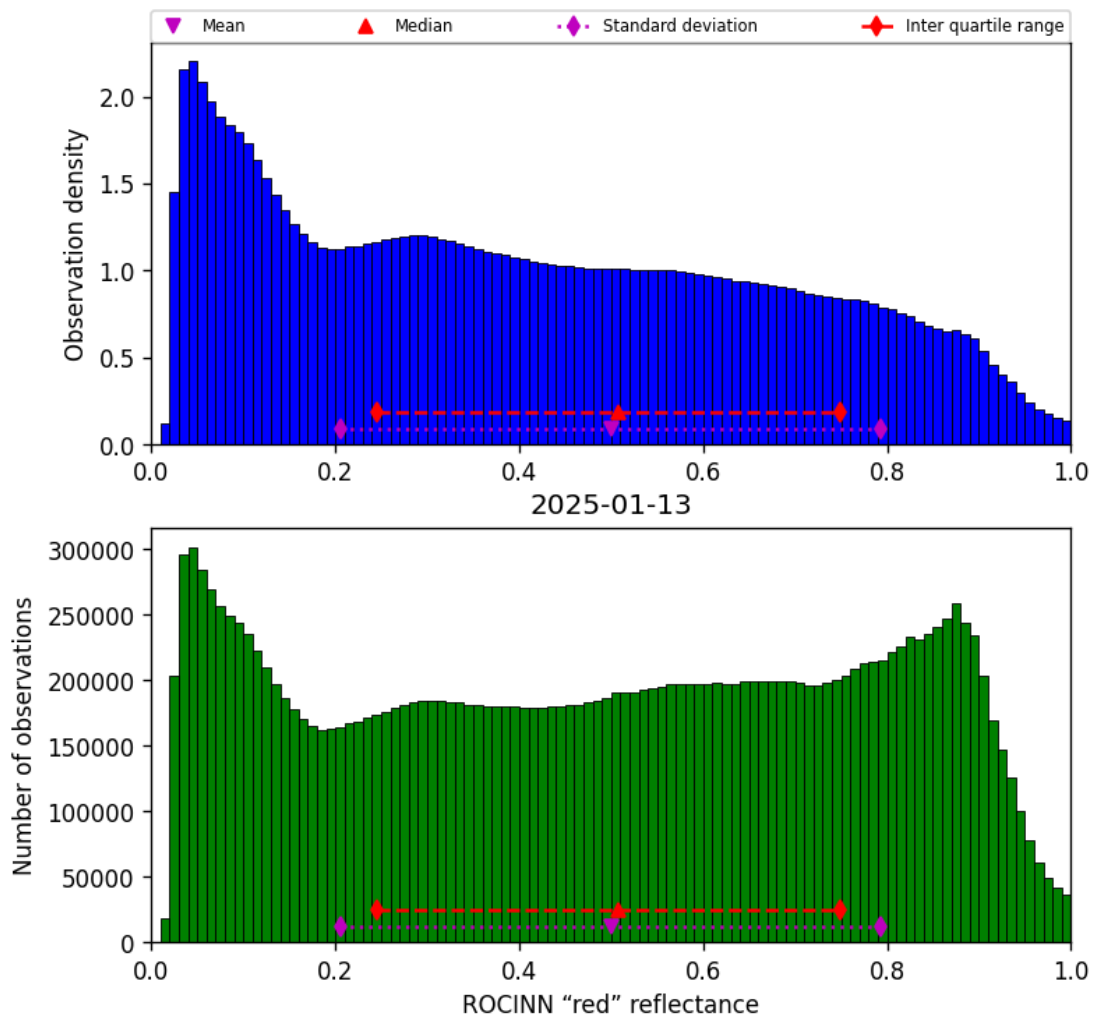
Figure 51: Histogram of “ROCINN “red” reflectance” for 2025-01-13 to 2025-01-14
