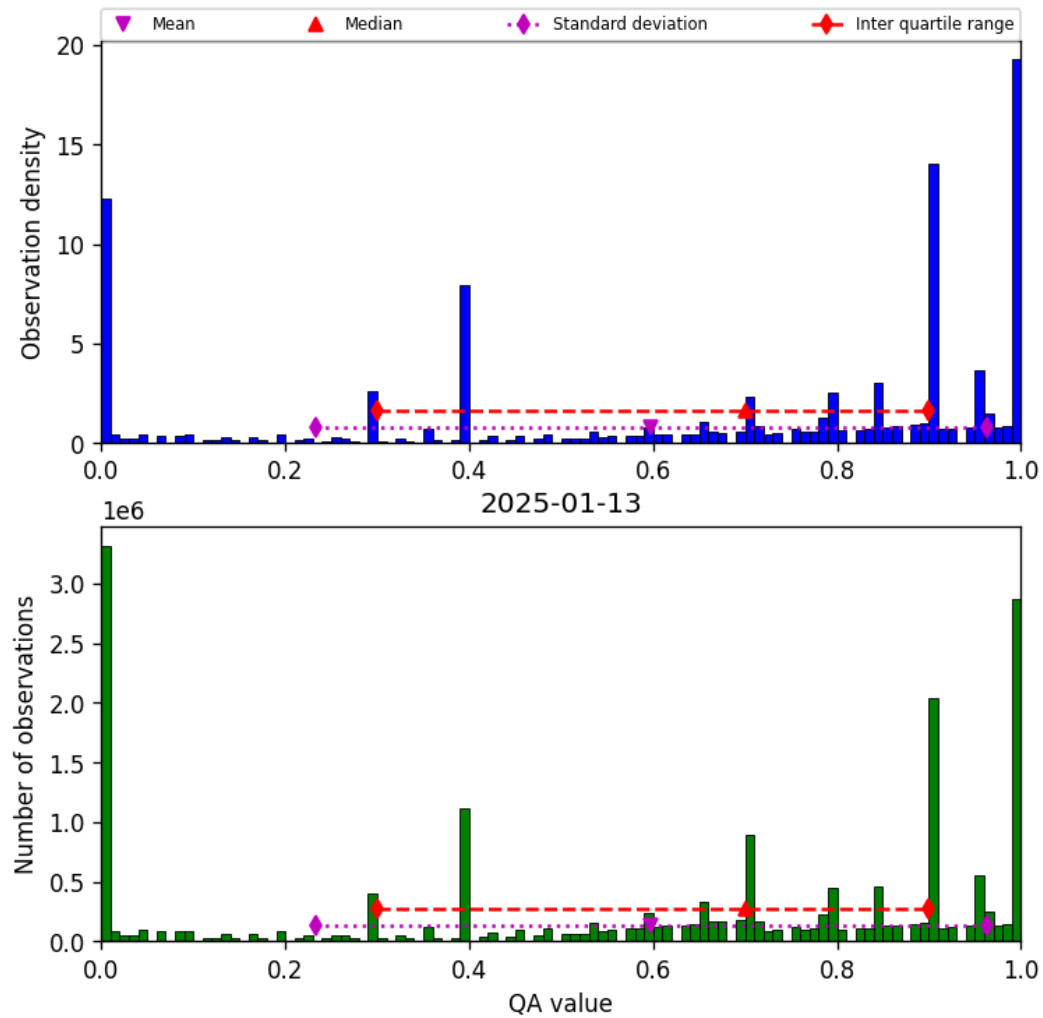
Figure 36: Histogram of “QA value” for 2025-01-13 to 2025-01-14
