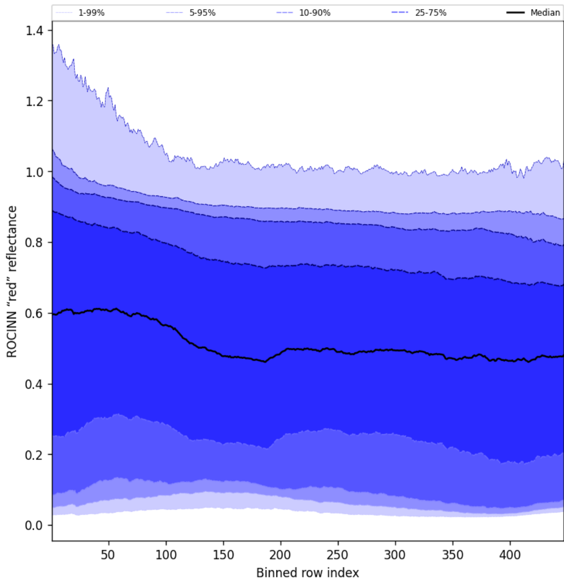
Figure 67: Along track statistics of "ROCINN "red" reflectance" for 2025-01-13 to 2025-01-14
