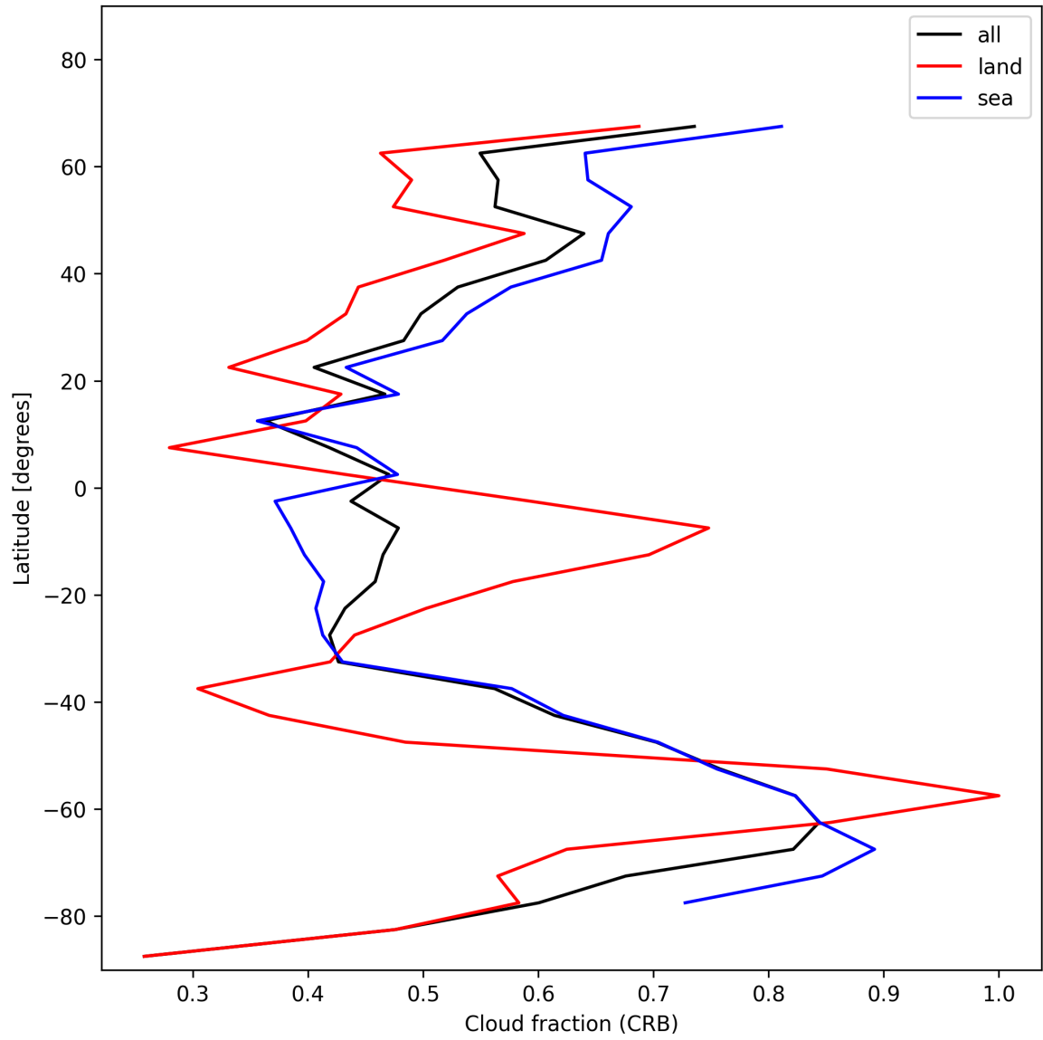
Figure 24: Zonal average of “Cloud fraction (CRB)” for 2025-01-13 to 2025-01-14.
