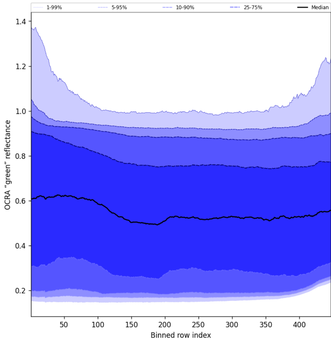
Figure 66: Along track statistics of “OCRA “green” reflectance” for 2025-01-13 to 2025-01-14
