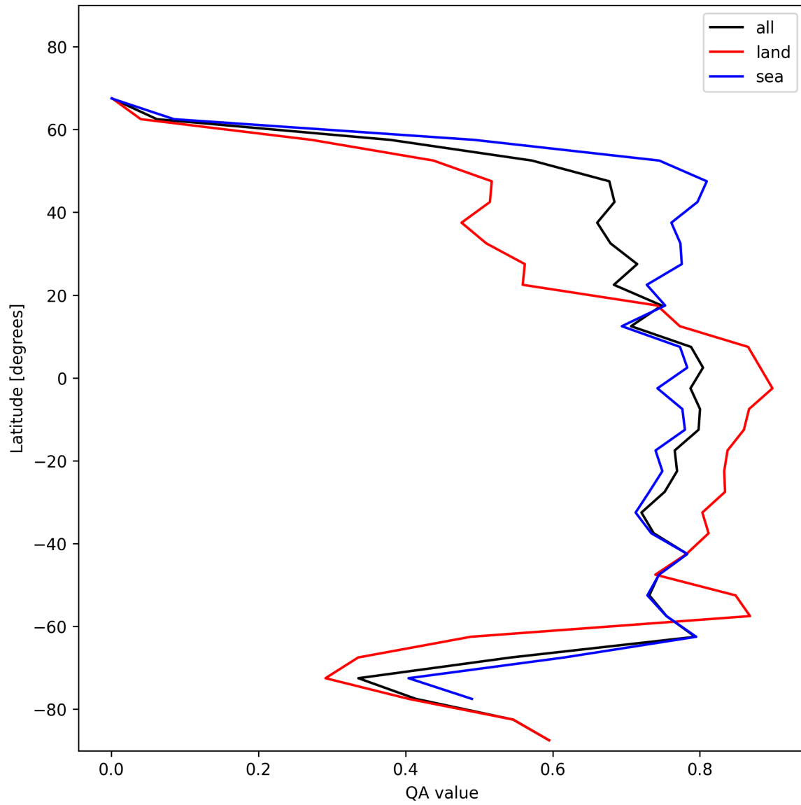
Figure 20: Zonal average of “QA value” for 2025-01-13 to 2025-01-14.
