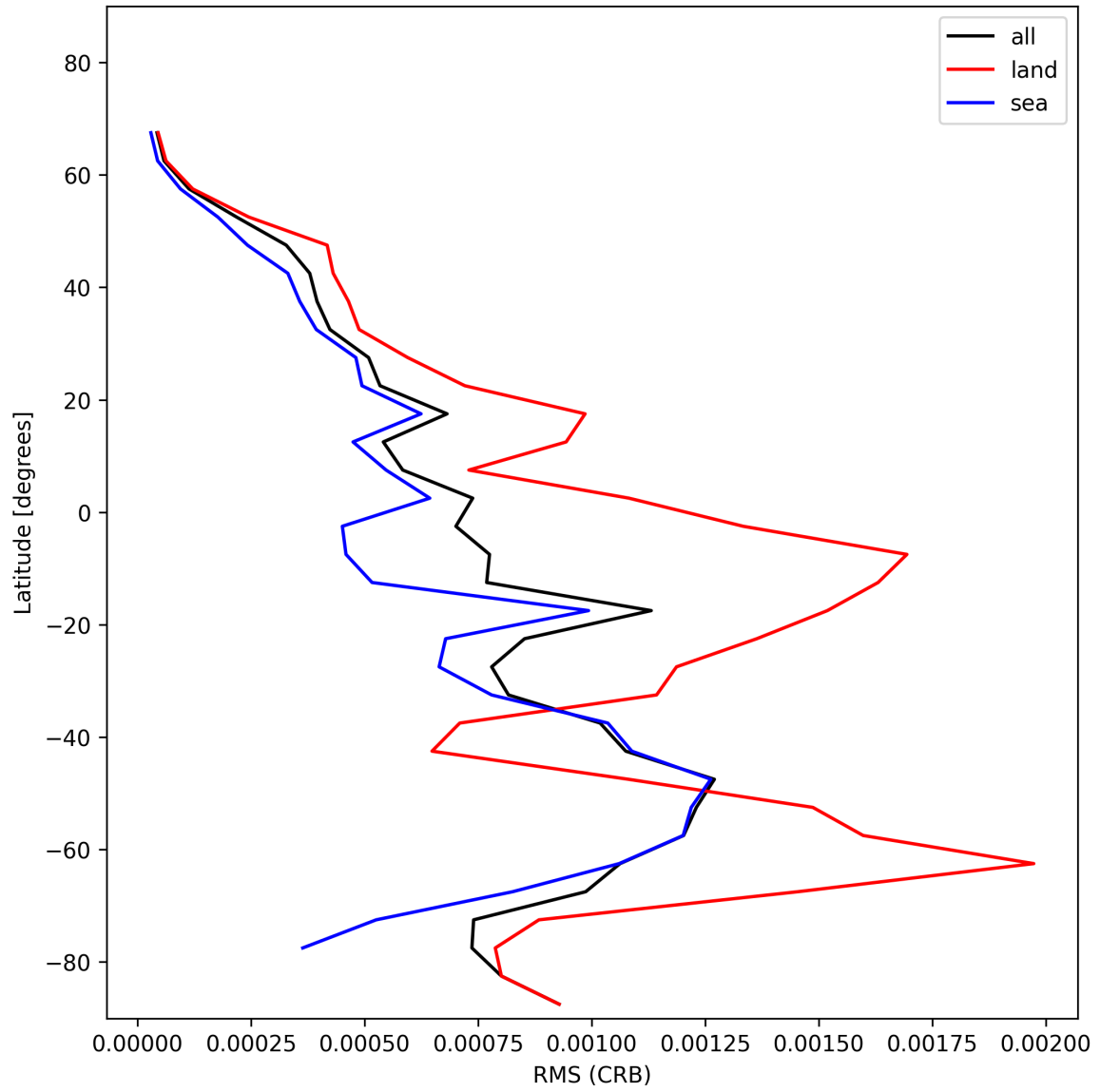
Figure 30: Zonal average of “RMS (CRB)” for 2025-01-13 to 2025-01-14.
