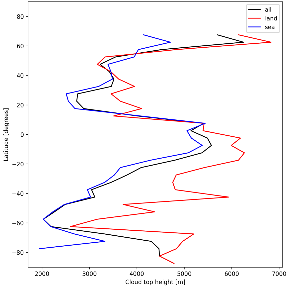
Figure 22: Zonal average of “Cloud top height” for 2025-01-13 to 2025-01-14.
