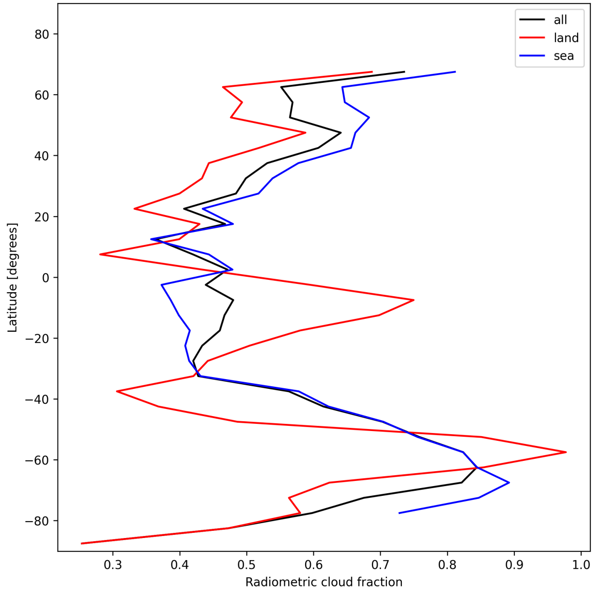
Figure 21: Zonal average of “Radiometric cloud fraction” for 2025-01-13 to 2025-01-14.
