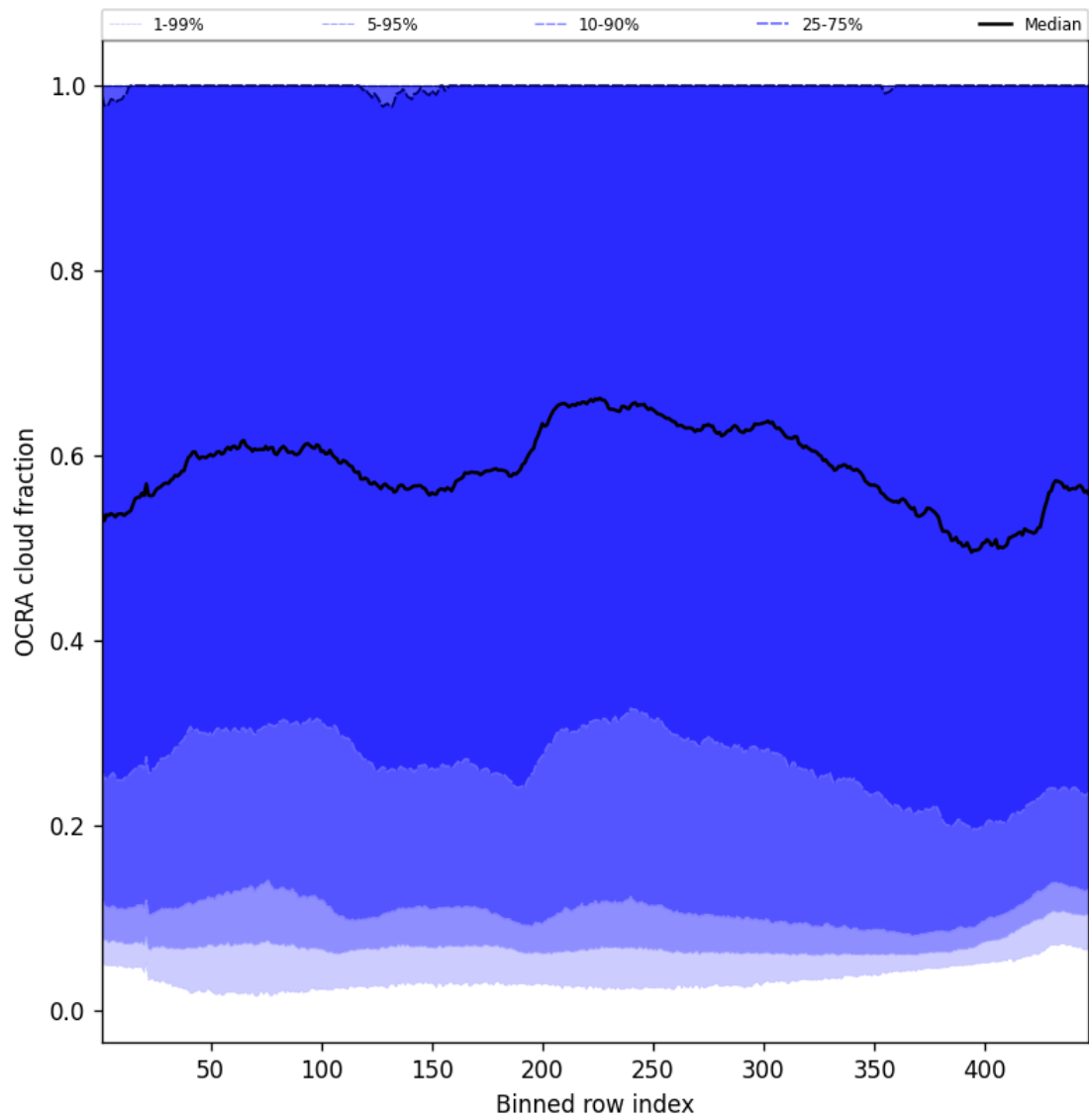
Figure 64: Along track statistics of “OCRA cloud fraction” for 2025-01-13 to 2025-01-14
