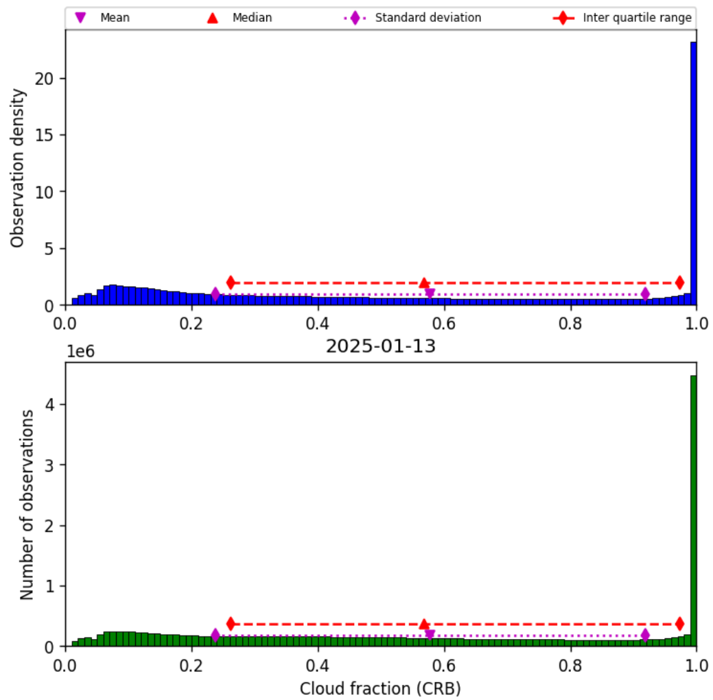
Figure 40: Histogram of “Cloud fraction (CRB)” for 2025-01-13 to 2025-01-14
