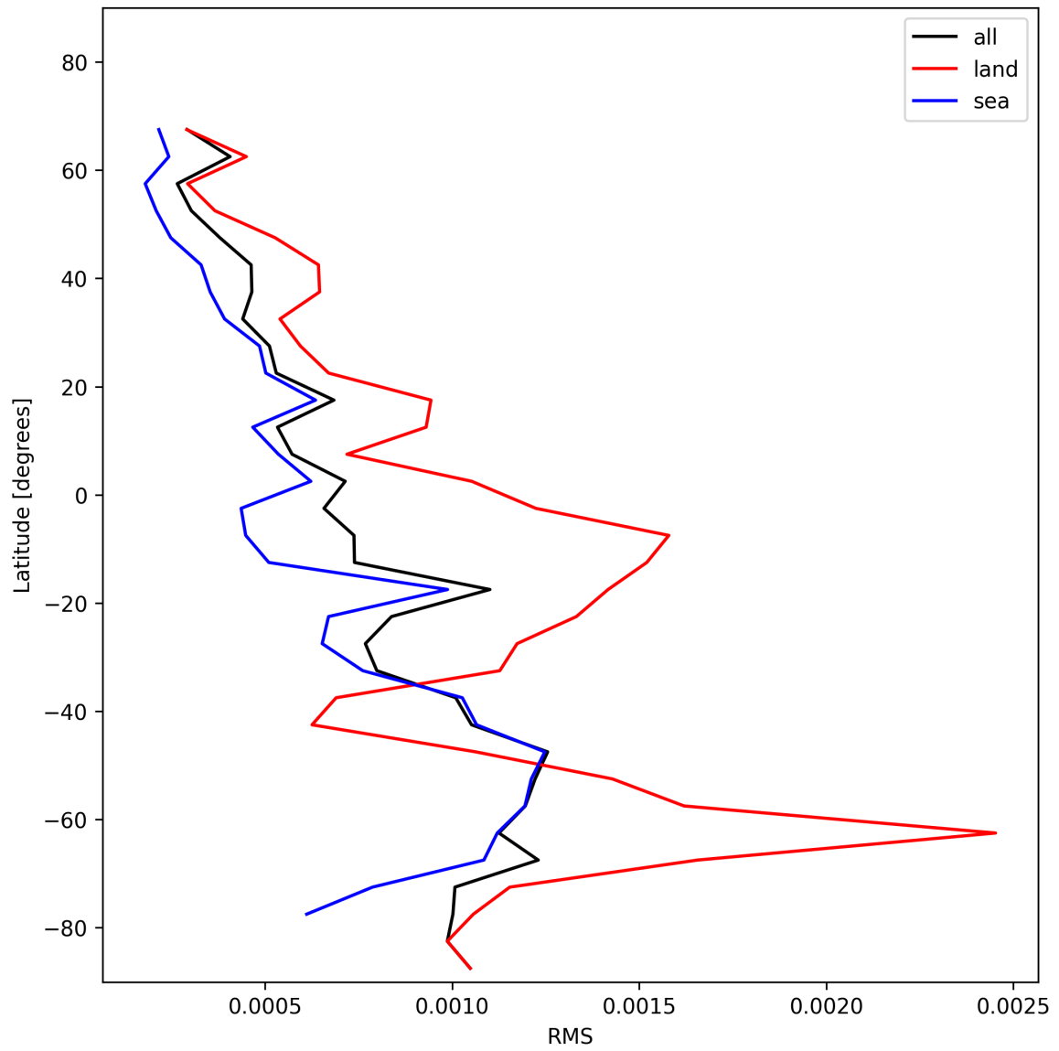
Figure 29: Zonal average of “RMS” for 2025-01-13 to 2025-01-14.
