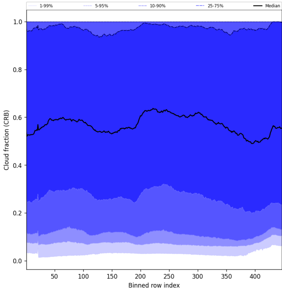
Figure 56: Along track statistics of “Cloud fraction (CRB)” for 2025-01-13 to 2025-01-14
