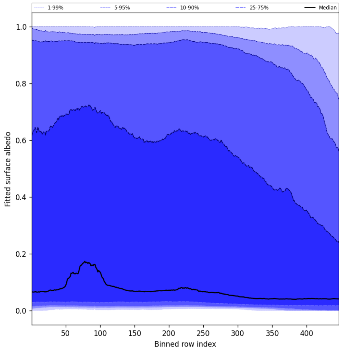
Figure 59: Along track statistics of “Fitted surface albedo” for 2025-01-13 to 2025-01-14
