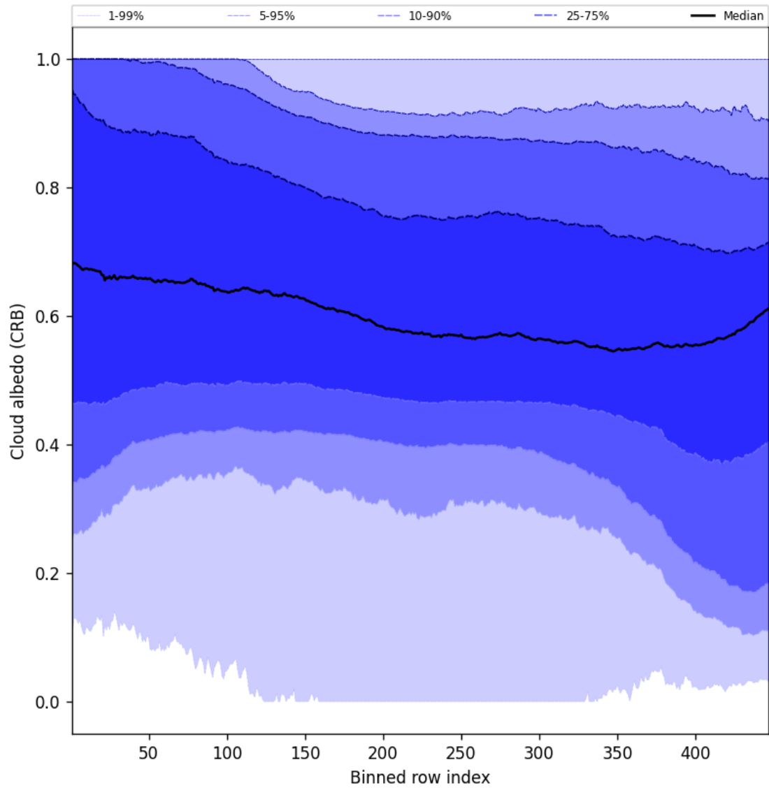
Figure 58: Along track statistics of “Cloud albedo (CRB)” for 2025-01-13 to 2025-01-14
