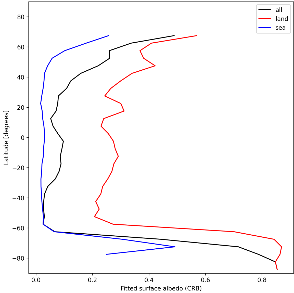
Figure 28: Zonal average of “Fitted surface albedo (CRB)” for 2025-01-13 to 2025-01-14.
