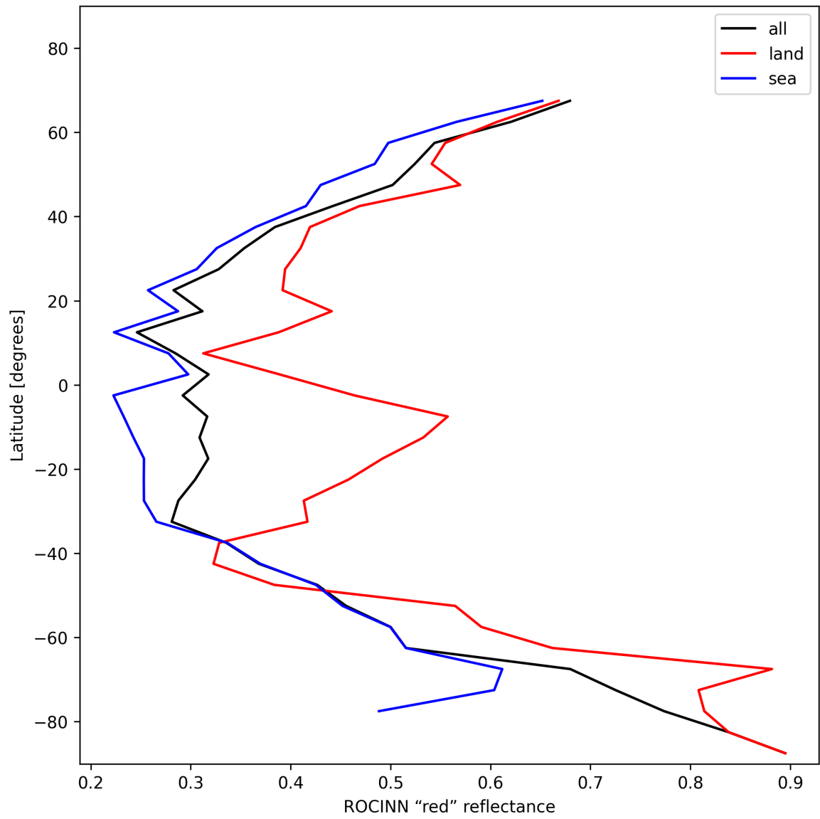
Figure 35: Zonal average of “ROCINN “red” reflectance” for 2025-01-13 to 2025-01-14.
