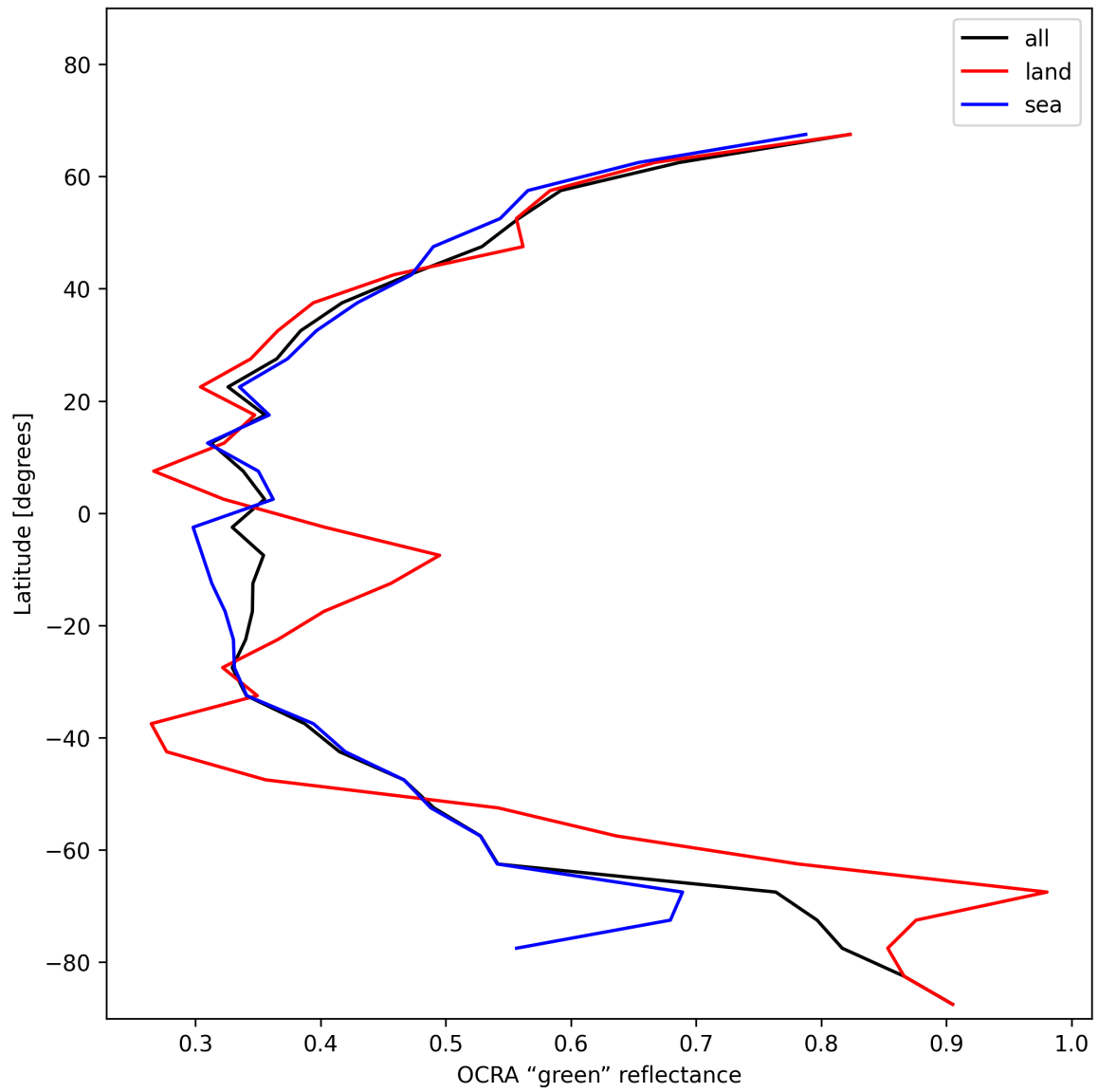
Figure 34: Zonal average of “OCRA “green” reflectance” for 2025-01-13 to 2025-01-14.
