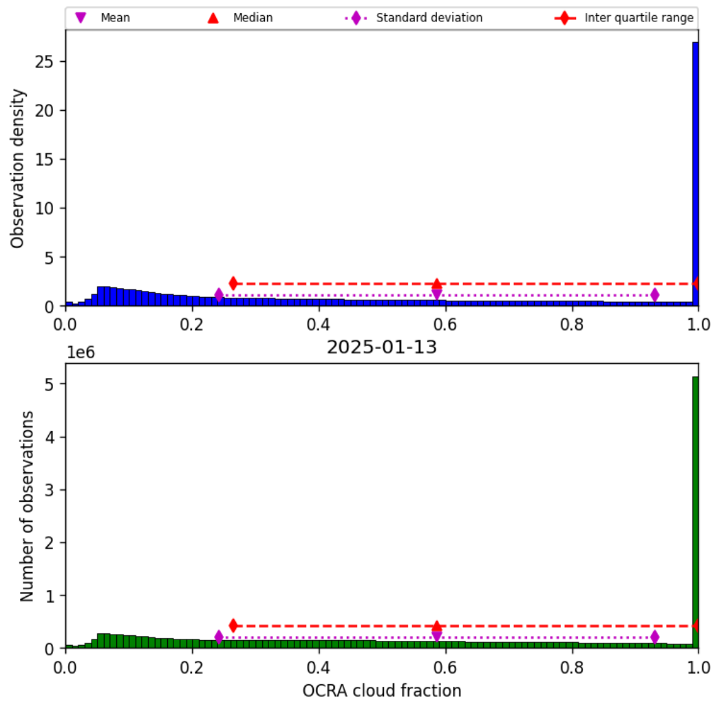
Figure 48: Histogram of “OCRA cloud fraction” for 2025-01-13 to 2025-01-14
