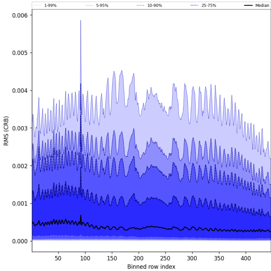
Figure 62: Along track statistics of “RMS (CRB)” for 2025-01-13 to 2025-01-14
