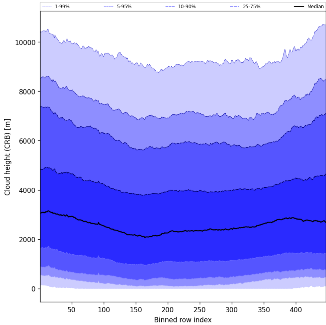
Figure 57: Along track statistics of “Cloud height (CRB)” for 2025-01-13 to 2025-01-14
