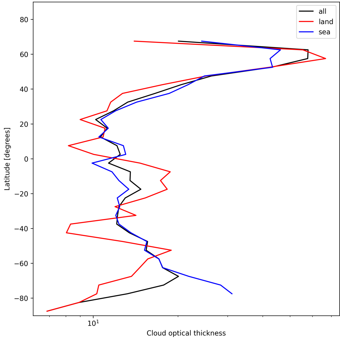
Figure 23: Zonal average of “Cloud optical thickness” for 2025-01-13 to 2025-01-14.
