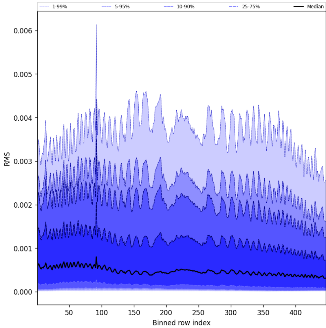
Figure 61: Along track statistics of “RMS” for 2025-01-13 to 2025-01-14
