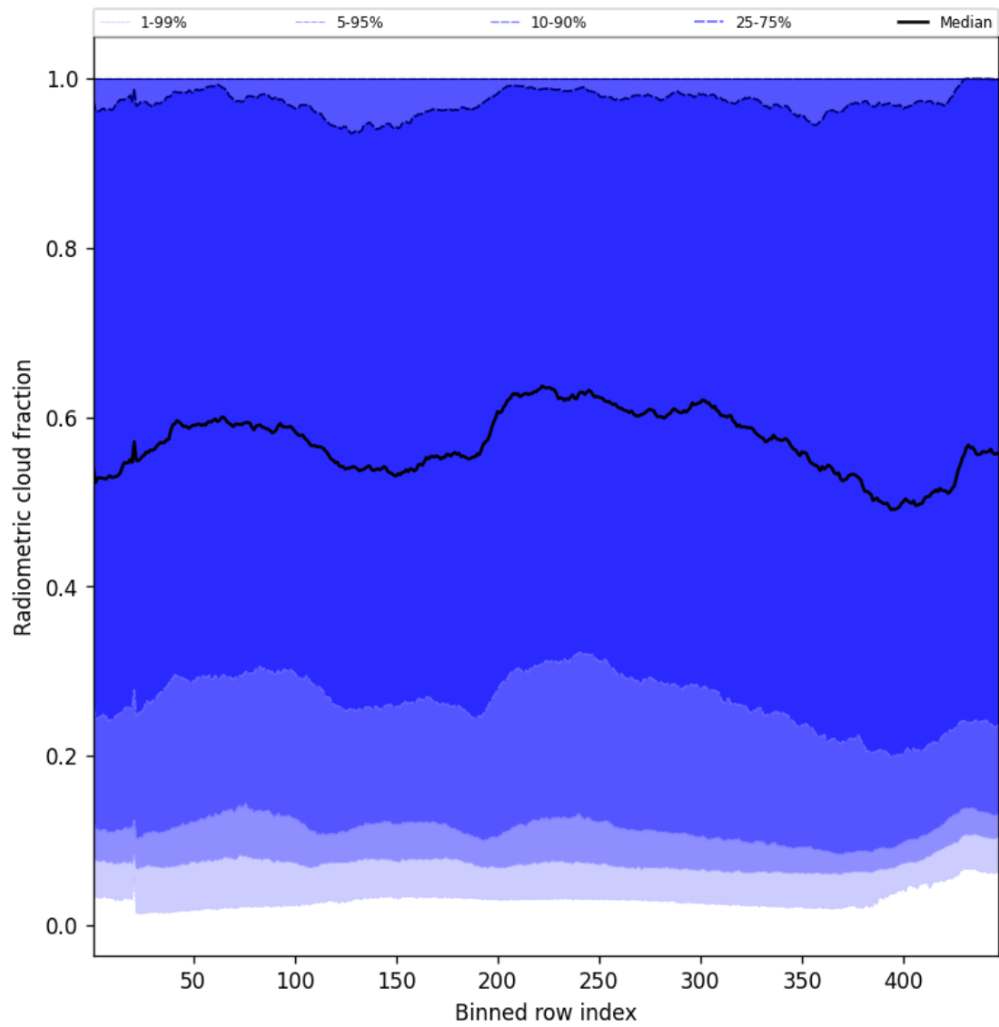
Figure 53: Along track statistics of “Radiometric cloud fraction” for 2025-01-13 to 2025-01-14
