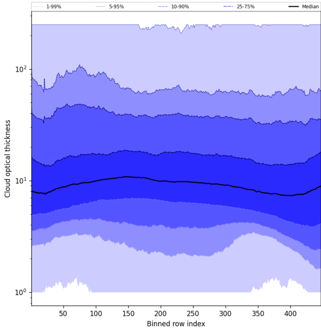
Figure 55: Along track statistics of “Cloud optical thickness” for 2025-01-13 to 2025-01-14
