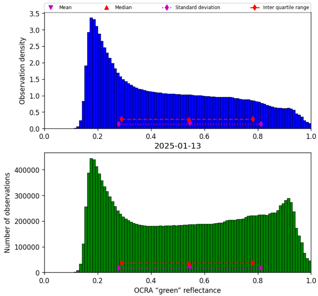
Figure 50: Histogram of “OCRA “green” reflectance” for 2025-01-13 to 2025-01-14
