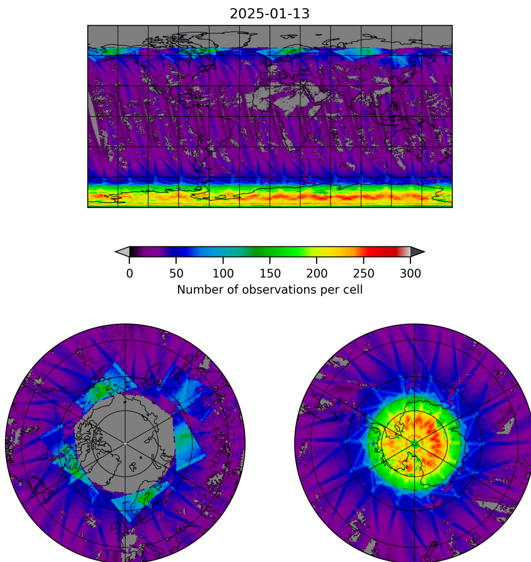
Figure 19: Map of the number of observations for 2025-01-13 to 2025-01-14
