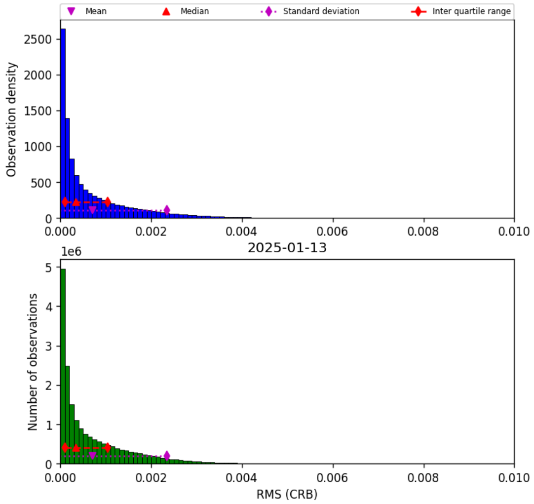
Figure 46: Histogram of “RMS (CRB)” for 2025-01-13 to 2025-01-14
