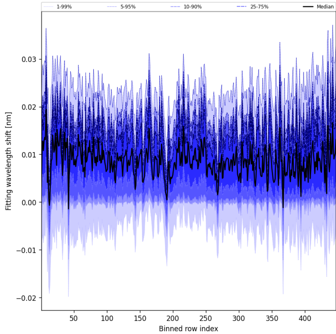
Figure 63: Along track statistics of “Fitting wavelength shift” for 2025-01-13 to 2025-01-14
