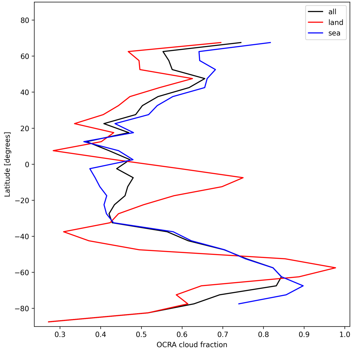
Figure 32: Zonal average of “OCRA cloud fraction” for 2025-01-13 to 2025-01-14.
