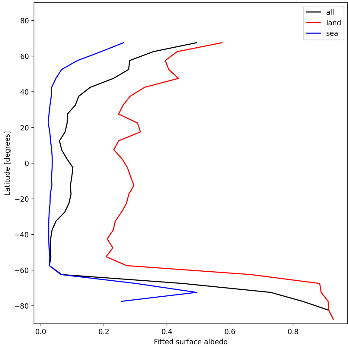
Figure 27: Zonal average of “Fitted surface albedo” for 2025-01-13 to 2025-01-14.
