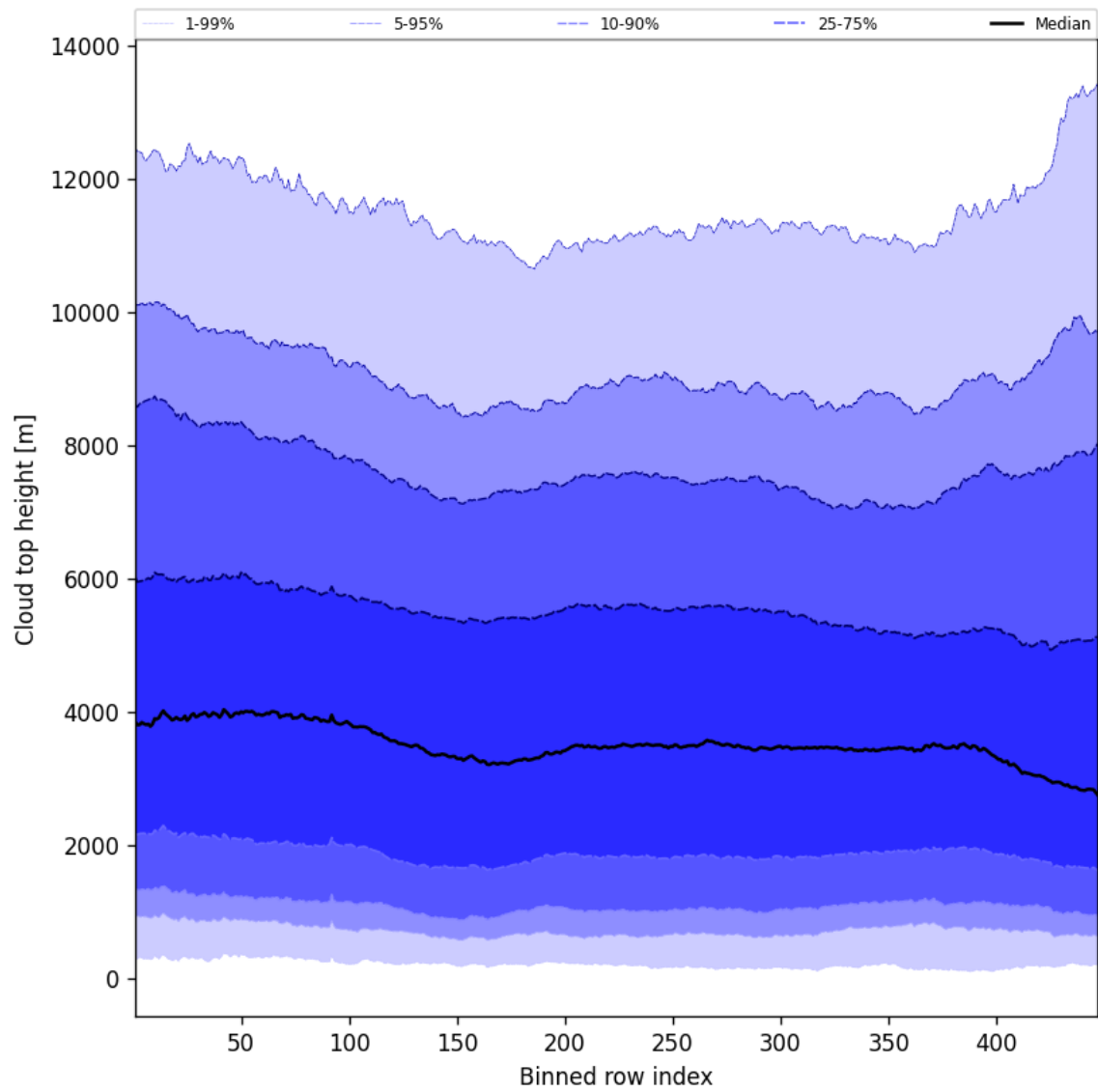
Figure 54: Along track statistics of “Cloud top height” for 2025-01-13 to 2025-01-14
