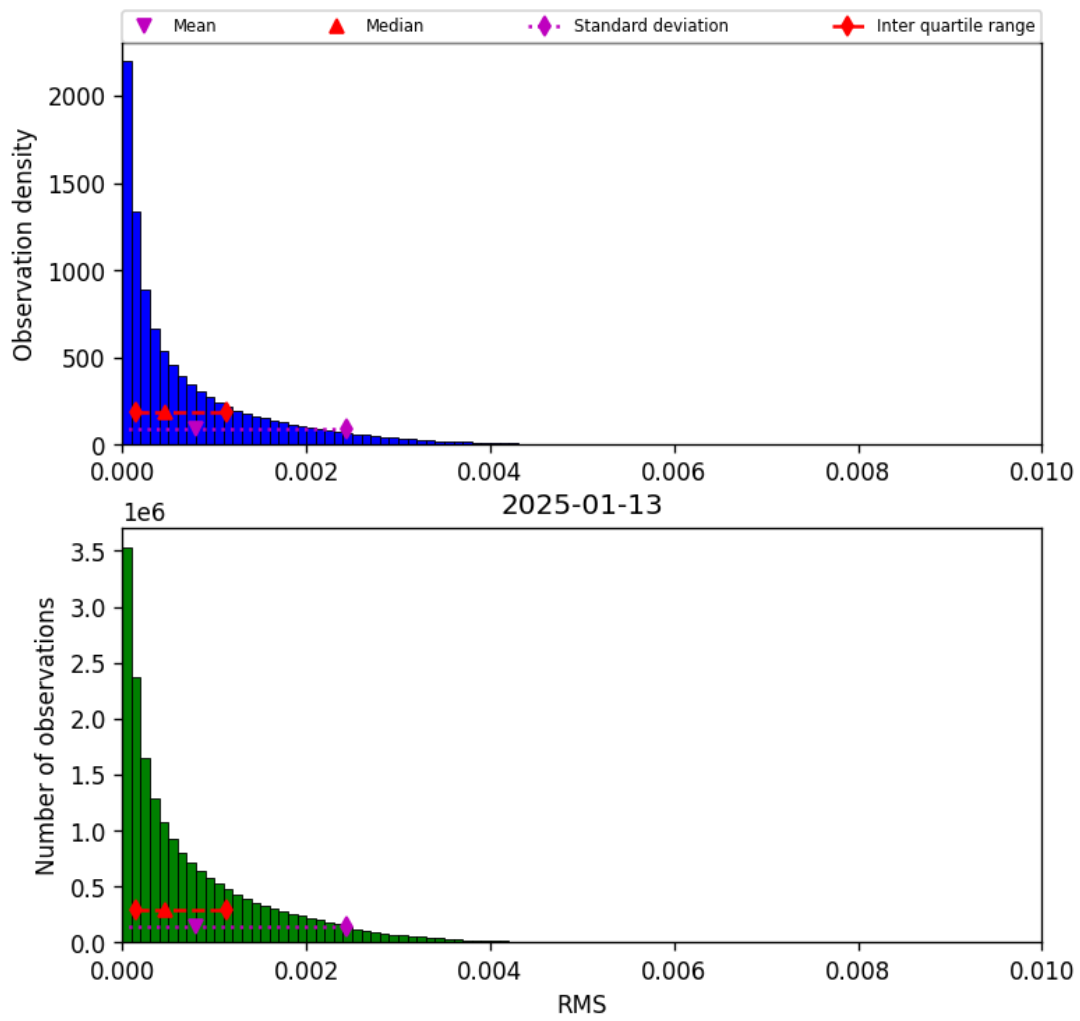
Figure 45: Histogram of “RMS” for 2025-01-13 to 2025-01-14
