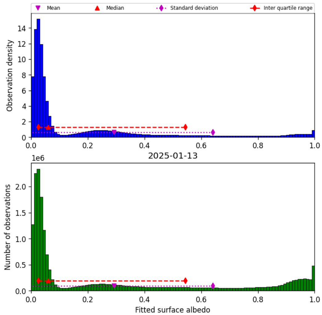
Figure 43: Histogram of “Fitted surface albedo” for 2025-01-13 to 2025-01-14
