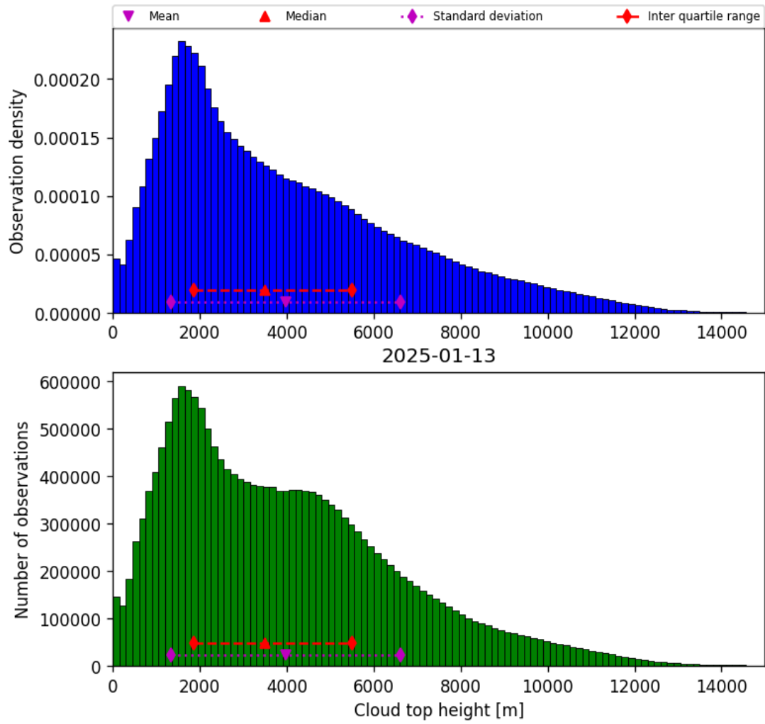
Figure 38: Histogram of “Cloud top height” for 2025-01-13 to 2025-01-14
