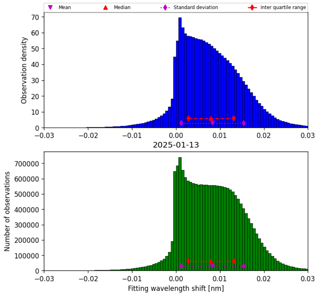
Figure 47: Histogram of “Fitting wavelength shift” for 2025-01-13 to 2025-01-14
