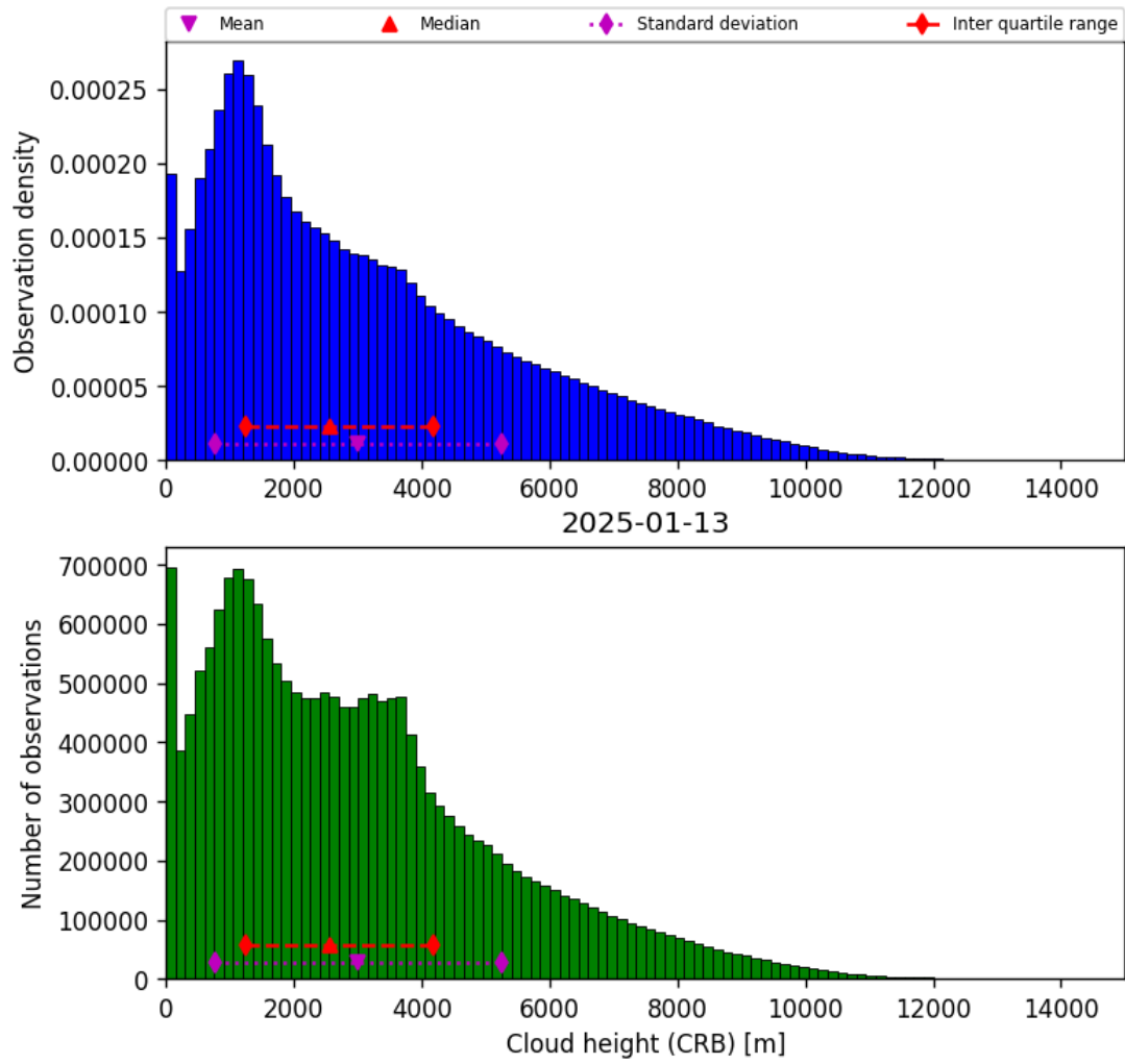
Figure 41: Histogram of “Cloud height (CRB)” for 2025-01-13 to 2025-01-14
