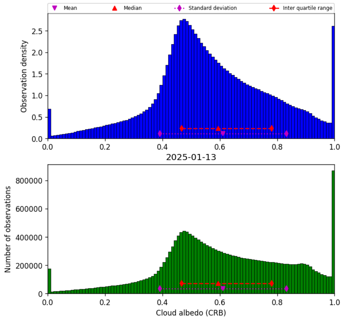
Figure 42: Histogram of “Cloud albedo (CRB)” for 2025-01-13 to 2025-01-14
