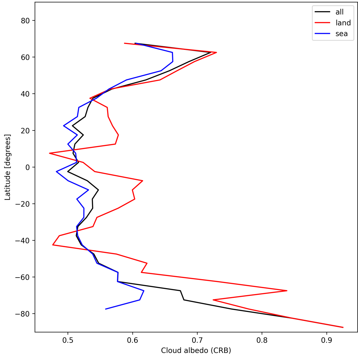
Figure 26: Zonal average of “Cloud albedo (CRB)” for 2025-01-13 to 2025-01-14.
