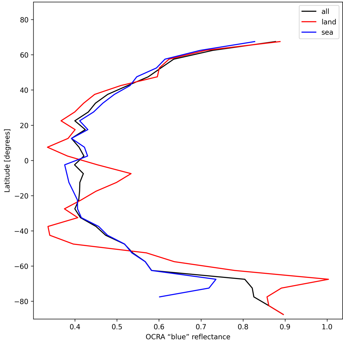
Figure 33: Zonal average of “OCRA “blue” reflectance” for 2025-01-13 to 2025-01-14.
