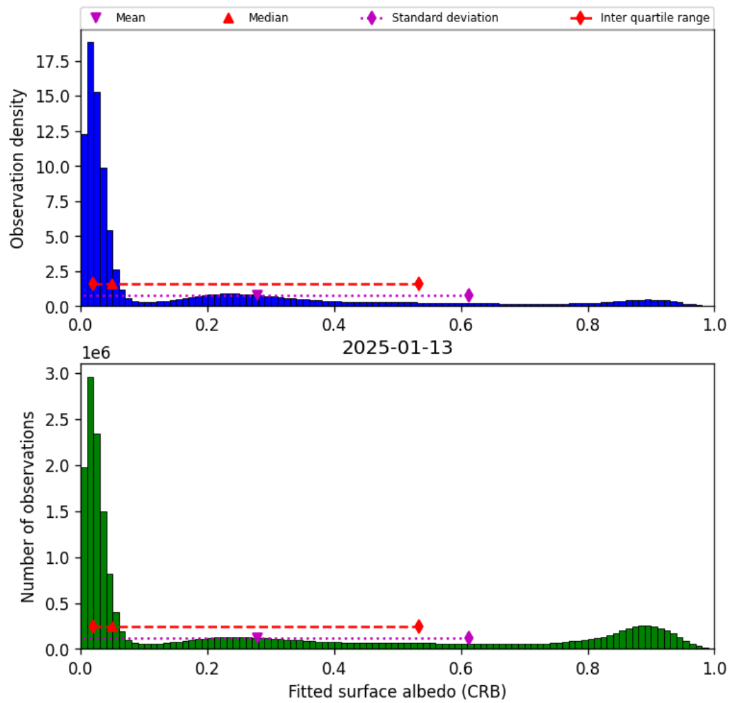
Figure 44: Histogram of “Fitted surface albedo (CRB)” for 2025-01-13 to 2025-01-14
