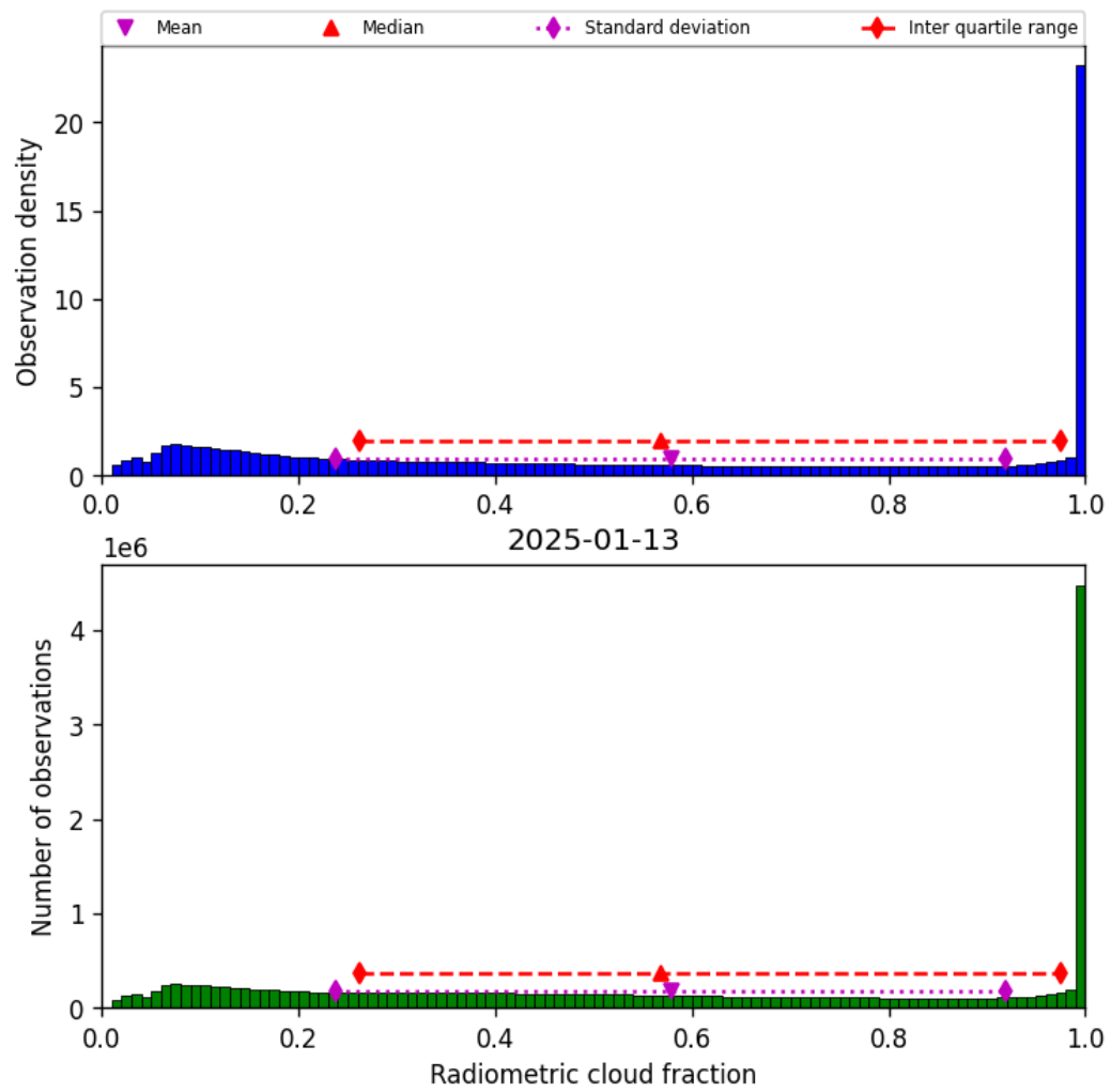
Figure 37: Histogram of “Radiometric cloud fraction” for 2025-01-13 to 2025-01-14
