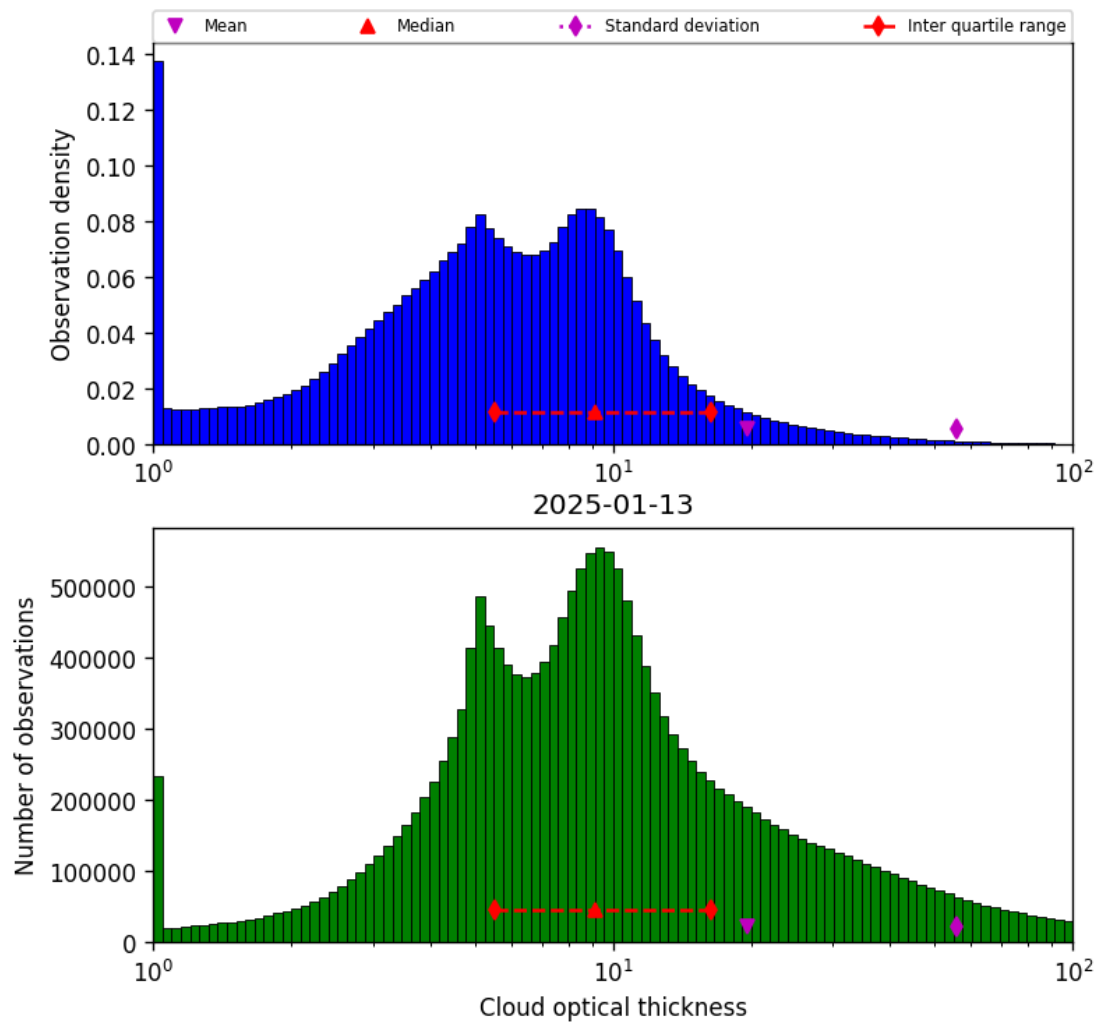
Figure 39: Histogram of “Cloud optical thickness” for 2025-01-13 to 2025-01-14
