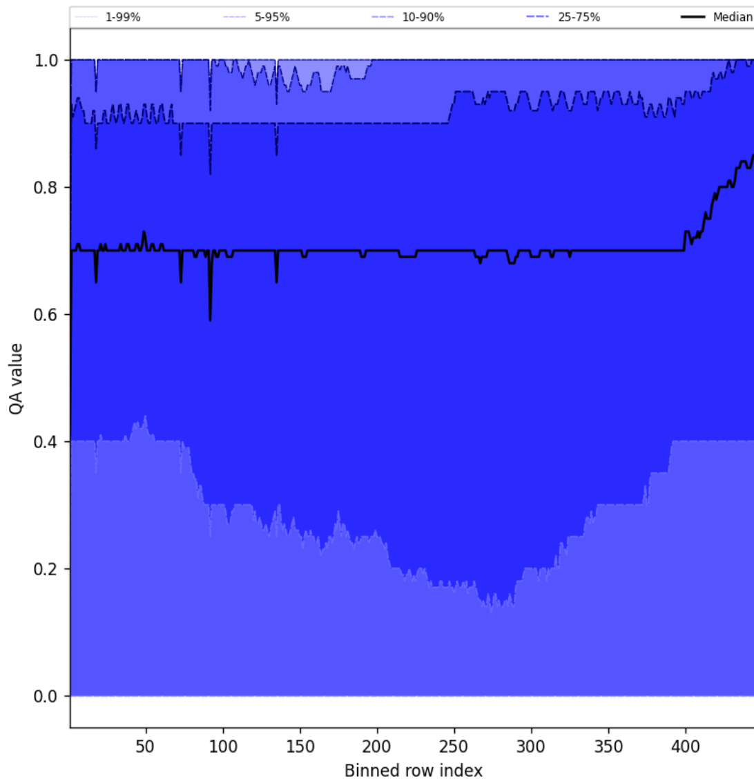
Figure 52: Along track statistics of “QA value” for 2025-01-13 to 2025-01-14
