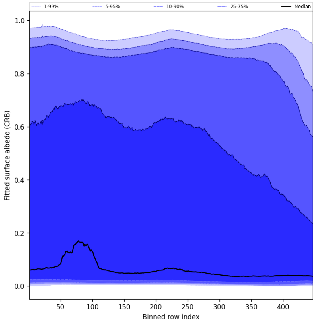
Figure 60: Along track statistics of “Fitted surface albedo (CRB)” for 2025-01-13 to 2025-01-14
