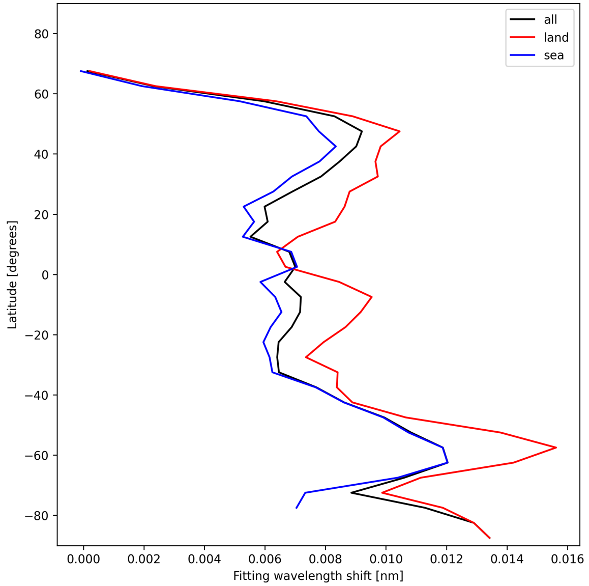
Figure 31: Zonal average of “Fitting wavelength shift” for 2025-01-13 to 2025-01-14.
