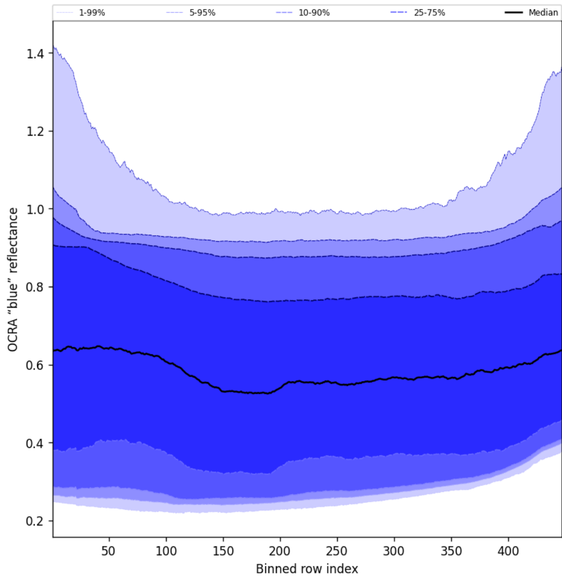
Figure 65: Along track statistics of “OCRA “blue” reflectance” for 2025-01-13 to 2025-01-14
