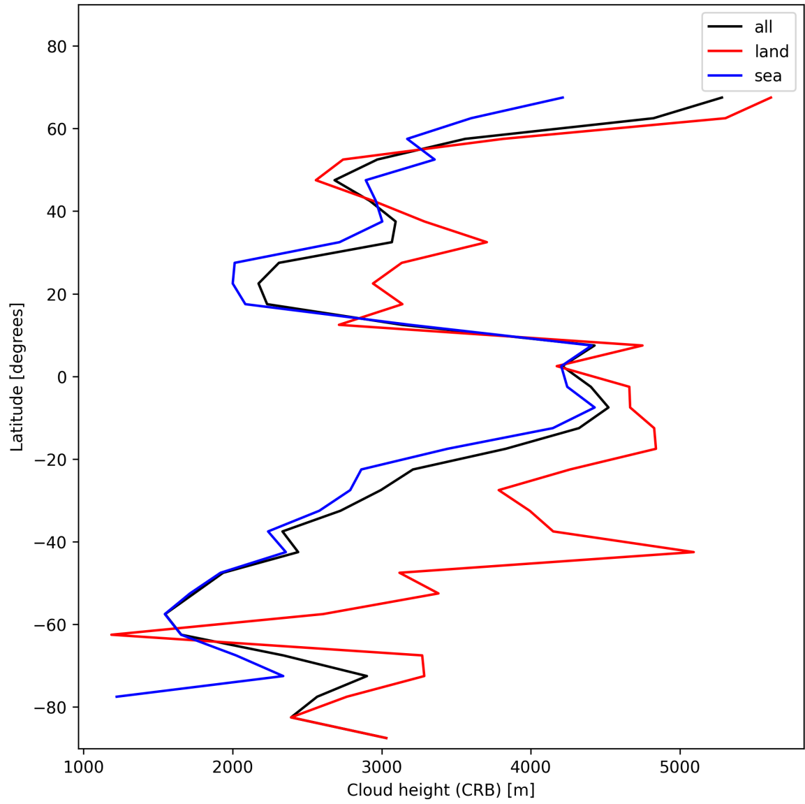
Figure 25: Zonal average of “Cloud height (CRB)” for 2025-01-13 to 2025-01-14.
