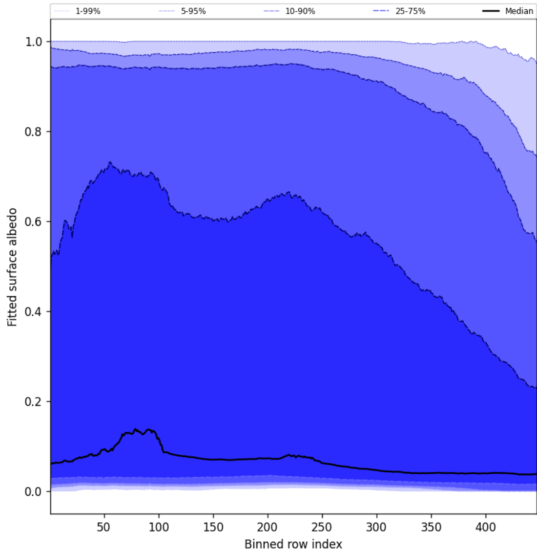
Figure 59: Along track statistics of “Fitted surface albedo” for 2025-01-16 to 2025-01-17
