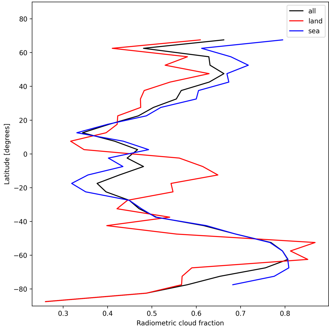
Figure 21: Zonal average of “Radiometric cloud fraction” for 2025-01-16 to 2025-01-17.
