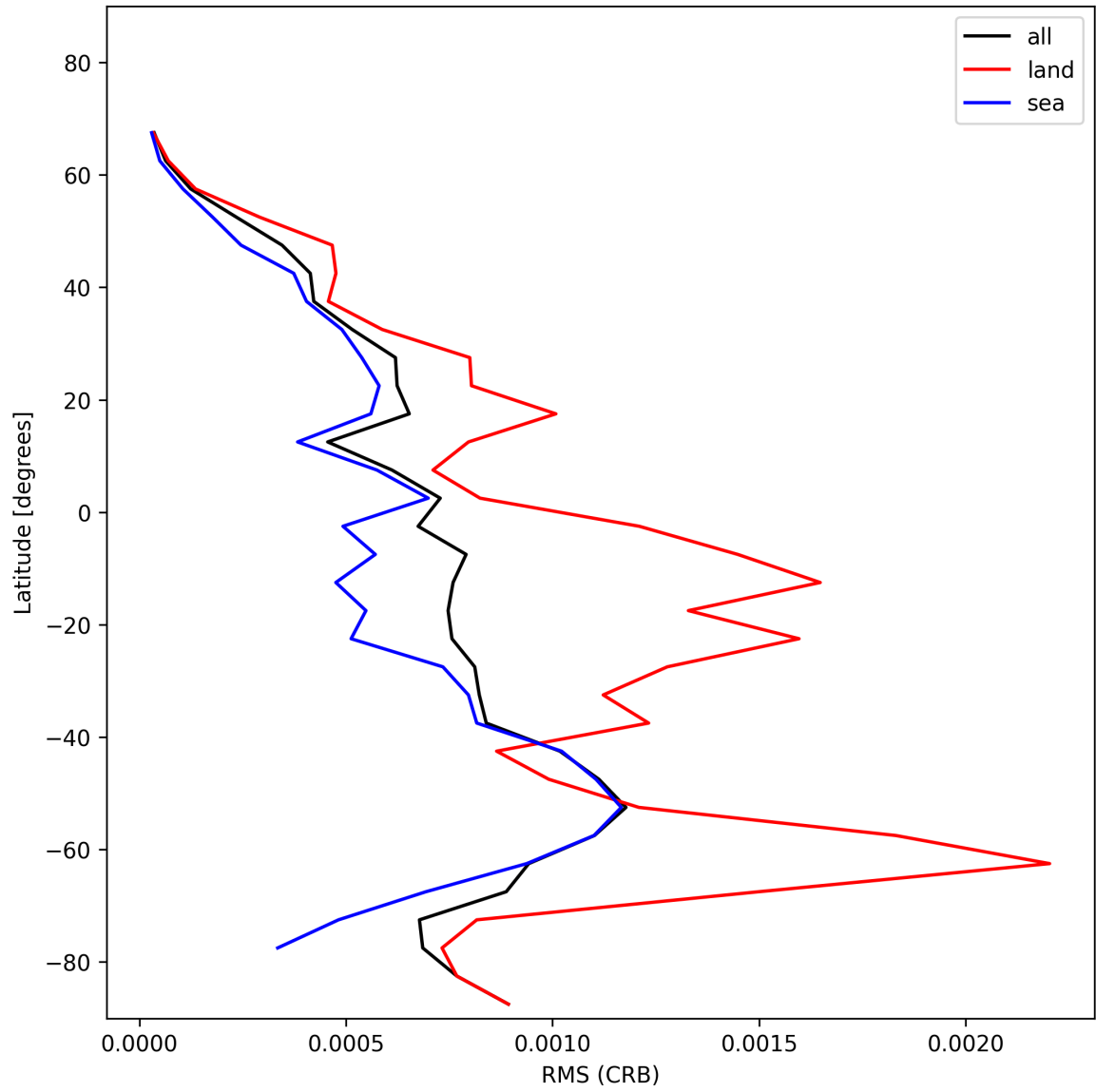
Figure 30: Zonal average of “RMS (CRB)” for 2025-01-16 to 2025-01-17.
