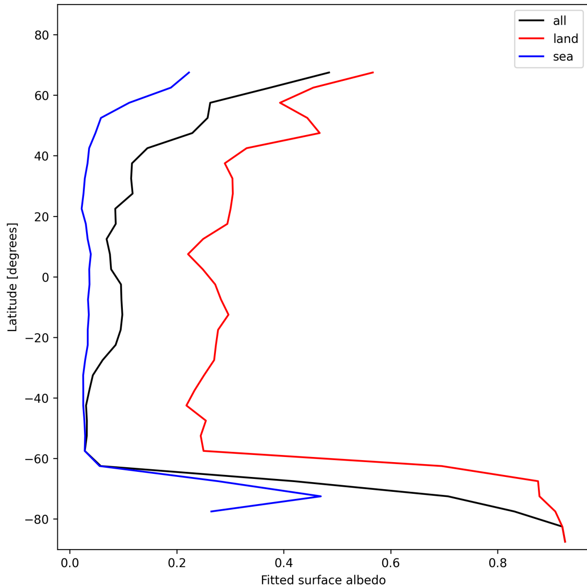
Figure 27: Zonal average of “Fitted surface albedo” for 2025-01-16 to 2025-01-17.
