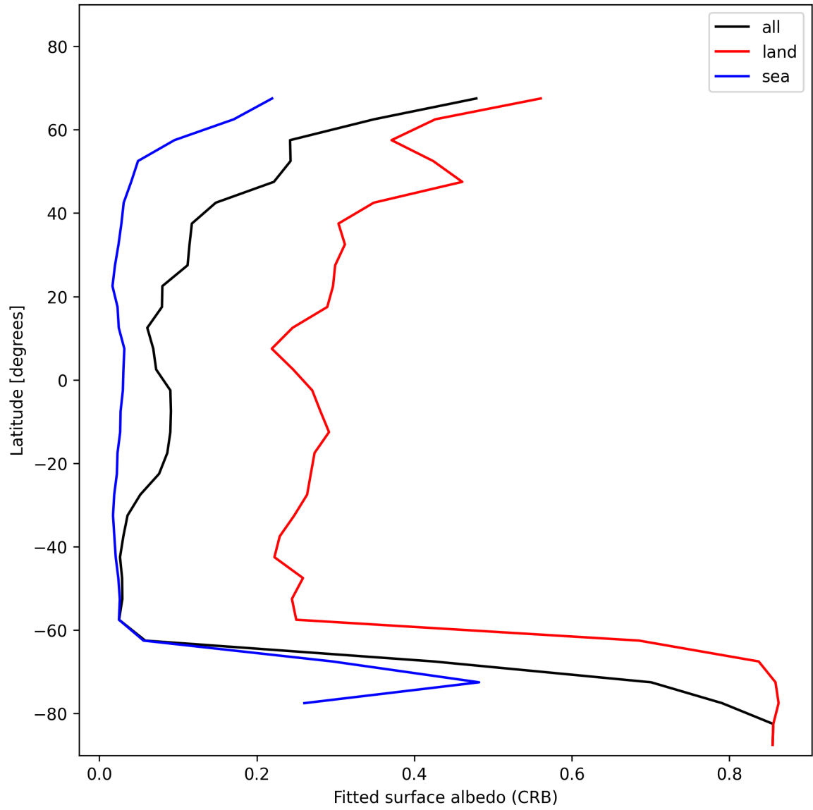
Figure 28: Zonal average of “Fitted surface albedo (CRB)” for 2025-01-16 to 2025-01-17.
