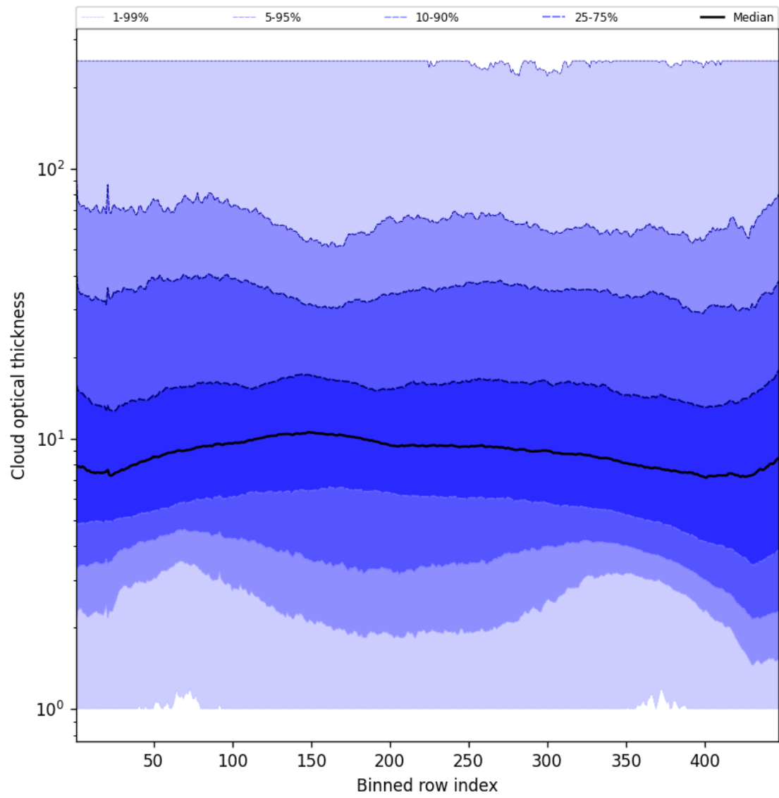
Figure 55: Along track statistics of “Cloud optical thickness” for 2025-01-16 to 2025-01-17
