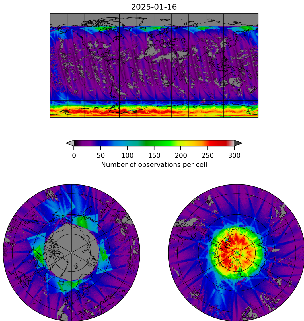
Figure 19: Map of the number of observations for 2025-01-16 to 2025-01-17
