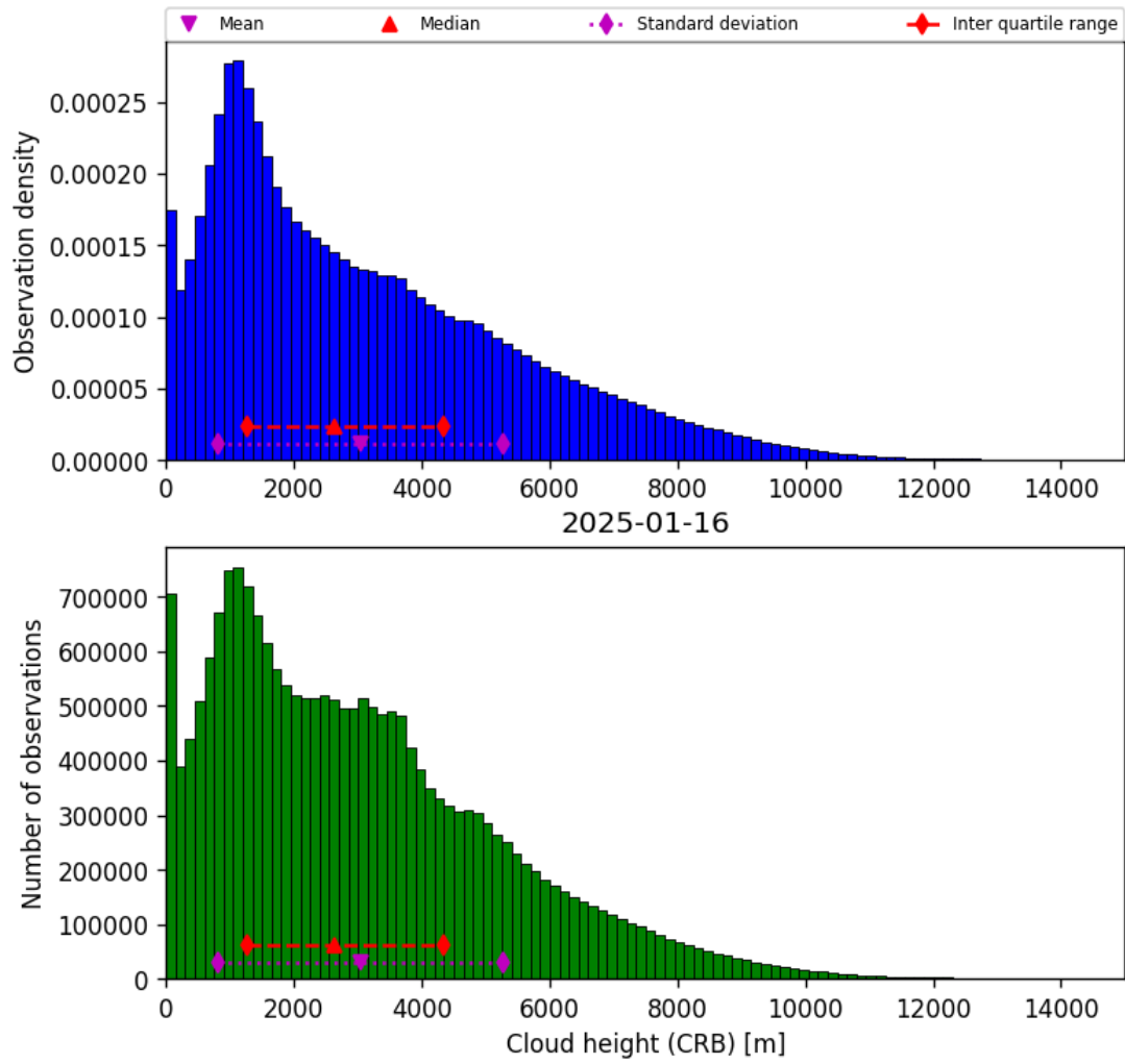
Figure 41: Histogram of “Cloud height (CRB)” for 2025-01-16 to 2025-01-17
