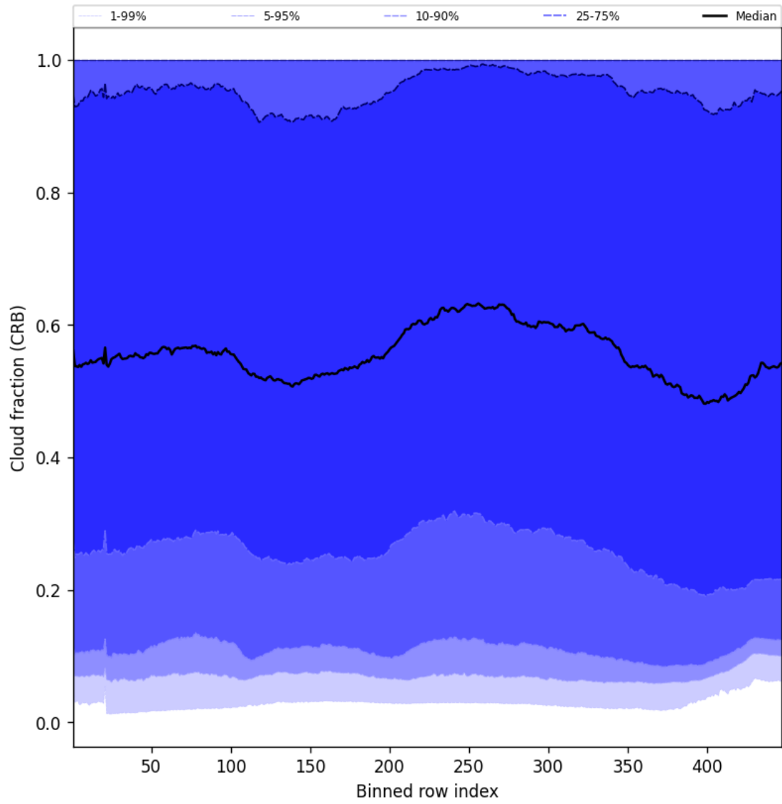
Figure 56: Along track statistics of “Cloud fraction (CRB)” for 2025-01-16 to 2025-01-17
