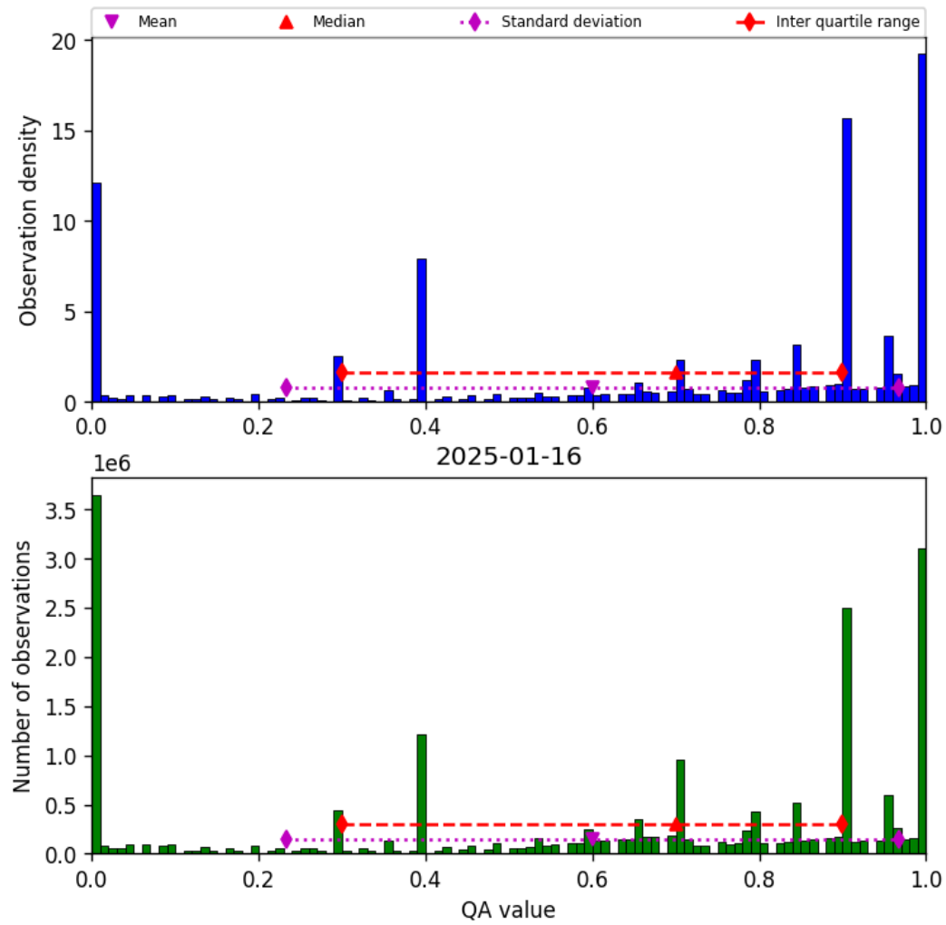
Figure 36: Histogram of “QA value” for 2025-01-16 to 2025-01-17
