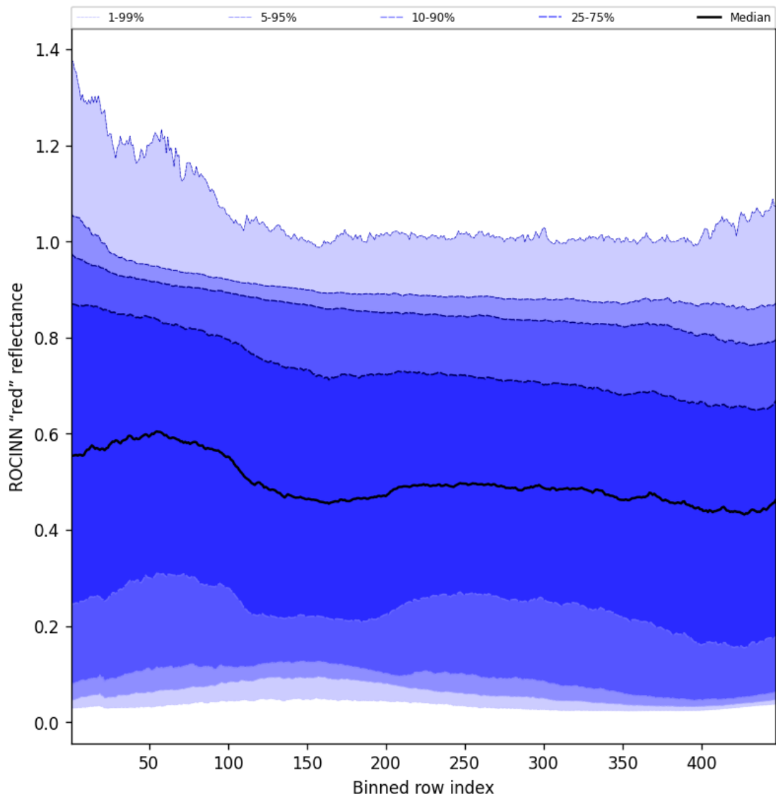
Figure 67: Along track statistics of “ROCINN “red” reflectance” for 2025-01-16 to 2025-01-17
