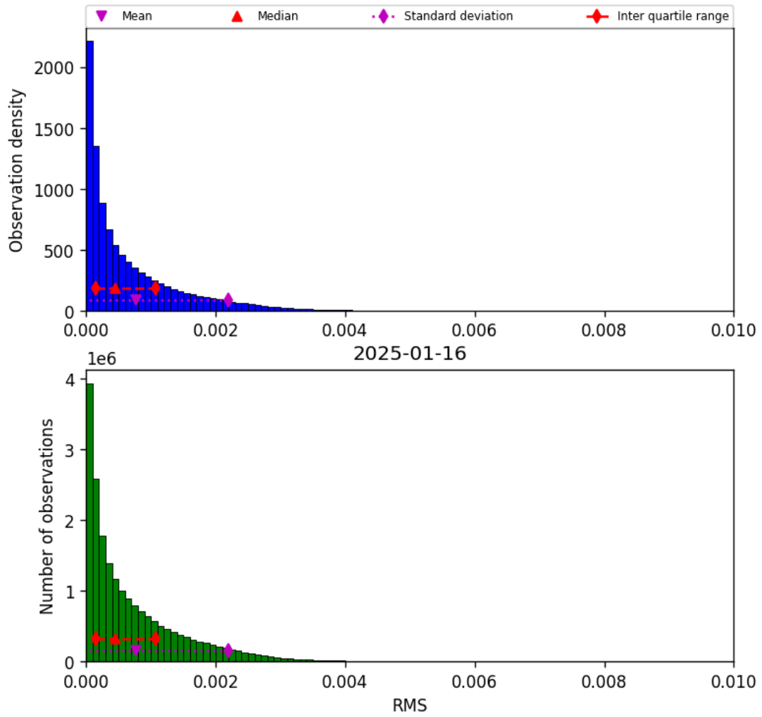
Figure 45: Histogram of “RMS” for 2025-01-16 to 2025-01-17
