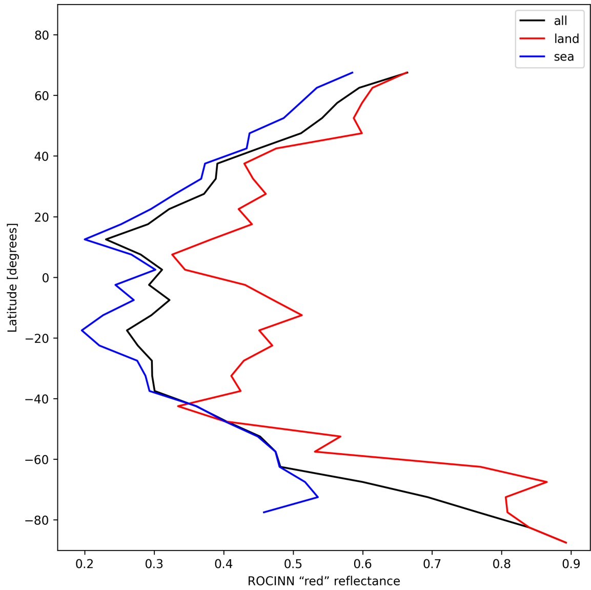
Figure 35: Zonal average of “ROCINN “red” reflectance” for 2025-01-16 to 2025-01-17.
