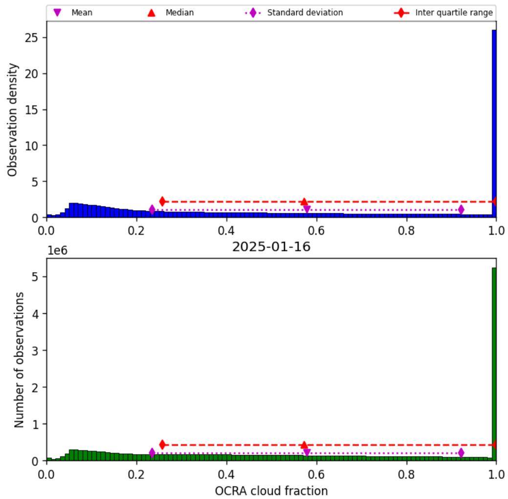
Figure 48: Histogram of “OCRA cloud fraction” for 2025-01-16 to 2025-01-17
