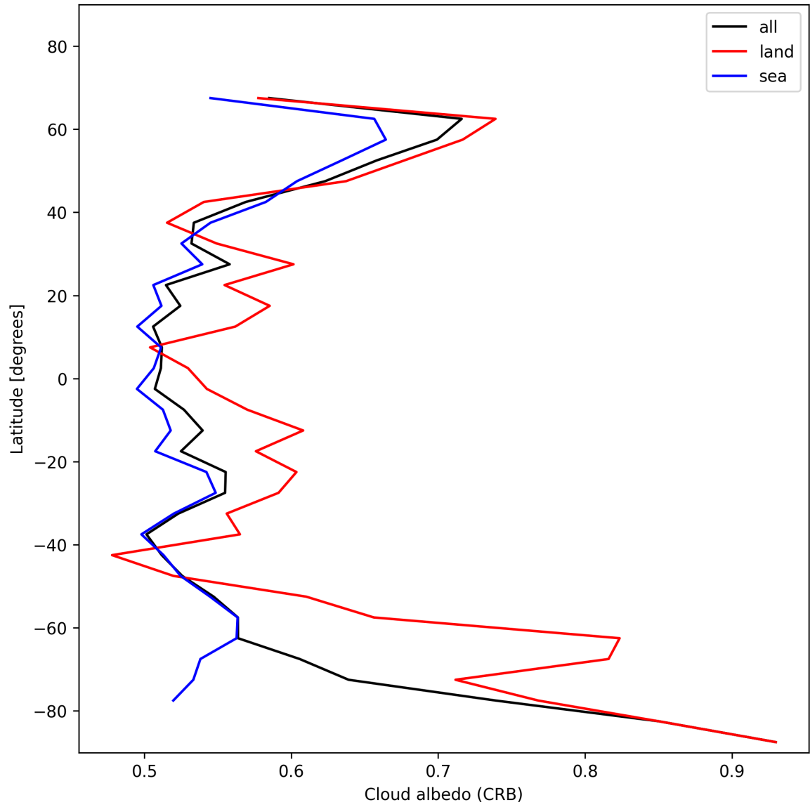
Figure 26: Zonal average of “Cloud albedo (CRB)” for 2025-01-16 to 2025-01-17.
