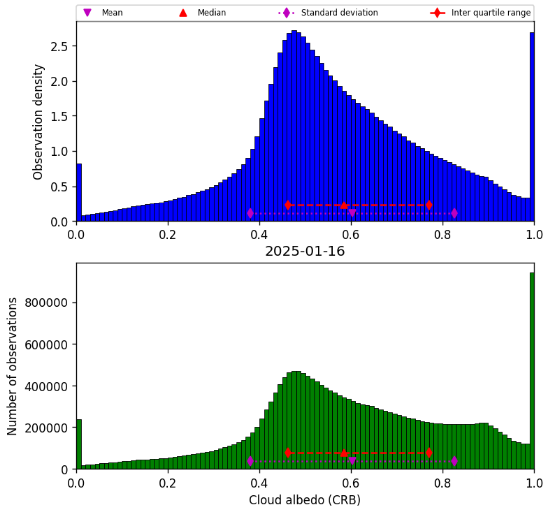
Figure 42: Histogram of “Cloud albedo (CRB)” for 2025-01-16 to 2025-01-17
