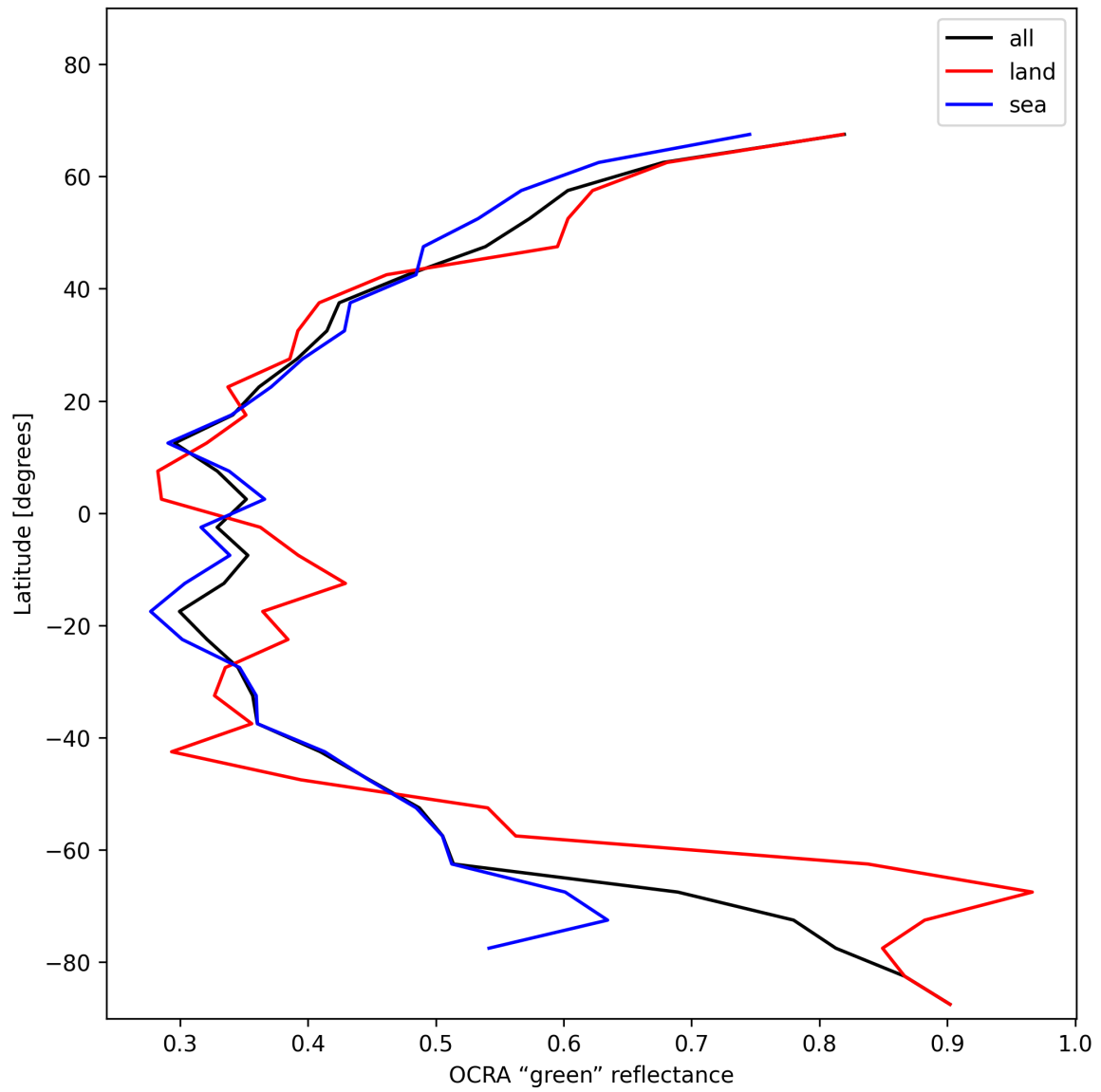
Figure 34: Zonal average of “OCRA “green” reflectance” for 2025-01-16 to 2025-01-17.
