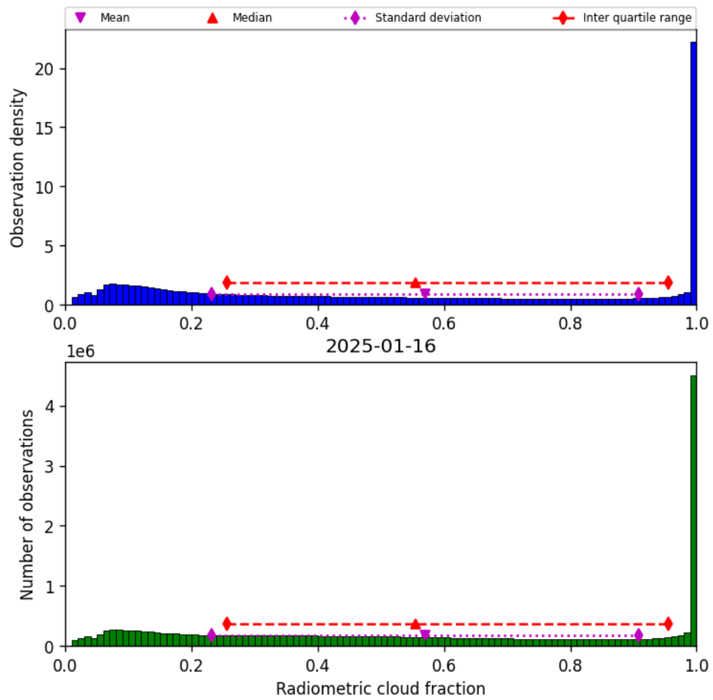
Figure 37: Histogram of “Radiometric cloud fraction” for 2025-01-16 to 2025-01-17
