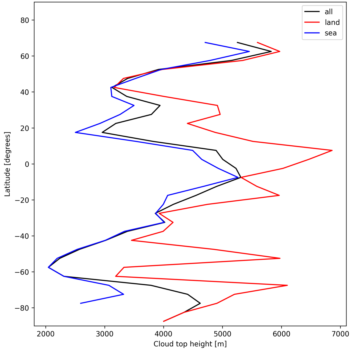
Figure 22: Zonal average of “Cloud top height” for 2025-01-16 to 2025-01-17.
