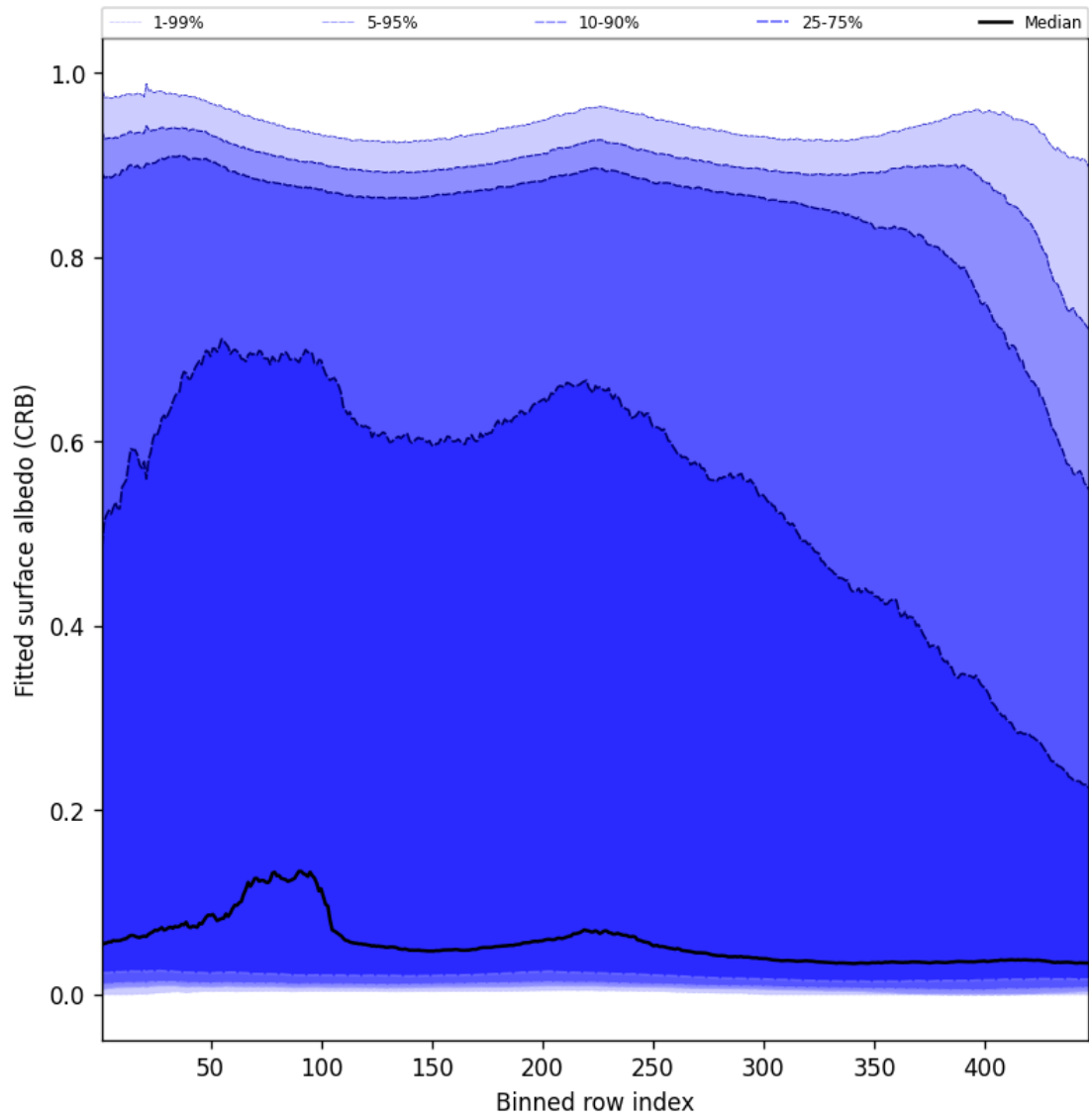
Figure 60: Along track statistics of “Fitted surface albedo (CRB)” for 2025-01-16 to 2025-01-17
