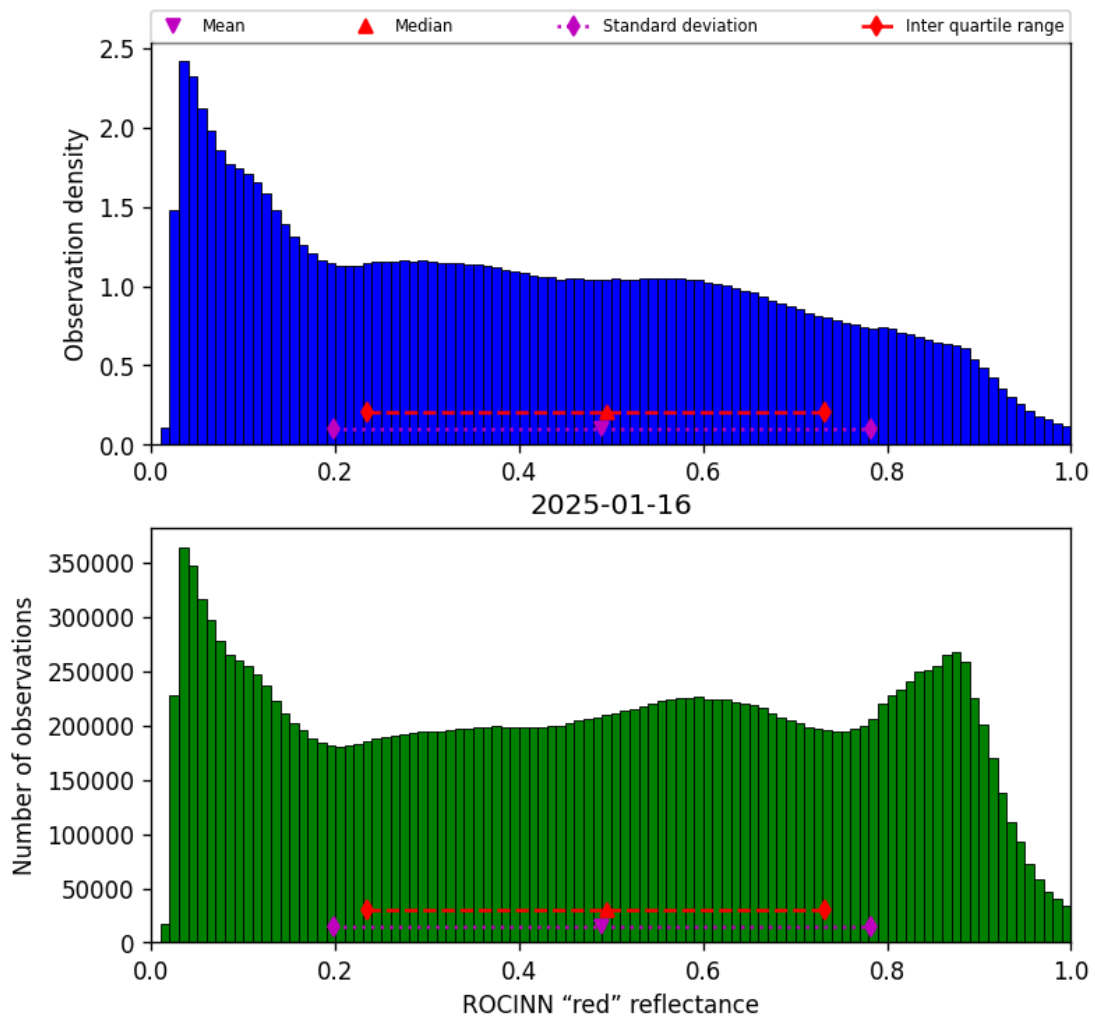
Figure 51: Histogram of “ROCINN “red” reflectance” for 2025-01-16 to 2025-01-17
