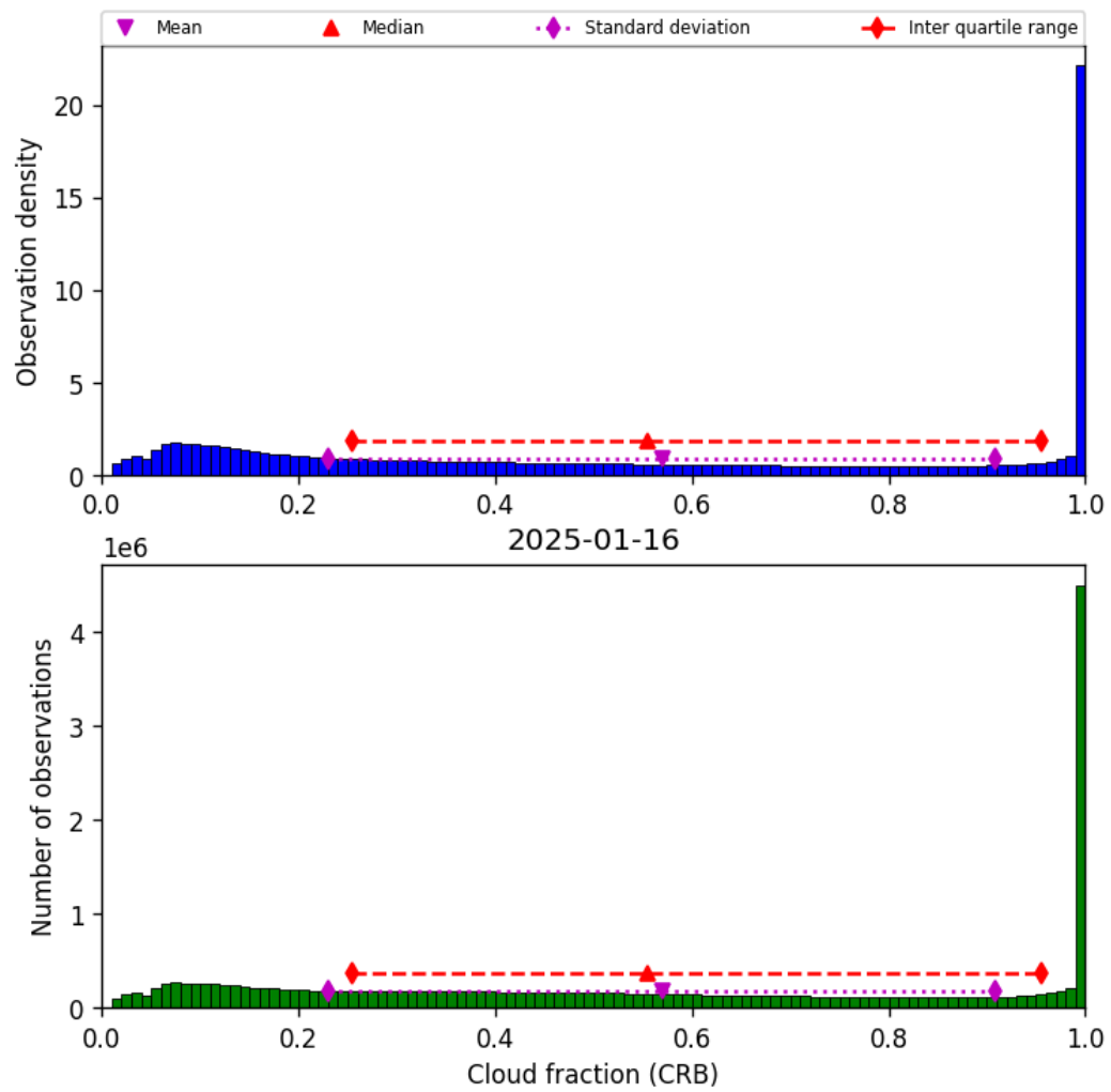
Figure 40: Histogram of "Cloud fraction (CRB)" for 2025-01-16 to 2025-01-17
