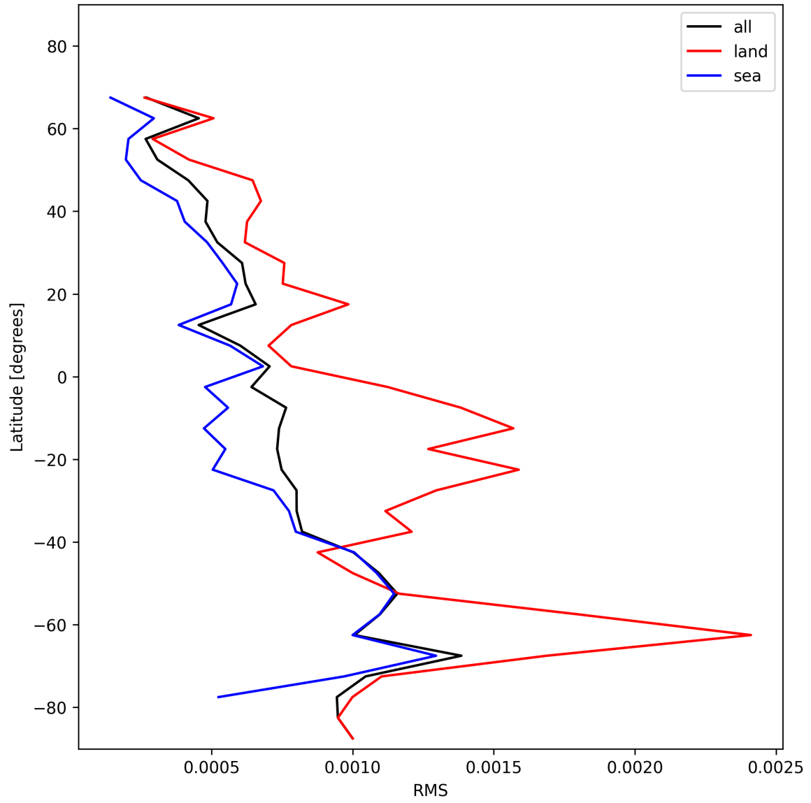
Figure 29: Zonal average of “RMS” for 2025-01-16 to 2025-01-17.
