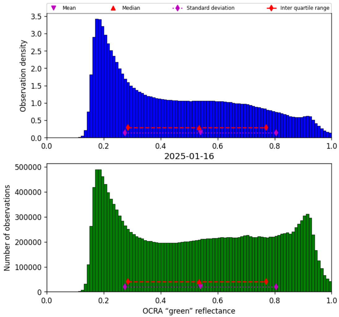
Figure 50: Histogram of “OCRA “green” reflectance” for 2025-01-16 to 2025-01-17
