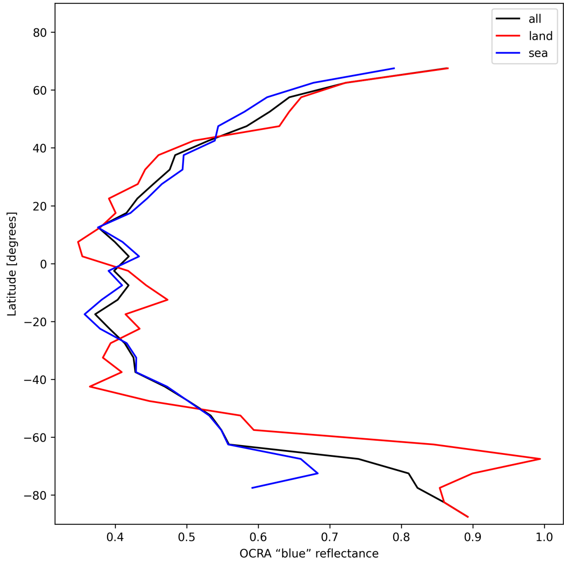
Figure 33: Zonal average of “OCRA “blue” reflectance” for 2025-01-16 to 2025-01-17.
