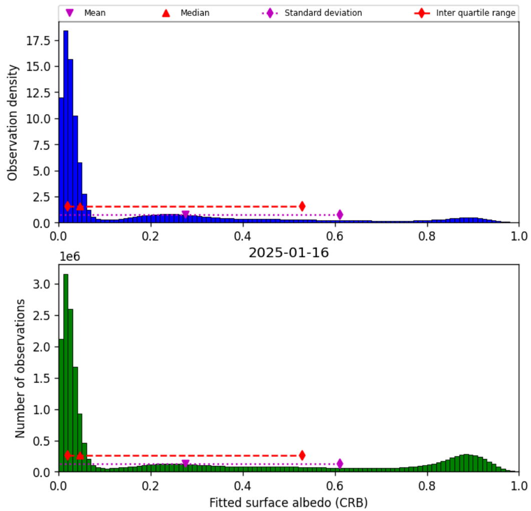
Figure 44: Histogram of “Fitted surface albedo (CRB)” for 2025-01-16 to 2025-01-17
