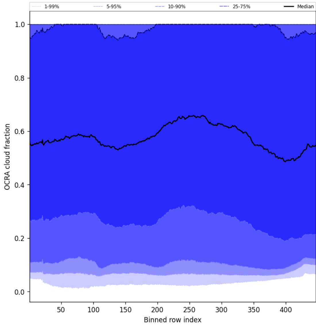
Figure 64: Along track statistics of “OCRA cloud fraction” for 2025-01-16 to 2025-01-17
