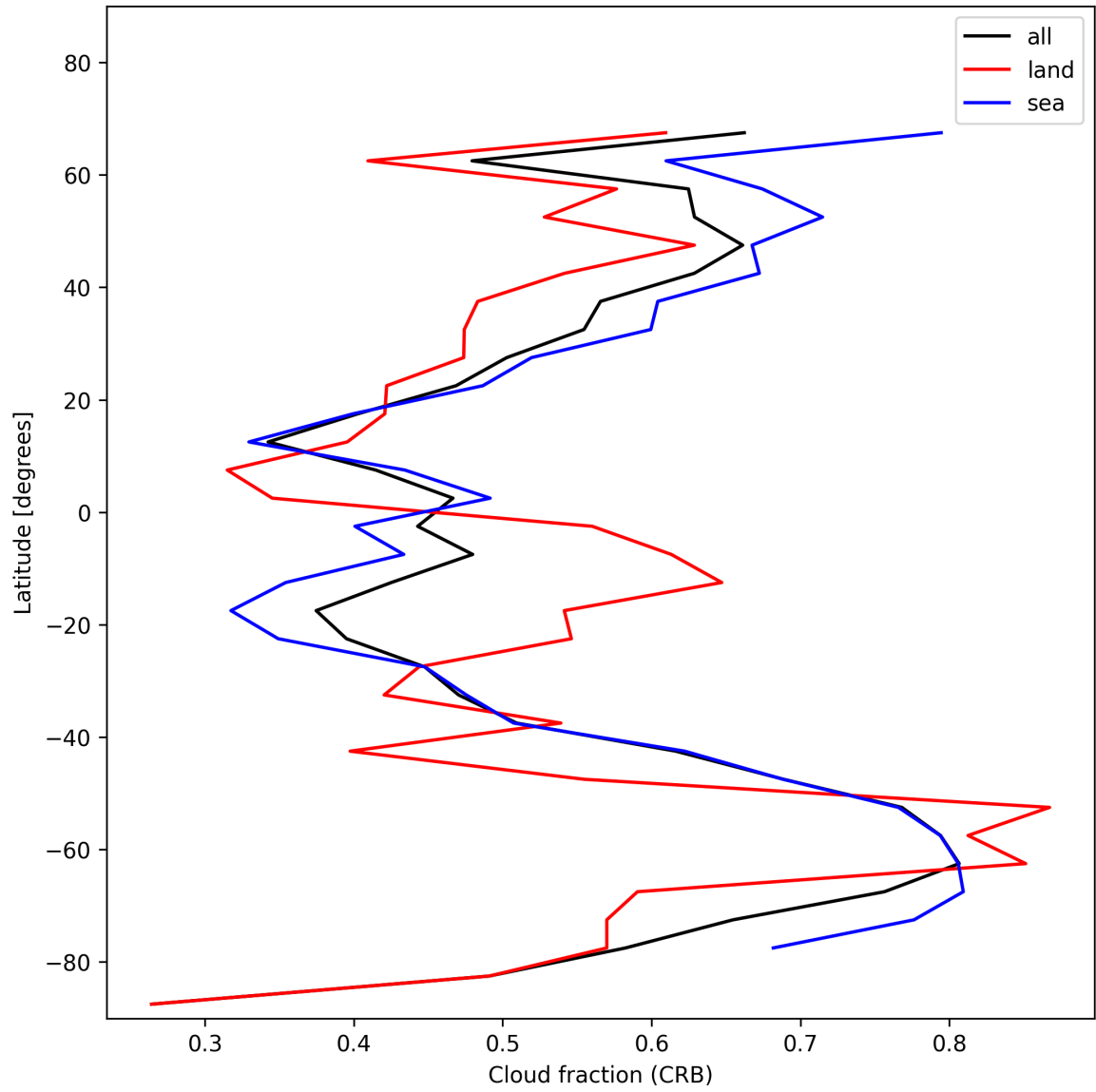
Figure 24: Zonal average of “Cloud fraction (CRB)” for 2025-01-16 to 2025-01-17.
