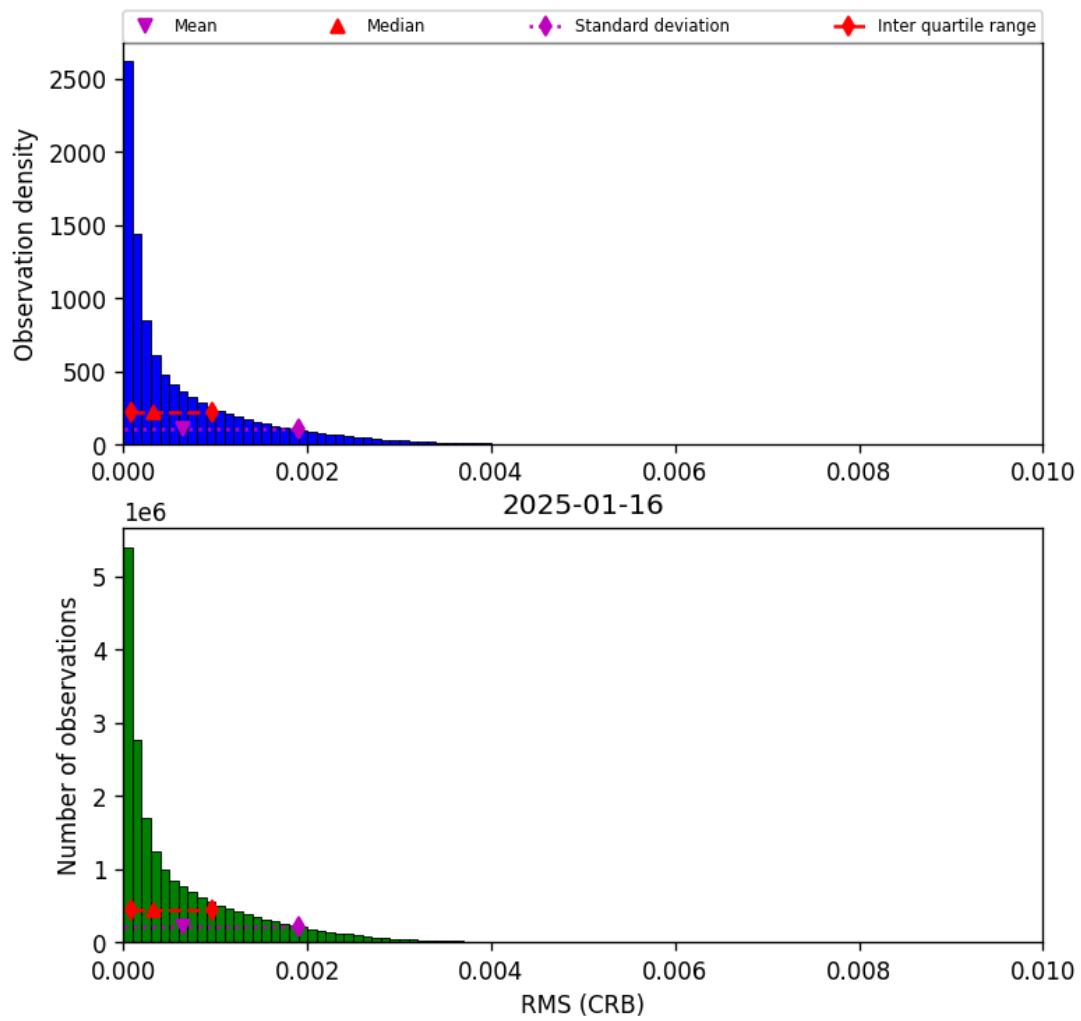
Figure 46: Histogram of “RMS (CRB)” for 2025-01-16 to 2025-01-17
