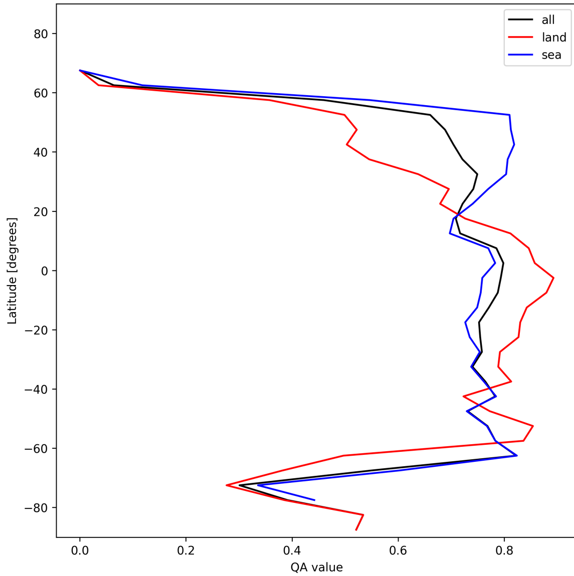
Figure 20: Zonal average of “QA value” for 2025-01-16 to 2025-01-17.
