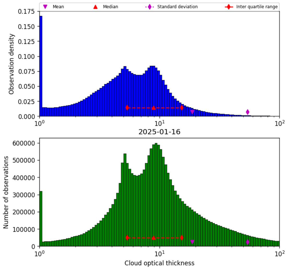
Figure 39: Histogram of “Cloud optical thickness” for 2025-01-16 to 2025-01-17
