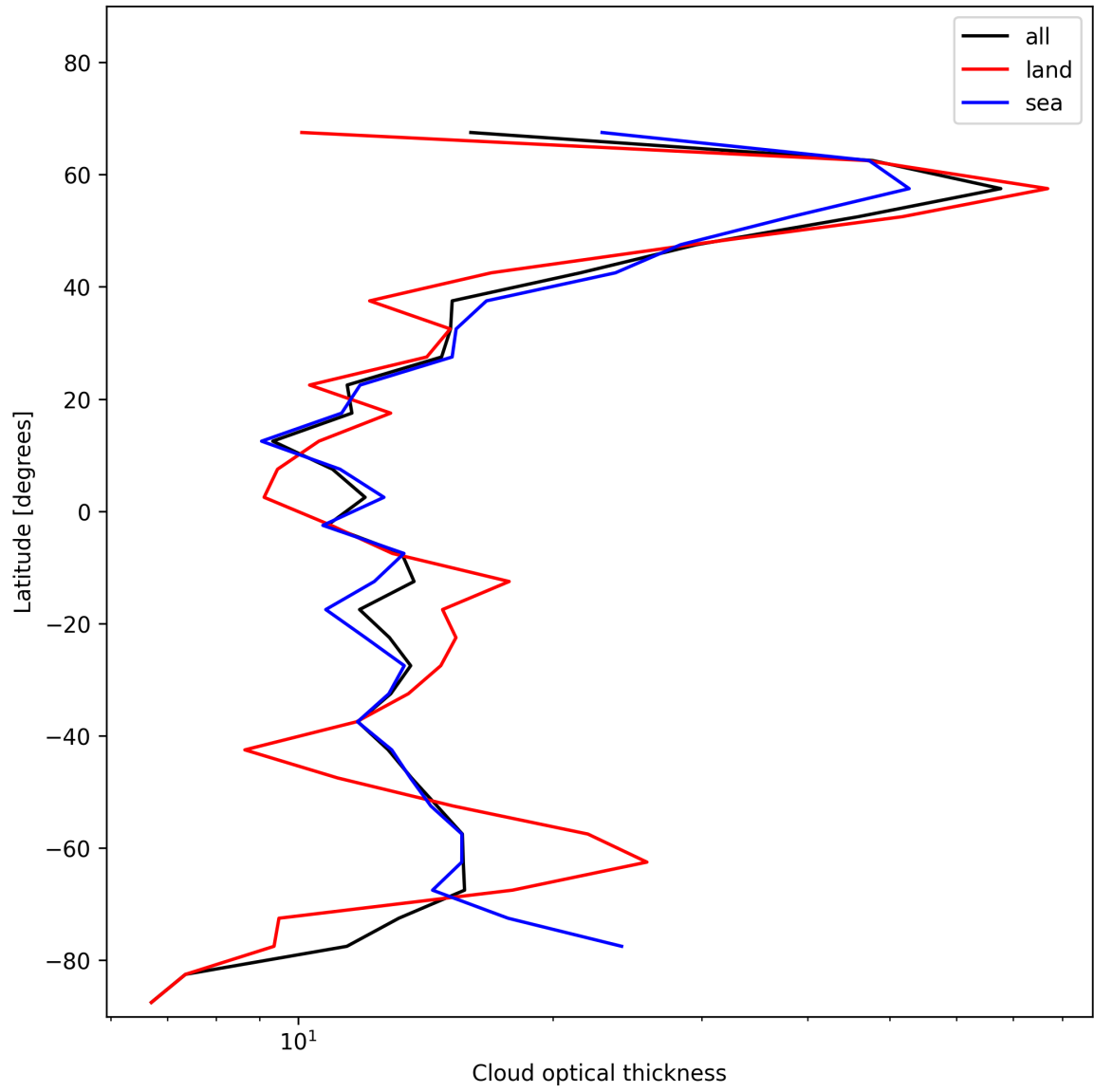
Figure 23: Zonal average of “Cloud optical thickness” for 2025-01-16 to 2025-01-17.
