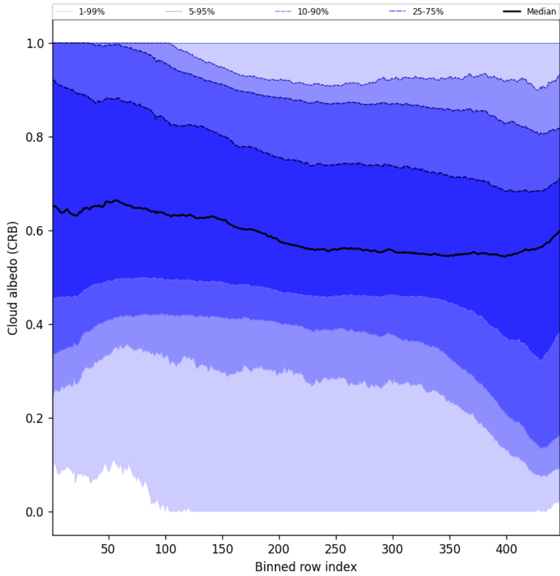
Figure 58: Along track statistics of “Cloud albedo (CRB)” for 2025-01-16 to 2025-01-17
