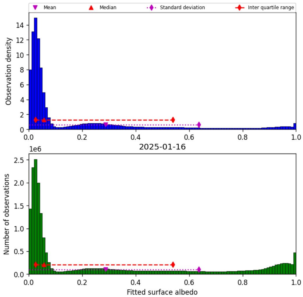
Figure 43: Histogram of “Fitted surface albedo” for 2025-01-16 to 2025-01-17
