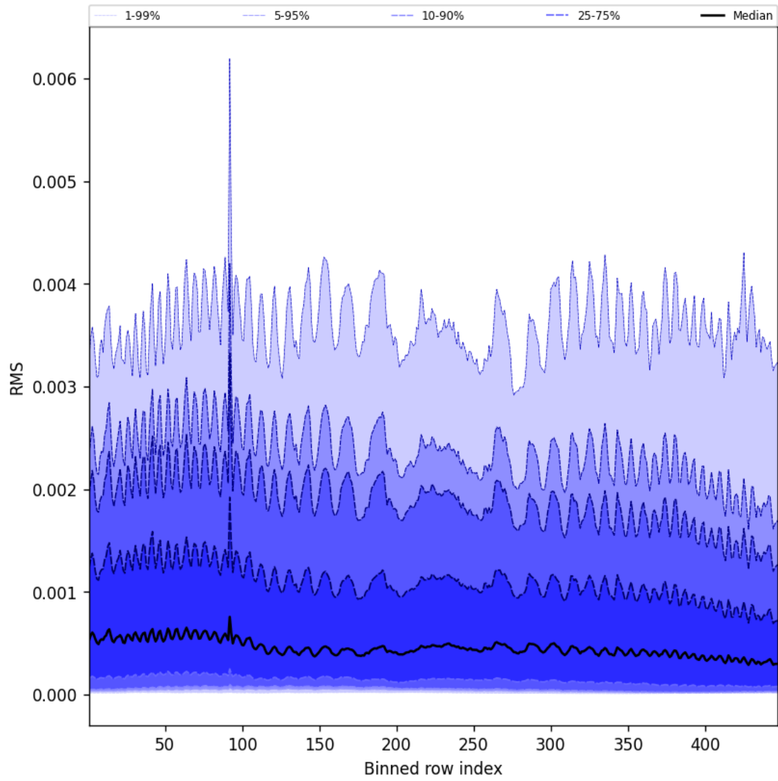
Figure 61: Along track statistics of “RMS” for 2025-01-16 to 2025-01-17
