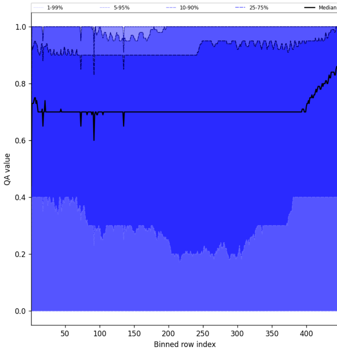
Figure 52: Along track statistics of “QA value” for 2025-01-16 to 2025-01-17
