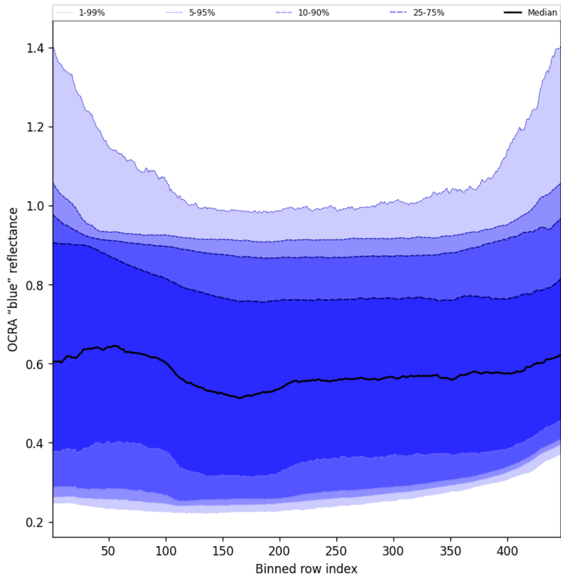
Figure 65: Along track statistics of “OCRA “blue” reflectance” for 2025-01-16 to 2025-01-17
