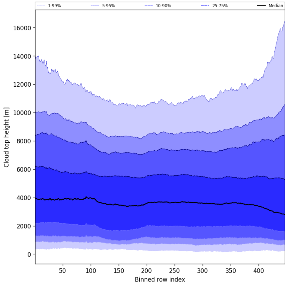
Figure 54: Along track statistics of “Cloud top height” for 2025-01-16 to 2025-01-17
