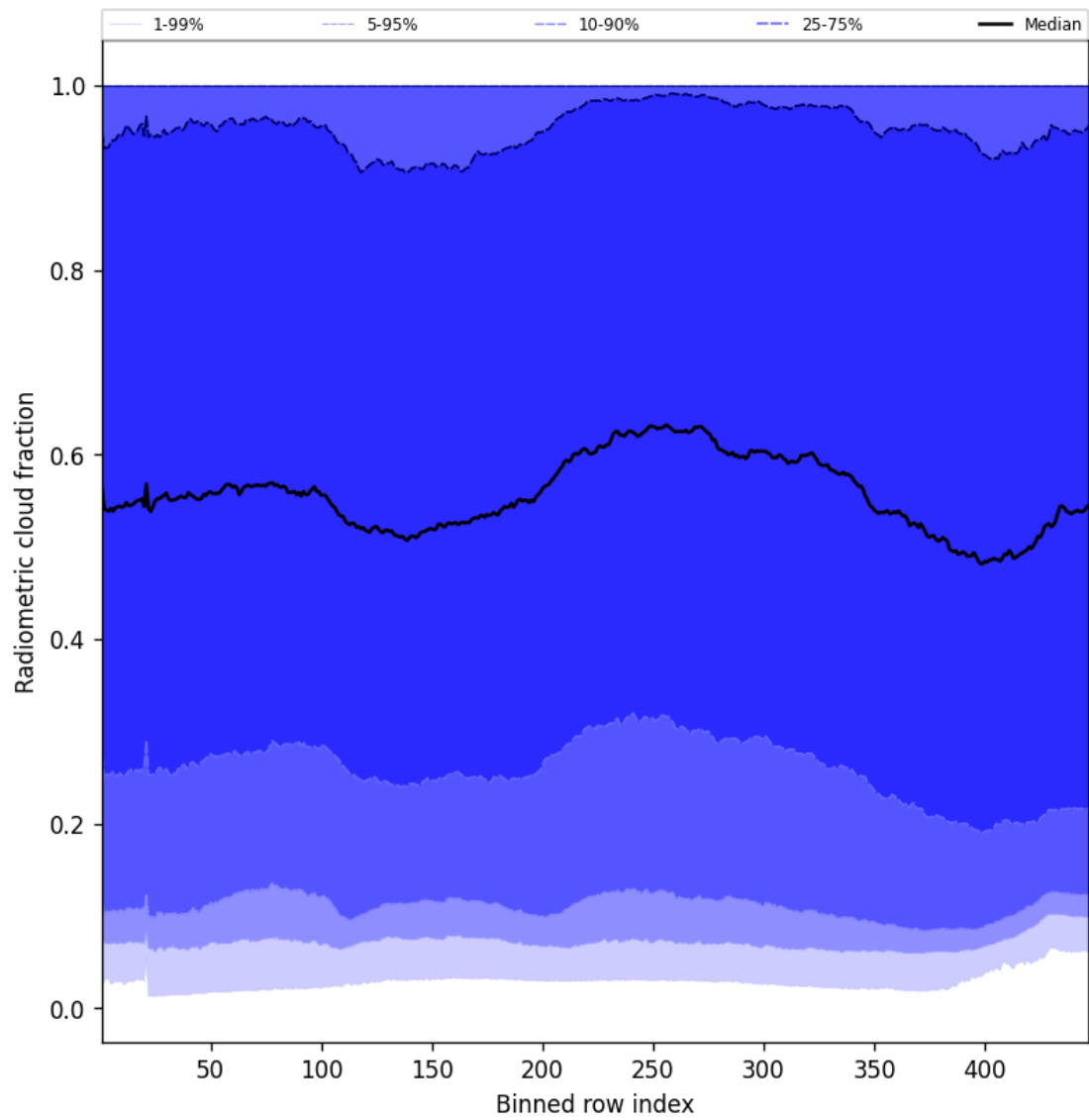
Figure 53: Along track statistics of “Radiometric cloud fraction” for 2025-01-16 to 2025-01-17
