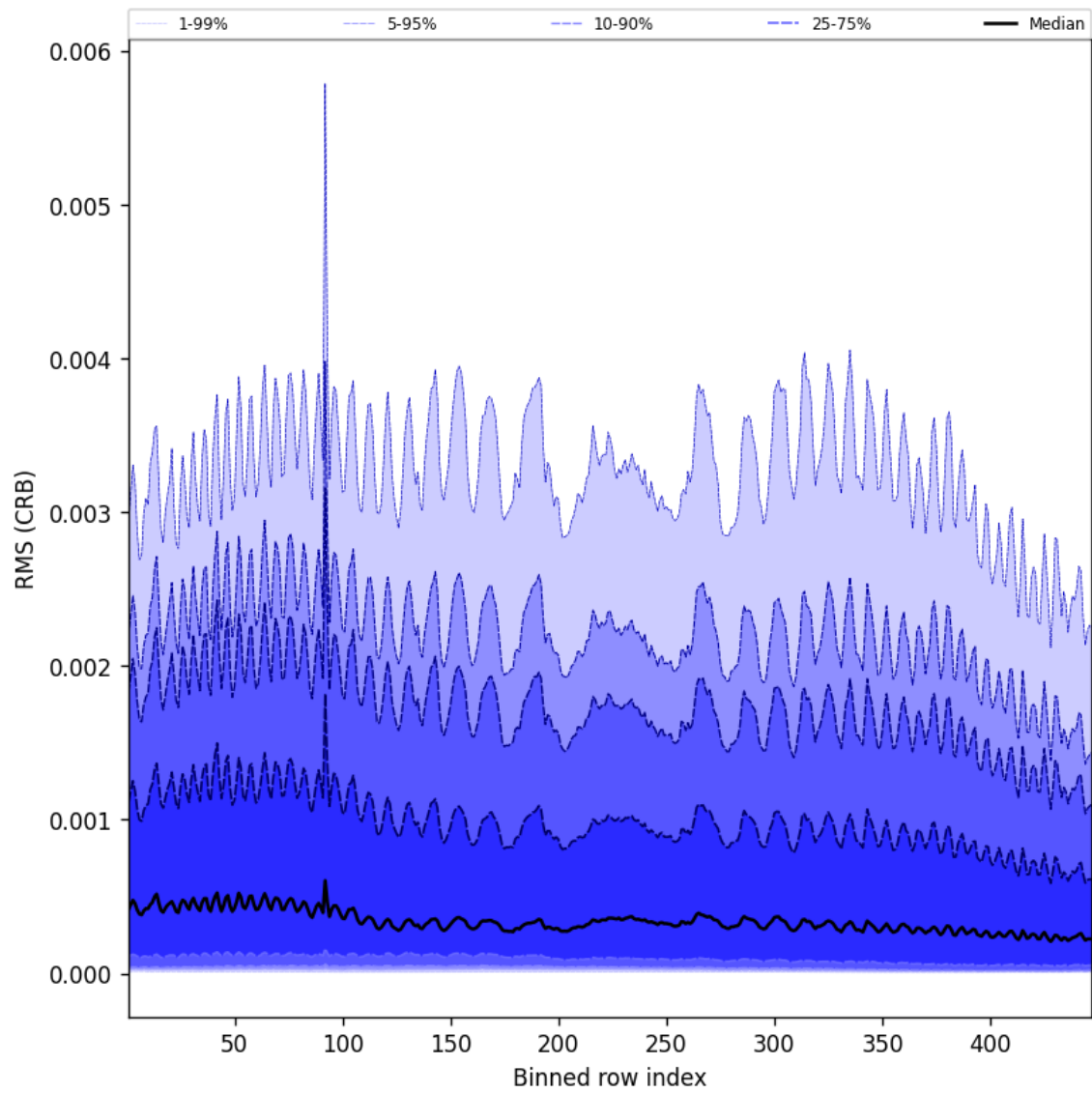
Figure 62: Along track statistics of “RMS (CRB)” for 2025-01-16 to 2025-01-17
