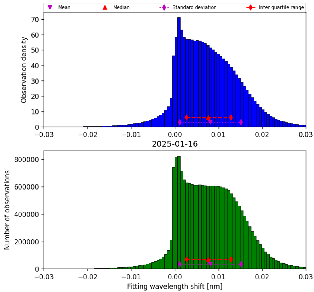
Figure 47: Histogram of “Fitting wavelength shift” for 2025-01-16 to 2025-01-17
