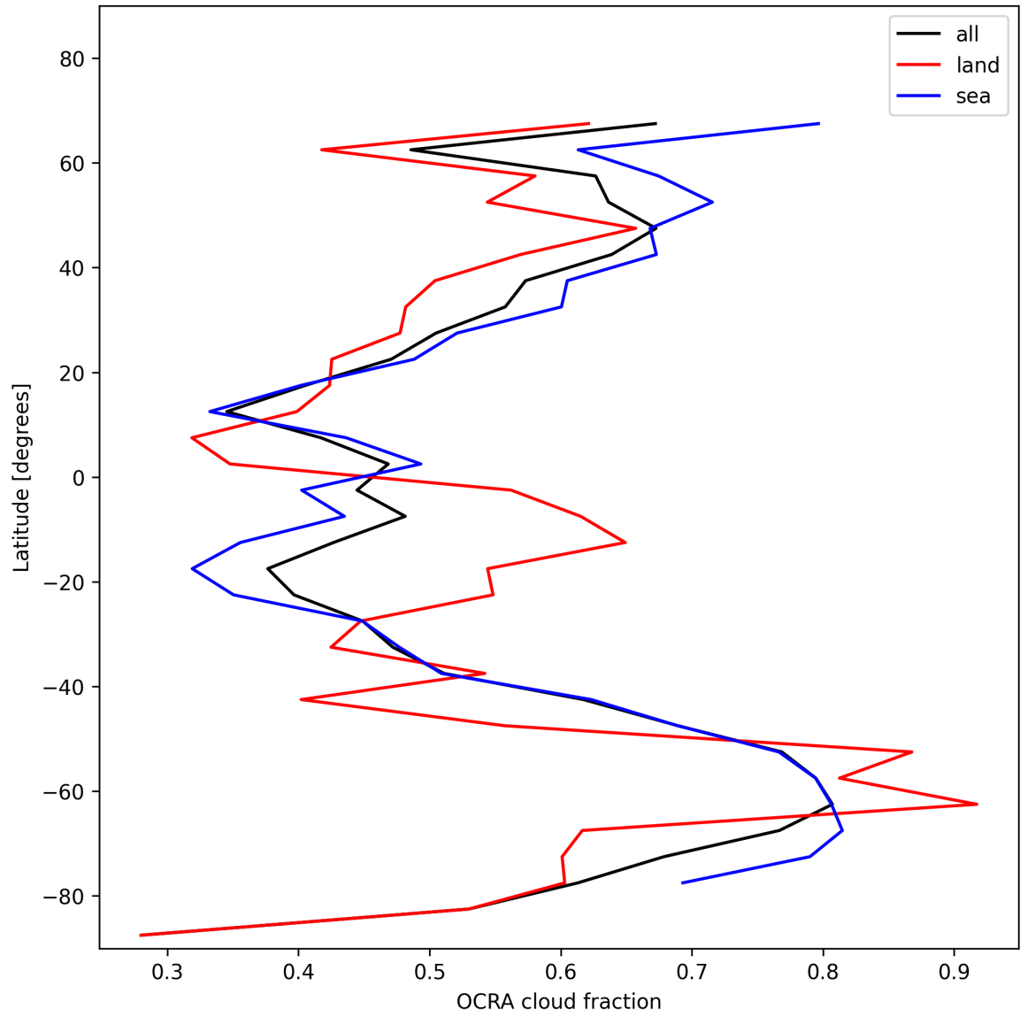
Figure 32: Zonal average of “OCRA cloud fraction” for 2025-01-16 to 2025-01-17.
