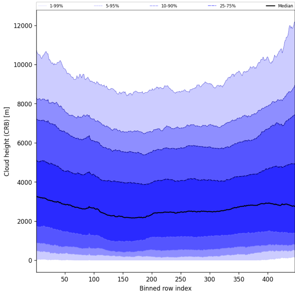
Figure 57: Along track statistics of “Cloud height (CRB)” for 2025-01-16 to 2025-01-17
