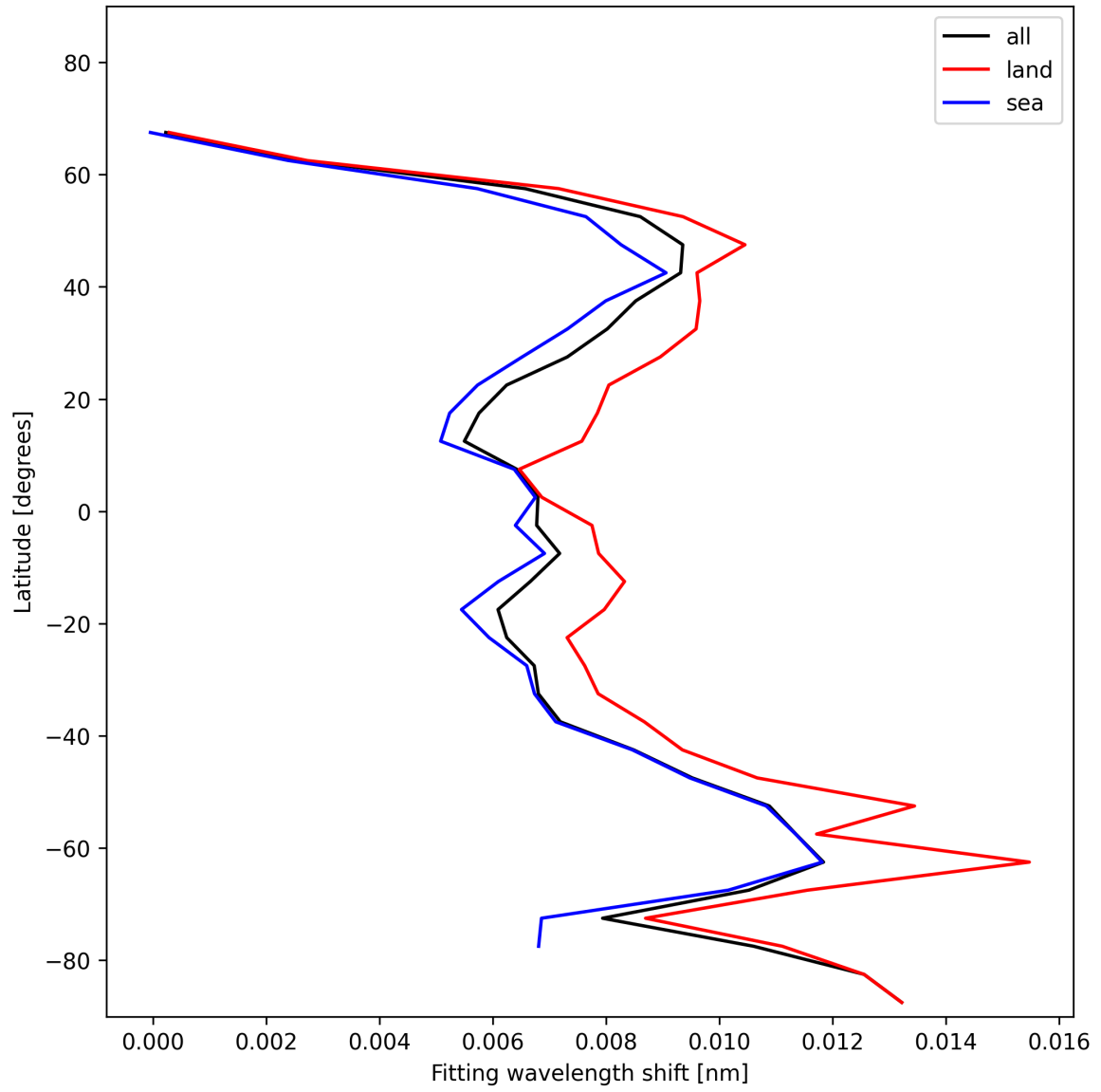
Figure 31: Zonal average of “Fitting wavelength shift” for 2025-01-16 to 2025-01-17.
