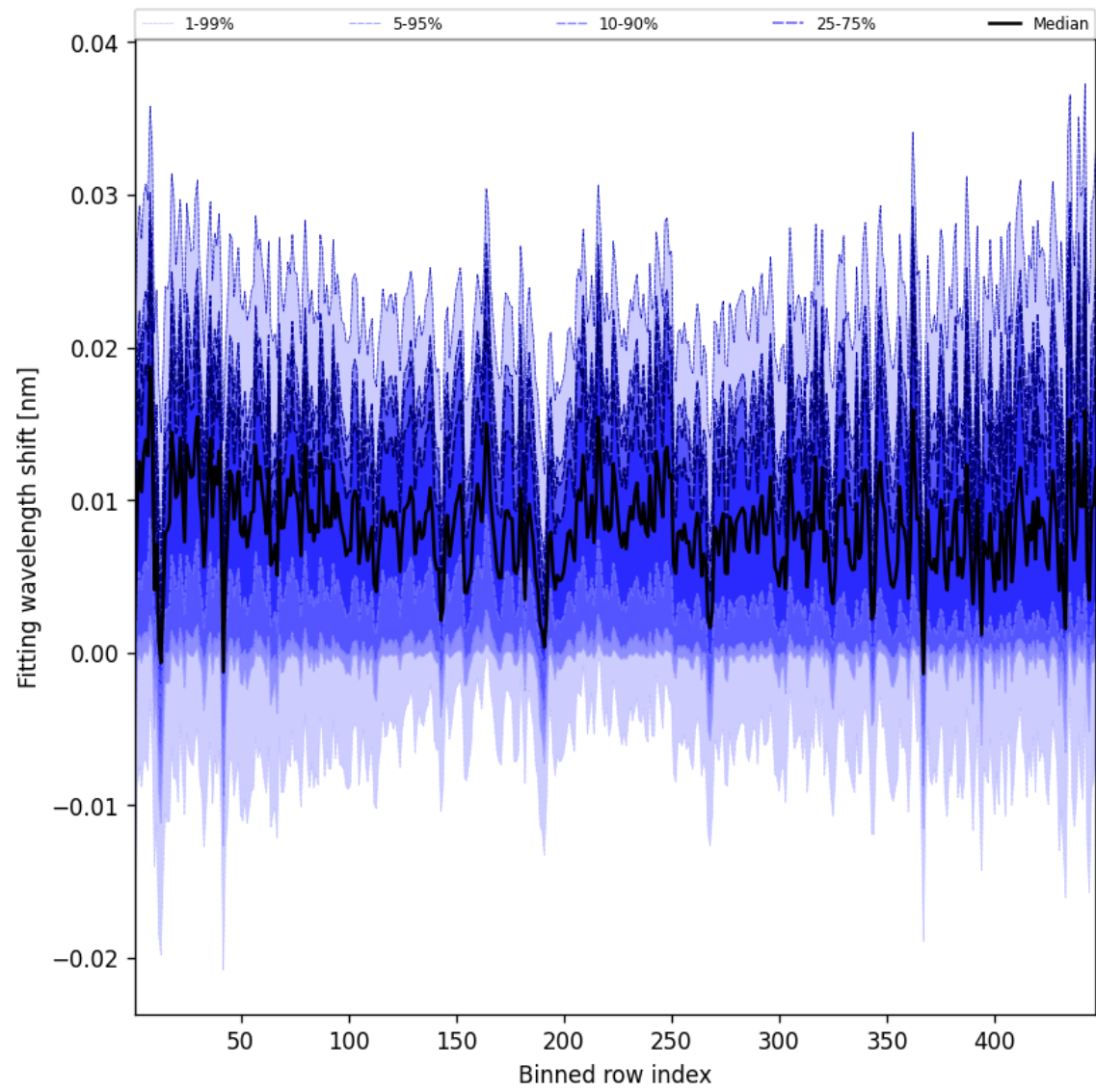
Figure 63: Along track statistics of “Fitting wavelength shift” for 2025-01-16 to 2025-01-17
