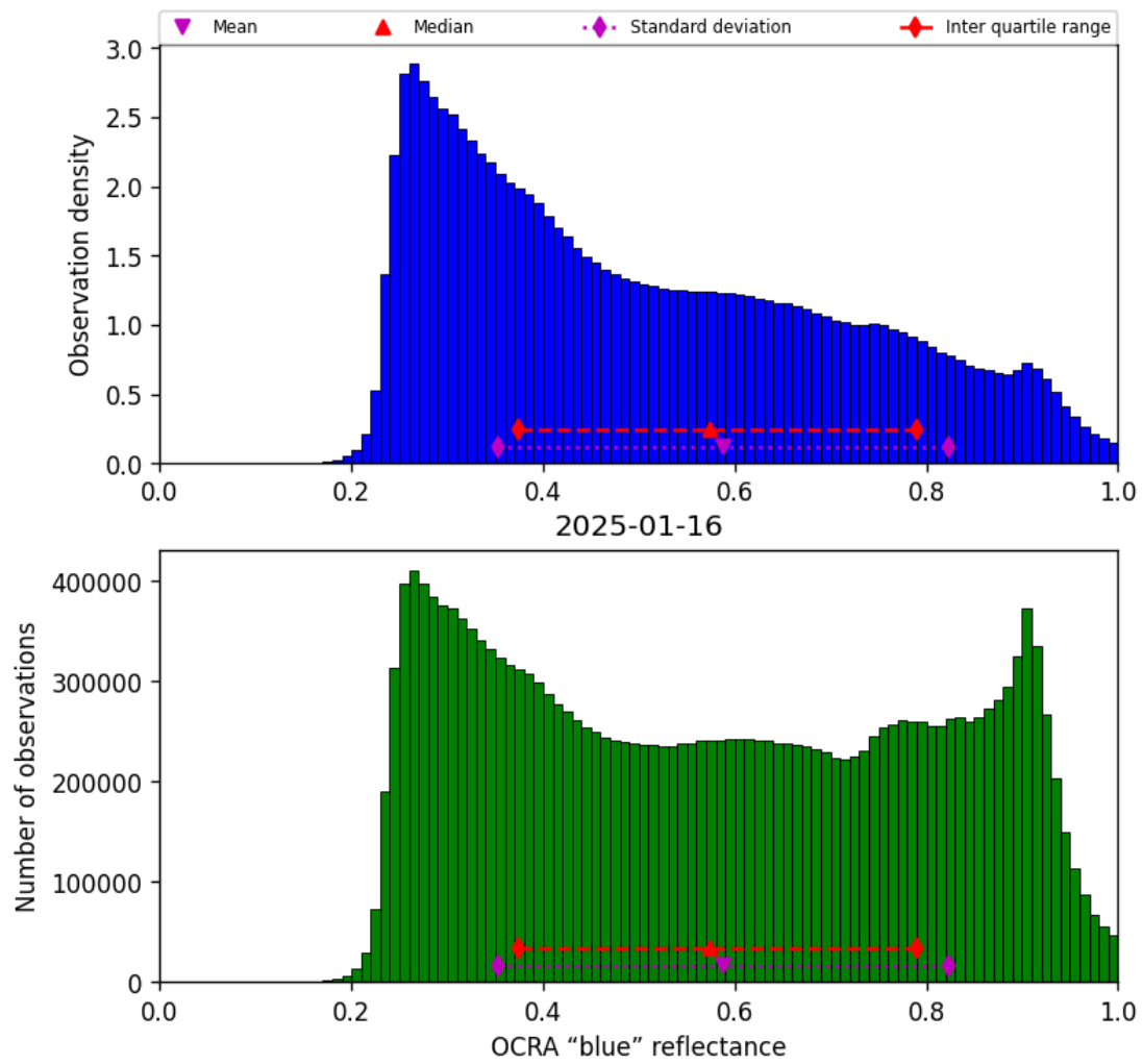
Figure 49: Histogram of “OCRA “blue” reflectance” for 2025-01-16 to 2025-01-17
