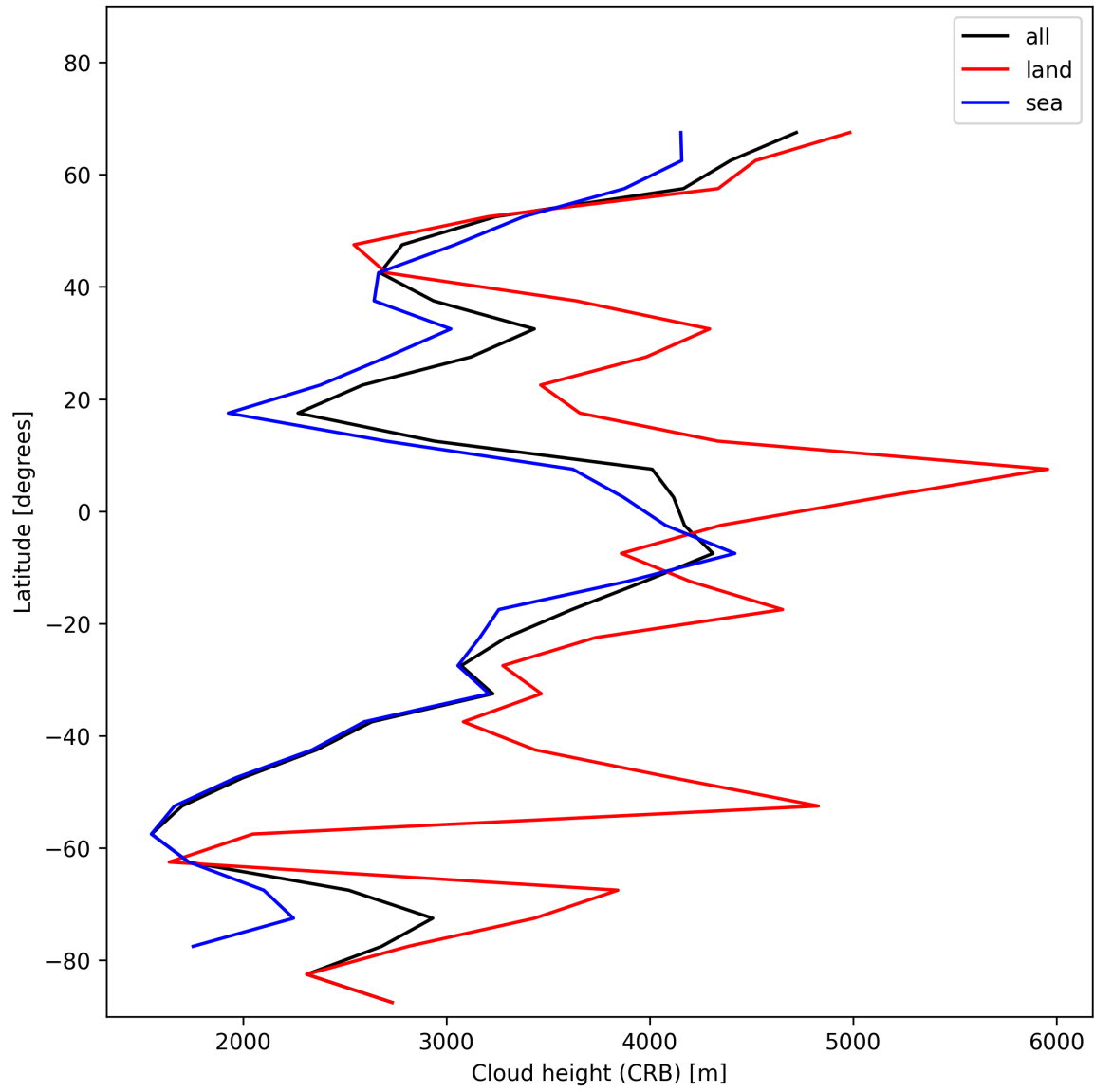
Figure 25: Zonal average of “Cloud height (CRB)” for 2025-01-16 to 2025-01-17.
