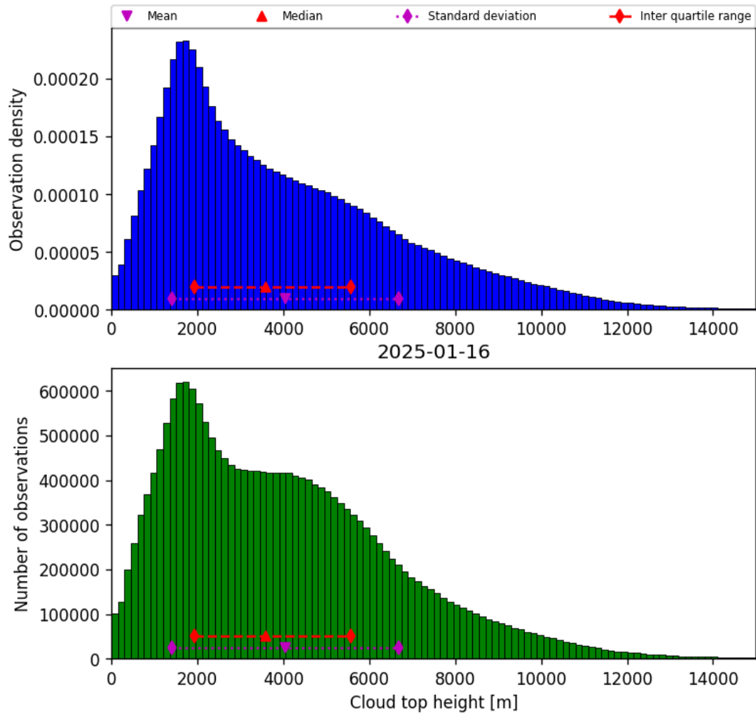
Figure 38: Histogram of “Cloud top height” for 2025-01-16 to 2025-01-17
