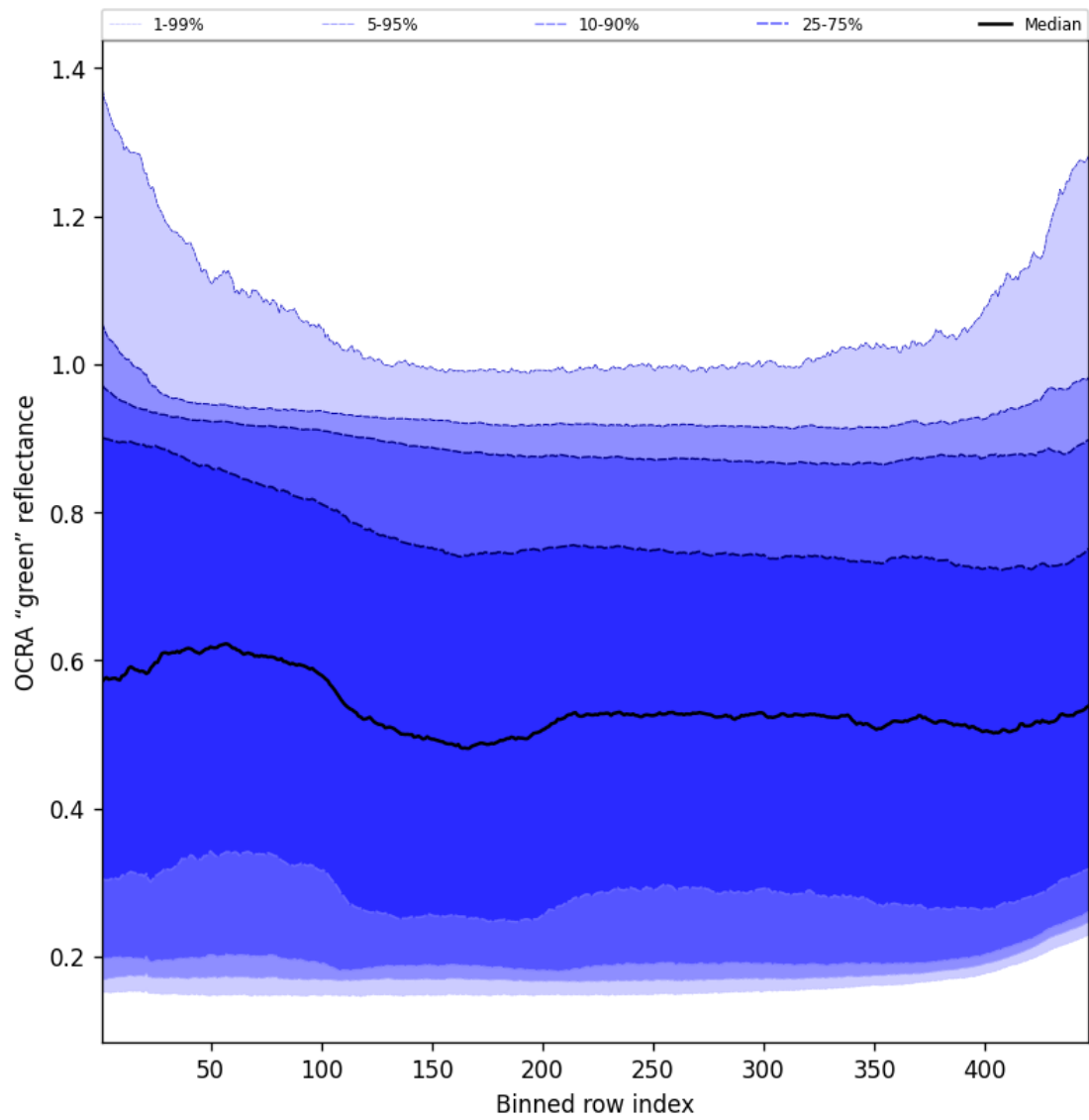
Figure 66: Along track statistics of “OCRA “green” reflectance” for 2025-01-16 to 2025-01-17
