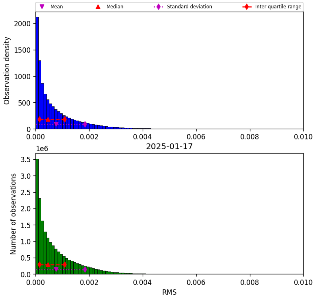
Figure 45: Histogram of “RMS” for 2025-01-17 to 2025-01-18
