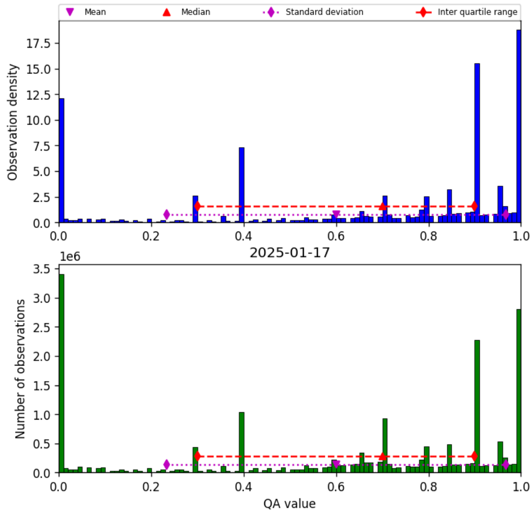
Figure 36: Histogram of “QA value” for 2025-01-17 to 2025-01-18
