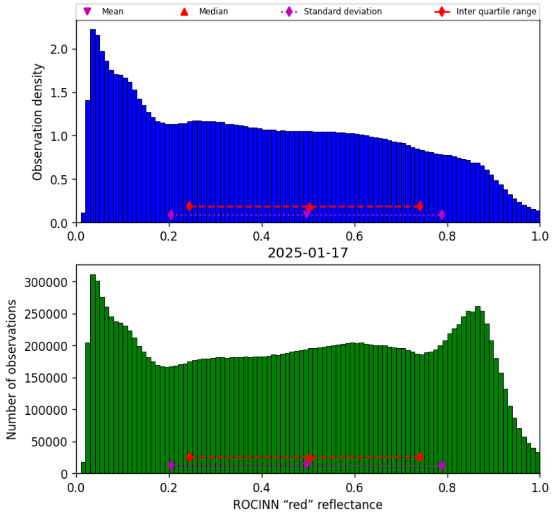
Figure 51: Histogram of “ROCINN “red” reflectance” for 2025-01-17 to 2025-01-18
