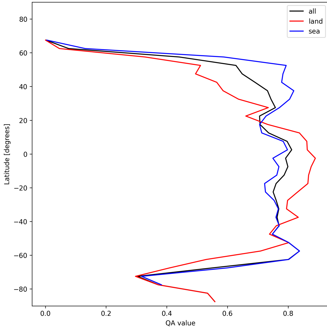
Figure 20: Zonal average of “QA value” for 2025-01-17 to 2025-01-18.
