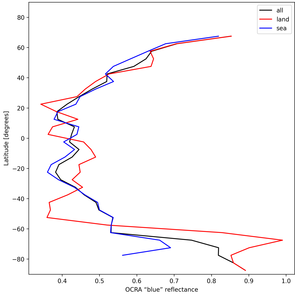
Figure 33: Zonal average of “OCRA “blue” reflectance” for 2025-01-17 to 2025-01-18.
