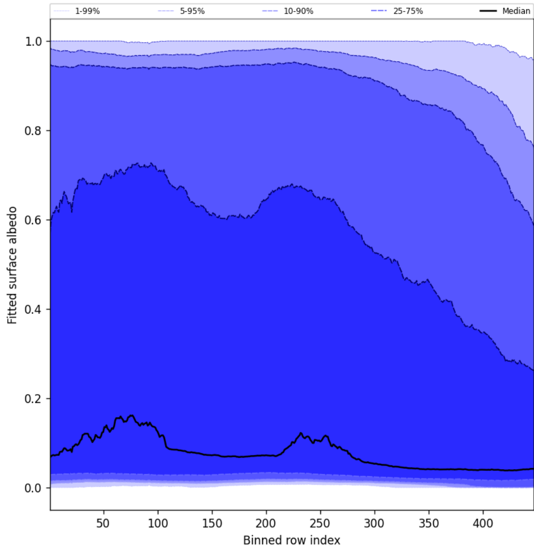
Figure 59: Along track statistics of “Fitted surface albedo” for 2025-01-17 to 2025-01-18
