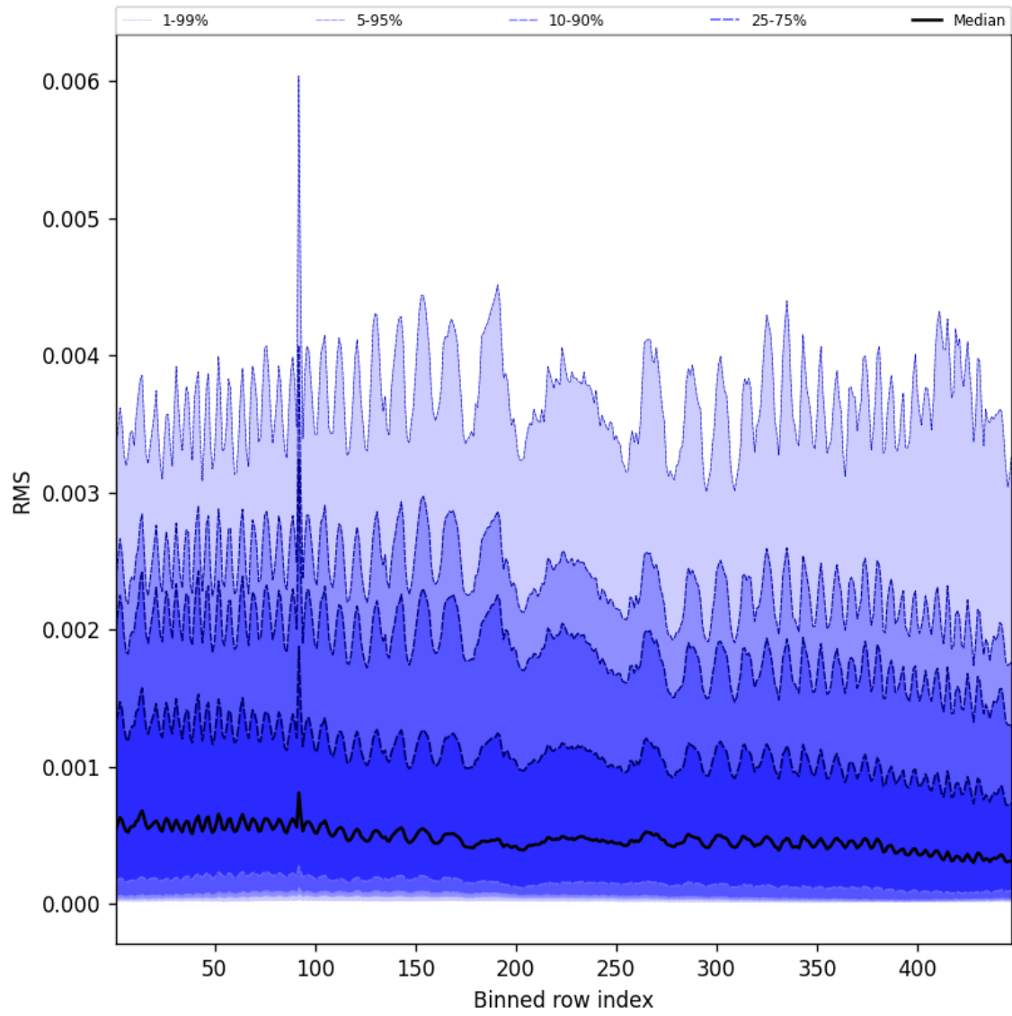
Figure 61: Along track statistics of “RMS” for 2025-01-17 to 2025-01-18
