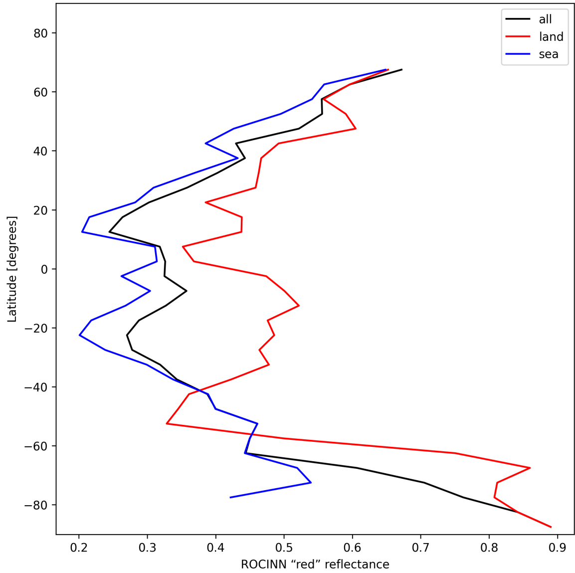
Figure 35: Zonal average of “ROCINN “red” reflectance” for 2025-01-17 to 2025-01-18.
