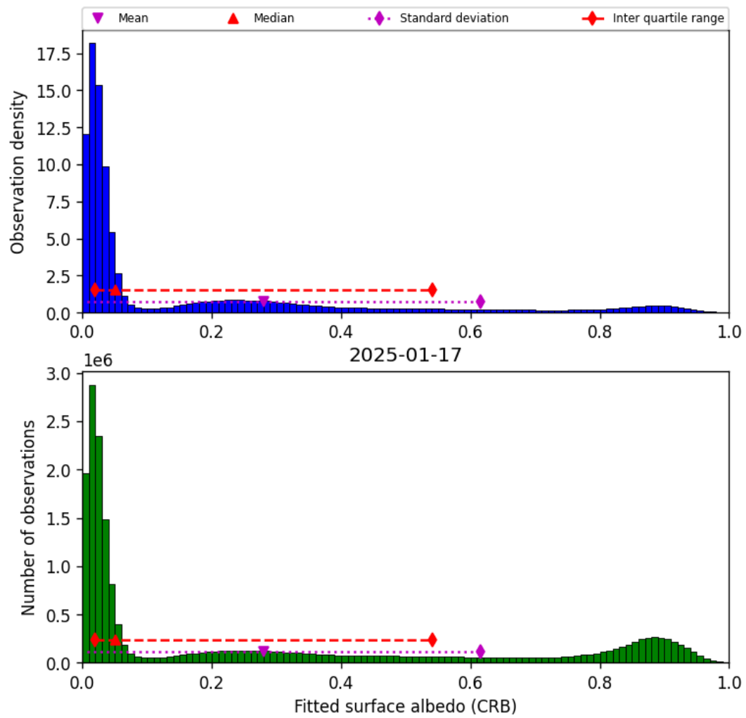
Figure 44: Histogram of “Fitted surface albedo (CRB)” for 2025-01-17 to 2025-01-18
