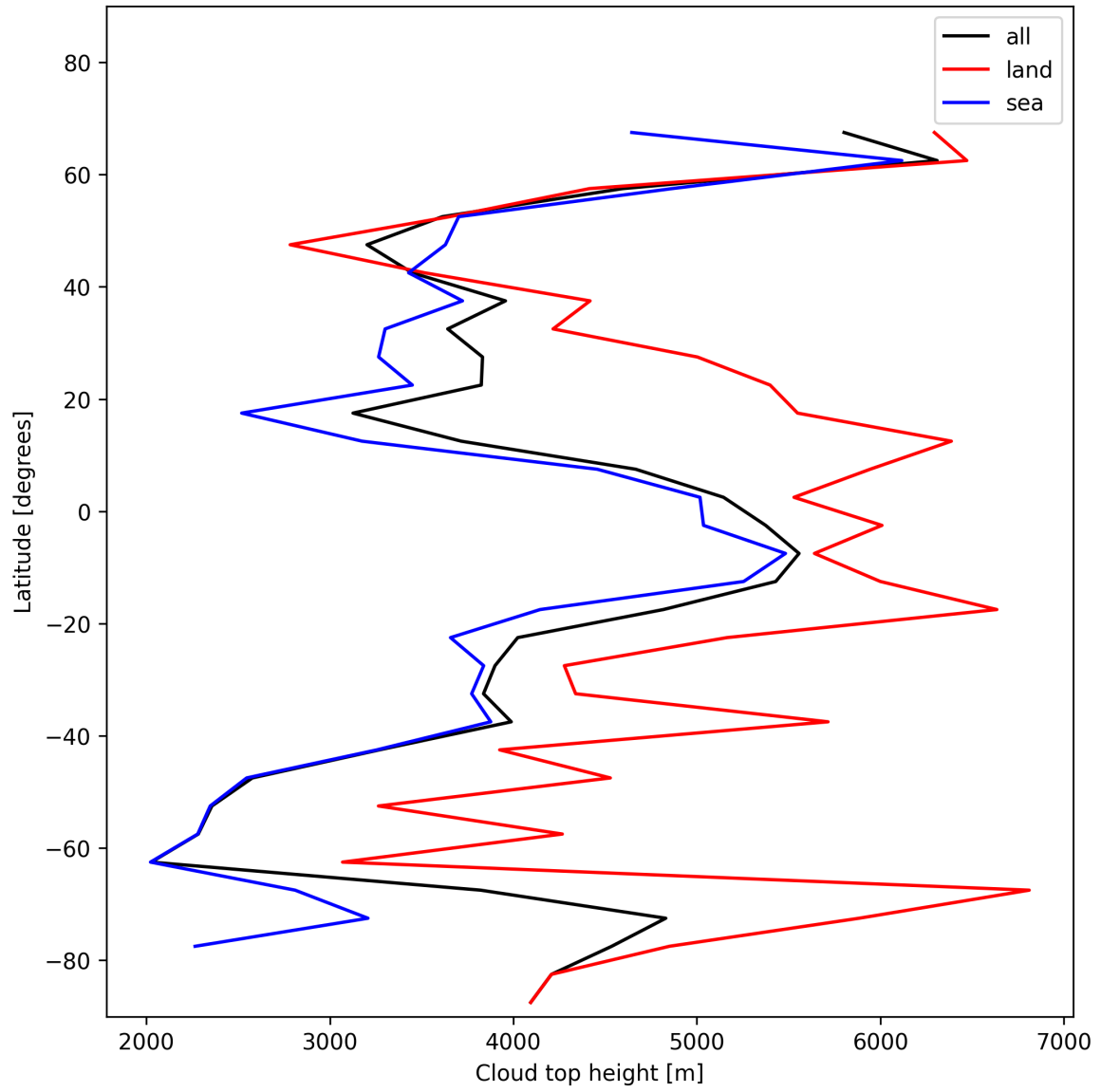
Figure 22: Zonal average of “Cloud top height” for 2025-01-17 to 2025-01-18.
