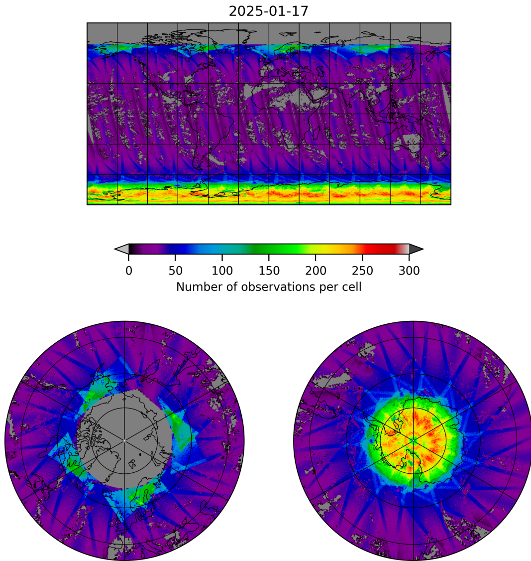
Figure 19: Map of the number of observations for 2025-01-17 to 2025-01-18
