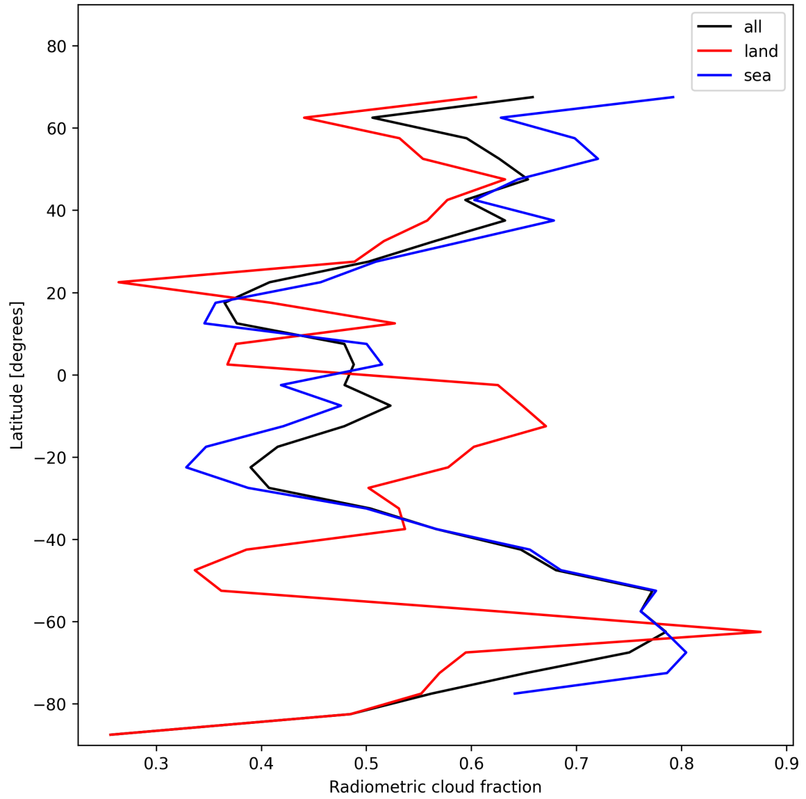
Figure 21: Zonal average of “Radiometric cloud fraction” for 2025-01-17 to 2025-01-18.
