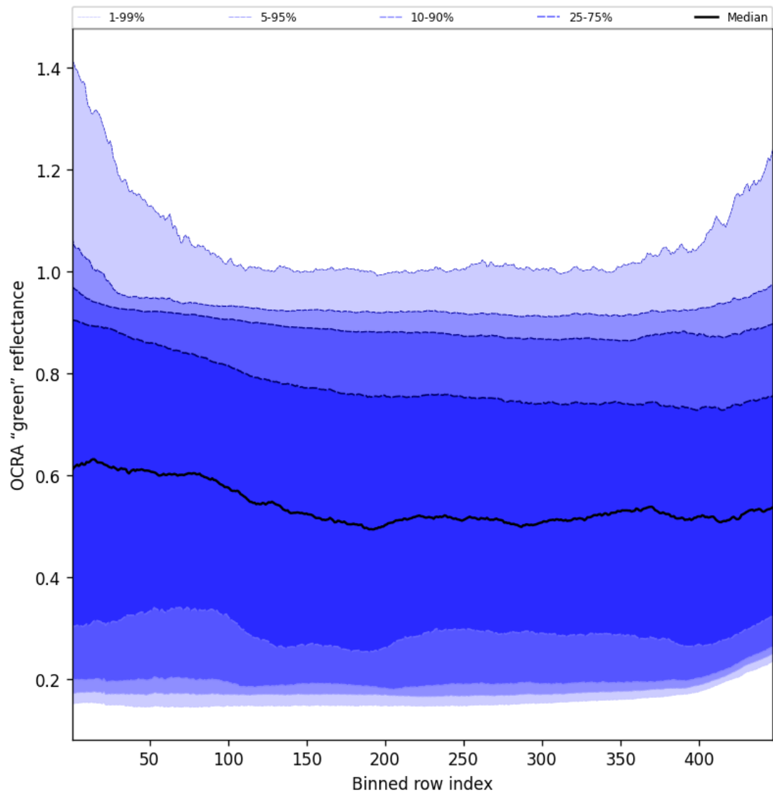
Figure 66: Along track statistics of “OCRA “green” reflectance” for 2025-01-17 to 2025-01-18
