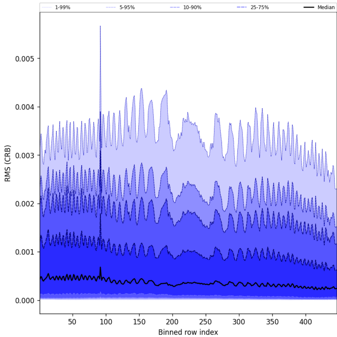
Figure 62: Along track statistics of “RMS (CRB)” for 2025-01-17 to 2025-01-18
