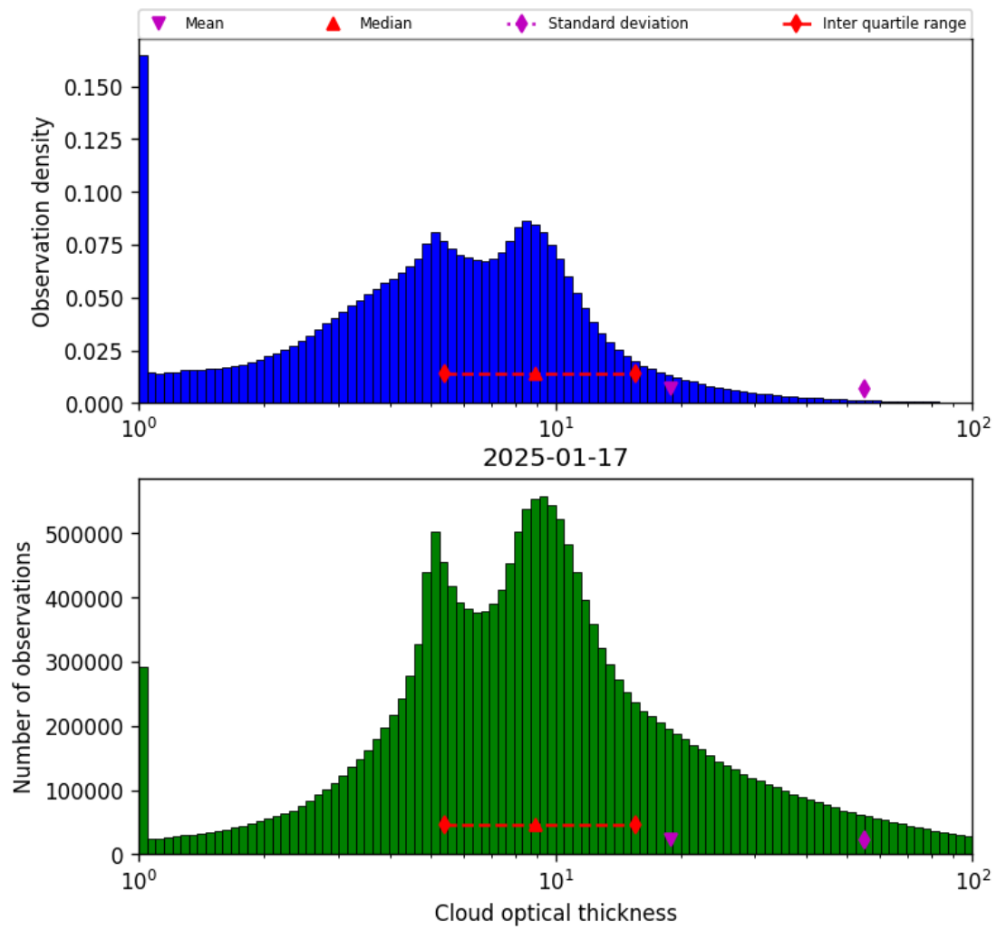
Figure 39: Histogram of “Cloud optical thickness” for 2025-01-17 to 2025-01-18
