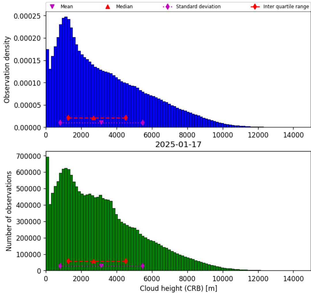
Figure 41: Histogram of “Cloud height (CRB)” for 2025-01-17 to 2025-01-18
