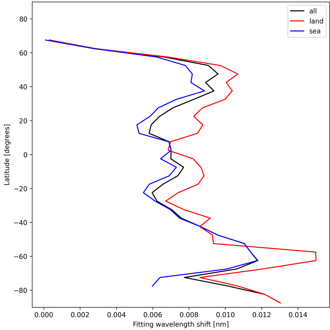
Figure 31: Zonal average of “Fitting wavelength shift” for 2025-01-17 to 2025-01-18.
