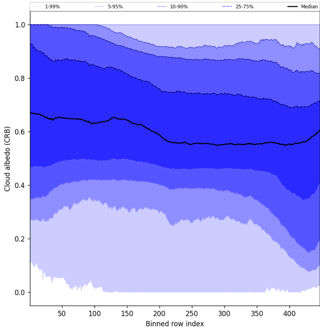
Figure 58: Along track statistics of “Cloud albedo (CRB)” for 2025-01-17 to 2025-01-18
