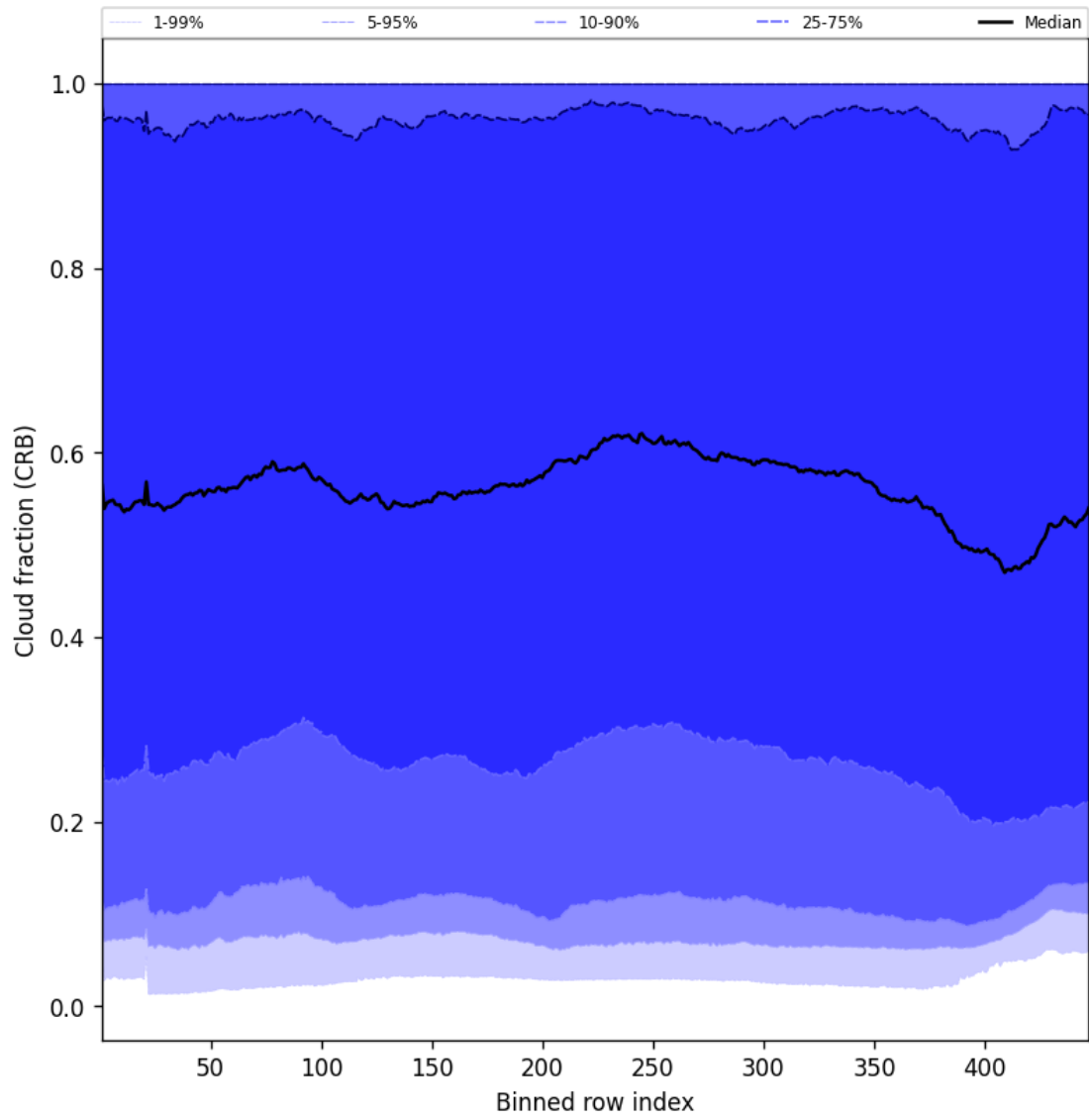
Figure 56: Along track statistics of “Cloud fraction (CRB)” for 2025-01-17 to 2025-01-18
