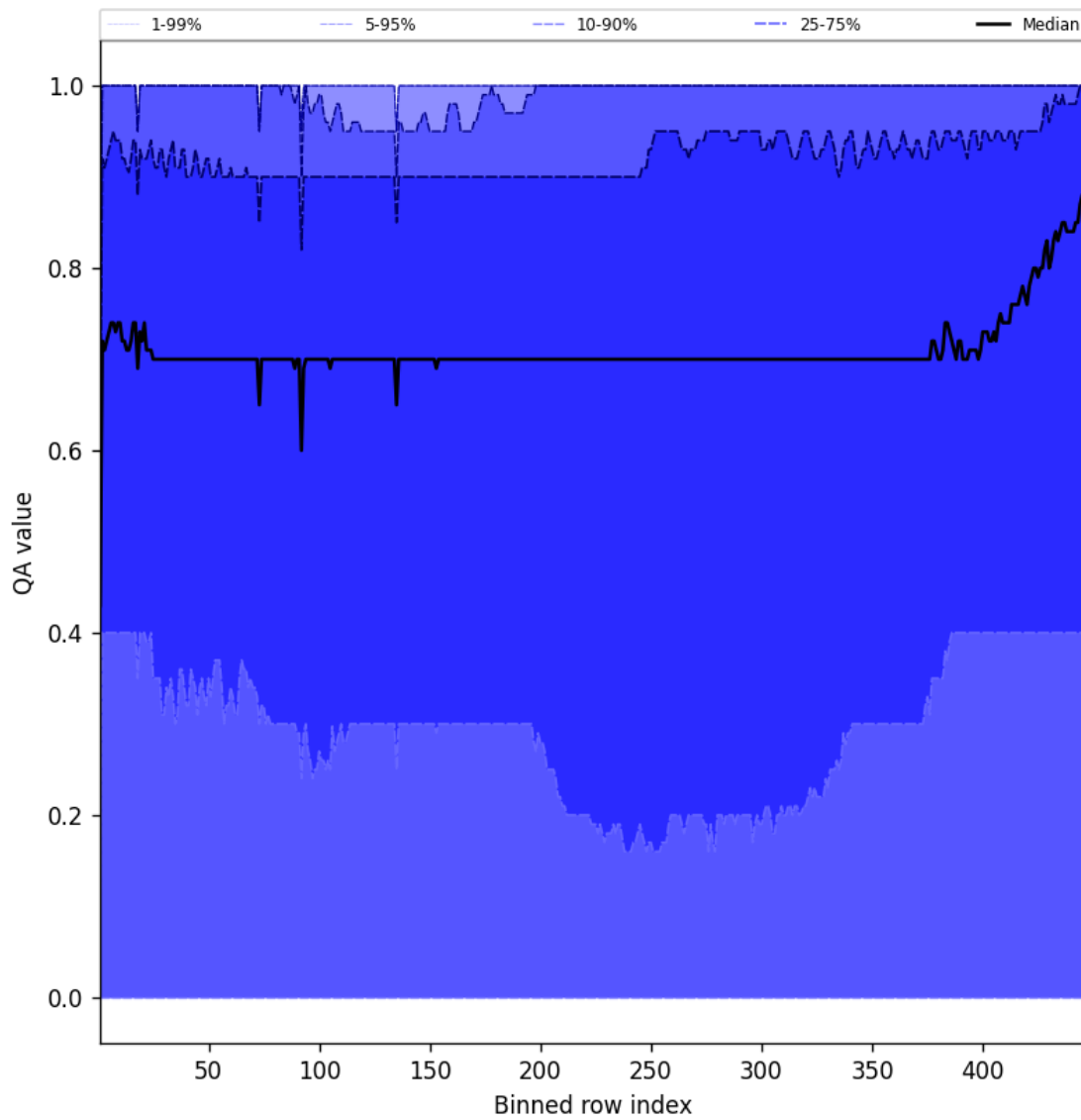
Figure 52: Along track statistics of “QA value” for 2025-01-17 to 2025-01-18
