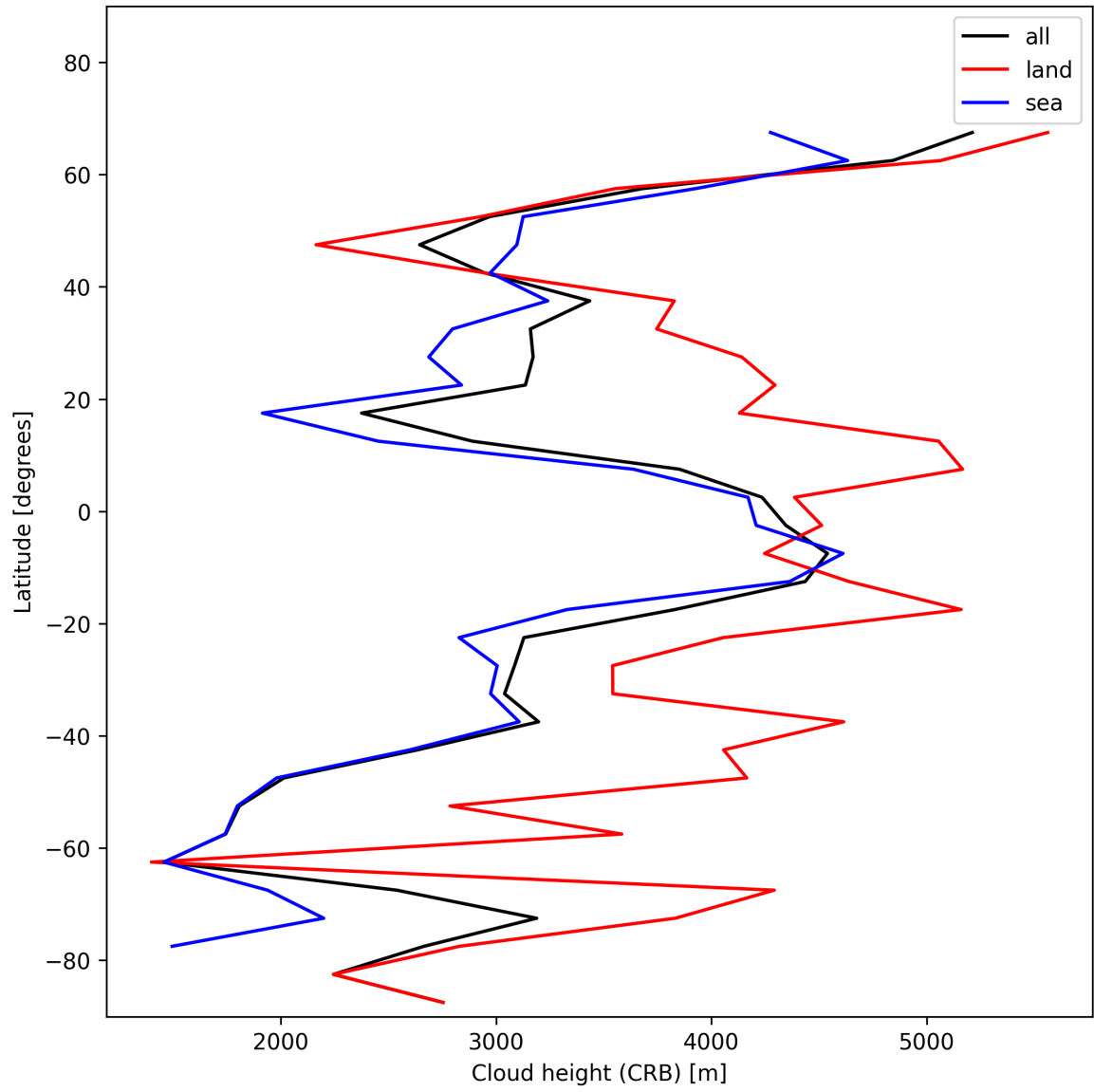
Figure 25: Zonal average of “Cloud height (CRB)” for 2025-01-17 to 2025-01-18.
