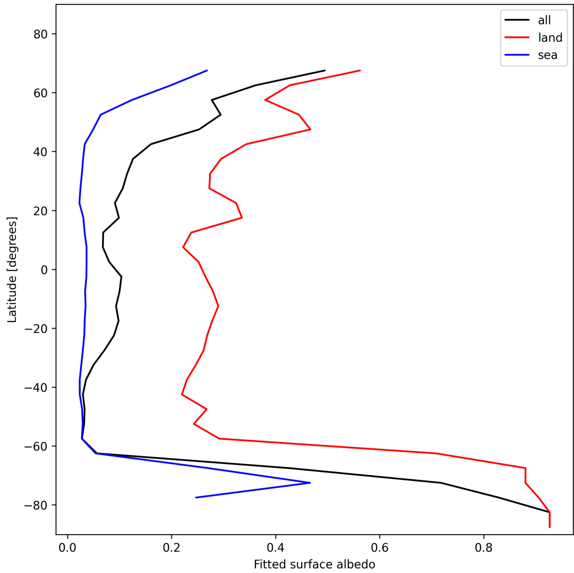
Figure 27: Zonal average of “Fitted surface albedo” for 2025-01-17 to 2025-01-18.
