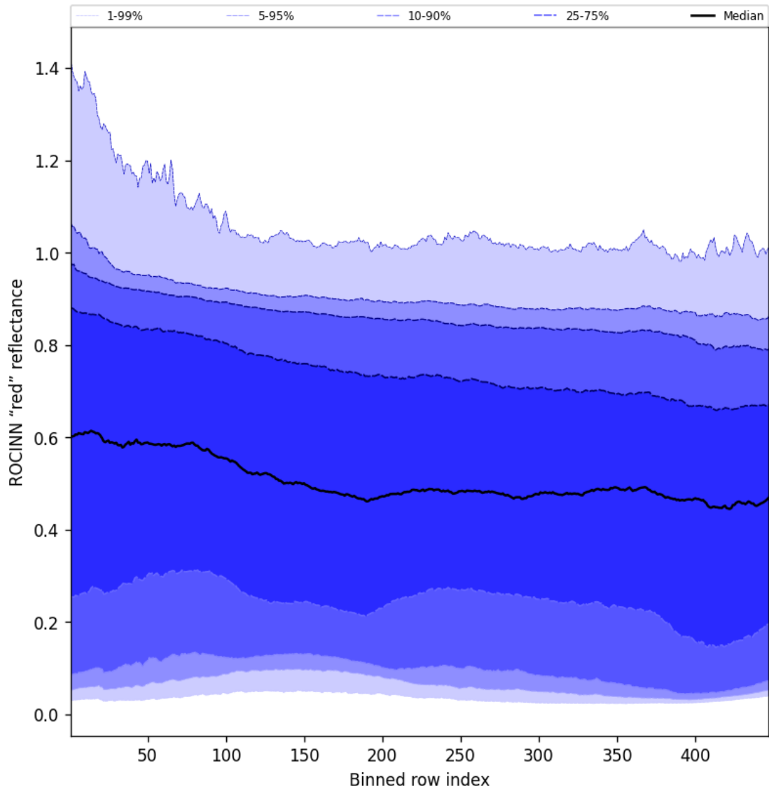
Figure 67: Along track statistics of “ROCINN “red” reflectance” for 2025-01-17 to 2025-01-18
