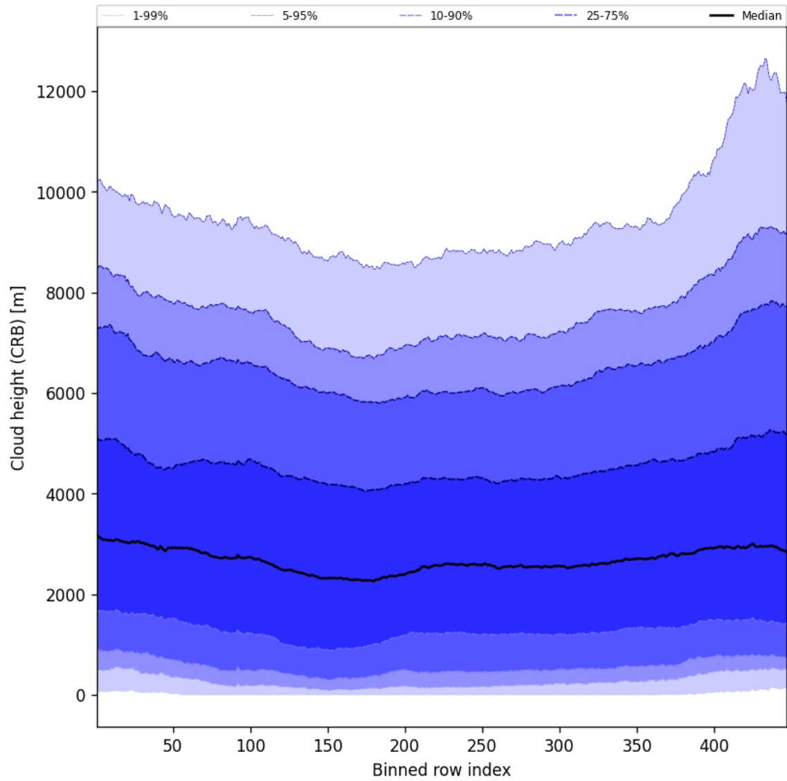
Figure 57: Along track statistics of “Cloud height (CRB)” for 2025-01-17 to 2025-01-18
