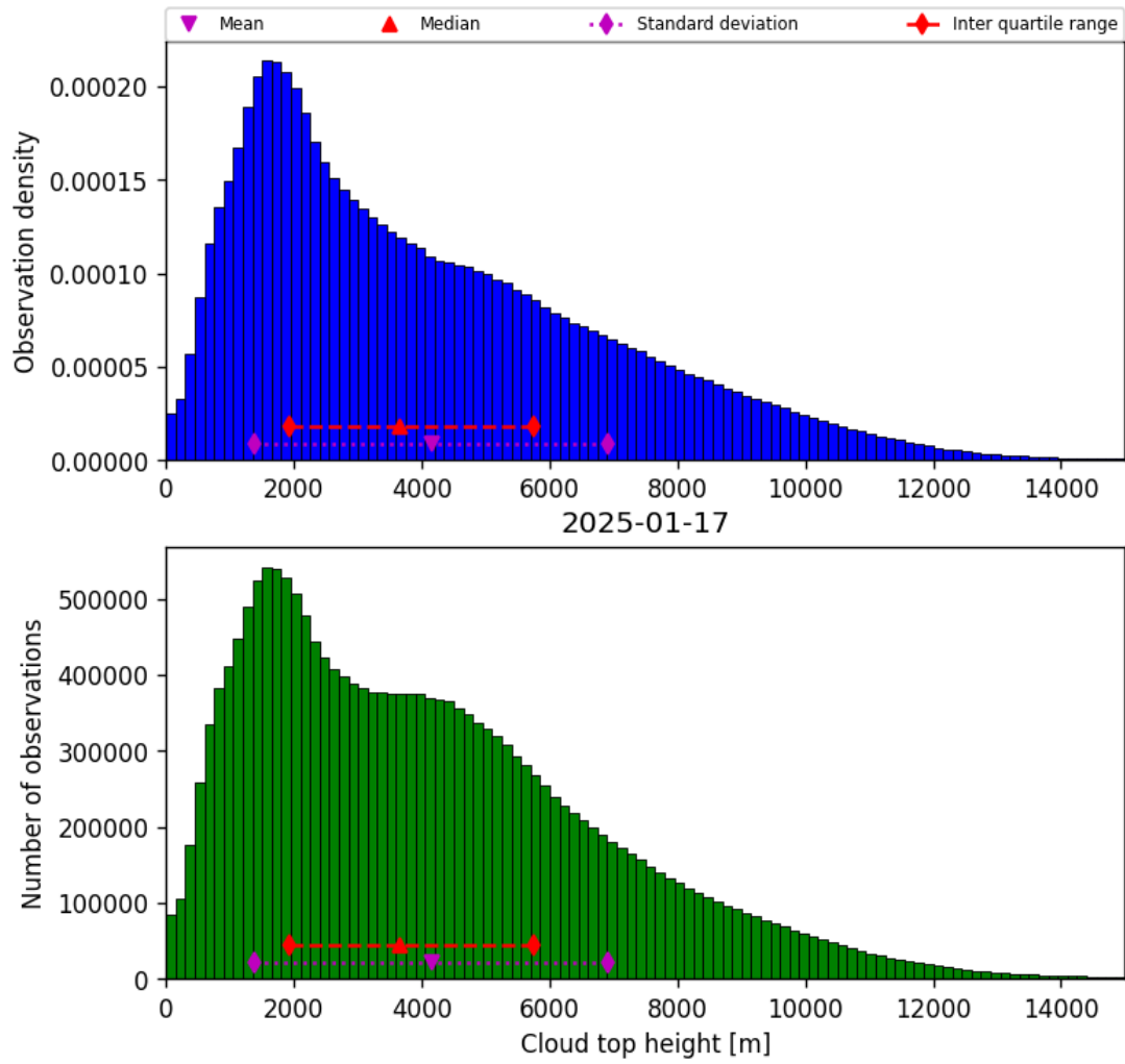
Figure 38: Histogram of “Cloud top height” for 2025-01-17 to 2025-01-18
