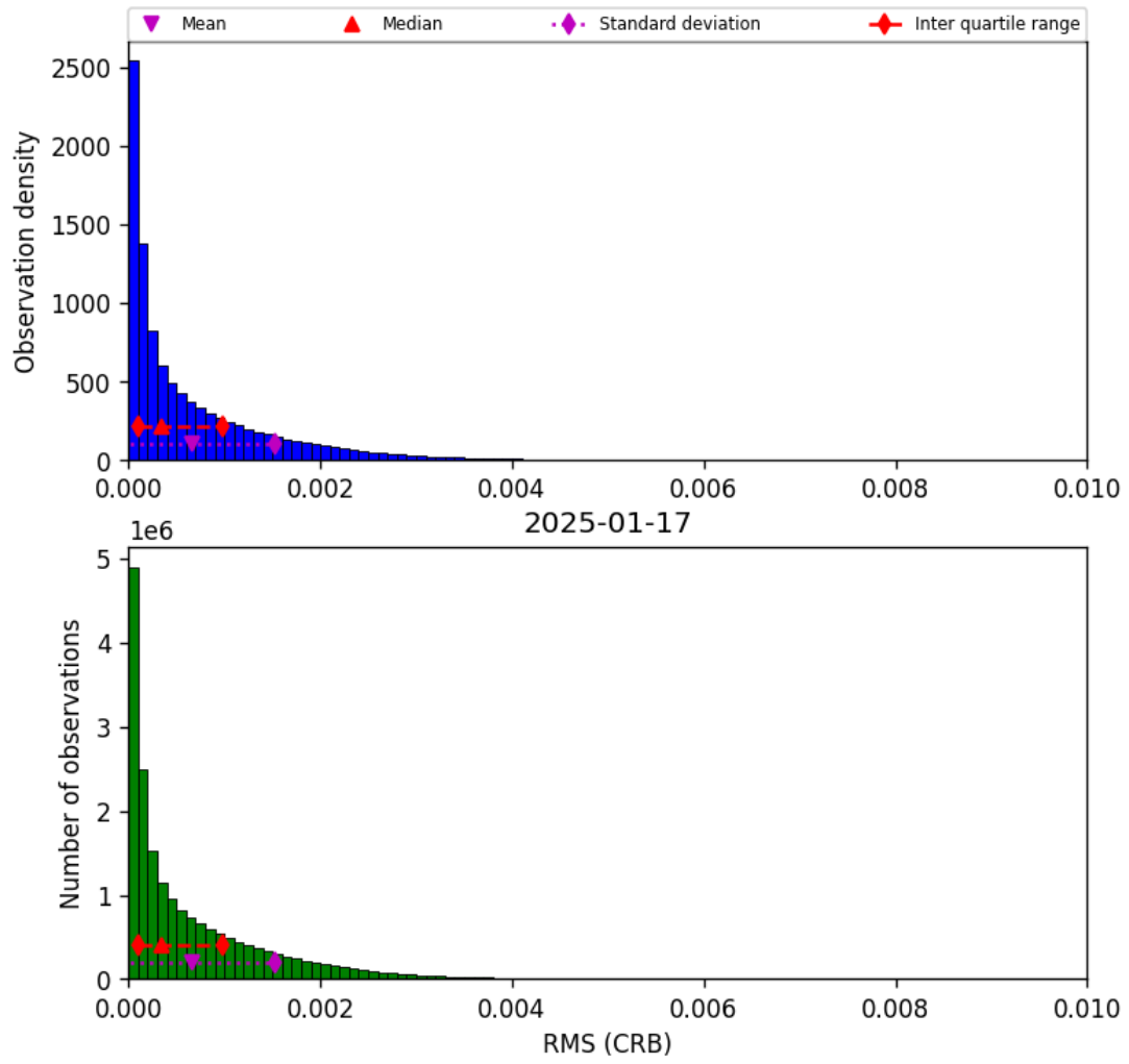
Figure 46: Histogram of “RMS (CRB)” for 2025-01-17 to 2025-01-18
