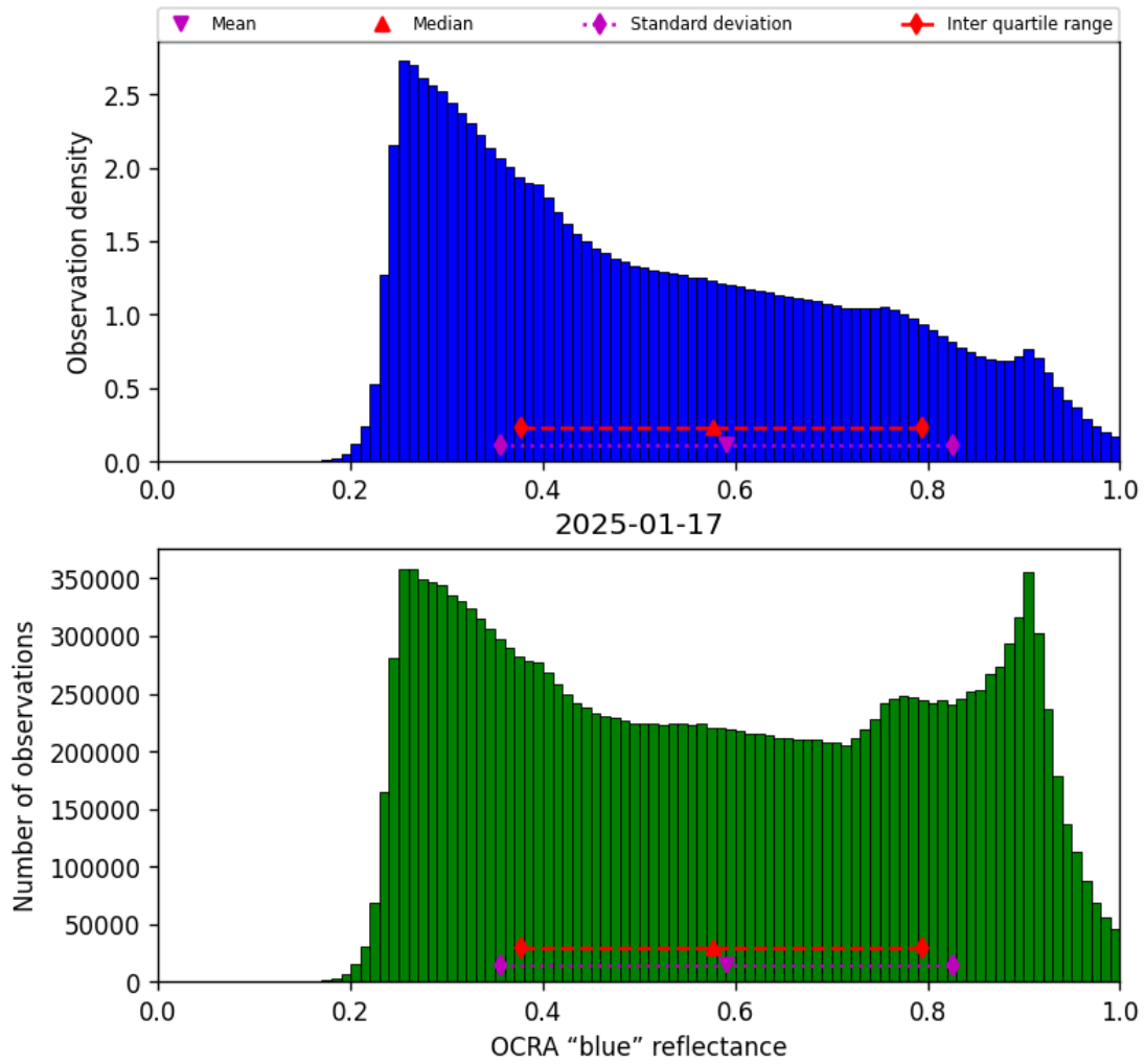
Figure 49: Histogram of “OCRA “blue” reflectance” for 2025-01-17 to 2025-01-18
