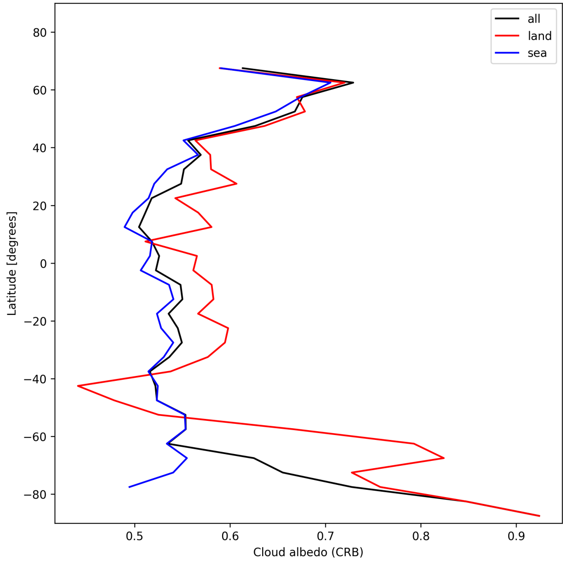
Figure 26: Zonal average of “Cloud albedo (CRB)” for 2025-01-17 to 2025-01-18.
