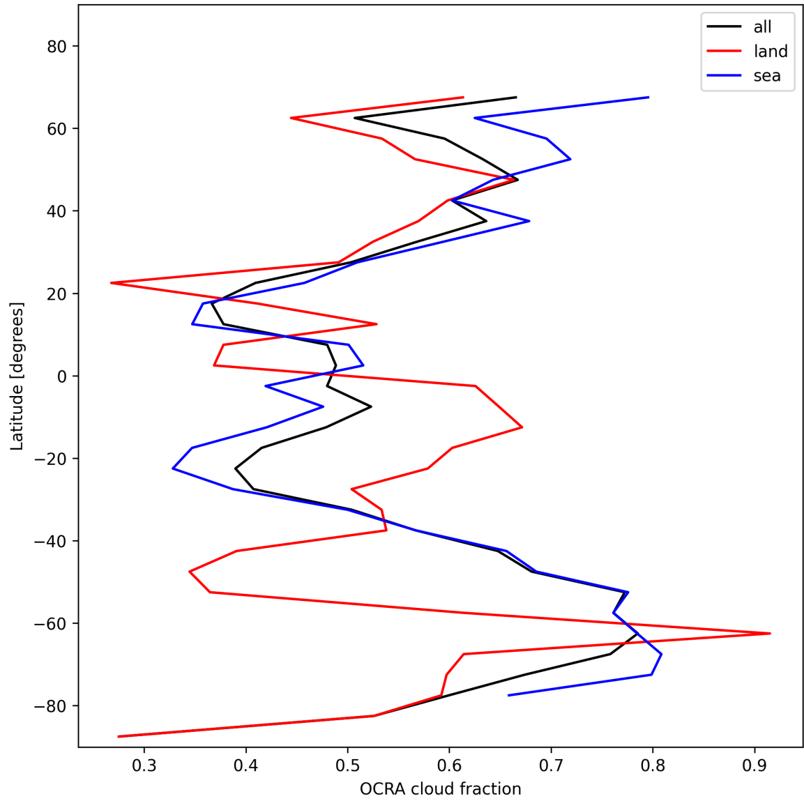
Figure 32: Zonal average of “OCRA cloud fraction” for 2025-01-17 to 2025-01-18.
