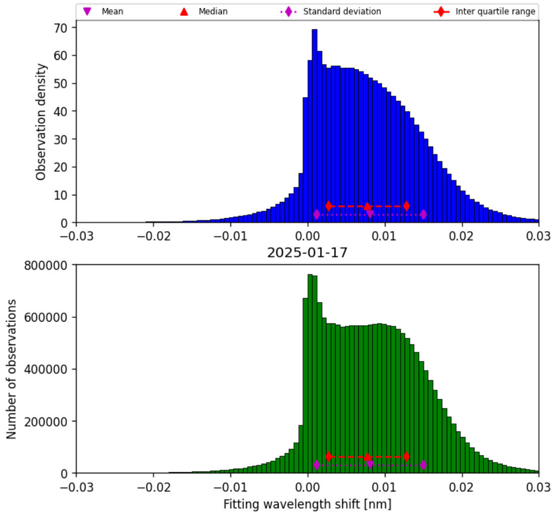
Figure 47: Histogram of “Fitting wavelength shift” for 2025-01-17 to 2025-01-18
