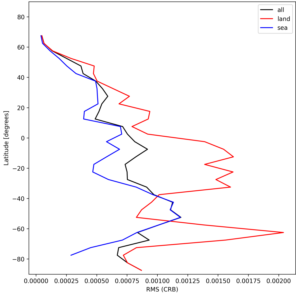
Figure 30: Zonal average of “RMS (CRB)” for 2025-01-17 to 2025-01-18.
