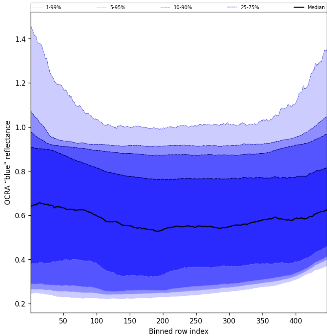
Figure 65: Along track statistics of “OCRA “blue” reflectance” for 2025-01-17 to 2025-01-18
