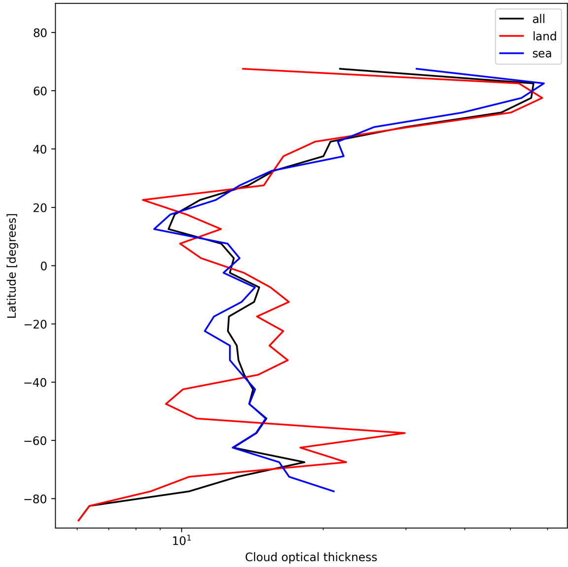
Figure 23: Zonal average of “Cloud optical thickness” for 2025-01-17 to 2025-01-18.
