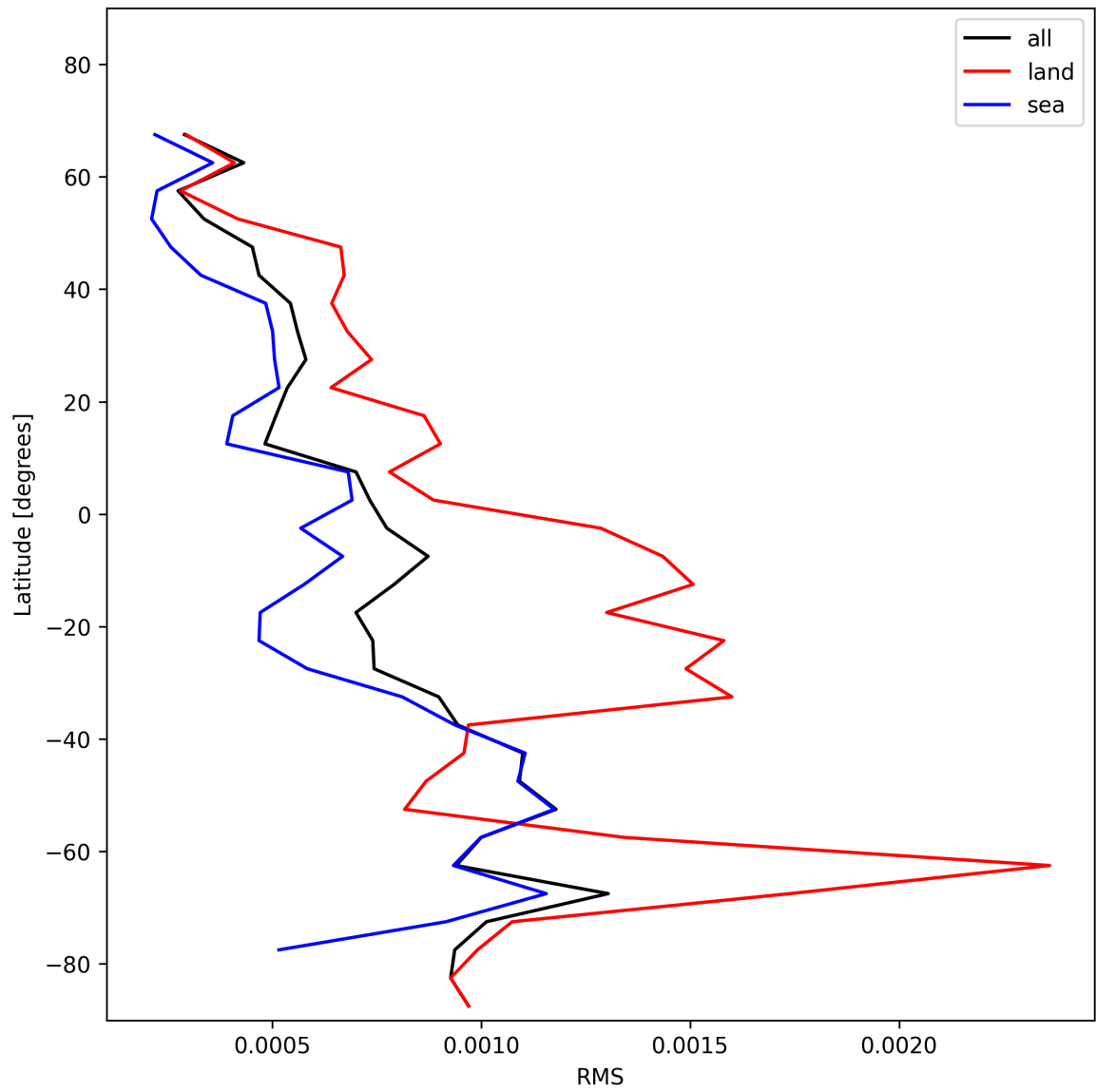
Figure 29: Zonal average of “RMS” for 2025-01-17 to 2025-01-18.
