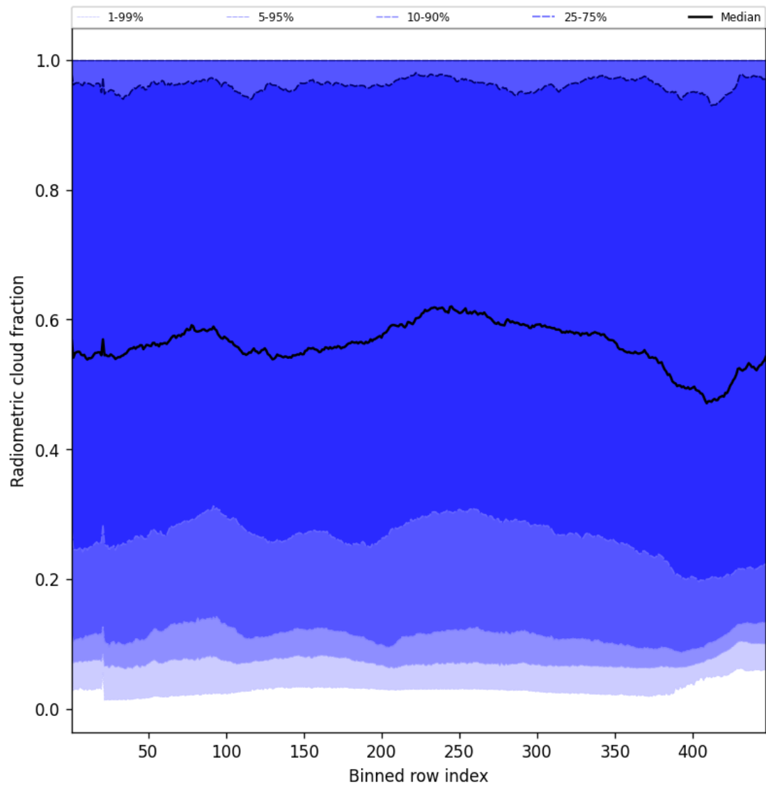
Figure 53: Along track statistics of “Radiometric cloud fraction” for 2025-01-17 to 2025-01-18
