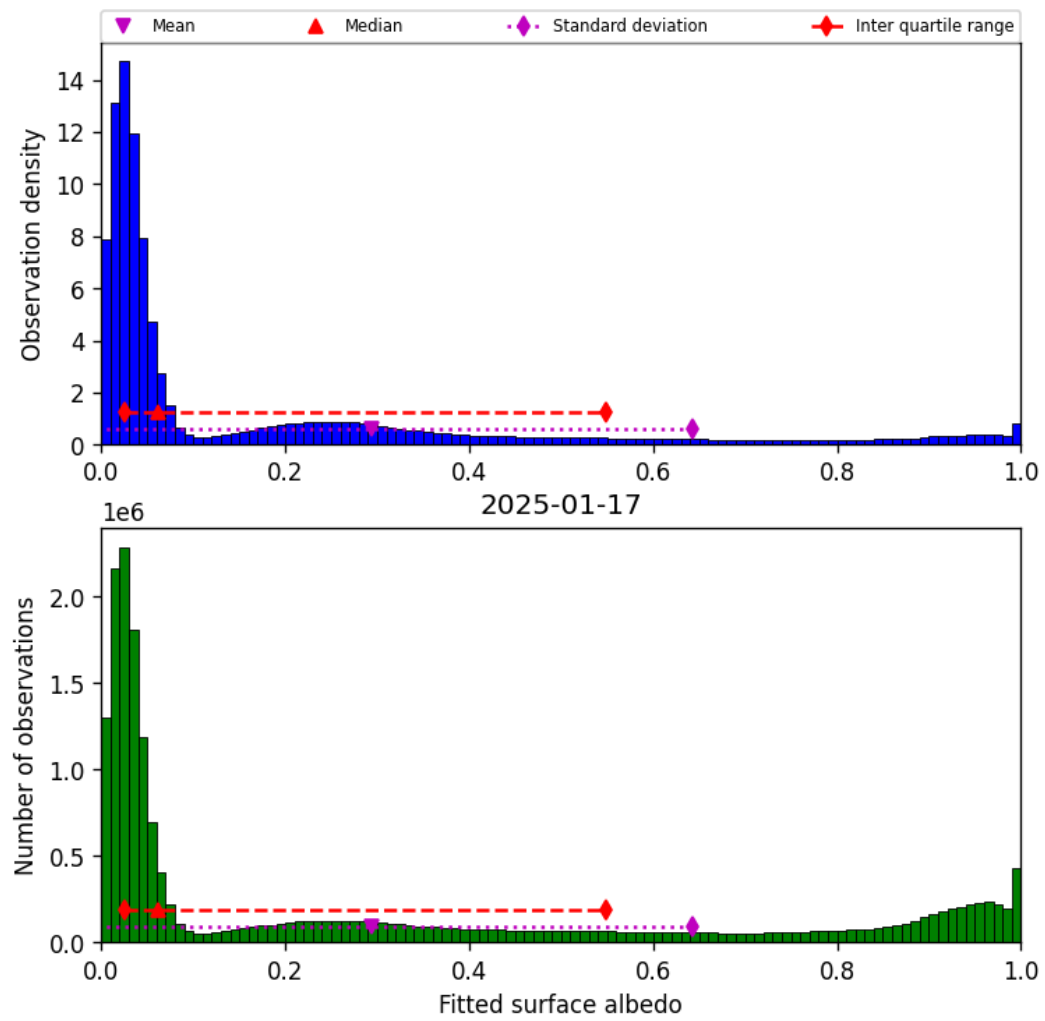
Figure 43: Histogram of “Fitted surface albedo” for 2025-01-17 to 2025-01-18
