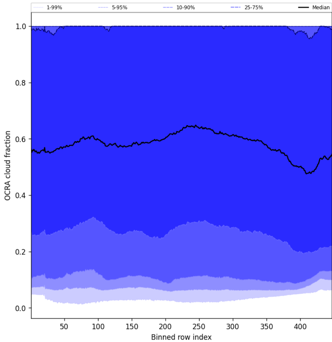
Figure 64: Along track statistics of “OCRA cloud fraction” for 2025-01-17 to 2025-01-18
