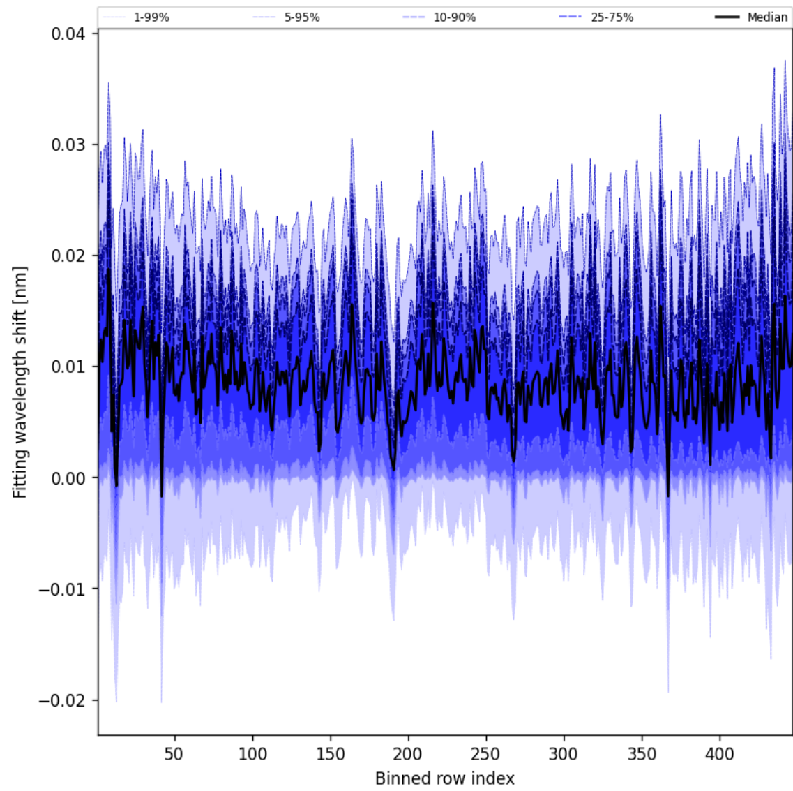
Figure 63: Along track statistics of “Fitting wavelength shift” for 2025-01-17 to 2025-01-18
