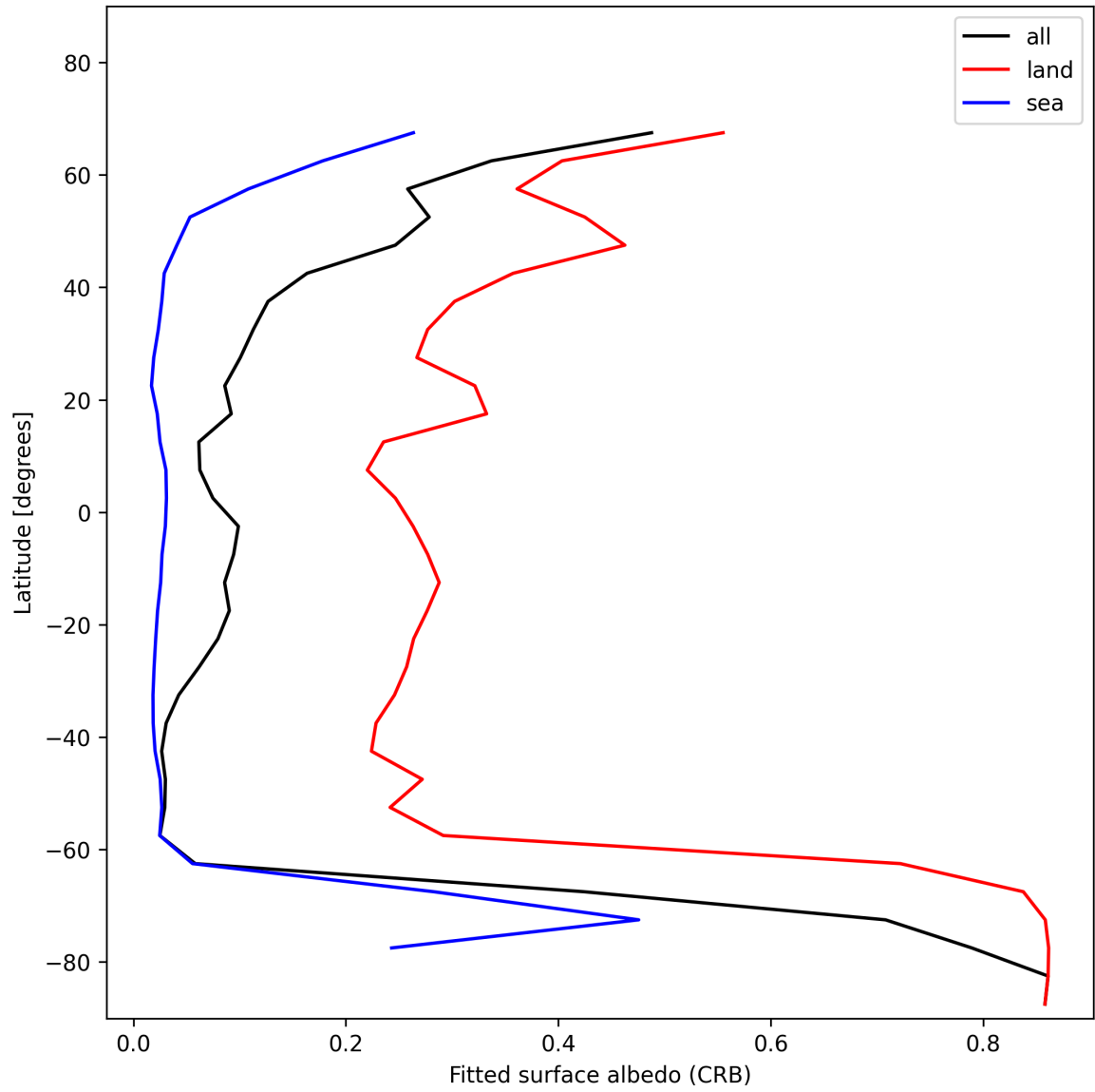
Figure 28: Zonal average of “Fitted surface albedo (CRB)” for 2025-01-17 to 2025-01-18.
