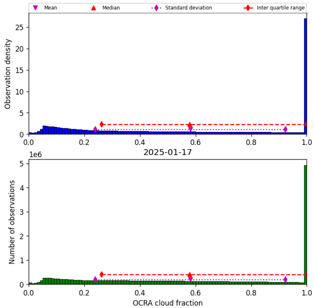
Figure 48: Histogram of “OCRA cloud fraction” for 2025-01-17 to 2025-01-18
