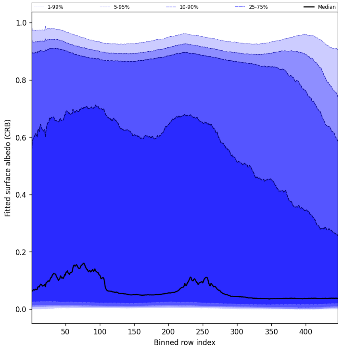
Figure 60: Along track statistics of “Fitted surface albedo (CRB)” for 2025-01-17 to 2025-01-18
