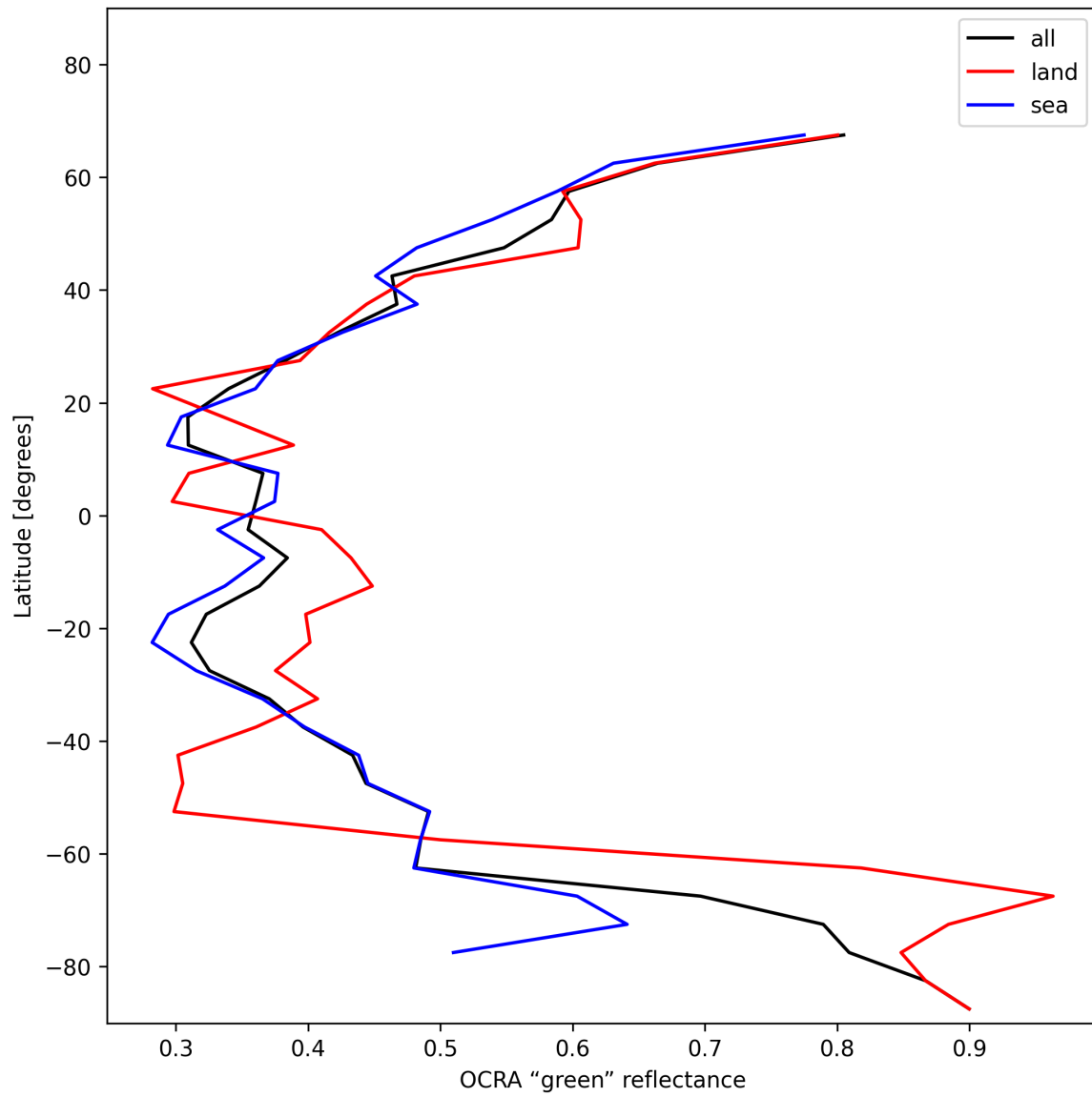
Figure 34: Zonal average of “OCRA “green” reflectance” for 2025-01-17 to 2025-01-18.
