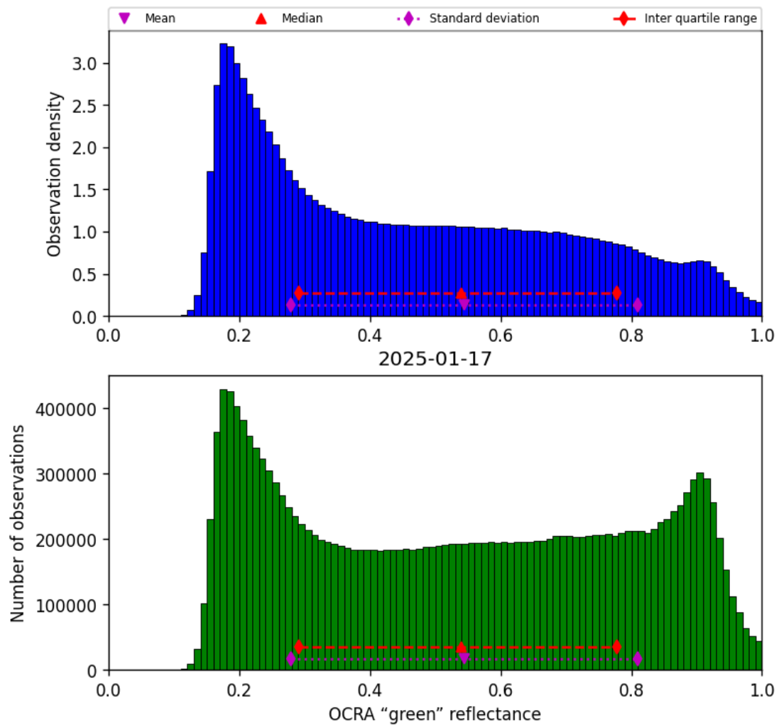
Figure 50: Histogram of “OCRA “green” reflectance” for 2025-01-17 to 2025-01-18
