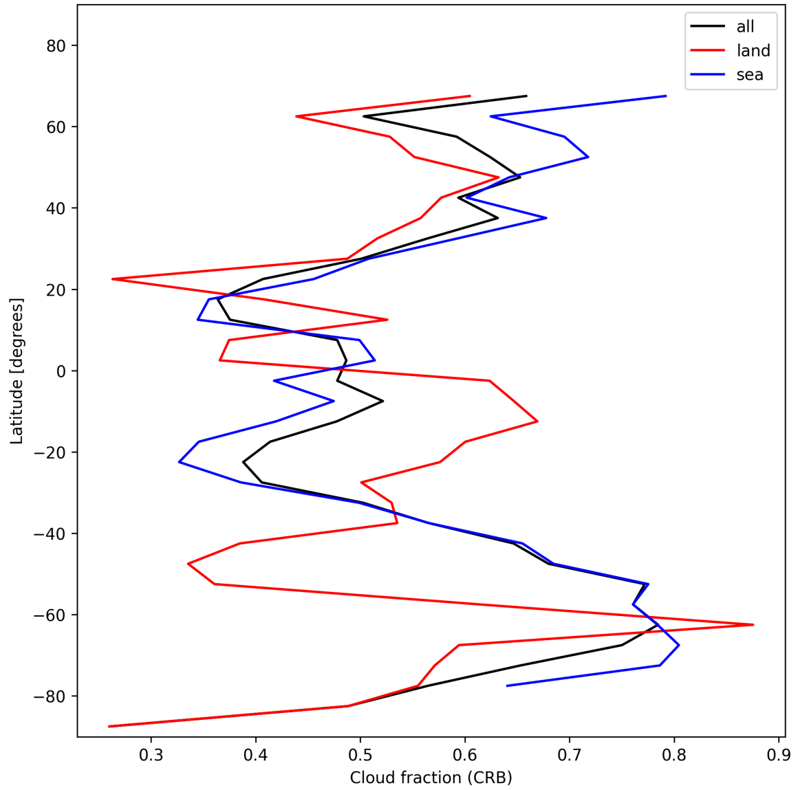
Figure 24: Zonal average of “Cloud fraction (CRB)” for 2025-01-17 to 2025-01-18.
