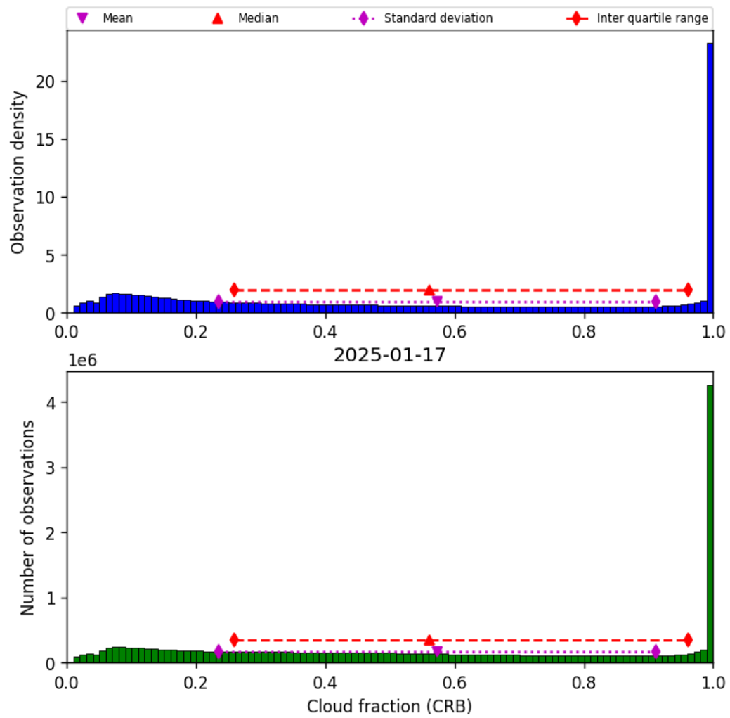
Figure 40: Histogram of “Cloud fraction (CRB)” for 2025-01-17 to 2025-01-18
