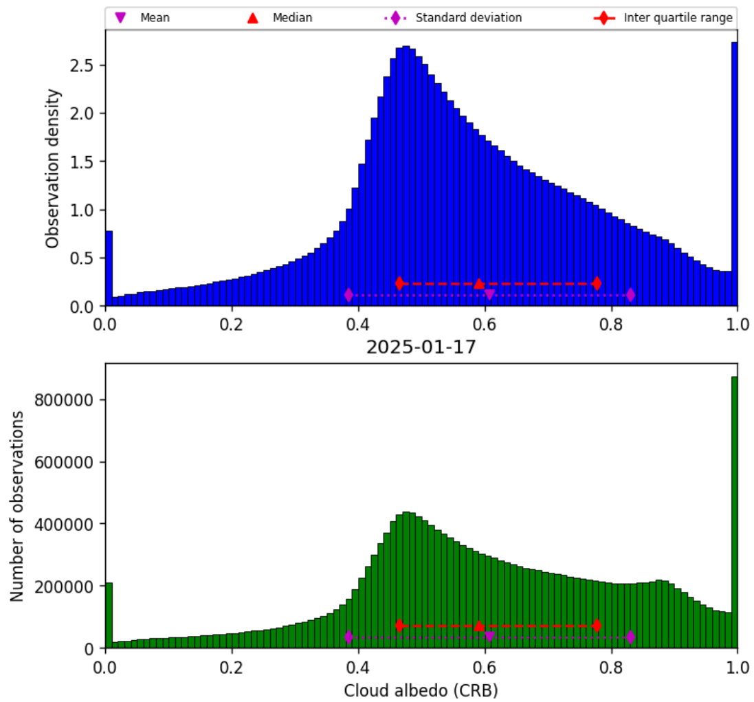
Figure 42: Histogram of “Cloud albedo (CRB)” for 2025-01-17 to 2025-01-18
