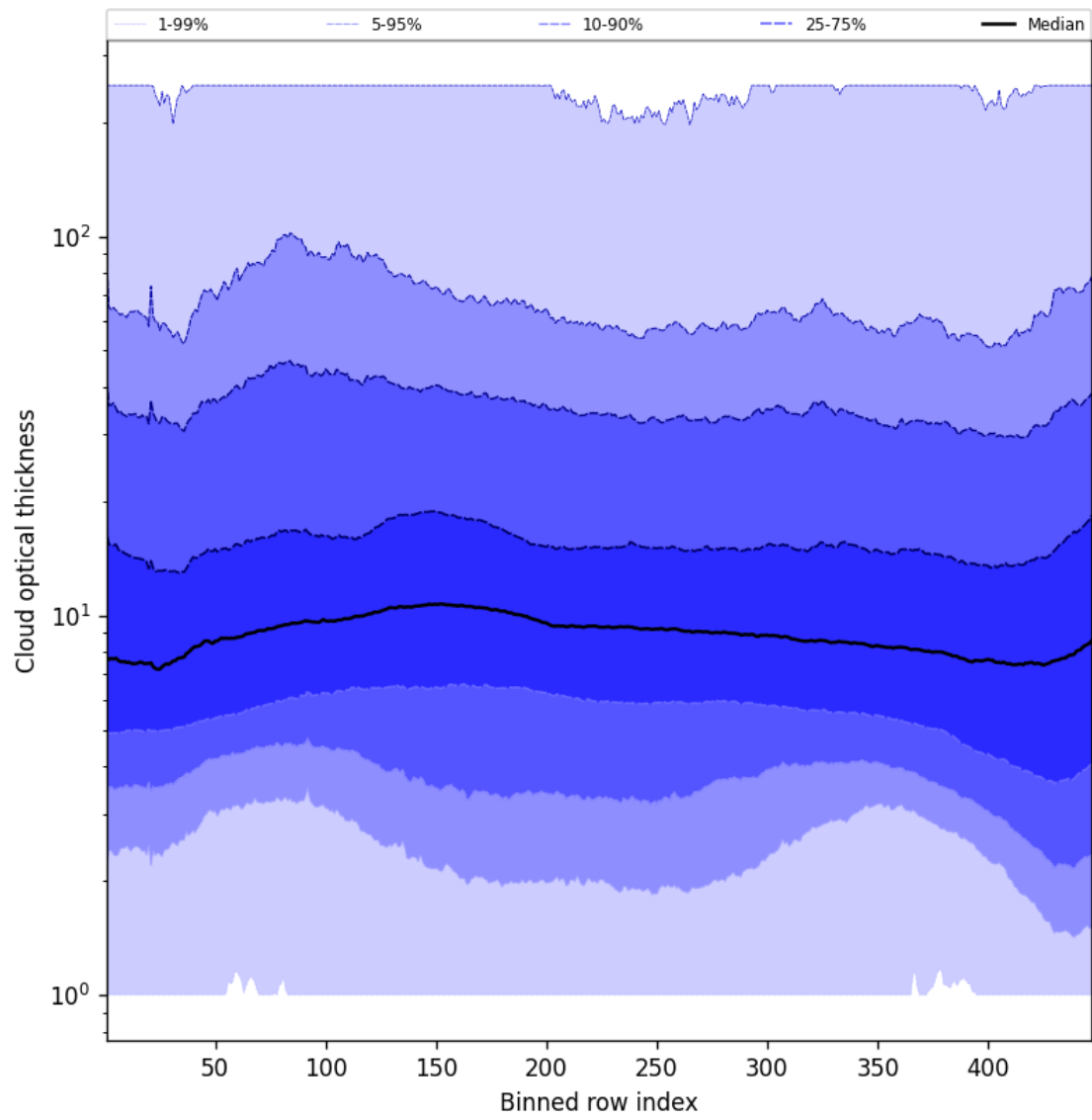
Figure 55: Along track statistics of “Cloud optical thickness” for 2025-01-17 to 2025-01-18
