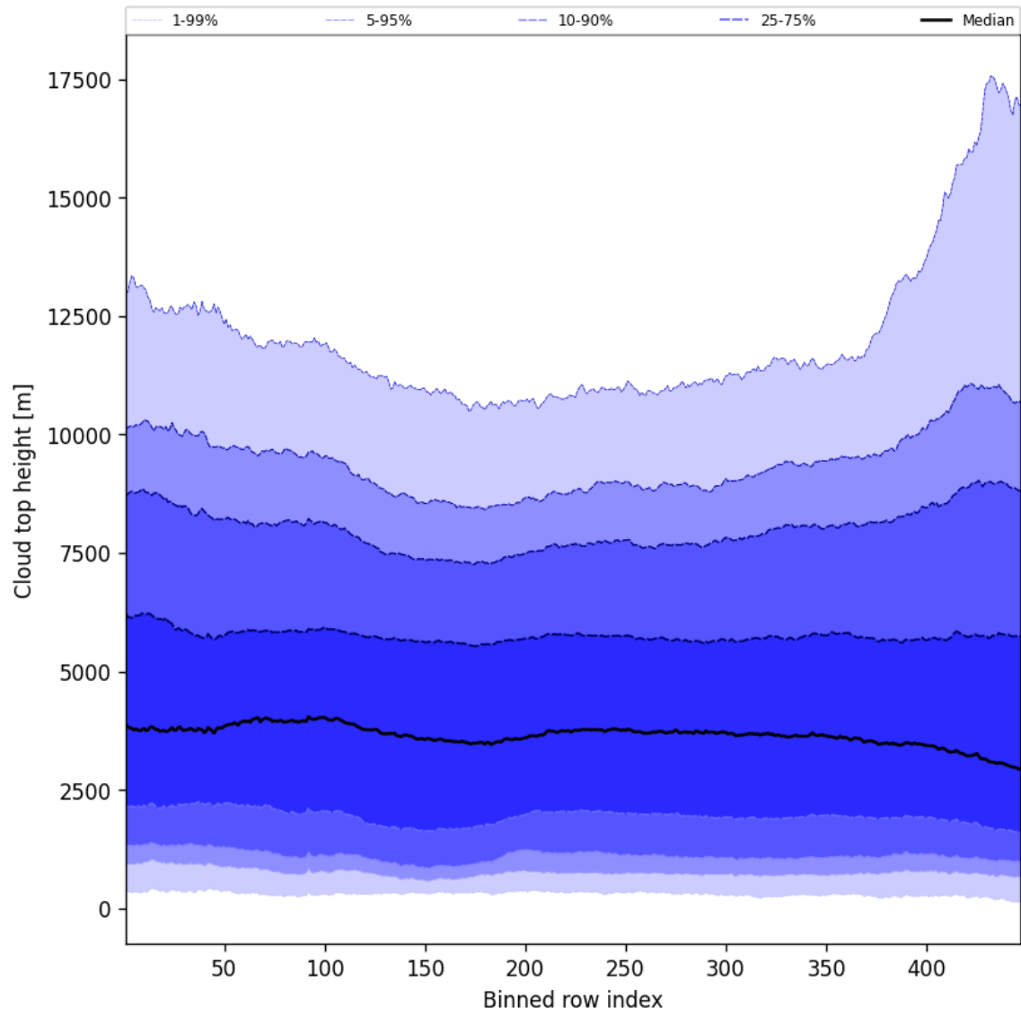
Figure 54: Along track statistics of “Cloud top height” for 2025-01-17 to 2025-01-18
