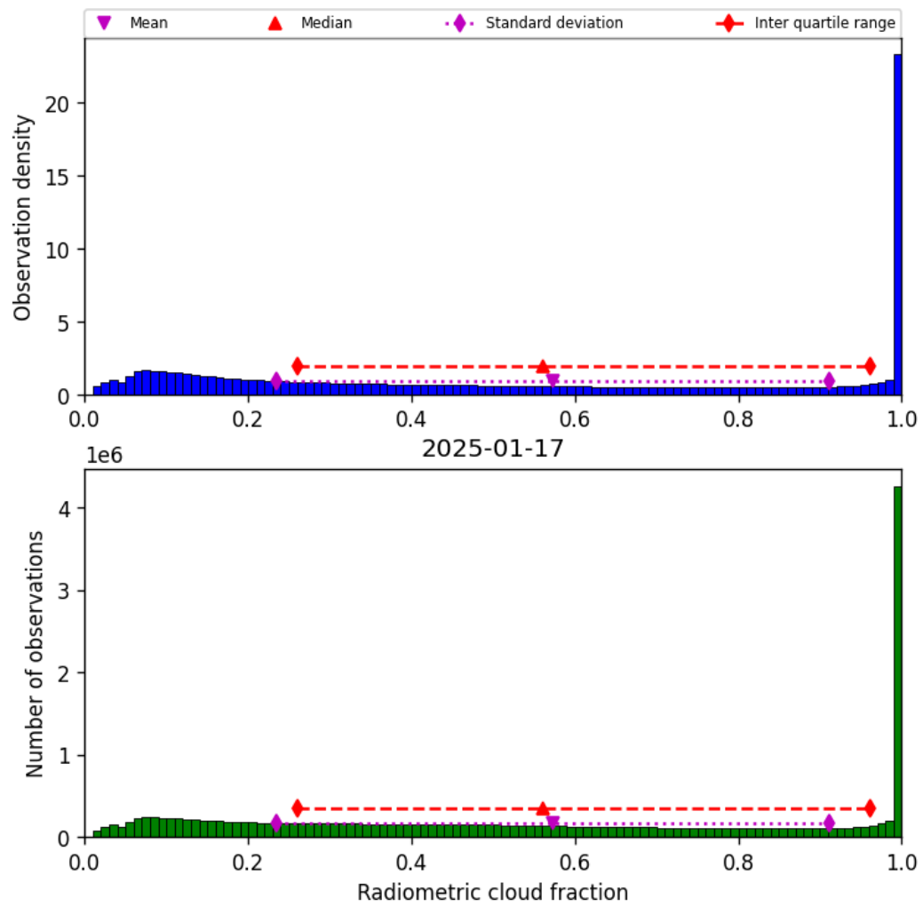
Figure 37: Histogram of “Radiometric cloud fraction” for 2025-01-17 to 2025-01-18
