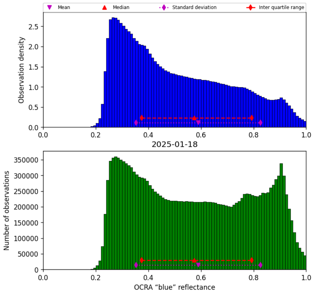
Figure 49: Histogram of "OCRA "blue" reflectance" for 2025-01-18 to 2025-01-19
