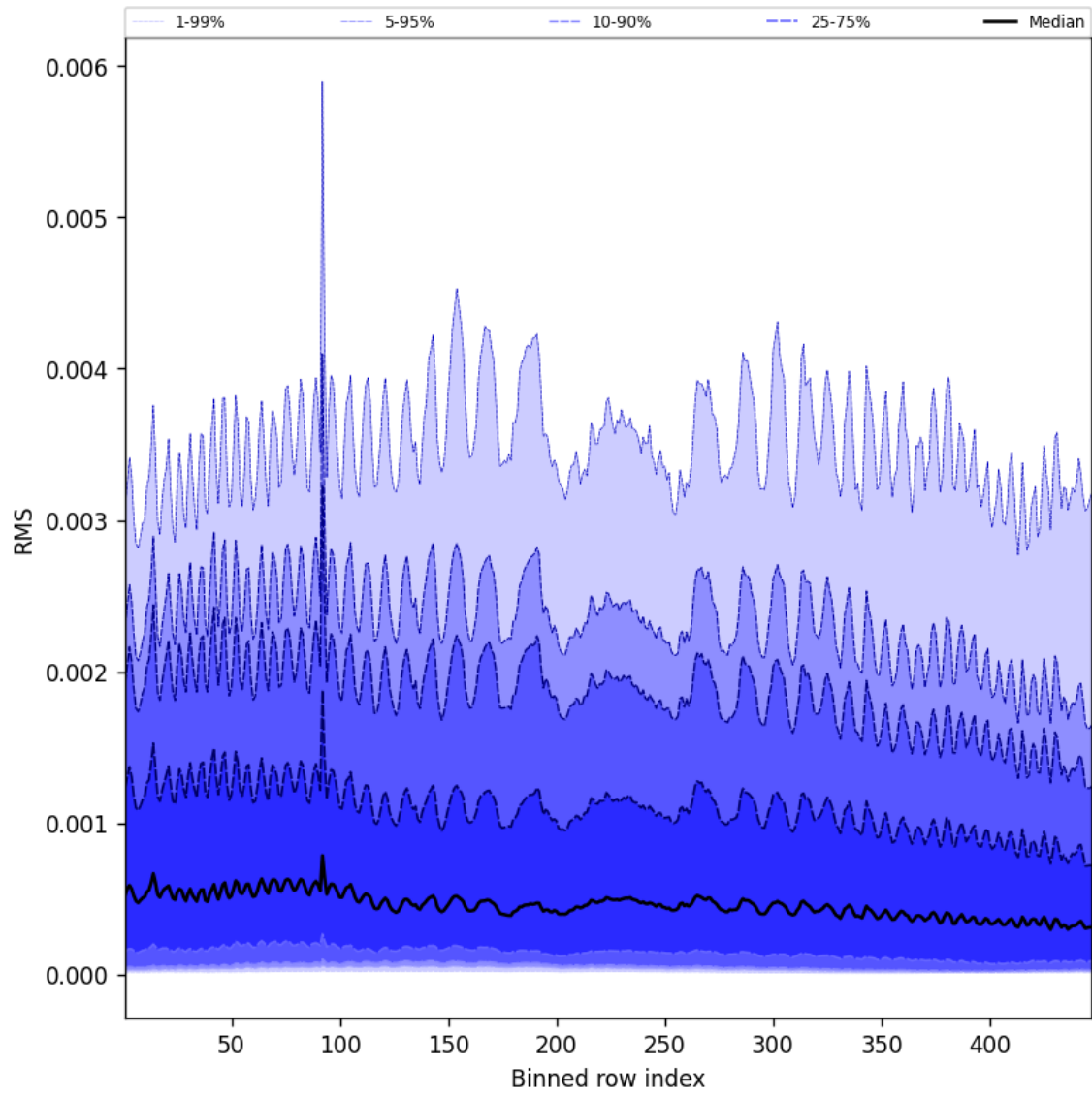
Figure 61: Along track statistics of “RMS” for 2025-01-18 to 2025-01-19
