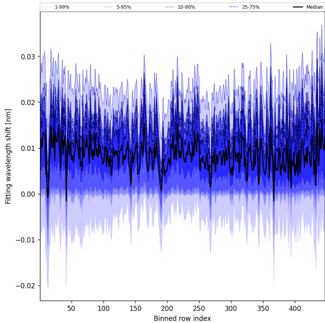
Figure 63: Along track statistics of “Fitting wavelength shift” for 2025-01-18 to 2025-01-19
