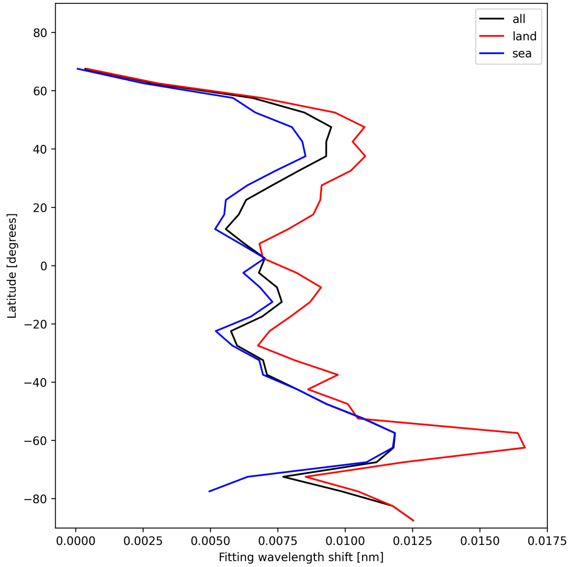
Figure 31: Zonal average of “Fitting wavelength shift” for 2025-01-18 to 2025-01-19.
