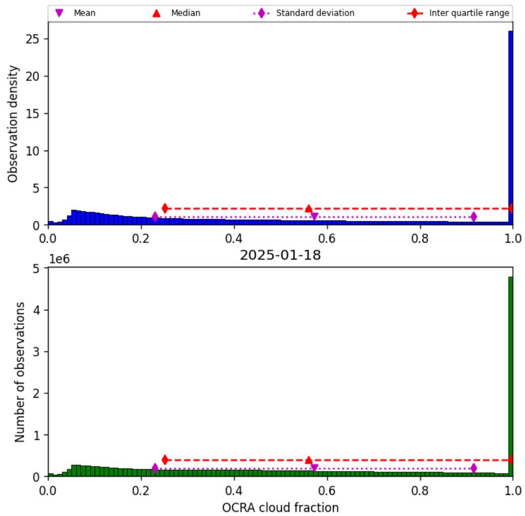
Figure 48: Histogram of “OCRA cloud fraction” for 2025-01-18 to 2025-01-19
