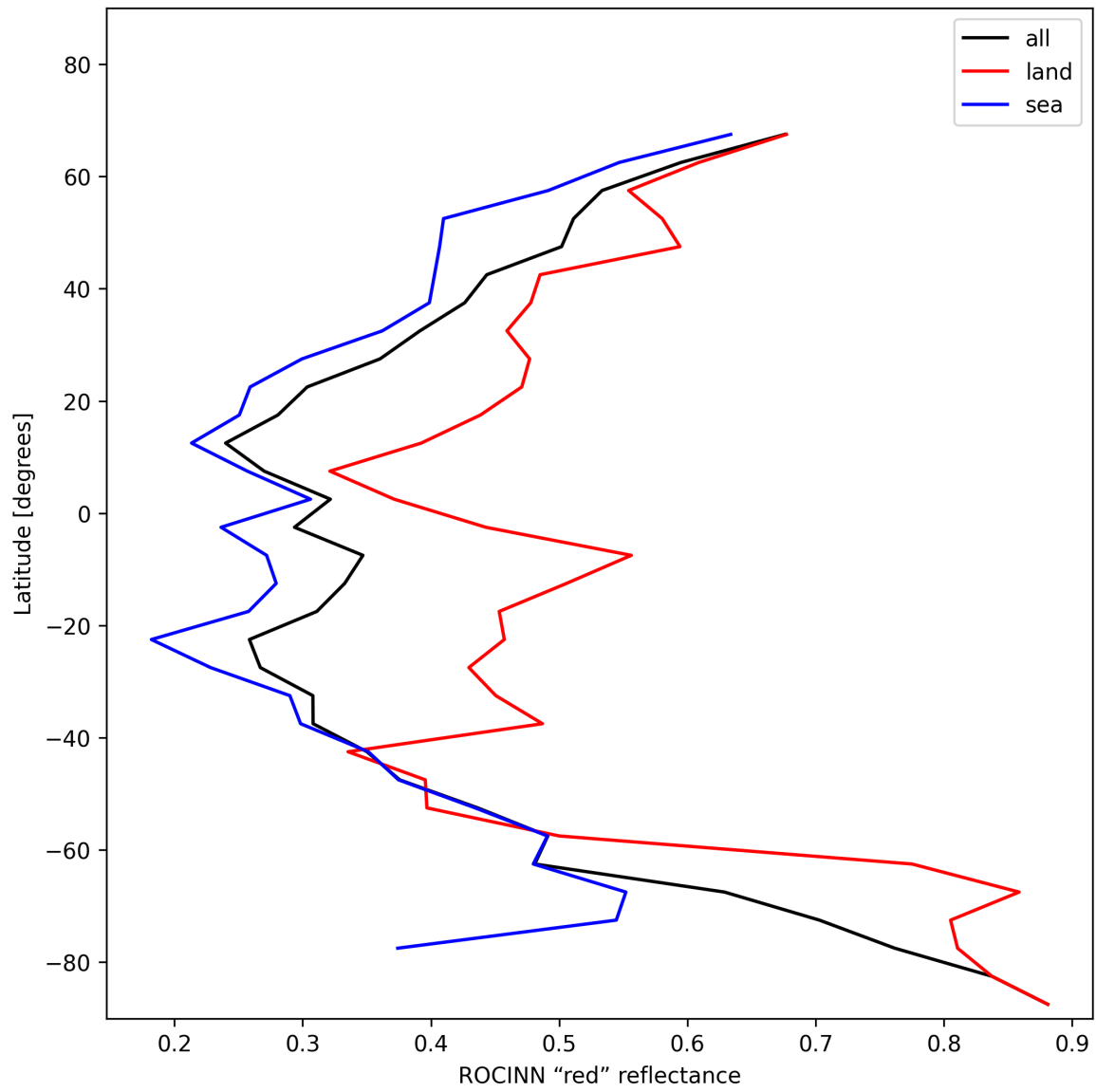
Figure 35: Zonal average of “ROCINN “red” reflectance” for 2025-01-18 to 2025-01-19.
