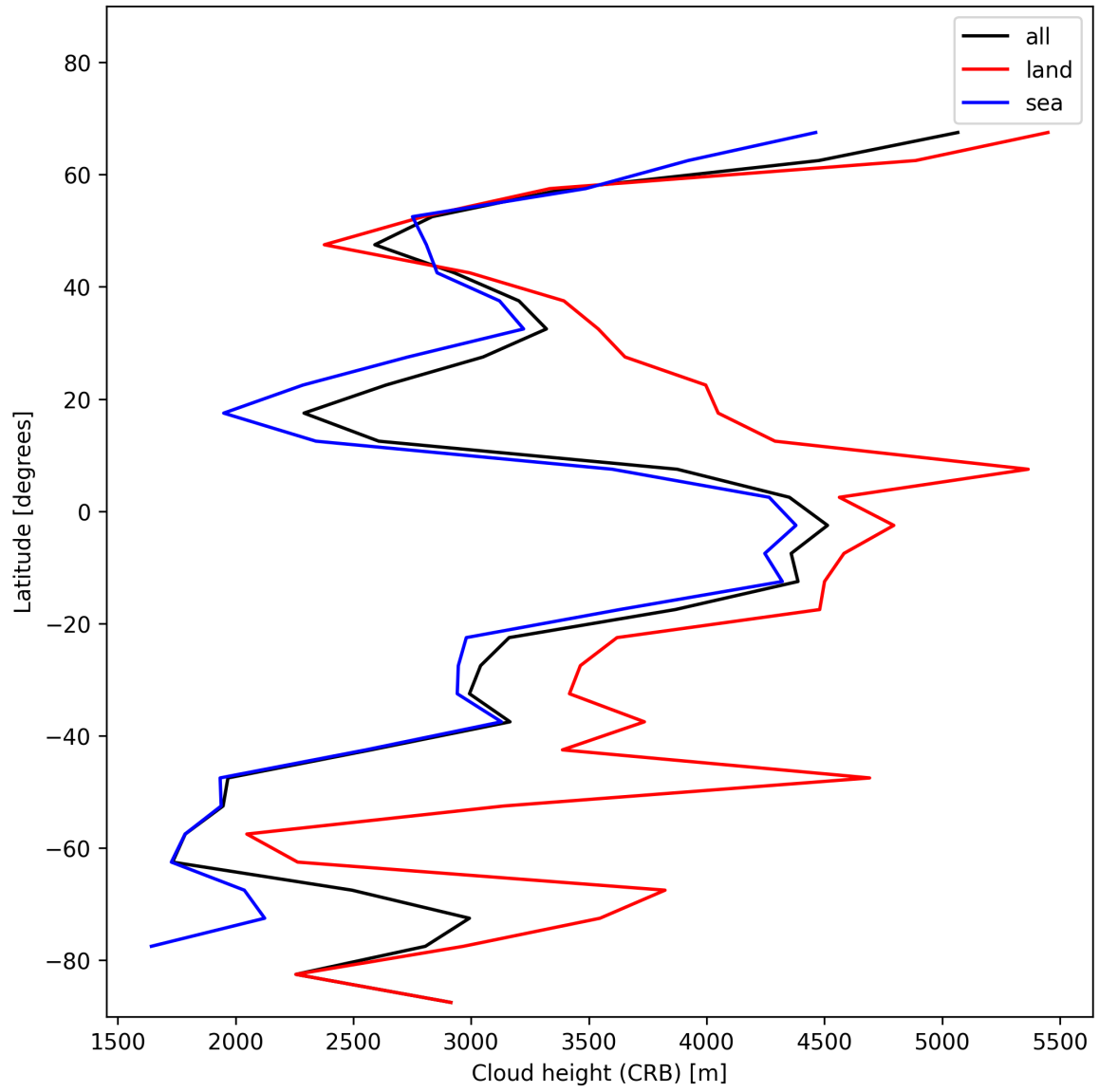
Figure 25: Zonal average of “Cloud height (CRB)” for 2025-01-18 to 2025-01-19.
