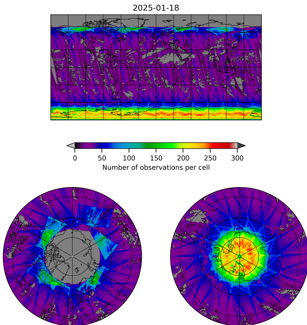
Figure 19: Map of the number of observations for 2025-01-18 to 2025-01-19
