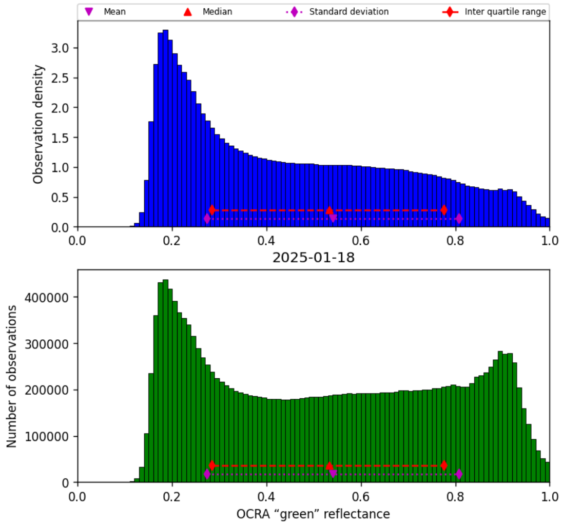
Figure 50: Histogram of “OCRA “green” reflectance” for 2025-01-18 to 2025-01-19
