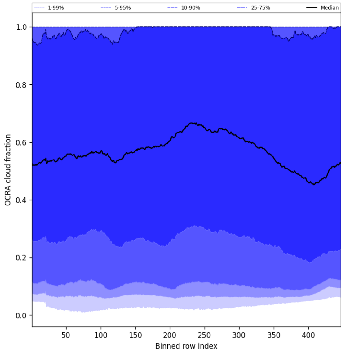
Figure 64: Along track statistics of “OCRA cloud fraction” for 2025-01-18 to 2025-01-19
