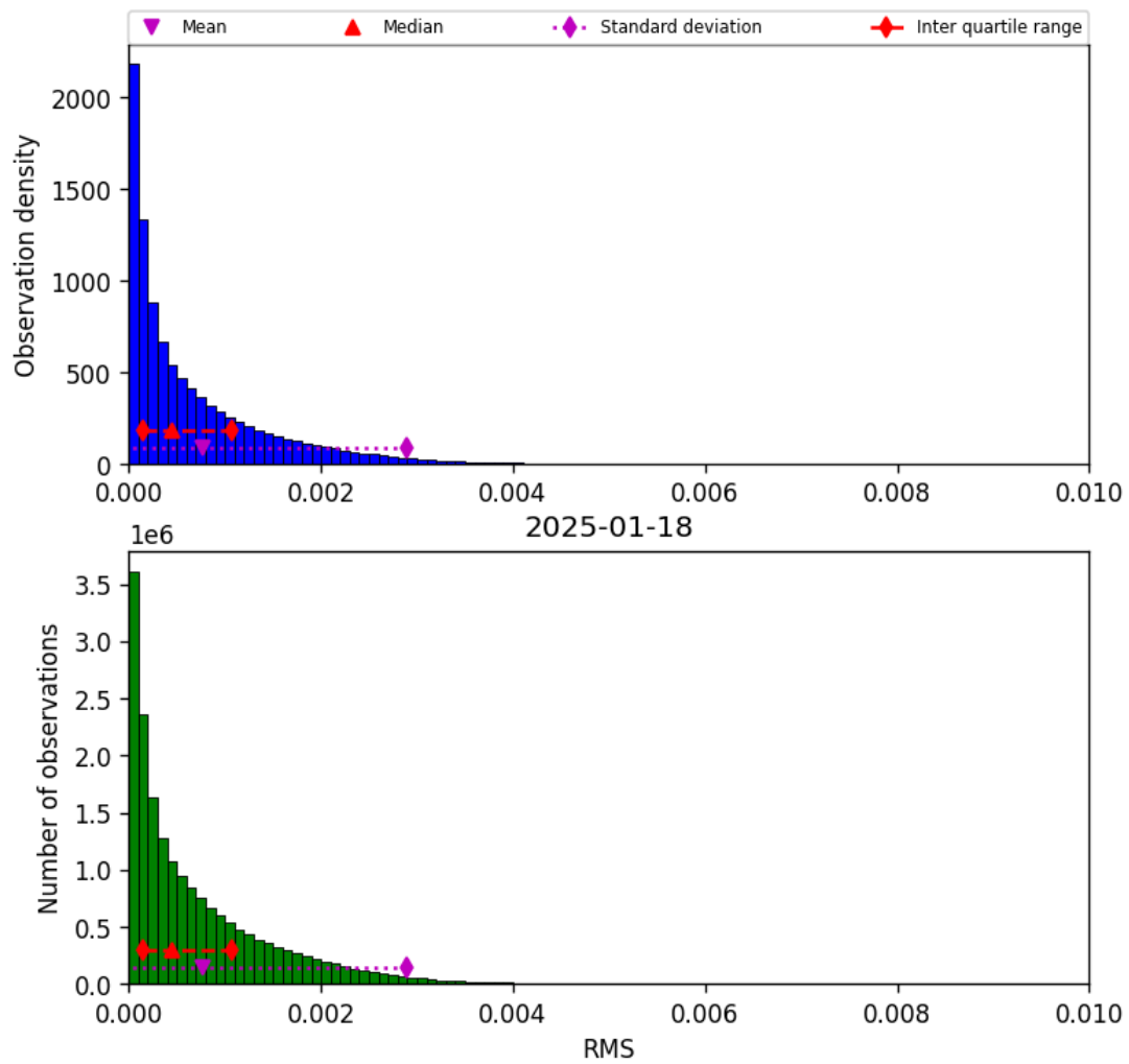
Figure 45: Histogram of “RMS” for 2025-01-18 to 2025-01-19
