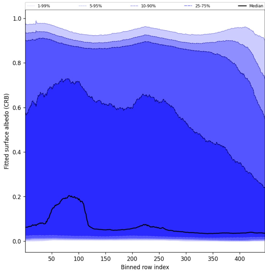
Figure 60: Along track statistics of “Fitted surface albedo (CRB)” for 2025-01-18 to 2025-01-19
