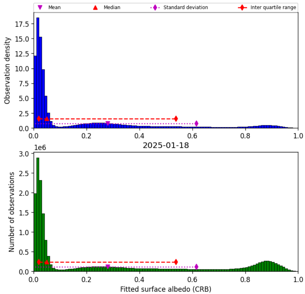
Figure 44: Histogram of “Fitted surface albedo (CRB)” for 2025-01-18 to 2025-01-19
