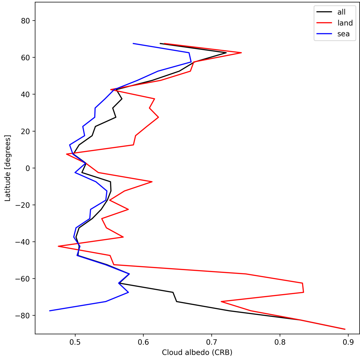
Figure 26: Zonal average of “Cloud albedo (CRB)” for 2025-01-18 to 2025-01-19.
