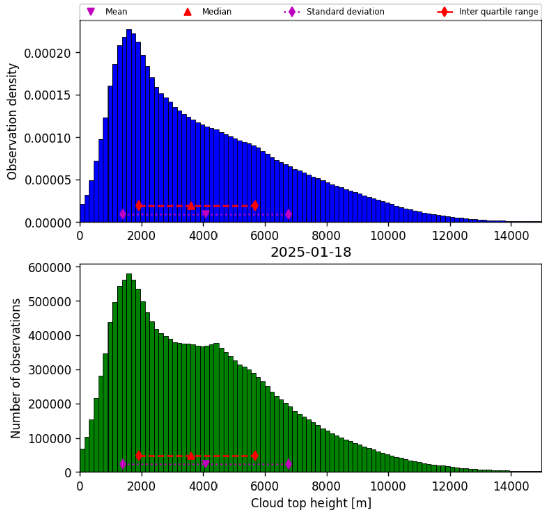
Figure 38: Histogram of “Cloud top height” for 2025-01-18 to 2025-01-19
