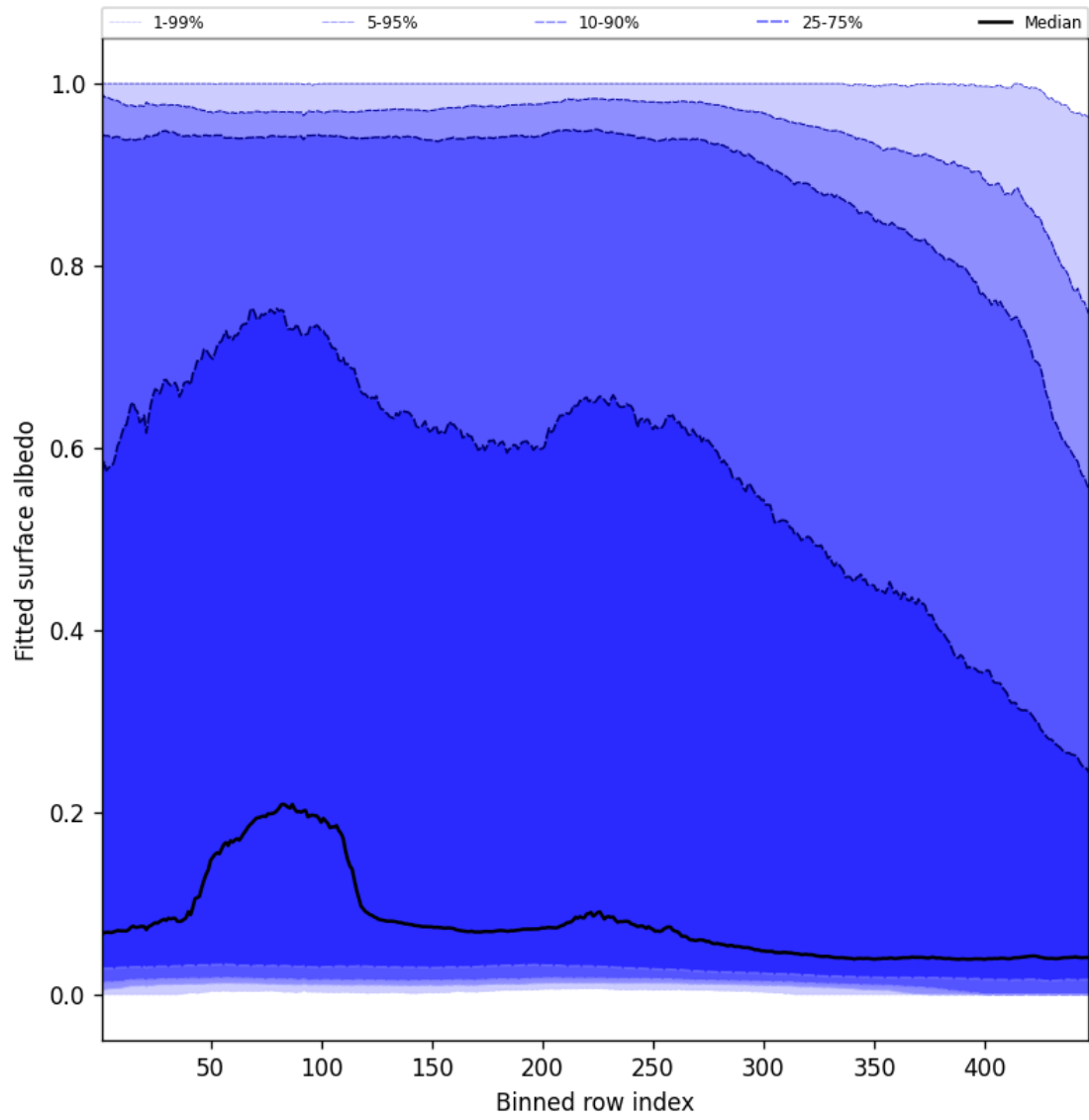
Figure 59: Along track statistics of “Fitted surface albedo” for 2025-01-18 to 2025-01-19
