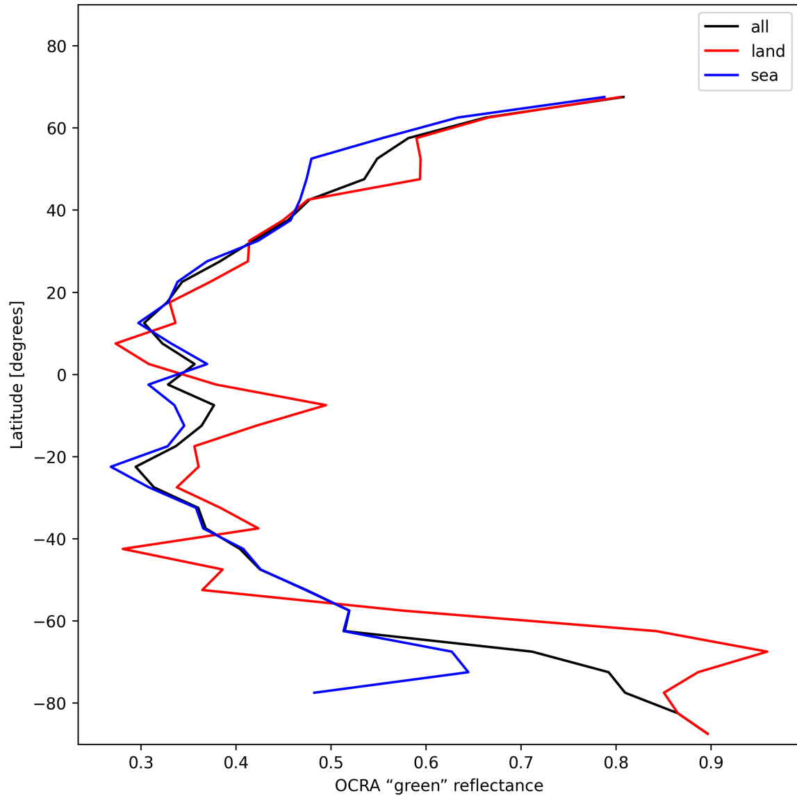
Figure 34: Zonal average of “OCRA “green” reflectance” for 2025-01-18 to 2025-01-19.
