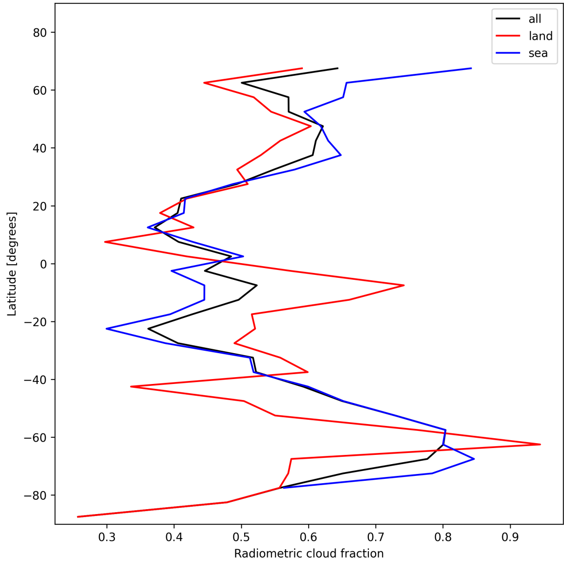
Figure 21: Zonal average of “Radiometric cloud fraction” for 2025-01-18 to 2025-01-19.
