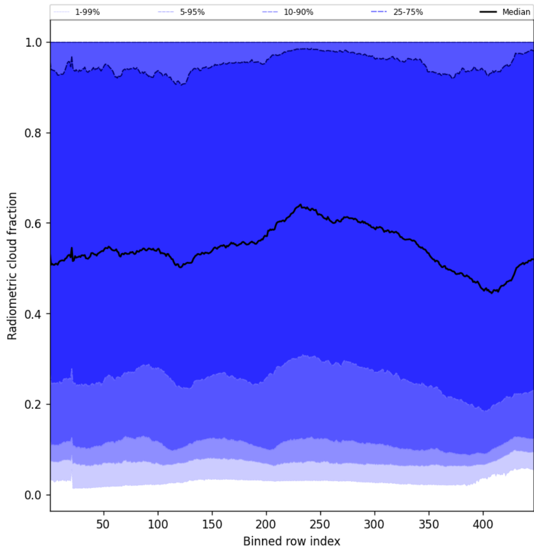
Figure 53: Along track statistics of “Radiometric cloud fraction” for 2025-01-18 to 2025-01-19
