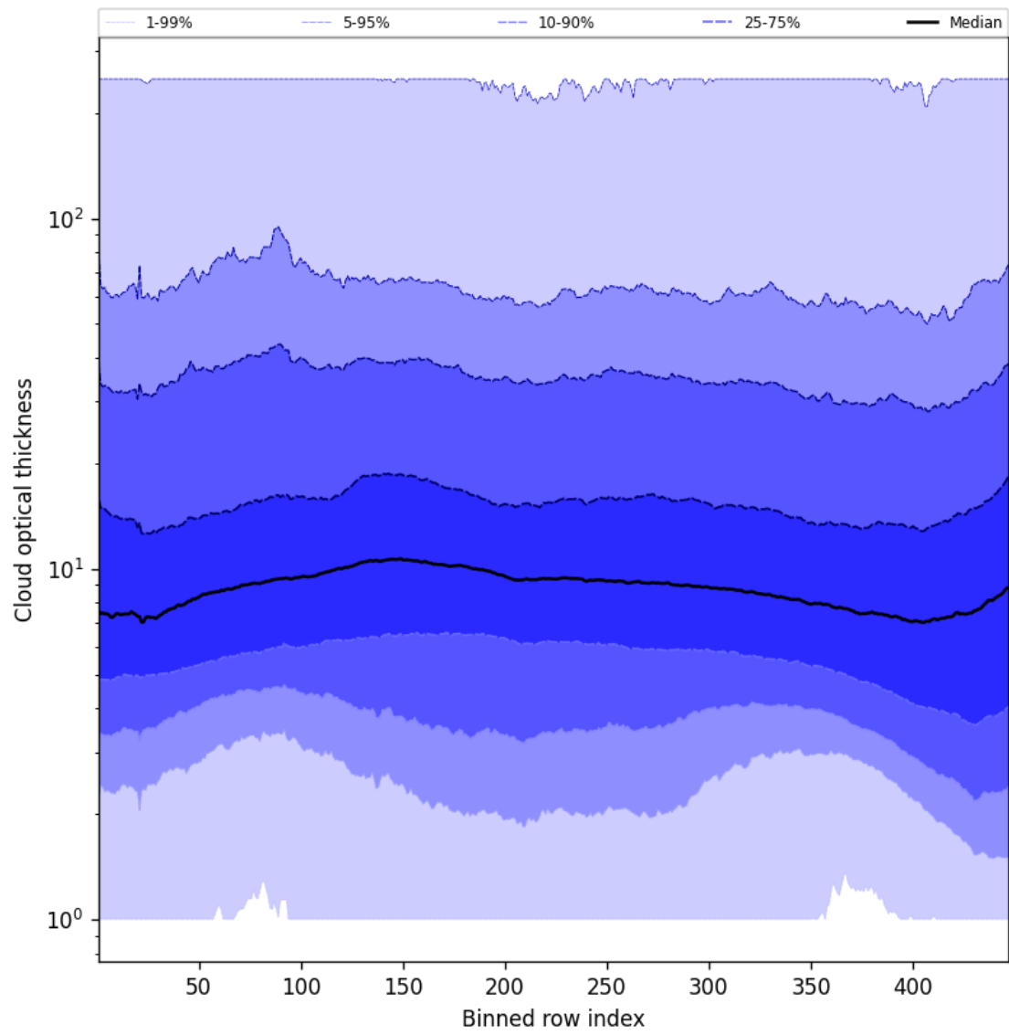
Figure 55: Along track statistics of “Cloud optical thickness” for 2025-01-18 to 2025-01-19
