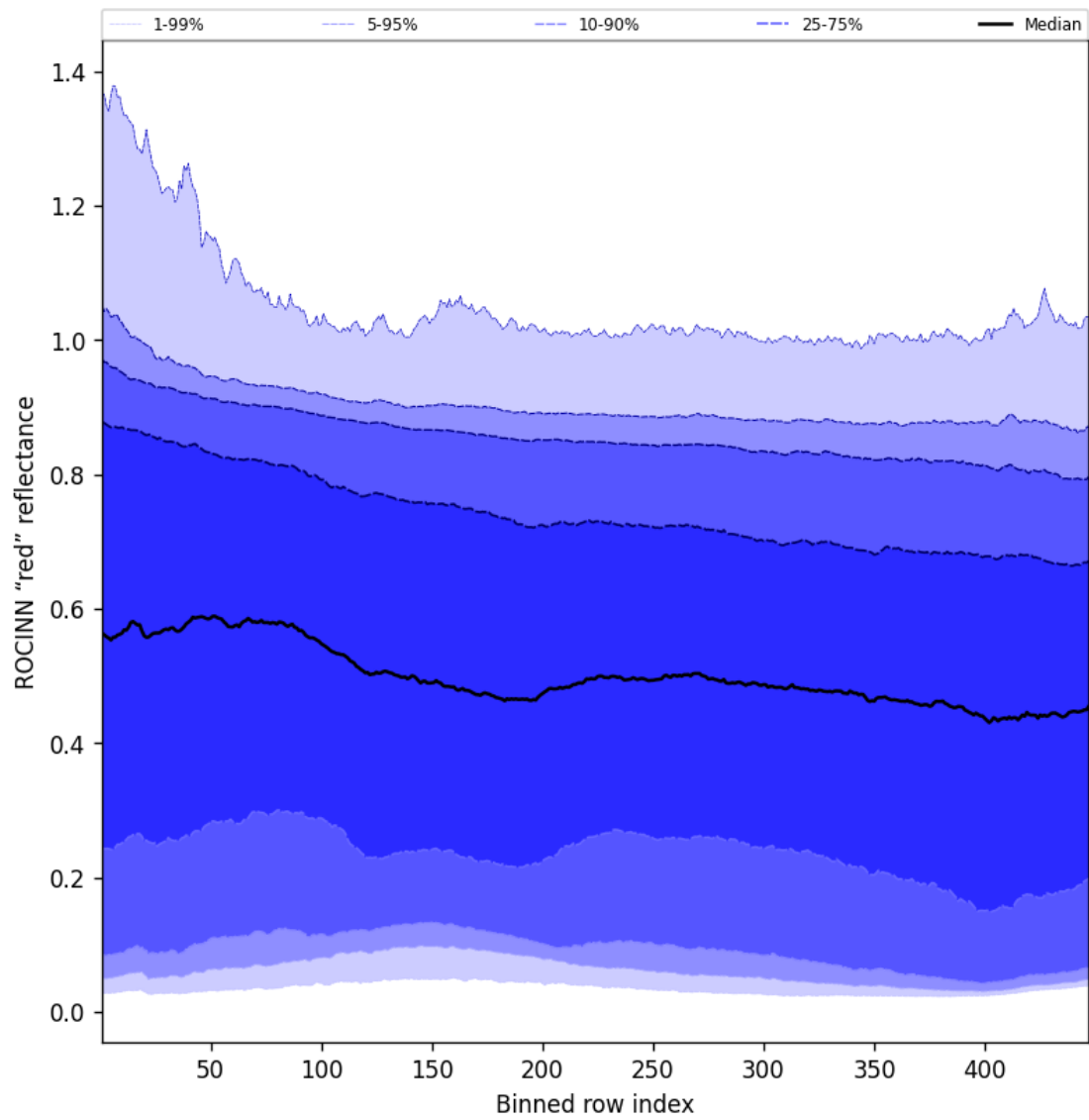
Figure 67: Along track statistics of “ROCINN “red” reflectance” for 2025-01-18 to 2025-01-19
