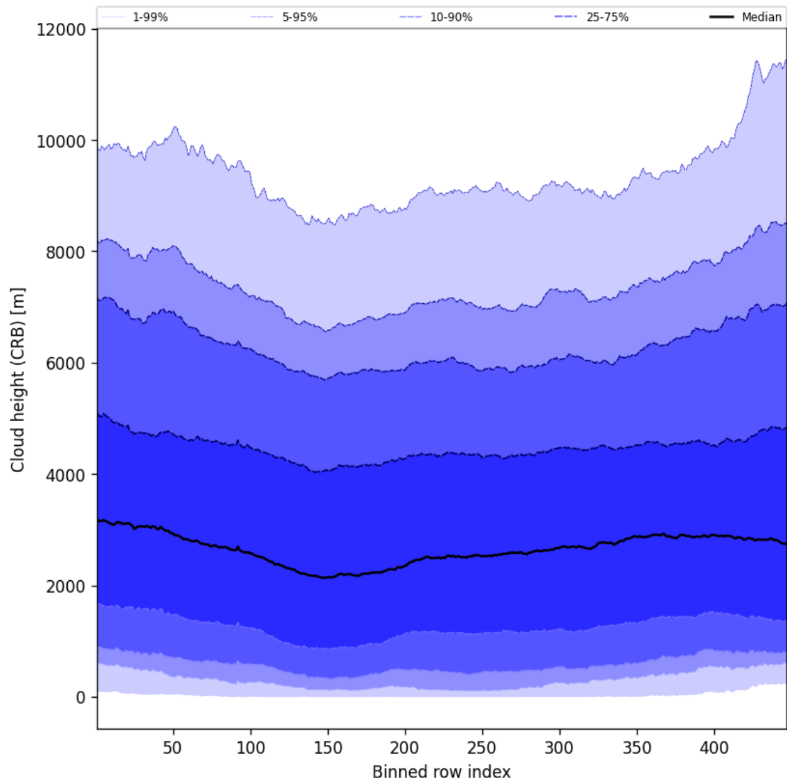
Figure 57: Along track statistics of “Cloud height (CRB)” for 2025-01-18 to 2025-01-19
