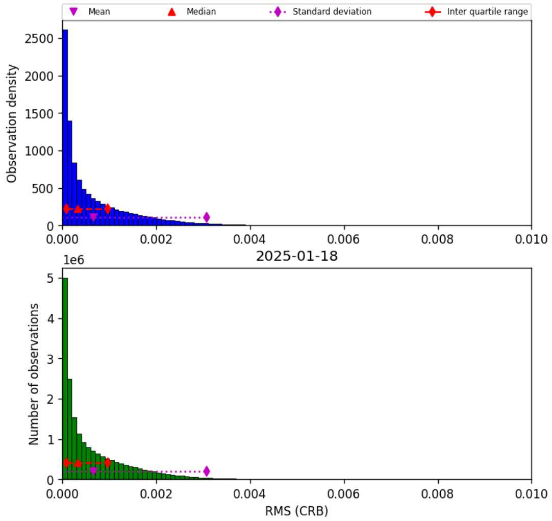
Figure 46: Histogram of "RMS (CRB)" for 2025-01-18 to 2025-01-19
