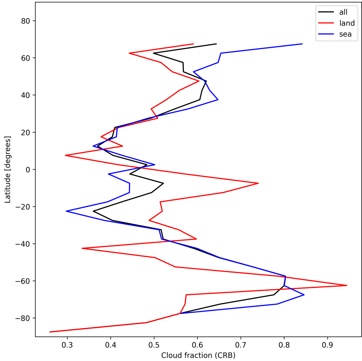
Figure 24: Zonal average of “Cloud fraction (CRB)” for 2025-01-18 to 2025-01-19.
