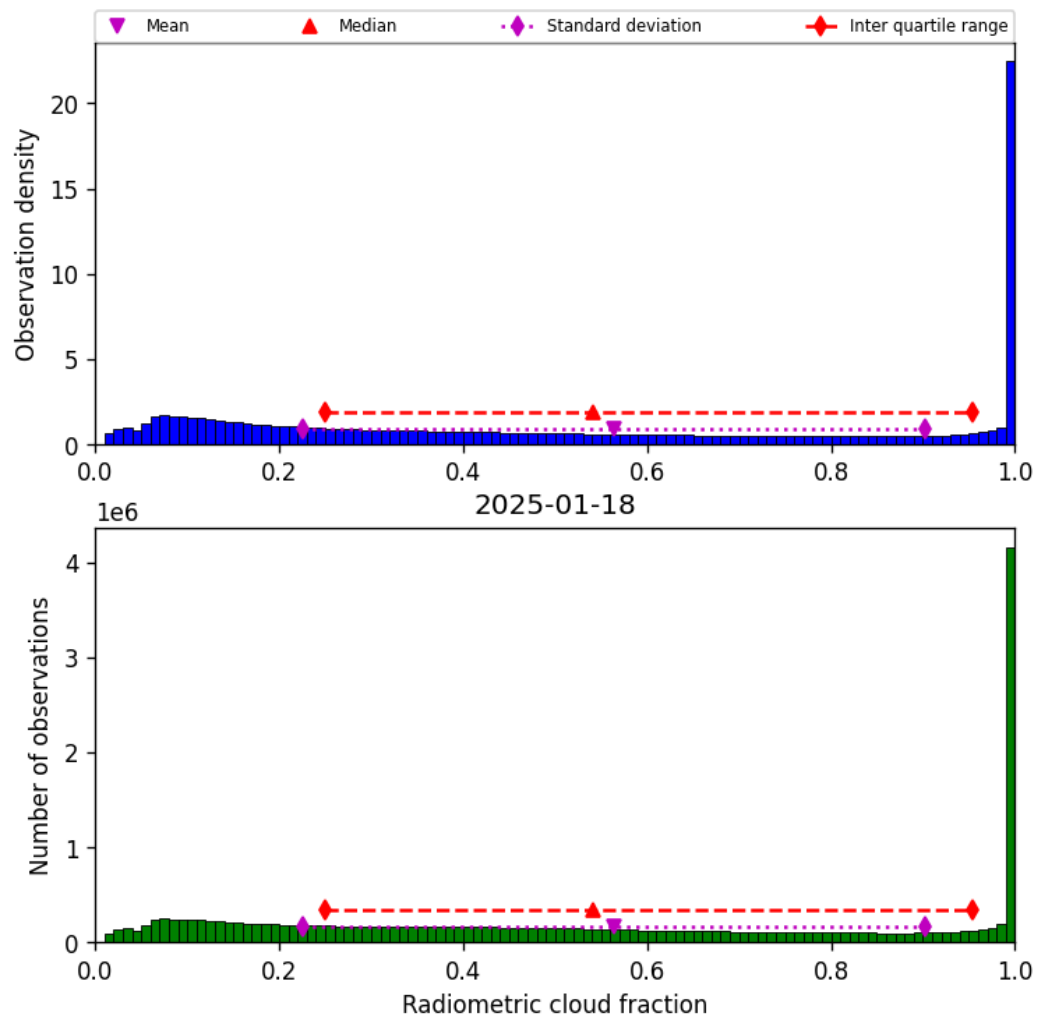
Figure 37: Histogram of “Radiometric cloud fraction” for 2025-01-18 to 2025-01-19
