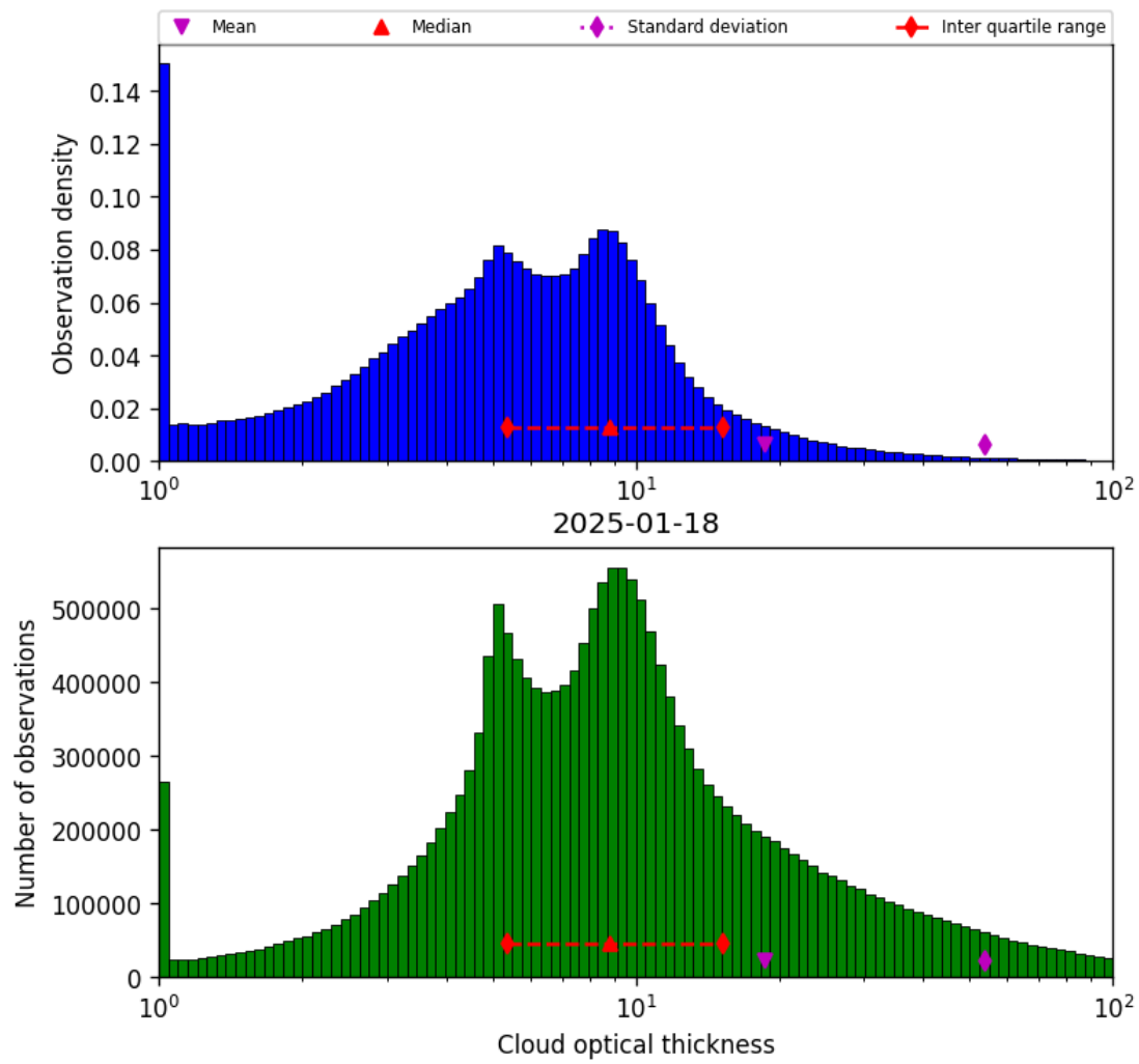
Figure 39: Histogram of “Cloud optical thickness” for 2025-01-18 to 2025-01-19
