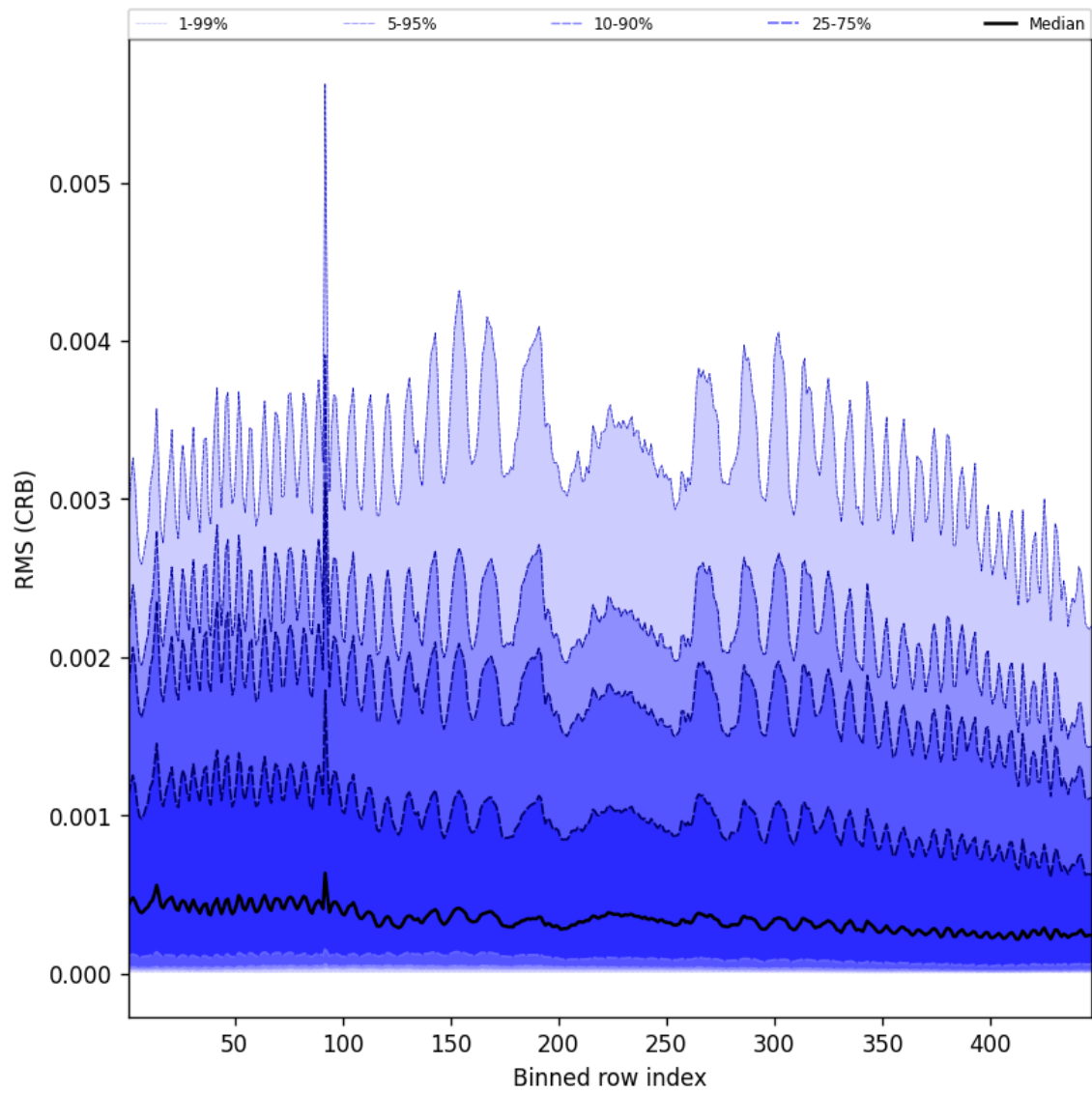
Figure 62: Along track statistics of “RMS (CRB)” for 2025-01-18 to 2025-01-19
