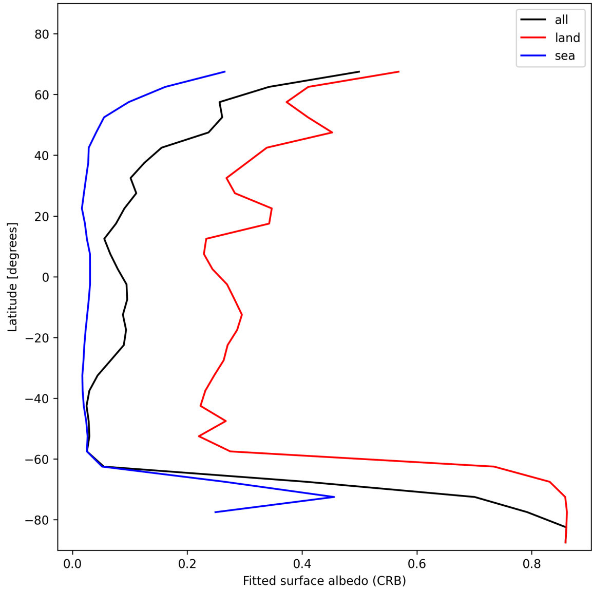
Figure 28: Zonal average of “Fitted surface albedo (CRB)” for 2025-01-18 to 2025-01-19.
