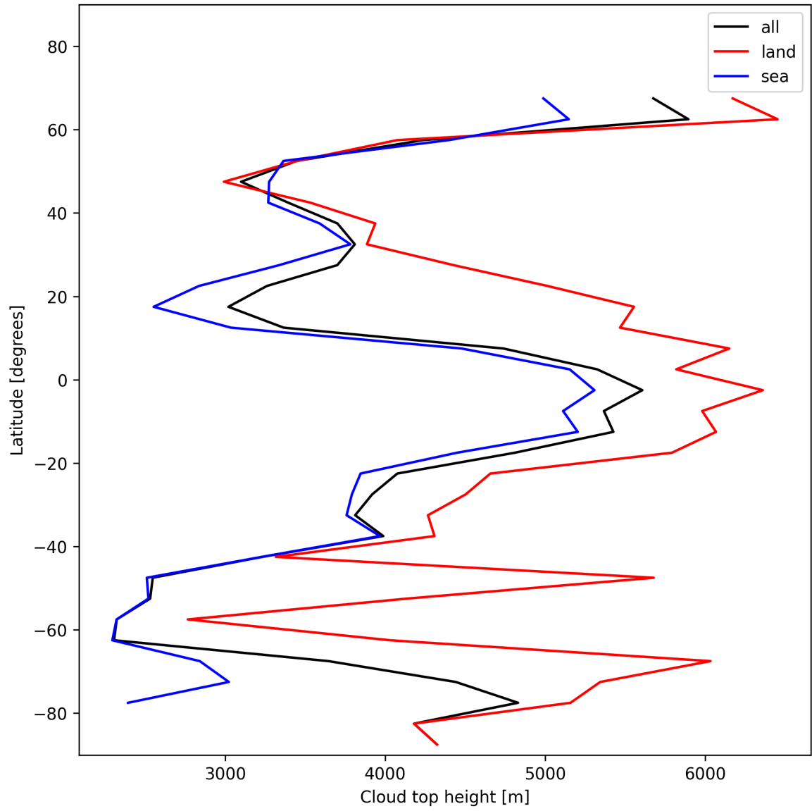
Figure 22: Zonal average of “Cloud top height” for 2025-01-18 to 2025-01-19.
