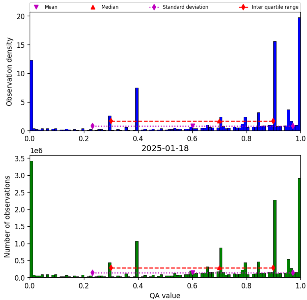
Figure 36: Histogram of “QA value” for 2025-01-18 to 2025-01-19
