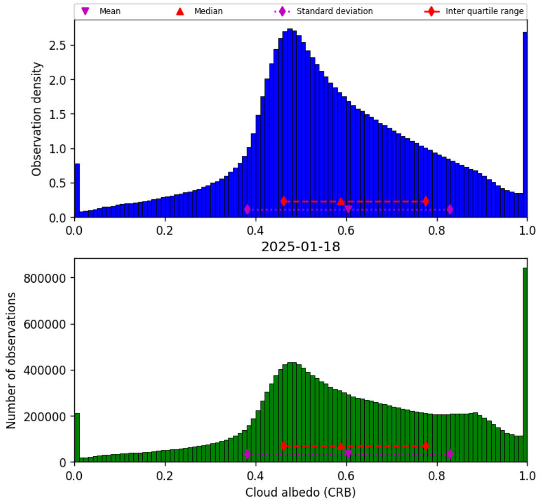
Figure 42: Histogram of “Cloud albedo (CRB)” for 2025-01-18 to 2025-01-19
