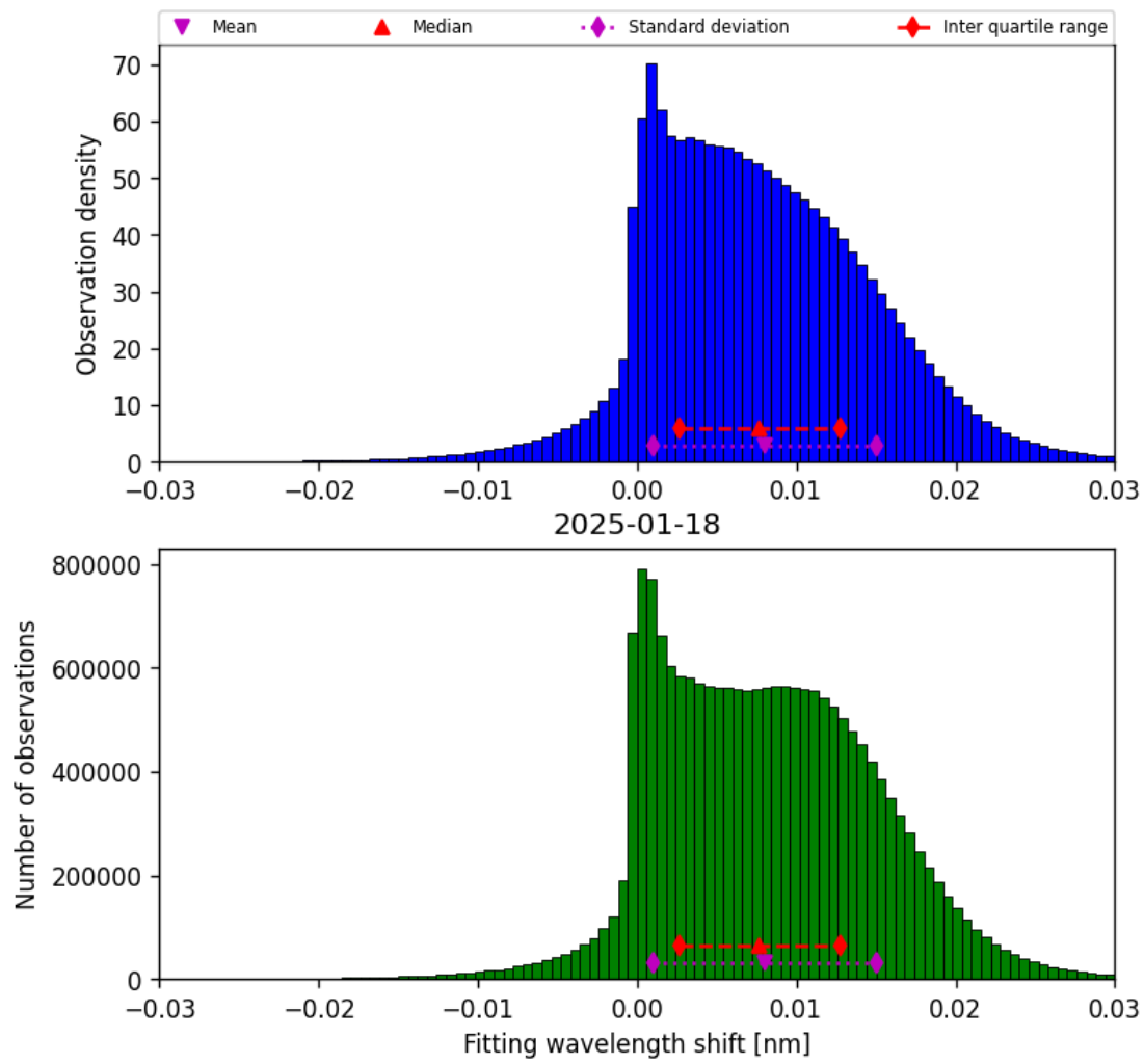
Figure 47: Histogram of “Fitting wavelength shift” for 2025-01-18 to 2025-01-19
