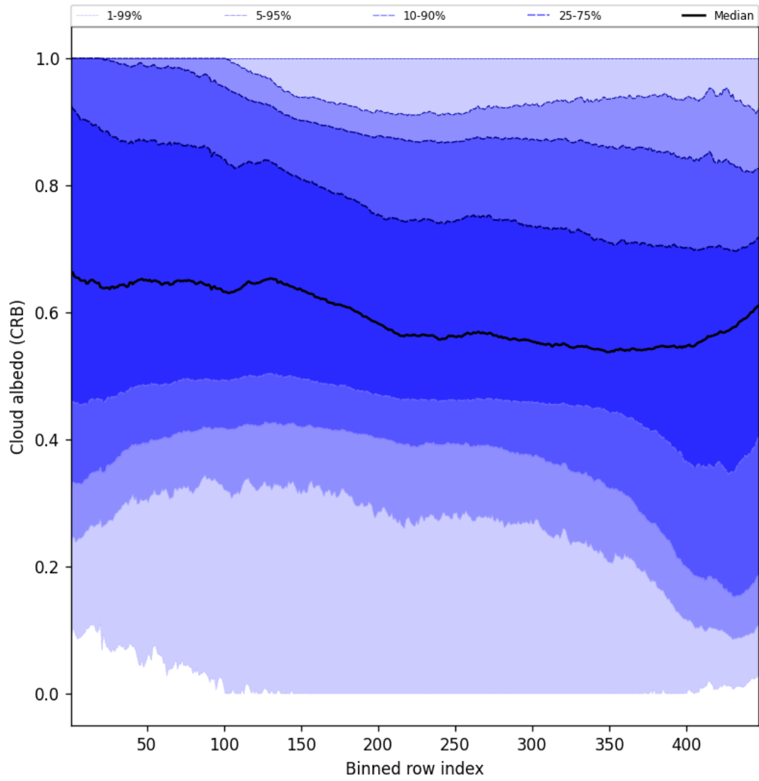
Figure 58: Along track statistics of “Cloud albedo (CRB)” for 2025-01-18 to 2025-01-19
