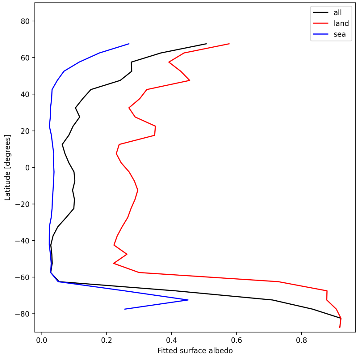
Figure 27: Zonal average of “Fitted surface albedo” for 2025-01-18 to 2025-01-19.
