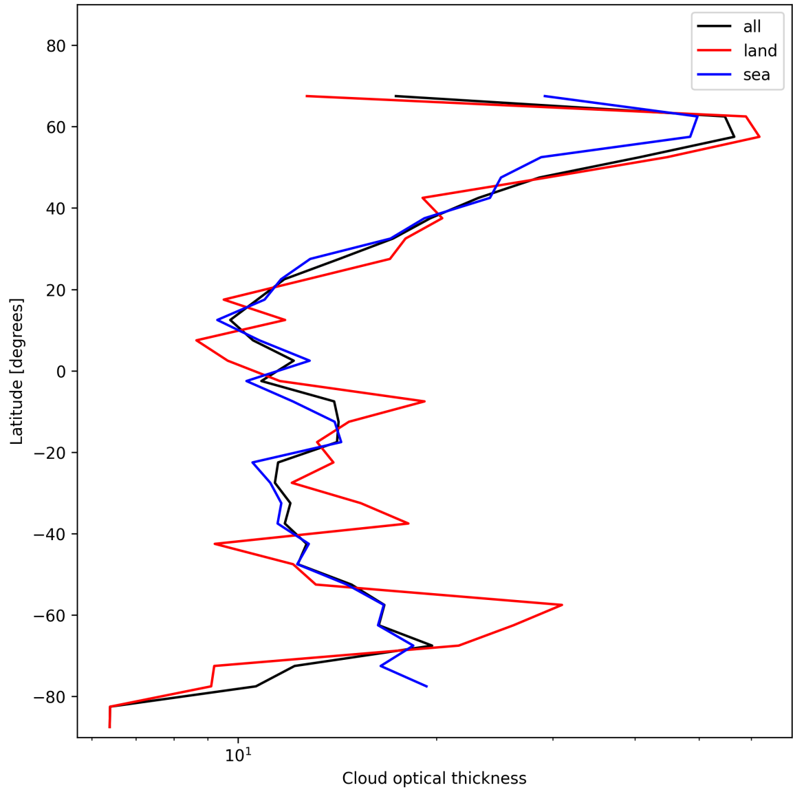
Figure 23: Zonal average of “Cloud optical thickness” for 2025-01-18 to 2025-01-19.
