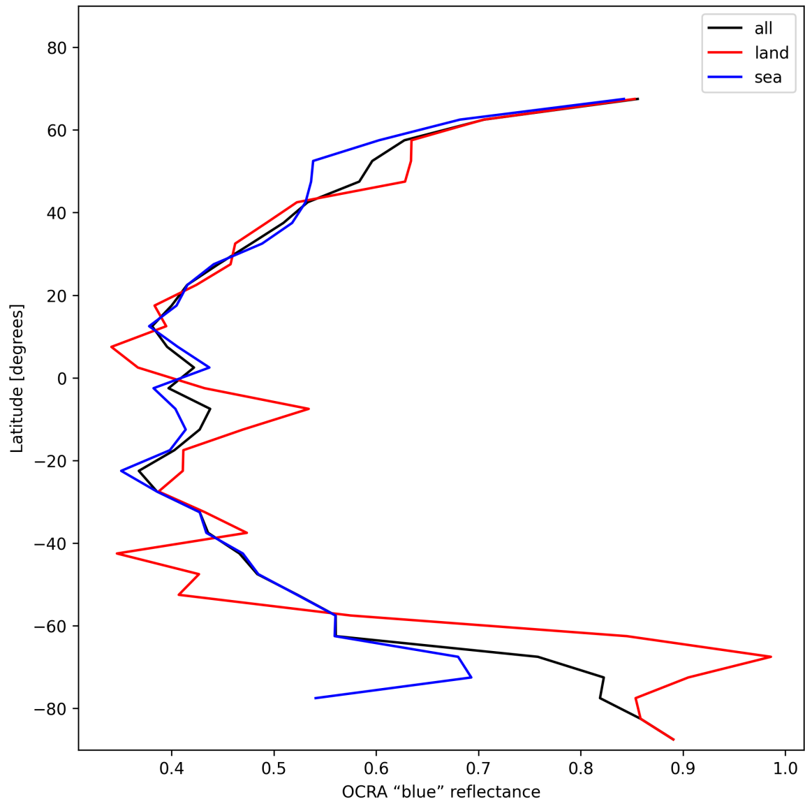
Figure 33: Zonal average of “OCRA “blue” reflectance” for 2025-01-18 to 2025-01-19.
