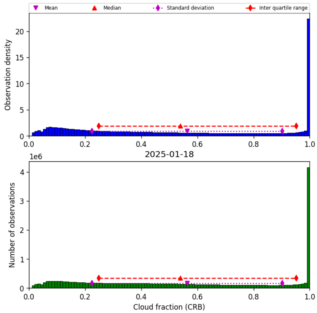
Figure 40: Histogram of “Cloud fraction (CRB)” for 2025-01-18 to 2025-01-19
