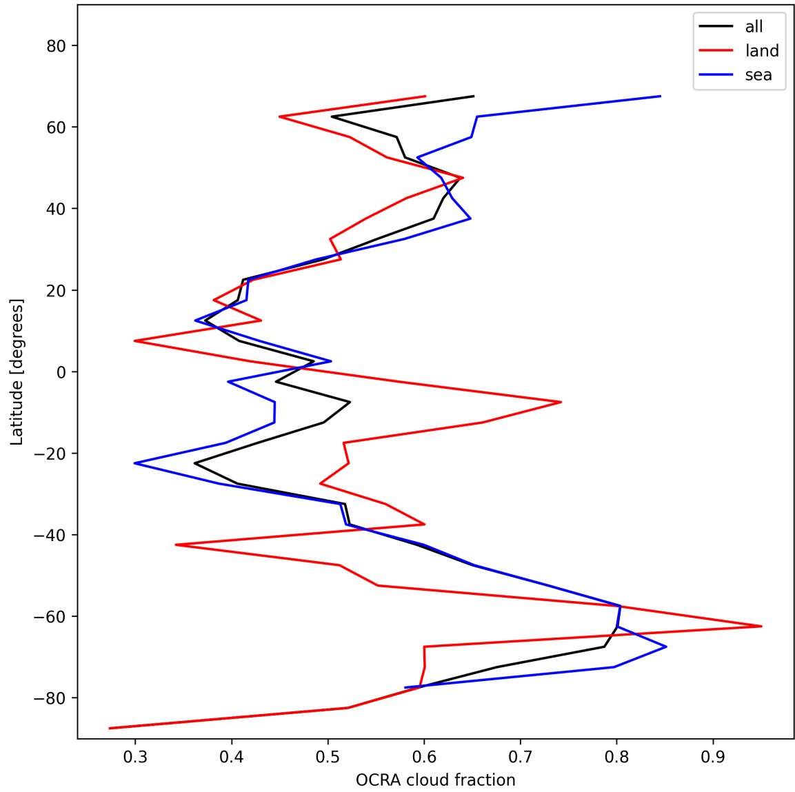
Figure 32: Zonal average of “OCRA cloud fraction” for 2025-01-18 to 2025-01-19.
