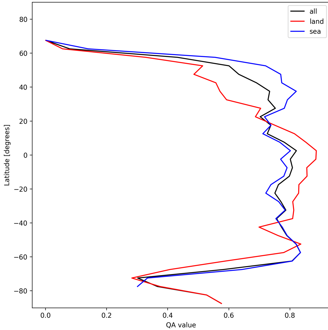
Figure 20: Zonal average of “QA value” for 2025-01-18 to 2025-01-19.
