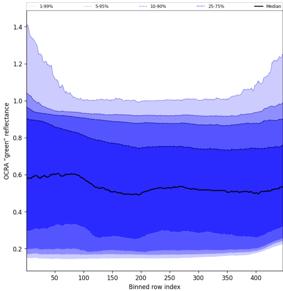
Figure 66: Along track statistics of “OCRA “green” reflectance” for 2025-01-18 to 2025-01-19
