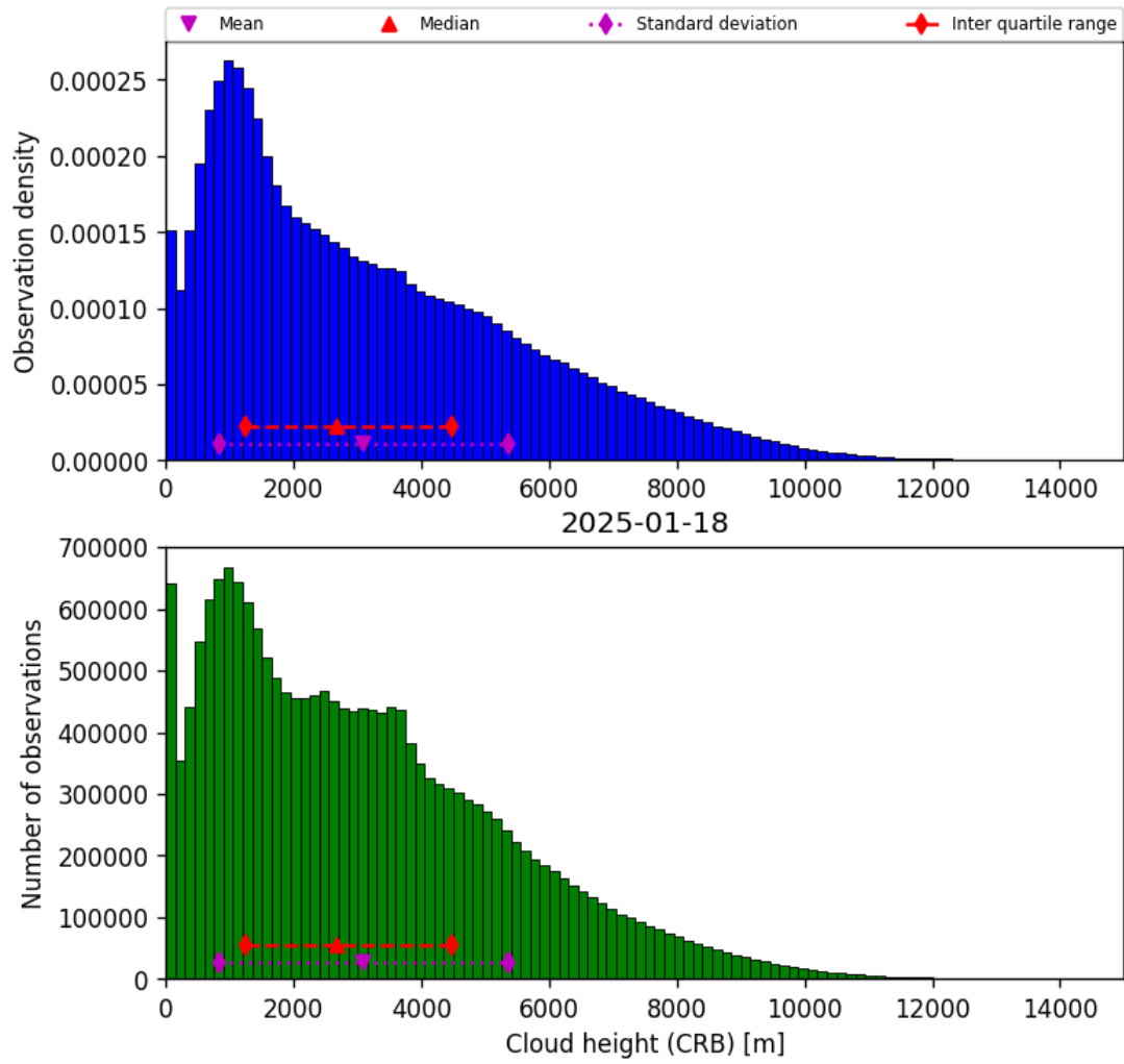
Figure 41: Histogram of “Cloud height (CRB)” for 2025-01-18 to 2025-01-19
