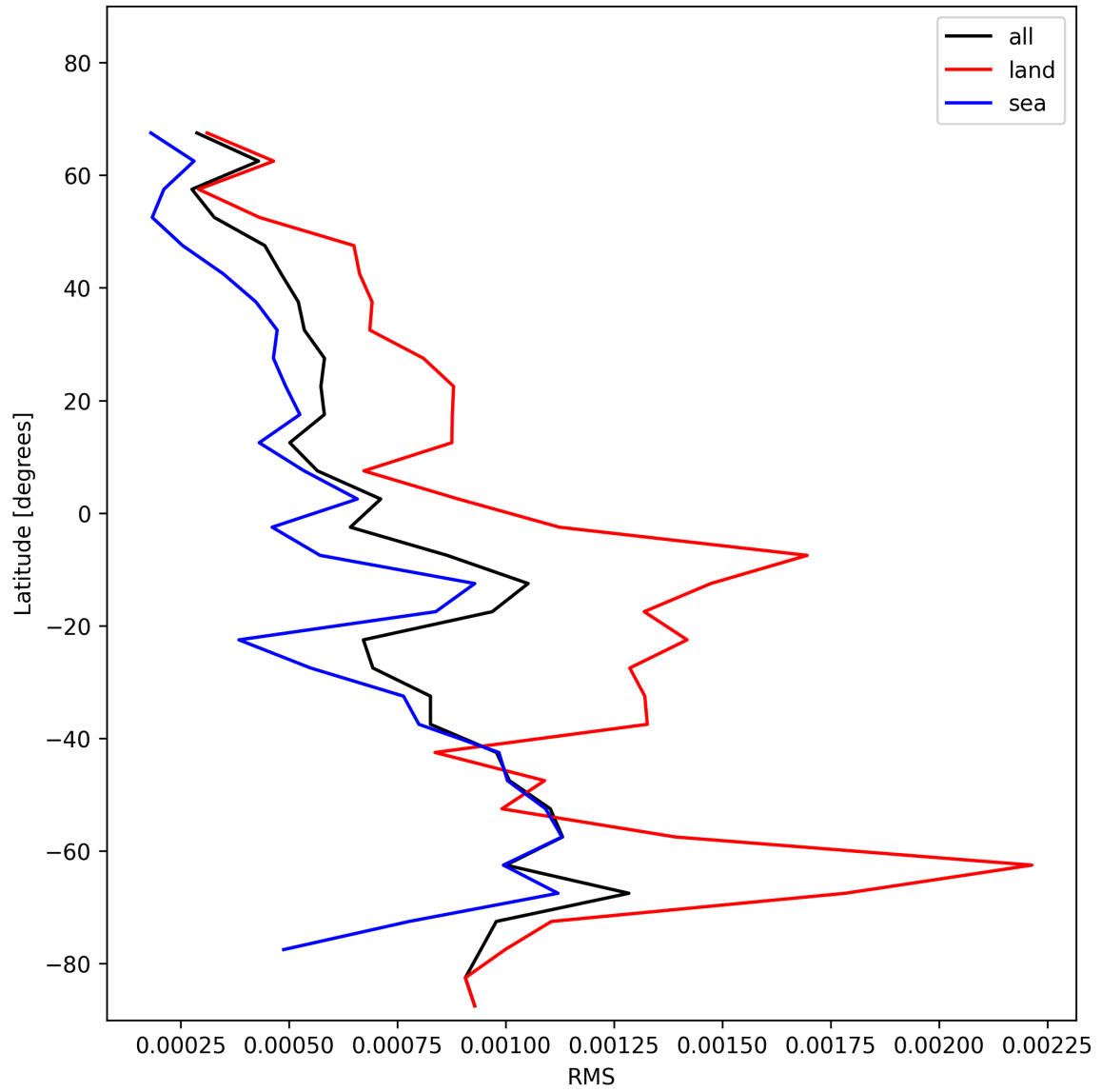
Figure 29: Zonal average of “RMS” for 2025-01-18 to 2025-01-19.
