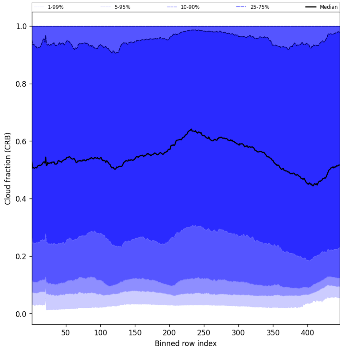
Figure 56: Along track statistics of “Cloud fraction (CRB)” for 2025-01-18 to 2025-01-19
