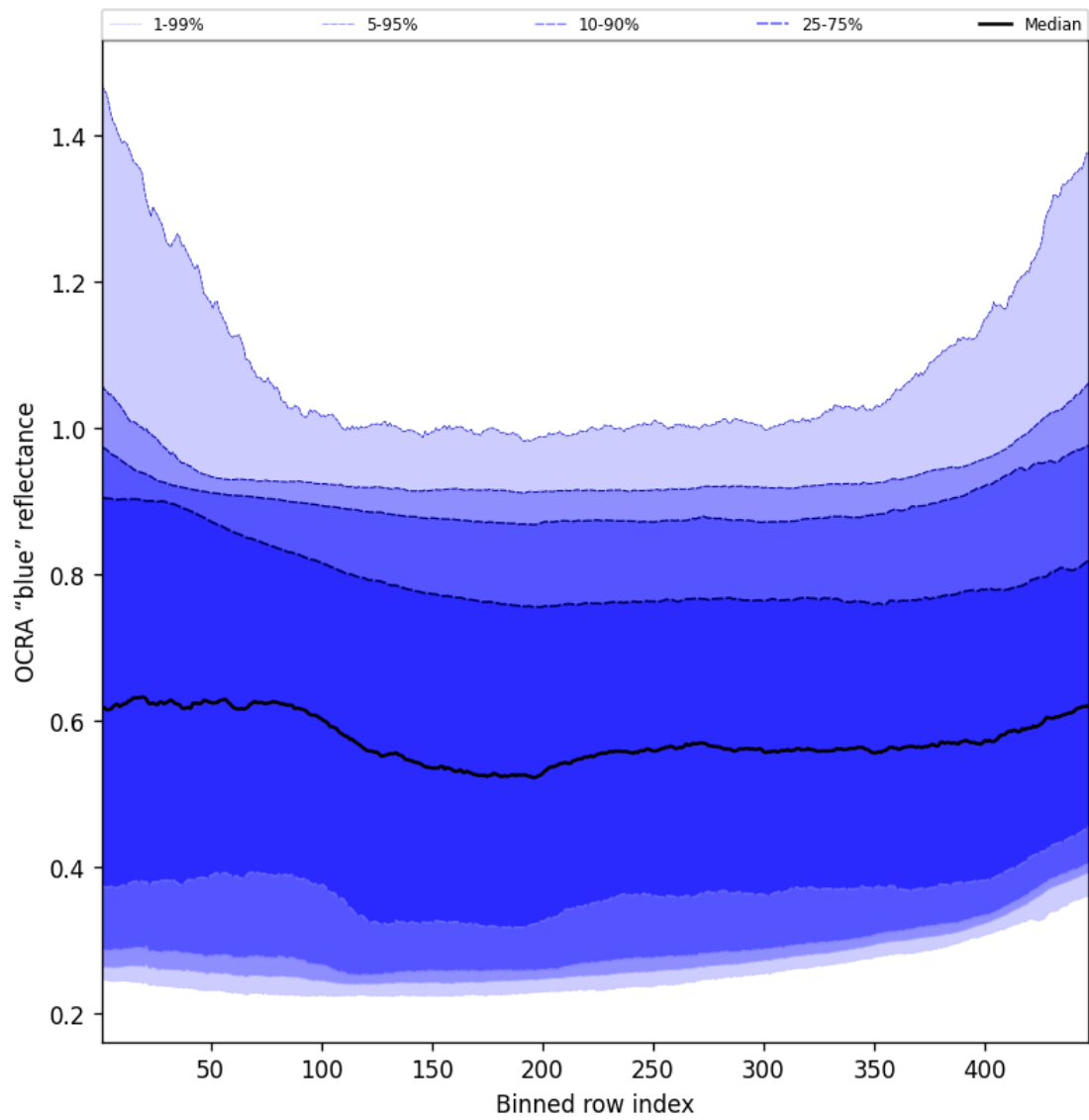
Figure 65: Along track statistics of “OCRA “blue” reflectance” for 2025-01-18 to 2025-01-19
