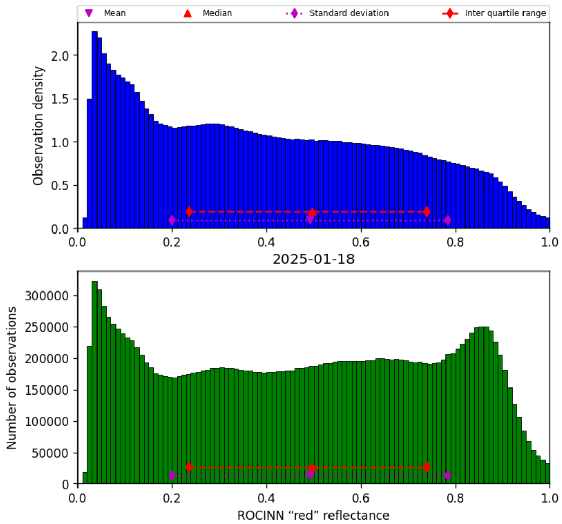
Figure 51: Histogram of “ROCINN “red” reflectance” for 2025-01-18 to 2025-01-19
