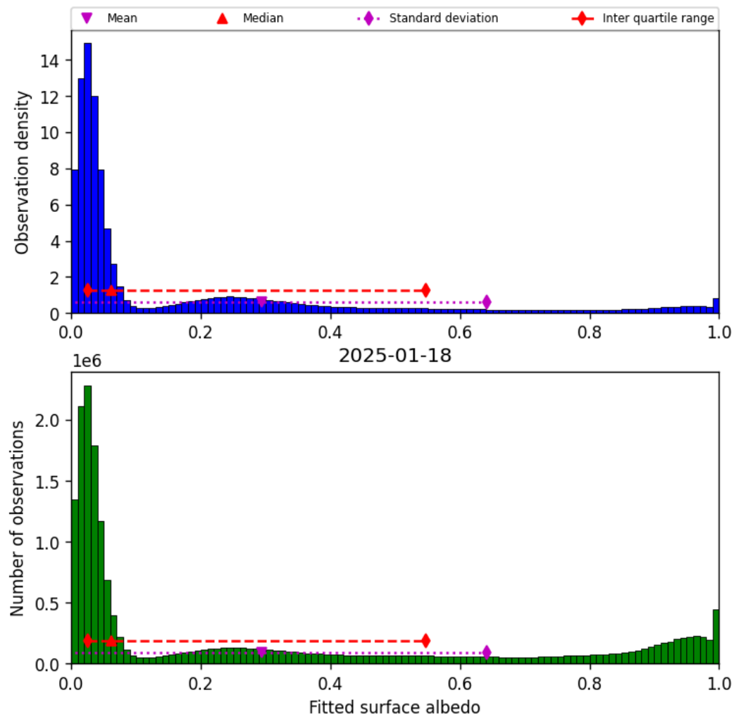
Figure 43: Histogram of “Fitted surface albedo” for 2025-01-18 to 2025-01-19
