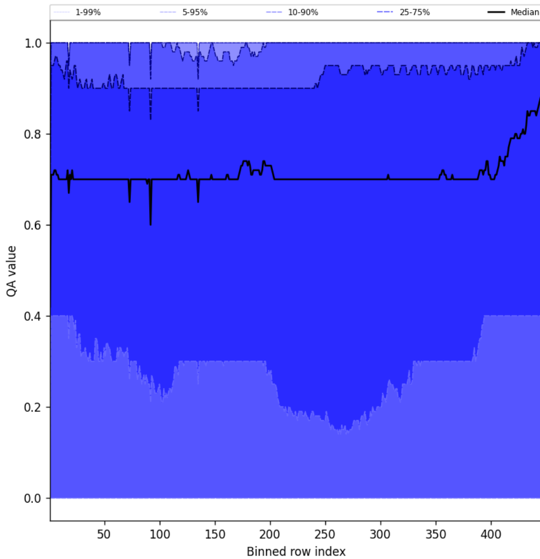
Figure 52: Along track statistics of “QA value” for 2025-01-18 to 2025-01-19
