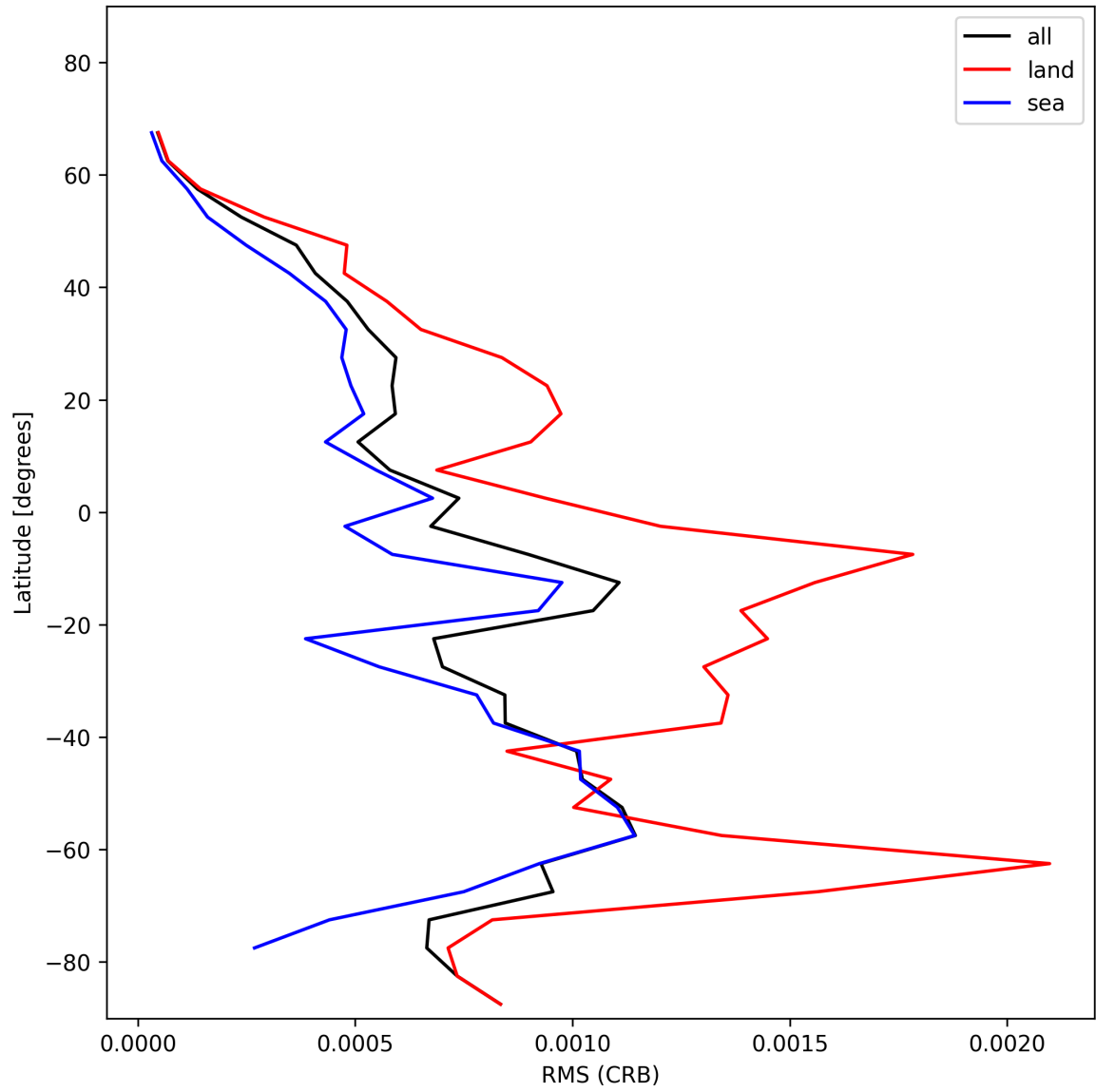
Figure 30: Zonal average of “RMS (CRB)” for 2025-01-18 to 2025-01-19.
