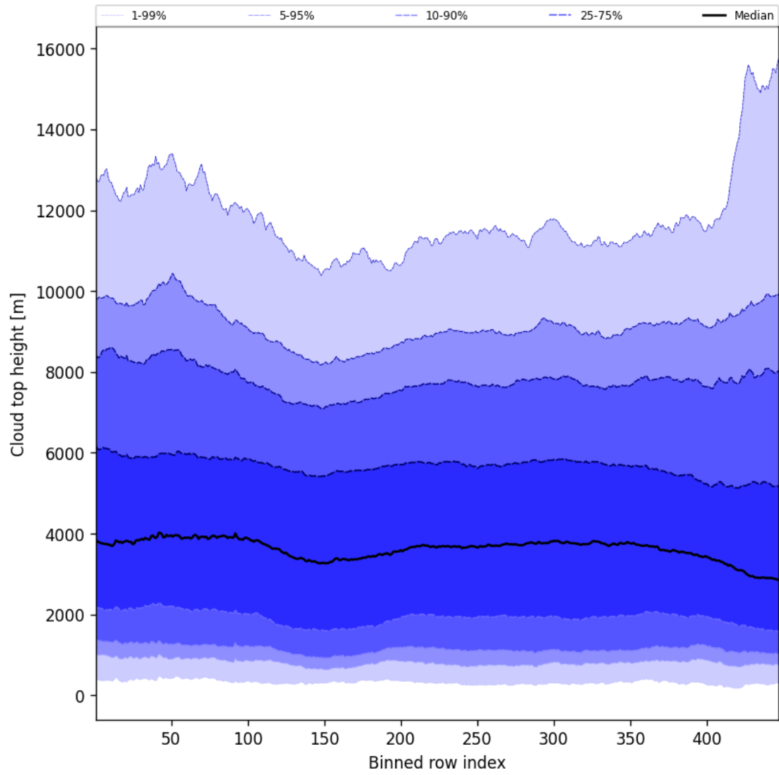
Figure 54: Along track statistics of “Cloud top height” for 2025-01-18 to 2025-01-19
