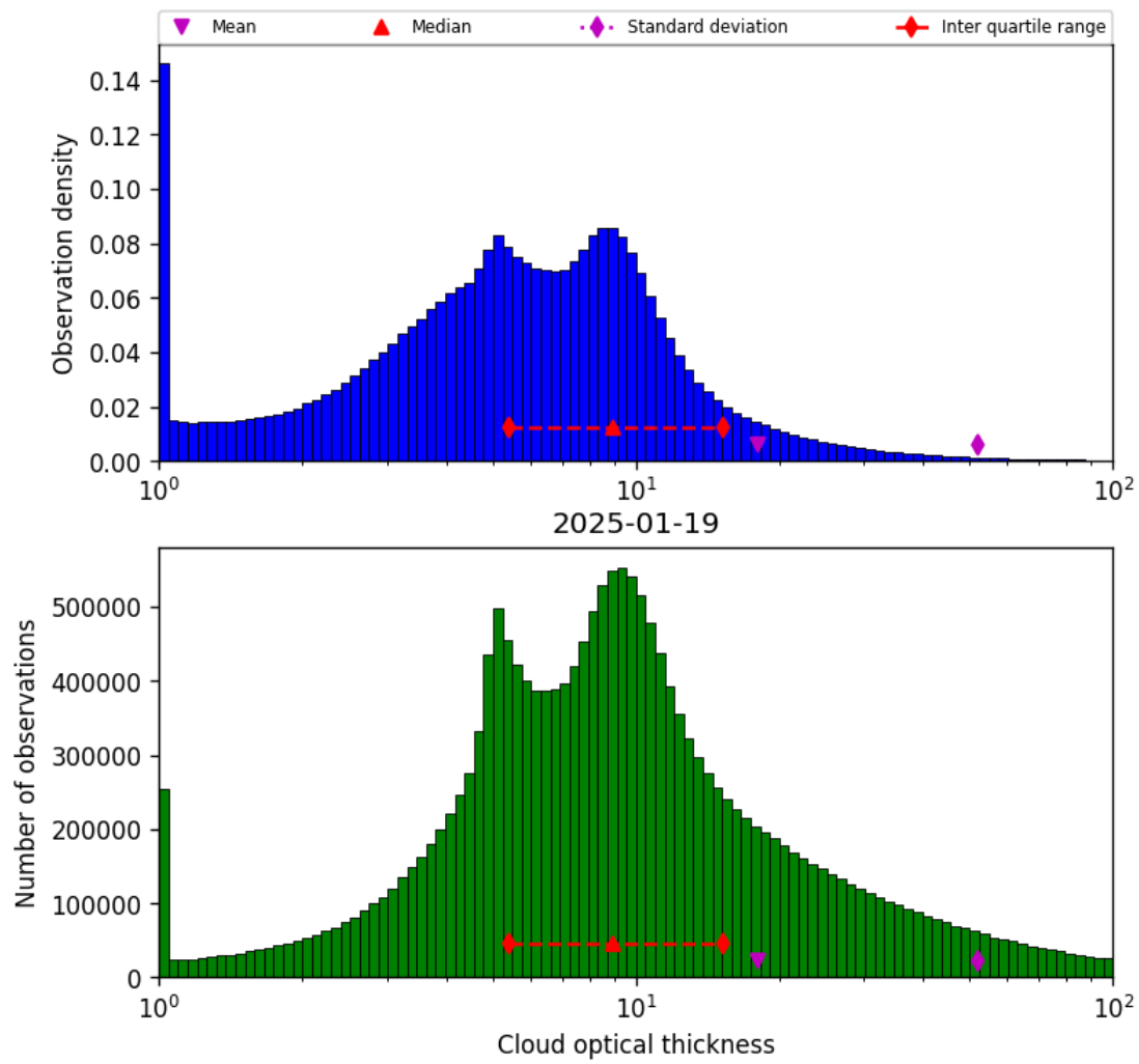
Figure 39: Histogram of “Cloud optical thickness” for 2025-01-19 to 2025-01-20
