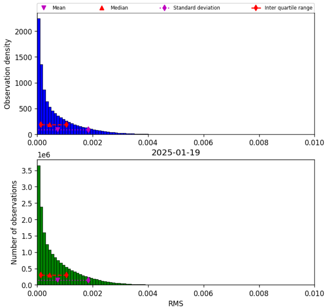
Figure 45: Histogram of “RMS” for 2025-01-19 to 2025-01-20
