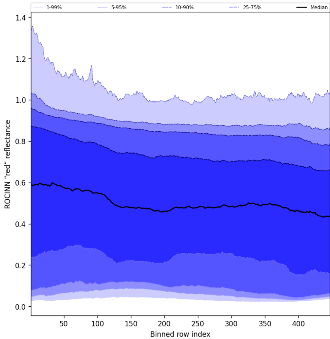
Figure 67: Along track statistics of “ROCINN “red” reflectance” for 2025-01-19 to 2025-01-20
