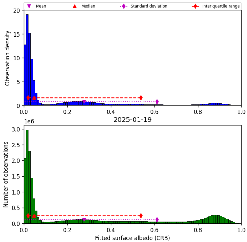
Figure 44: Histogram of “Fitted surface albedo (CRB)” for 2025-01-19 to 2025-01-20
