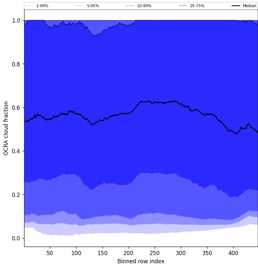
Figure 64: Along track statistics of “OCRA cloud fraction” for 2025-01-19 to 2025-01-20
