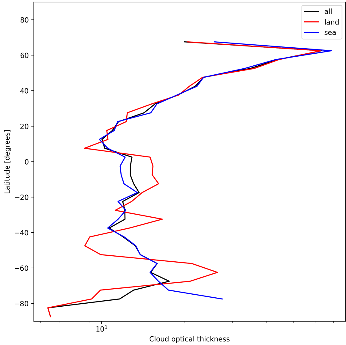
Figure 23: Zonal average of “Cloud optical thickness” for 2025-01-19 to 2025-01-20.
