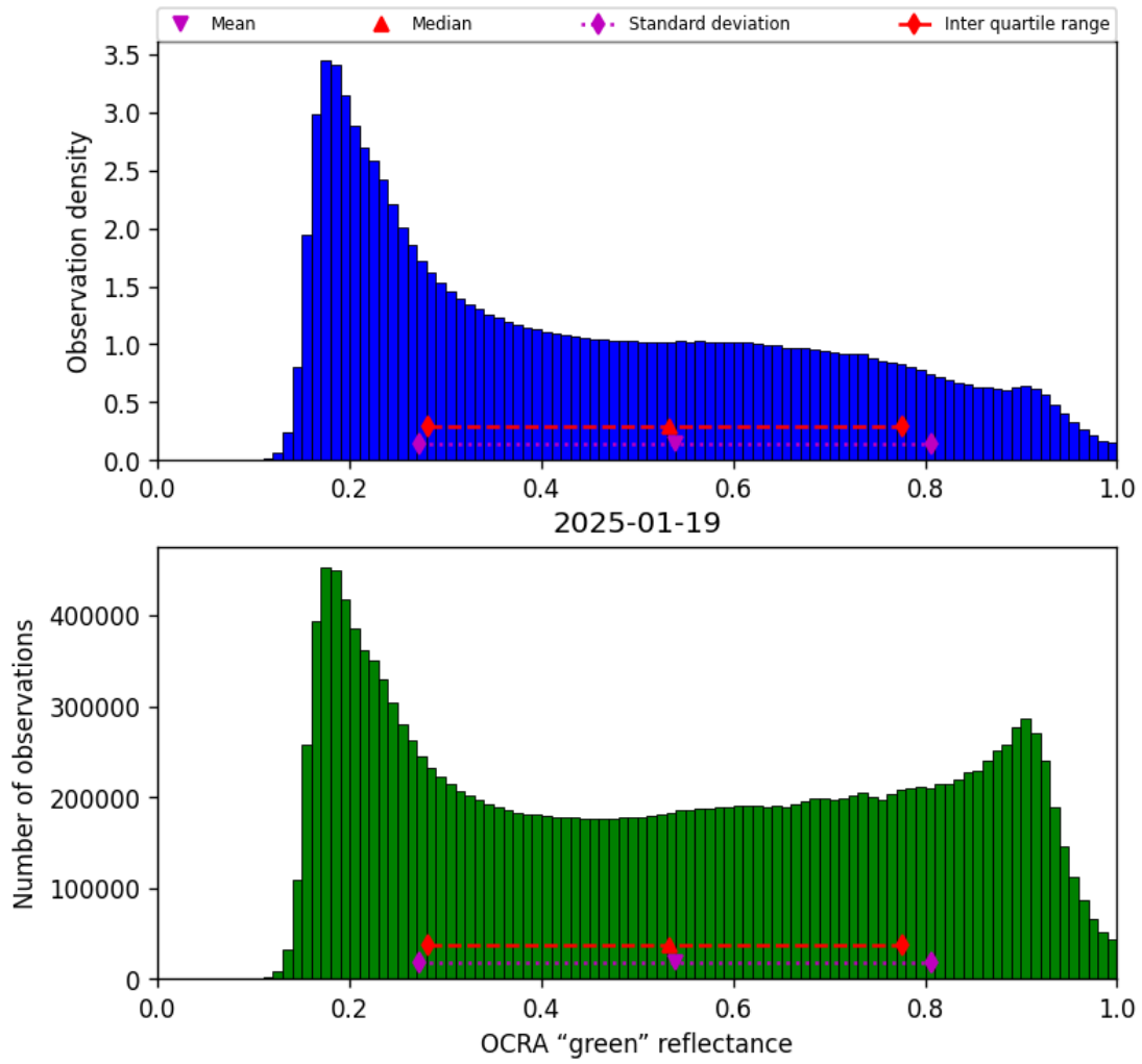
Figure 50: Histogram of “OCRA “green” reflectance” for 2025-01-19 to 2025-01-20
