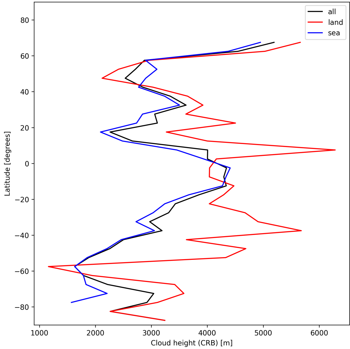
Figure 25: Zonal average of “Cloud height (CRB)” for 2025-01-19 to 2025-01-20.
