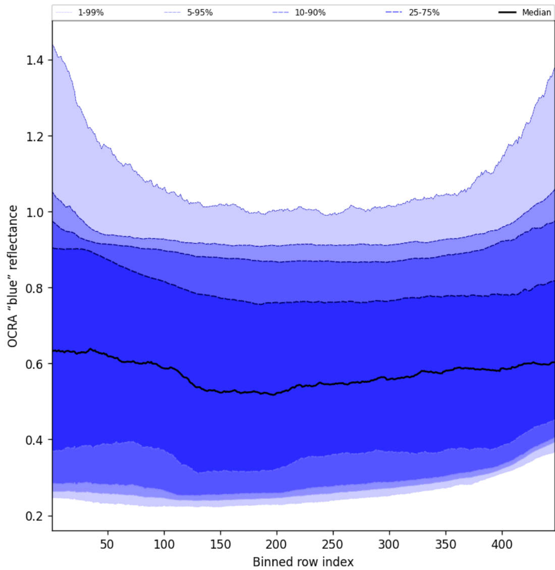
Figure 65: Along track statistics of “OCRA “blue” reflectance” for 2025-01-19 to 2025-01-20
