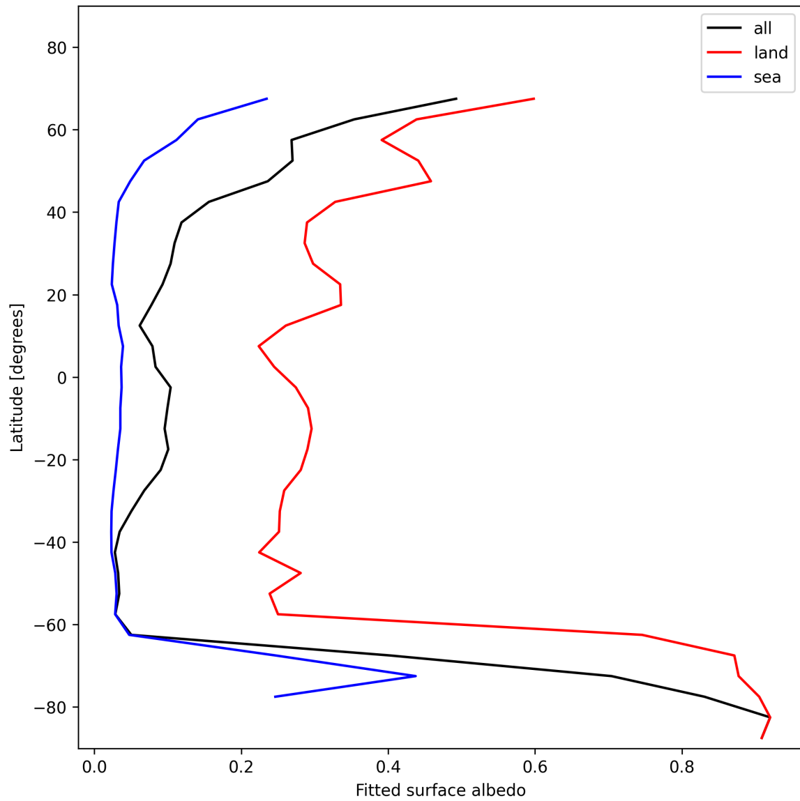
Figure 27: Zonal average of “Fitted surface albedo” for 2025-01-19 to 2025-01-20.
