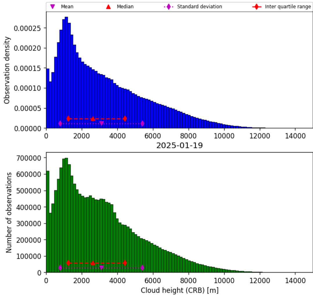
Figure 41: Histogram of “Cloud height (CRB)” for 2025-01-19 to 2025-01-20
