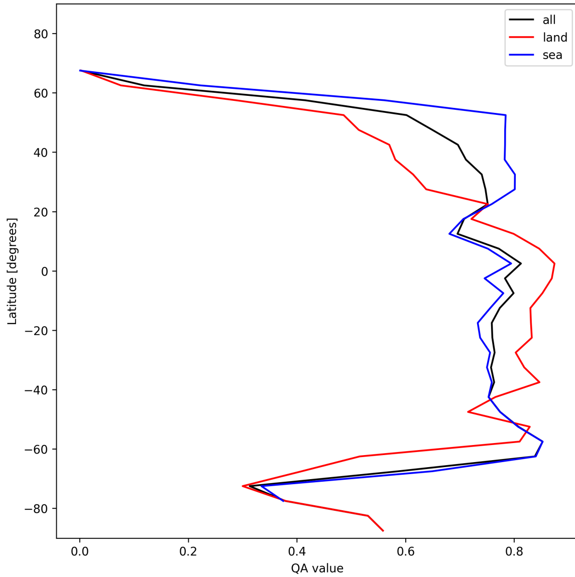
Figure 20: Zonal average of “QA value” for 2025-01-19 to 2025-01-20.
