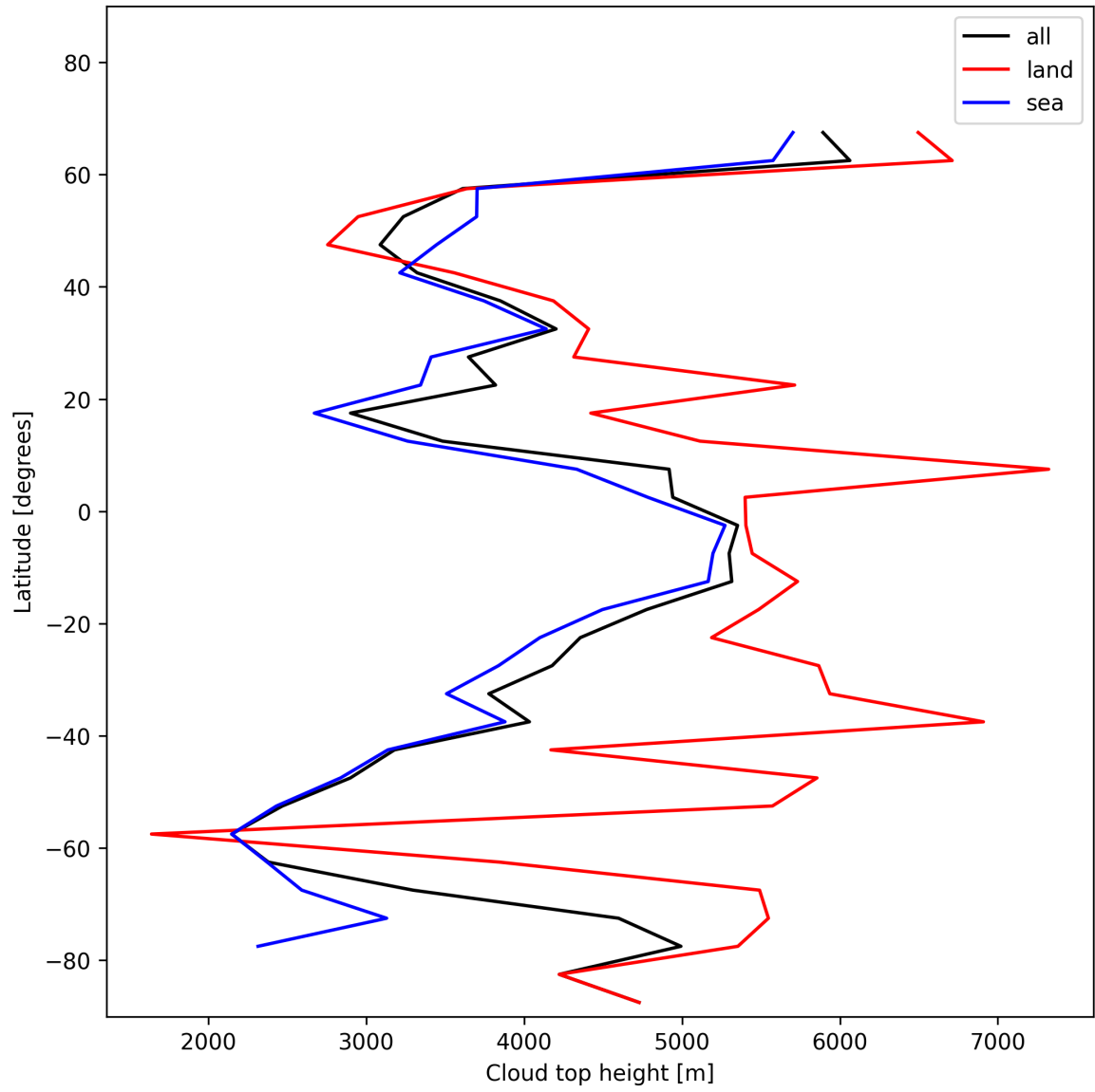
Figure 22: Zonal average of “Cloud top height” for 2025-01-19 to 2025-01-20.
