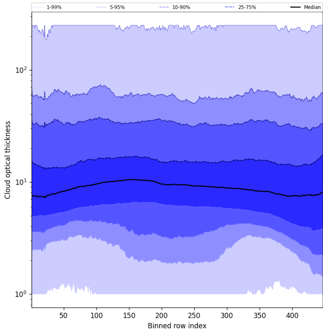
Figure 55: Along track statistics of “Cloud optical thickness” for 2025-01-19 to 2025-01-20
