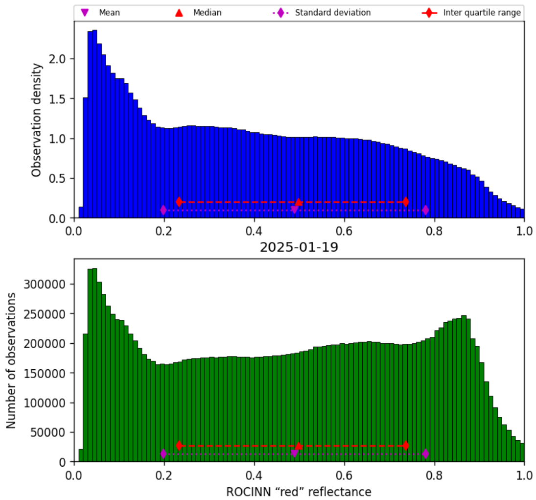
Figure 51: Histogram of “ROCINN “red” reflectance” for 2025-01-19 to 2025-01-20
