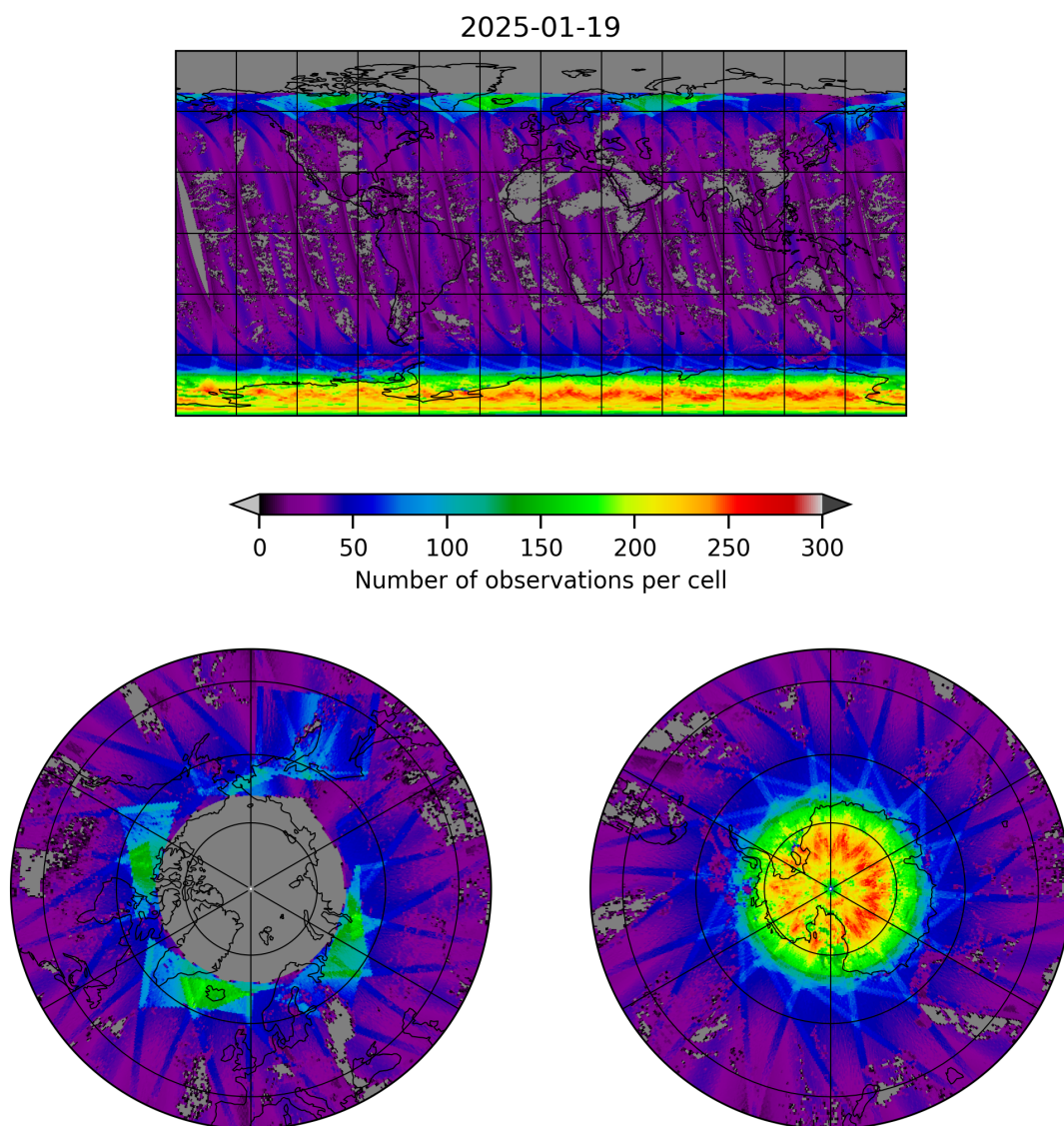
Figure 19: Map of the number of observations for 2025-01-19 to 2025-01-20
