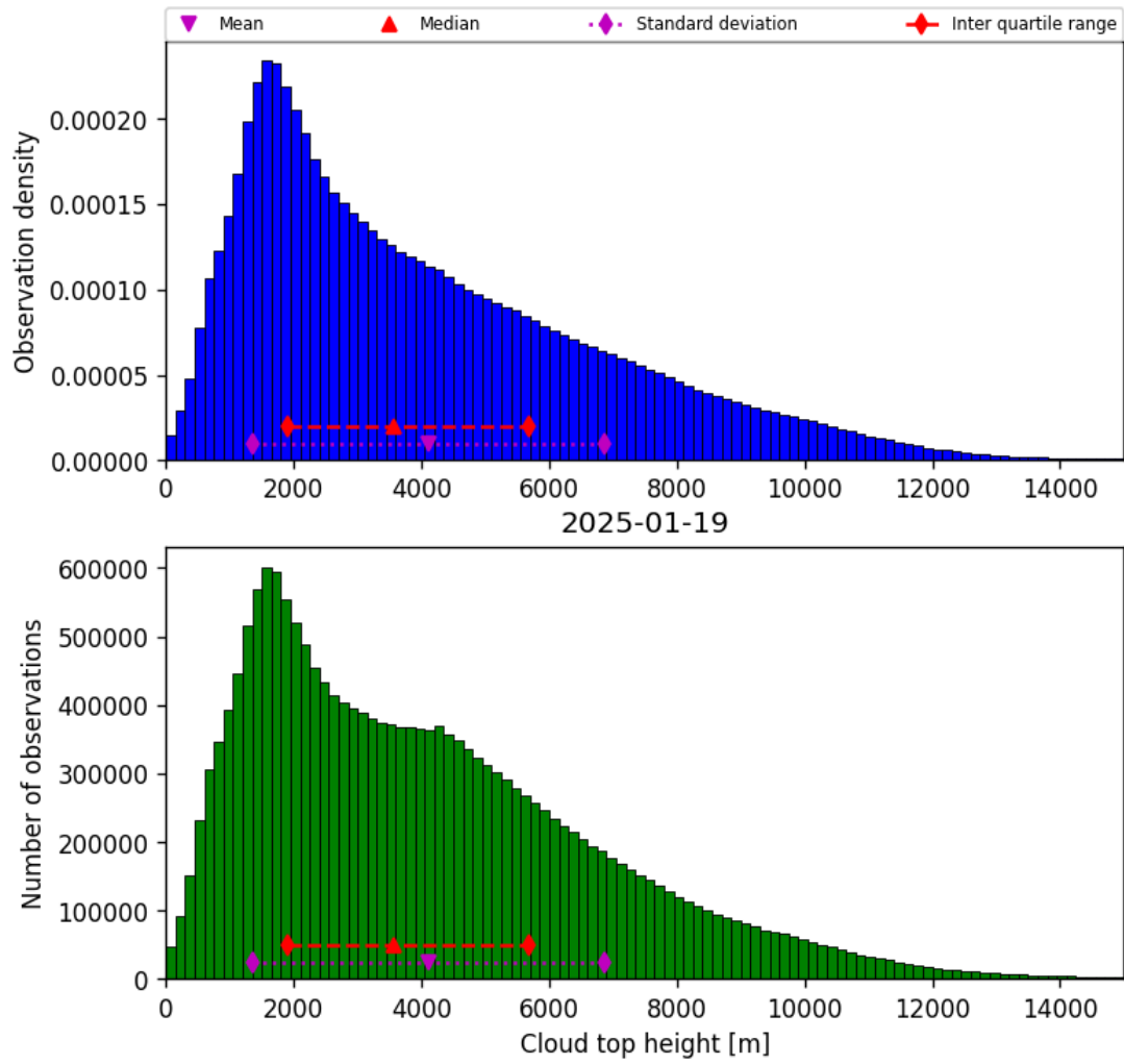
Figure 38: Histogram of “Cloud top height” for 2025-01-19 to 2025-01-20
