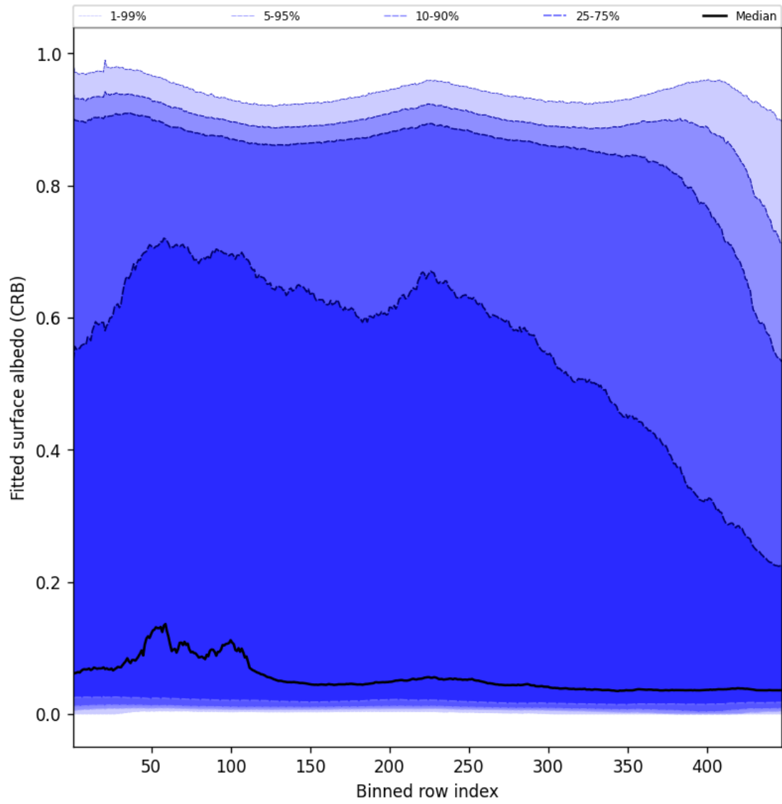
Figure 60: Along track statistics of “Fitted surface albedo (CRB)” for 2025-01-19 to 2025-01-20
