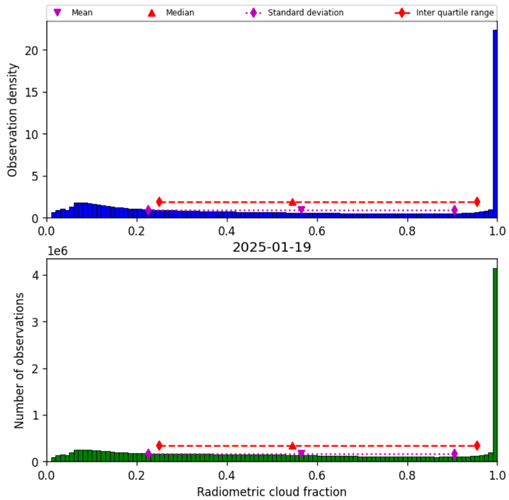
Figure 37: Histogram of “Radiometric cloud fraction” for 2025-01-19 to 2025-01-20
