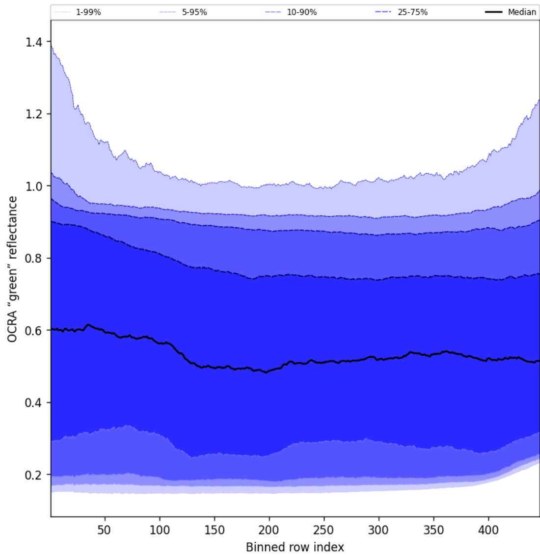
Figure 66: Along track statistics of “OCRA “green” reflectance” for 2025-01-19 to 2025-01-20
