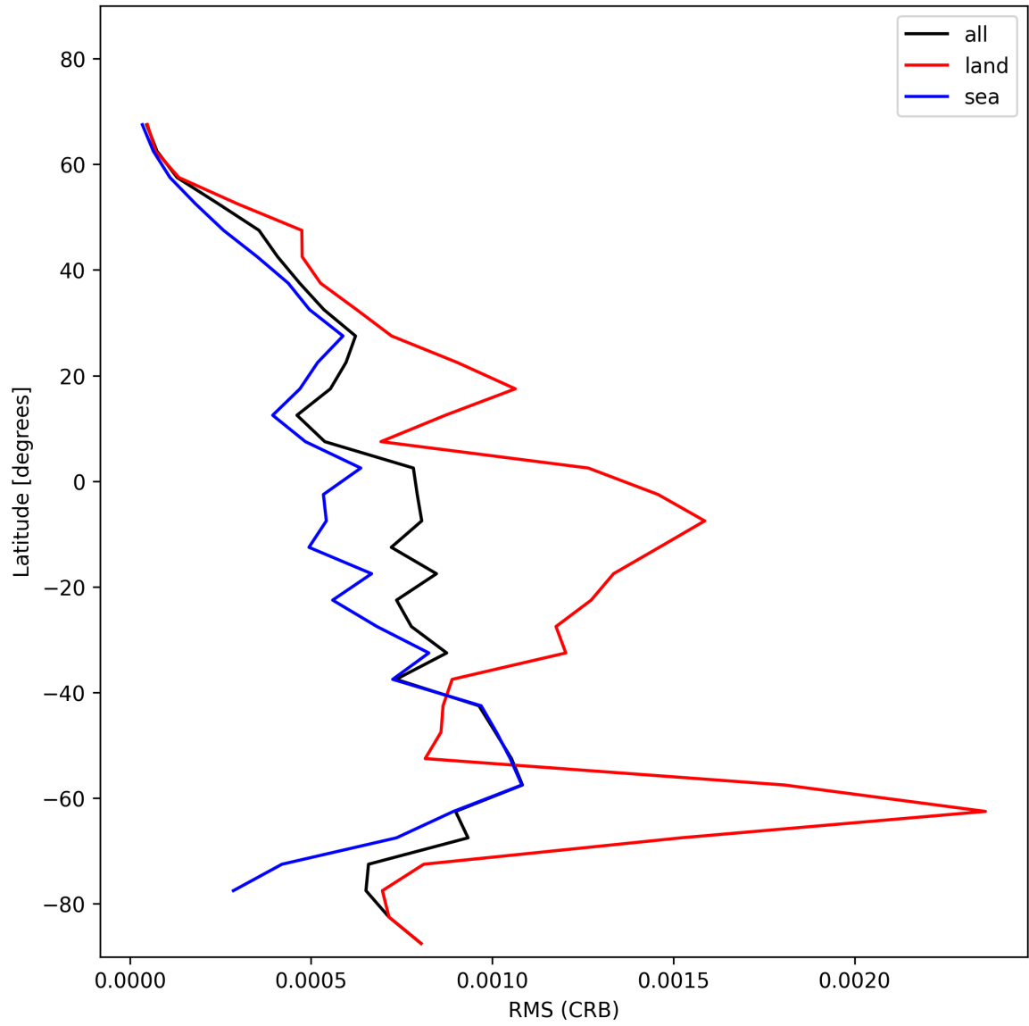
Figure 30: Zonal average of “RMS (CRB)” for 2025-01-19 to 2025-01-20.
