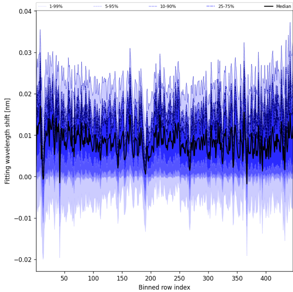
Figure 63: Along track statistics of “Fitting wavelength shift” for 2025-01-19 to 2025-01-20
