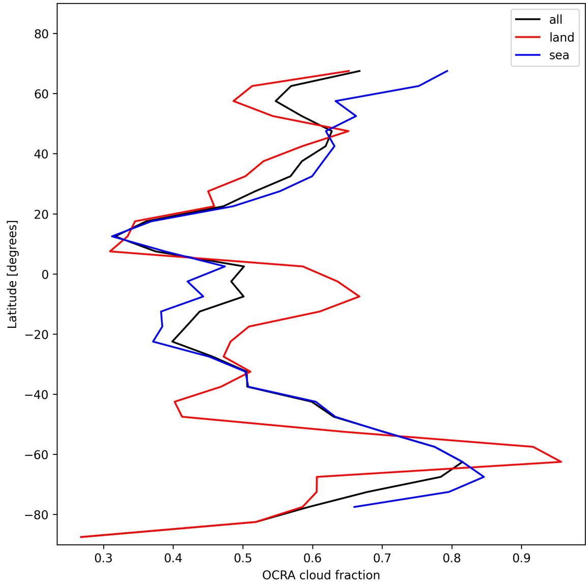
Figure 32: Zonal average of “OCRA cloud fraction” for 2025-01-19 to 2025-01-20.
