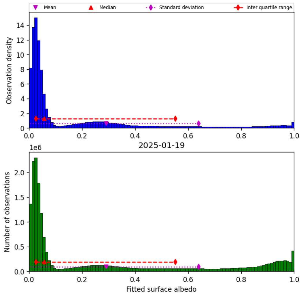
Figure 43: Histogram of “Fitted surface albedo” for 2025-01-19 to 2025-01-20
