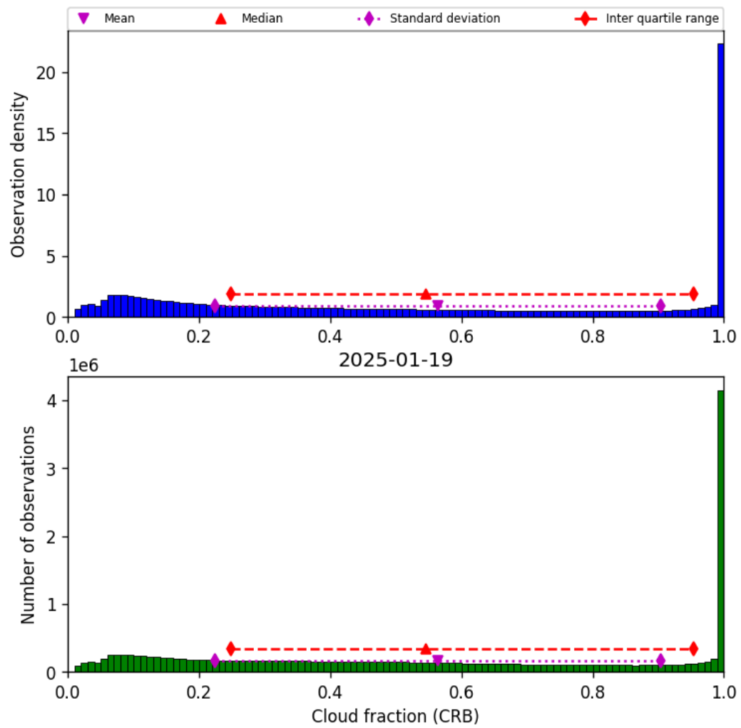
Figure 40: Histogram of “Cloud fraction (CRB)” for 2025-01-19 to 2025-01-20
