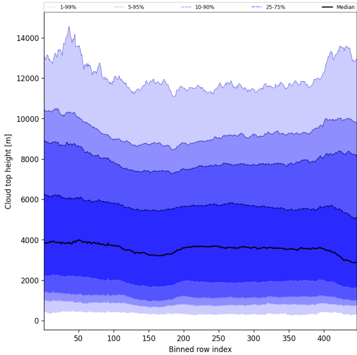
Figure 54: Along track statistics of “Cloud top height” for 2025-01-19 to 2025-01-20
