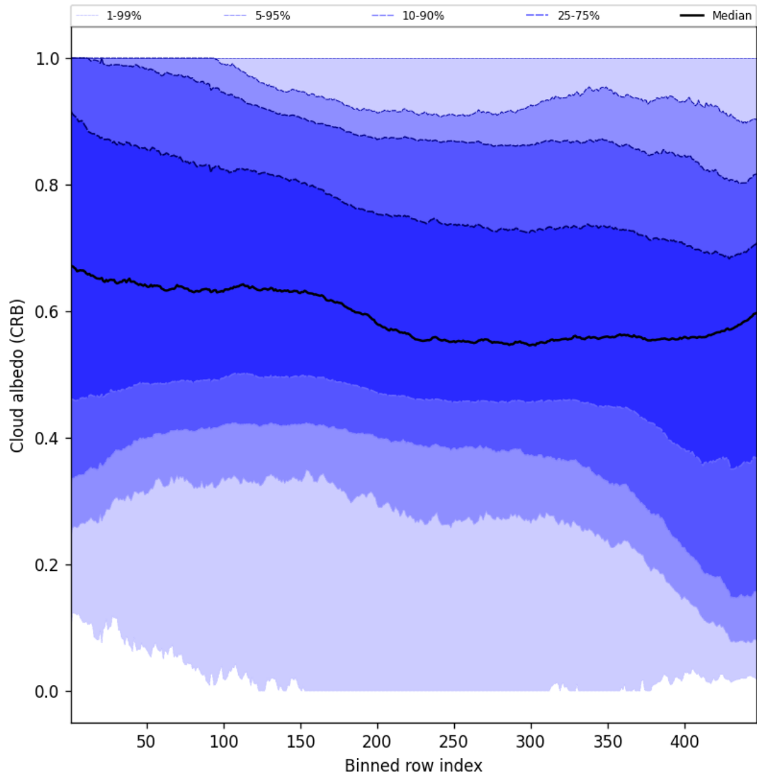
Figure 58: Along track statistics of “Cloud albedo (CRB)” for 2025-01-19 to 2025-01-20
