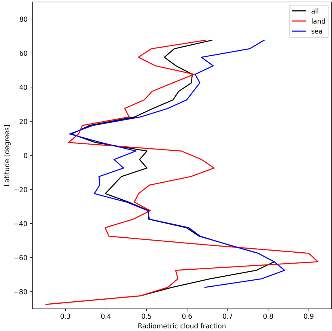
Figure 21: Zonal average of “Radiometric cloud fraction” for 2025-01-19 to 2025-01-20.
