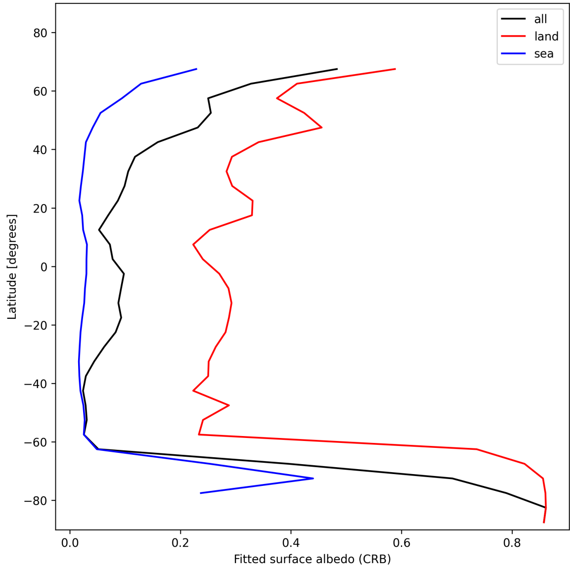
Figure 28: Zonal average of “Fitted surface albedo (CRB)” for 2025-01-19 to 2025-01-20.
