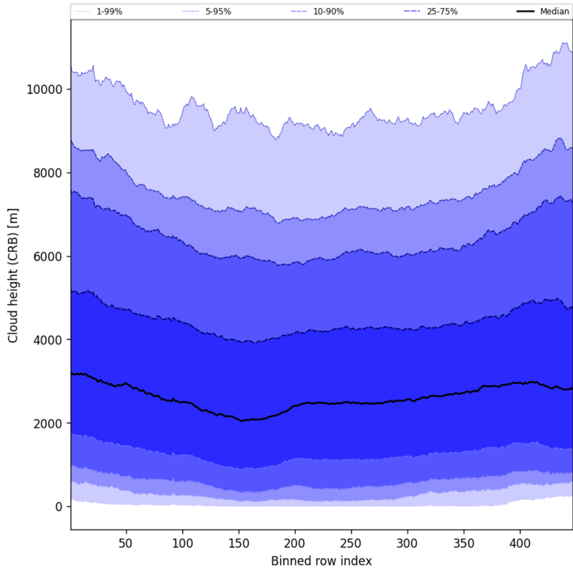
Figure 57: Along track statistics of “Cloud height (CRB)” for 2025-01-19 to 2025-01-20
