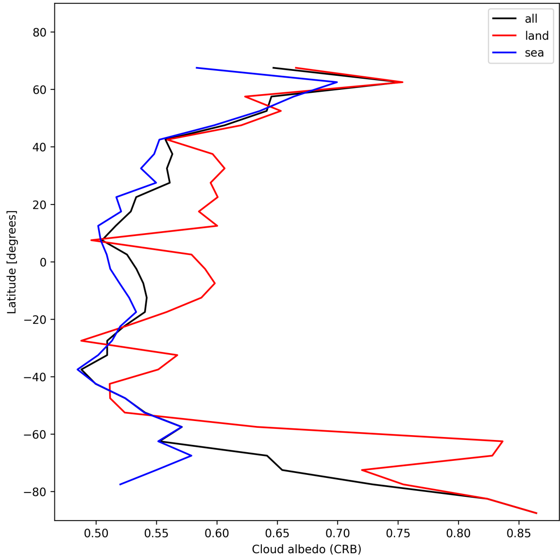
Figure 26: Zonal average of “Cloud albedo (CRB)” for 2025-01-19 to 2025-01-20.
