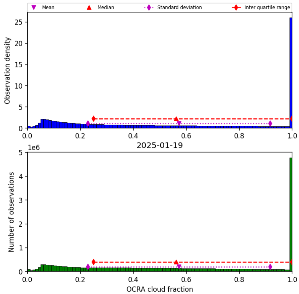
Figure 48: Histogram of “OCRA cloud fraction” for 2025-01-19 to 2025-01-20
