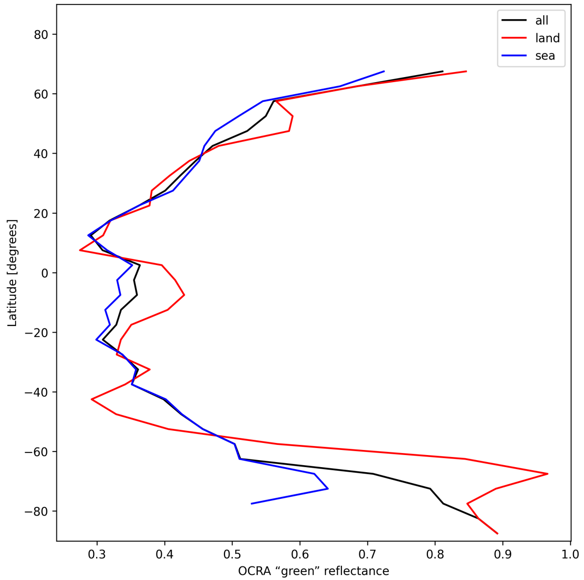
Figure 34: Zonal average of “OCRA “green” reflectance” for 2025-01-19 to 2025-01-20.
