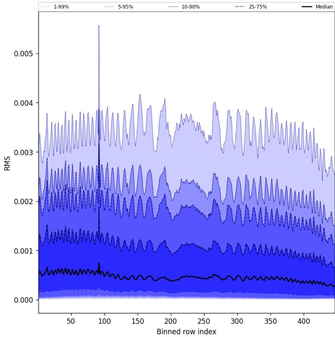
Figure 61: Along track statistics of “RMS” for 2025-01-19 to 2025-01-20
