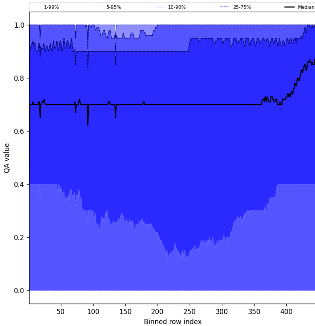
Figure 52: Along track statistics of “QA value” for 2025-01-19 to 2025-01-20
