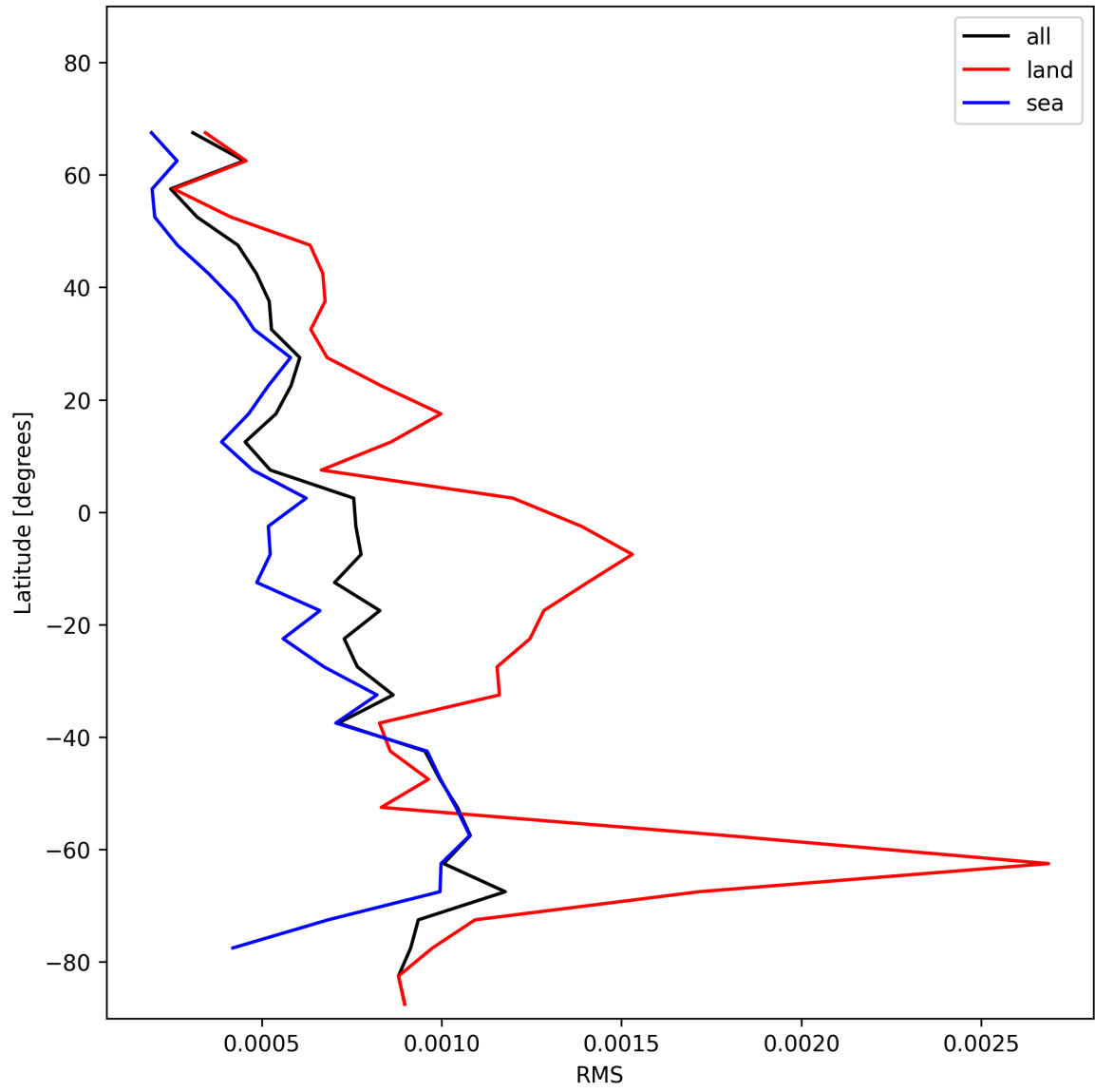
Figure 29: Zonal average of “RMS” for 2025-01-19 to 2025-01-20.
