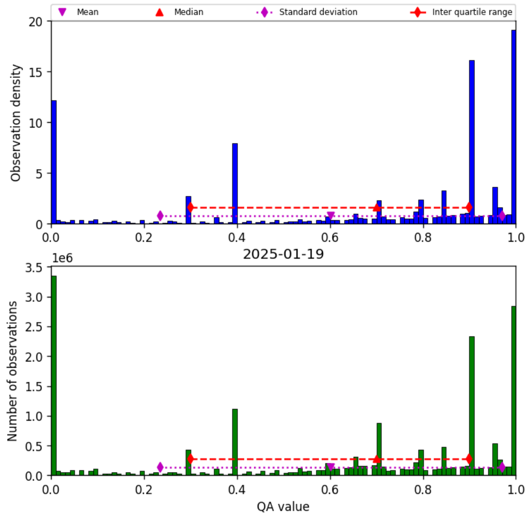
Figure 36: Histogram of “QA value” for 2025-01-19 to 2025-01-20
