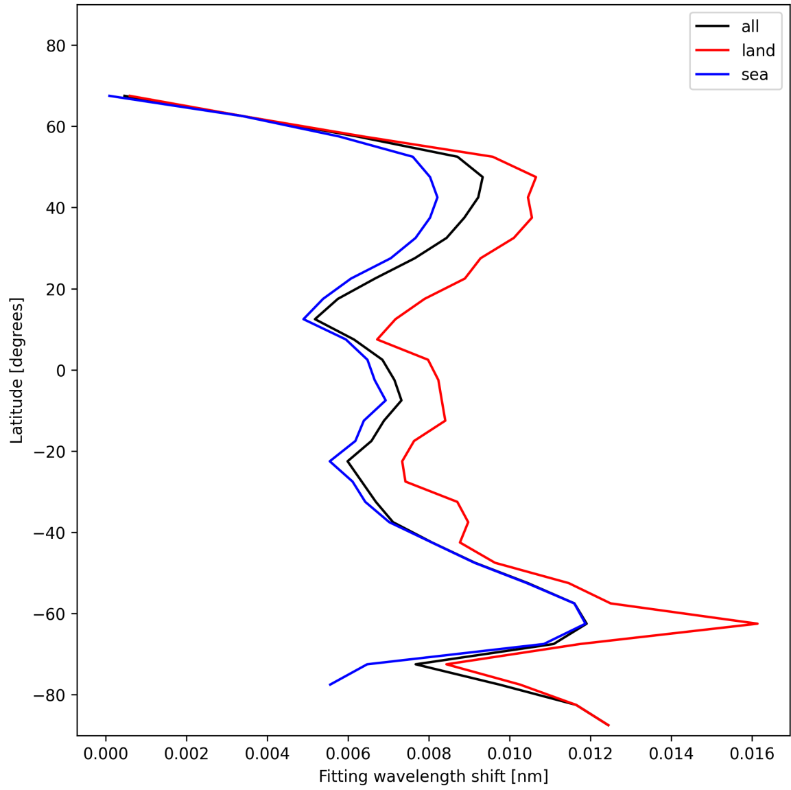
Figure 31: Zonal average of “Fitting wavelength shift” for 2025-01-19 to 2025-01-20.
