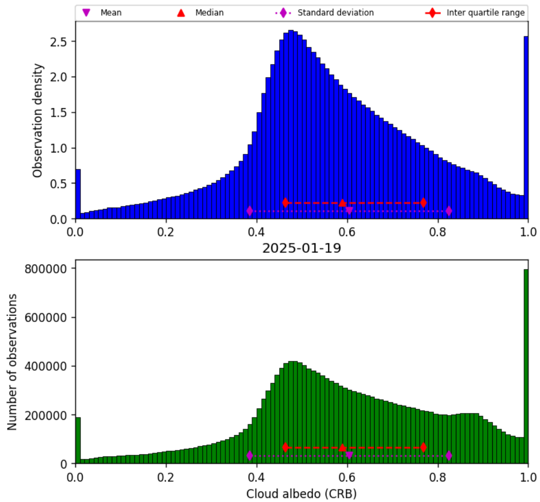
Figure 42: Histogram of “Cloud albedo (CRB)” for 2025-01-19 to 2025-01-20
