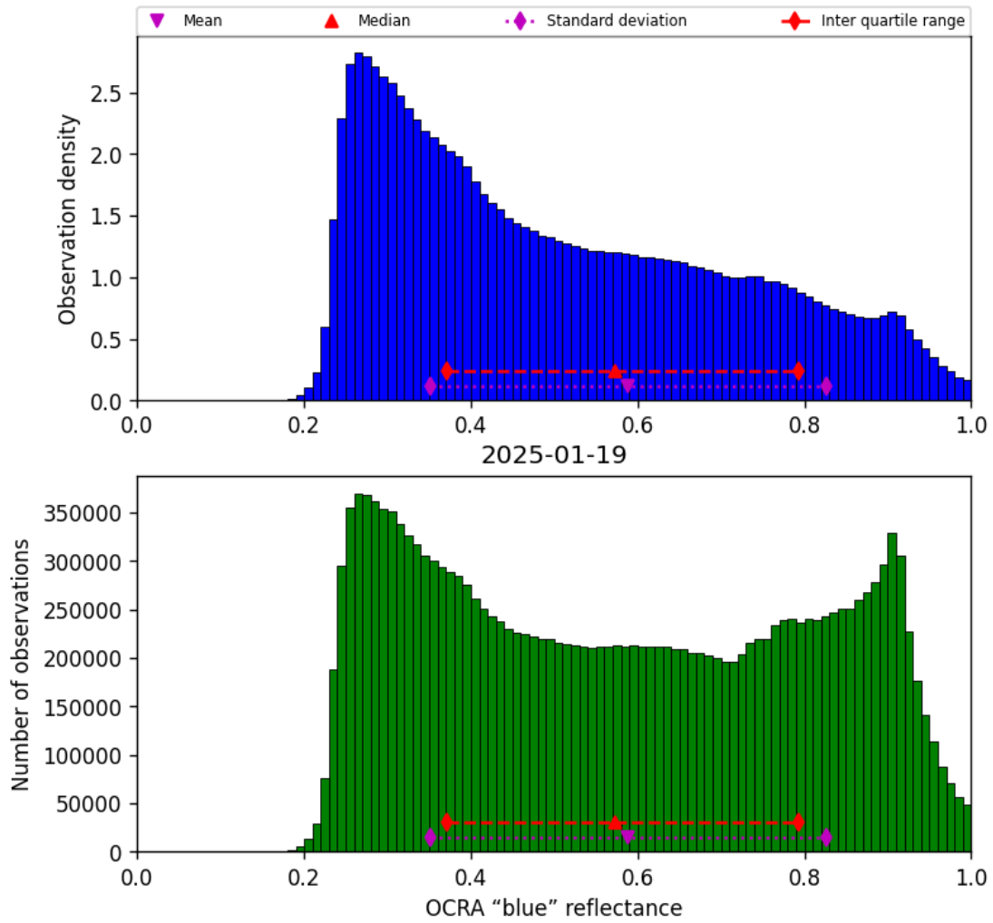
Figure 49: Histogram of “OCRA “blue” reflectance” for 2025-01-19 to 2025-01-20
