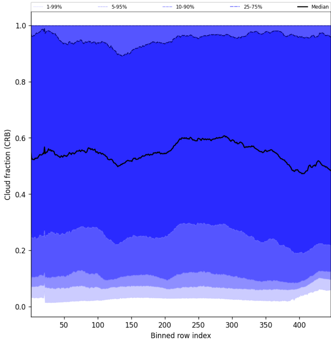
Figure 56: Along track statistics of “Cloud fraction (CRB)” for 2025-01-19 to 2025-01-20
