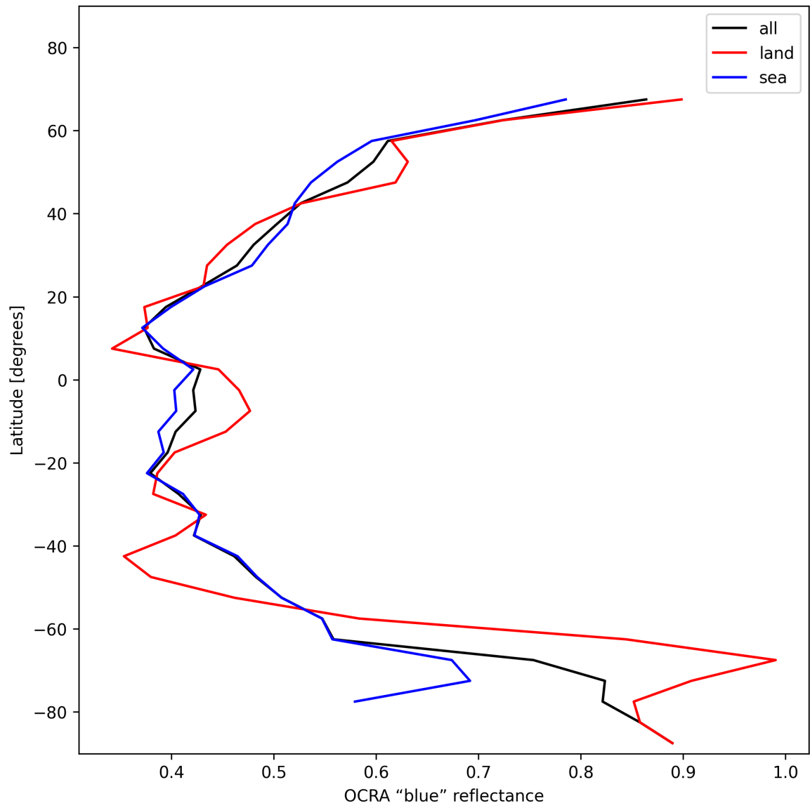
Figure 33: Zonal average of “OCRA “blue” reflectance” for 2025-01-19 to 2025-01-20.
