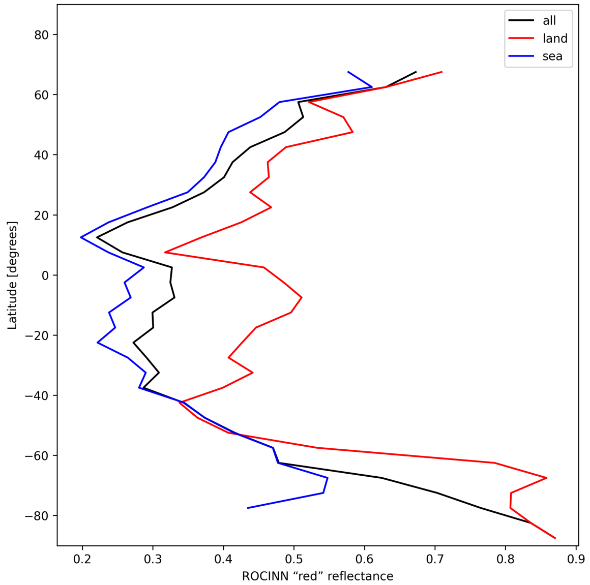
Figure 35: Zonal average of "ROCINN "red" reflectance" for 2025-01-19 to 2025-01-20.
