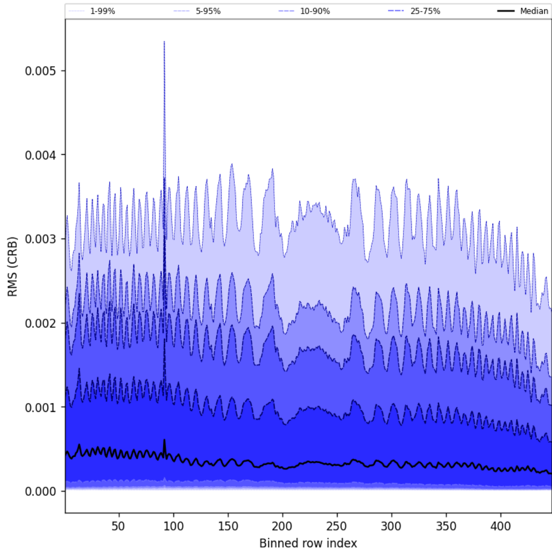
Figure 62: Along track statistics of “RMS (CRB)” for 2025-01-19 to 2025-01-20
