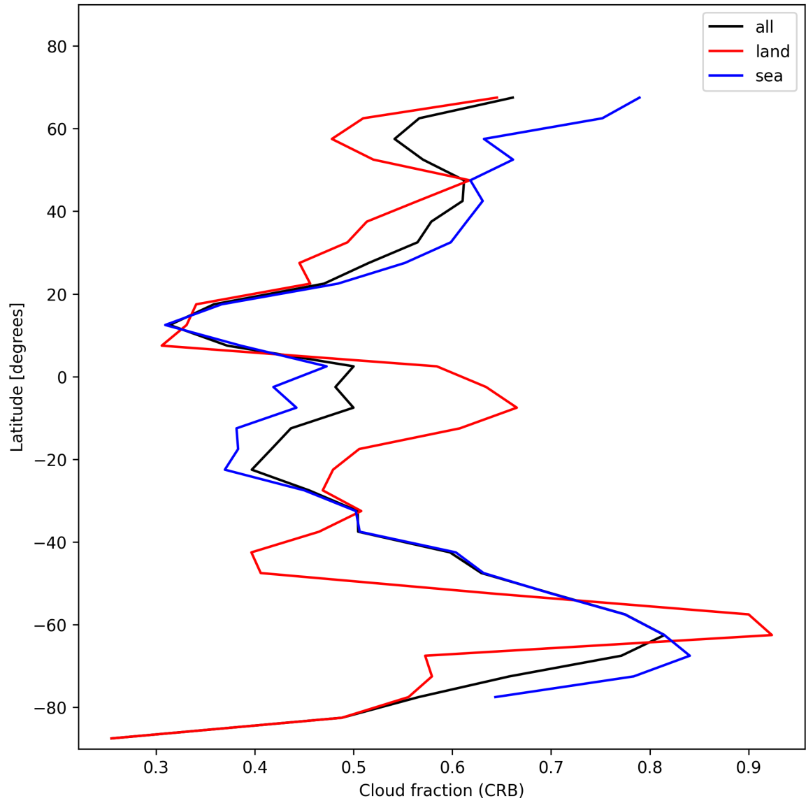
Figure 24: Zonal average of “Cloud fraction (CRB)” for 2025-01-19 to 2025-01-20.
