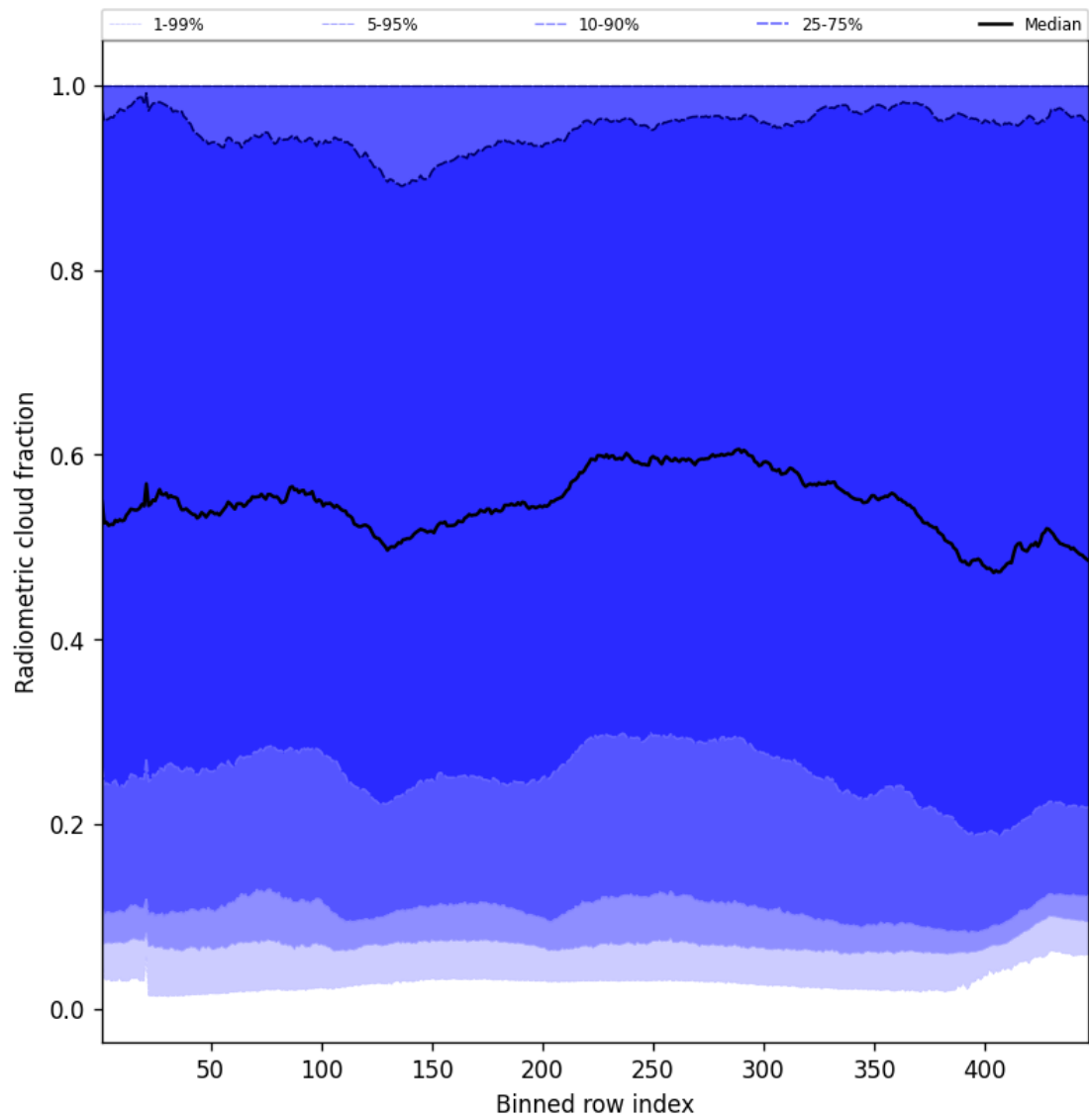
Figure 53: Along track statistics of “Radiometric cloud fraction” for 2025-01-19 to 2025-01-20
