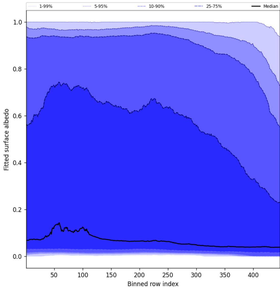
Figure 59: Along track statistics of “Fitted surface albedo” for 2025-01-19 to 2025-01-20
