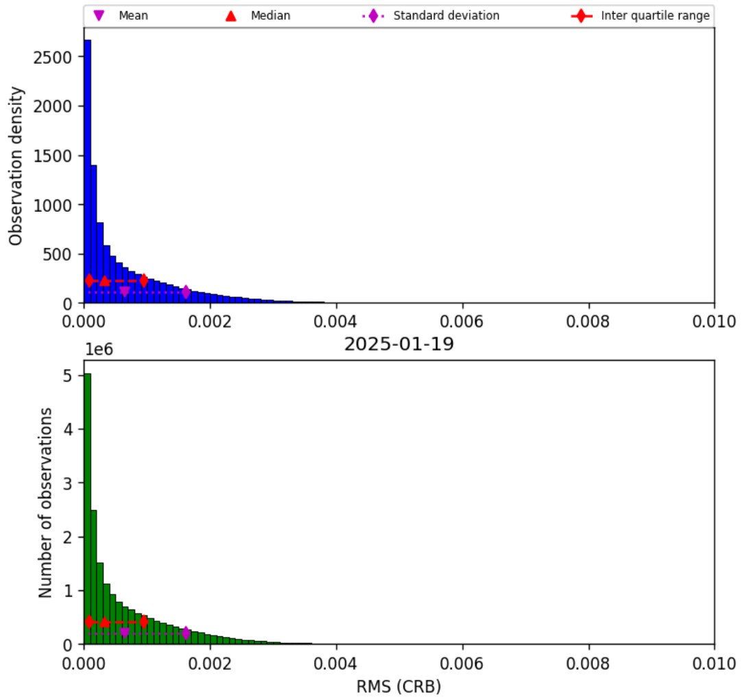
Figure 46: Histogram of "RMS (CRB)" for 2025-01-19 to 2025-01-20
