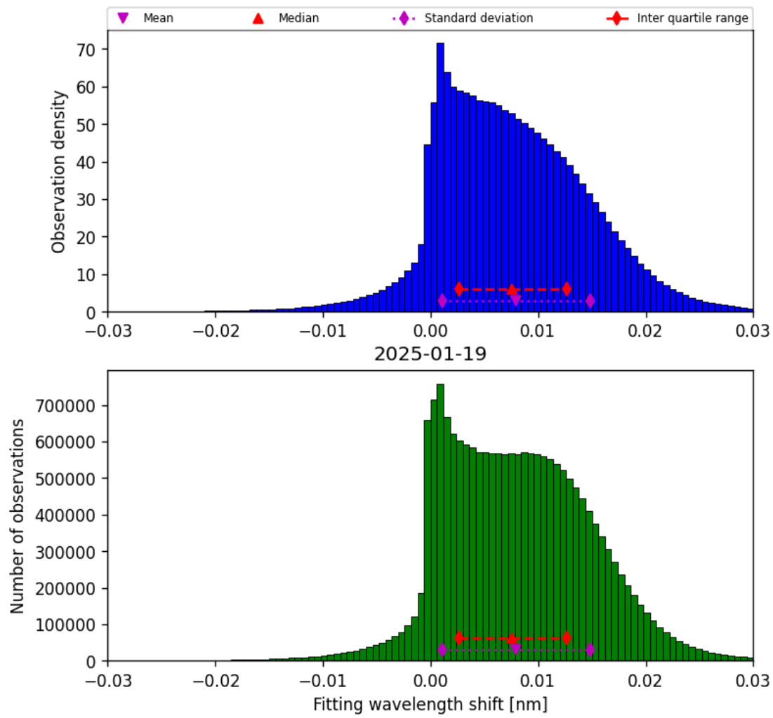
Figure 47: Histogram of “Fitting wavelength shift” for 2025-01-19 to 2025-01-20
