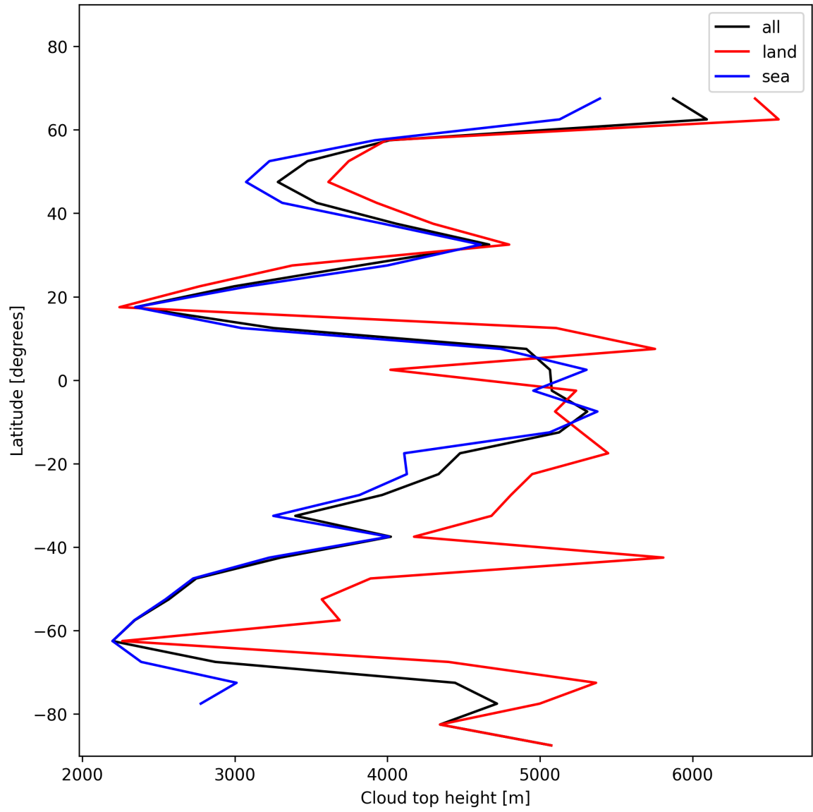
Figure 22: Zonal average of “Cloud top height” for 2025-01-21 to 2025-01-21.
