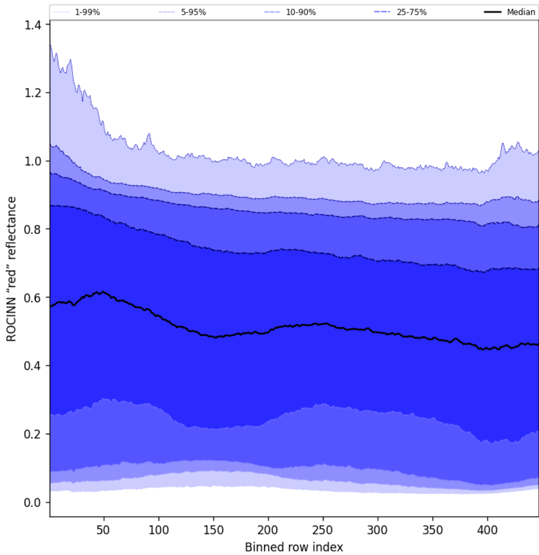
Figure 67: Along track statistics of “ROCINN “red” reflectance” for 2025-01-21 to 2025-01-21
