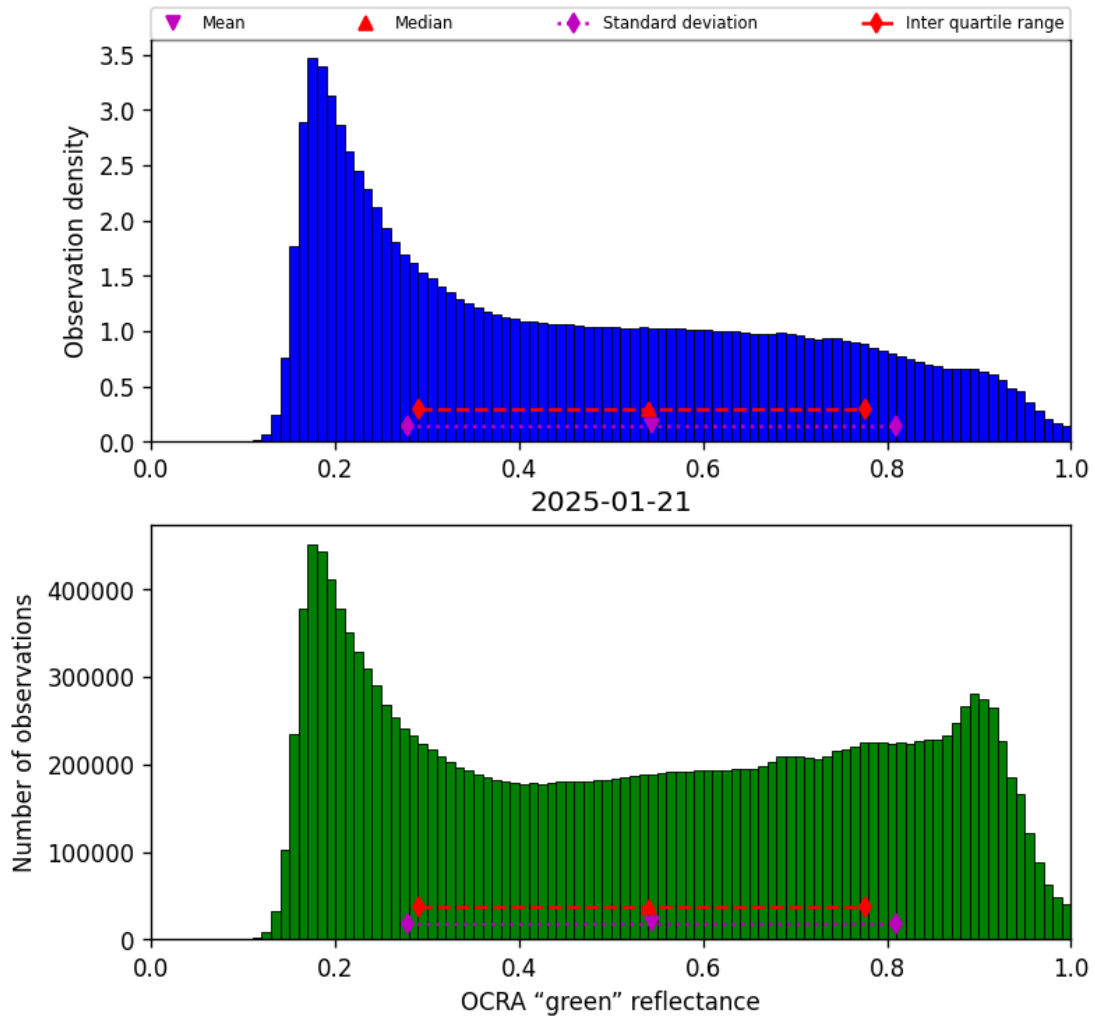
Figure 50: Histogram of “OCRA “green” reflectance” for 2025-01-21 to 2025-01-21
