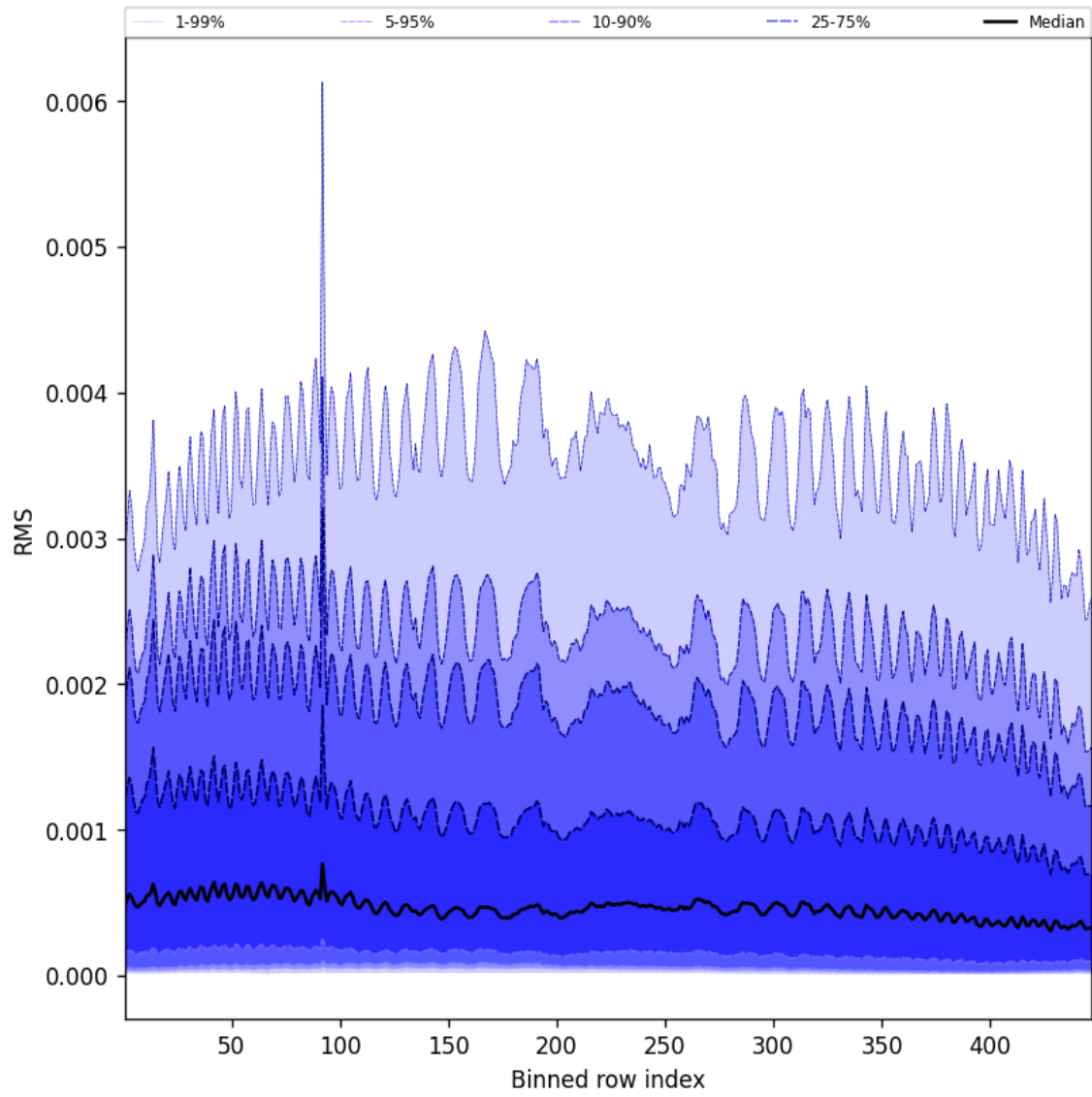
Figure 61: Along track statistics of “RMS” for 2025-01-21 to 2025-01-21
