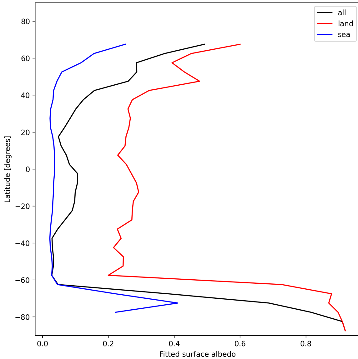
Figure 27: Zonal average of “Fitted surface albedo” for 2025-01-21 to 2025-01-21.
