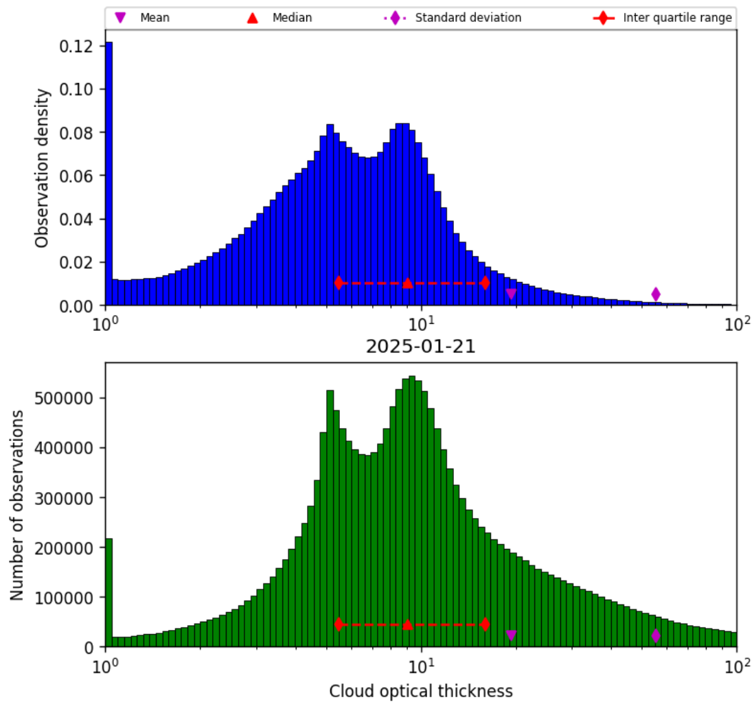
Figure 39: Histogram of “Cloud optical thickness” for 2025-01-21 to 2025-01-21
