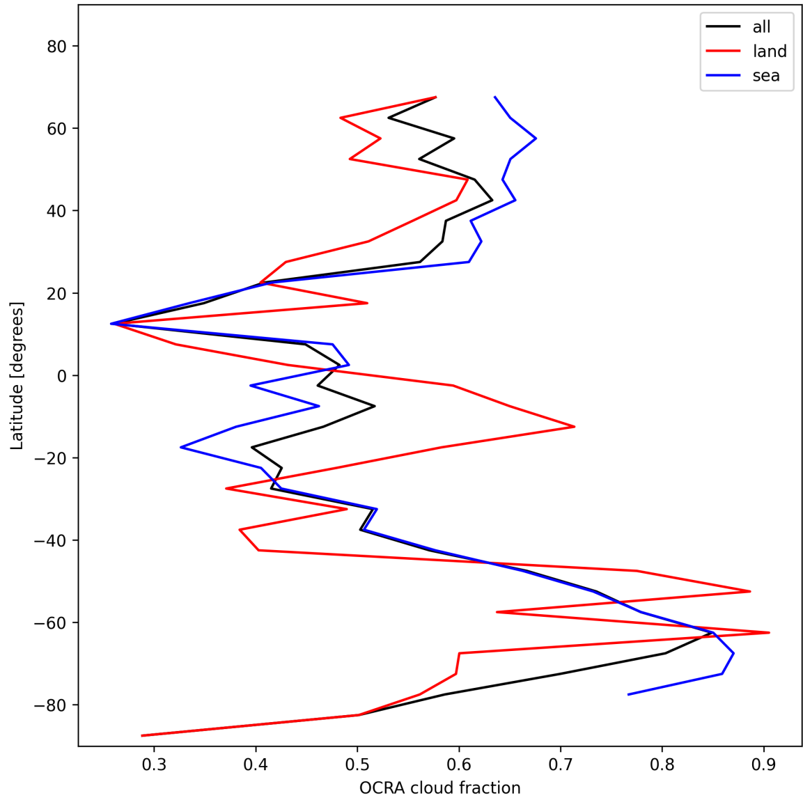
Figure 32: Zonal average of “OCRA cloud fraction” for 2025-01-21 to 2025-01-21.
