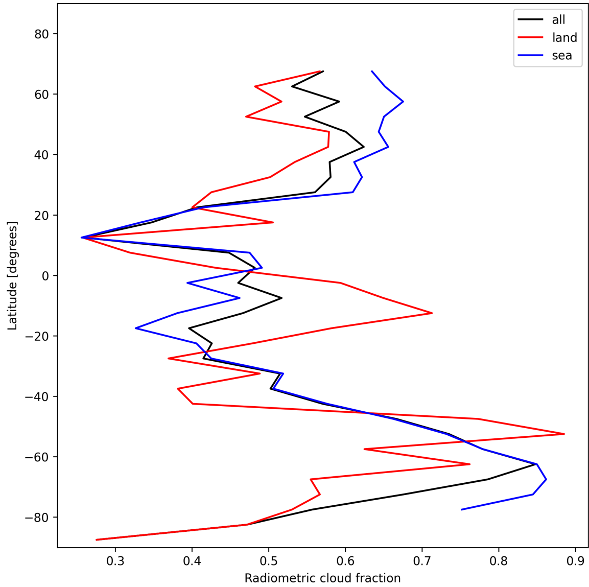
Figure 21: Zonal average of “Radiometric cloud fraction” for 2025-01-21 to 2025-01-21.
