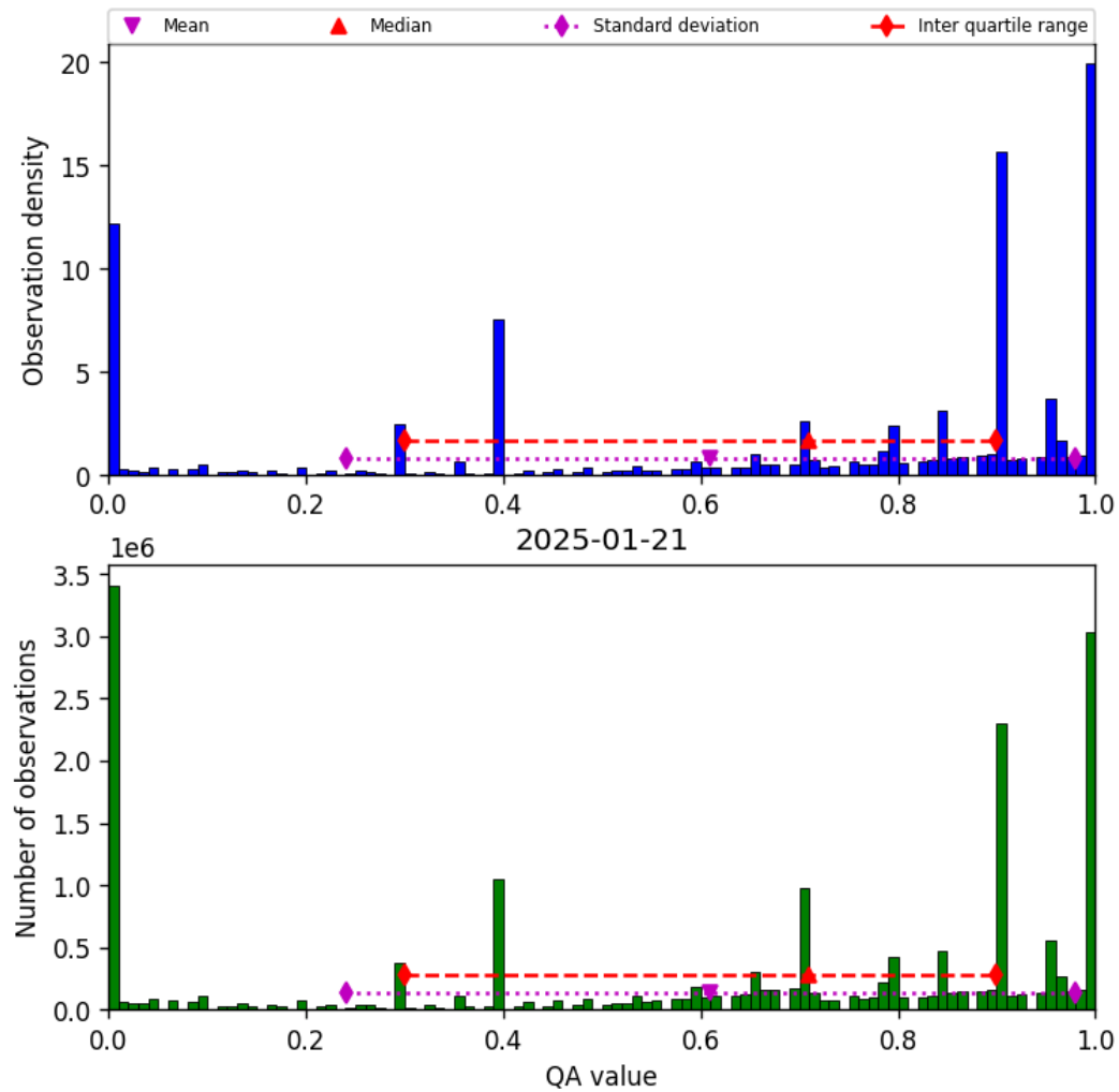
Figure 36: Histogram of “QA value” for 2025-01-21 to 2025-01-21
