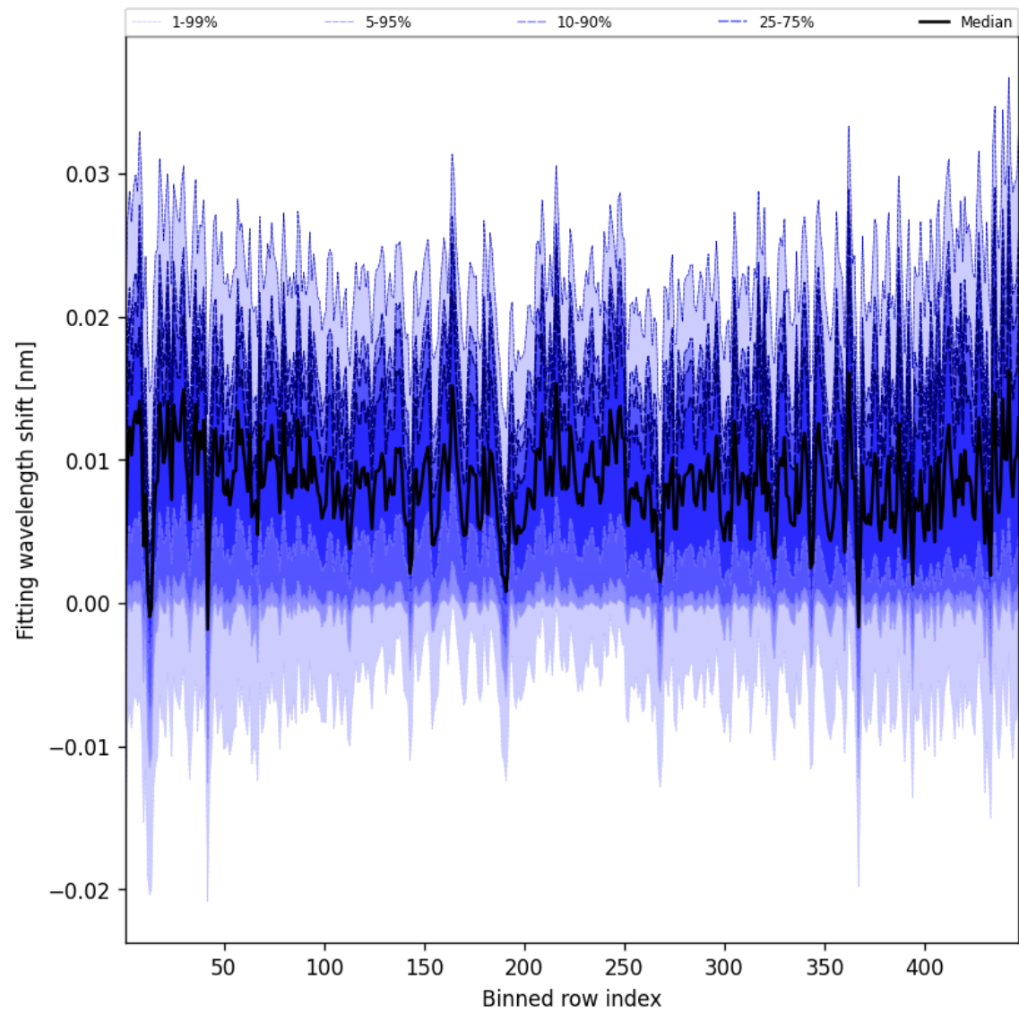
Figure 63: Along track statistics of “Fitting wavelength shift” for 2025-01-21 to 2025-01-21
