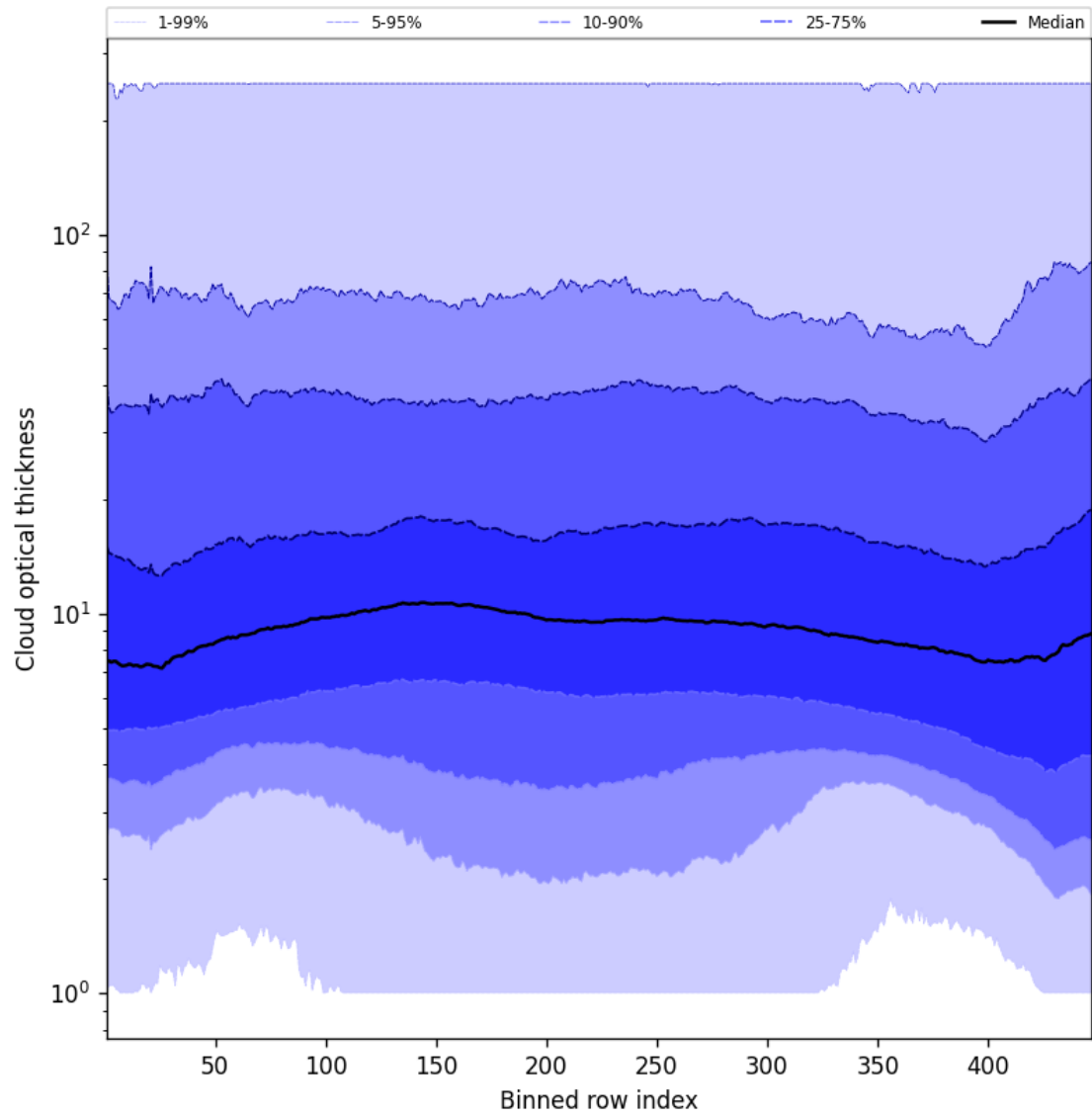
Figure 55: Along track statistics of “Cloud optical thickness” for 2025-01-21 to 2025-01-21
