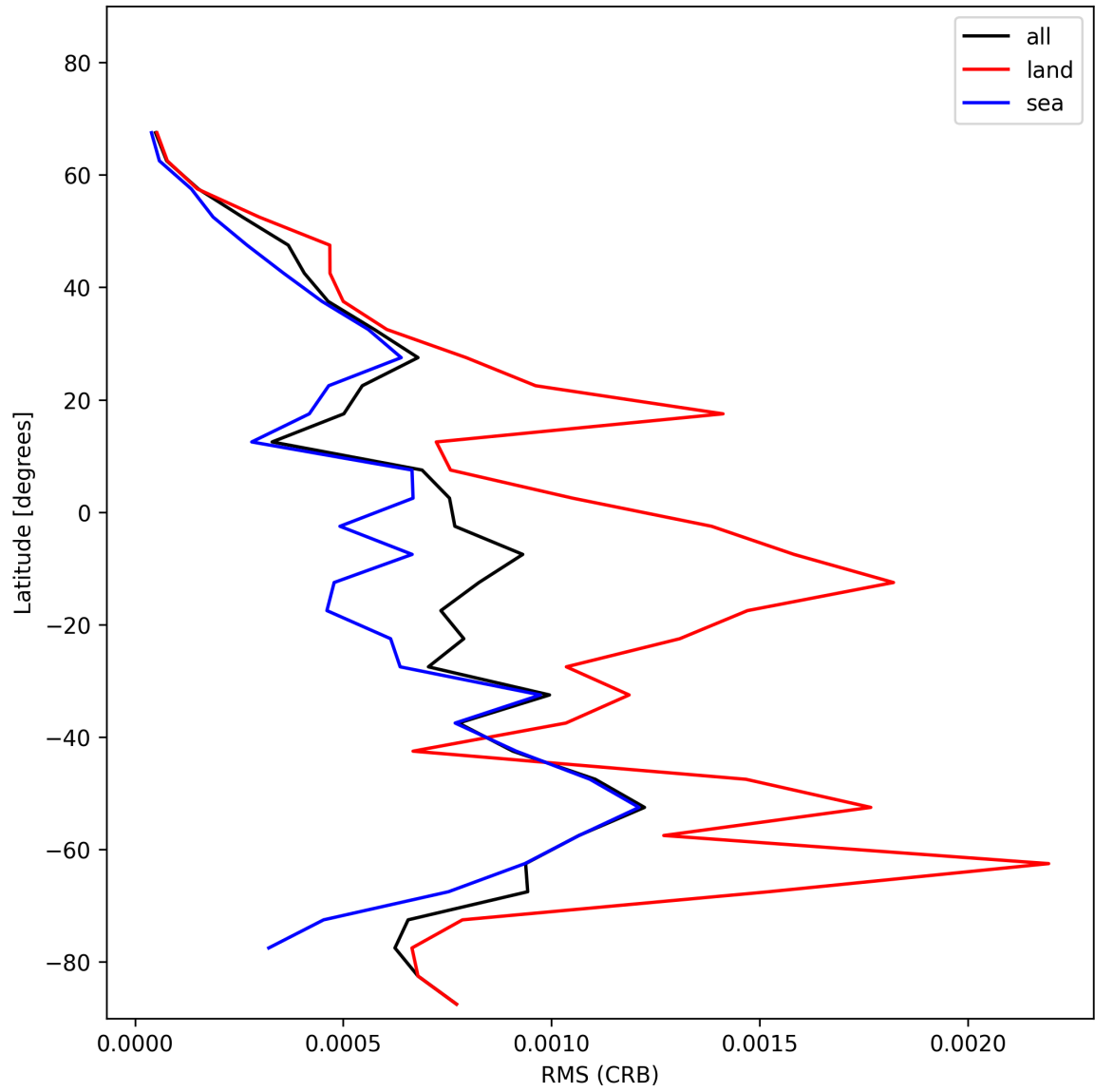
Figure 30: Zonal average of “RMS (CRB)” for 2025-01-21 to 2025-01-21.
