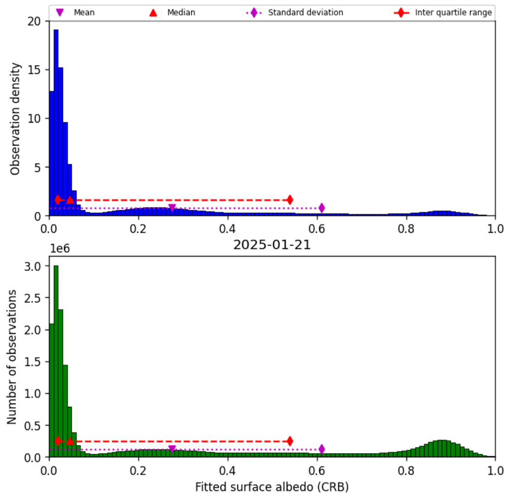
Figure 44: Histogram of “Fitted surface albedo (CRB)” for 2025-01-21 to 2025-01-21
