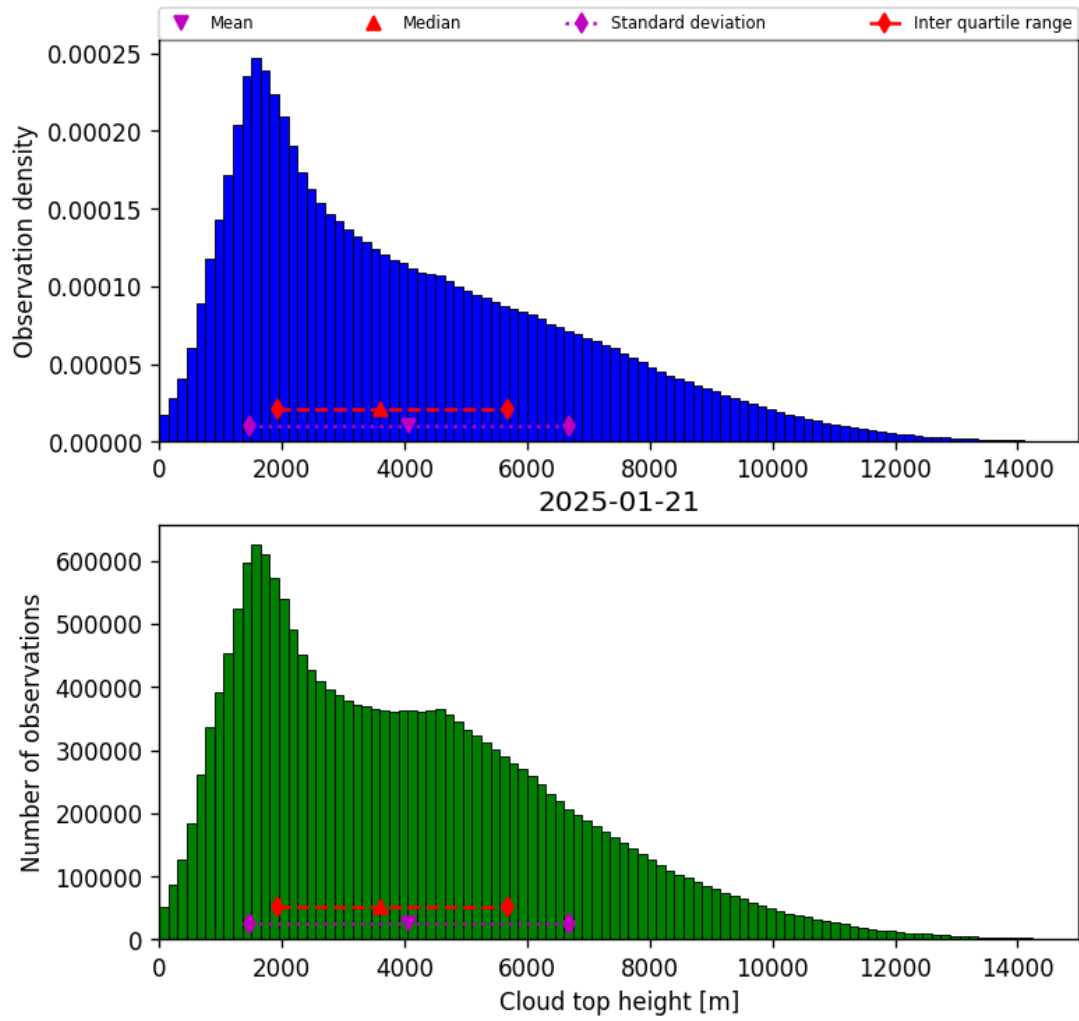
Figure 38: Histogram of “Cloud top height” for 2025-01-21 to 2025-01-21
