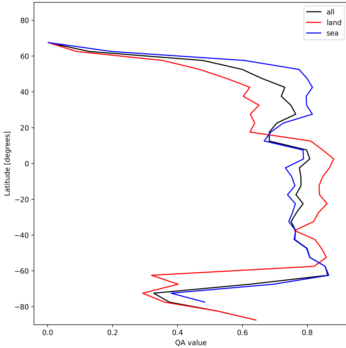
Figure 20: Zonal average of “QA value” for 2025-01-21 to 2025-01-21.
