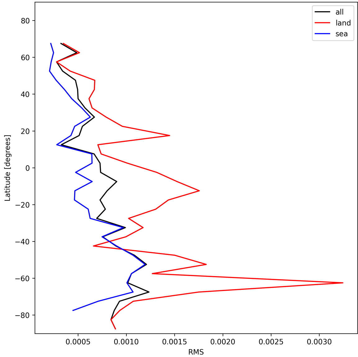
Figure 29: Zonal average of “RMS” for 2025-01-21 to 2025-01-21.
