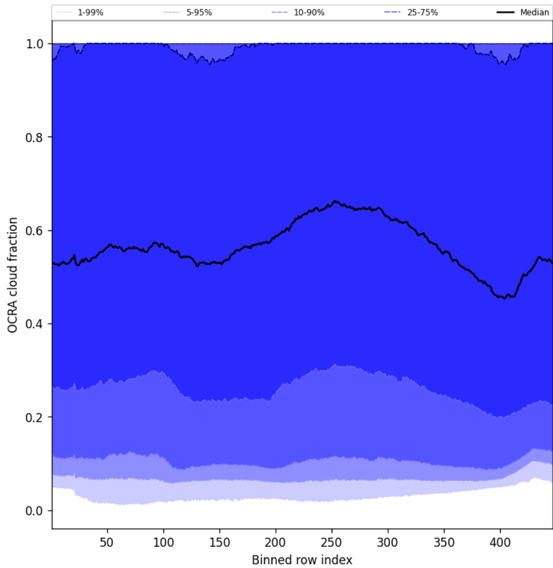
Figure 64: Along track statistics of “OCRA cloud fraction” for 2025-01-21 to 2025-01-21
