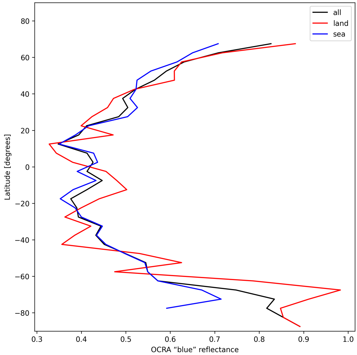
Figure 33: Zonal average of “OCRA “blue” reflectance” for 2025-01-21 to 2025-01-21.
