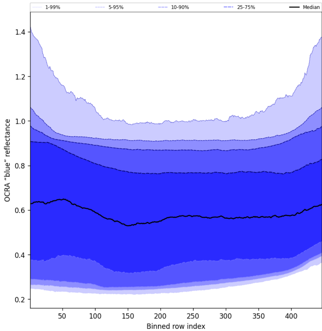
Figure 65: Along track statistics of “OCRA “blue” reflectance” for 2025-01-21 to 2025-01-21
