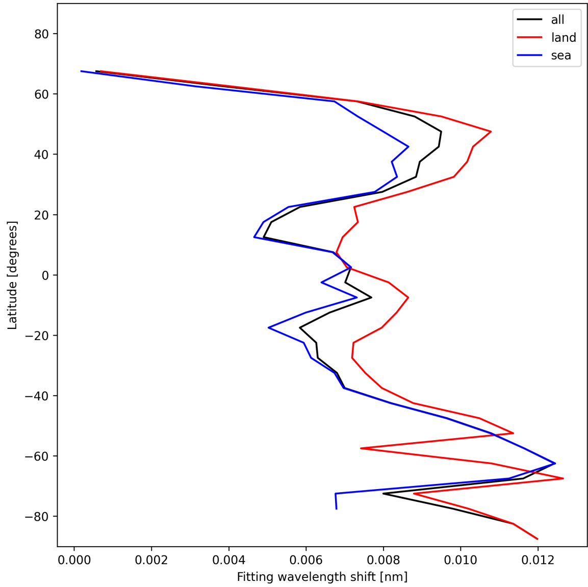
Figure 31: Zonal average of “Fitting wavelength shift” for 2025-01-21 to 2025-01-21.
