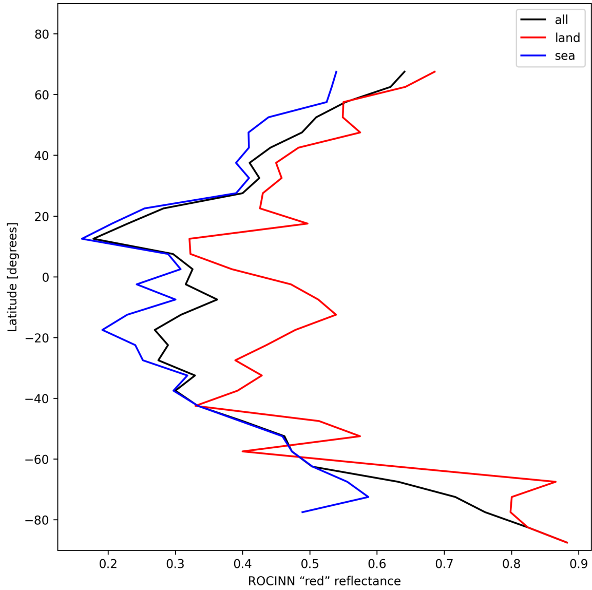
Figure 35: Zonal average of “ROCINN “red” reflectance” for 2025-01-21 to 2025-01-21.
