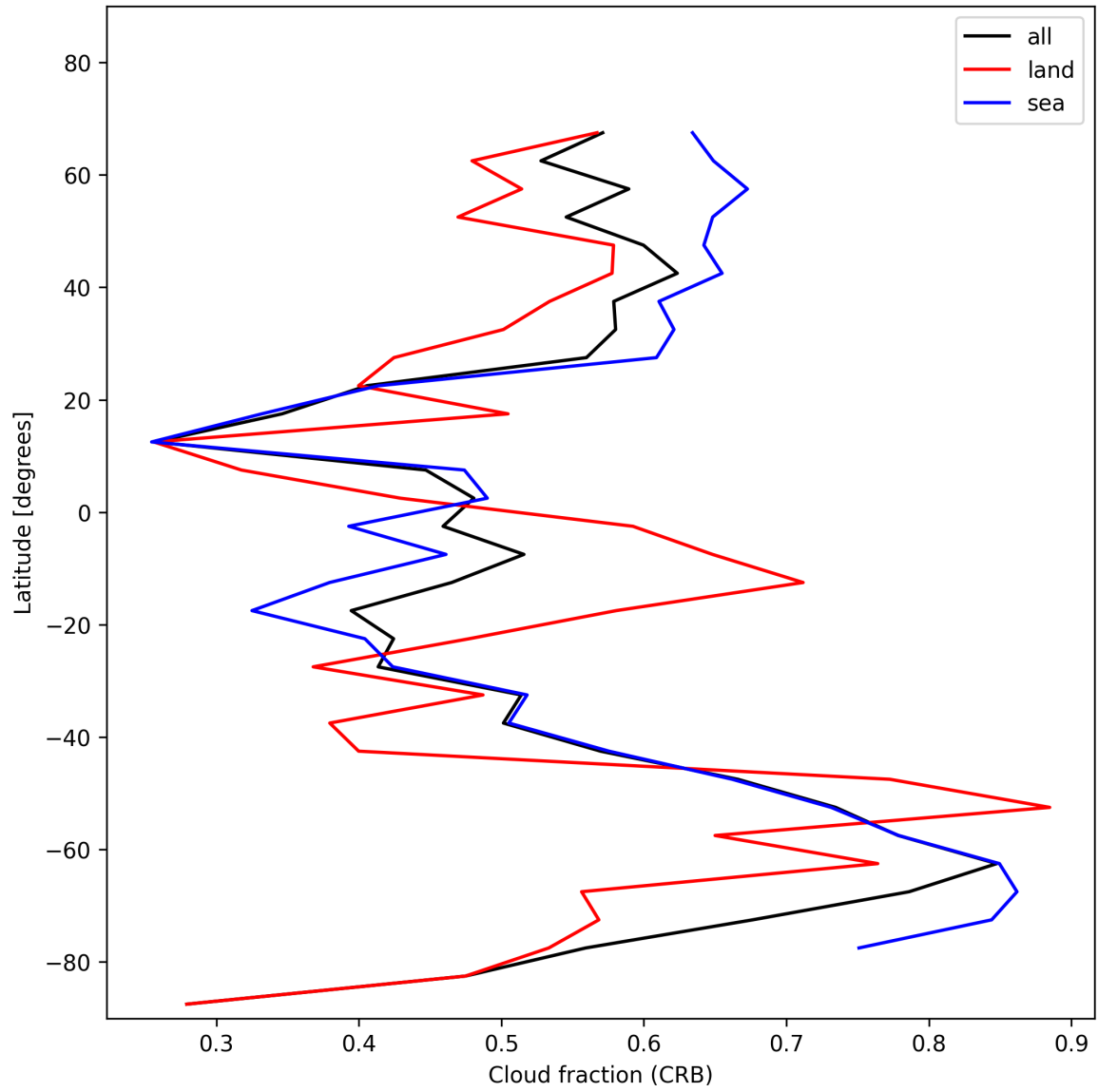
Figure 24: Zonal average of “Cloud fraction (CRB)” for 2025-01-21 to 2025-01-21.
