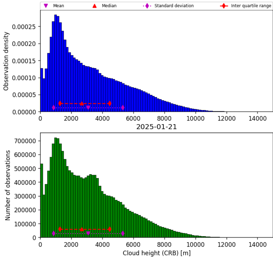
Figure 41: Histogram of “Cloud height (CRB)” for 2025-01-21 to 2025-01-21
