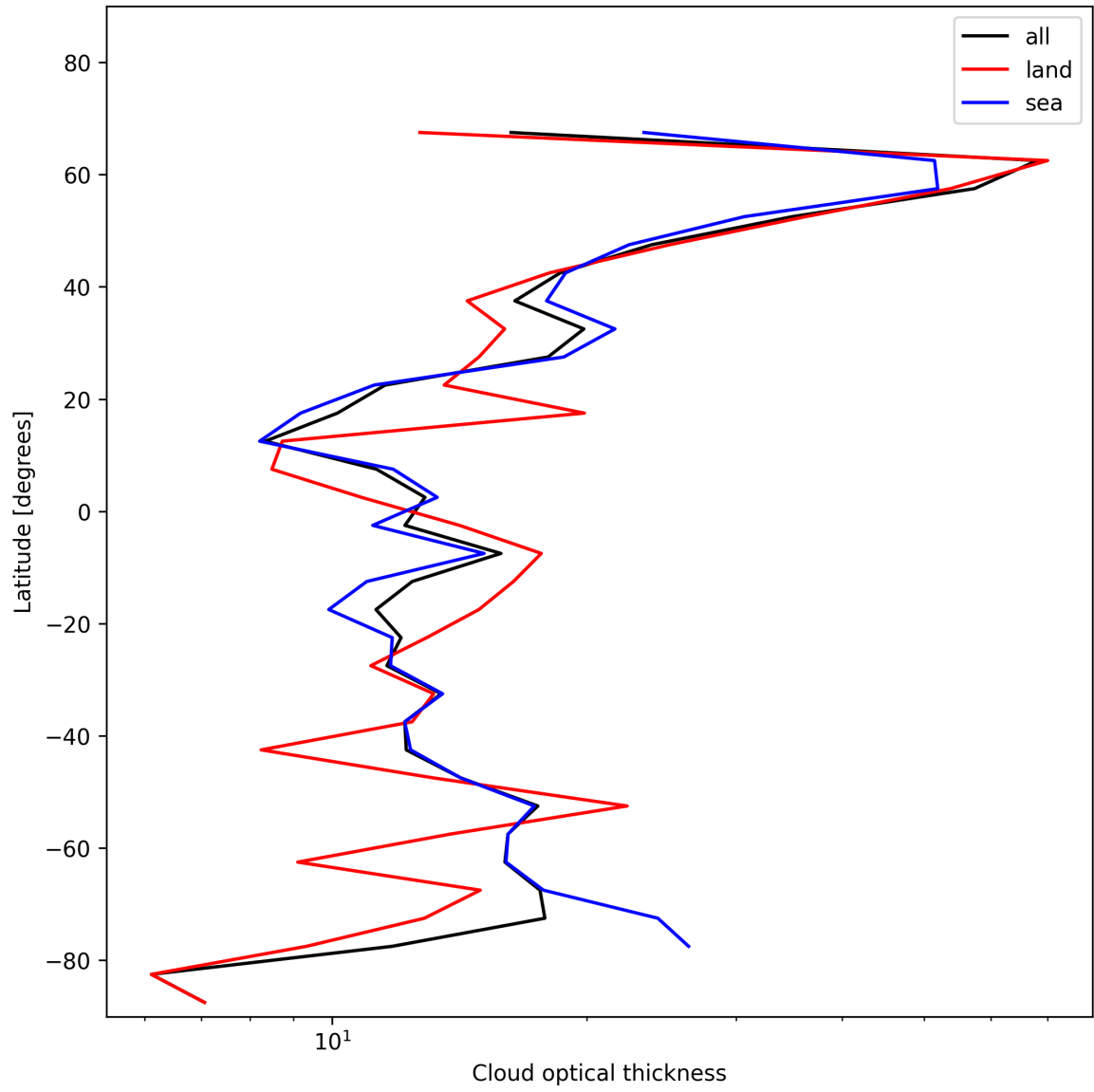
Figure 23: Zonal average of “Cloud optical thickness” for 2025-01-21 to 2025-01-21.
