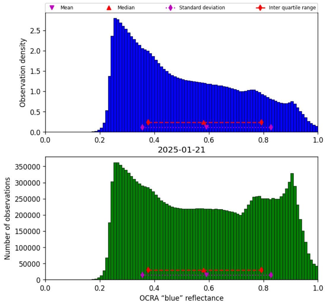
Figure 49: Histogram of “OCRA “blue” reflectance” for 2025-01-21 to 2025-01-21
