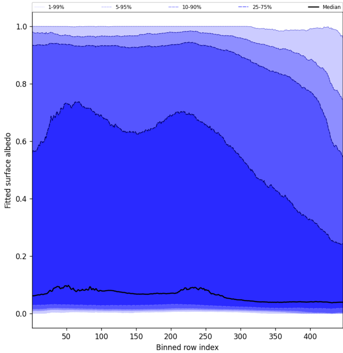
Figure 59: Along track statistics of “Fitted surface albedo” for 2025-01-21 to 2025-01-21
