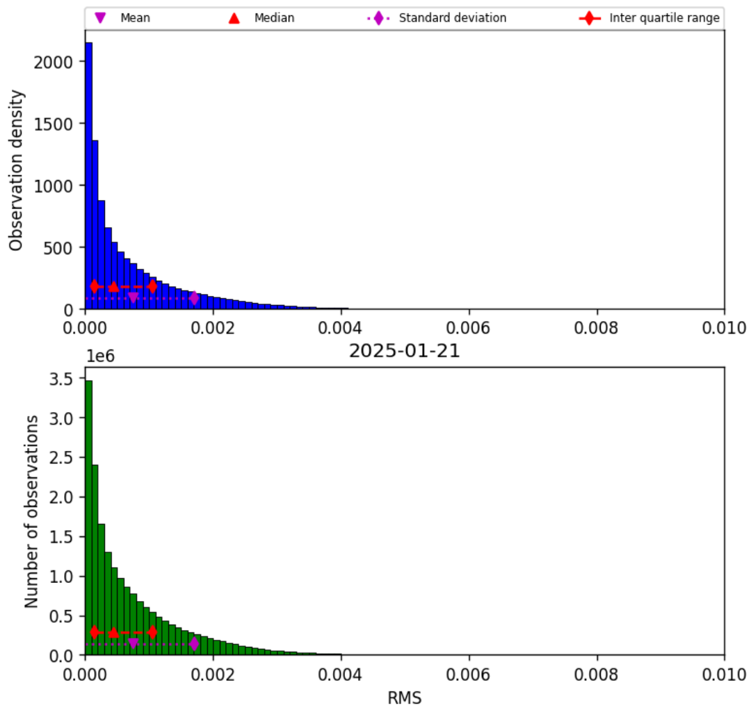
Figure 45: Histogram of “RMS” for 2025-01-21 to 2025-01-21
