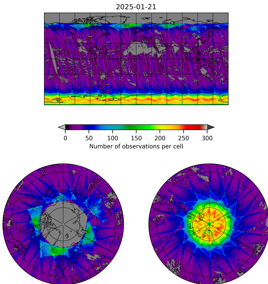
Figure 19: Map of the number of observations for 2025-01-21 to 2025-01-21
