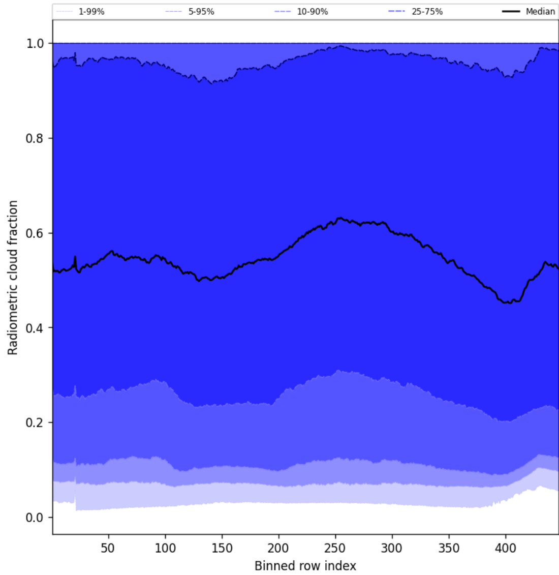
Figure 53: Along track statistics of “Radiometric cloud fraction” for 2025-01-21 to 2025-01-21
