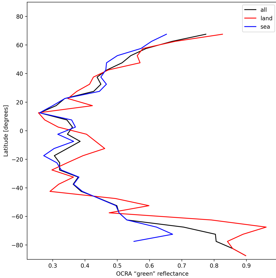
Figure 34: Zonal average of “OCRA “green” reflectance” for 2025-01-21 to 2025-01-21.
