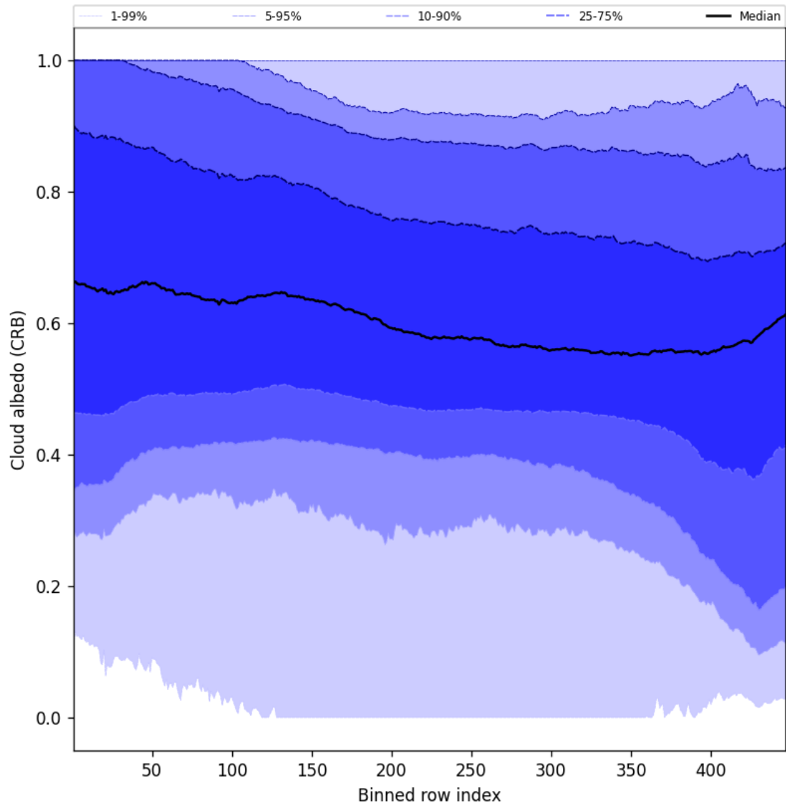
Figure 58: Along track statistics of “Cloud albedo (CRB)” for 2025-01-21 to 2025-01-21
