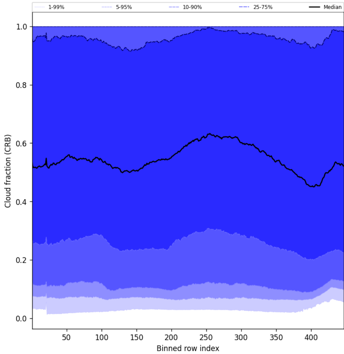
Figure 56: Along track statistics of “Cloud fraction (CRB)” for 2025-01-21 to 2025-01-21
