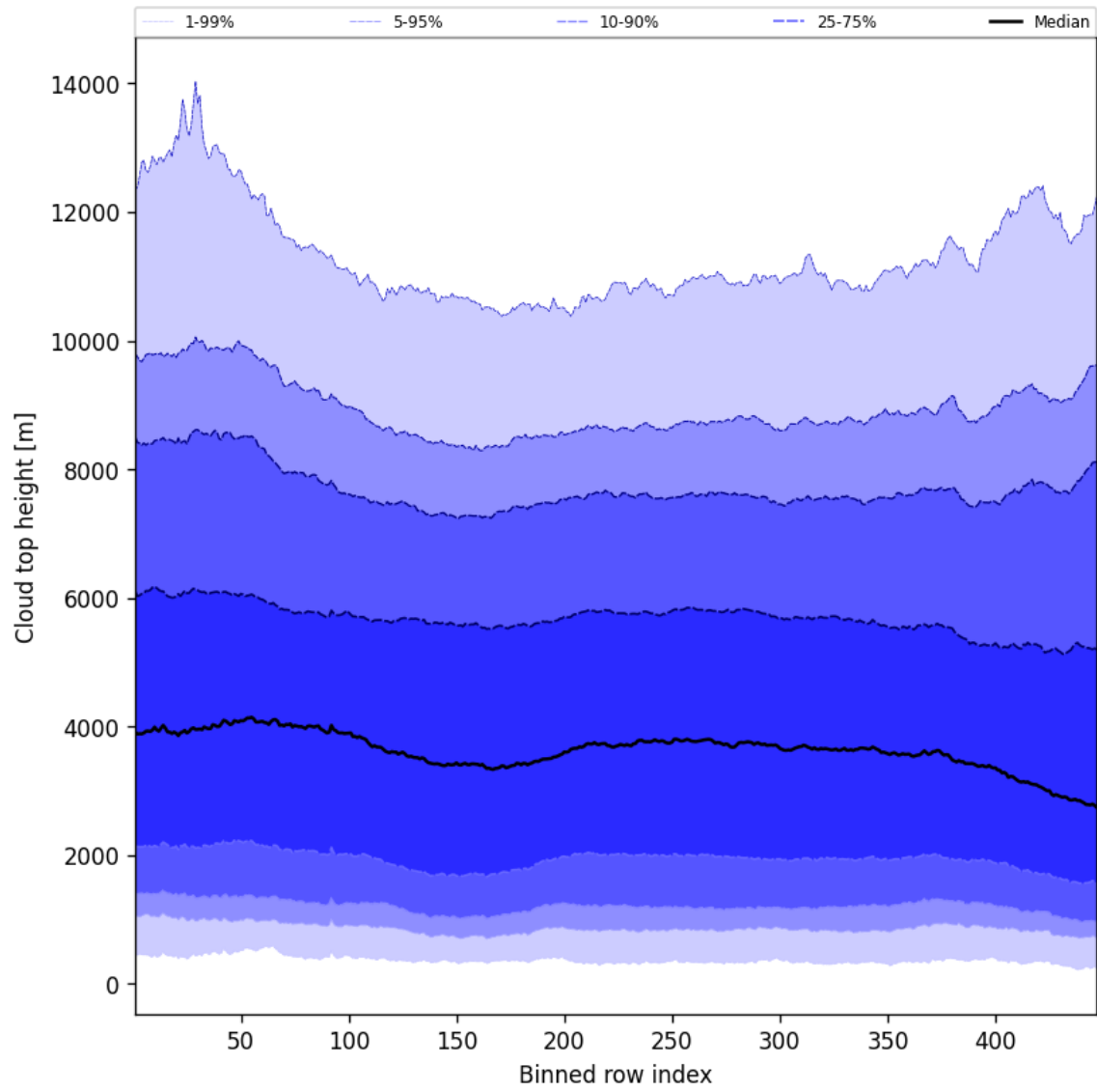
Figure 54: Along track statistics of “Cloud top height” for 2025-01-21 to 2025-01-21
