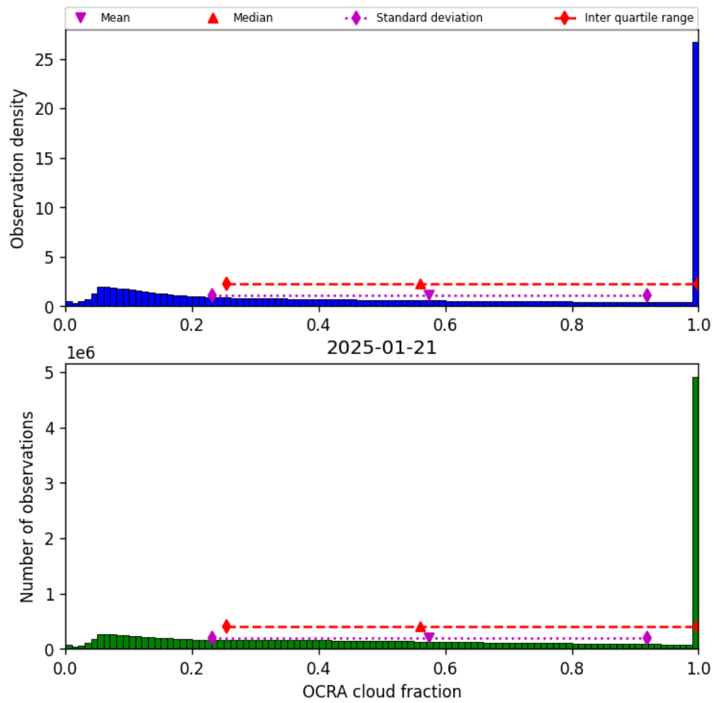
Figure 48: Histogram of “OCRA cloud fraction” for 2025-01-21 to 2025-01-21
