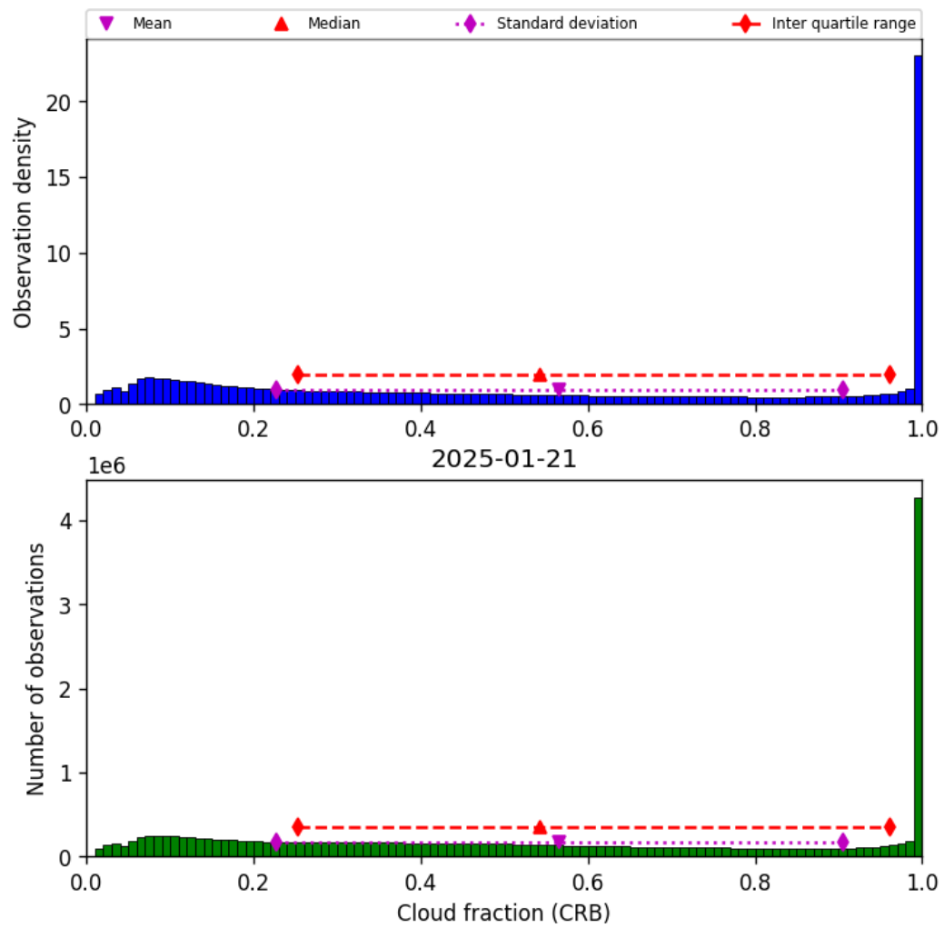
Figure 40: Histogram of “Cloud fraction (CRB)” for 2025-01-21 to 2025-01-21
