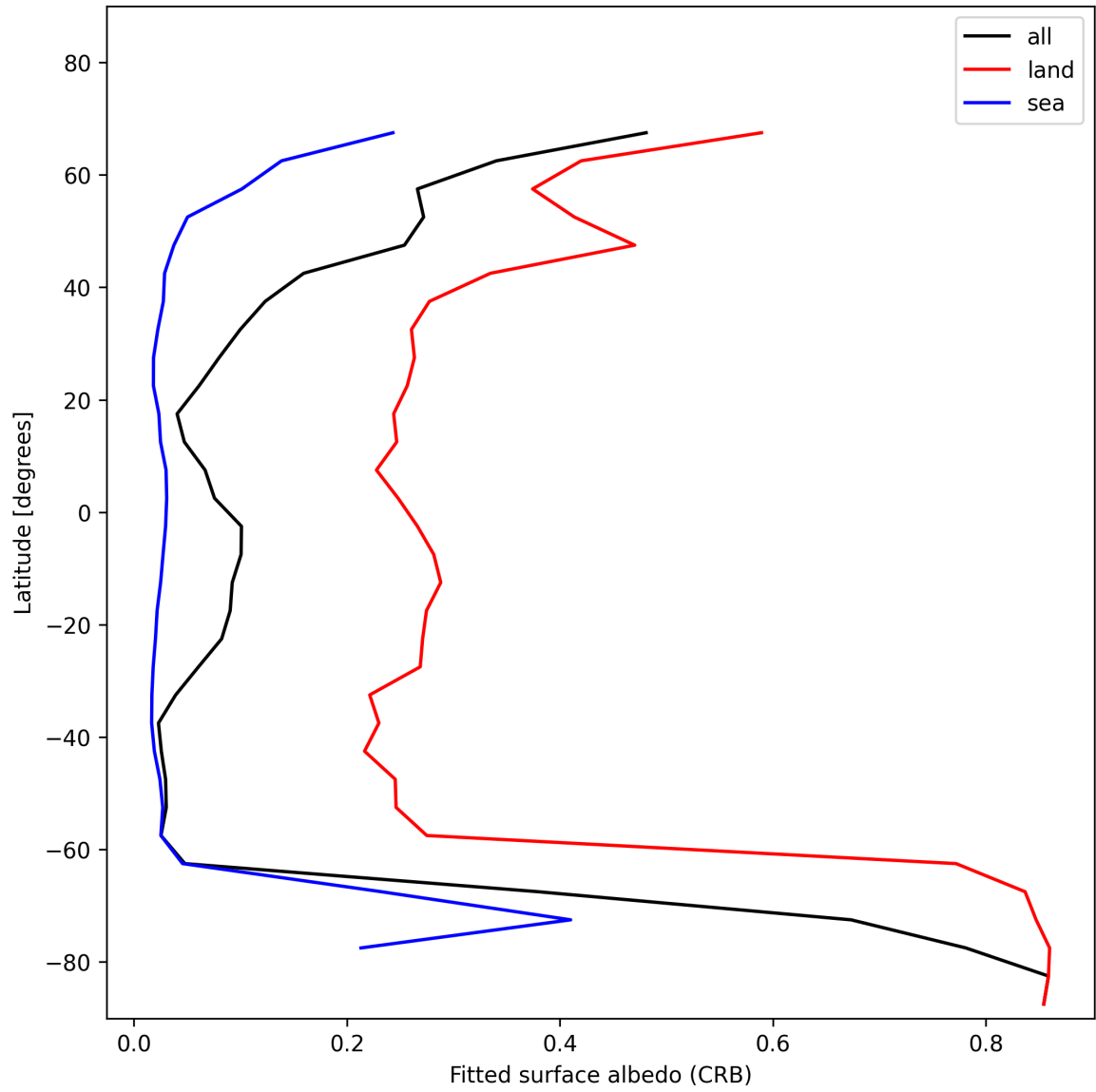
Figure 28: Zonal average of “Fitted surface albedo (CRB)” for 2025-01-21 to 2025-01-21.
