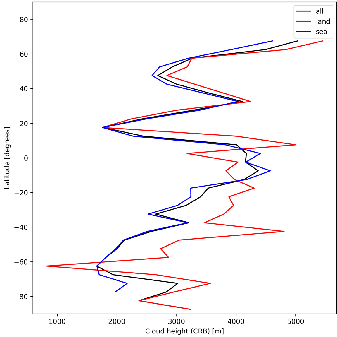
Figure 25: Zonal average of “Cloud height (CRB)” for 2025-01-21 to 2025-01-21.
