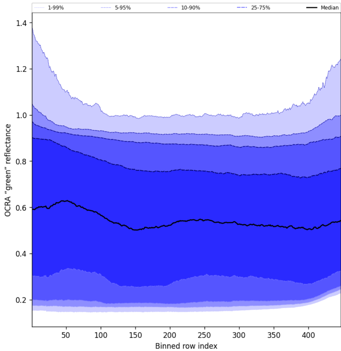
Figure 66: Along track statistics of "OCRA "green" reflectance" for 2025-01-21 to 2025-01-21
