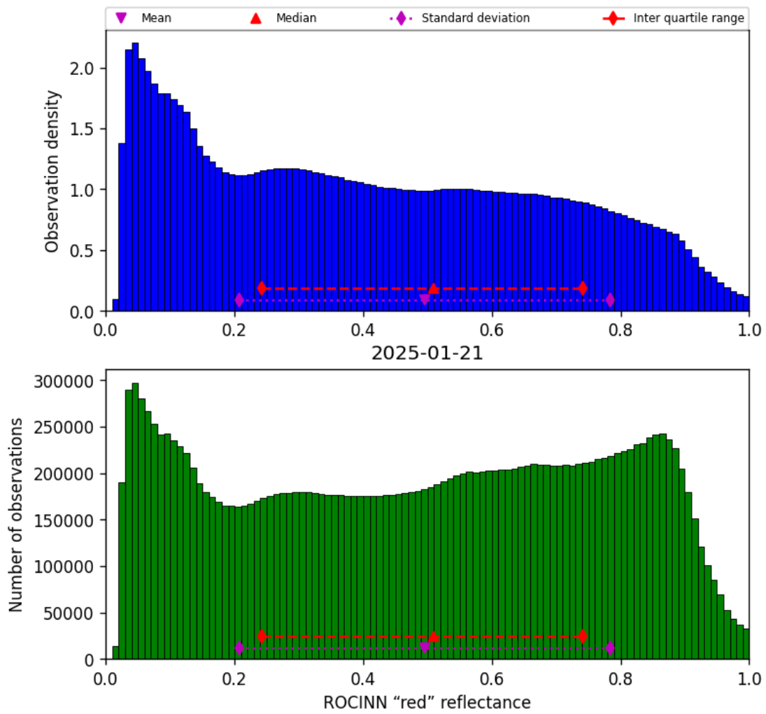
Figure 51: Histogram of “ROCINN “red” reflectance” for 2025-01-21 to 2025-01-21
