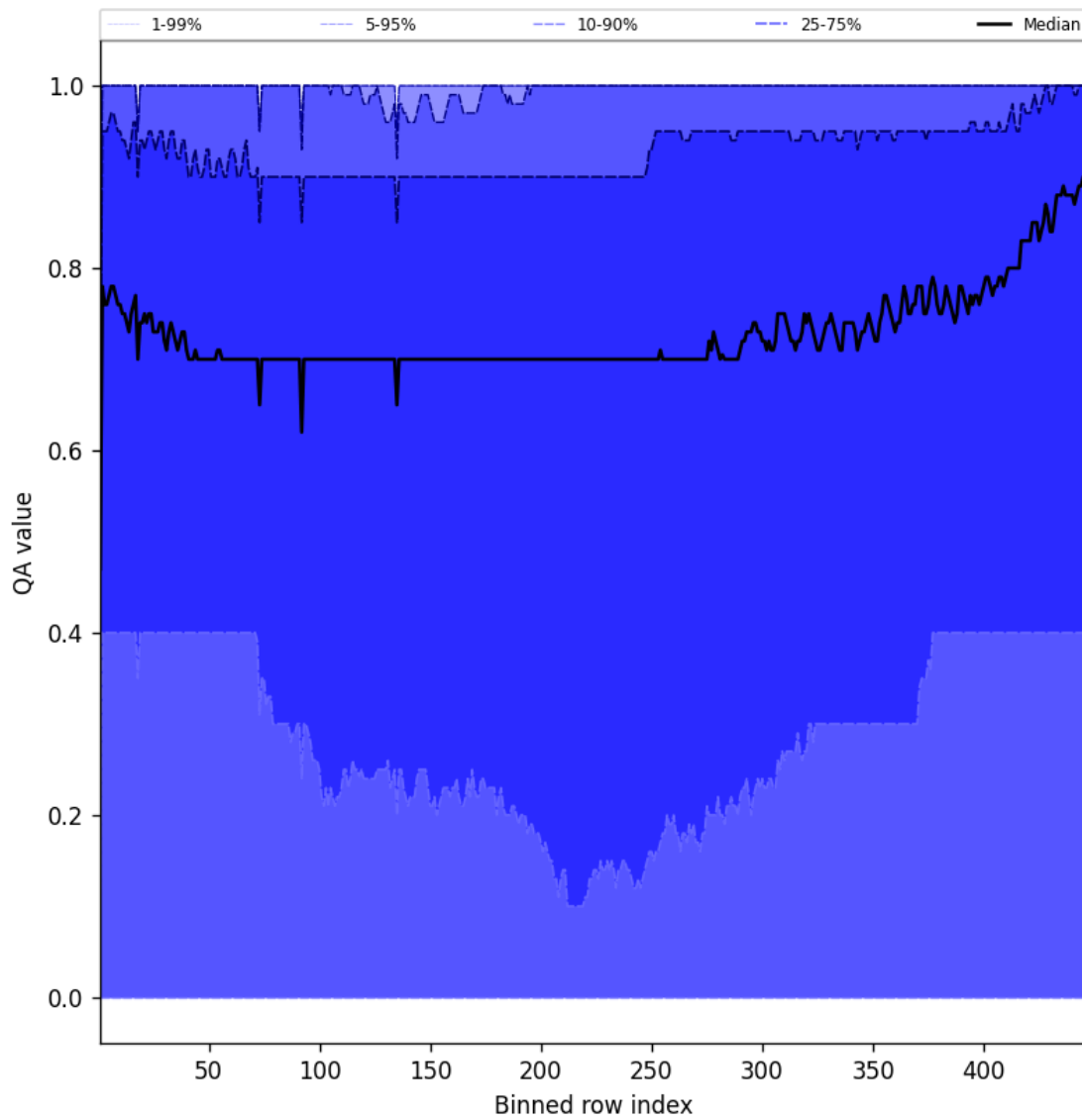
Figure 52: Along track statistics of “QA value” for 2025-01-21 to 2025-01-21
