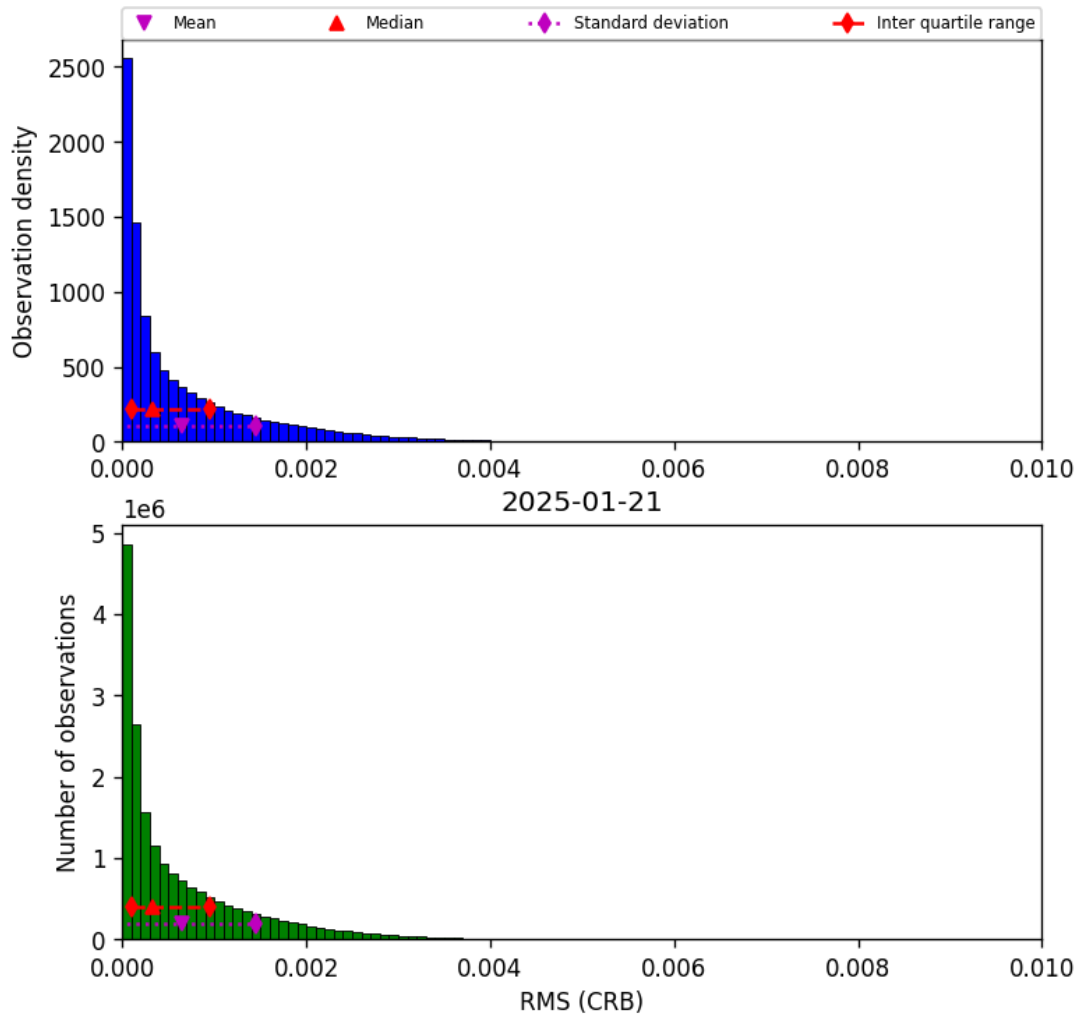
Figure 46: Histogram of “RMS (CRB)” for 2025-01-21 to 2025-01-21
