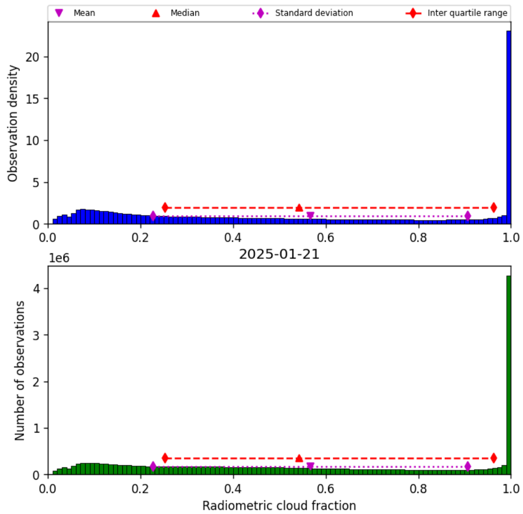
Figure 37: Histogram of “Radiometric cloud fraction” for 2025-01-21 to 2025-01-21
