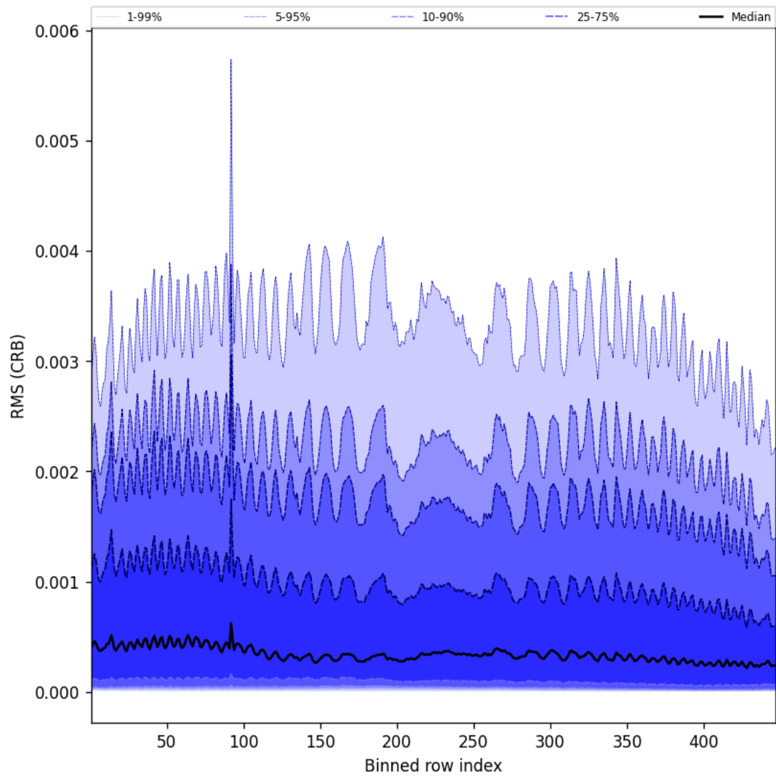
Figure 62: Along track statistics of “RMS (CRB)” for 2025-01-21 to 2025-01-21
