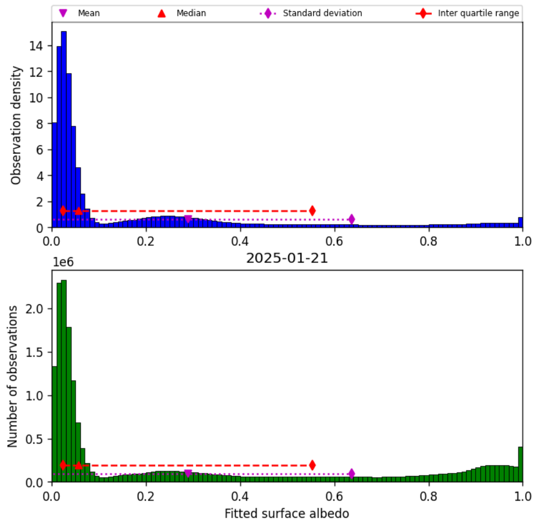
Figure 43: Histogram of “Fitted surface albedo” for 2025-01-21 to 2025-01-21
