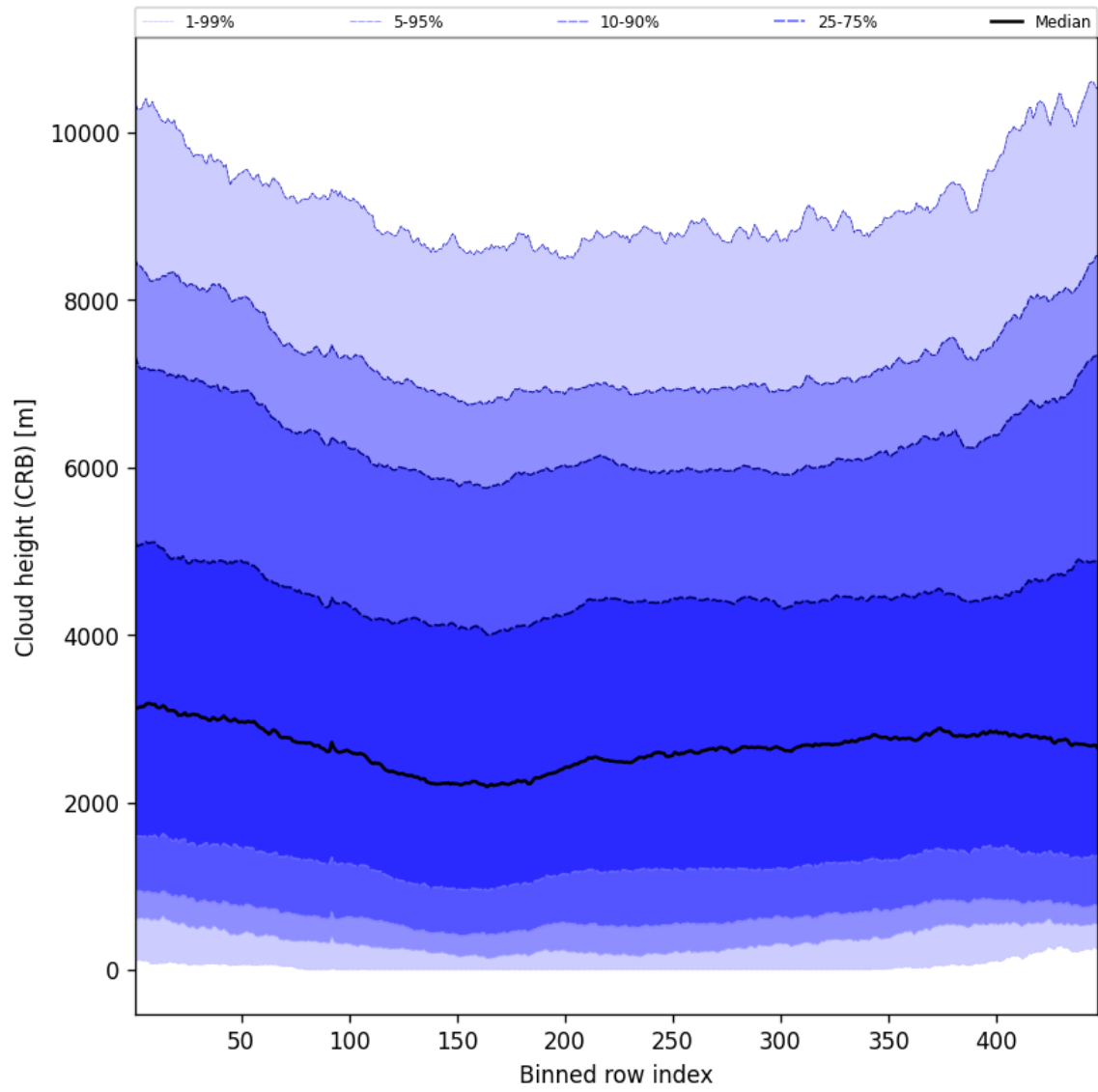
Figure 57: Along track statistics of “Cloud height (CRB)” for 2025-01-21 to 2025-01-21
