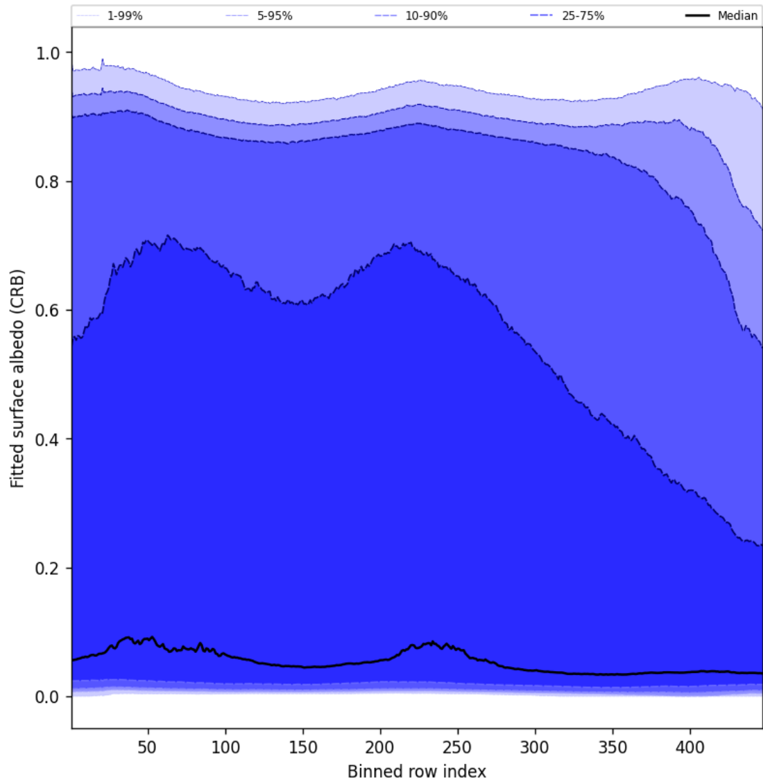
Figure 60: Along track statistics of “Fitted surface albedo (CRB)” for 2025-01-21 to 2025-01-21
