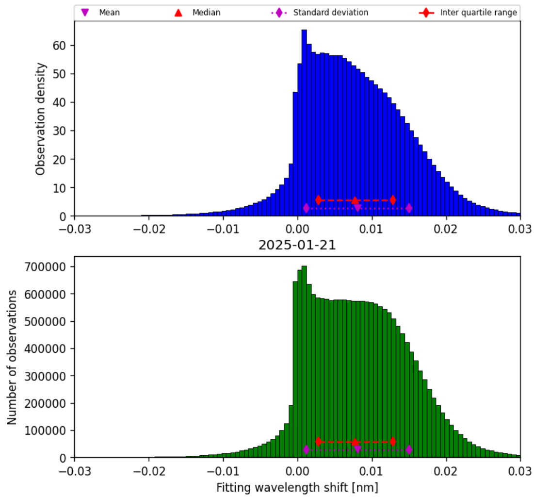
Figure 47: Histogram of “Fitting wavelength shift” for 2025-01-21 to 2025-01-21
