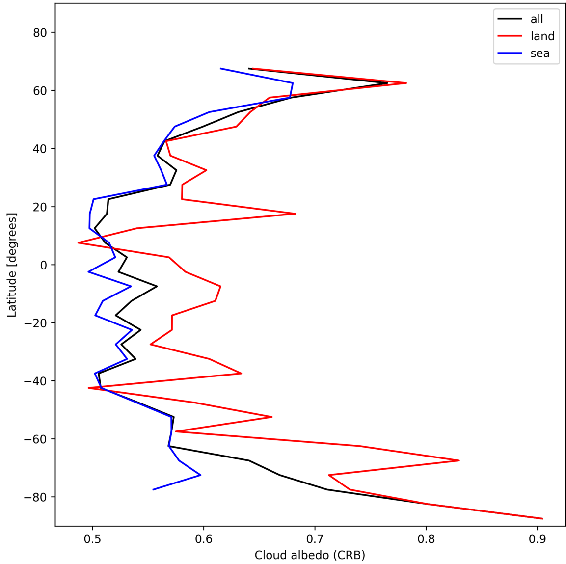
Figure 26: Zonal average of “Cloud albedo (CRB)” for 2025-01-21 to 2025-01-21.
