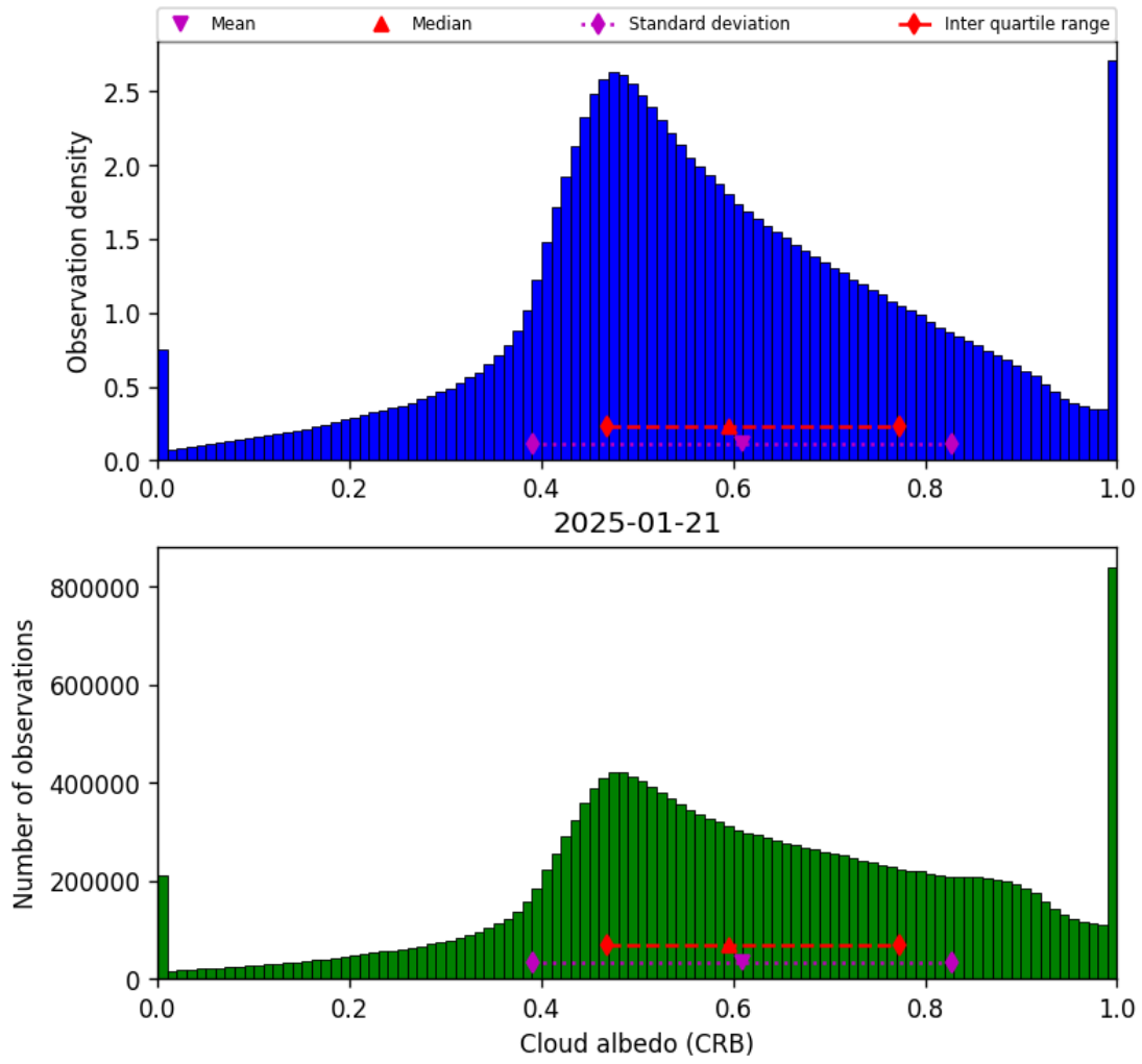
Figure 42: Histogram of “Cloud albedo (CRB)” for 2025-01-21 to 2025-01-21
