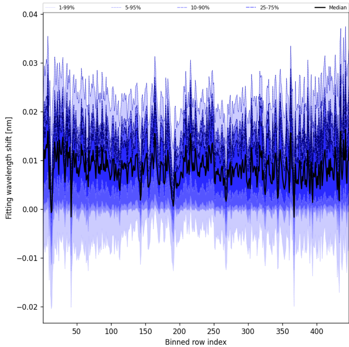
Figure 63: Along track statistics of “Fitting wavelength shift” for 2025-01-22 to 2025-01-23
