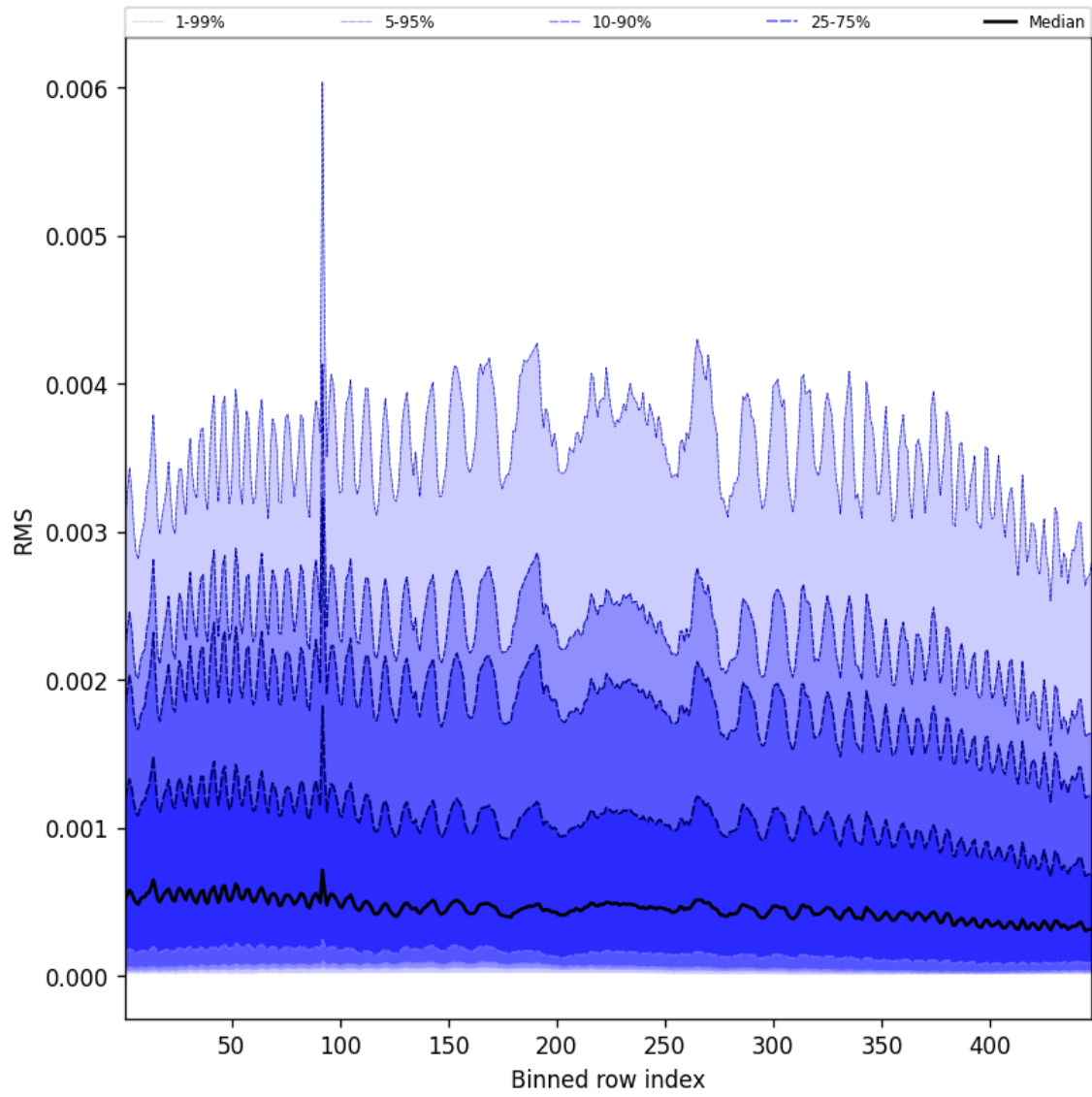
Figure 61: Along track statistics of “RMS” for 2025-01-22 to 2025-01-23
