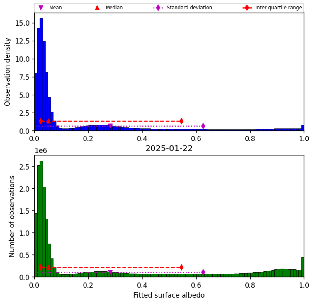
Figure 43: Histogram of “Fitted surface albedo” for 2025-01-22 to 2025-01-23
