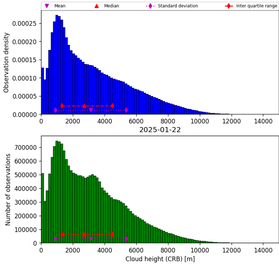
Figure 41: Histogram of “Cloud height (CRB)” for 2025-01-22 to 2025-01-23
