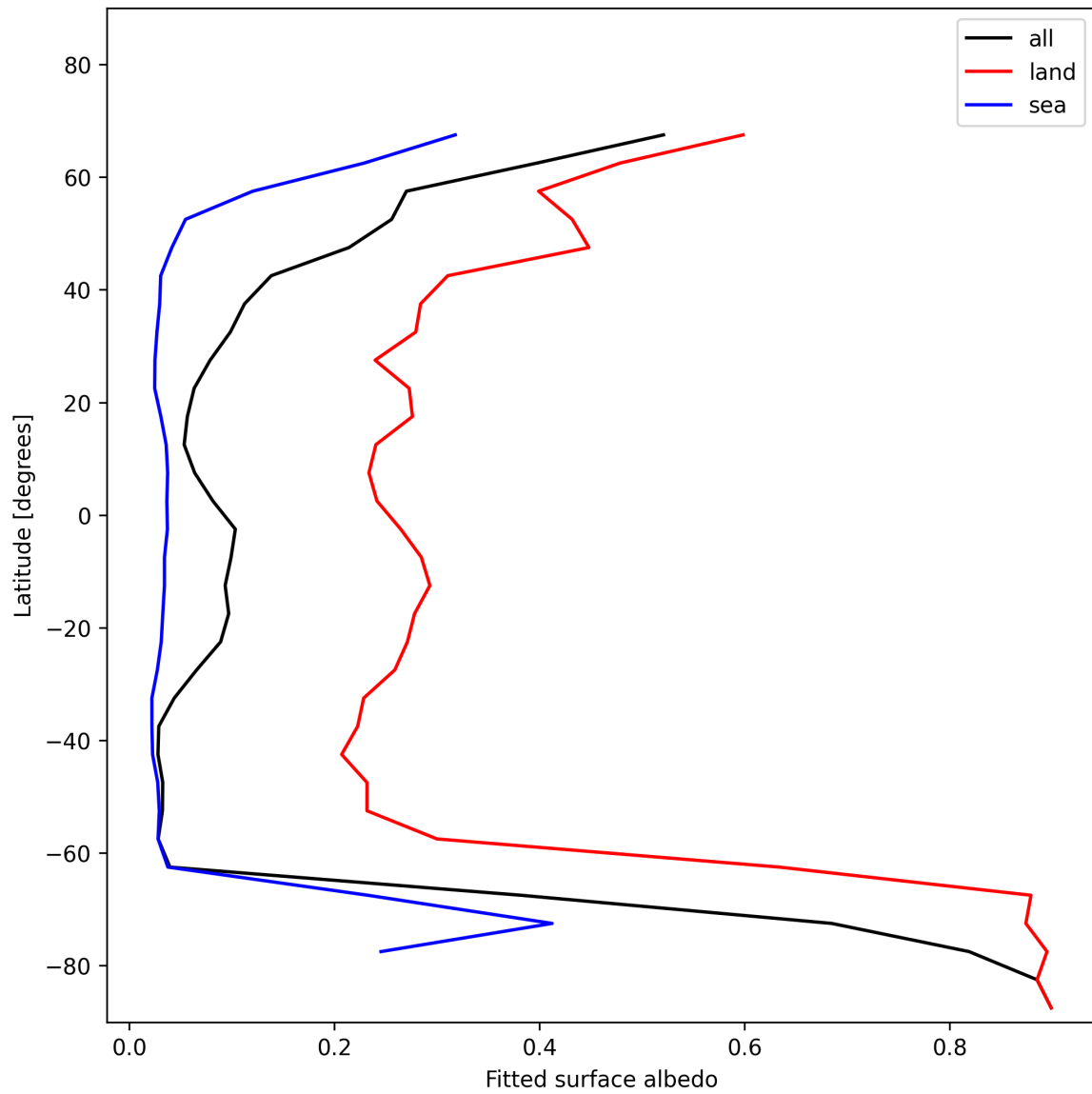
Figure 27: Zonal average of “Fitted surface albedo” for 2025-01-22 to 2025-01-23.
