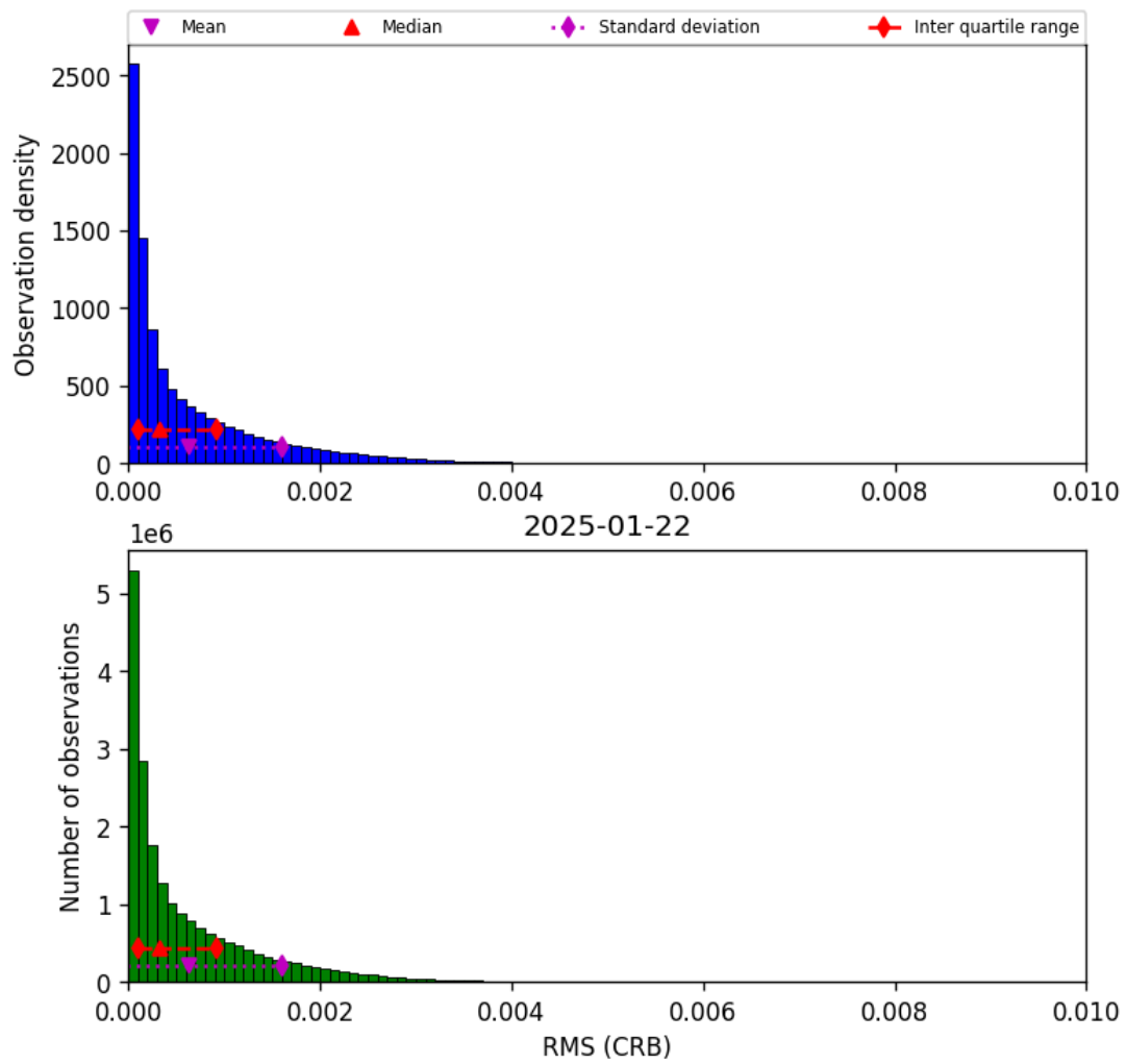
Figure 46: Histogram of “RMS (CRB)” for 2025-01-22 to 2025-01-23
