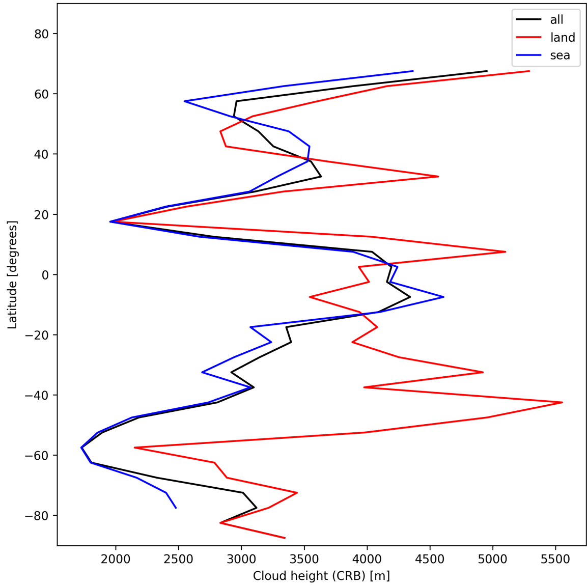
Figure 25: Zonal average of “Cloud height (CRB)” for 2025-01-22 to 2025-01-23.
