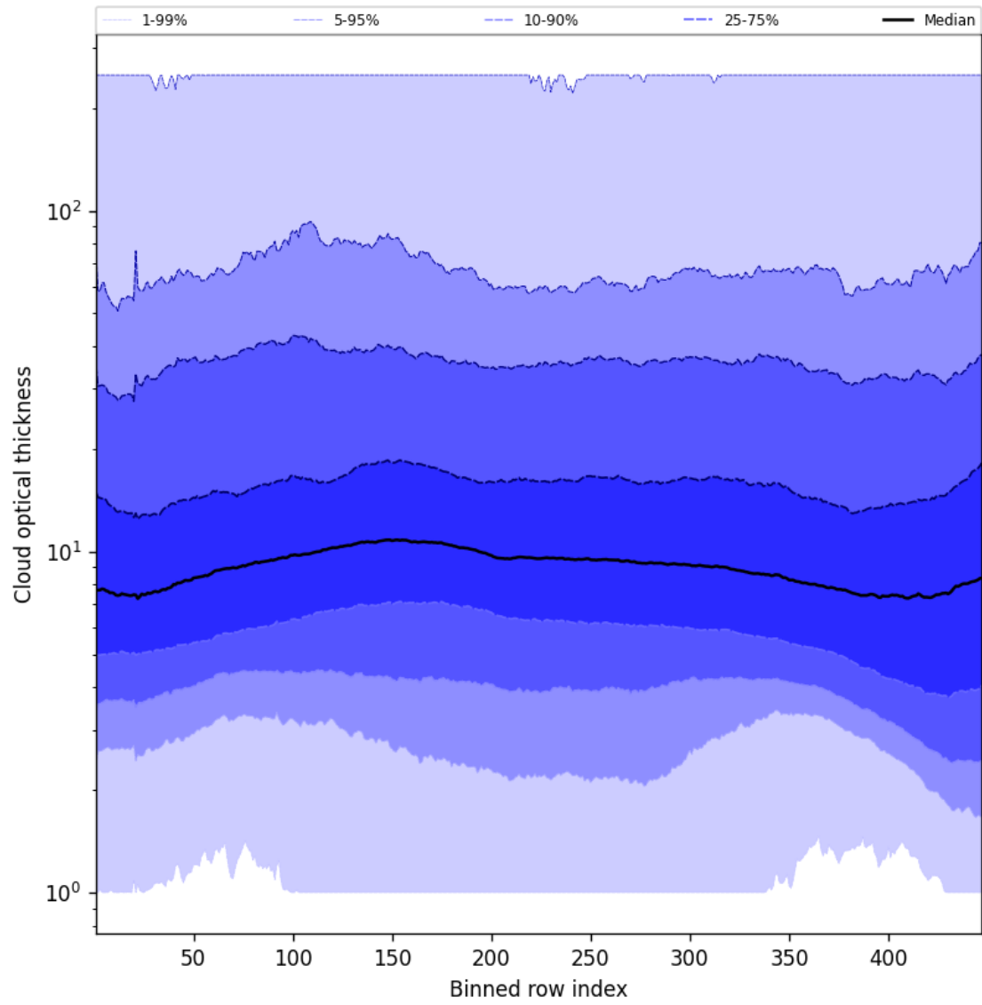
Figure 55: Along track statistics of “Cloud optical thickness” for 2025-01-22 to 2025-01-23
