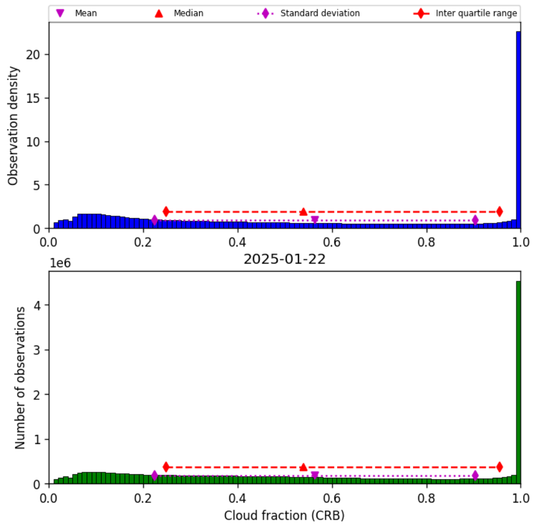
Figure 40: Histogram of “Cloud fraction (CRB)” for 2025-01-22 to 2025-01-23
