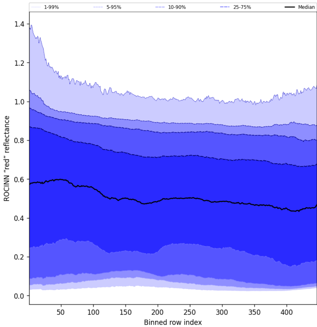
Figure 67: Along track statistics of “ROCINN “red” reflectance” for 2025-01-22 to 2025-01-23
