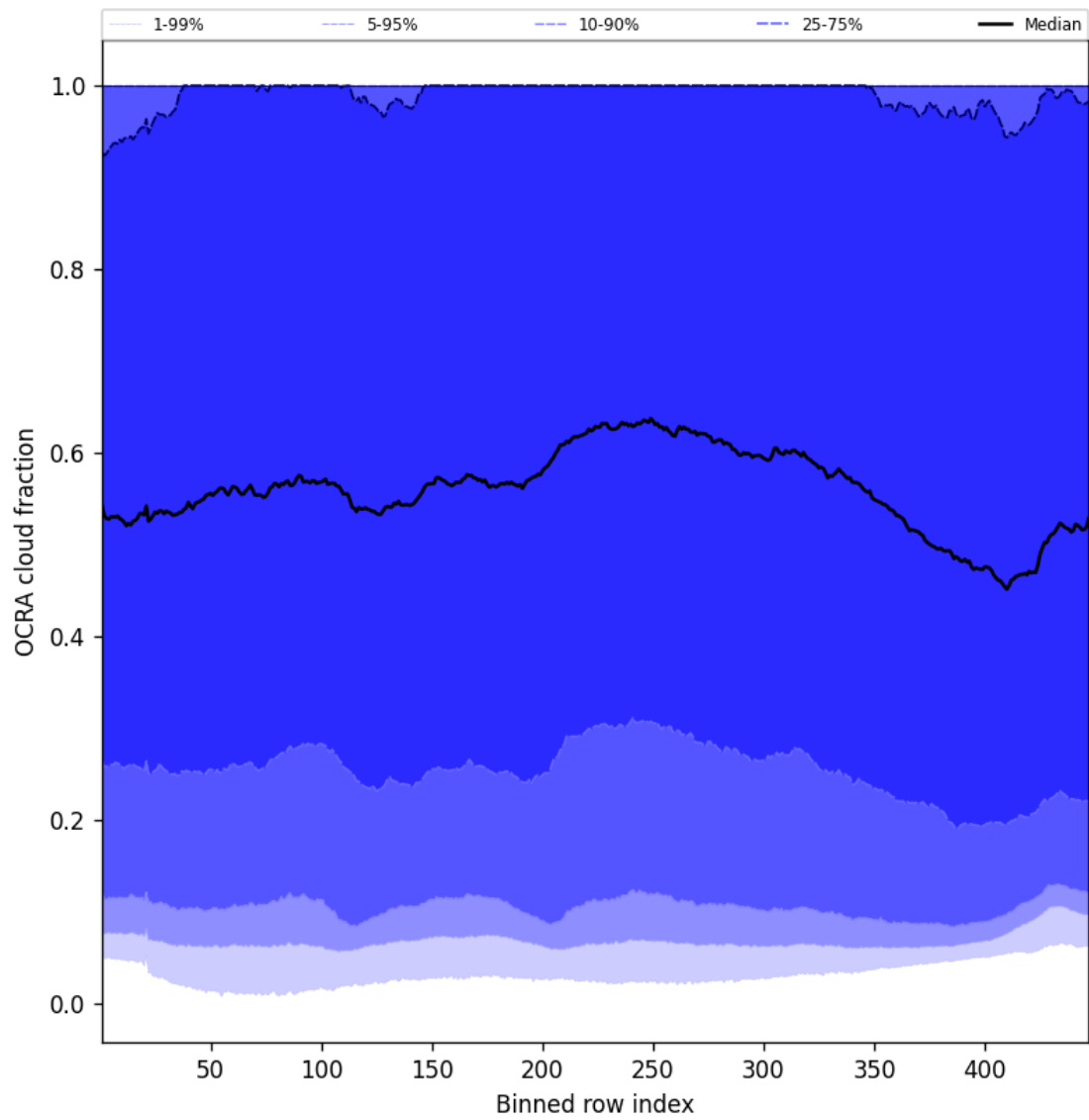
Figure 64: Along track statistics of “OCRA cloud fraction” for 2025-01-22 to 2025-01-23
