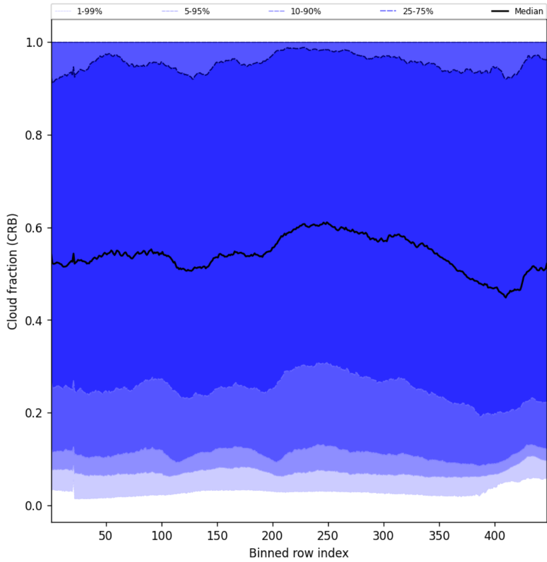
Figure 56: Along track statistics of “Cloud fraction (CRB)” for 2025-01-22 to 2025-01-23
