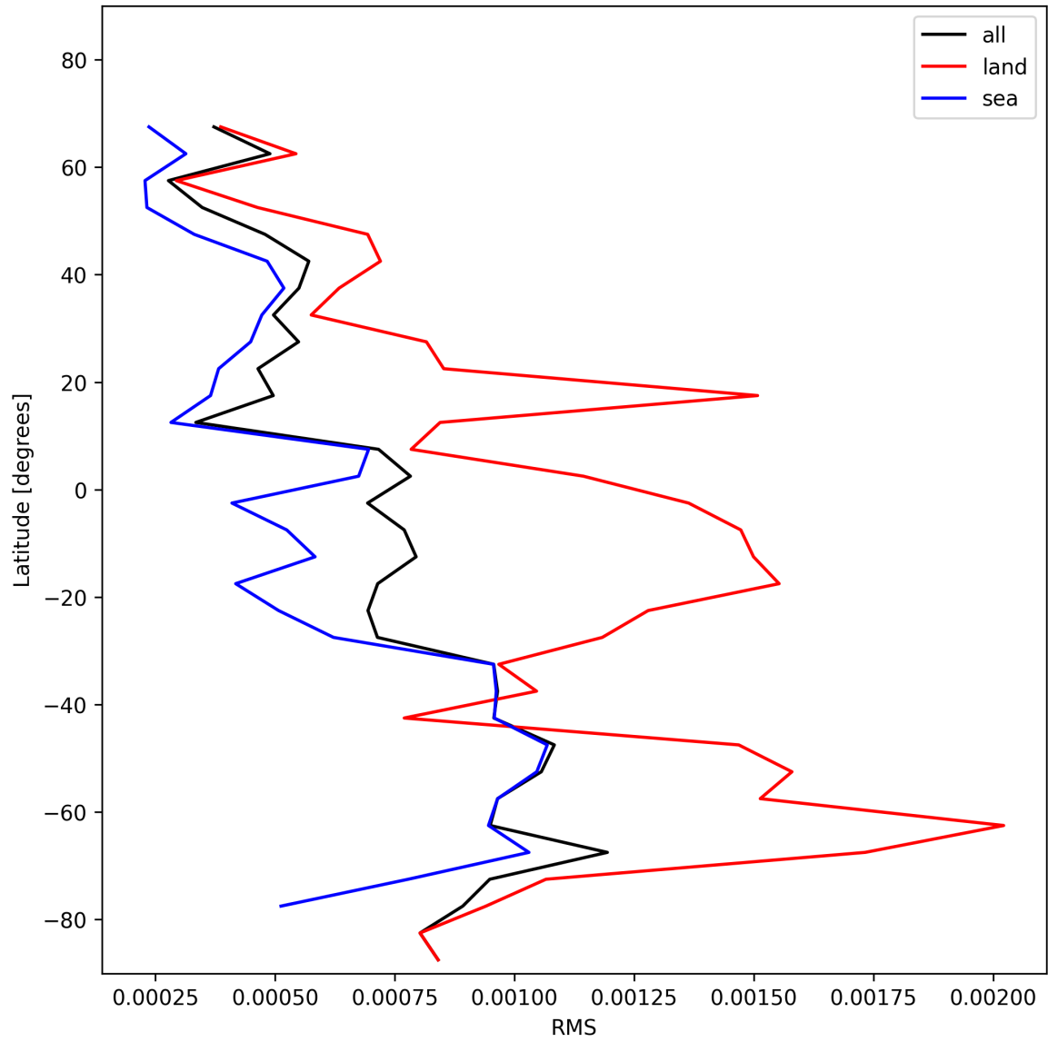
Figure 29: Zonal average of “RMS” for 2025-01-22 to 2025-01-23.
