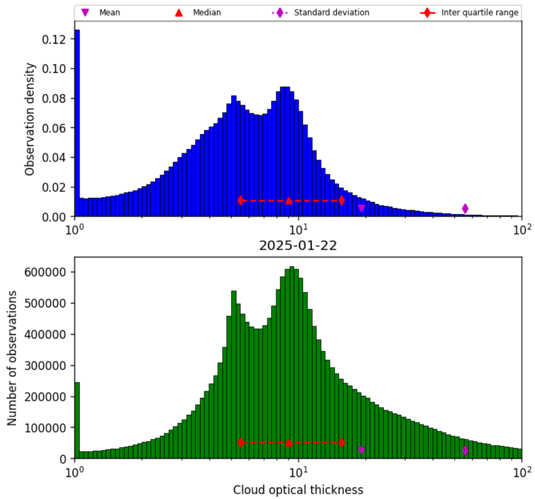
Figure 39: Histogram of “Cloud optical thickness” for 2025-01-22 to 2025-01-23
