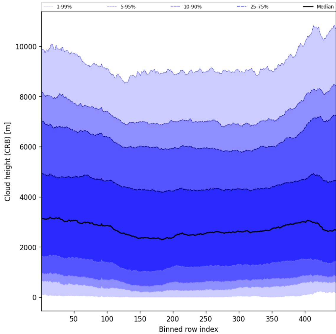
Figure 57: Along track statistics of “Cloud height (CRB)” for 2025-01-22 to 2025-01-23
