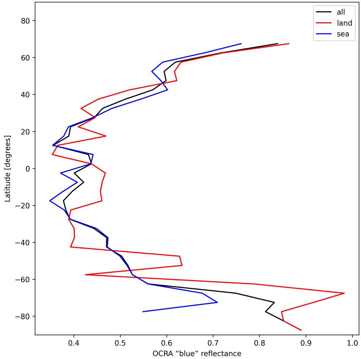
Figure 33: Zonal average of “OCRA “blue” reflectance” for 2025-01-22 to 2025-01-23.
