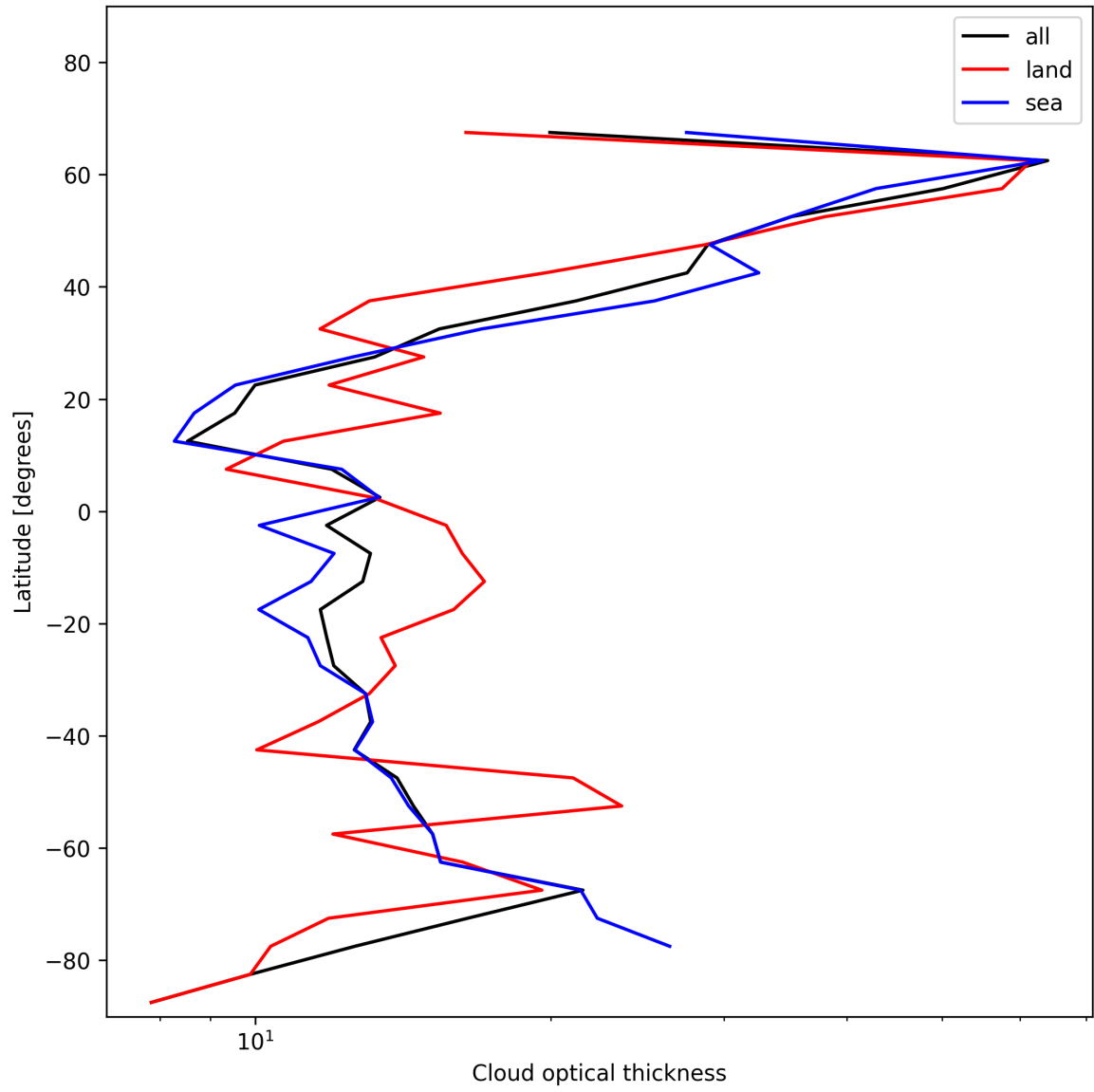
Figure 23: Zonal average of “Cloud optical thickness” for 2025-01-22 to 2025-01-23.
