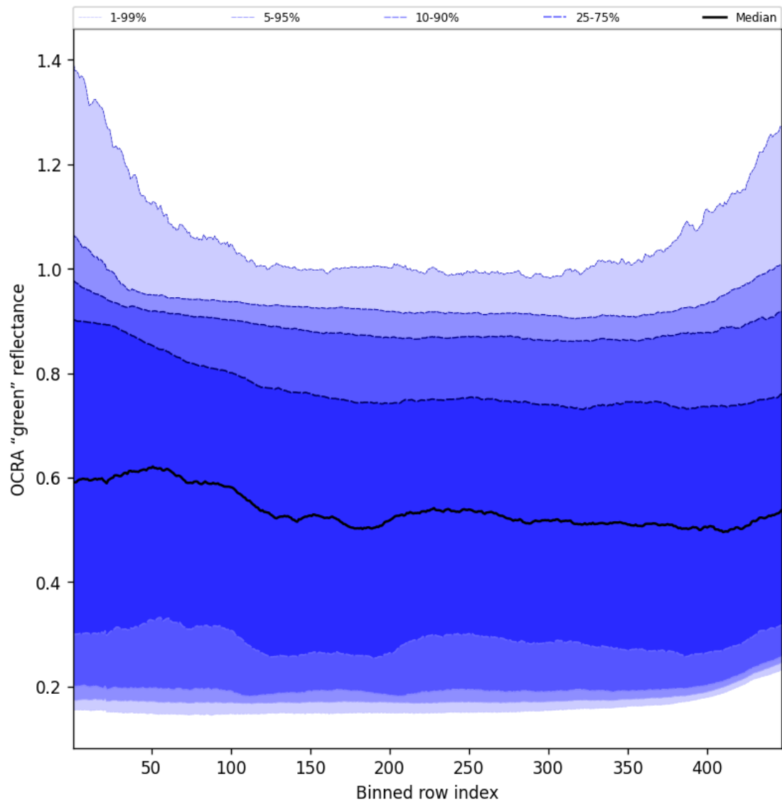
Figure 66: Along track statistics of “OCRA “green” reflectance” for 2025-01-22 to 2025-01-23
