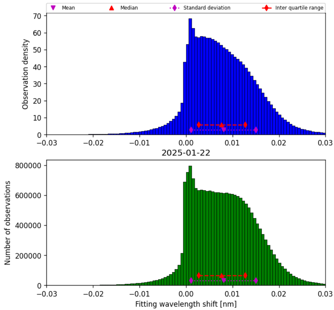
Figure 47: Histogram of “Fitting wavelength shift” for 2025-01-22 to 2025-01-23
