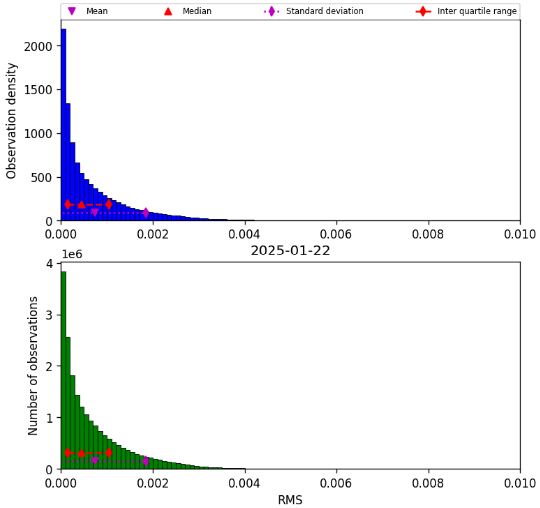
Figure 45: Histogram of “RMS” for 2025-01-22 to 2025-01-23
