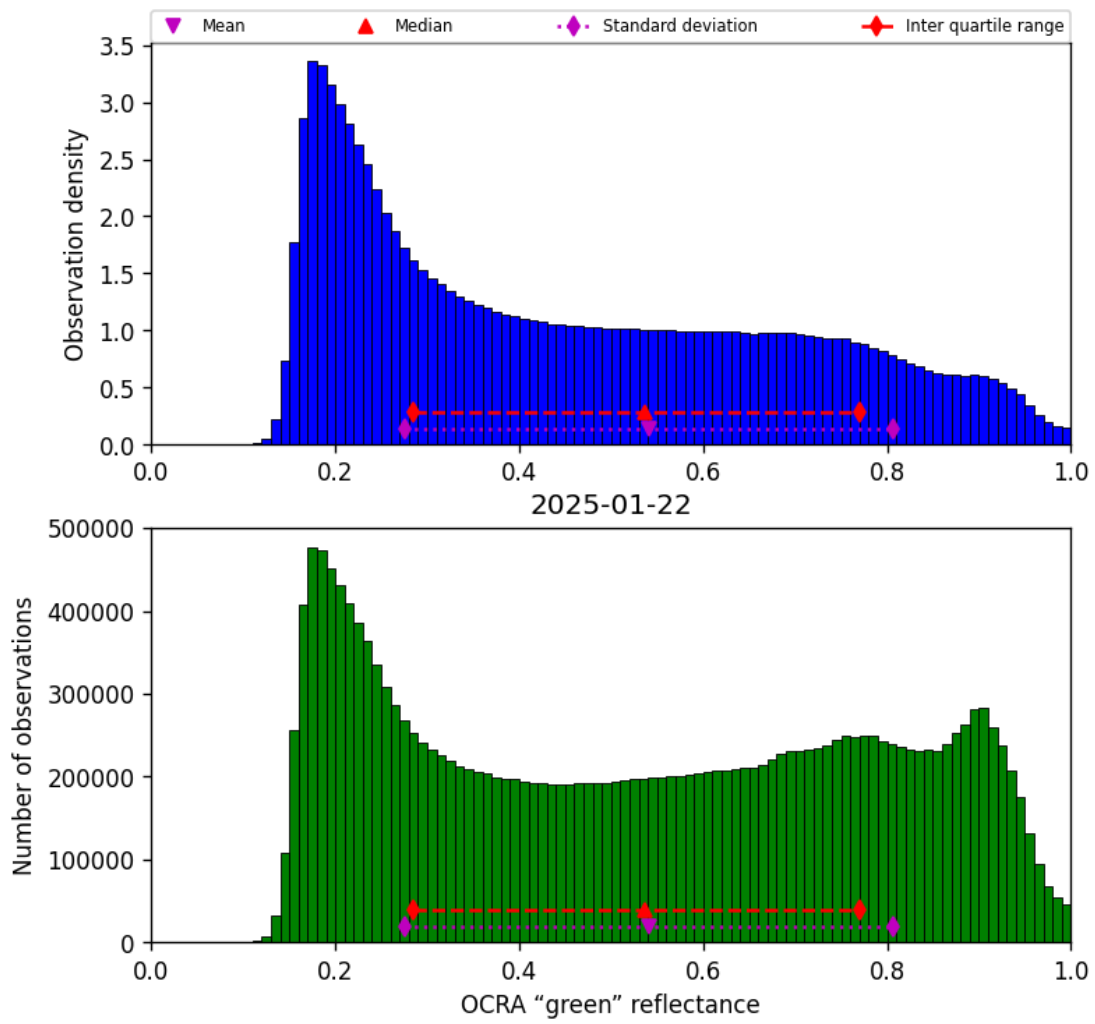
Figure 50: Histogram of “OCRA “green” reflectance” for 2025-01-22 to 2025-01-23
