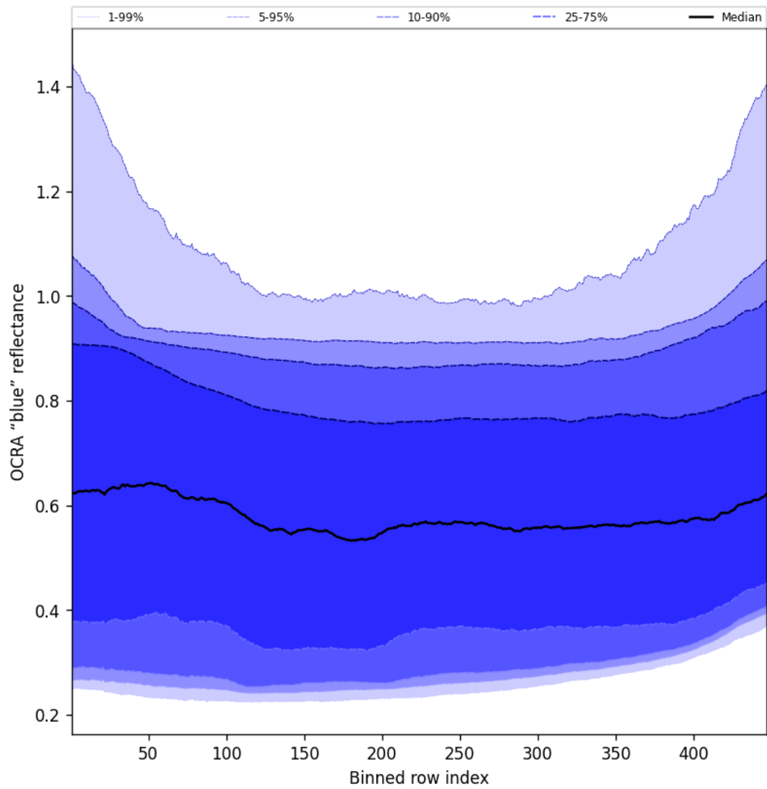
Figure 65: Along track statistics of "OCRA "blue" reflectance" for 2025-01-22 to 2025-01-23
