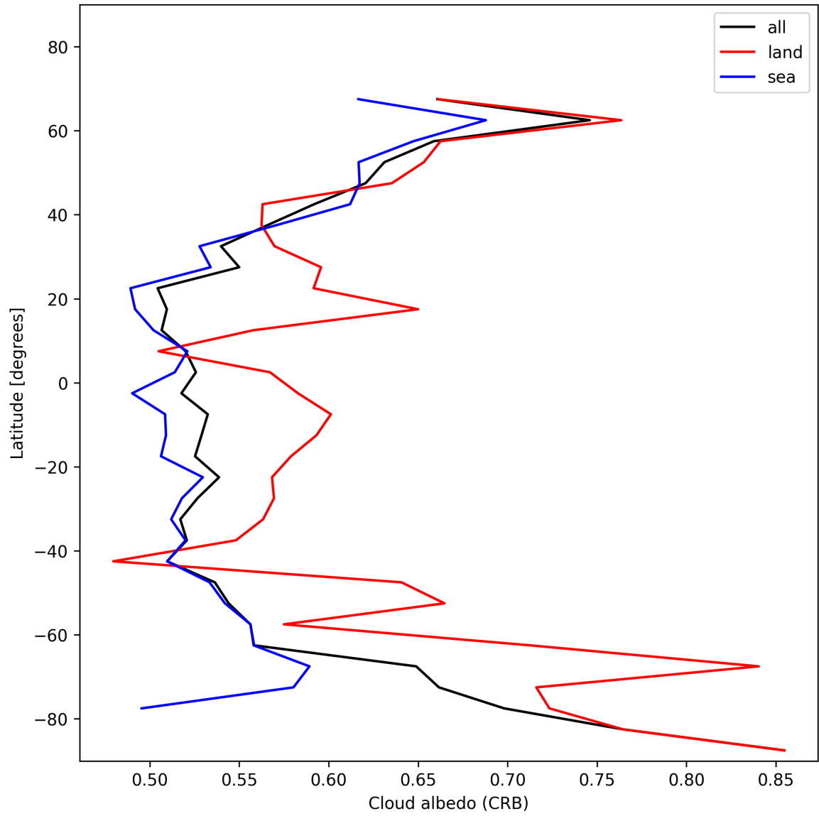
Figure 26: Zonal average of “Cloud albedo (CRB)” for 2025-01-22 to 2025-01-23.
