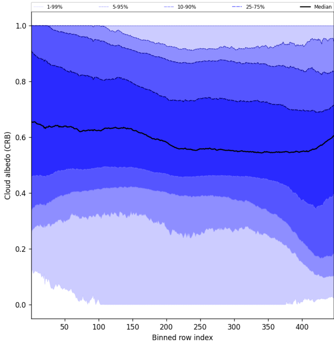
Figure 58: Along track statistics of “Cloud albedo (CRB)” for 2025-01-22 to 2025-01-23
