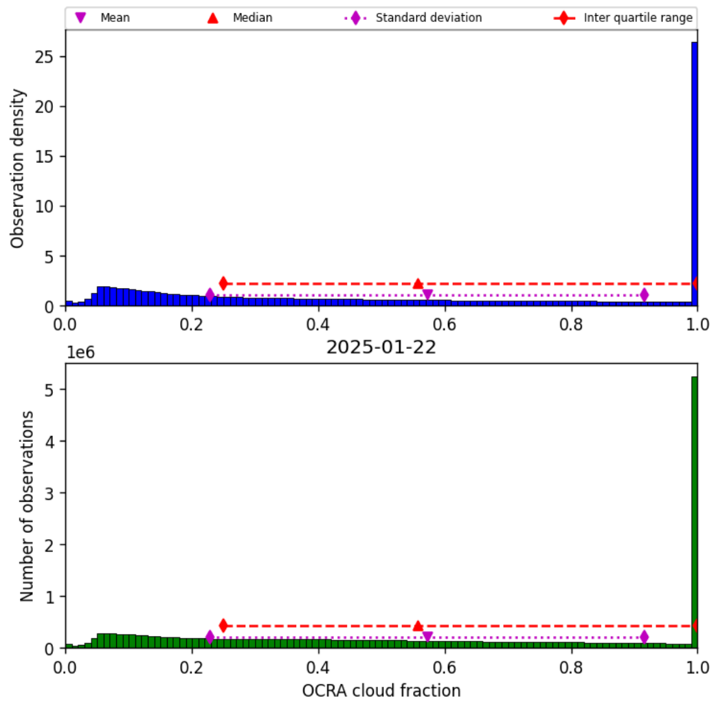
Figure 48: Histogram of “OCRA cloud fraction” for 2025-01-22 to 2025-01-23
