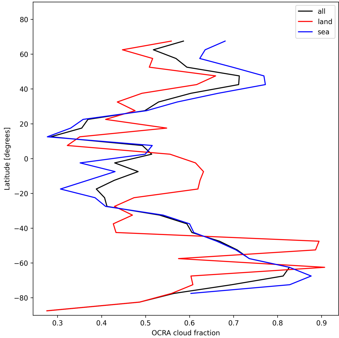
Figure 32: Zonal average of “OCRA cloud fraction” for 2025-01-22 to 2025-01-23.
