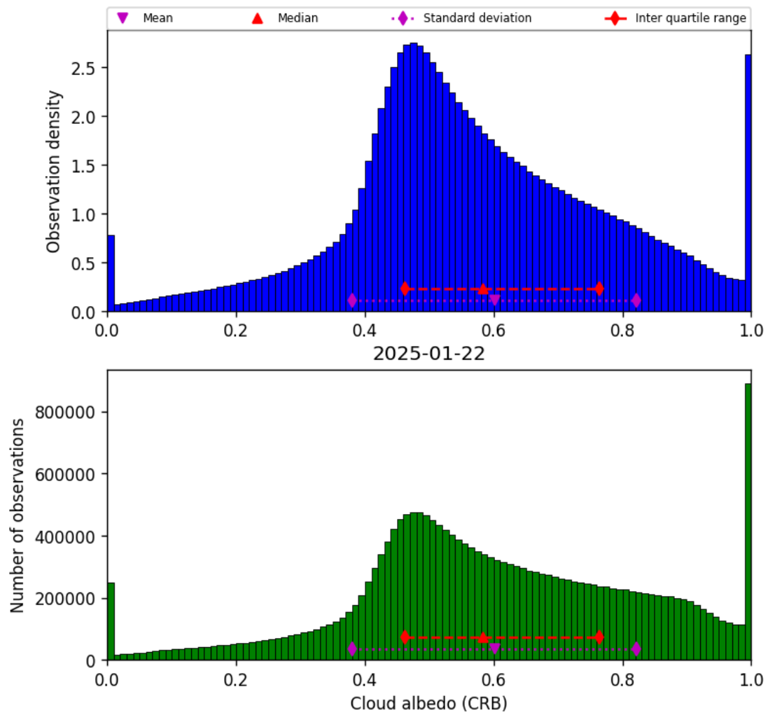
Figure 42: Histogram of “Cloud albedo (CRB)” for 2025-01-22 to 2025-01-23
