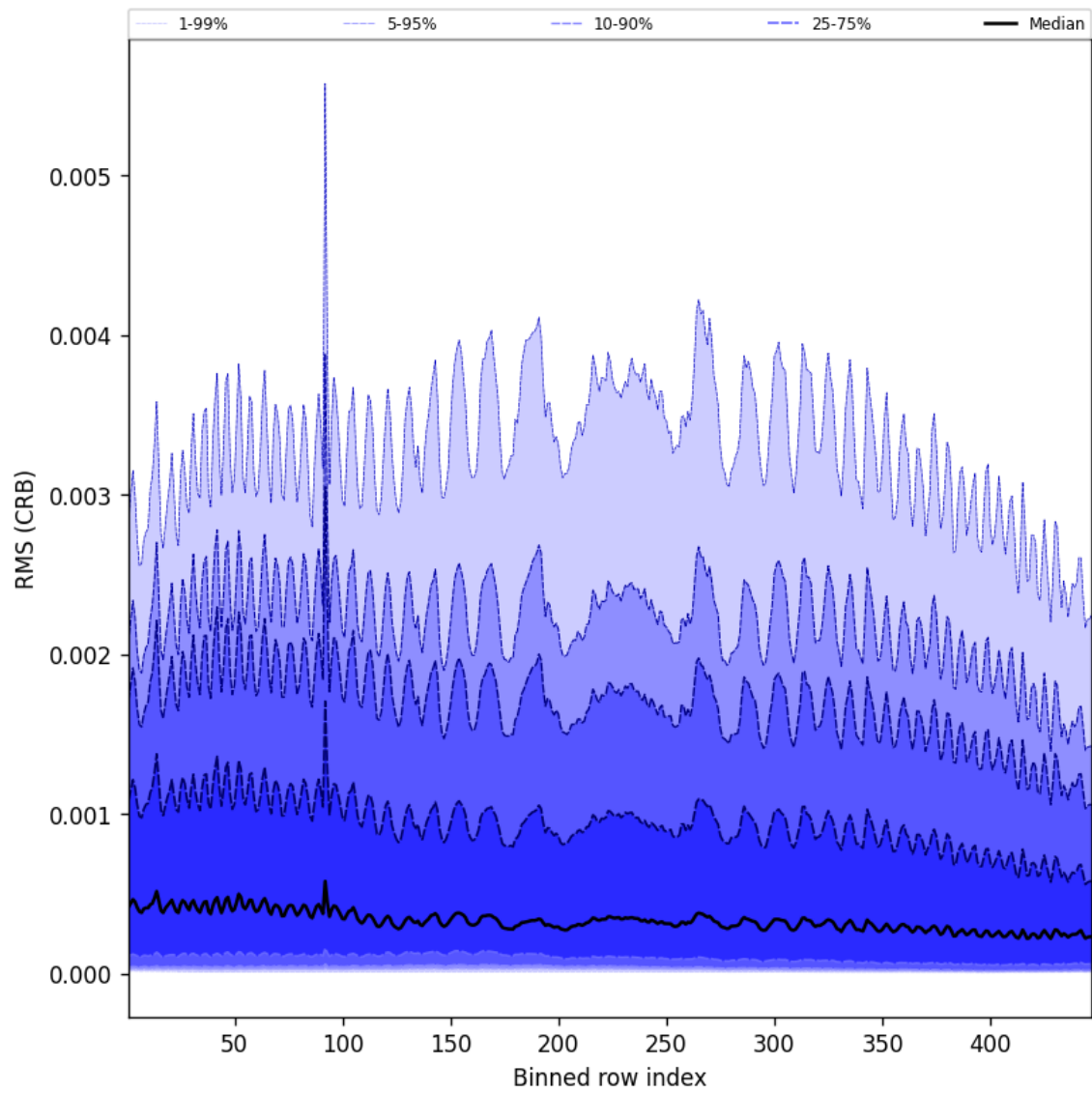
Figure 62: Along track statistics of “RMS (CRB)” for 2025-01-22 to 2025-01-23
