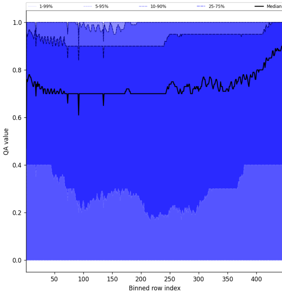
Figure 52: Along track statistics of “QA value” for 2025-01-22 to 2025-01-23
