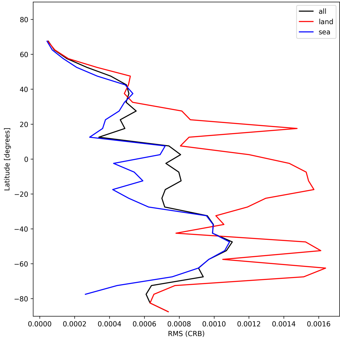
Figure 30: Zonal average of “RMS (CRB)” for 2025-01-22 to 2025-01-23.
