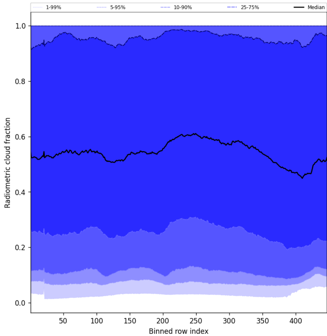
Figure 53: Along track statistics of “Radiometric cloud fraction” for 2025-01-22 to 2025-01-23
