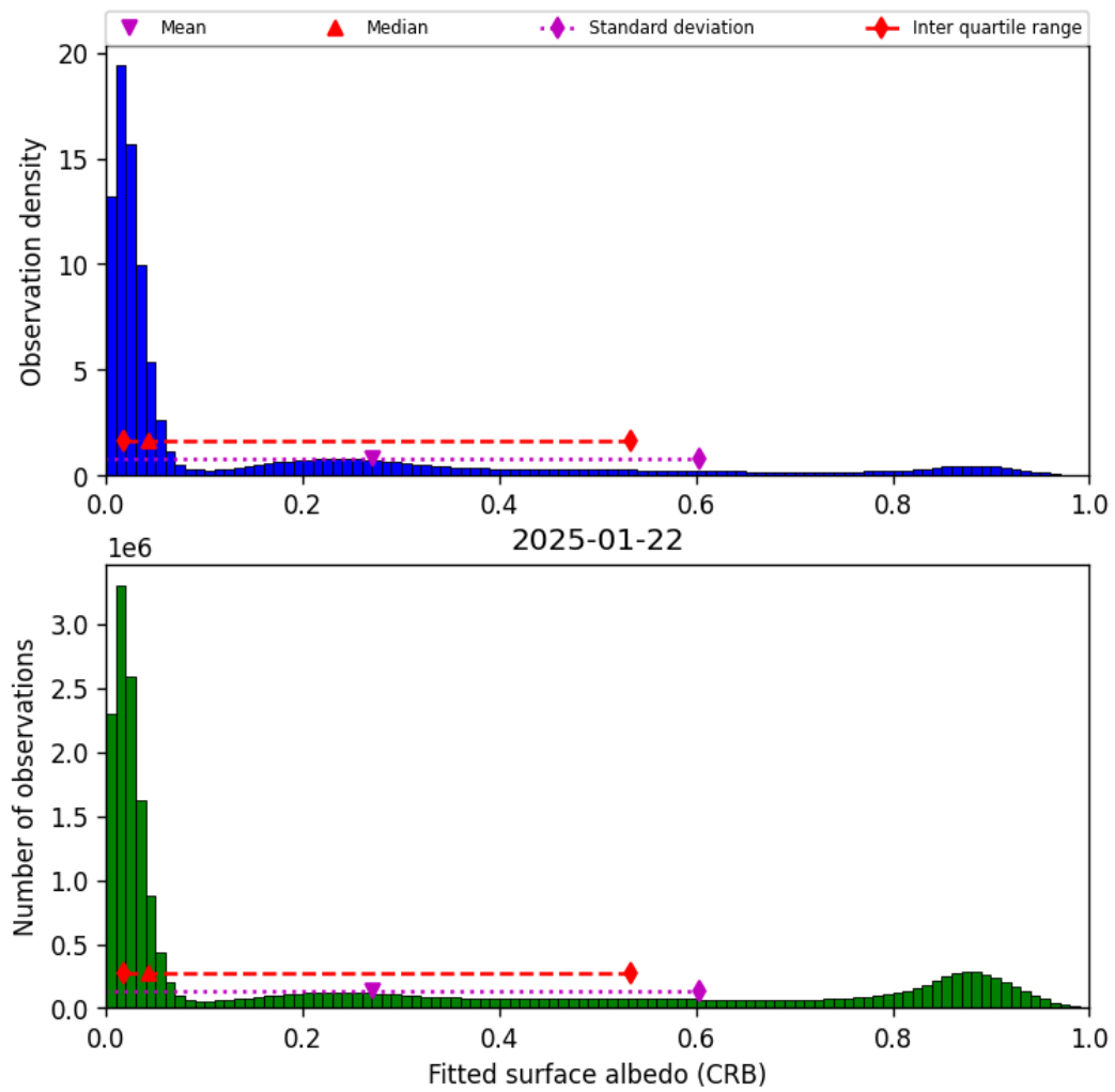
Figure 44: Histogram of “Fitted surface albedo (CRB)” for 2025-01-22 to 2025-01-23
