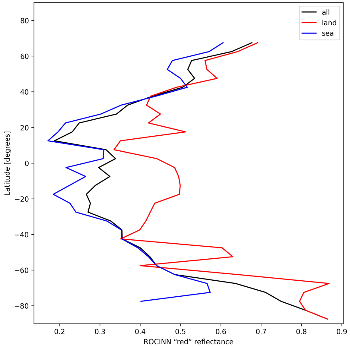
Figure 35: Zonal average of “ROCINN “red” reflectance” for 2025-01-22 to 2025-01-23.
