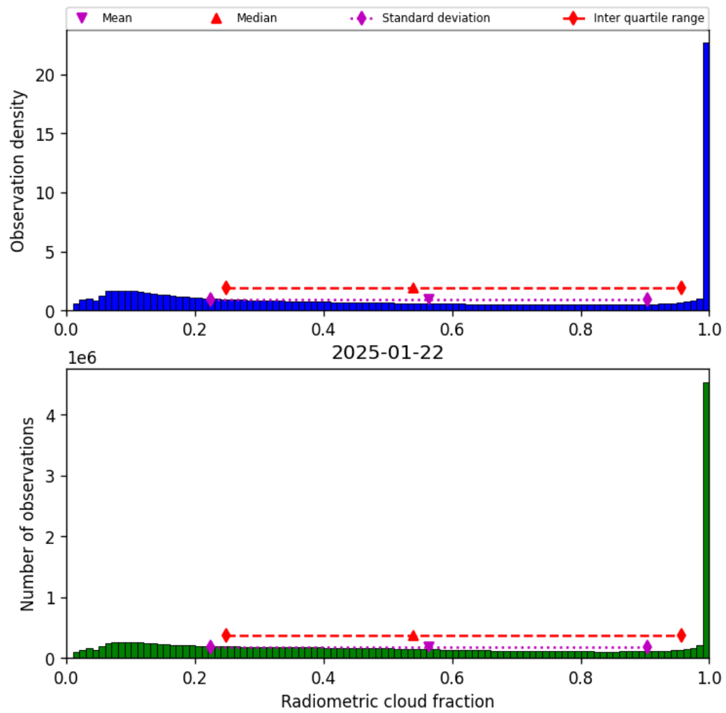
Figure 37: Histogram of “Radiometric cloud fraction” for 2025-01-22 to 2025-01-23
