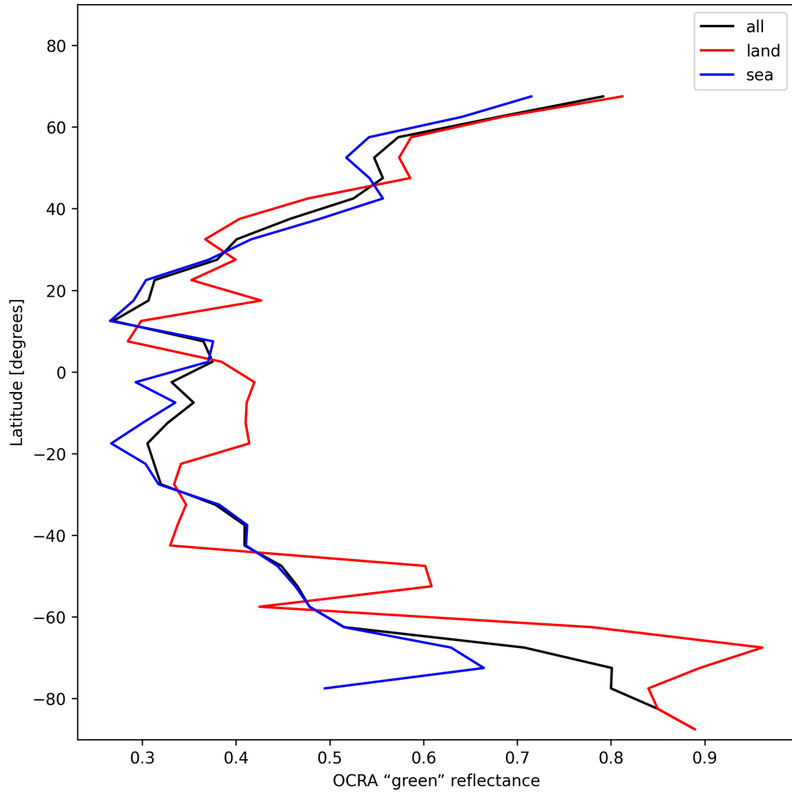
Figure 34: Zonal average of “OCRA “green” reflectance” for 2025-01-22 to 2025-01-23.
