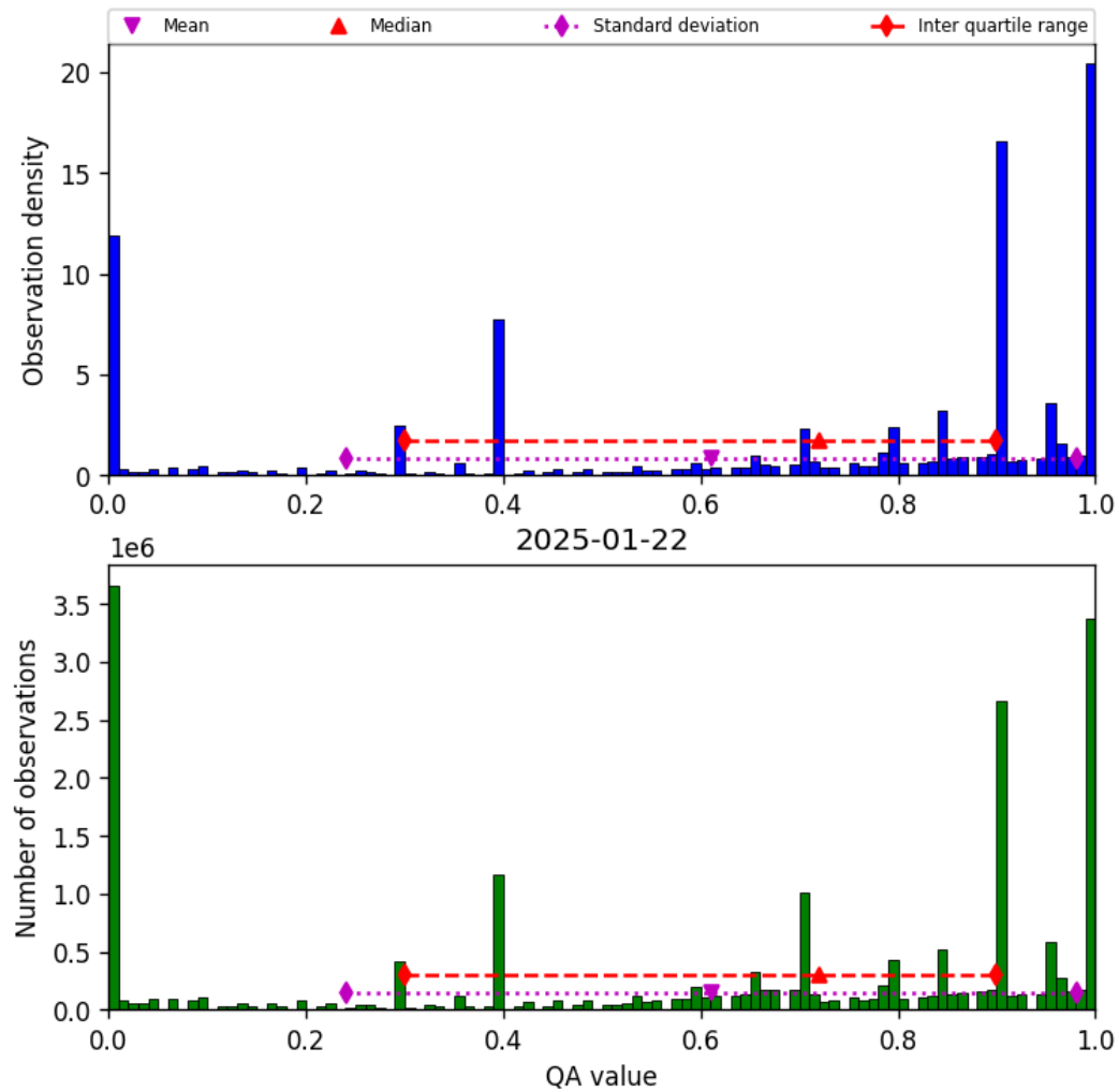
Figure 36: Histogram of “QA value” for 2025-01-22 to 2025-01-23
