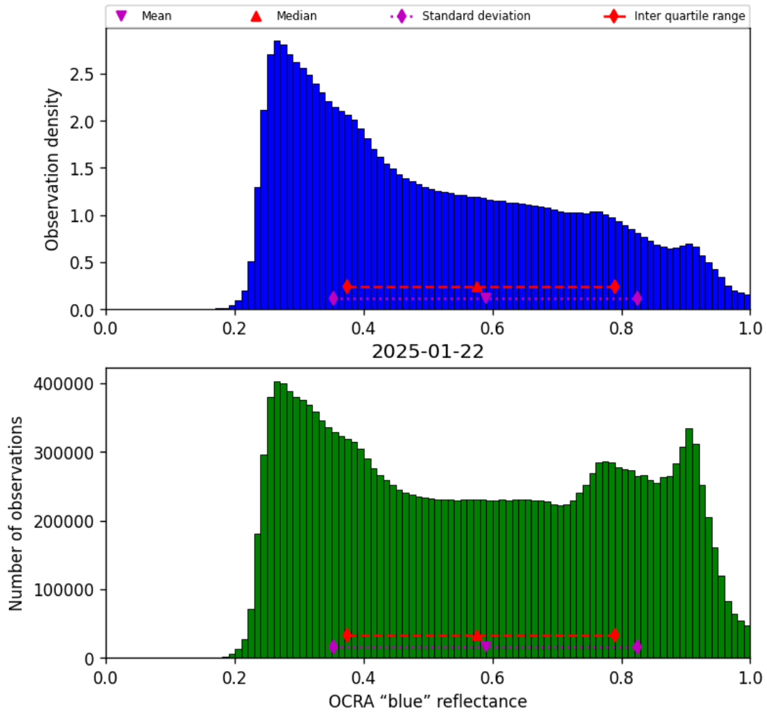
Figure 49: Histogram of “OCRA “blue” reflectance” for 2025-01-22 to 2025-01-23
