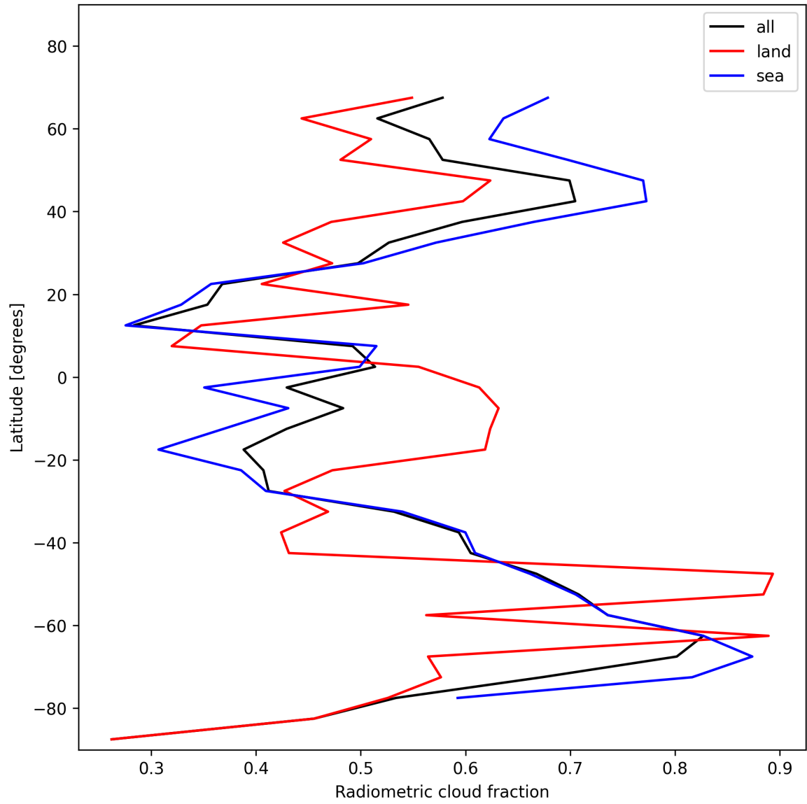
Figure 21: Zonal average of “Radiometric cloud fraction” for 2025-01-22 to 2025-01-23.
