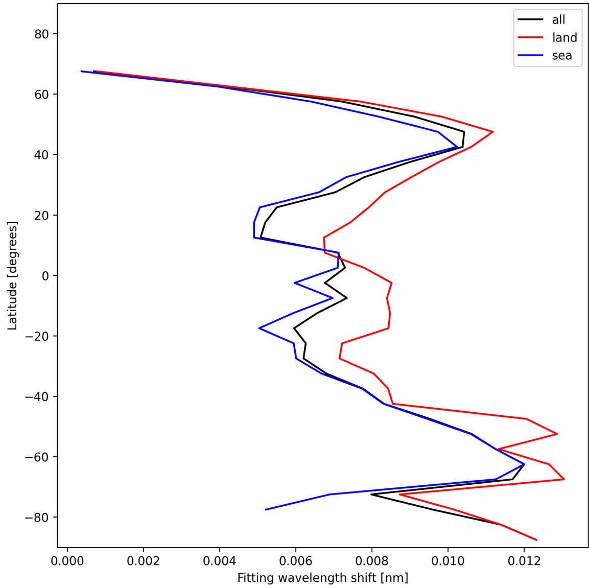
Figure 31: Zonal average of “Fitting wavelength shift” for 2025-01-22 to 2025-01-23.
