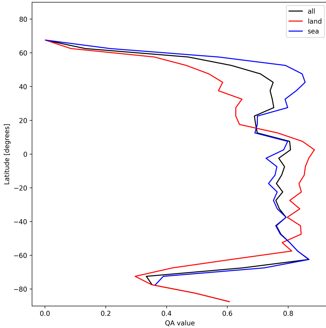
Figure 20: Zonal average of “QA value” for 2025-01-22 to 2025-01-23.
