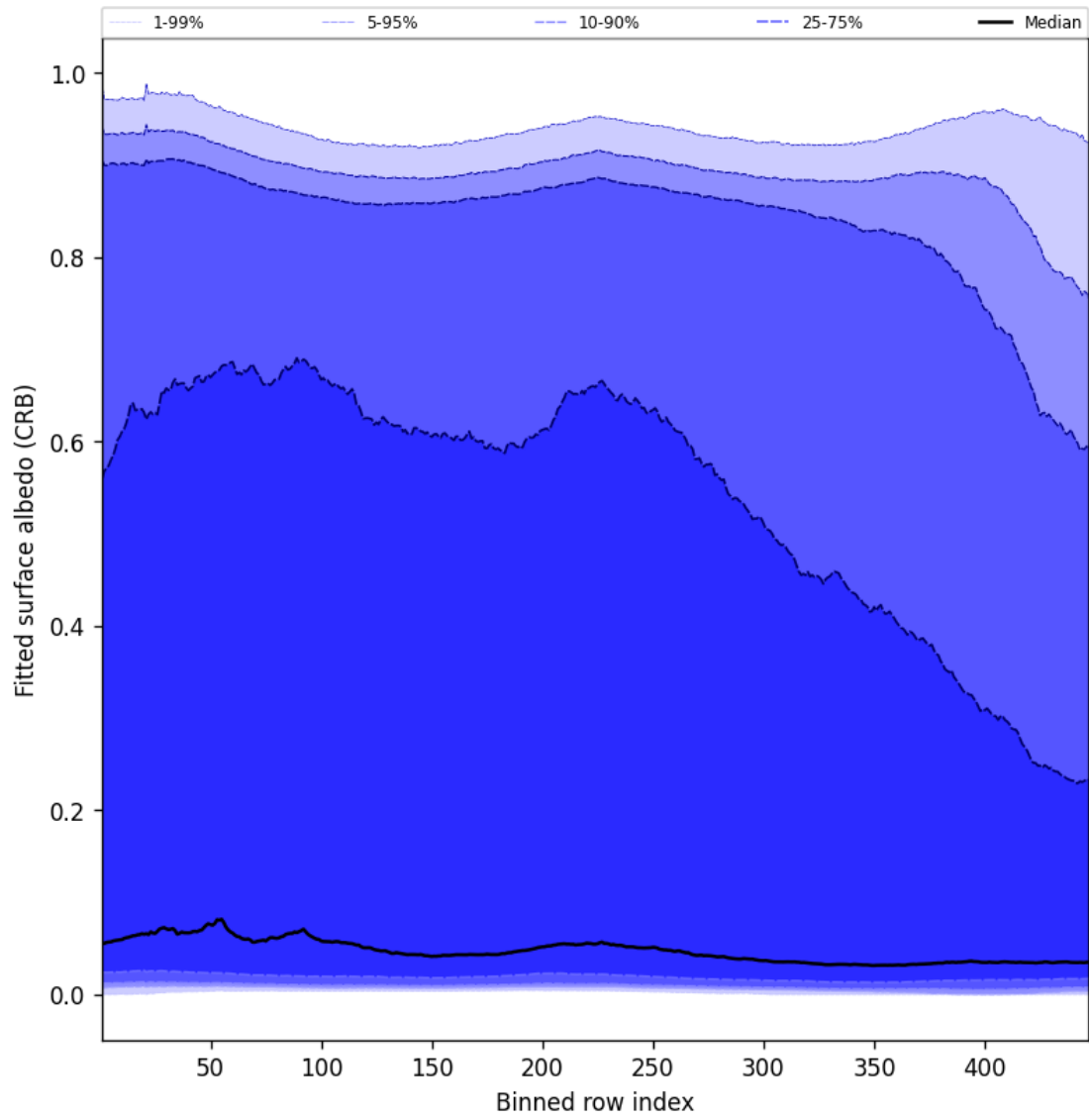
Figure 60: Along track statistics of “Fitted surface albedo (CRB)” for 2025-01-22 to 2025-01-23
