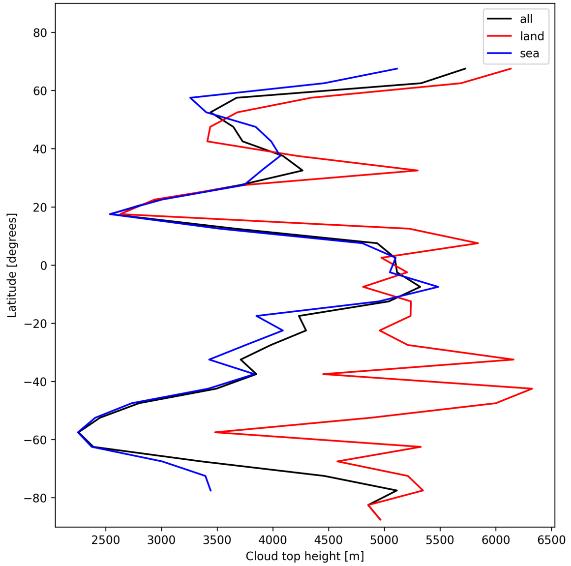
Figure 22: Zonal average of “Cloud top height” for 2025-01-22 to 2025-01-23.
