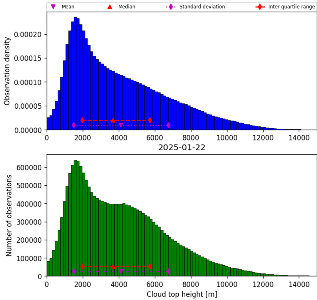
Figure 38: Histogram of “Cloud top height” for 2025-01-22 to 2025-01-23
