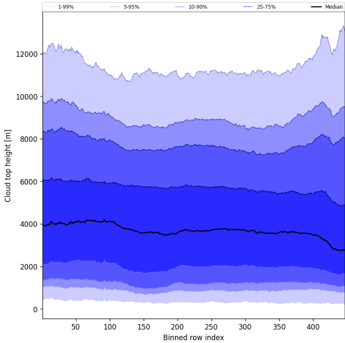
Figure 54: Along track statistics of “Cloud top height” for 2025-01-22 to 2025-01-23
