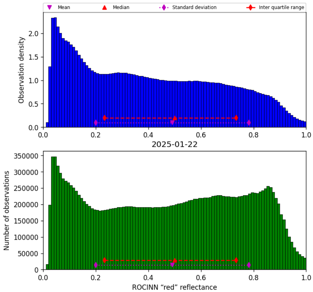
Figure 51: Histogram of “ROCINN “red” reflectance” for 2025-01-22 to 2025-01-23
