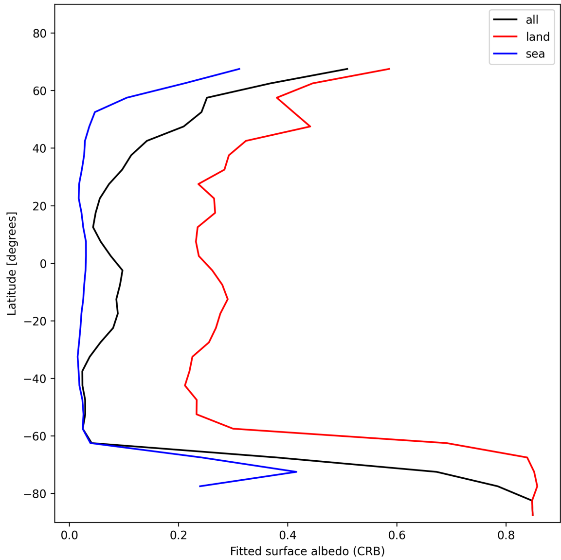
Figure 28: Zonal average of “Fitted surface albedo (CRB)” for 2025-01-22 to 2025-01-23.
