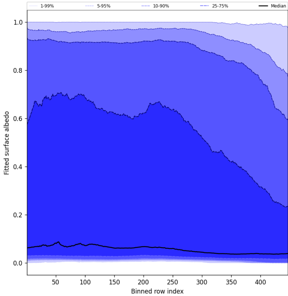
Figure 59: Along track statistics of “Fitted surface albedo” for 2025-01-22 to 2025-01-23
