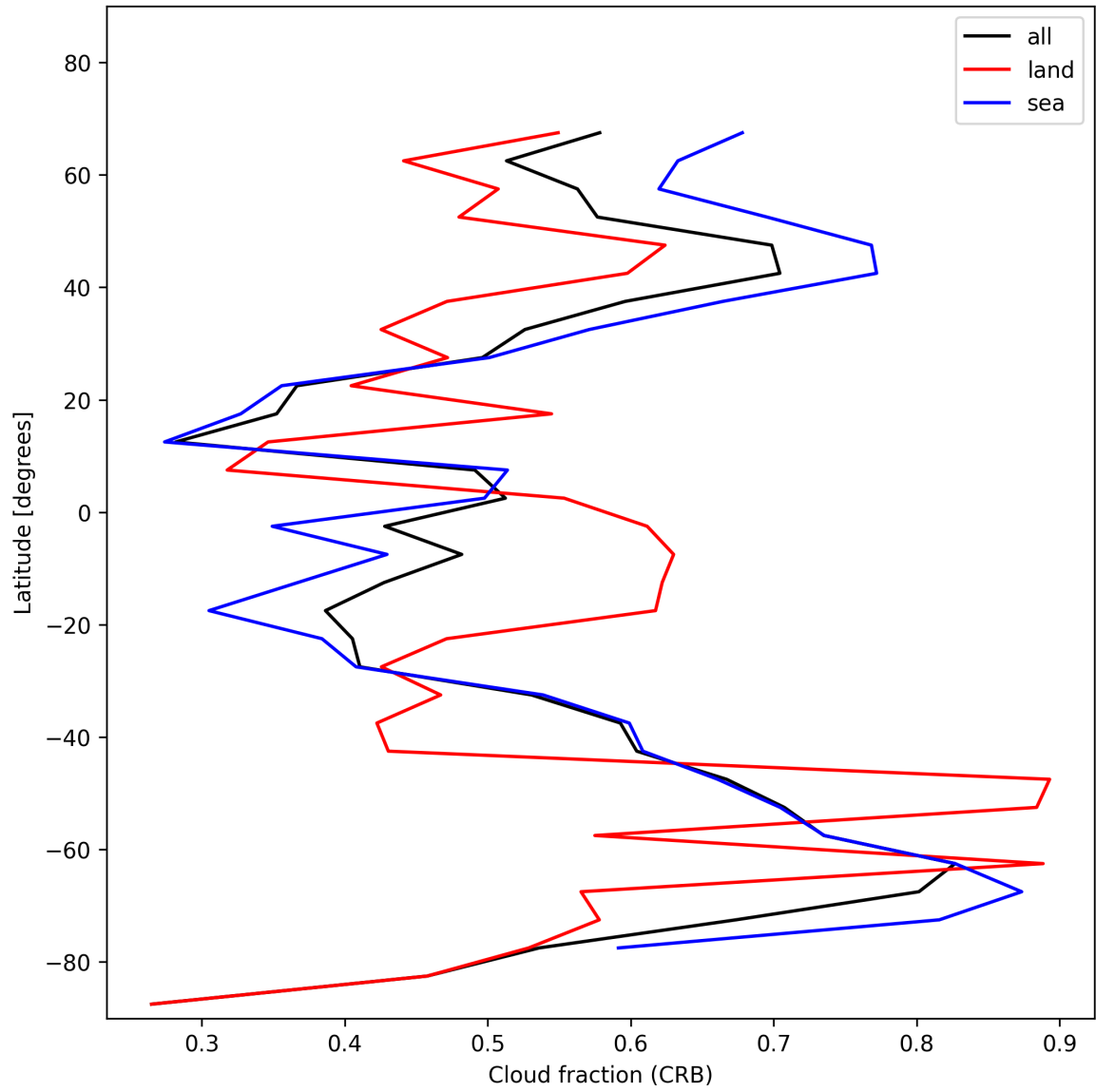
Figure 24: Zonal average of “Cloud fraction (CRB)” for 2025-01-22 to 2025-01-23.
