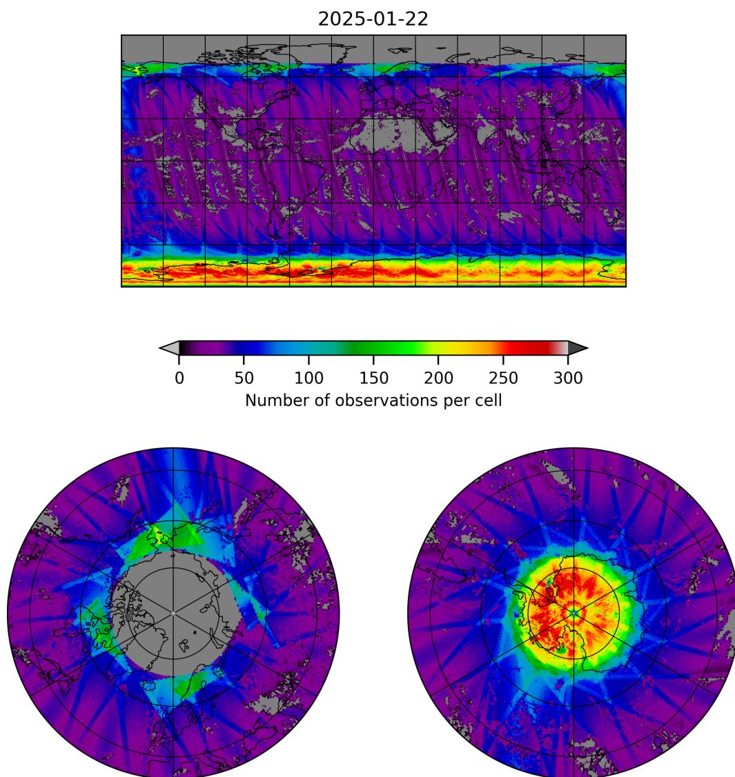
Figure 19: Map of the number of observations for 2025-01-22 to 2025-01-23
