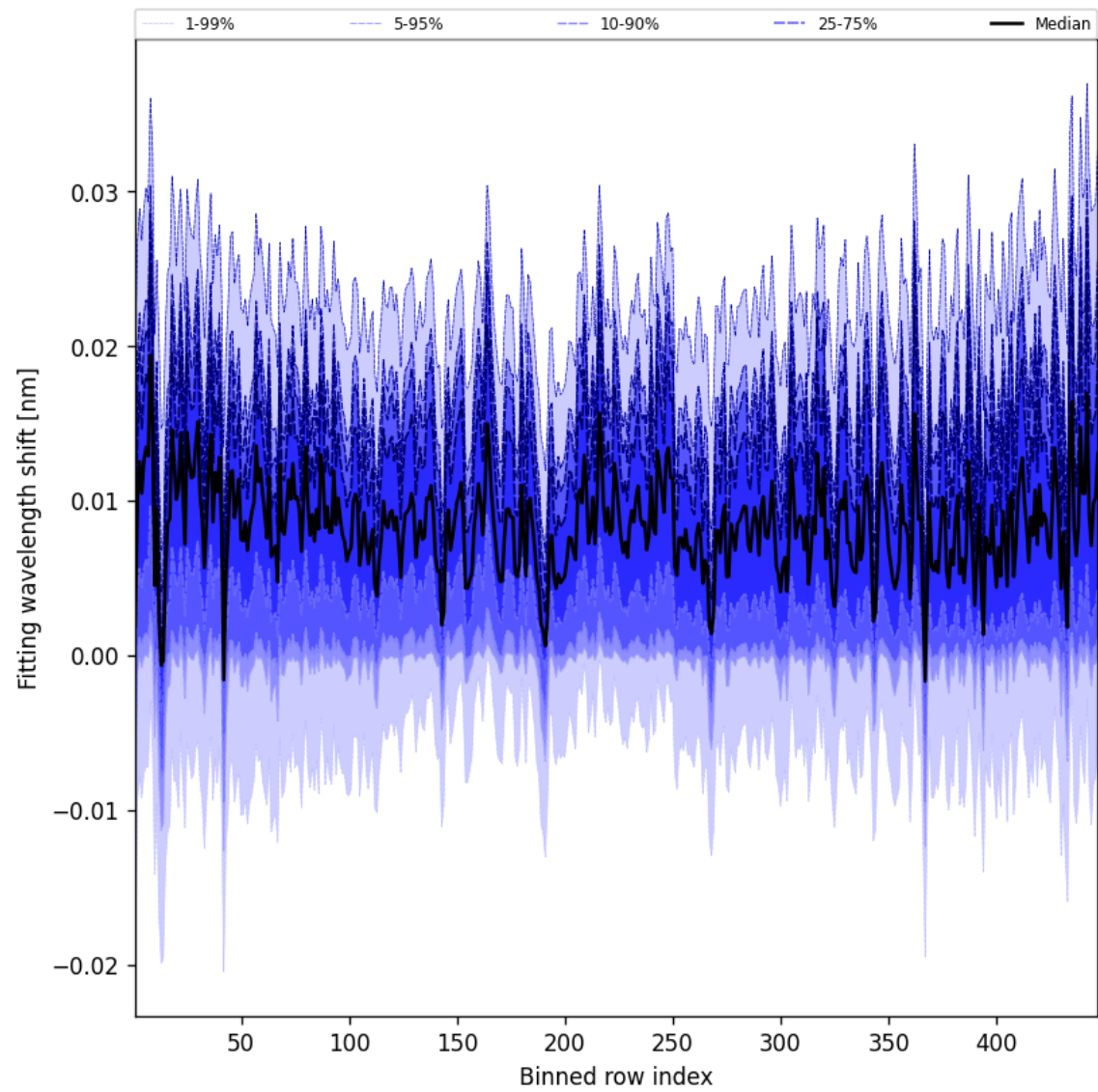
Figure 63: Along track statistics of “Fitting wavelength shift” for 2025-01-23 to 2025-01-24
