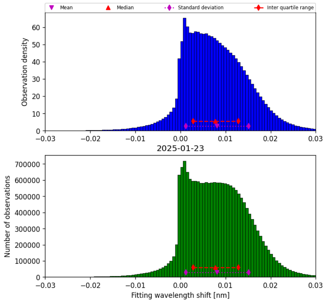
Figure 47: Histogram of “Fitting wavelength shift” for 2025-01-23 to 2025-01-24
