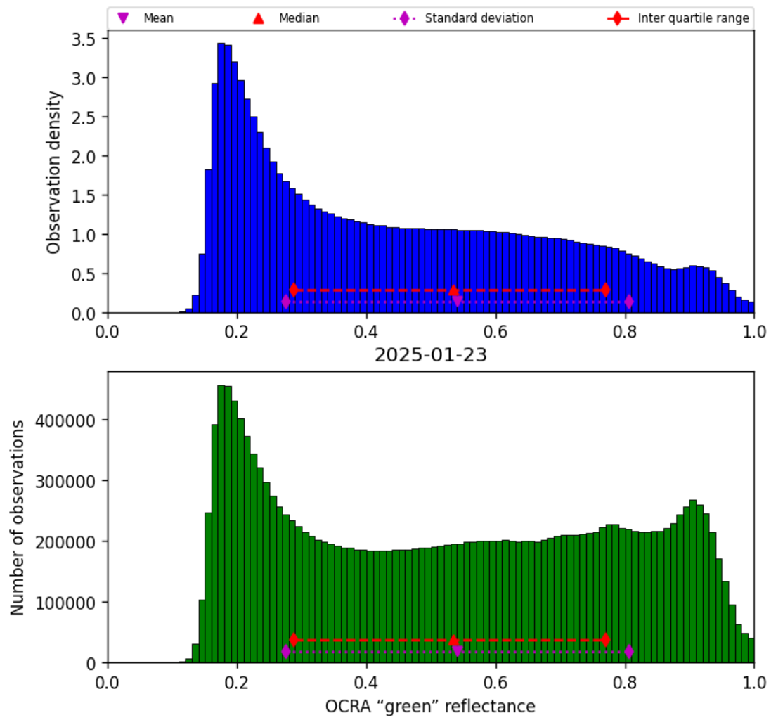
Figure 50: Histogram of “OCRA “green” reflectance” for 2025-01-23 to 2025-01-24
