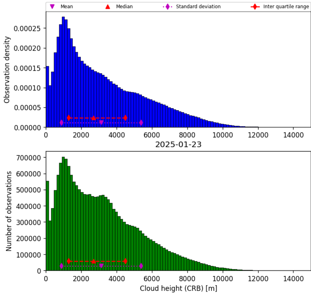
Figure 41: Histogram of “Cloud height (CRB)” for 2025-01-23 to 2025-01-24
