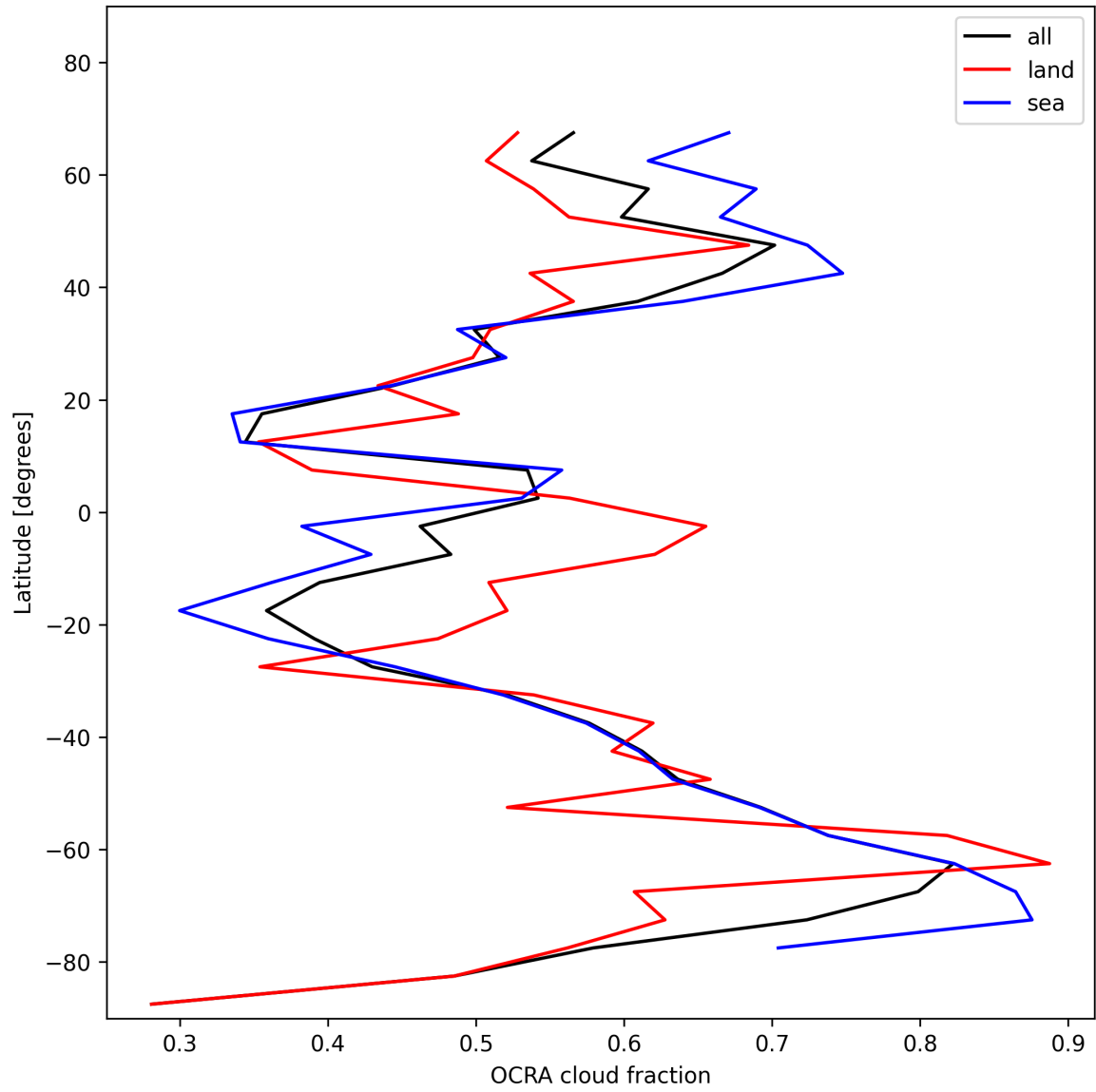
Figure 32: Zonal average of “OCRA cloud fraction” for 2025-01-23 to 2025-01-24.
