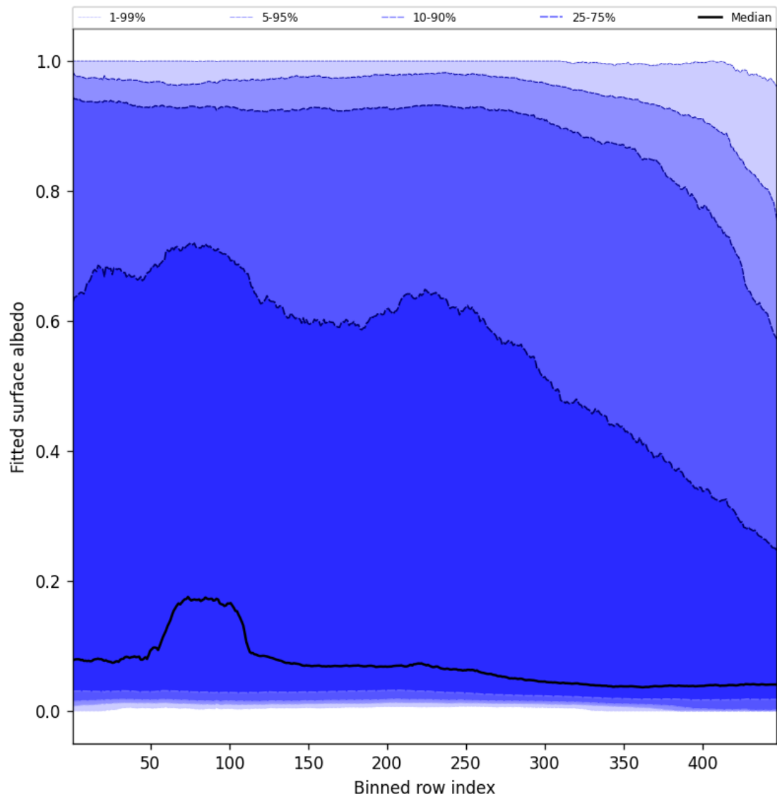
Figure 59: Along track statistics of “Fitted surface albedo” for 2025-01-23 to 2025-01-24
