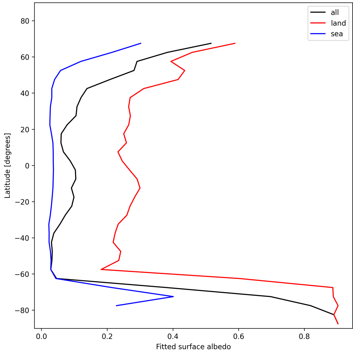
Figure 27: Zonal average of “Fitted surface albedo” for 2025-01-23 to 2025-01-24.
