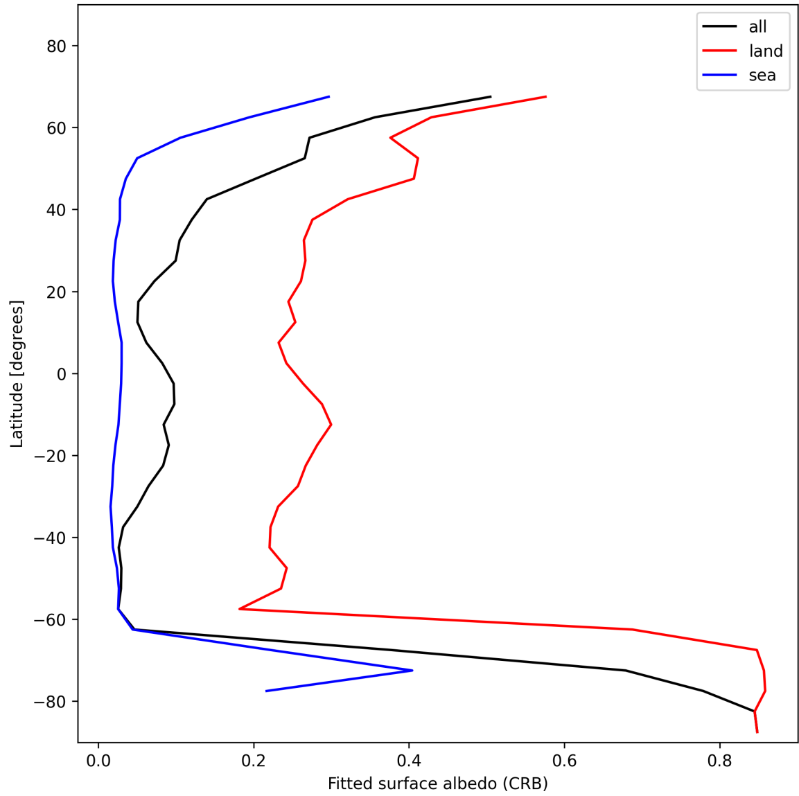
Figure 28: Zonal average of “Fitted surface albedo (CRB)” for 2025-01-23 to 2025-01-24.
