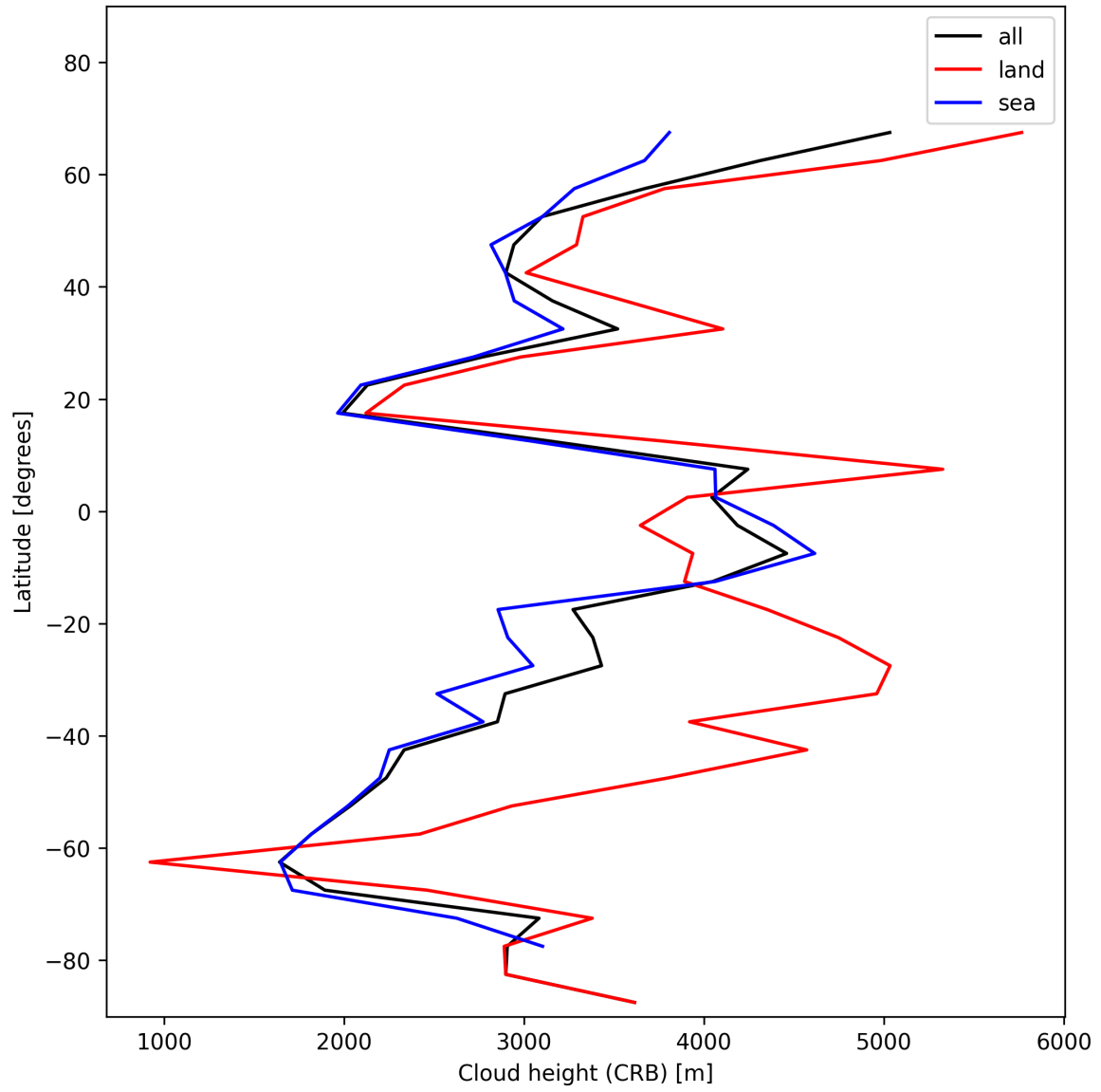
Figure 25: Zonal average of “Cloud height (CRB)” for 2025-01-23 to 2025-01-24.
