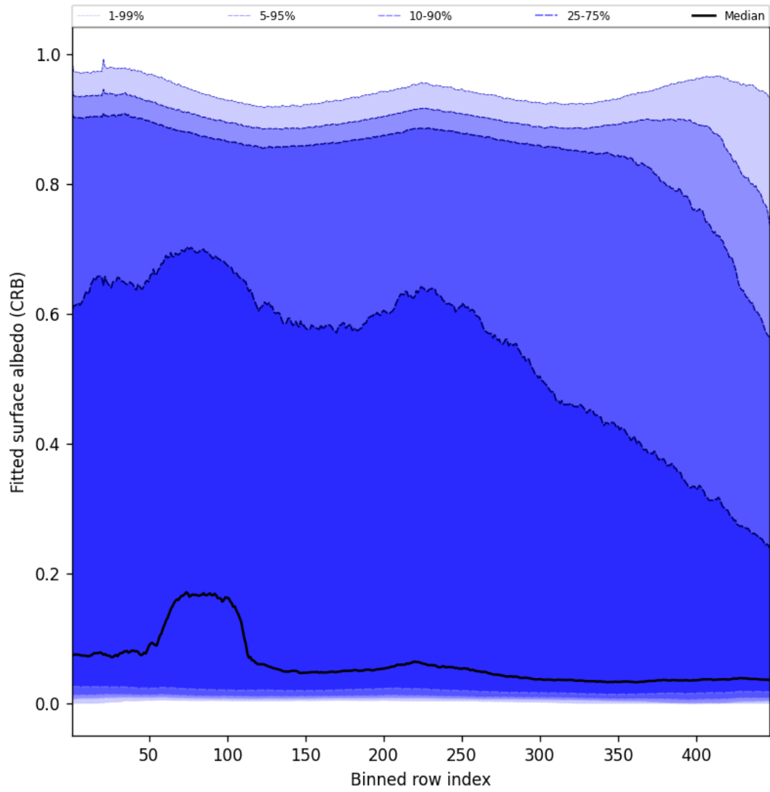
Figure 60: Along track statistics of “Fitted surface albedo (CRB)” for 2025-01-23 to 2025-01-24
