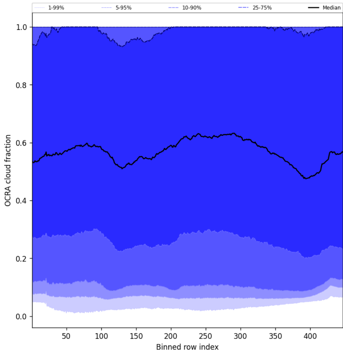
Figure 64: Along track statistics of “OCRA cloud fraction” for 2025-01-23 to 2025-01-24
