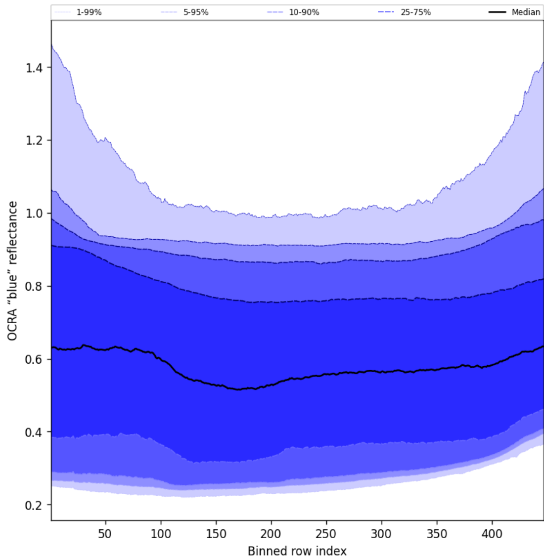
Figure 65: Along track statistics of “OCRA “blue” reflectance” for 2025-01-23 to 2025-01-24
