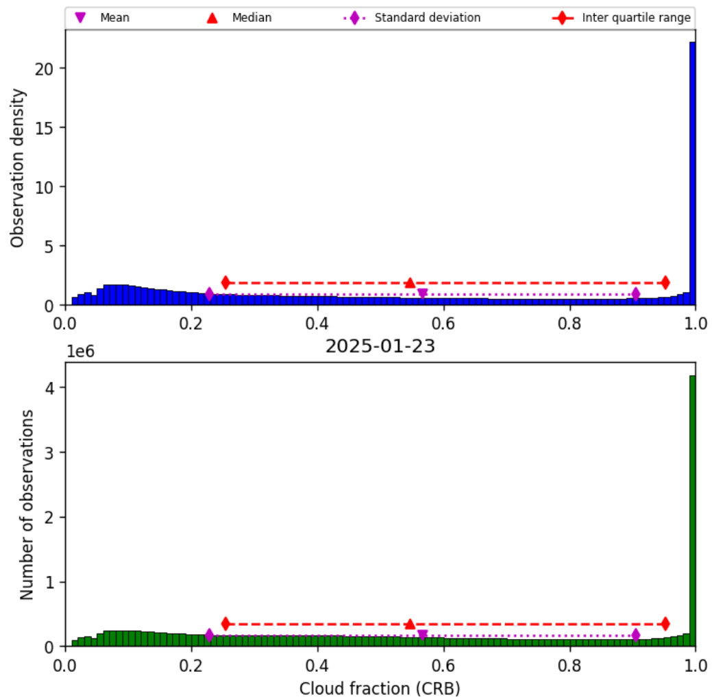
Figure 40: Histogram of “Cloud fraction (CRB)” for 2025-01-23 to 2025-01-24
