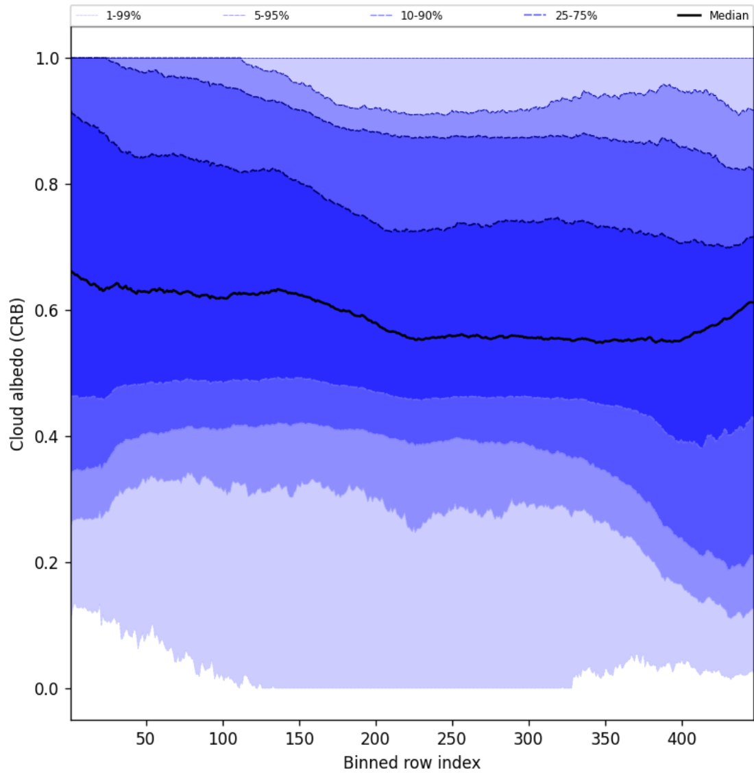
Figure 58: Along track statistics of “Cloud albedo (CRB)” for 2025-01-23 to 2025-01-24
