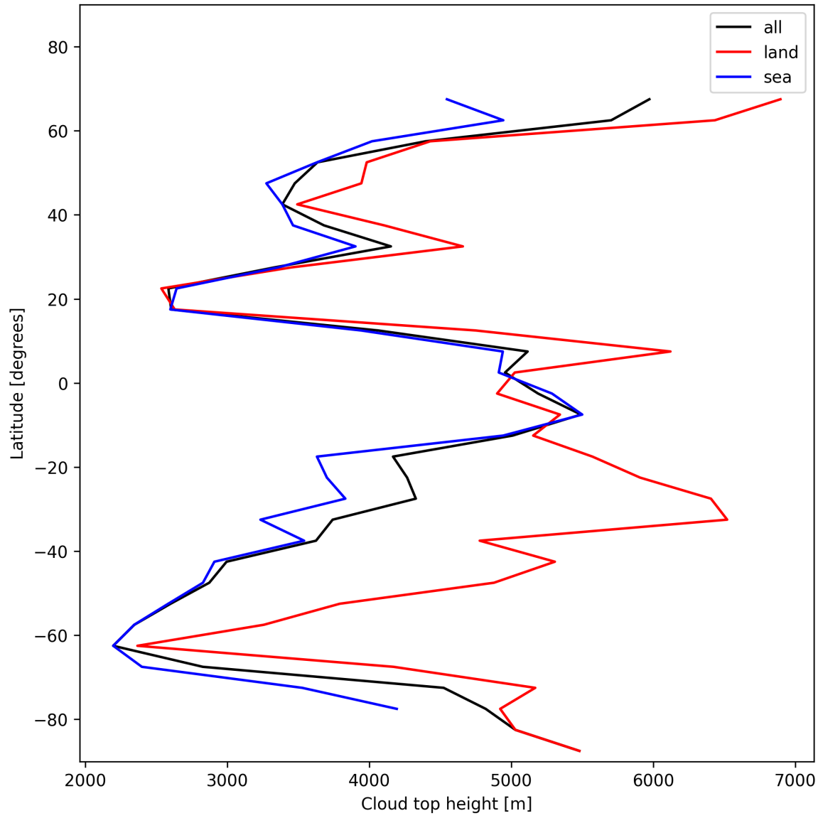
Figure 22: Zonal average of “Cloud top height” for 2025-01-23 to 2025-01-24.
