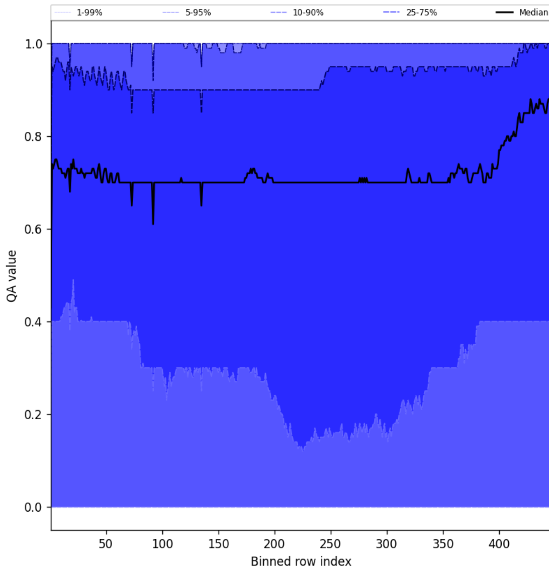
Figure 52: Along track statistics of “QA value” for 2025-01-23 to 2025-01-24
