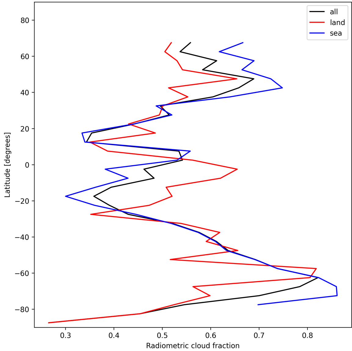
Figure 21: Zonal average of “Radiometric cloud fraction” for 2025-01-23 to 2025-01-24.
