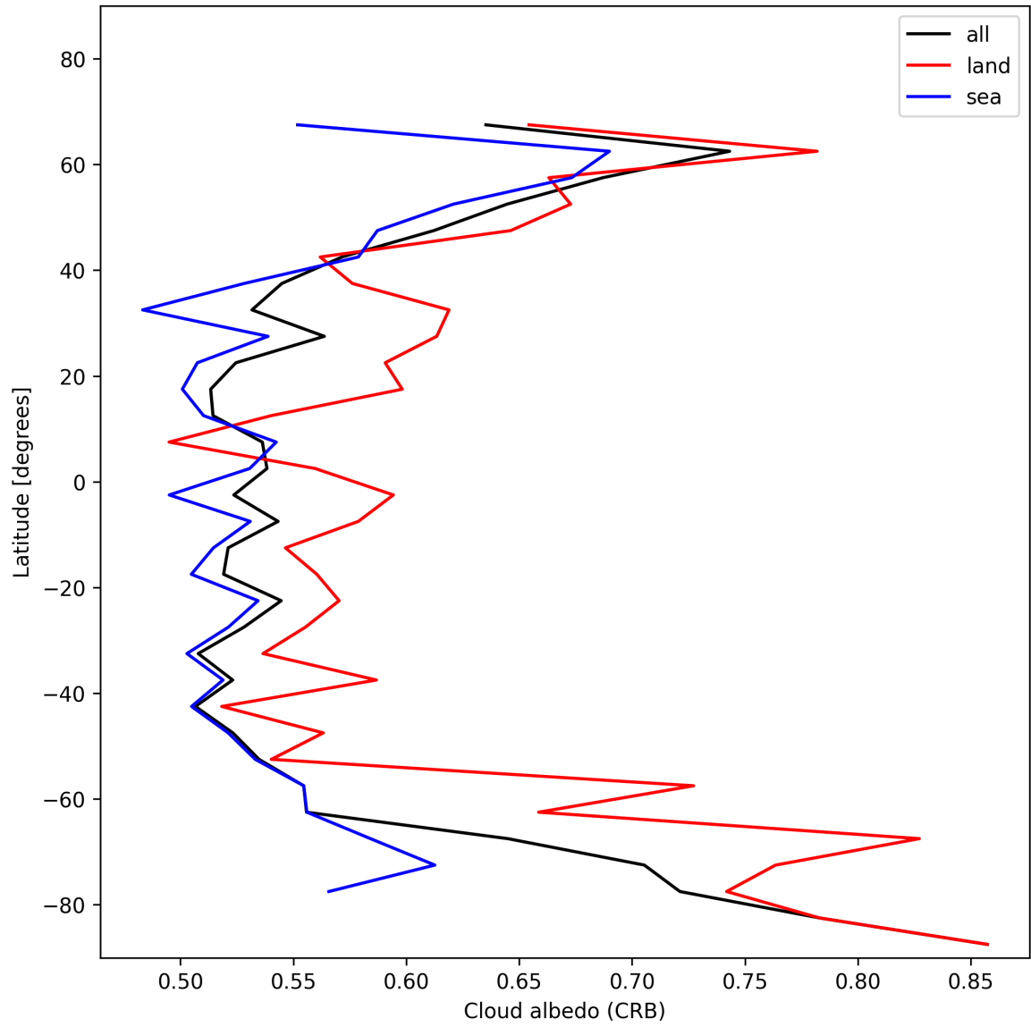
Figure 26: Zonal average of “Cloud albedo (CRB)” for 2025-01-23 to 2025-01-24.
