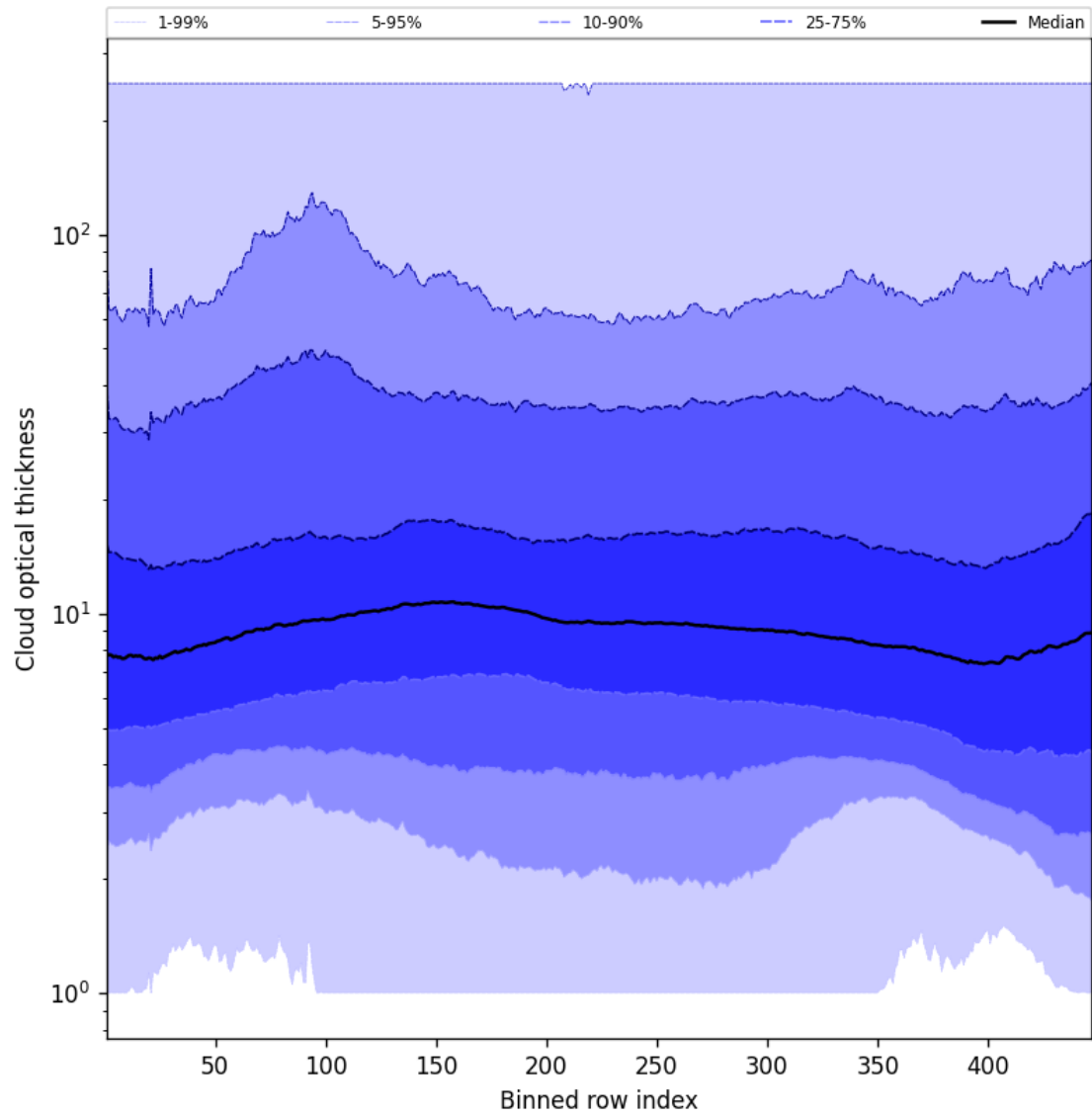
Figure 55: Along track statistics of “Cloud optical thickness” for 2025-01-23 to 2025-01-24
