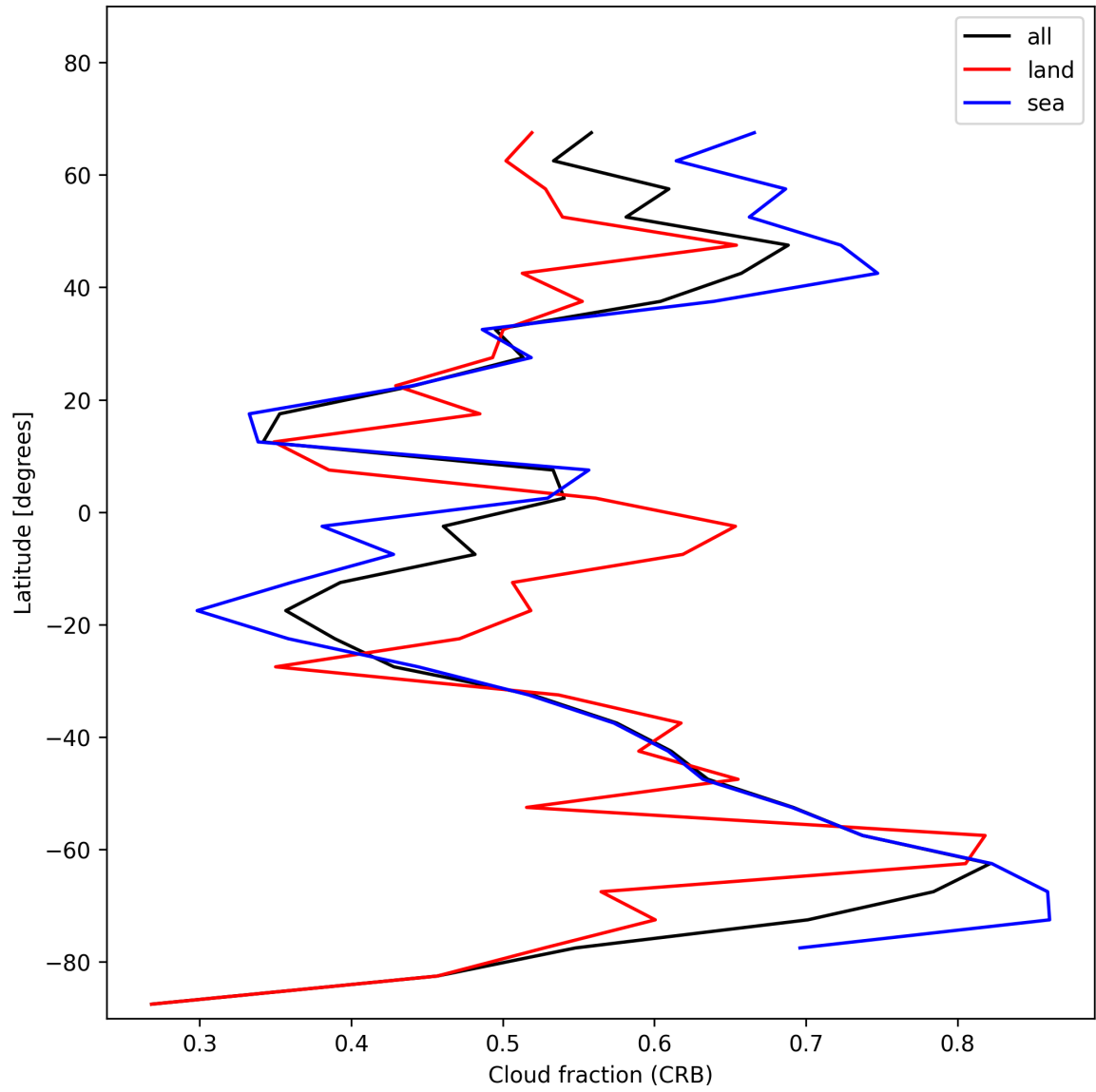
Figure 24: Zonal average of “Cloud fraction (CRB)” for 2025-01-23 to 2025-01-24.
