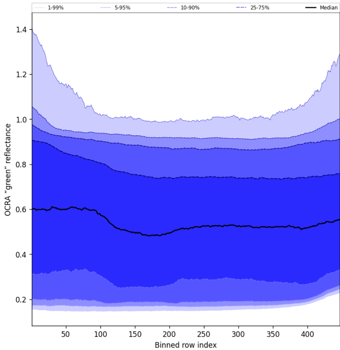
Figure 66: Along track statistics of “OCRA “green” reflectance” for 2025-01-23 to 2025-01-24
