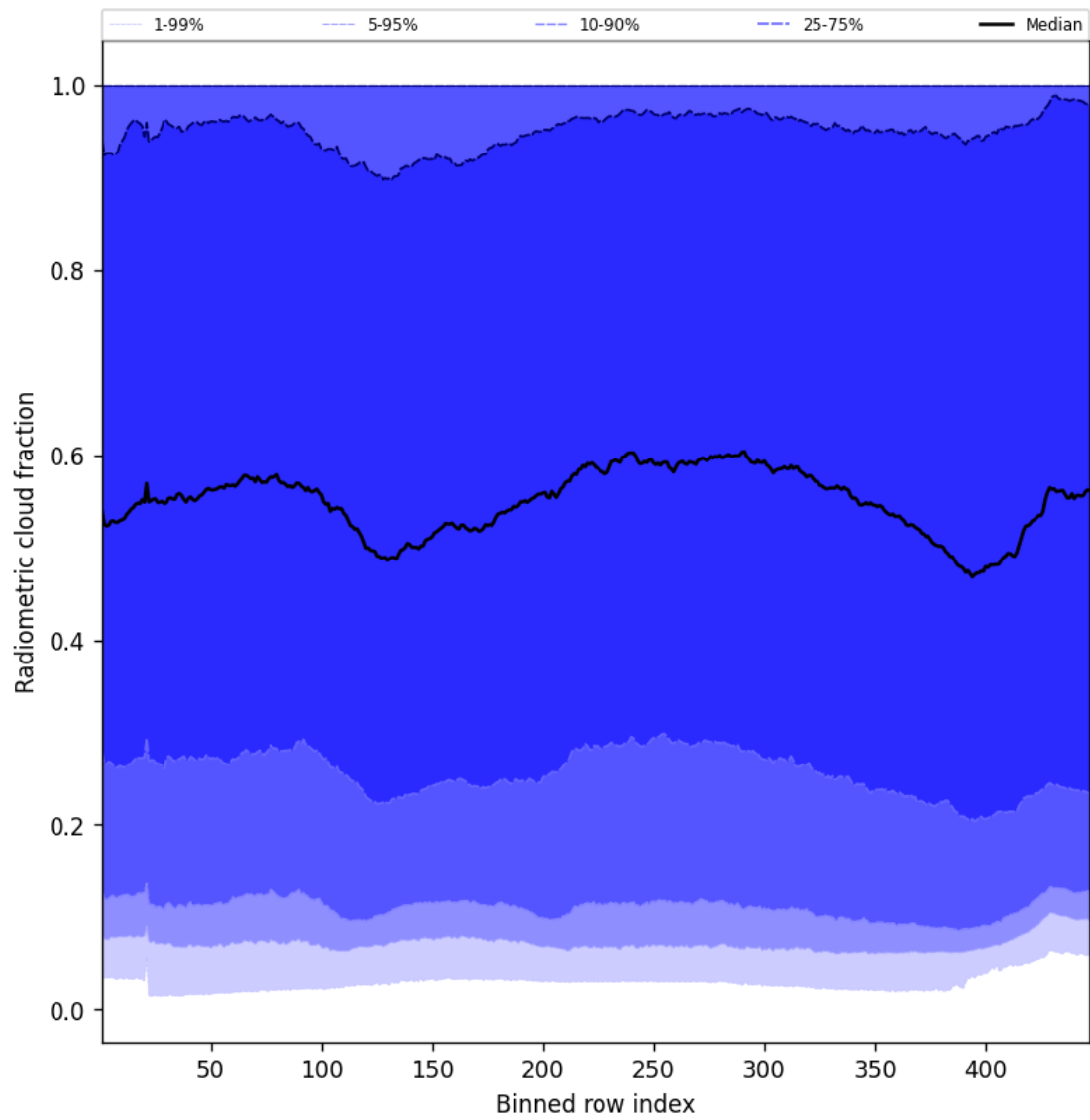
Figure 53: Along track statistics of “Radiometric cloud fraction” for 2025-01-23 to 2025-01-24
