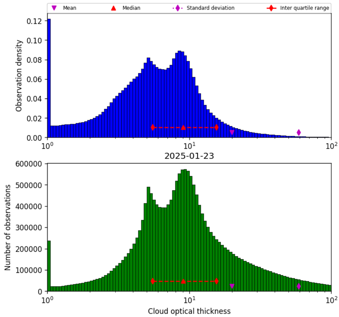
Figure 39: Histogram of “Cloud optical thickness” for 2025-01-23 to 2025-01-24
