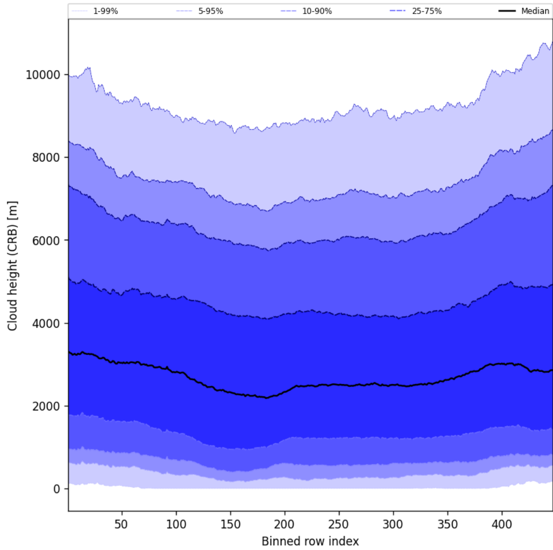
Figure 57: Along track statistics of “Cloud height (CRB)” for 2025-01-23 to 2025-01-24
