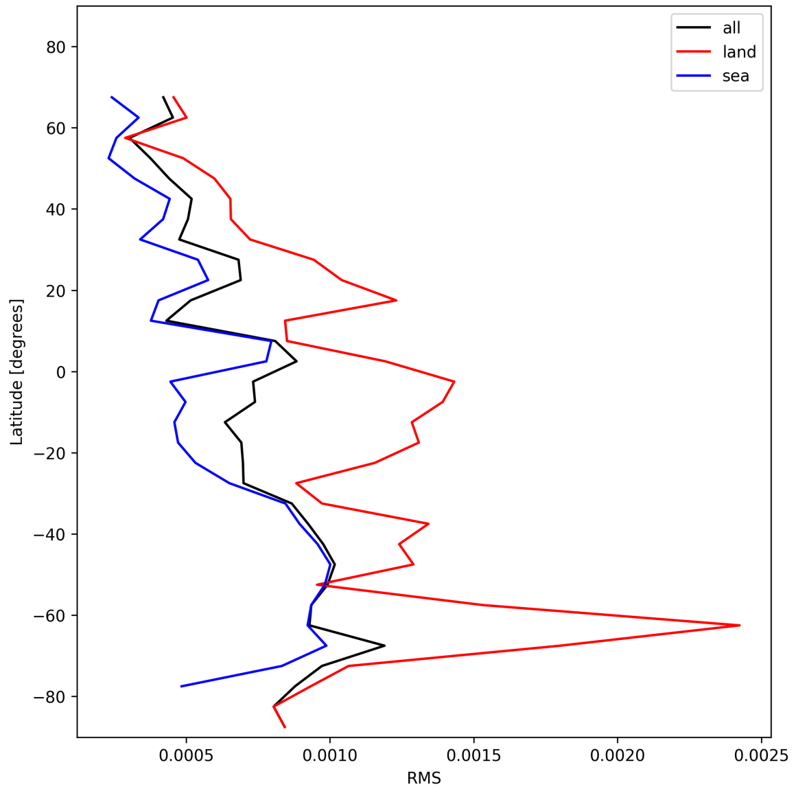
Figure 29: Zonal average of “RMS” for 2025-01-23 to 2025-01-24.
