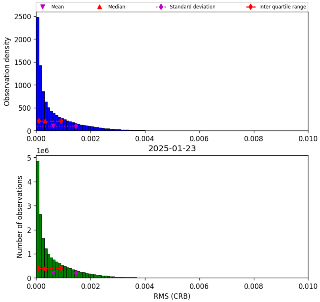
Figure 46: Histogram of “RMS (CRB)” for 2025-01-23 to 2025-01-24
