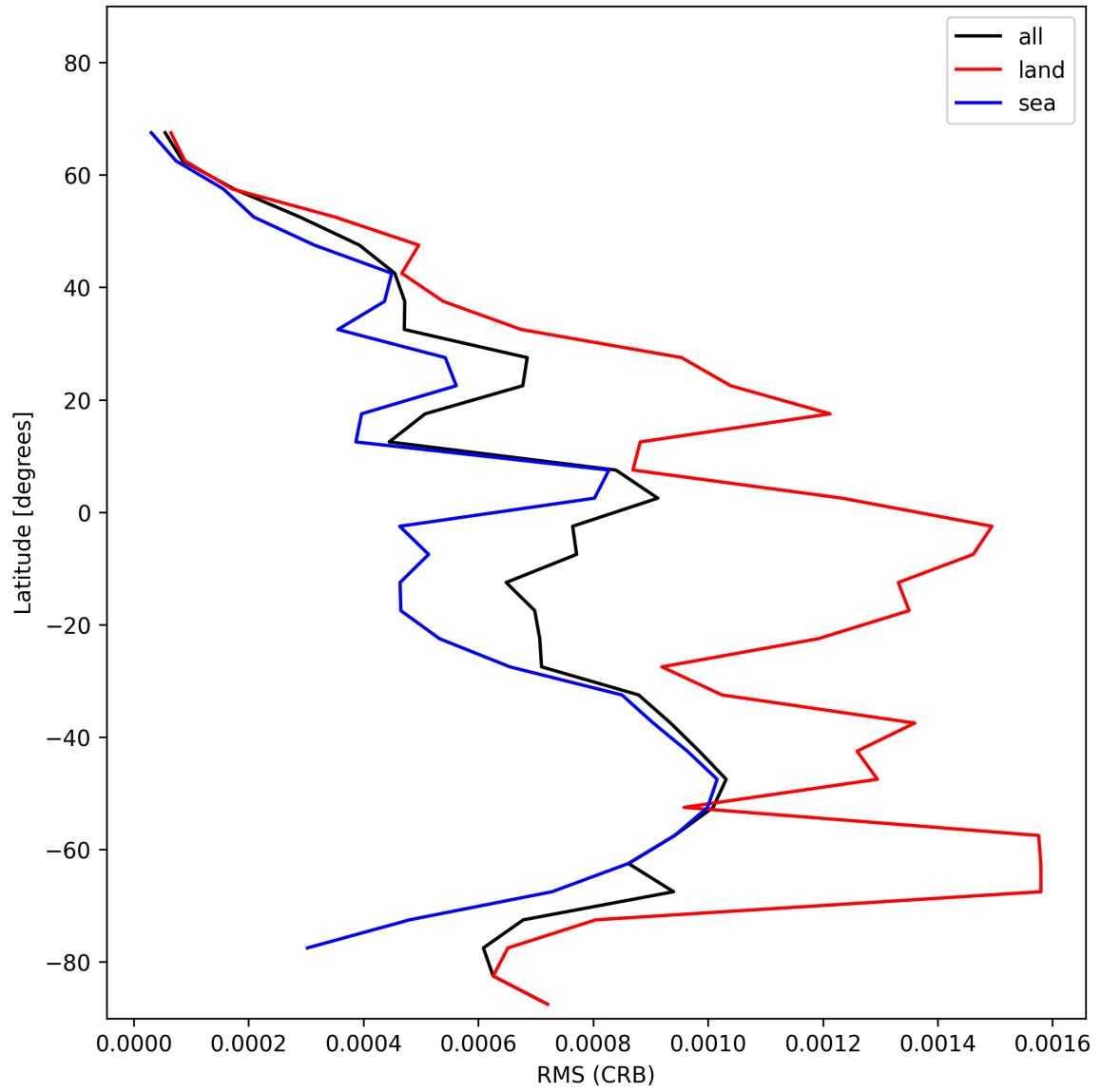
Figure 30: Zonal average of “RMS (CRB)” for 2025-01-23 to 2025-01-24.
