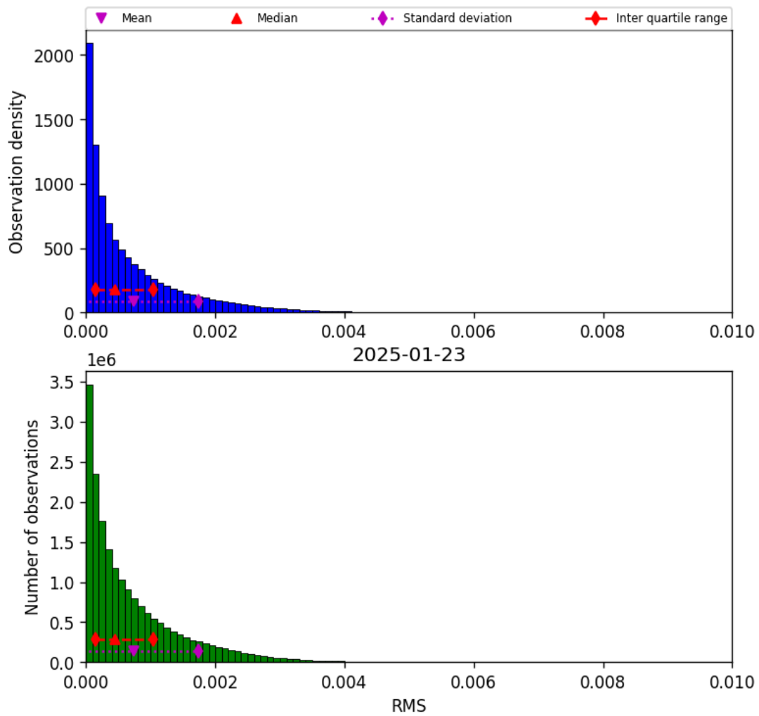
Figure 45: Histogram of “RMS” for 2025-01-23 to 2025-01-24
