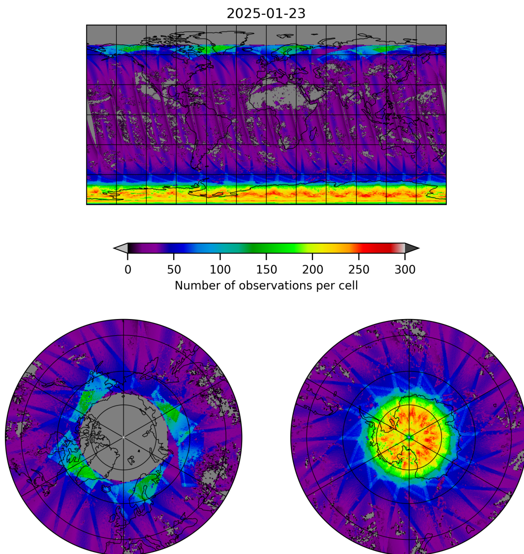
Figure 19: Map of the number of observations for 2025-01-23 to 2025-01-24
