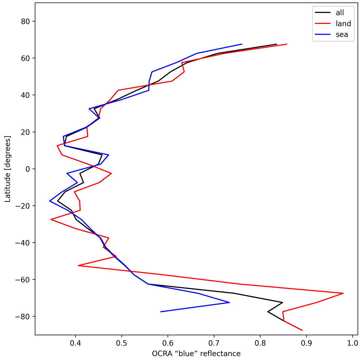
Figure 33: Zonal average of “OCRA “blue” reflectance” for 2025-01-23 to 2025-01-24.
