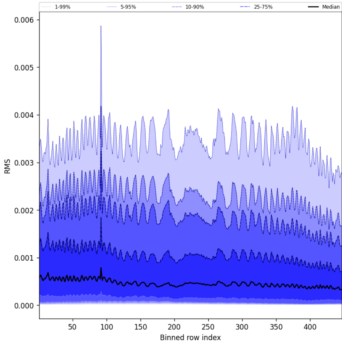
Figure 61: Along track statistics of “RMS” for 2025-01-23 to 2025-01-24
