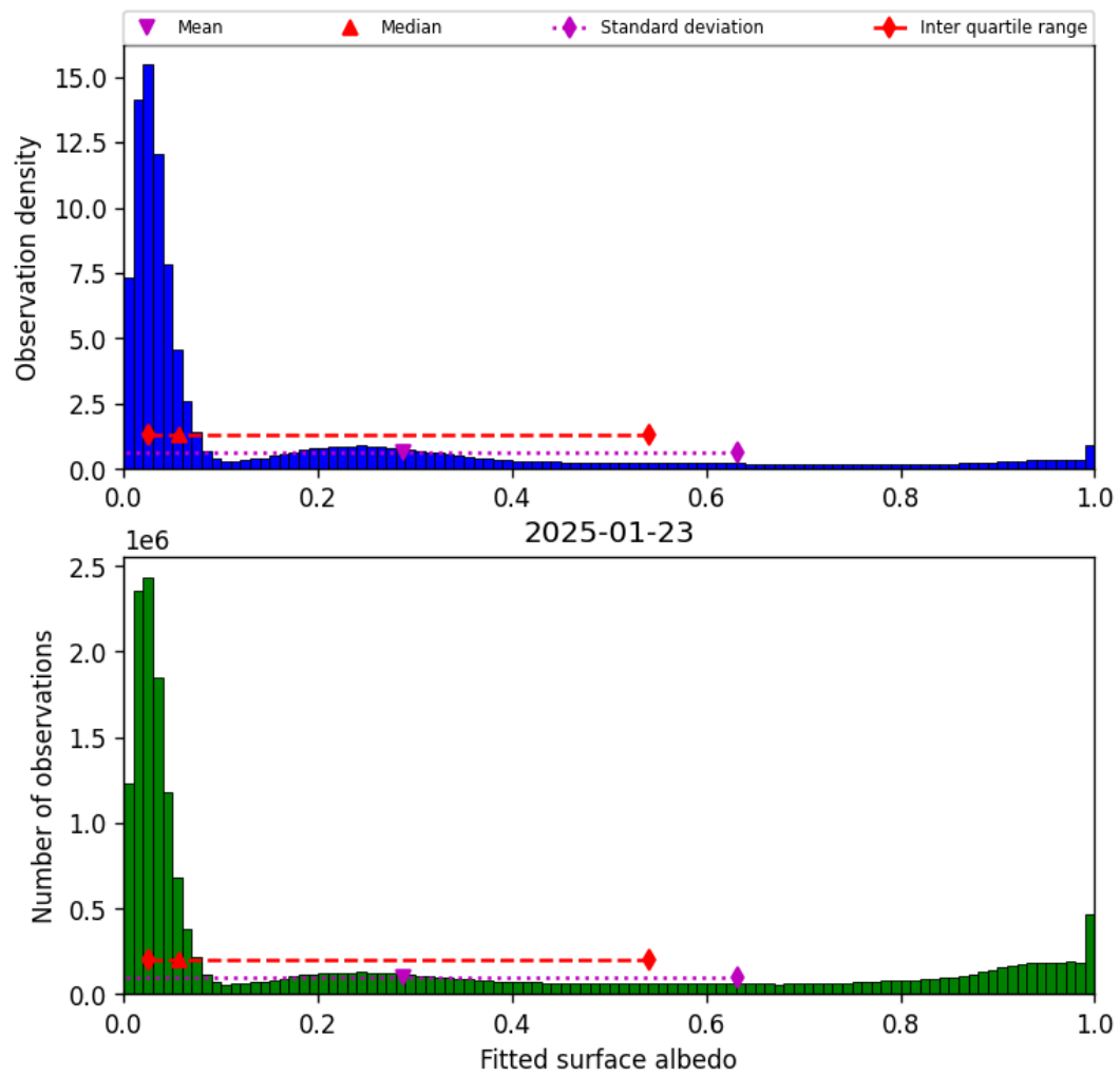
Figure 43: Histogram of “Fitted surface albedo” for 2025-01-23 to 2025-01-24
