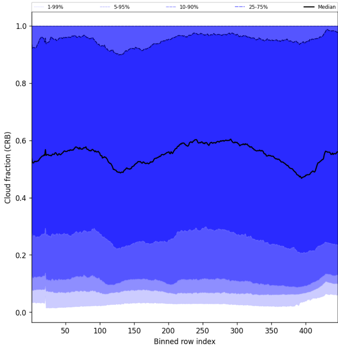
Figure 56: Along track statistics of “Cloud fraction (CRB)” for 2025-01-23 to 2025-01-24
