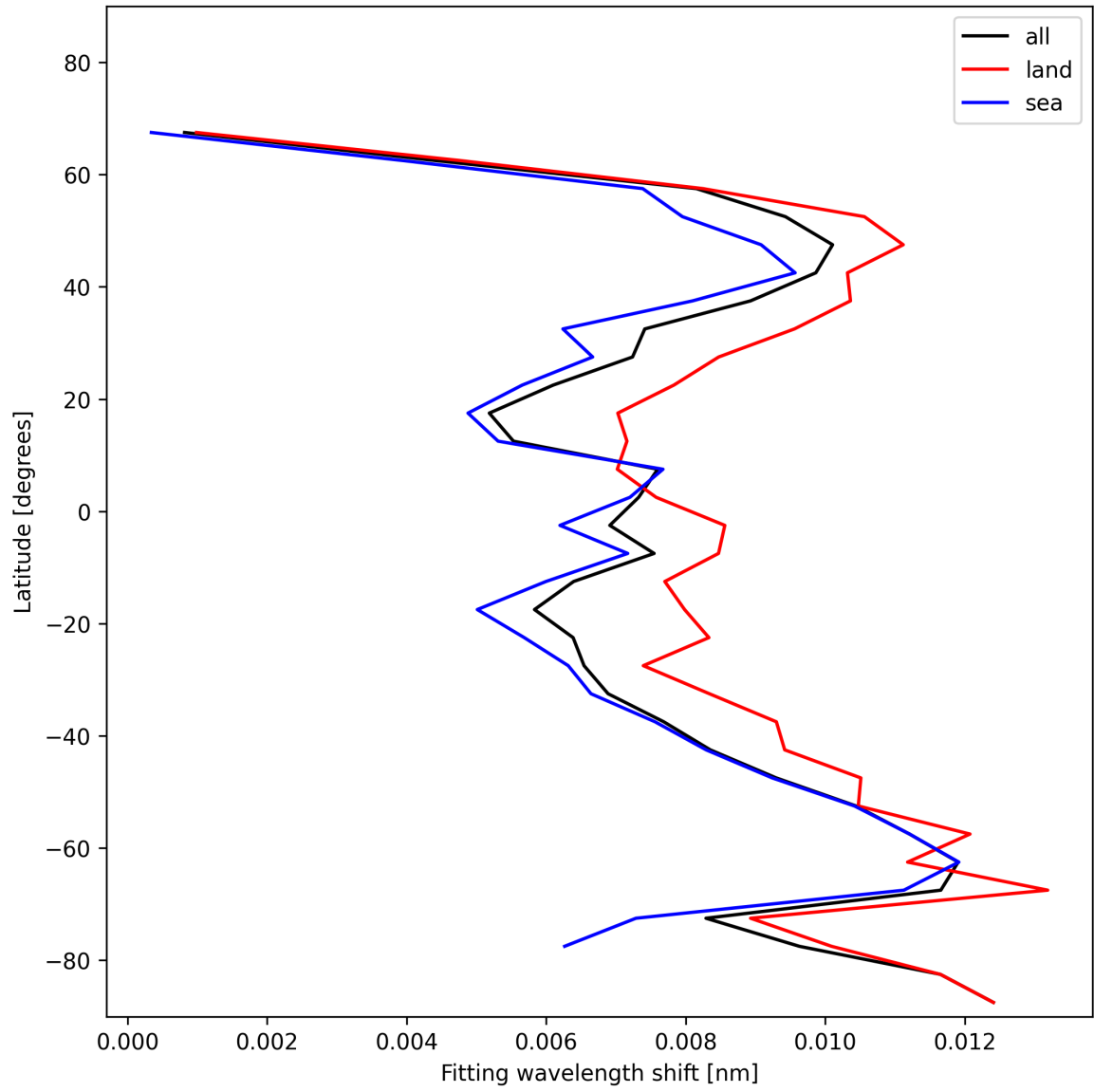
Figure 31: Zonal average of “Fitting wavelength shift” for 2025-01-23 to 2025-01-24.
