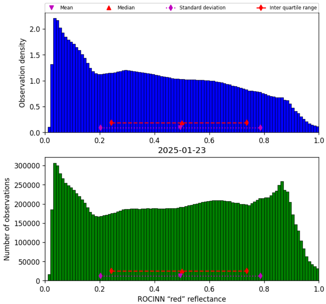
Figure 51: Histogram of “ROCINN “red” reflectance” for 2025-01-23 to 2025-01-24
