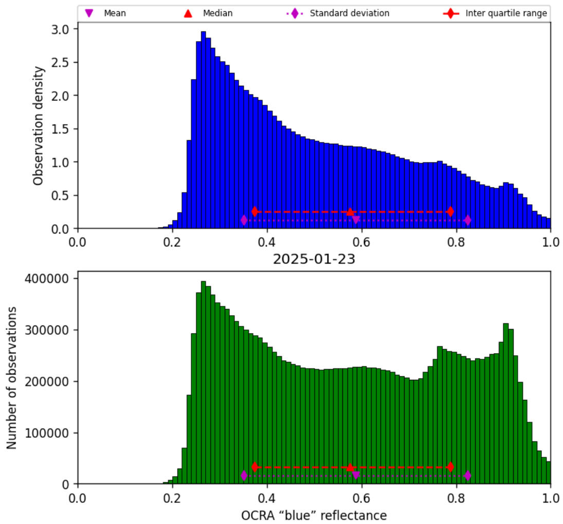
Figure 49: Histogram of "OCRA "blue" reflectance" for 2025-01-23 to 2025-01-24
