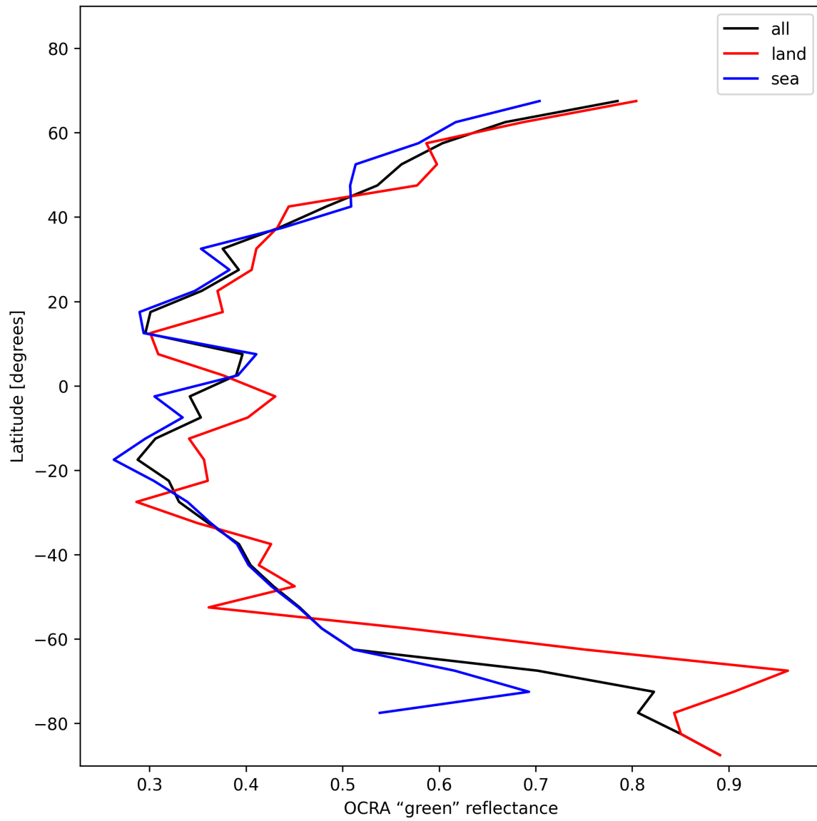
Figure 34: Zonal average of “OCRA “green” reflectance” for 2025-01-23 to 2025-01-24.
