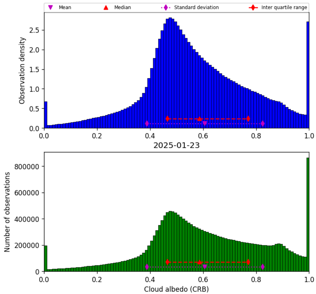
Figure 42: Histogram of “Cloud albedo (CRB)” for 2025-01-23 to 2025-01-24
