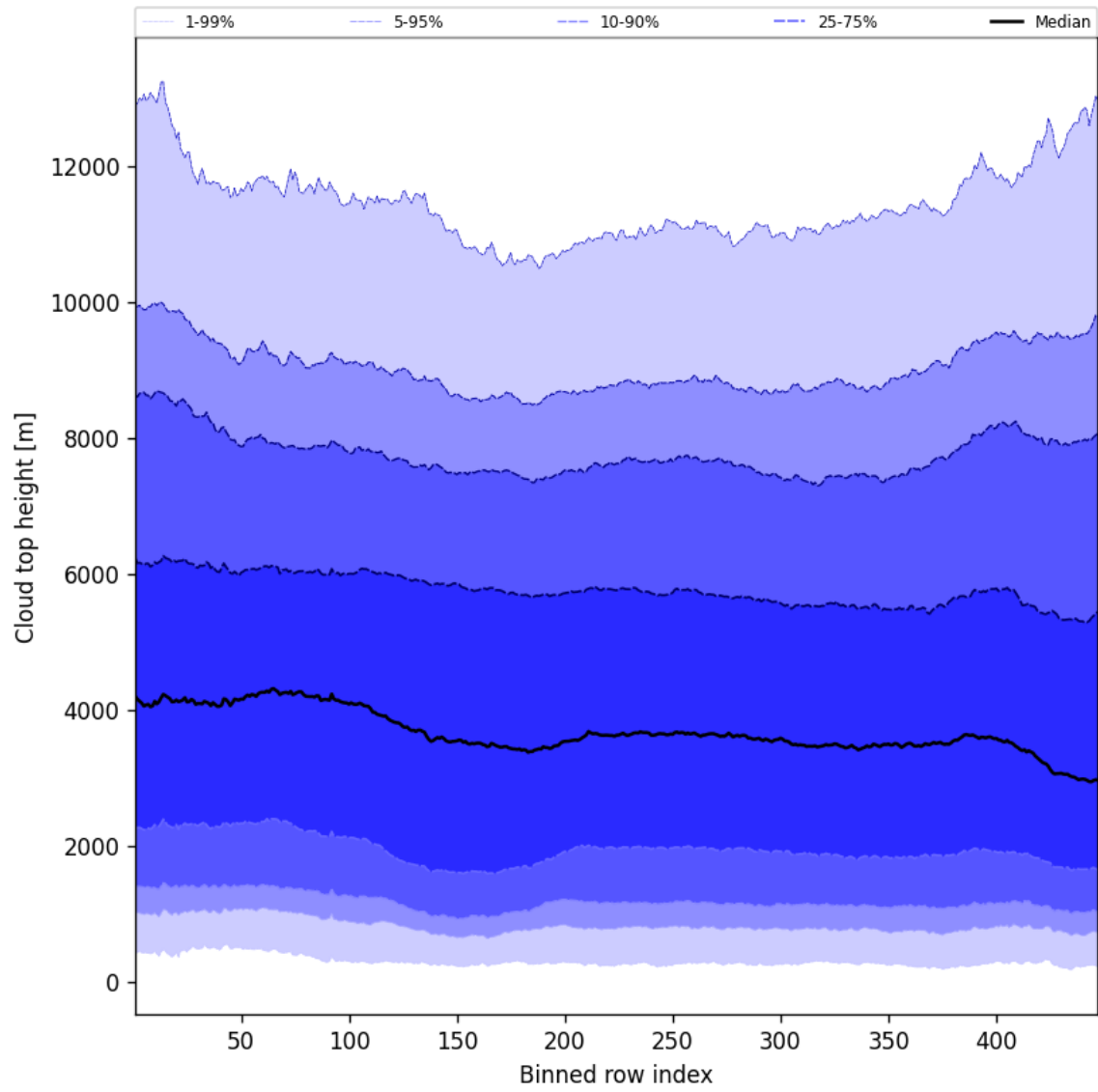
Figure 54: Along track statistics of “Cloud top height” for 2025-01-23 to 2025-01-24
