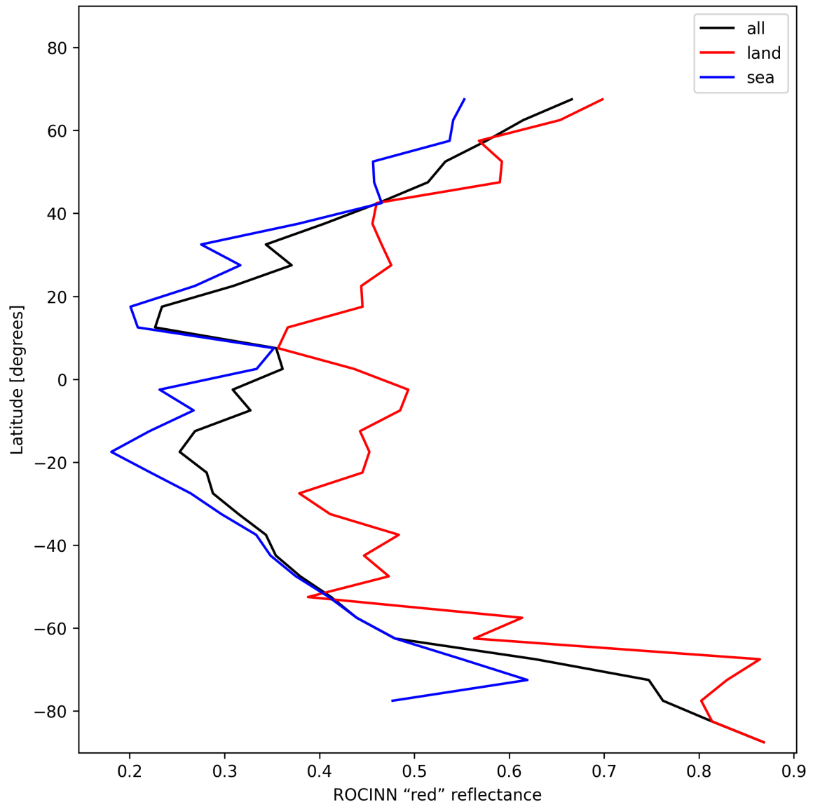
Figure 35: Zonal average of “ROCINN “red” reflectance” for 2025-01-23 to 2025-01-24.
