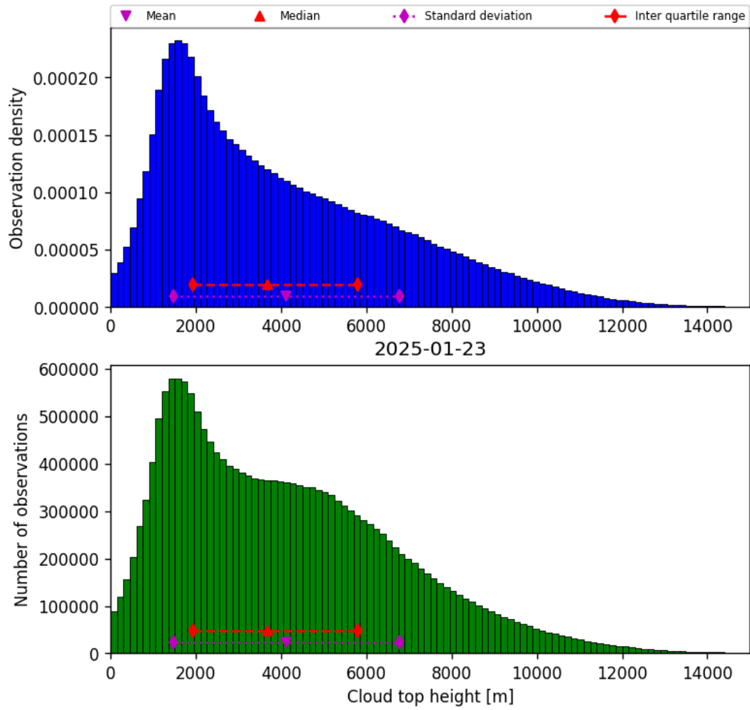
Figure 38: Histogram of “Cloud top height” for 2025-01-23 to 2025-01-24
