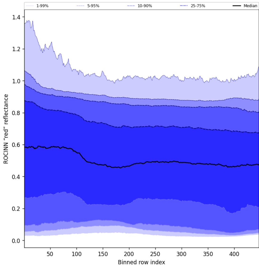
Figure 67: Along track statistics of “ROCINN “red” reflectance” for 2025-01-23 to 2025-01-24
