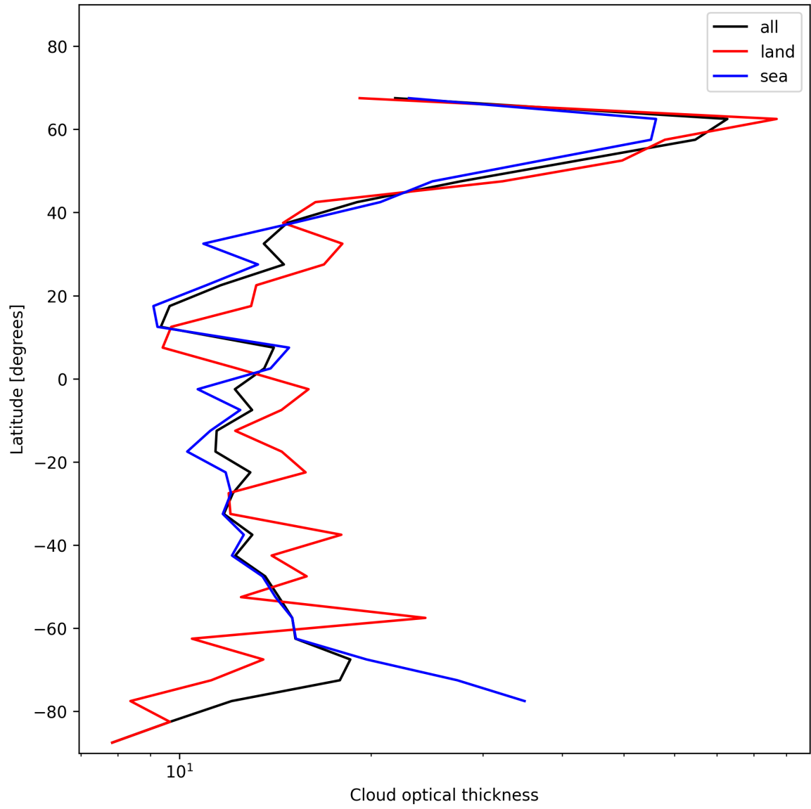
Figure 23: Zonal average of “Cloud optical thickness” for 2025-01-23 to 2025-01-24.
