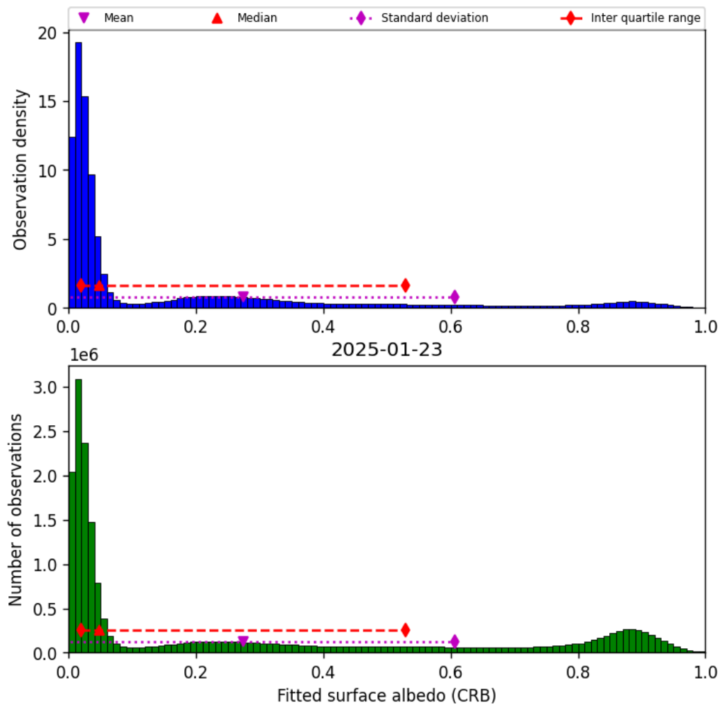
Figure 44: Histogram of “Fitted surface albedo (CRB)” for 2025-01-23 to 2025-01-24
