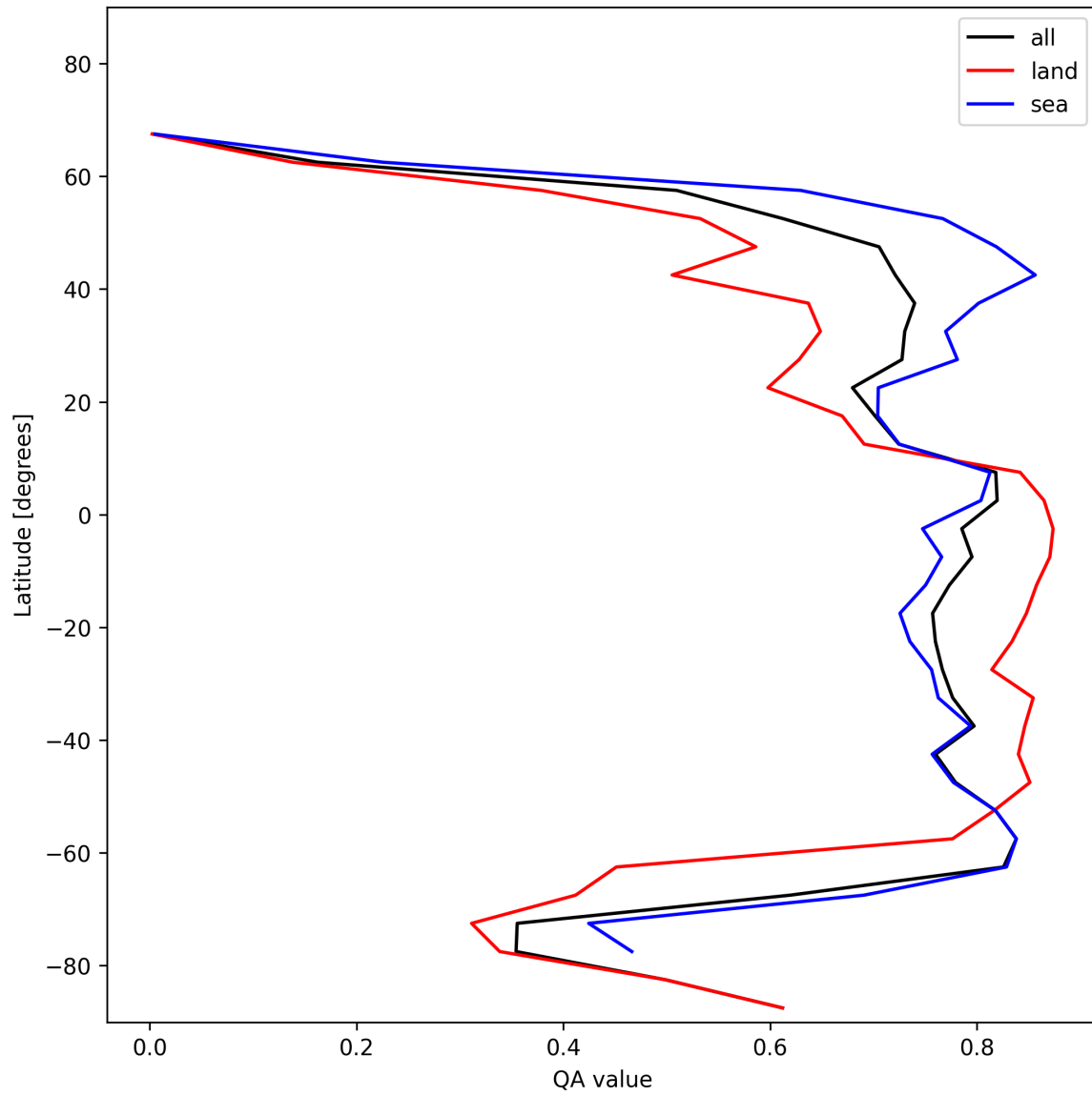
Figure 20: Zonal average of “QA value” for 2025-01-23 to 2025-01-24.
