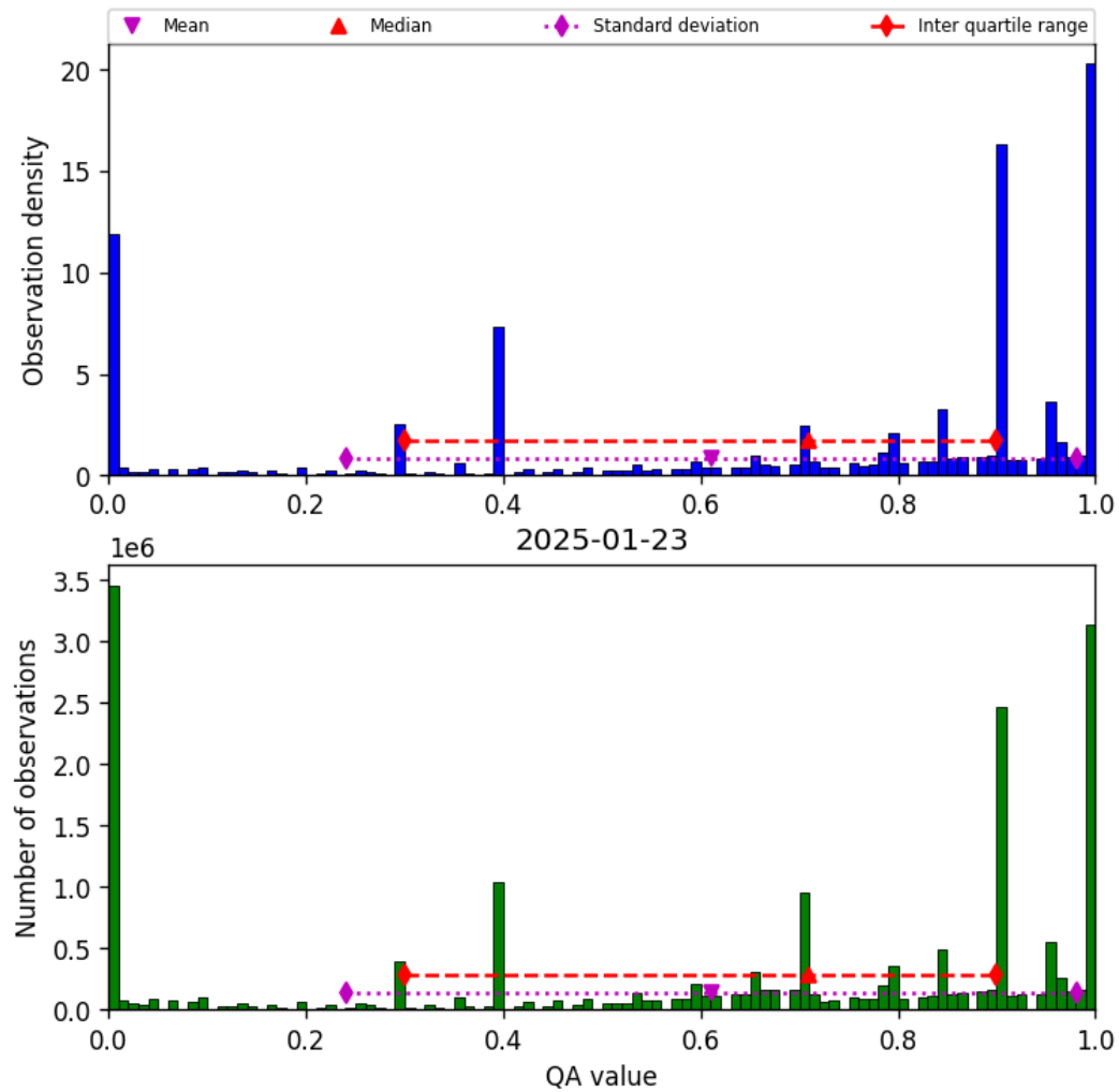
Figure 36: Histogram of “QA value” for 2025-01-23 to 2025-01-24
