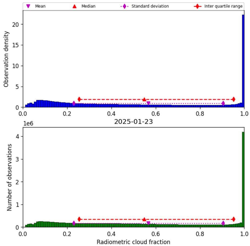
Figure 37: Histogram of “Radiometric cloud fraction” for 2025-01-23 to 2025-01-24
