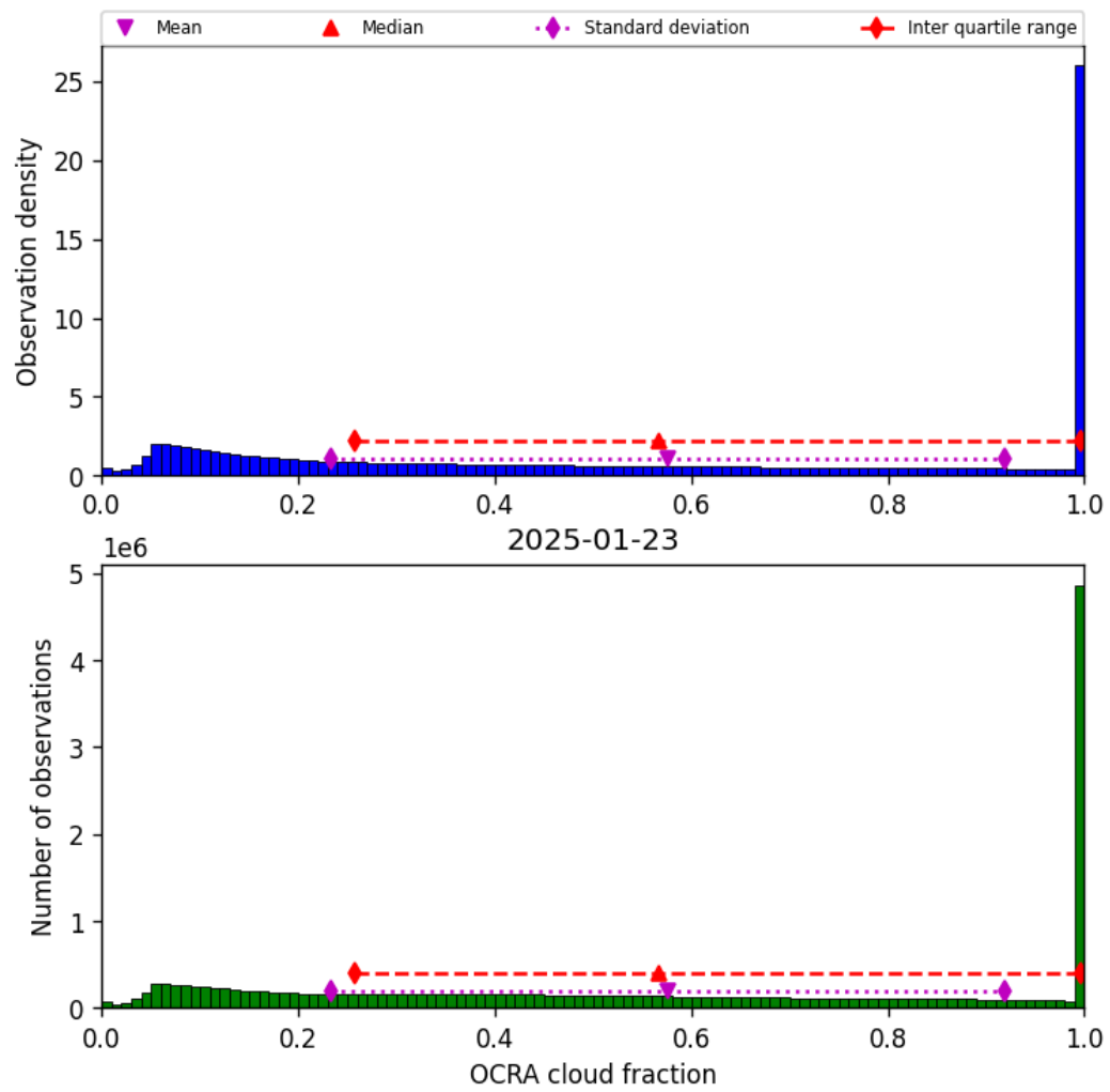
Figure 48: Histogram of “OCRA cloud fraction” for 2025-01-23 to 2025-01-24
