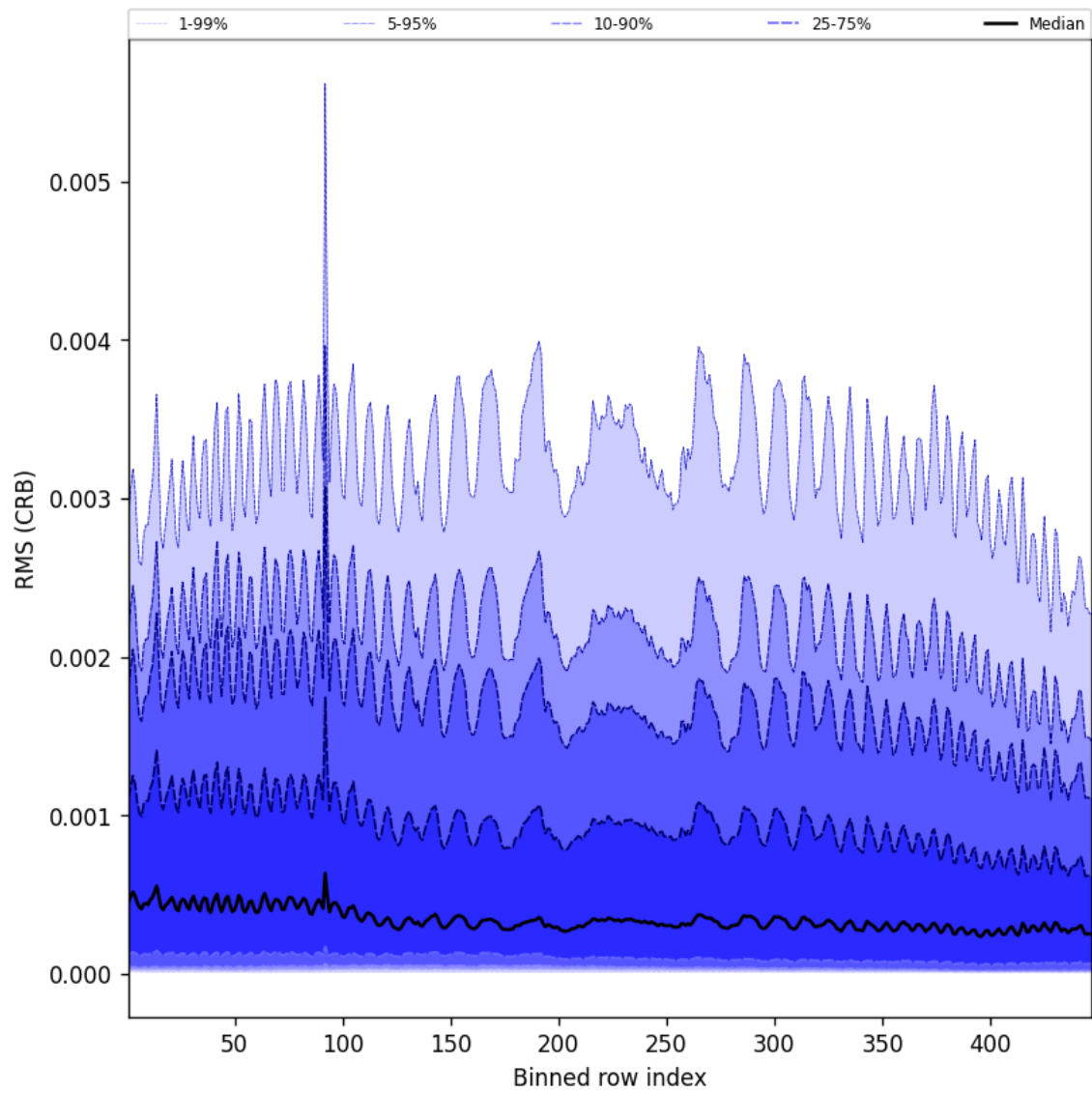
Figure 62: Along track statistics of “RMS (CRB)” for 2025-01-23 to 2025-01-24
