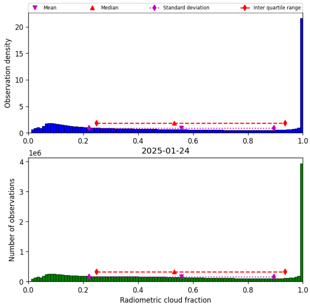
Figure 37: Histogram of “Radiometric cloud fraction” for 2025-01-24 to 2025-01-25
