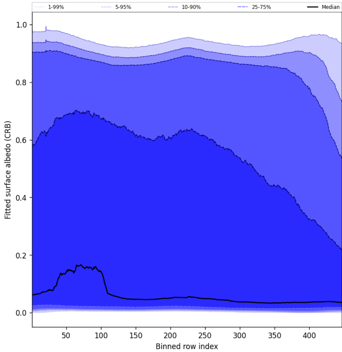
Figure 60: Along track statistics of “Fitted surface albedo (CRB)” for 2025-01-24 to 2025-01-25
