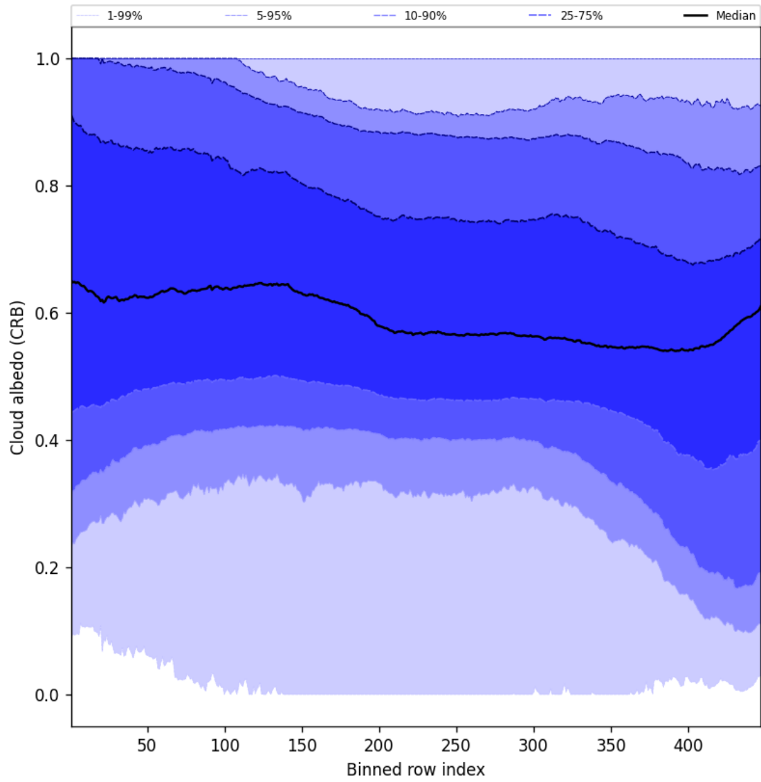
Figure 58: Along track statistics of “Cloud albedo (CRB)” for 2025-01-24 to 2025-01-25
