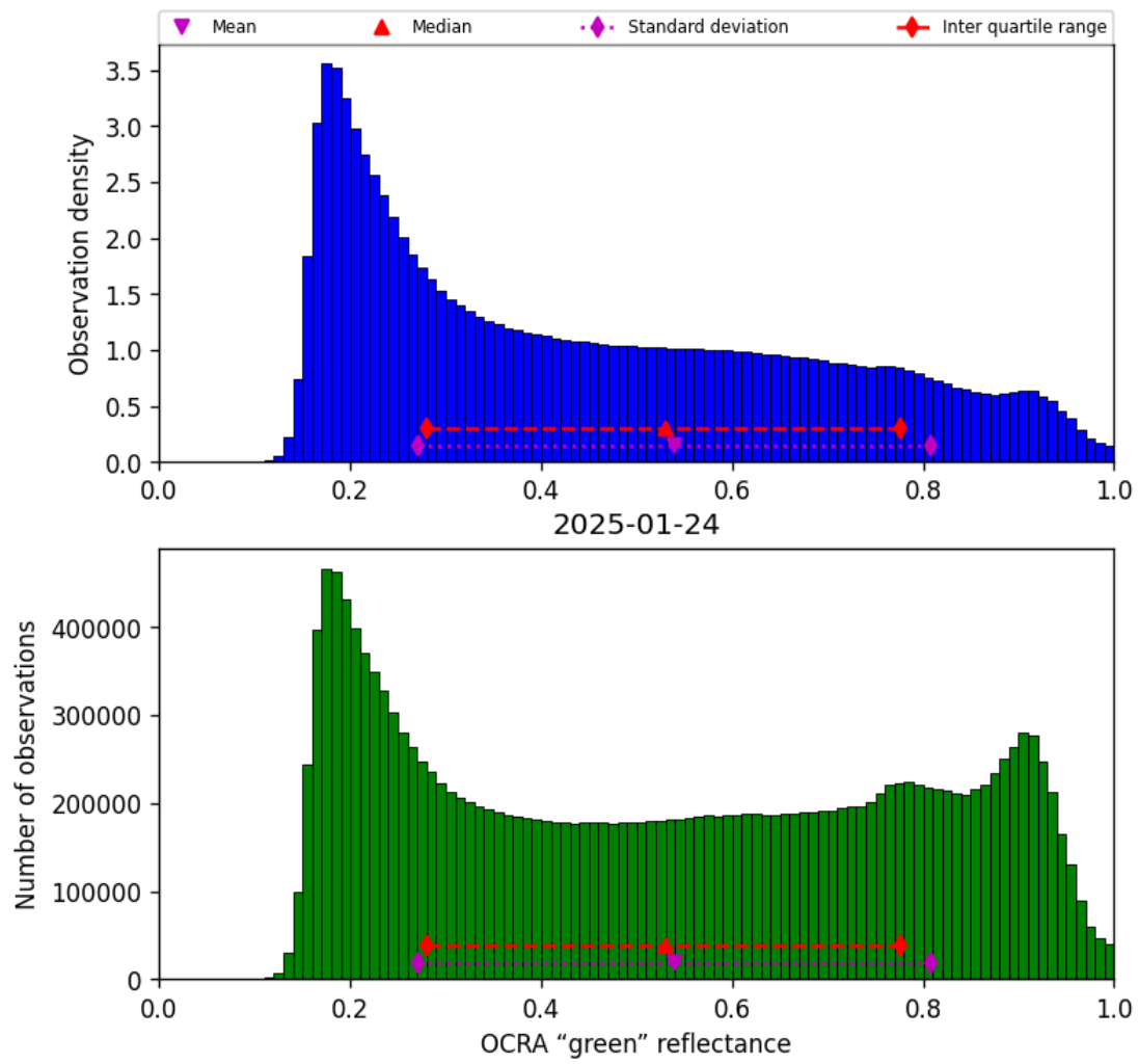
Figure 50: Histogram of “OCRA “green” reflectance” for 2025-01-24 to 2025-01-25
