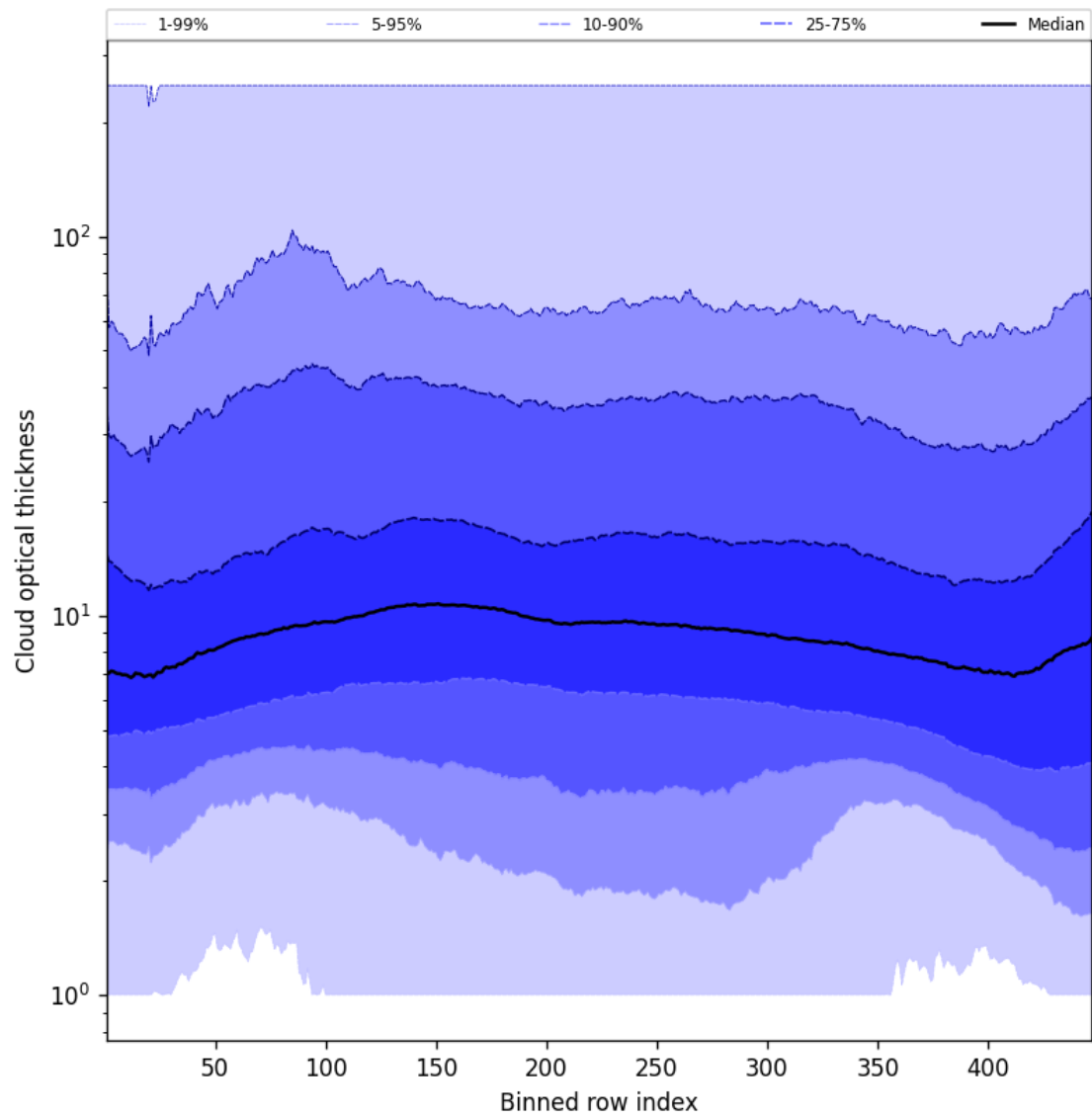
Figure 55: Along track statistics of “Cloud optical thickness” for 2025-01-24 to 2025-01-25
