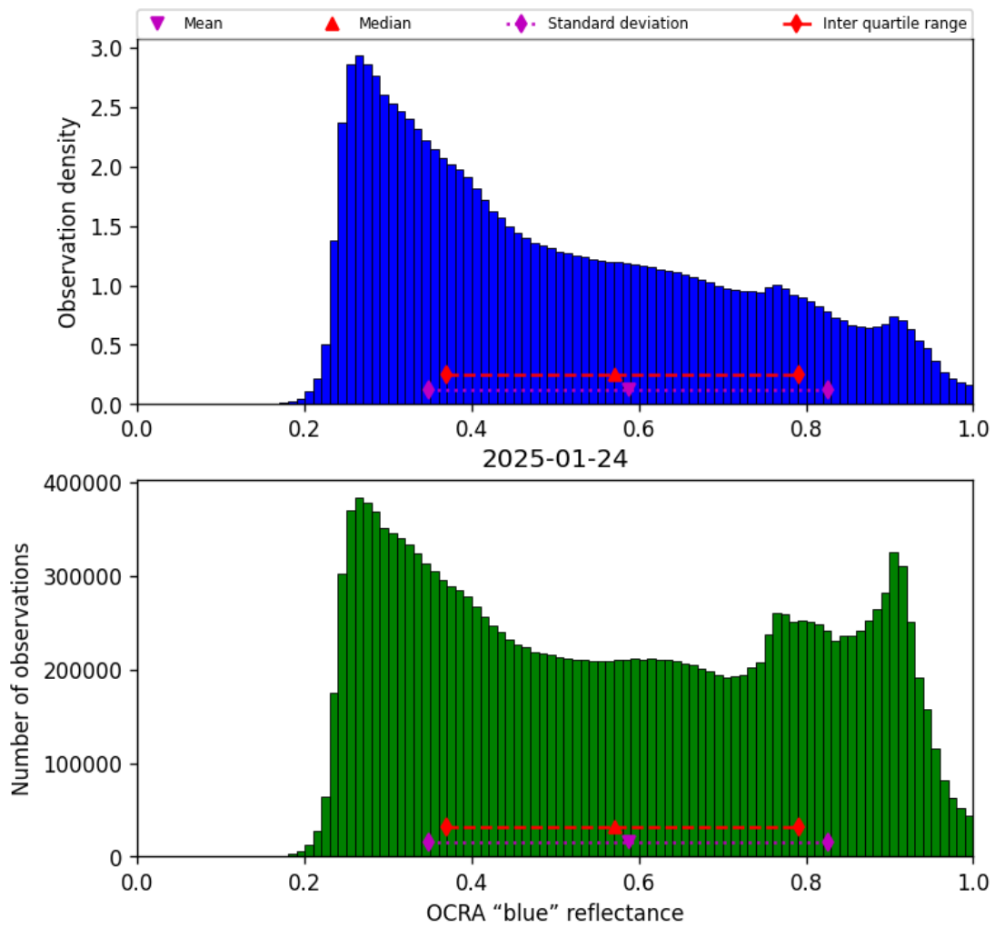
Figure 49: Histogram of “OCRA “blue” reflectance” for 2025-01-24 to 2025-01-25
