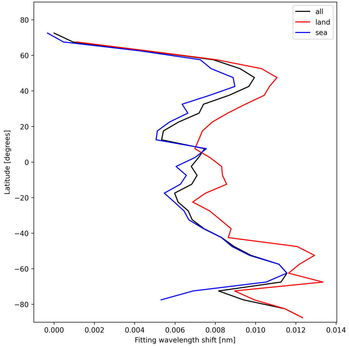
Figure 31: Zonal average of “Fitting wavelength shift” for 2025-01-24 to 2025-01-25.
