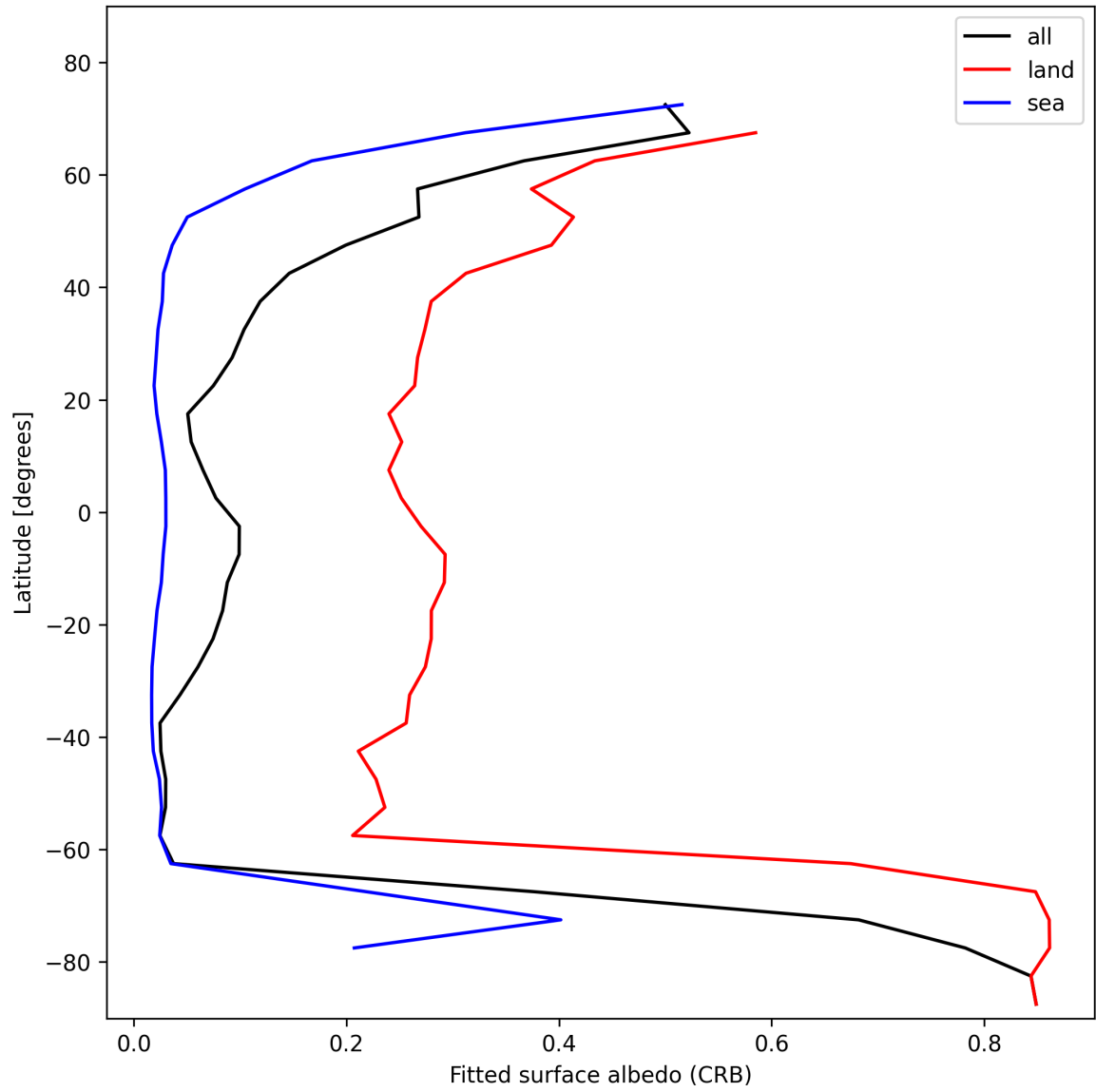
Figure 28: Zonal average of “Fitted surface albedo (CRB)” for 2025-01-24 to 2025-01-25.
