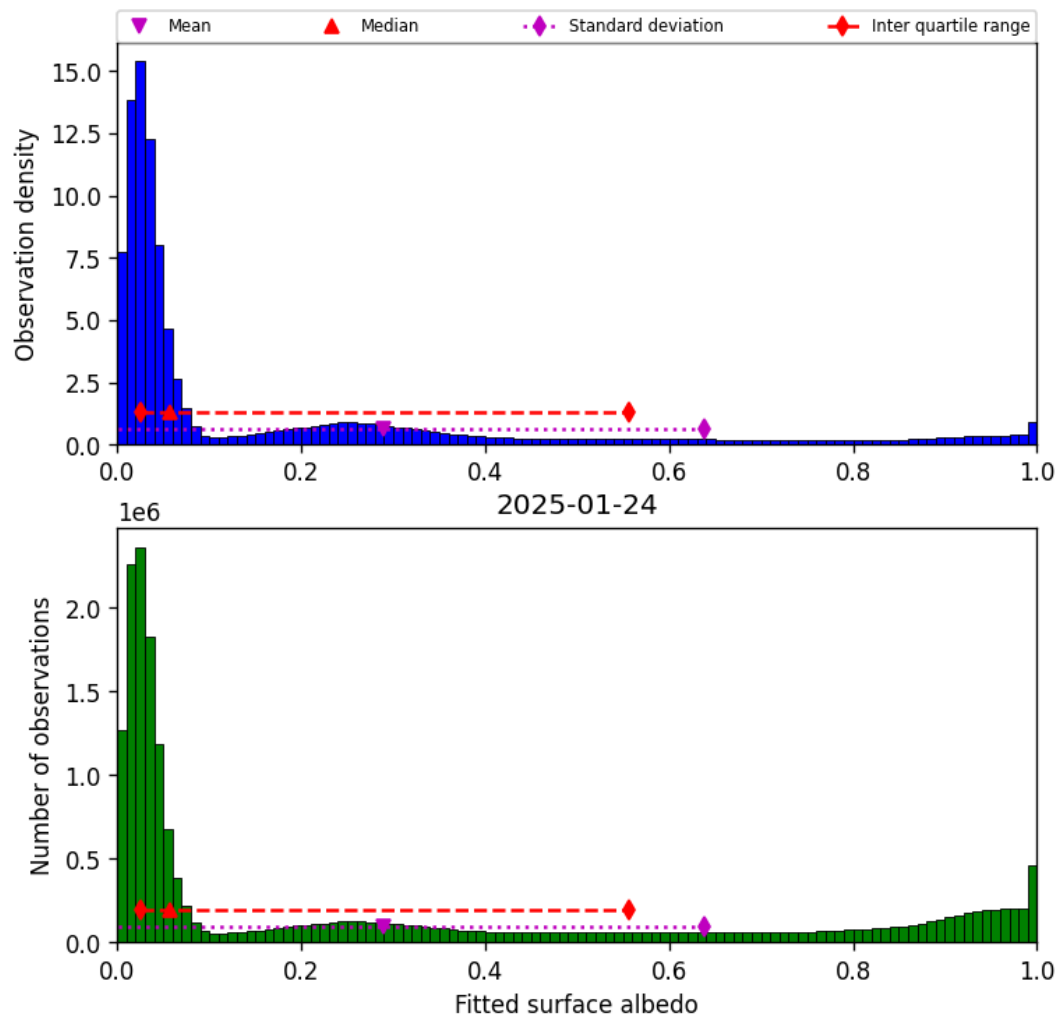
Figure 43: Histogram of “Fitted surface albedo” for 2025-01-24 to 2025-01-25
