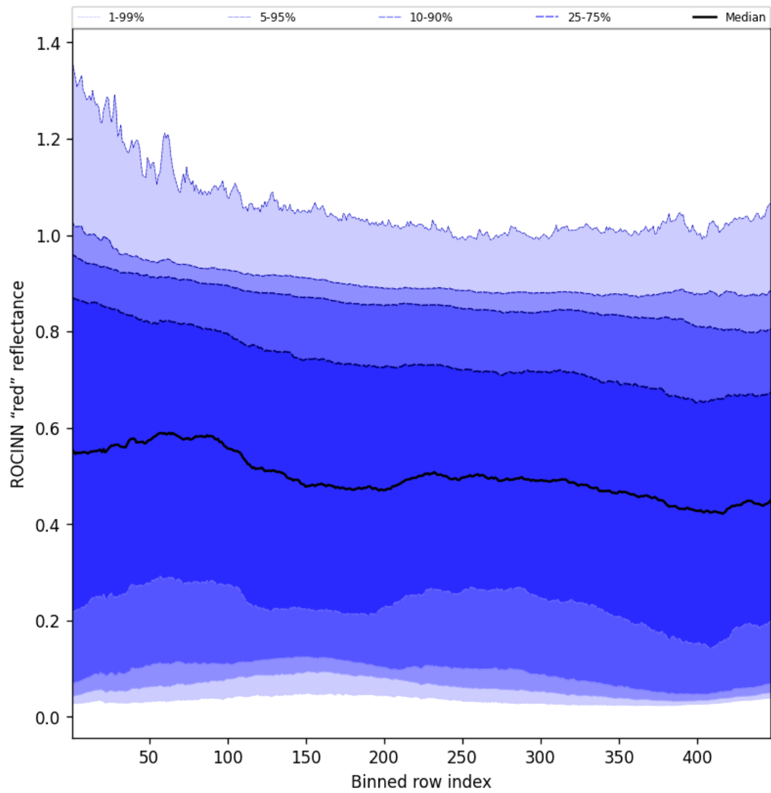
Figure 67: Along track statistics of "ROCINN "red" reflectance" for 2025-01-24 to 2025-01-25
