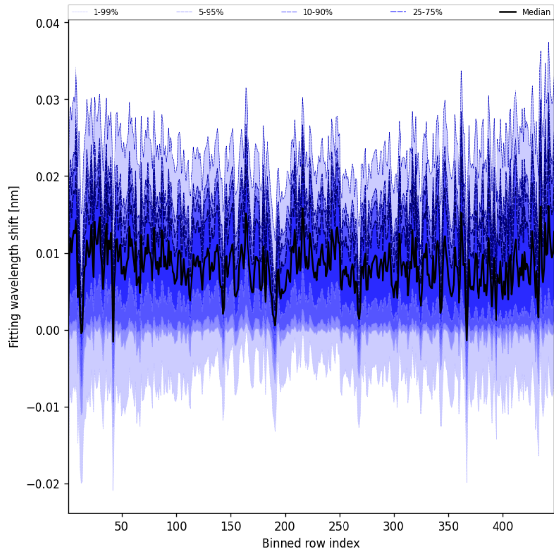
Figure 63: Along track statistics of “Fitting wavelength shift” for 2025-01-24 to 2025-01-25
