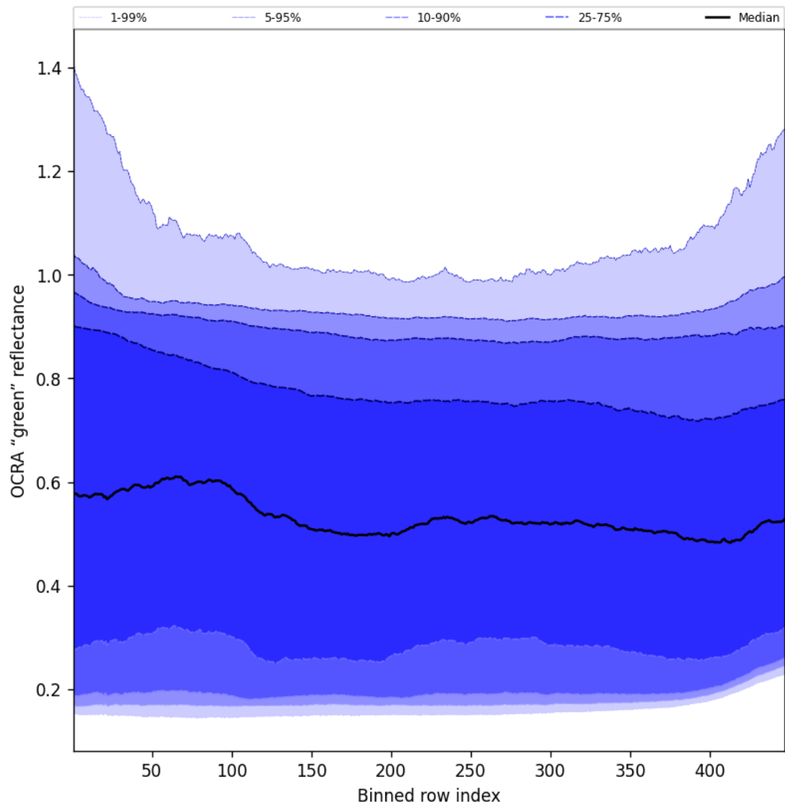
Figure 66: Along track statistics of “OCRA “green” reflectance” for 2025-01-24 to 2025-01-25
