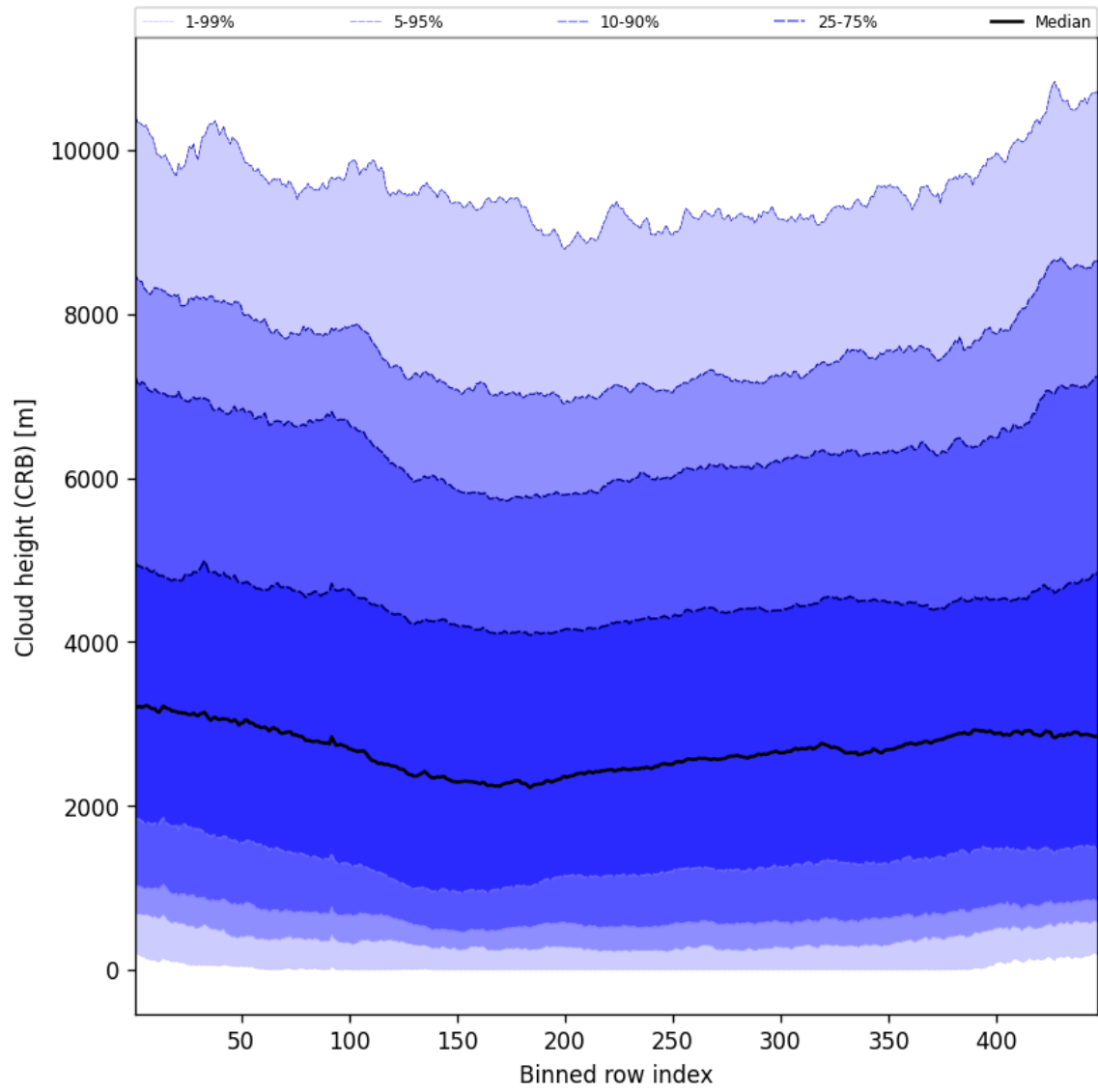
Figure 57: Along track statistics of “Cloud height (CRB)” for 2025-01-24 to 2025-01-25
