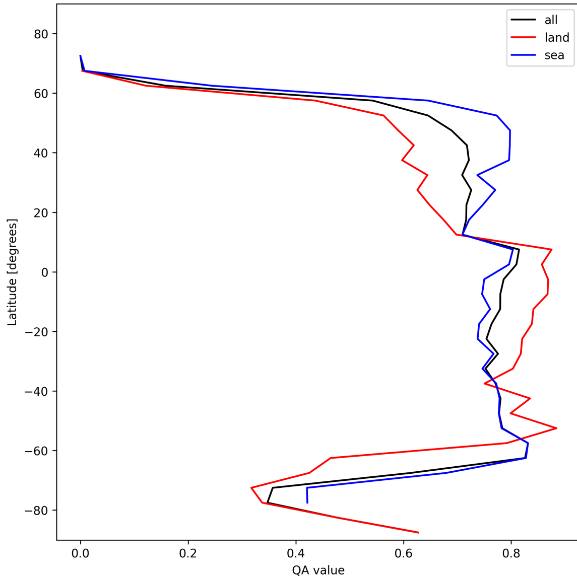
Figure 20: Zonal average of “QA value” for 2025-01-24 to 2025-01-25.
