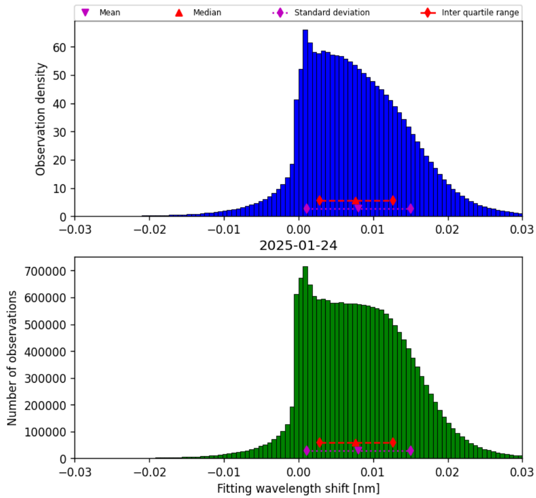
Figure 47: Histogram of “Fitting wavelength shift” for 2025-01-24 to 2025-01-25
