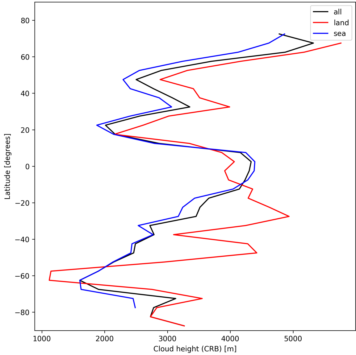
Figure 25: Zonal average of “Cloud height (CRB)” for 2025-01-24 to 2025-01-25.
