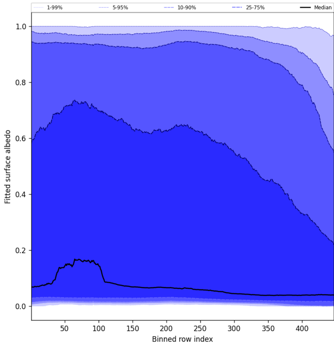
Figure 59: Along track statistics of “Fitted surface albedo” for 2025-01-24 to 2025-01-25
