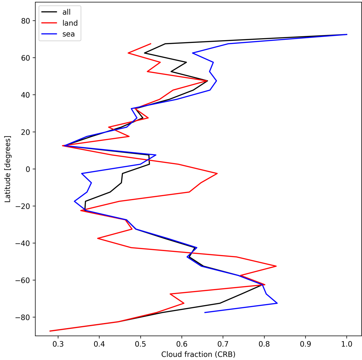
Figure 24: Zonal average of “Cloud fraction (CRB)” for 2025-01-24 to 2025-01-25.
