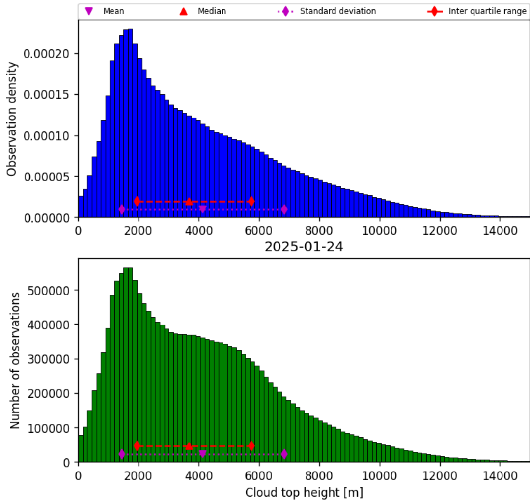
Figure 38: Histogram of “Cloud top height” for 2025-01-24 to 2025-01-25
