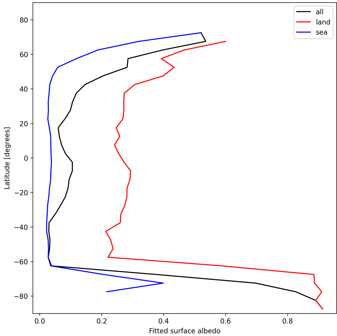
Figure 27: Zonal average of “Fitted surface albedo” for 2025-01-24 to 2025-01-25.
