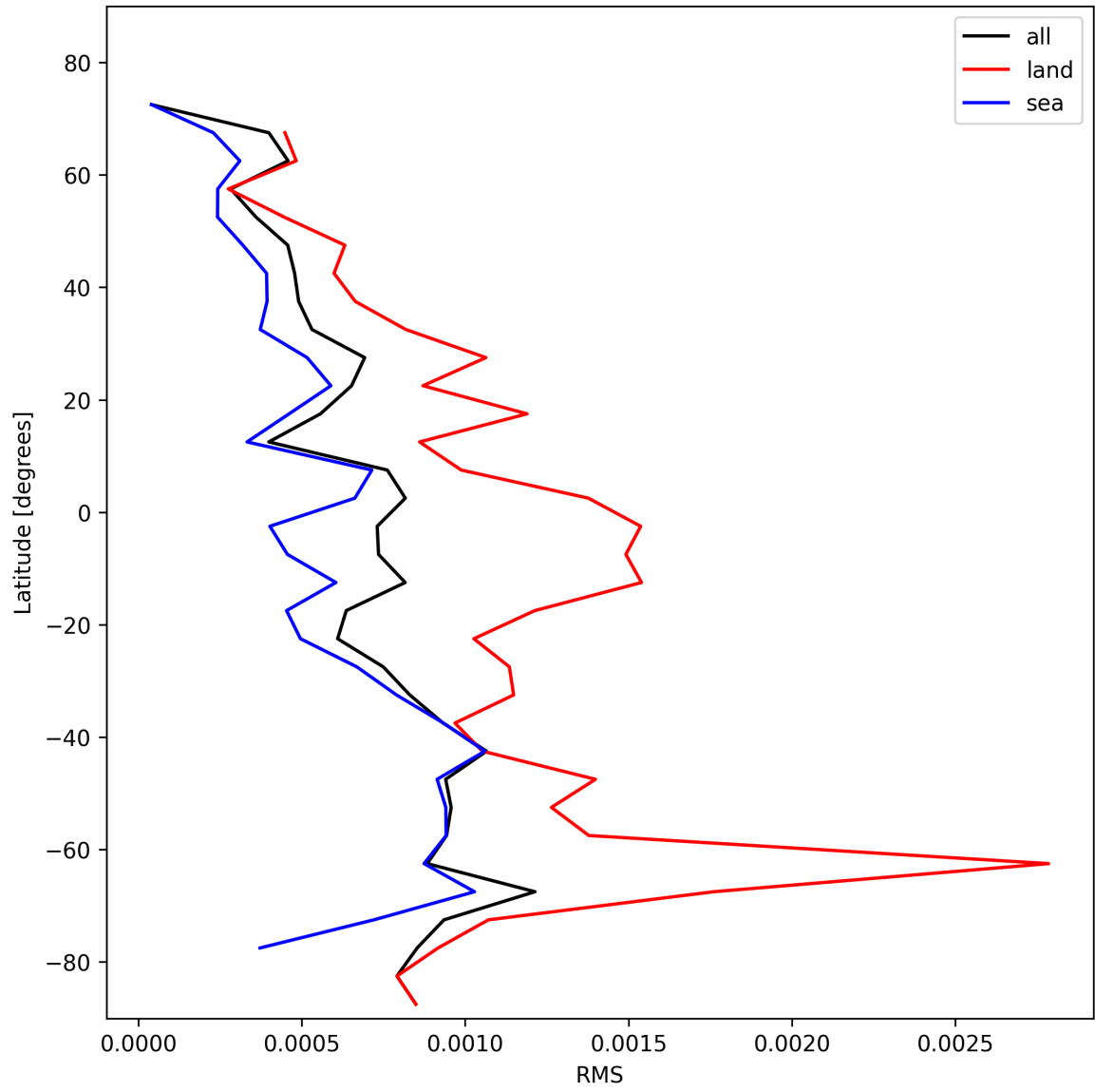
Figure 29: Zonal average of “RMS” for 2025-01-24 to 2025-01-25.
