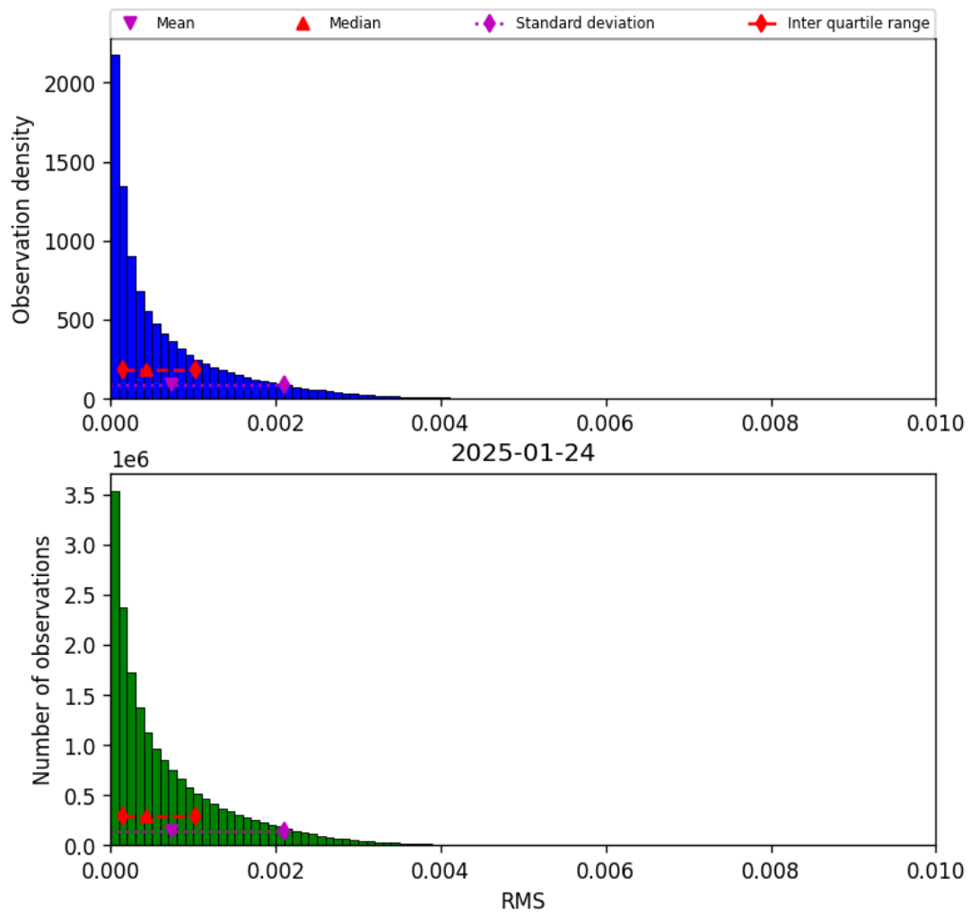
Figure 45: Histogram of “RMS” for 2025-01-24 to 2025-01-25
