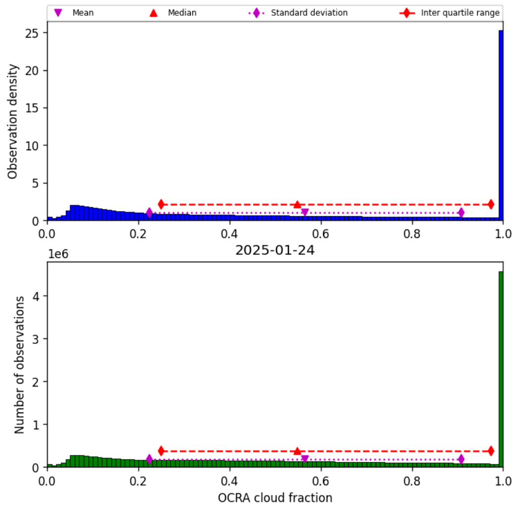
Figure 48: Histogram of “OCRA cloud fraction” for 2025-01-24 to 2025-01-25
