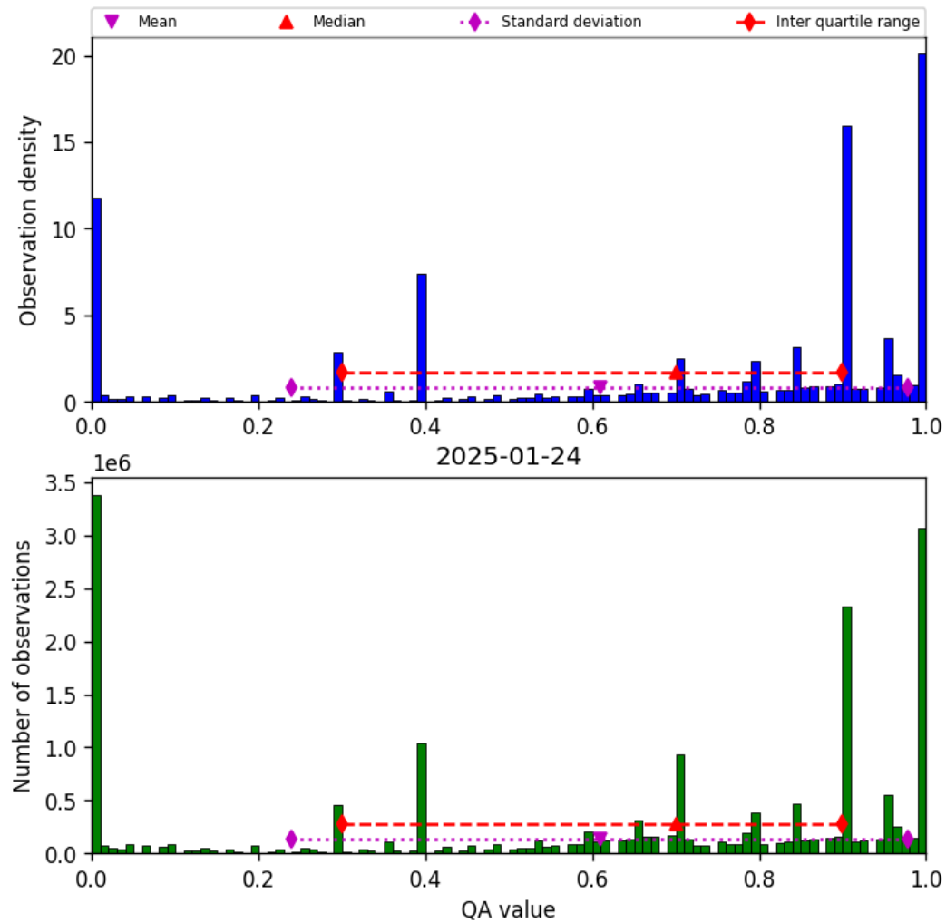
Figure 36: Histogram of “QA value” for 2025-01-24 to 2025-01-25
