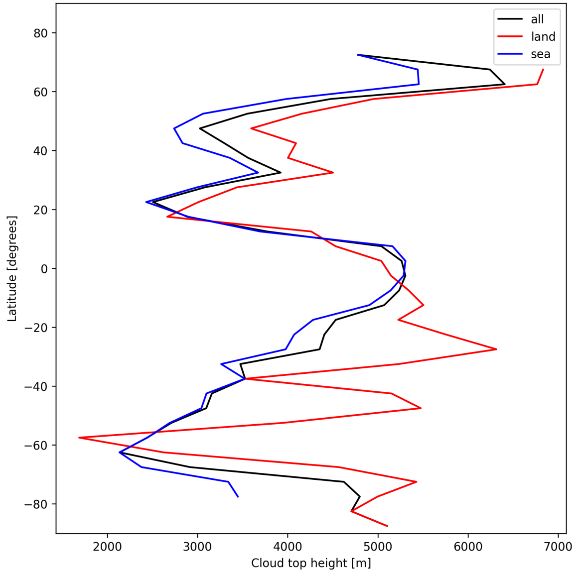
Figure 22: Zonal average of “Cloud top height” for 2025-01-24 to 2025-01-25.
