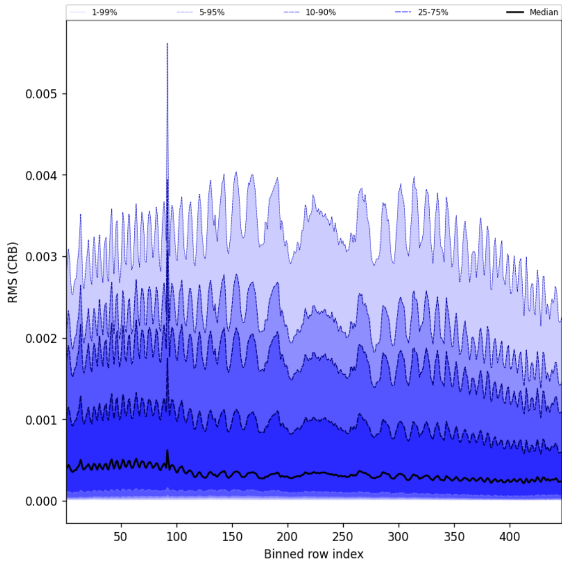
Figure 62: Along track statistics of “RMS (CRB)” for 2025-01-24 to 2025-01-25
