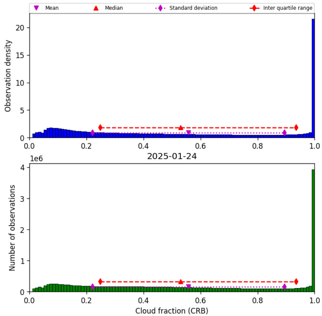
Figure 40: Histogram of “Cloud fraction (CRB)” for 2025-01-24 to 2025-01-25
