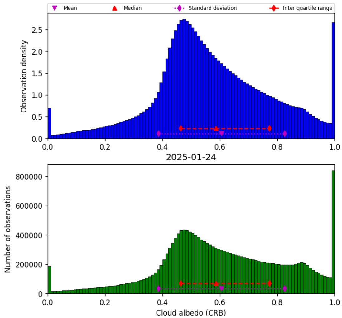
Figure 42: Histogram of “Cloud albedo (CRB)” for 2025-01-24 to 2025-01-25
