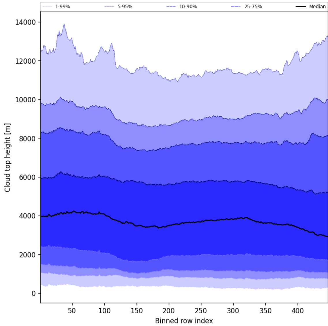
Figure 54: Along track statistics of “Cloud top height” for 2025-01-24 to 2025-01-25
