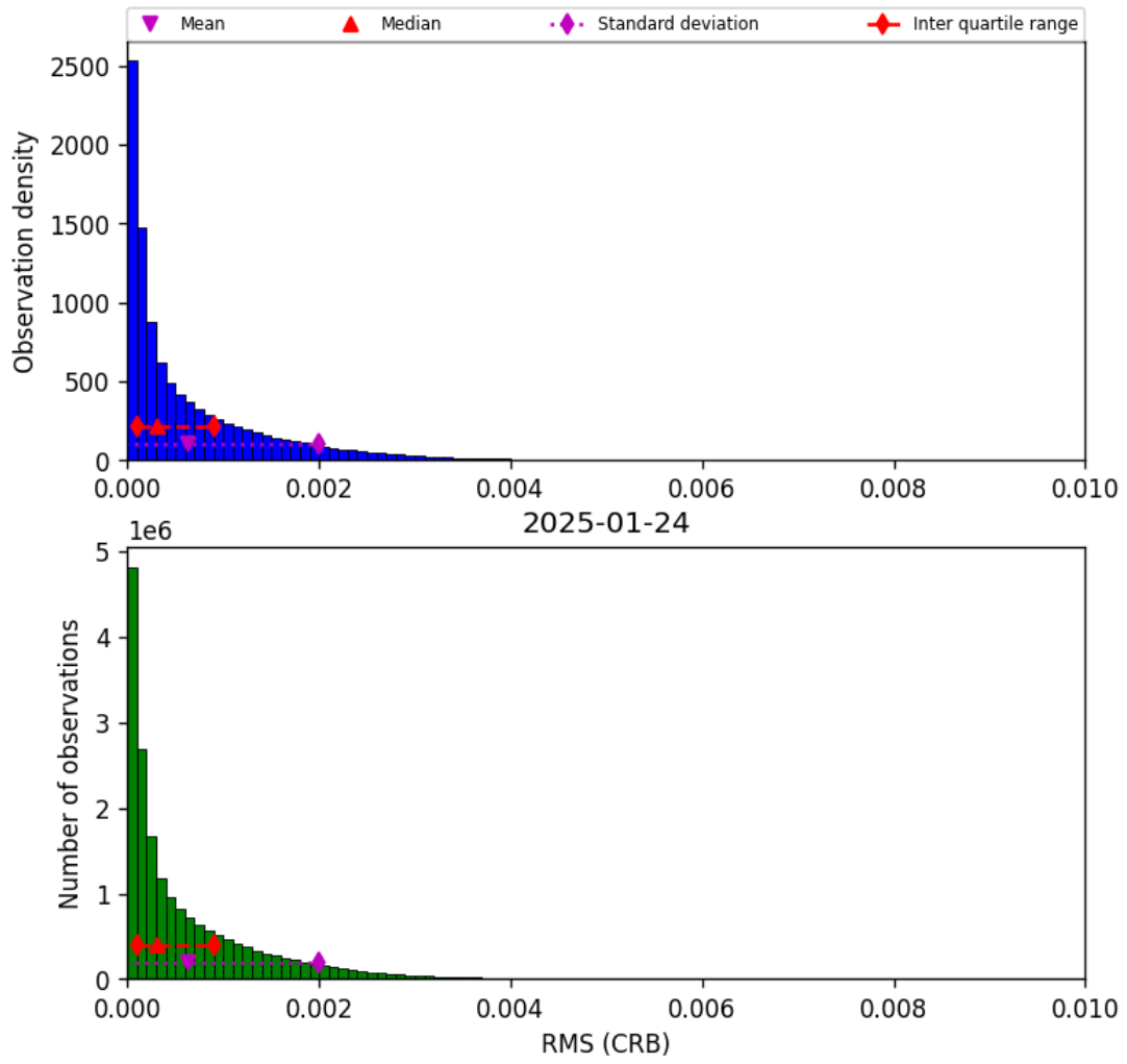
Figure 46: Histogram of “RMS (CRB)” for 2025-01-24 to 2025-01-25
