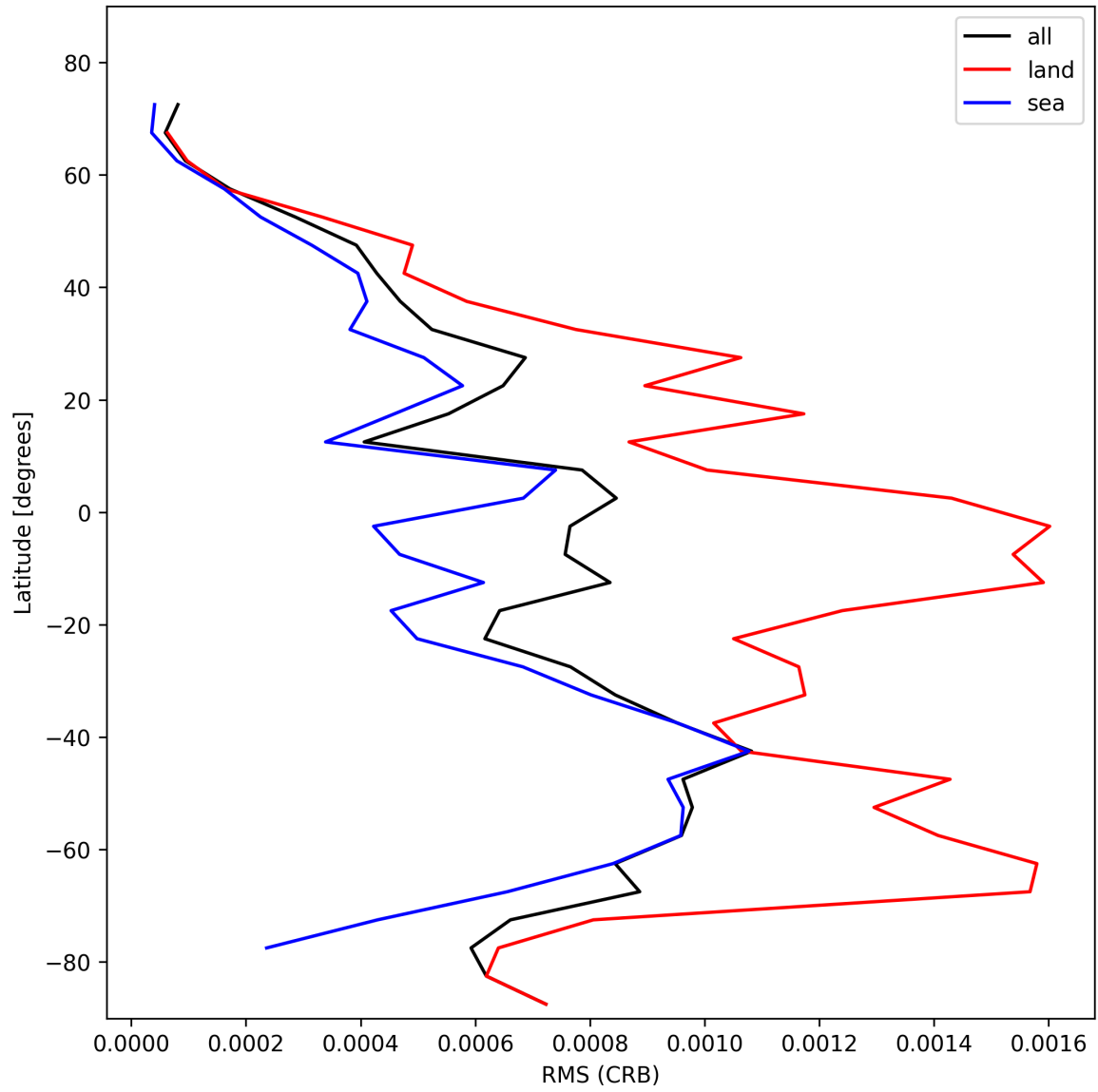
Figure 30: Zonal average of “RMS (CRB)” for 2025-01-24 to 2025-01-25.
