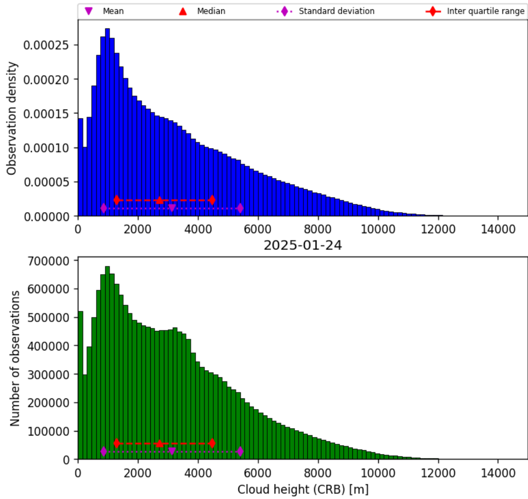
Figure 41: Histogram of “Cloud height (CRB)” for 2025-01-24 to 2025-01-25
