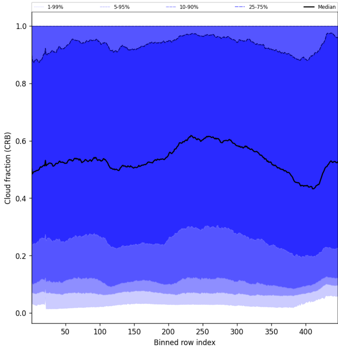
Figure 56: Along track statistics of “Cloud fraction (CRB)” for 2025-01-24 to 2025-01-25
