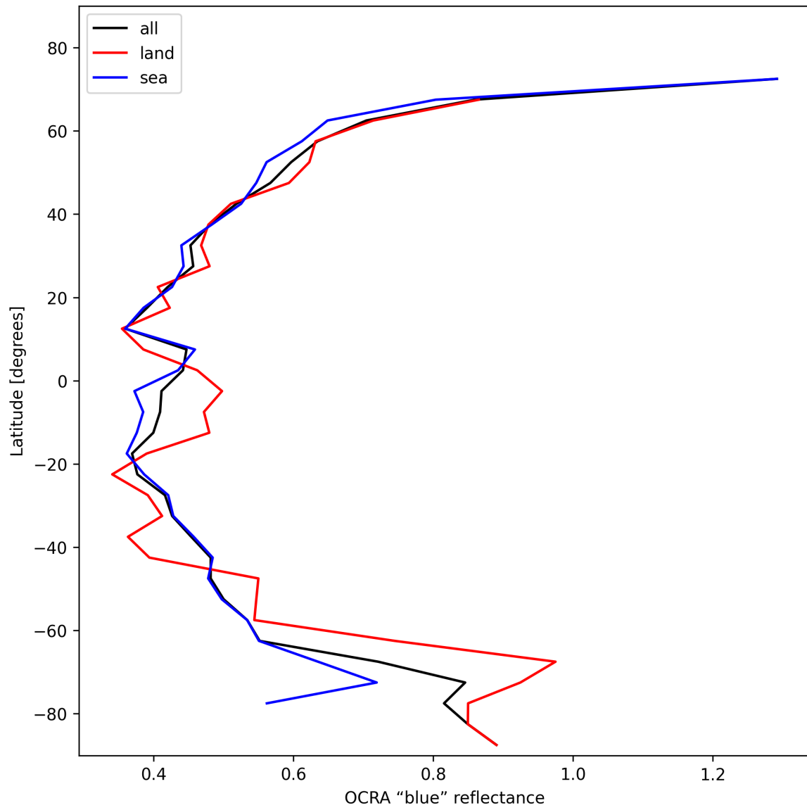
Figure 33: Zonal average of “OCRA “blue” reflectance” for 2025-01-24 to 2025-01-25.
