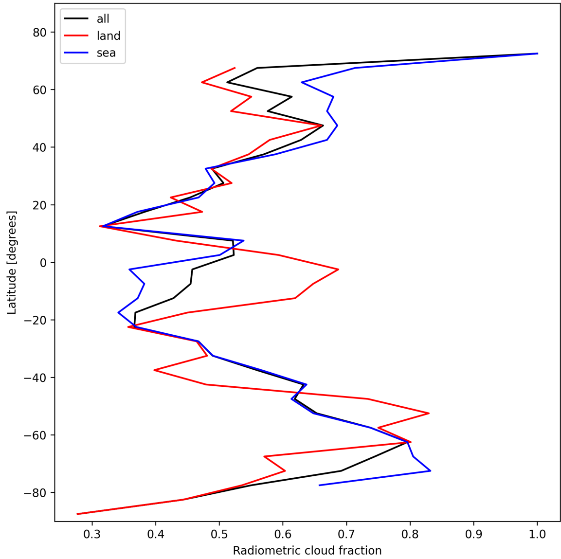
Figure 21: Zonal average of “Radiometric cloud fraction” for 2025-01-24 to 2025-01-25.
