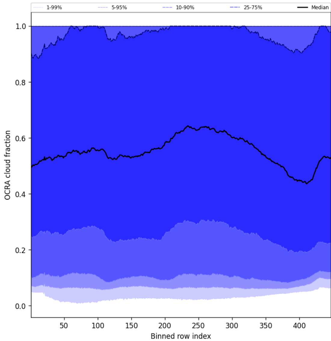
Figure 64: Along track statistics of “OCRA cloud fraction” for 2025-01-24 to 2025-01-25
