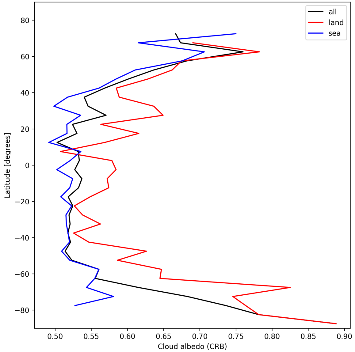
Figure 26: Zonal average of “Cloud albedo (CRB)” for 2025-01-24 to 2025-01-25.
