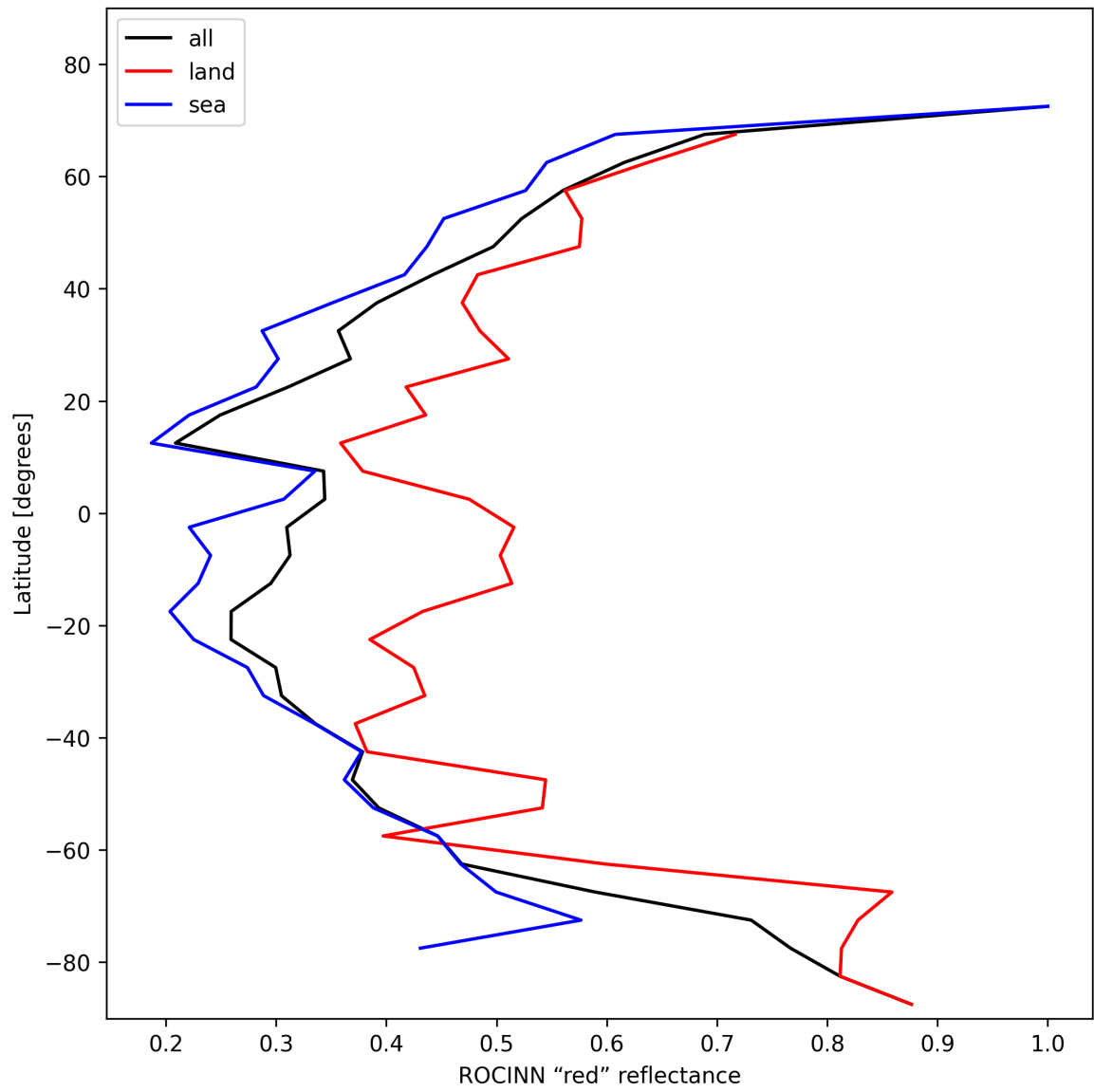
Figure 35: Zonal average of “ROCINN “red” reflectance” for 2025-01-24 to 2025-01-25.
