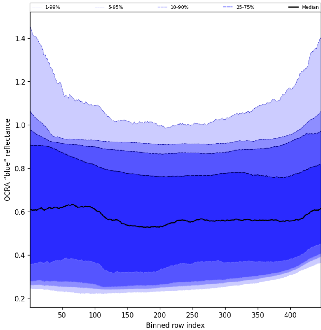
Figure 65: Along track statistics of "OCRA "blue" reflectance" for 2025-01-24 to 2025-01-25
