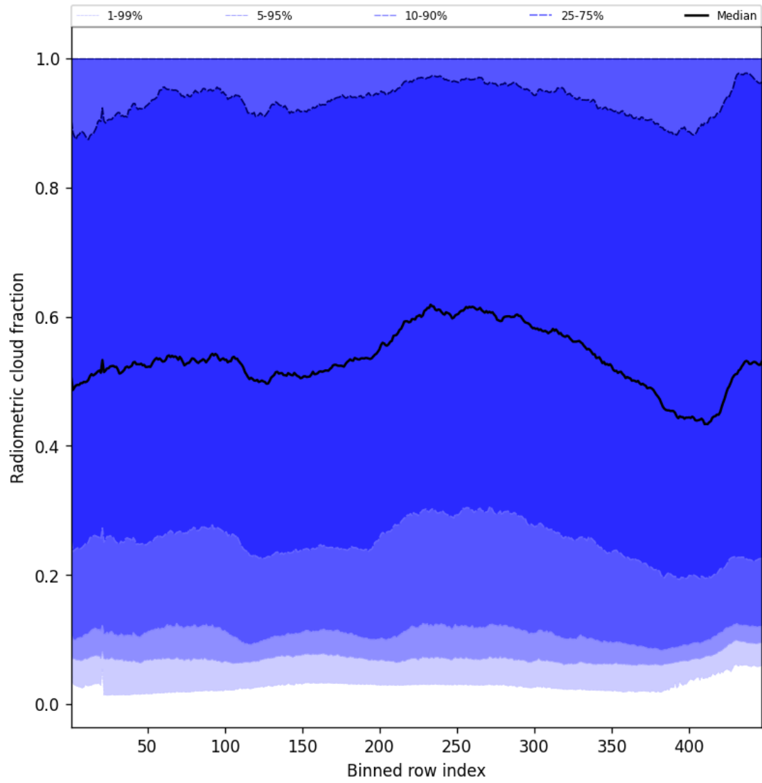
Figure 53: Along track statistics of “Radiometric cloud fraction” for 2025-01-24 to 2025-01-25
