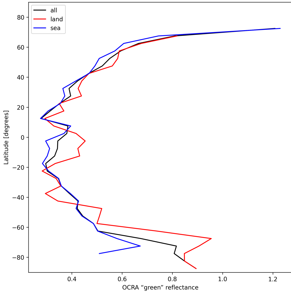
Figure 34: Zonal average of “OCRA “green” reflectance” for 2025-01-24 to 2025-01-25.
