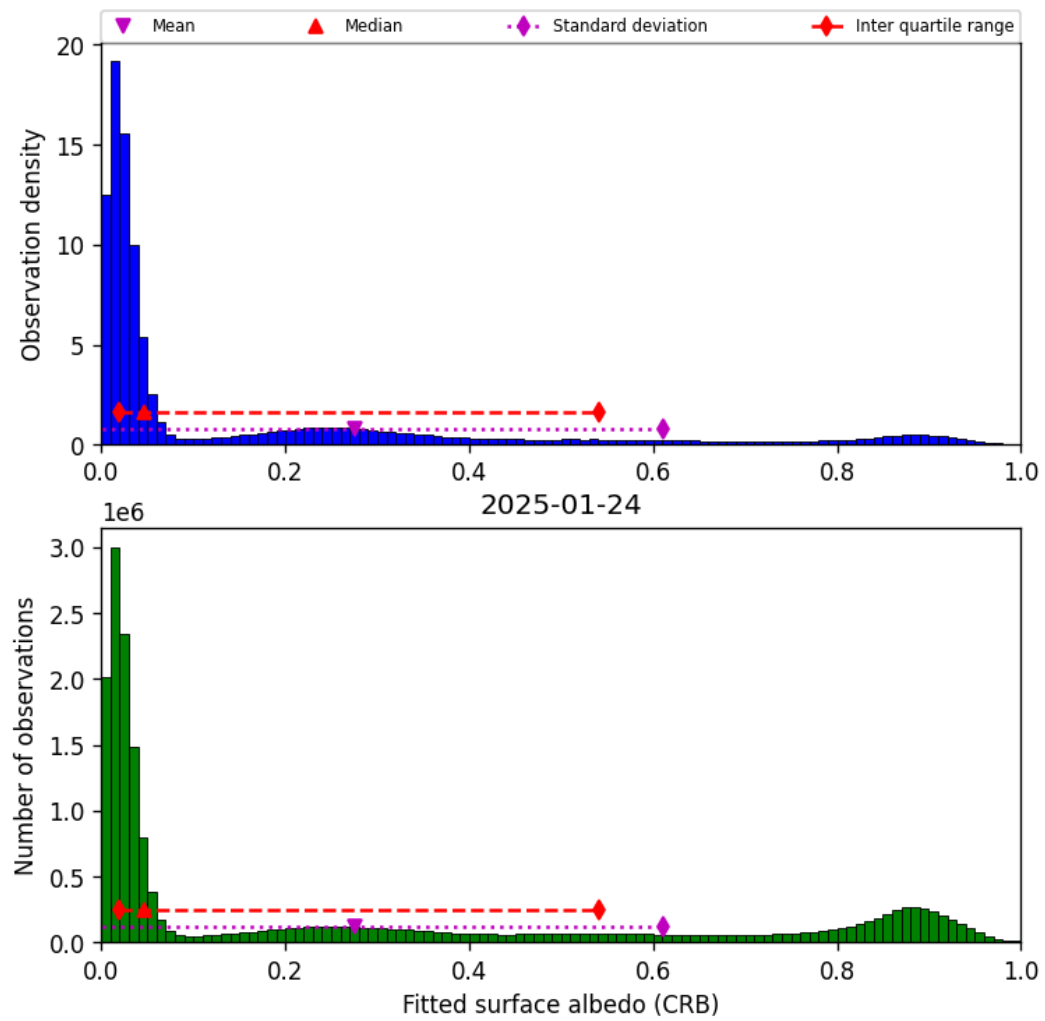
Figure 44: Histogram of “Fitted surface albedo (CRB)” for 2025-01-24 to 2025-01-25
