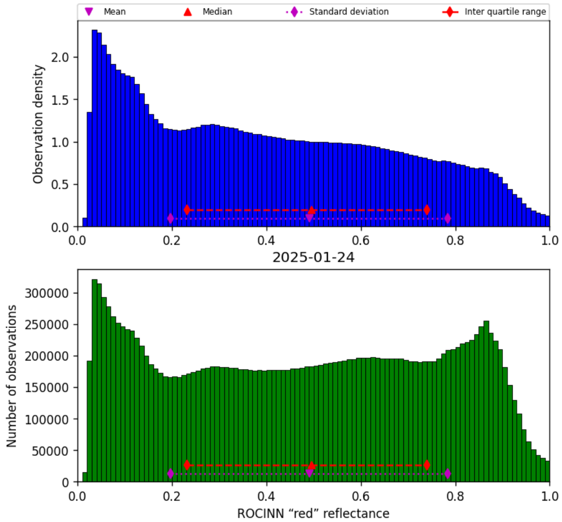
Figure 51: Histogram of “ROCINN “red” reflectance” for 2025-01-24 to 2025-01-25
