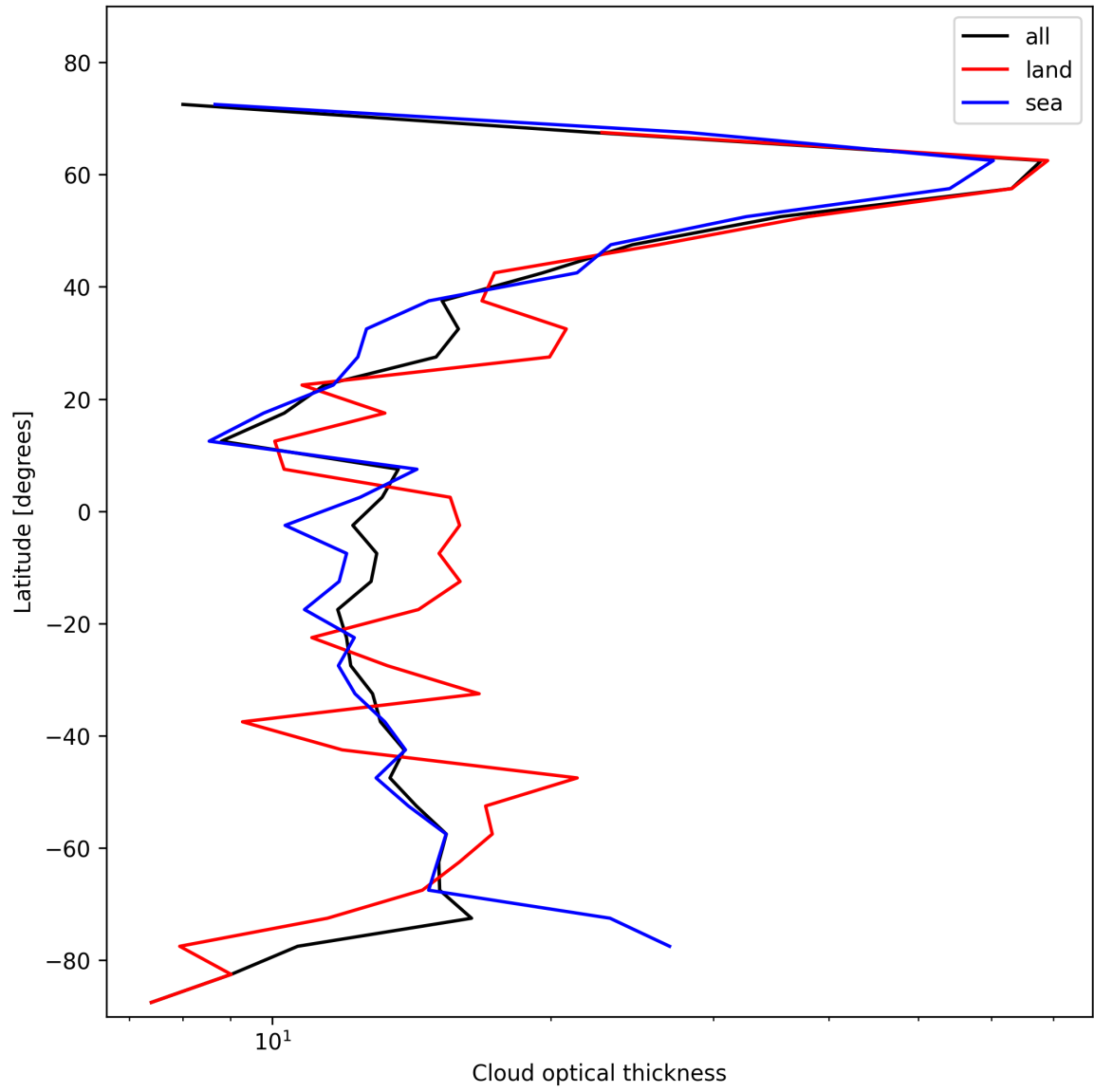
Figure 23: Zonal average of “Cloud optical thickness” for 2025-01-24 to 2025-01-25.
