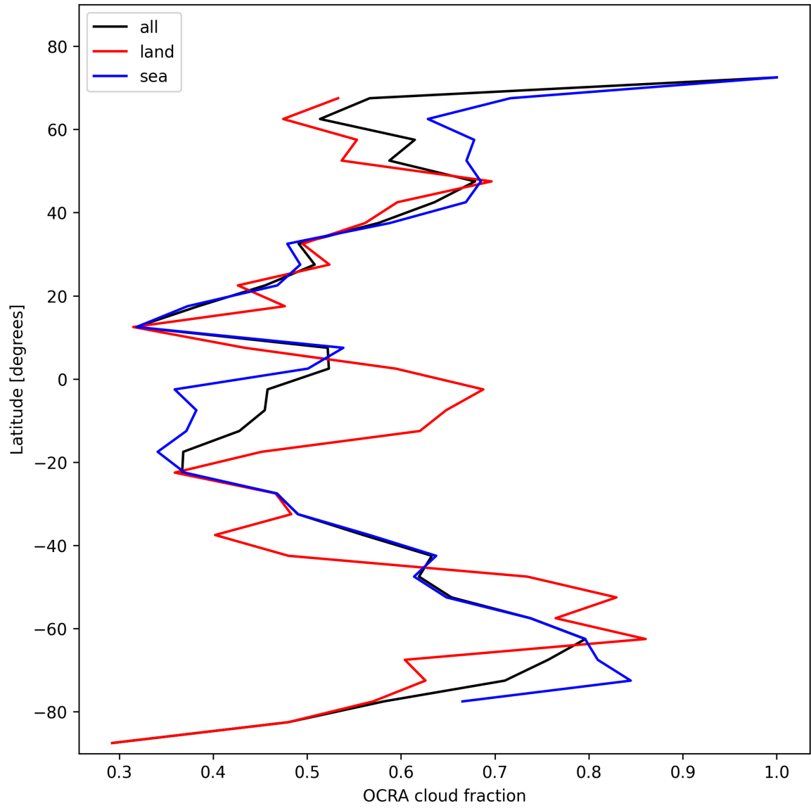
Figure 32: Zonal average of “OCRA cloud fraction” for 2025-01-24 to 2025-01-25.
