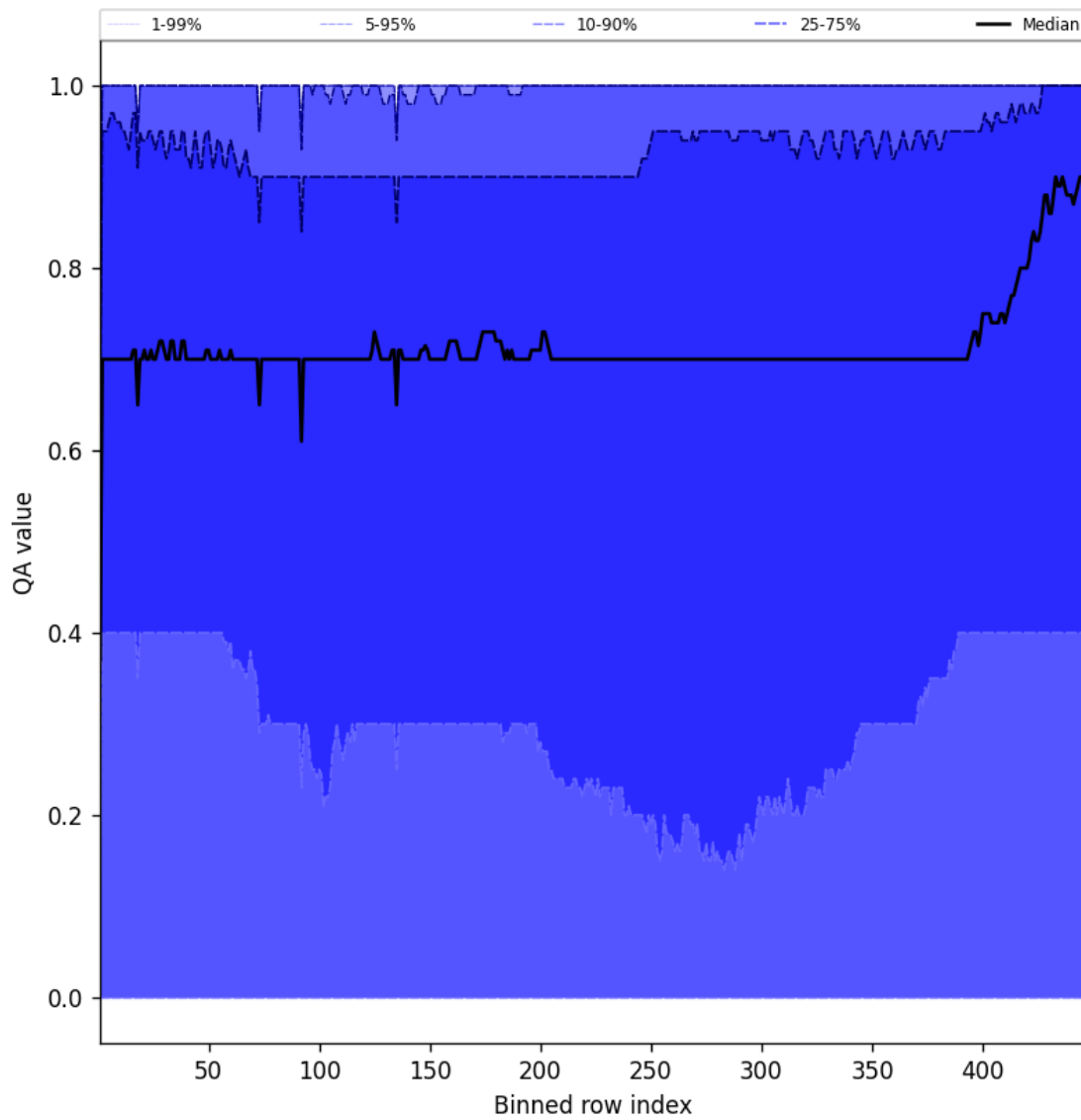
Figure 52: Along track statistics of “QA value” for 2025-01-24 to 2025-01-25
