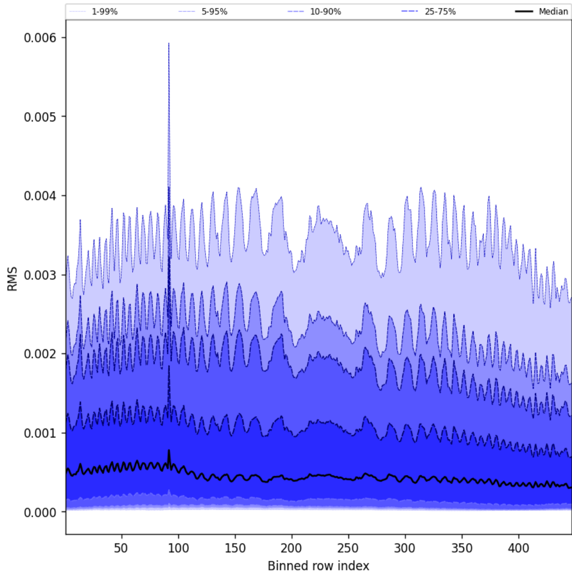
Figure 61: Along track statistics of “RMS” for 2025-01-24 to 2025-01-25
