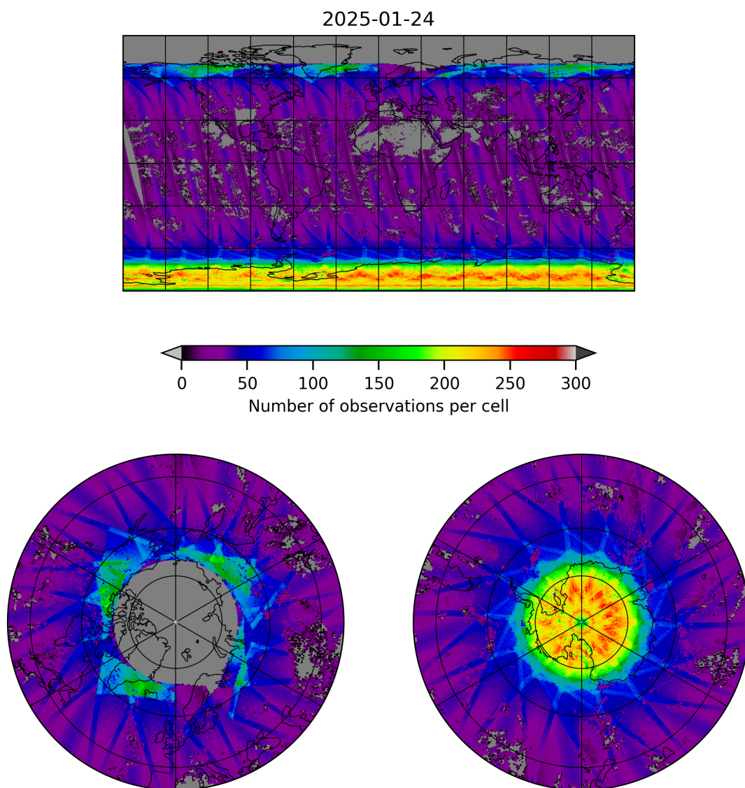
Figure 19: Map of the number of observations for 2025-01-24 to 2025-01-25
