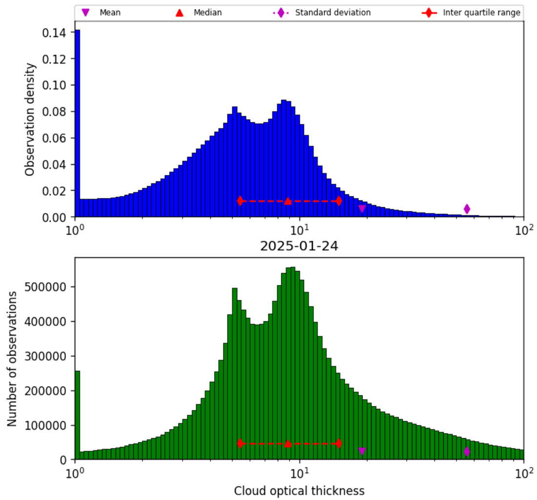
Figure 39: Histogram of “Cloud optical thickness” for 2025-01-24 to 2025-01-25
