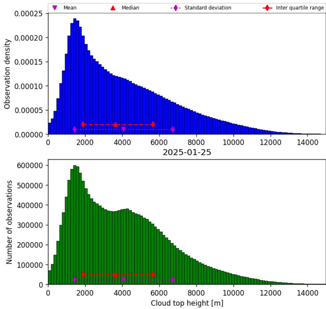
Figure 38: Histogram of “Cloud top height” for 2025-01-25 to 2025-01-26
