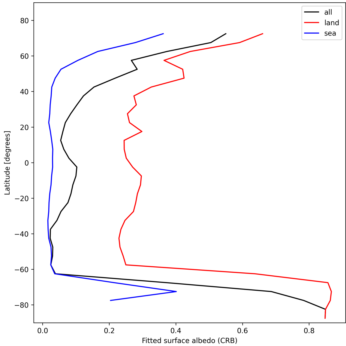
Figure 28: Zonal average of “Fitted surface albedo (CRB)” for 2025-01-25 to 2025-01-26.
