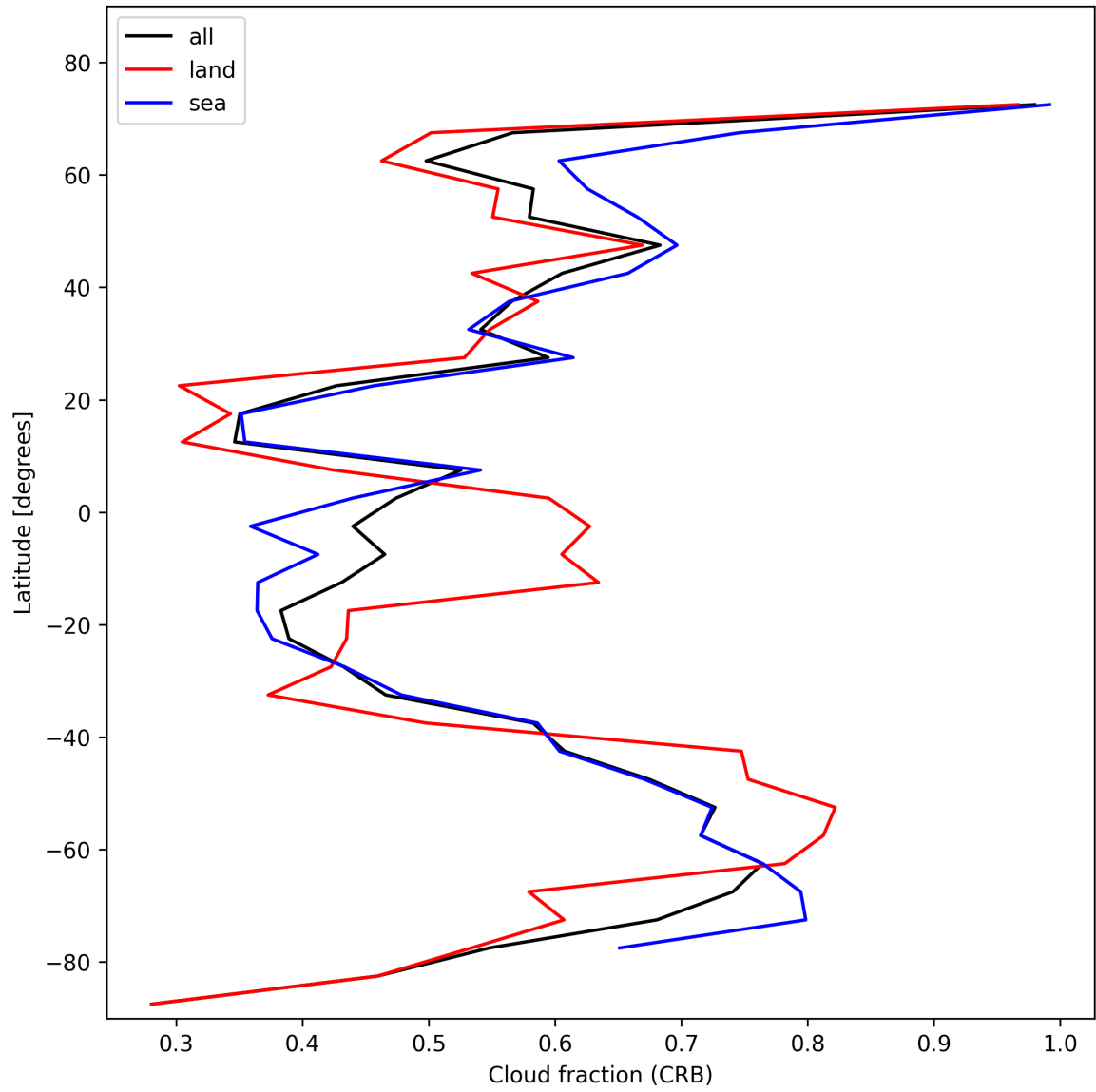
Figure 24: Zonal average of “Cloud fraction (CRB)” for 2025-01-25 to 2025-01-26.
