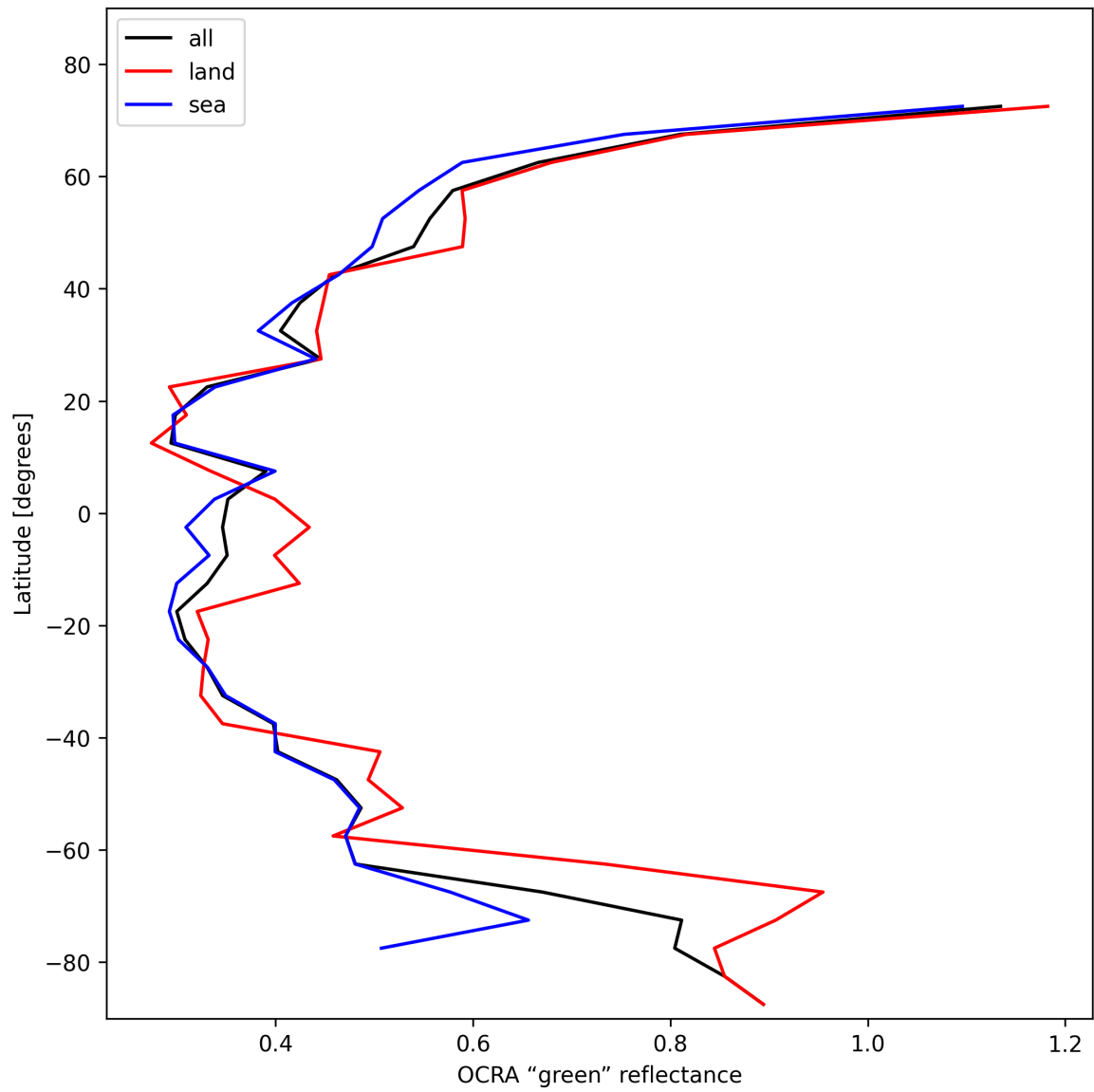
Figure 34: Zonal average of “OCRA “green” reflectance” for 2025-01-25 to 2025-01-26.
