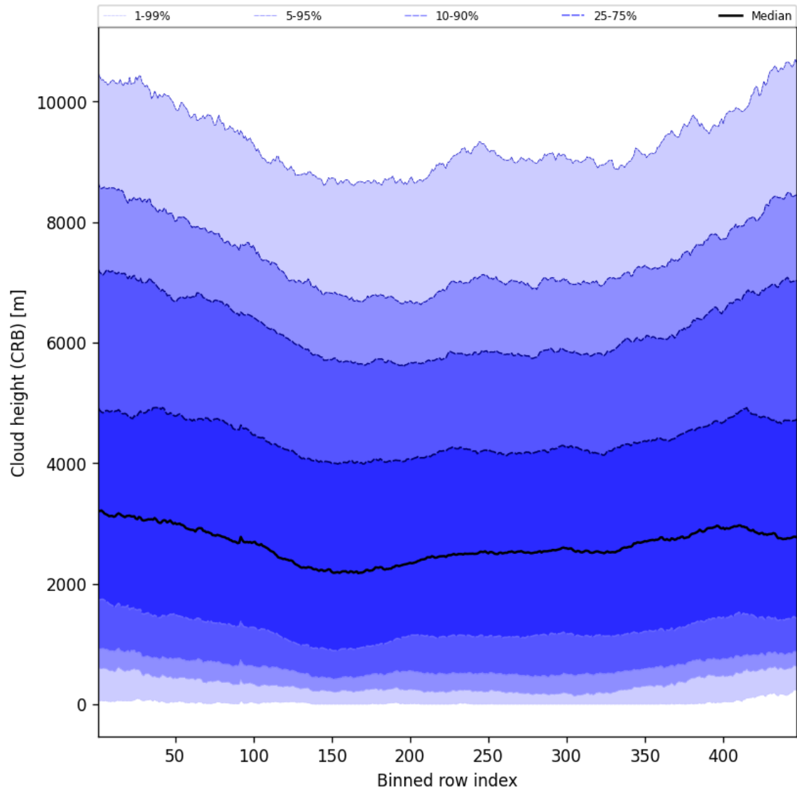
Figure 57: Along track statistics of “Cloud height (CRB)” for 2025-01-25 to 2025-01-26
