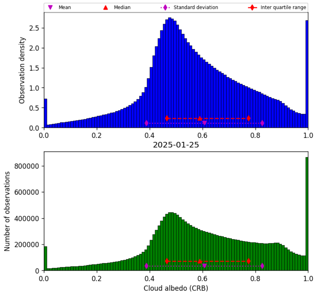
Figure 42: Histogram of “Cloud albedo (CRB)” for 2025-01-25 to 2025-01-26
