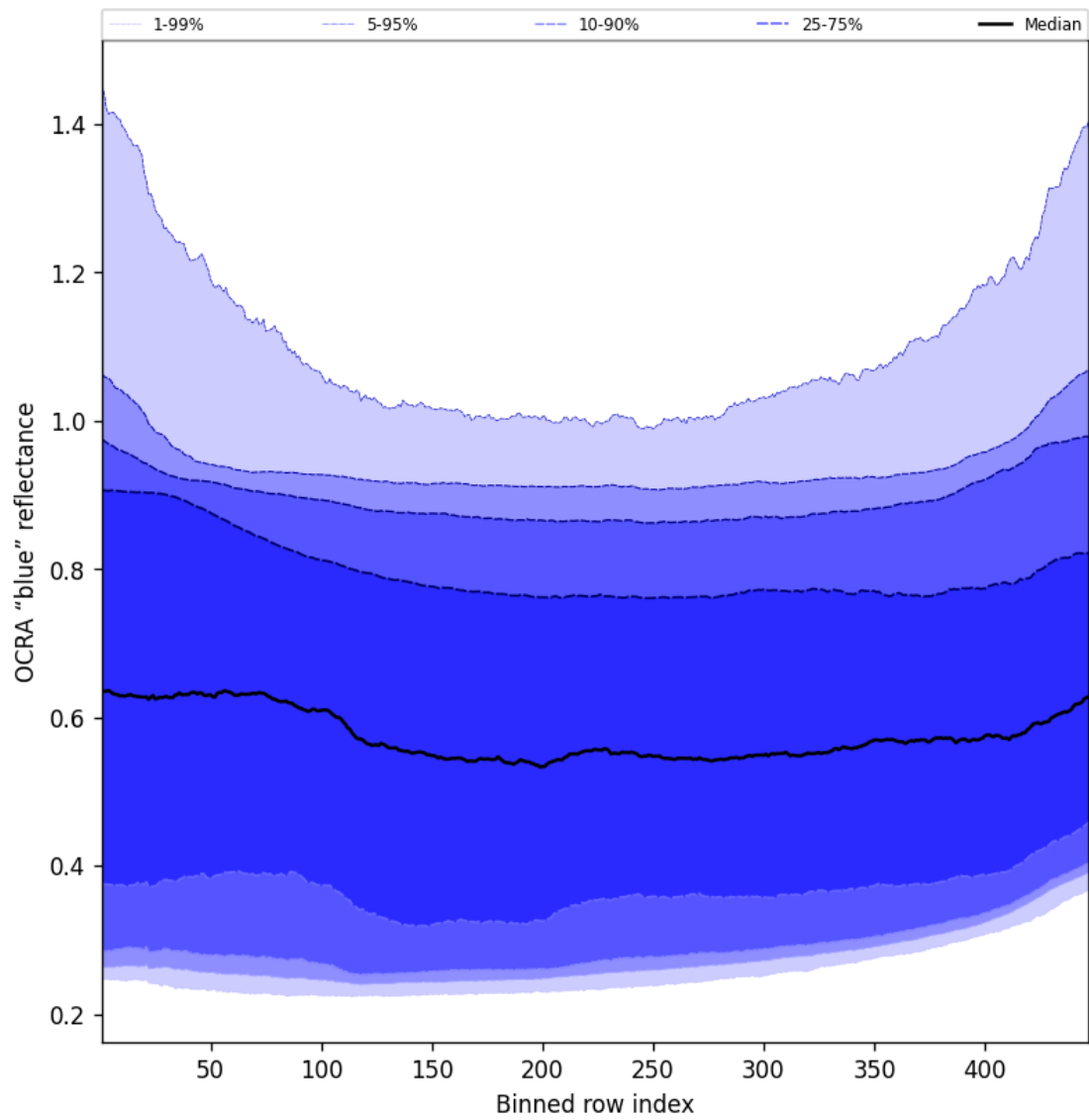
Figure 65: Along track statistics of “OCRA “blue” reflectance” for 2025-01-25 to 2025-01-26
