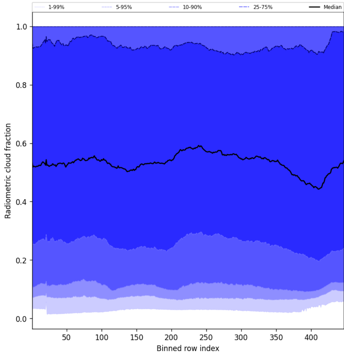
Figure 53: Along track statistics of “Radiometric cloud fraction” for 2025-01-25 to 2025-01-26
