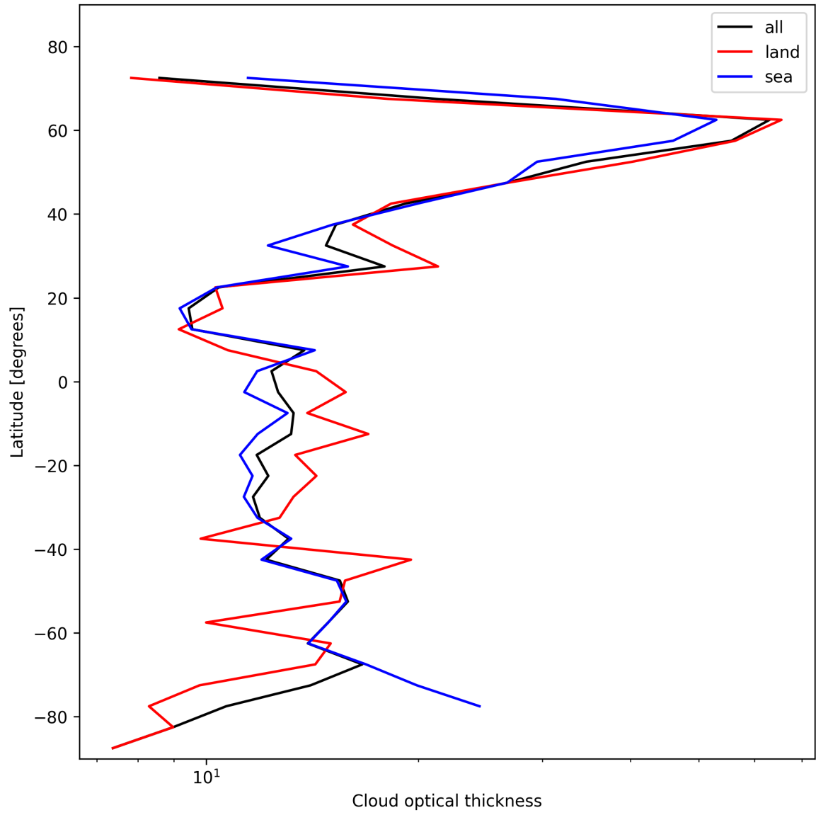
Figure 23: Zonal average of “Cloud optical thickness” for 2025-01-25 to 2025-01-26.
