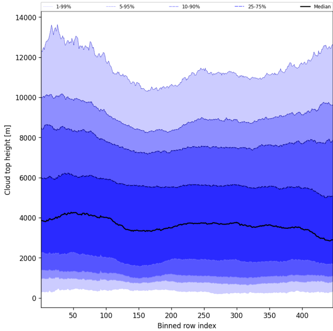
Figure 54: Along track statistics of “Cloud top height” for 2025-01-25 to 2025-01-26
