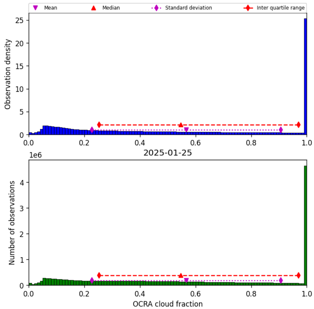
Figure 48: Histogram of “OCRA cloud fraction” for 2025-01-25 to 2025-01-26
