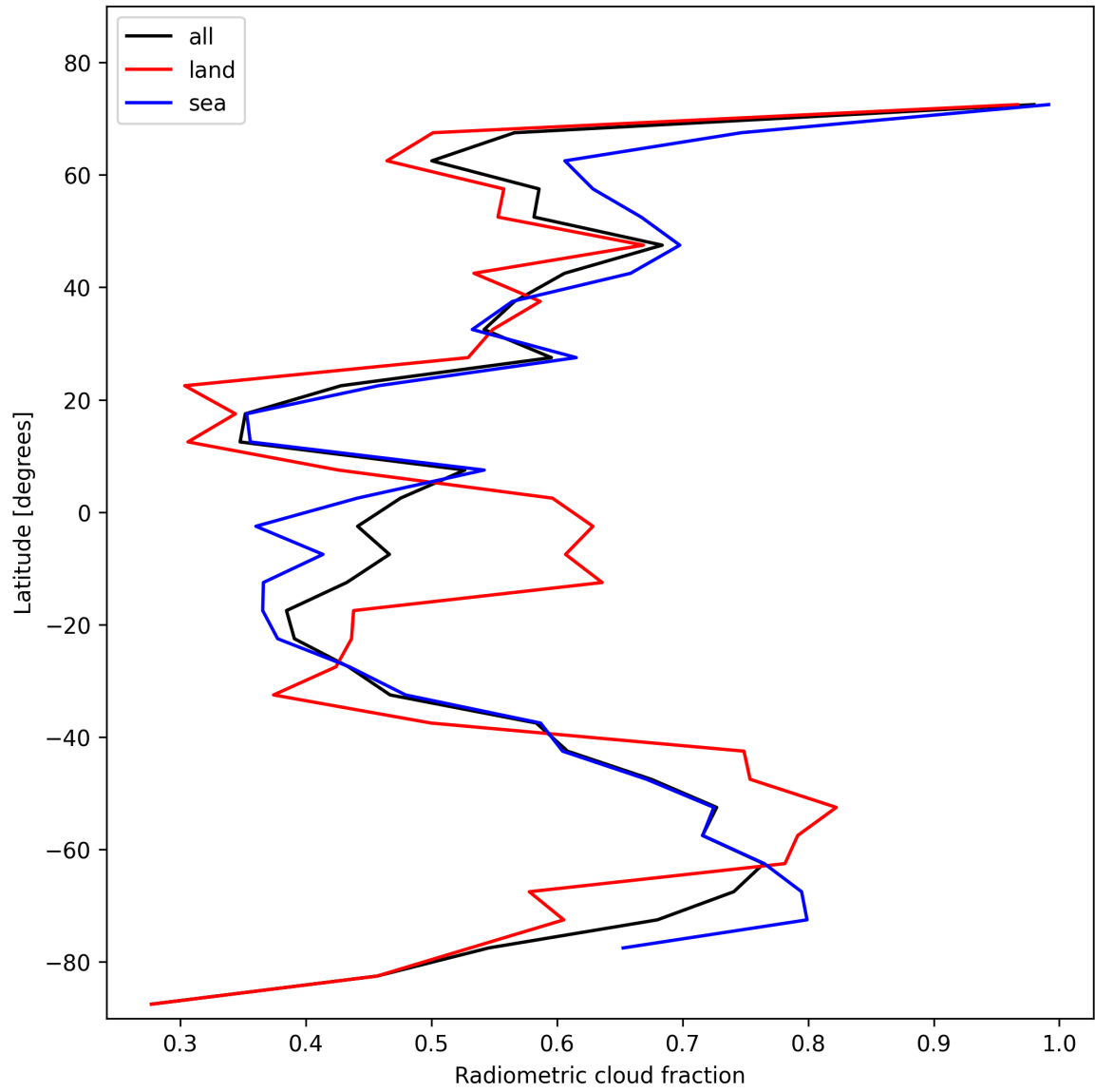
Figure 21: Zonal average of “Radiometric cloud fraction” for 2025-01-25 to 2025-01-26.
