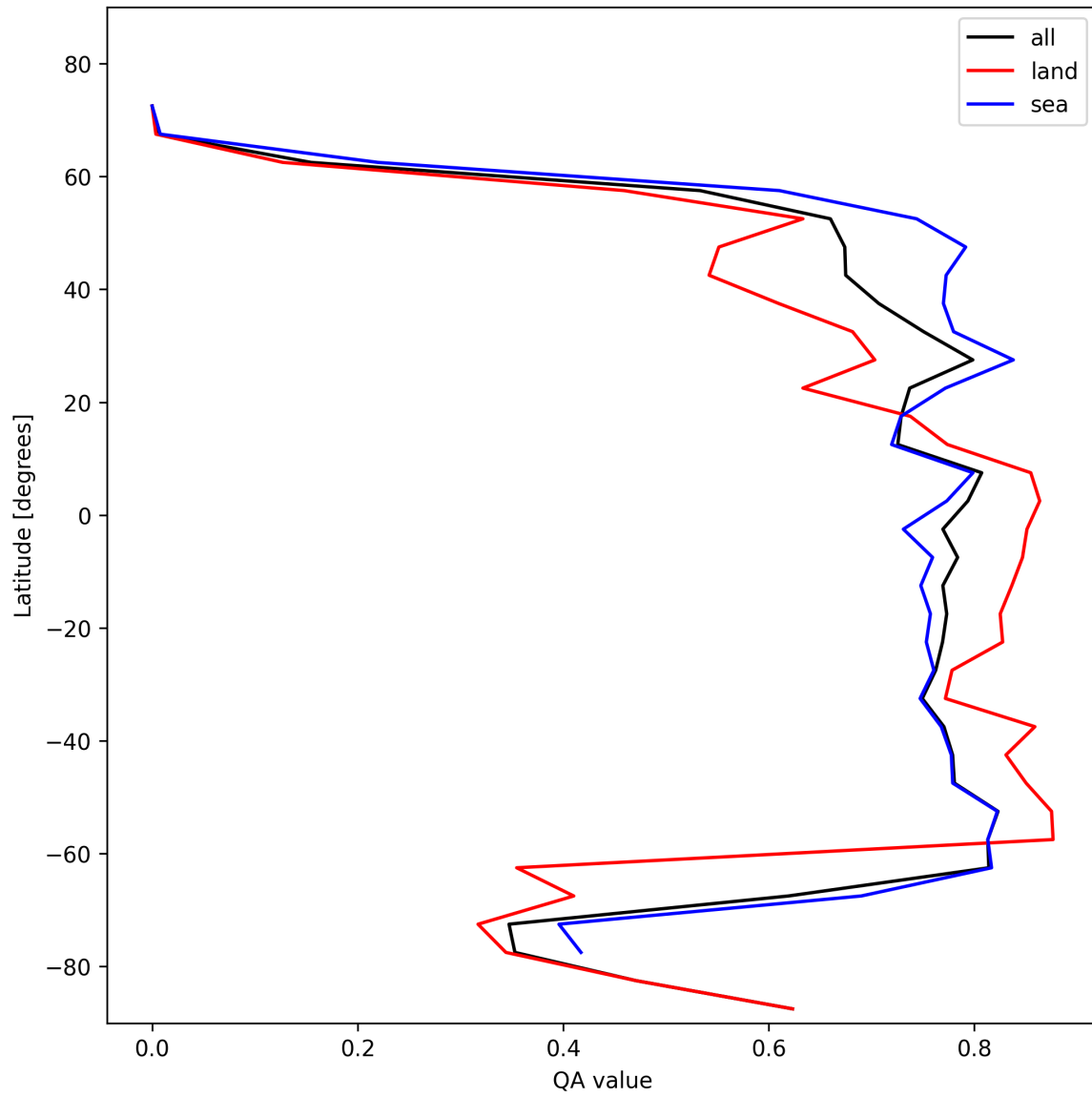
Figure 20: Zonal average of “QA value” for 2025-01-25 to 2025-01-26.
