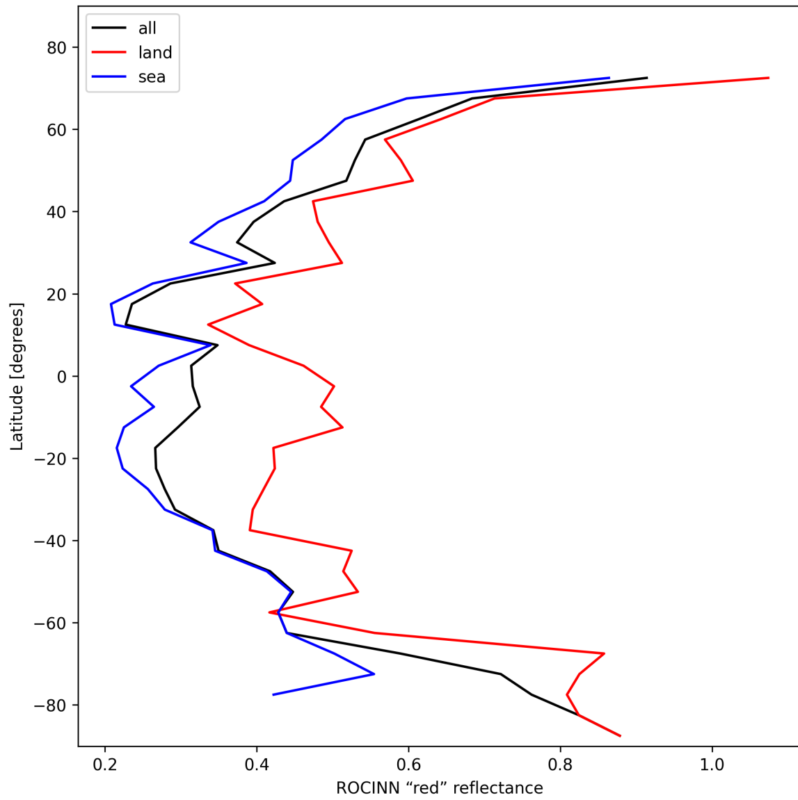
Figure 35: Zonal average of “ROCINN “red” reflectance” for 2025-01-25 to 2025-01-26.
