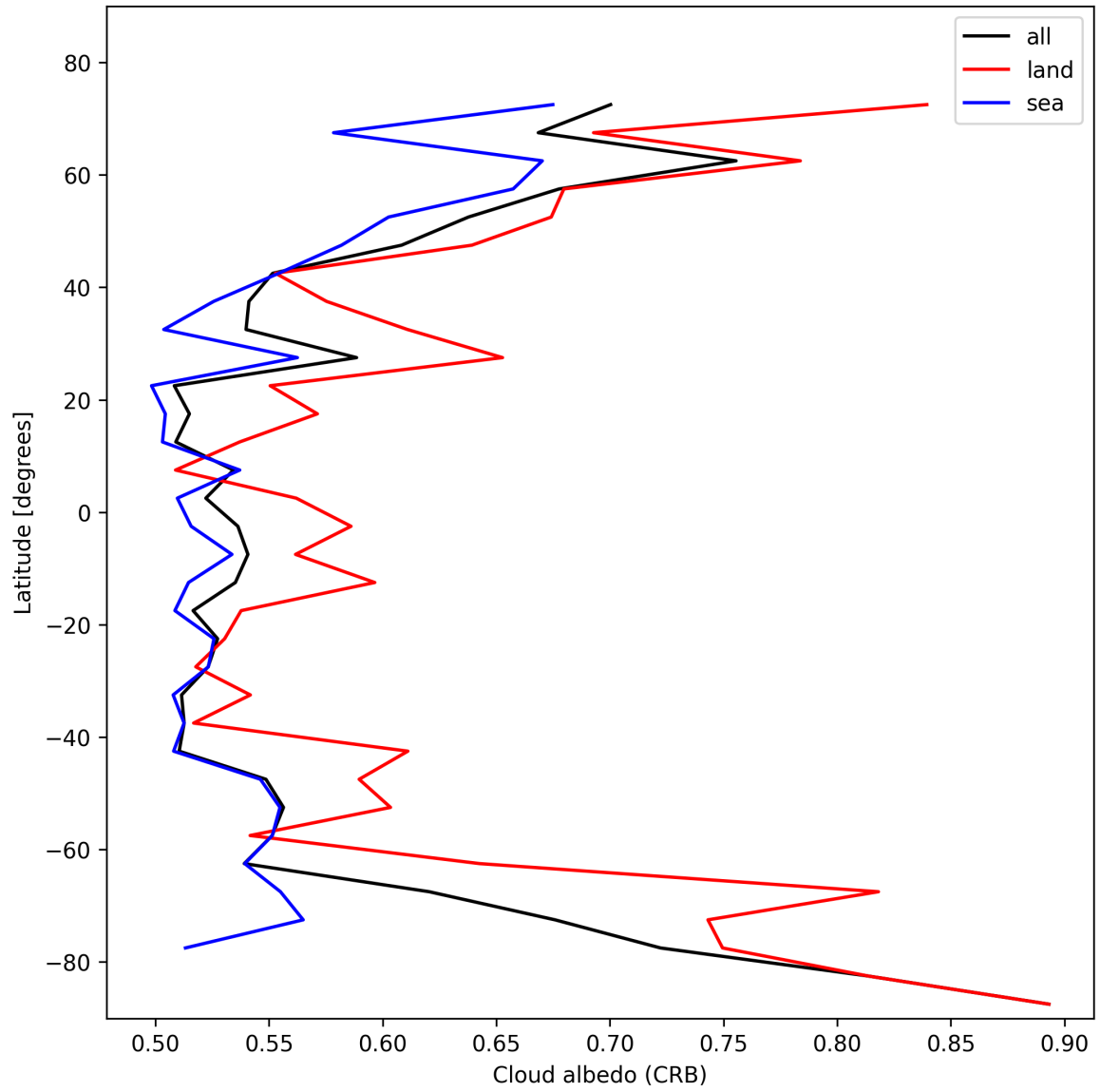
Figure 26: Zonal average of “Cloud albedo (CRB)” for 2025-01-25 to 2025-01-26.
