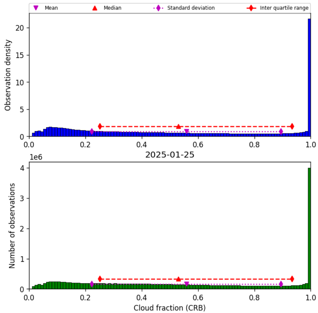
Figure 40: Histogram of “Cloud fraction (CRB)” for 2025-01-25 to 2025-01-26
