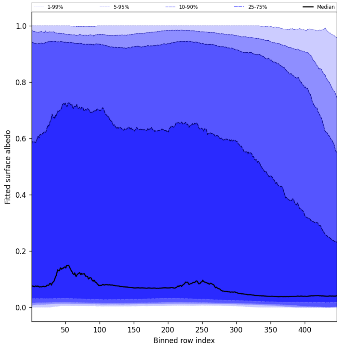
Figure 59: Along track statistics of “Fitted surface albedo” for 2025-01-25 to 2025-01-26
