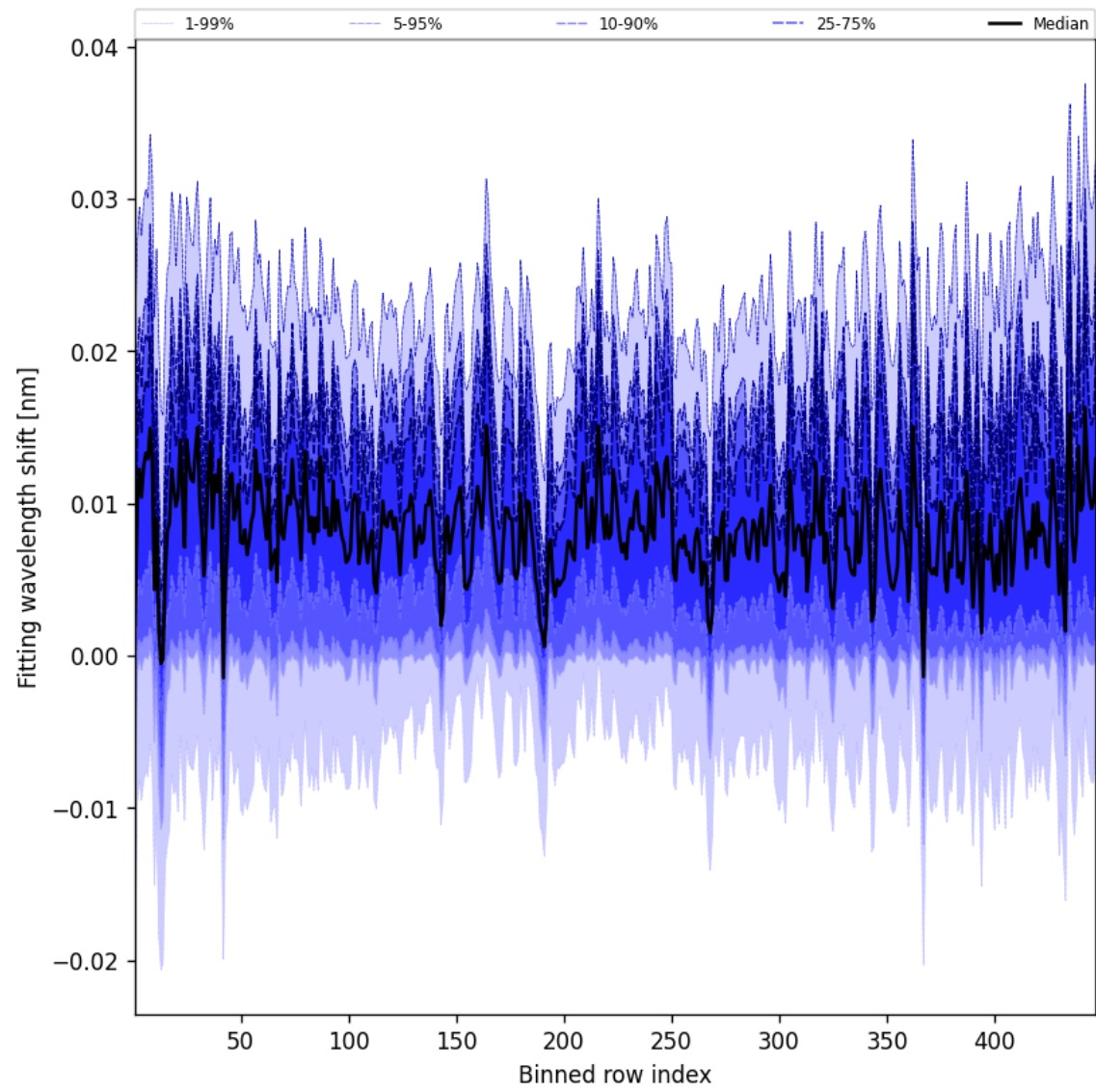
Figure 63: Along track statistics of “Fitting wavelength shift” for 2025-01-25 to 2025-01-26
