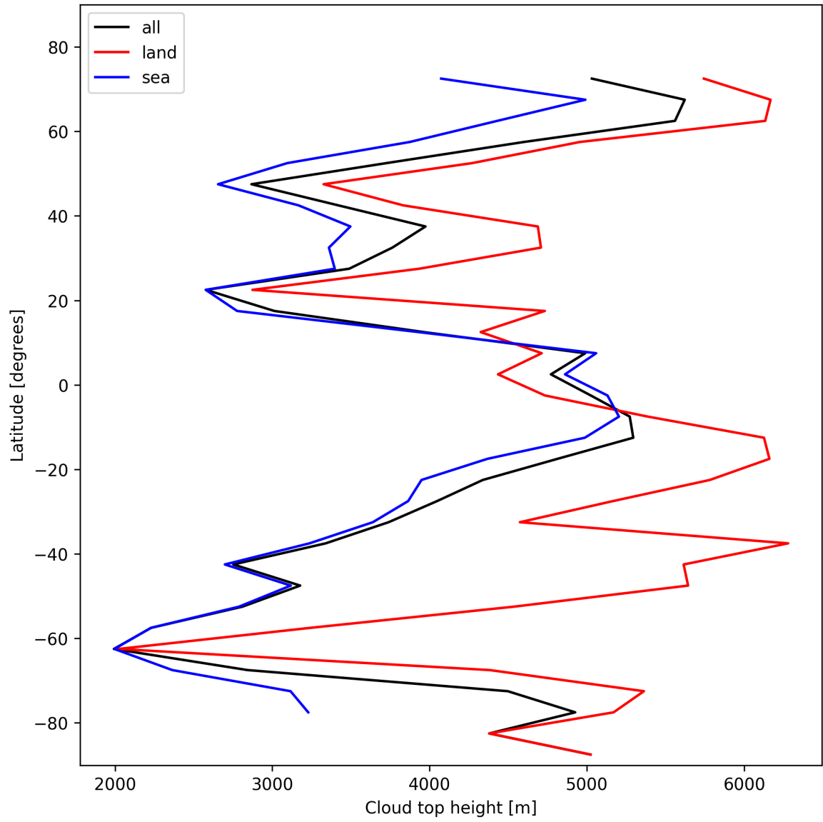
Figure 22: Zonal average of “Cloud top height” for 2025-01-25 to 2025-01-26.
