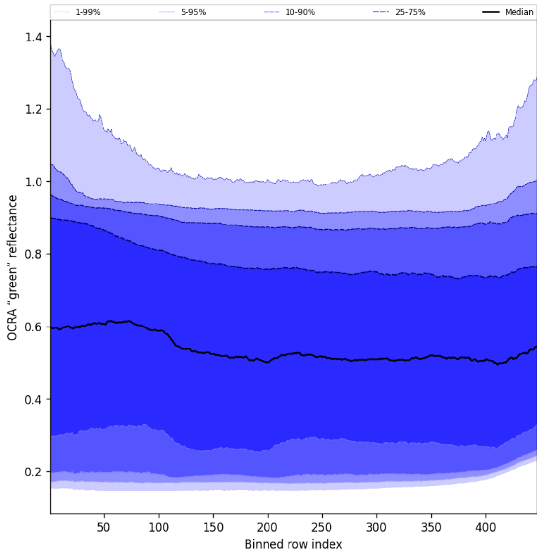
Figure 66: Along track statistics of “OCRA “green” reflectance” for 2025-01-25 to 2025-01-26
