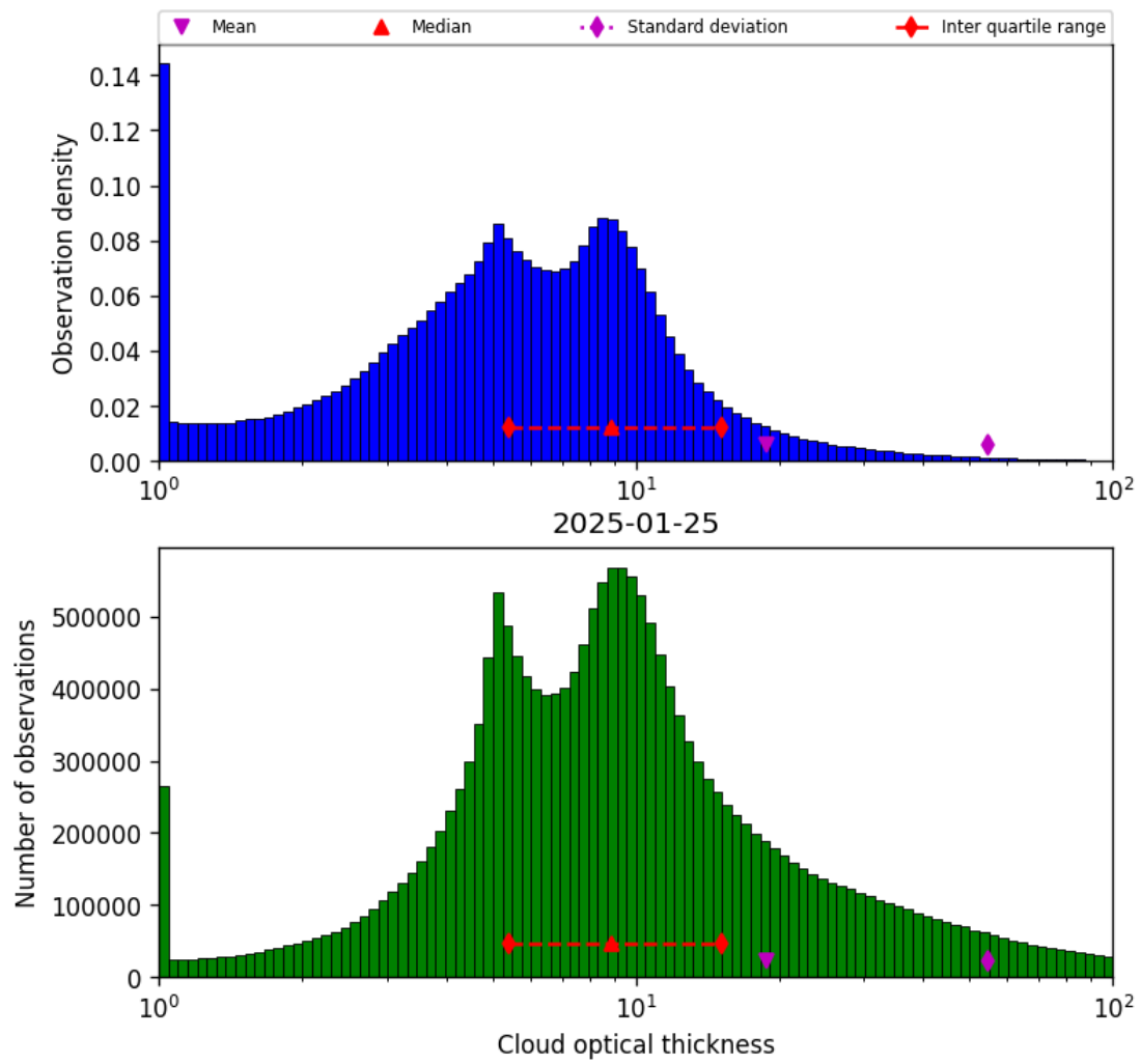
Figure 39: Histogram of “Cloud optical thickness” for 2025-01-25 to 2025-01-26
