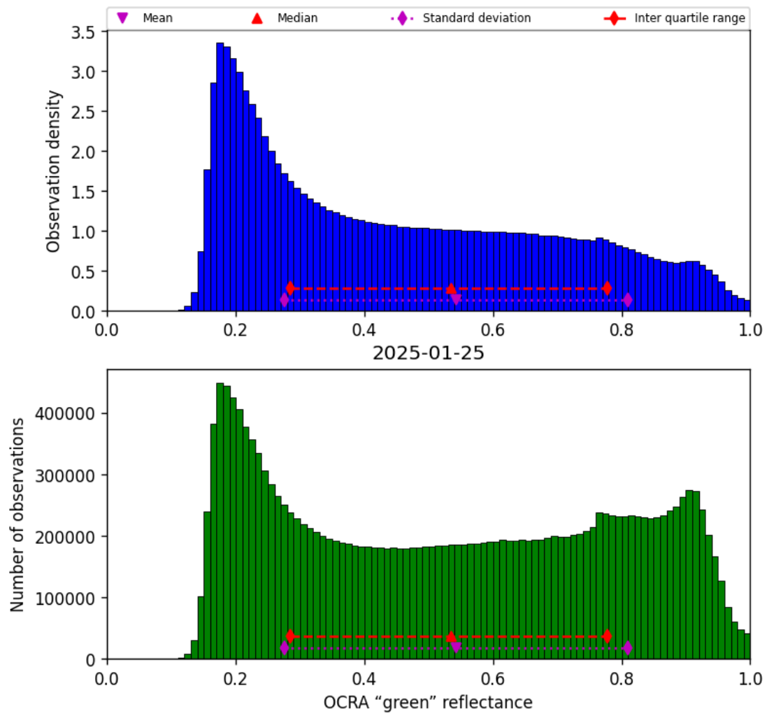
Figure 50: Histogram of “OCRA “green” reflectance” for 2025-01-25 to 2025-01-26
