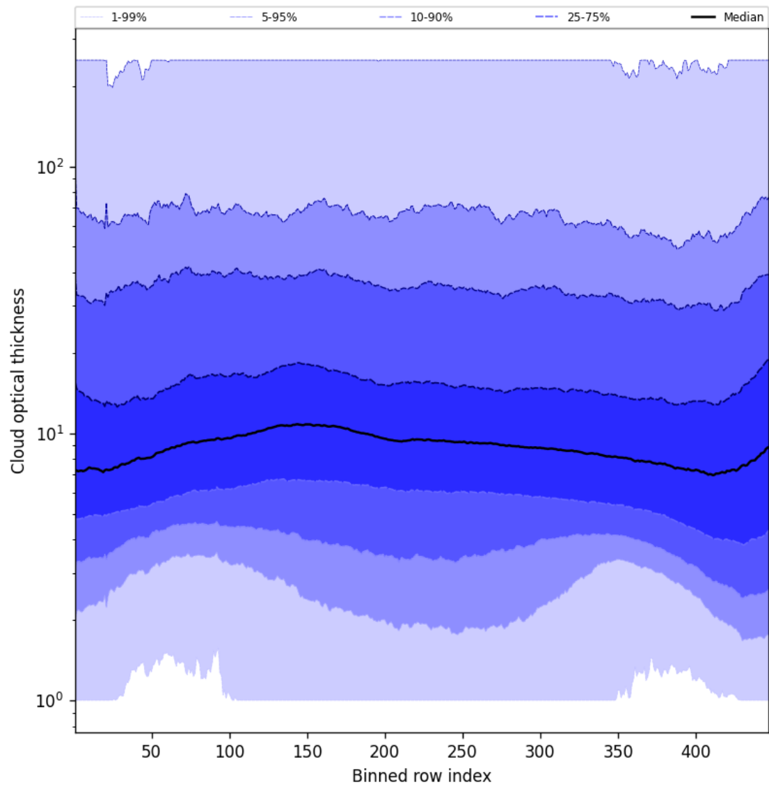
Figure 55: Along track statistics of “Cloud optical thickness” for 2025-01-25 to 2025-01-26
