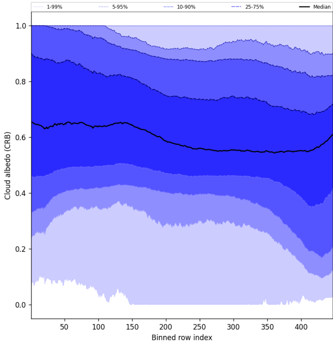
Figure 58: Along track statistics of “Cloud albedo (CRB)” for 2025-01-25 to 2025-01-26
