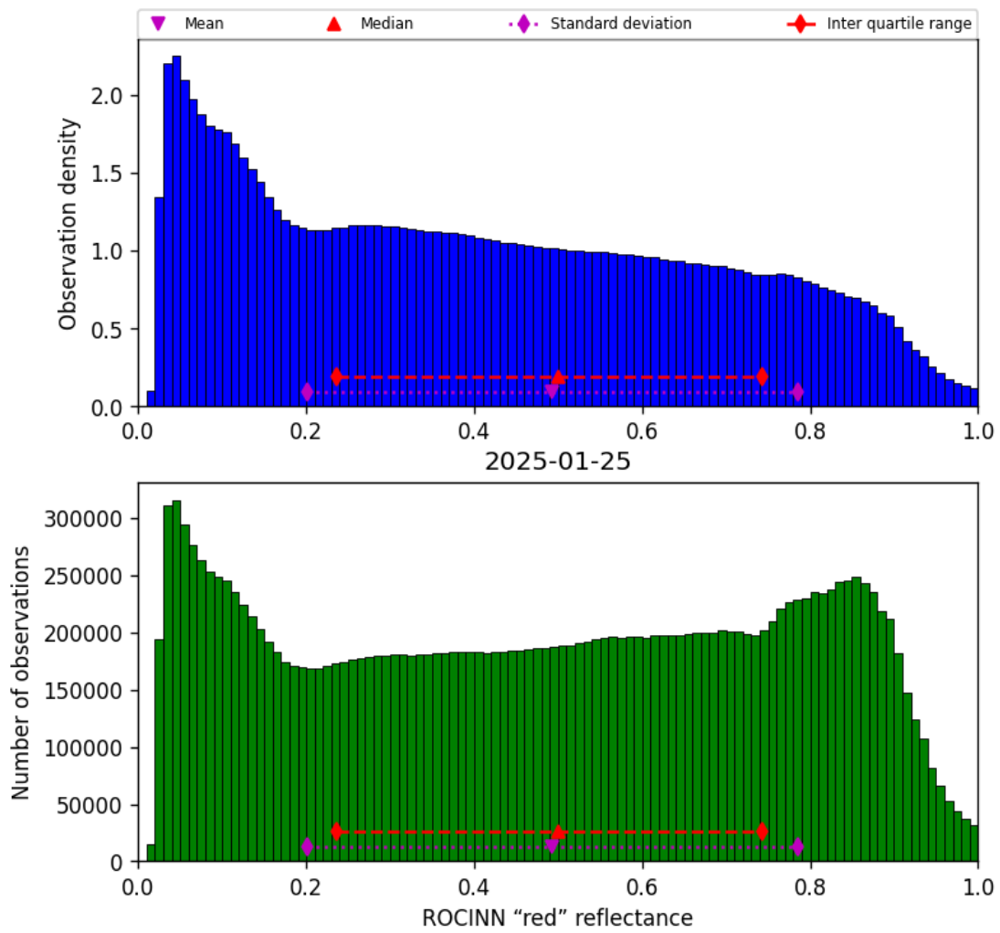
Figure 51: Histogram of “ROCINN “red” reflectance” for 2025-01-25 to 2025-01-26
