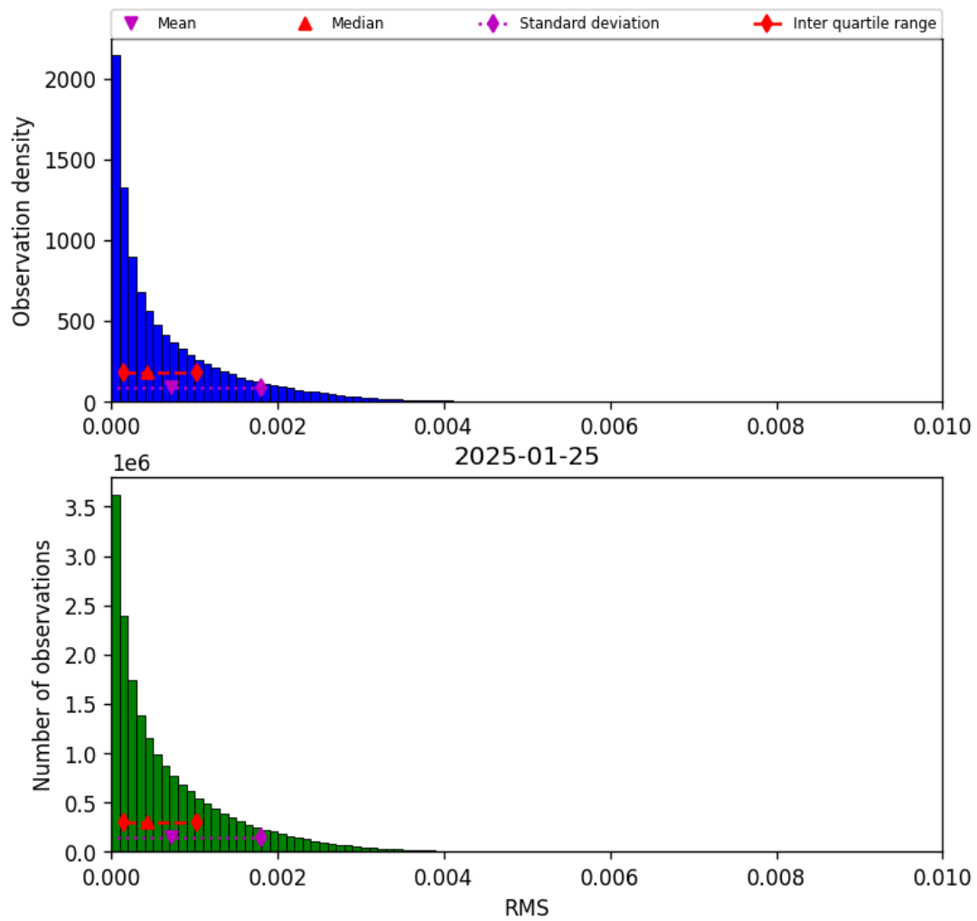
Figure 45: Histogram of “RMS” for 2025-01-25 to 2025-01-26
