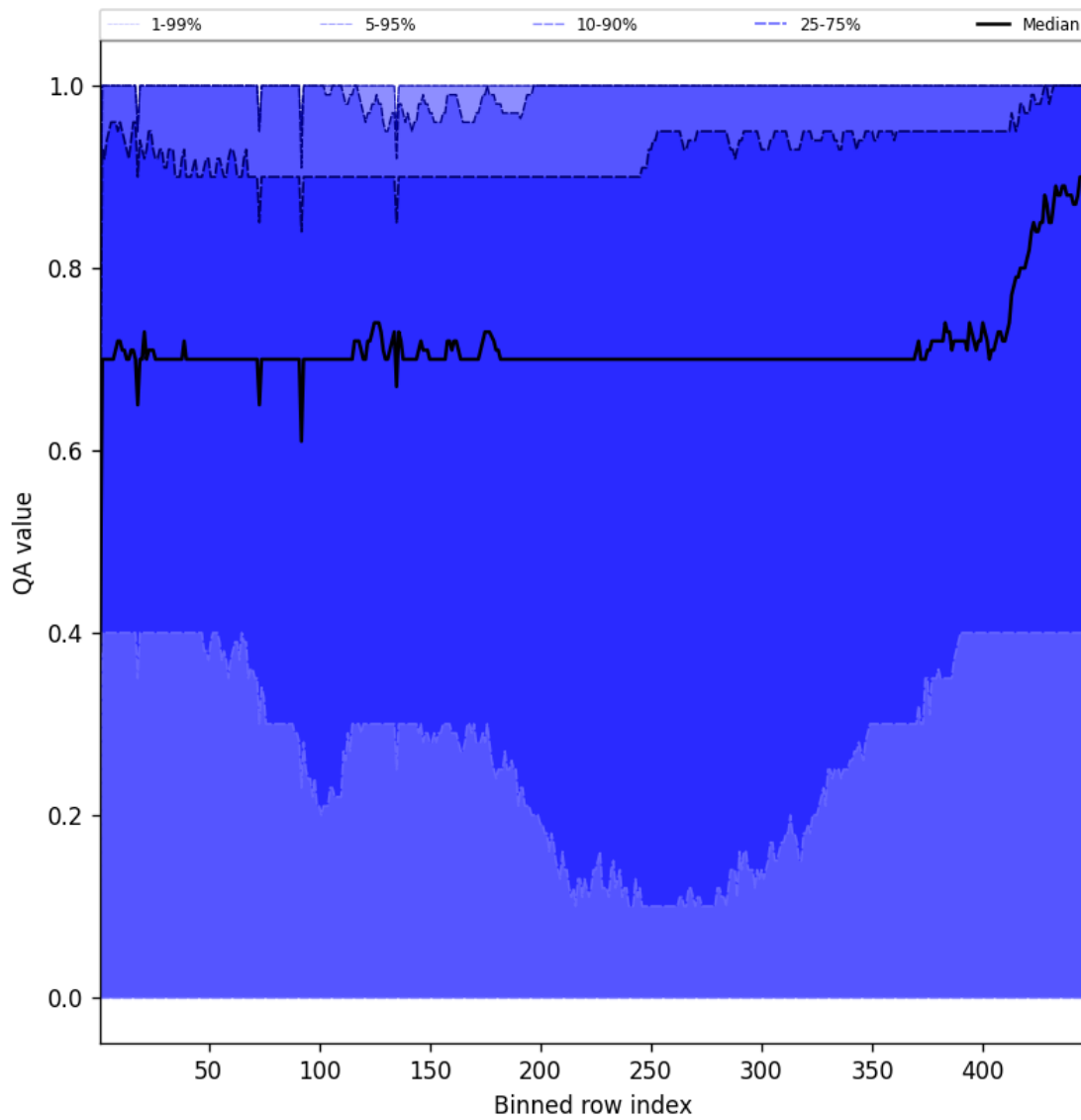
Figure 52: Along track statistics of "QA value" for 2025-01-25 to 2025-01-26
