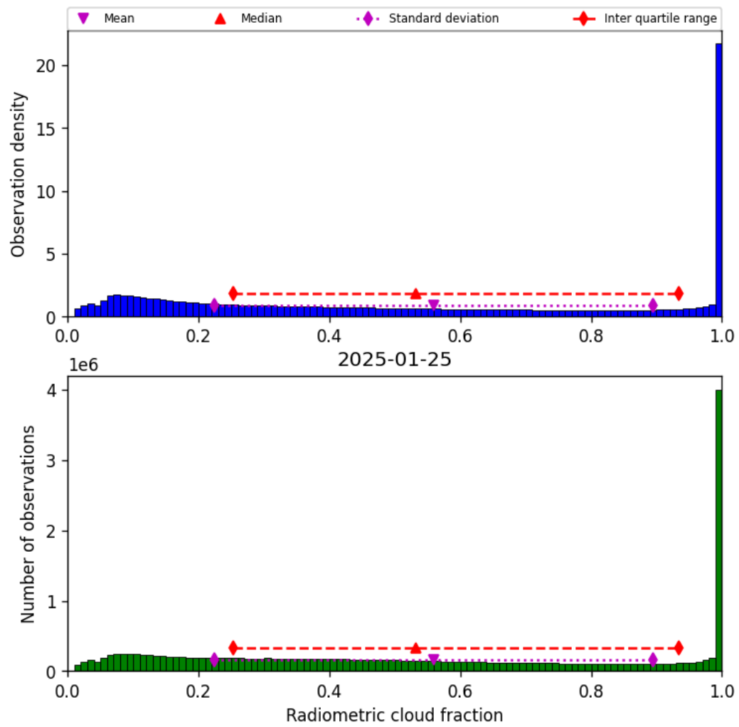
Figure 37: Histogram of “Radiometric cloud fraction” for 2025-01-25 to 2025-01-26
