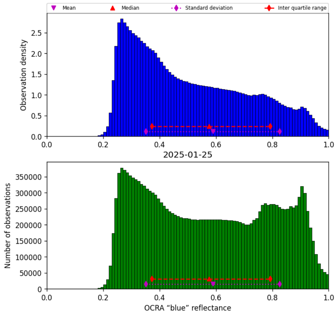
Figure 49: Histogram of “OCRA “blue” reflectance” for 2025-01-25 to 2025-01-26
