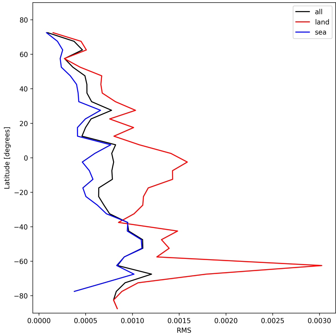
Figure 29: Zonal average of “RMS” for 2025-01-25 to 2025-01-26.
