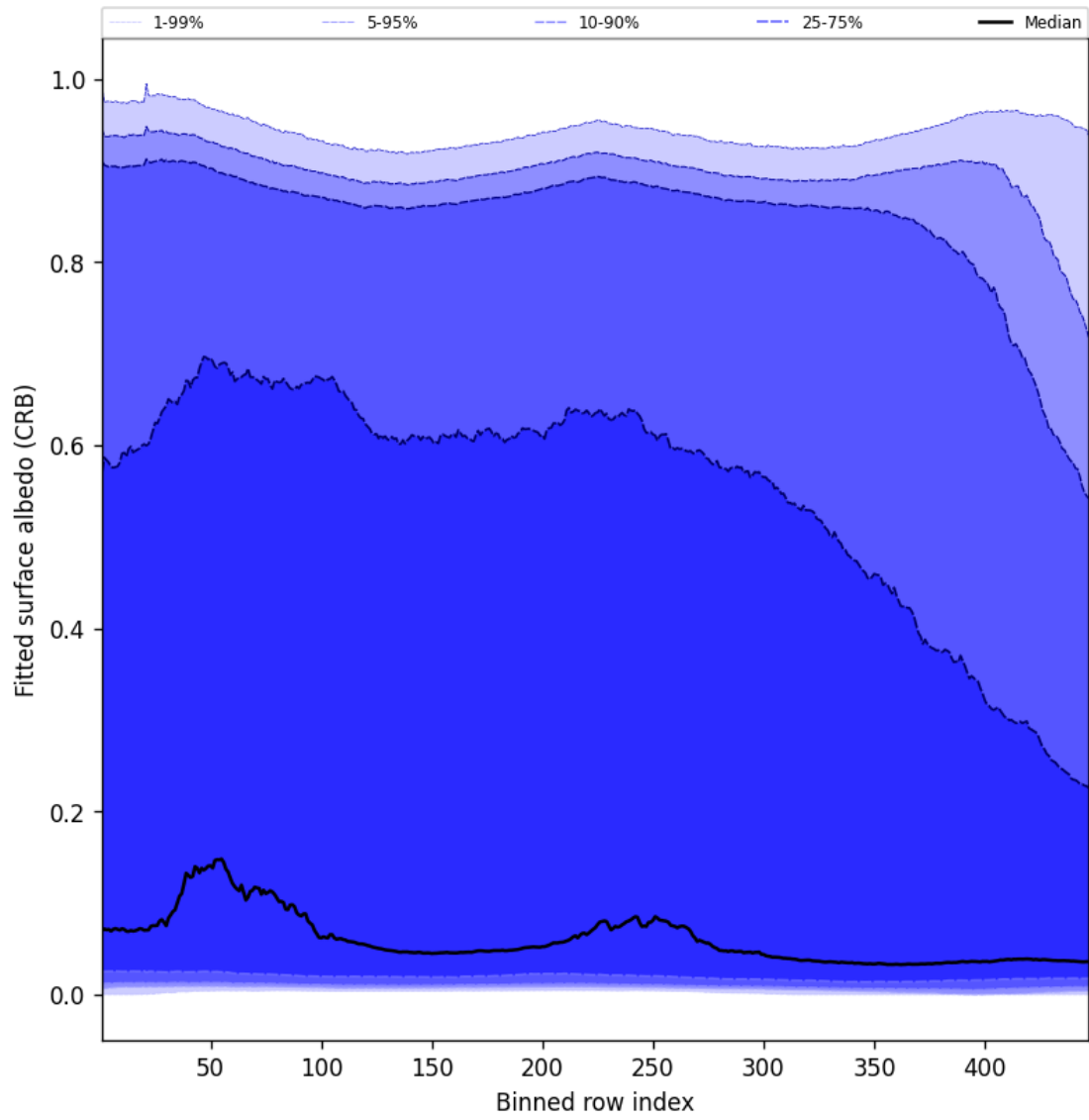
Figure 60: Along track statistics of “Fitted surface albedo (CRB)” for 2025-01-25 to 2025-01-26
