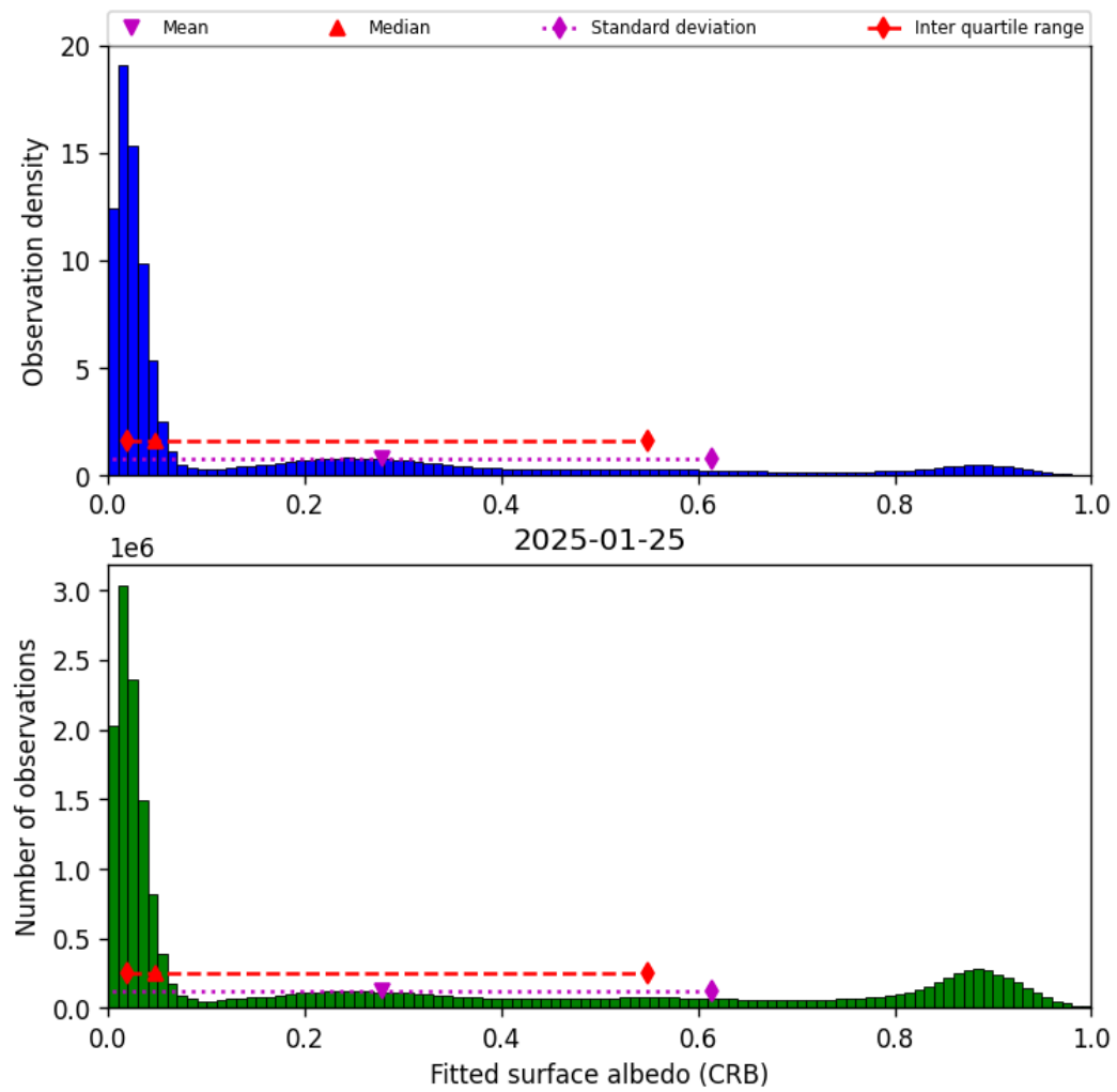
Figure 44: Histogram of “Fitted surface albedo (CRB)” for 2025-01-25 to 2025-01-26
