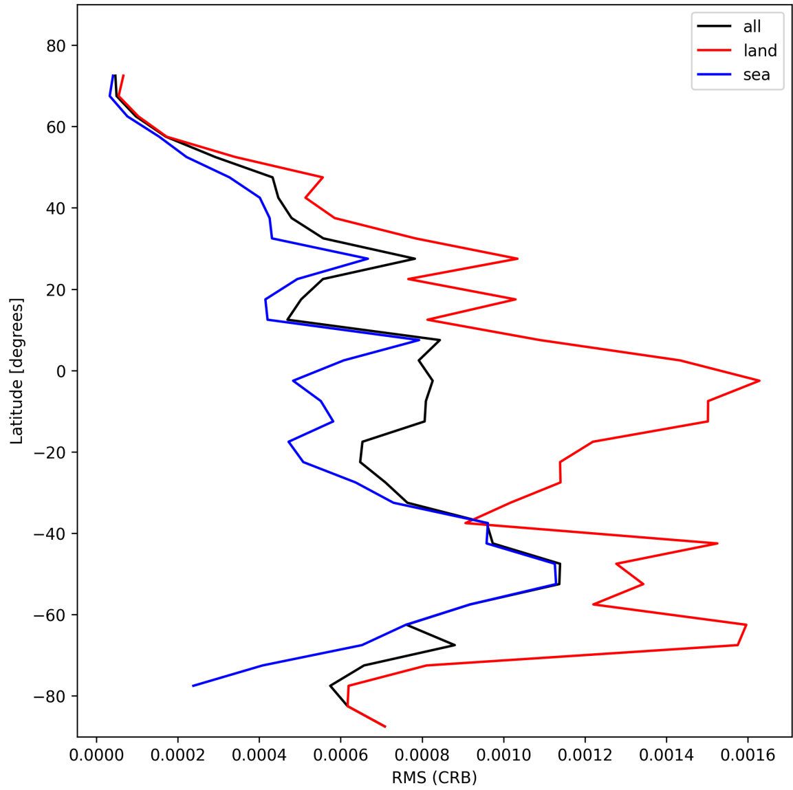
Figure 30: Zonal average of “RMS (CRB)” for 2025-01-25 to 2025-01-26.
