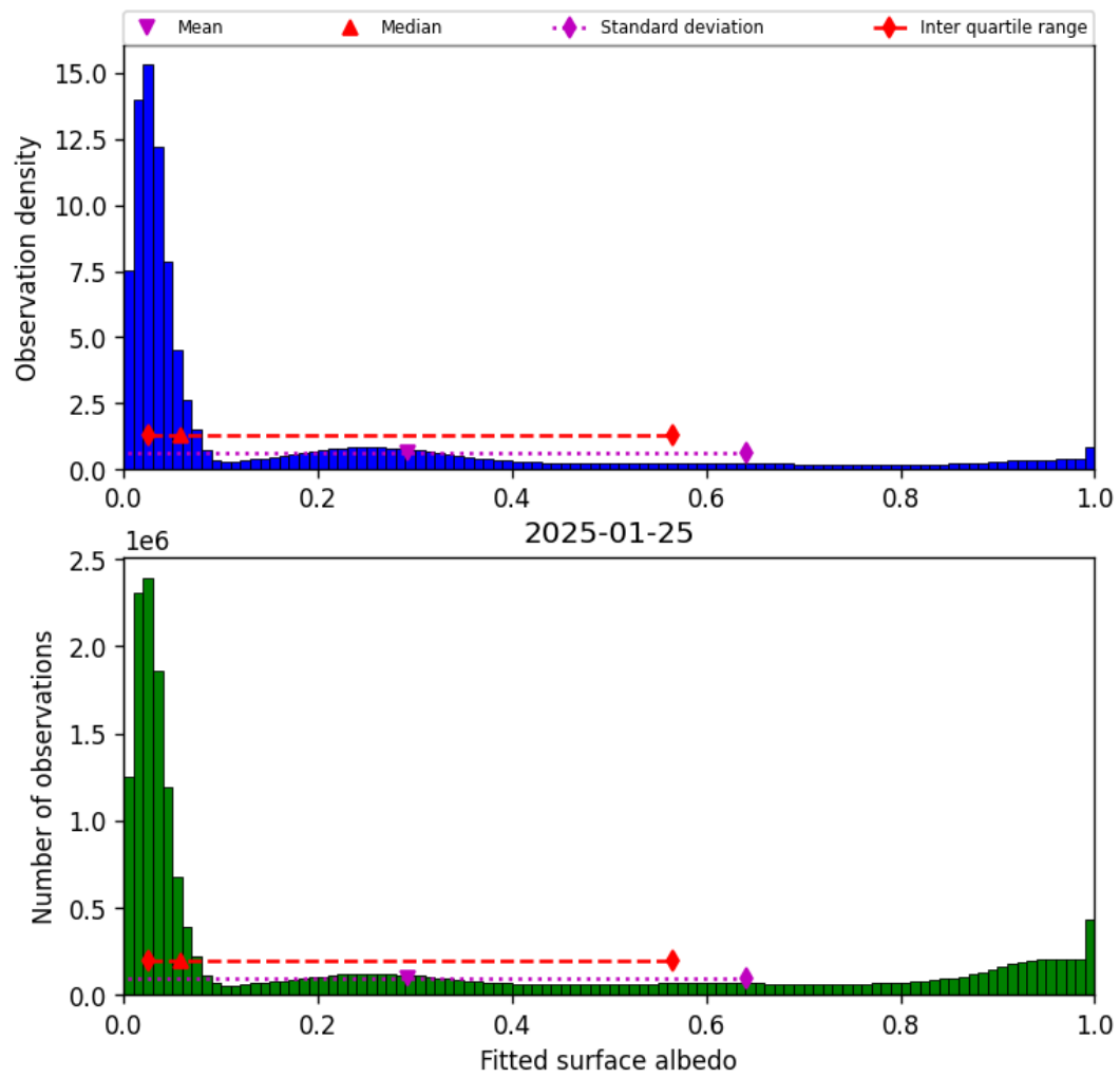
Figure 43: Histogram of “Fitted surface albedo” for 2025-01-25 to 2025-01-26
