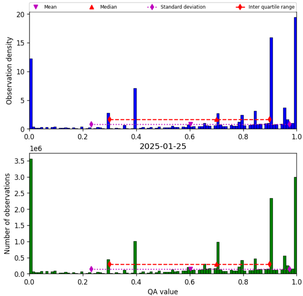
Figure 36: Histogram of “QA value” for 2025-01-25 to 2025-01-26
