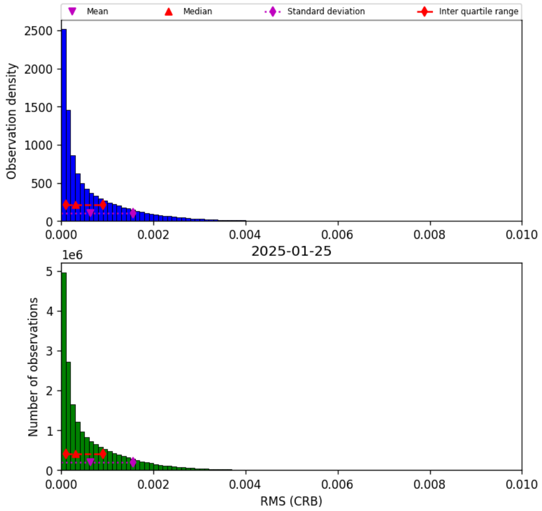
Figure 46: Histogram of “RMS (CRB)” for 2025-01-25 to 2025-01-26
