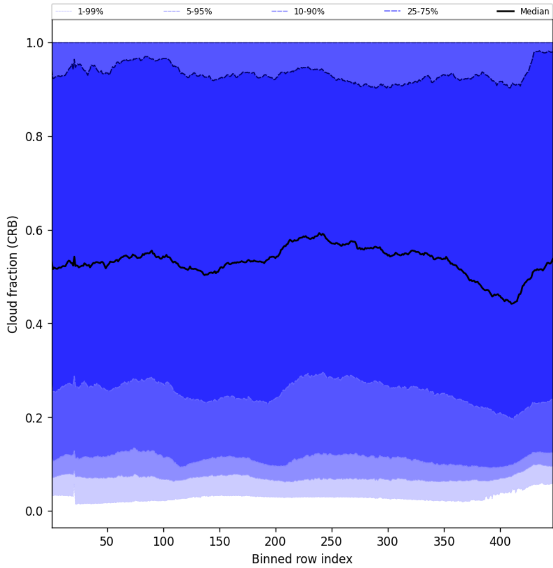
Figure 56: Along track statistics of “Cloud fraction (CRB)” for 2025-01-25 to 2025-01-26
