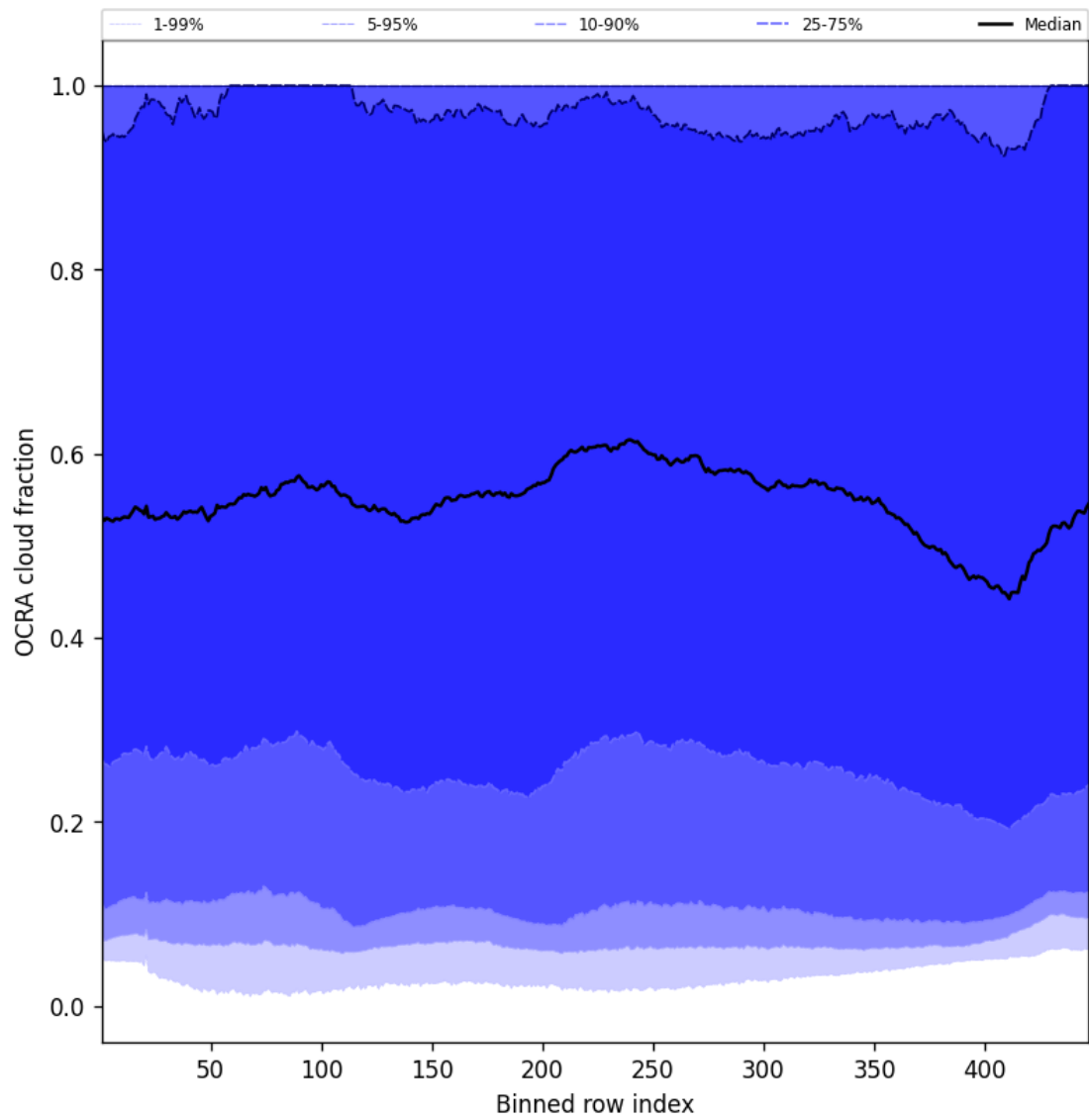
Figure 64: Along track statistics of “OCRA cloud fraction” for 2025-01-25 to 2025-01-26
