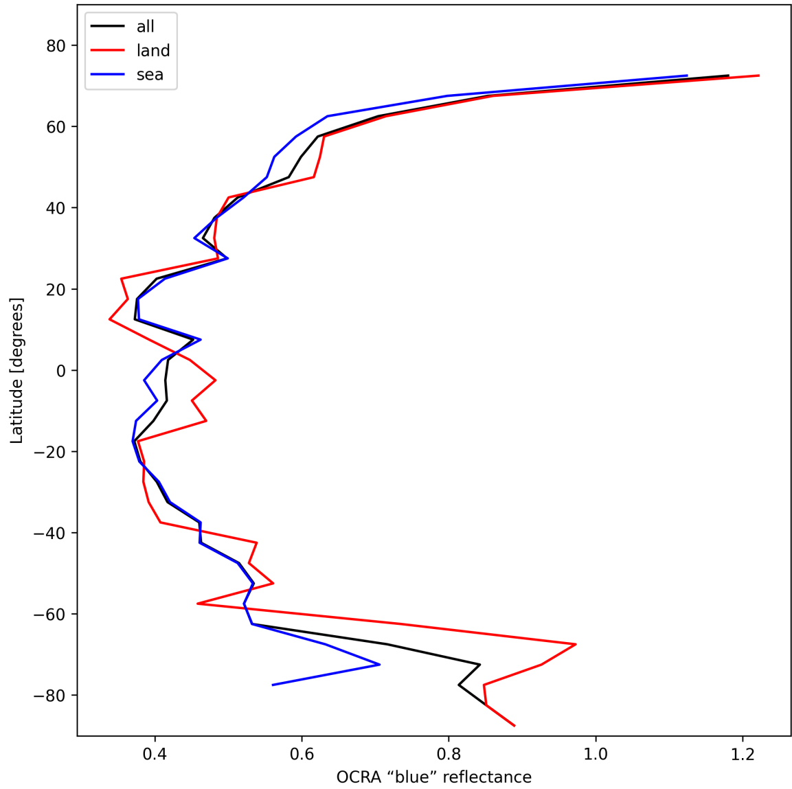
Figure 33: Zonal average of “OCRA “blue” reflectance” for 2025-01-25 to 2025-01-26.
