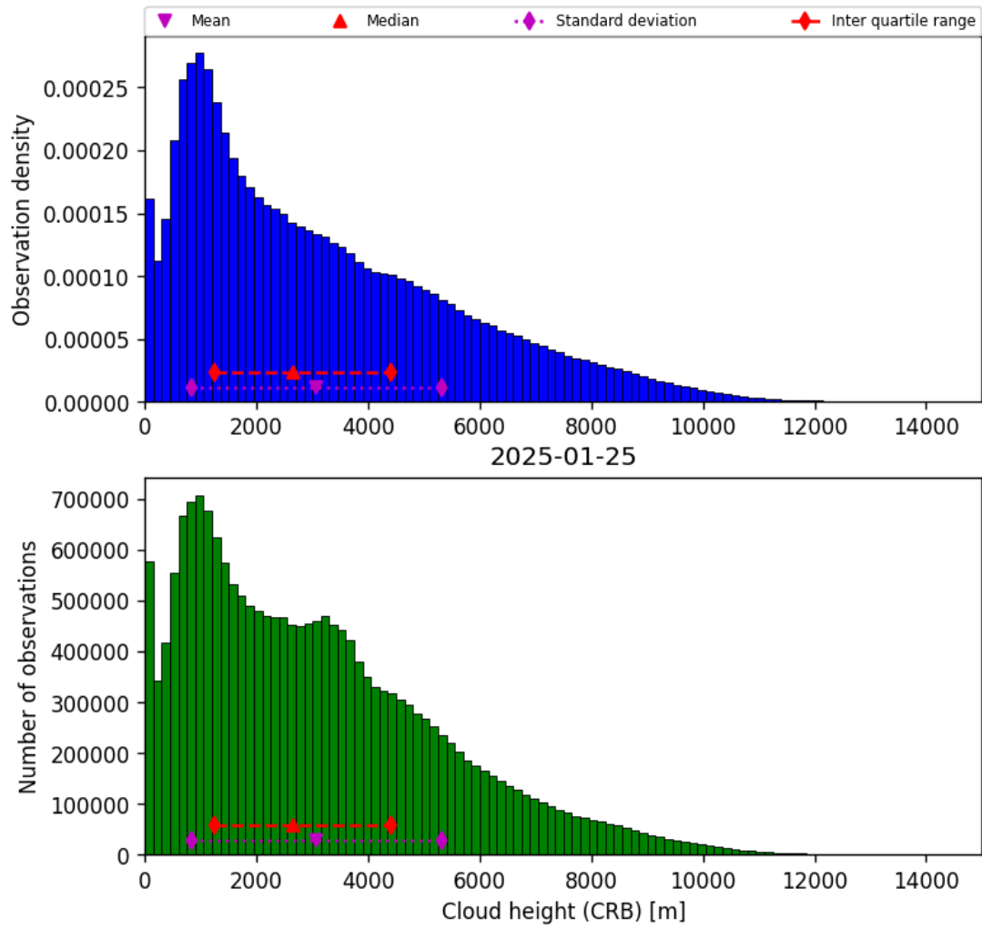
Figure 41: Histogram of “Cloud height (CRB)” for 2025-01-25 to 2025-01-26
