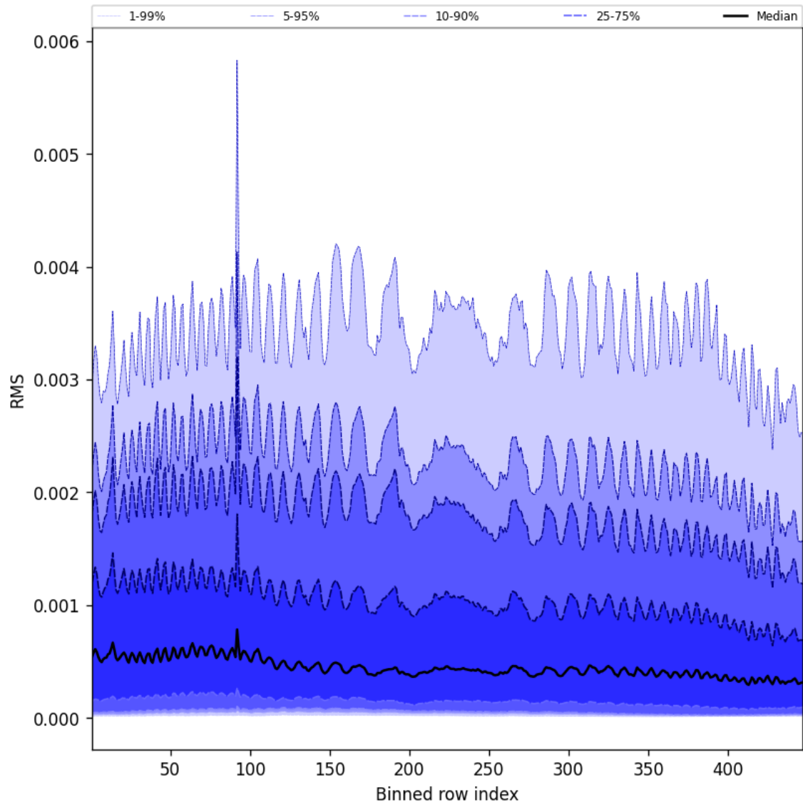
Figure 61: Along track statistics of “RMS” for 2025-01-25 to 2025-01-26
