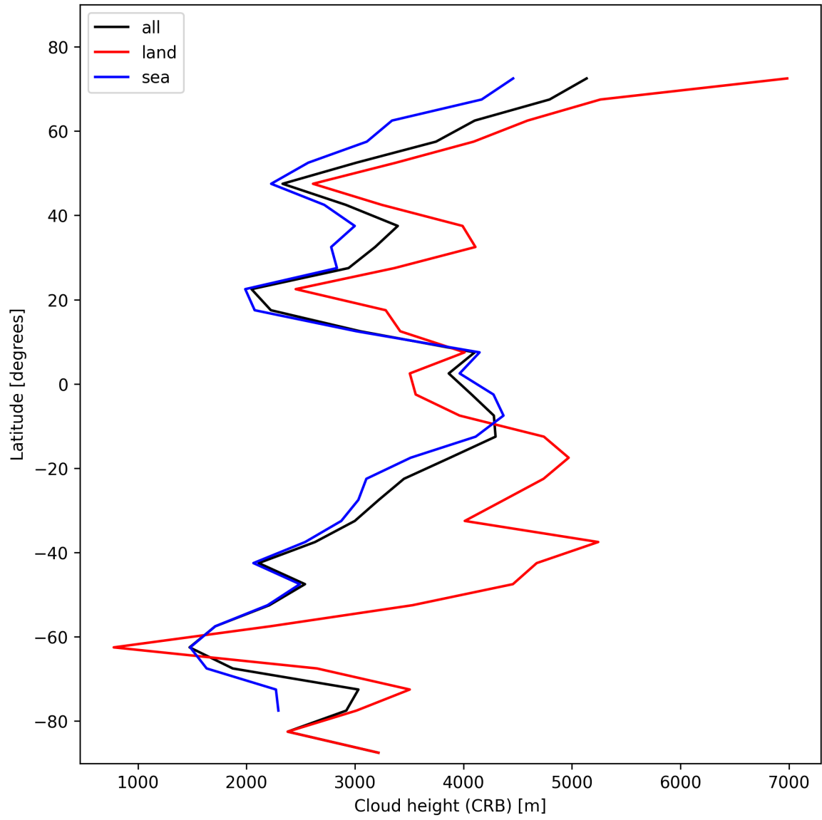
Figure 25: Zonal average of “Cloud height (CRB)” for 2025-01-25 to 2025-01-26.
