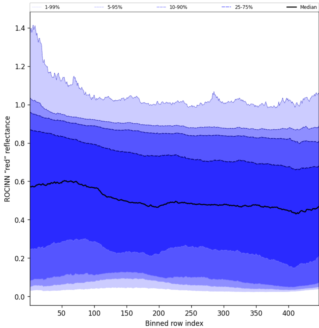
Figure 67: Along track statistics of “ROCINN “red” reflectance” for 2025-01-25 to 2025-01-26
