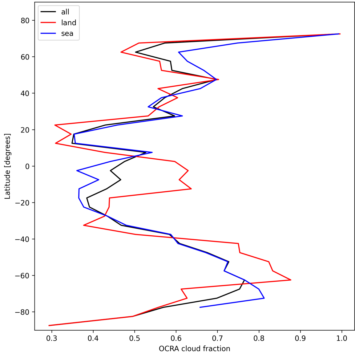
Figure 32: Zonal average of “OCRA cloud fraction” for 2025-01-25 to 2025-01-26.
