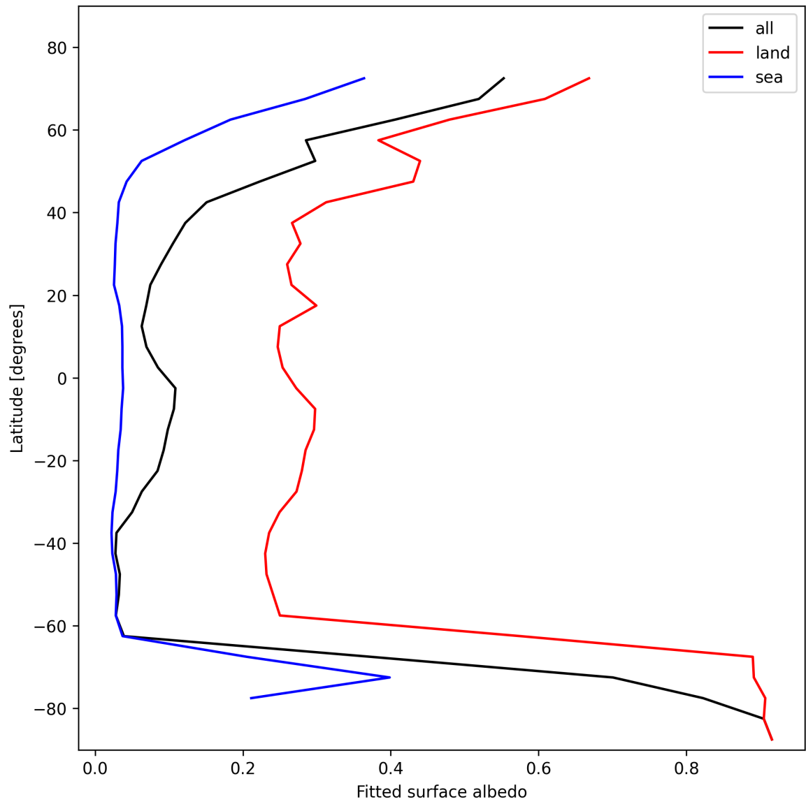
Figure 27: Zonal average of “Fitted surface albedo” for 2025-01-25 to 2025-01-26.
