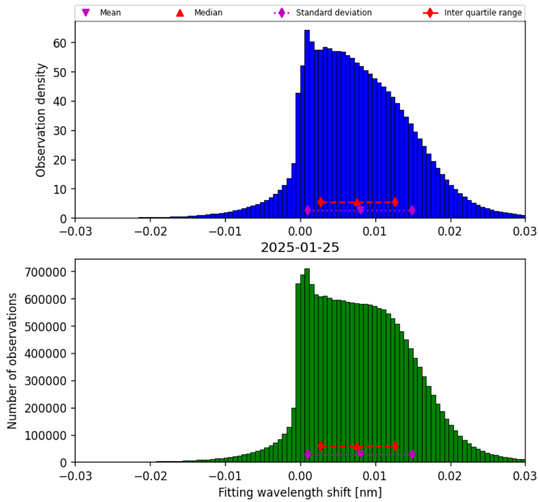
Figure 47: Histogram of “Fitting wavelength shift” for 2025-01-25 to 2025-01-26
