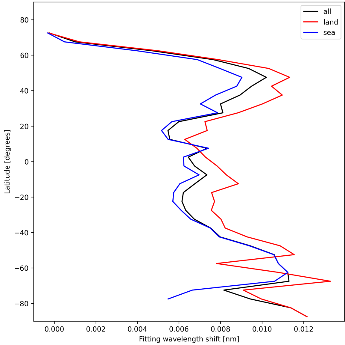
Figure 31: Zonal average of “Fitting wavelength shift” for 2025-01-25 to 2025-01-26.
