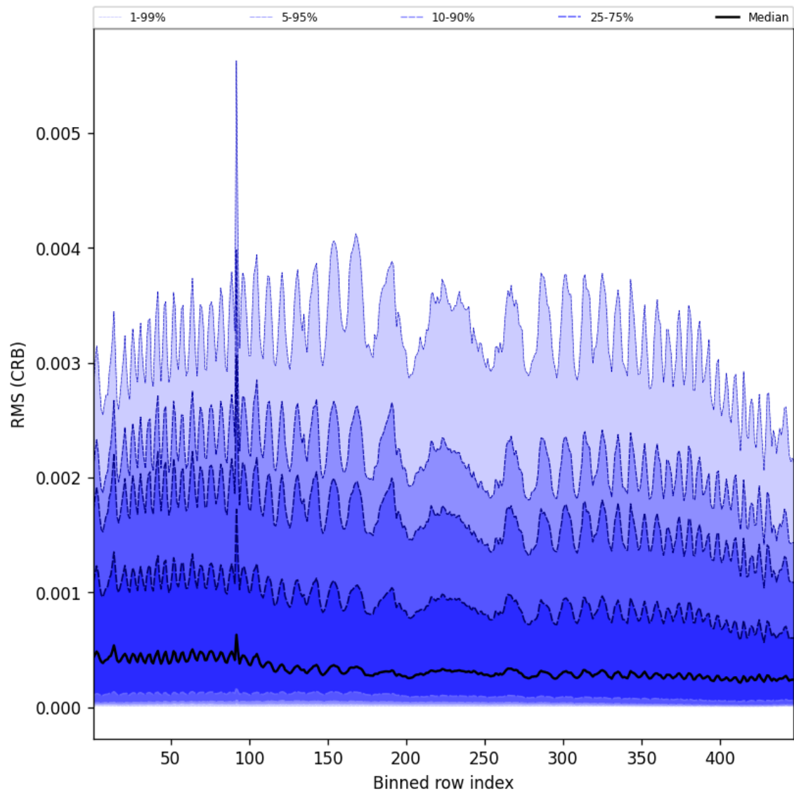
Figure 62: Along track statistics of “RMS (CRB)” for 2025-01-25 to 2025-01-26
