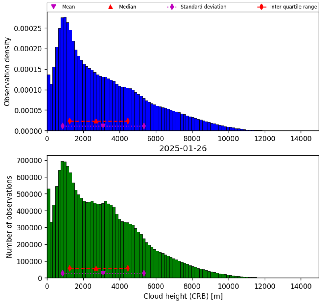
Figure 41: Histogram of “Cloud height (CRB)” for 2025-01-26 to 2025-01-26
