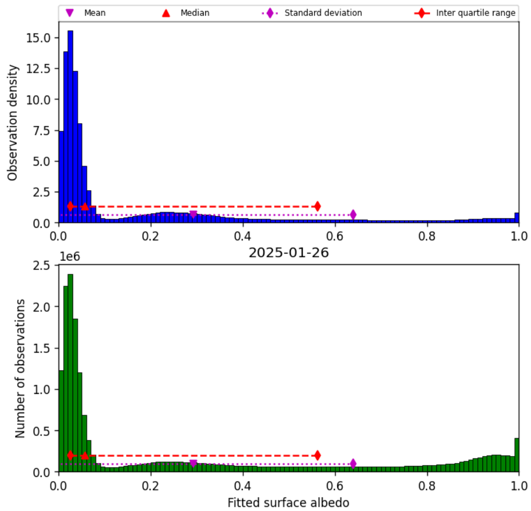
Figure 43: Histogram of “Fitted surface albedo” for 2025-01-26 to 2025-01-26
