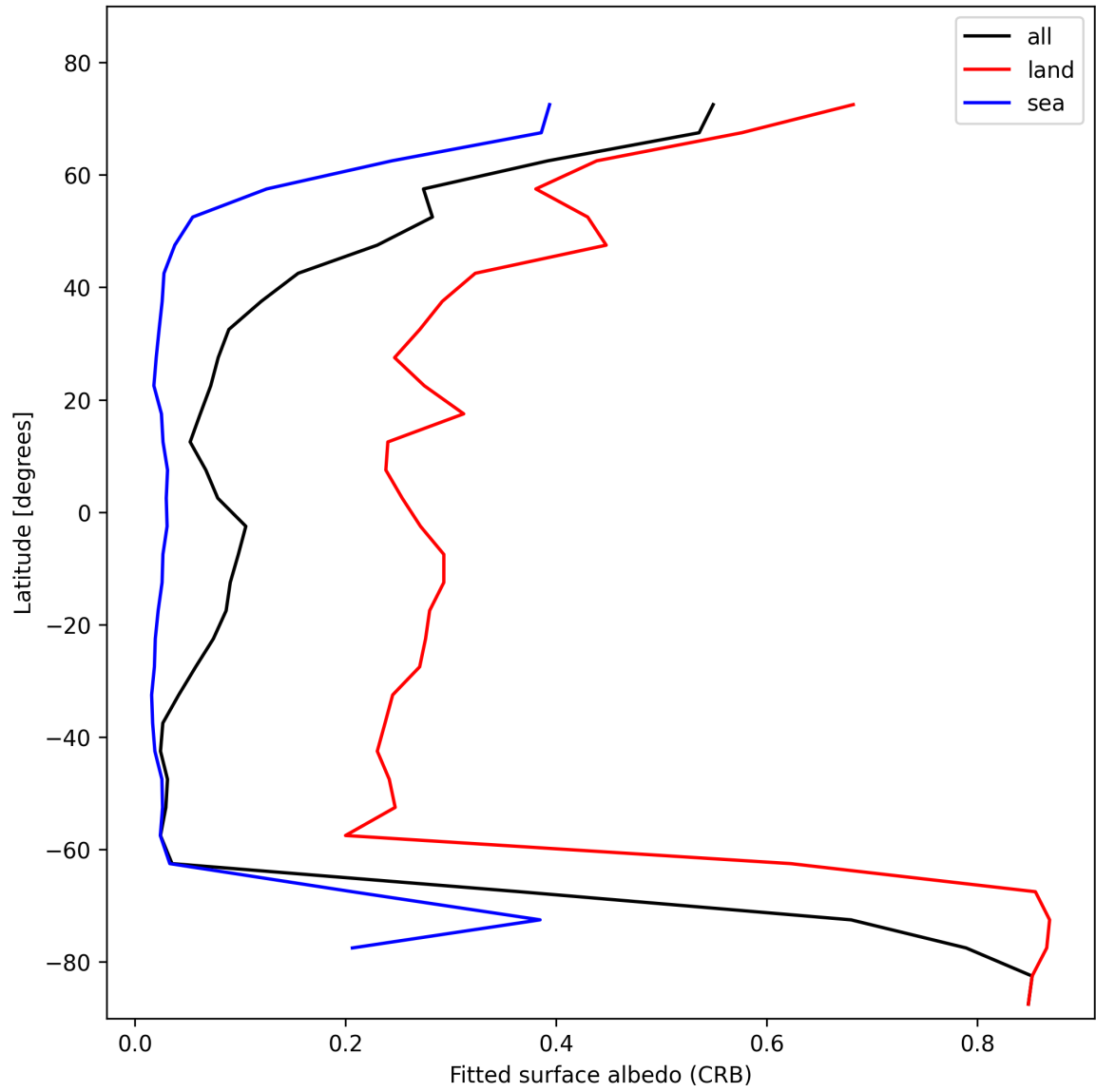
Figure 28: Zonal average of “Fitted surface albedo (CRB)” for 2025-01-26 to 2025-01-26.
