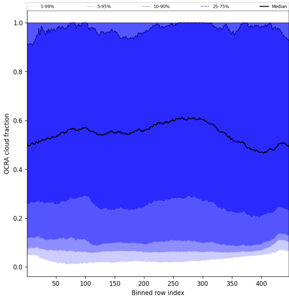
Figure 64: Along track statistics of “OCRA cloud fraction” for 2025-01-26 to 2025-01-26
