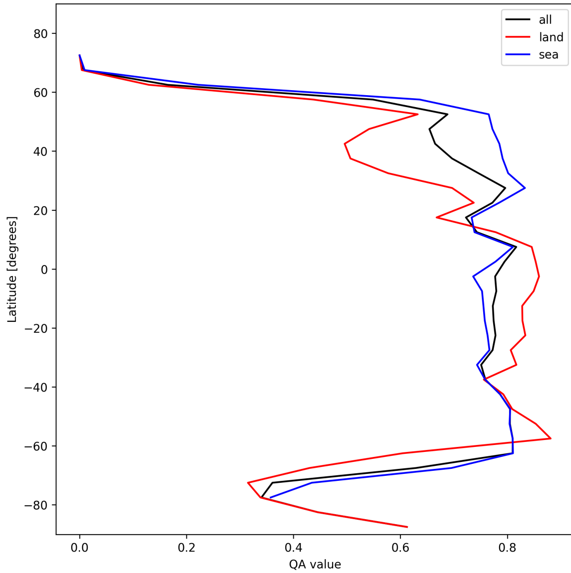
Figure 20: Zonal average of “QA value” for 2025-01-26 to 2025-01-26.
