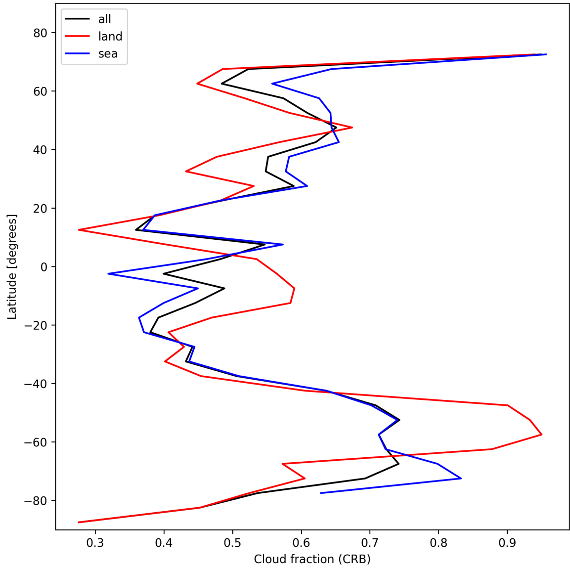
Figure 24: Zonal average of “Cloud fraction (CRB)” for 2025-01-26 to 2025-01-26.
