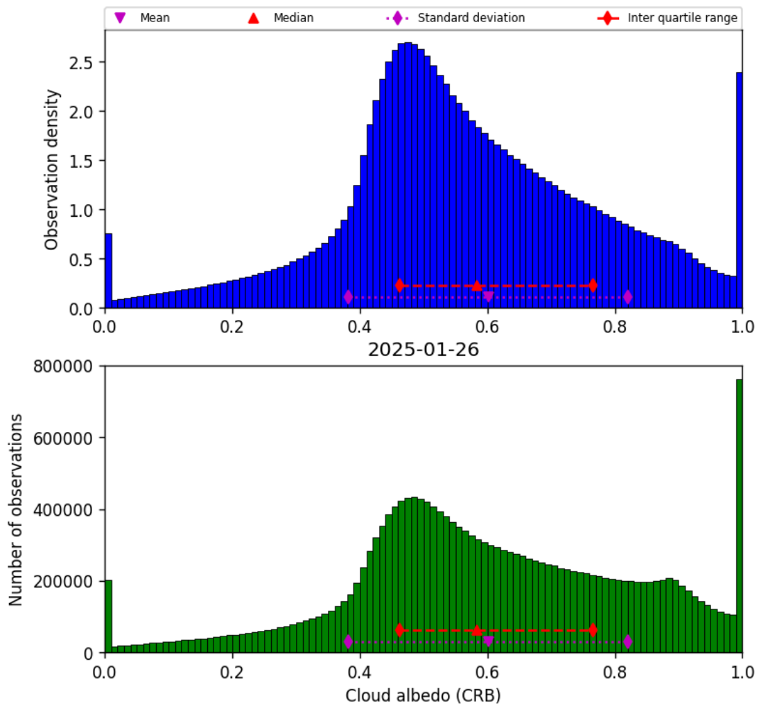
Figure 42: Histogram of “Cloud albedo (CRB)” for 2025-01-26 to 2025-01-26
