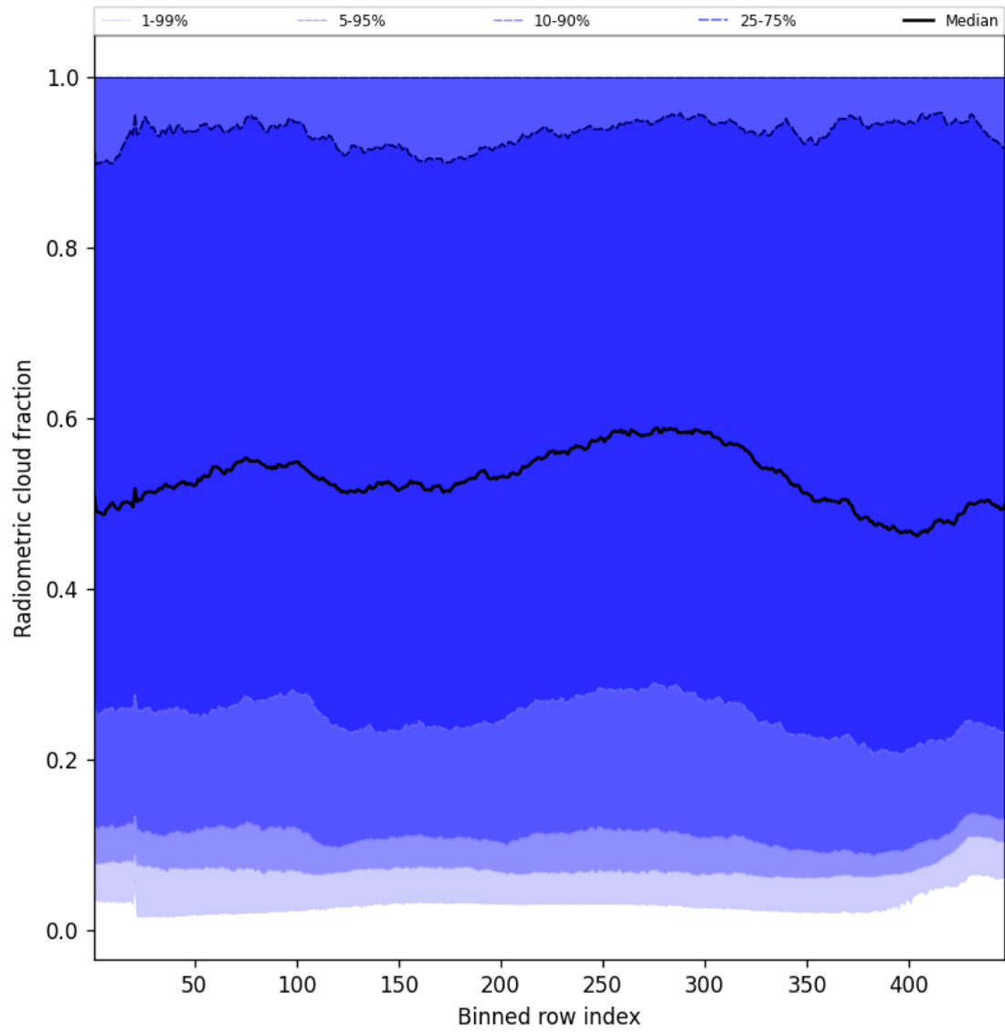
Figure 53: Along track statistics of “Radiometric cloud fraction” for 2025-01-26 to 2025-01-26
