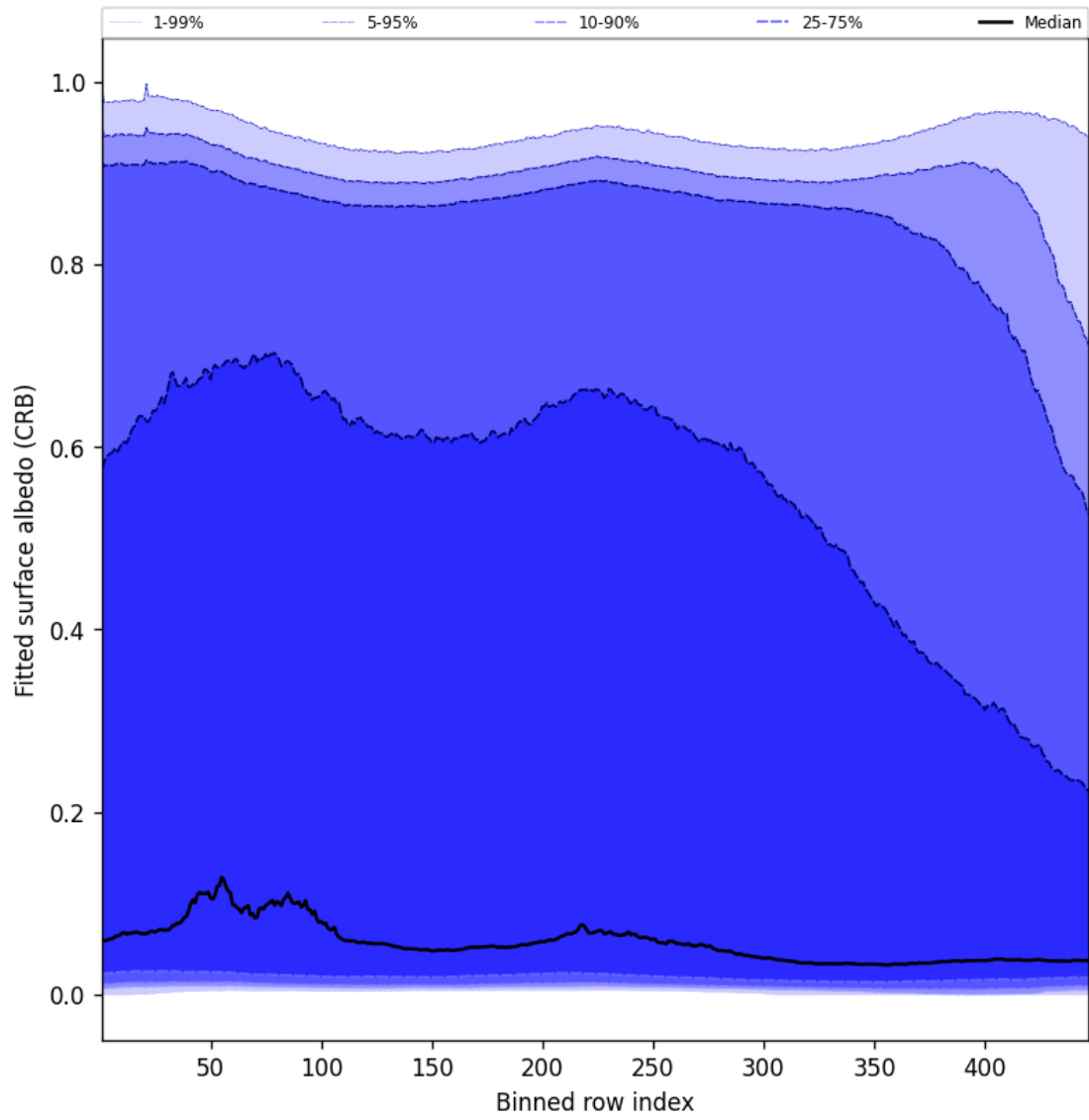
Figure 60: Along track statistics of “Fitted surface albedo (CRB)” for 2025-01-26 to 2025-01-26
