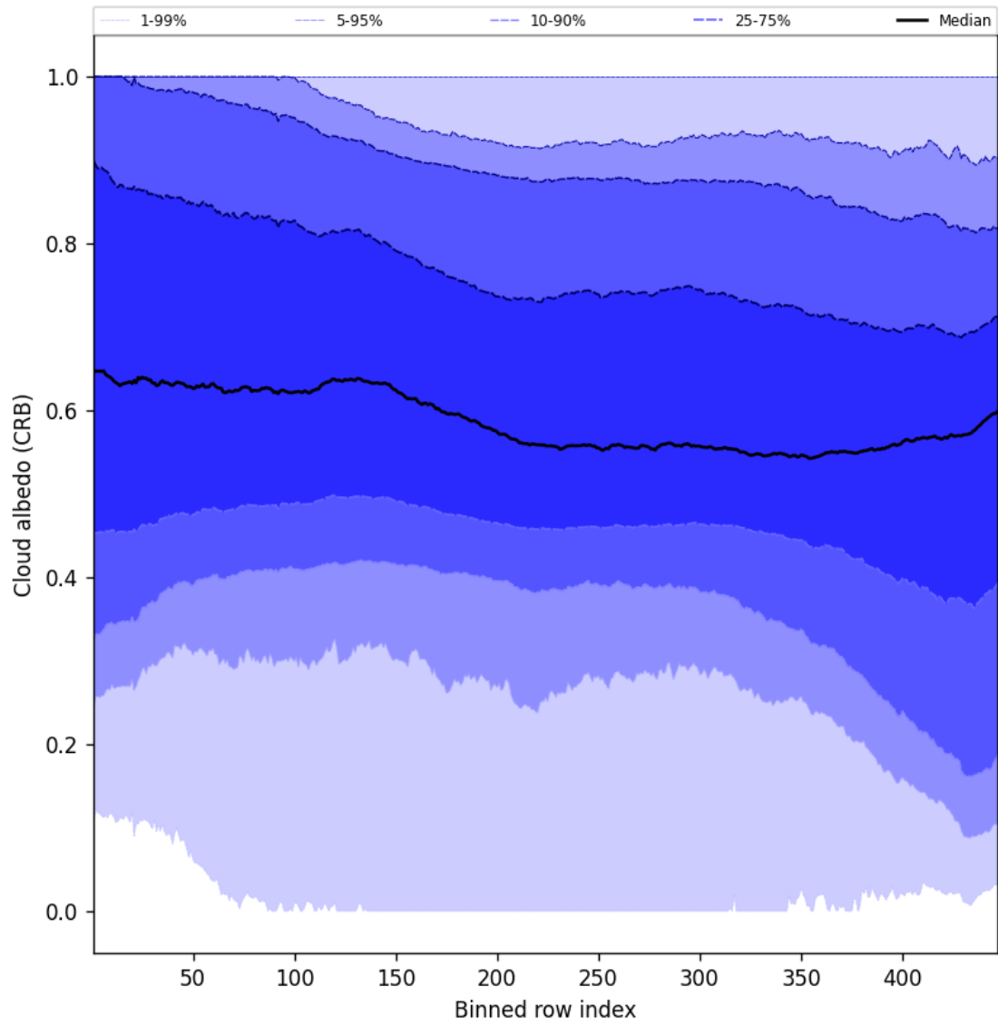
Figure 58: Along track statistics of “Cloud albedo (CRB)” for 2025-01-26 to 2025-01-26
