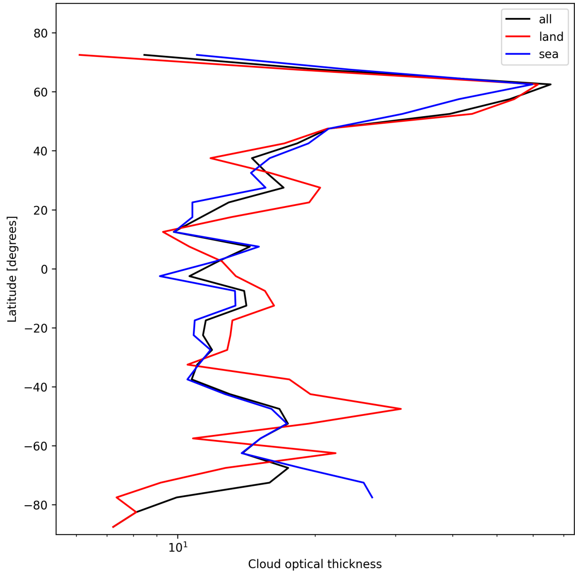
Figure 23: Zonal average of “Cloud optical thickness” for 2025-01-26 to 2025-01-26.
