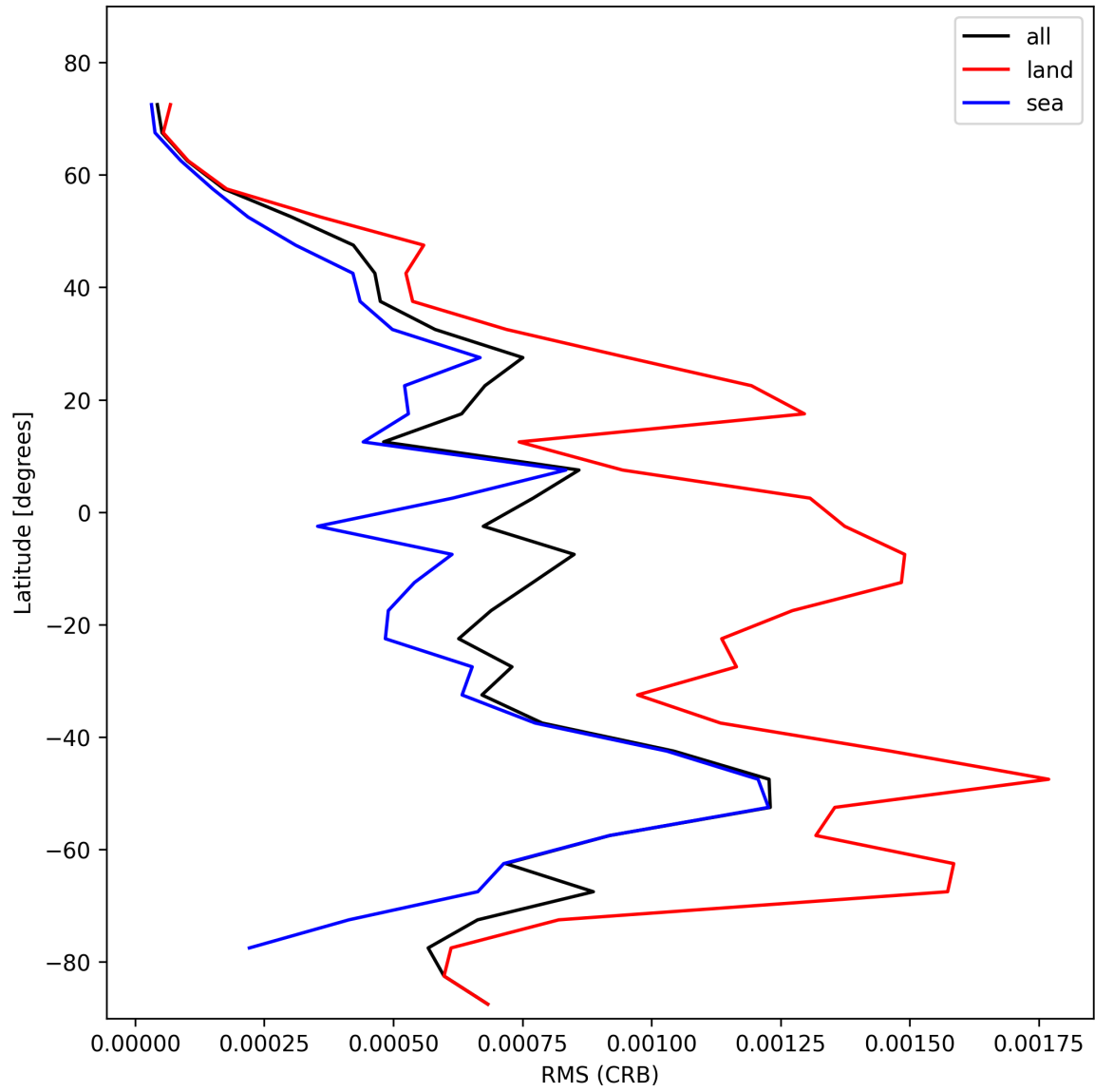
Figure 30: Zonal average of “RMS (CRB)” for 2025-01-26 to 2025-01-26.
