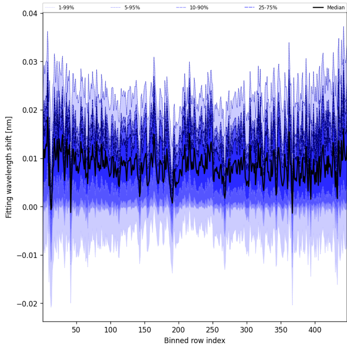
Figure 63: Along track statistics of “Fitting wavelength shift” for 2025-01-26 to 2025-01-26
