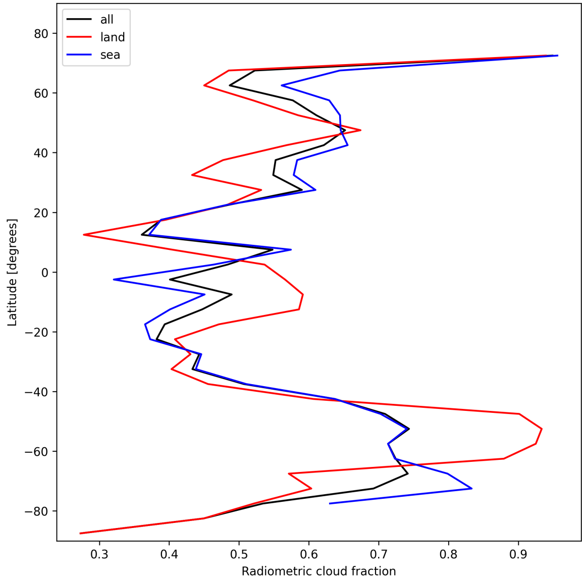
Figure 21: Zonal average of “Radiometric cloud fraction” for 2025-01-26 to 2025-01-26.
