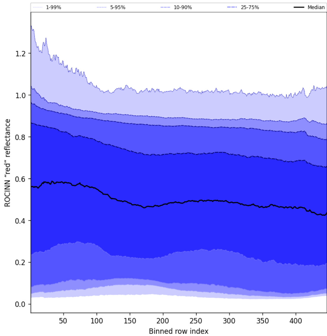
Figure 67: Along track statistics of “ROCINN “red” reflectance” for 2025-01-26 to 2025-01-26
