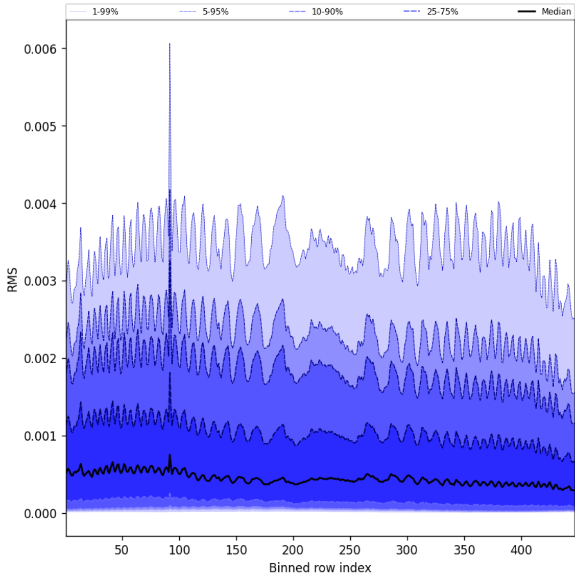
Figure 61: Along track statistics of “RMS” for 2025-01-26 to 2025-01-26
