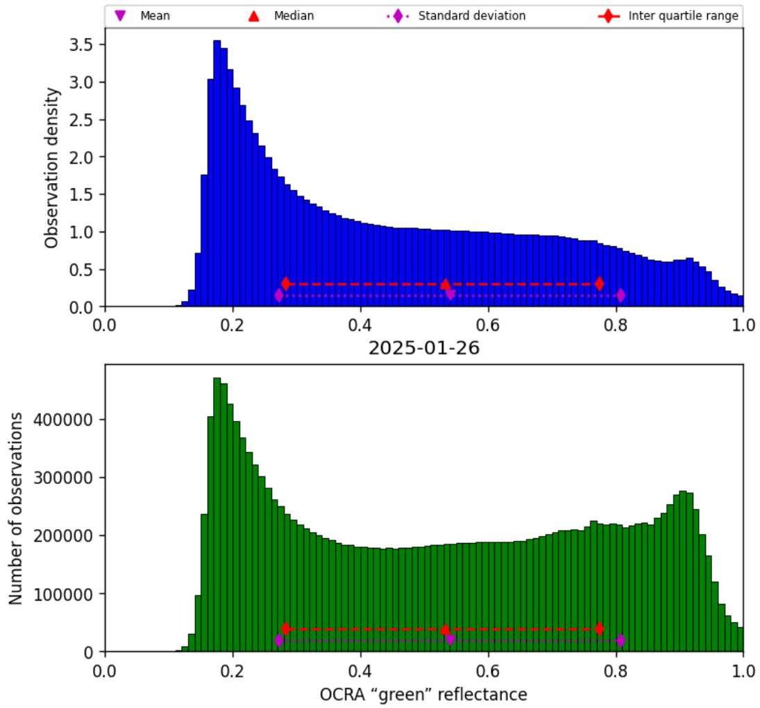
Figure 50: Histogram of “OCRA “green” reflectance” for 2025-01-26 to 2025-01-26
