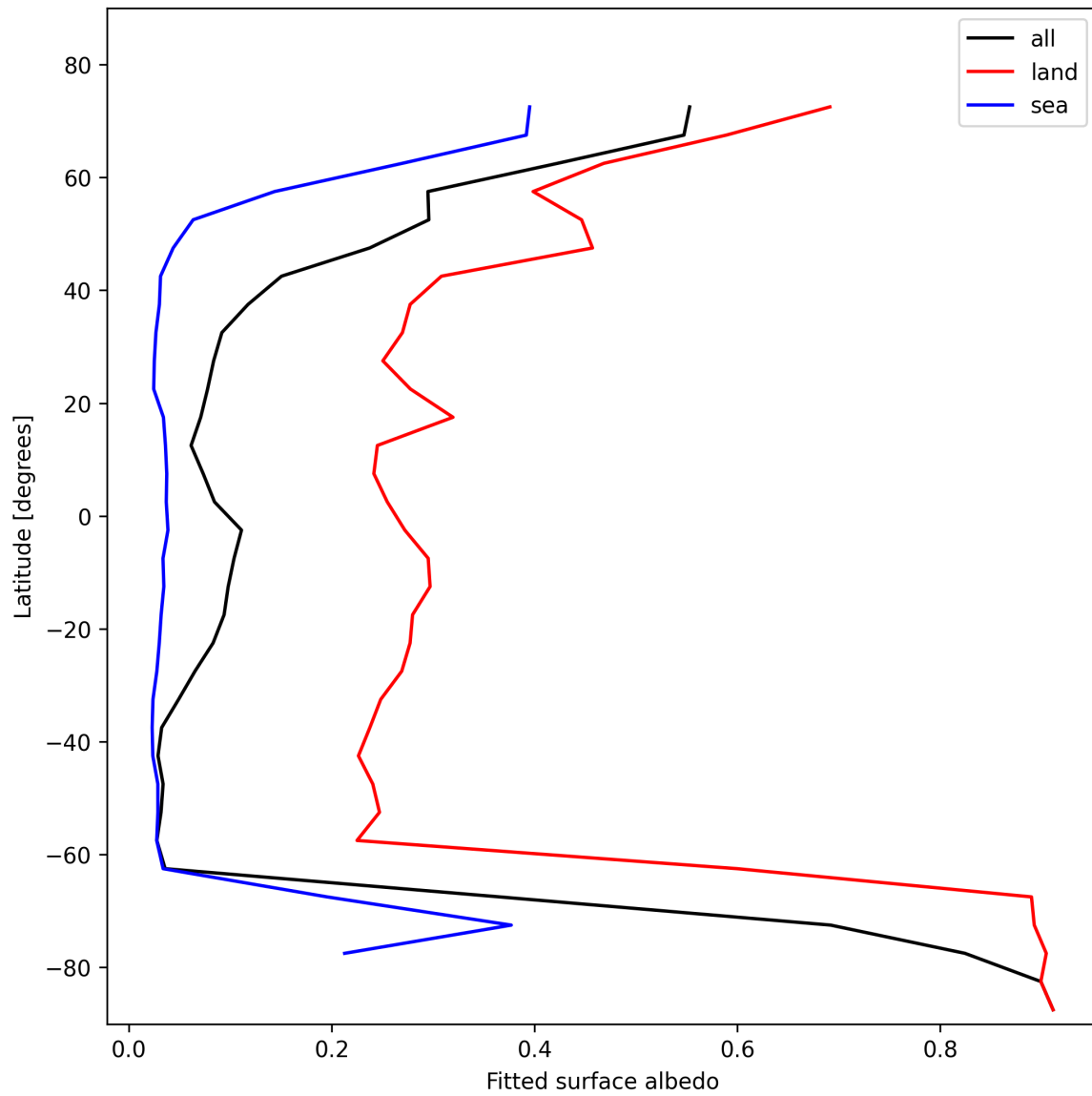
Figure 27: Zonal average of “Fitted surface albedo” for 2025-01-26 to 2025-01-26.
