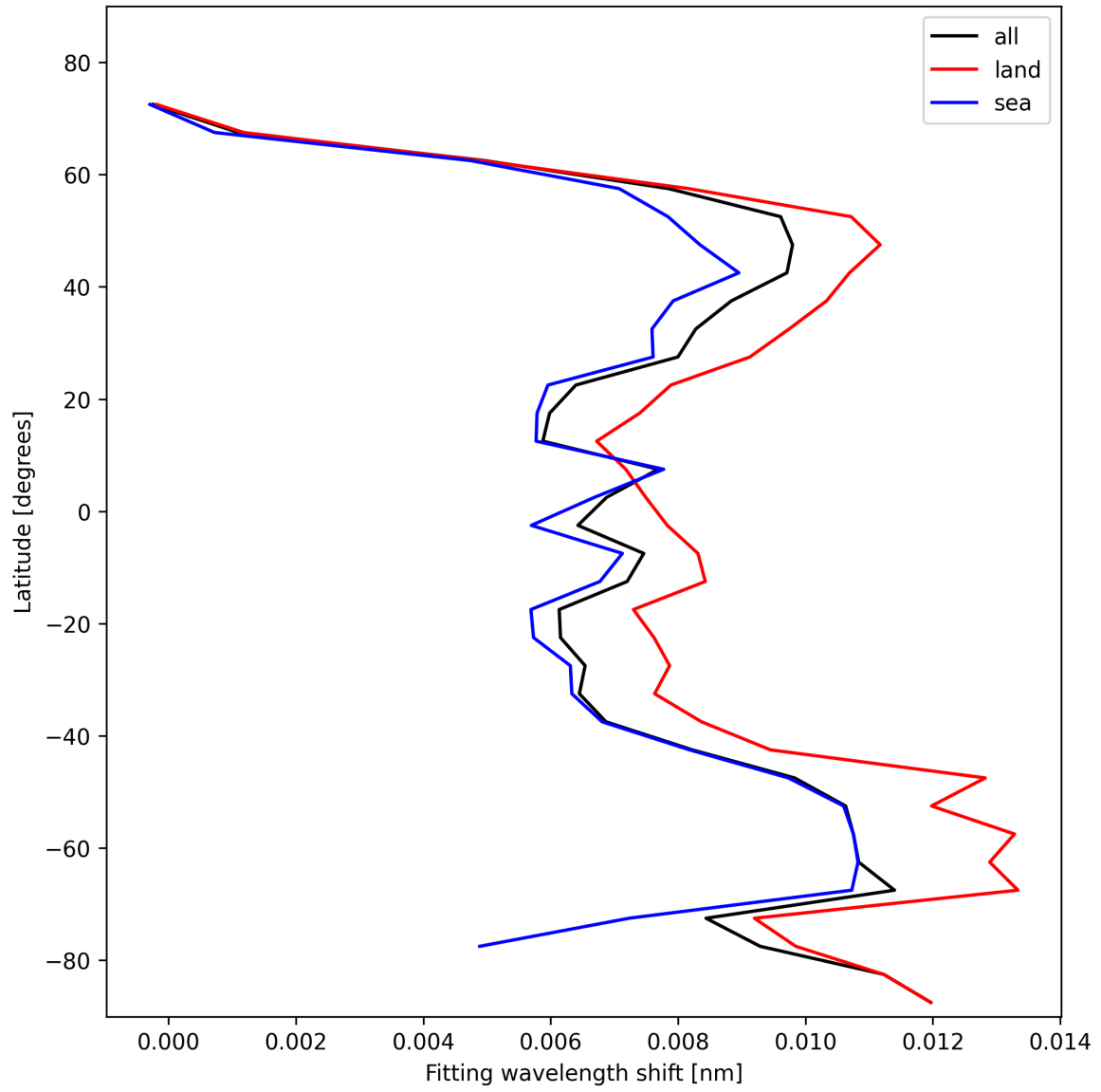
Figure 31: Zonal average of “Fitting wavelength shift” for 2025-01-26 to 2025-01-26.
