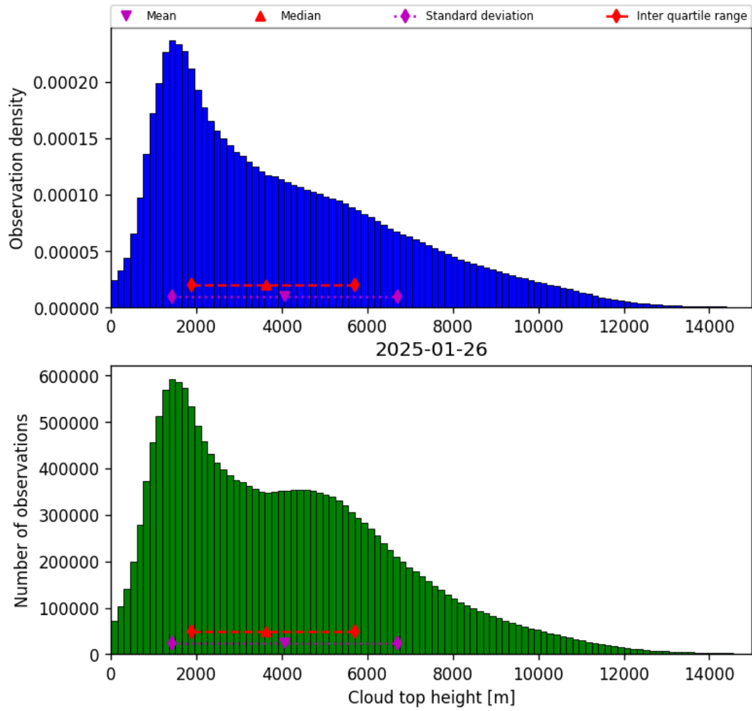
Figure 38: Histogram of “Cloud top height” for 2025-01-26 to 2025-01-26
