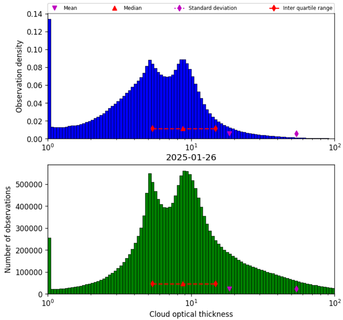
Figure 39: Histogram of “Cloud optical thickness” for 2025-01-26 to 2025-01-26
