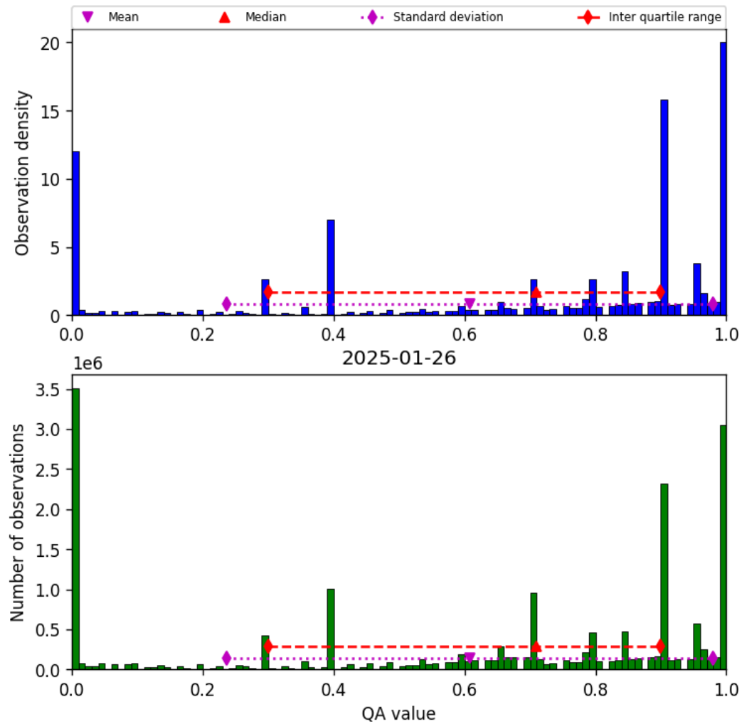
Figure 36: Histogram of “QA value” for 2025-01-26 to 2025-01-26
