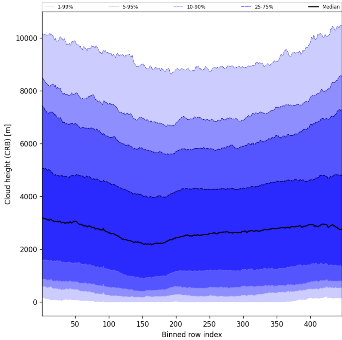
Figure 57: Along track statistics of “Cloud height (CRB)” for 2025-01-26 to 2025-01-26
