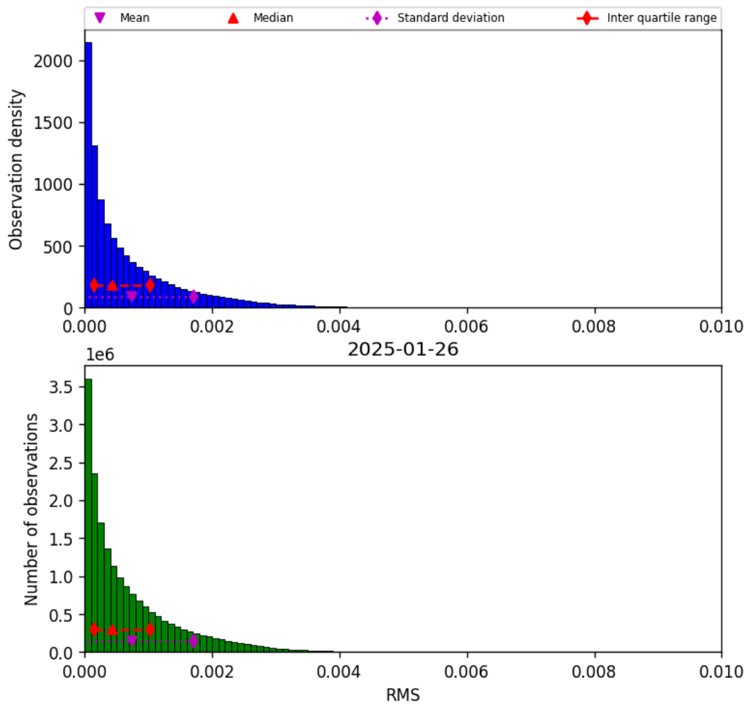
Figure 45: Histogram of “RMS” for 2025-01-26 to 2025-01-26
