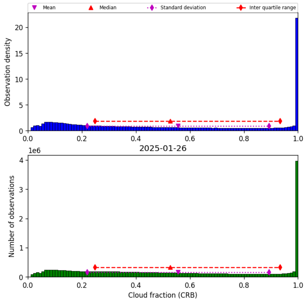
Figure 40: Histogram of “Cloud fraction (CRB)” for 2025-01-26 to 2025-01-26
