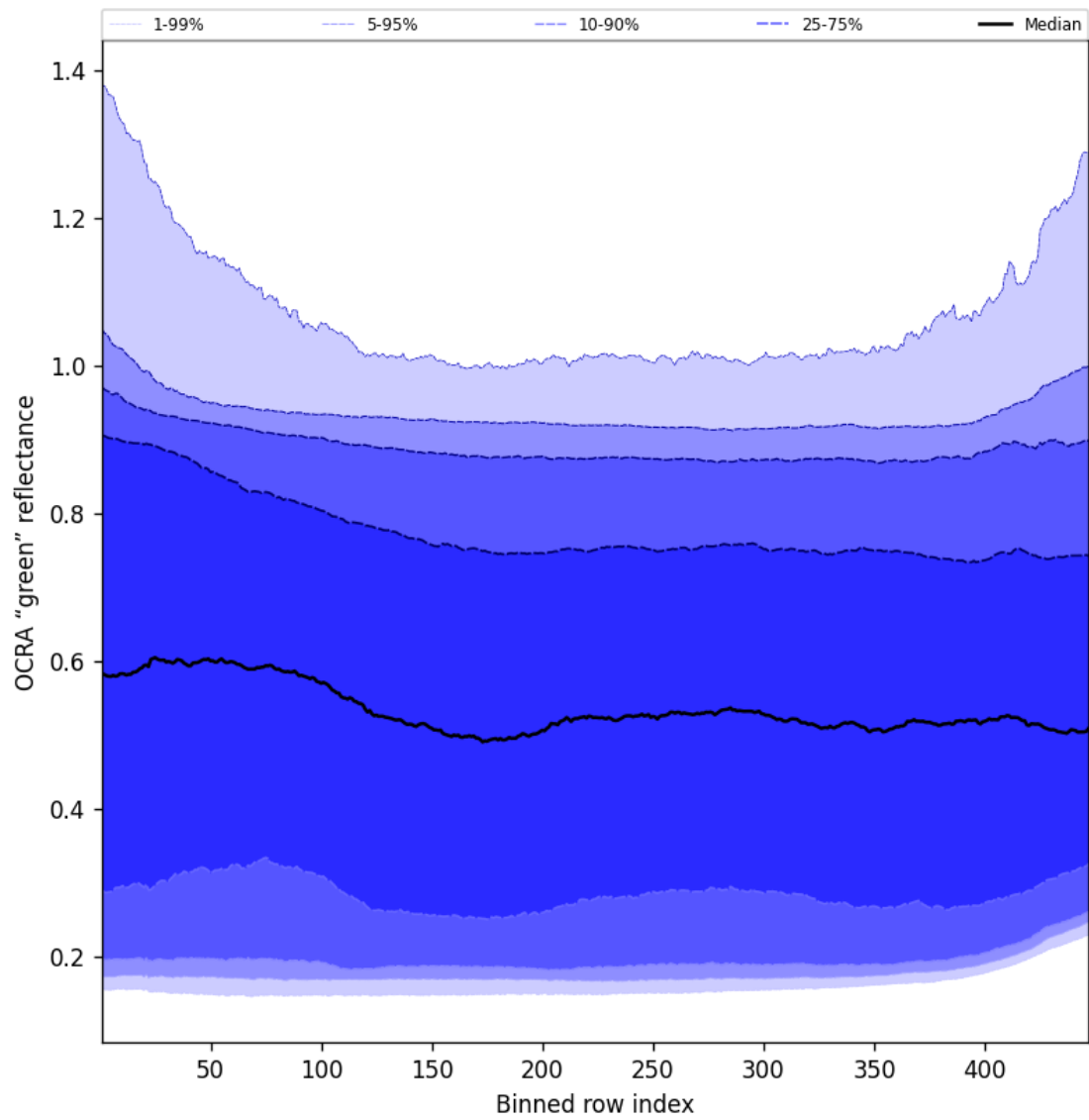
Figure 66: Along track statistics of "OCRA "green" reflectance" for 2025-01-26 to 2025-01-26
