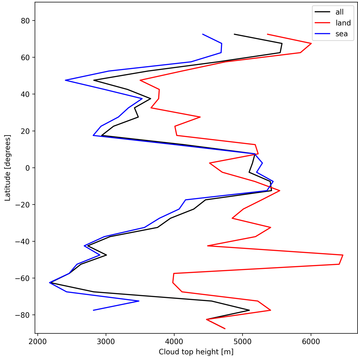
Figure 22: Zonal average of “Cloud top height” for 2025-01-26 to 2025-01-26.
