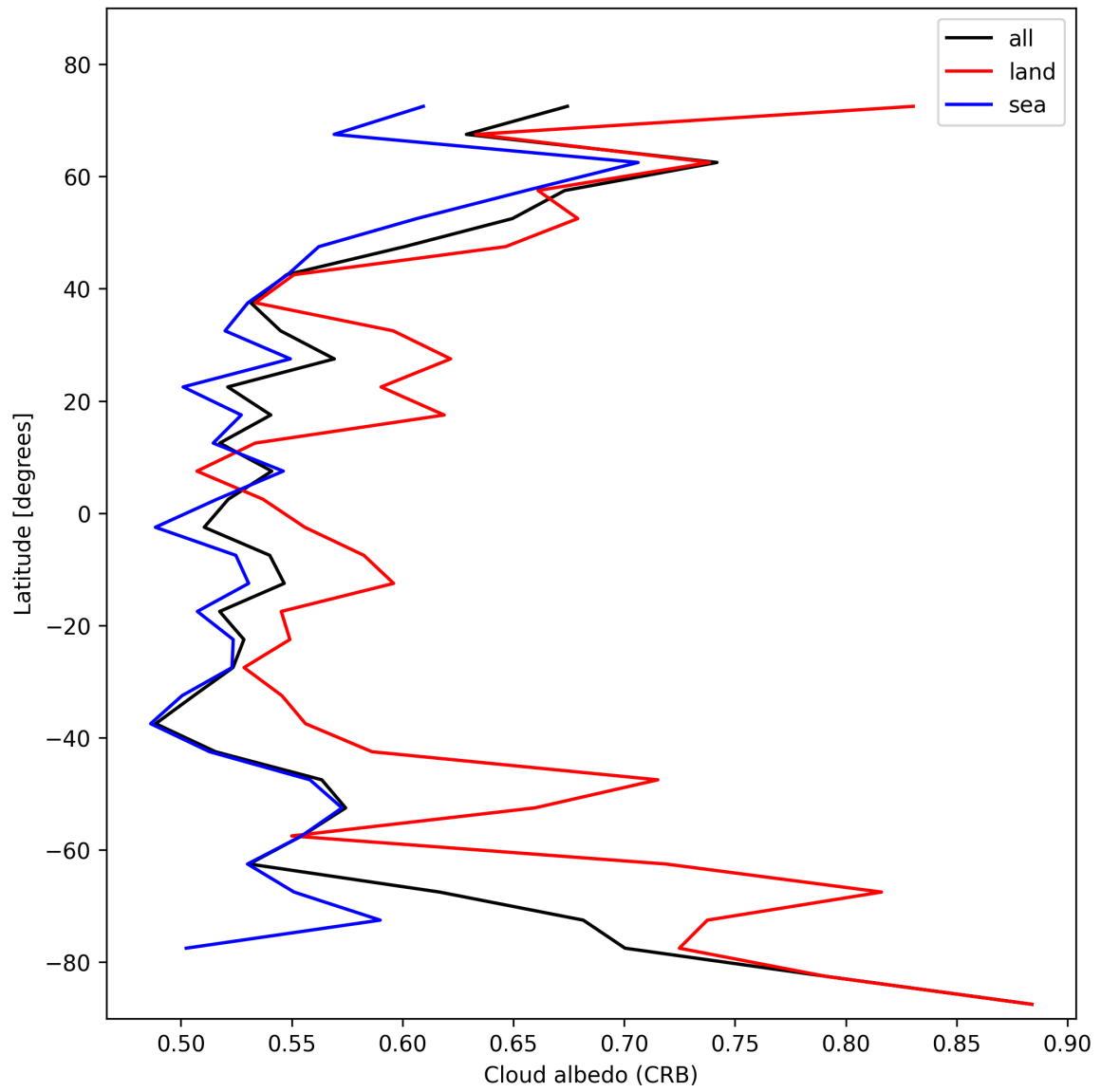
Figure 26: Zonal average of “Cloud albedo (CRB)” for 2025-01-26 to 2025-01-26.
