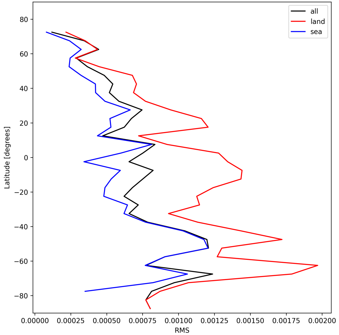
Figure 29: Zonal average of “RMS” for 2025-01-26 to 2025-01-26.
