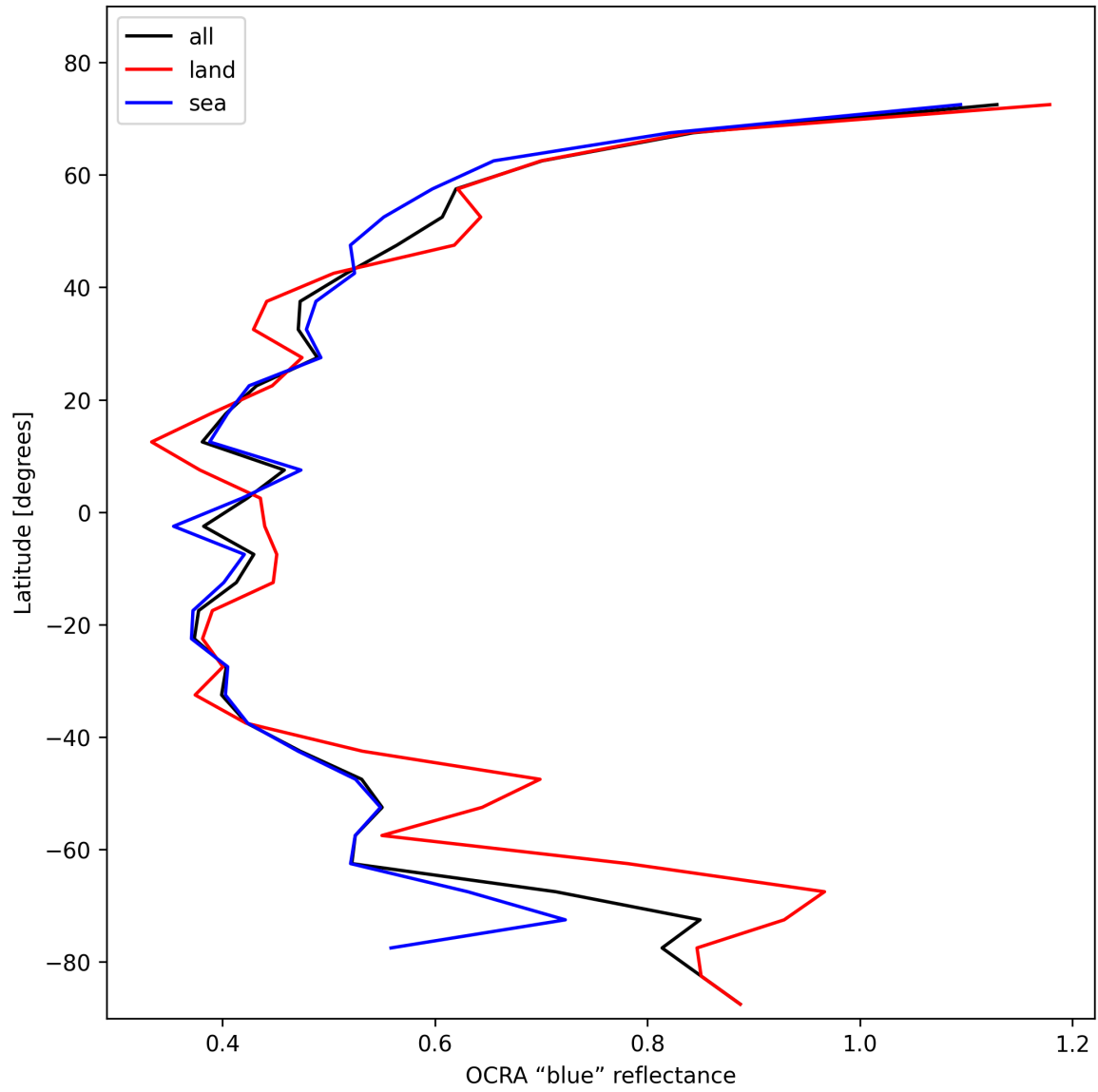
Figure 33: Zonal average of “OCRA “blue” reflectance” for 2025-01-26 to 2025-01-26.
