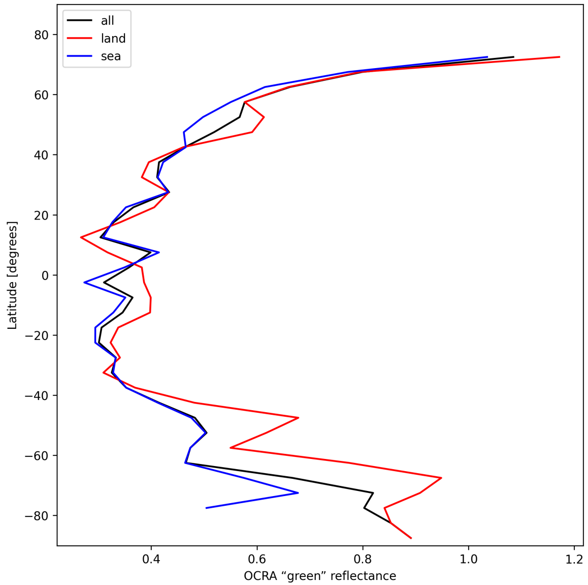
Figure 34: Zonal average of “OCRA “green” reflectance” for 2025-01-26 to 2025-01-26.
