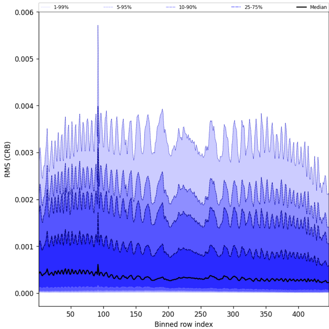
Figure 62: Along track statistics of “RMS (CRB)” for 2025-01-26 to 2025-01-26
