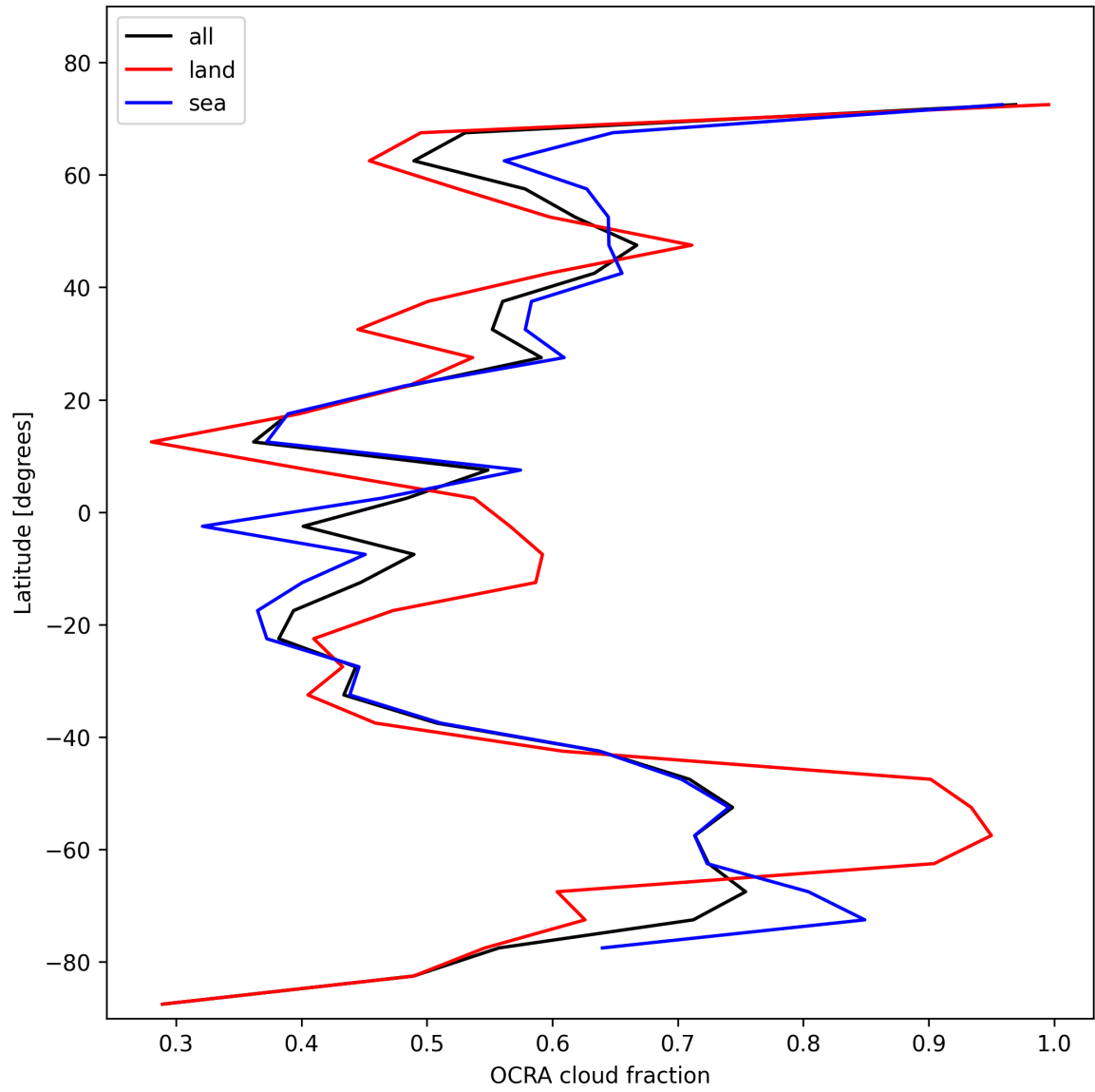
Figure 32: Zonal average of “OCRA cloud fraction” for 2025-01-26 to 2025-01-26.
