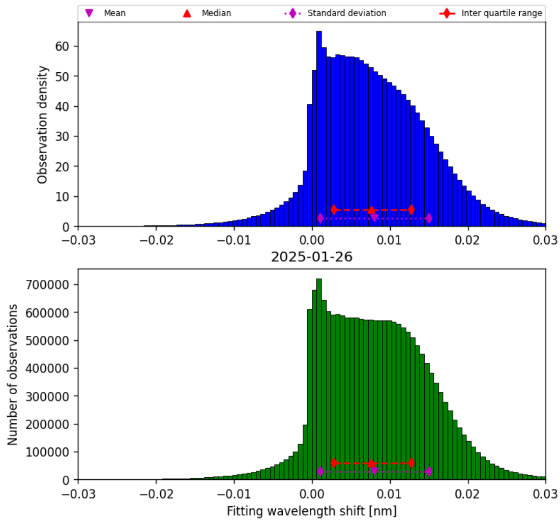
Figure 47: Histogram of “Fitting wavelength shift” for 2025-01-26 to 2025-01-26
