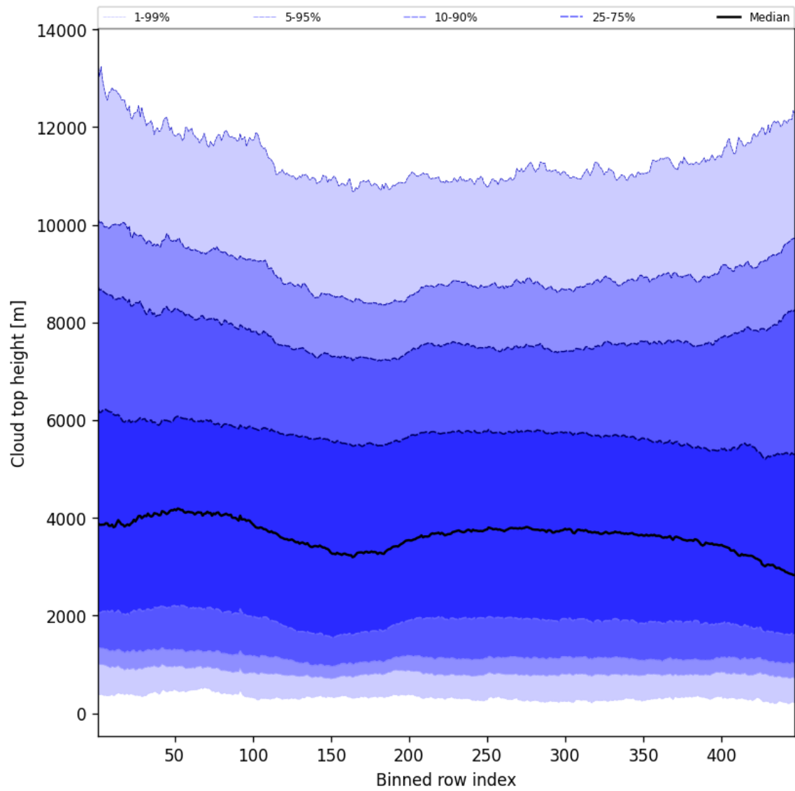
Figure 54: Along track statistics of “Cloud top height” for 2025-01-26 to 2025-01-26
