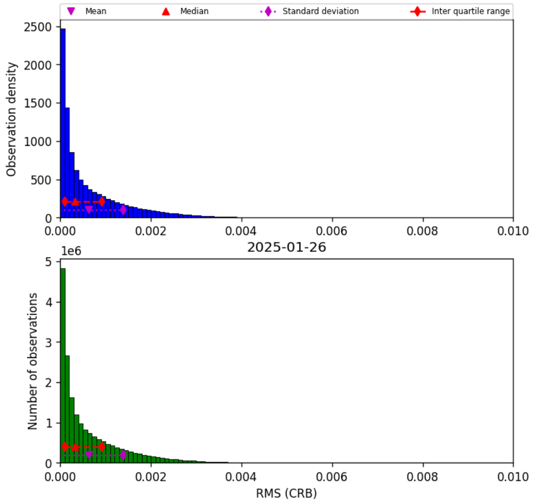
Figure 46: Histogram of “RMS (CRB)” for 2025-01-26 to 2025-01-26
