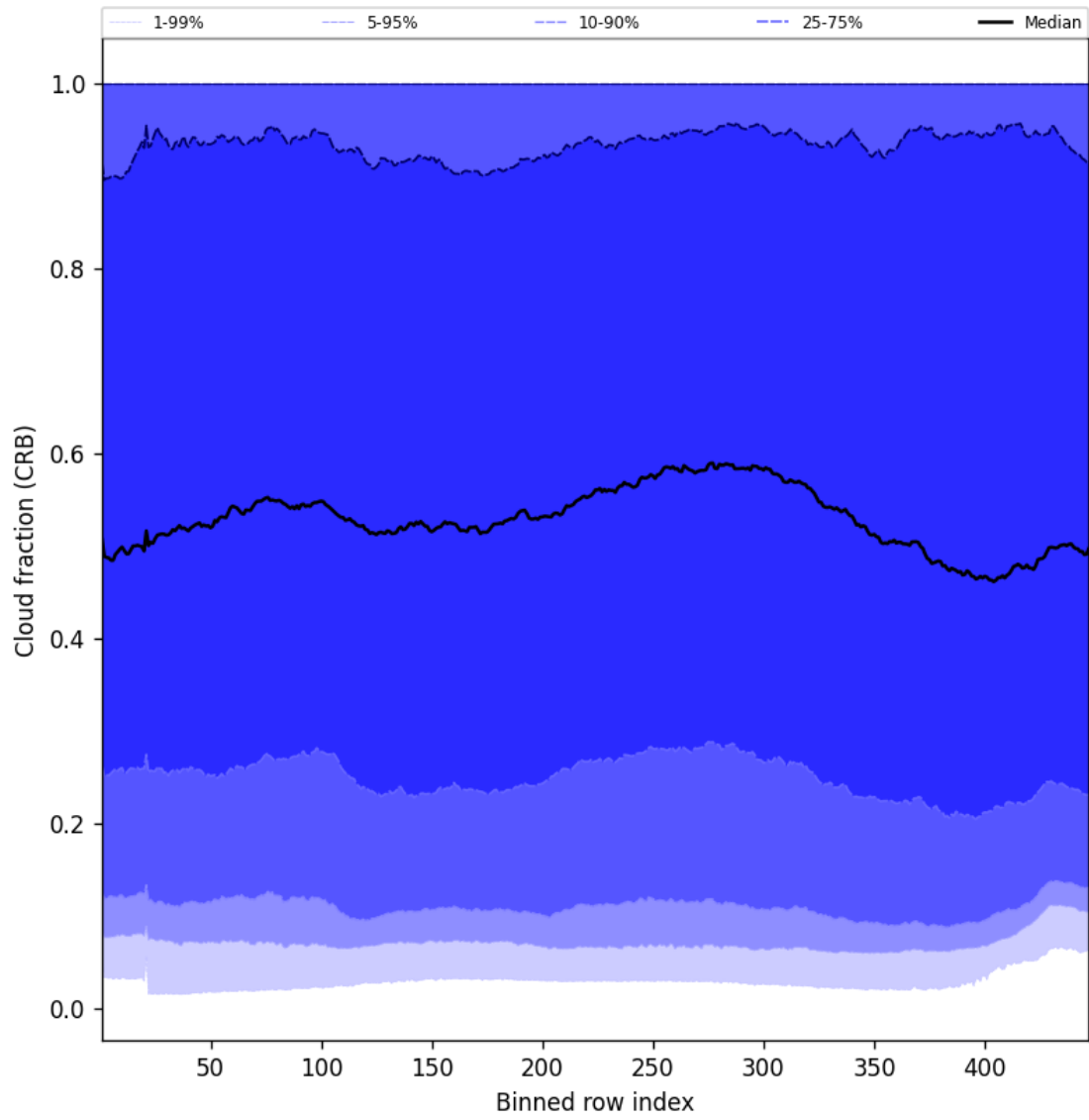
Figure 56: Along track statistics of “Cloud fraction (CRB)” for 2025-01-26 to 2025-01-26
