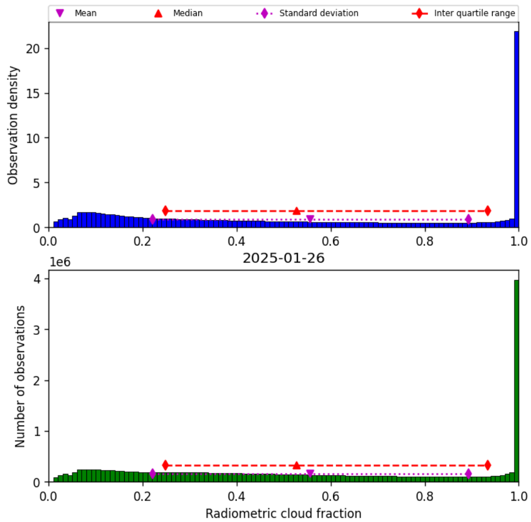
Figure 37: Histogram of “Radiometric cloud fraction” for 2025-01-26 to 2025-01-26
