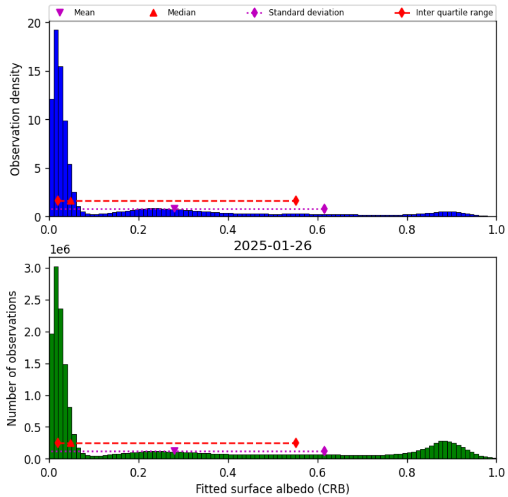
Figure 44: Histogram of “Fitted surface albedo (CRB)” for 2025-01-26 to 2025-01-26
