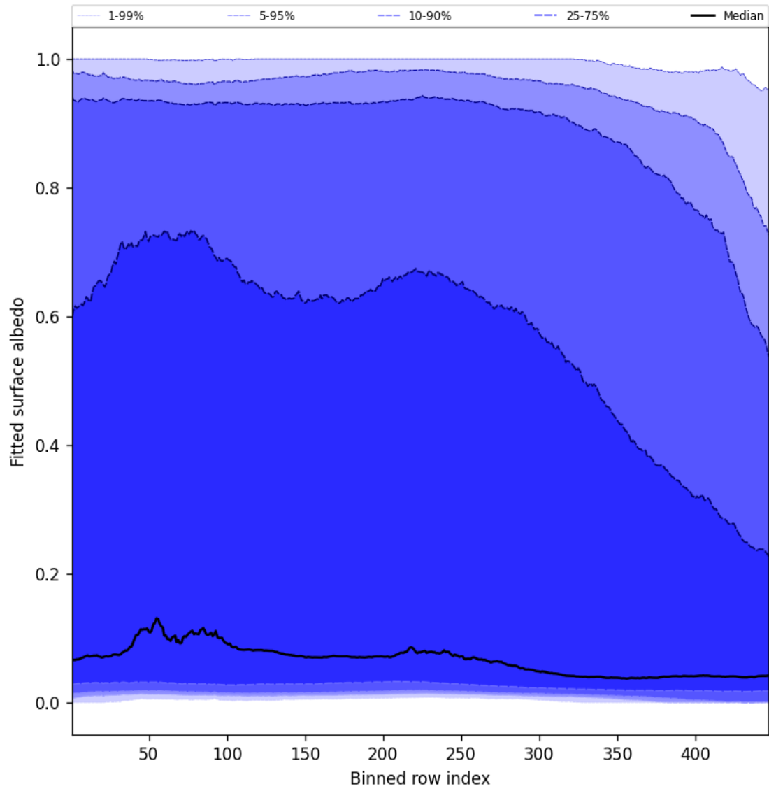
Figure 59: Along track statistics of “Fitted surface albedo” for 2025-01-26 to 2025-01-26
