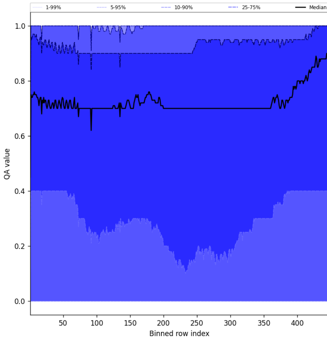
Figure 52: Along track statistics of “QA value” for 2025-01-26 to 2025-01-26
