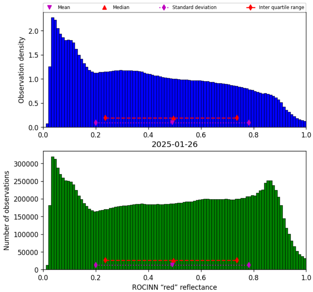
Figure 51: Histogram of “ROCINN “red” reflectance” for 2025-01-26 to 2025-01-26
