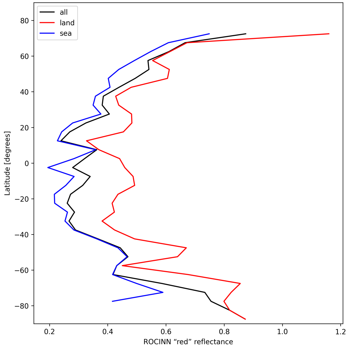
Figure 35: Zonal average of “ROCINN “red” reflectance” for 2025-01-26 to 2025-01-26.
