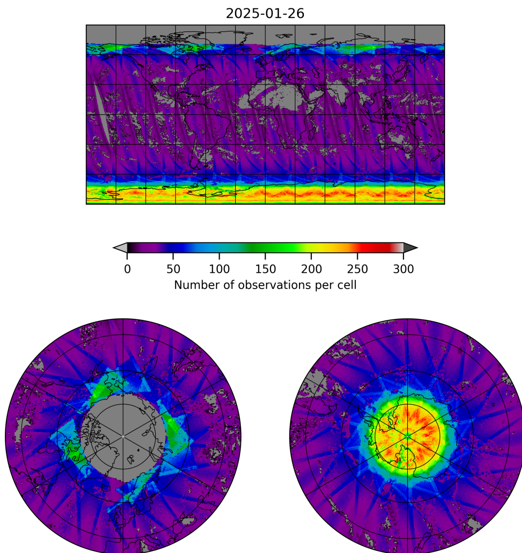
Figure 19: Map of the number of observations for 2025-01-26 to 2025-01-26
