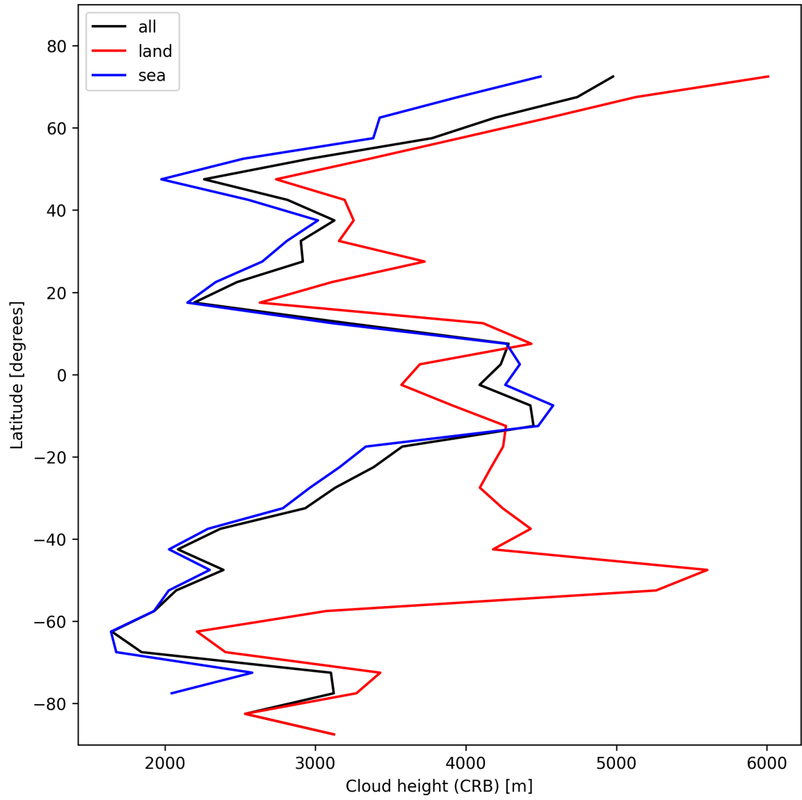
Figure 25: Zonal average of “Cloud height (CRB)” for 2025-01-26 to 2025-01-26.
