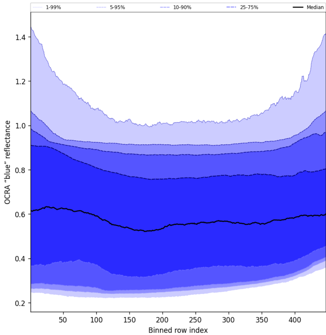
Figure 65: Along track statistics of “OCRA “blue” reflectance” for 2025-01-26 to 2025-01-26
