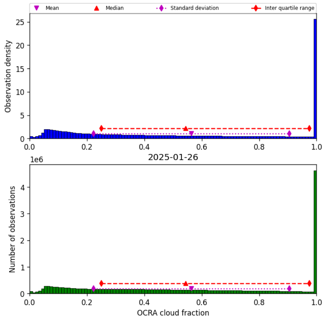
Figure 48: Histogram of “OCRA cloud fraction” for 2025-01-26 to 2025-01-26
