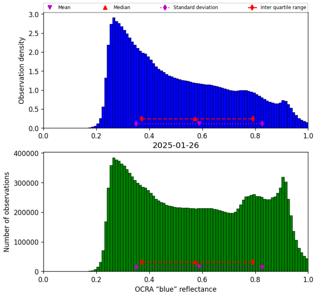
Figure 49: Histogram of “OCRA “blue” reflectance” for 2025-01-26 to 2025-01-26
