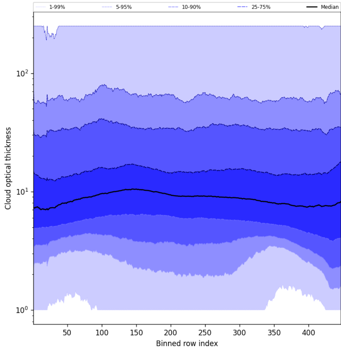
Figure 55: Along track statistics of “Cloud optical thickness” for 2025-01-26 to 2025-01-26
