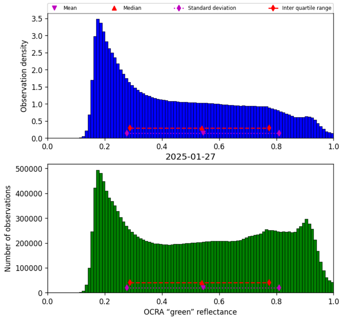
Figure 50: Histogram of “OCRA “green” reflectance” for 2025-01-27 to 2025-01-28
