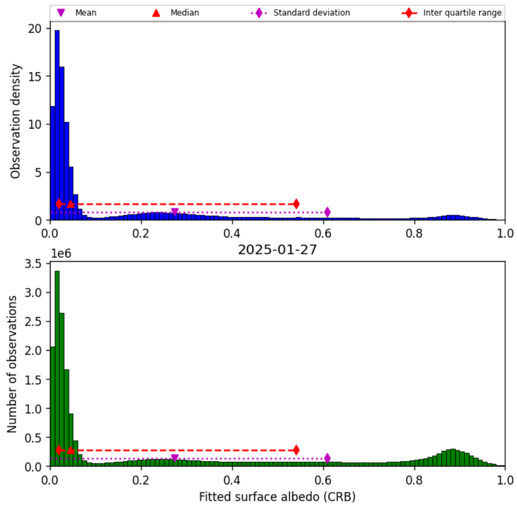
Figure 44: Histogram of “Fitted surface albedo (CRB)” for 2025-01-27 to 2025-01-28
