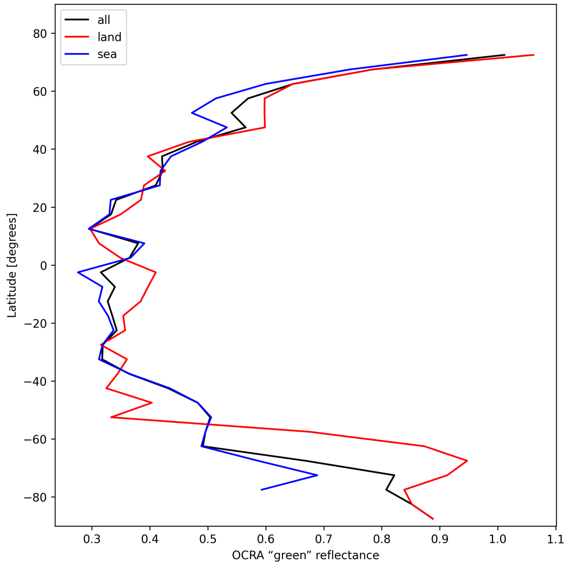
Figure 34: Zonal average of “OCRA “green” reflectance” for 2025-01-27 to 2025-01-28.
