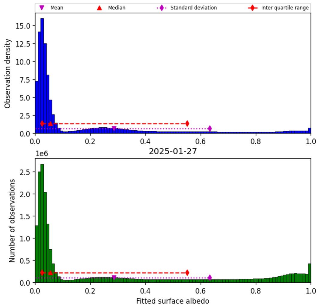
Figure 43: Histogram of “Fitted surface albedo” for 2025-01-27 to 2025-01-28
