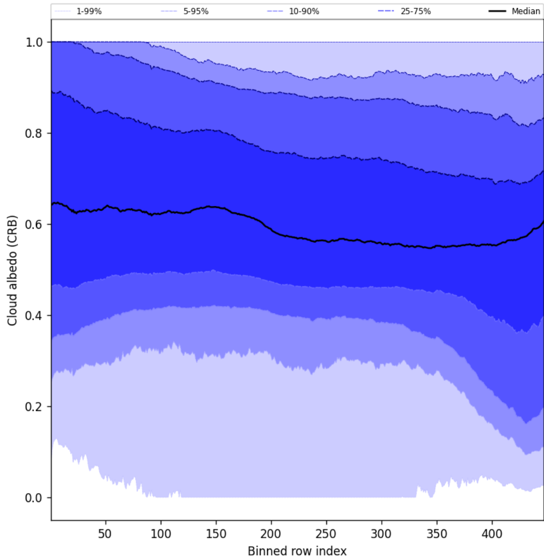
Figure 58: Along track statistics of “Cloud albedo (CRB)” for 2025-01-27 to 2025-01-28
