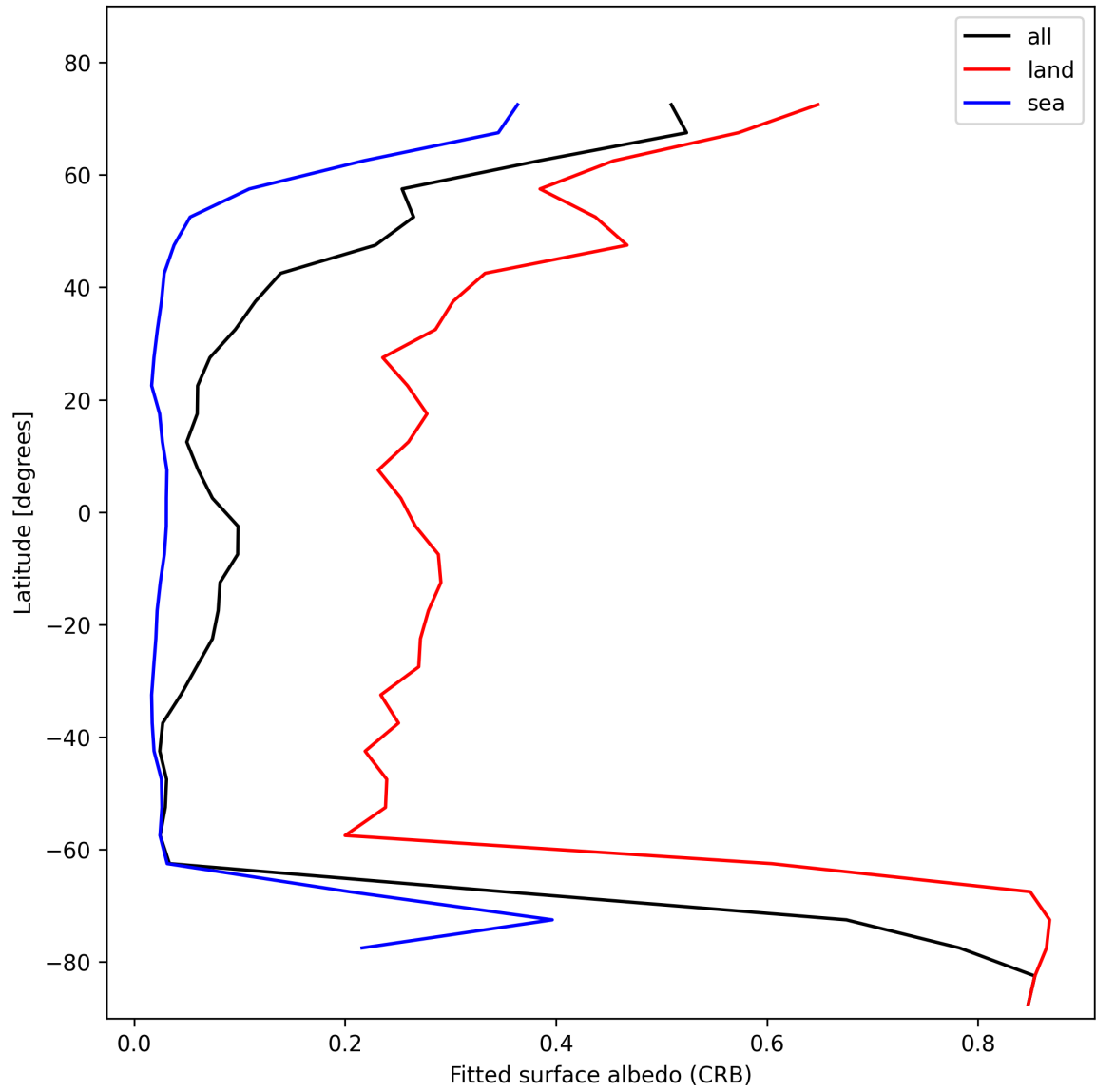
Figure 28: Zonal average of “Fitted surface albedo (CRB)” for 2025-01-27 to 2025-01-28.
