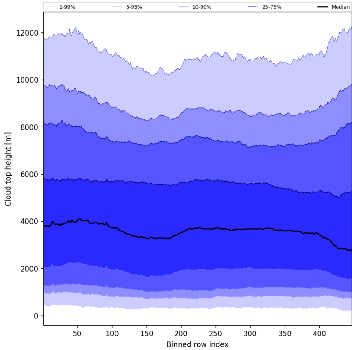
Figure 54: Along track statistics of “Cloud top height” for 2025-01-27 to 2025-01-28
