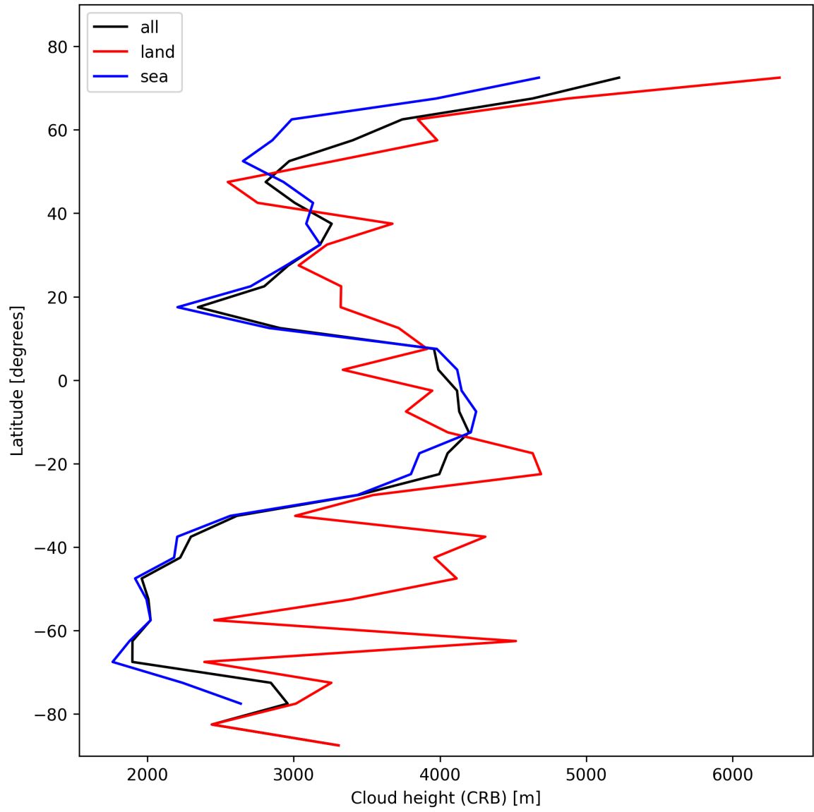
Figure 25: Zonal average of “Cloud height (CRB)” for 2025-01-27 to 2025-01-28.
