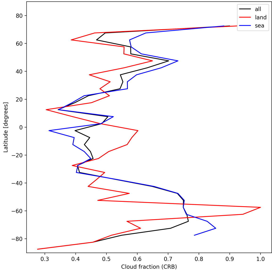
Figure 24: Zonal average of “Cloud fraction (CRB)” for 2025-01-27 to 2025-01-28.
