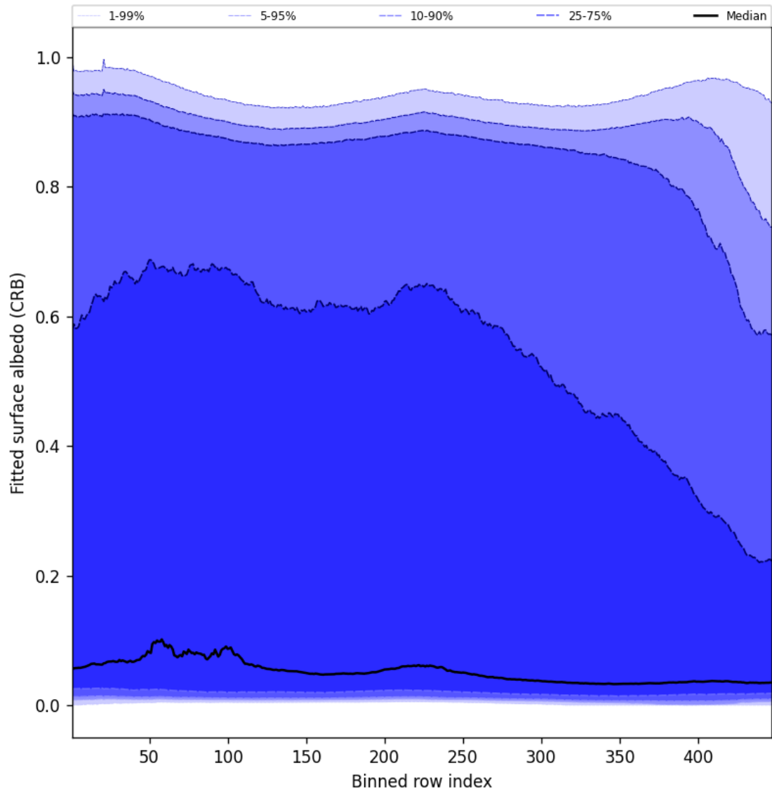
Figure 60: Along track statistics of “Fitted surface albedo (CRB)” for 2025-01-27 to 2025-01-28
