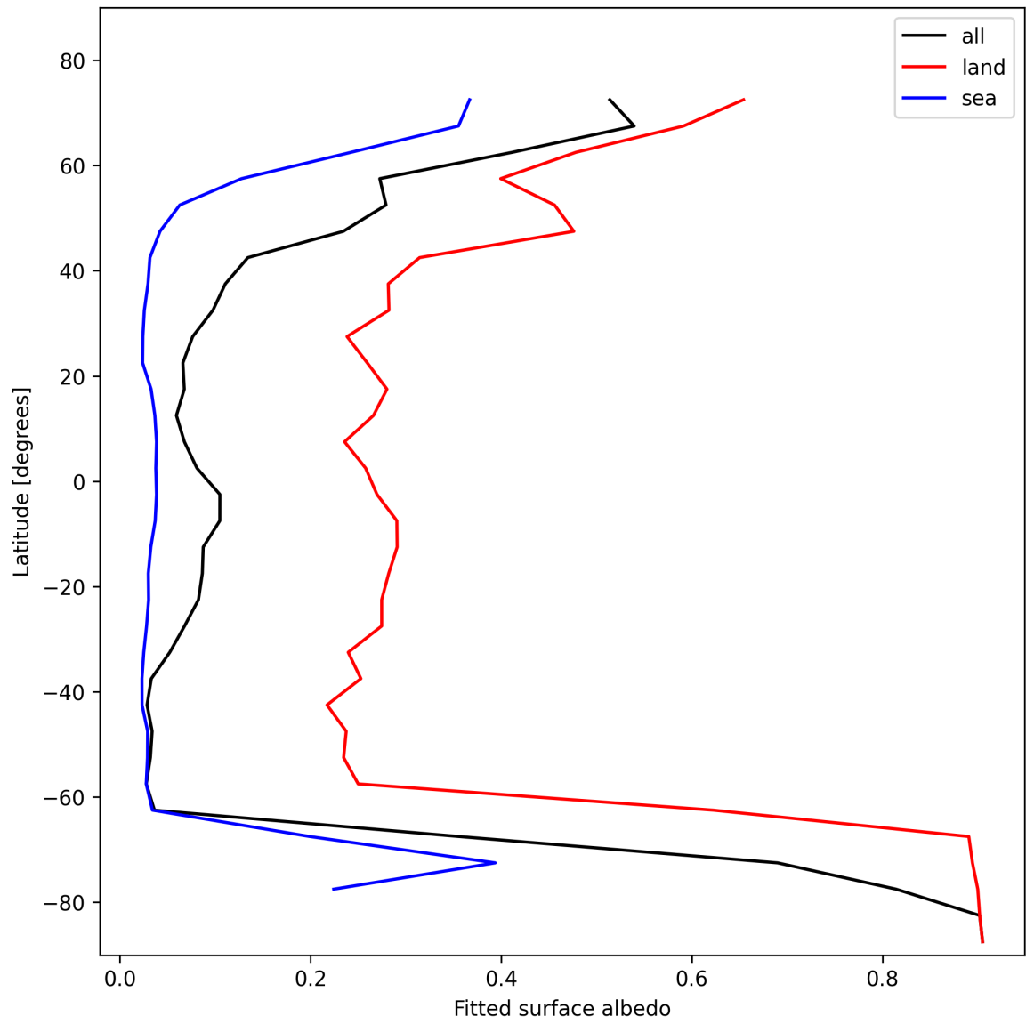
Figure 27: Zonal average of “Fitted surface albedo” for 2025-01-27 to 2025-01-28.
