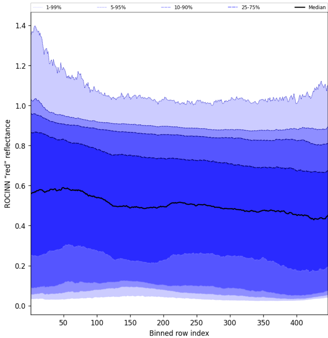
Figure 67: Along track statistics of "ROCINN "red" reflectance" for 2025-01-27 to 2025-01-28
