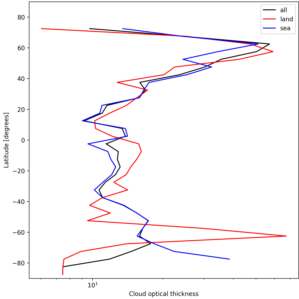
Figure 23: Zonal average of “Cloud optical thickness” for 2025-01-27 to 2025-01-28.
