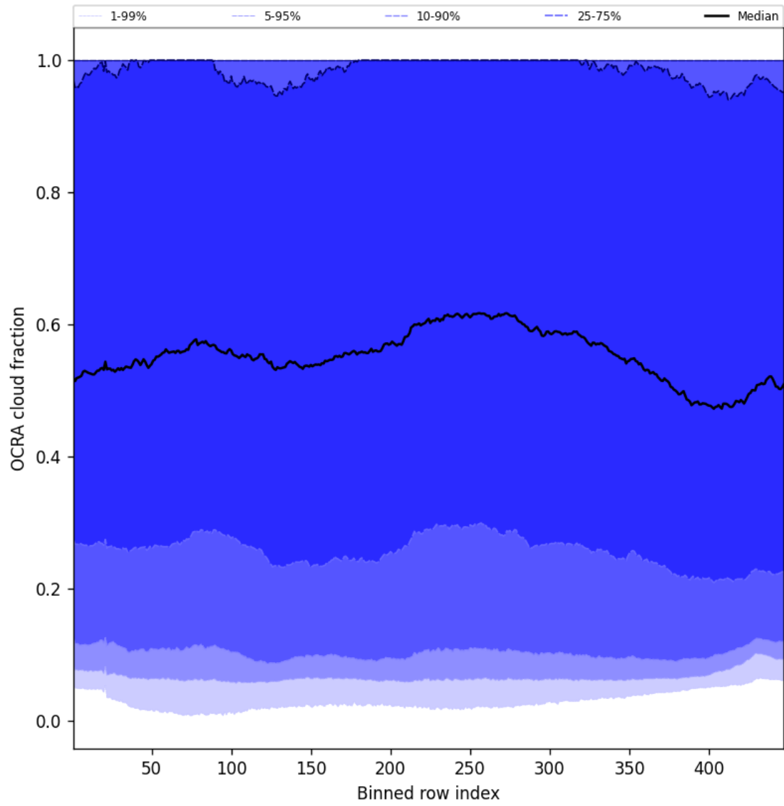
Figure 64: Along track statistics of “OCRA cloud fraction” for 2025-01-27 to 2025-01-28
