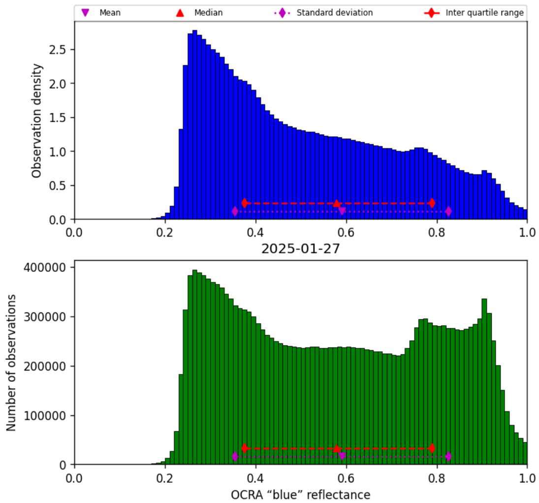
Figure 49: Histogram of “OCRA “blue” reflectance” for 2025-01-27 to 2025-01-28
