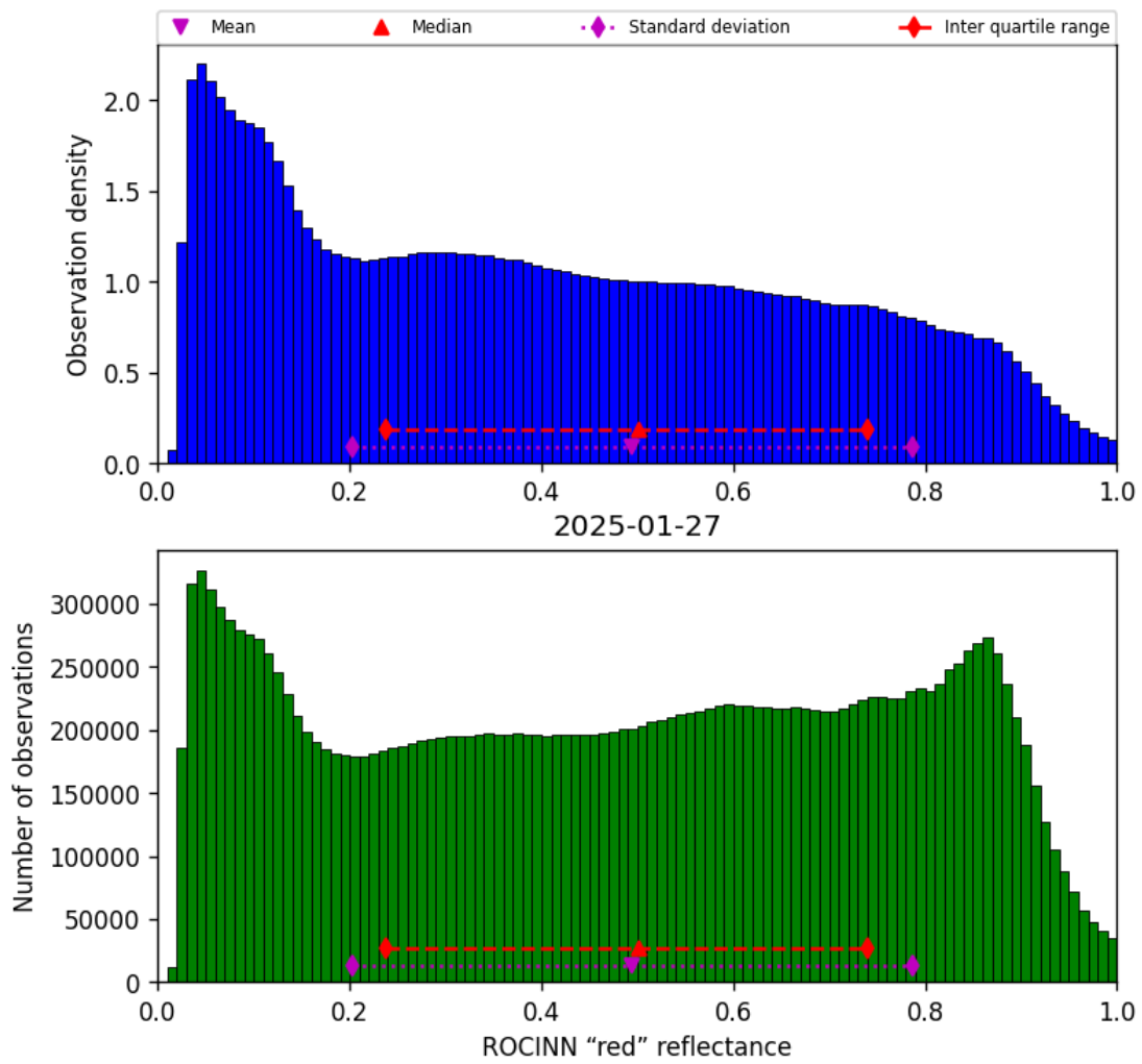
Figure 51: Histogram of "ROCINN "red" reflectance" for 2025-01-27 to 2025-01-28
