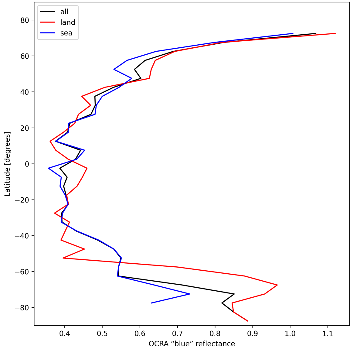
Figure 33: Zonal average of “OCRA “blue” reflectance” for 2025-01-27 to 2025-01-28.
