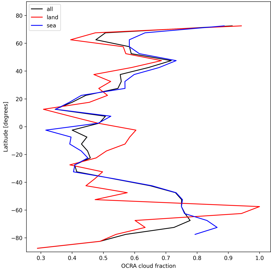
Figure 32: Zonal average of “OCRA cloud fraction” for 2025-01-27 to 2025-01-28.
