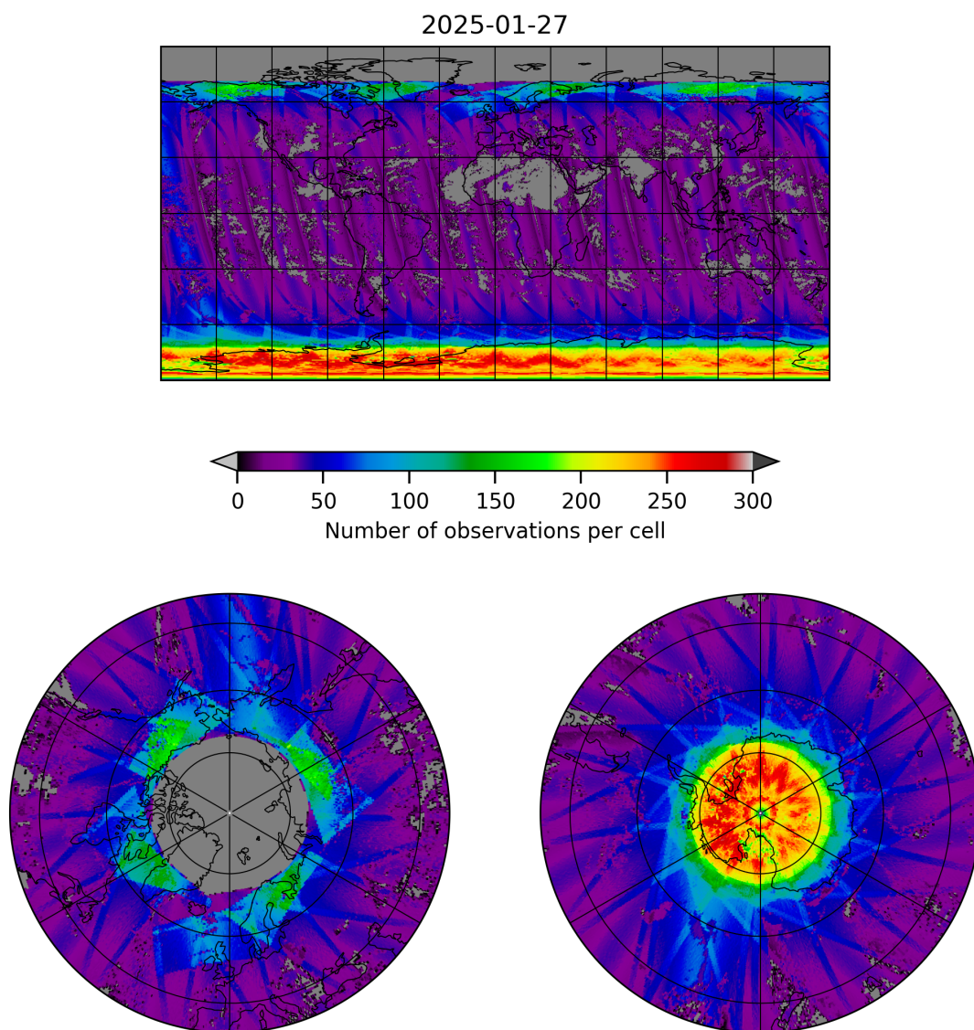
Figure 19: Map of the number of observations for 2025-01-27 to 2025-01-28
