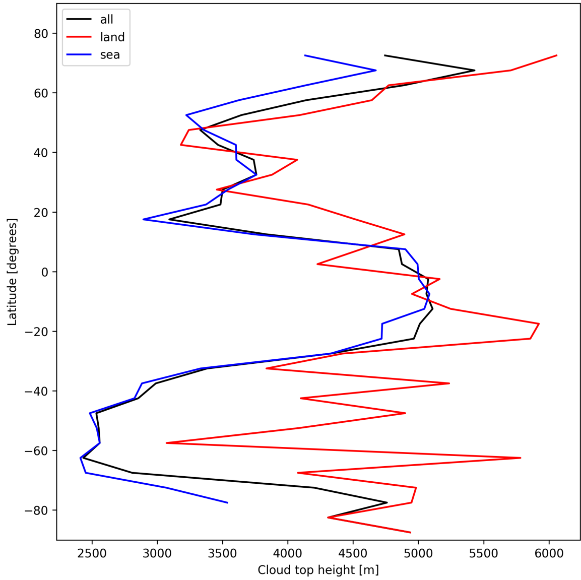
Figure 22: Zonal average of “Cloud top height” for 2025-01-27 to 2025-01-28.
