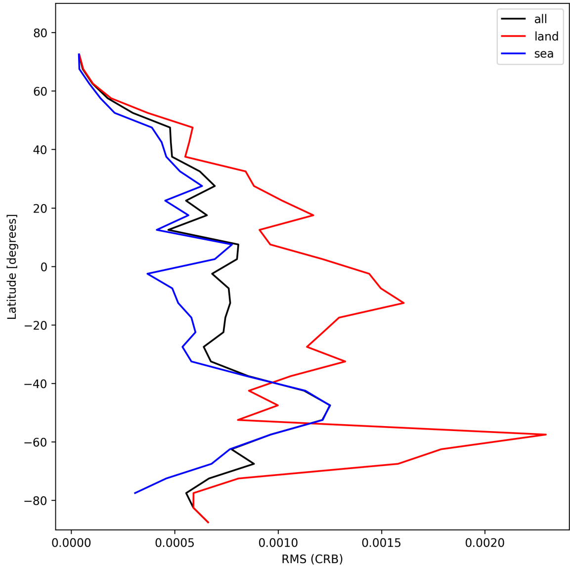
Figure 30: Zonal average of “RMS (CRB)” for 2025-01-27 to 2025-01-28.
