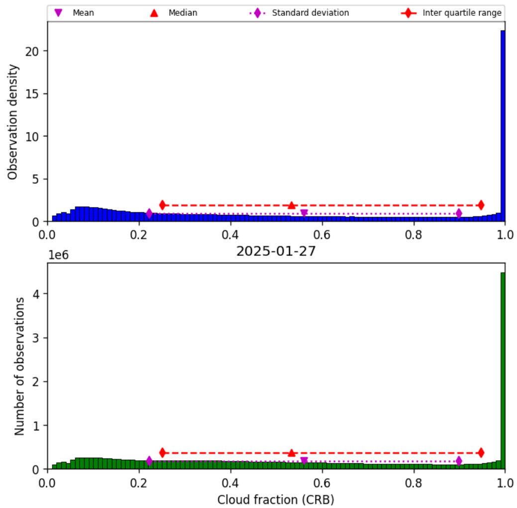
Figure 40: Histogram of “Cloud fraction (CRB)” for 2025-01-27 to 2025-01-28
