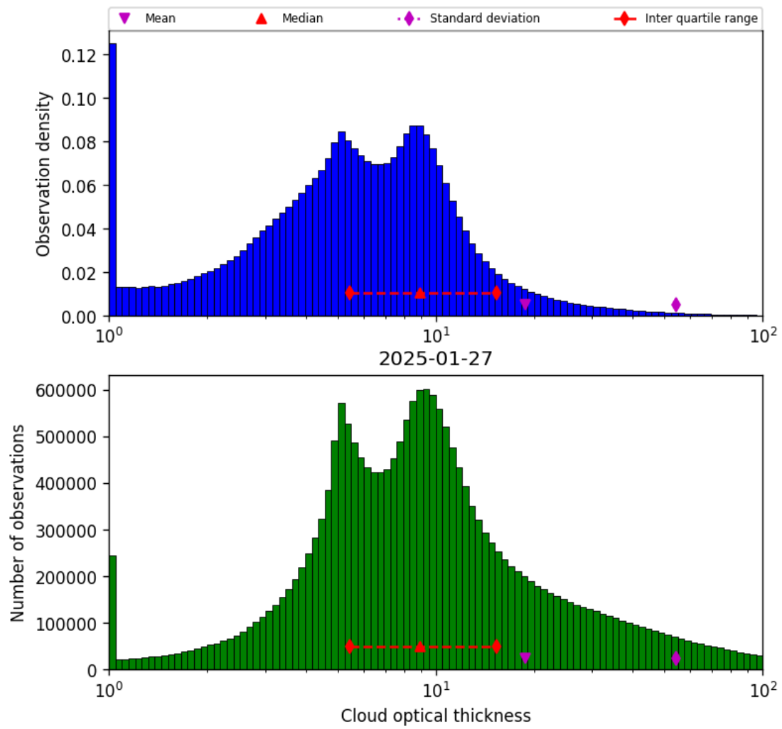
Figure 39: Histogram of “Cloud optical thickness” for 2025-01-27 to 2025-01-28
