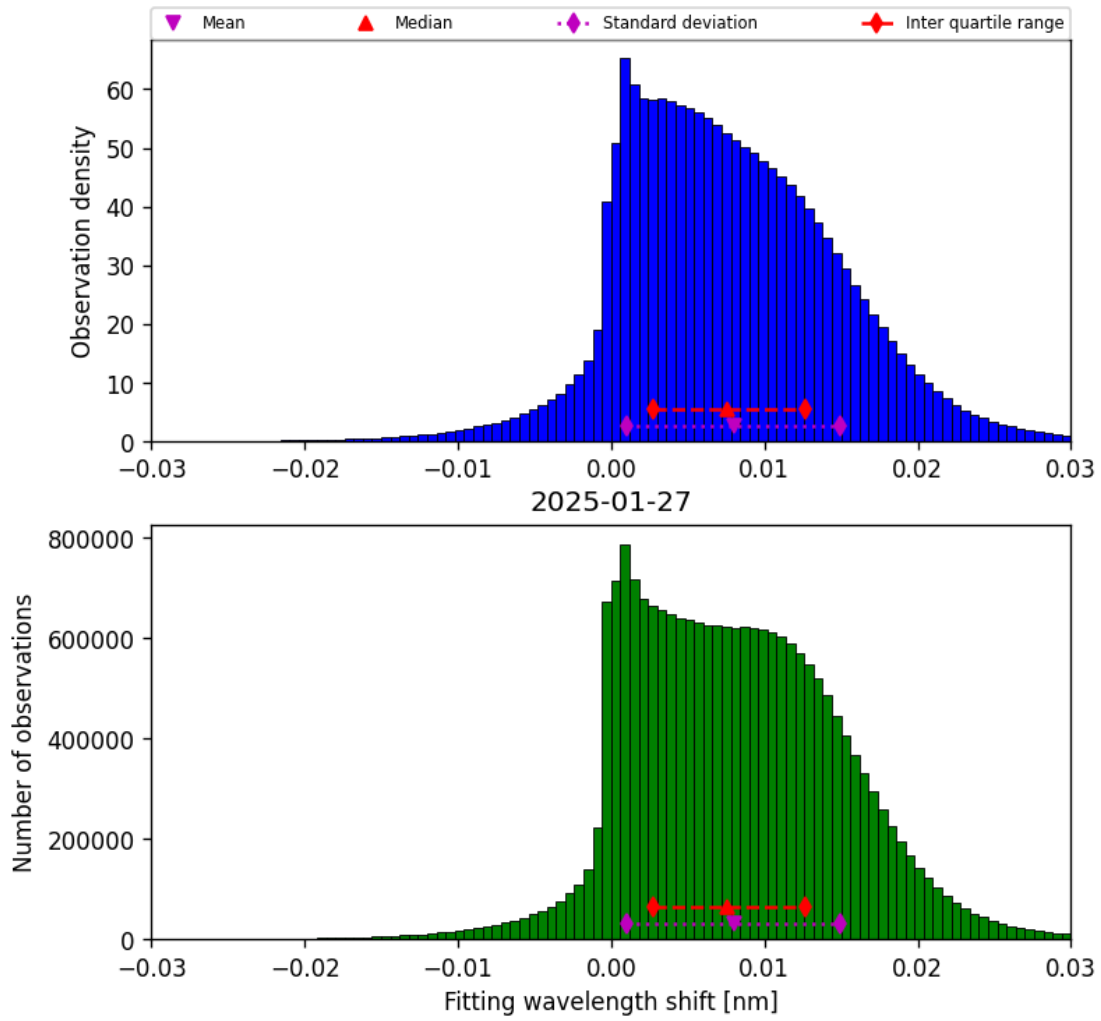
Figure 47: Histogram of “Fitting wavelength shift” for 2025-01-27 to 2025-01-28
