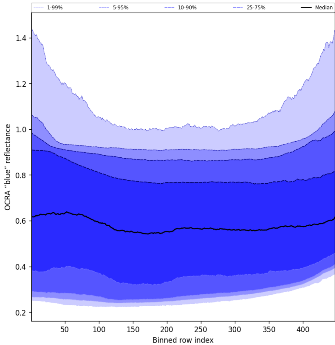
Figure 65: Along track statistics of “OCRA “blue” reflectance” for 2025-01-27 to 2025-01-28
