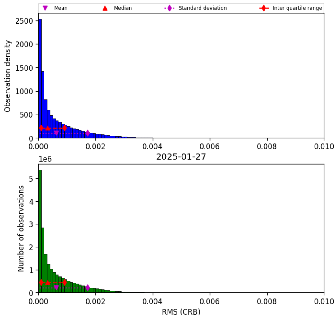
Figure 46: Histogram of “RMS (CRB)” for 2025-01-27 to 2025-01-28
