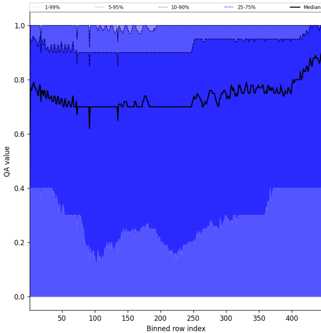
Figure 52: Along track statistics of “QA value” for 2025-01-27 to 2025-01-28
