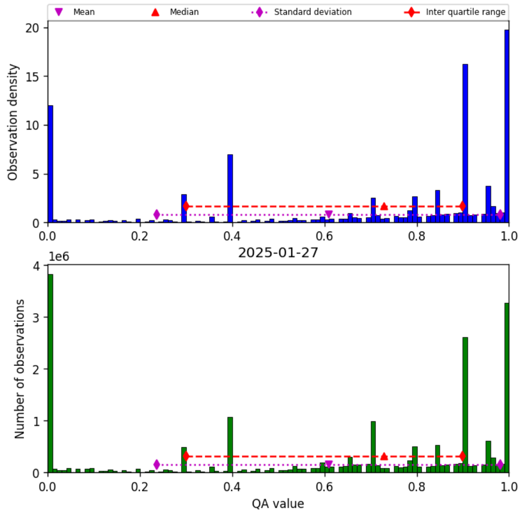
Figure 36: Histogram of “QA value” for 2025-01-27 to 2025-01-28
