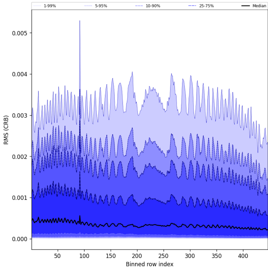
Figure 62: Along track statistics of “RMS (CRB)” for 2025-01-27 to 2025-01-28
