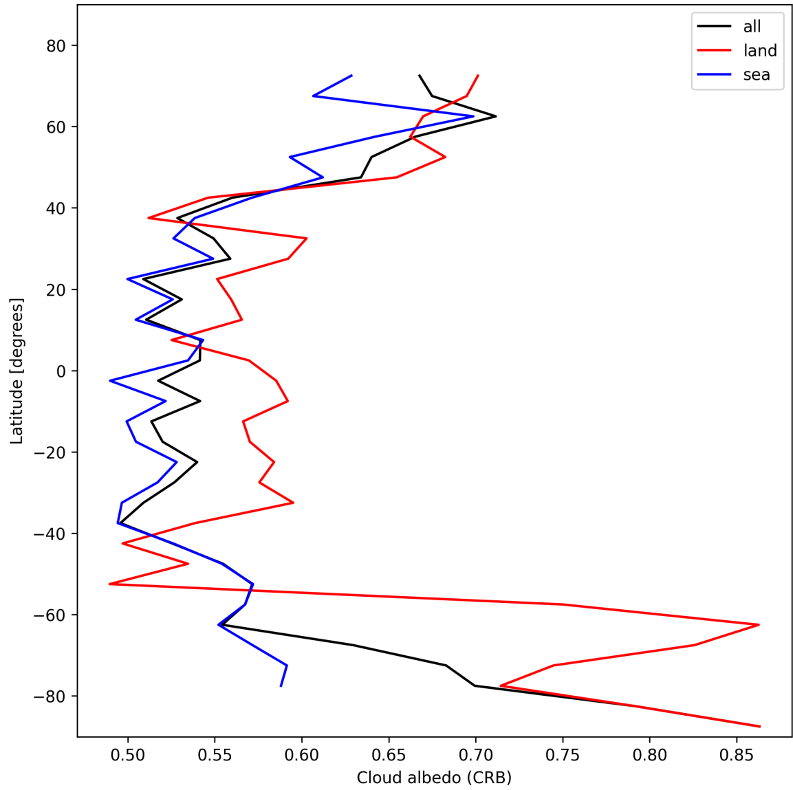
Figure 26: Zonal average of “Cloud albedo (CRB)” for 2025-01-27 to 2025-01-28.
