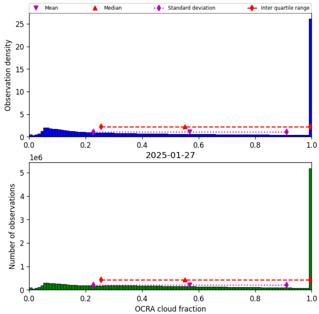
Figure 48: Histogram of “OCRA cloud fraction” for 2025-01-27 to 2025-01-28
