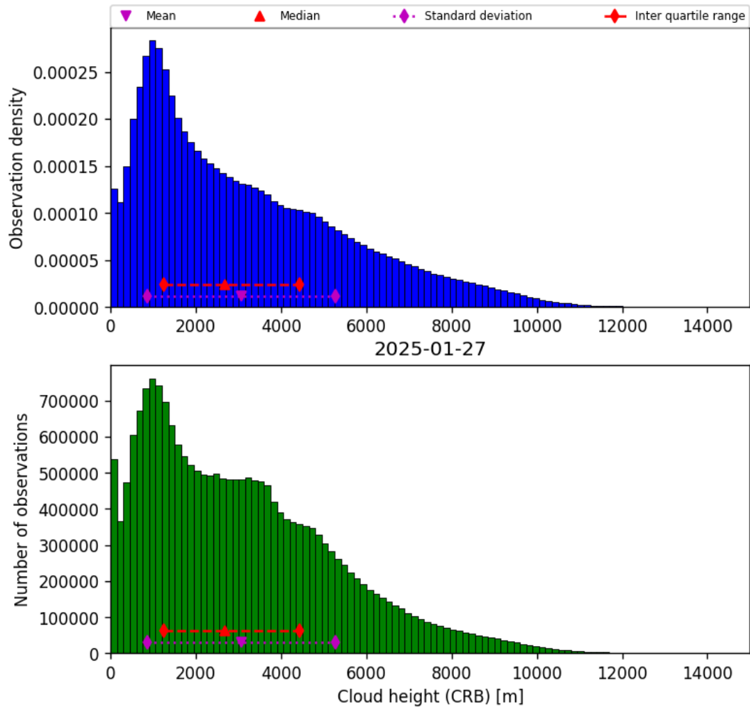
Figure 41: Histogram of “Cloud height (CRB)” for 2025-01-27 to 2025-01-28
