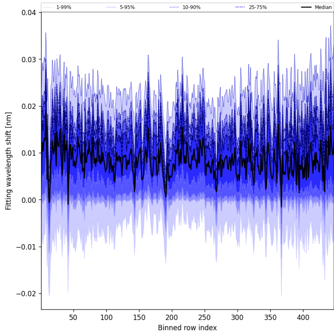
Figure 63: Along track statistics of “Fitting wavelength shift” for 2025-01-27 to 2025-01-28
