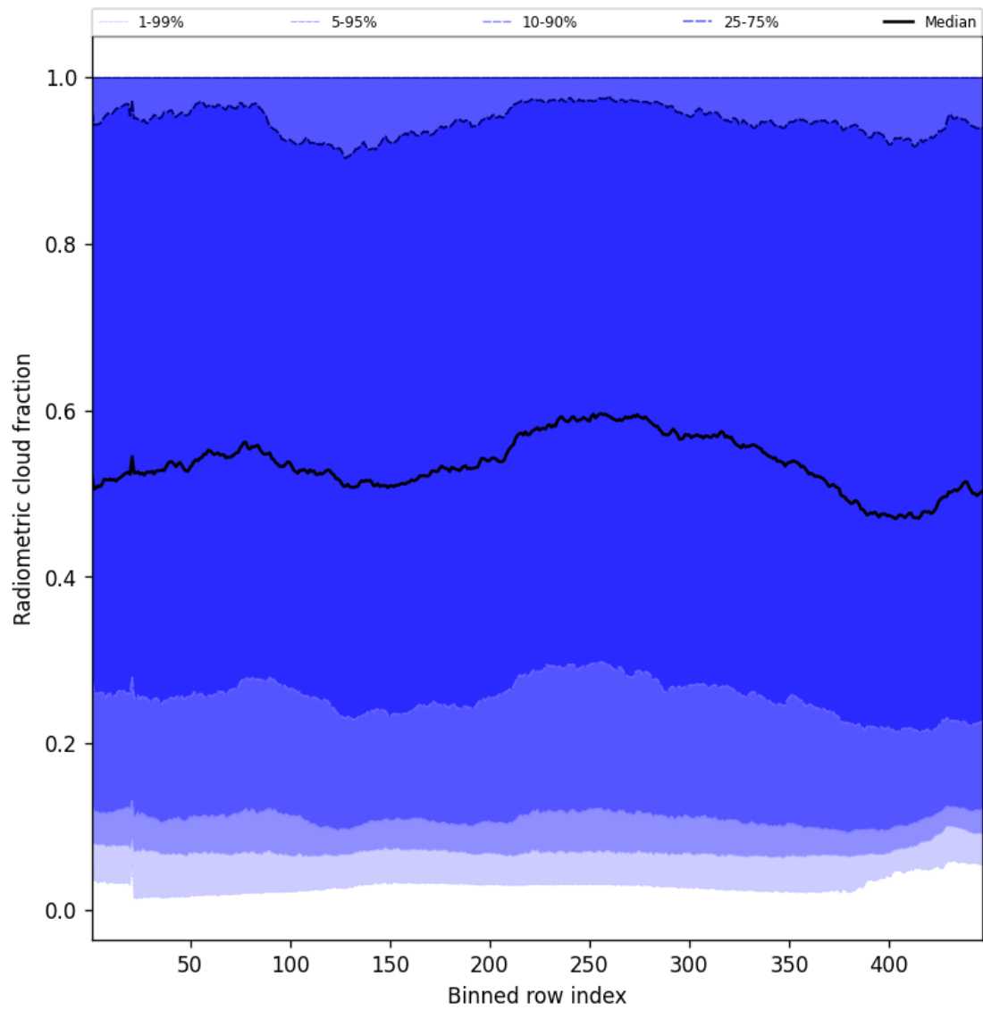
Figure 53: Along track statistics of “Radiometric cloud fraction” for 2025-01-27 to 2025-01-28
