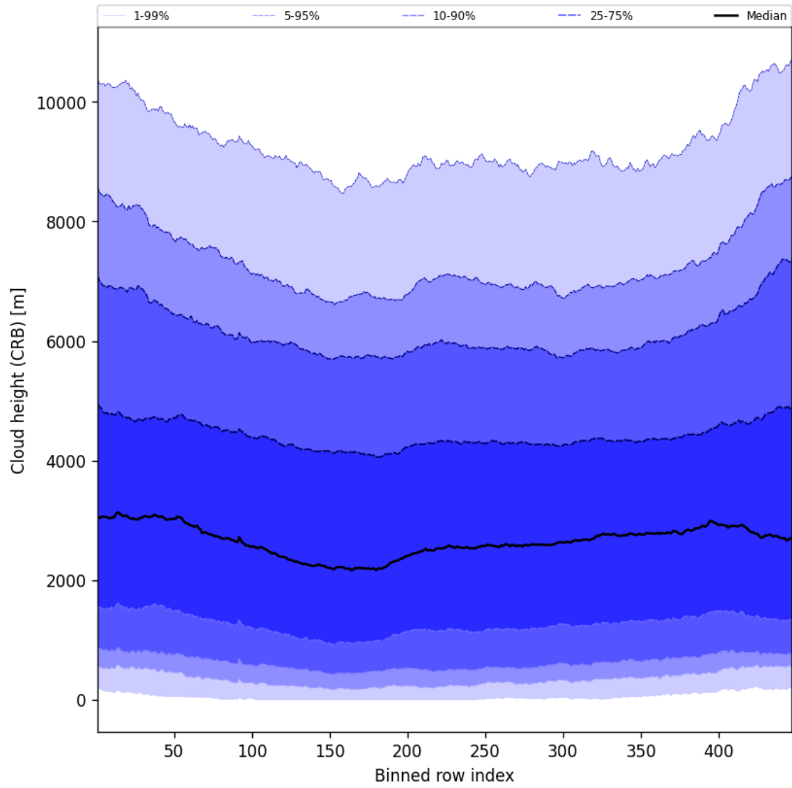
Figure 57: Along track statistics of “Cloud height (CRB)” for 2025-01-27 to 2025-01-28
