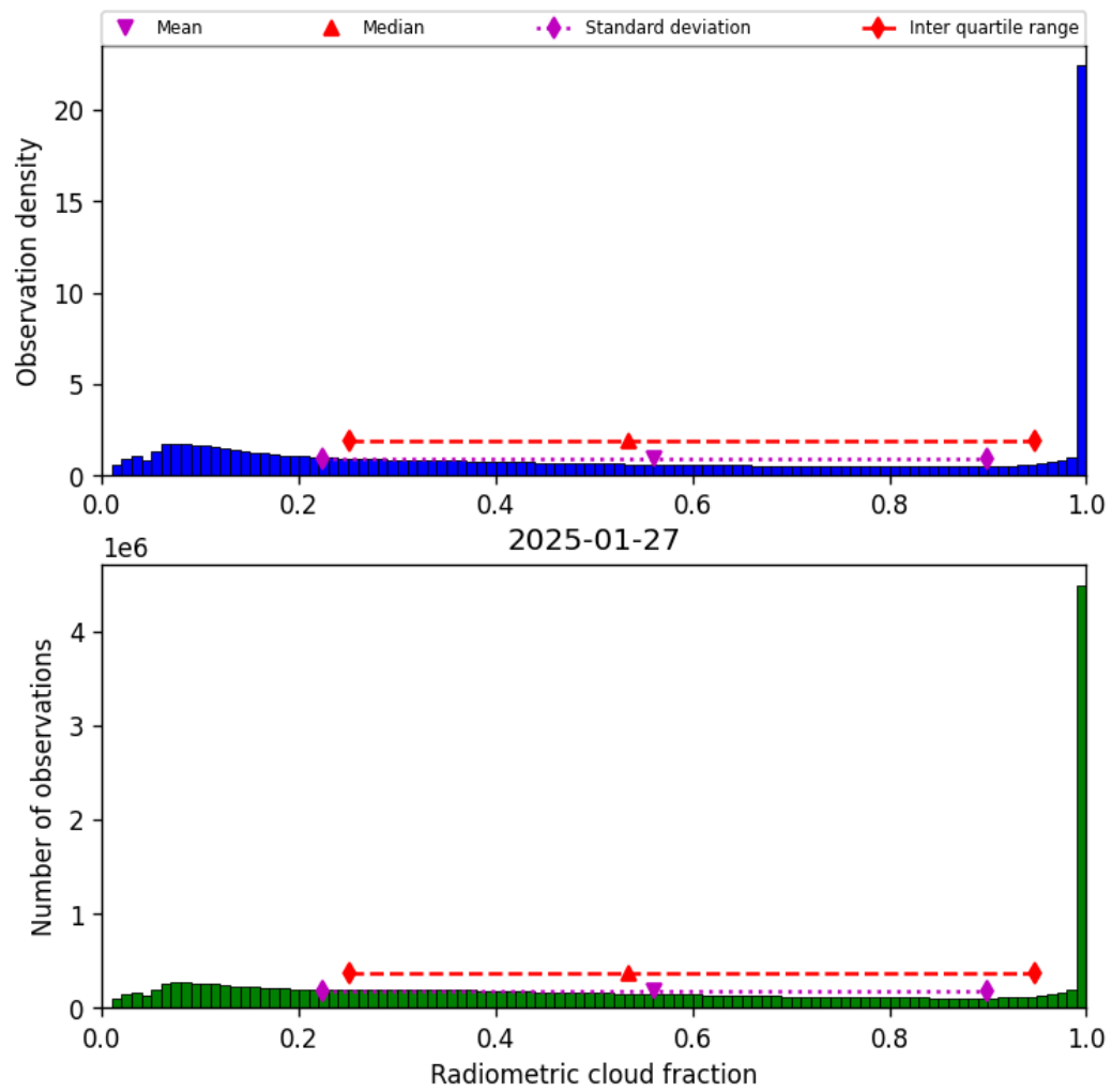
Figure 37: Histogram of “Radiometric cloud fraction” for 2025-01-27 to 2025-01-28
