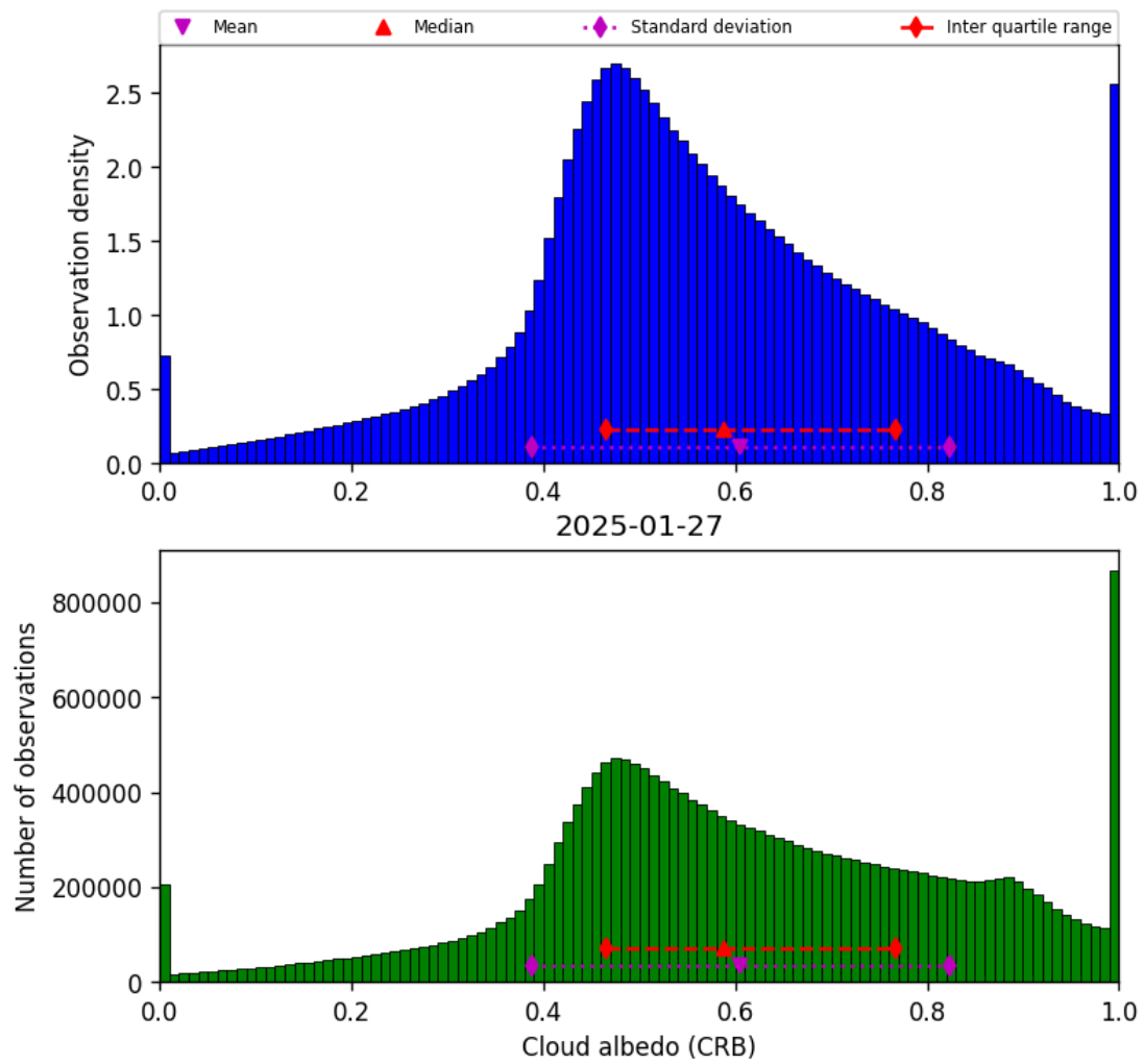
Figure 42: Histogram of “Cloud albedo (CRB)” for 2025-01-27 to 2025-01-28
