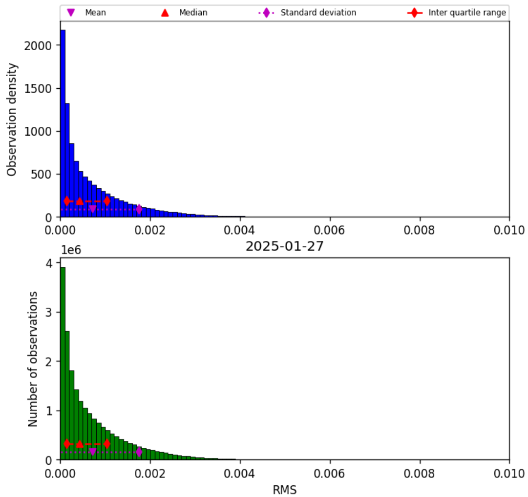
Figure 45: Histogram of “RMS” for 2025-01-27 to 2025-01-28
