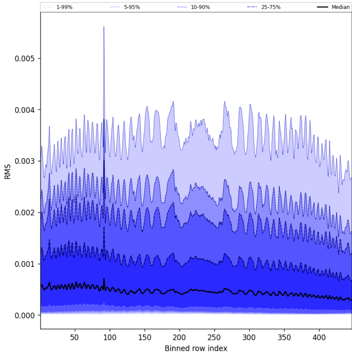
Figure 61: Along track statistics of “RMS” for 2025-01-27 to 2025-01-28
