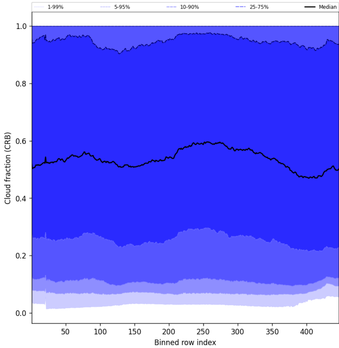
Figure 56: Along track statistics of “Cloud fraction (CRB)” for 2025-01-27 to 2025-01-28
