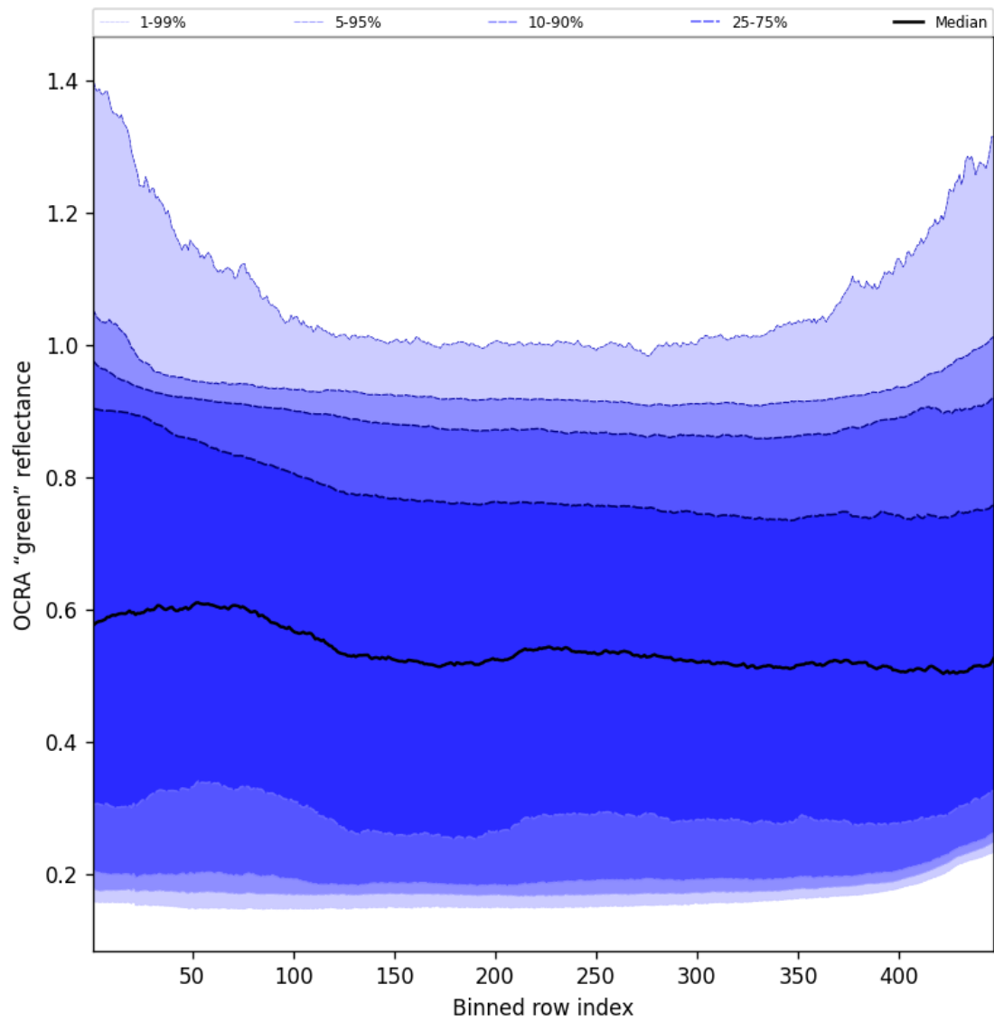
Figure 66: Along track statistics of "OCRA "green" reflectance" for 2025-01-27 to 2025-01-28
