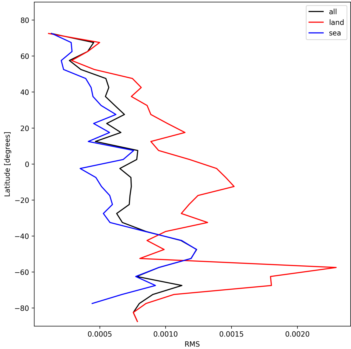
Figure 29: Zonal average of “RMS” for 2025-01-27 to 2025-01-28.
