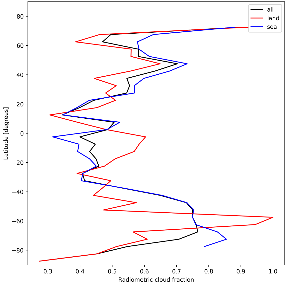
Figure 21: Zonal average of “Radiometric cloud fraction” for 2025-01-27 to 2025-01-28.
