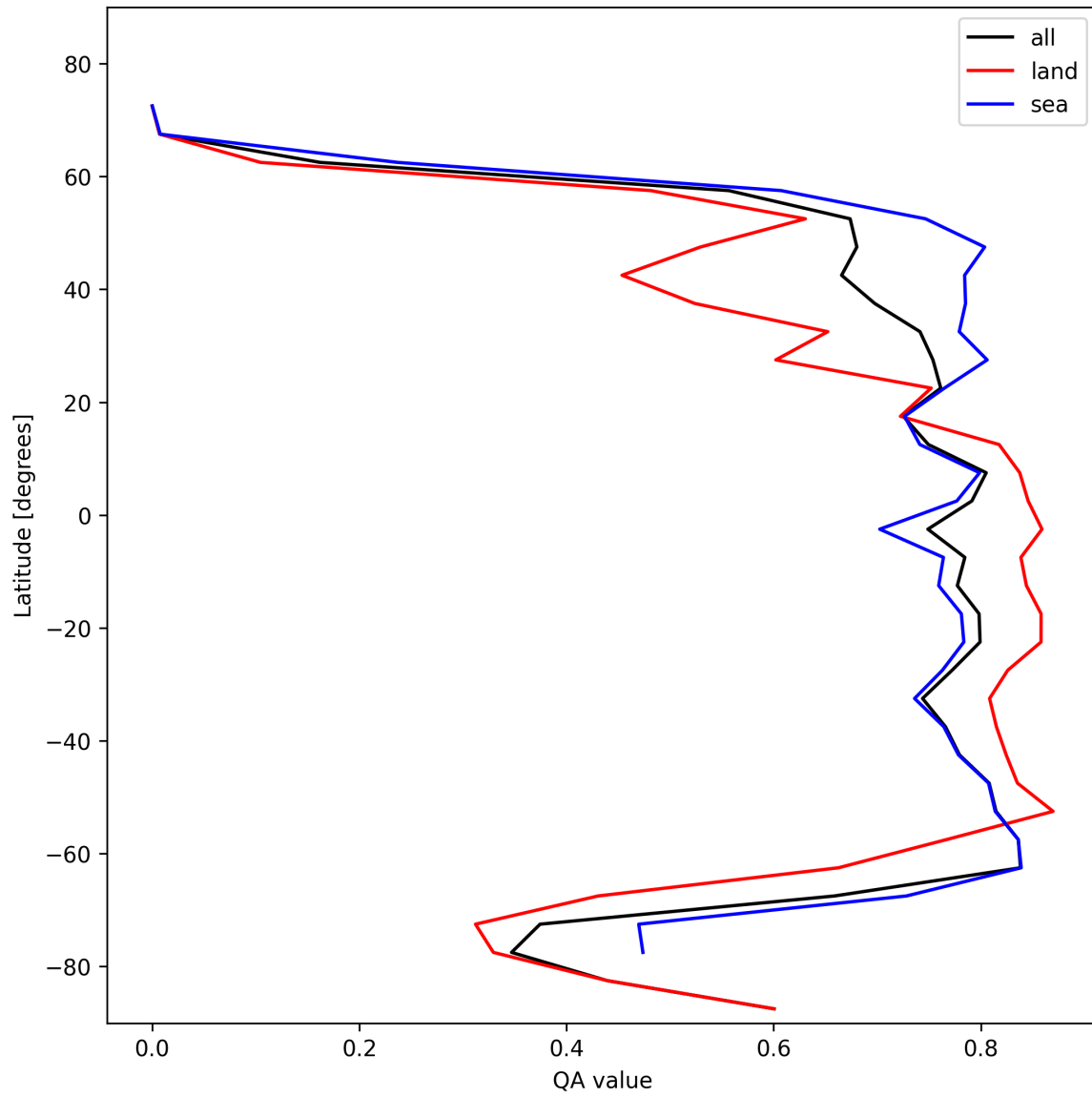
Figure 20: Zonal average of “QA value” for 2025-01-27 to 2025-01-28.
