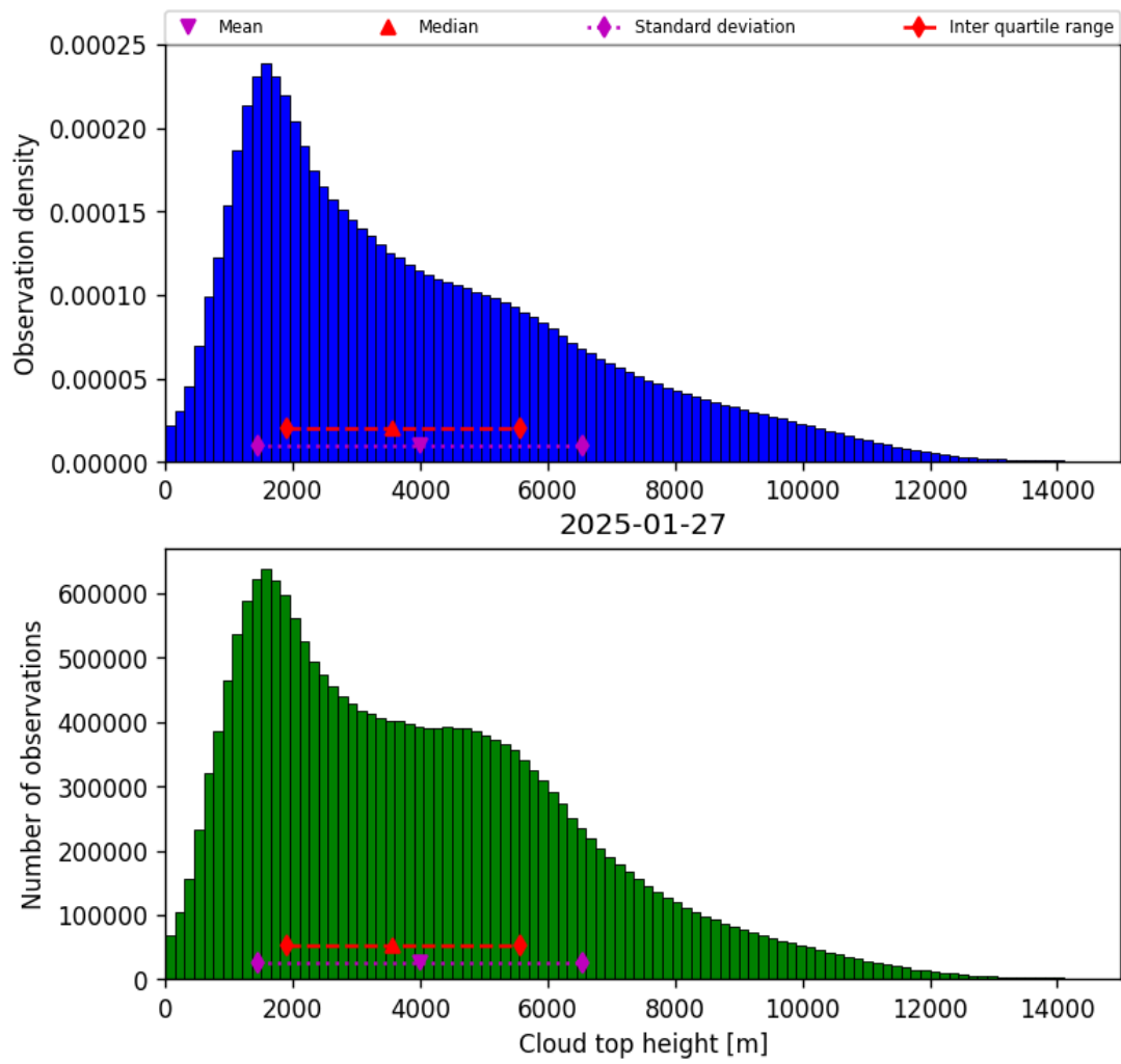
Figure 38: Histogram of “Cloud top height” for 2025-01-27 to 2025-01-28
