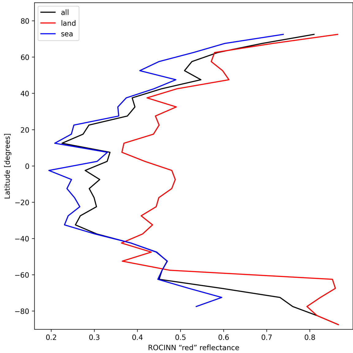
Figure 35: Zonal average of “ROCINN “red” reflectance” for 2025-01-27 to 2025-01-28.
