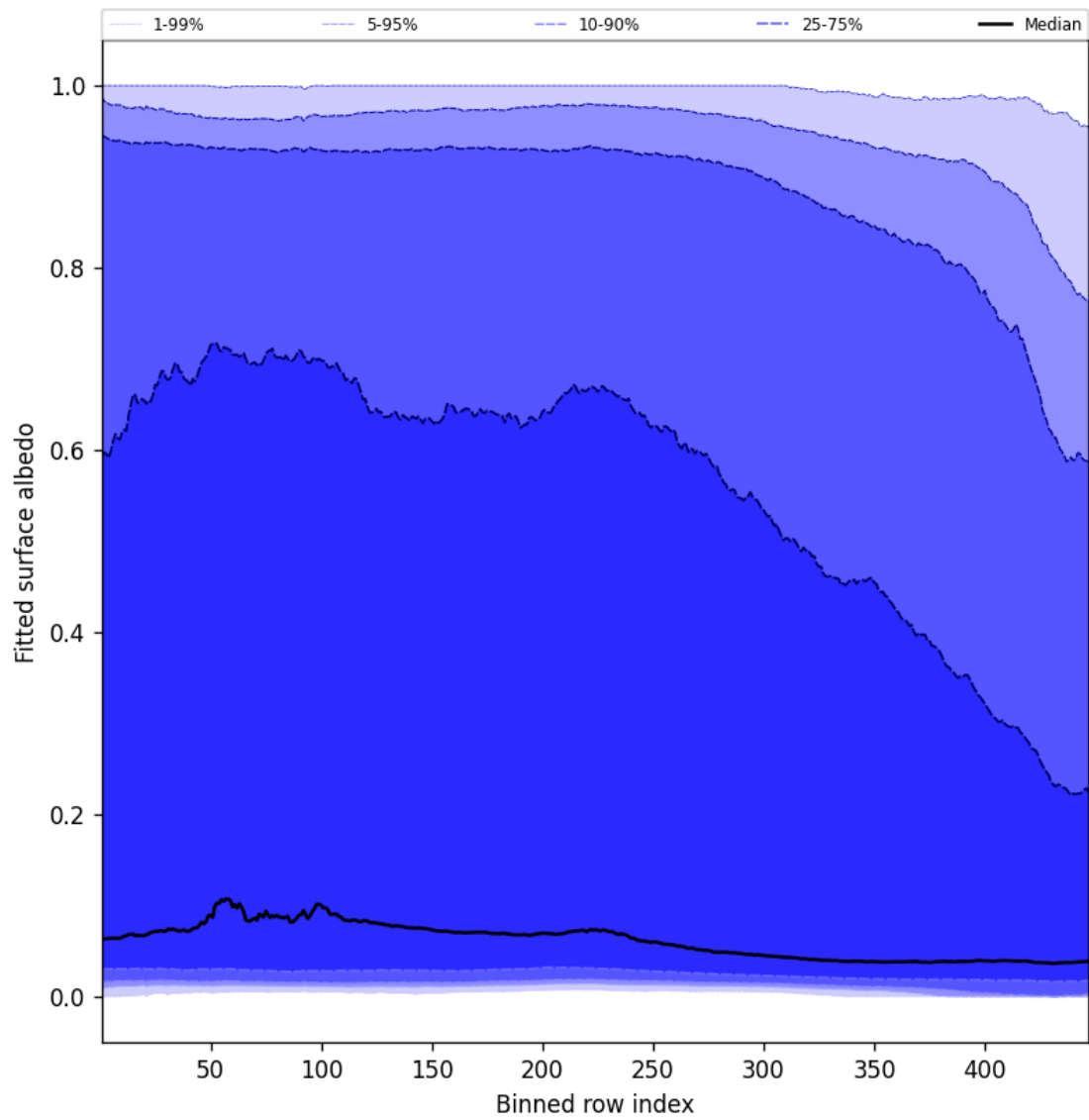
Figure 59: Along track statistics of “Fitted surface albedo” for 2025-01-27 to 2025-01-28
