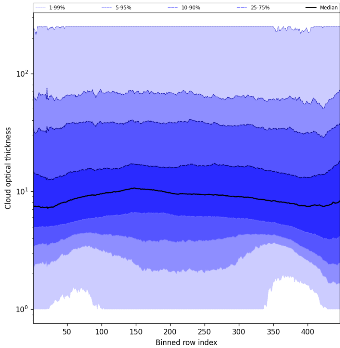
Figure 55: Along track statistics of “Cloud optical thickness” for 2025-01-27 to 2025-01-28
