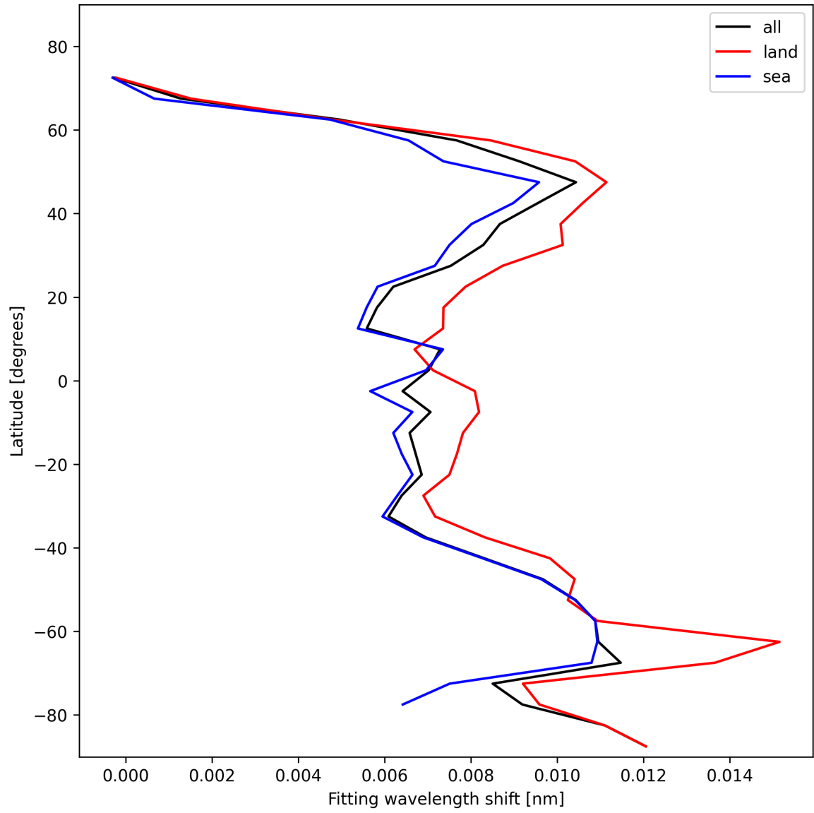
Figure 31: Zonal average of “Fitting wavelength shift” for 2025-01-27 to 2025-01-28.
