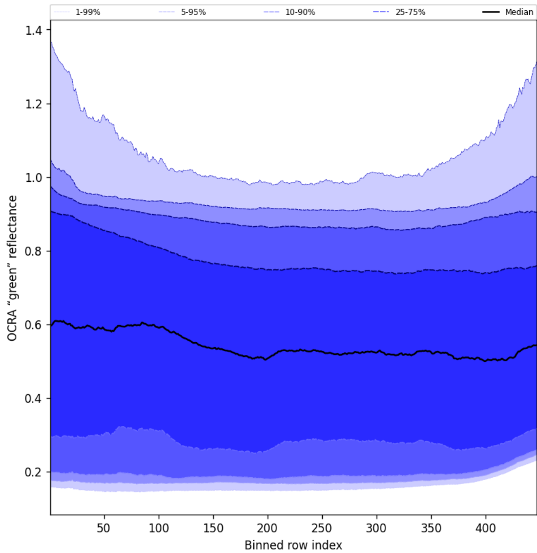
Figure 66: Along track statistics of “OCRA “green” reflectance” for 2025-01-28 to 2025-01-29
