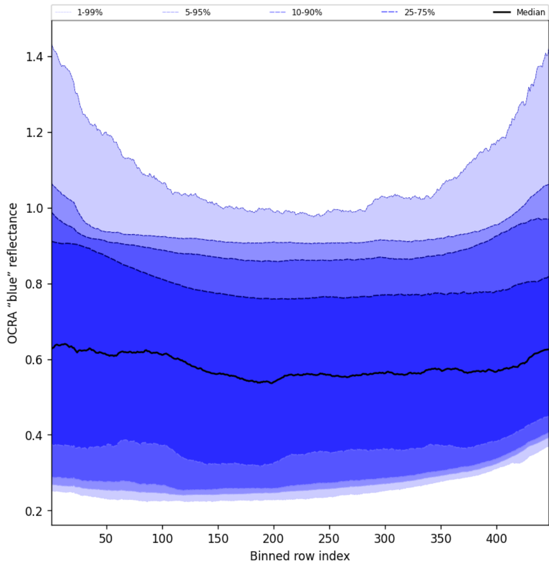
Figure 65: Along track statistics of "OCRA "blue" reflectance" for 2025-01-28 to 2025-01-29
