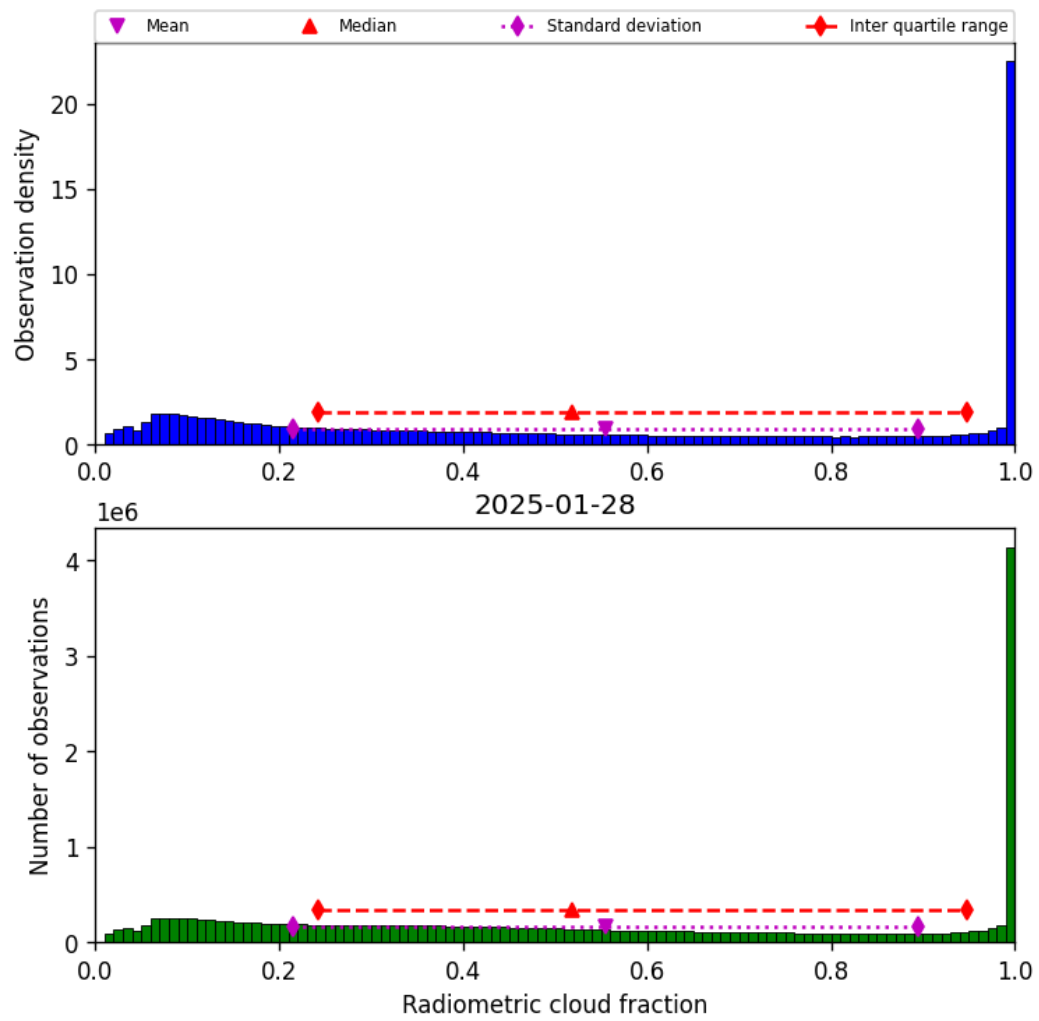
Figure 37: Histogram of “Radiometric cloud fraction” for 2025-01-28 to 2025-01-29
