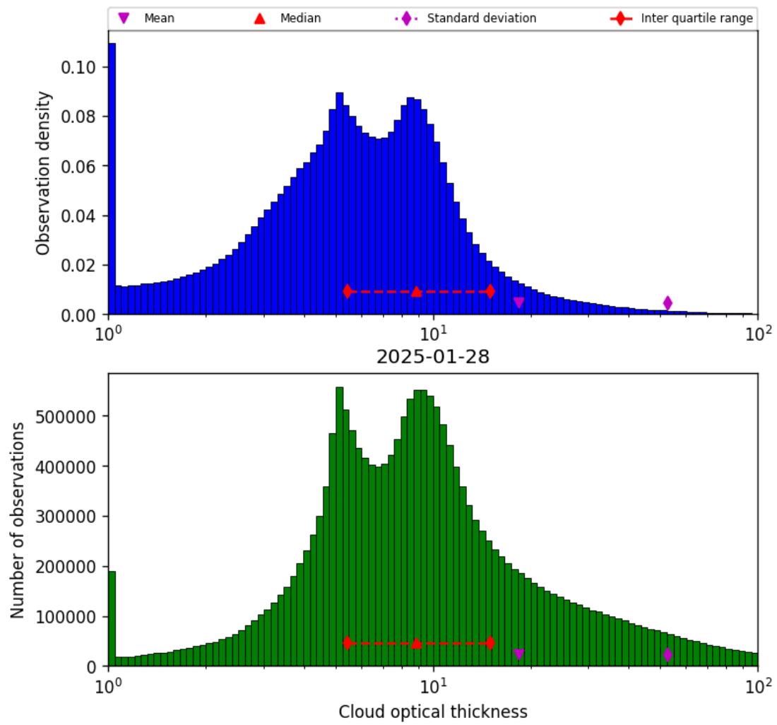
Figure 39: Histogram of “Cloud optical thickness” for 2025-01-28 to 2025-01-29
