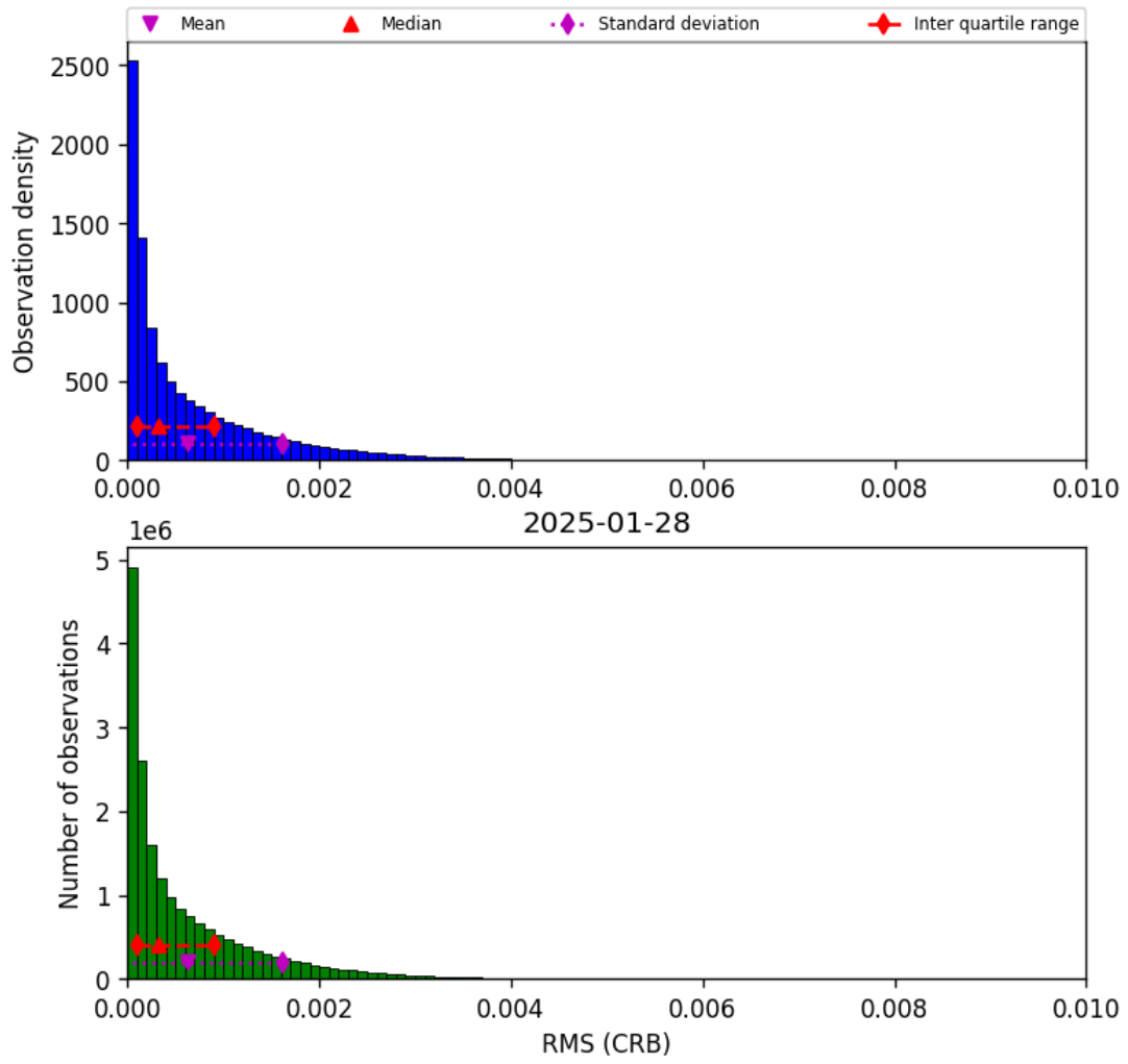
Figure 46: Histogram of “RMS (CRB)” for 2025-01-28 to 2025-01-29
