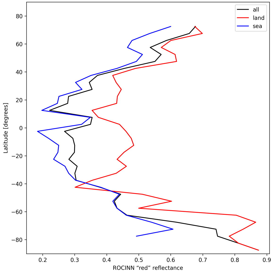
Figure 35: Zonal average of "ROCINN "red" reflectance" for 2025-01-28 to 2025-01-29.
