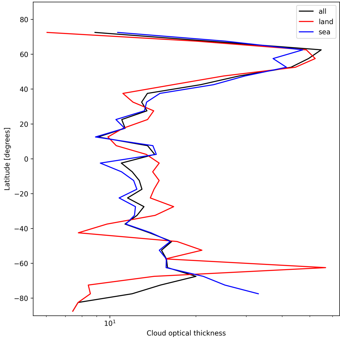
Figure 23: Zonal average of “Cloud optical thickness” for 2025-01-28 to 2025-01-29.
