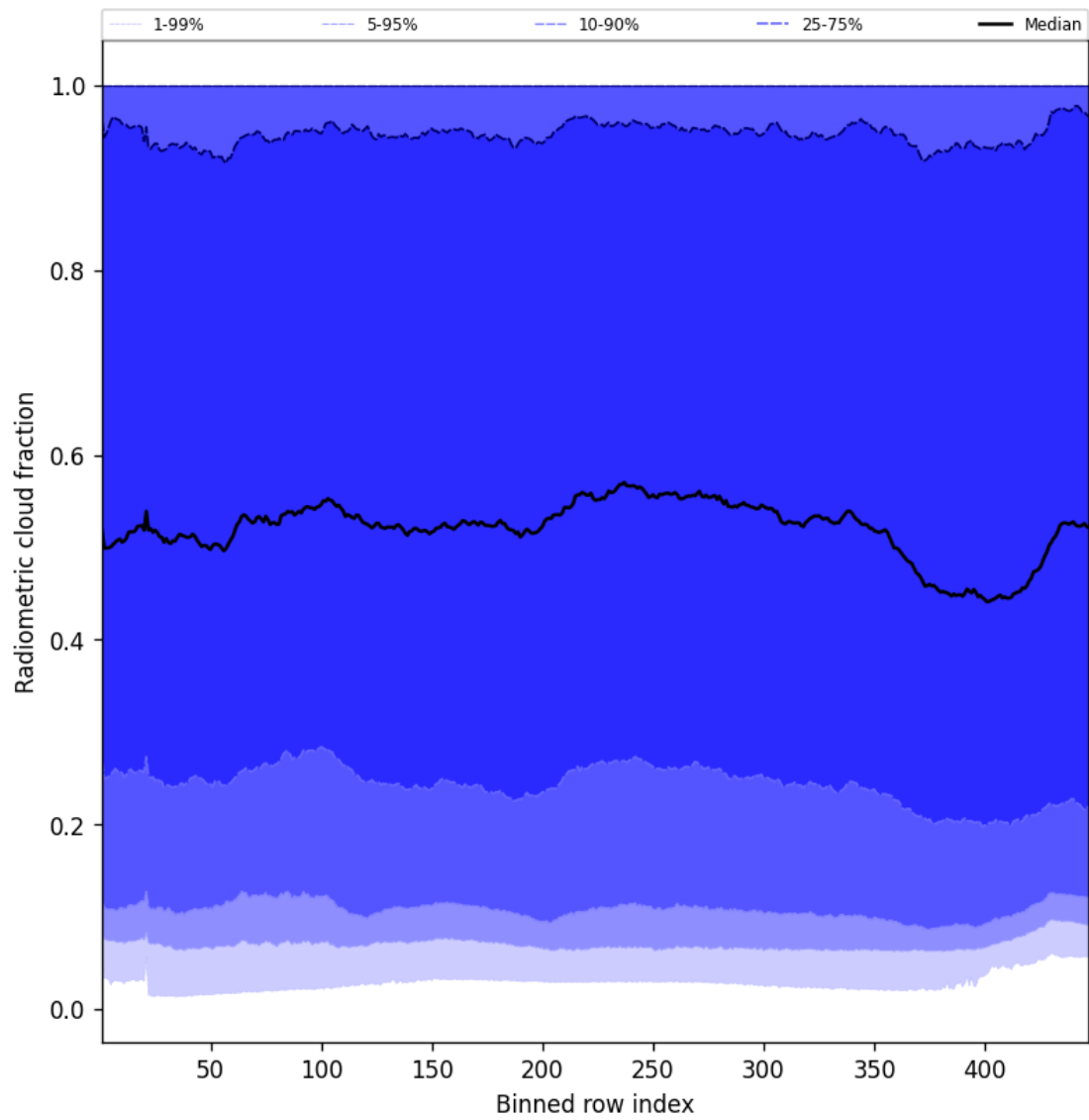
Figure 53: Along track statistics of “Radiometric cloud fraction” for 2025-01-28 to 2025-01-29
