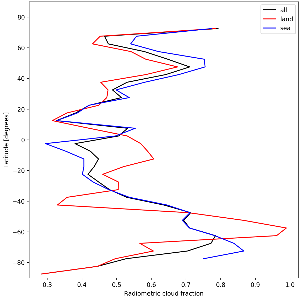
Figure 21: Zonal average of “Radiometric cloud fraction” for 2025-01-28 to 2025-01-29.
