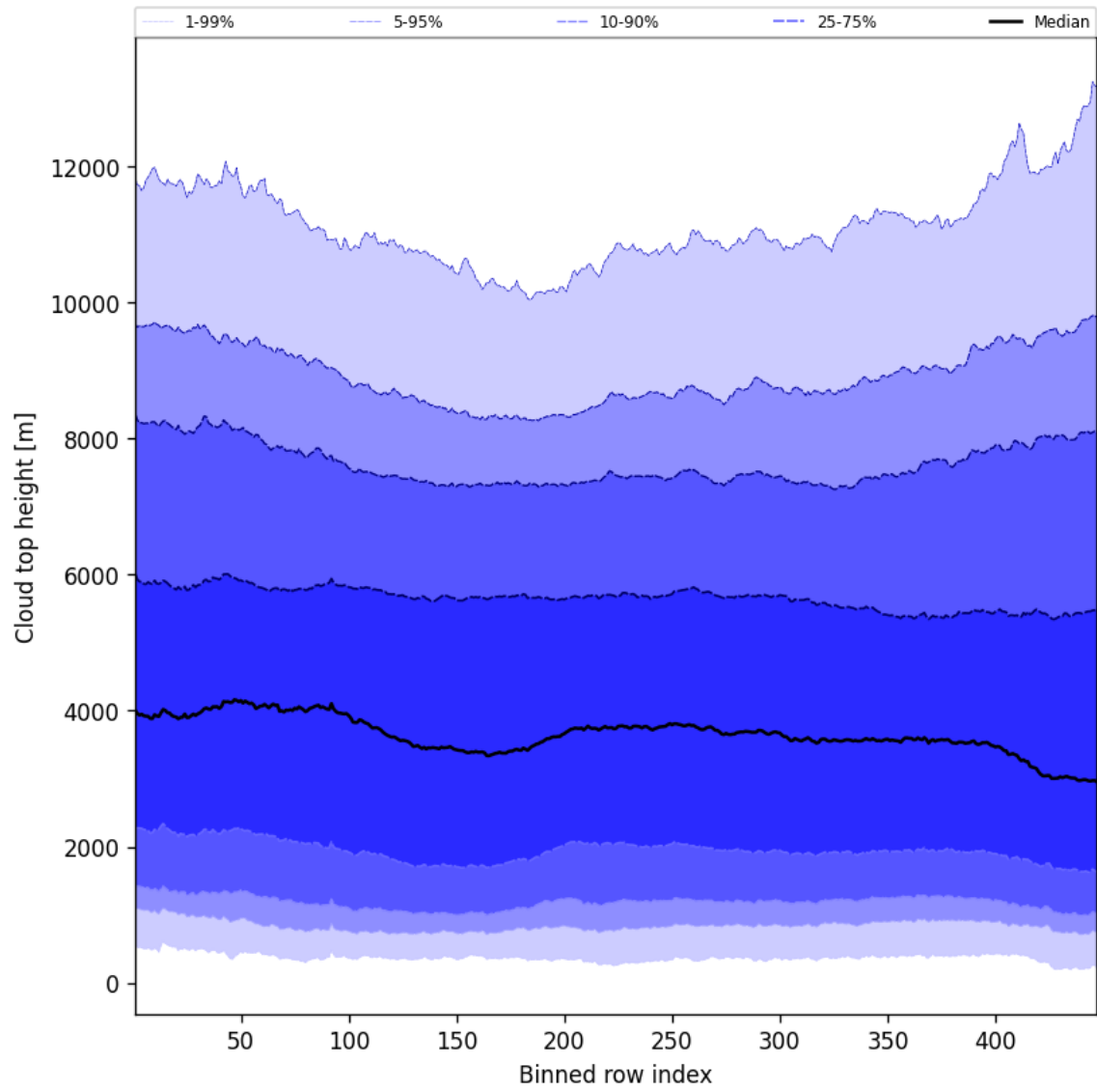
Figure 54: Along track statistics of “Cloud top height” for 2025-01-28 to 2025-01-29
