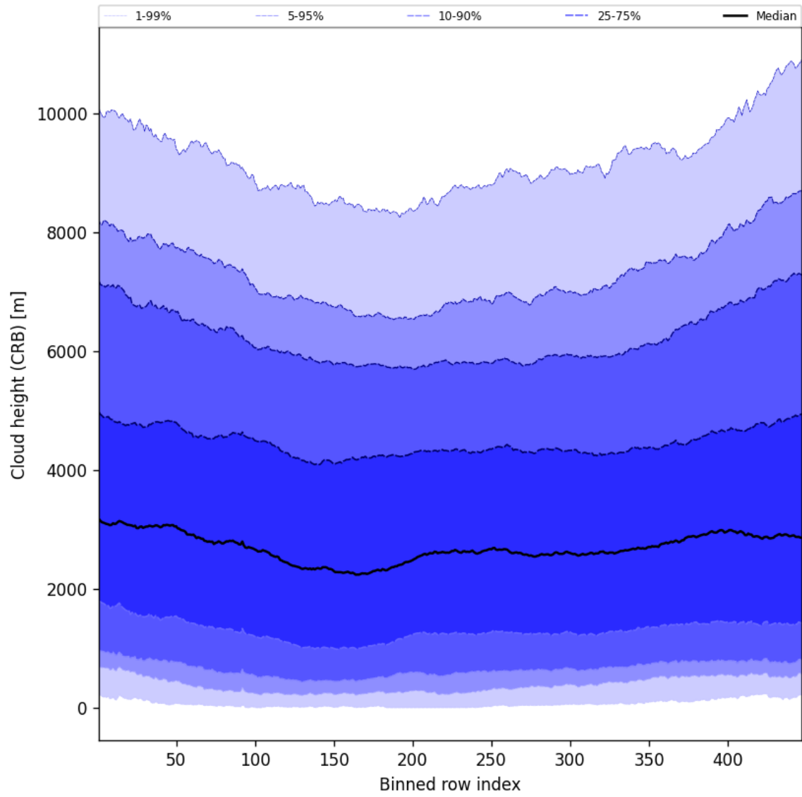
Figure 57: Along track statistics of “Cloud height (CRB)” for 2025-01-28 to 2025-01-29
