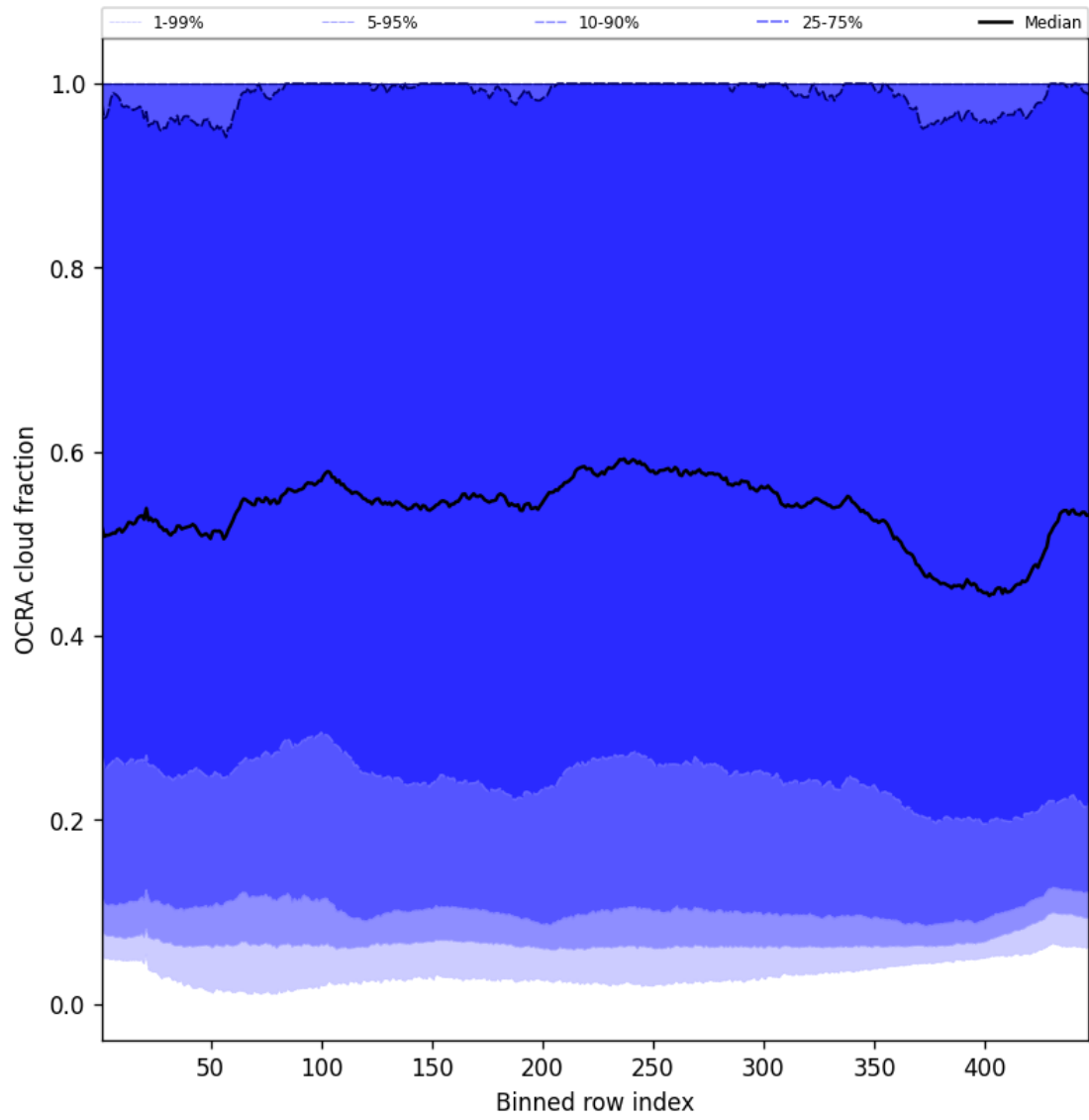
Figure 64: Along track statistics of “OCRA cloud fraction” for 2025-01-28 to 2025-01-29
