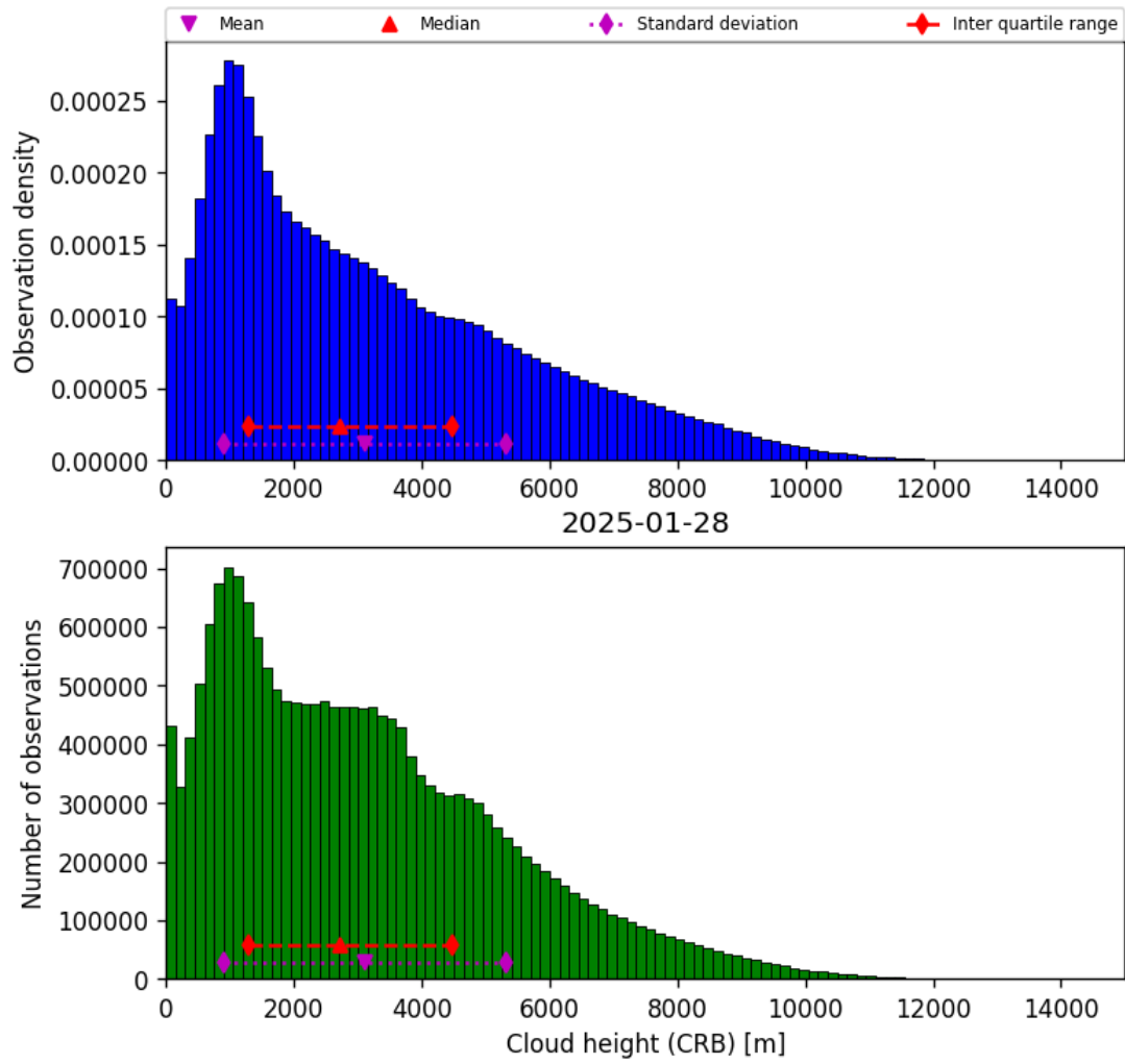
Figure 41: Histogram of “Cloud height (CRB)” for 2025-01-28 to 2025-01-29
