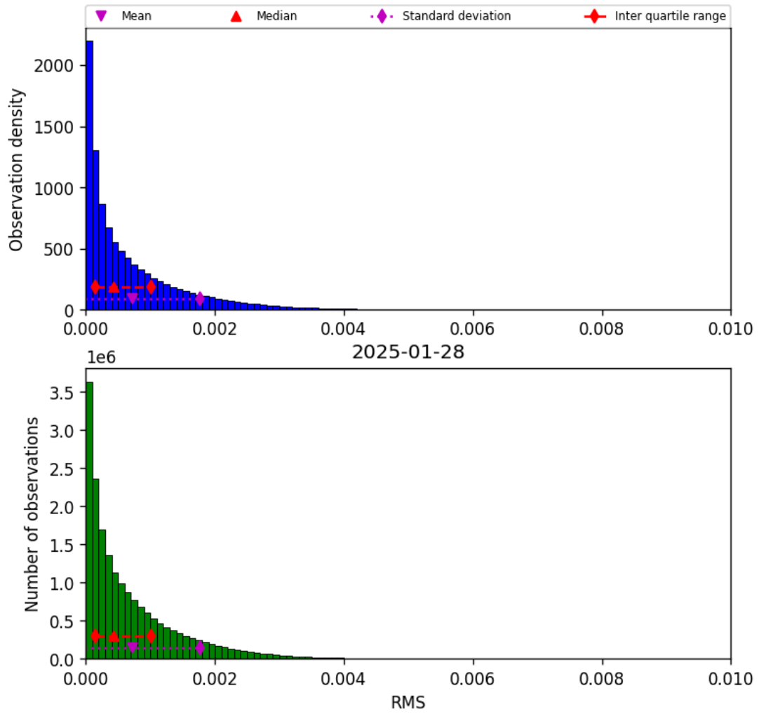
Figure 45: Histogram of “RMS” for 2025-01-28 to 2025-01-29
