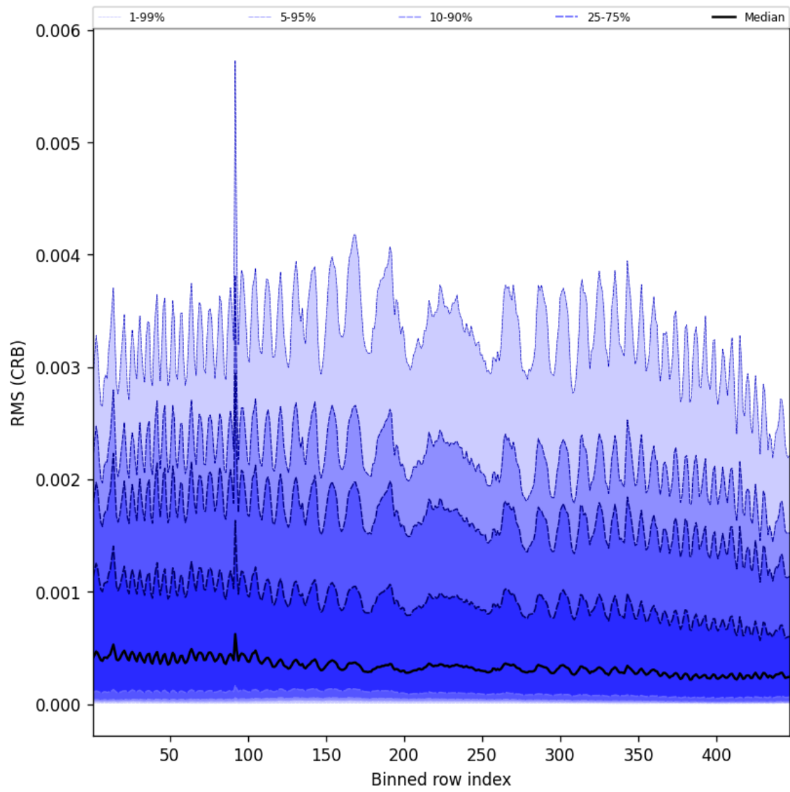
Figure 62: Along track statistics of “RMS (CRB)” for 2025-01-28 to 2025-01-29
