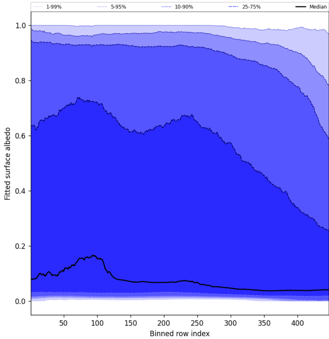
Figure 59: Along track statistics of “Fitted surface albedo” for 2025-01-28 to 2025-01-29
