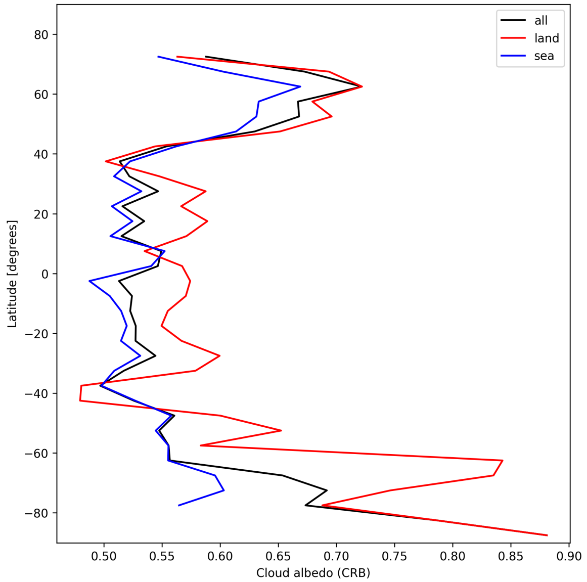
Figure 26: Zonal average of “Cloud albedo (CRB)” for 2025-01-28 to 2025-01-29.
