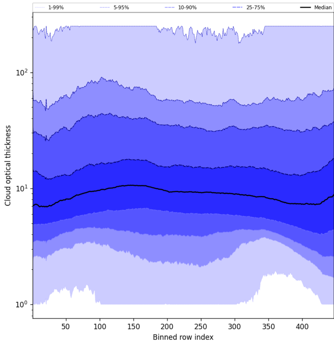
Figure 55: Along track statistics of “Cloud optical thickness” for 2025-01-28 to 2025-01-29
