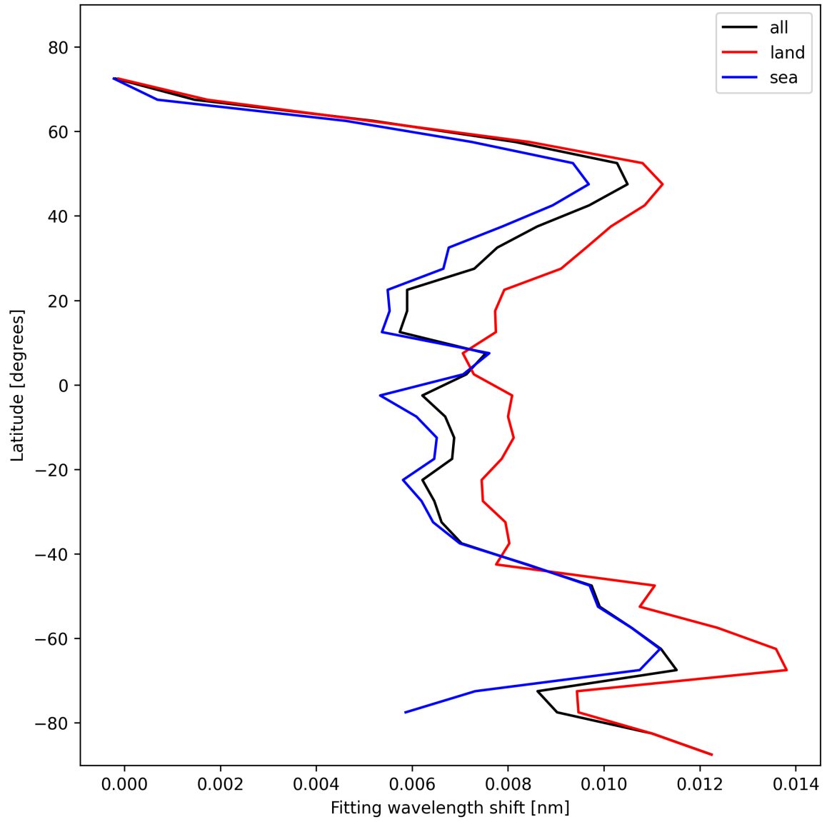
Figure 31: Zonal average of “Fitting wavelength shift” for 2025-01-28 to 2025-01-29.
