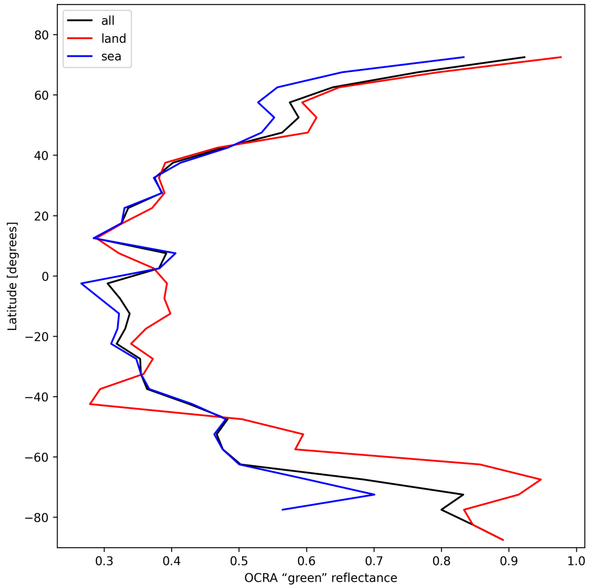
Figure 34: Zonal average of “OCRA “green” reflectance” for 2025-01-28 to 2025-01-29.
