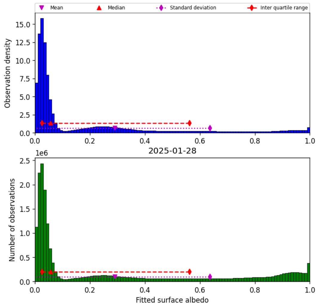
Figure 43: Histogram of “Fitted surface albedo” for 2025-01-28 to 2025-01-29
