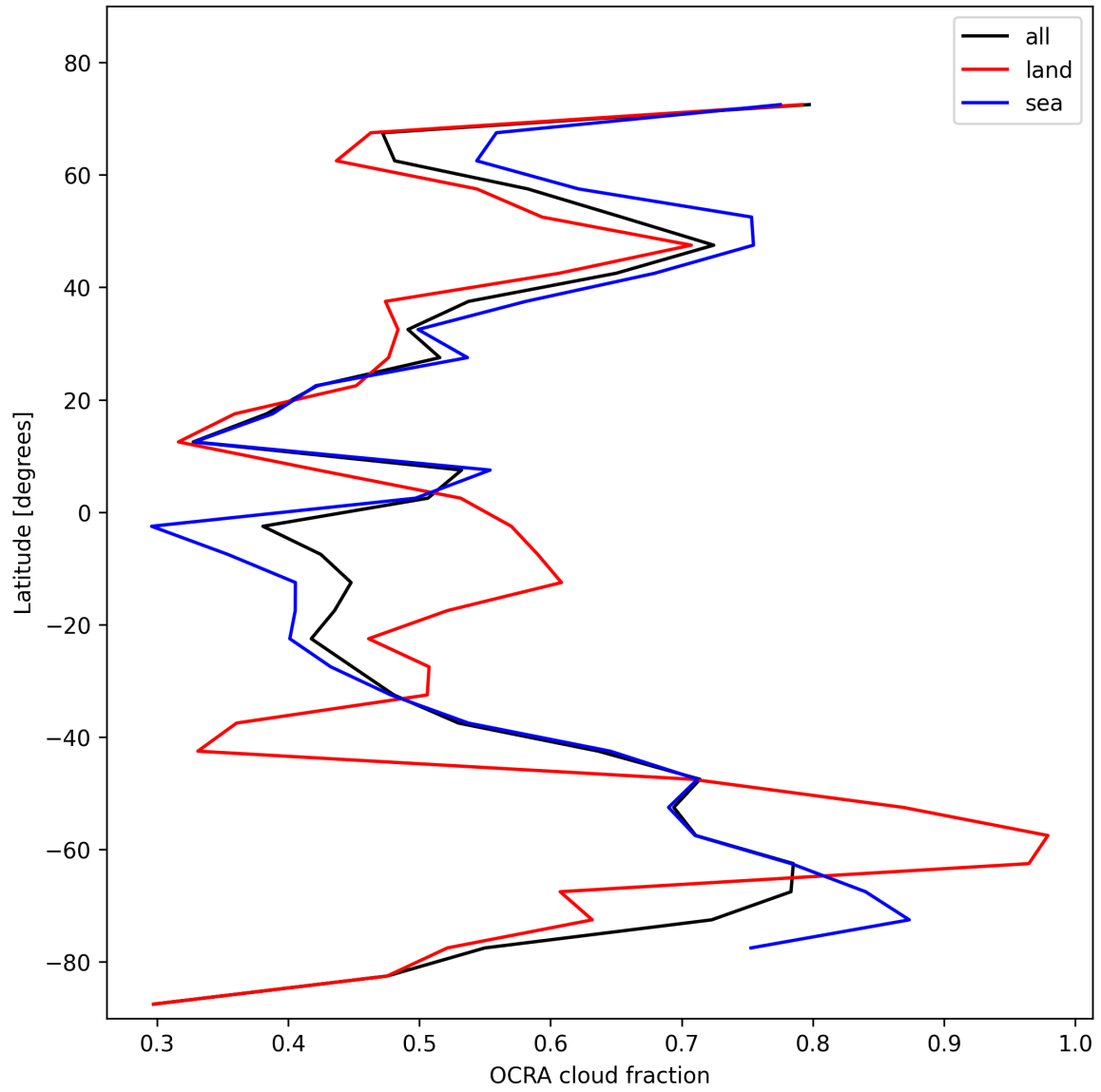
Figure 32: Zonal average of “OCRA cloud fraction” for 2025-01-28 to 2025-01-29.
