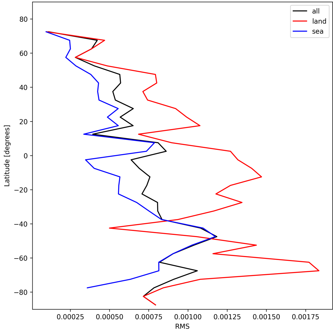
Figure 29: Zonal average of “RMS” for 2025-01-28 to 2025-01-29.
