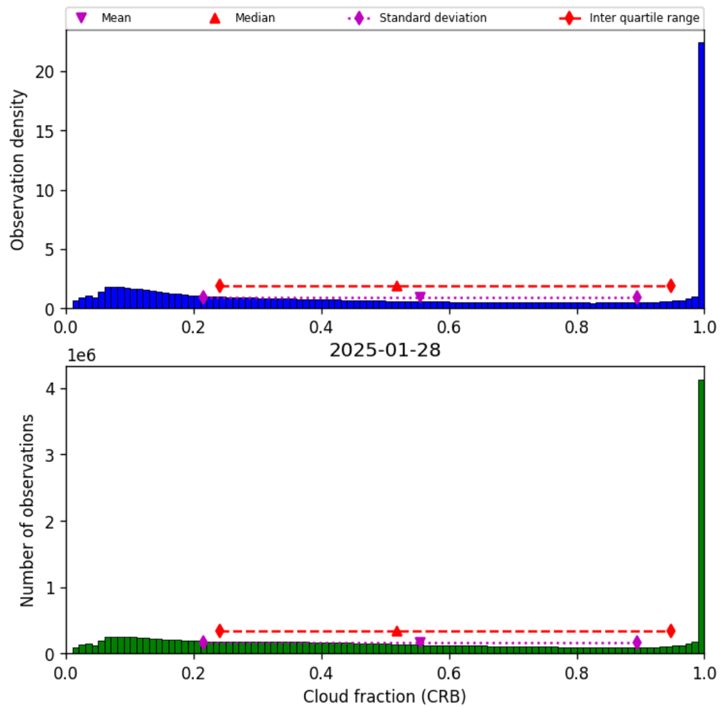
Figure 40: Histogram of “Cloud fraction (CRB)” for 2025-01-28 to 2025-01-29
