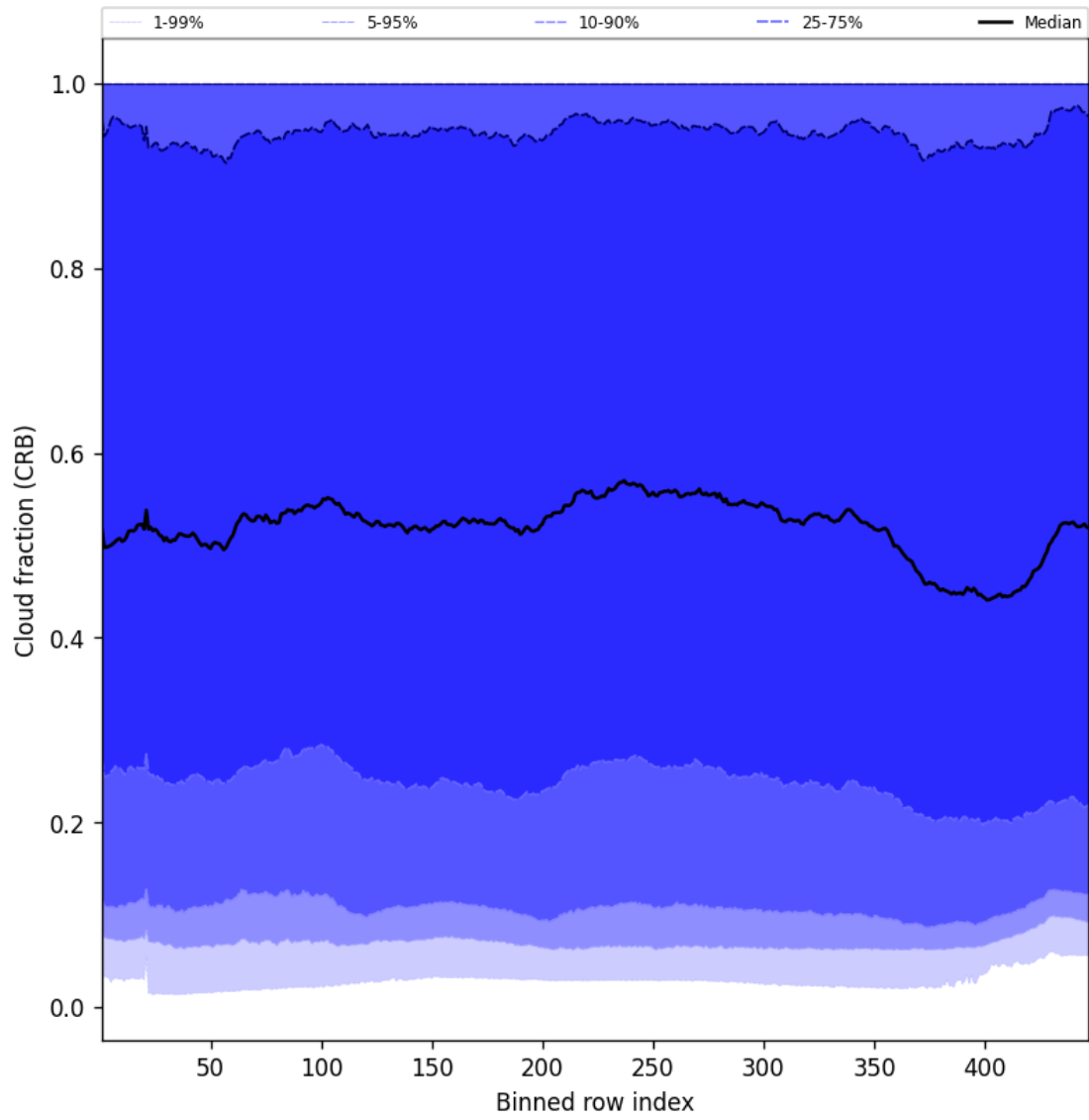
Figure 56: Along track statistics of “Cloud fraction (CRB)” for 2025-01-28 to 2025-01-29
