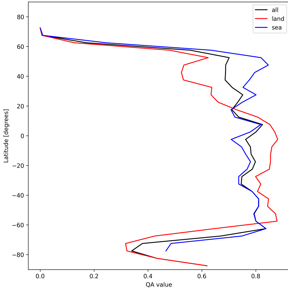
Figure 20: Zonal average of “QA value” for 2025-01-28 to 2025-01-29.
