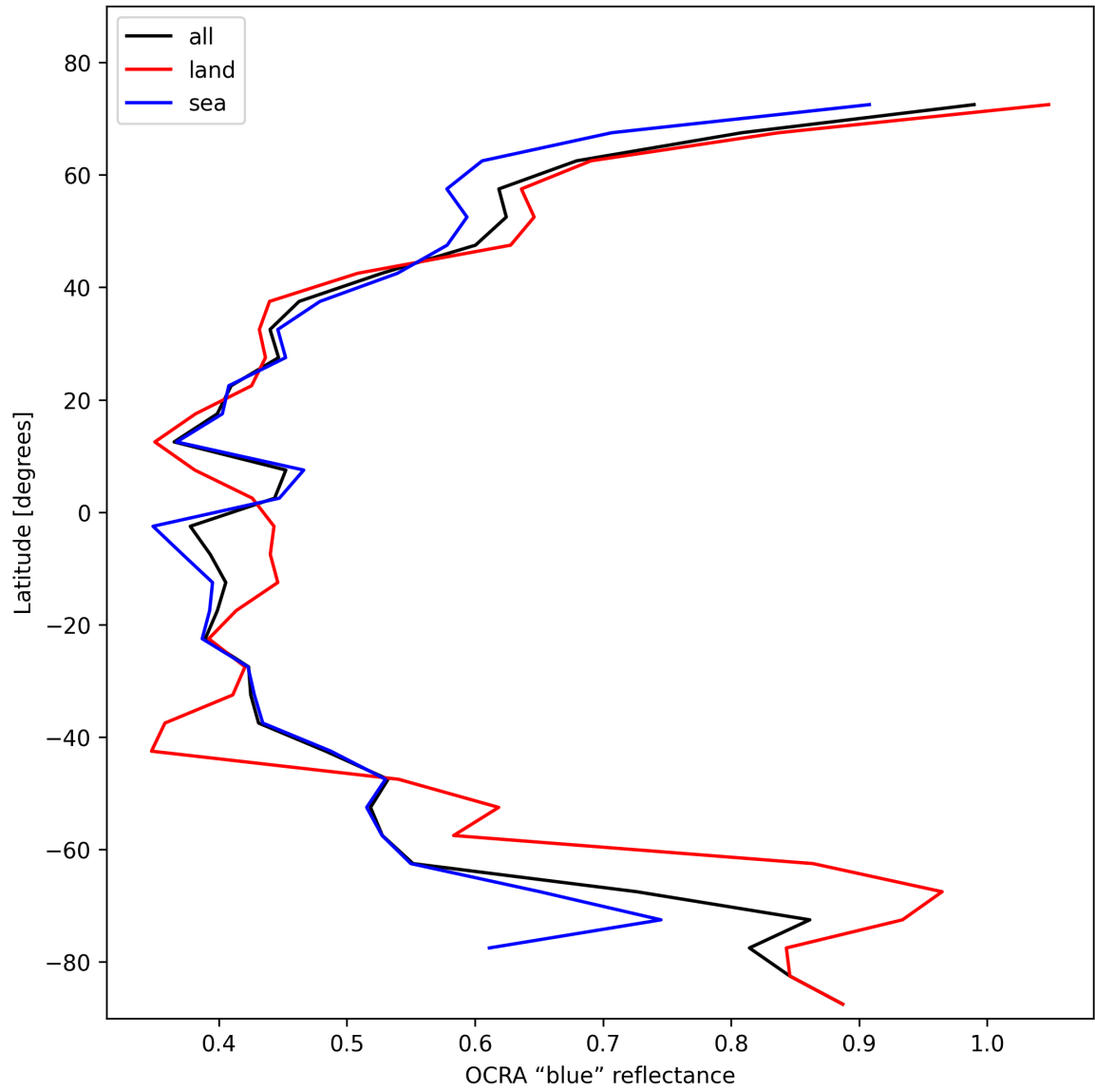
Figure 33: Zonal average of “OCRA “blue” reflectance” for 2025-01-28 to 2025-01-29.
