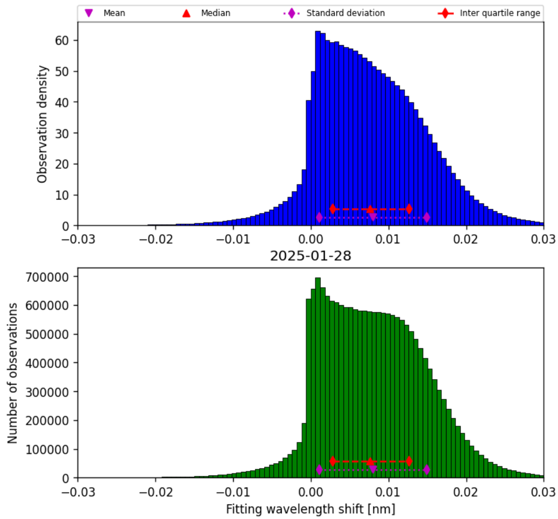
Figure 47: Histogram of “Fitting wavelength shift” for 2025-01-28 to 2025-01-29
