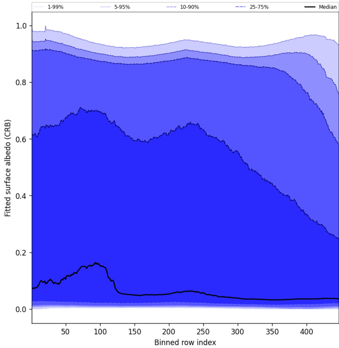
Figure 60: Along track statistics of “Fitted surface albedo (CRB)” for 2025-01-28 to 2025-01-29
