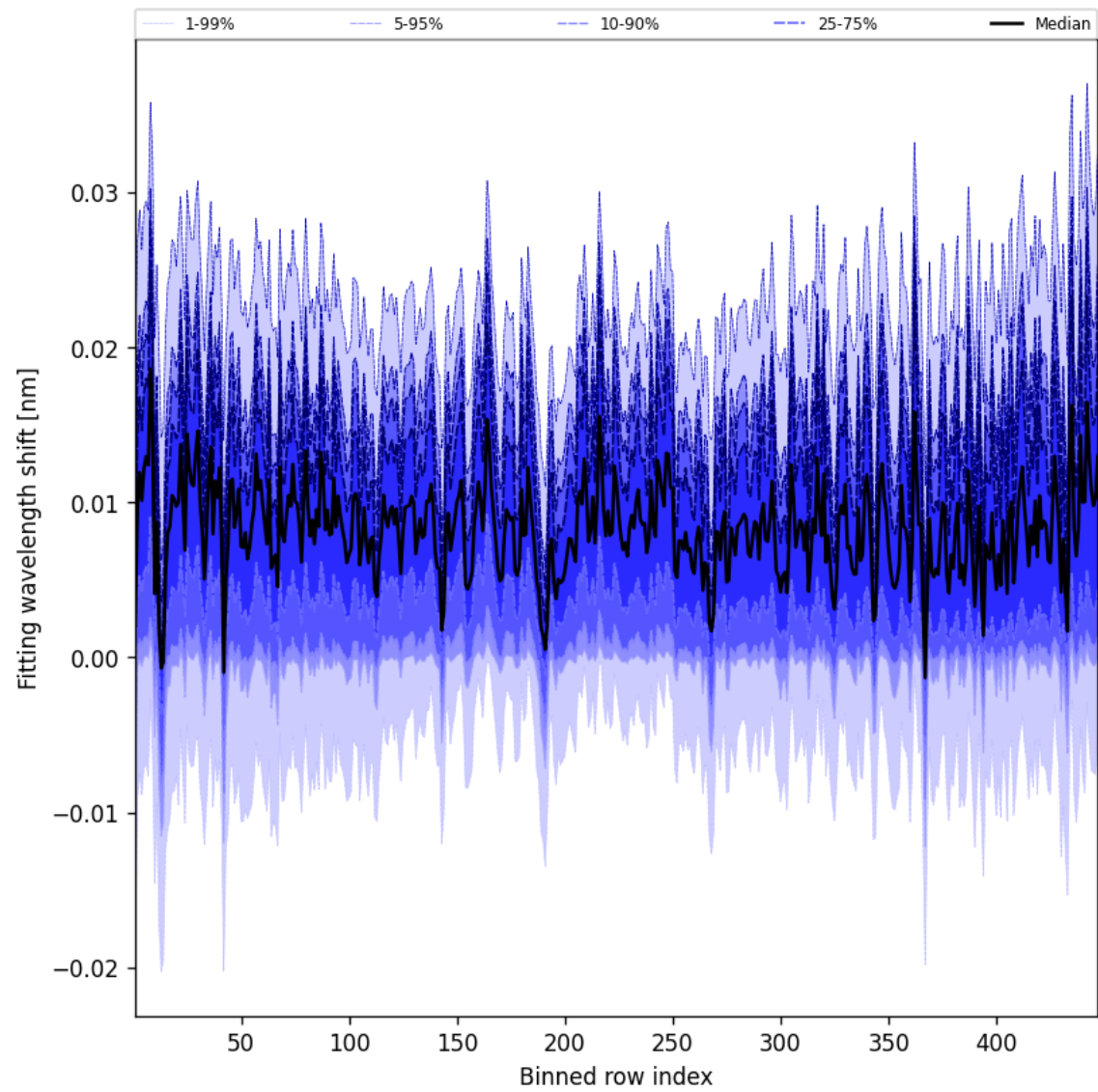
Figure 63: Along track statistics of “Fitting wavelength shift” for 2025-01-28 to 2025-01-29
