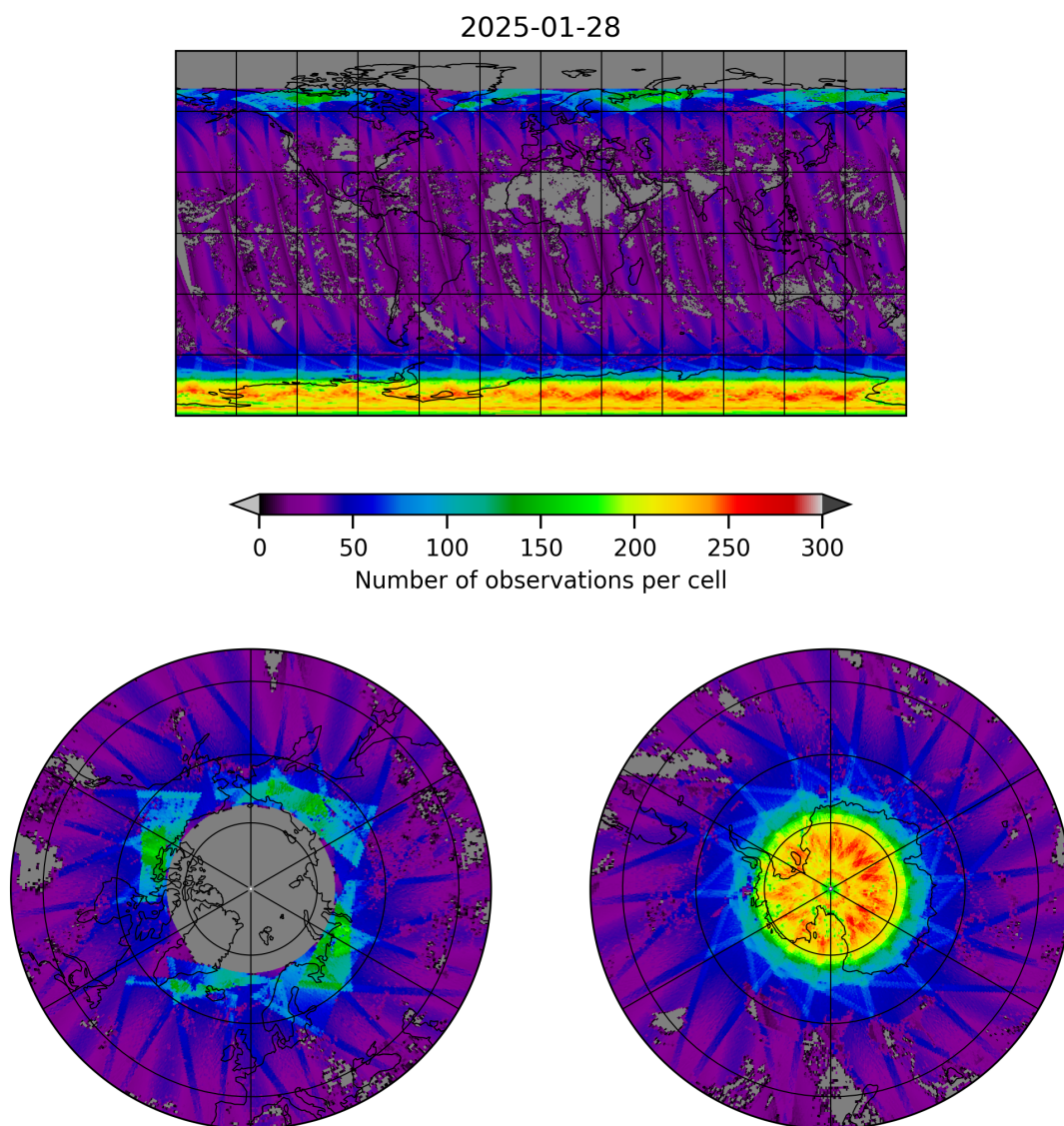
Figure 19: Map of the number of observations for 2025-01-28 to 2025-01-29
