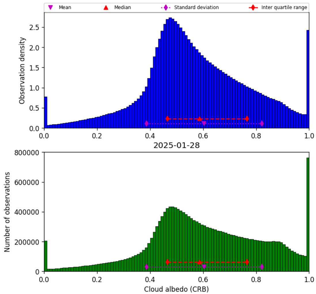
Figure 42: Histogram of “Cloud albedo (CRB)” for 2025-01-28 to 2025-01-29
