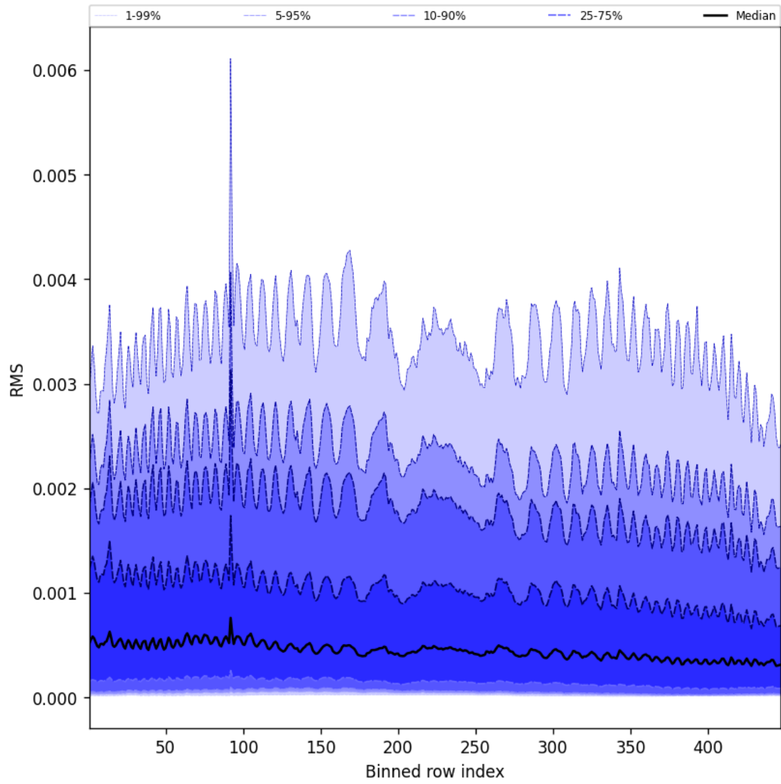
Figure 61: Along track statistics of “RMS” for 2025-01-28 to 2025-01-29
