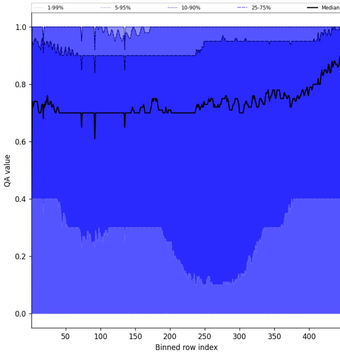
Figure 52: Along track statistics of “QA value” for 2025-01-28 to 2025-01-29
