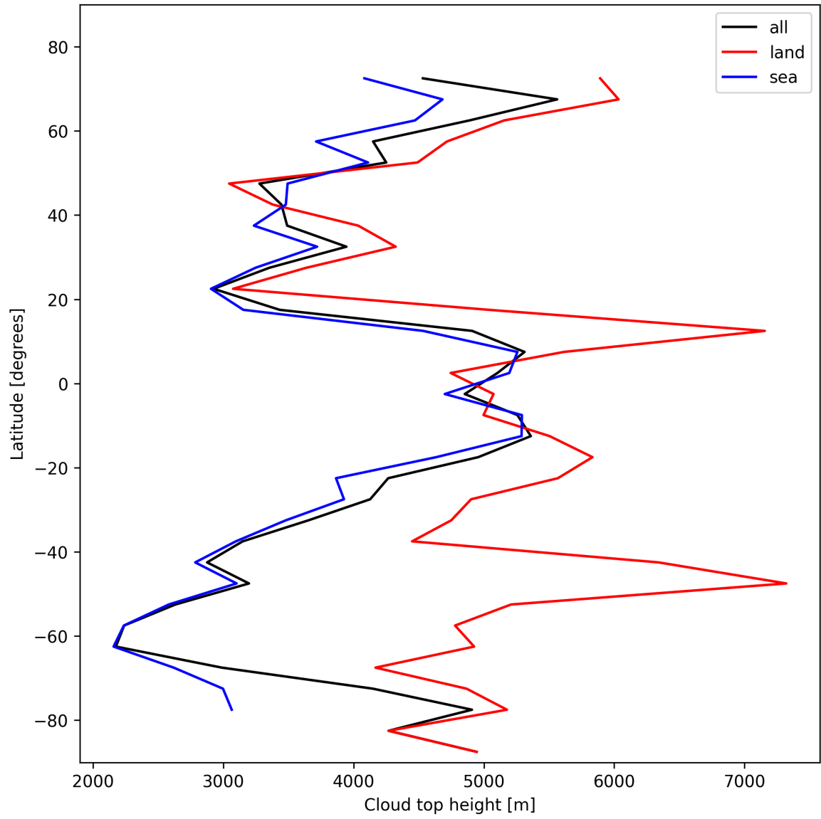
Figure 22: Zonal average of “Cloud top height” for 2025-01-28 to 2025-01-29.
