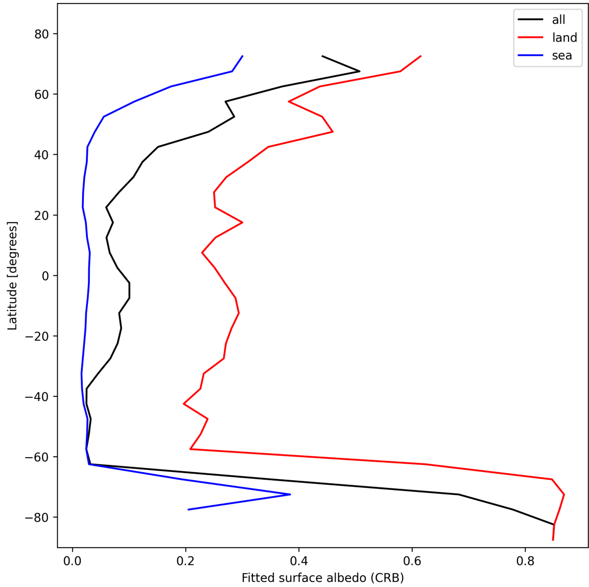
Figure 28: Zonal average of “Fitted surface albedo (CRB)” for 2025-01-28 to 2025-01-29.
