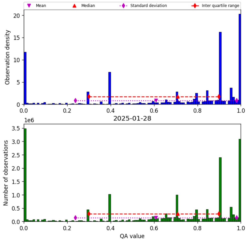
Figure 36: Histogram of “QA value” for 2025-01-28 to 2025-01-29
