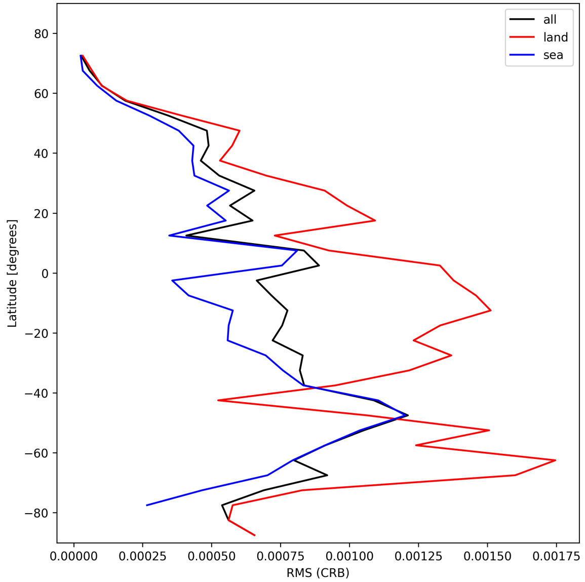
Figure 30: Zonal average of “RMS (CRB)” for 2025-01-28 to 2025-01-29.
