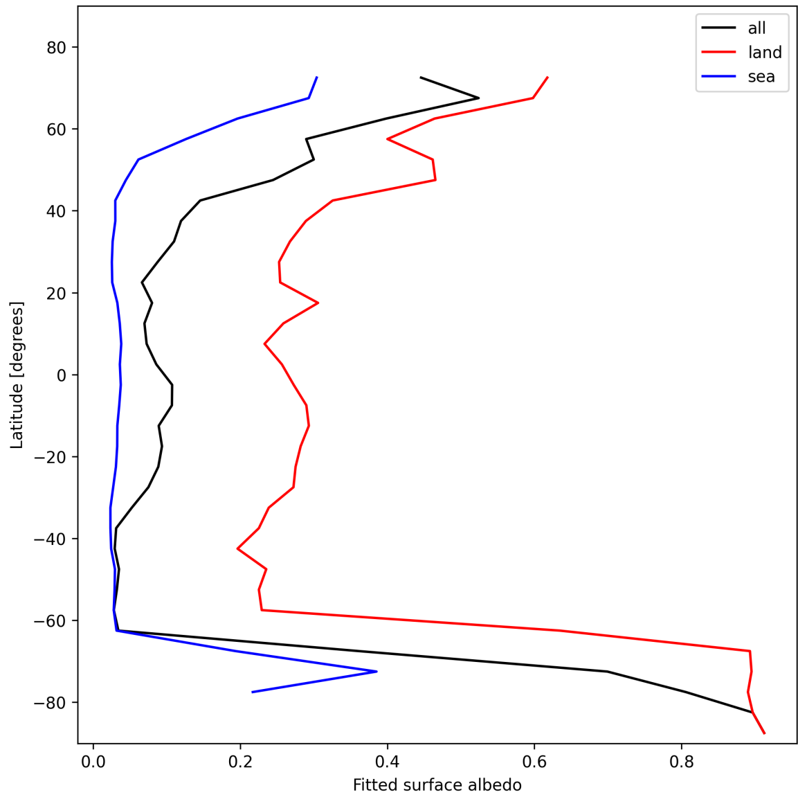
Figure 27: Zonal average of “Fitted surface albedo” for 2025-01-28 to 2025-01-29.
