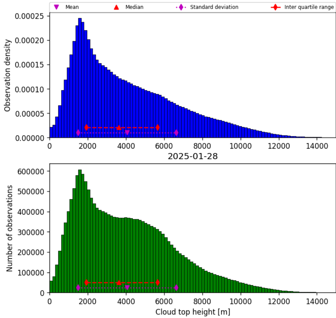
Figure 38: Histogram of “Cloud top height” for 2025-01-28 to 2025-01-29
