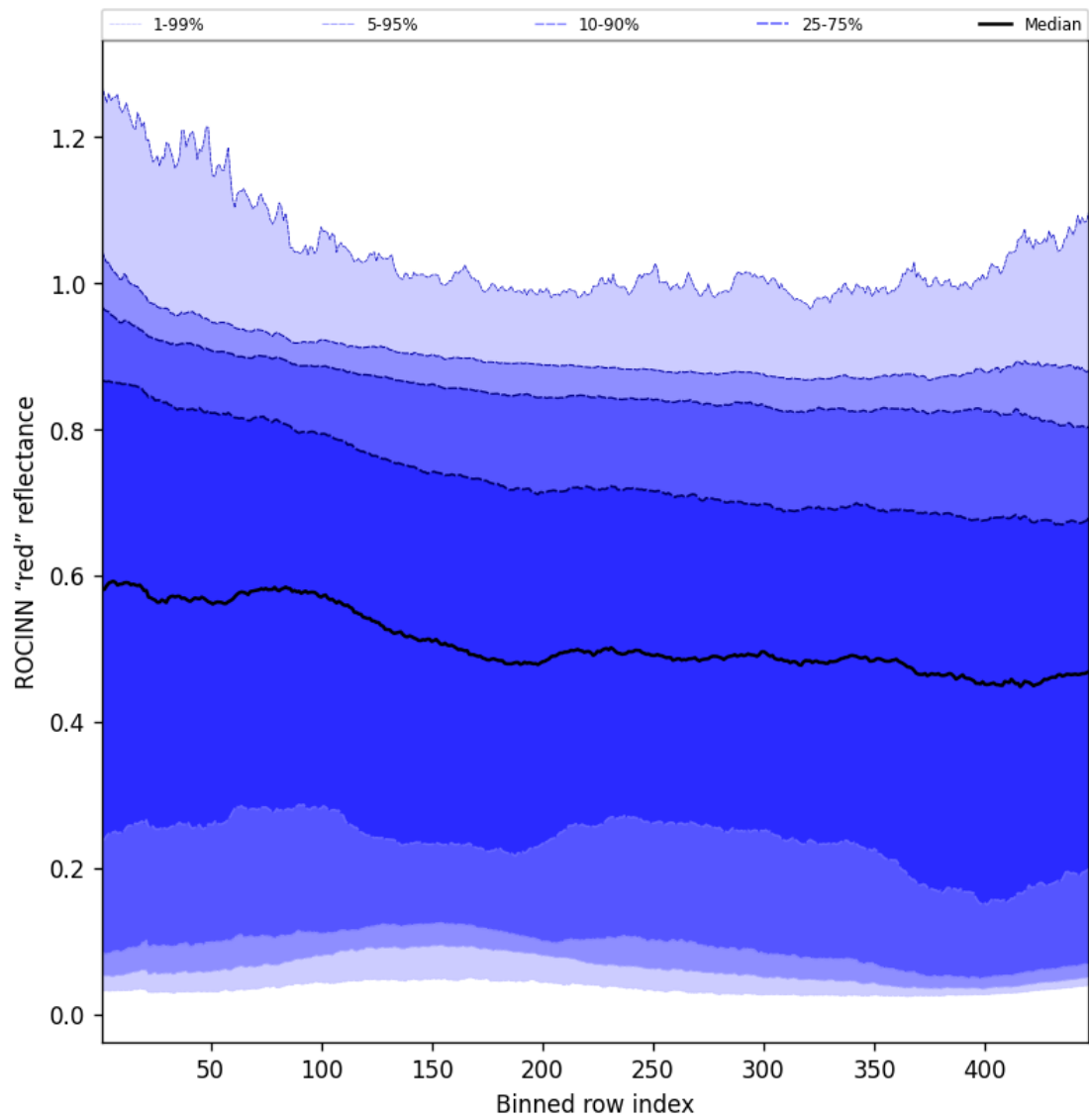
Figure 67: Along track statistics of “ROCINN “red” reflectance” for 2025-01-28 to 2025-01-29
