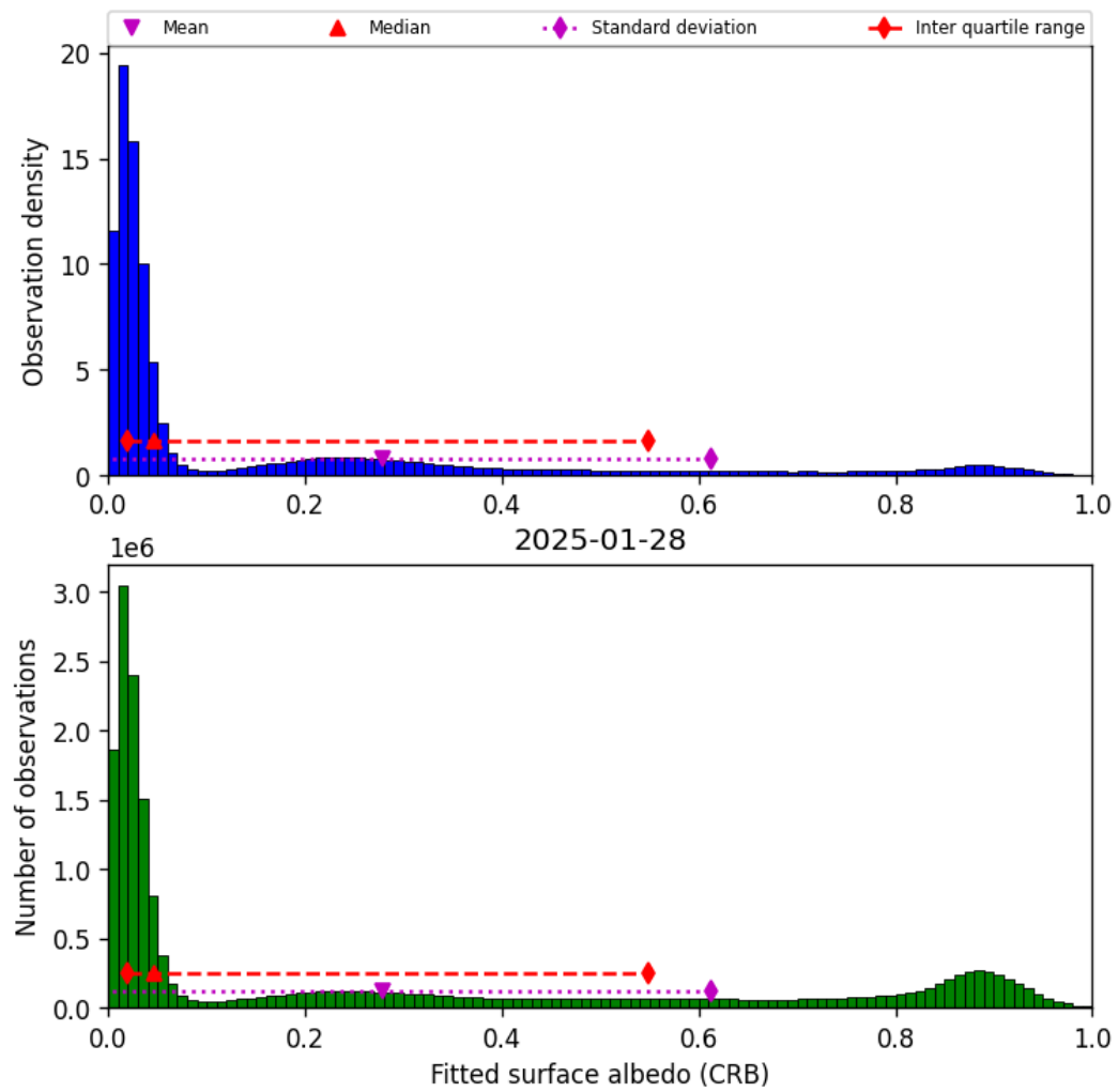
Figure 44: Histogram of “Fitted surface albedo (CRB)” for 2025-01-28 to 2025-01-29
