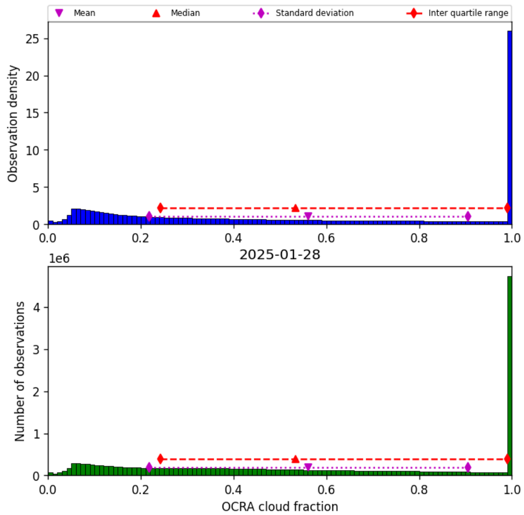
Figure 48: Histogram of “OCRA cloud fraction” for 2025-01-28 to 2025-01-29
