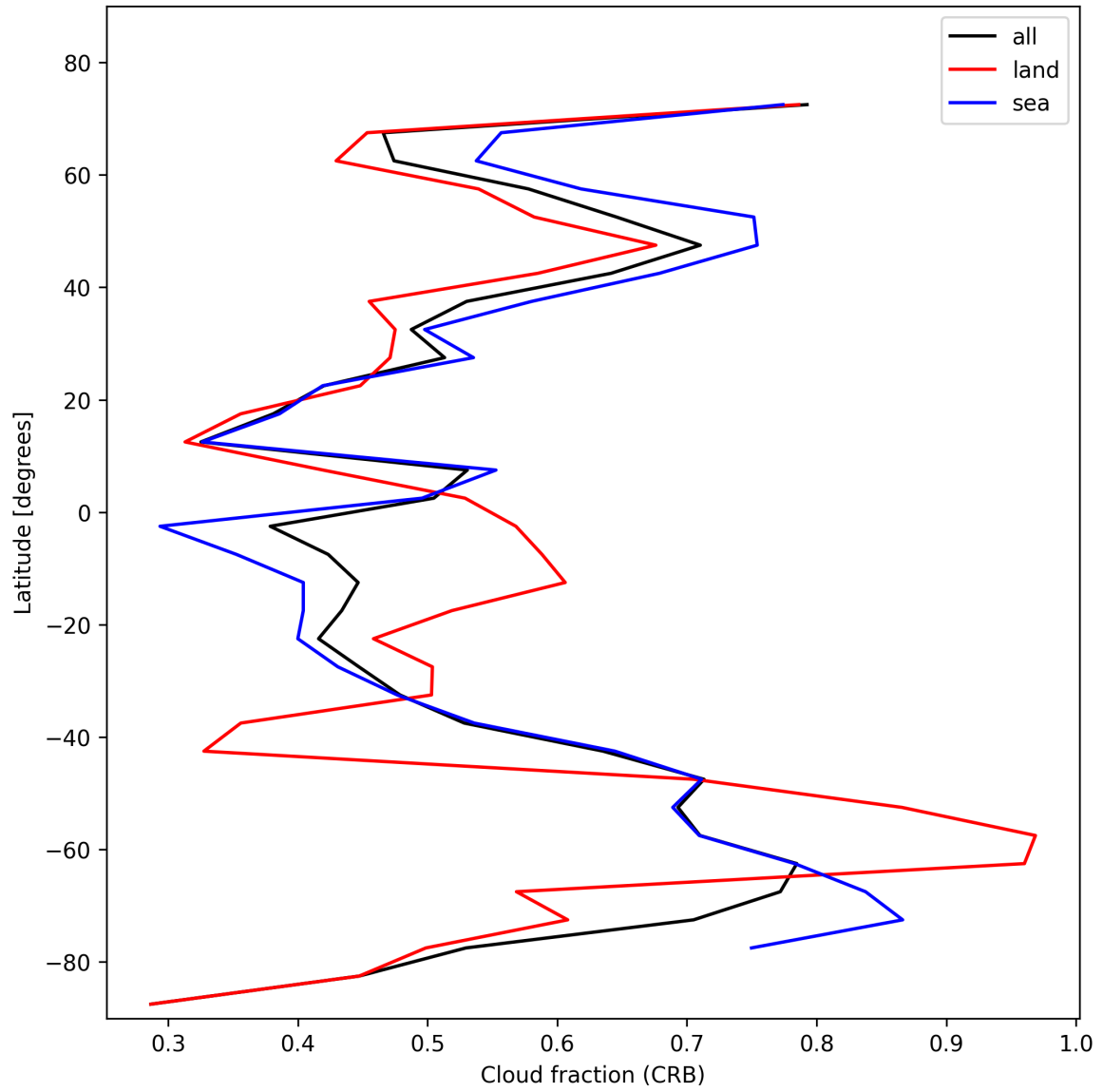
Figure 24: Zonal average of “Cloud fraction (CRB)” for 2025-01-28 to 2025-01-29.
