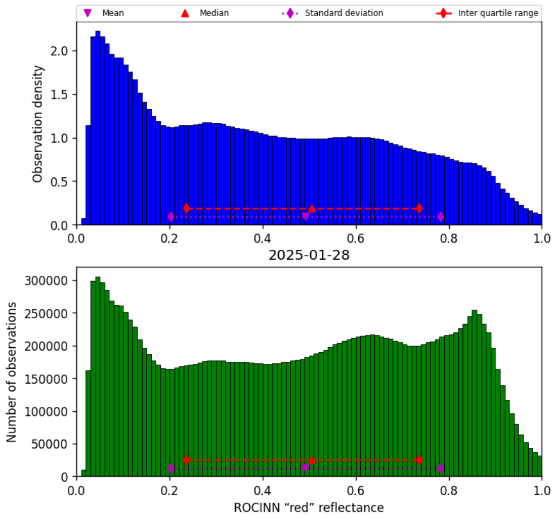
Figure 51: Histogram of “ROCINN “red” reflectance” for 2025-01-28 to 2025-01-29
