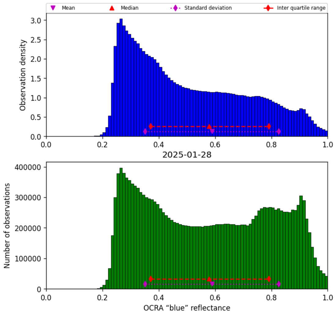
Figure 49: Histogram of "OCRA "blue" reflectance" for 2025-01-28 to 2025-01-29
