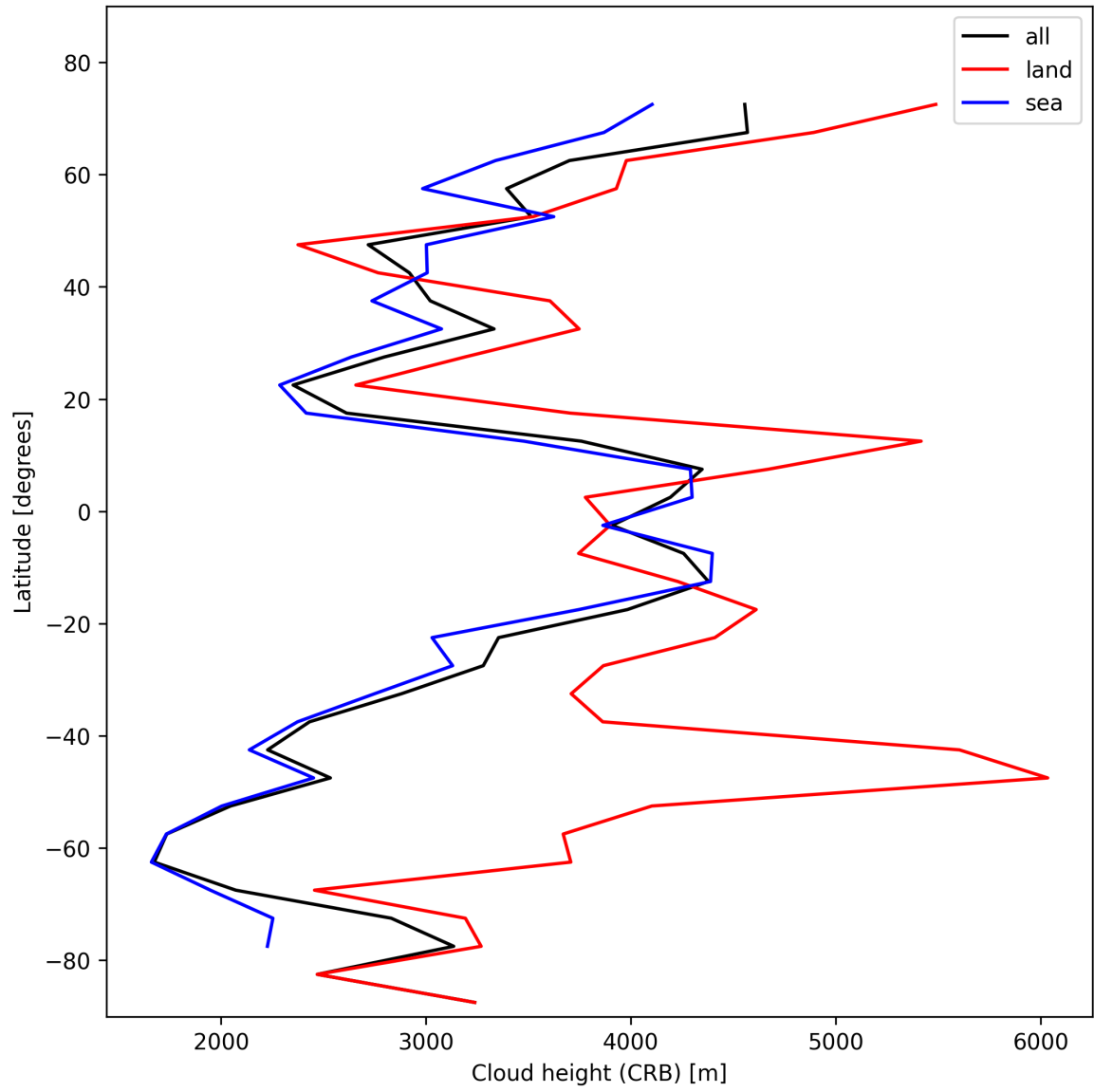
Figure 25: Zonal average of “Cloud height (CRB)” for 2025-01-28 to 2025-01-29.
