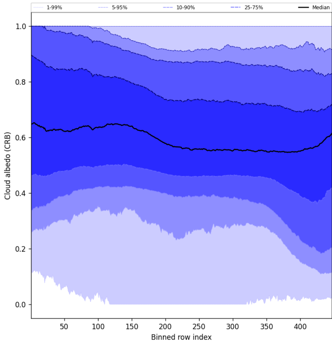
Figure 58: Along track statistics of “Cloud albedo (CRB)” for 2025-01-28 to 2025-01-29
