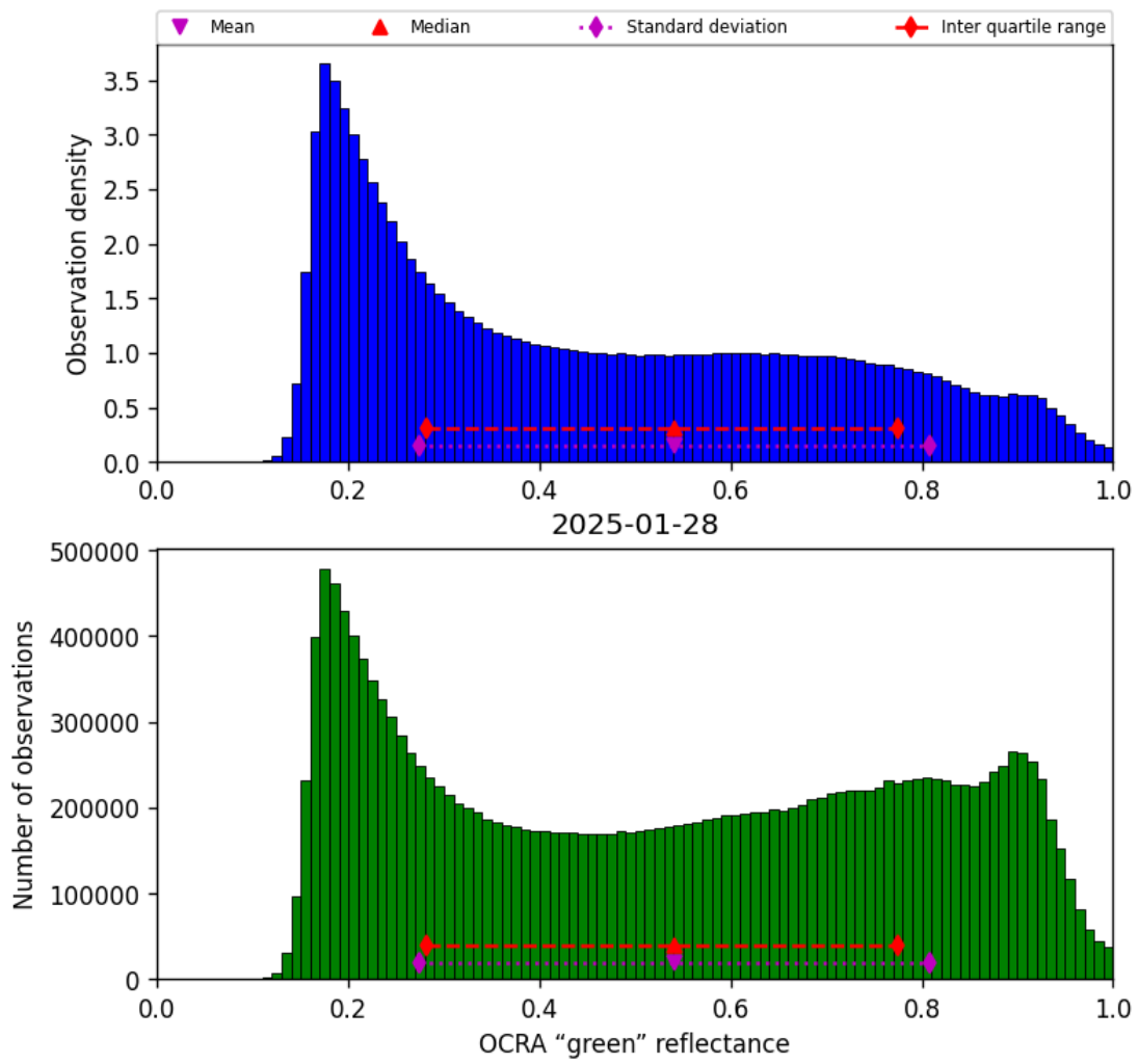
Figure 50: Histogram of “OCRA “green” reflectance” for 2025-01-28 to 2025-01-29
