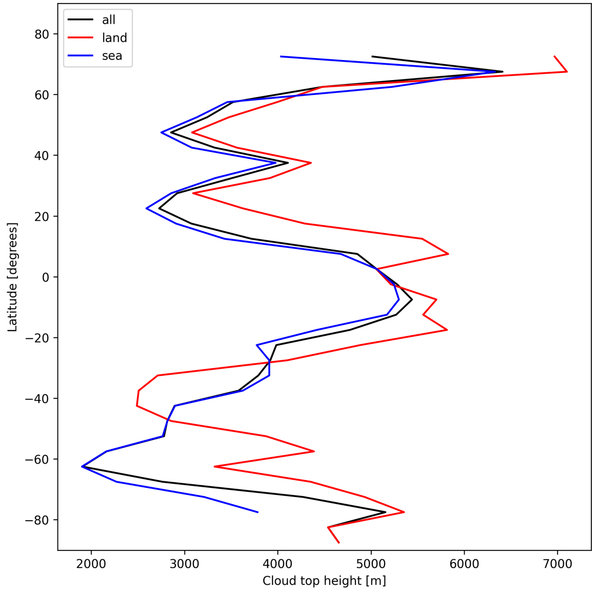
Figure 22: Zonal average of “Cloud top height” for 2025-01-31 to 2025-01-31.
