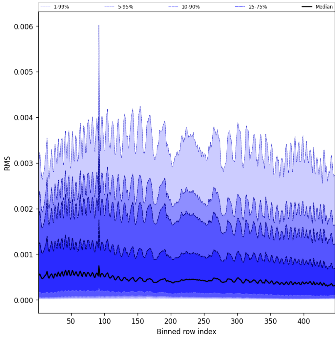
Figure 61: Along track statistics of “RMS” for 2025-01-31 to 2025-01-31
