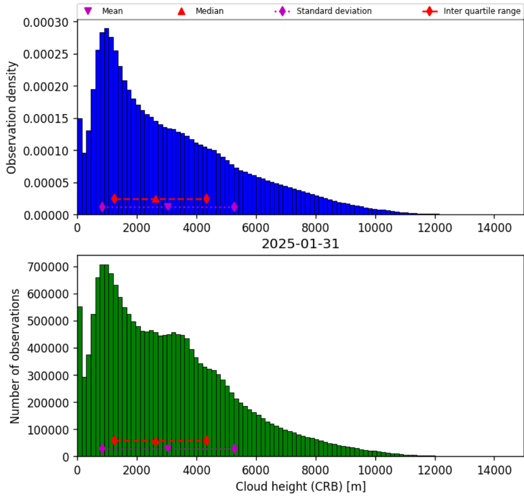
Figure 41: Histogram of “Cloud height (CRB)” for 2025-01-31 to 2025-01-31
