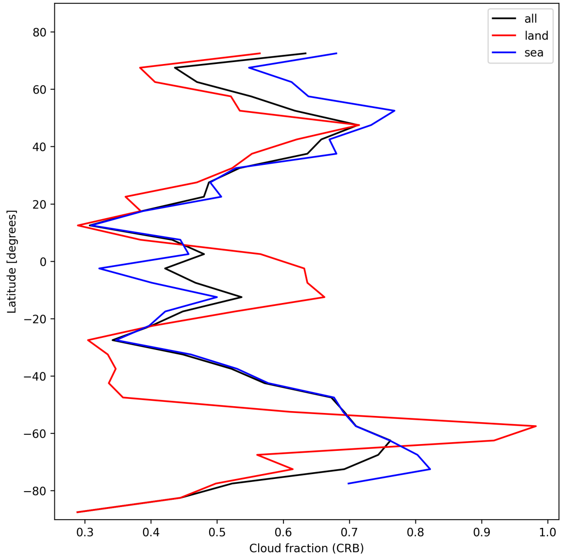
Figure 24: Zonal average of “Cloud fraction (CRB)” for 2025-01-31 to 2025-01-31.
