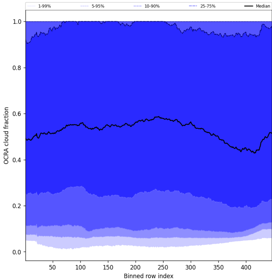
Figure 64: Along track statistics of “OCRA cloud fraction” for 2025-01-31 to 2025-01-31
