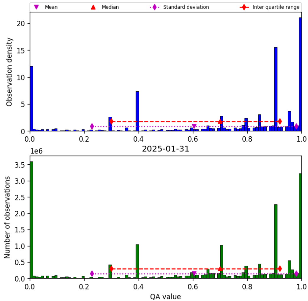
Figure 36: Histogram of “QA value” for 2025-01-31 to 2025-01-31
