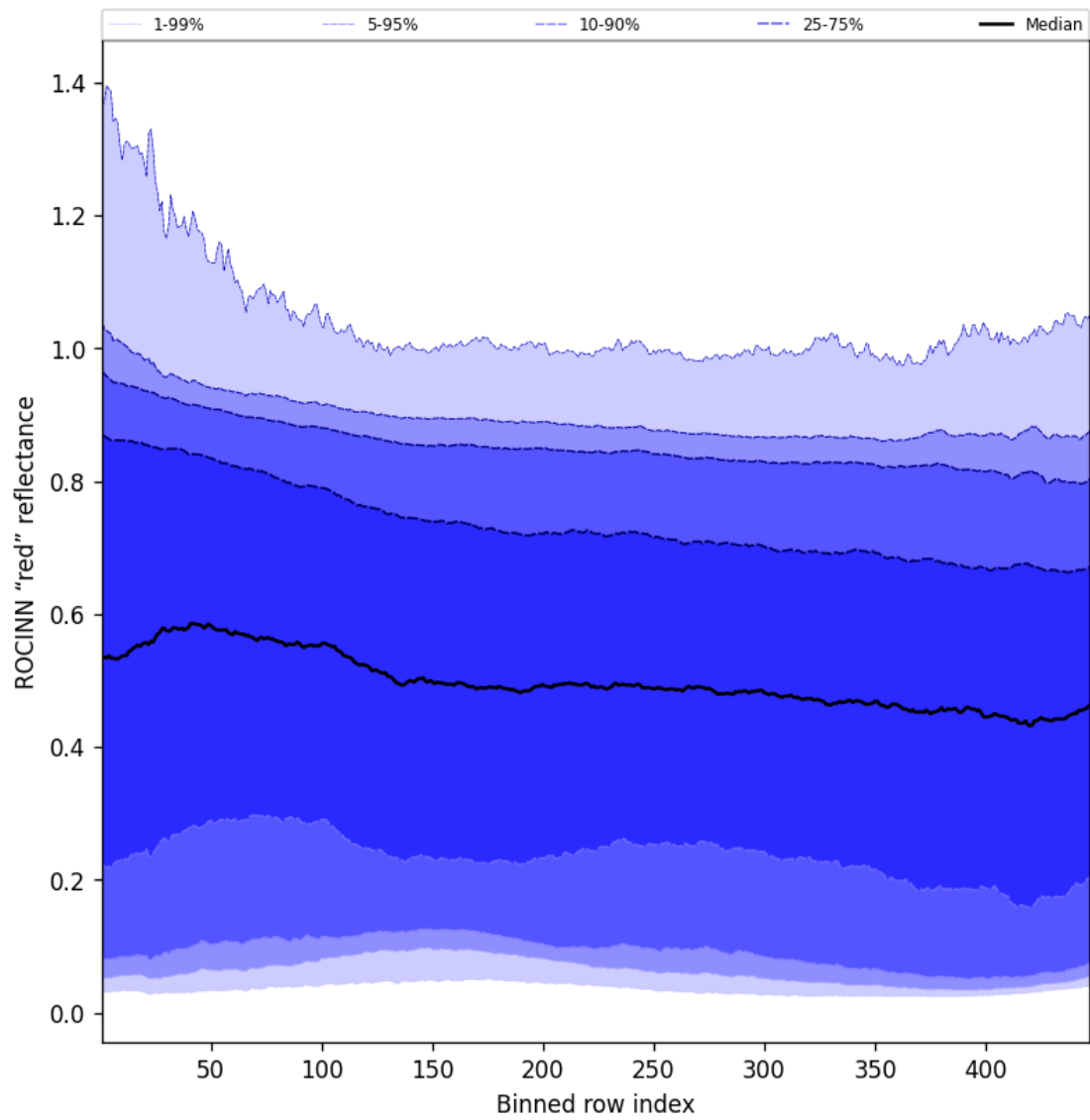
Figure 67: Along track statistics of “ROCINN “red” reflectance” for 2025-01-31 to 2025-01-31
