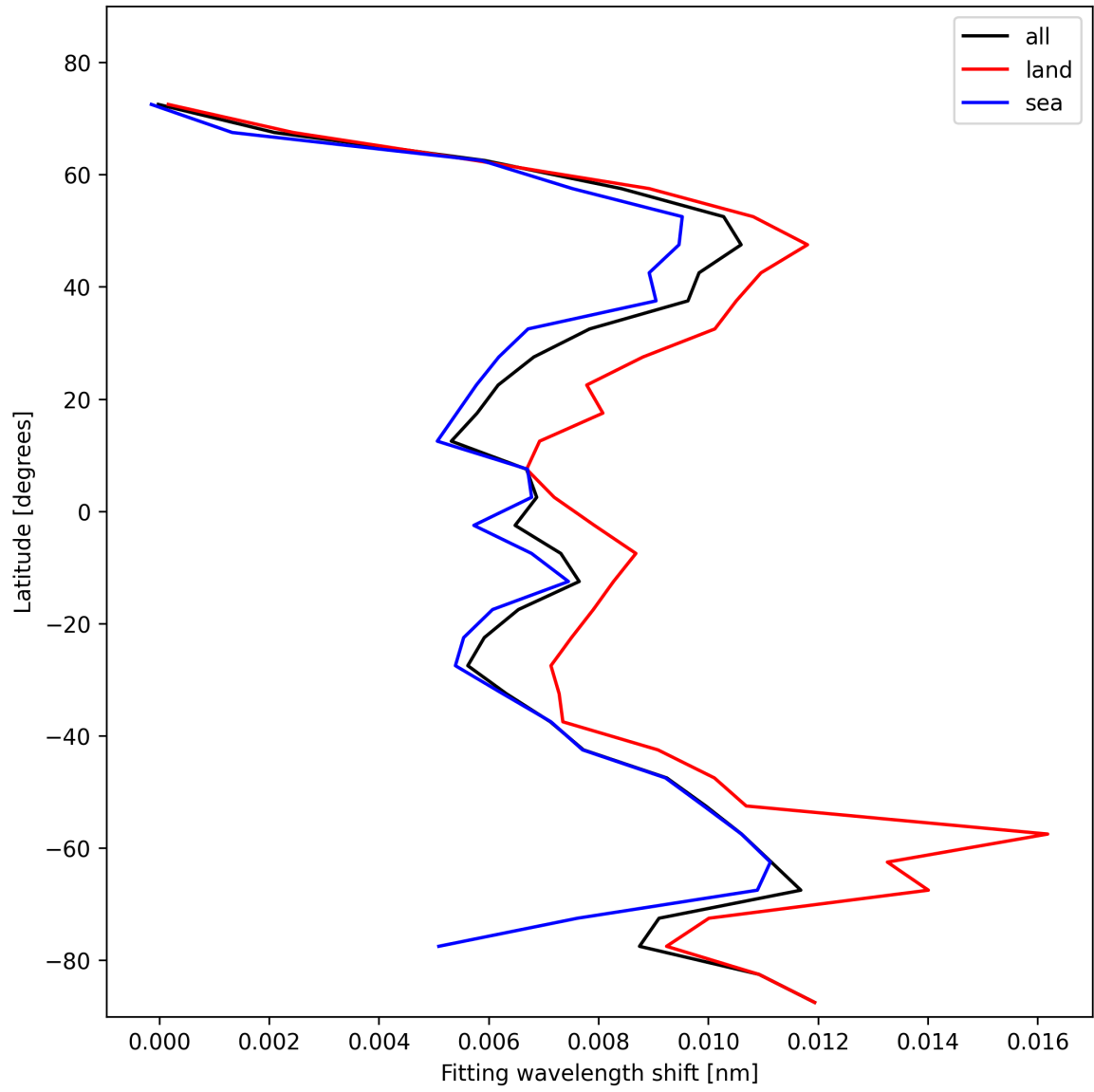
Figure 31: Zonal average of “Fitting wavelength shift” for 2025-01-31 to 2025-01-31.
