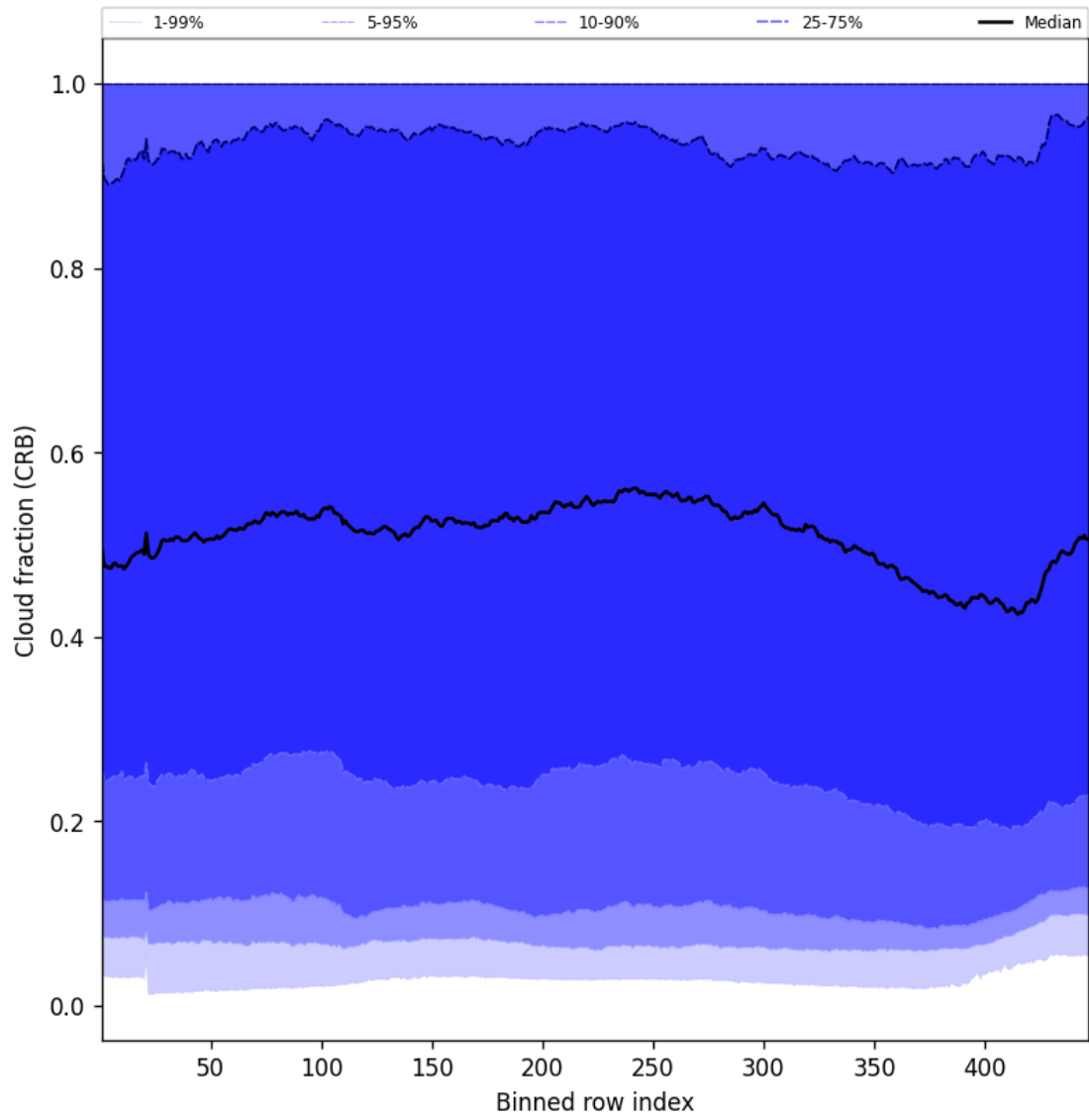
Figure 56: Along track statistics of “Cloud fraction (CRB)” for 2025-01-31 to 2025-01-31
