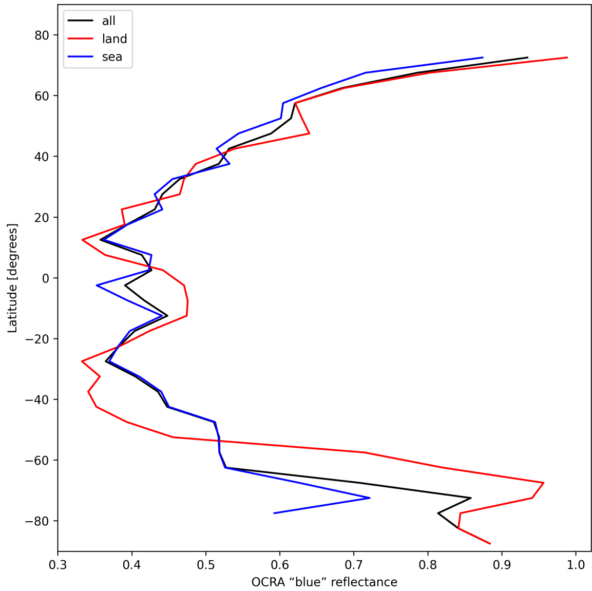
Figure 33: Zonal average of “OCRA “blue” reflectance” for 2025-01-31 to 2025-01-31.
