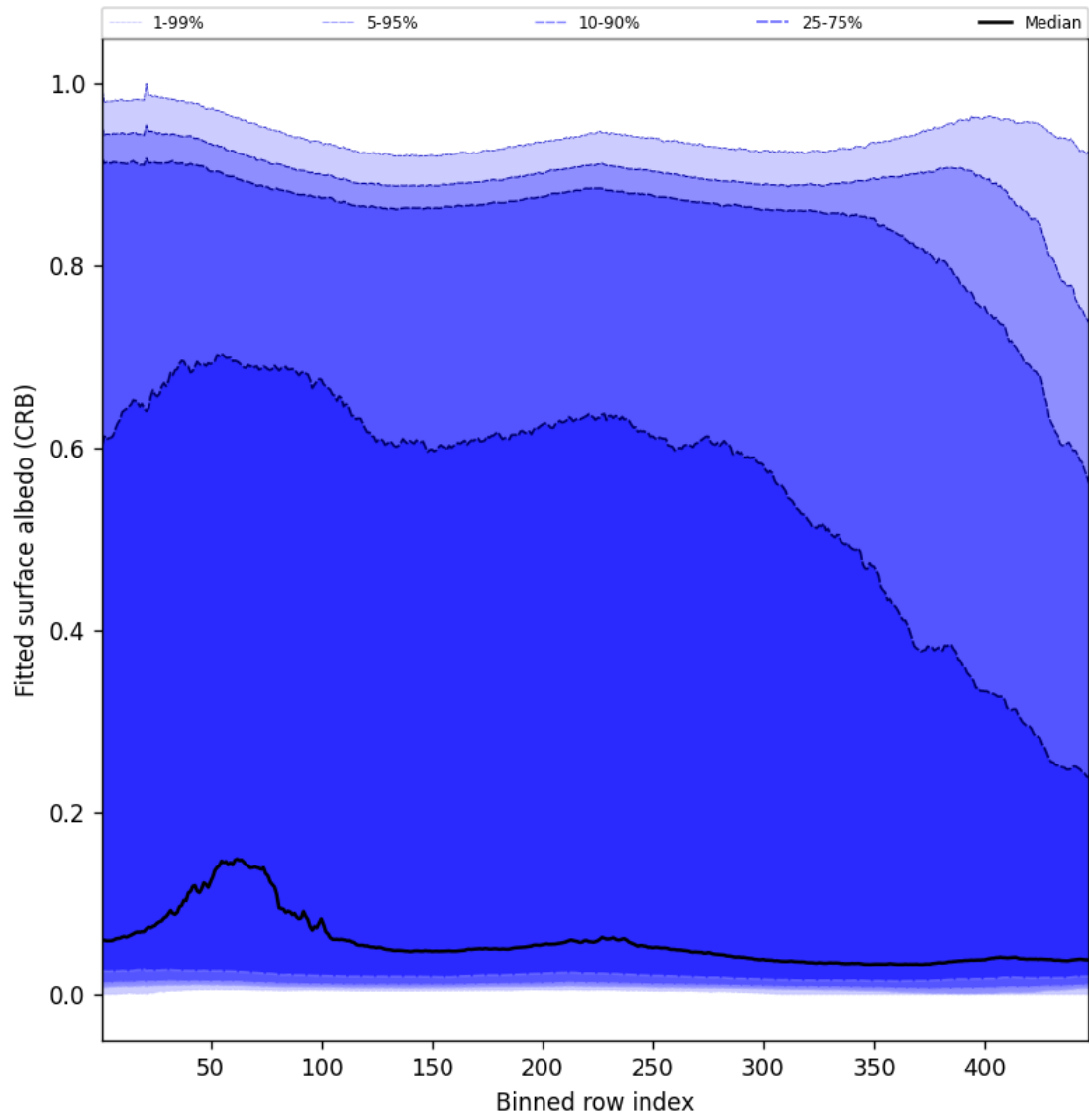
Figure 60: Along track statistics of “Fitted surface albedo (CRB)” for 2025-01-31 to 2025-01-31
