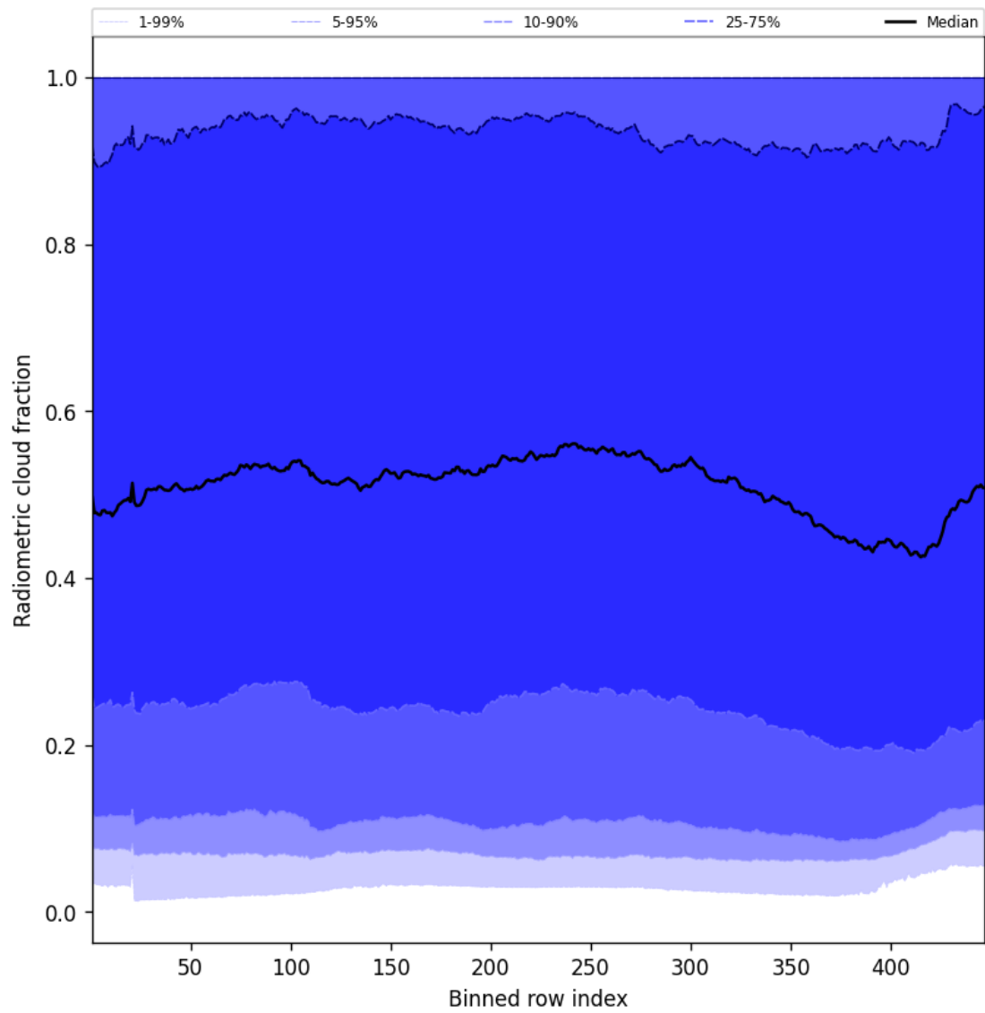
Figure 53: Along track statistics of “Radiometric cloud fraction” for 2025-01-31 to 2025-01-31
