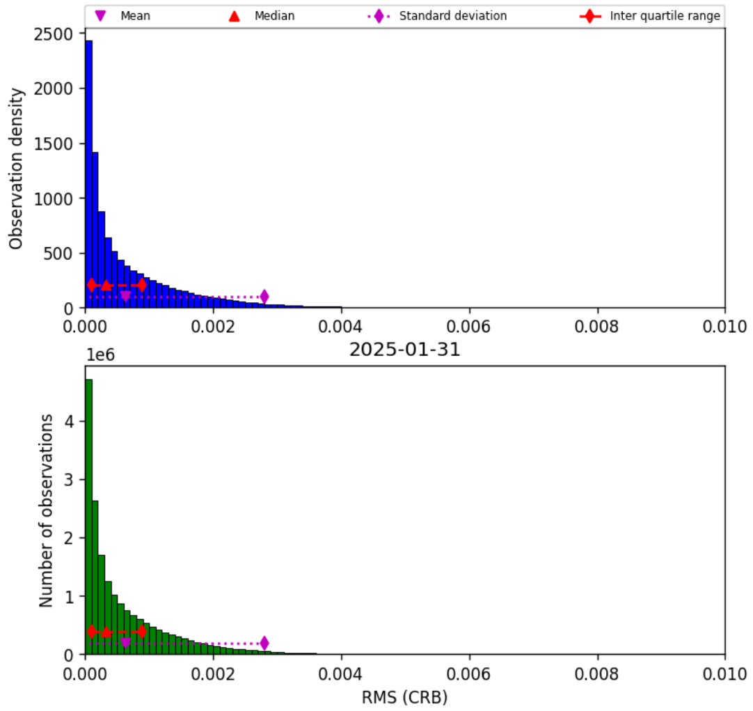
Figure 46: Histogram of “RMS (CRB)” for 2025-01-31 to 2025-01-31
