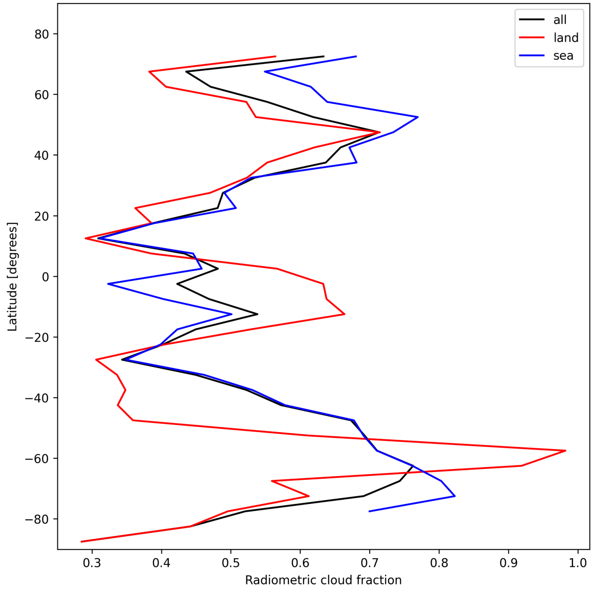
Figure 21: Zonal average of “Radiometric cloud fraction” for 2025-01-31 to 2025-01-31.
