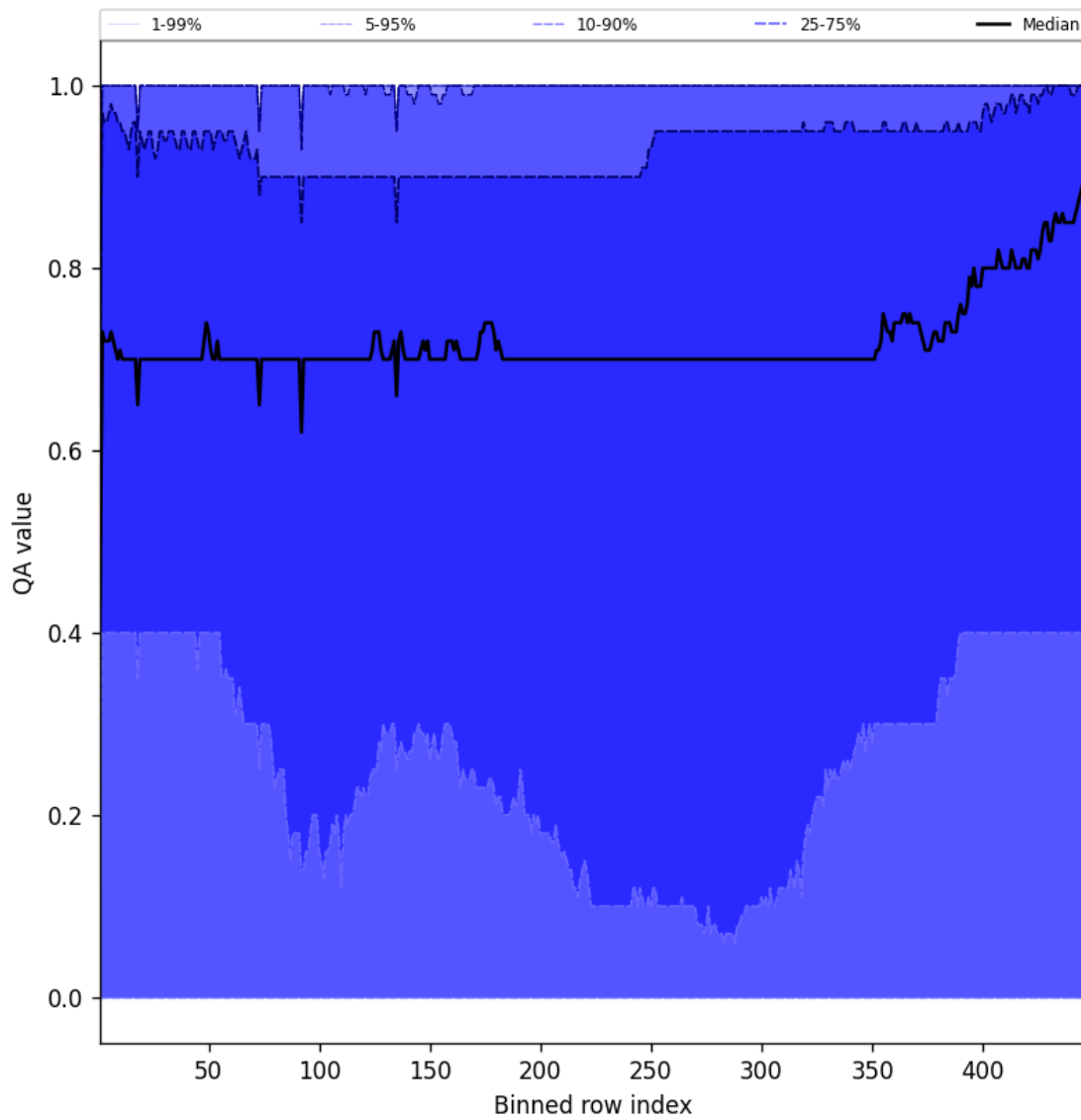
Figure 52: Along track statistics of “QA value” for 2025-01-31 to 2025-01-31
