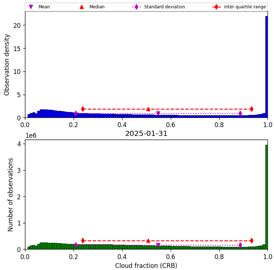
Figure 40: Histogram of “Cloud fraction (CRB)” for 2025-01-31 to 2025-01-31
