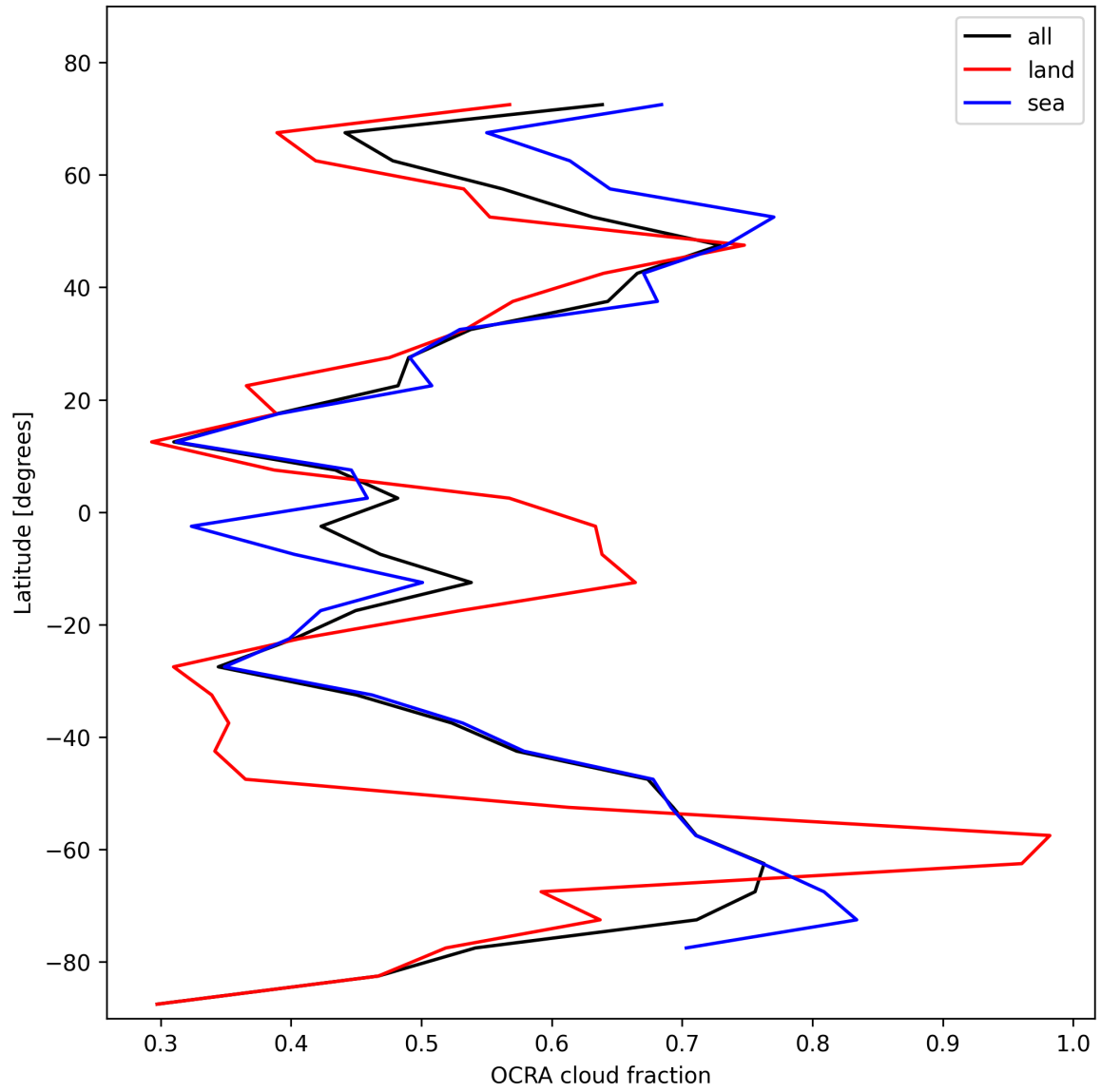
Figure 32: Zonal average of “OCRA cloud fraction” for 2025-01-31 to 2025-01-31.
