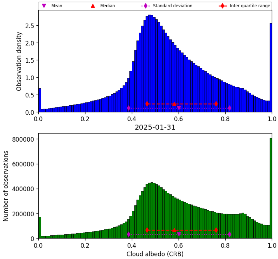
Figure 42: Histogram of “Cloud albedo (CRB)” for 2025-01-31 to 2025-01-31
