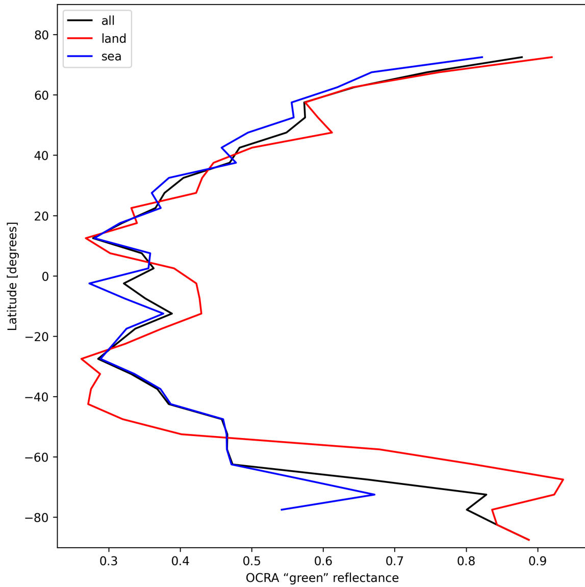
Figure 34: Zonal average of "OCRA "green" reflectance" for 2025-01-31 to 2025-01-31.
