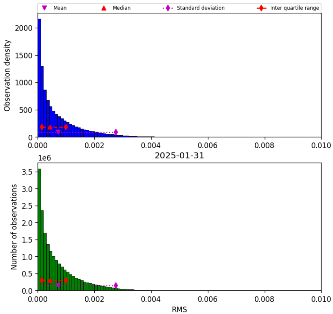
Figure 45: Histogram of “RMS” for 2025-01-31 to 2025-01-31
