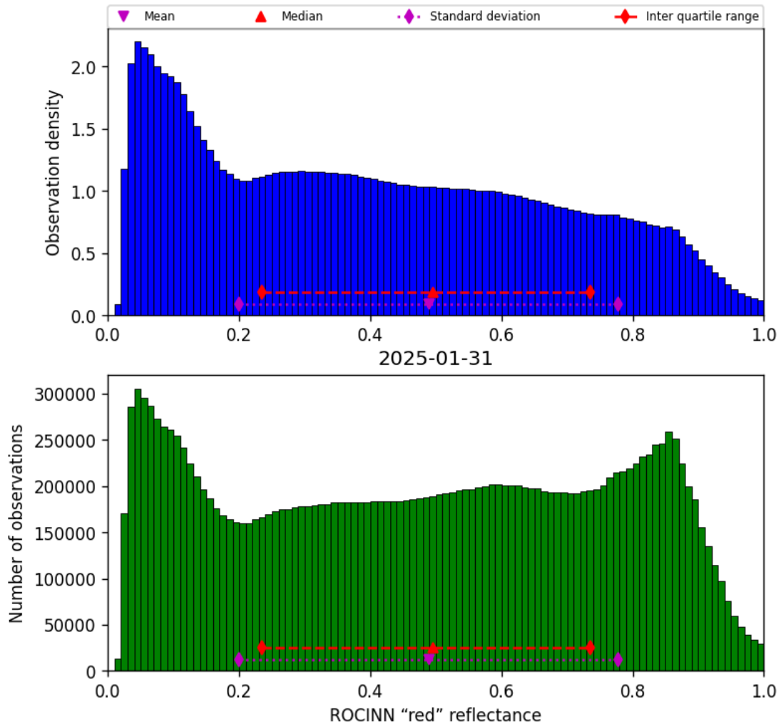
Figure 51: Histogram of “ROCINN “red” reflectance” for 2025-01-31 to 2025-01-31
