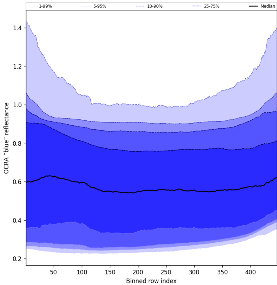
Figure 65: Along track statistics of "OCRA "blue" reflectance" for 2025-01-31 to 2025-01-31
