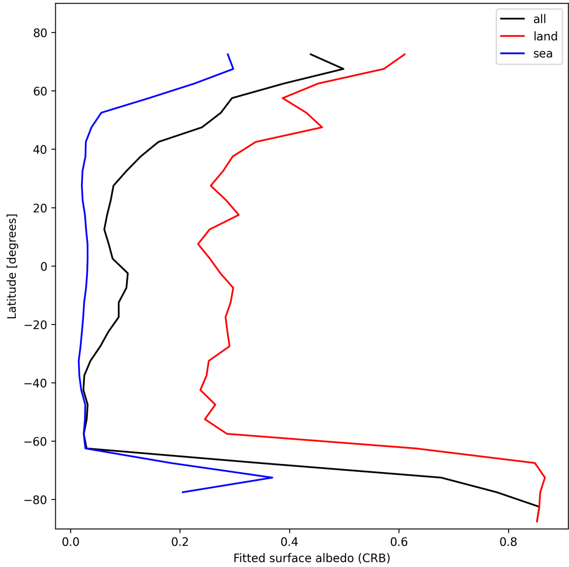
Figure 28: Zonal average of “Fitted surface albedo (CRB)” for 2025-01-31 to 2025-01-31.
