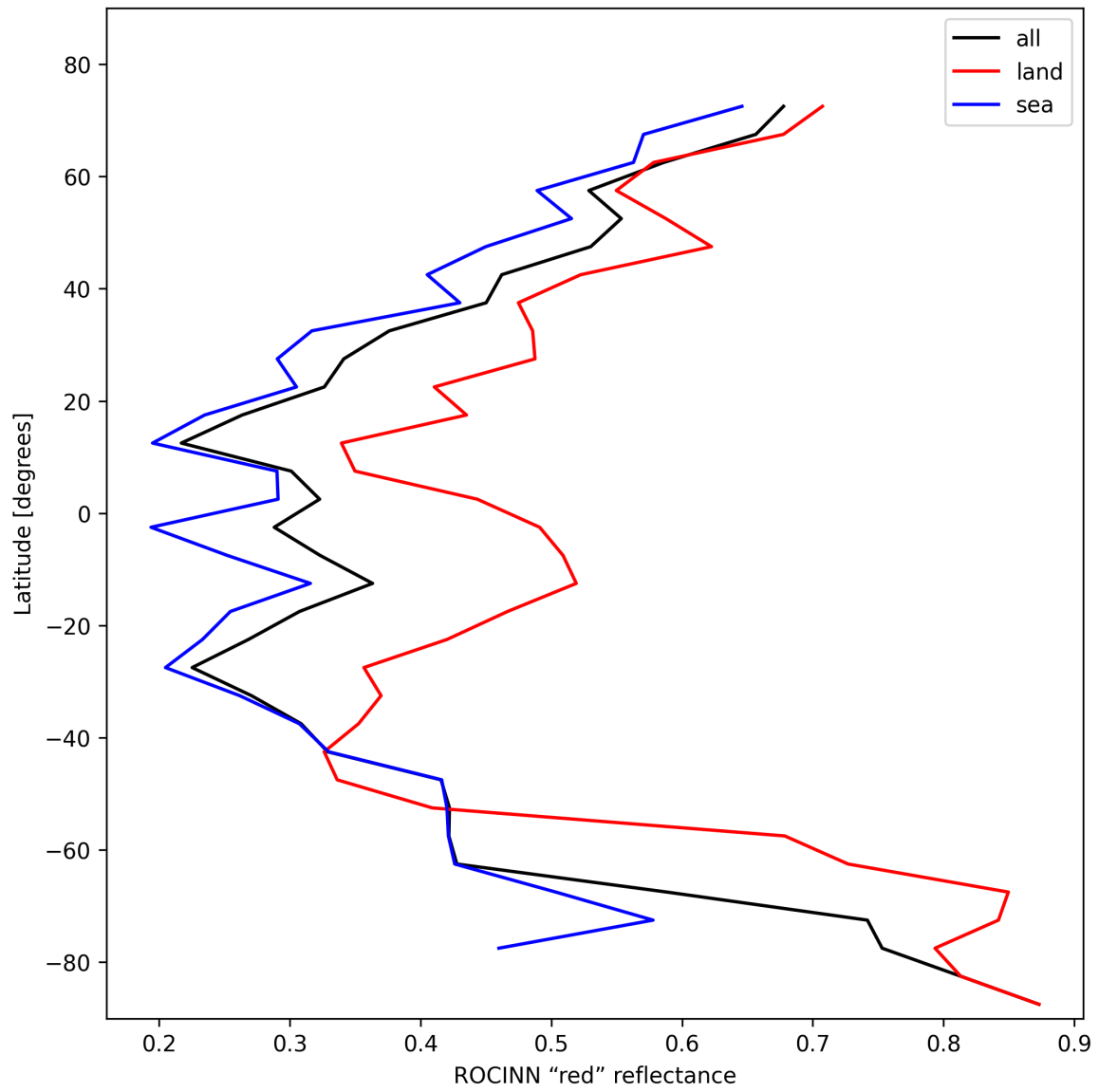
Figure 35: Zonal average of “ROCINN “red” reflectance” for 2025-01-31 to 2025-01-31.
