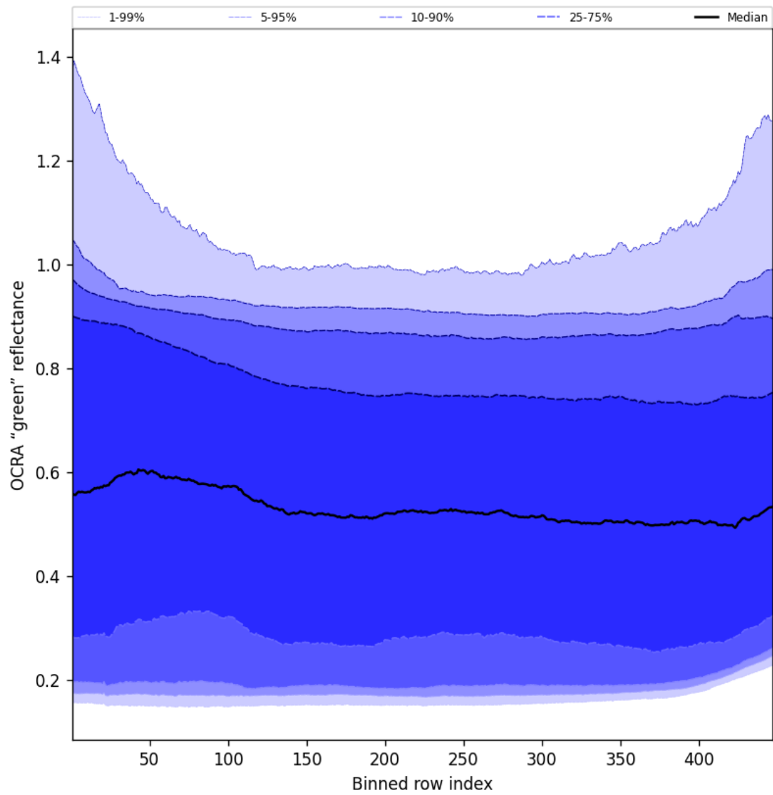
Figure 66: Along track statistics of “OCRA “green” reflectance” for 2025-01-31 to 2025-01-31
