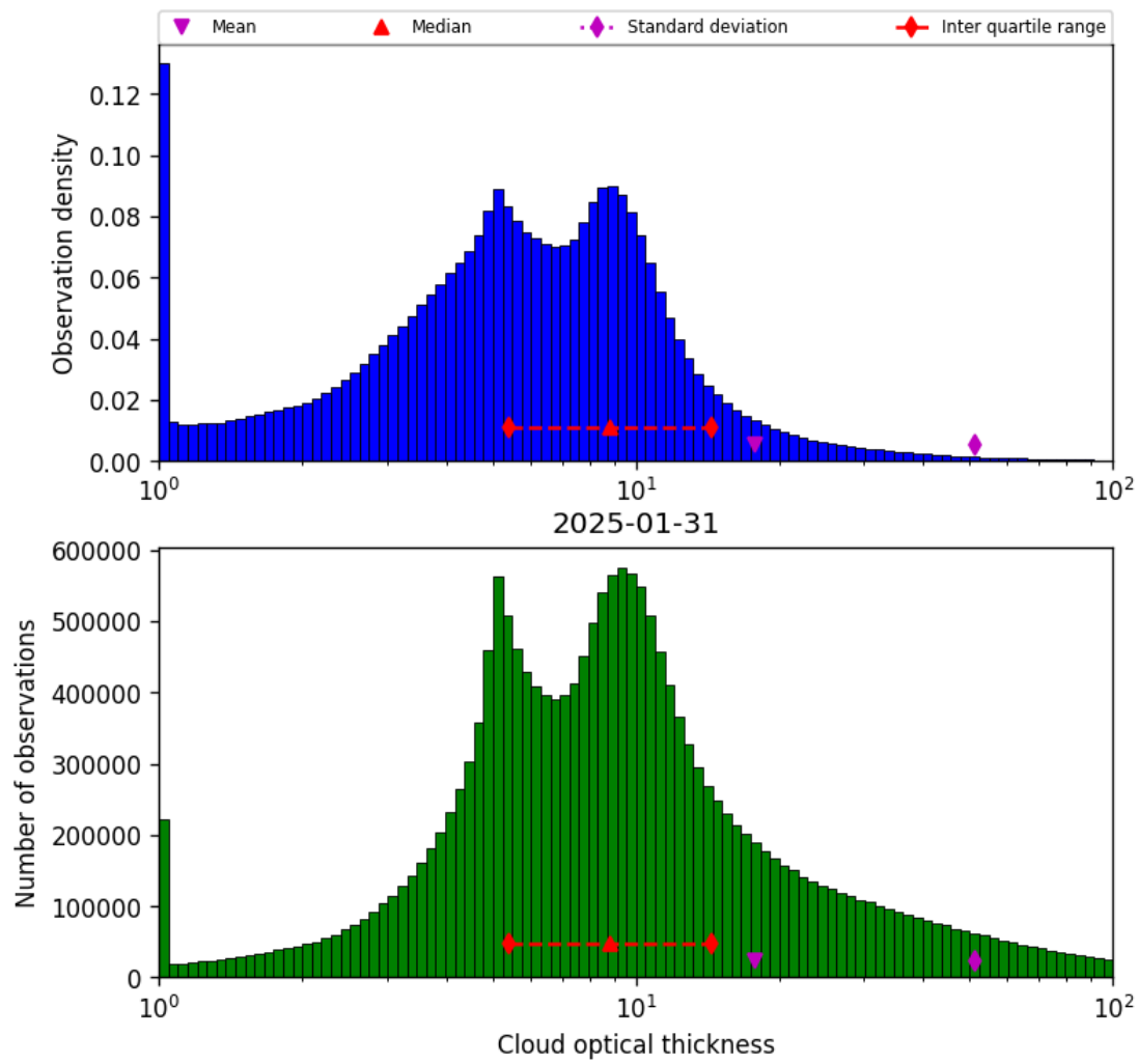
Figure 39: Histogram of “Cloud optical thickness” for 2025-01-31 to 2025-01-31
