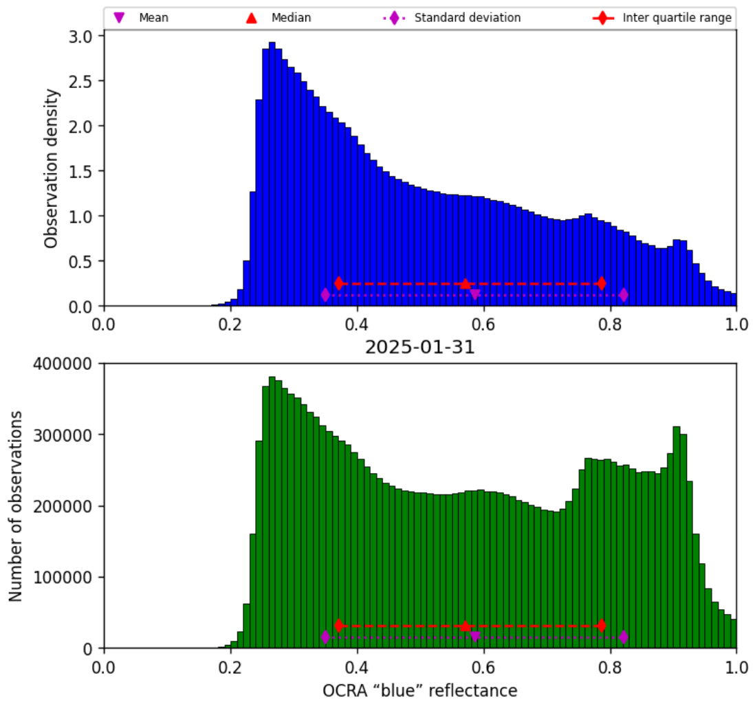
Figure 49: Histogram of “OCRA “blue” reflectance” for 2025-01-31 to 2025-01-31
