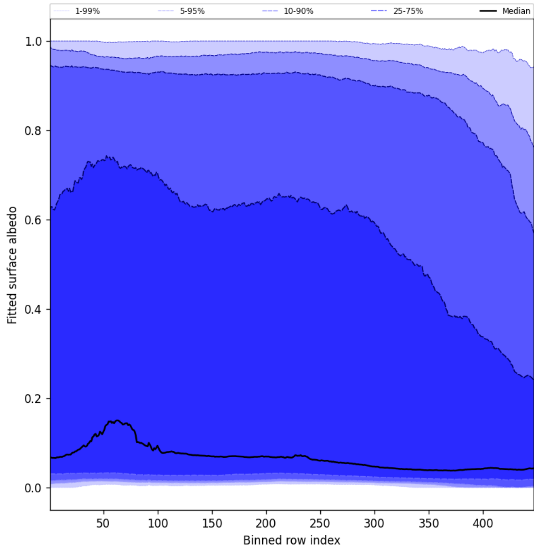
Figure 59: Along track statistics of “Fitted surface albedo” for 2025-01-31 to 2025-01-31
