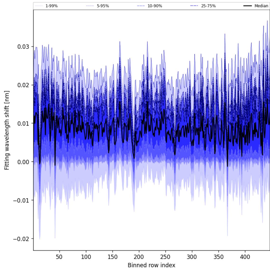
Figure 63: Along track statistics of “Fitting wavelength shift” for 2025-01-31 to 2025-01-31
