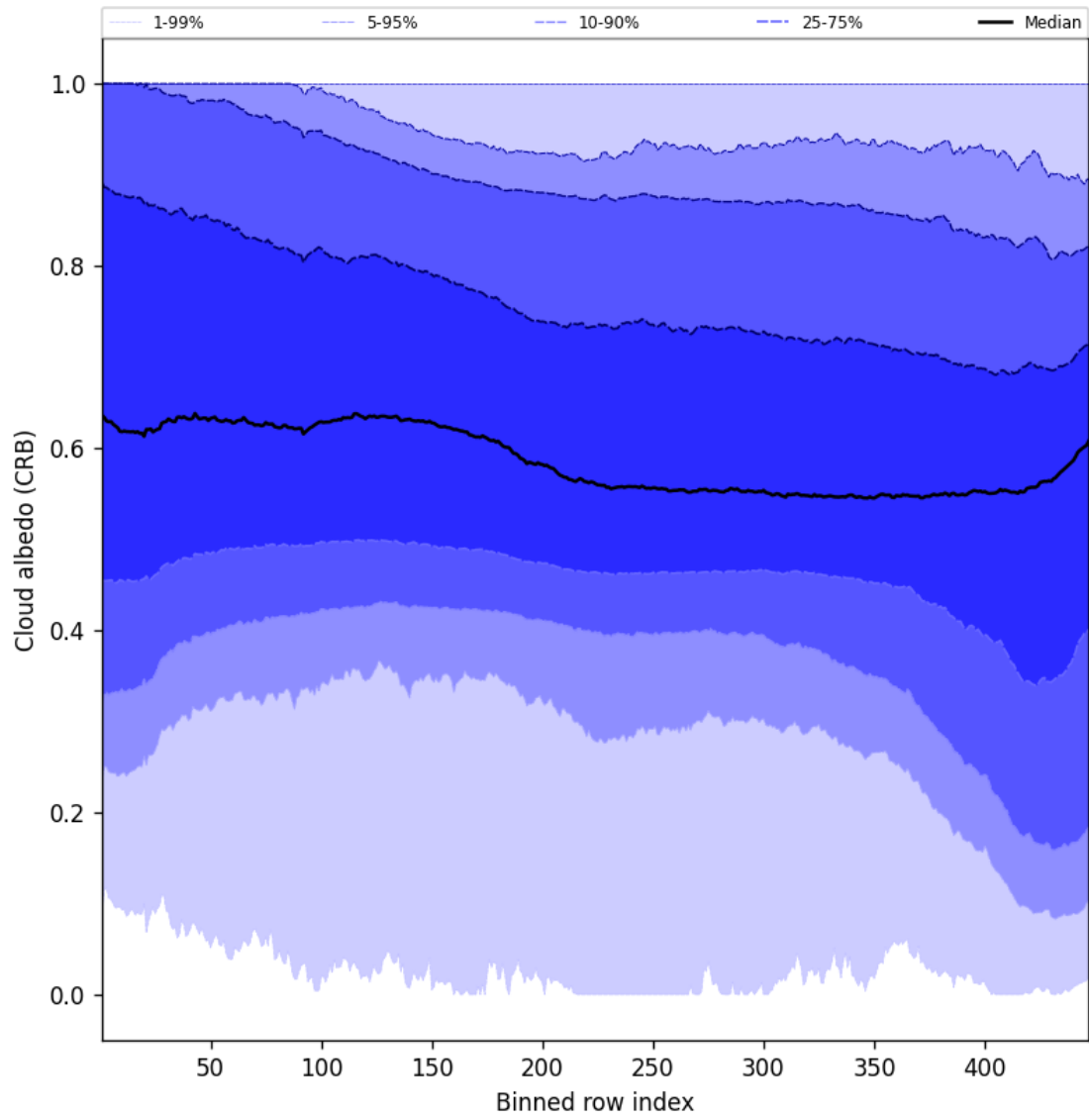
Figure 58: Along track statistics of “Cloud albedo (CRB)” for 2025-01-31 to 2025-01-31
