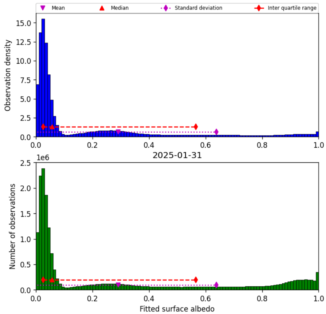
Figure 43: Histogram of “Fitted surface albedo” for 2025-01-31 to 2025-01-31
