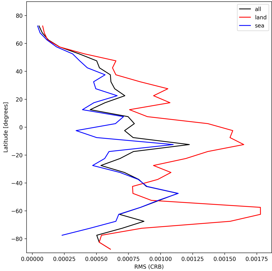
Figure 30: Zonal average of “RMS (CRB)” for 2025-01-31 to 2025-01-31.
