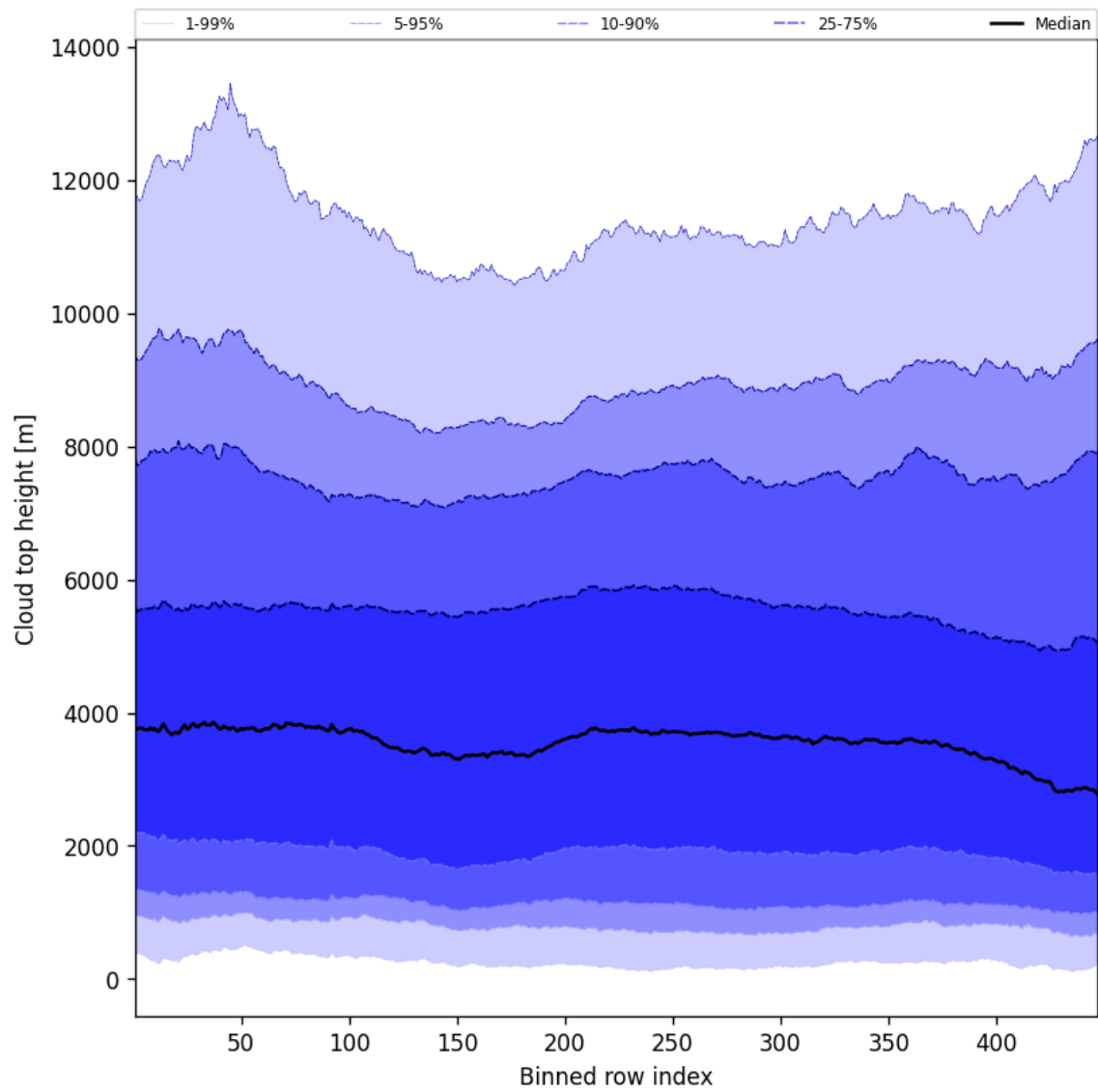
Figure 54: Along track statistics of “Cloud top height” for 2025-01-31 to 2025-01-31
