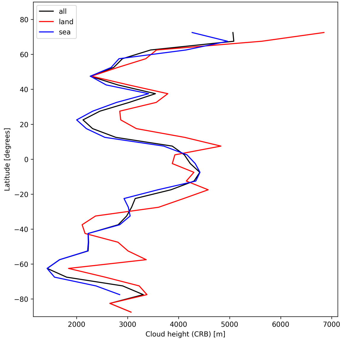
Figure 25: Zonal average of “Cloud height (CRB)” for 2025-01-31 to 2025-01-31.
