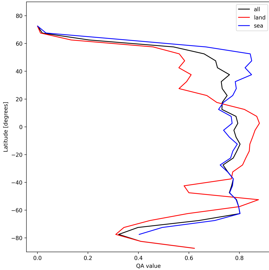
Figure 20: Zonal average of “QA value” for 2025-01-31 to 2025-01-31.
