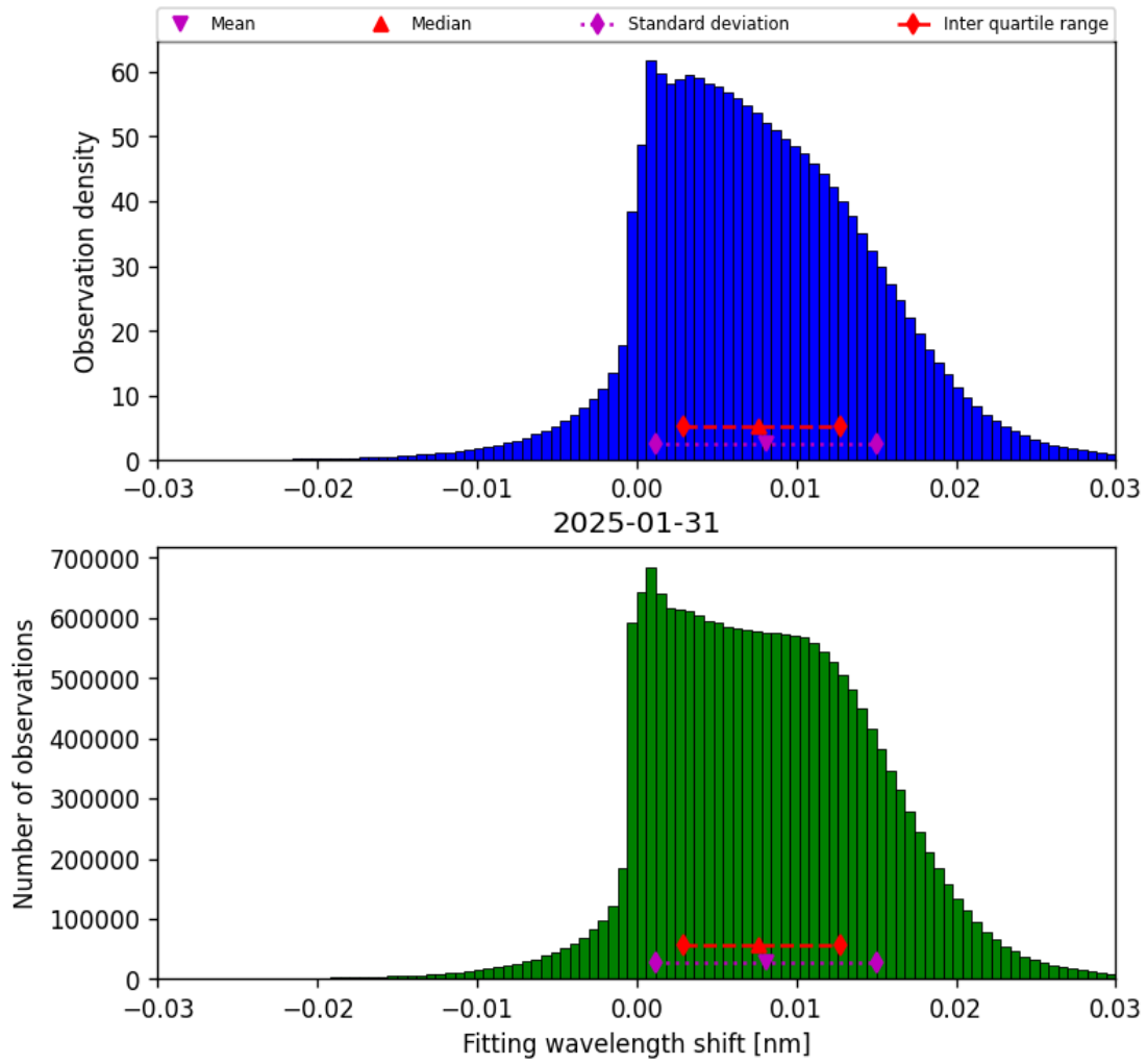
Figure 47: Histogram of “Fitting wavelength shift” for 2025-01-31 to 2025-01-31
