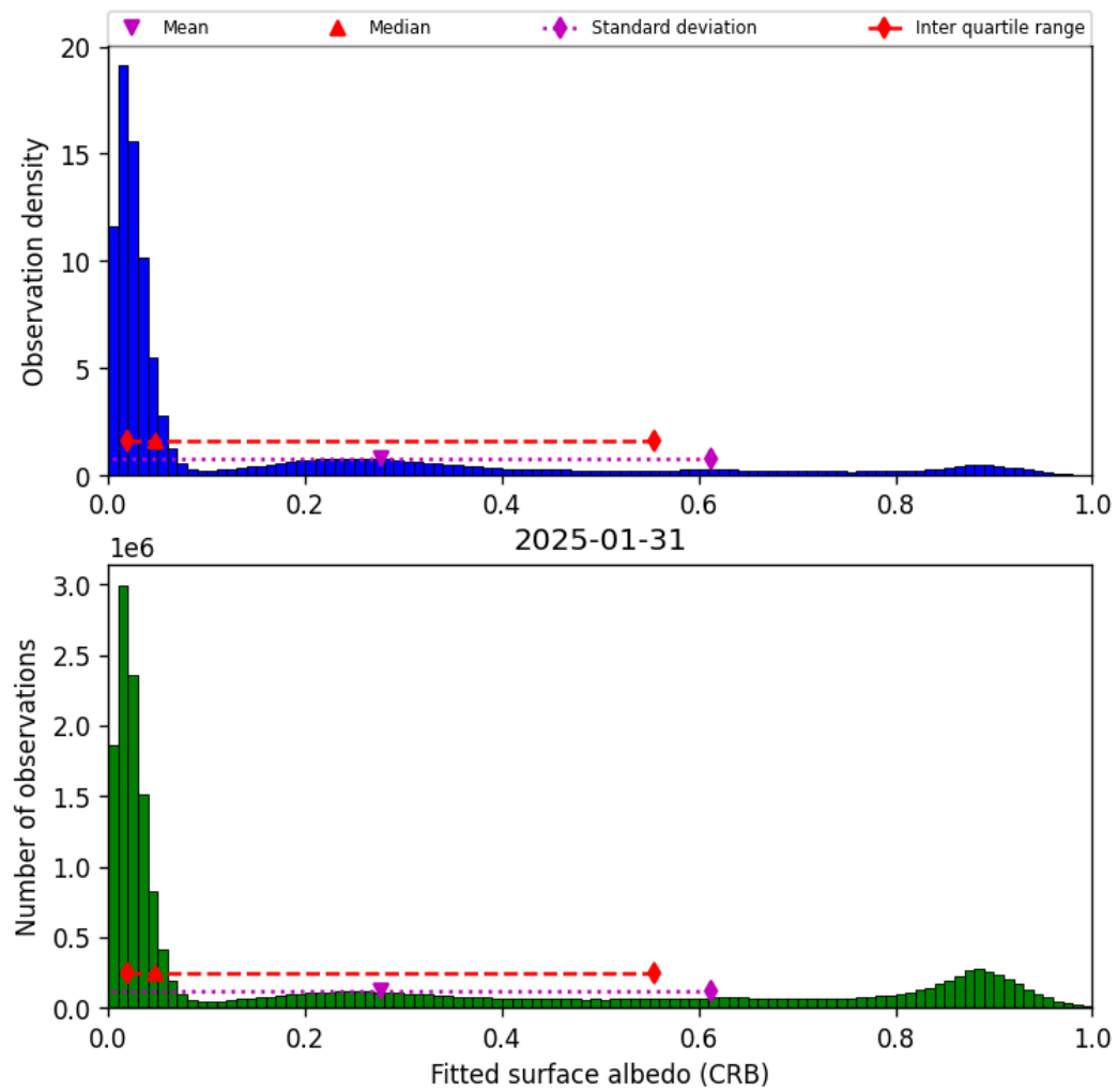
Figure 44: Histogram of “Fitted surface albedo (CRB)” for 2025-01-31 to 2025-01-31
