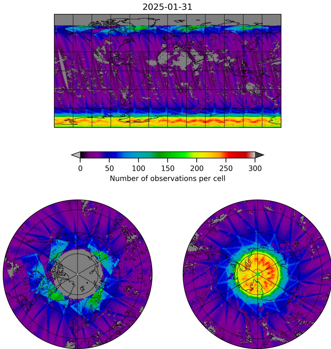
Figure 19: Map of the number of observations for 2025-01-31 to 2025-01-31
