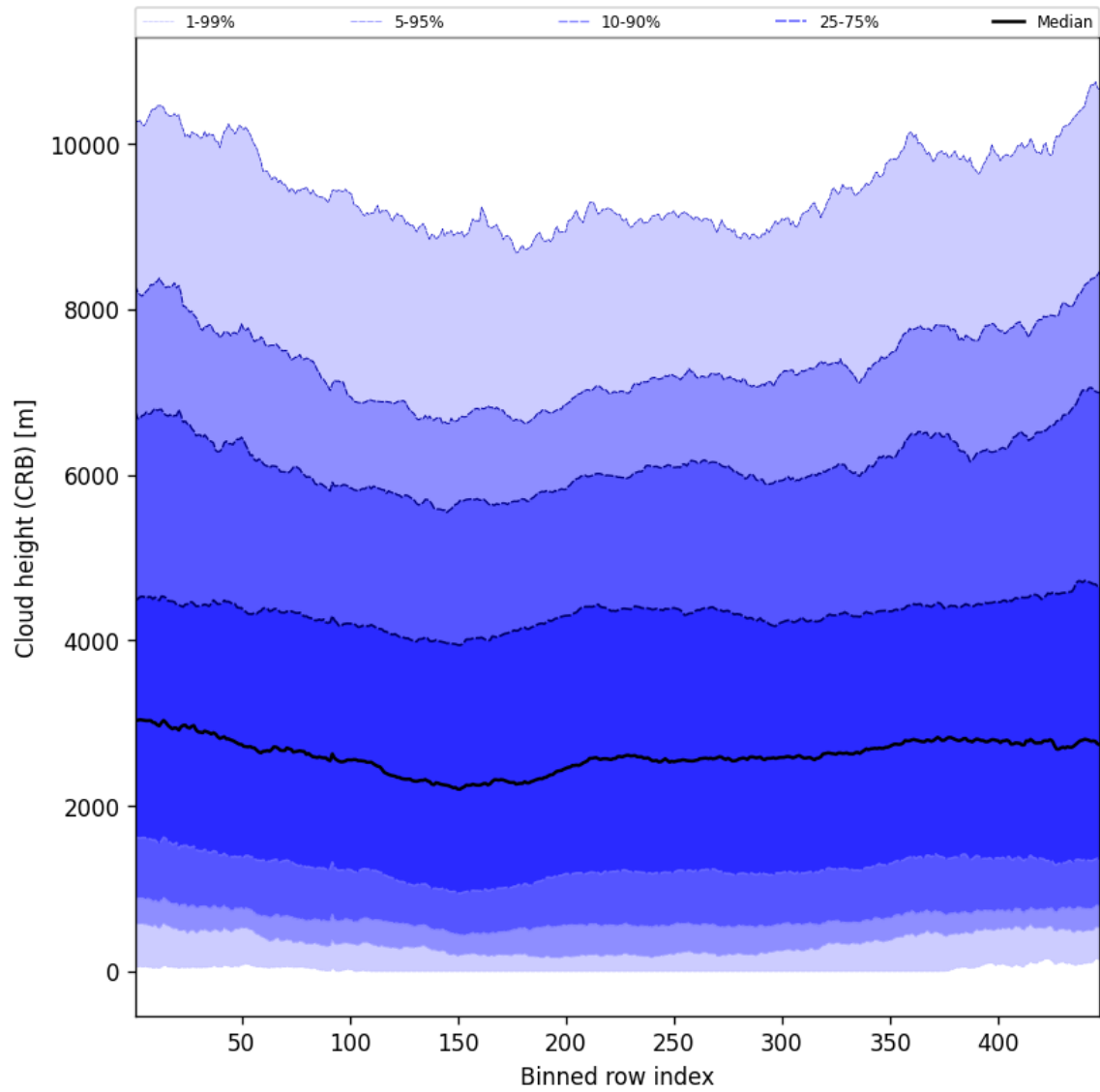
Figure 57: Along track statistics of “Cloud height (CRB)” for 2025-01-31 to 2025-01-31
