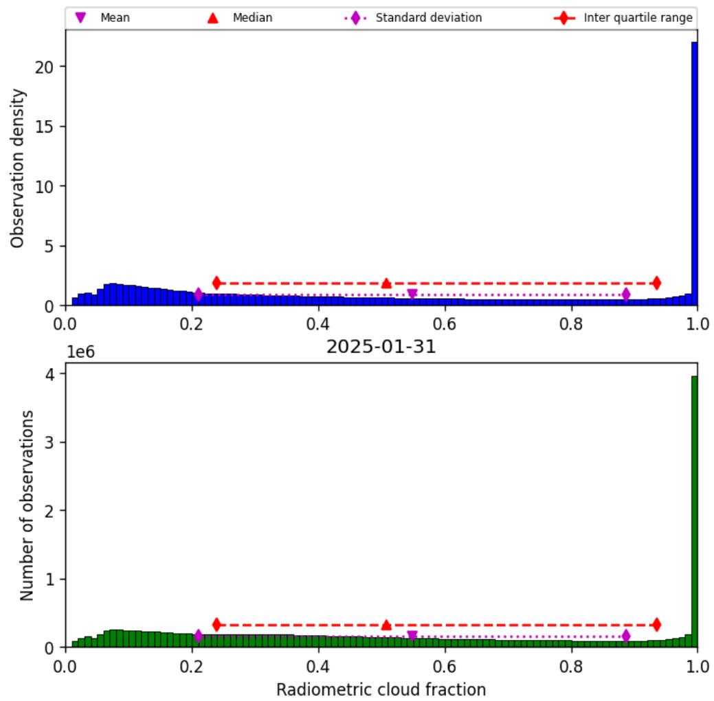
Figure 37: Histogram of “Radiometric cloud fraction” for 2025-01-31 to 2025-01-31
