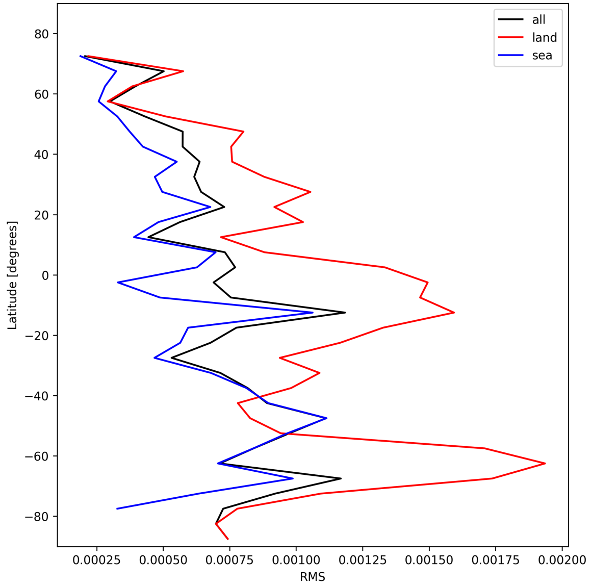
Figure 29: Zonal average of “RMS” for 2025-01-31 to 2025-01-31.
