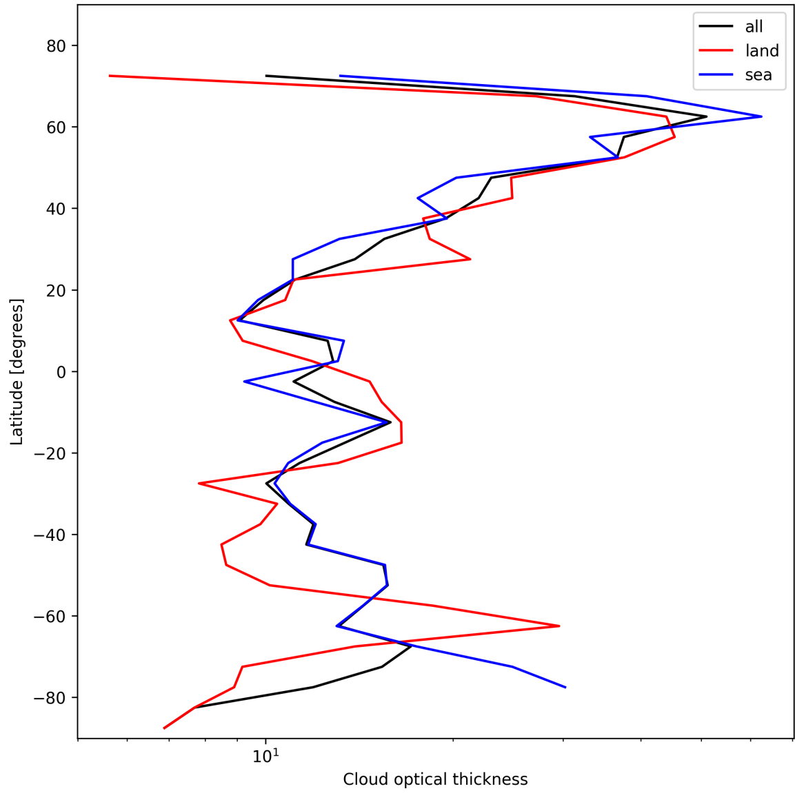
Figure 23: Zonal average of “Cloud optical thickness” for 2025-01-31 to 2025-01-31.
