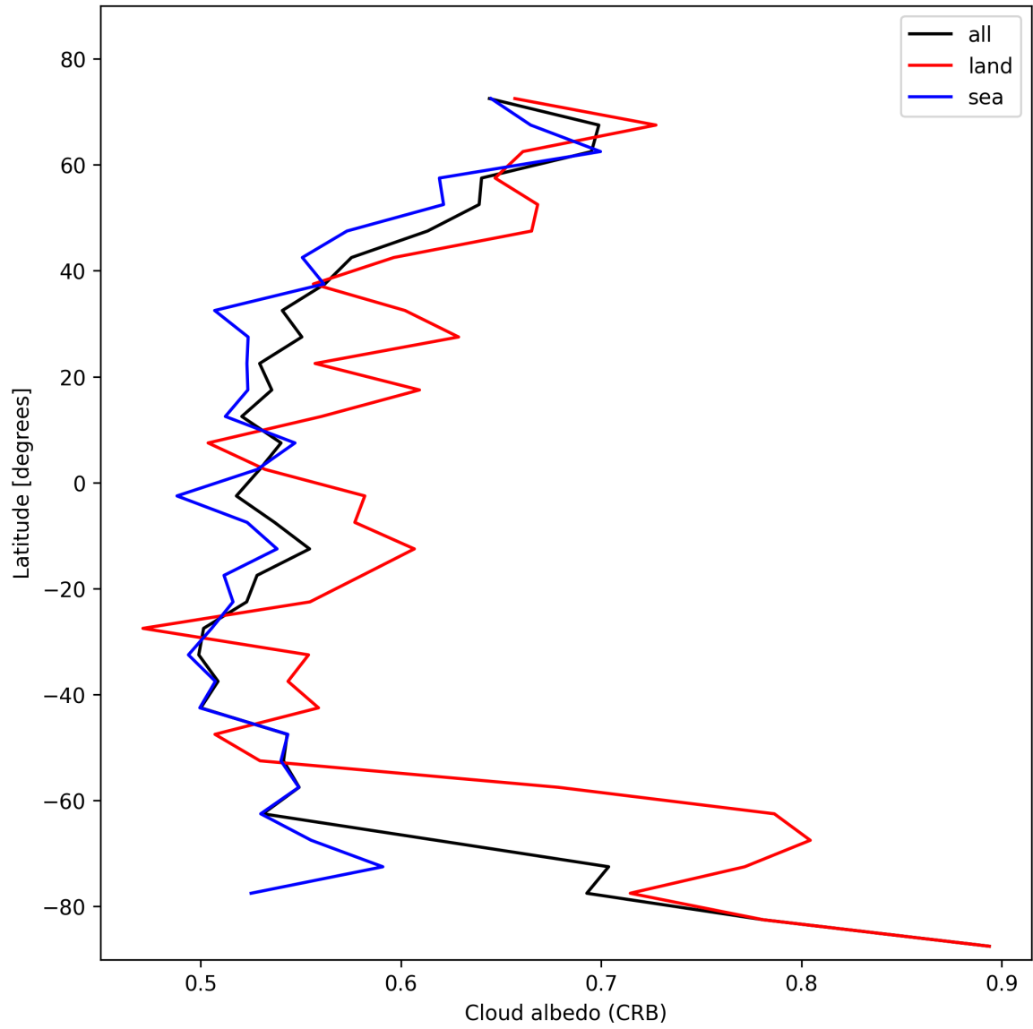
Figure 26: Zonal average of “Cloud albedo (CRB)” for 2025-01-31 to 2025-01-31.
