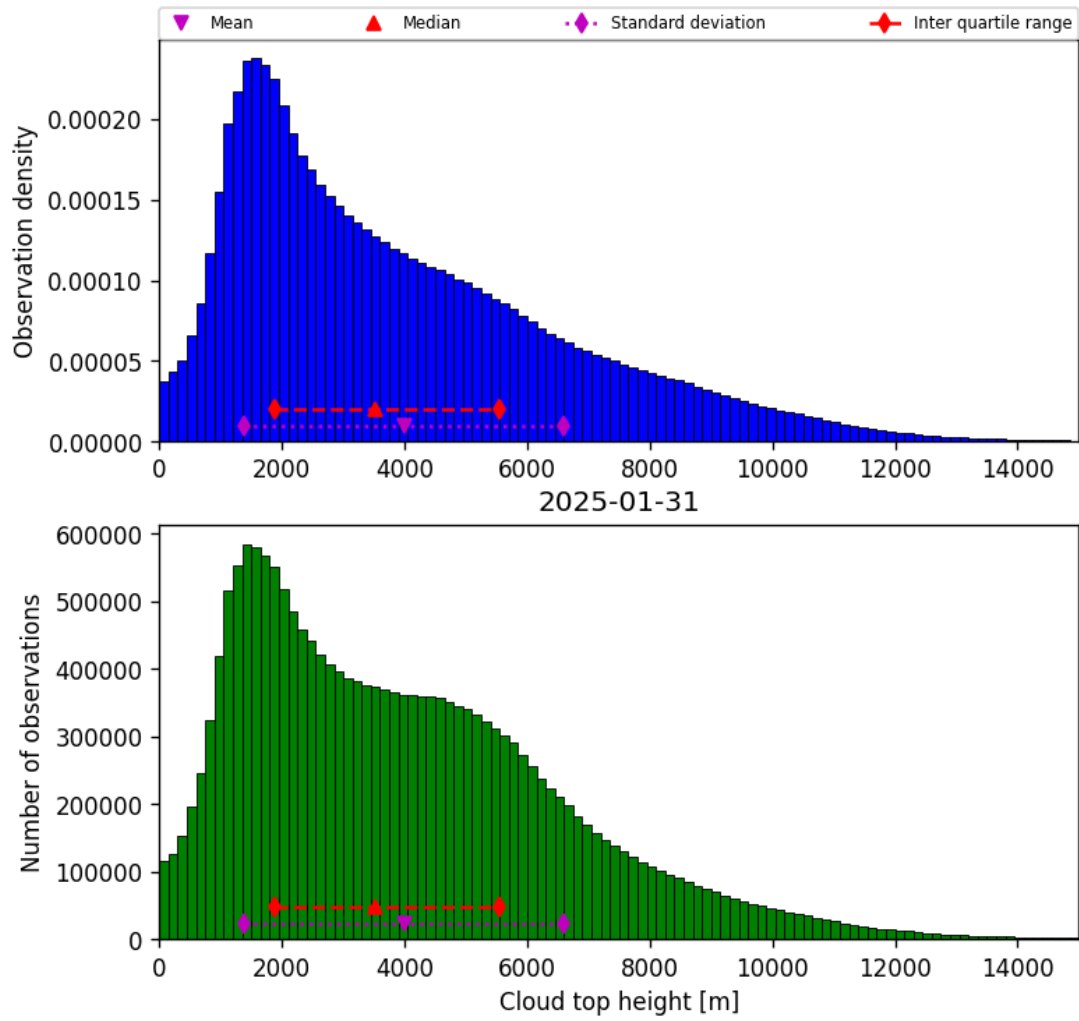
Figure 38: Histogram of “Cloud top height” for 2025-01-31 to 2025-01-31
