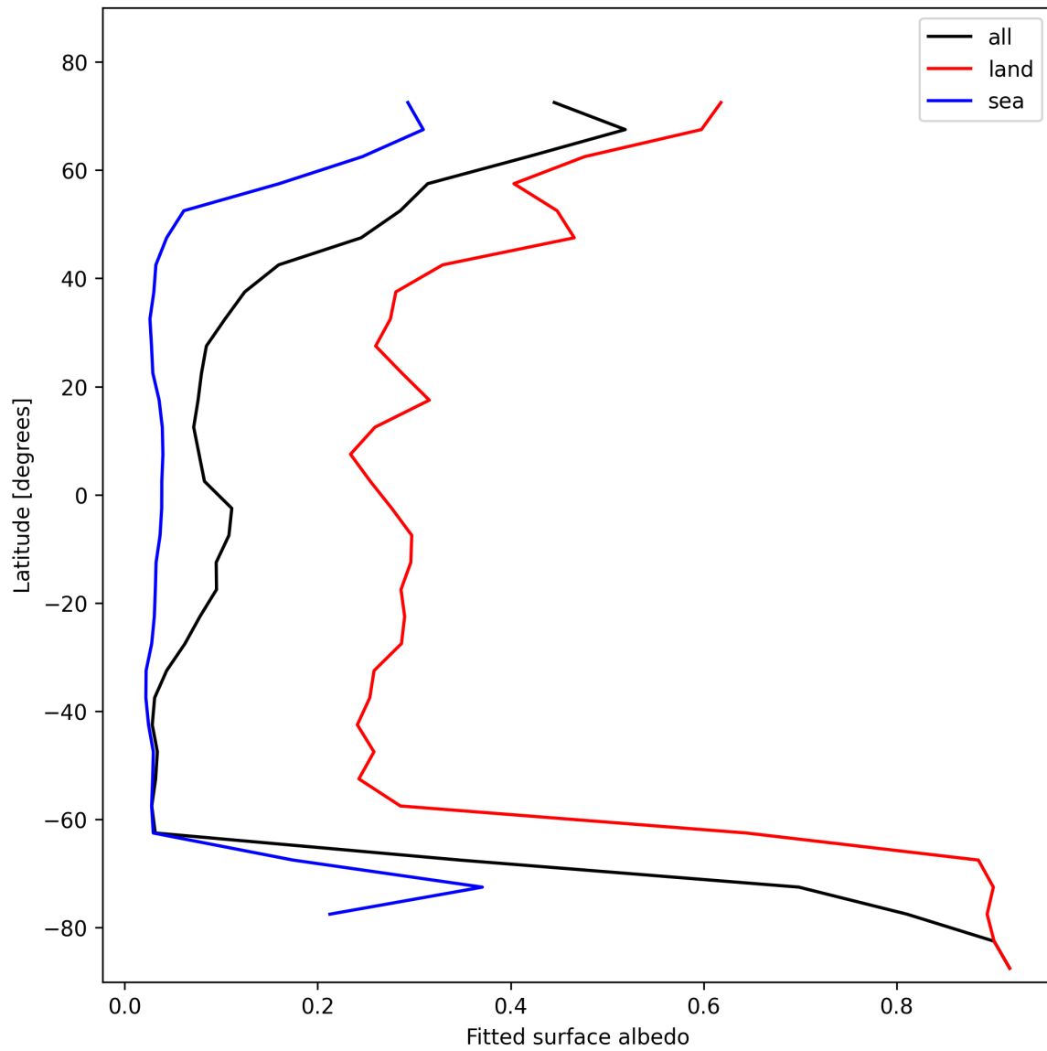
Figure 27: Zonal average of “Fitted surface albedo” for 2025-01-31 to 2025-01-31.
