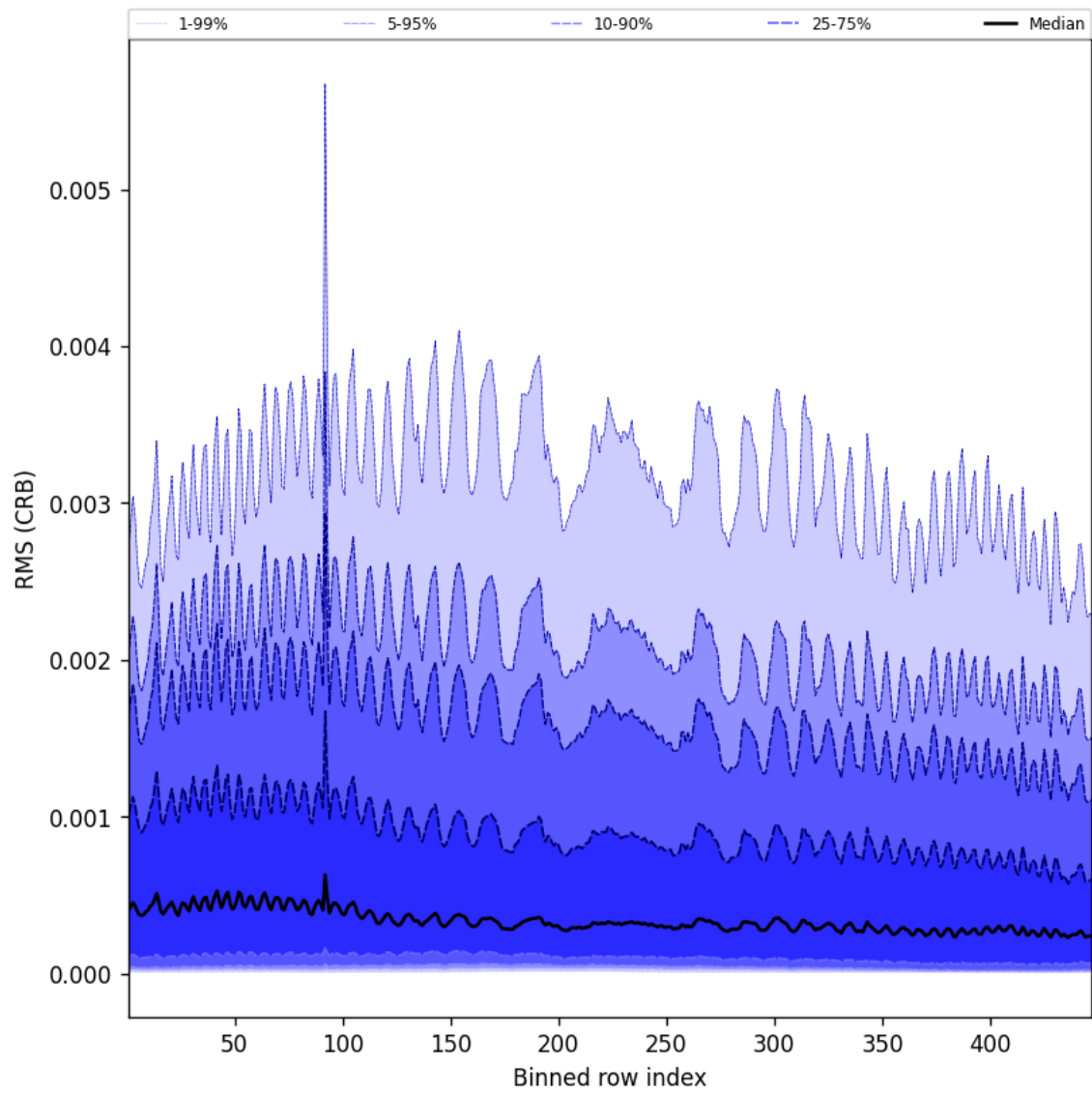
Figure 62: Along track statistics of “RMS (CRB)” for 2025-01-31 to 2025-01-31
