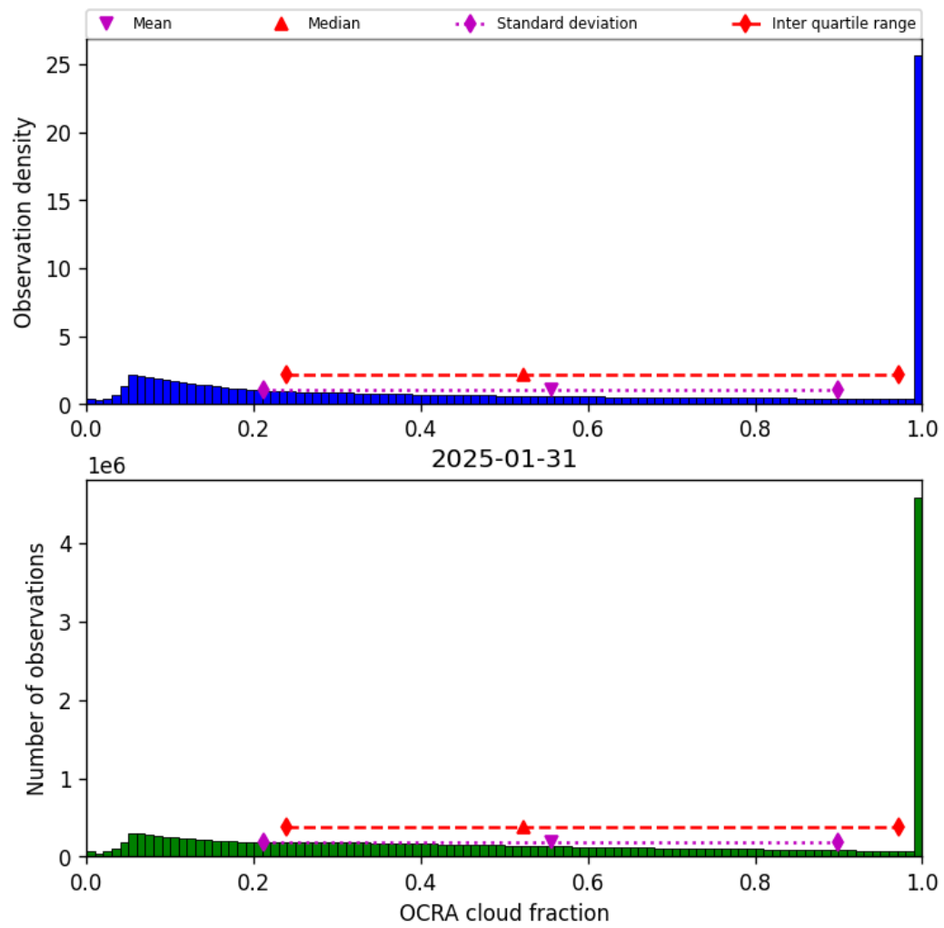
Figure 48: Histogram of “OCRA cloud fraction” for 2025-01-31 to 2025-01-31
