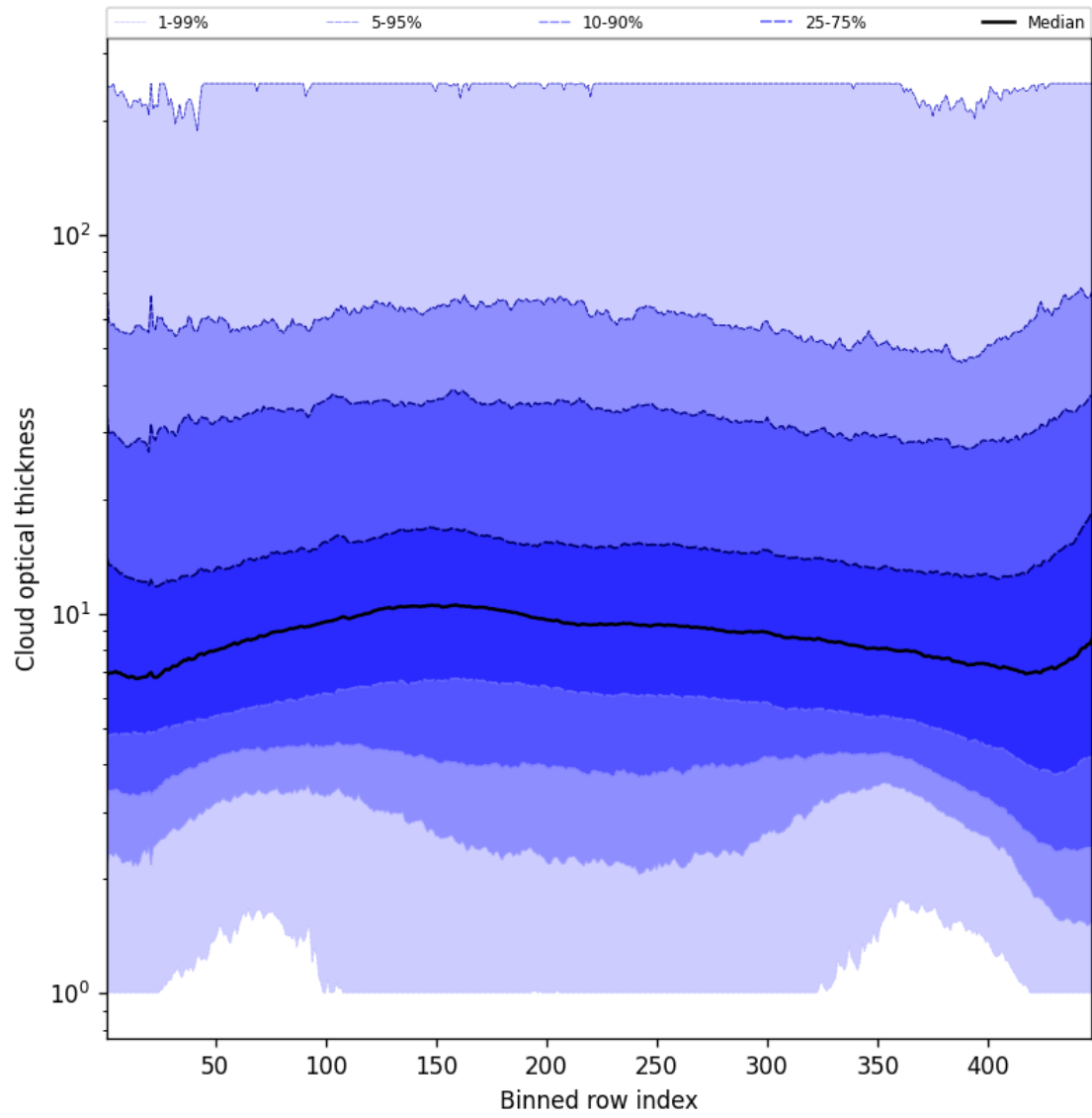
Figure 55: Along track statistics of “Cloud optical thickness” for 2025-01-31 to 2025-01-31
