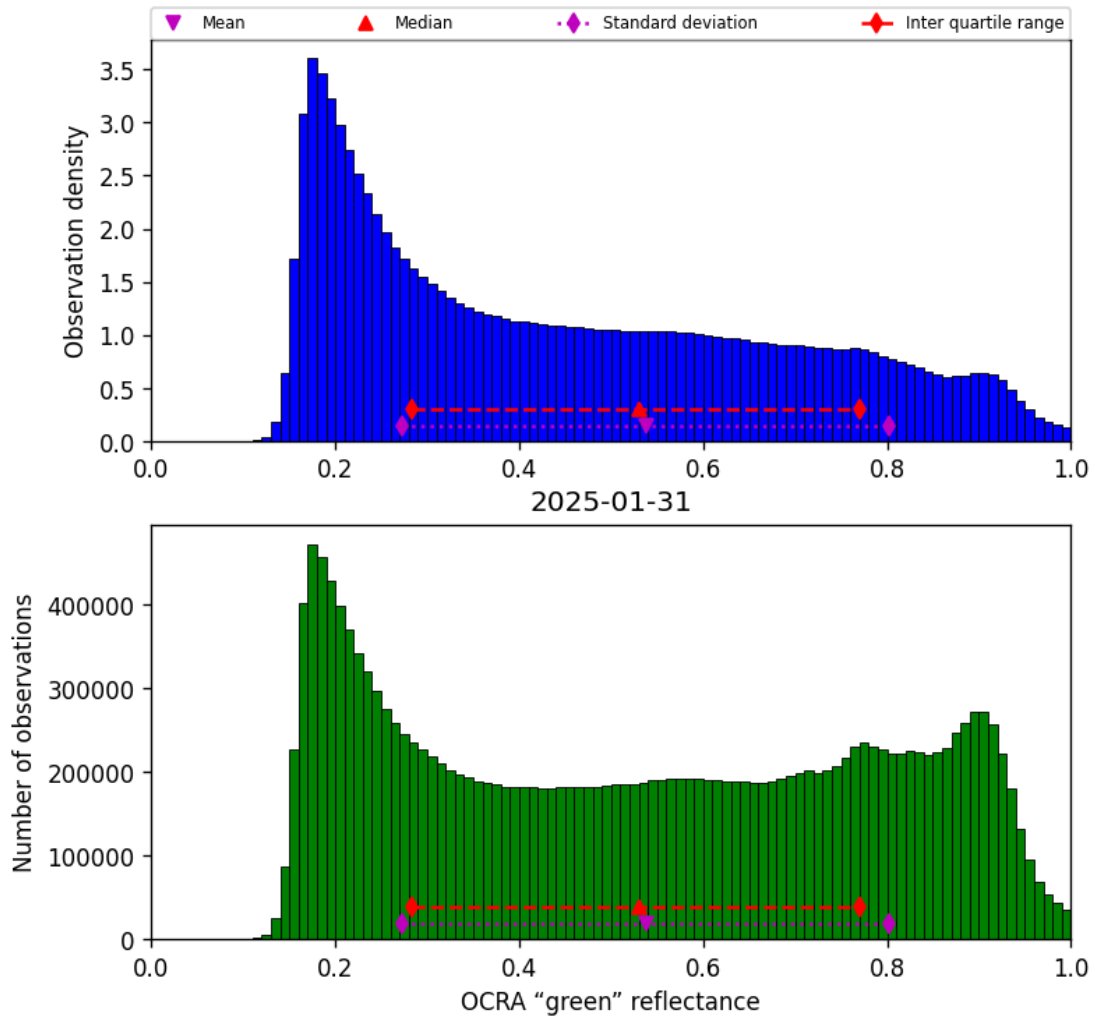
Figure 50: Histogram of “OCRA “green” reflectance” for 2025-01-31 to 2025-01-31
