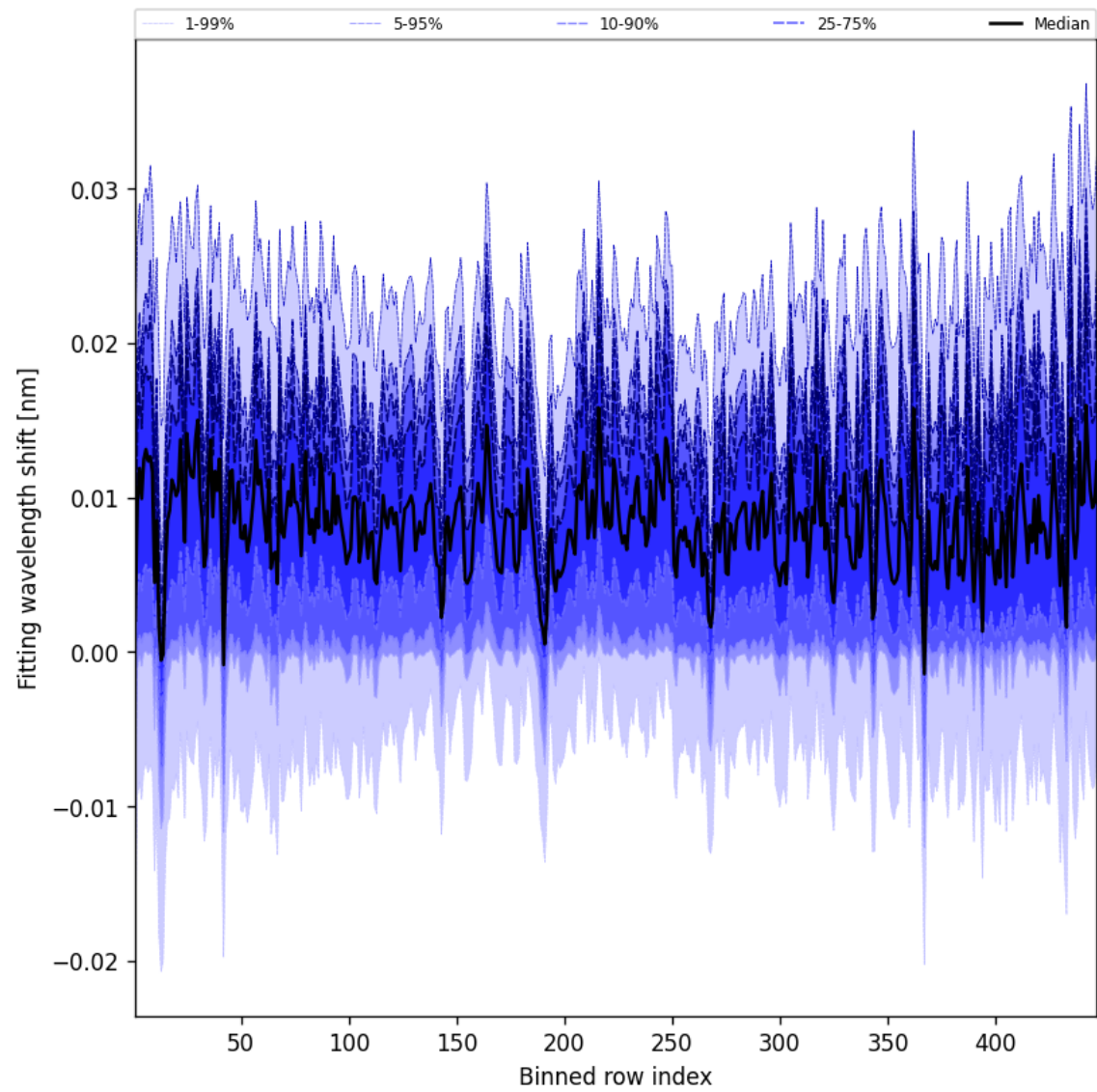
Figure 63: Along track statistics of “Fitting wavelength shift” for 2025-02-01 to 2025-02-02
