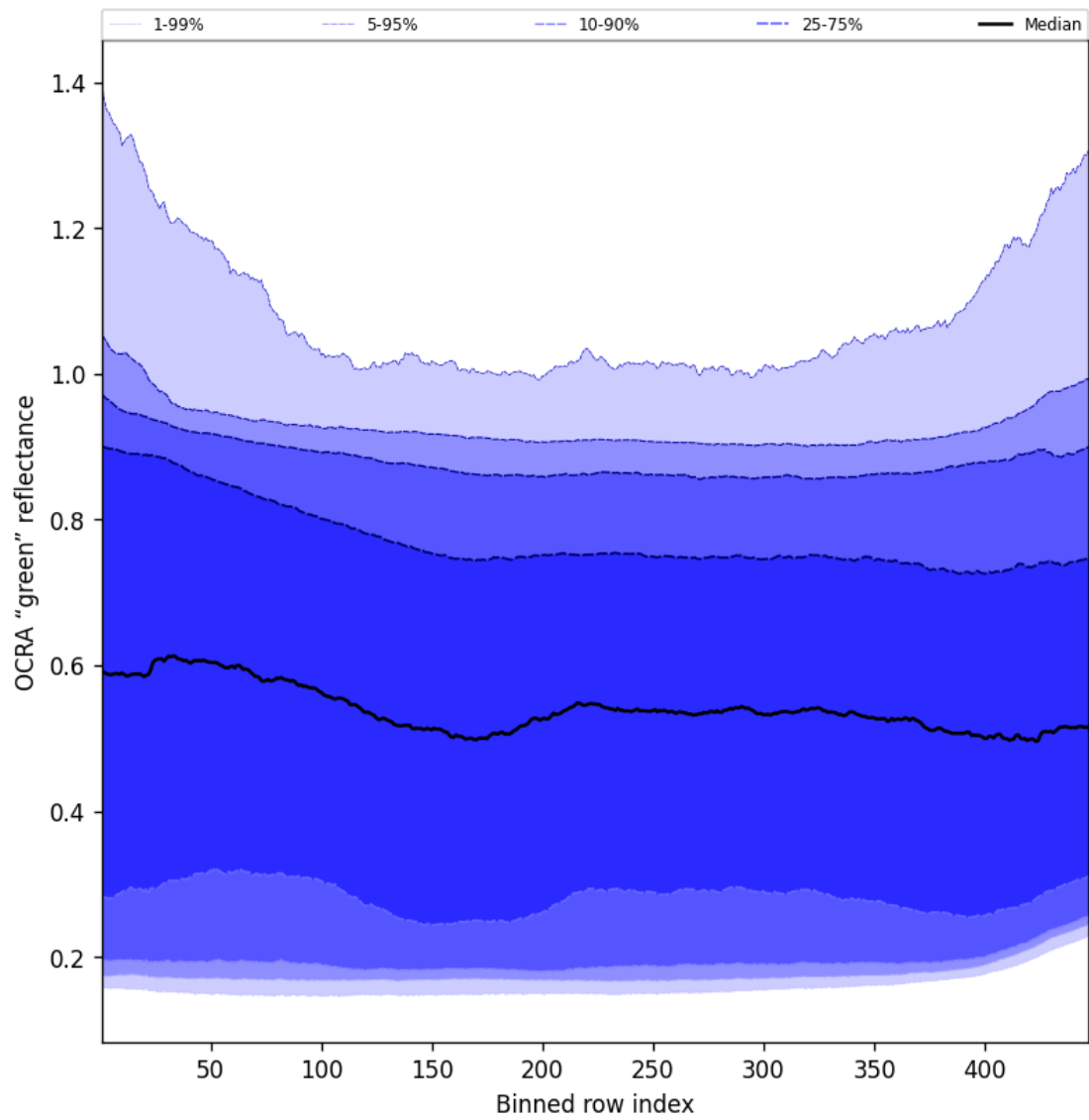
Figure 66: Along track statistics of “OCRA “green” reflectance” for 2025-02-01 to 2025-02-02
