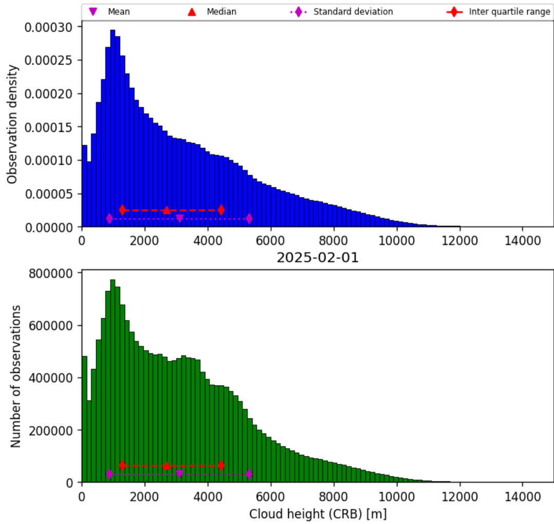
Figure 41: Histogram of “Cloud height (CRB)” for 2025-02-01 to 2025-02-02
