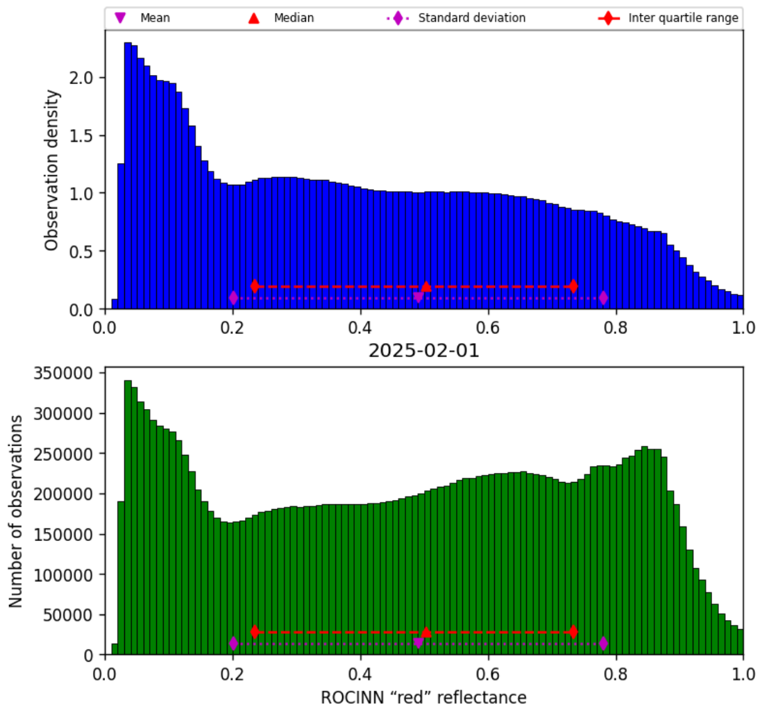
Figure 51: Histogram of “ROCINN “red” reflectance” for 2025-02-01 to 2025-02-02
