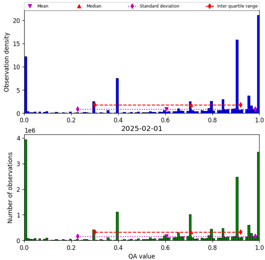
Figure 36: Histogram of “QA value” for 2025-02-01 to 2025-02-02
