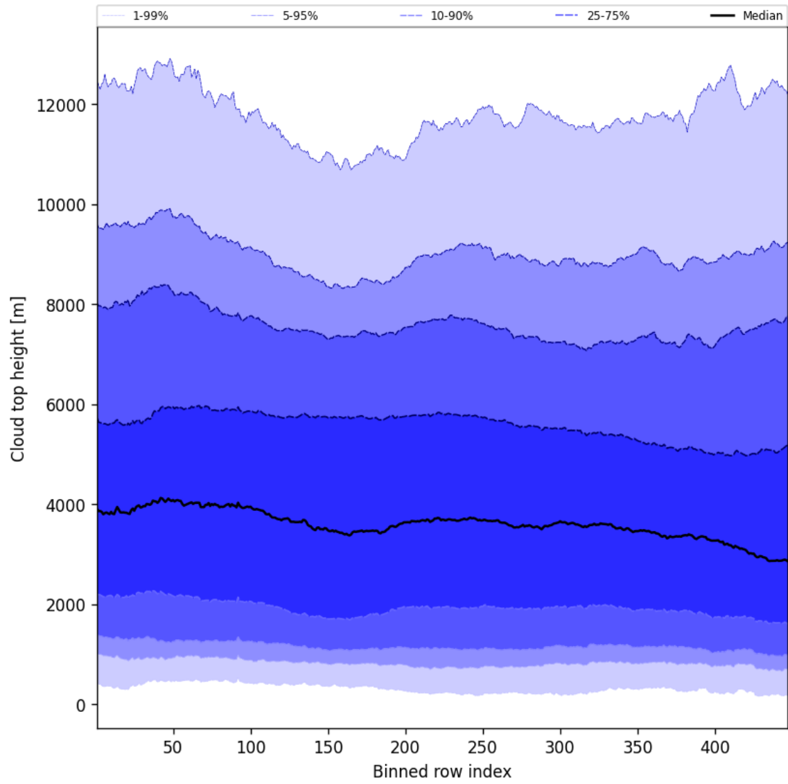
Figure 54: Along track statistics of “Cloud top height” for 2025-02-01 to 2025-02-02
