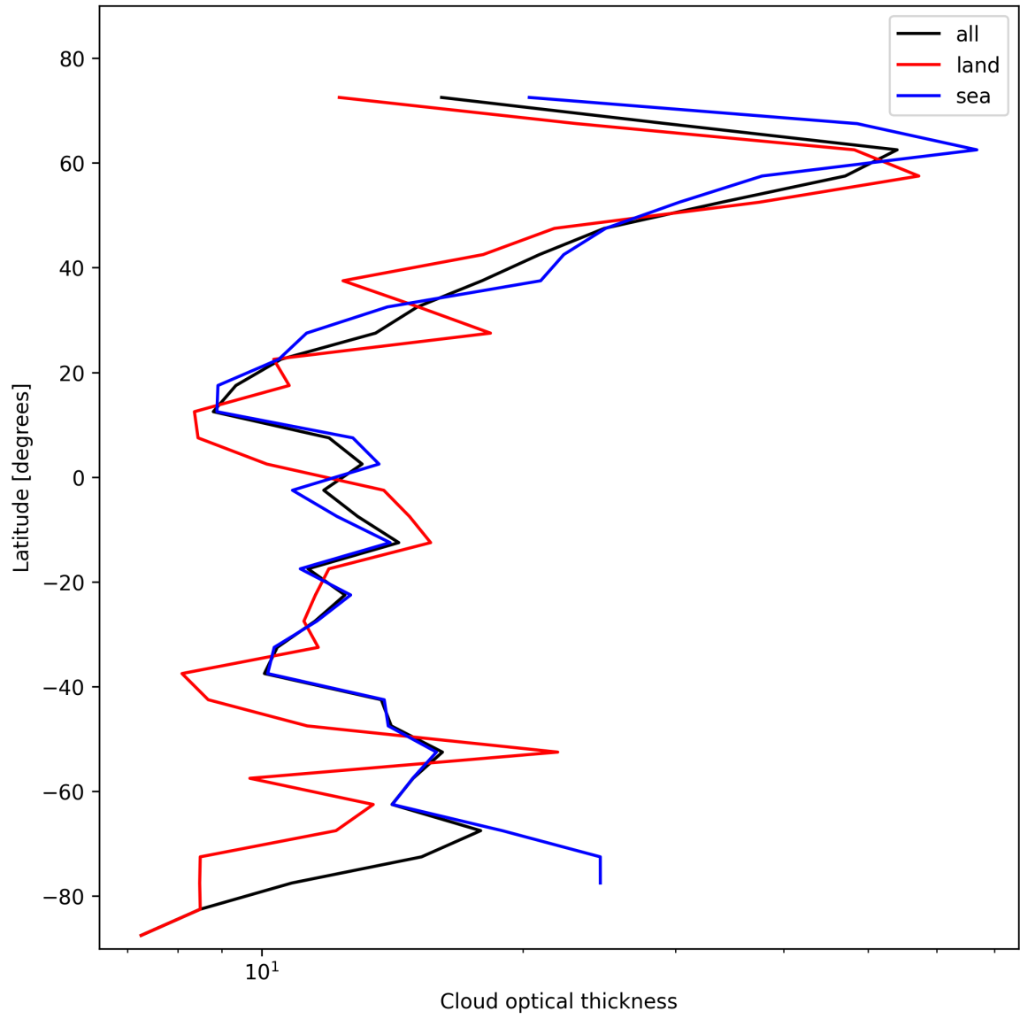
Figure 23: Zonal average of “Cloud optical thickness” for 2025-02-01 to 2025-02-02.
