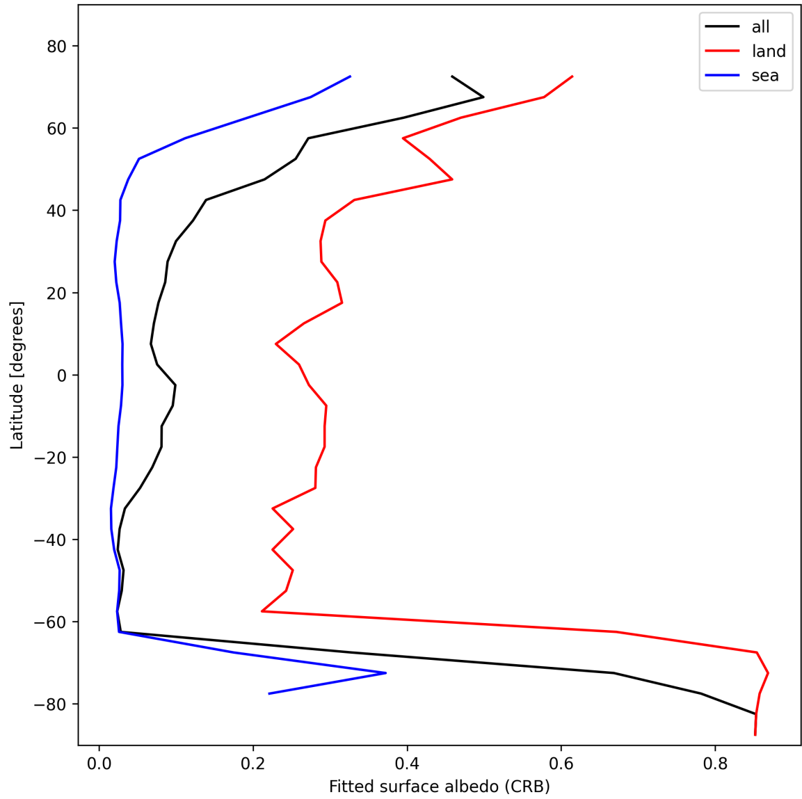
Figure 28: Zonal average of “Fitted surface albedo (CRB)” for 2025-02-01 to 2025-02-02.
