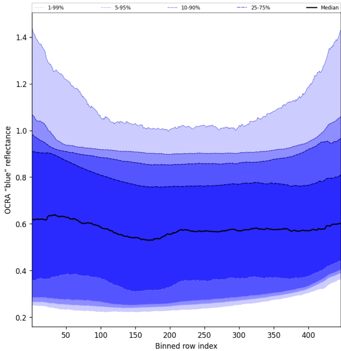
Figure 65: Along track statistics of “OCRA “blue” reflectance” for 2025-02-01 to 2025-02-02
