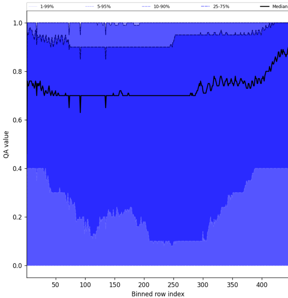
Figure 52: Along track statistics of “QA value” for 2025-02-01 to 2025-02-02
