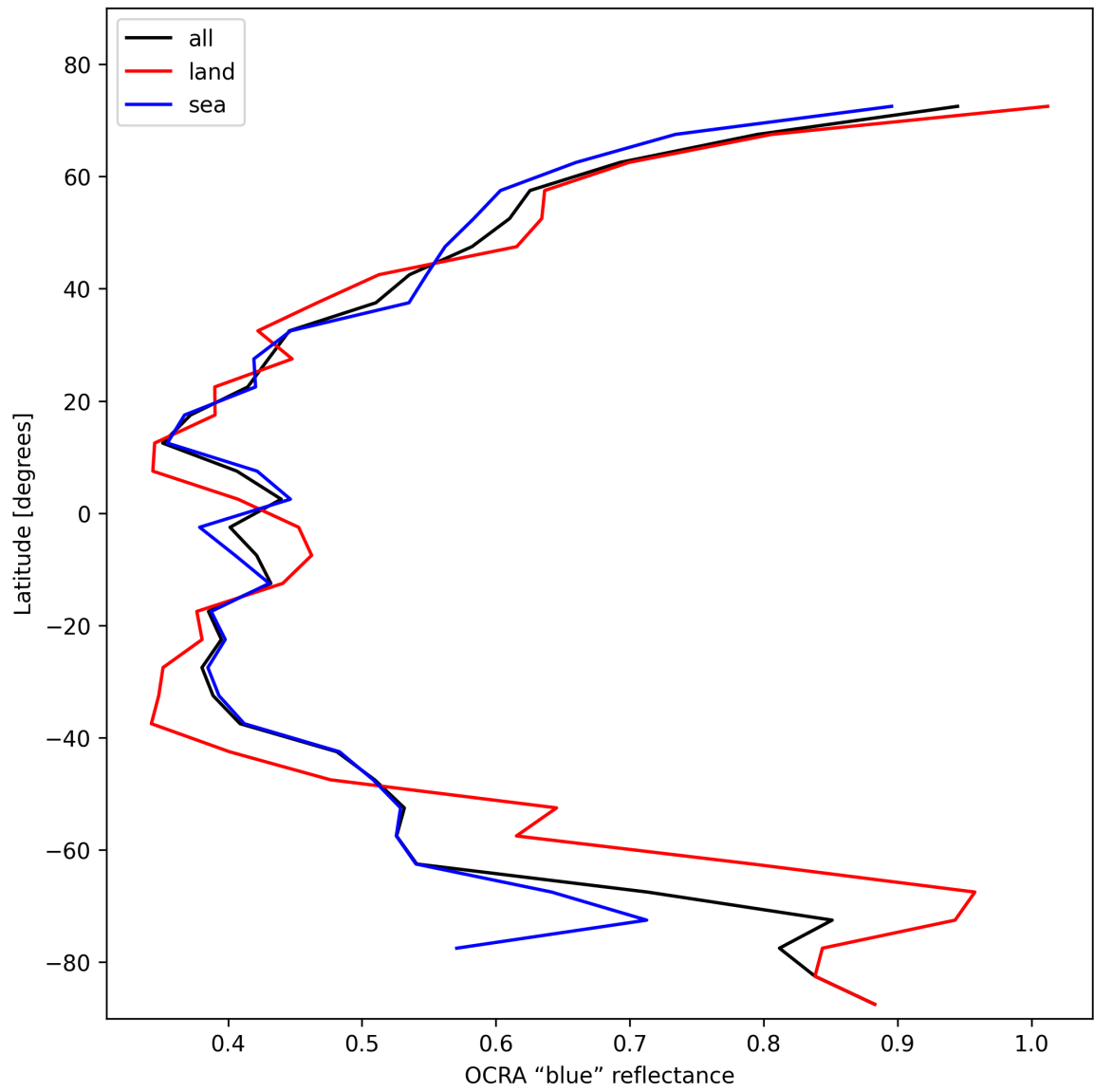
Figure 33: Zonal average of “OCRA “blue” reflectance” for 2025-02-01 to 2025-02-02.
