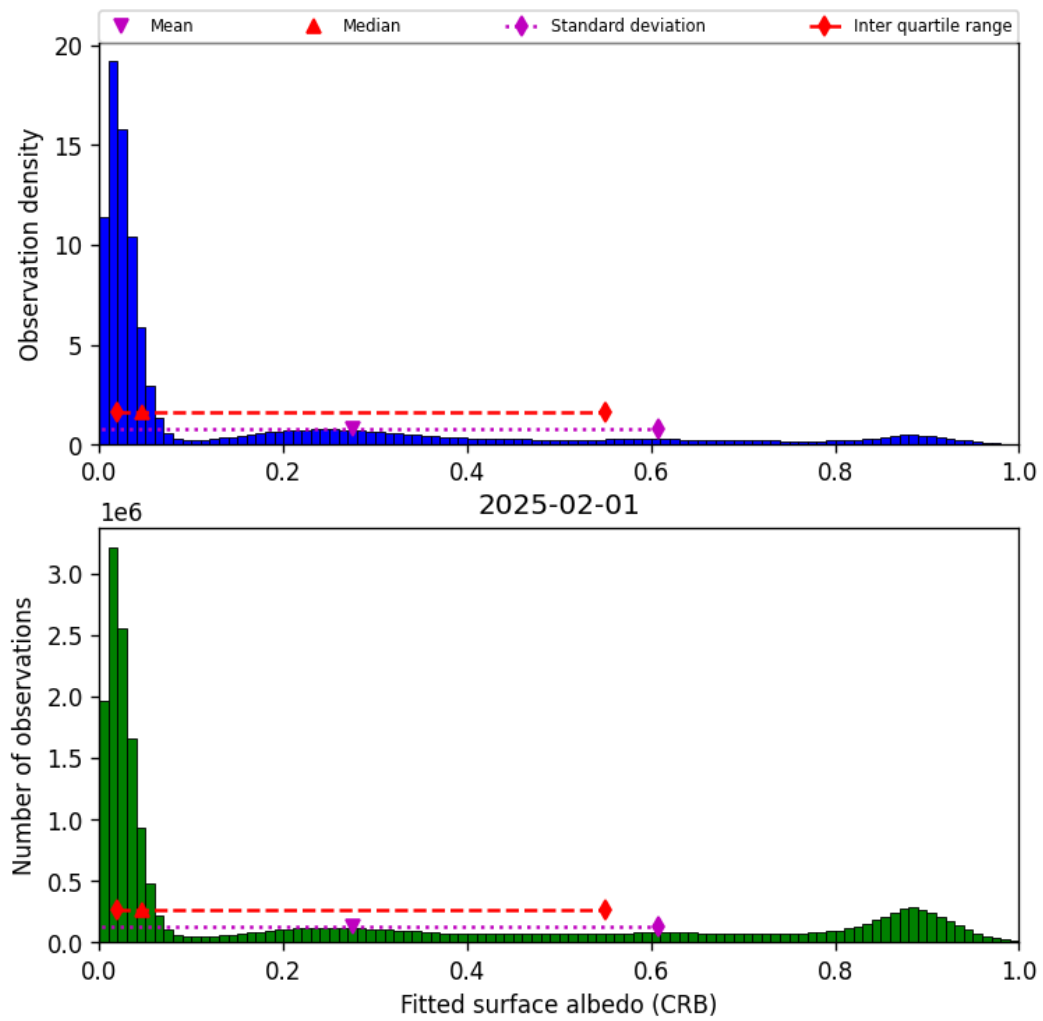
Figure 44: Histogram of “Fitted surface albedo (CRB)” for 2025-02-01 to 2025-02-02
