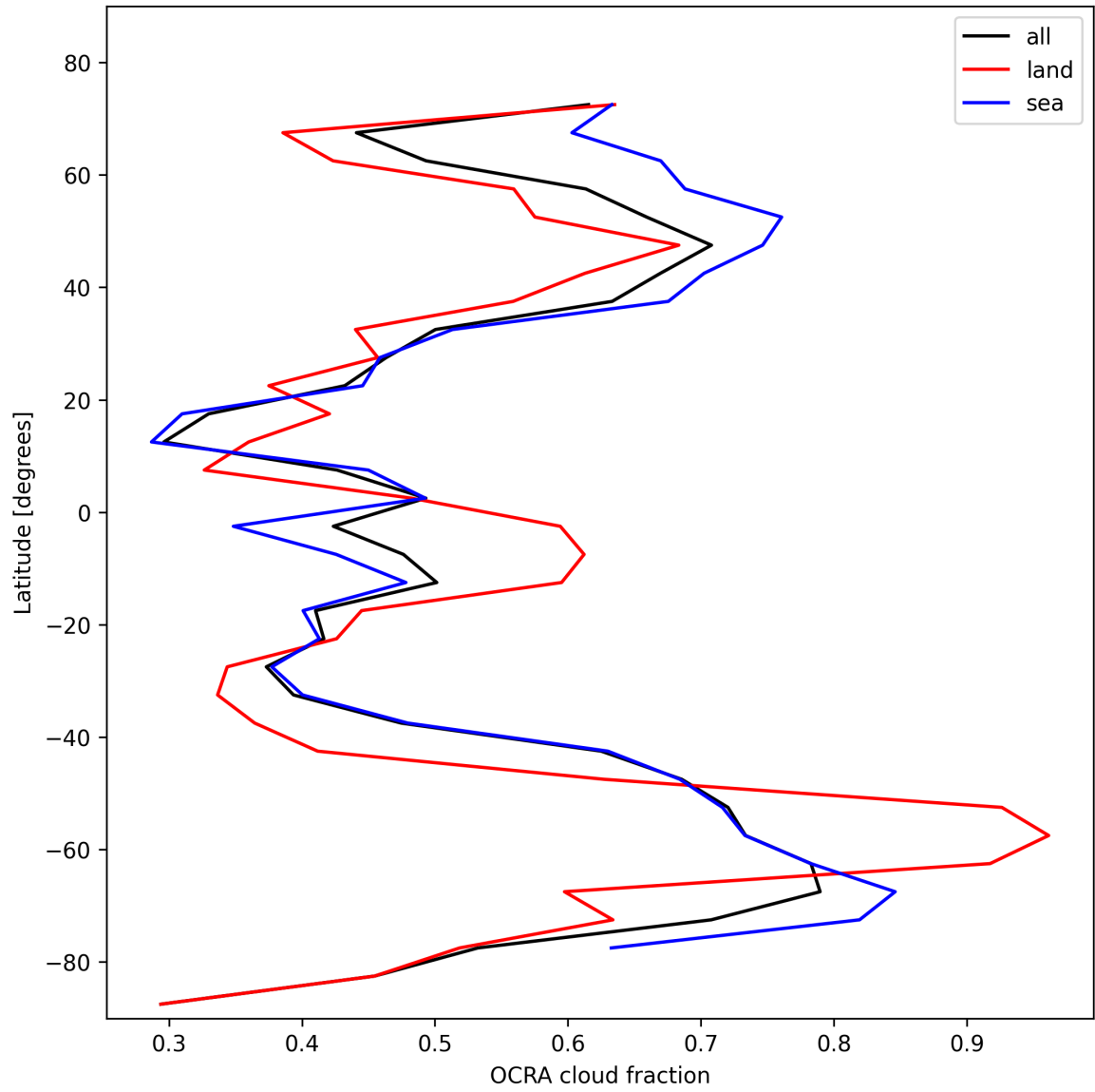
Figure 32: Zonal average of “OCRA cloud fraction” for 2025-02-01 to 2025-02-02.
