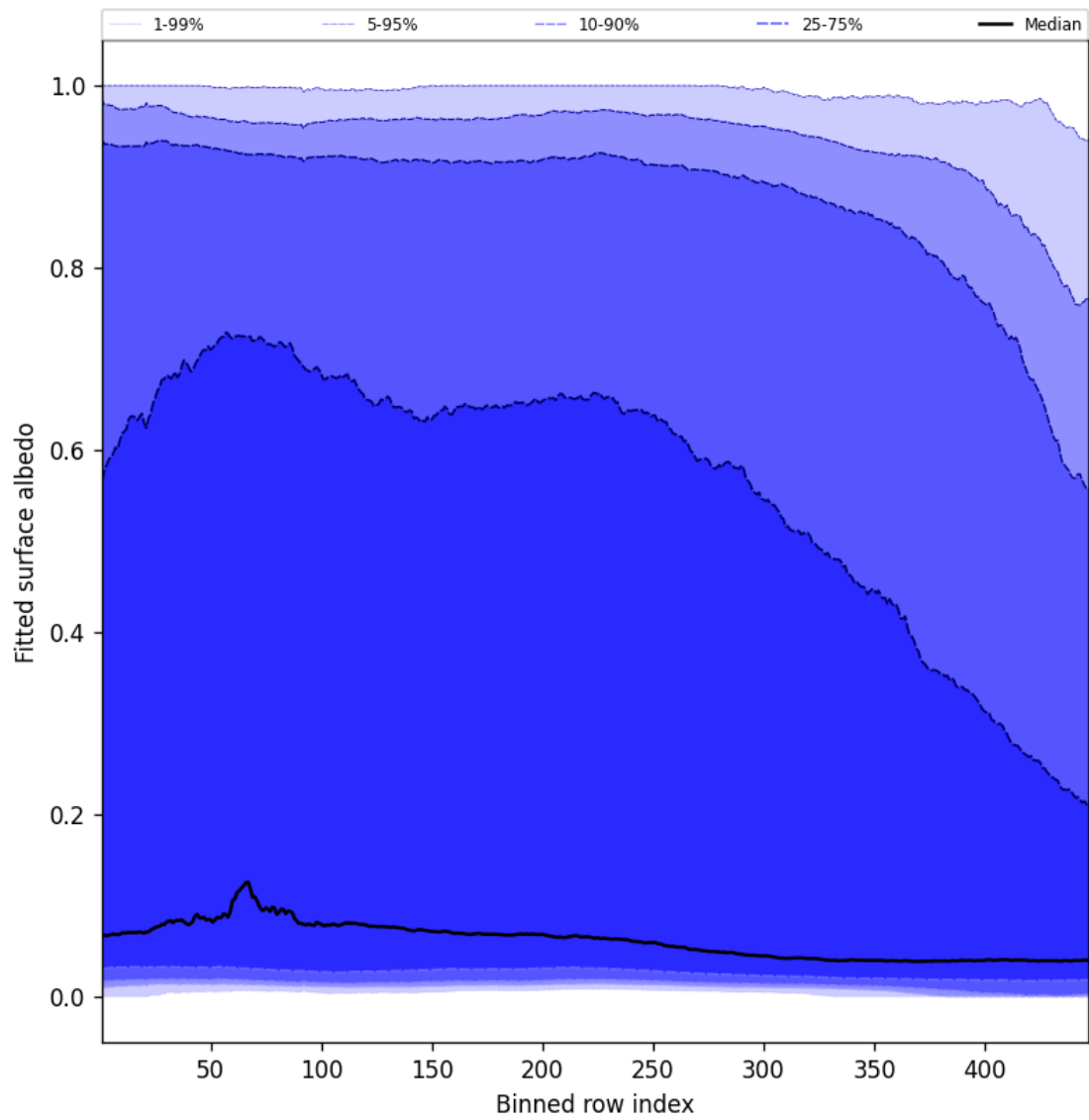
Figure 59: Along track statistics of “Fitted surface albedo” for 2025-02-01 to 2025-02-02
