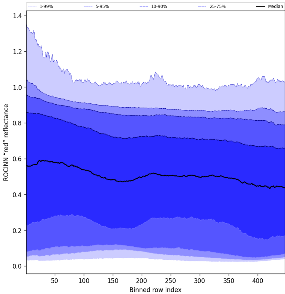
Figure 67: Along track statistics of “ROCINN “red” reflectance” for 2025-02-01 to 2025-02-02
