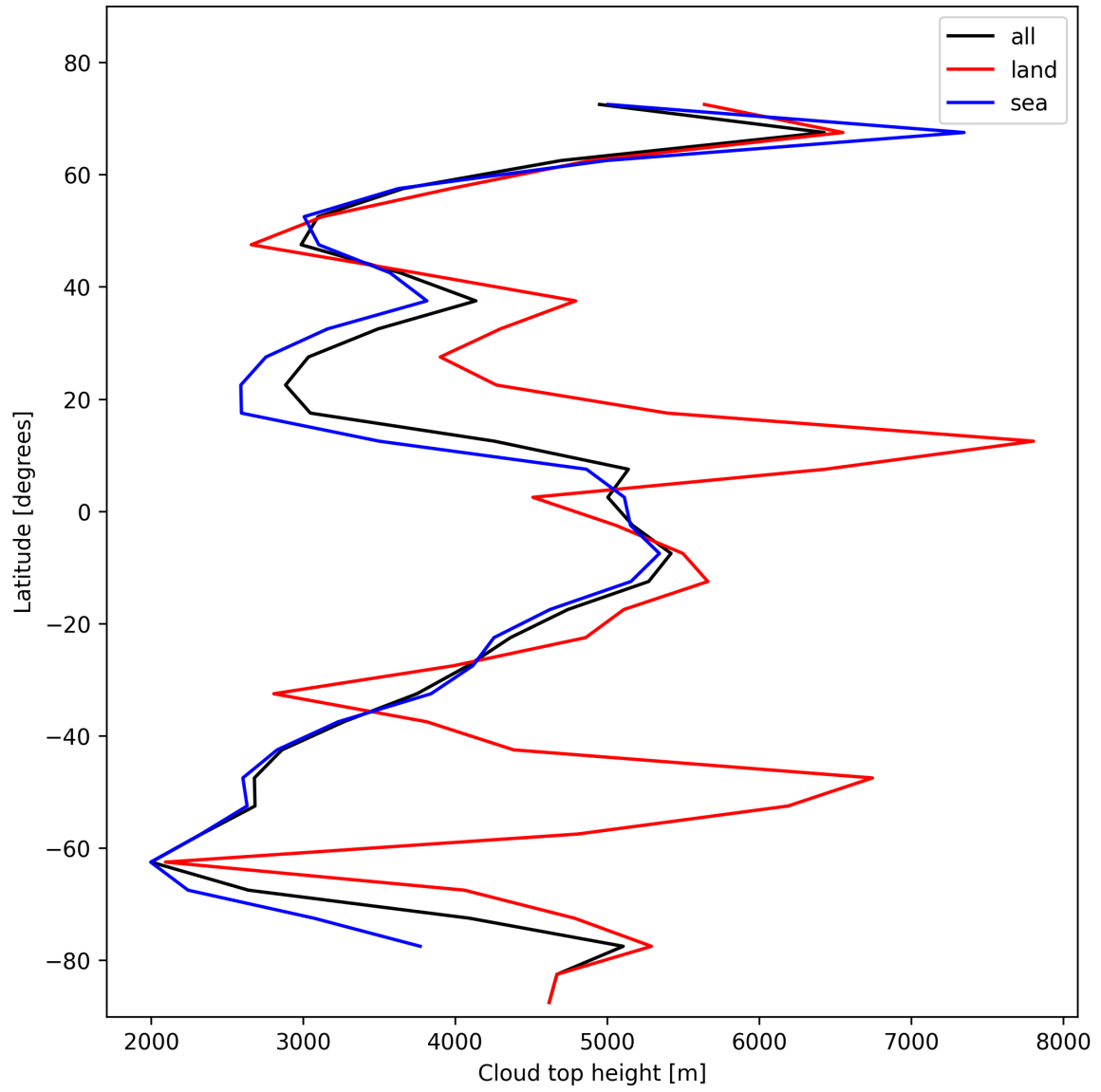
Figure 22: Zonal average of “Cloud top height” for 2025-02-01 to 2025-02-02.
