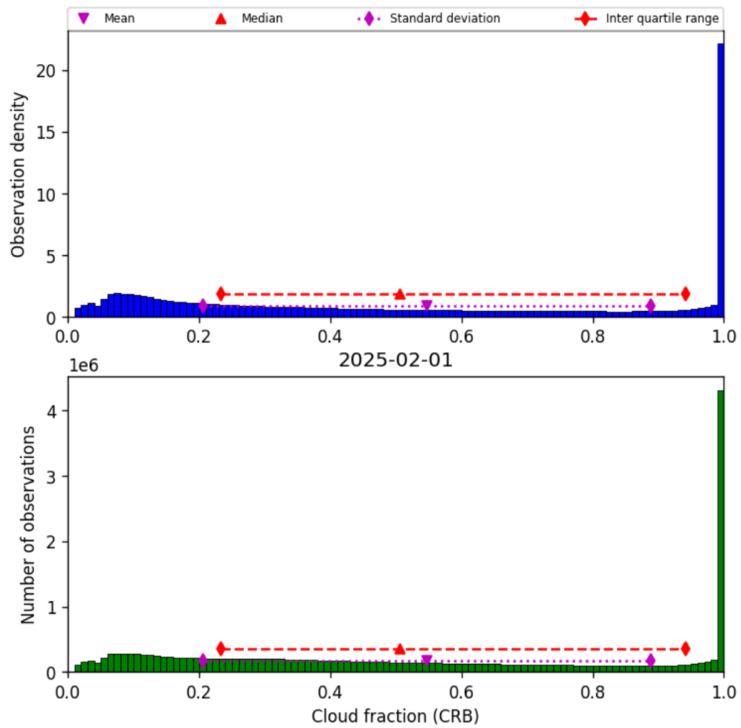
Figure 40: Histogram of "Cloud fraction (CRB)" for 2025-02-01 to 2025-02-02
