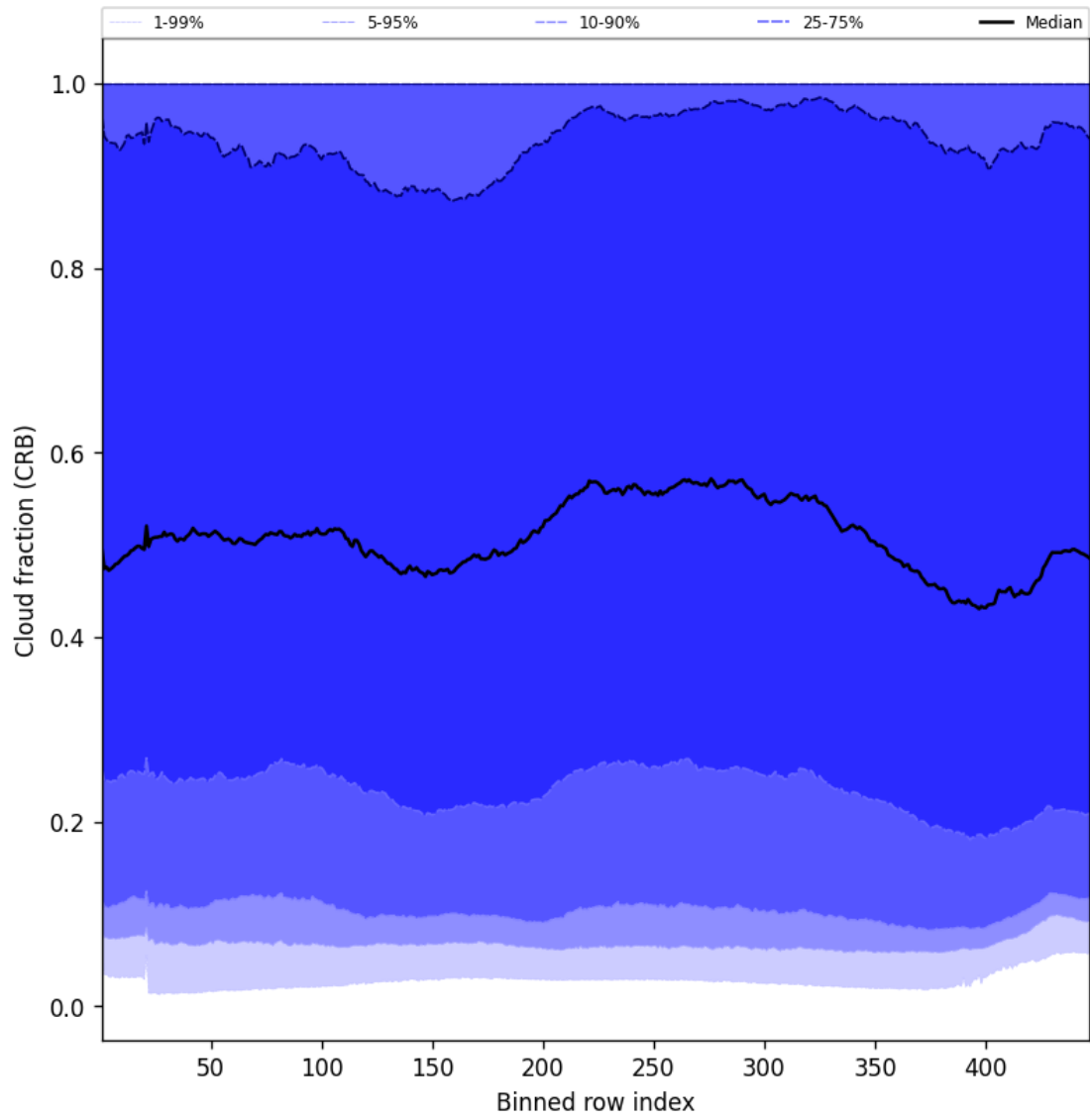
Figure 56: Along track statistics of “Cloud fraction (CRB)” for 2025-02-01 to 2025-02-02
