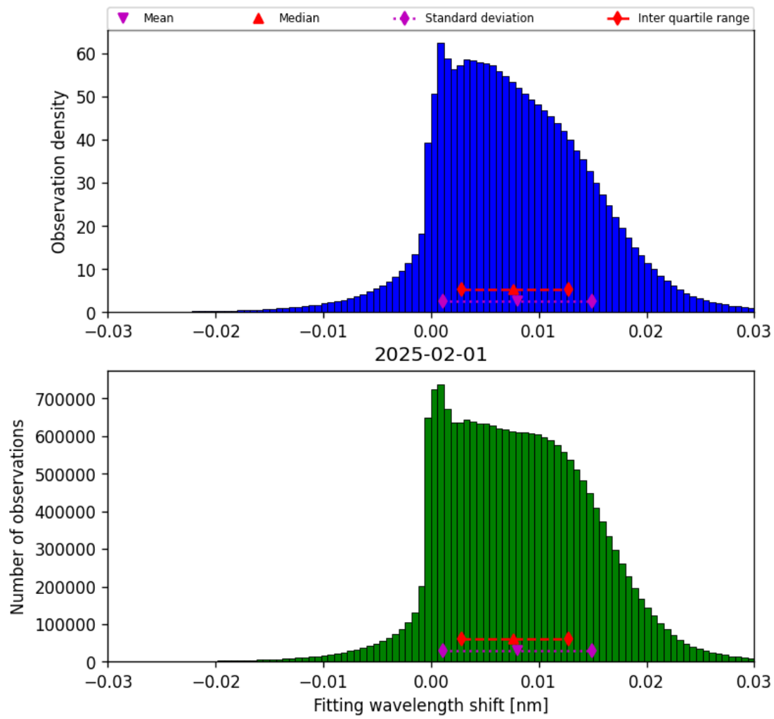
Figure 47: Histogram of “Fitting wavelength shift” for 2025-02-01 to 2025-02-02
