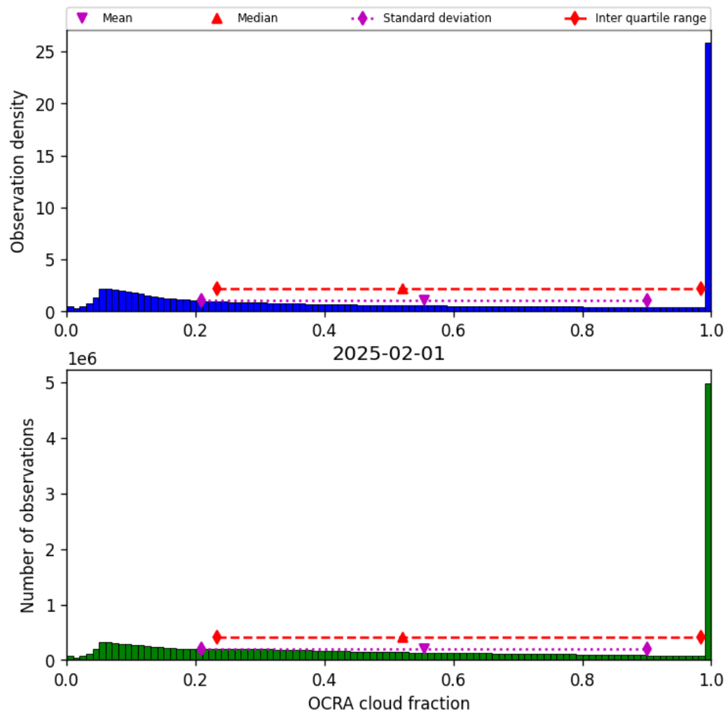
Figure 48: Histogram of “OCRA cloud fraction” for 2025-02-01 to 2025-02-02
