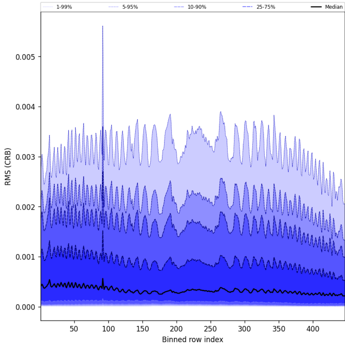
Figure 62: Along track statistics of “RMS (CRB)” for 2025-02-01 to 2025-02-02
