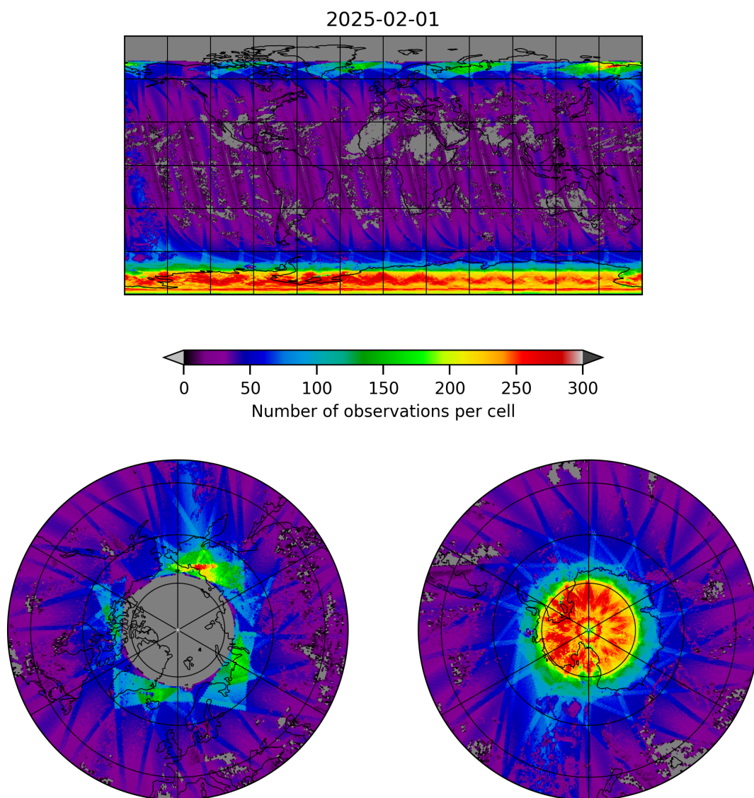
Figure 19: Map of the number of observations for 2025-02-01 to 2025-02-02
