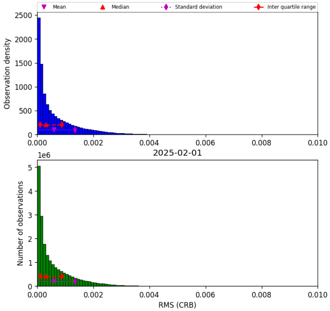
Figure 46: Histogram of “RMS (CRB)” for 2025-02-01 to 2025-02-02
