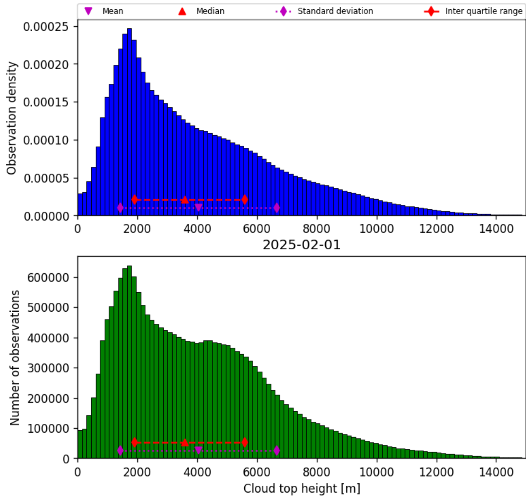
Figure 38: Histogram of “Cloud top height” for 2025-02-01 to 2025-02-02
