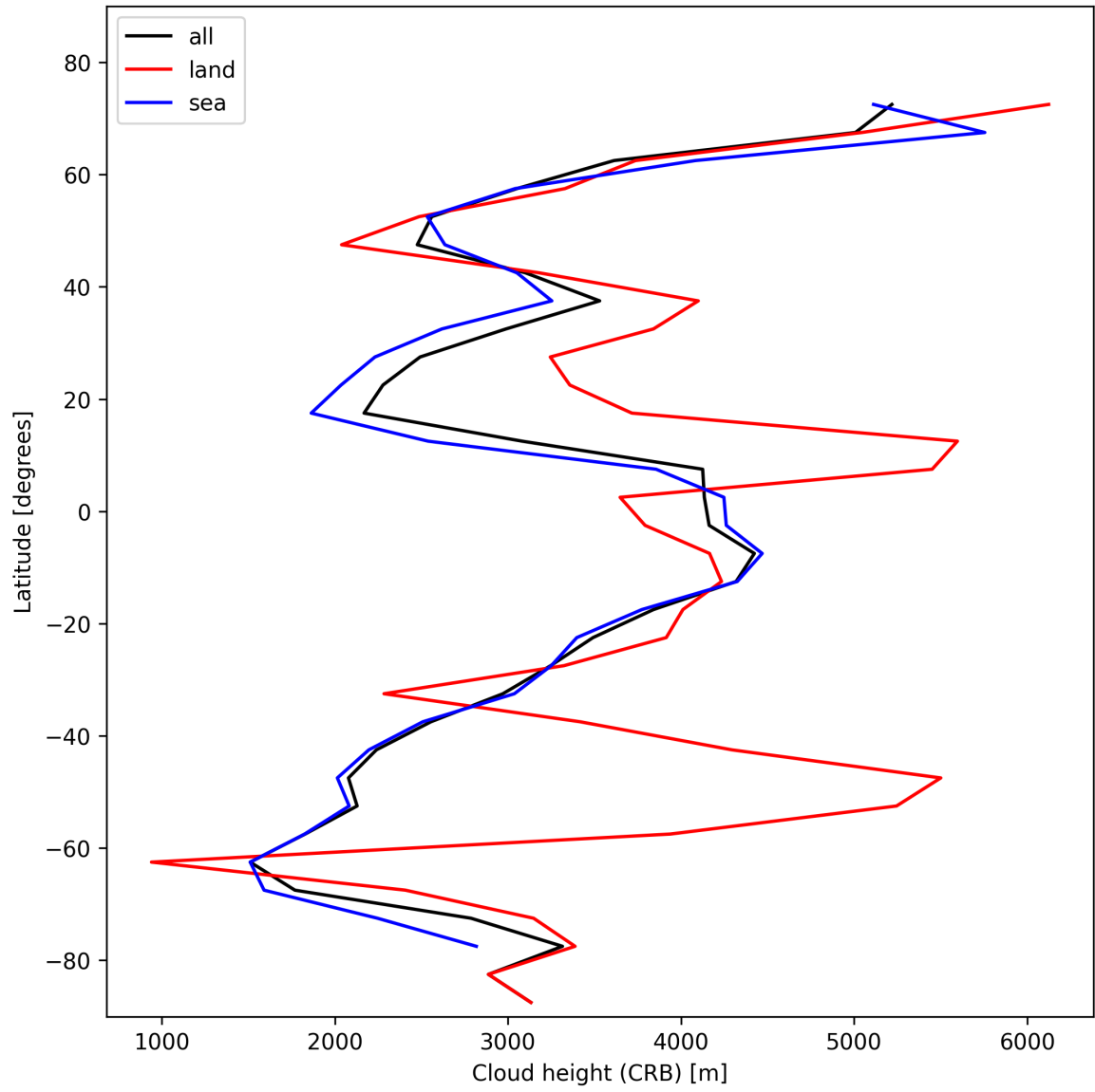
Figure 25: Zonal average of “Cloud height (CRB)” for 2025-02-01 to 2025-02-02.
