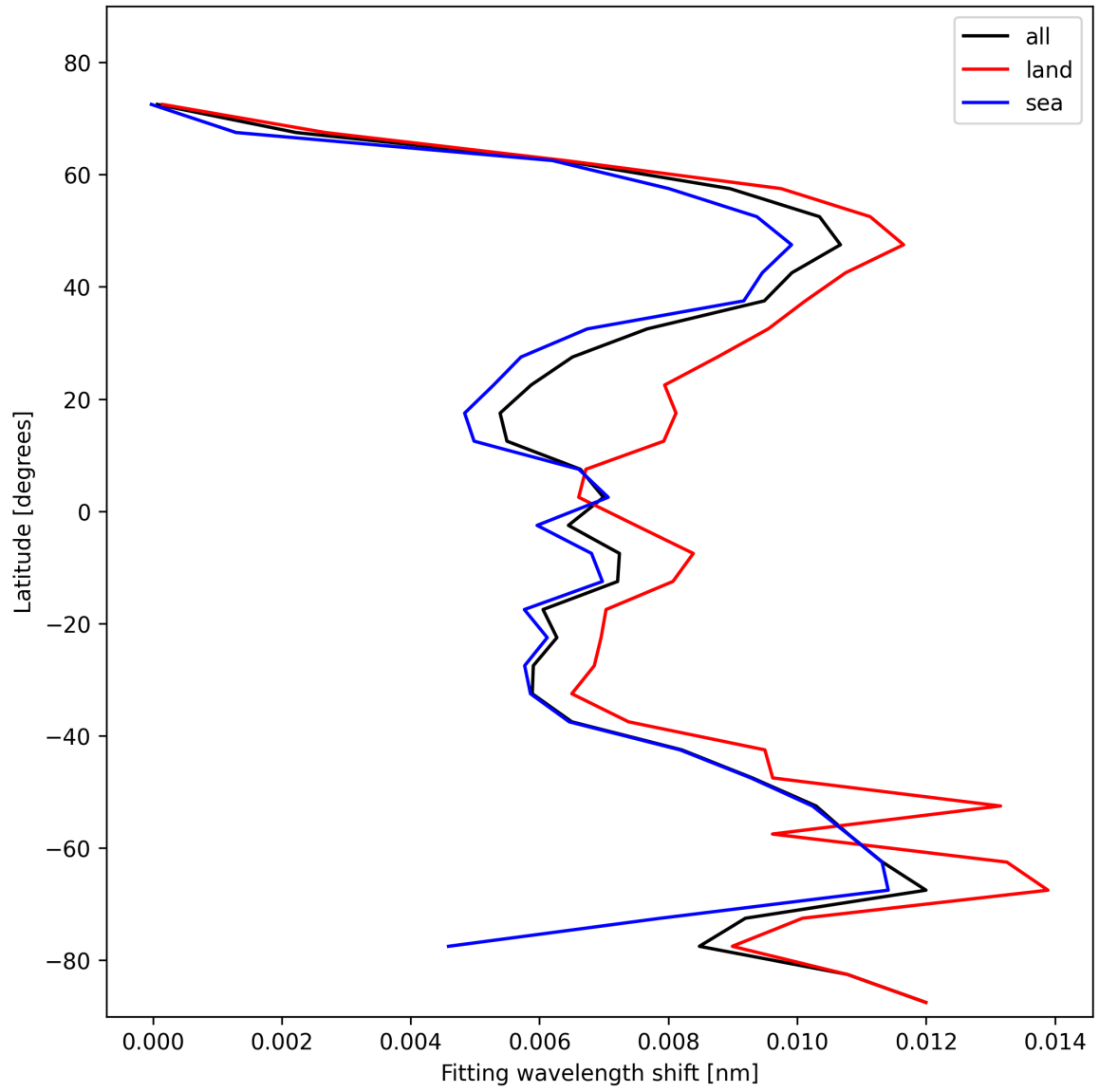
Figure 31: Zonal average of “Fitting wavelength shift” for 2025-02-01 to 2025-02-02.
