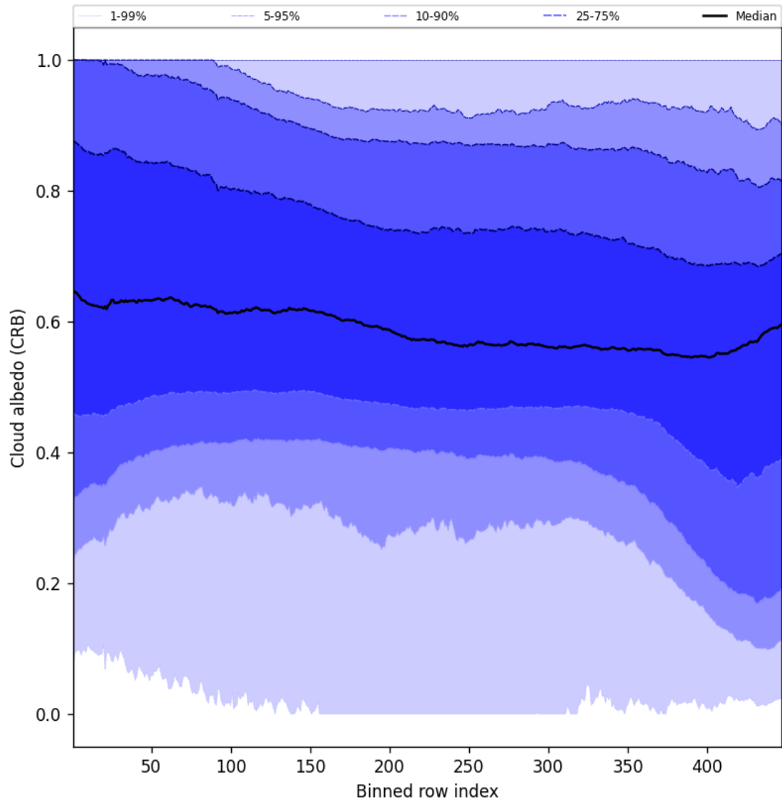
Figure 58: Along track statistics of “Cloud albedo (CRB)” for 2025-02-01 to 2025-02-02
