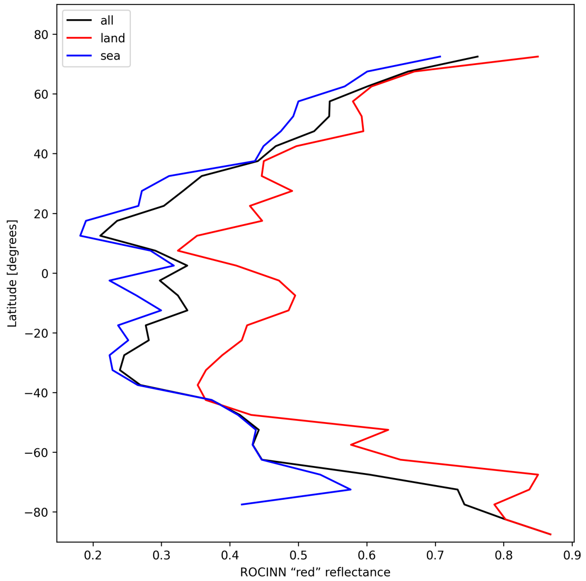
Figure 35: Zonal average of “ROCINN “red” reflectance” for 2025-02-01 to 2025-02-02.
