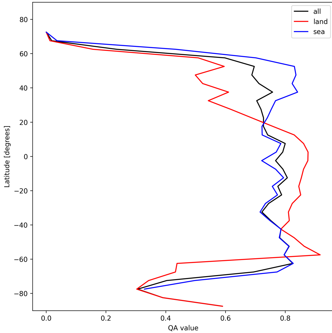
Figure 20: Zonal average of “QA value” for 2025-02-01 to 2025-02-02.
