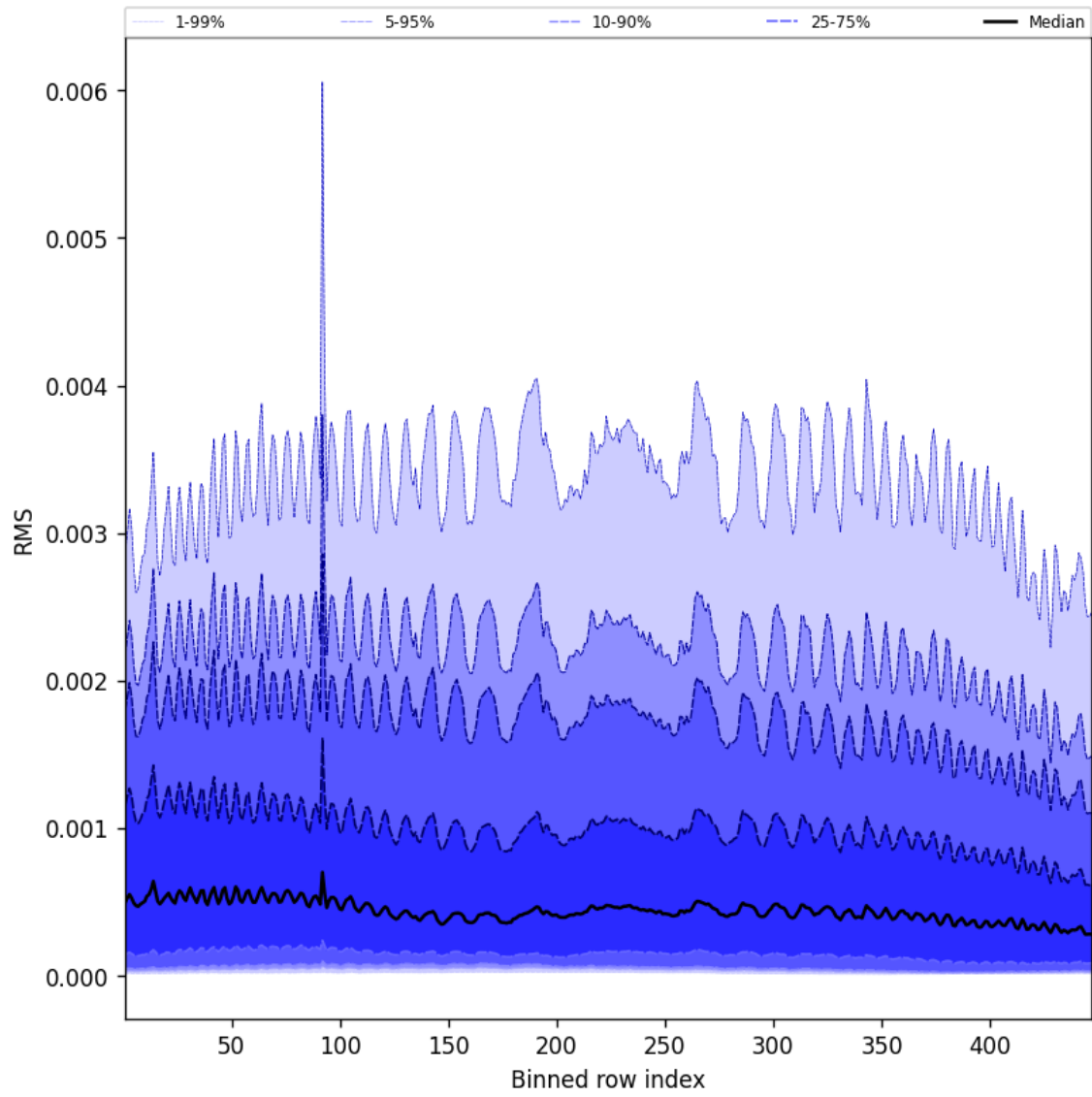
Figure 61: Along track statistics of “RMS” for 2025-02-01 to 2025-02-02
