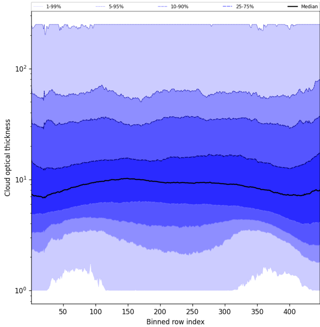
Figure 55: Along track statistics of “Cloud optical thickness” for 2025-02-01 to 2025-02-02
