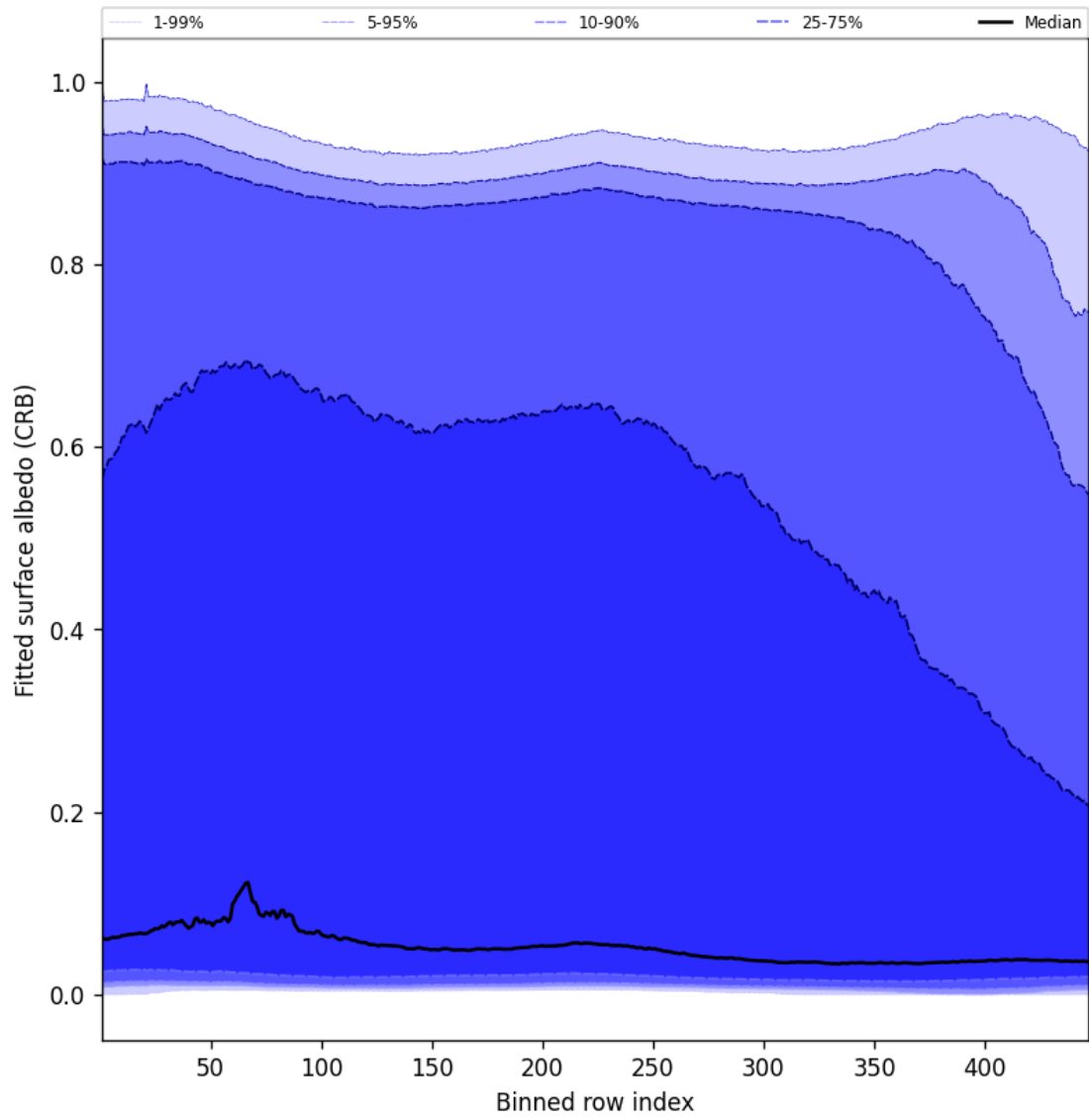
Figure 60: Along track statistics of “Fitted surface albedo (CRB)” for 2025-02-01 to 2025-02-02
