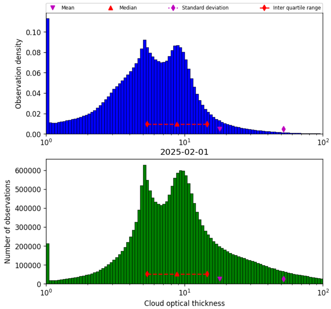
Figure 39: Histogram of “Cloud optical thickness” for 2025-02-01 to 2025-02-02
