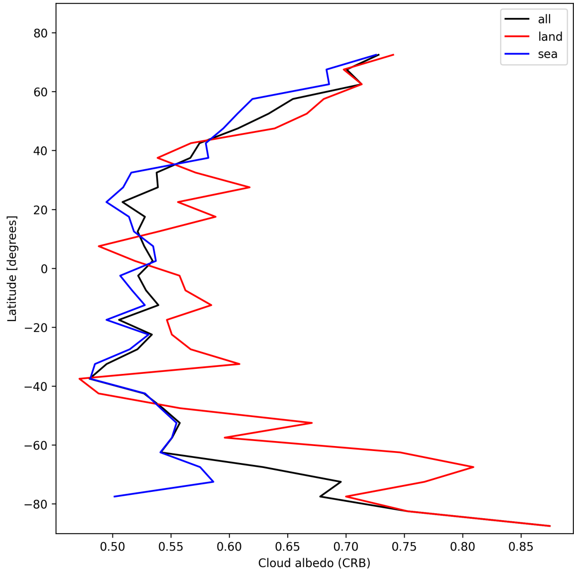
Figure 26: Zonal average of “Cloud albedo (CRB)” for 2025-02-01 to 2025-02-02.
