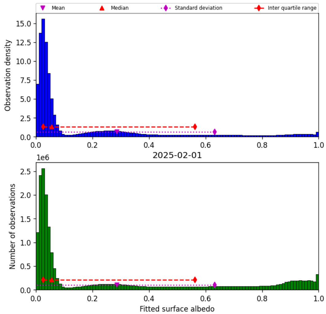
Figure 43: Histogram of “Fitted surface albedo” for 2025-02-01 to 2025-02-02
