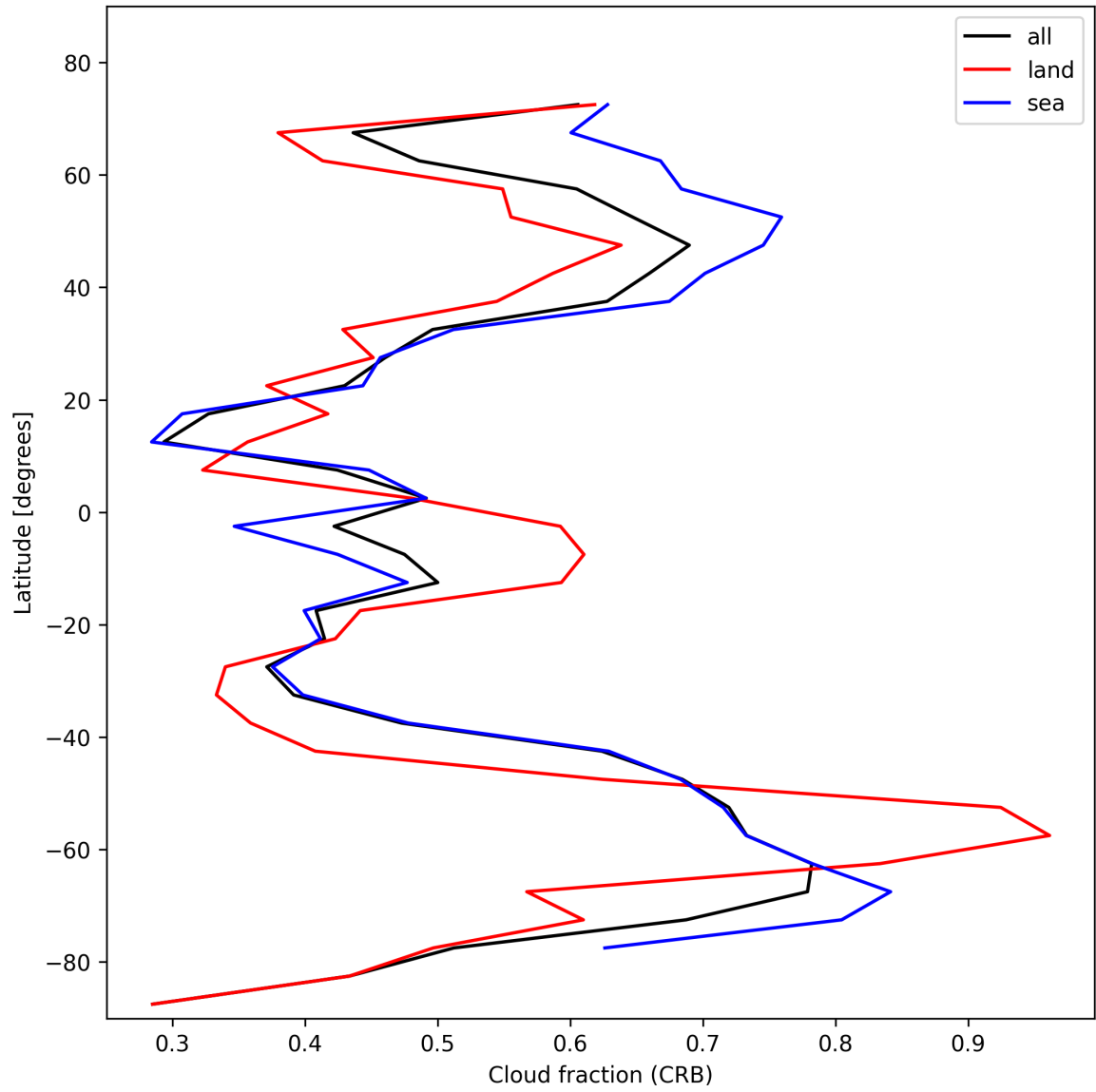
Figure 24: Zonal average of “Cloud fraction (CRB)” for 2025-02-01 to 2025-02-02.
