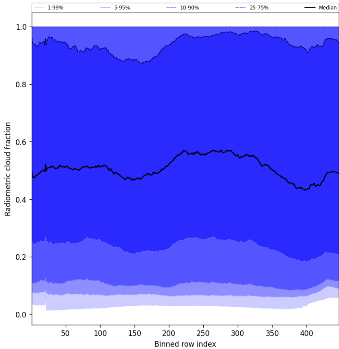
Figure 53: Along track statistics of “Radiometric cloud fraction” for 2025-02-01 to 2025-02-02
