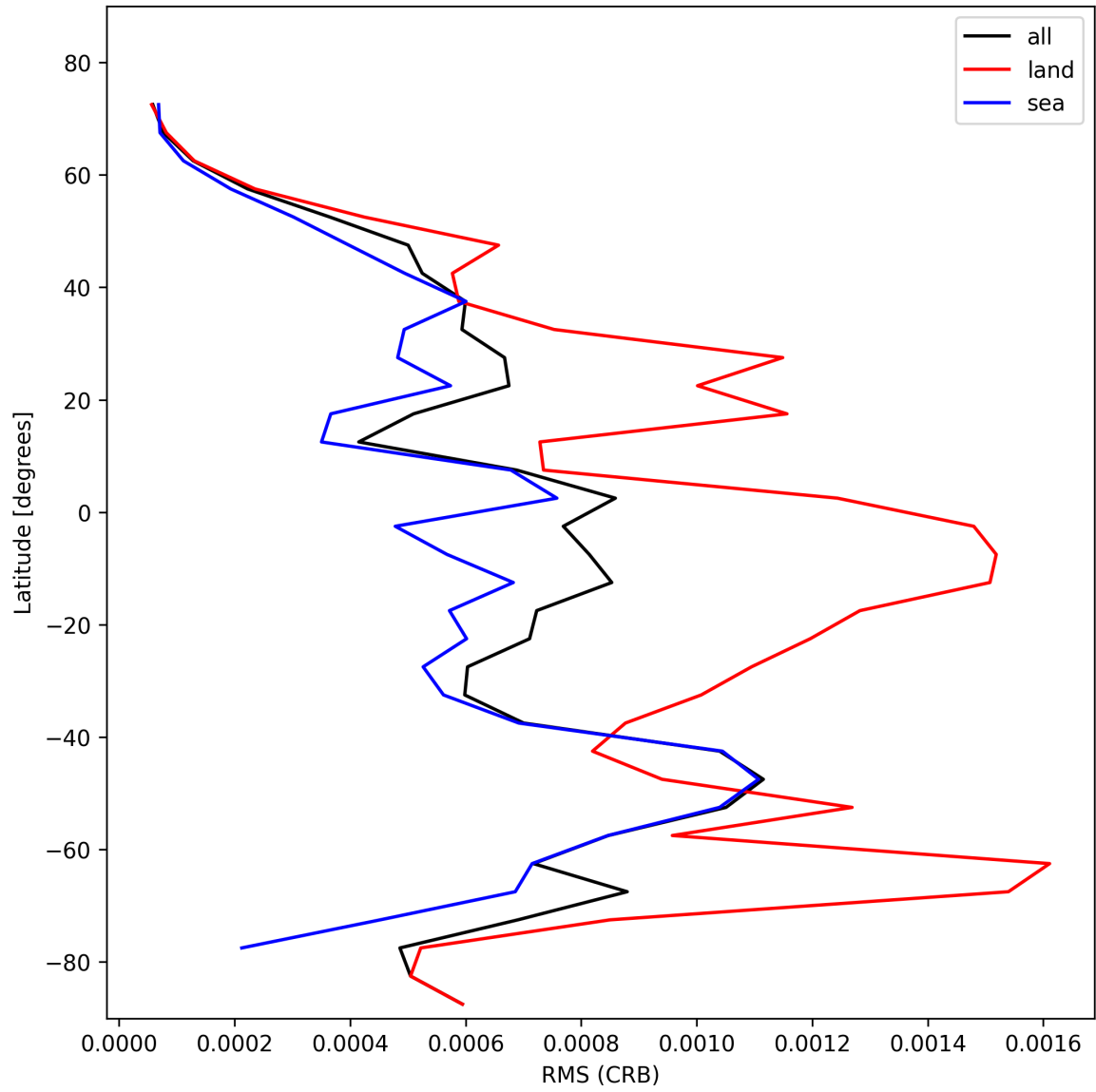
Figure 30: Zonal average of “RMS (CRB)” for 2025-02-01 to 2025-02-02.
