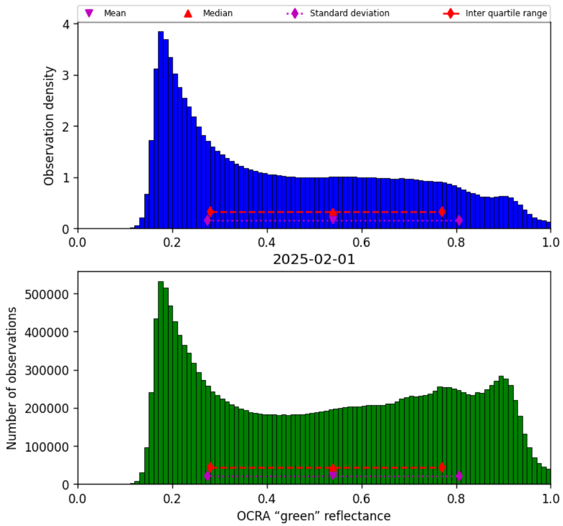
Figure 50: Histogram of “OCRA “green” reflectance” for 2025-02-01 to 2025-02-02
