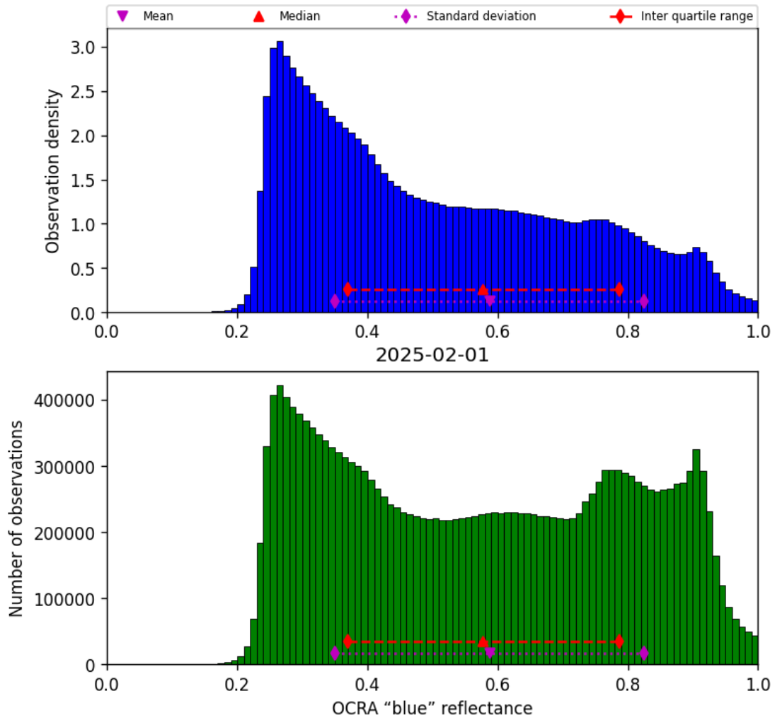
Figure 49: Histogram of “OCRA “blue” reflectance” for 2025-02-01 to 2025-02-02
