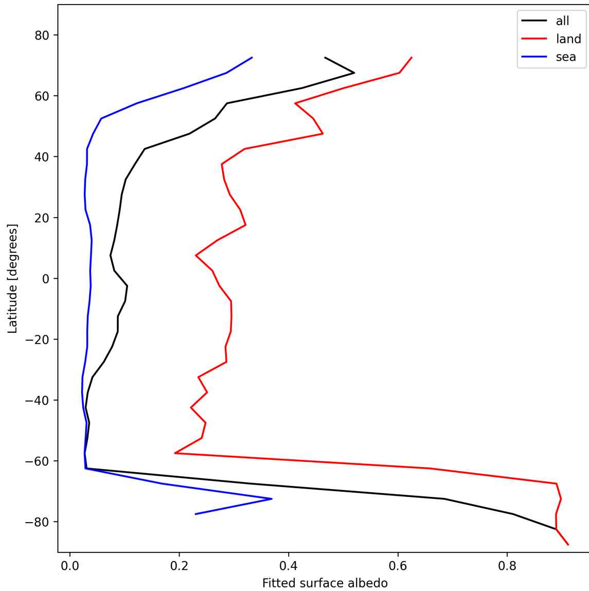
Figure 27: Zonal average of “Fitted surface albedo” for 2025-02-01 to 2025-02-02.
