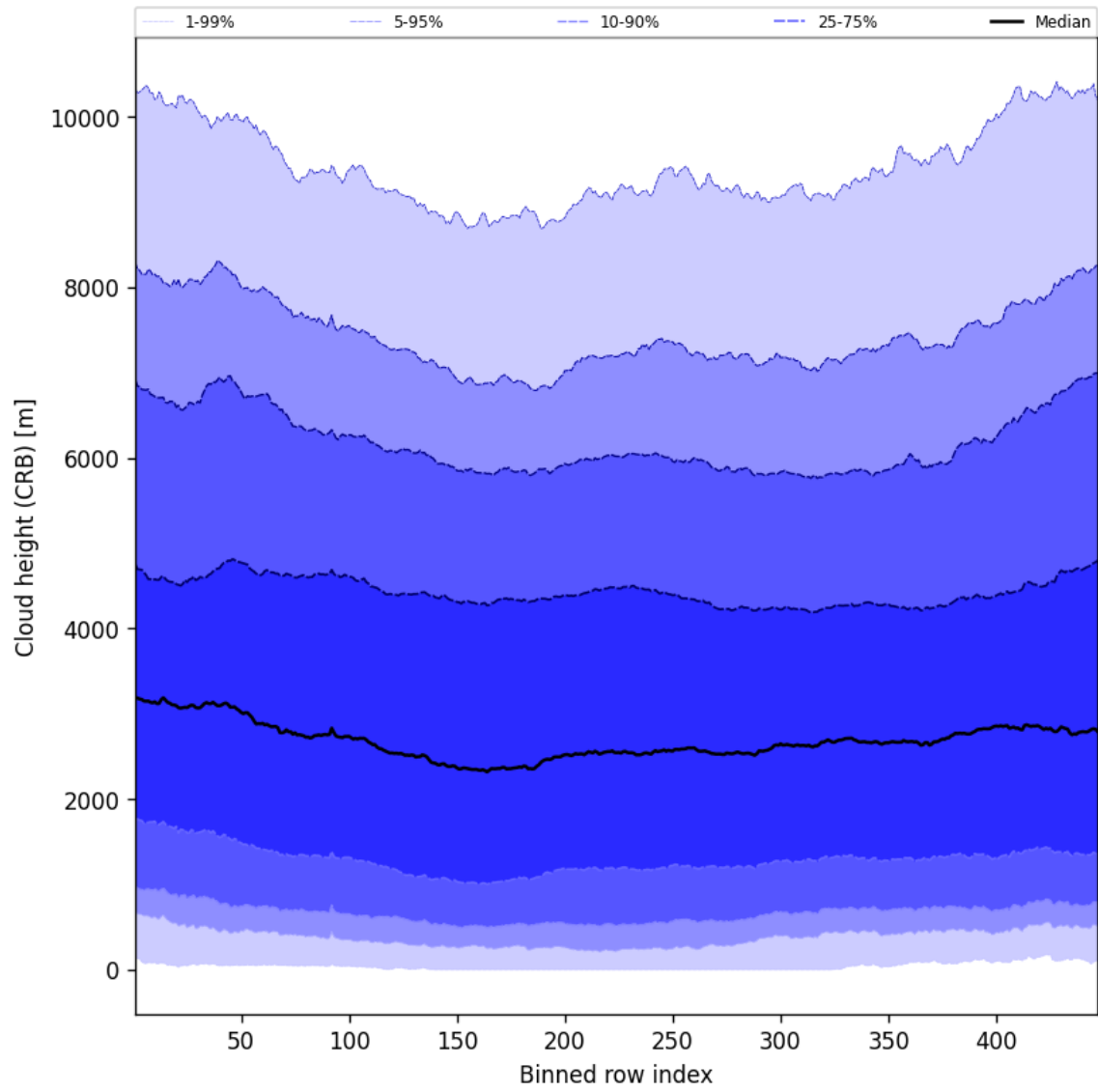
Figure 57: Along track statistics of “Cloud height (CRB)” for 2025-02-01 to 2025-02-02
