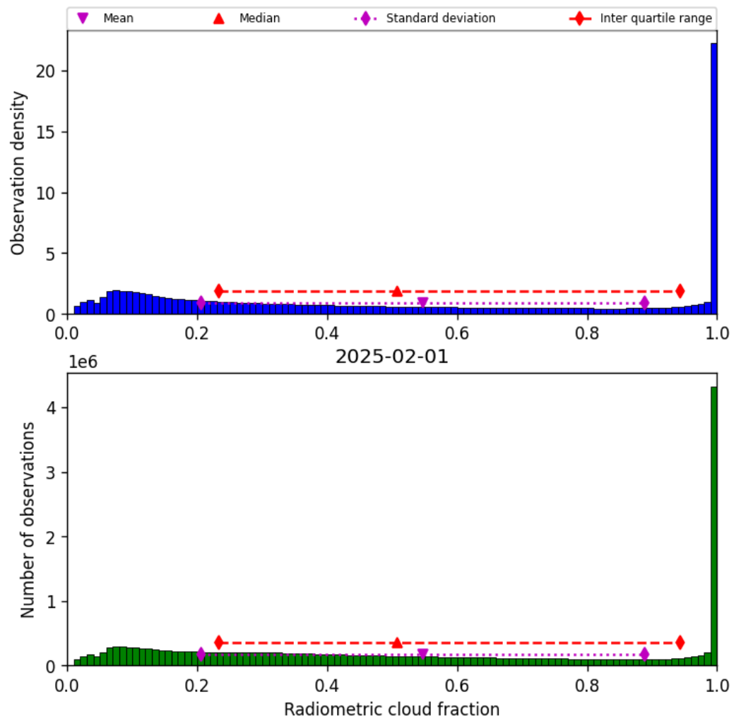
Figure 37: Histogram of “Radiometric cloud fraction” for 2025-02-01 to 2025-02-02
