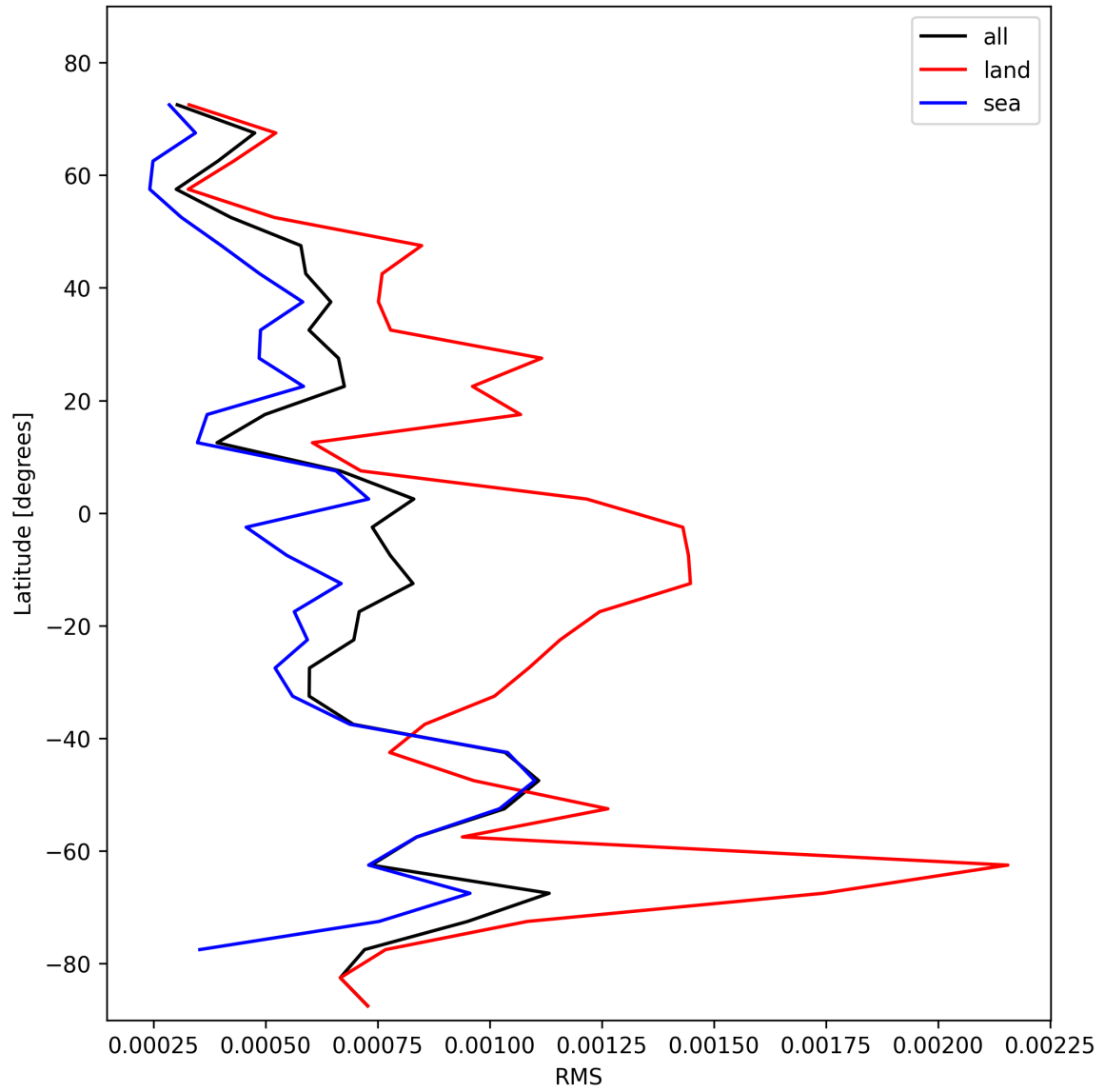
Figure 29: Zonal average of “RMS” for 2025-02-01 to 2025-02-02.
