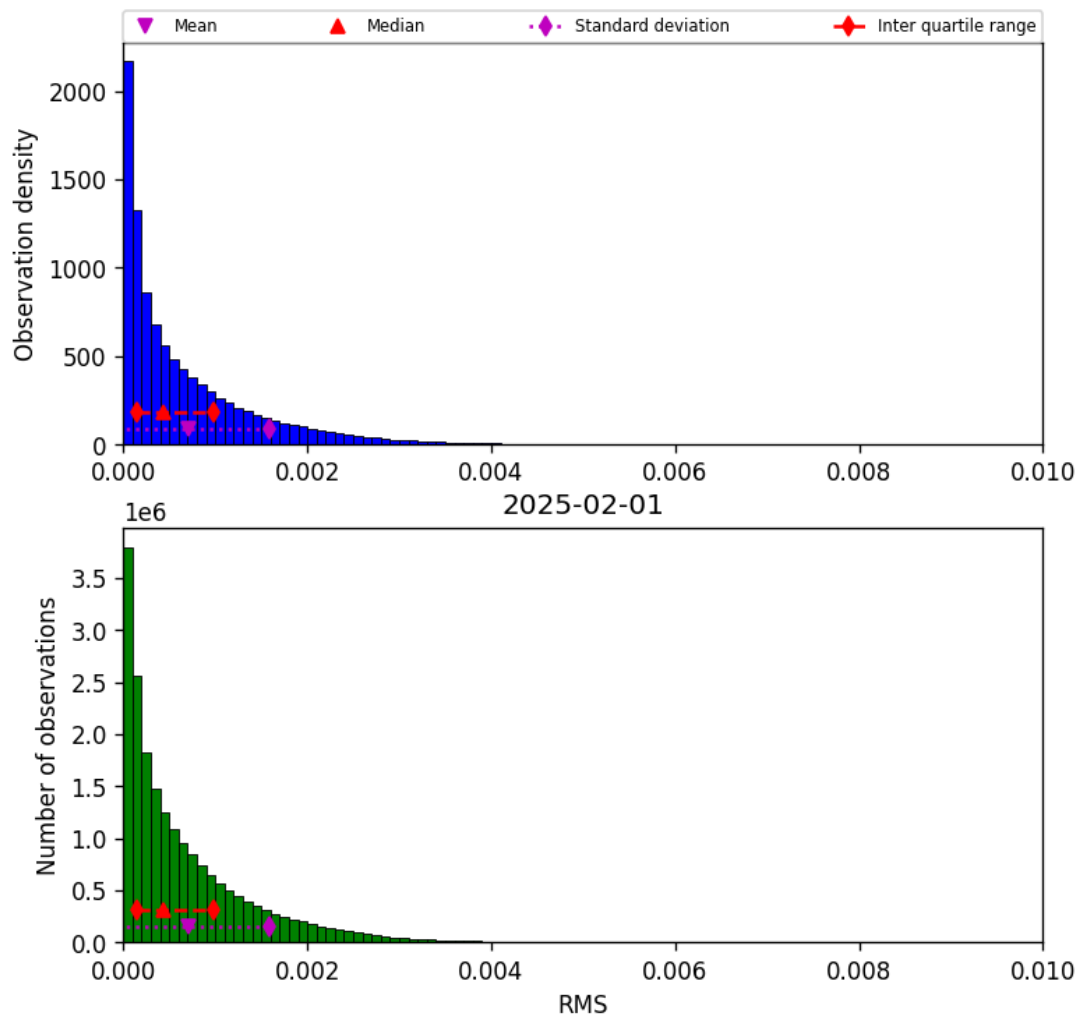
Figure 45: Histogram of “RMS” for 2025-02-01 to 2025-02-02
