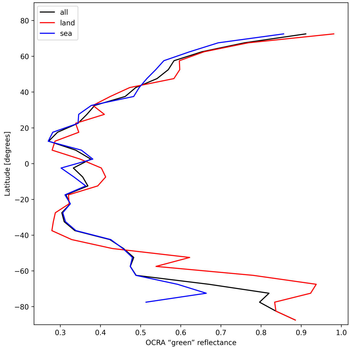
Figure 34: Zonal average of “OCRA “green” reflectance” for 2025-02-01 to 2025-02-02.
