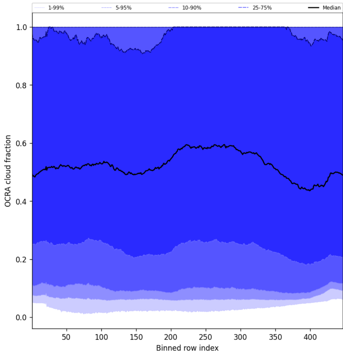
Figure 64: Along track statistics of “OCRA cloud fraction” for 2025-02-01 to 2025-02-02
