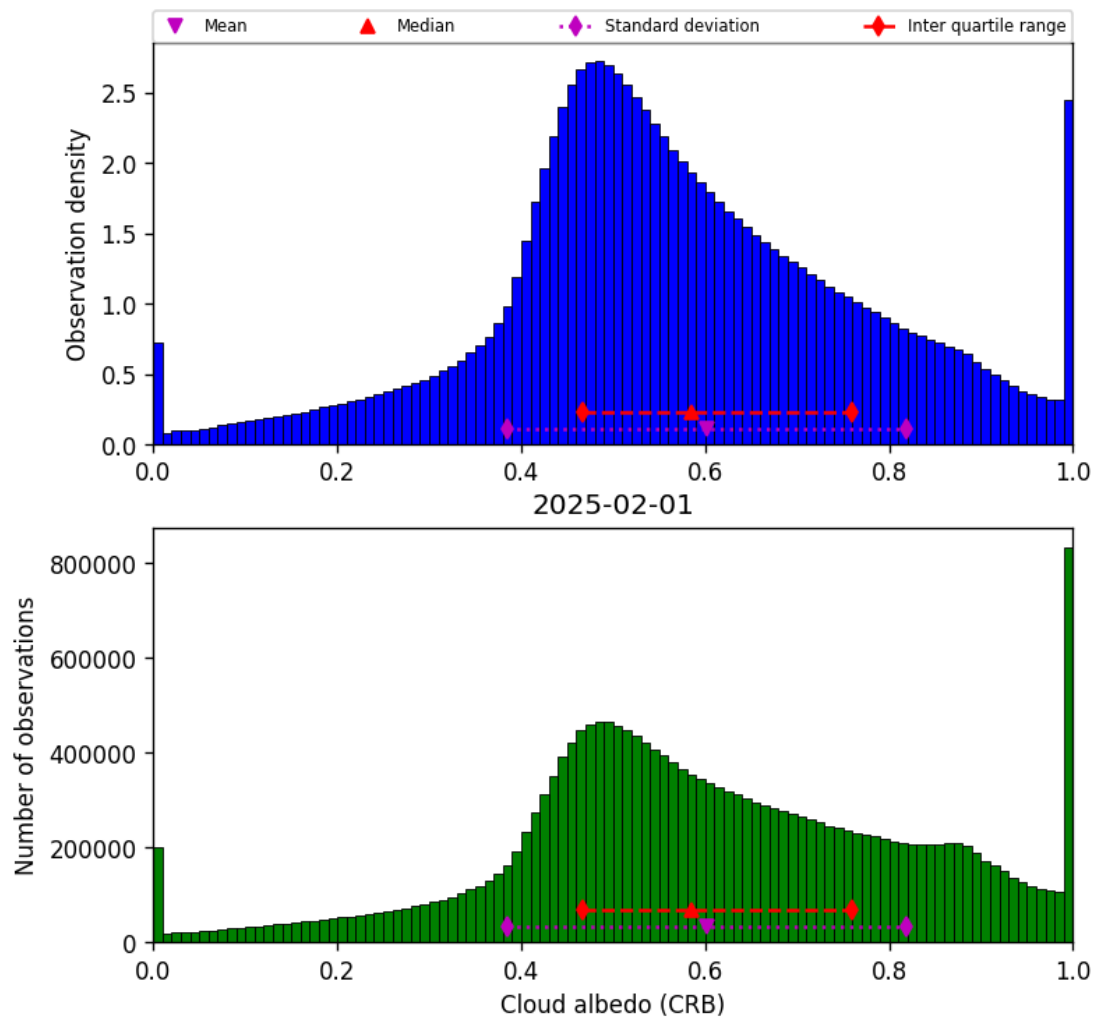
Figure 42: Histogram of “Cloud albedo (CRB)” for 2025-02-01 to 2025-02-02
