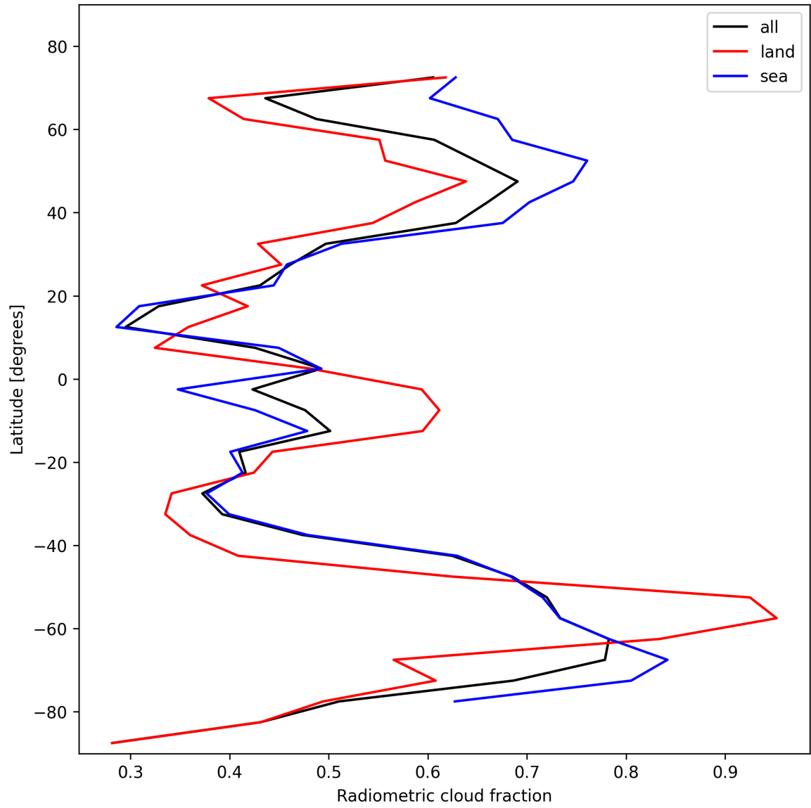
Figure 21: Zonal average of “Radiometric cloud fraction” for 2025-02-01 to 2025-02-02.
